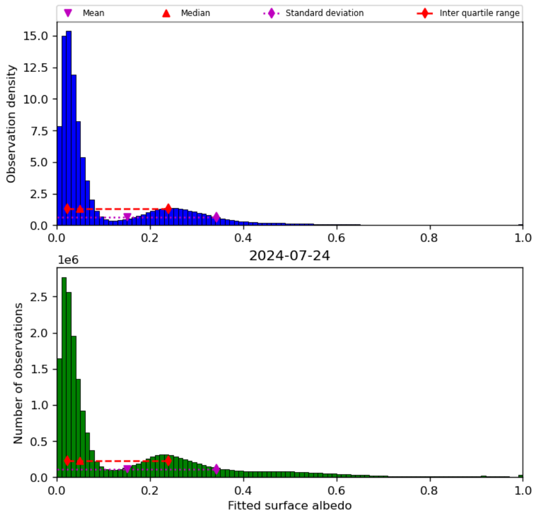
Figure 45: Histogram of “Fitted surface albedo” for 2024-07-23 to 2024-07-25
