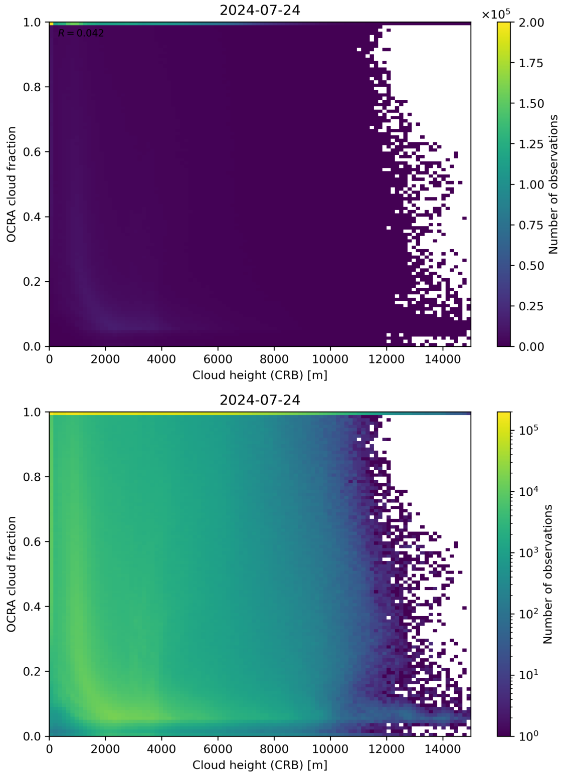
Figure 81: Scatter density plot of “Cloud height (CRB)” against “OCRA cloud fraction” for 2024-07-23 to 2024-07-25.
