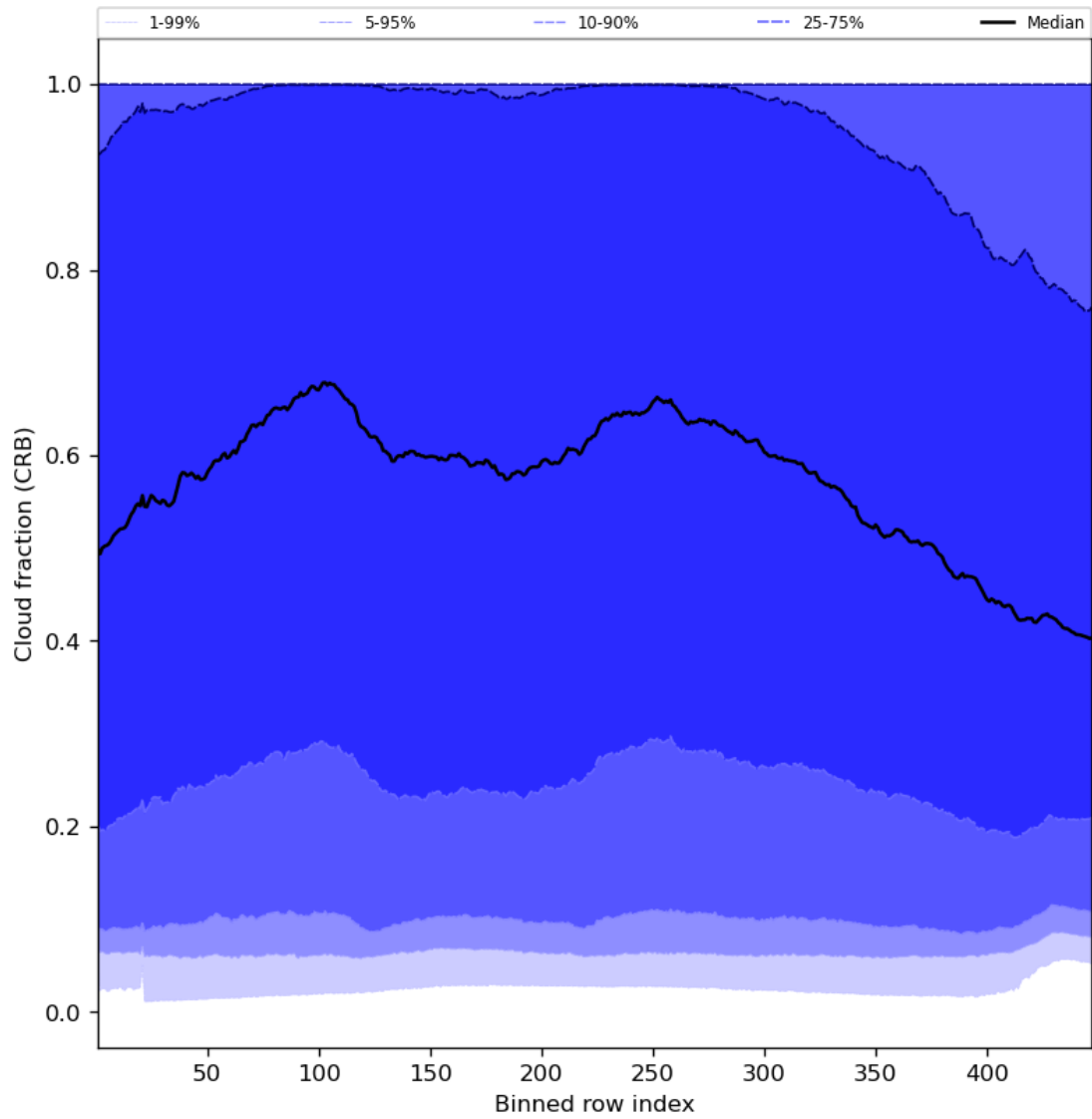
Figure 58: Along track statistics of “Cloud fraction (CRB)” for 2024-07-23 to 2024-07-25
