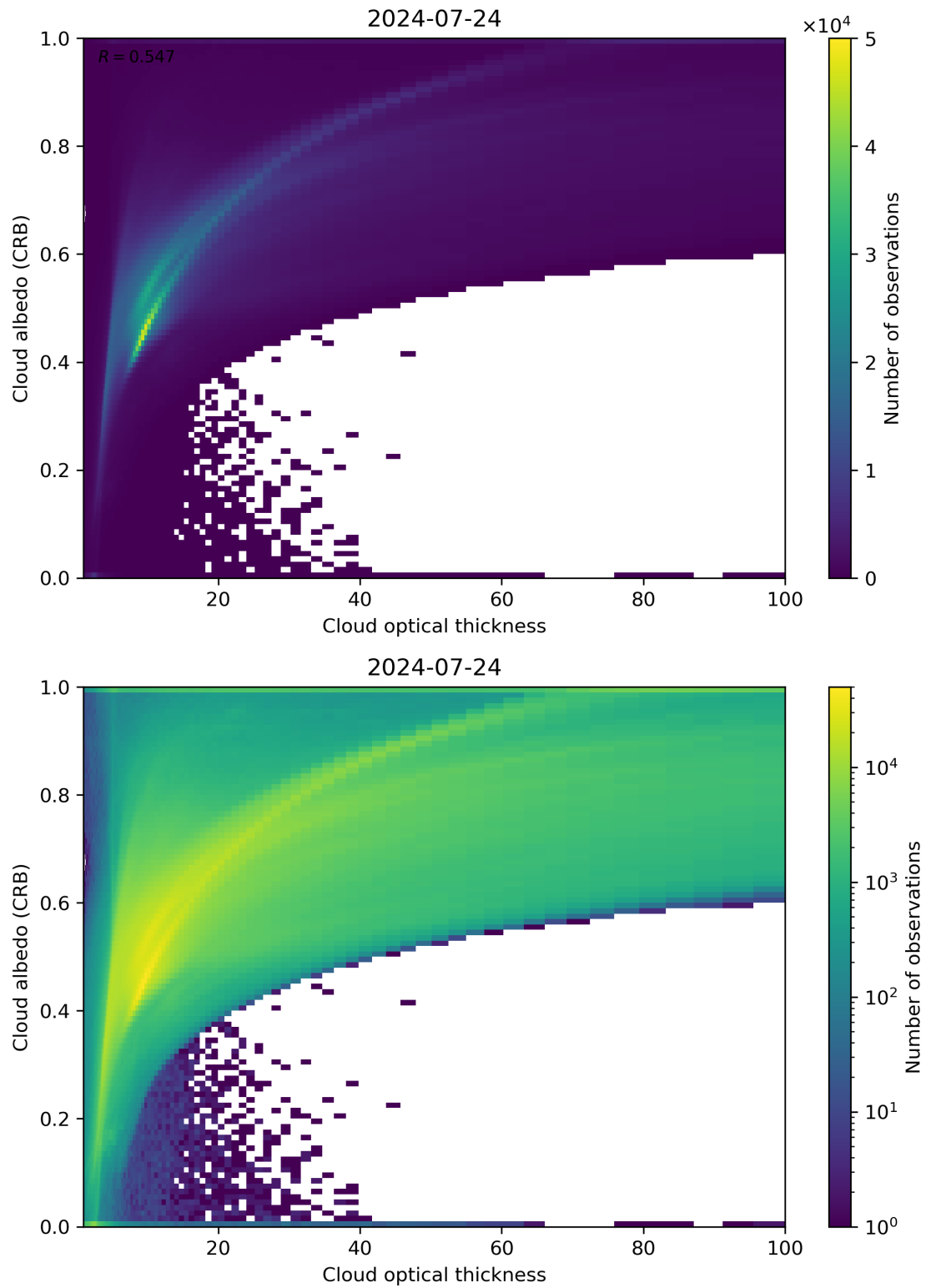
Figure 82: Scatter density plot of “Cloud optical thickness” against “Cloud albedo (CRB)” for 2024-07-23 to 2024-07-25.
