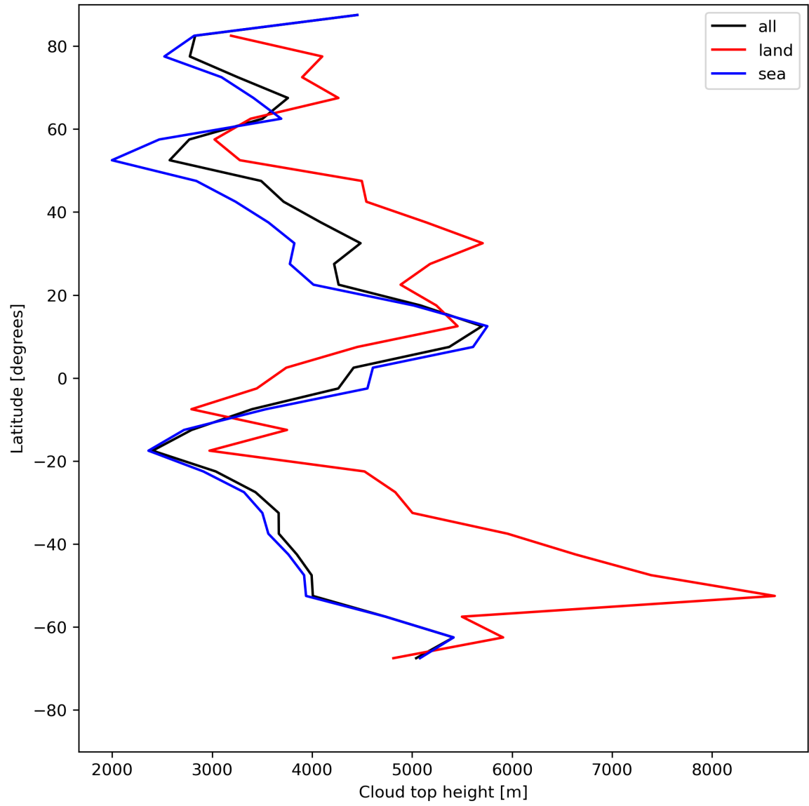
Figure 24: Zonal average of “Cloud top height” for 2024-07-23 to 2024-07-25.
