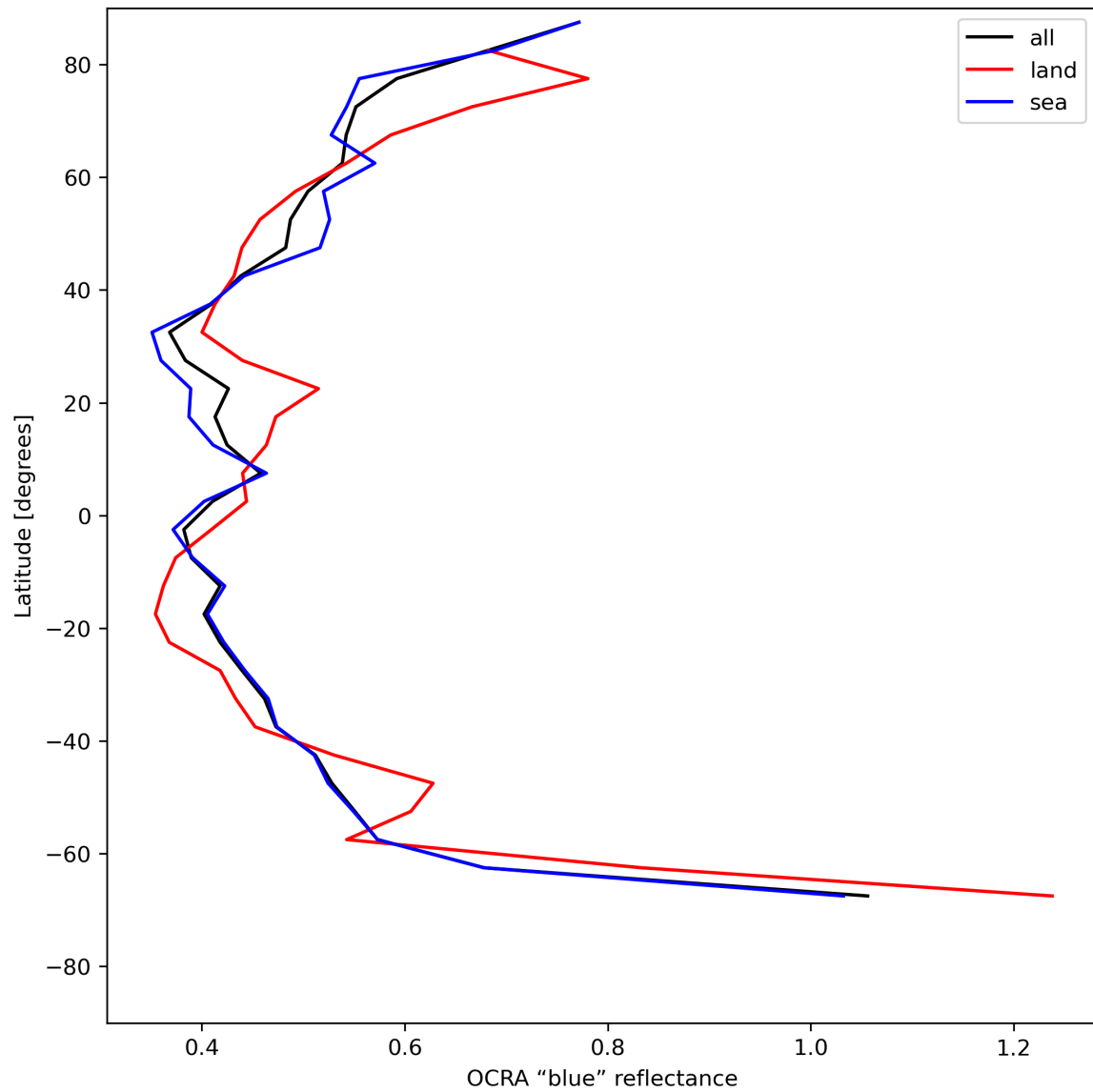
Figure 35: Zonal average of "OCRA "blue" reflectance" for 2024-07-23 to 2024-07-25.
