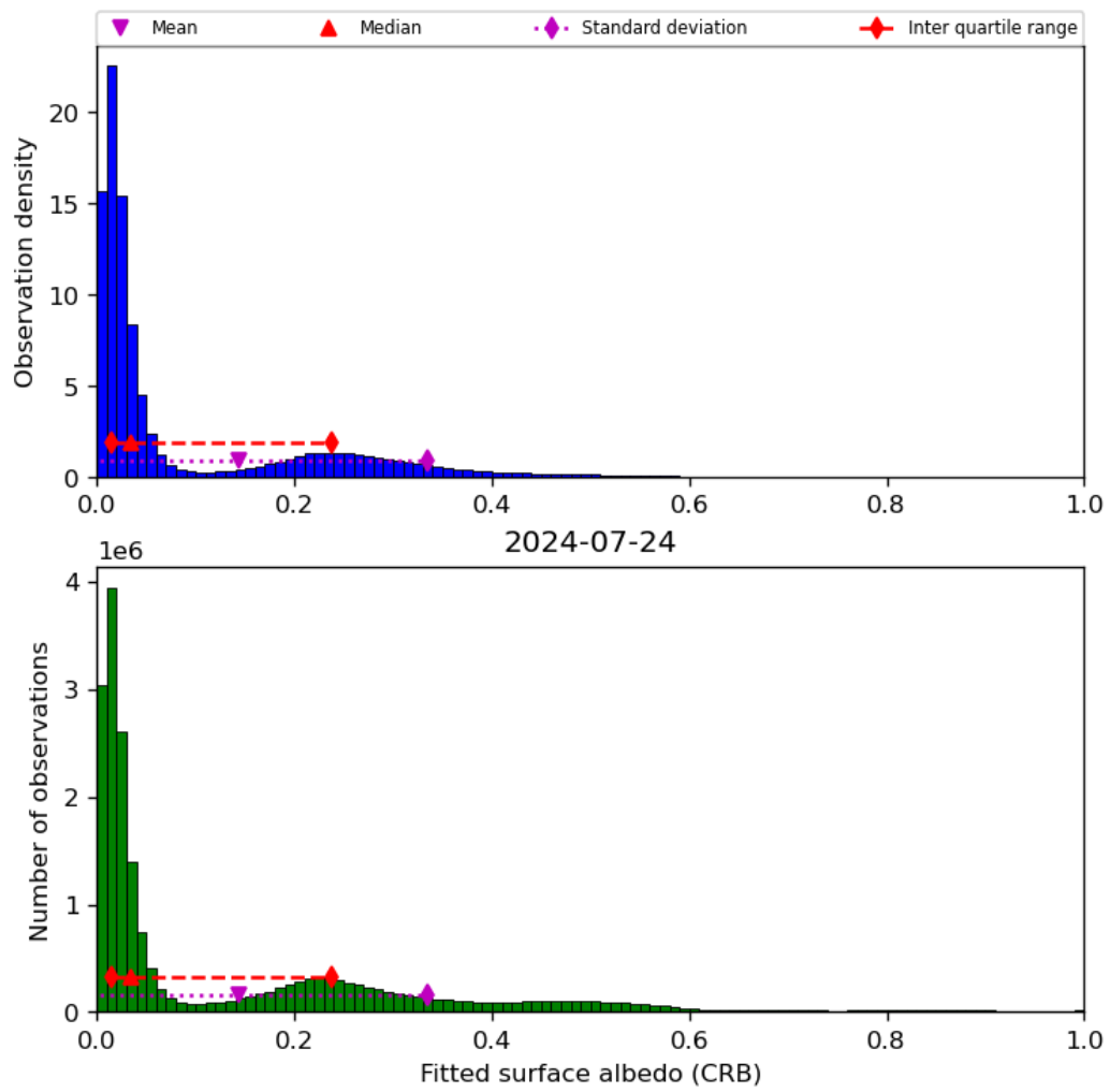
Figure 46: Histogram of “Fitted surface albedo (CRB)” for 2024-07-23 to 2024-07-25
