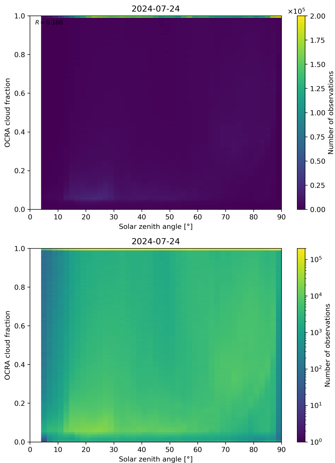
Figure 100: Scatter density plot of “Solar zenith angle” against “OCRA cloud fraction” for 2024-07-23 to 2024-07-25.
