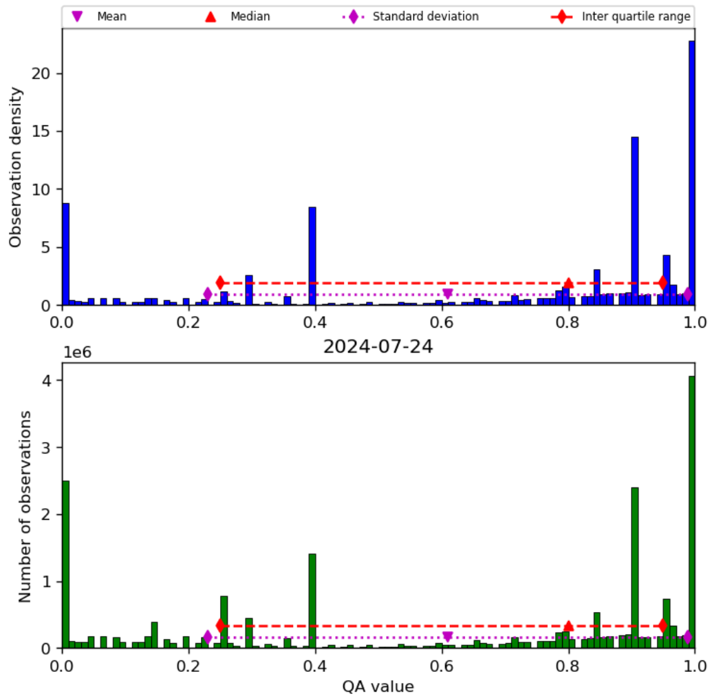
Figure 38: Histogram of “QA value” for 2024-07-23 to 2024-07-25
