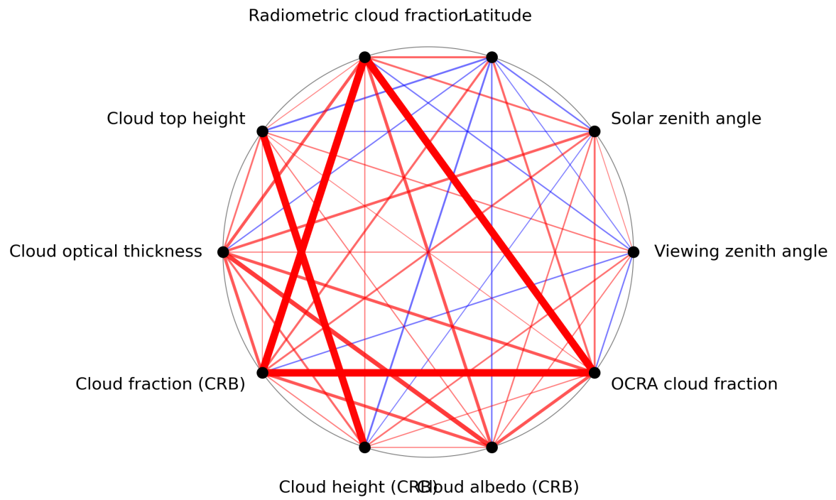
Figure 1: Map of correlation graph for 2024-07-23 to 2024-07-25.
