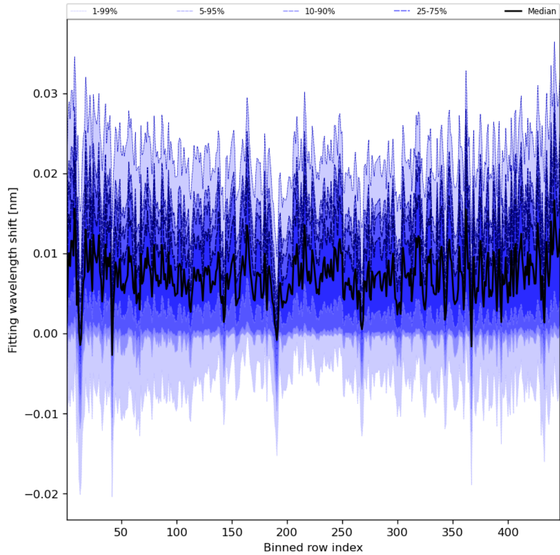
Figure 65: Along track statistics of “Fitting wavelength shift” for 2024-07-23 to 2024-07-25
