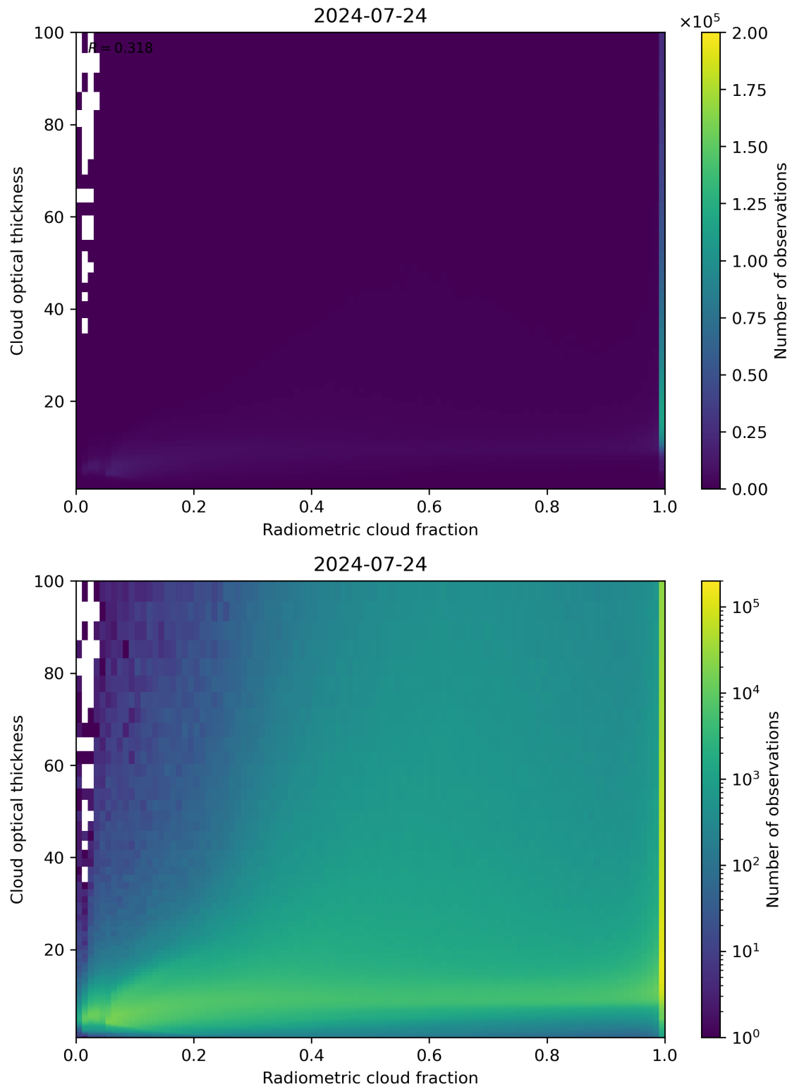
Figure 75: Scatter density plot of “Radiometric cloud fraction” against “Cloud optical thickness” for 2024-07-23 to 2024-07-25.
