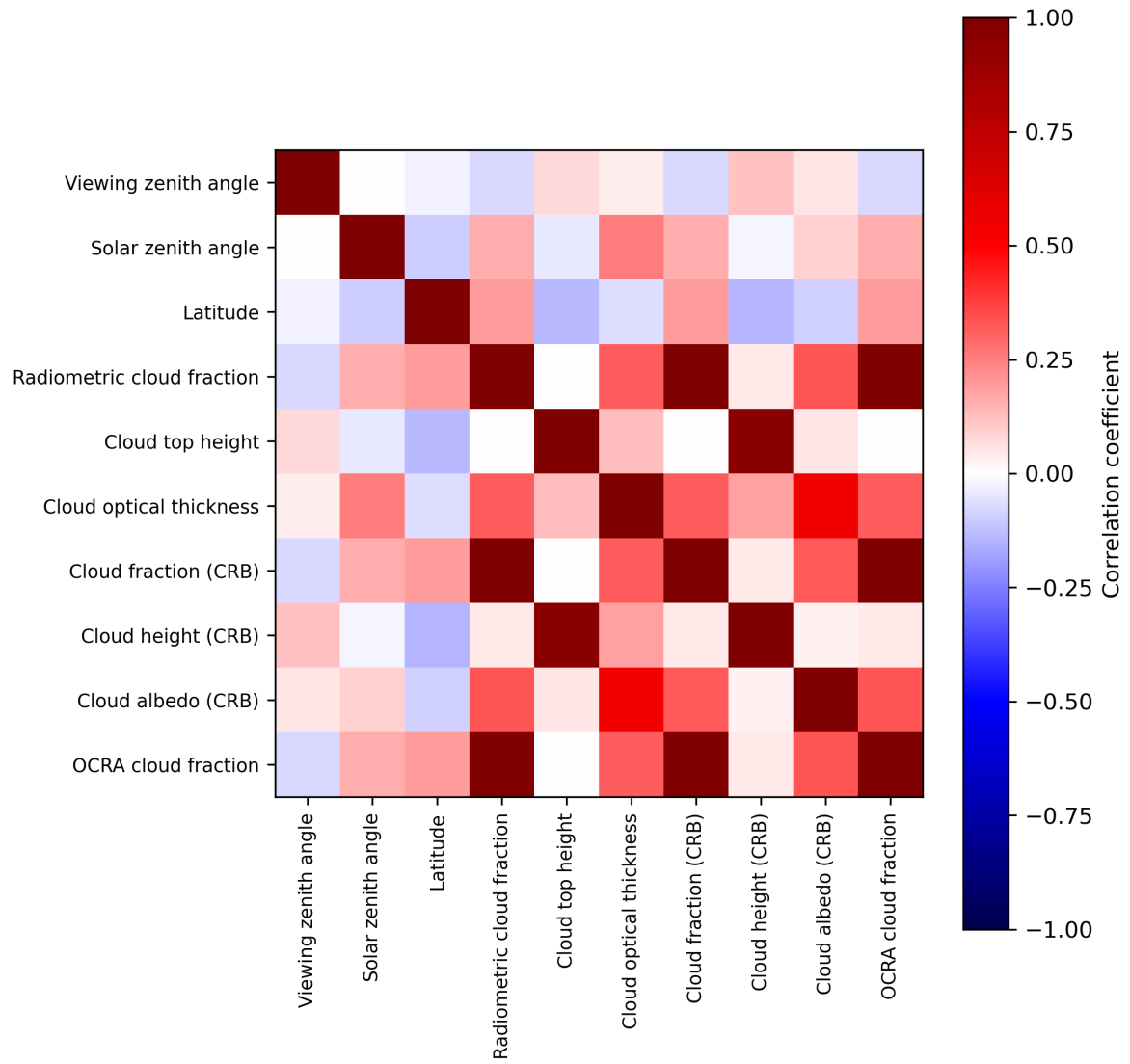
Figure 2: Map of correlation matrix for 2024-07-23 to 2024-07-25.
