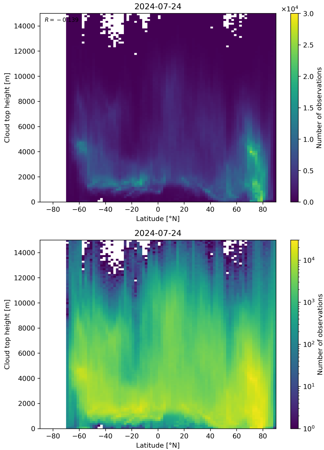
Figure 97: Scatter density plot of “Latitude” against “Cloud top height” for 2024-07-23 to 2024-07-25.
