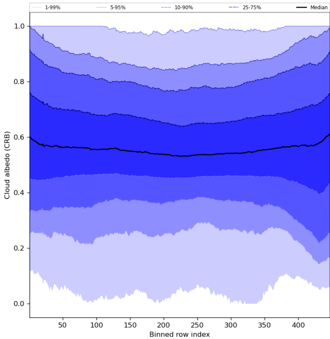
Figure 60: Along track statistics of “Cloud albedo (CRB)” for 2024-07-23 to 2024-07-25
