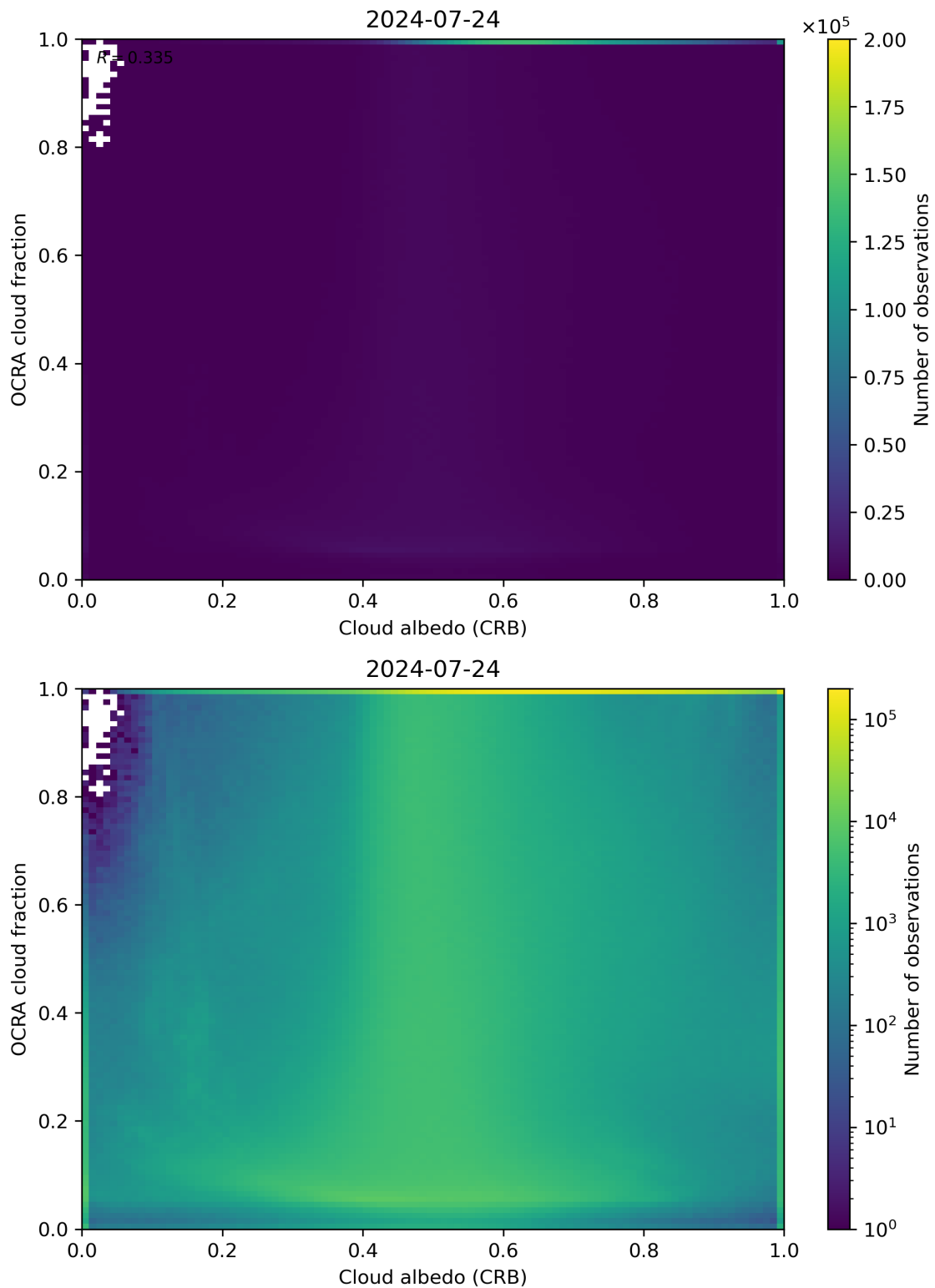
Figure 70: Scatter density plot of “Cloud albedo (CRB)” against “OCRA cloud fraction” for 2024-07-23 to 2024-07-25.
