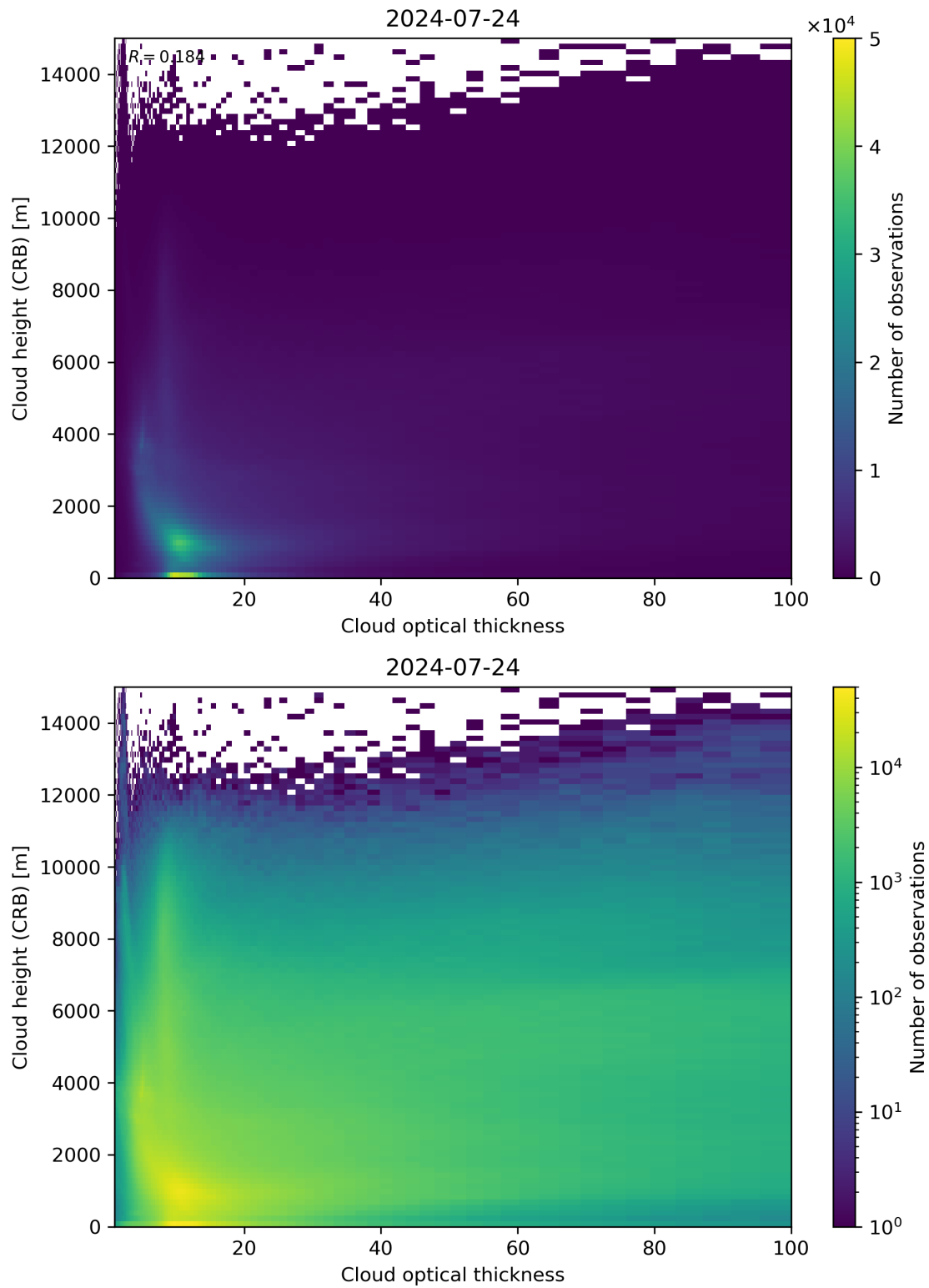
Figure 85: Scatter density plot of “Cloud optical thickness” against “Cloud height (CRB)” for 2024-07-23 to 2024-07-25.
