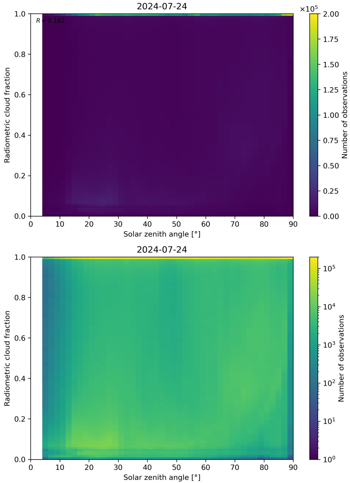
Figure 99: Scatter density plot of “Solar zenith angle” against “Radiometric cloud fraction” for 2024-07-23 to 2024-07-25.
