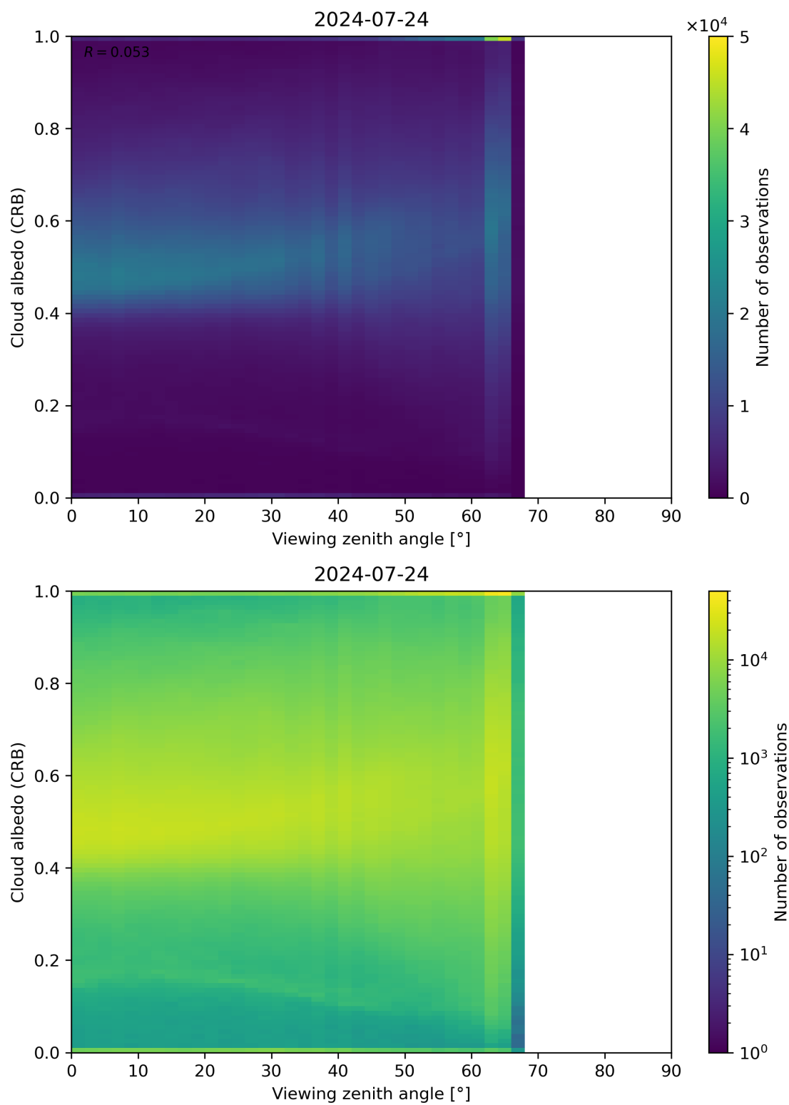
Figure 106: Scatter density plot of “Viewing zenith angle” against “Cloud albedo (CRB)” for 2024-07-23 to 2024-07-25.
