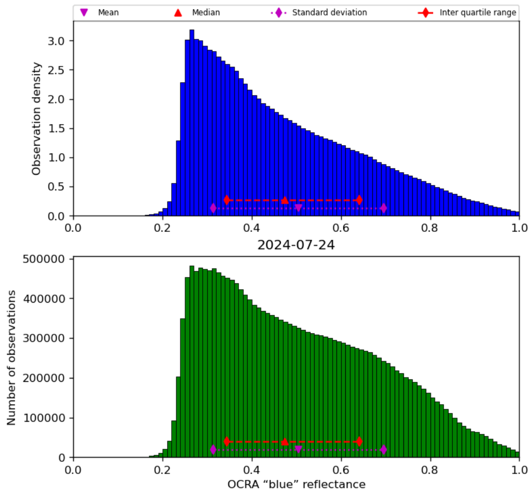
Figure 51: Histogram of “OCRA “blue” reflectance” for 2024-07-23 to 2024-07-25
