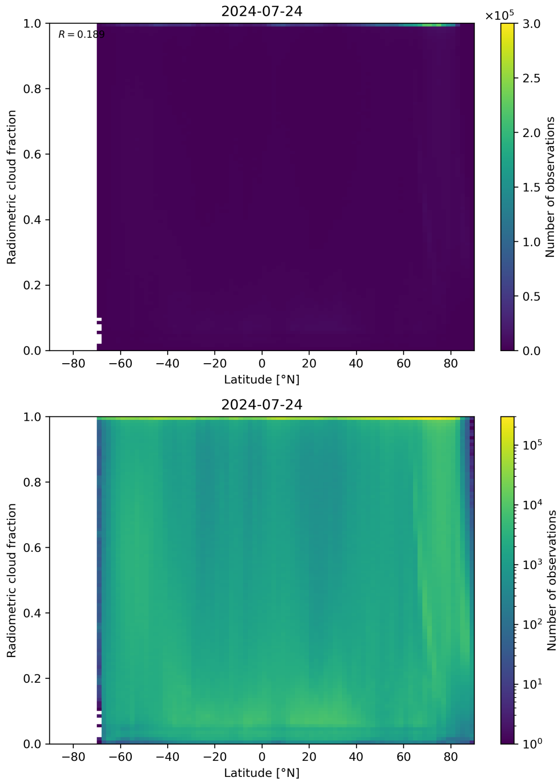
Figure 92: Scatter density plot of “Latitude” against “Radiometric cloud fraction” for 2024-07-23 to 2024-07-25.
