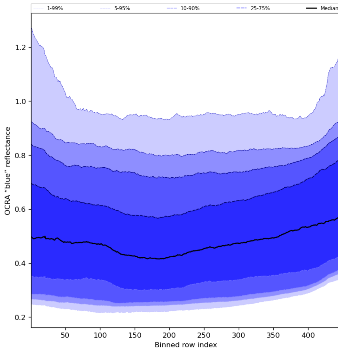
Figure 67: Along track statistics of “OCRA “blue” reflectance” for 2024-07-23 to 2024-07-25
