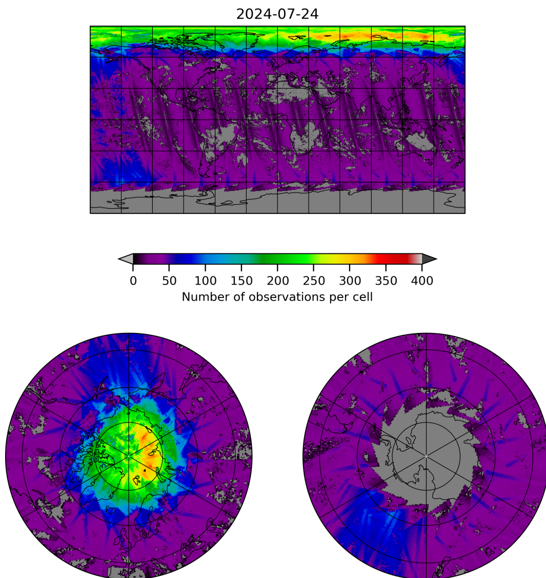
Figure 21: Map of the number of observations for 2024-07-23 to 2024-07-25
