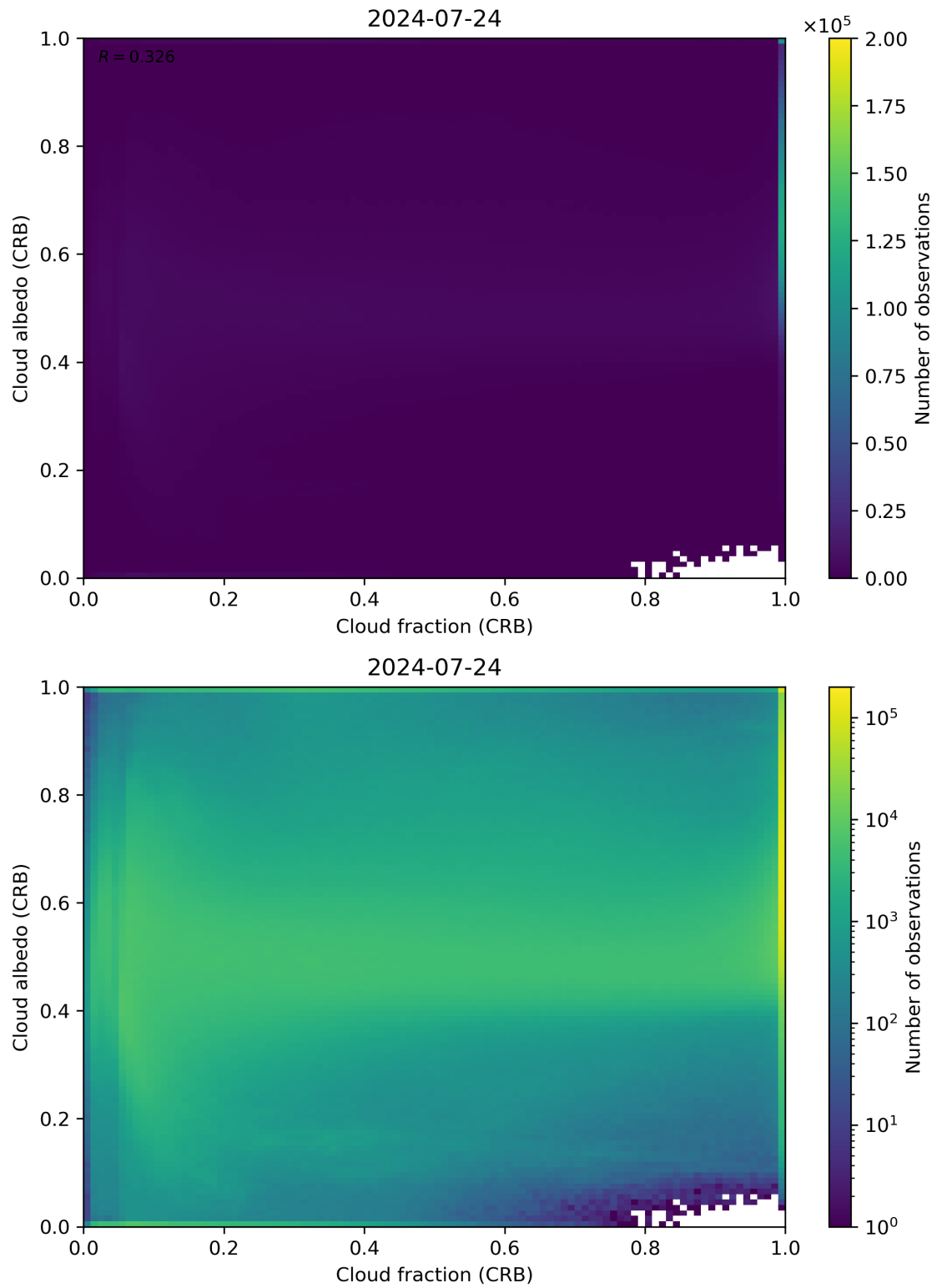
Figure 77: Scatter density plot of “Cloud fraction (CRB)” against “Cloud albedo (CRB)” for 2024-07-23 to 2024-07-25.
