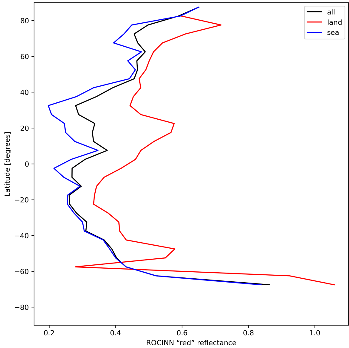
Figure 37: Zonal average of "ROCINN "red" reflectance" for 2024-07-23 to 2024-07-25.
