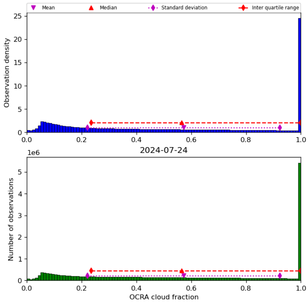
Figure 50: Histogram of “OCRA cloud fraction” for 2024-07-23 to 2024-07-25
