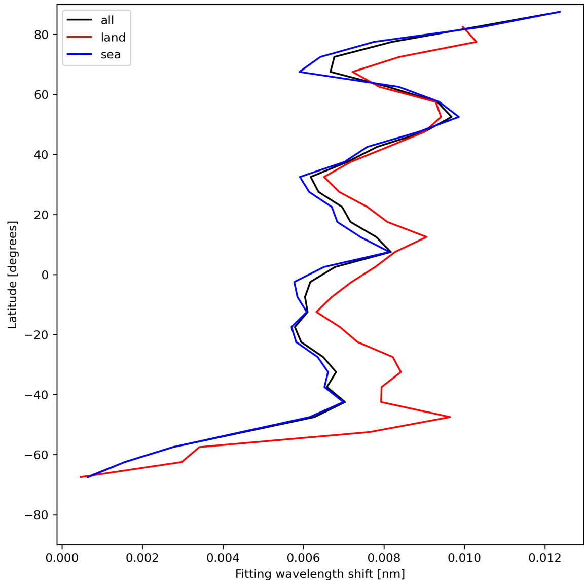
Figure 33: Zonal average of “Fitting wavelength shift” for 2024-07-23 to 2024-07-25.
