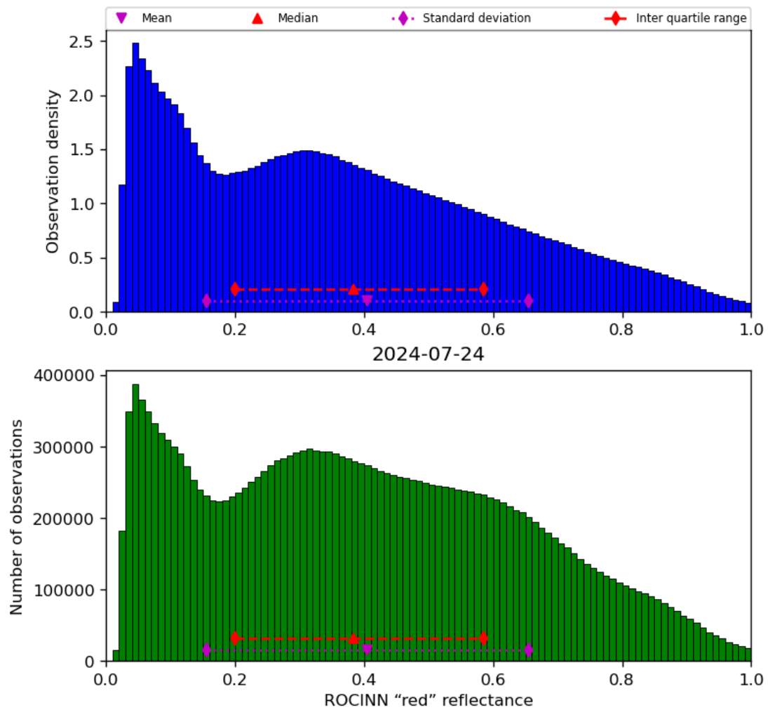
Figure 53: Histogram of “ROCINN “red” reflectance” for 2024-07-23 to 2024-07-25
