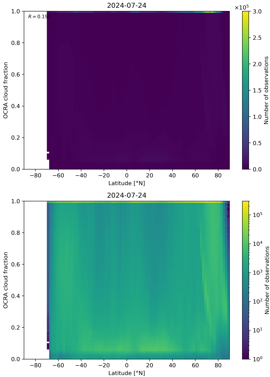
Figure 93: Scatter density plot of “Latitude” against “OCRA cloud fraction” for 2024-07-23 to 2024-07-25.
