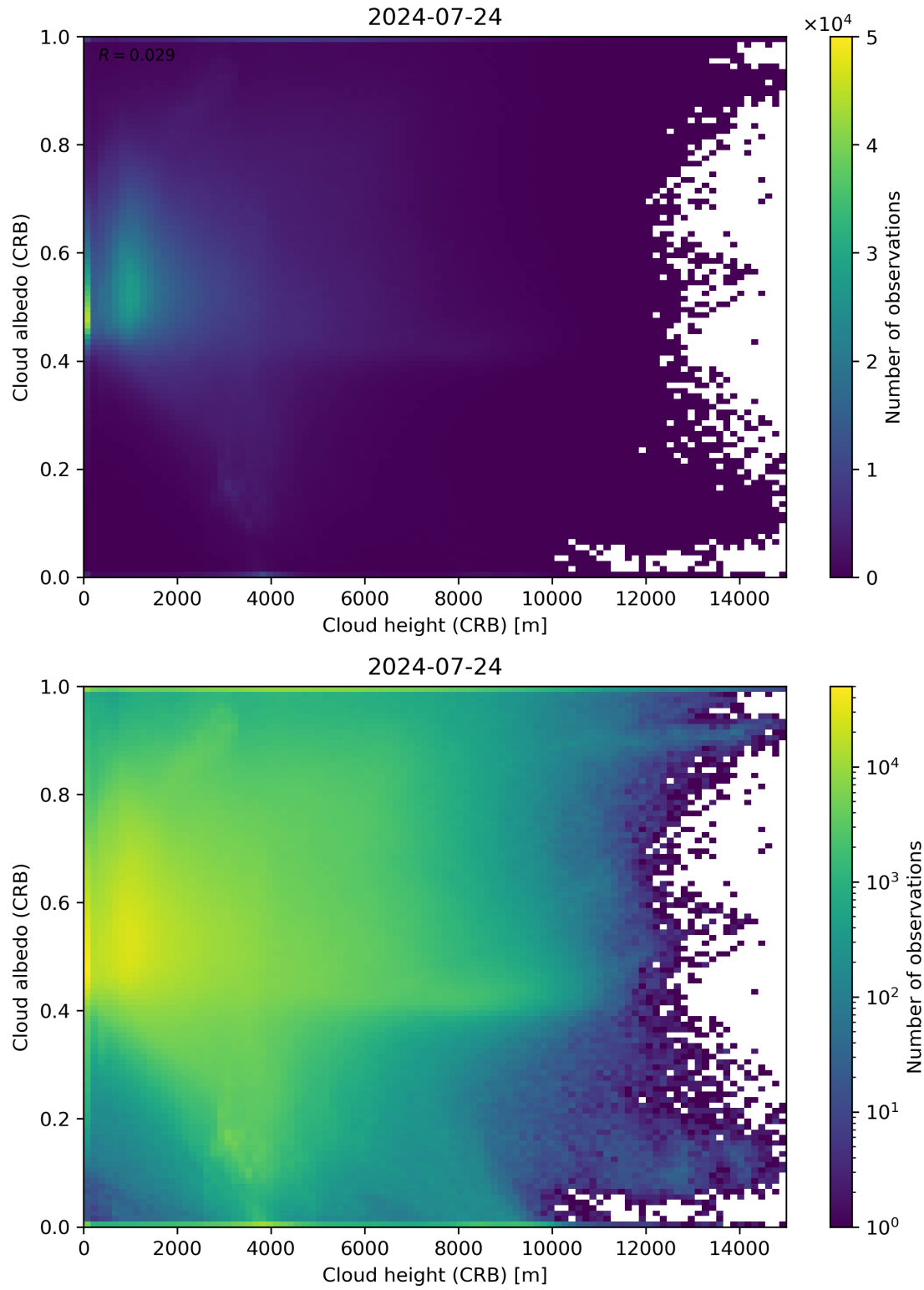
Figure 80: Scatter density plot of “Cloud height (CRB)” against “Cloud albedo (CRB)” for 2024-07-23 to 2024-07-25.
