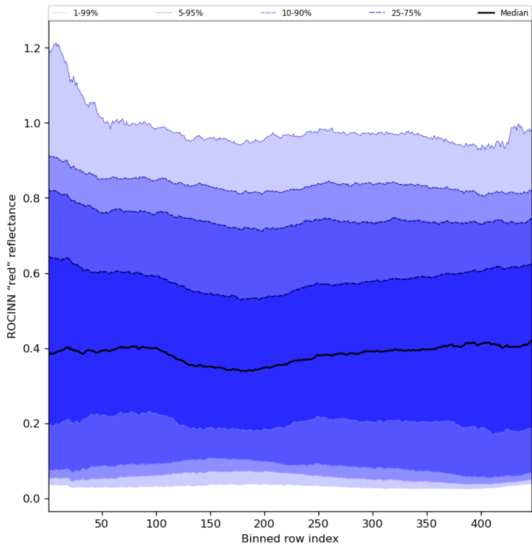
Figure 69: Along track statistics of "ROCINN "red" reflectance" for 2024-07-23 to 2024-07-25
