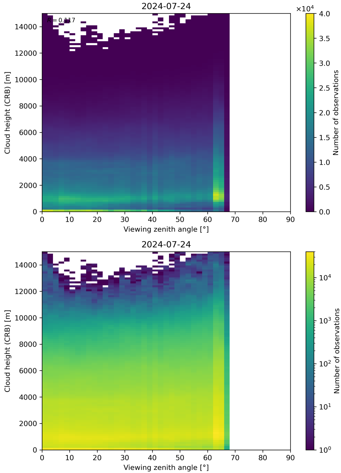
Figure 110: Scatter density plot of “Viewing zenith angle” against “Cloud height (CRB)” for 2024-07-23 to 2024-07-25.
