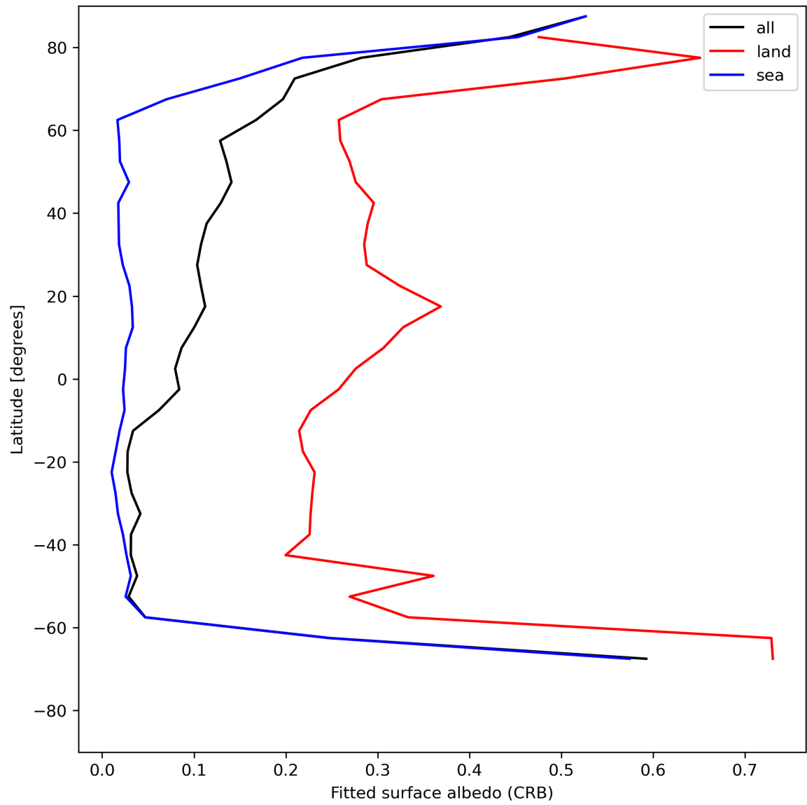
Figure 30: Zonal average of “Fitted surface albedo (CRB)” for 2024-07-23 to 2024-07-25.
