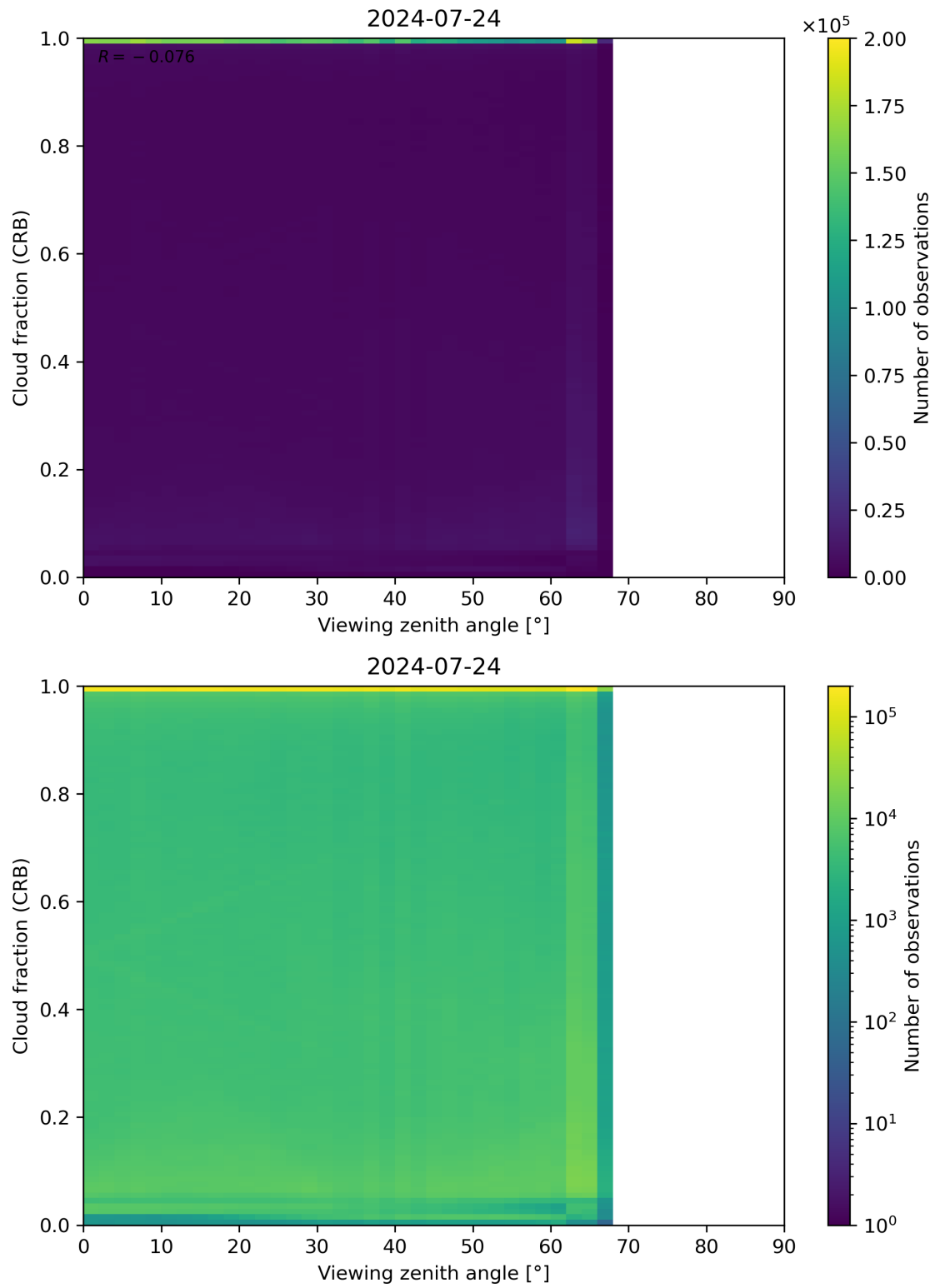
Figure 109: Scatter density plot of “Viewing zenith angle” against “Cloud fraction (CRB)” for 2024-07-23 to 2024-07-25.
