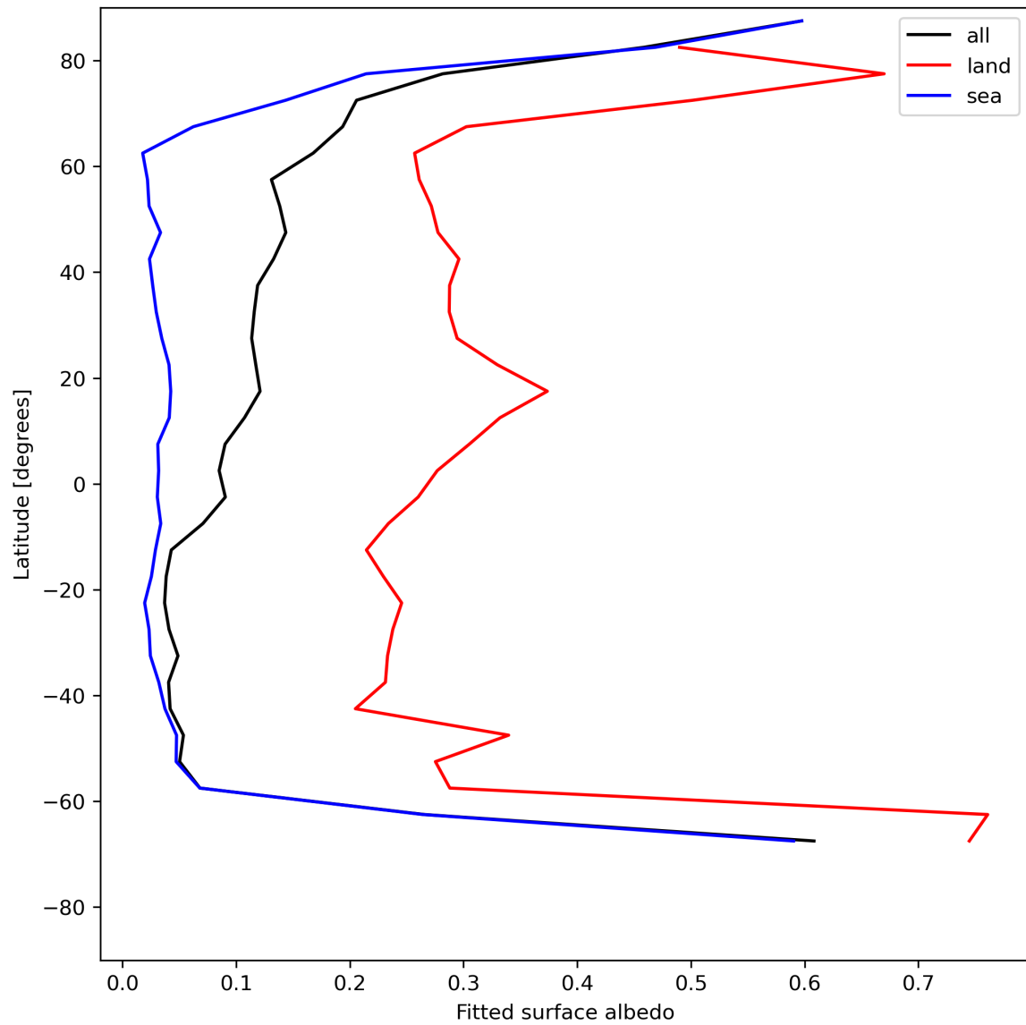
Figure 29: Zonal average of “Fitted surface albedo” for 2024-07-23 to 2024-07-25.
