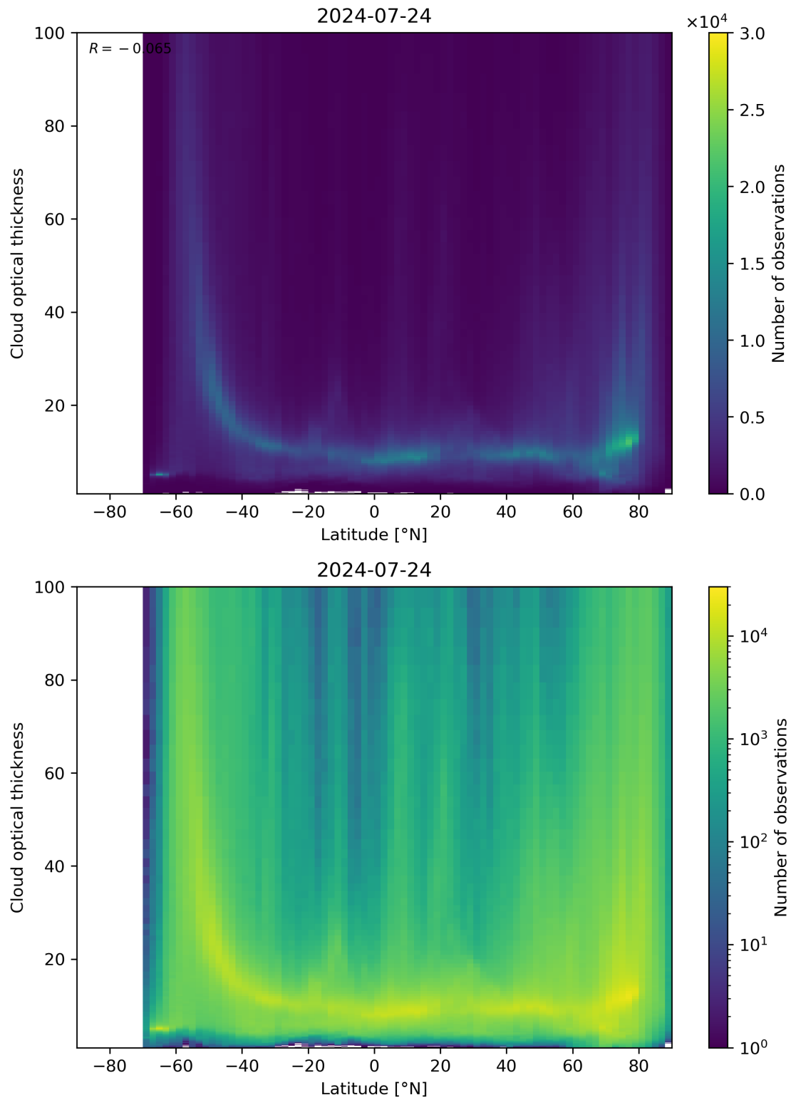
Figure 96: Scatter density plot of “Latitude” against “Cloud optical thickness” for 2024-07-23 to 2024-07-25.
