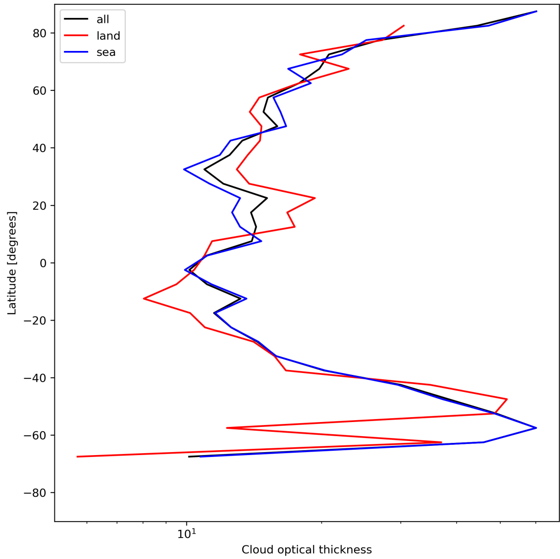
Figure 25: Zonal average of “Cloud optical thickness” for 2024-07-23 to 2024-07-25.
