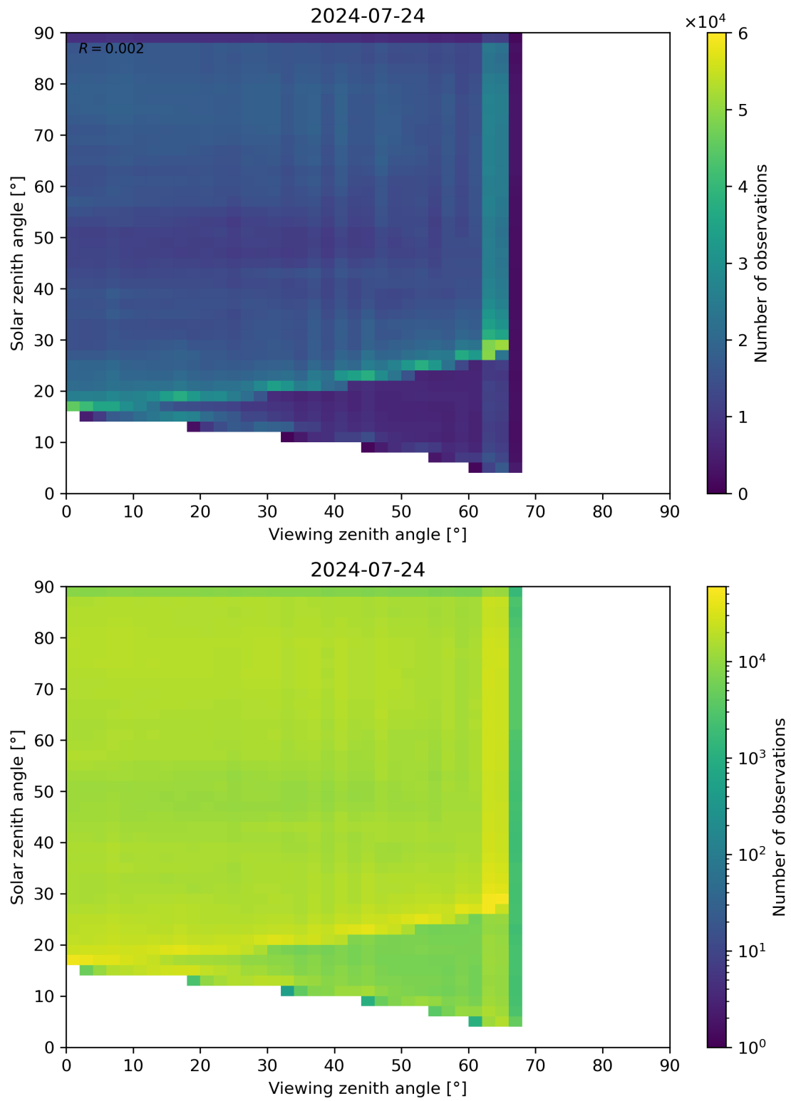
Figure 114: Scatter density plot of “Viewing zenith angle” against “Solar zenith angle” for 2024-07-23 to 2024-07-25.
