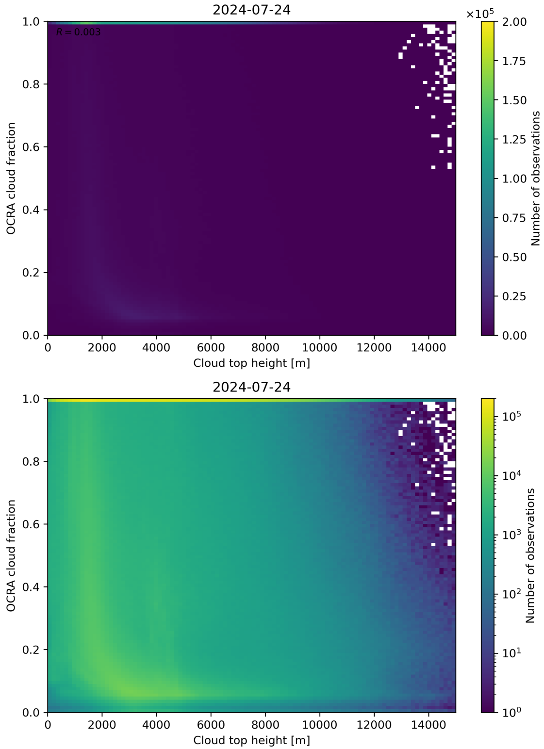
Figure 87: Scatter density plot of “Cloud top height” against “OCRA cloud fraction” for 2024-07-23 to 2024-07-25.
