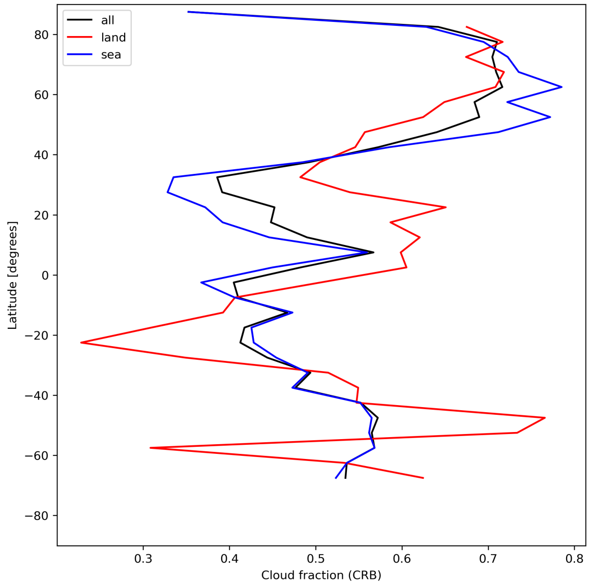
Figure 26: Zonal average of “Cloud fraction (CRB)” for 2024-07-23 to 2024-07-25.
