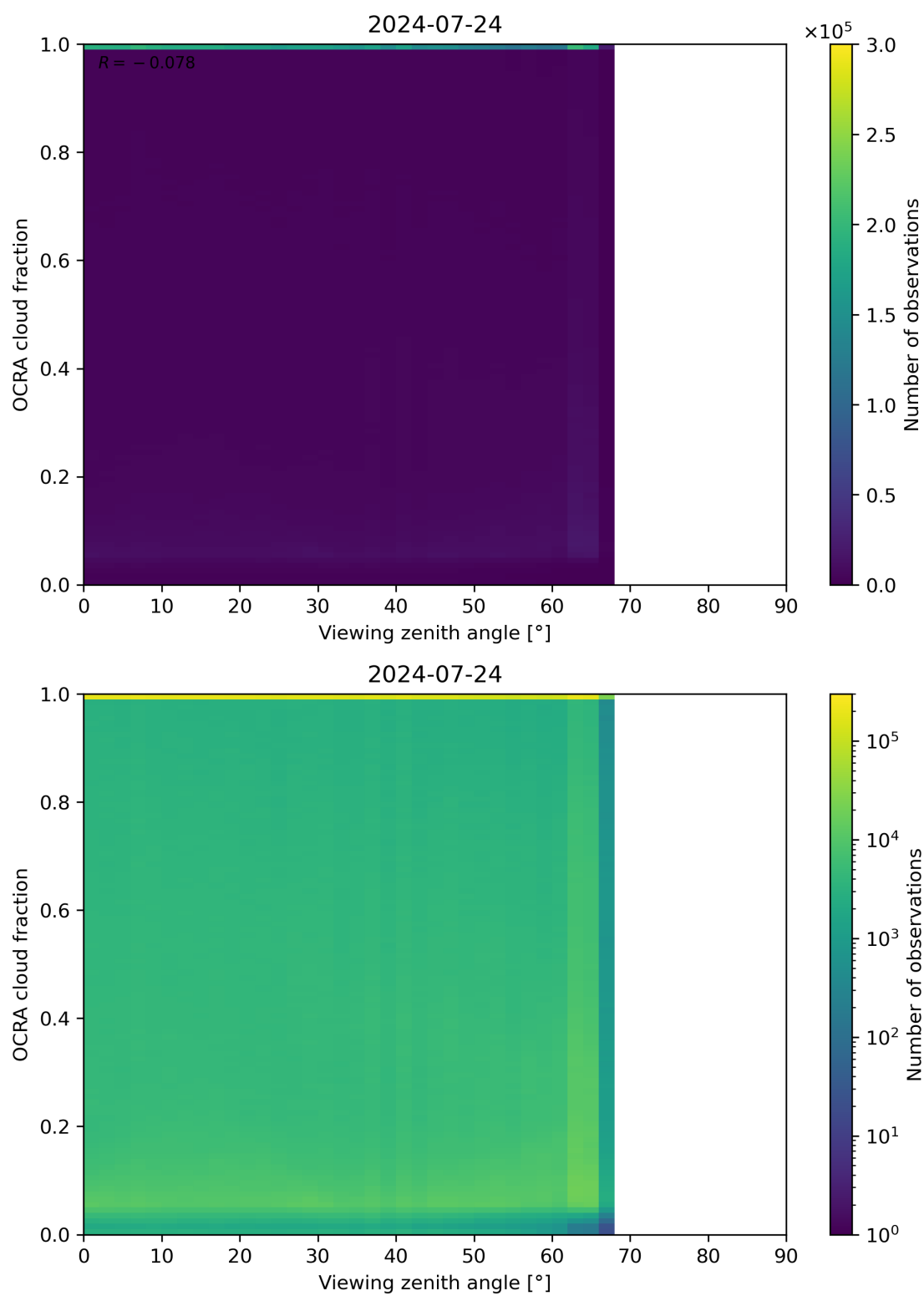
Figure 108: Scatter density plot of “Viewing zenith angle” against “OCRA cloud fraction” for 2024-07-23 to 2024-07-25.
