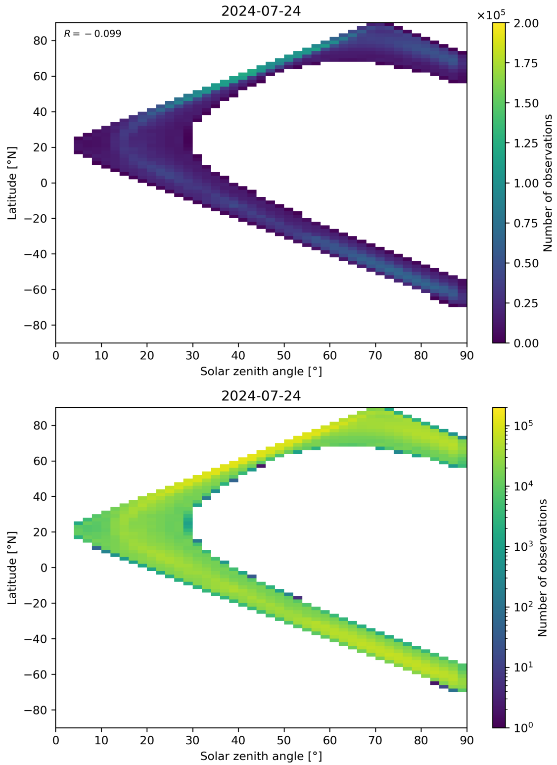
Figure 105: Scatter density plot of “Solar zenith angle” against “Latitude” for 2024-07-23 to 2024-07-25.
