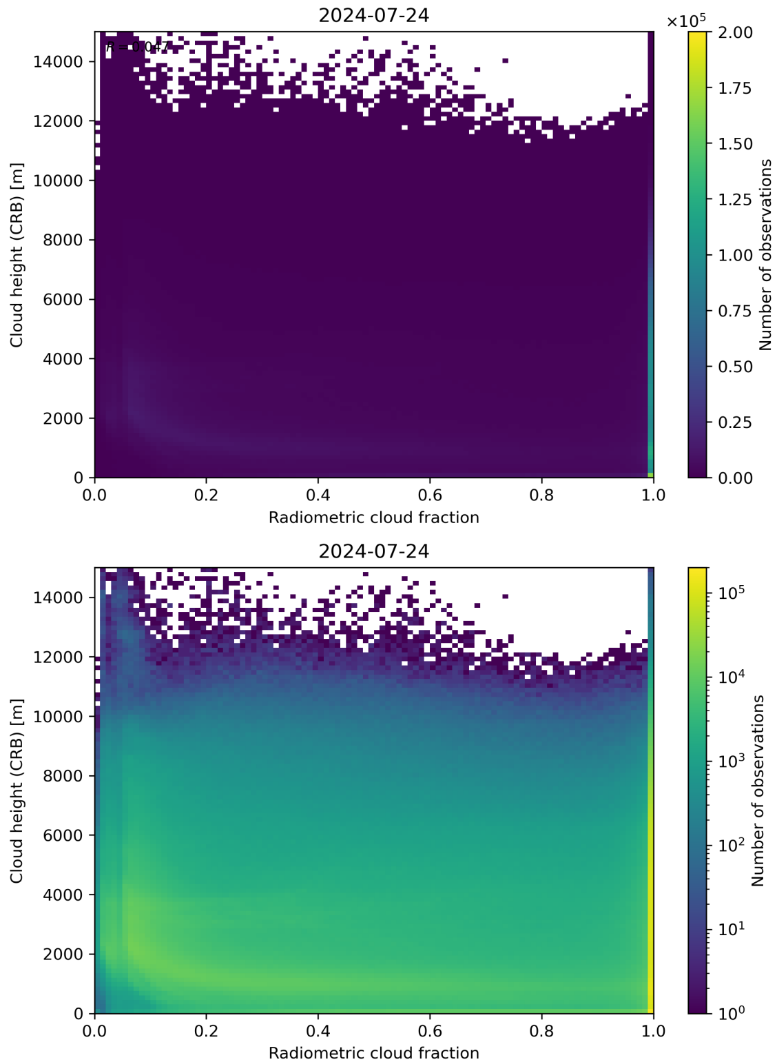
Figure 74: Scatter density plot of “Radiometric cloud fraction” against “Cloud height (CRB)” for 2024-07-23 to 2024-07-25.
