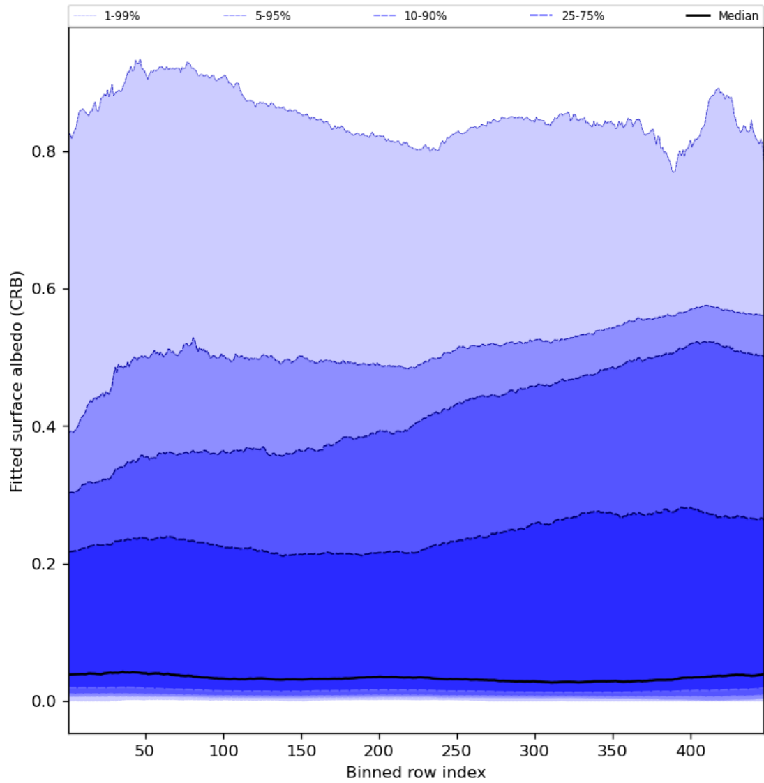
Figure 62: Along track statistics of “Fitted surface albedo (CRB)” for 2024-07-23 to 2024-07-25
