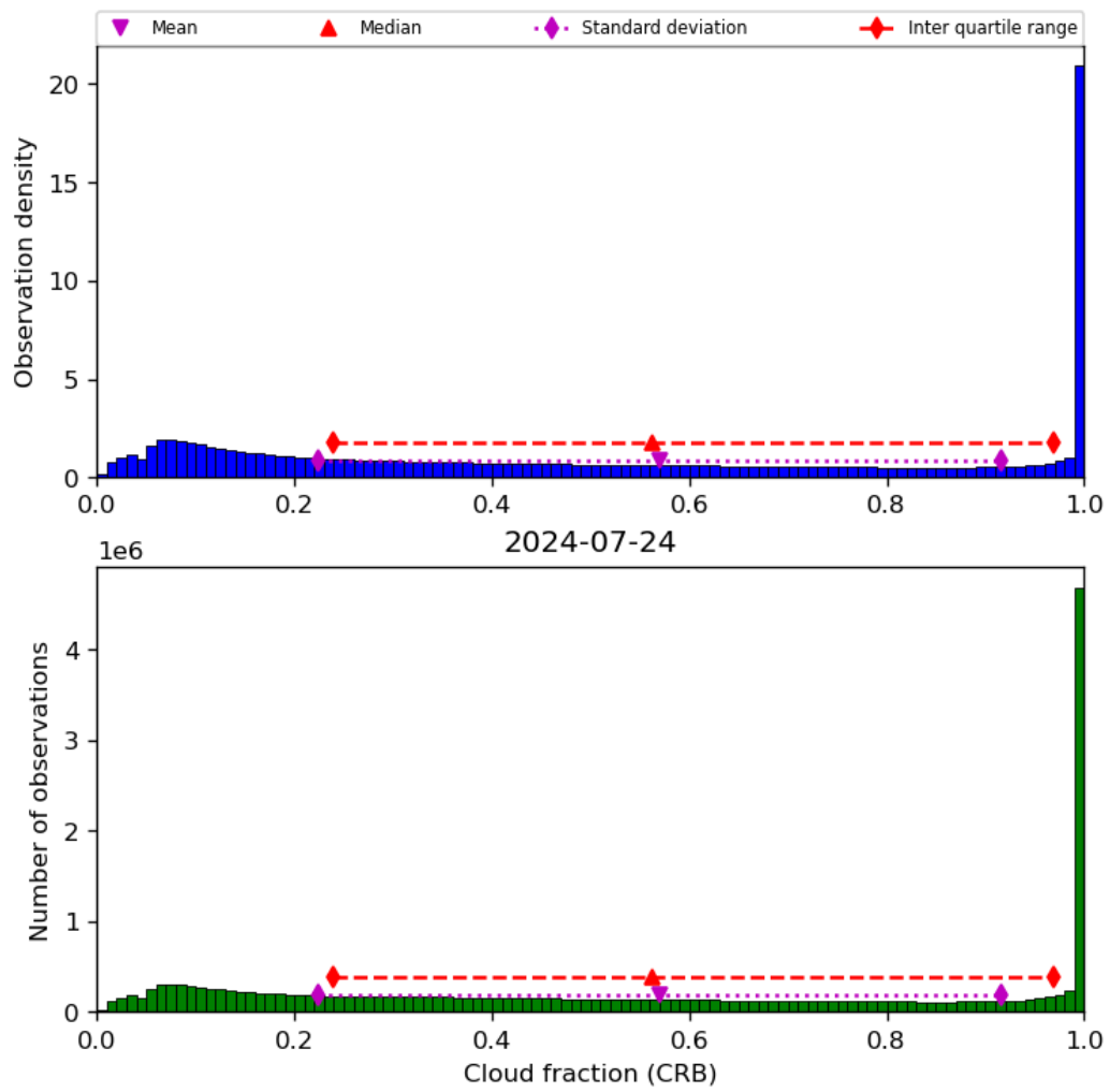
Figure 42: Histogram of “Cloud fraction (CRB)” for 2024-07-23 to 2024-07-25
