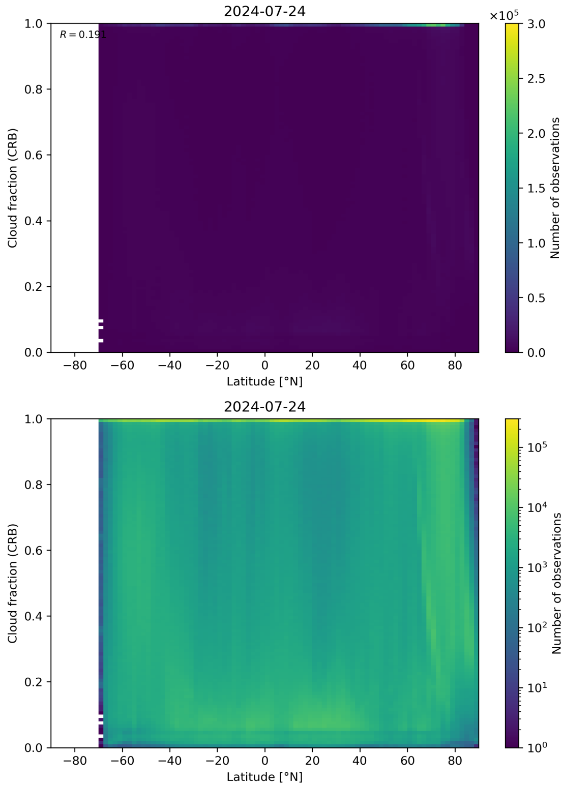
Figure 94: Scatter density plot of “Latitude” against “Cloud fraction (CRB)” for 2024-07-23 to 2024-07-25.
