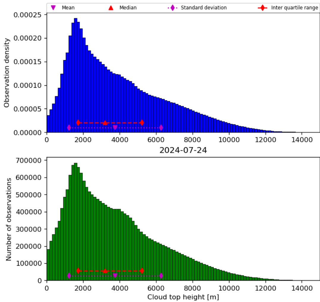
Figure 40: Histogram of “Cloud top height” for 2024-07-23 to 2024-07-25
