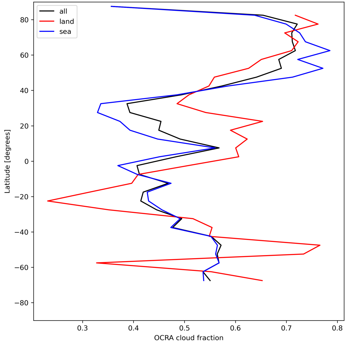
Figure 34: Zonal average of “OCRA cloud fraction” for 2024-07-23 to 2024-07-25.
