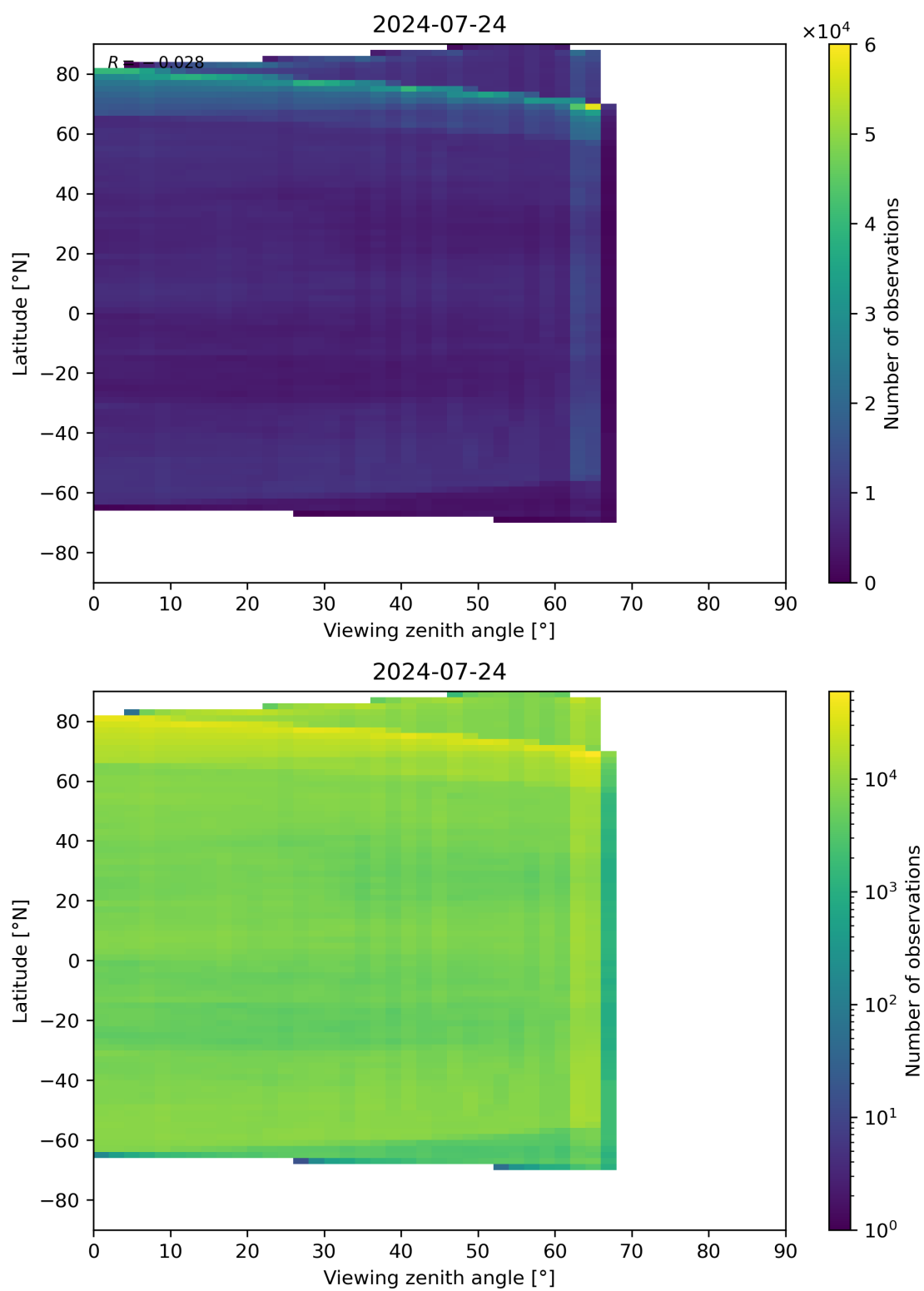
Figure 113: Scatter density plot of “Viewing zenith angle” against “Latitude” for 2024-07-23 to 2024-07-25.
