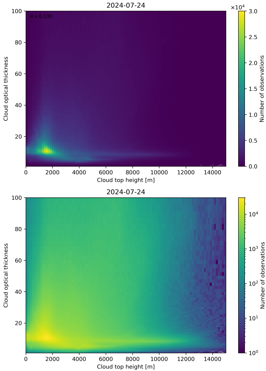
Figure 90: Scatter density plot of “Cloud top height” against “Cloud optical thickness” for 2024-07-23 to 2024-07-25.
