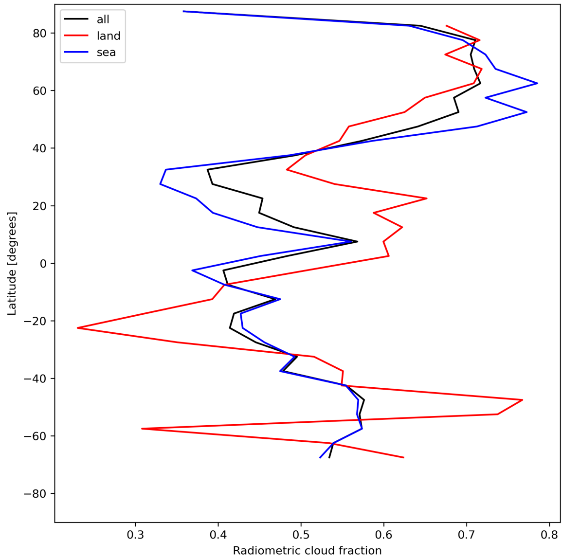
Figure 23: Zonal average of “Radiometric cloud fraction” for 2024-07-23 to 2024-07-25.
