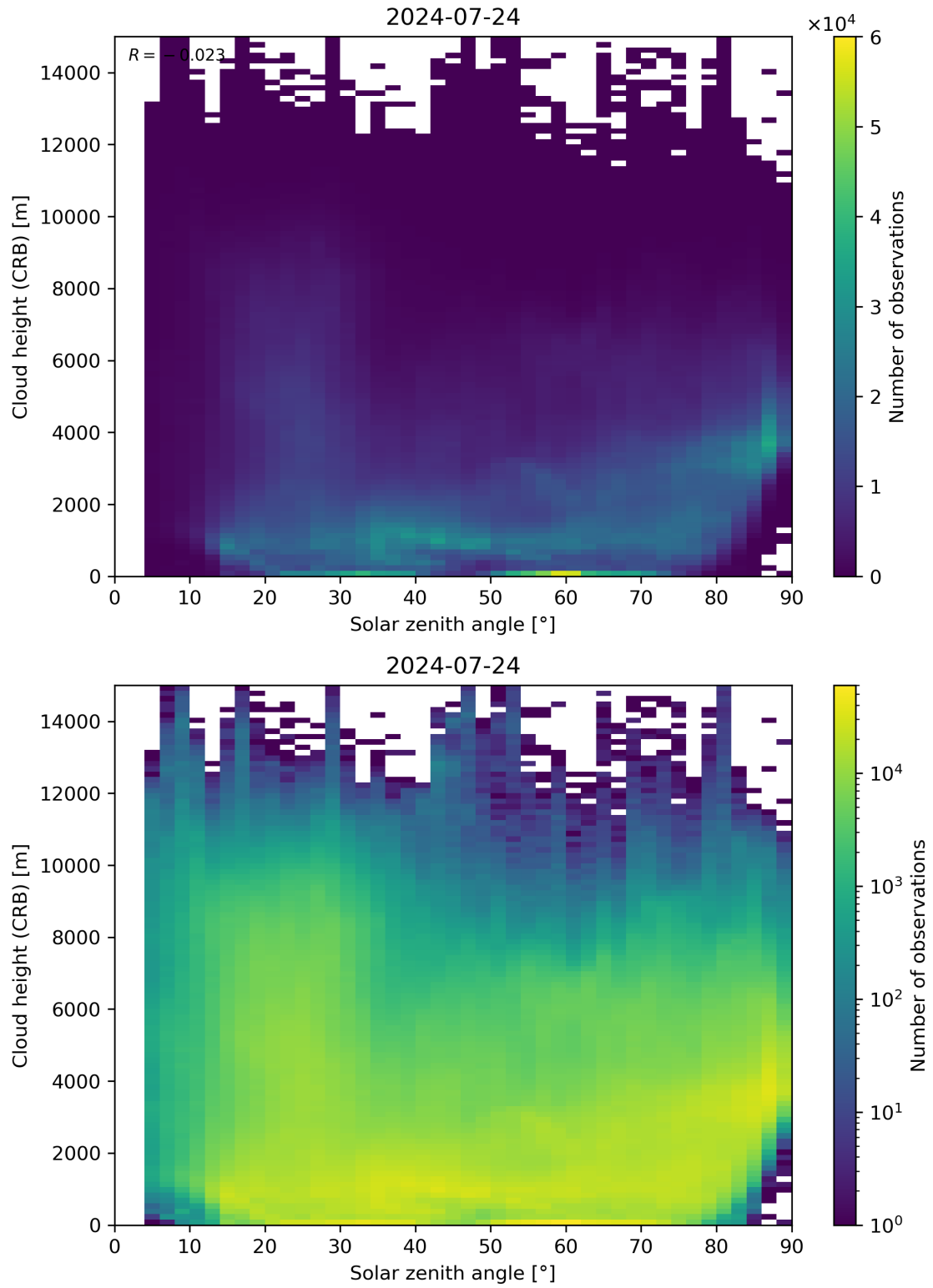
Figure 102: Scatter density plot of “Solar zenith angle” against “Cloud height (CRB)” for 2024-07-23 to 2024-07-25.
