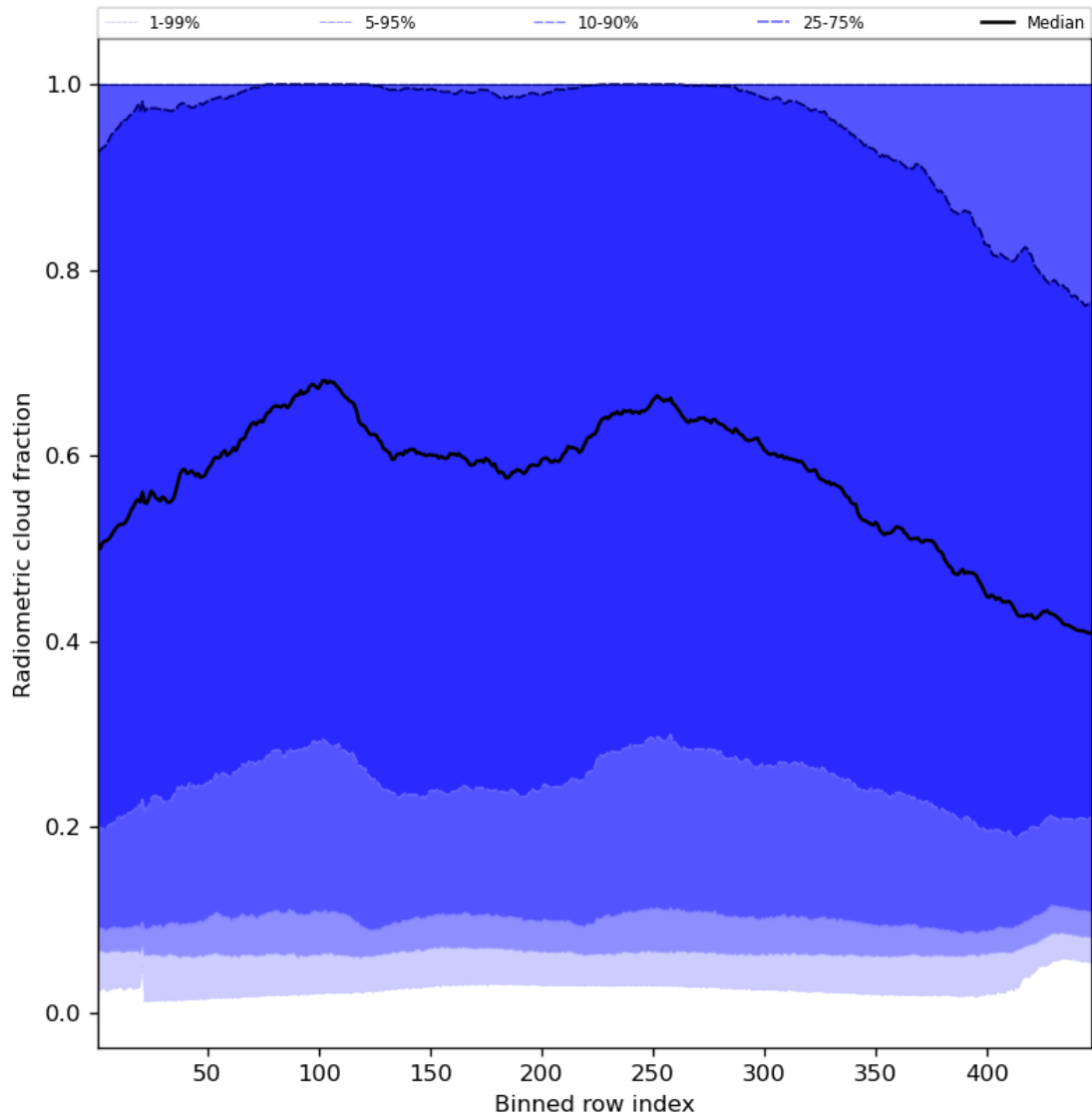
Figure 55: Along track statistics of “Radiometric cloud fraction” for 2024-07-23 to 2024-07-25
