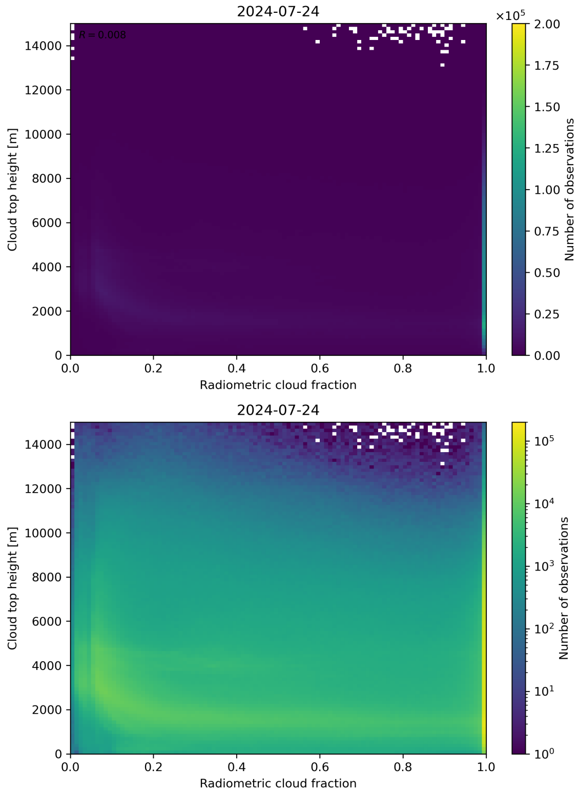
Figure 76: Scatter density plot of “Radiometric cloud fraction” against “Cloud top height” for 2024-07-23 to 2024-07-25.
