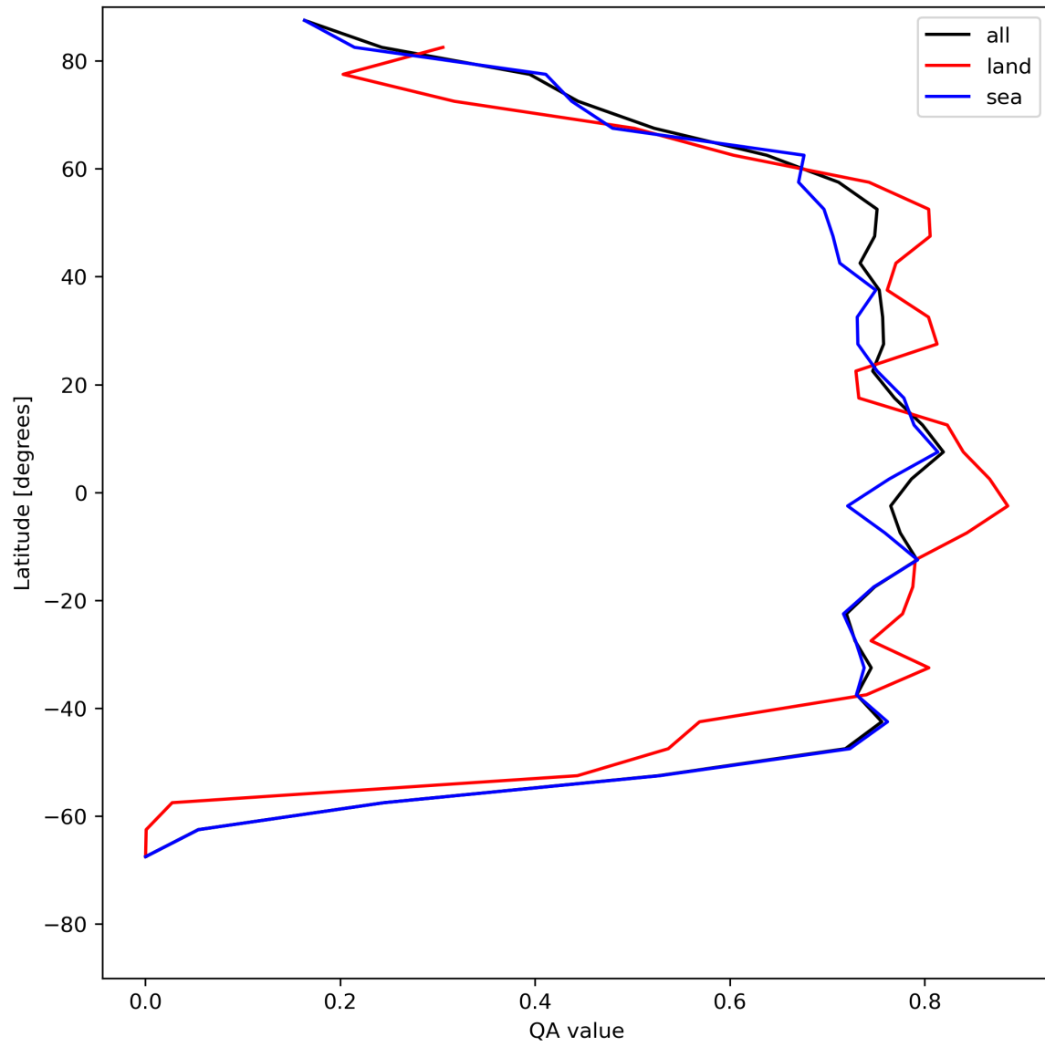
Figure 22: Zonal average of “QA value” for 2024-07-23 to 2024-07-25.
