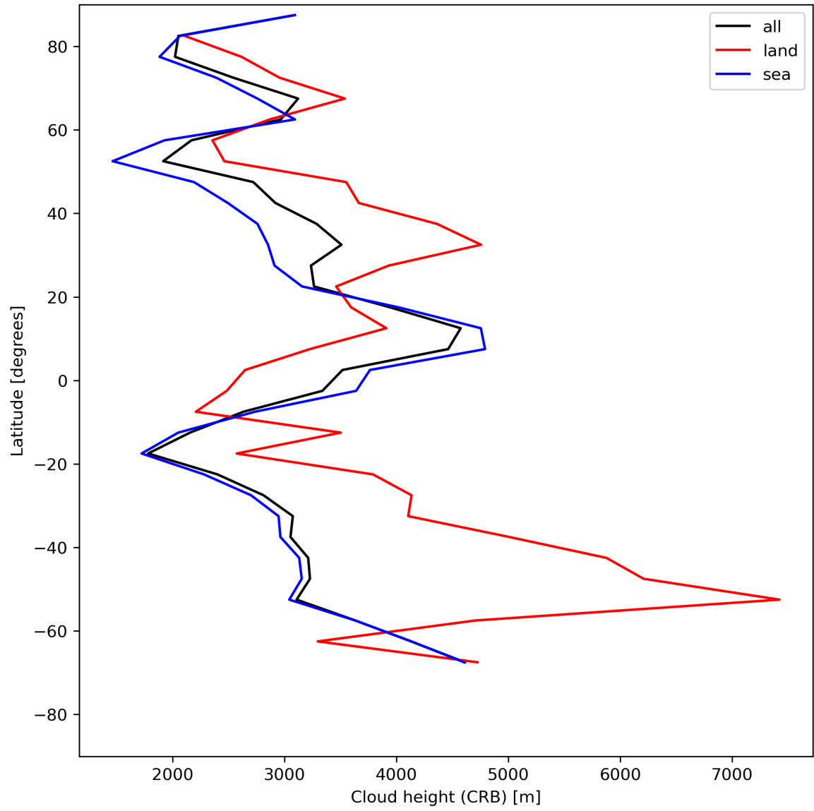
Figure 27: Zonal average of “Cloud height (CRB)” for 2024-07-23 to 2024-07-25.
