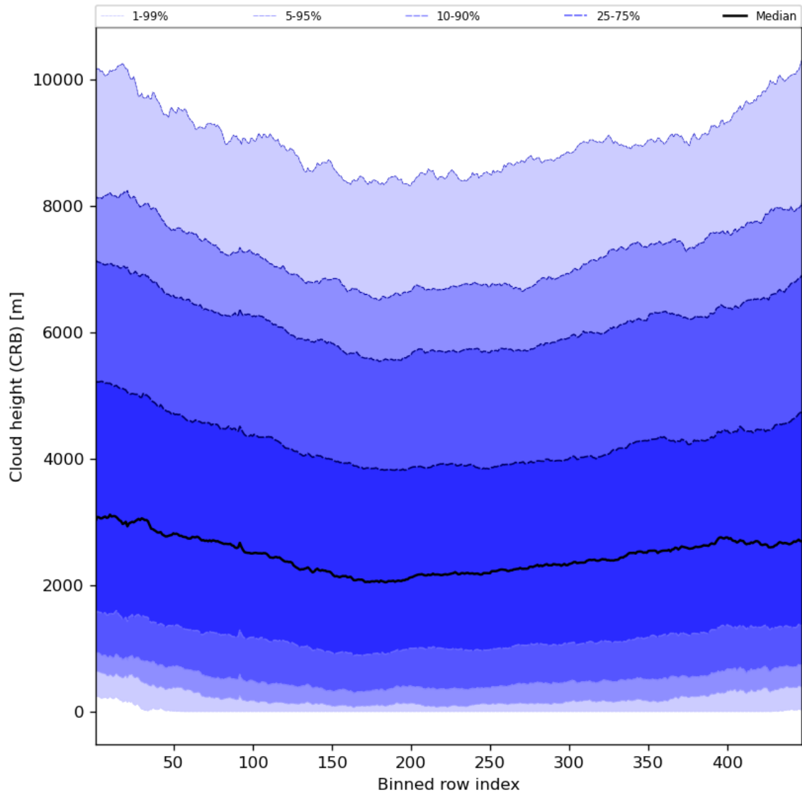
Figure 59: Along track statistics of “Cloud height (CRB)” for 2024-07-23 to 2024-07-25
