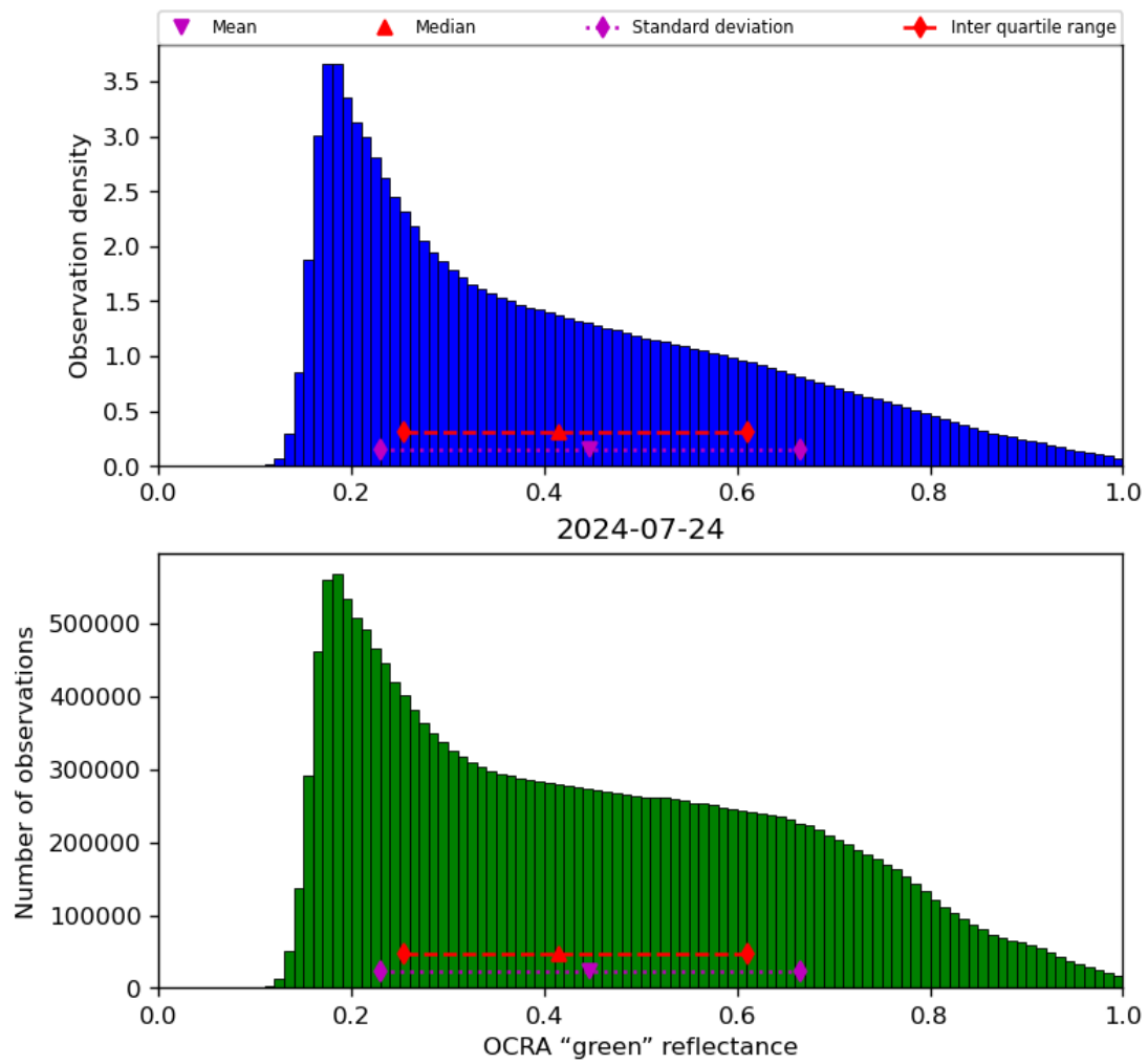
Figure 52: Histogram of “OCRA “green” reflectance” for 2024-07-23 to 2024-07-25
