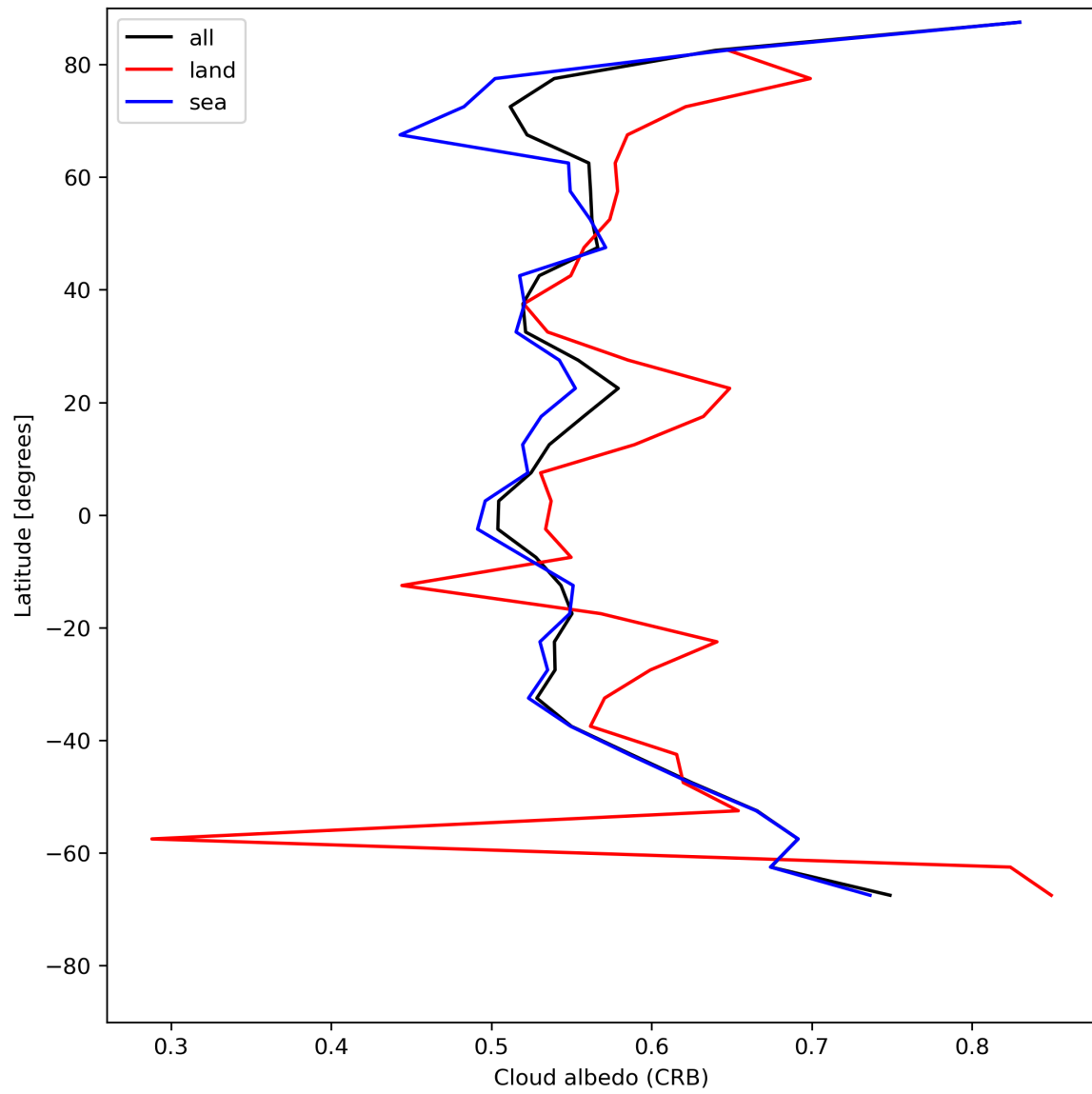
Figure 28: Zonal average of “Cloud albedo (CRB)” for 2024-07-23 to 2024-07-25.
