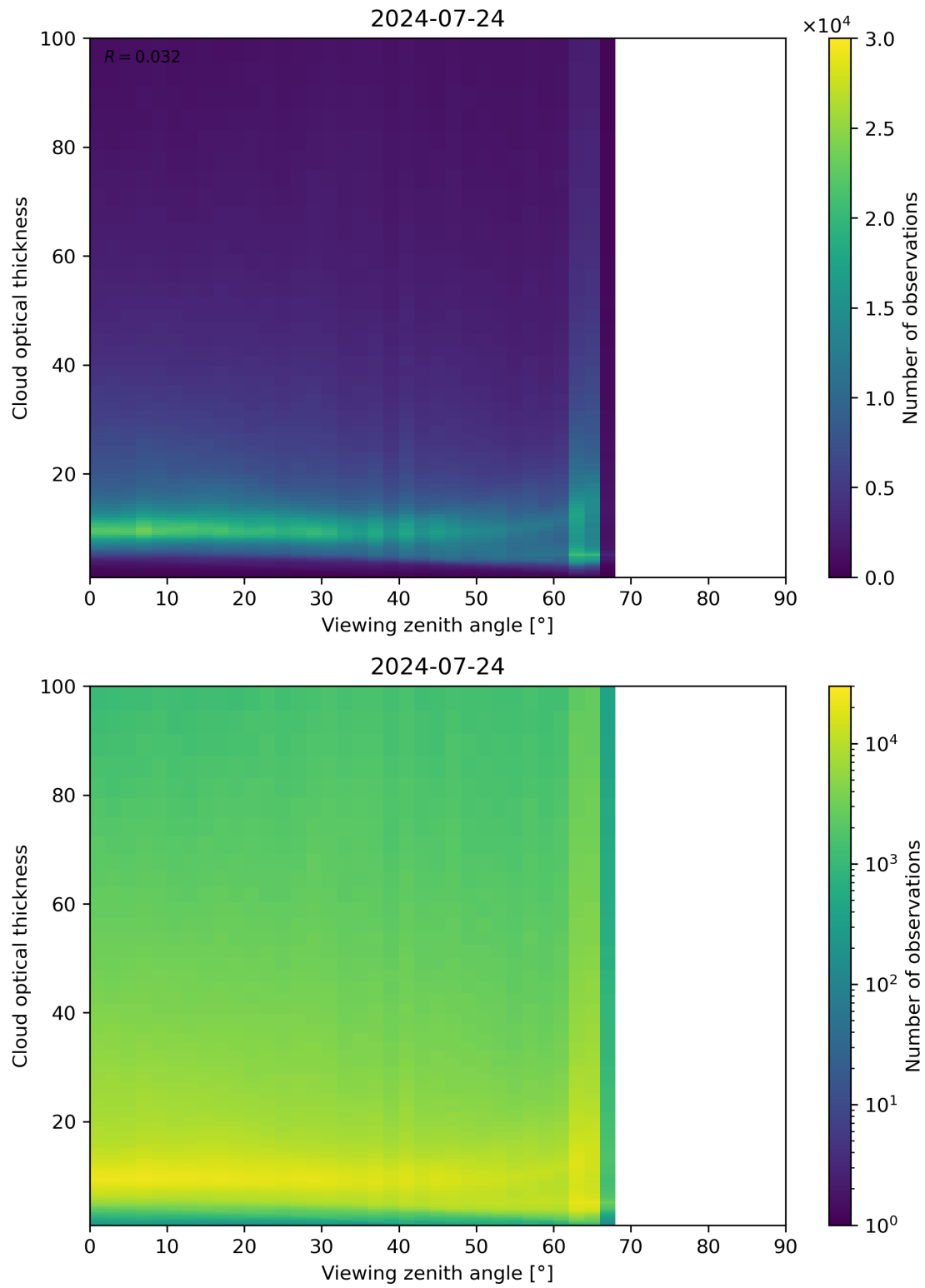
Figure 111: Scatter density plot of “Viewing zenith angle” against “Cloud optical thickness” for 2024-07-23 to 2024-07-25.
