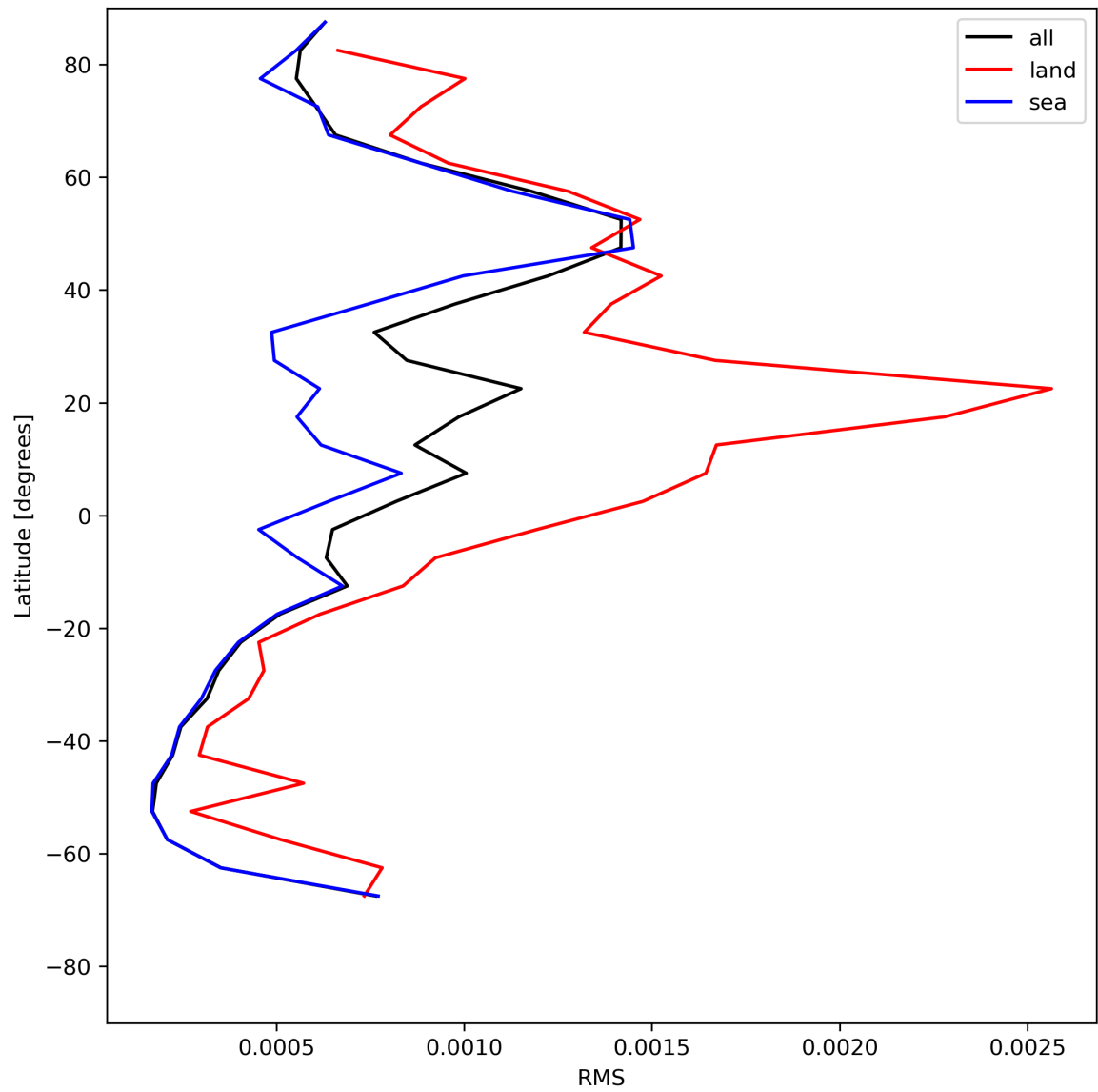
Figure 31: Zonal average of “RMS” for 2024-07-23 to 2024-07-25.
