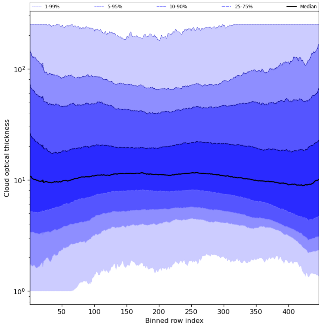
Figure 57: Along track statistics of “Cloud optical thickness” for 2024-07-23 to 2024-07-25
