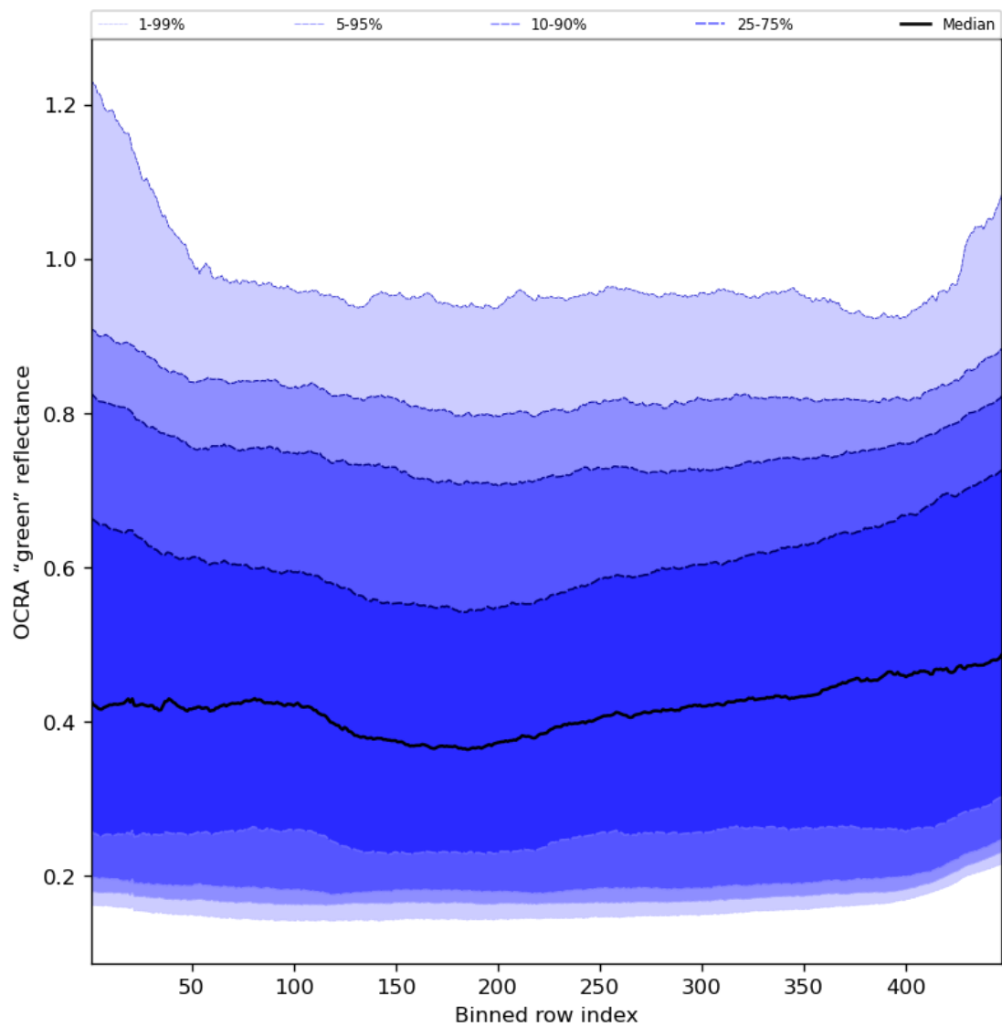
Figure 68: Along track statistics of “OCRA “green” reflectance” for 2024-07-23 to 2024-07-25
