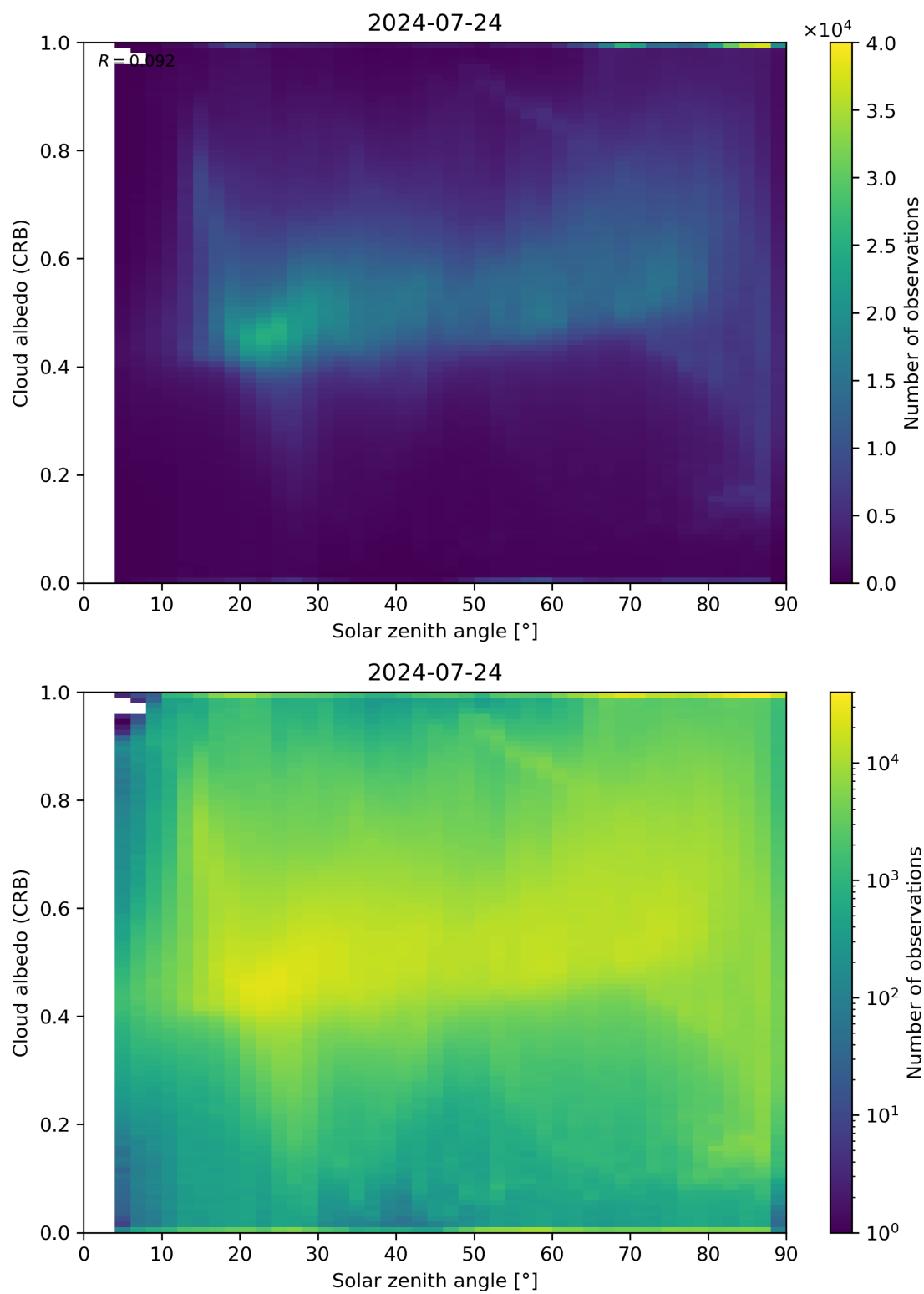
Figure 98: Scatter density plot of “Solar zenith angle” against “Cloud albedo (CRB)” for 2024-07-23 to 2024-07-25.
