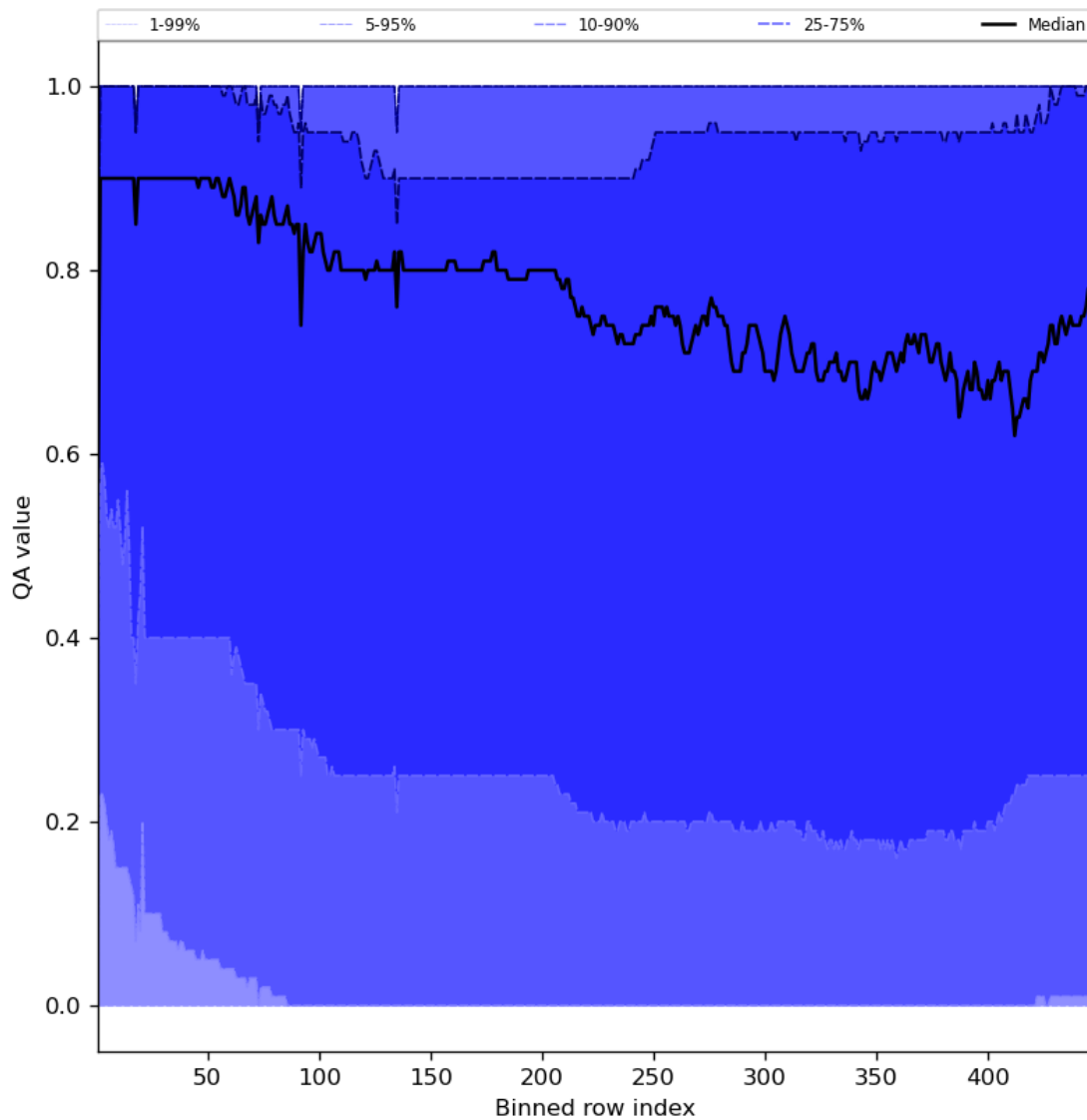
Figure 54: Along track statistics of “QA value” for 2024-07-23 to 2024-07-25
