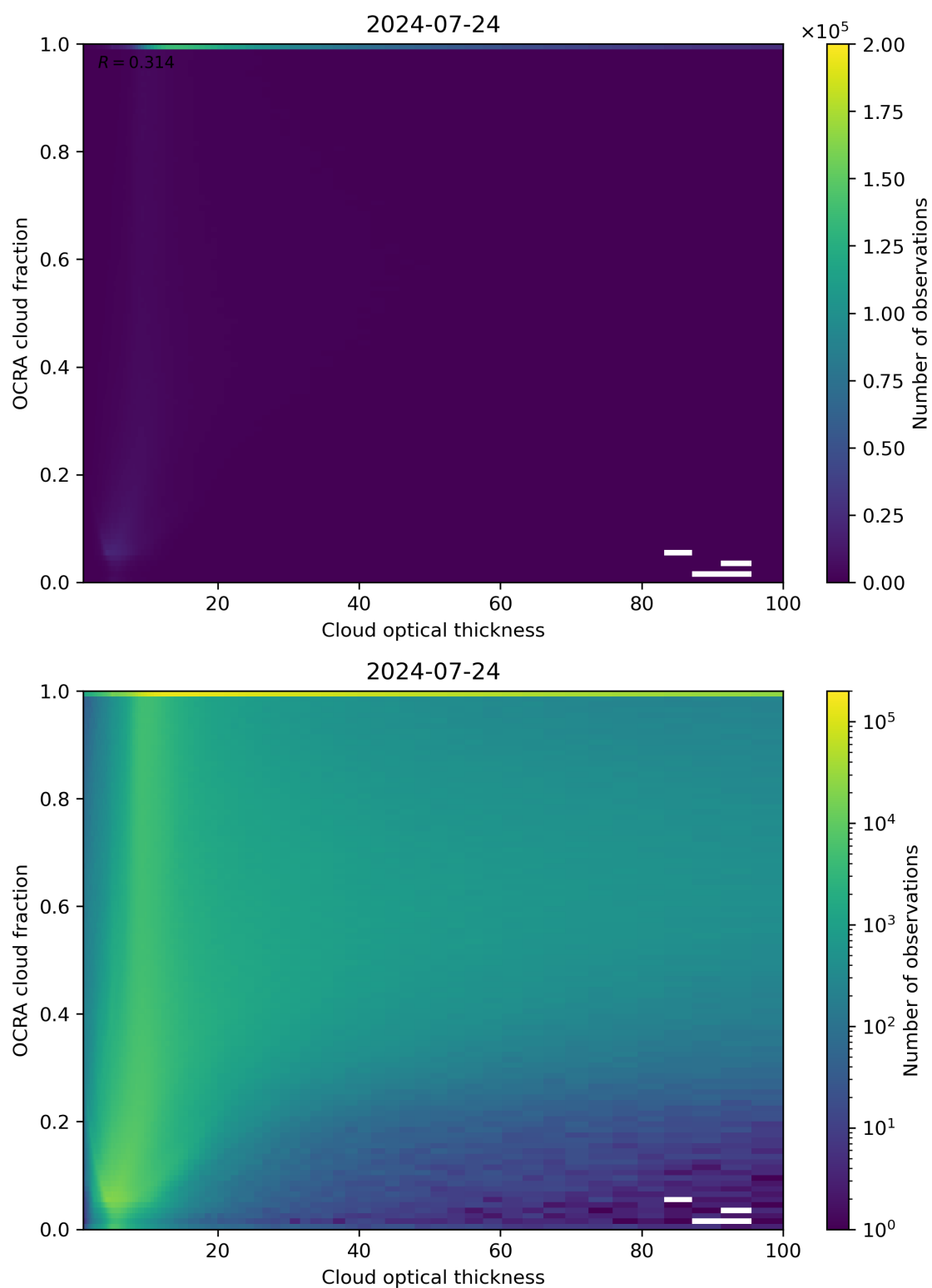
Figure 83: Scatter density plot of “Cloud optical thickness” against “OCRA cloud fraction” for 2024-07-23 to 2024-07-25.
