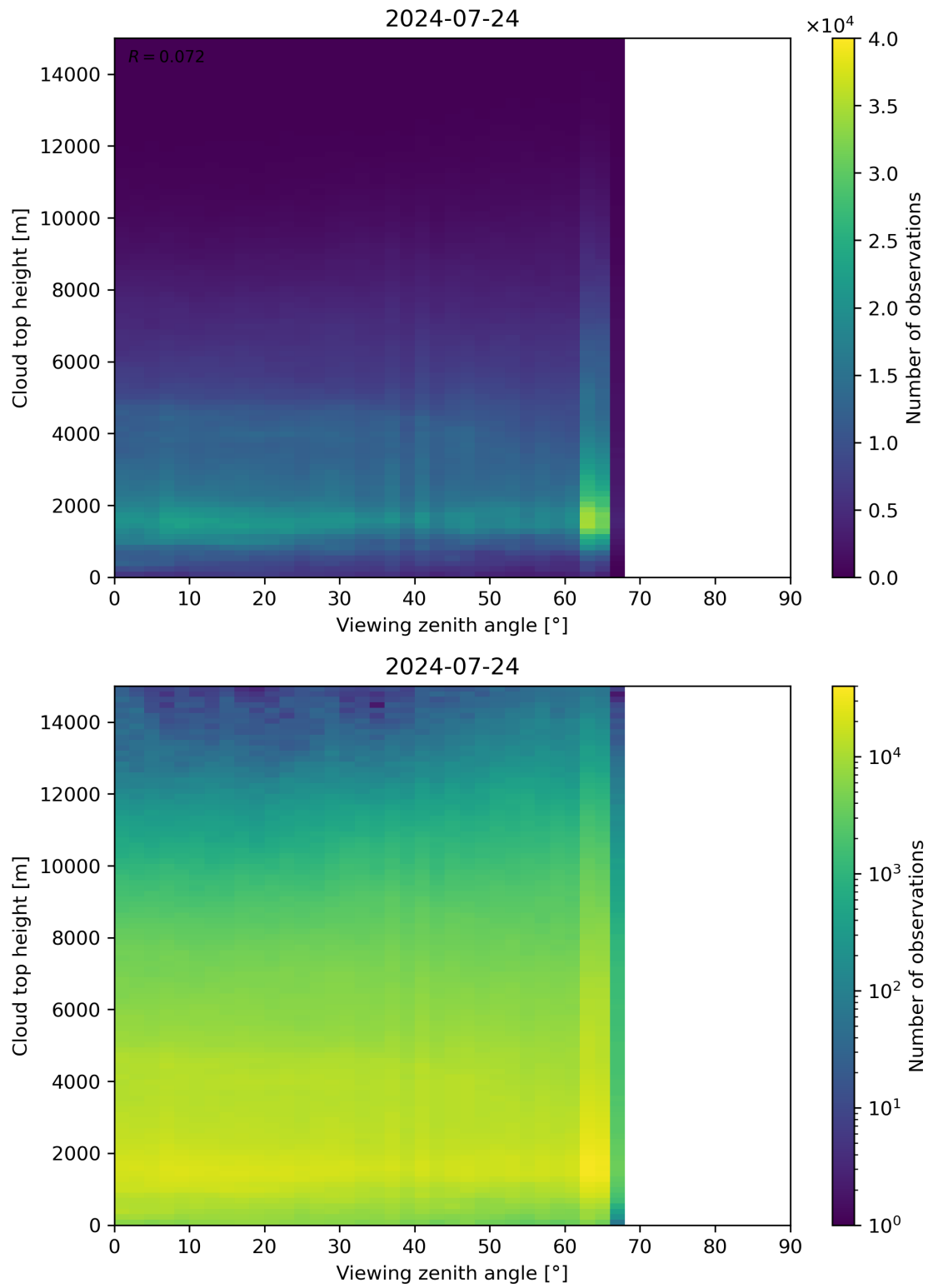
Figure 112: Scatter density plot of “Viewing zenith angle” against “Cloud top height” for 2024-07-23 to 2024-07-25.
