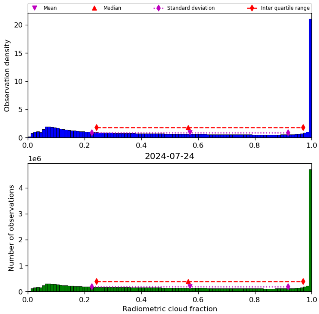
Figure 39: Histogram of “Radiometric cloud fraction” for 2024-07-23 to 2024-07-25
