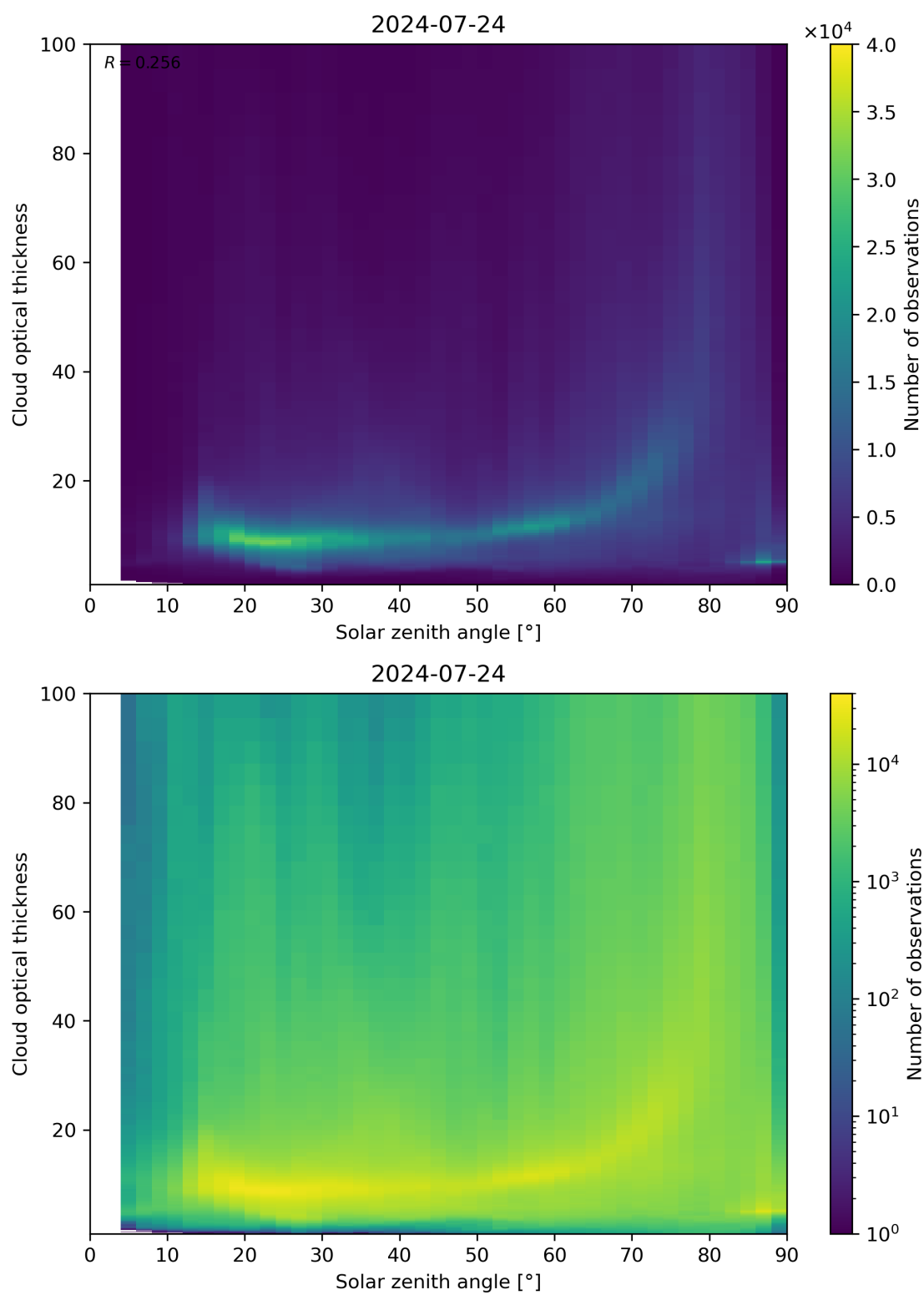
Figure 103: Scatter density plot of “Solar zenith angle” against “Cloud optical thickness” for 2024-07-23 to 2024-07-25.
