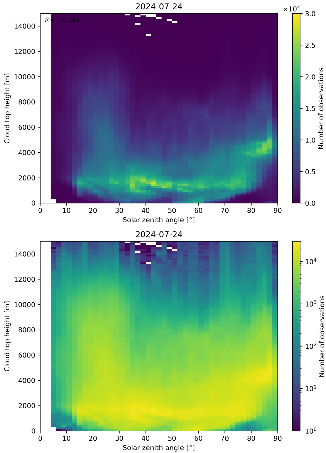
Figure 104: Scatter density plot of “Solar zenith angle” against “Cloud top height” for 2024-07-23 to 2024-07-25.
