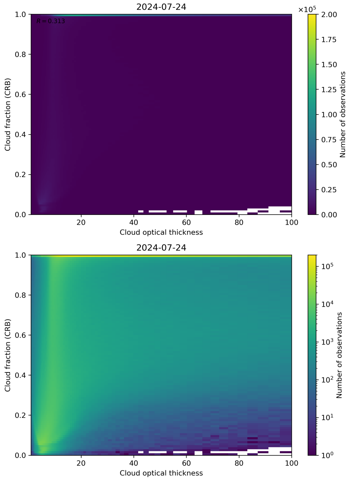
Figure 84: Scatter density plot of “Cloud optical thickness” against “Cloud fraction (CRB)” for 2024-07-23 to 2024-07-25.
