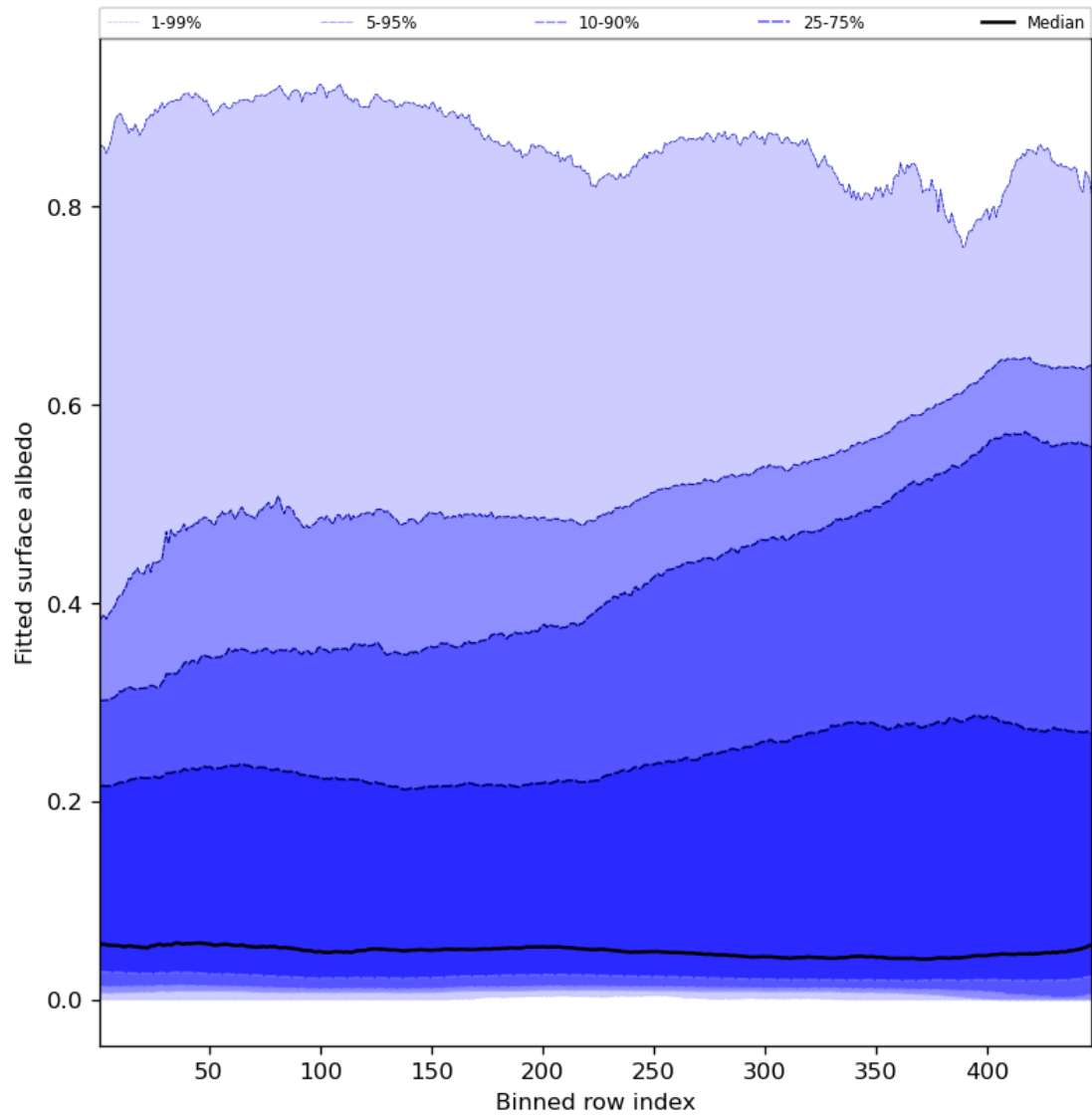
Figure 61: Along track statistics of “Fitted surface albedo” for 2024-07-23 to 2024-07-25
