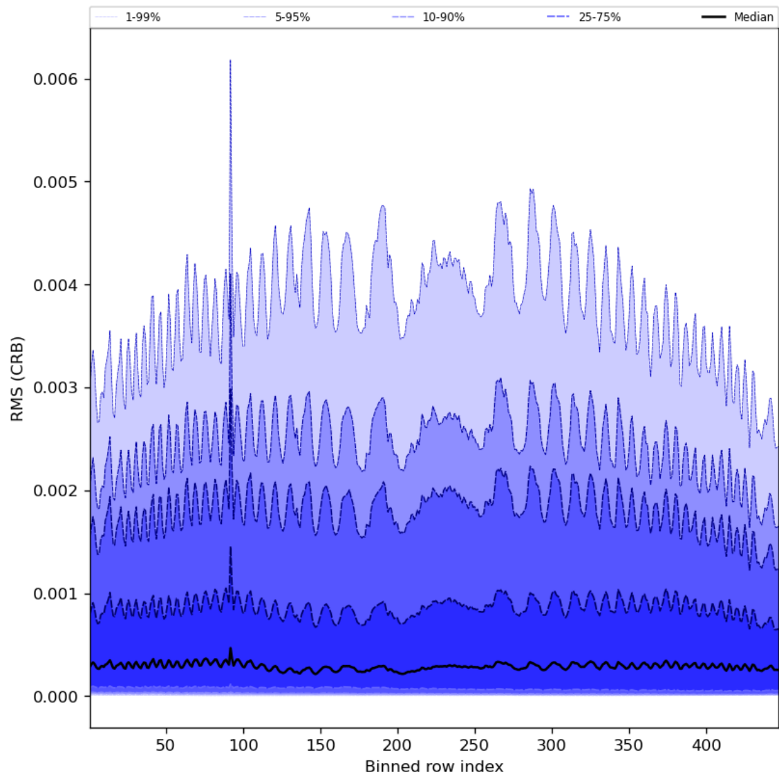
Figure 64: Along track statistics of “RMS (CRB)” for 2024-07-23 to 2024-07-25
