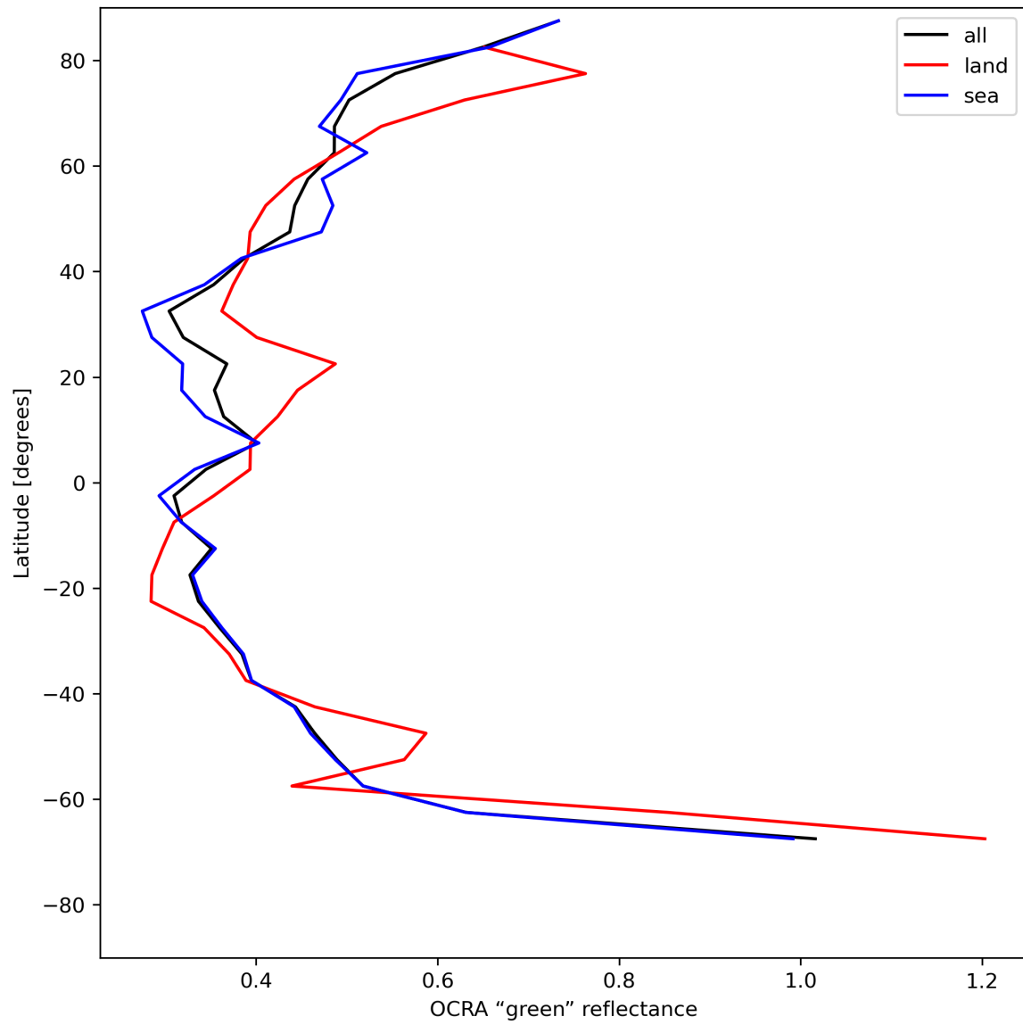
Figure 36: Zonal average of “OCRA “green” reflectance” for 2024-07-23 to 2024-07-25.
