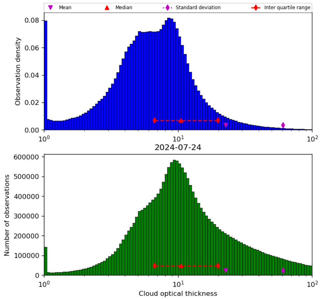
Figure 41: Histogram of “Cloud optical thickness” for 2024-07-23 to 2024-07-25
