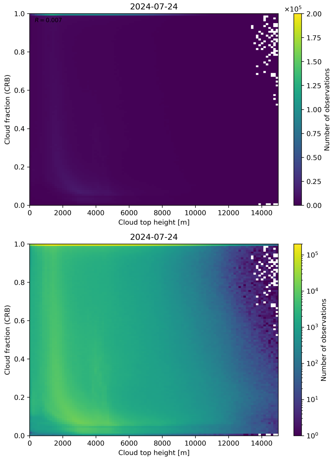
Figure 88: Scatter density plot of “Cloud top height” against “Cloud fraction (CRB)” for 2024-07-23 to 2024-07-25.
