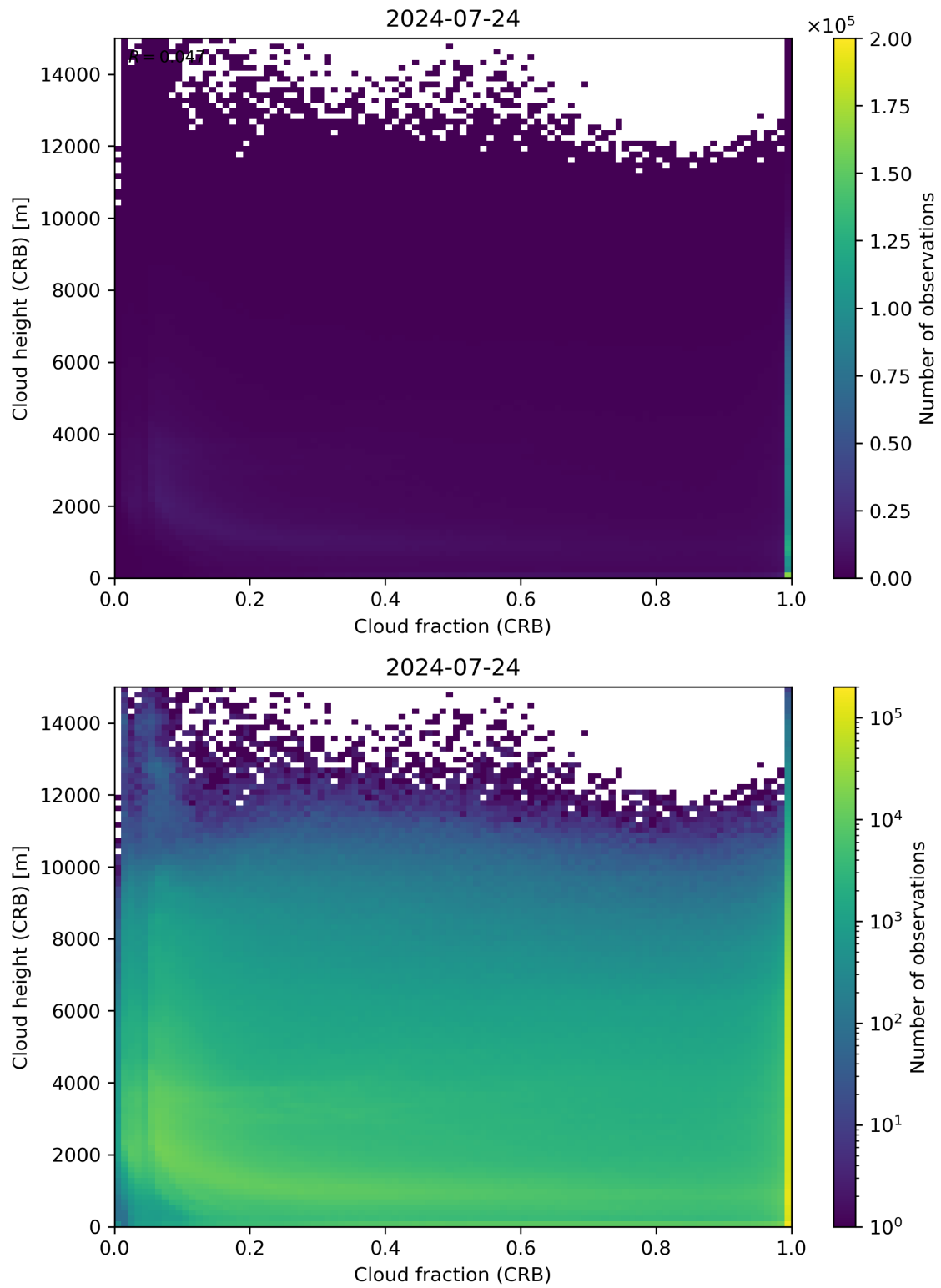
Figure 79: Scatter density plot of “Cloud fraction (CRB)” against “Cloud height (CRB)” for 2024-07-23 to 2024-07-25.
