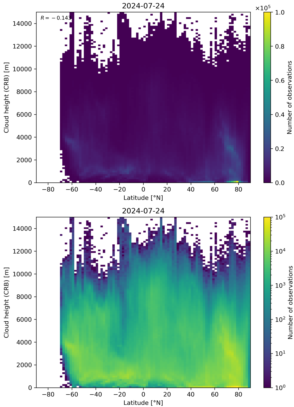
Figure 95: Scatter density plot of “Latitude” against “Cloud height (CRB)” for 2024-07-23 to 2024-07-25.
