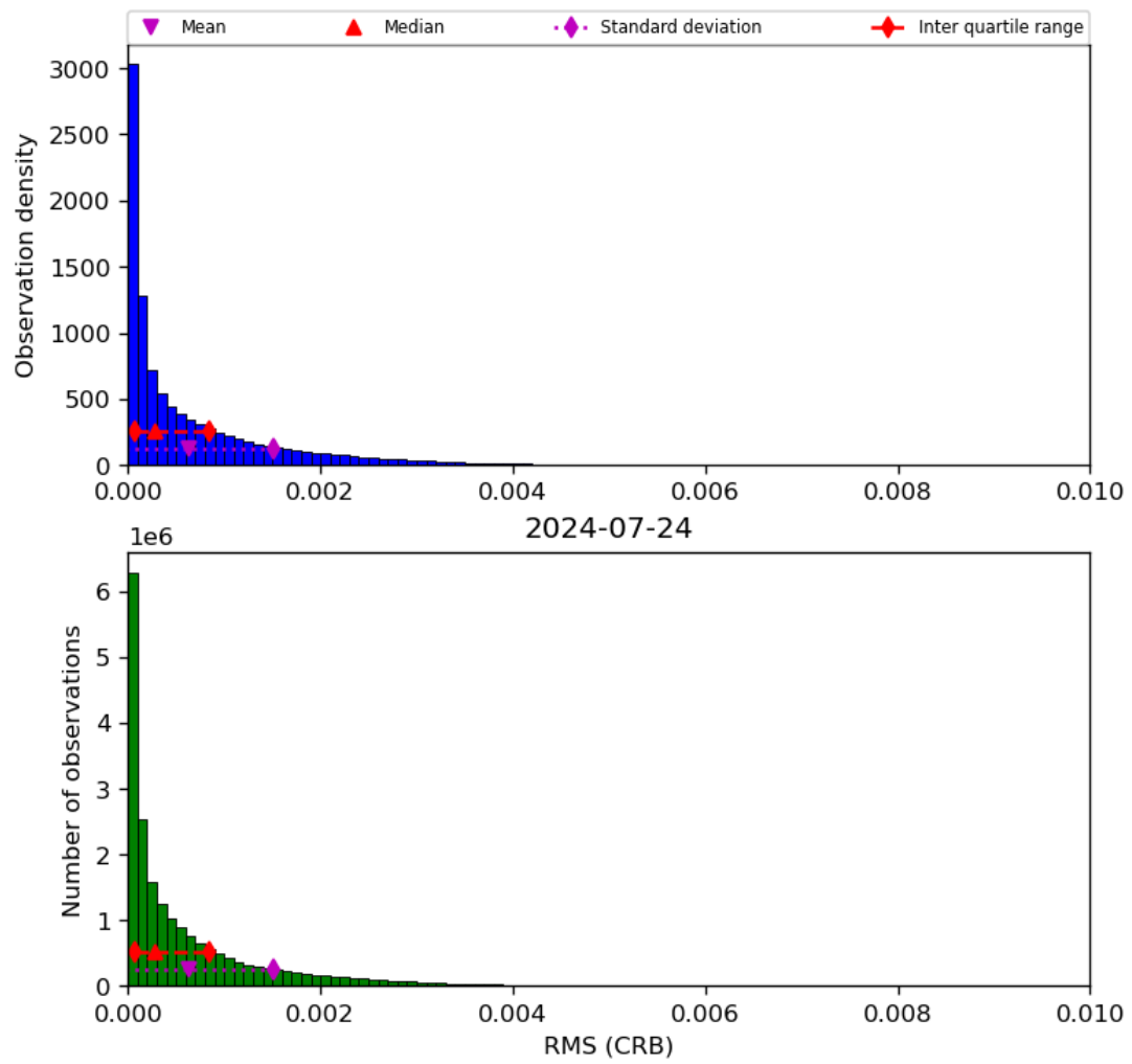
Figure 48: Histogram of “RMS (CRB)” for 2024-07-23 to 2024-07-25
