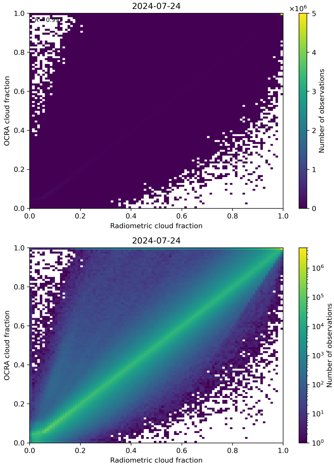
Figure 72: Scatter density plot of “Radiometric cloud fraction” against “OCRA cloud fraction” for 2024-07-23 to 2024-07-25.
