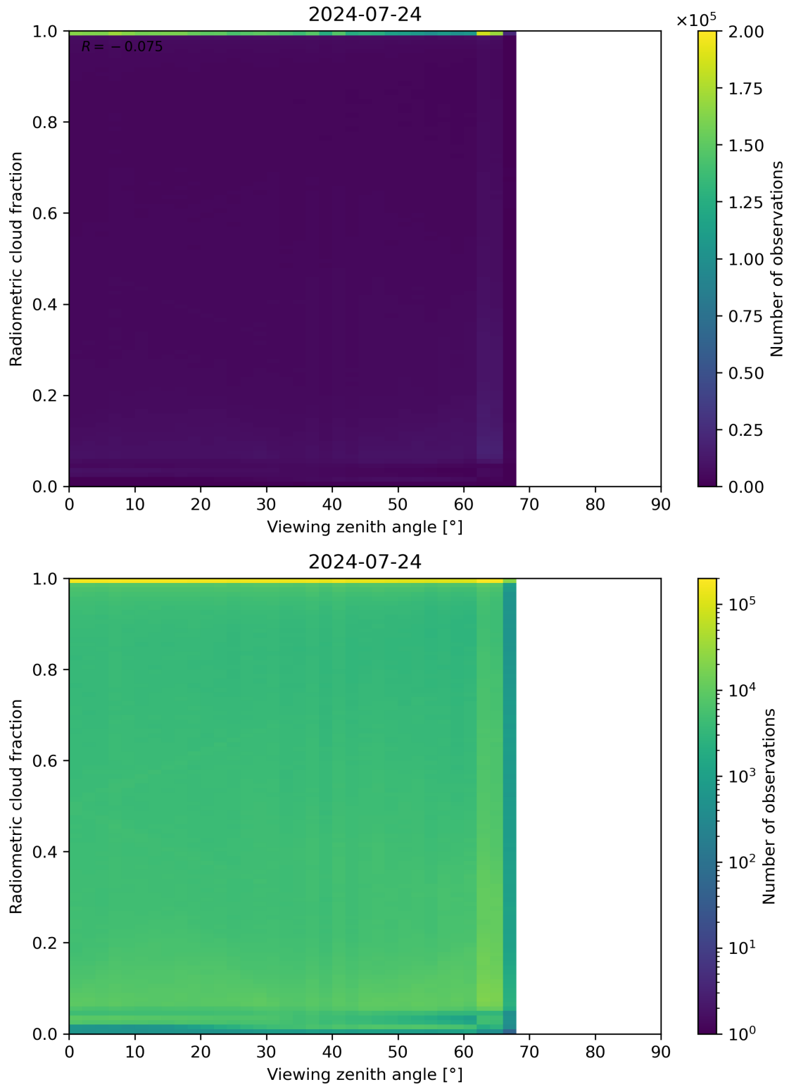
Figure 107: Scatter density plot of “Viewing zenith angle” against “Radiometric cloud fraction” for 2024-07-23 to 2024-07-25.
