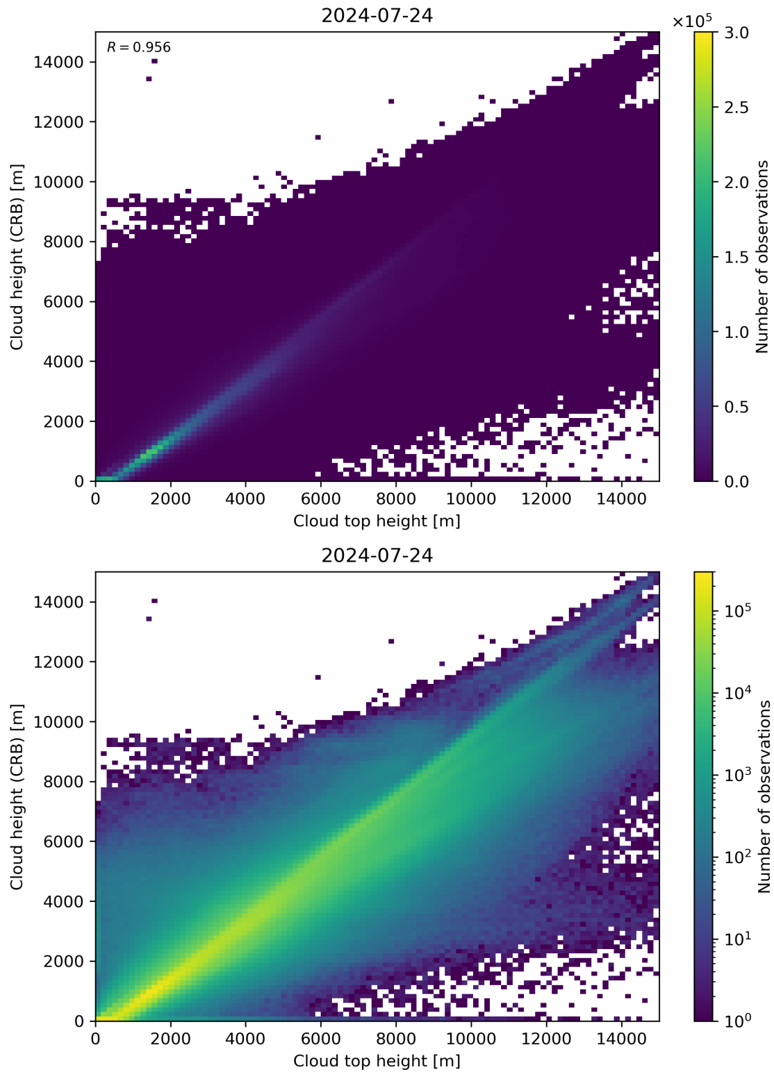
Figure 89: Scatter density plot of “Cloud top height” against “Cloud height (CRB)” for 2024-07-23 to 2024-07-25.
