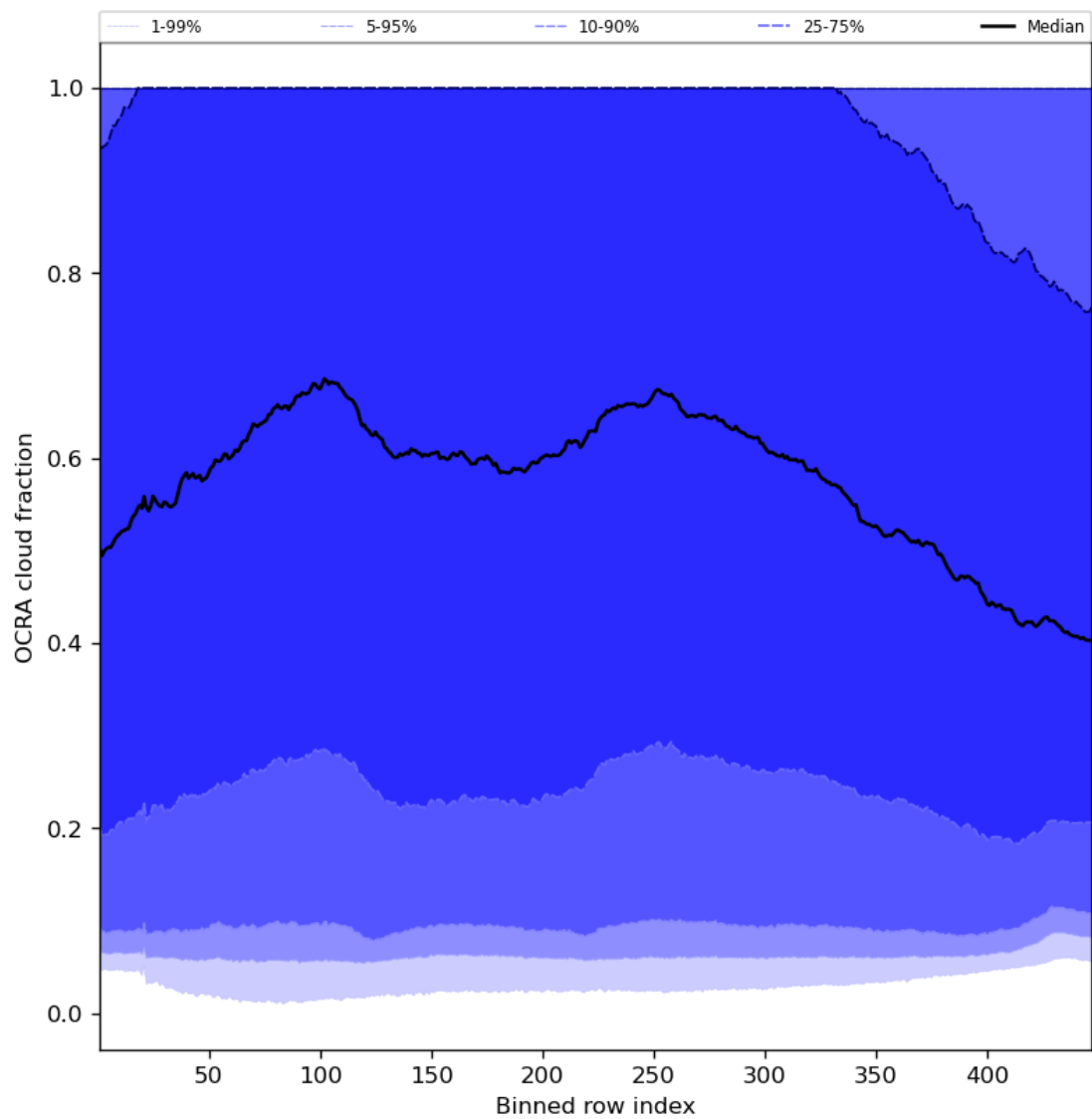
Figure 66: Along track statistics of “OCRA cloud fraction” for 2024-07-23 to 2024-07-25
