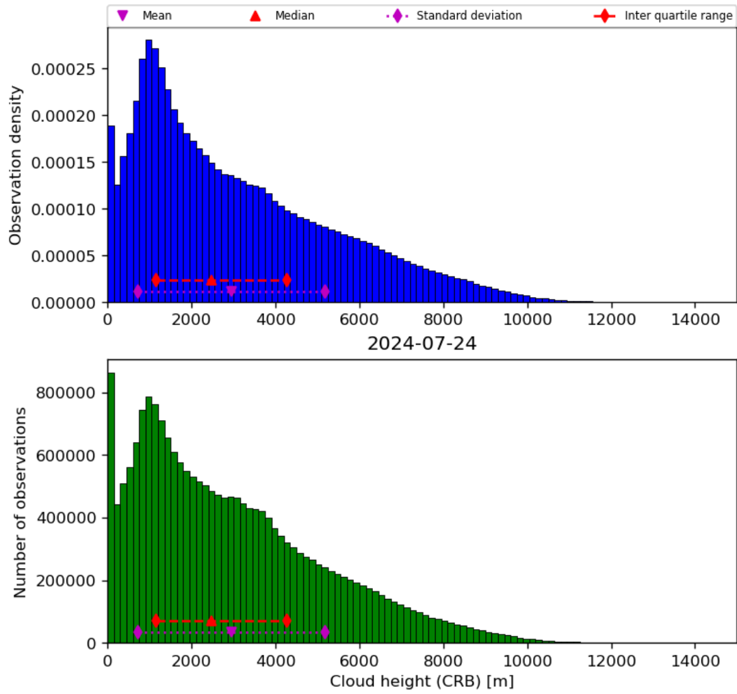
Figure 43: Histogram of “Cloud height (CRB)” for 2024-07-23 to 2024-07-25
