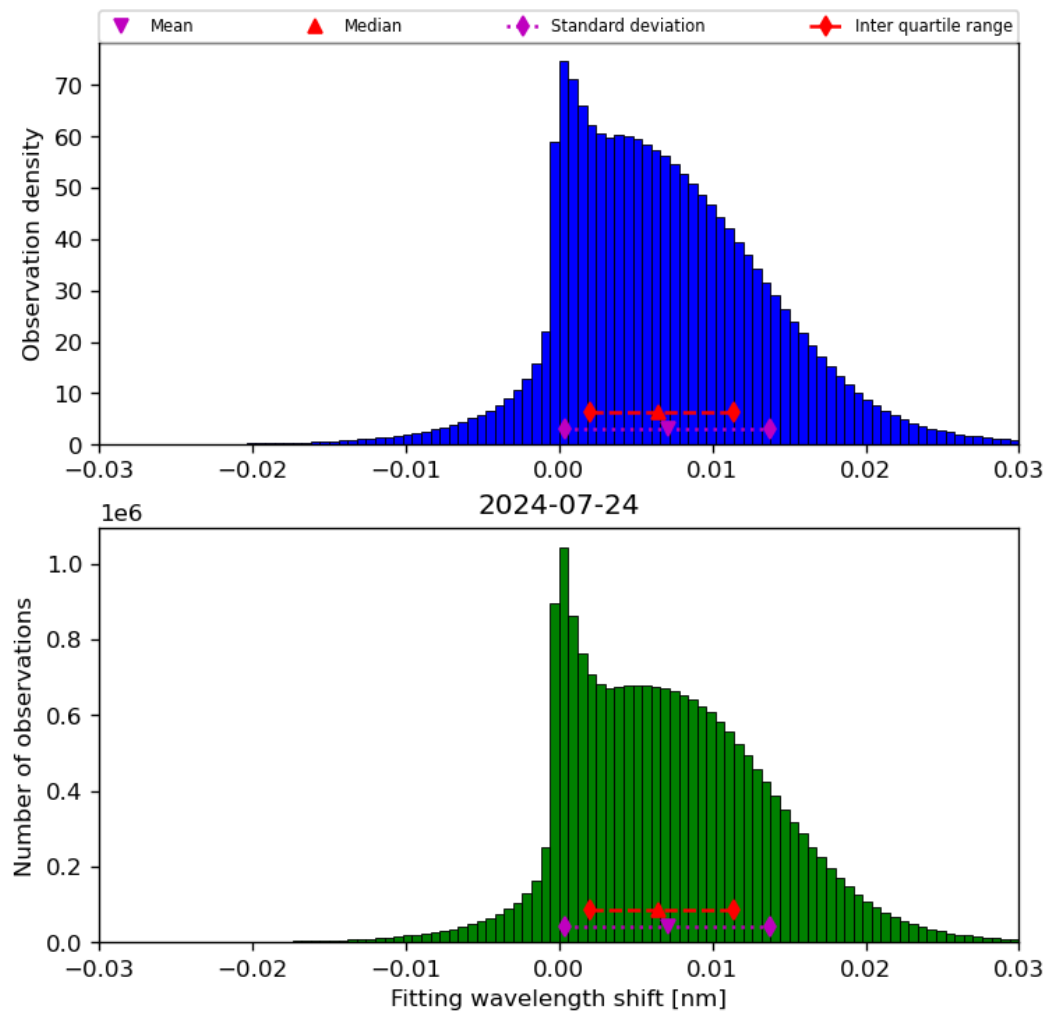
Figure 49: Histogram of “Fitting wavelength shift” for 2024-07-23 to 2024-07-25
