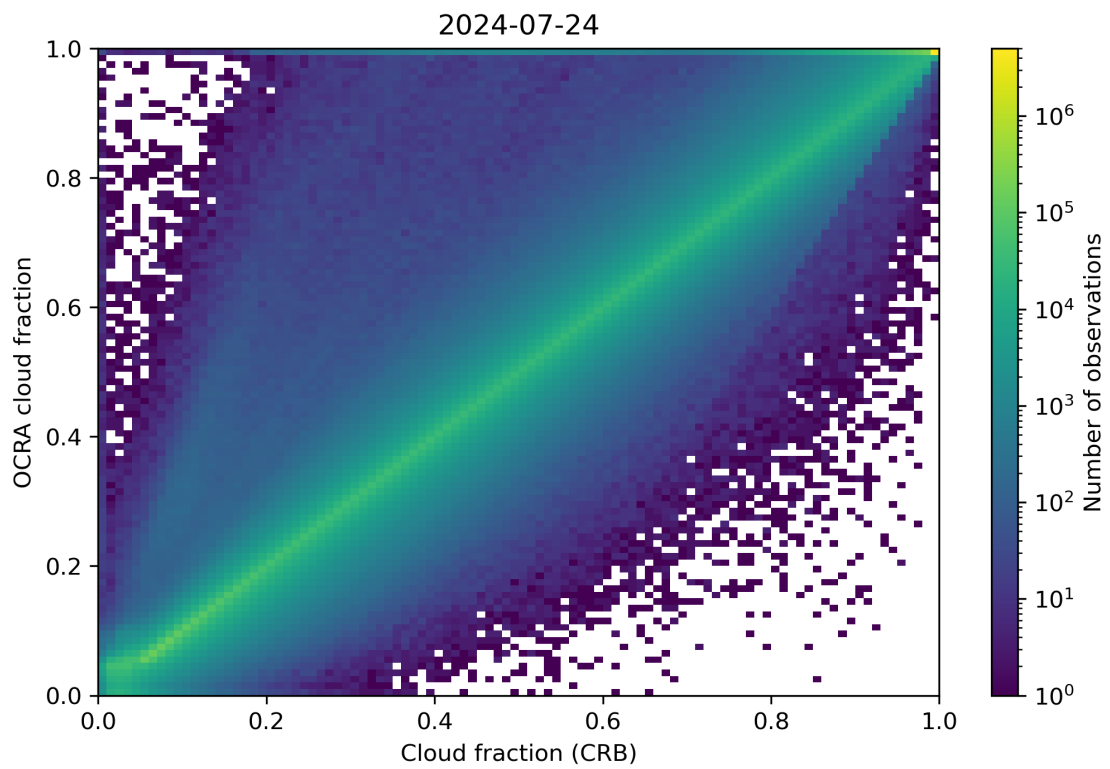
Figure 78: Scatter density plot of “Cloud fraction (CRB)” against “OCRA cloud fraction” for 2024-07-23 to 2024-07-25.
