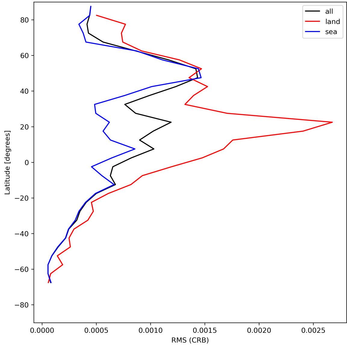
Figure 32: Zonal average of “RMS (CRB)” for 2024-07-23 to 2024-07-25.
