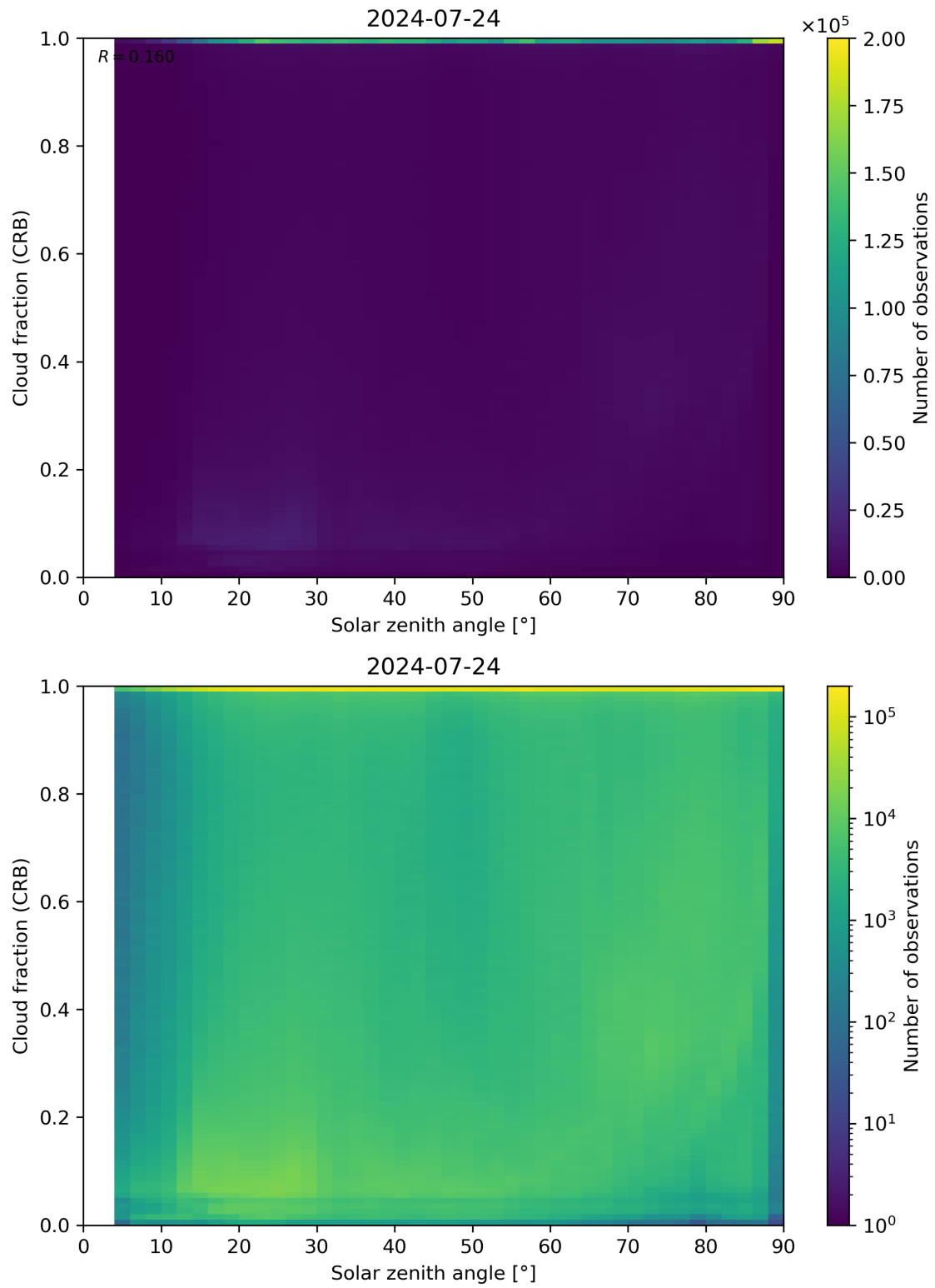
Figure 101: Scatter density plot of “Solar zenith angle” against “Cloud fraction (CRB)” for 2024-07-23 to 2024-07-25.
