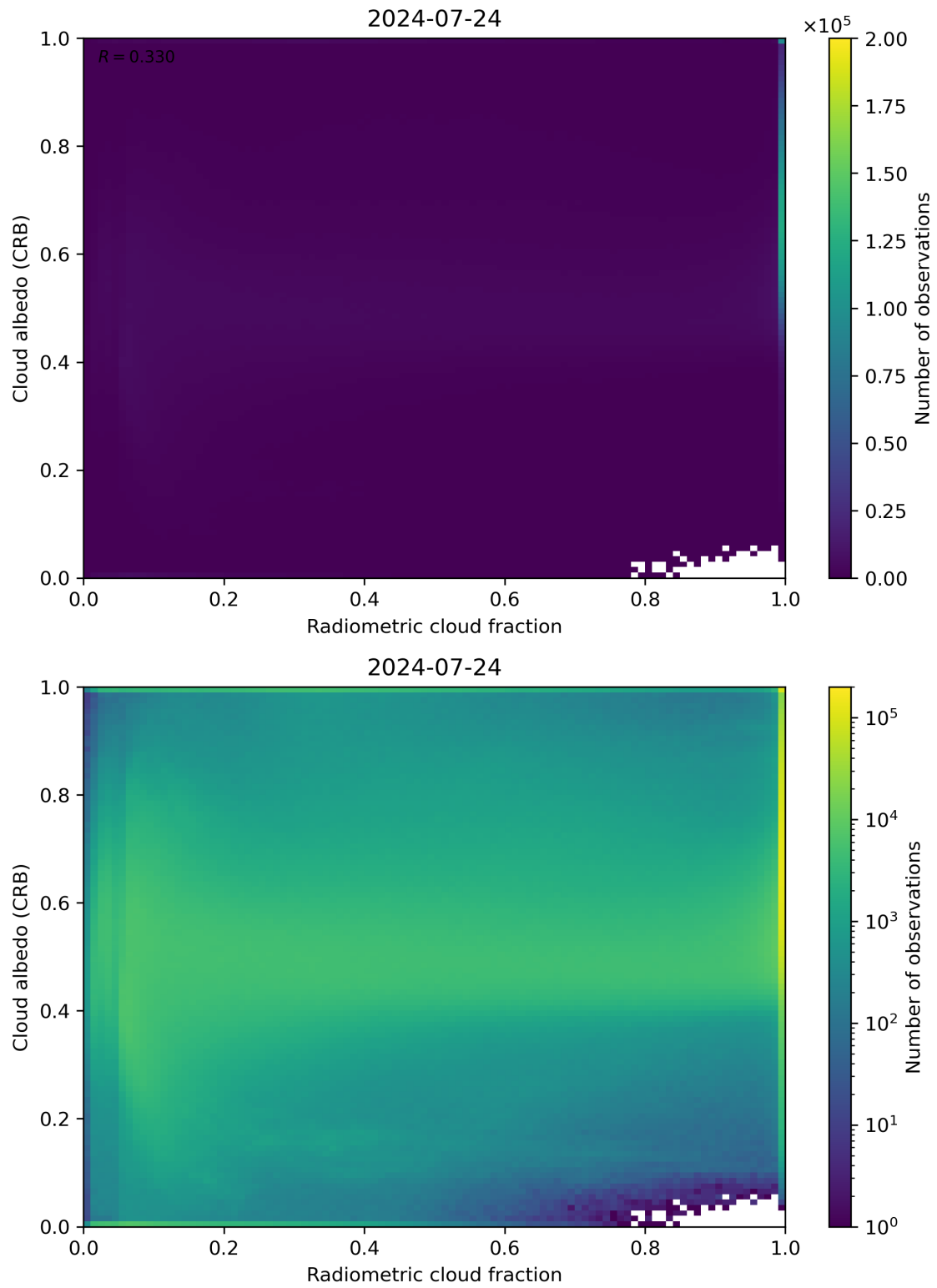
Figure 71: Scatter density plot of “Radiometric cloud fraction” against “Cloud albedo (CRB)” for 2024-07-23 to 2024-07-25.
