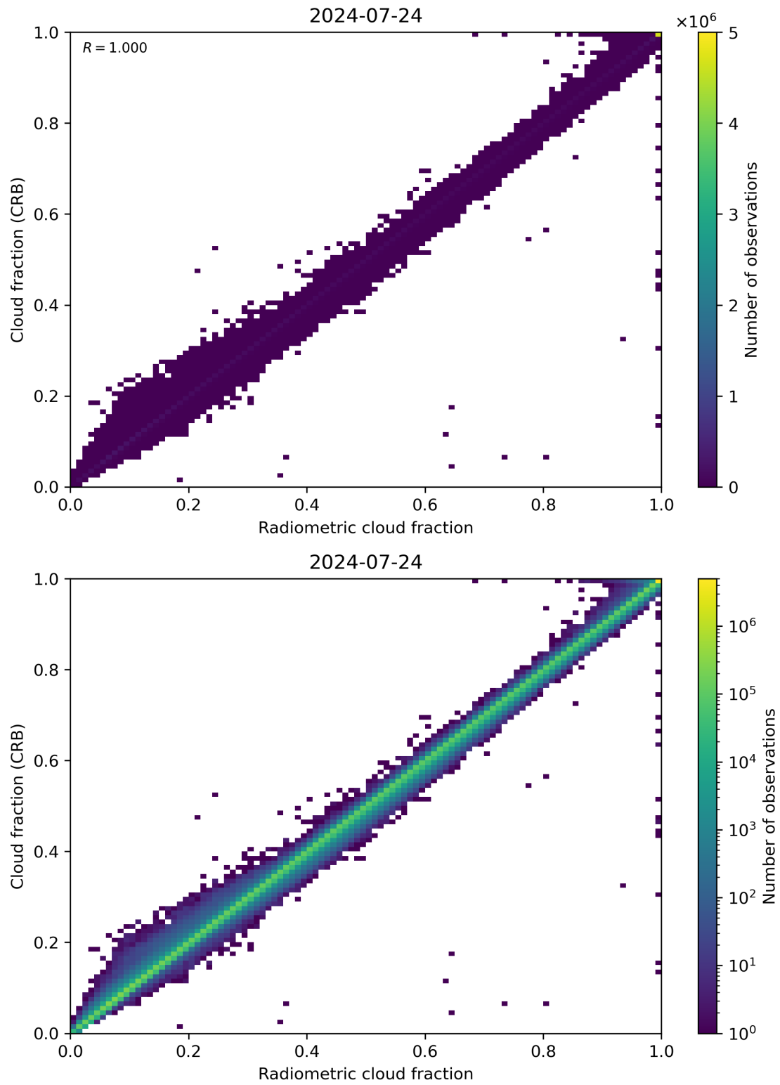
Figure 73: Scatter density plot of “Radiometric cloud fraction” against “Cloud fraction (CRB)” for 2024-07-23 to 2024-07-25.
