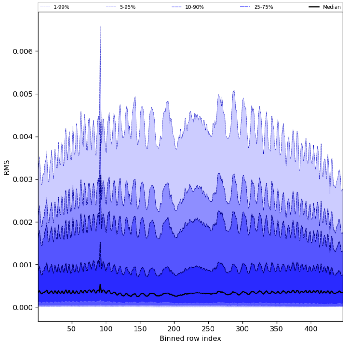
Figure 63: Along track statistics of “RMS” for 2024-07-23 to 2024-07-25
