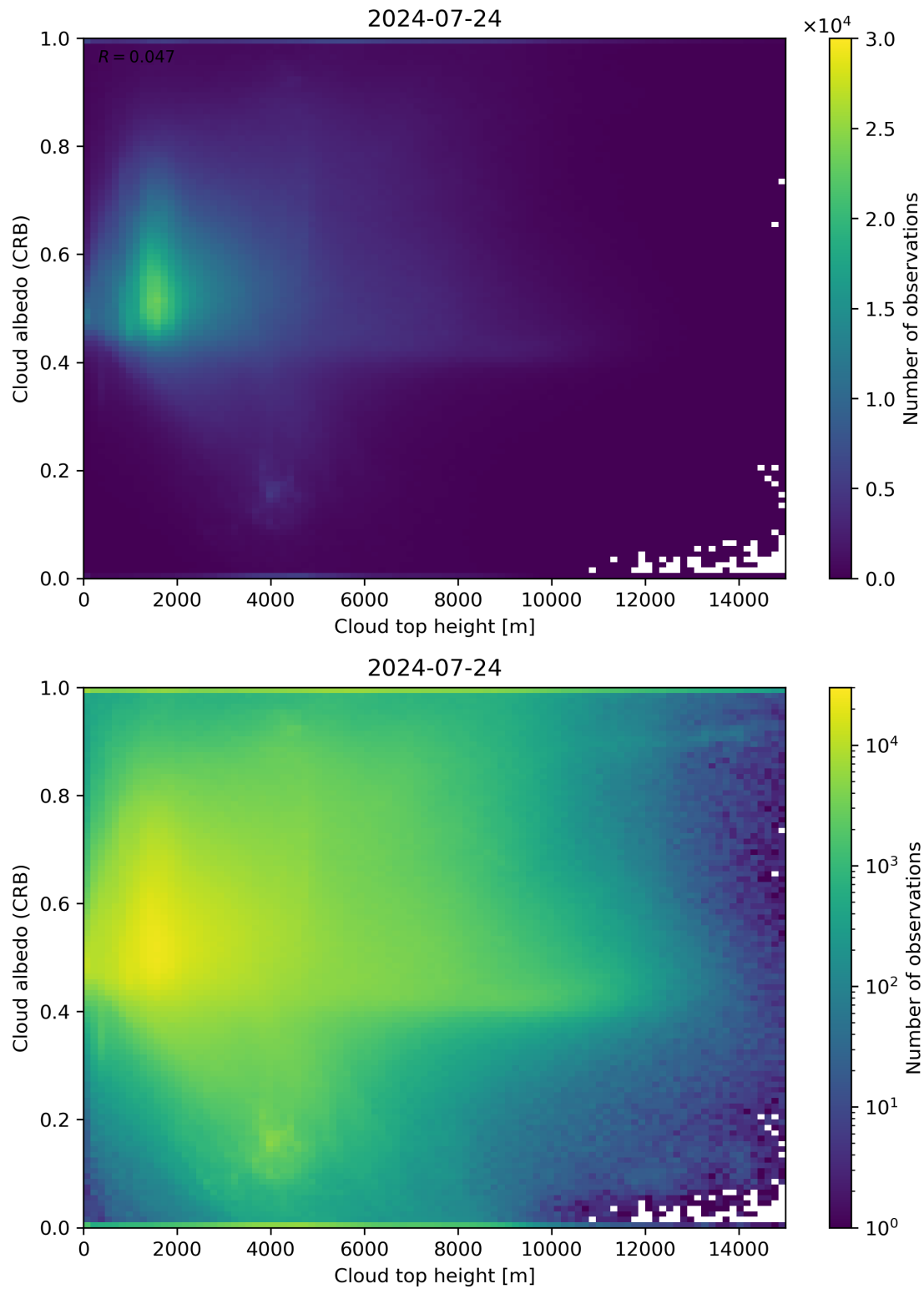
Figure 86: Scatter density plot of “Cloud top height” against “Cloud albedo (CRB)” for 2024-07-23 to 2024-07-25.
