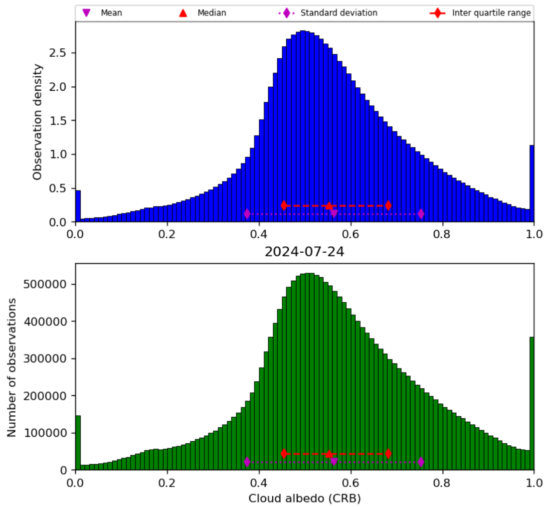
Figure 44: Histogram of “Cloud albedo (CRB)” for 2024-07-23 to 2024-07-25
