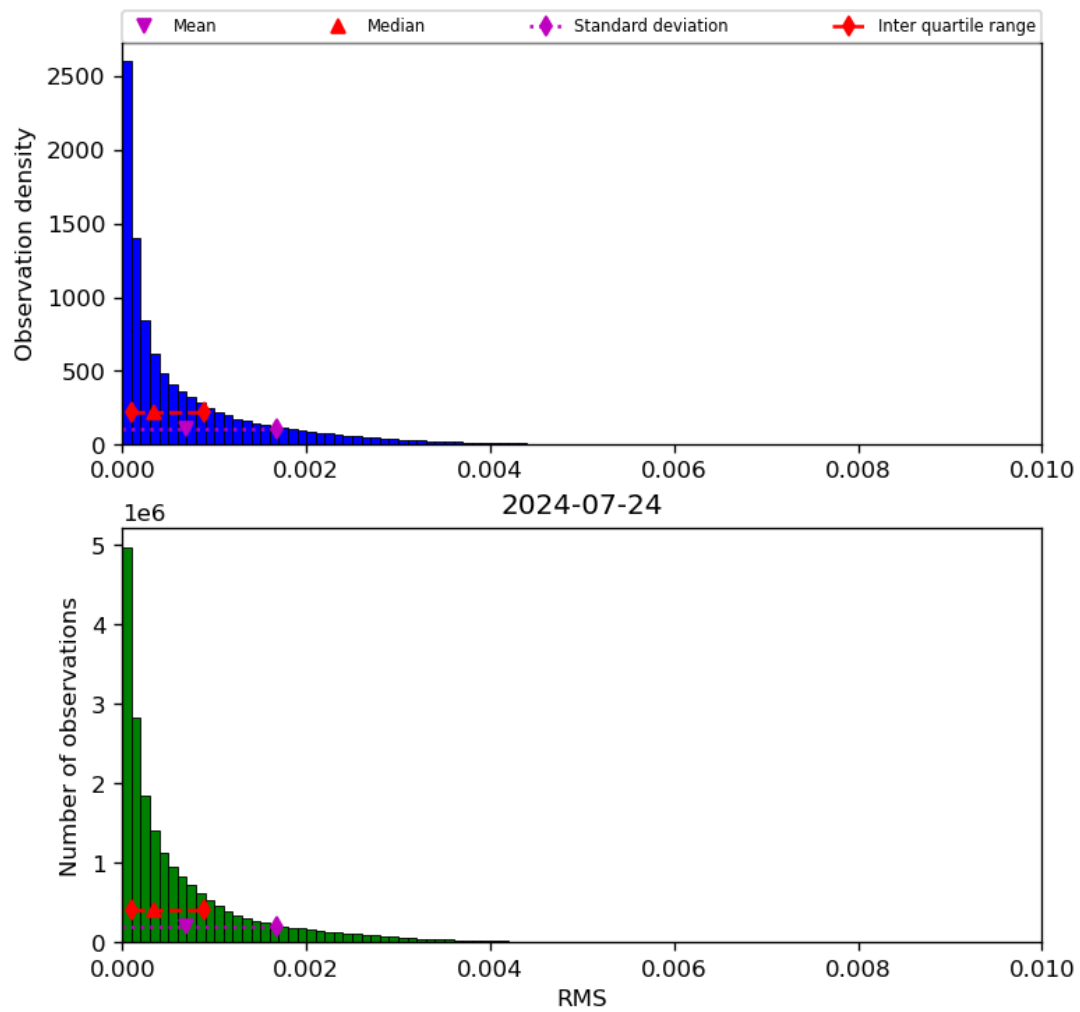
Figure 47: Histogram of “RMS” for 2024-07-23 to 2024-07-25
