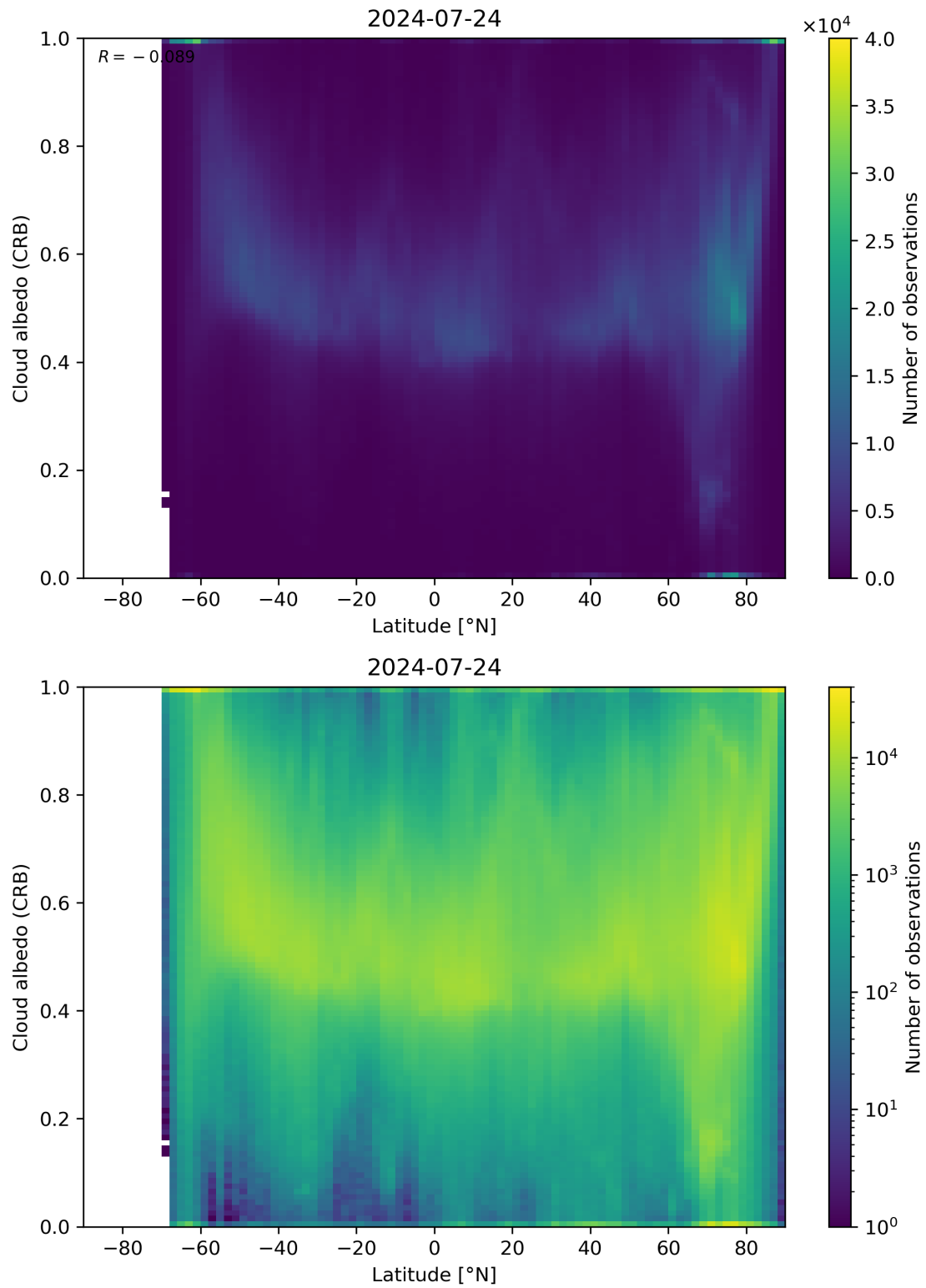
Figure 91: Scatter density plot of “Latitude” against “Cloud albedo (CRB)” for 2024-07-23 to 2024-07-25.
