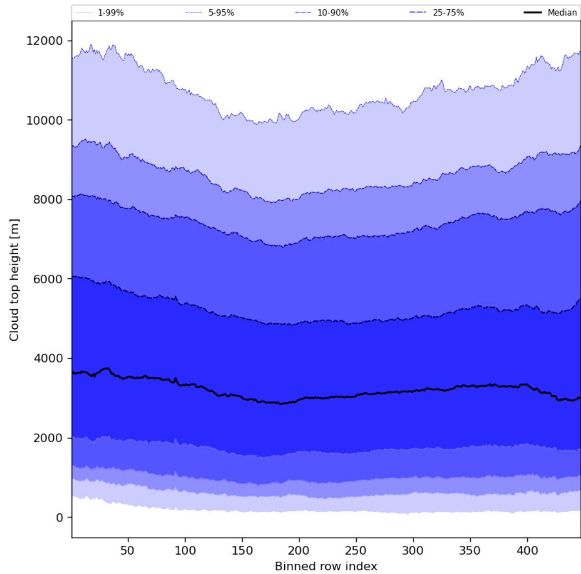
Figure 56: Along track statistics of “Cloud top height” for 2024-07-23 to 2024-07-25
