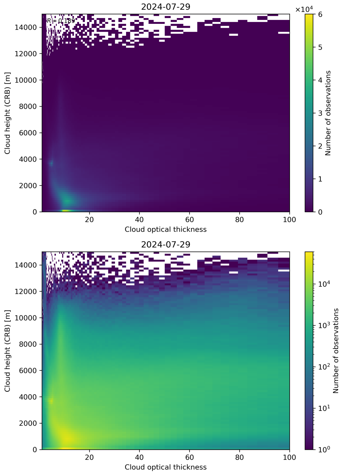
Figure 85: Scatter density plot of “Cloud optical thickness” against “Cloud height (CRB)” for 2024-07-28 to 2024-07-30.
