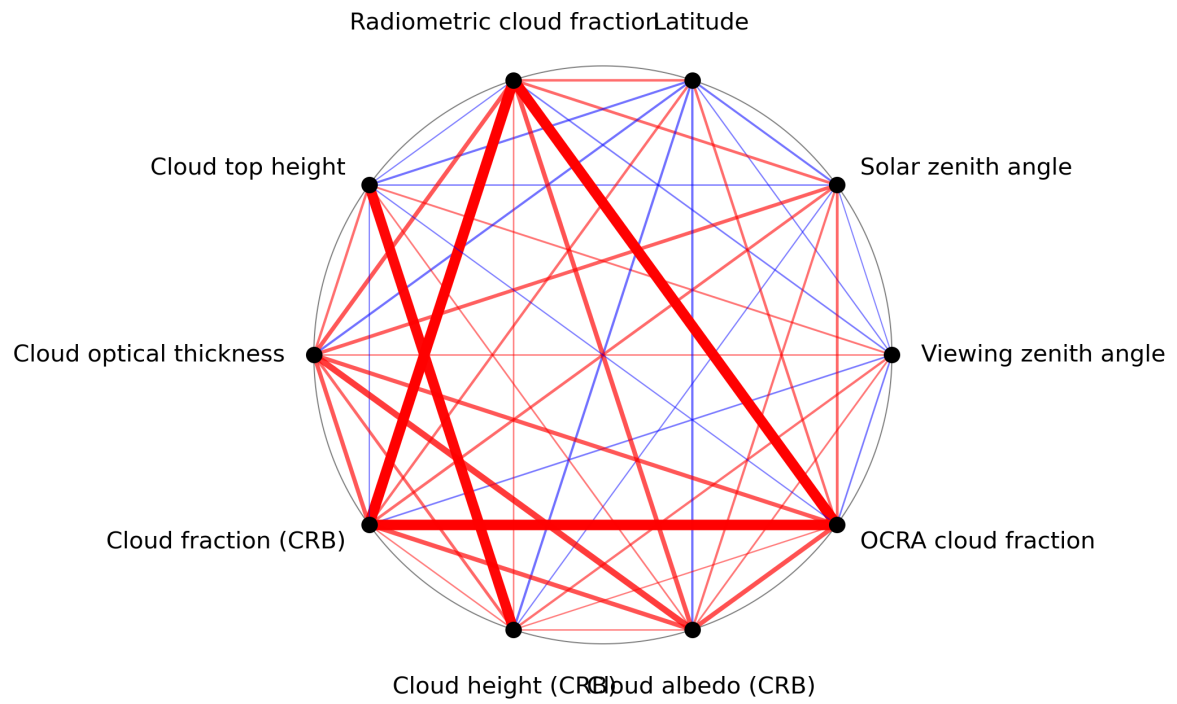
Figure 1: Map of correlation graph for 2024-07-28 to 2024-07-30.
