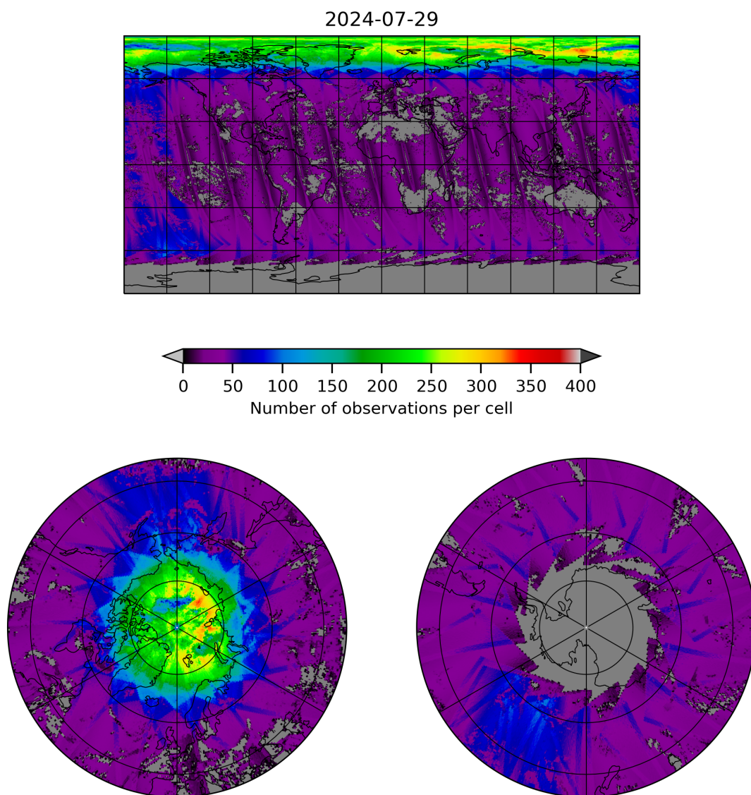
Figure 21: Map of the number of observations for 2024-07-28 to 2024-07-30
