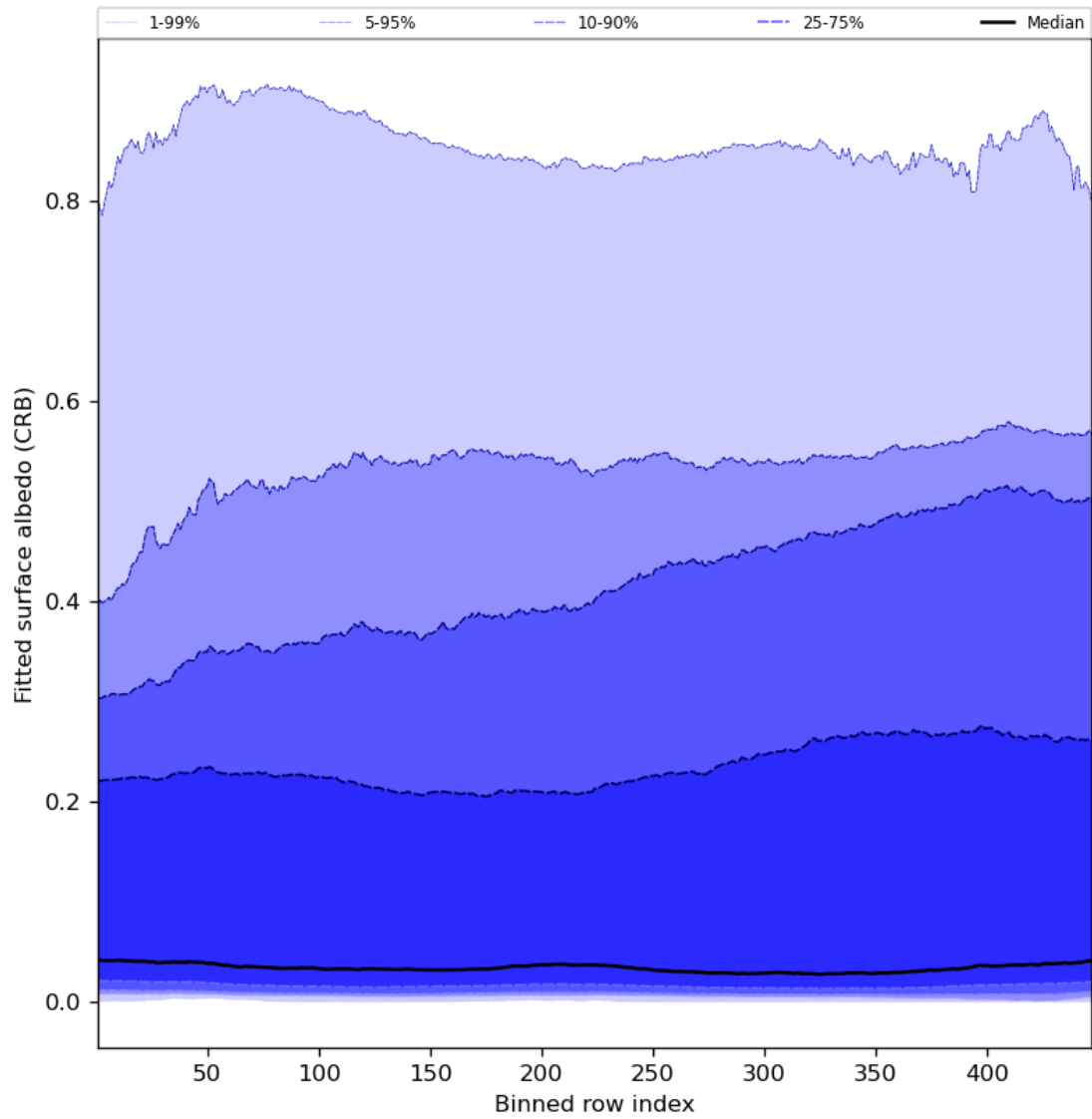
Figure 62: Along track statistics of “Fitted surface albedo (CRB)” for 2024-07-28 to 2024-07-30
