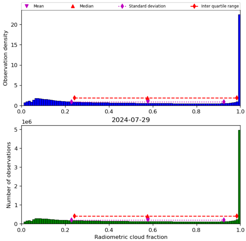
Figure 39: Histogram of “Radiometric cloud fraction” for 2024-07-28 to 2024-07-30
