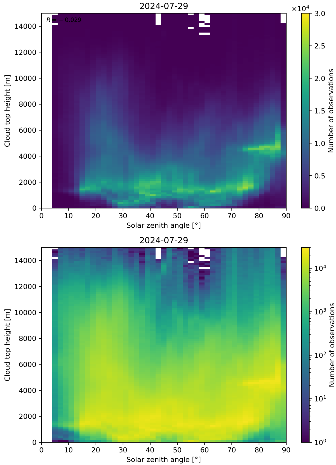
Figure 104: Scatter density plot of “Solar zenith angle” against “Cloud top height” for 2024-07-28 to 2024-07-30.
