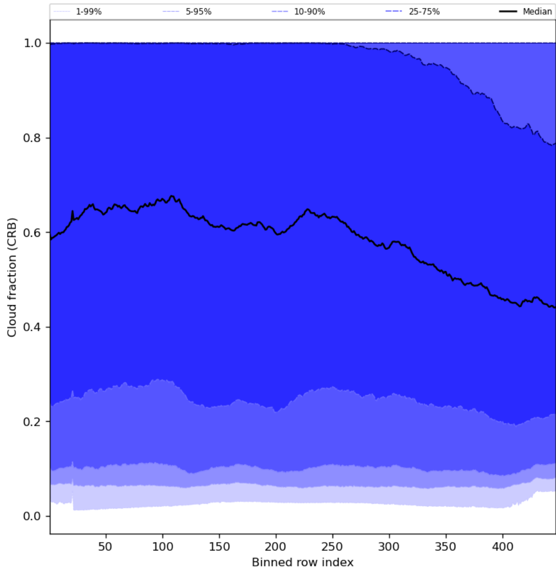
Figure 58: Along track statistics of “Cloud fraction (CRB)” for 2024-07-28 to 2024-07-30
