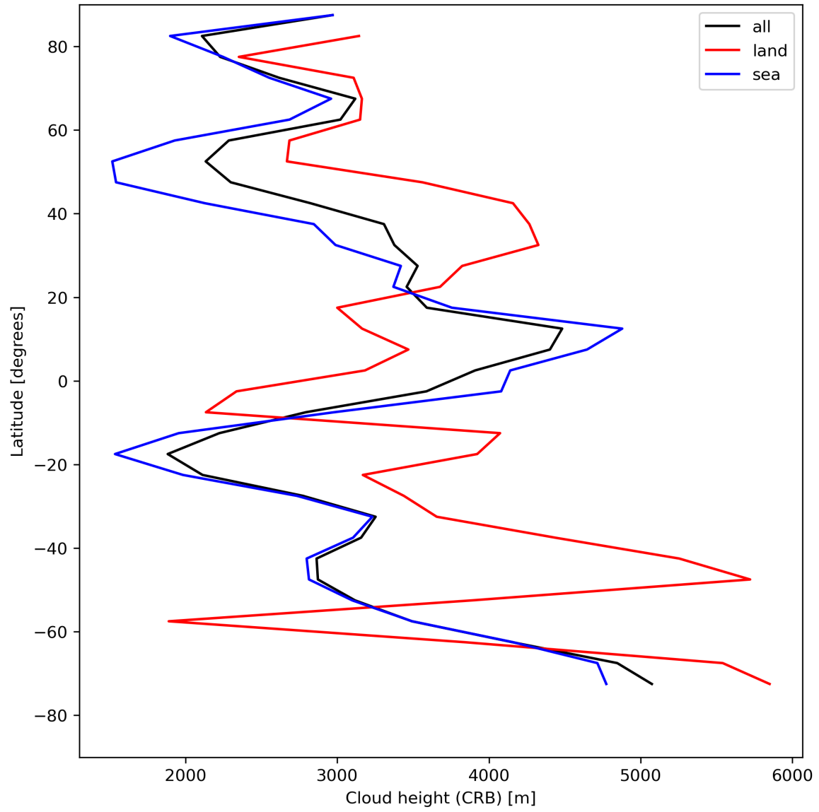
Figure 27: Zonal average of “Cloud height (CRB)” for 2024-07-28 to 2024-07-30.
