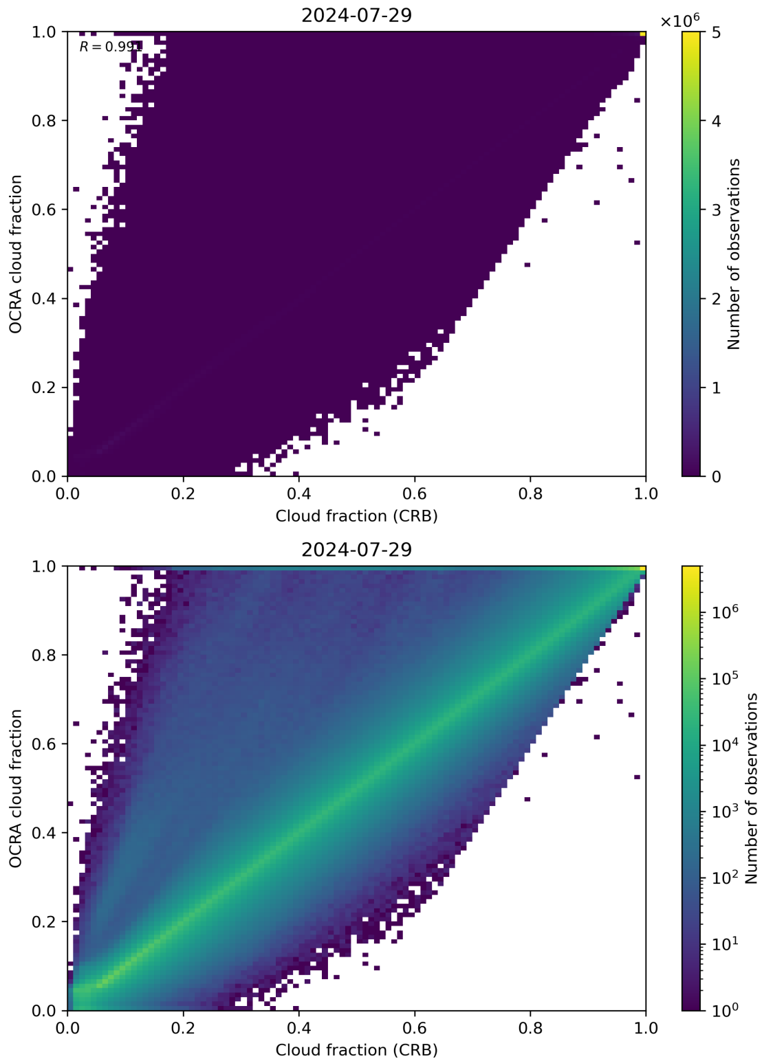
Figure 78: Scatter density plot of “Cloud fraction (CRB)” against “OCRA cloud fraction” for 2024-07-28 to 2024-07-30.
