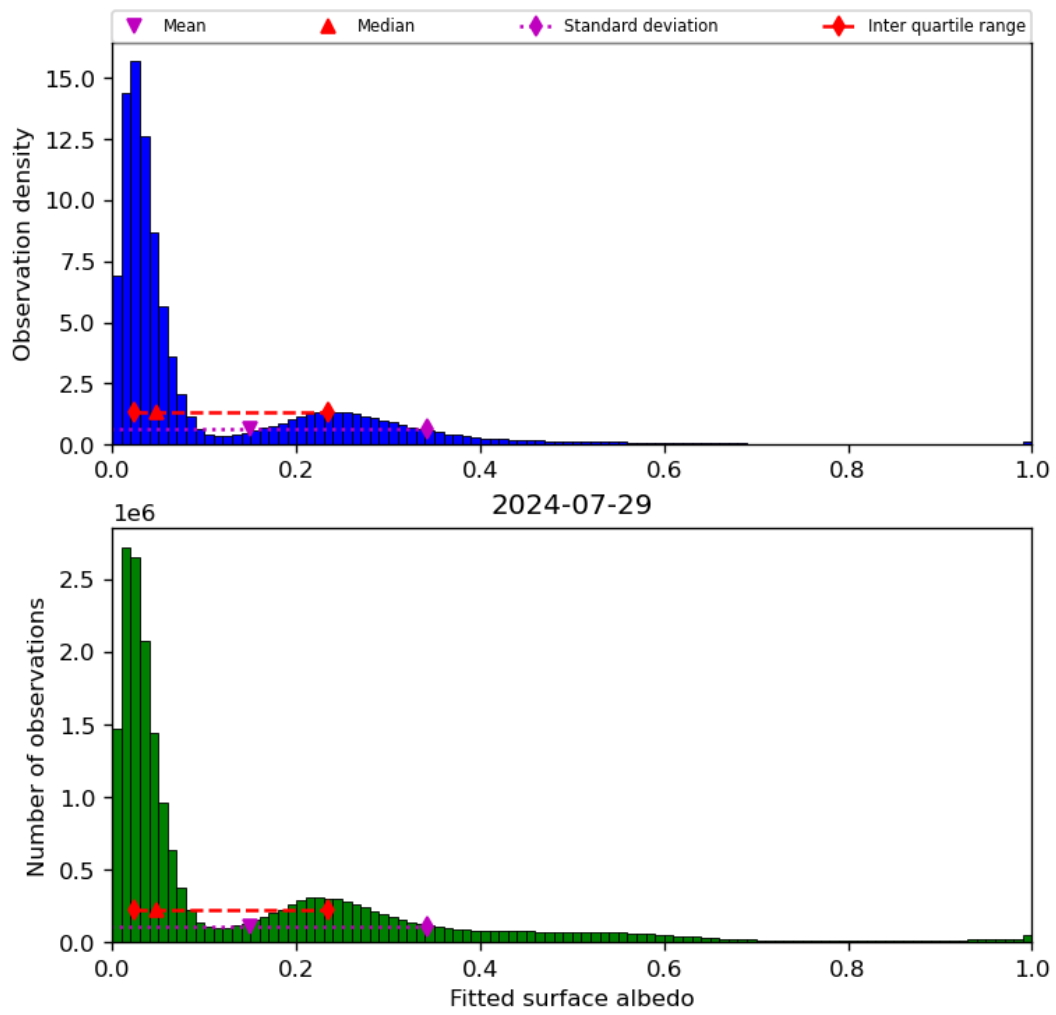
Figure 45: Histogram of “Fitted surface albedo” for 2024-07-28 to 2024-07-30
