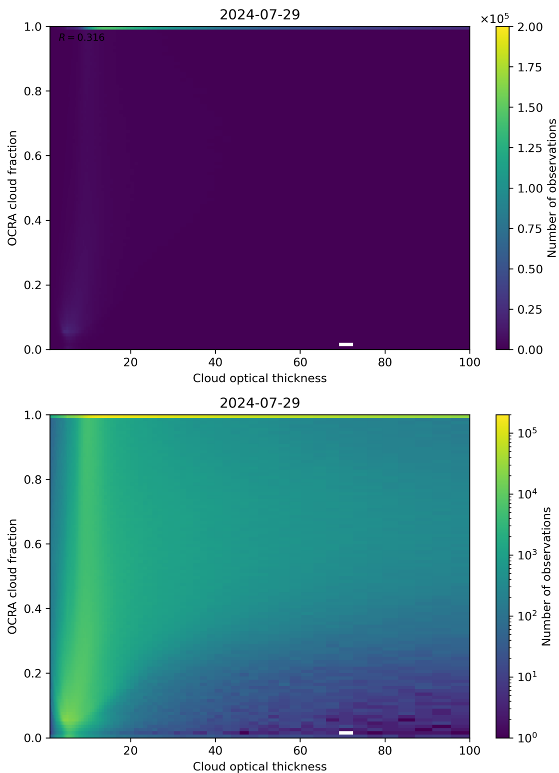
Figure 83: Scatter density plot of “Cloud optical thickness” against “OCRA cloud fraction” for 2024-07-28 to 2024-07-30.
