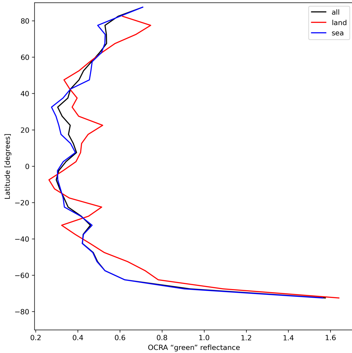
Figure 36: Zonal average of “OCRA “green” reflectance” for 2024-07-28 to 2024-07-30.
