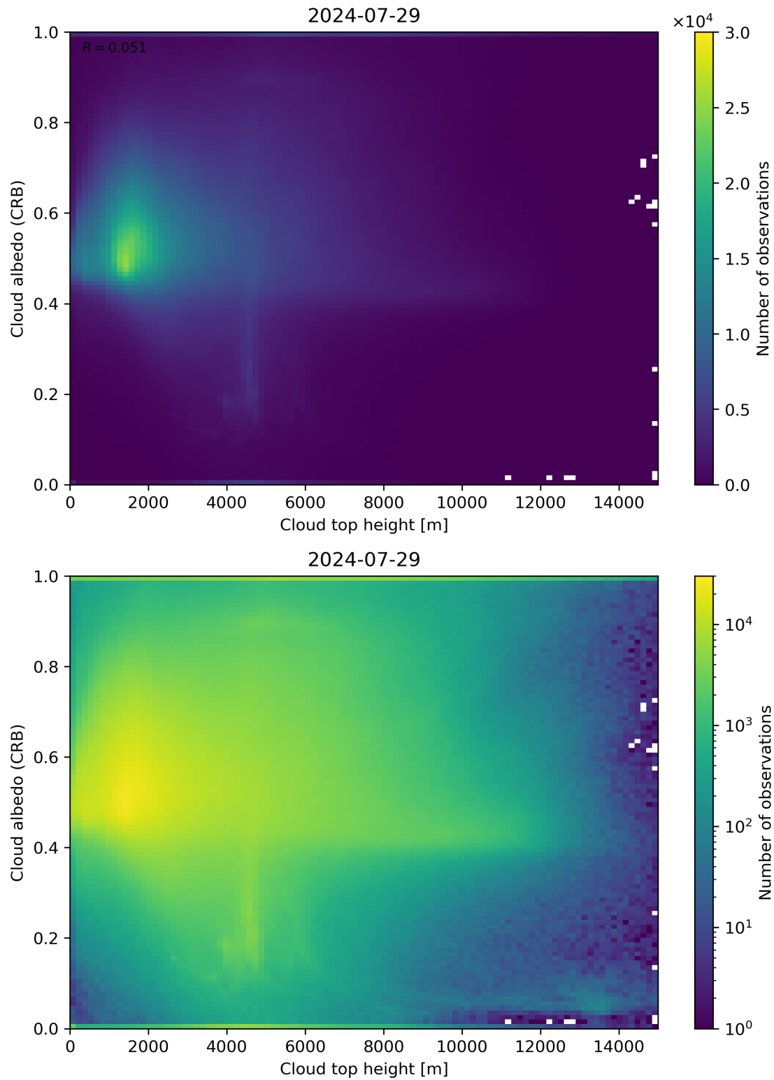
Figure 86: Scatter density plot of “Cloud top height” against “Cloud albedo (CRB)” for 2024-07-28 to 2024-07-30.
