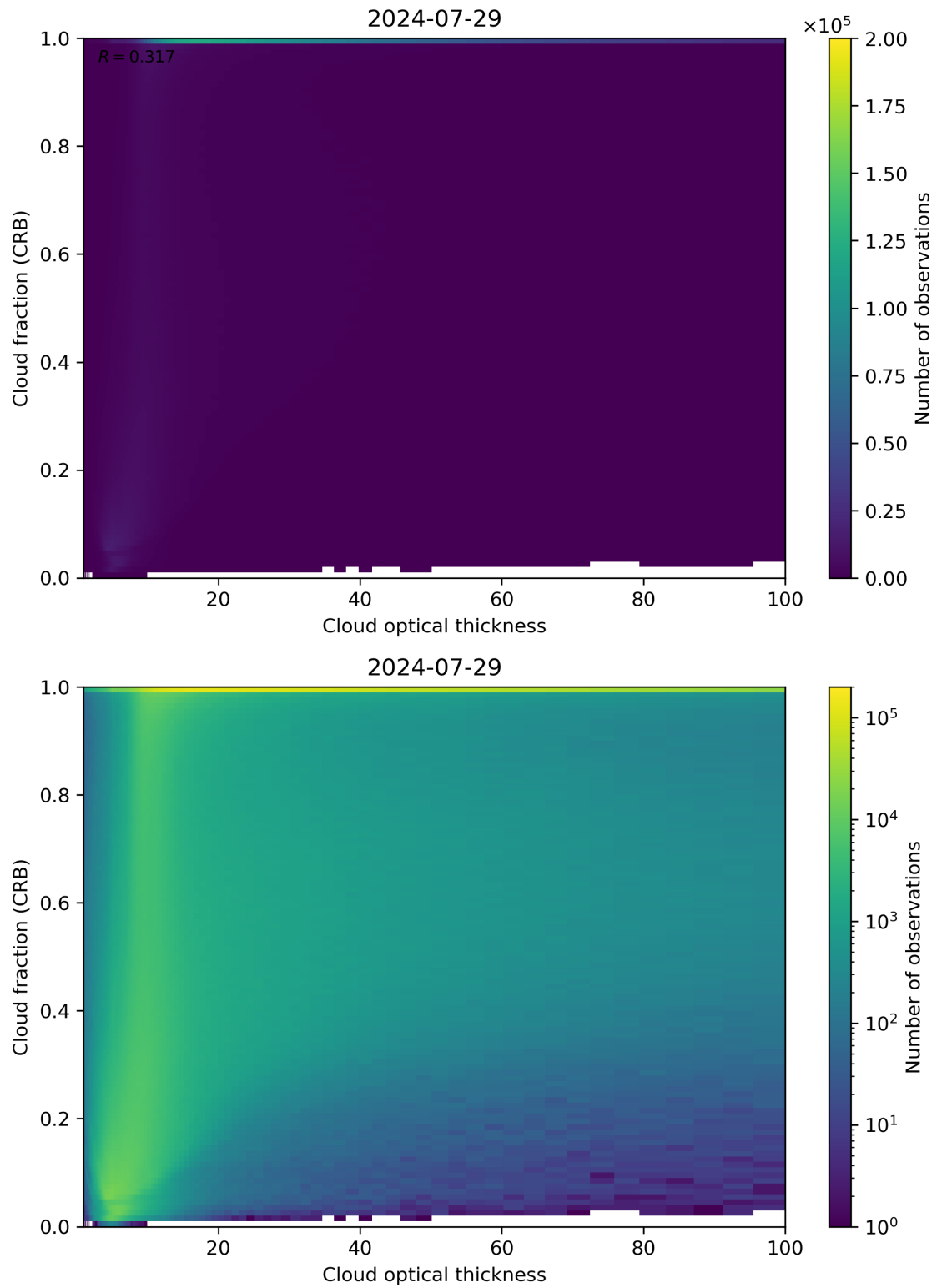
Figure 84: Scatter density plot of “Cloud optical thickness” against “Cloud fraction (CRB)” for 2024-07-28 to 2024-07-30.
