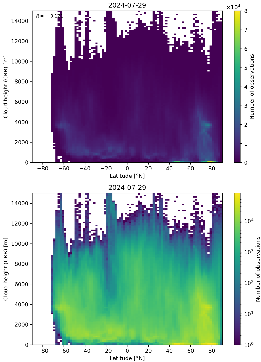
Figure 95: Scatter density plot of “Latitude” against “Cloud height (CRB)” for 2024-07-28 to 2024-07-30.
