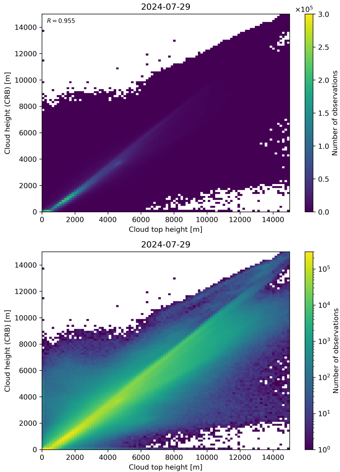
Figure 89: Scatter density plot of “Cloud top height” against “Cloud height (CRB)” for 2024-07-28 to 2024-07-30.
