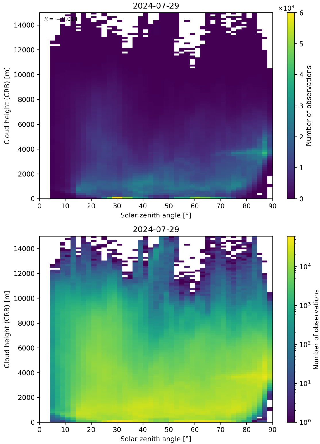
Figure 102: Scatter density plot of “Solar zenith angle” against “Cloud height (CRB)” for 2024-07-28 to 2024-07-30.
