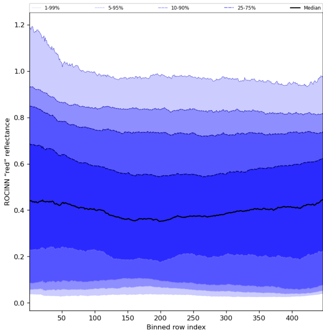
Figure 69: Along track statistics of “ROCINN “red” reflectance” for 2024-07-28 to 2024-07-30
