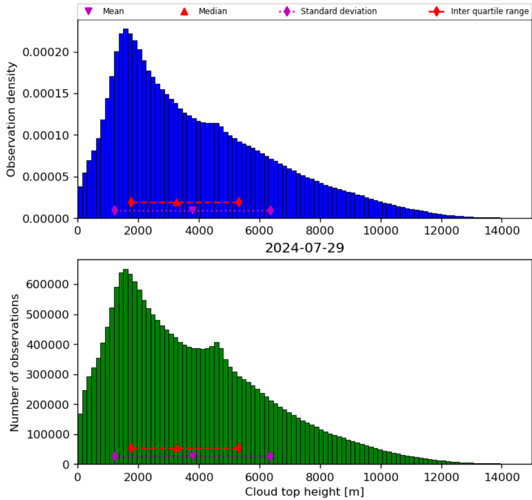
Figure 40: Histogram of “Cloud top height” for 2024-07-28 to 2024-07-30
