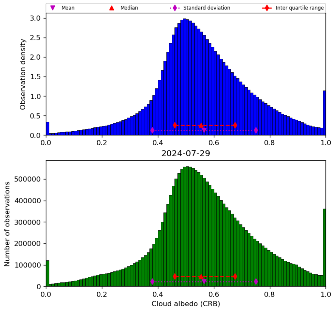
Figure 44: Histogram of “Cloud albedo (CRB)” for 2024-07-28 to 2024-07-30
