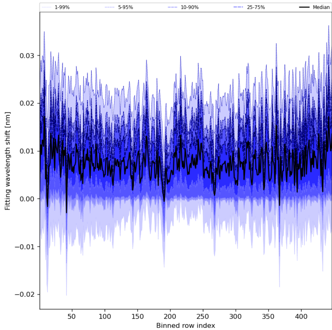
Figure 65: Along track statistics of “Fitting wavelength shift” for 2024-07-28 to 2024-07-30
