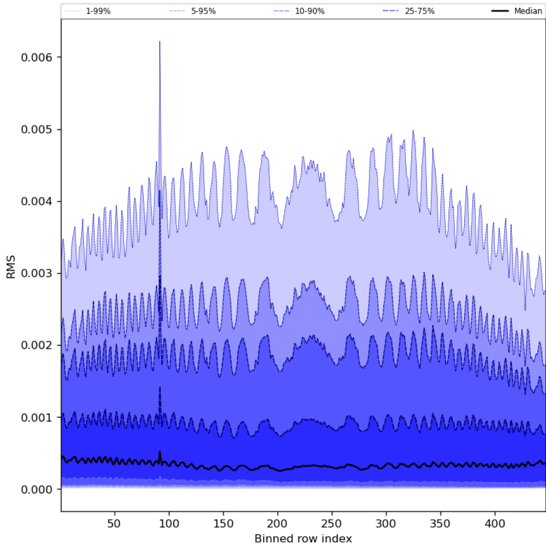
Figure 63: Along track statistics of “RMS” for 2024-07-28 to 2024-07-30
