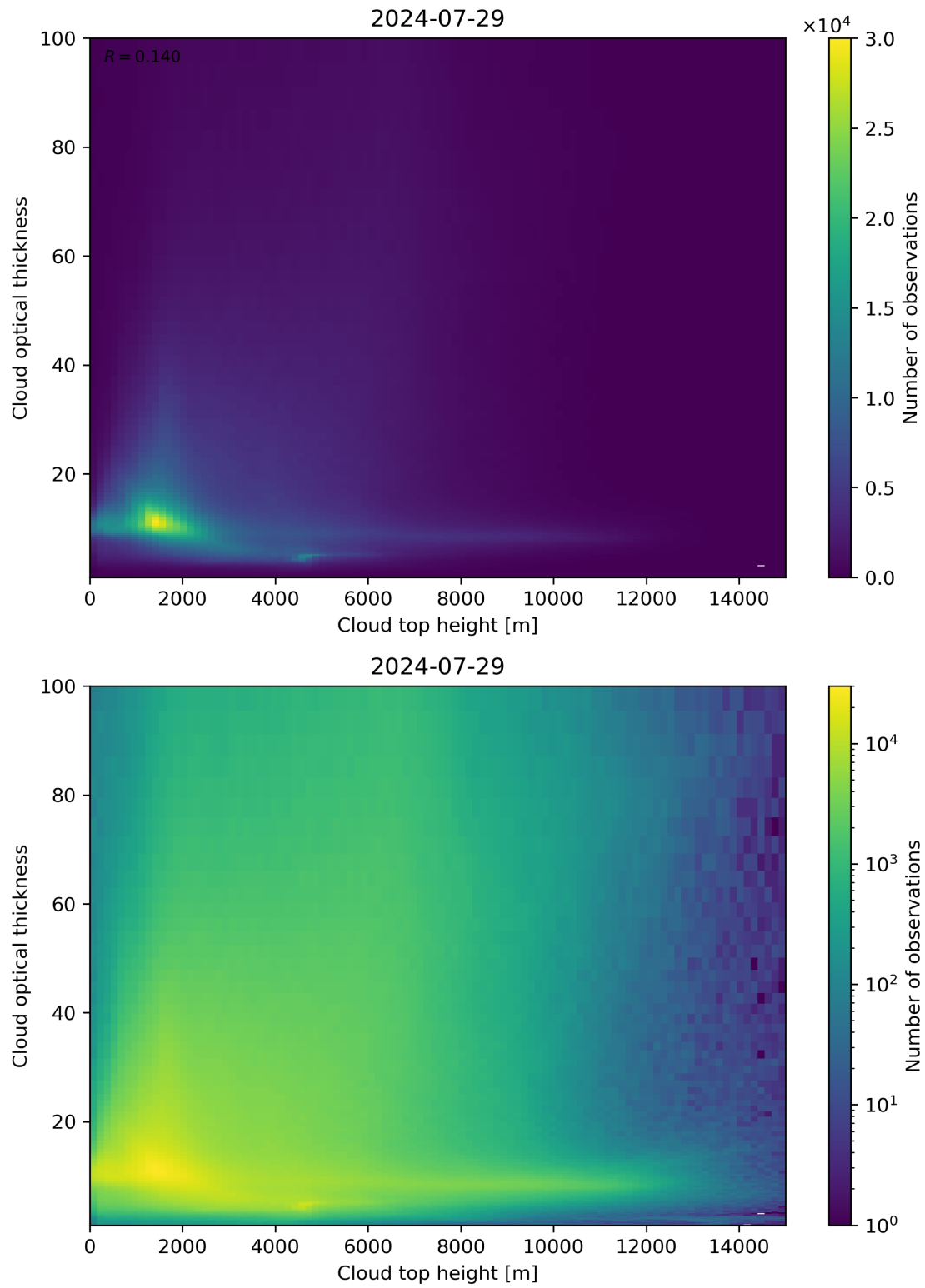
Figure 90: Scatter density plot of “Cloud top height” against “Cloud optical thickness” for 2024-07-28 to 2024-07-30.
