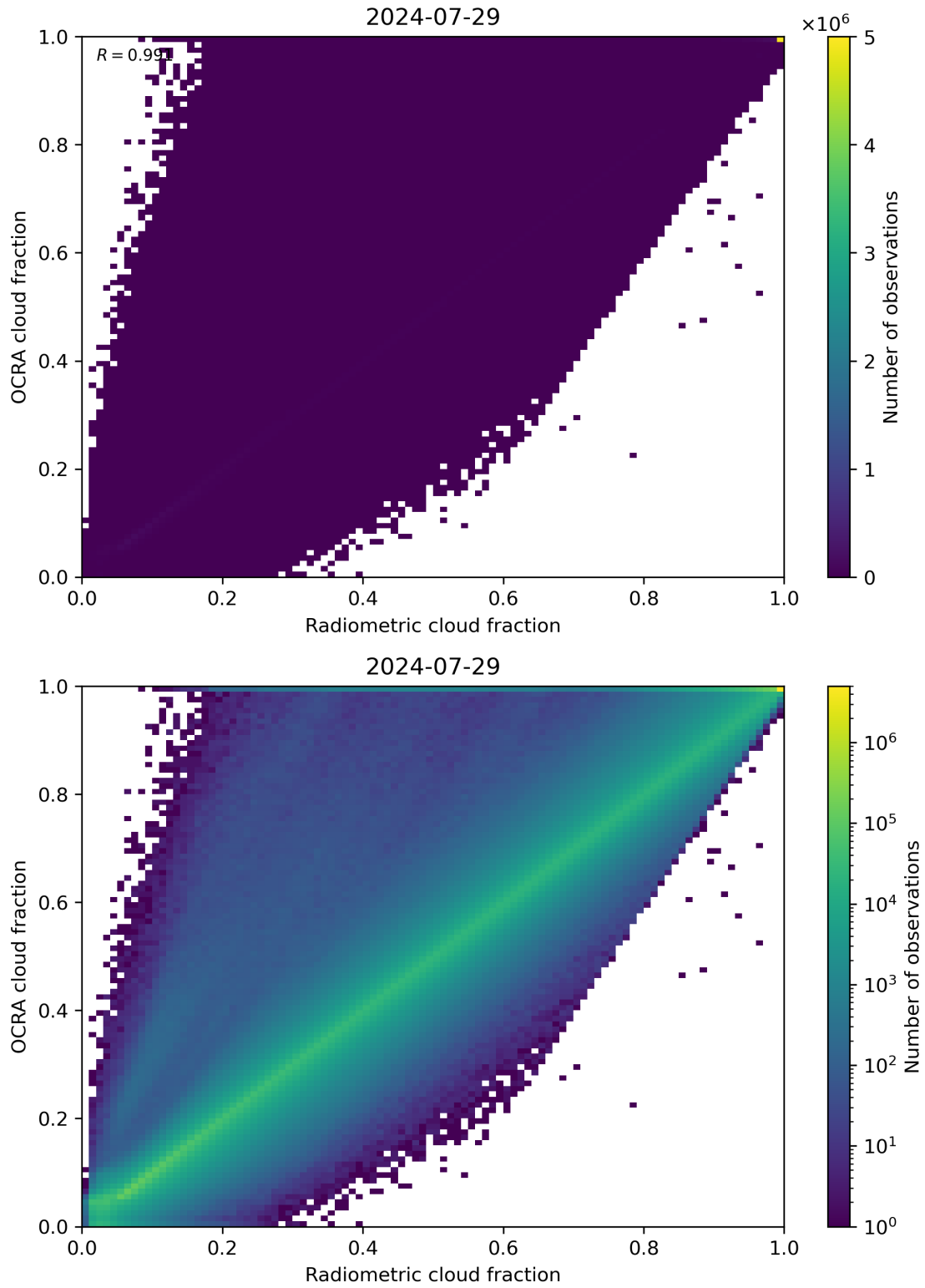
Figure 72: Scatter density plot of “Radiometric cloud fraction” against “OCRA cloud fraction” for 2024-07-28 to 2024-07-30.
