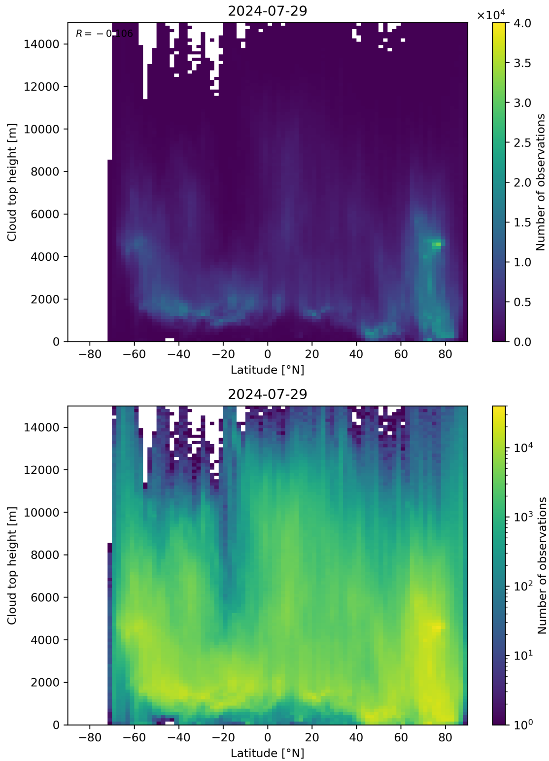
Figure 97: Scatter density plot of “Latitude” against “Cloud top height” for 2024-07-28 to 2024-07-30.
