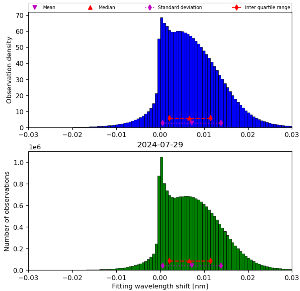
Figure 49: Histogram of “Fitting wavelength shift” for 2024-07-28 to 2024-07-30
