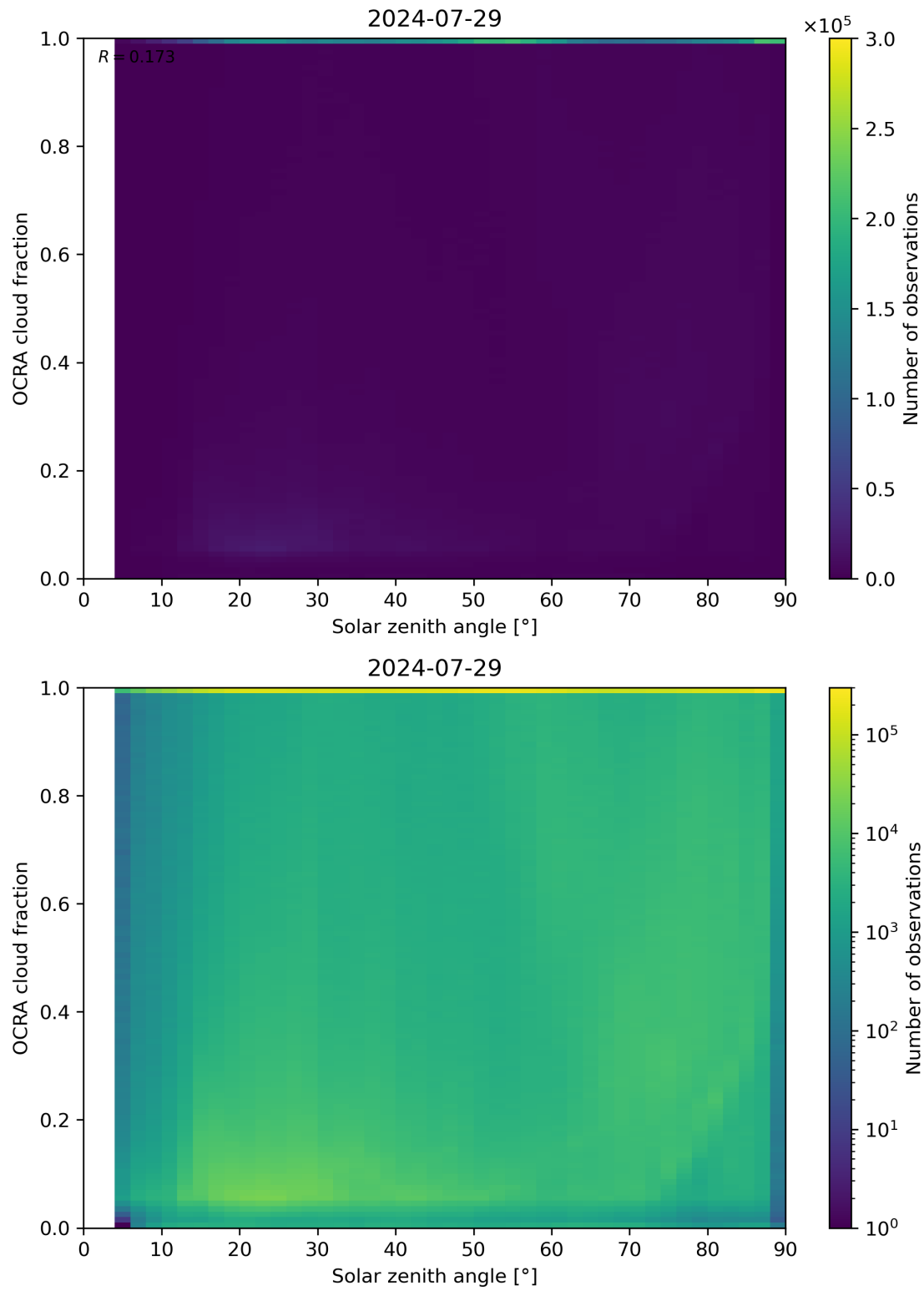
Figure 100: Scatter density plot of “Solar zenith angle” against “OCRA cloud fraction” for 2024-07-28 to 2024-07-30.
