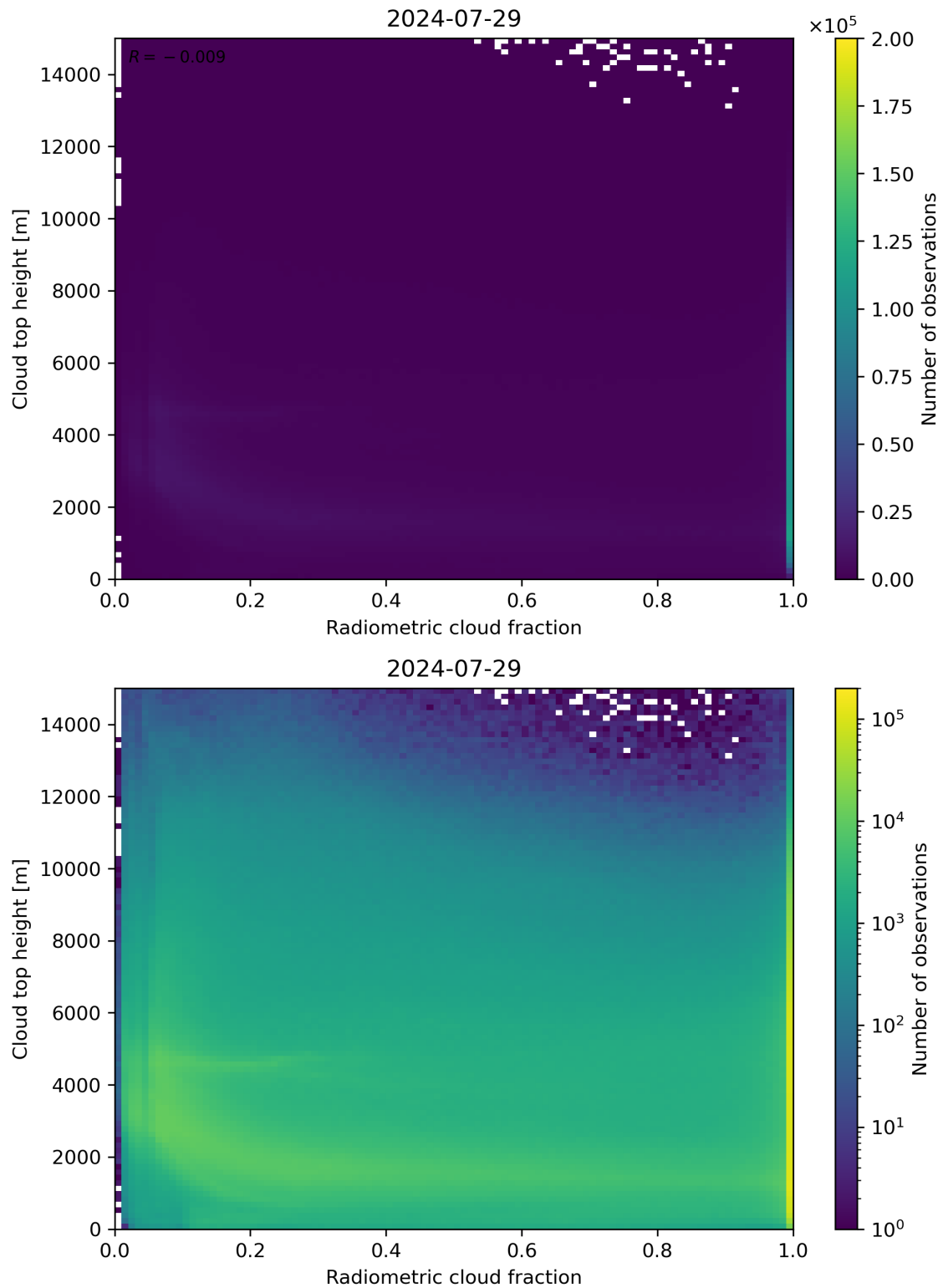
Figure 76: Scatter density plot of “Radiometric cloud fraction” against “Cloud top height” for 2024-07-28 to 2024-07-30.
