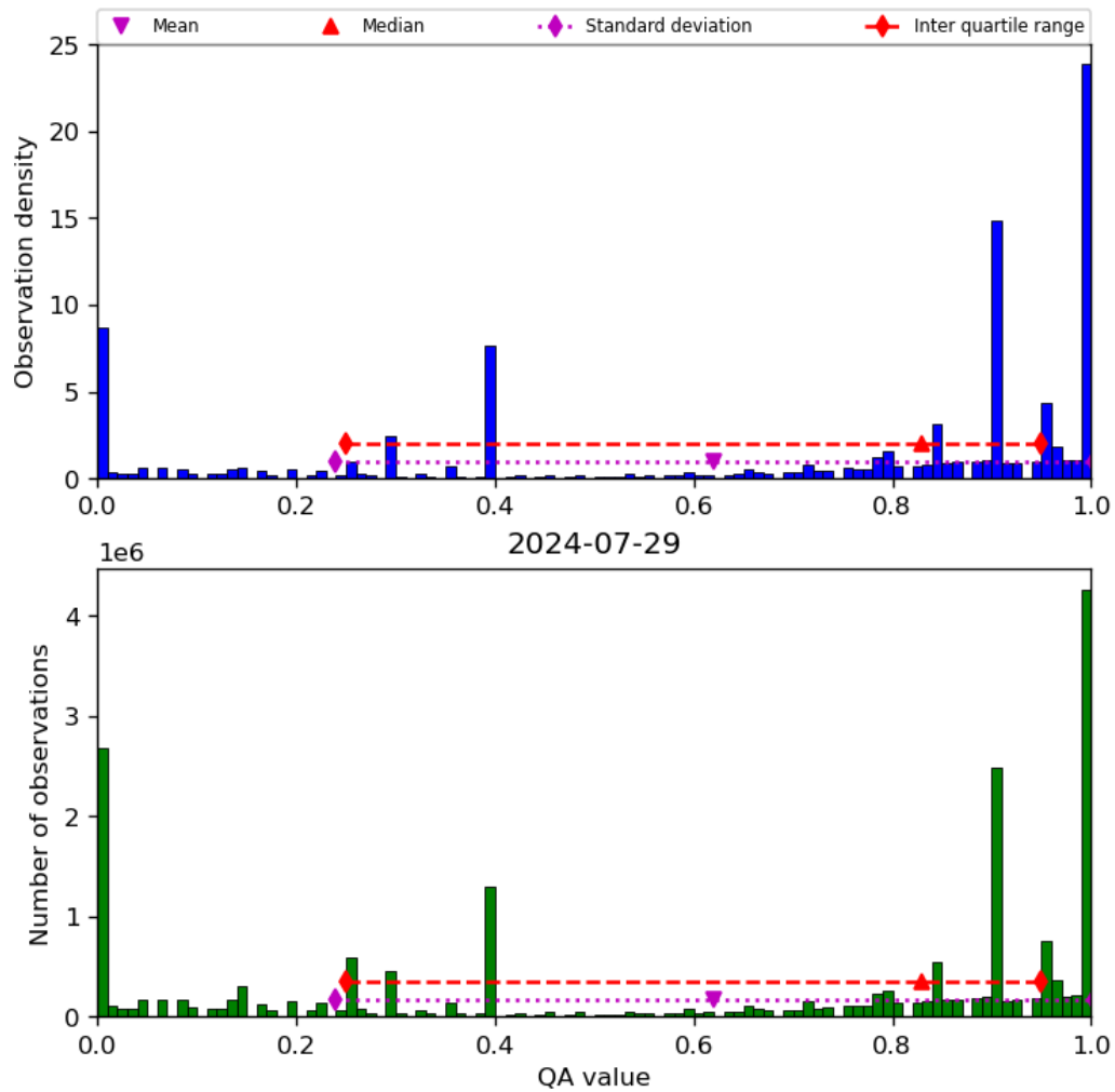
Figure 38: Histogram of “QA value” for 2024-07-28 to 2024-07-30
