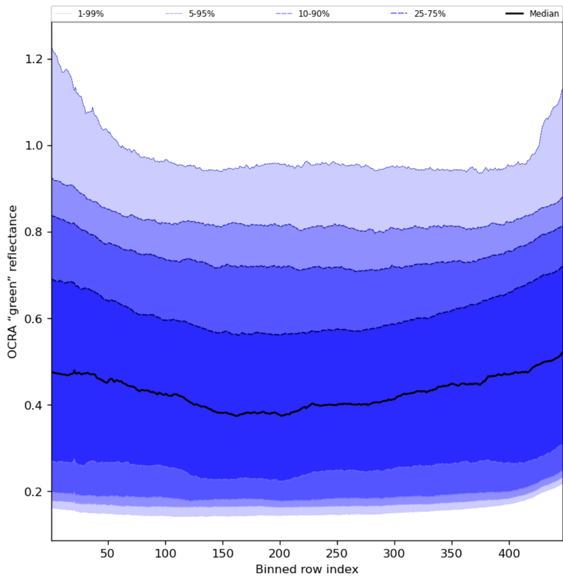
Figure 68: Along track statistics of “OCRA “green” reflectance” for 2024-07-28 to 2024-07-30
