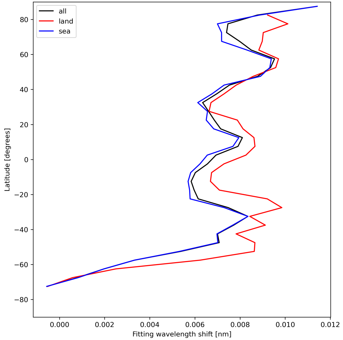
Figure 33: Zonal average of “Fitting wavelength shift” for 2024-07-28 to 2024-07-30.
