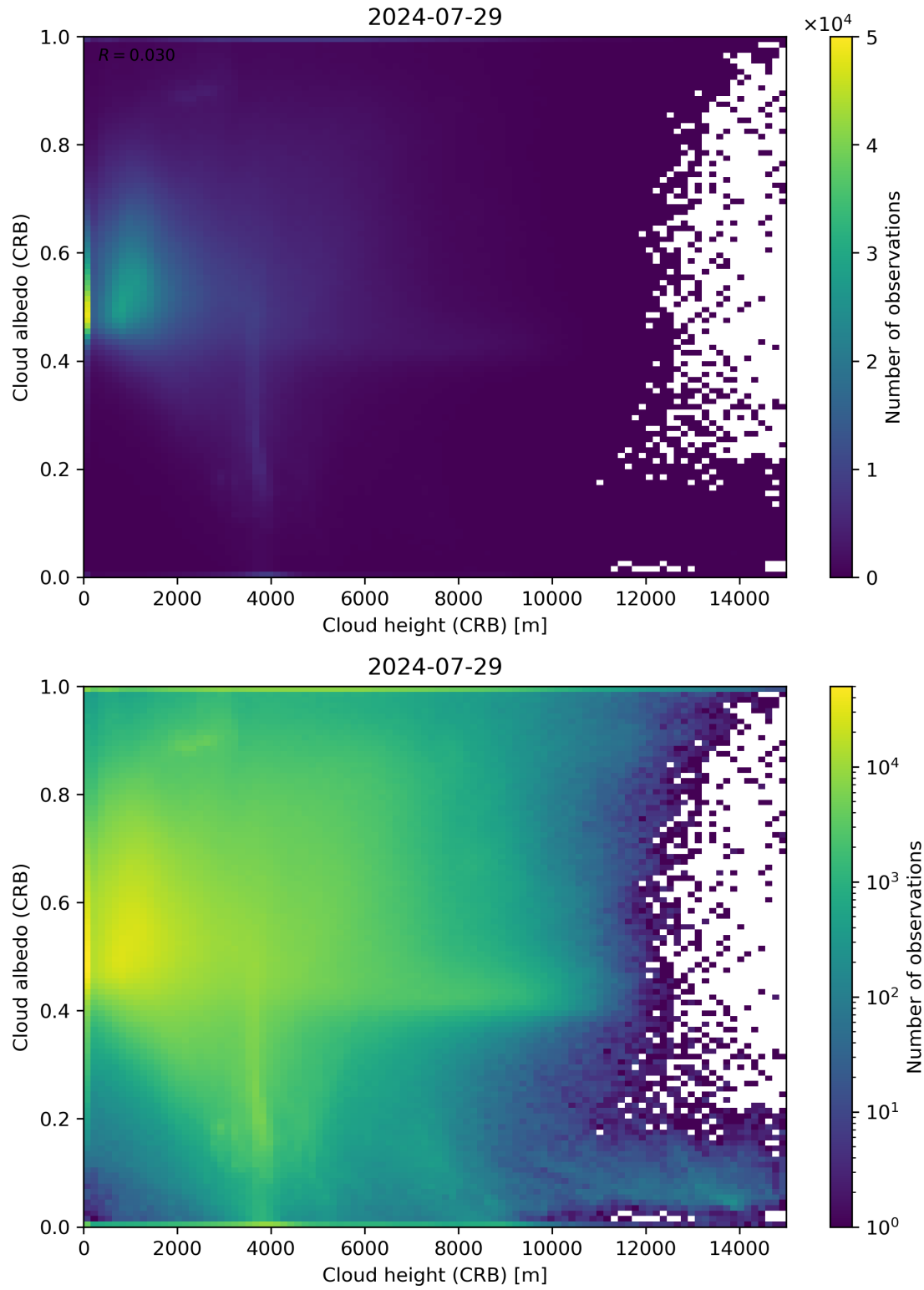
Figure 80: Scatter density plot of “Cloud height (CRB)” against “Cloud albedo (CRB)” for 2024-07-28 to 2024-07-30.
