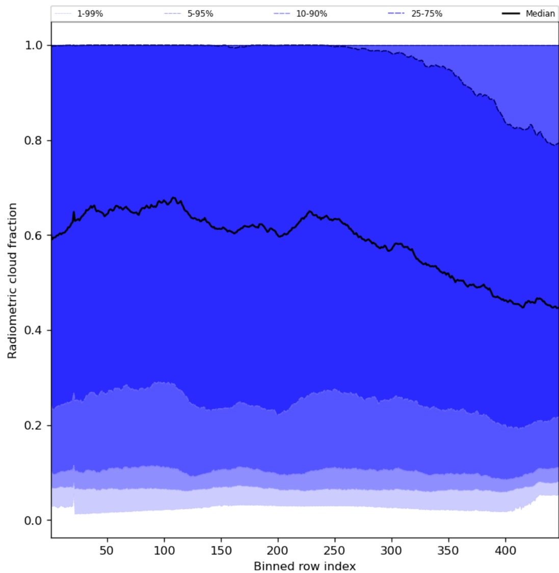
Figure 55: Along track statistics of “Radiometric cloud fraction” for 2024-07-28 to 2024-07-30
