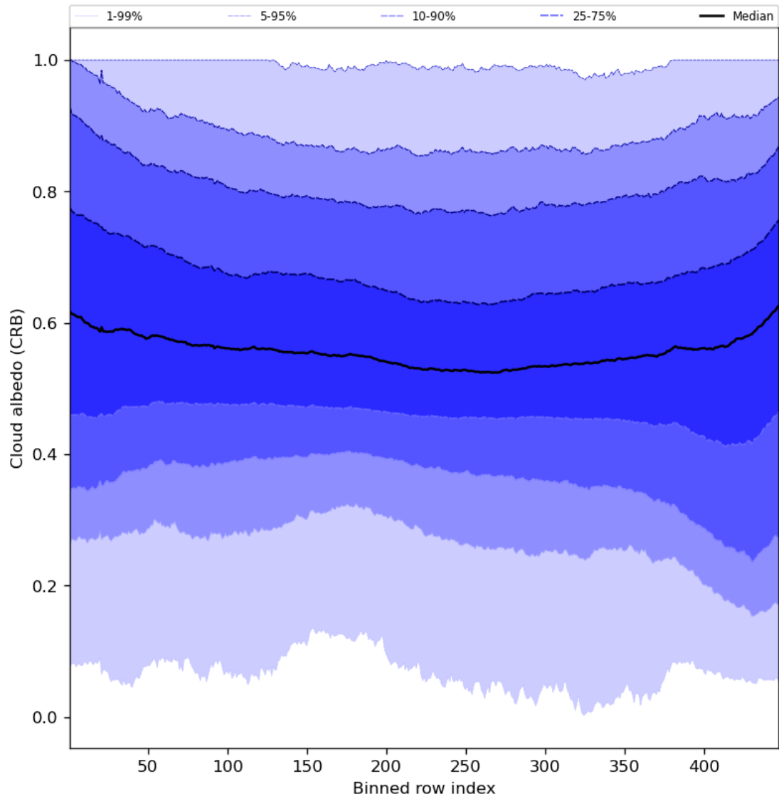
Figure 60: Along track statistics of “Cloud albedo (CRB)” for 2024-07-28 to 2024-07-30
