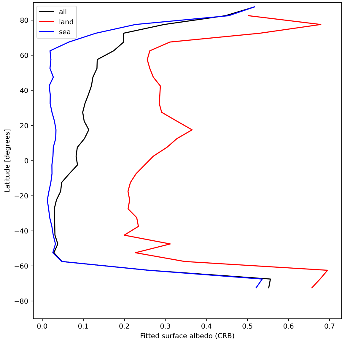
Figure 30: Zonal average of “Fitted surface albedo (CRB)” for 2024-07-28 to 2024-07-30.
