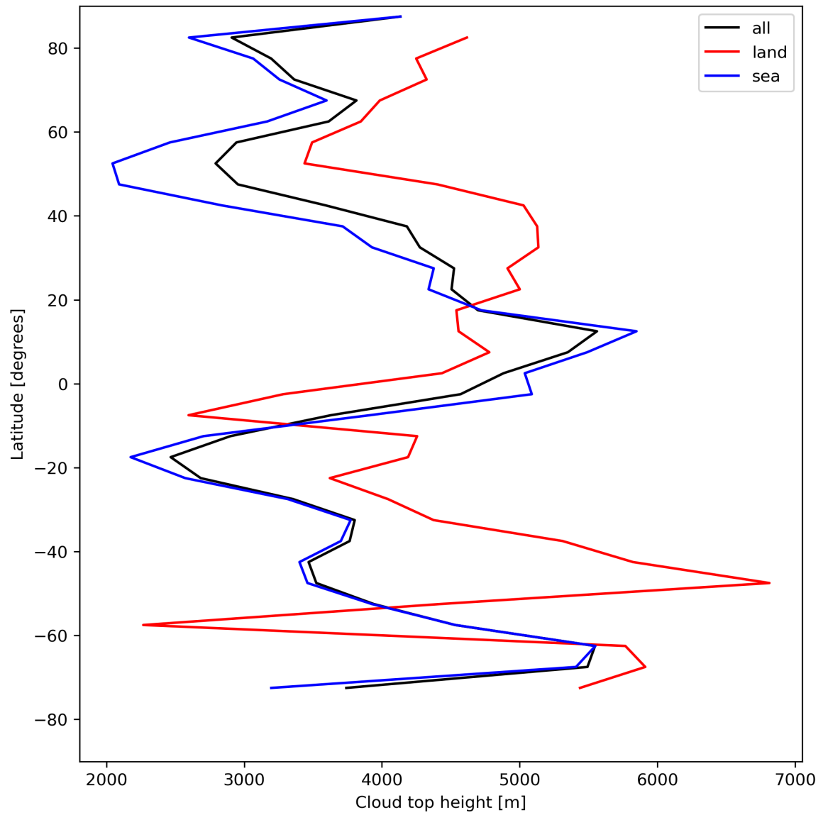
Figure 24: Zonal average of “Cloud top height” for 2024-07-28 to 2024-07-30.
