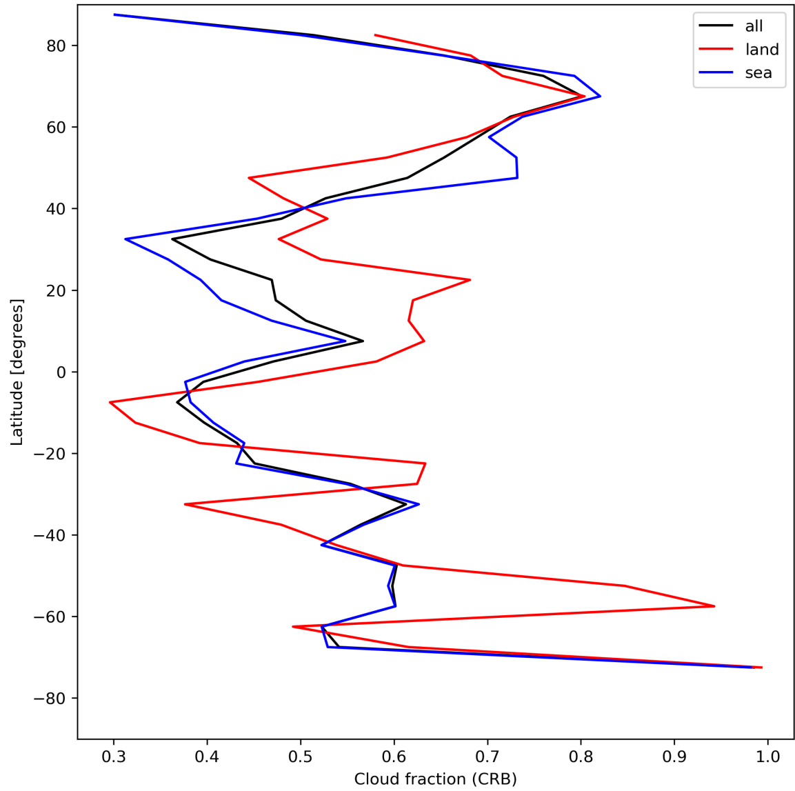
Figure 26: Zonal average of “Cloud fraction (CRB)” for 2024-07-28 to 2024-07-30.
