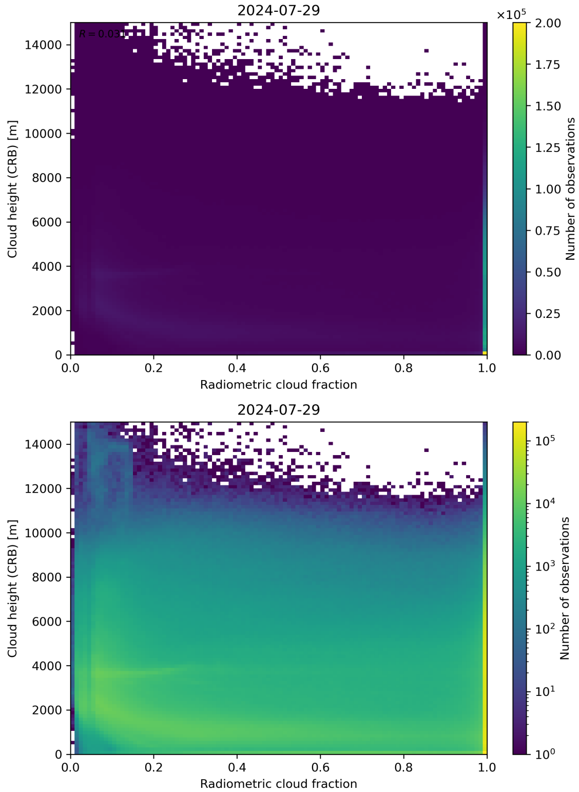
Figure 74: Scatter density plot of “Radiometric cloud fraction” against “Cloud height (CRB)” for 2024-07-28 to 2024-07-30.
