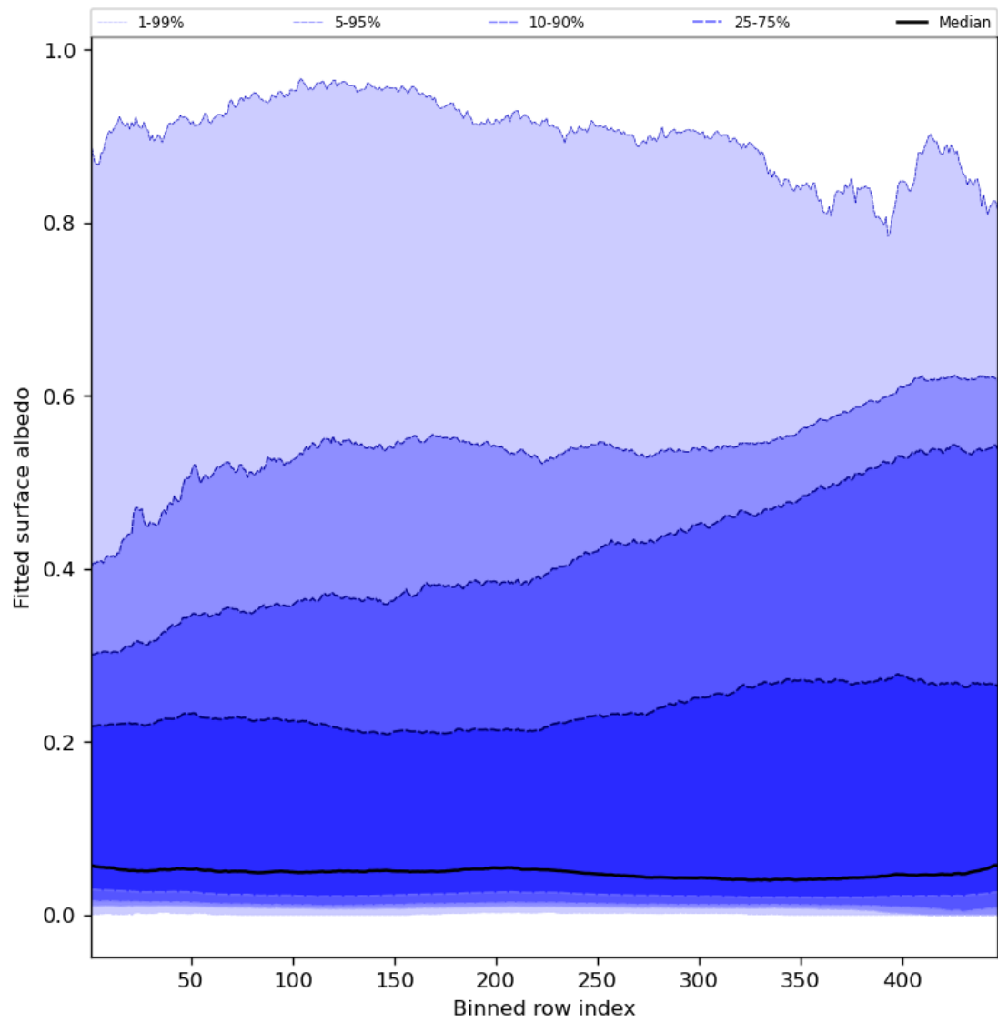
Figure 61: Along track statistics of “Fitted surface albedo” for 2024-07-28 to 2024-07-30
