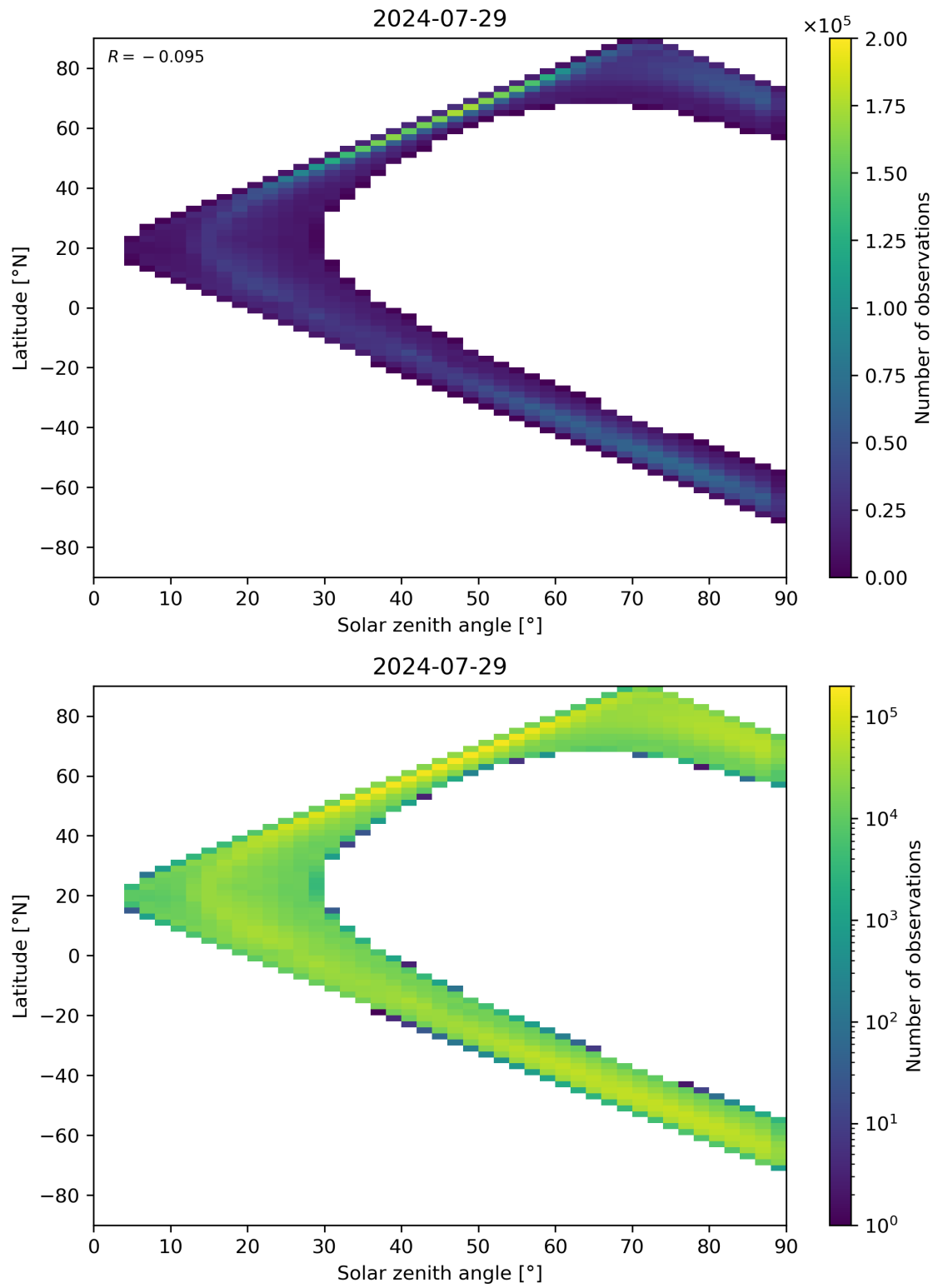
Figure 105: Scatter density plot of “Solar zenith angle” against “Latitude” for 2024-07-28 to 2024-07-30.
