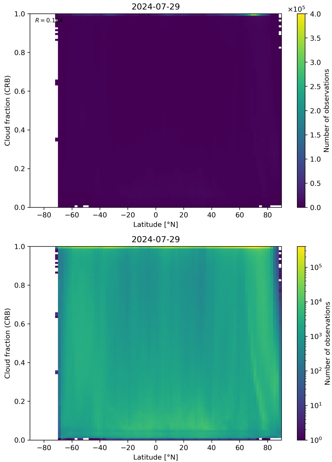
Figure 94: Scatter density plot of “Latitude” against “Cloud fraction (CRB)” for 2024-07-28 to 2024-07-30.
