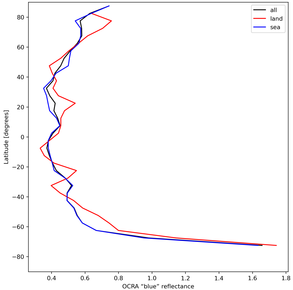
Figure 35: Zonal average of “OCRA “blue” reflectance” for 2024-07-28 to 2024-07-30.
