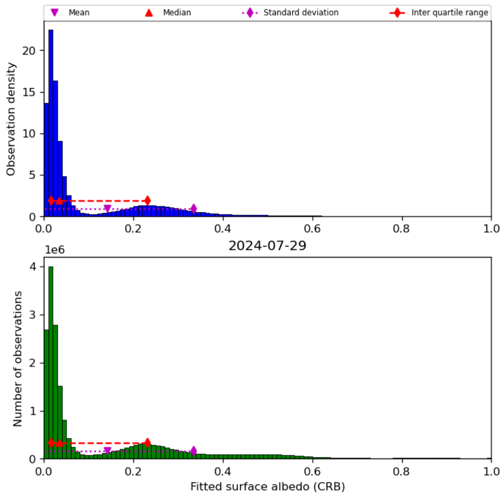
Figure 46: Histogram of “Fitted surface albedo (CRB)” for 2024-07-28 to 2024-07-30
