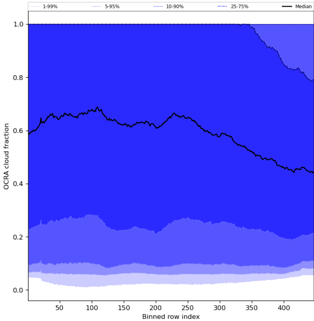
Figure 66: Along track statistics of “OCRA cloud fraction” for 2024-07-28 to 2024-07-30
