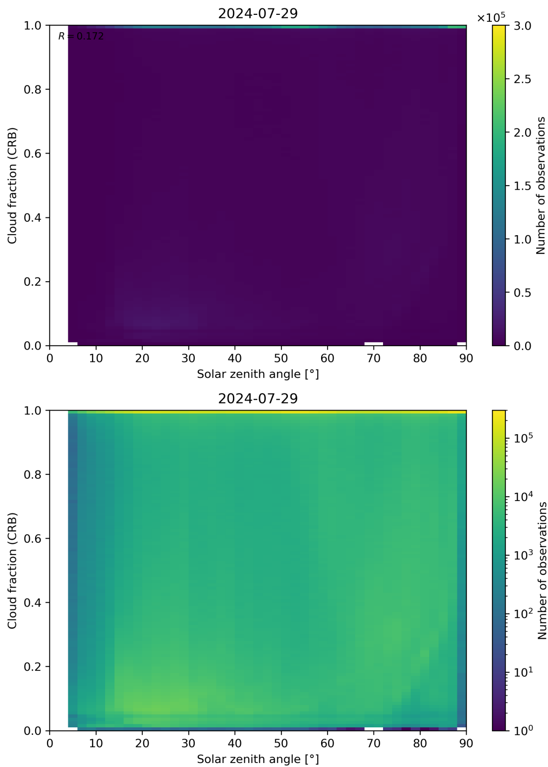
Figure 101: Scatter density plot of “Solar zenith angle” against “Cloud fraction (CRB)” for 2024-07-28 to 2024-07-30.
