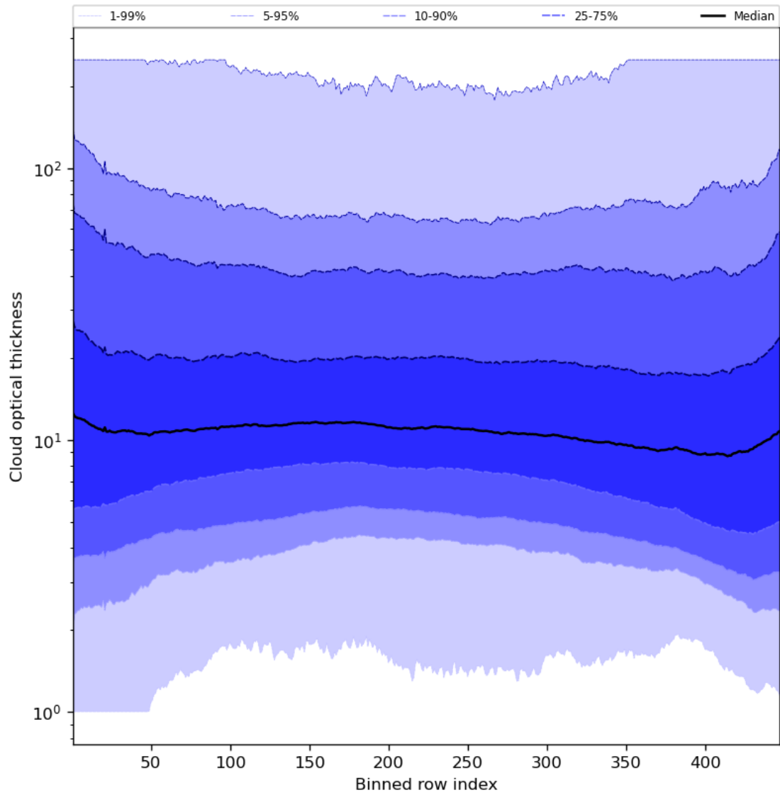
Figure 57: Along track statistics of “Cloud optical thickness” for 2024-07-28 to 2024-07-30
