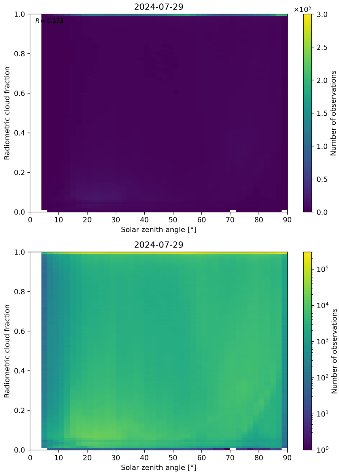
Figure 99: Scatter density plot of “Solar zenith angle” against “Radiometric cloud fraction” for 2024-07-28 to 2024-07-30.
