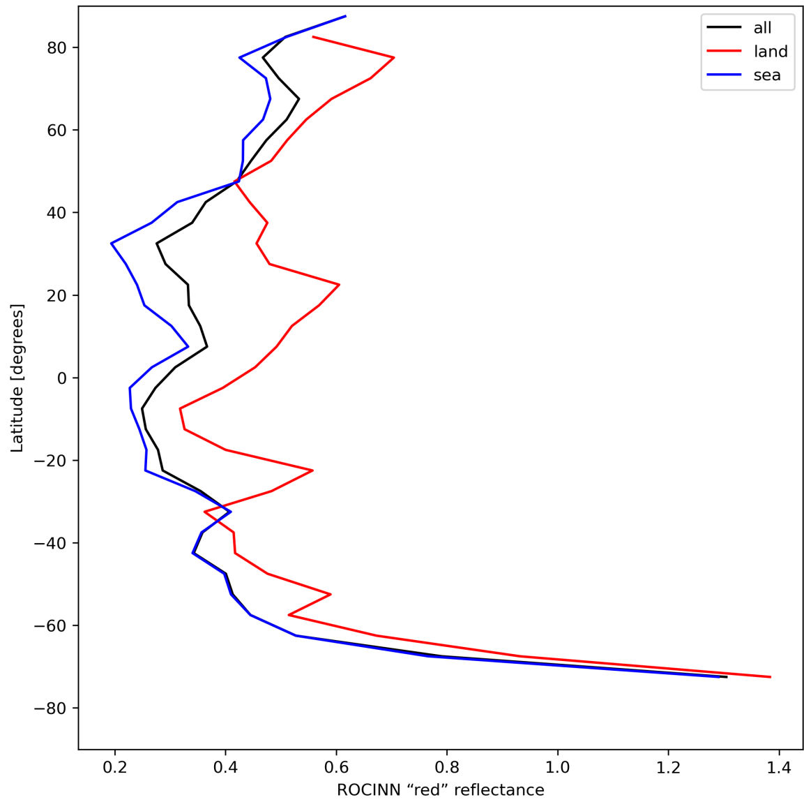
Figure 37: Zonal average of “ROCINN “red” reflectance” for 2024-07-28 to 2024-07-30.
