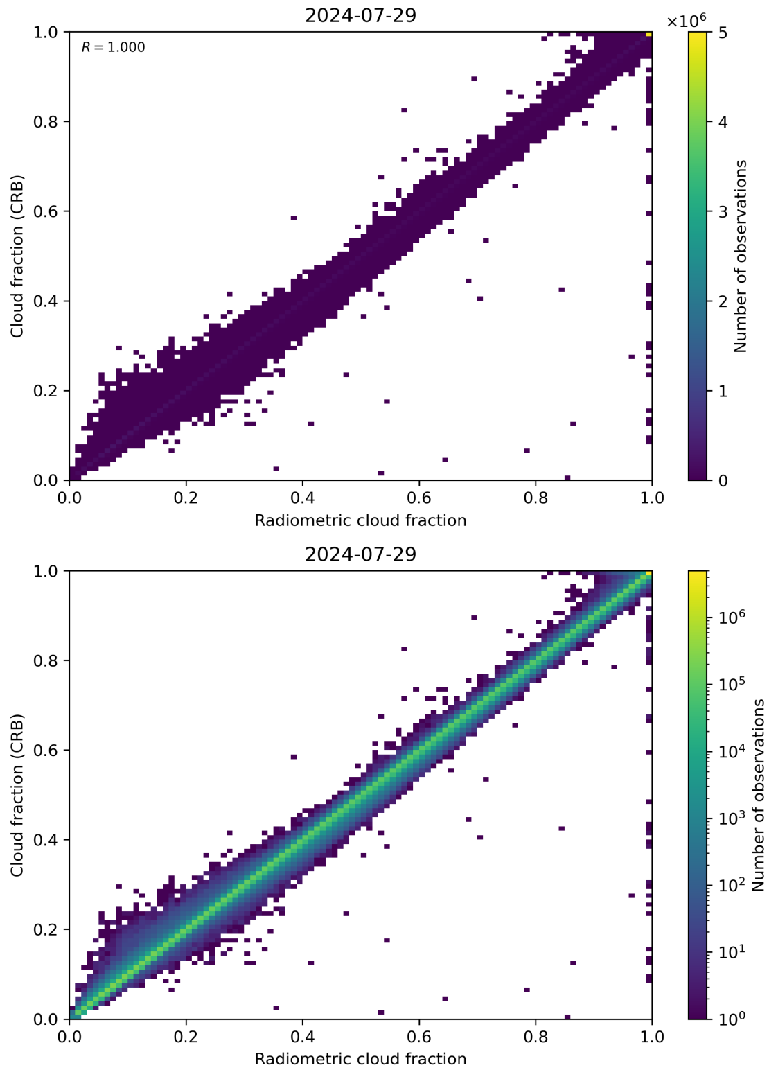
Figure 73: Scatter density plot of “Radiometric cloud fraction” against “Cloud fraction (CRB)” for 2024-07-28 to 2024-07-30.
