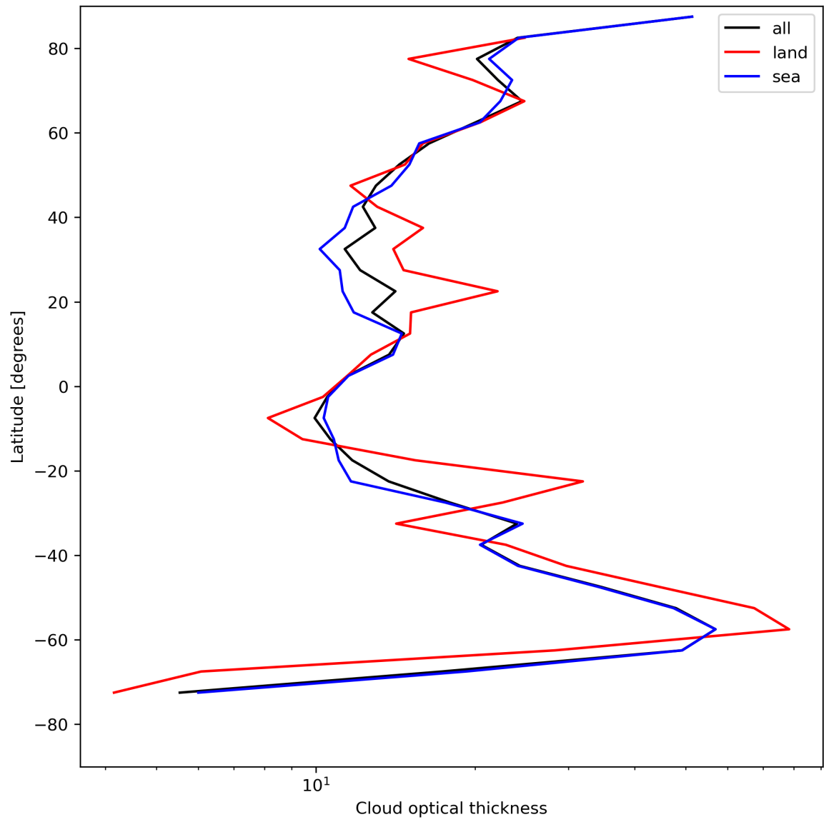
Figure 25: Zonal average of “Cloud optical thickness” for 2024-07-28 to 2024-07-30.
