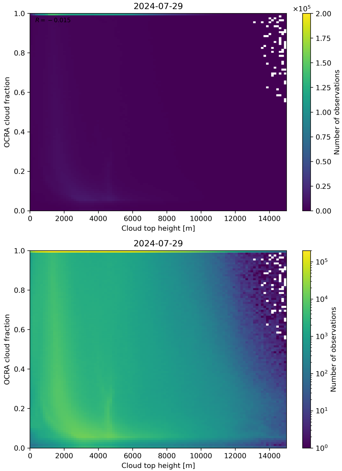
Figure 87: Scatter density plot of “Cloud top height” against “OCRA cloud fraction” for 2024-07-28 to 2024-07-30.
