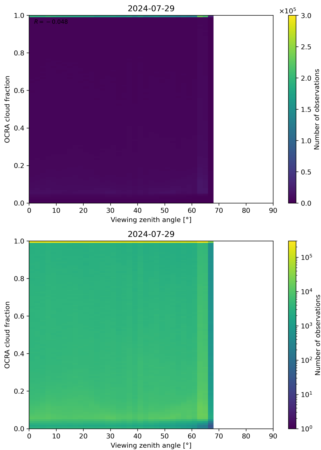
Figure 108: Scatter density plot of “Viewing zenith angle” against “OCRA cloud fraction” for 2024-07-28 to 2024-07-30.
