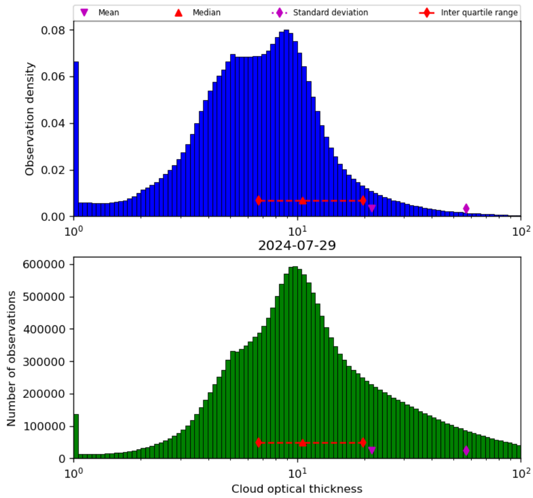
Figure 41: Histogram of “Cloud optical thickness” for 2024-07-28 to 2024-07-30
