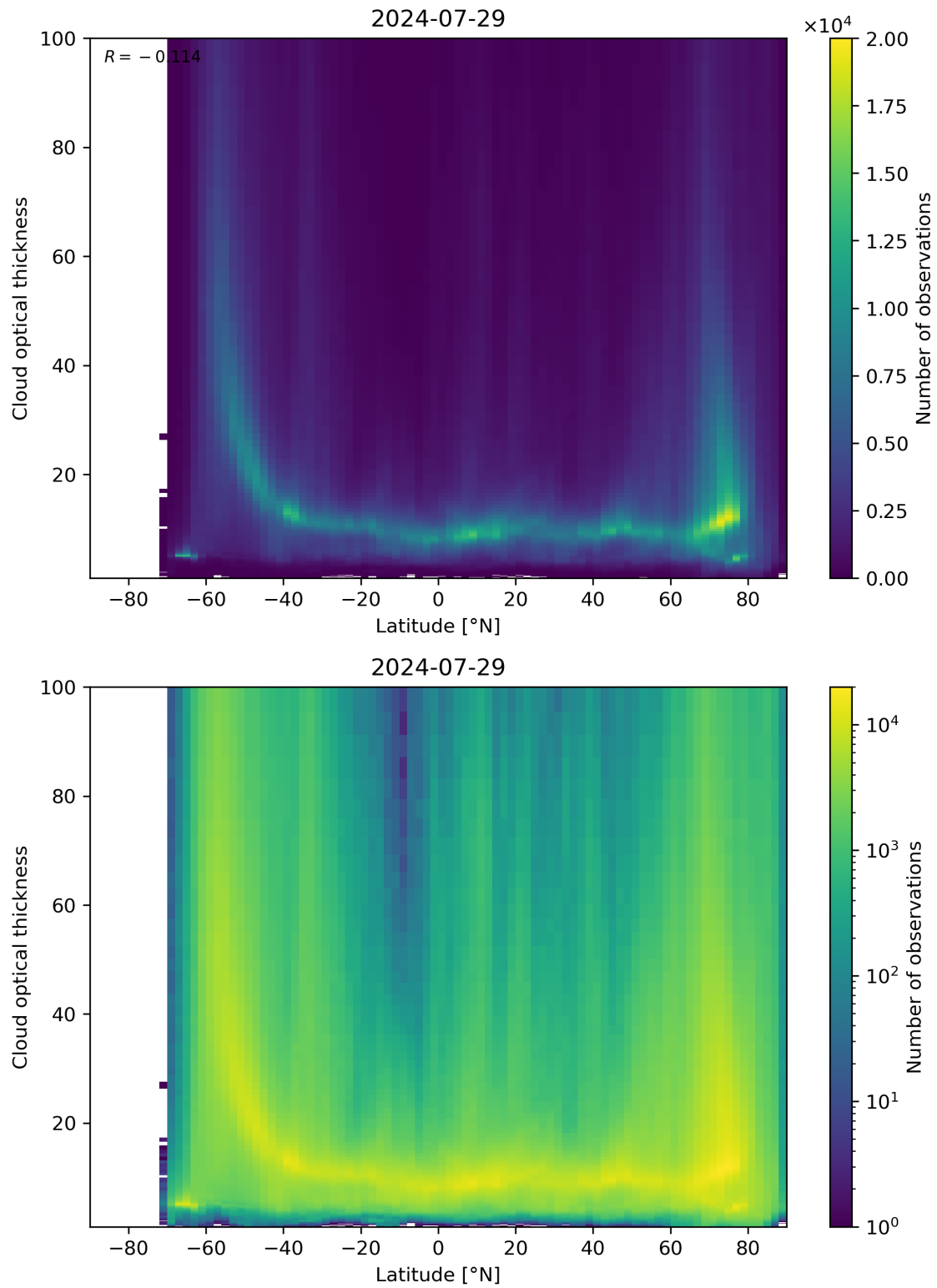
Figure 96: Scatter density plot of “Latitude” against “Cloud optical thickness” for 2024-07-28 to 2024-07-30.
