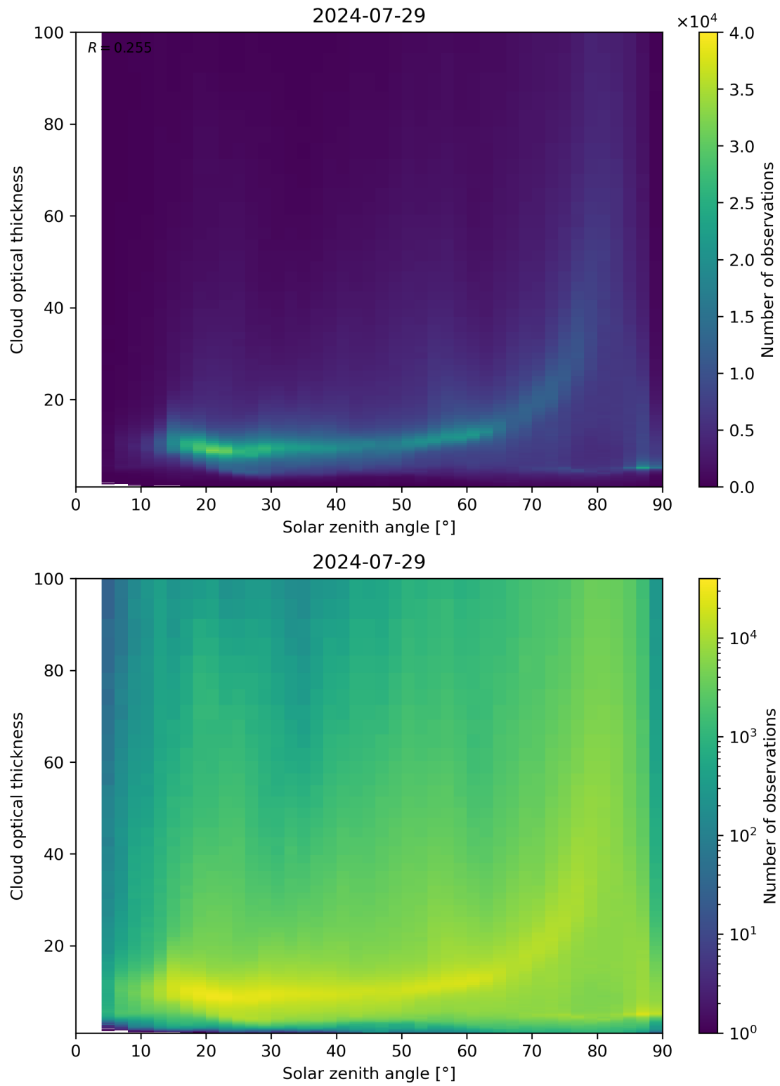
Figure 103: Scatter density plot of “Solar zenith angle” against “Cloud optical thickness” for 2024-07-28 to 2024-07-30.
