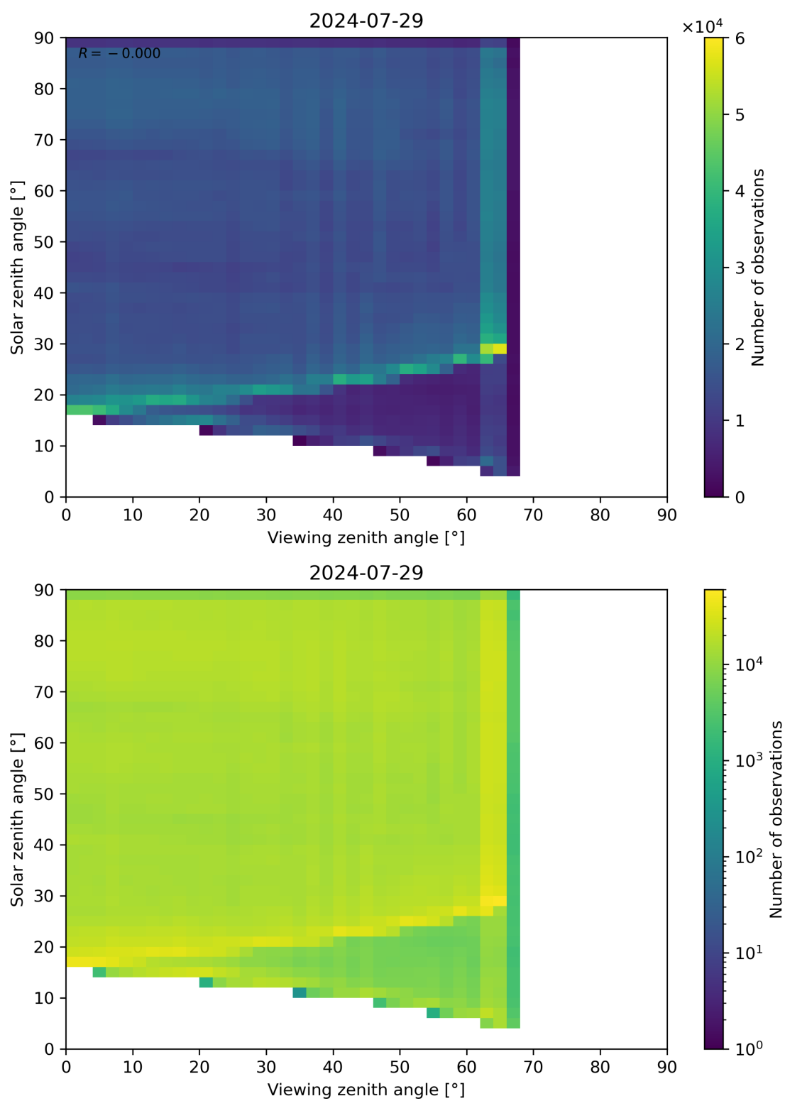
Figure 114: Scatter density plot of “Viewing zenith angle” against “Solar zenith angle” for 2024-07-28 to 2024-07-30.
