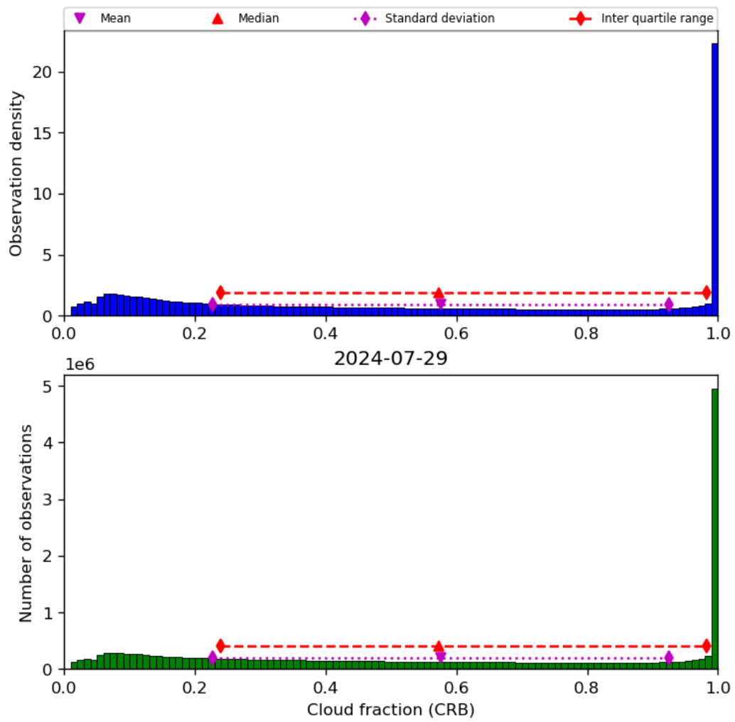
Figure 42: Histogram of “Cloud fraction (CRB)” for 2024-07-28 to 2024-07-30
