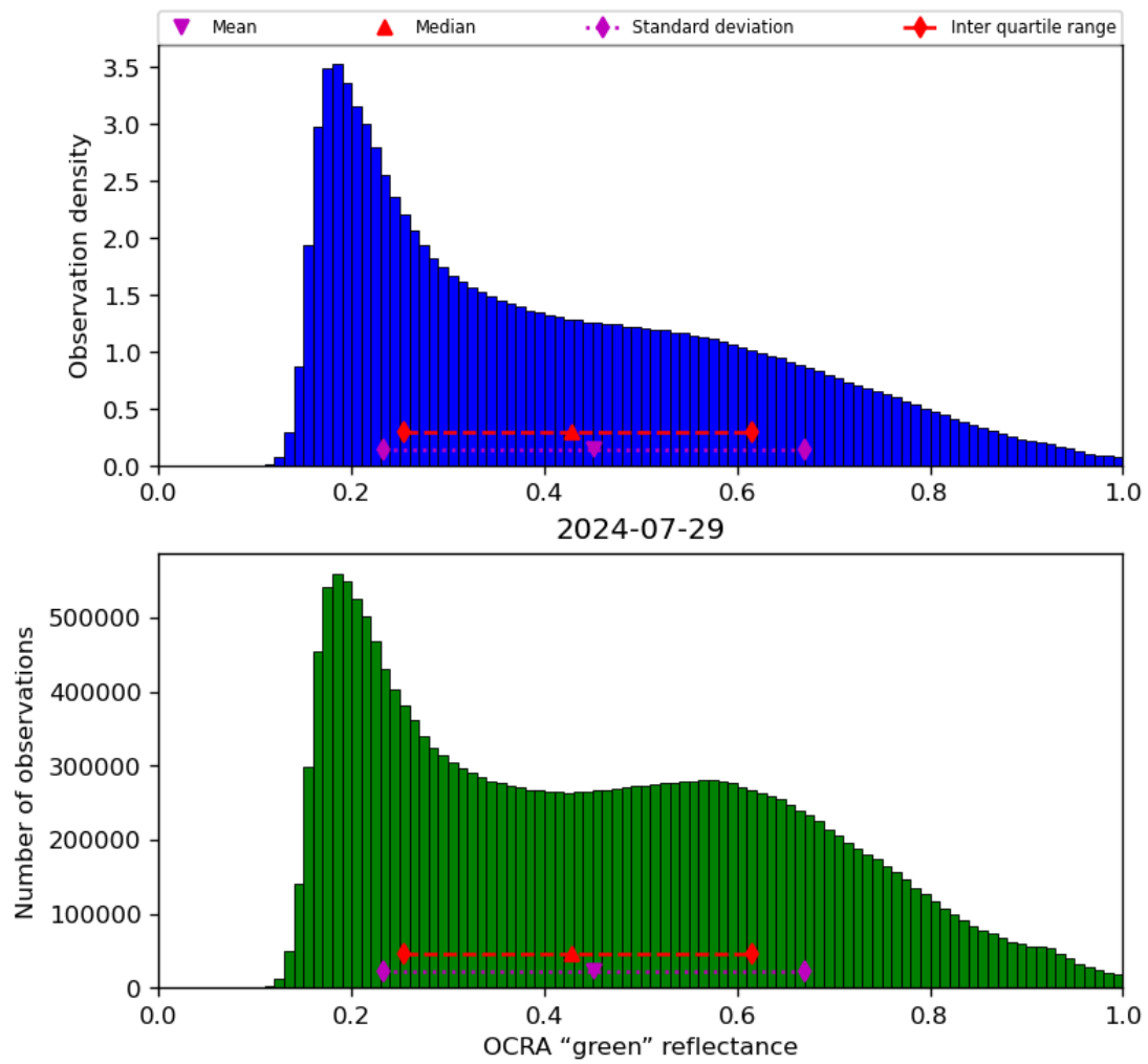
Figure 52: Histogram of “OCRA “green” reflectance” for 2024-07-28 to 2024-07-30
