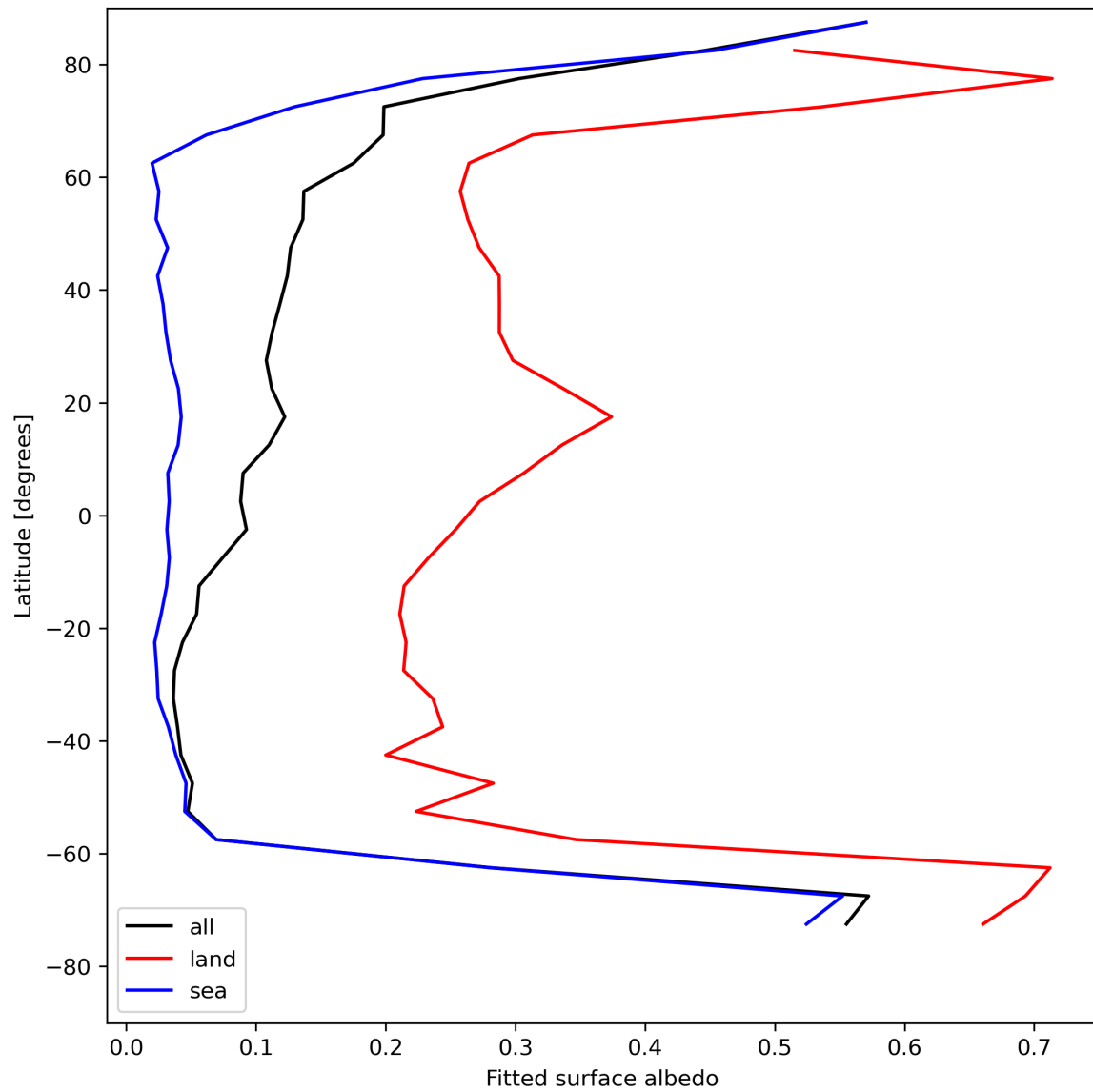
Figure 29: Zonal average of “Fitted surface albedo” for 2024-07-28 to 2024-07-30.
