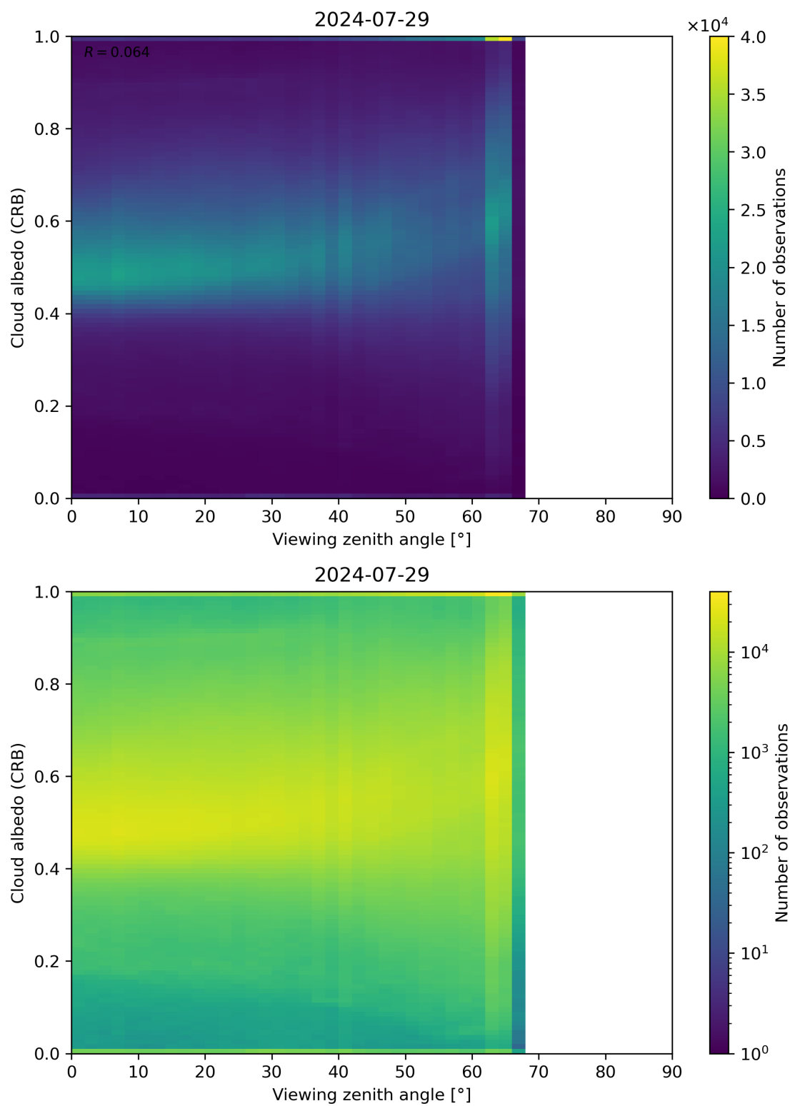
Figure 106: Scatter density plot of “Viewing zenith angle” against “Cloud albedo (CRB)” for 2024-07-28 to 2024-07-30.
