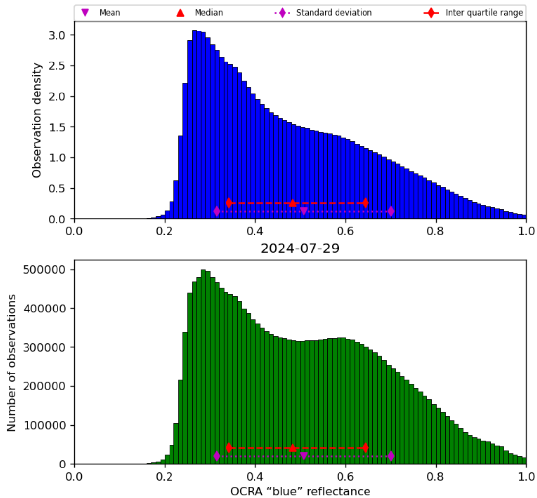
Figure 51: Histogram of “OCRA “blue” reflectance” for 2024-07-28 to 2024-07-30
