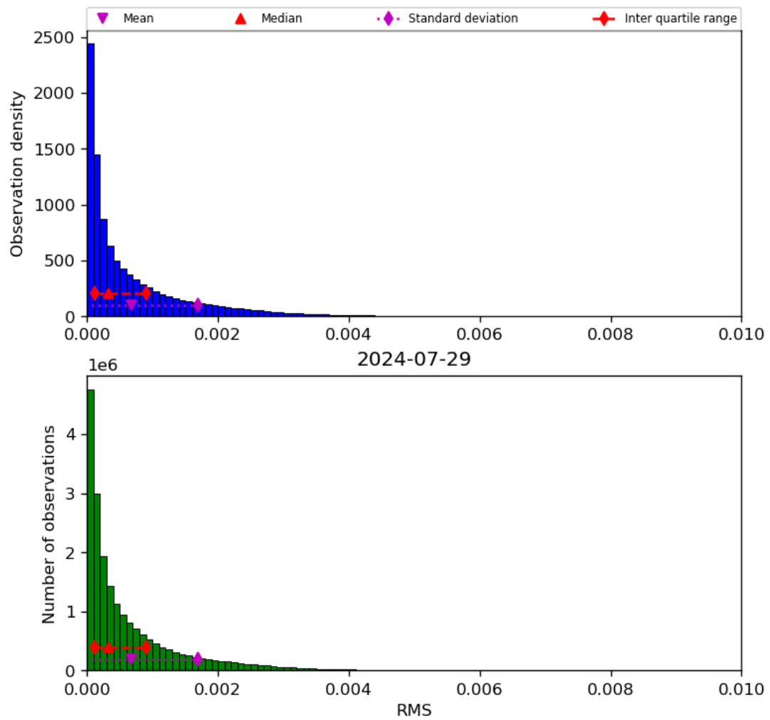
Figure 47: Histogram of “RMS” for 2024-07-28 to 2024-07-30
