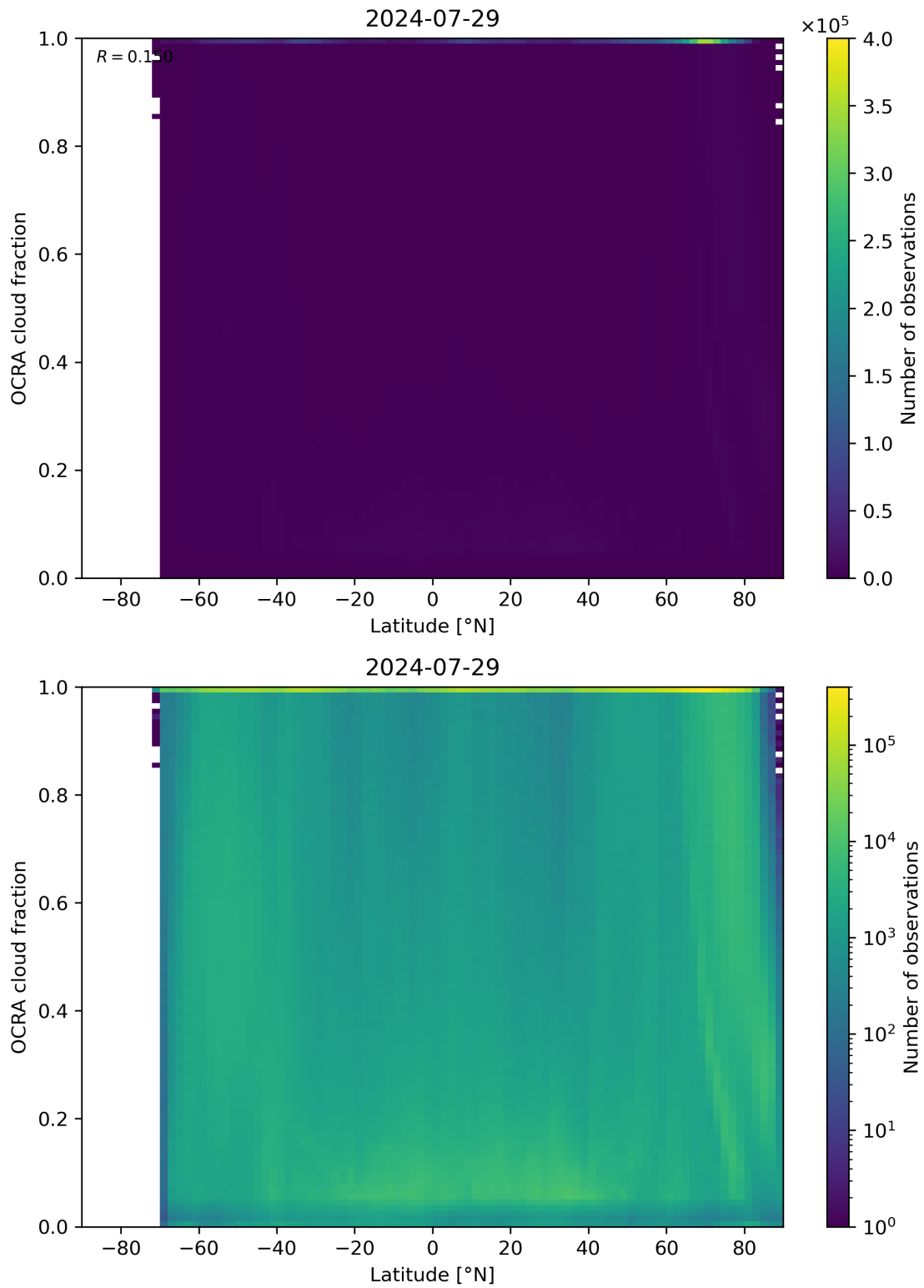
Figure 93: Scatter density plot of “Latitude” against “OCRA cloud fraction” for 2024-07-28 to 2024-07-30.
