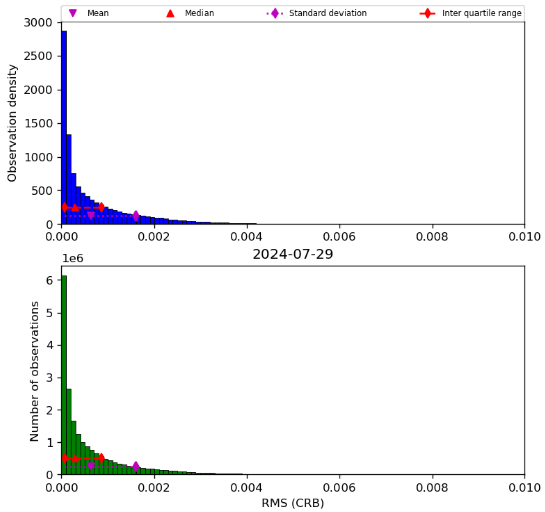
Figure 48: Histogram of “RMS (CRB)” for 2024-07-28 to 2024-07-30
