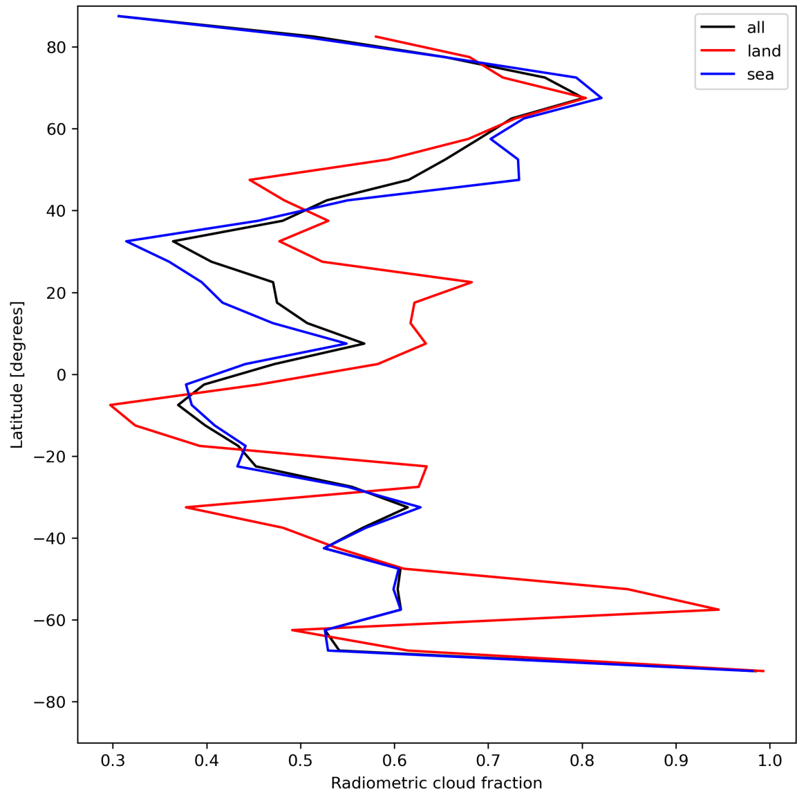
Figure 23: Zonal average of “Radiometric cloud fraction” for 2024-07-28 to 2024-07-30.
