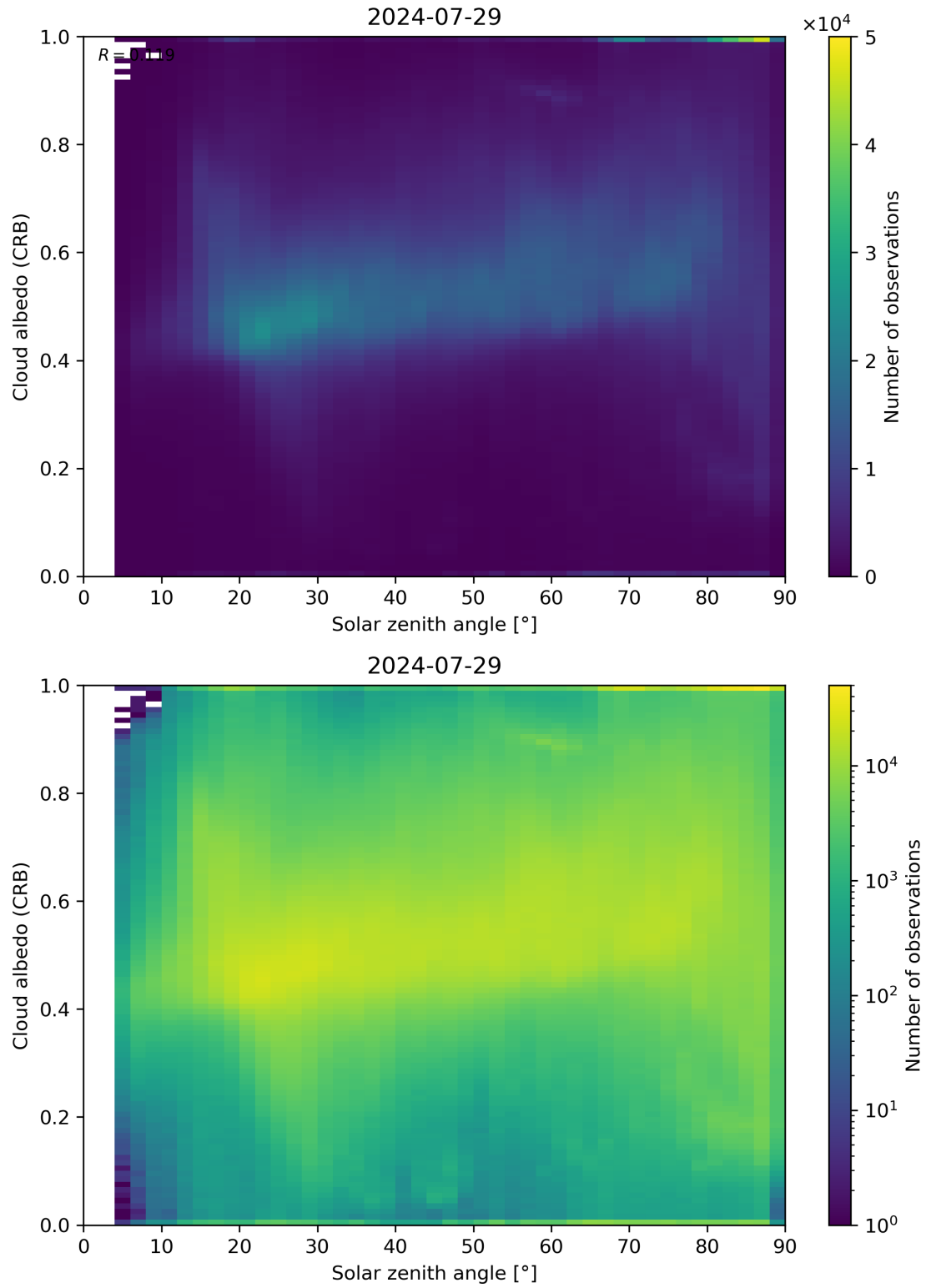
Figure 98: Scatter density plot of “Solar zenith angle” against “Cloud albedo (CRB)” for 2024-07-28 to 2024-07-30.
