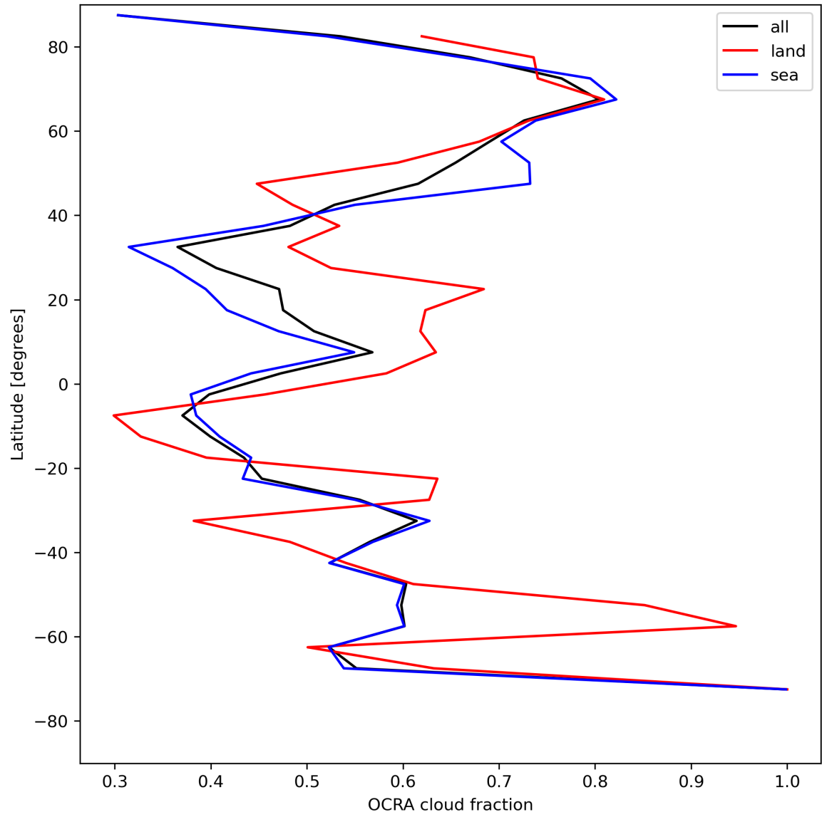
Figure 34: Zonal average of “OCRA cloud fraction” for 2024-07-28 to 2024-07-30.
