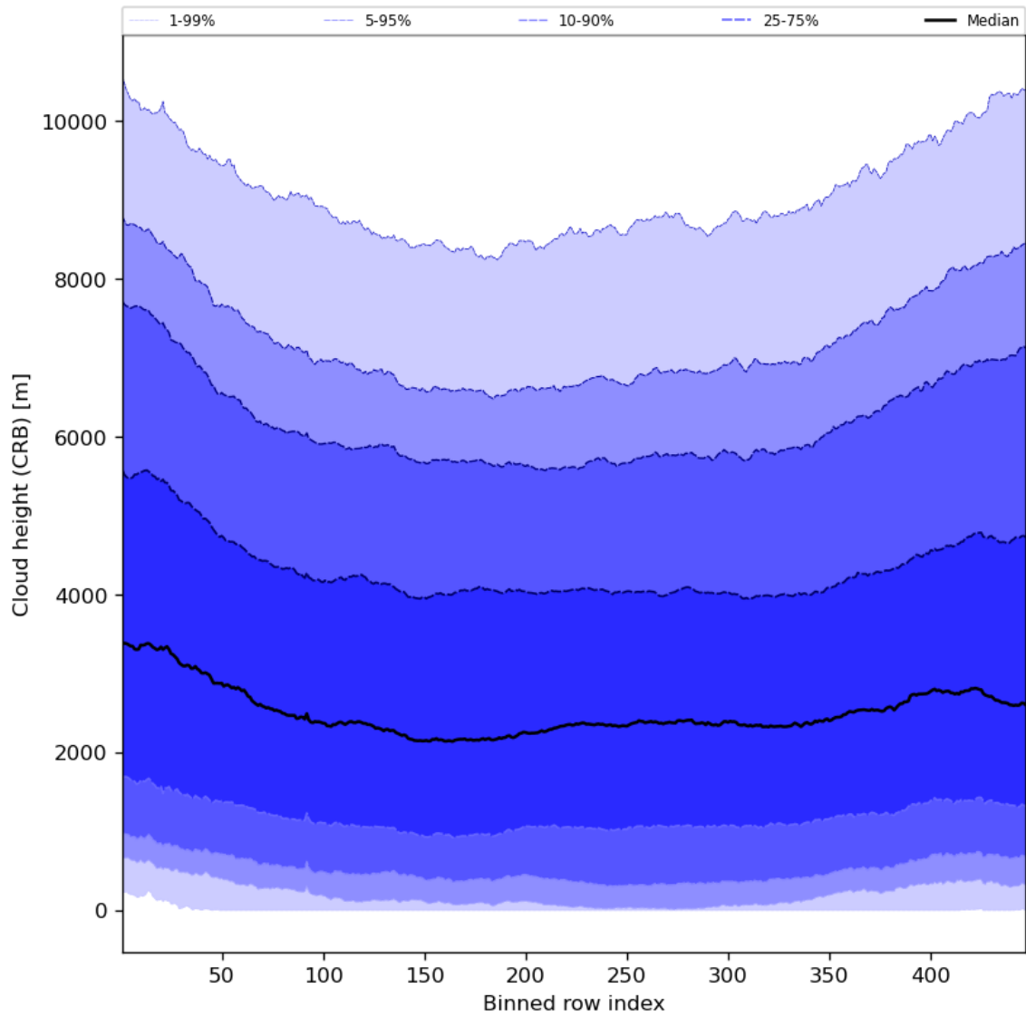
Figure 59: Along track statistics of “Cloud height (CRB)” for 2024-07-28 to 2024-07-30
