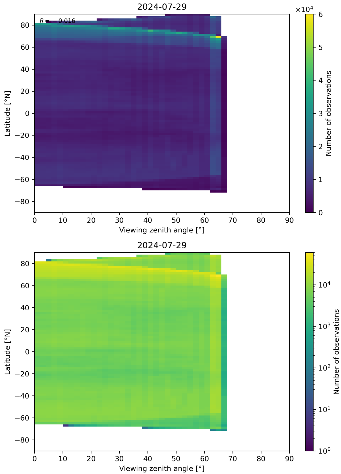
Figure 113: Scatter density plot of “Viewing zenith angle” against “Latitude” for 2024-07-28 to 2024-07-30.
