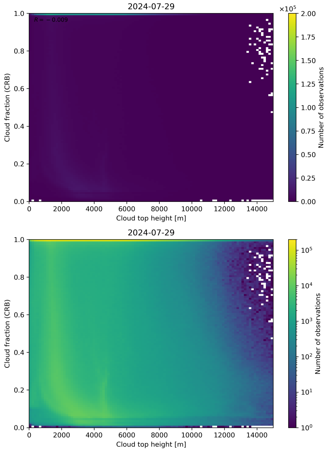
Figure 88: Scatter density plot of “Cloud top height” against “Cloud fraction (CRB)” for 2024-07-28 to 2024-07-30.
