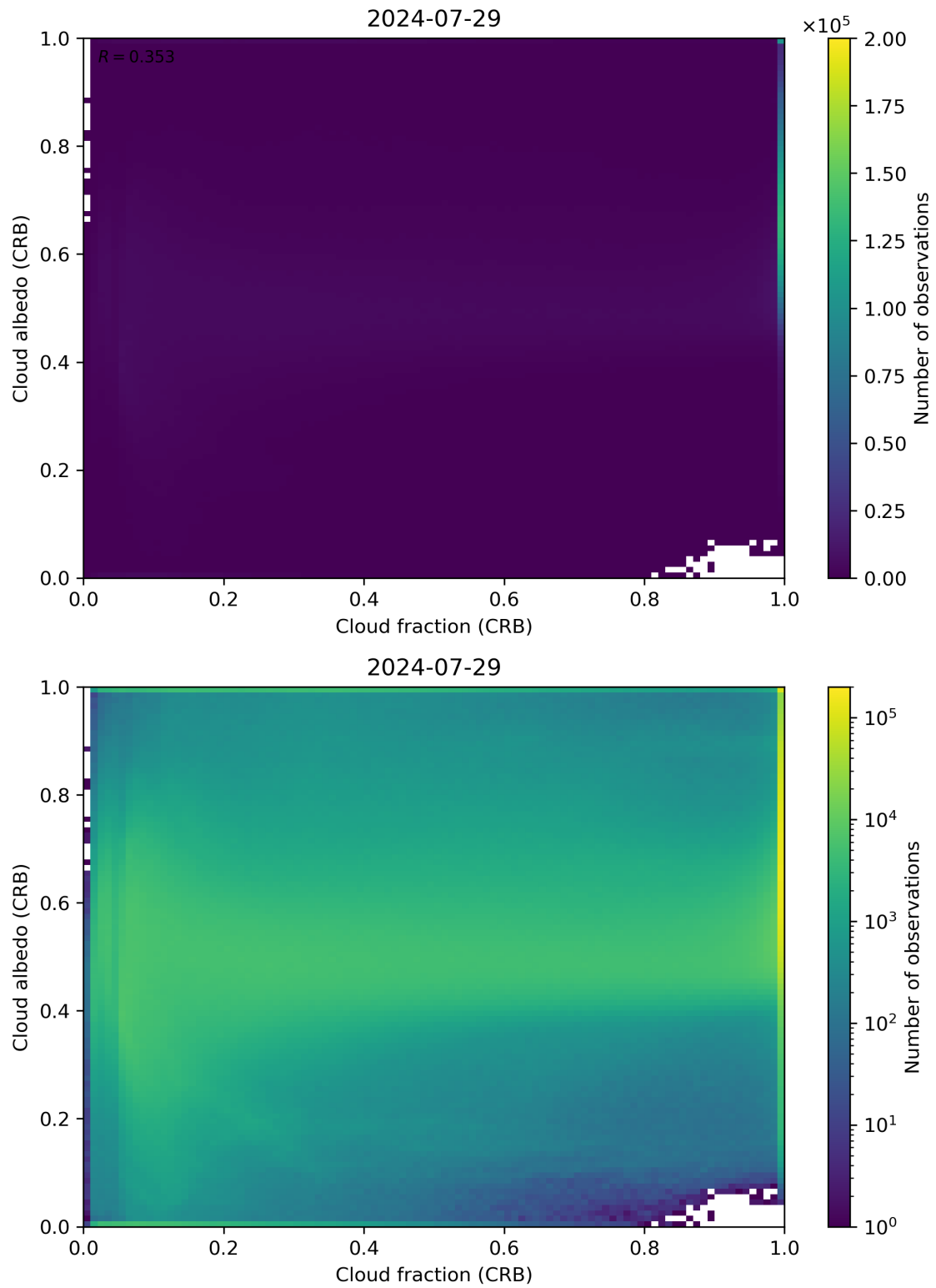
Figure 77: Scatter density plot of “Cloud fraction (CRB)” against “Cloud albedo (CRB)” for 2024-07-28 to 2024-07-30.
