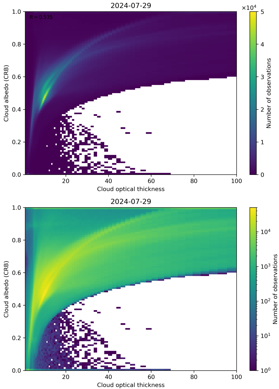
Figure 82: Scatter density plot of “Cloud optical thickness” against “Cloud albedo (CRB)” for 2024-07-28 to 2024-07-30.
