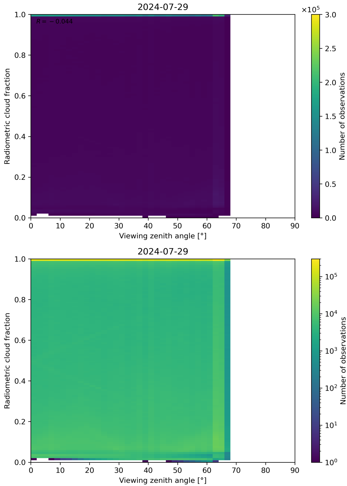
Figure 107: Scatter density plot of “Viewing zenith angle” against “Radiometric cloud fraction” for 2024-07-28 to 2024-07-30.
