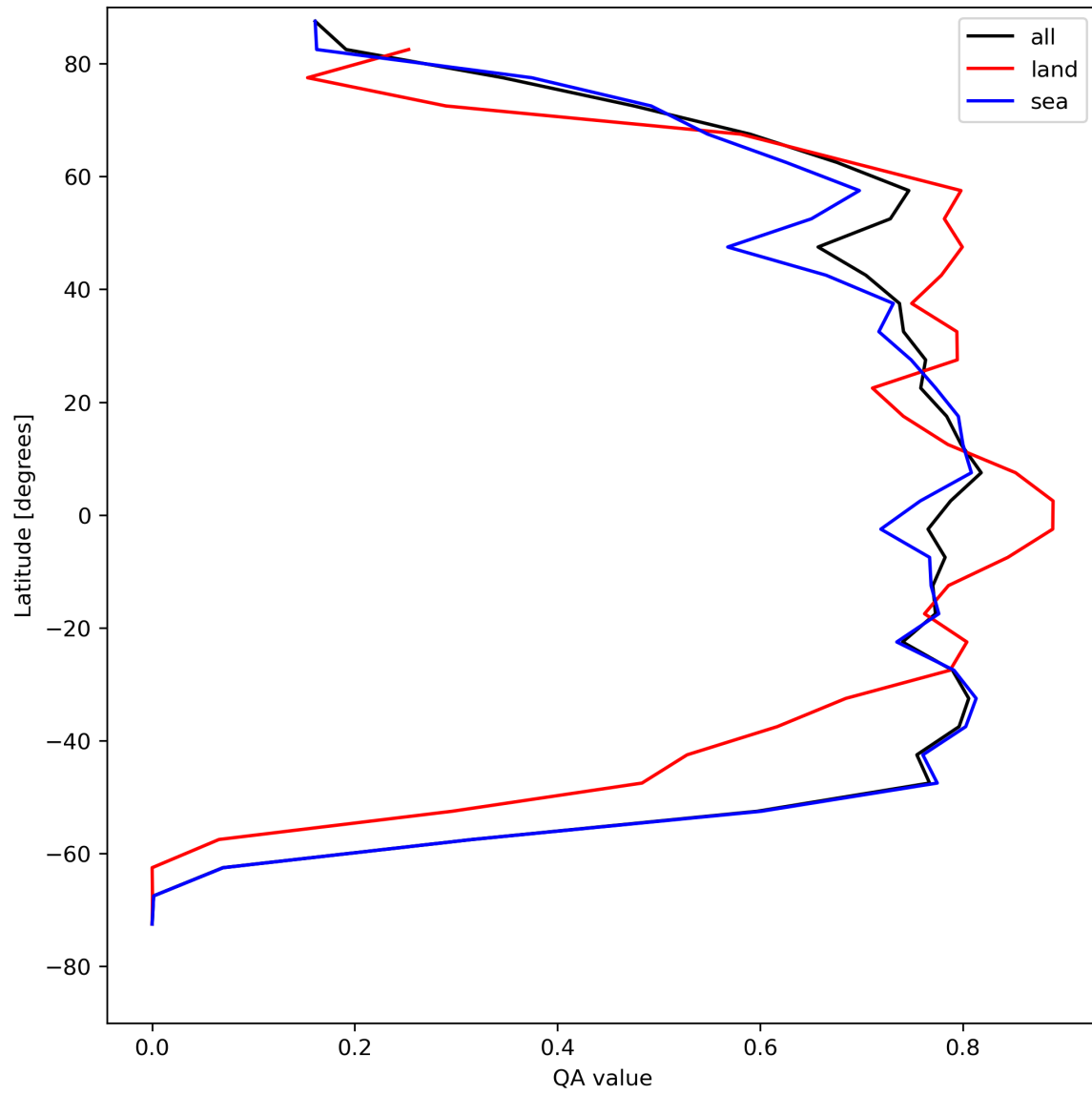
Figure 22: Zonal average of “QA value” for 2024-07-28 to 2024-07-30.
