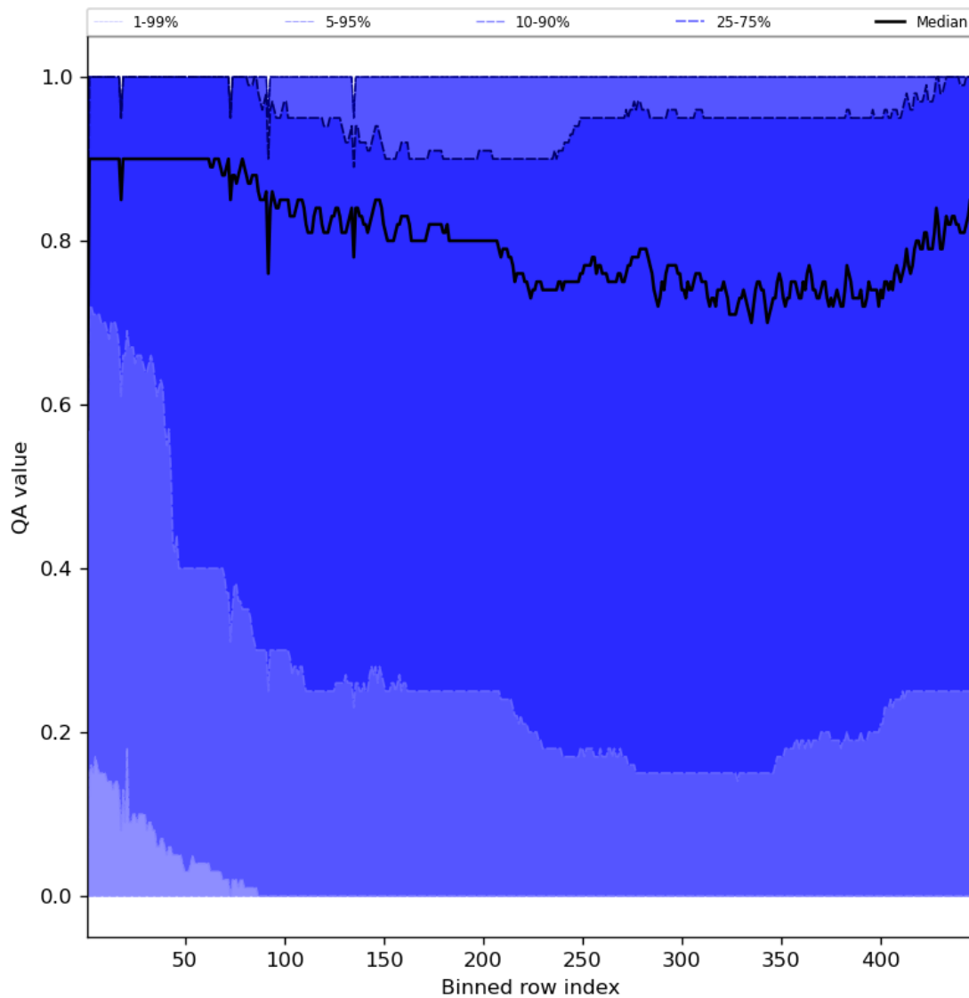
Figure 54: Along track statistics of “QA value” for 2024-07-28 to 2024-07-30
