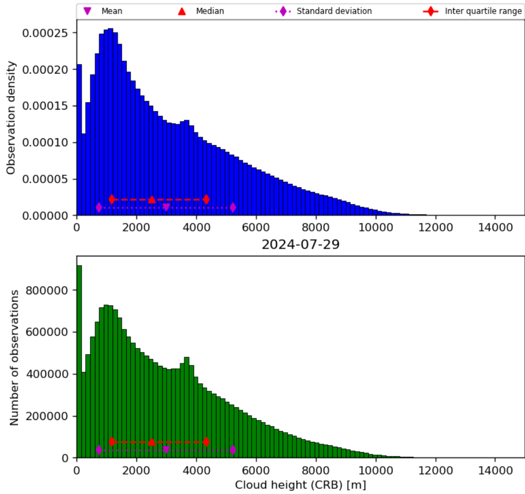
Figure 43: Histogram of “Cloud height (CRB)” for 2024-07-28 to 2024-07-30
