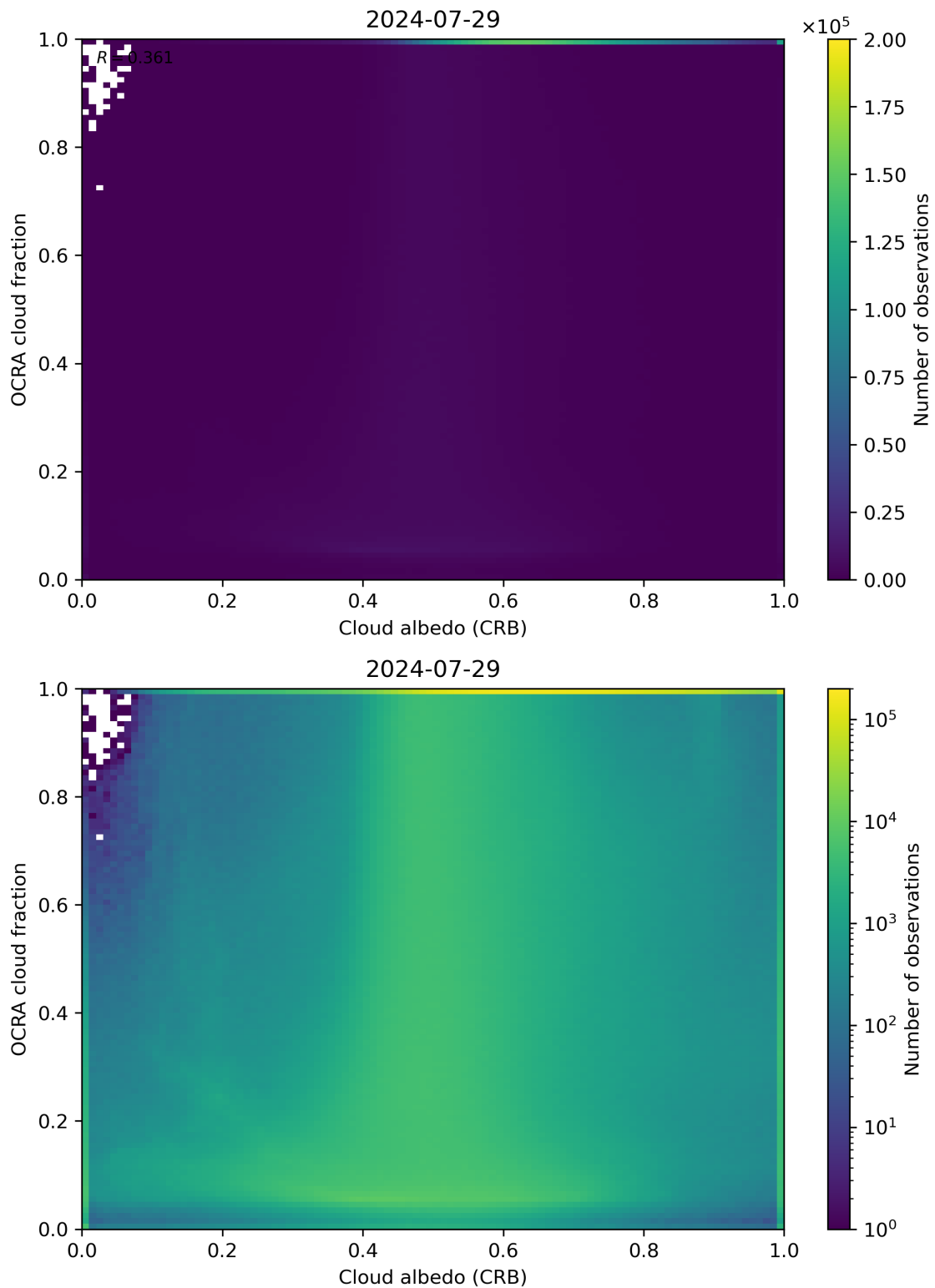
Figure 70: Scatter density plot of “Cloud albedo (CRB)” against “OCRA cloud fraction” for 2024-07-28 to 2024-07-30.
