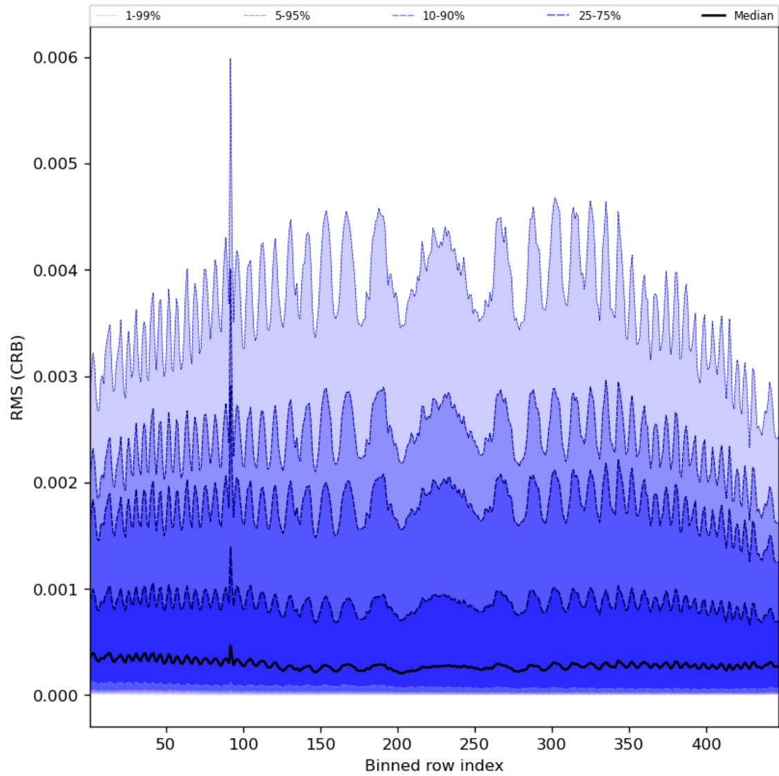
Figure 64: Along track statistics of “RMS (CRB)” for 2024-07-28 to 2024-07-30
