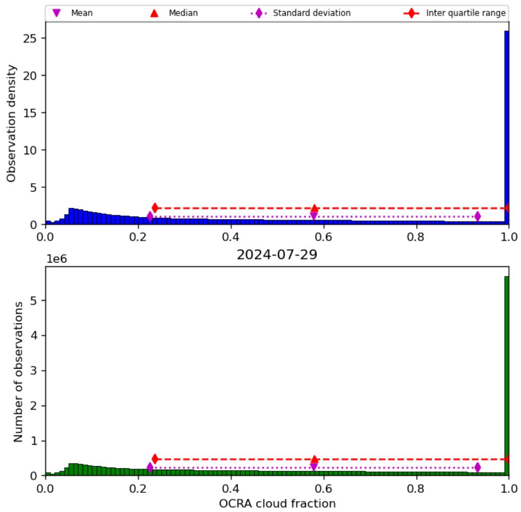
Figure 50: Histogram of “OCRA cloud fraction” for 2024-07-28 to 2024-07-30
