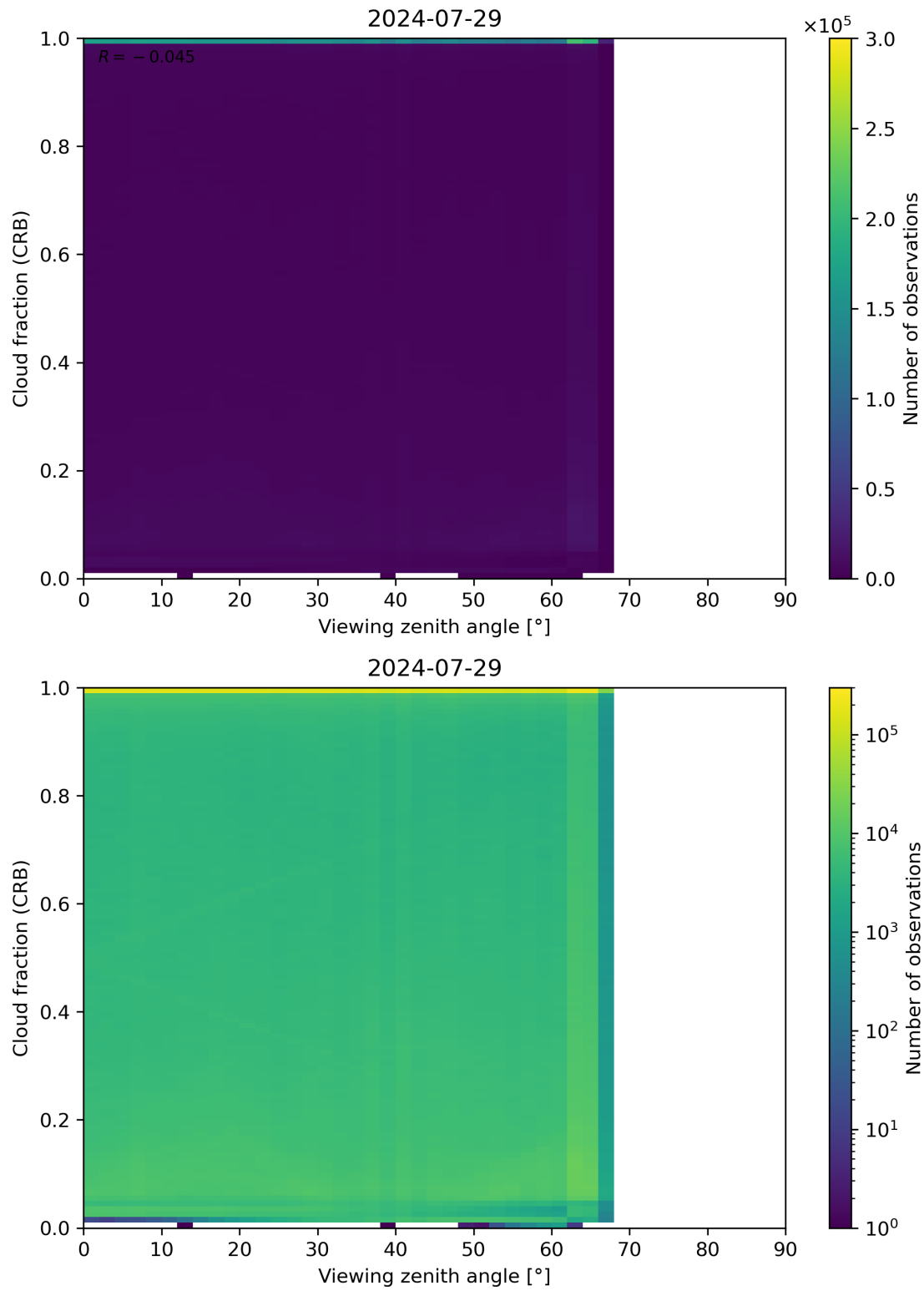
Figure 109: Scatter density plot of “Viewing zenith angle” against “Cloud fraction (CRB)” for 2024-07-28 to 2024-07-30.
