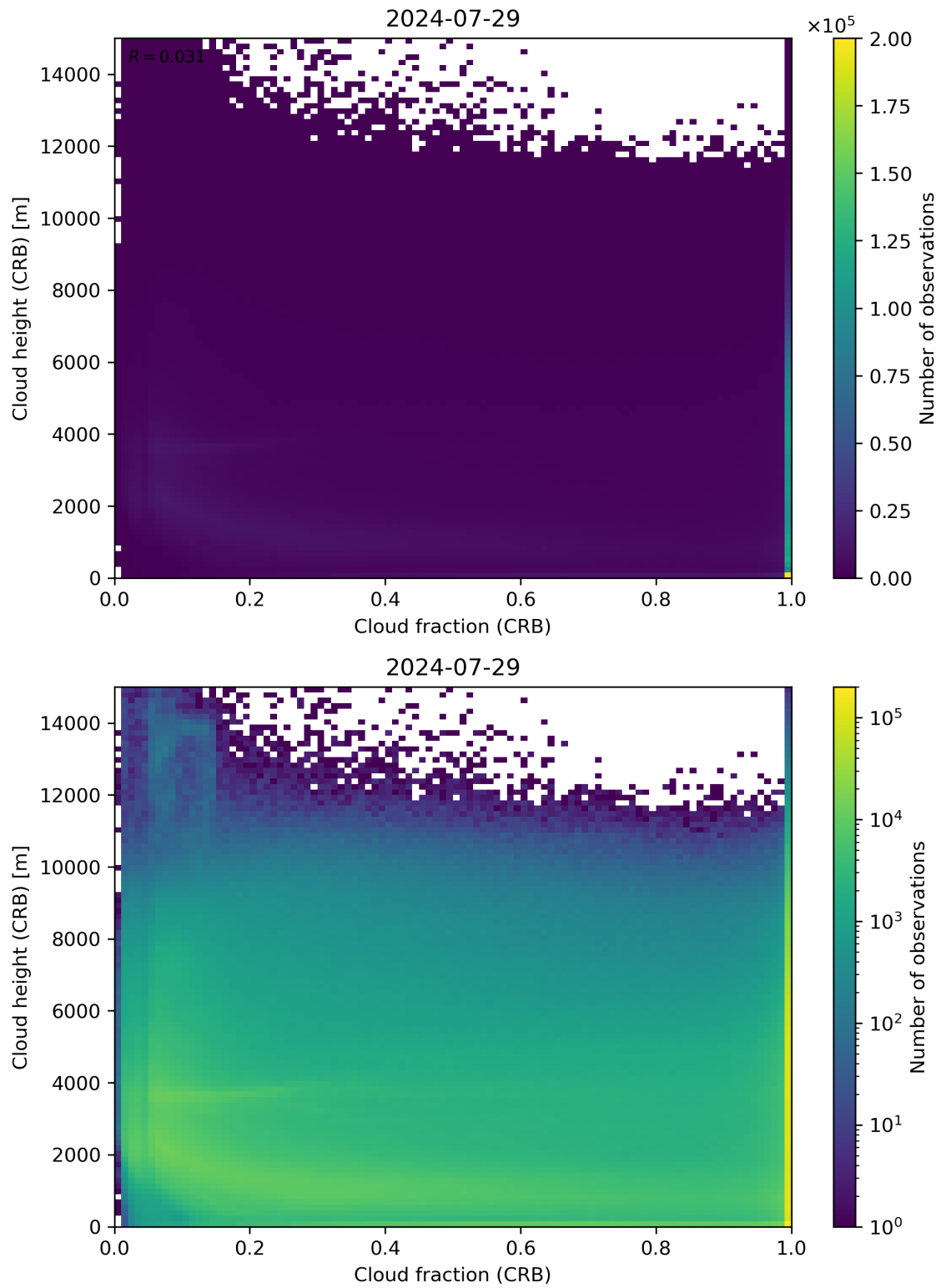
Figure 79: Scatter density plot of “Cloud fraction (CRB)” against “Cloud height (CRB)” for 2024-07-28 to 2024-07-30.
