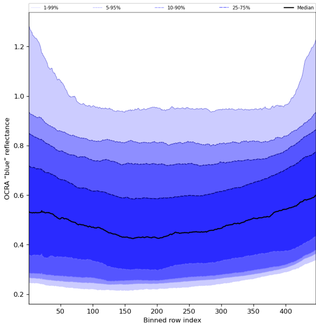
Figure 67: Along track statistics of “OCRA “blue” reflectance” for 2024-07-28 to 2024-07-30
