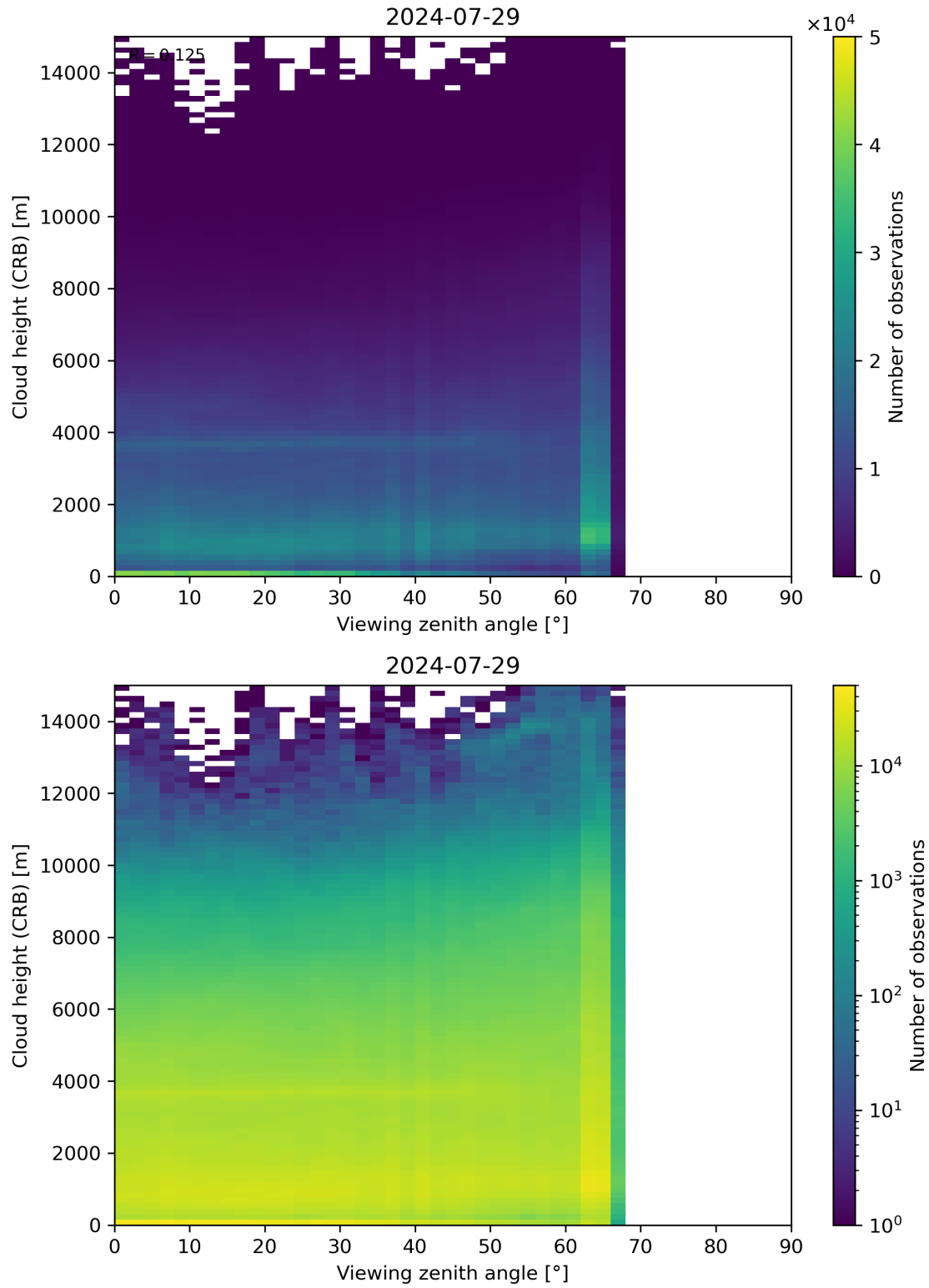
Figure 110: Scatter density plot of “Viewing zenith angle” against “Cloud height (CRB)” for 2024-07-28 to 2024-07-30.
