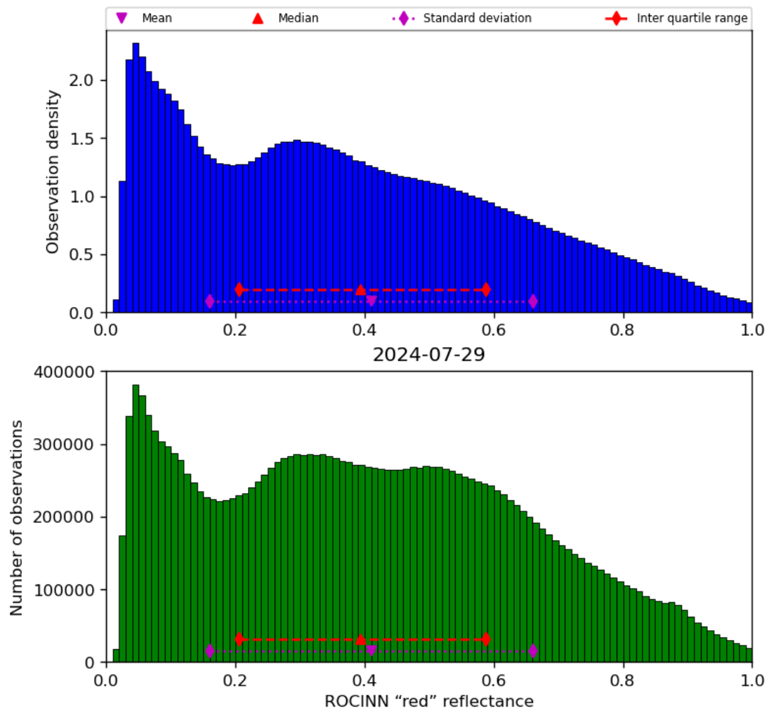
Figure 53: Histogram of “ROCINN “red” reflectance” for 2024-07-28 to 2024-07-30
