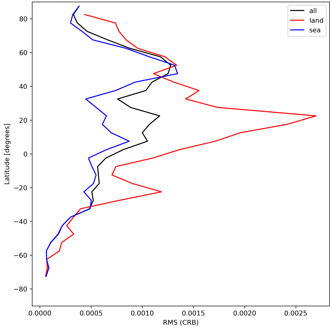
Figure 32: Zonal average of “RMS (CRB)” for 2024-07-28 to 2024-07-30.
