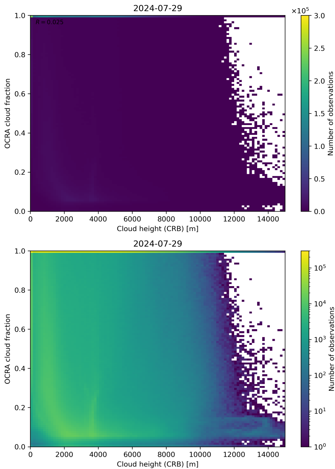
Figure 81: Scatter density plot of “Cloud height (CRB)” against “OCRA cloud fraction” for 2024-07-28 to 2024-07-30.
