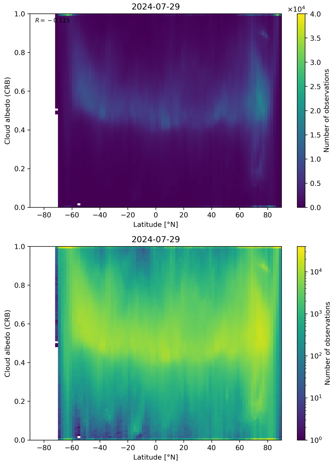
Figure 91: Scatter density plot of “Latitude” against “Cloud albedo (CRB)” for 2024-07-28 to 2024-07-30.
