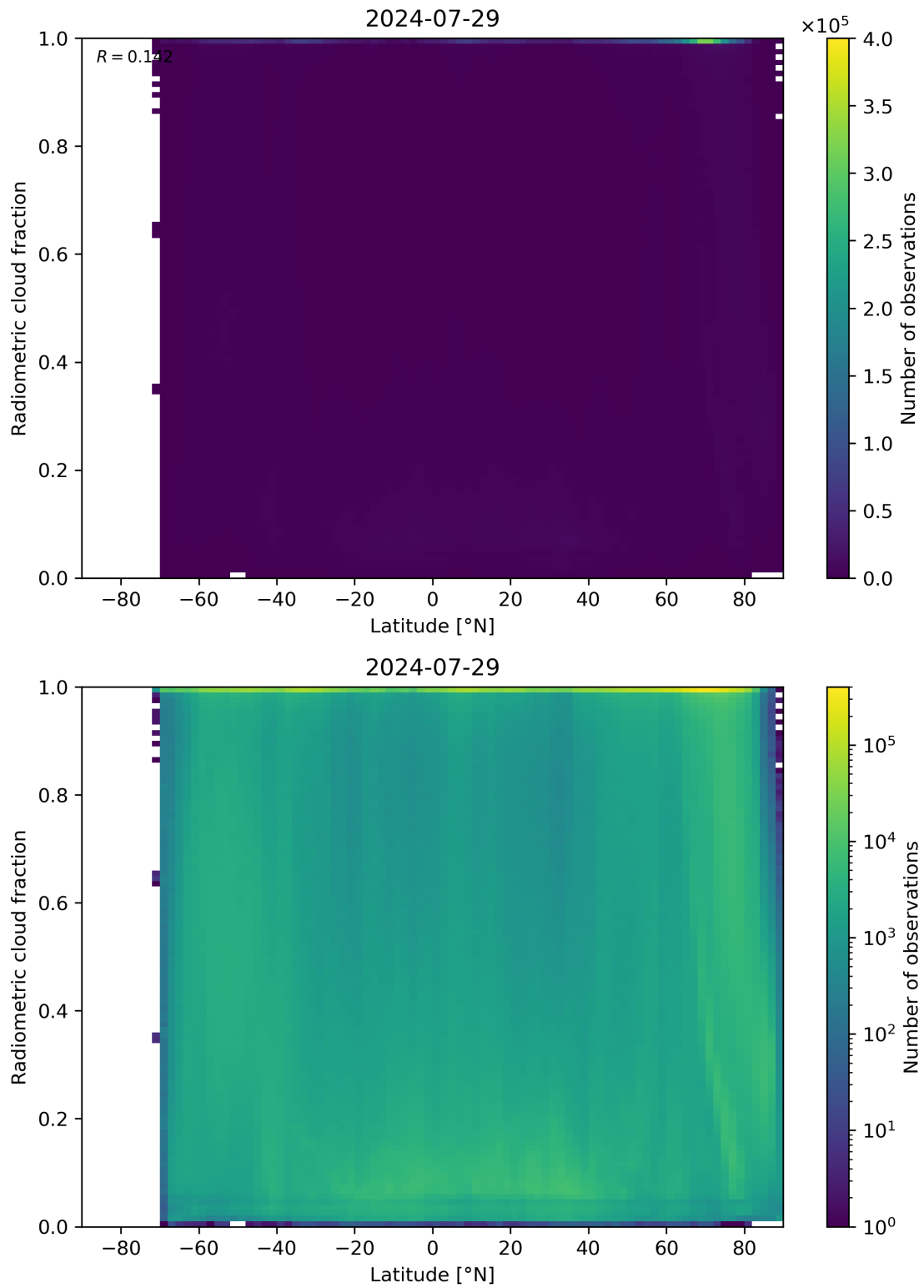
Figure 92: Scatter density plot of “Latitude” against “Radiometric cloud fraction” for 2024-07-28 to 2024-07-30.
