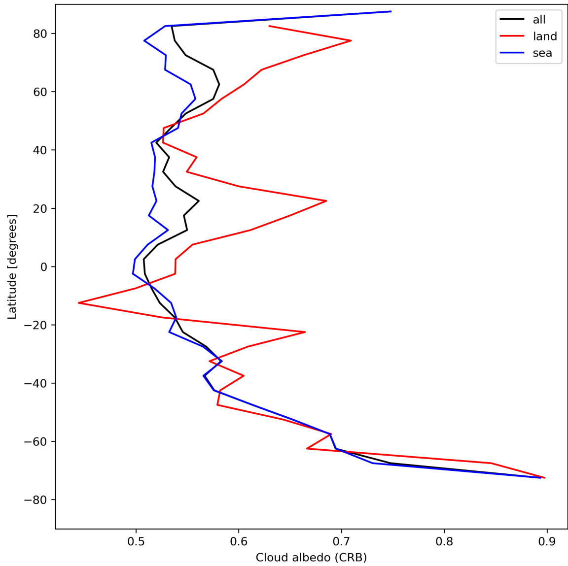
Figure 28: Zonal average of “Cloud albedo (CRB)” for 2024-07-28 to 2024-07-30.
