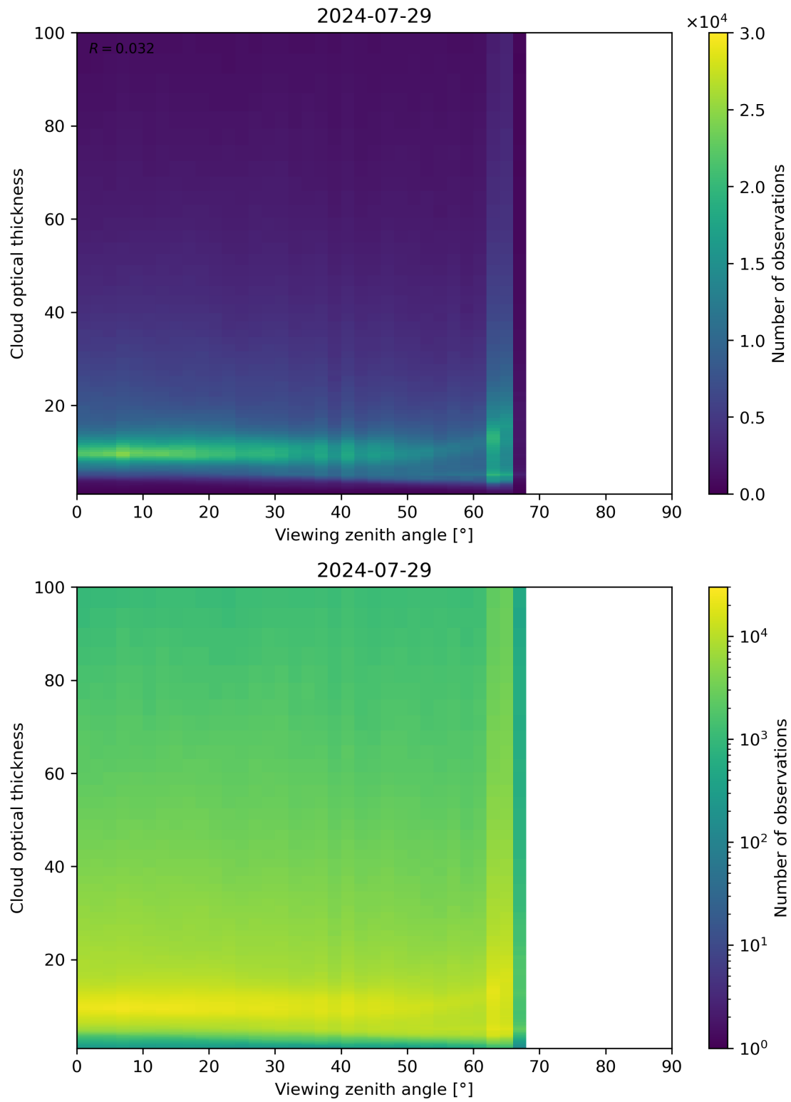
Figure 111: Scatter density plot of “Viewing zenith angle” against “Cloud optical thickness” for 2024-07-28 to 2024-07-30.
