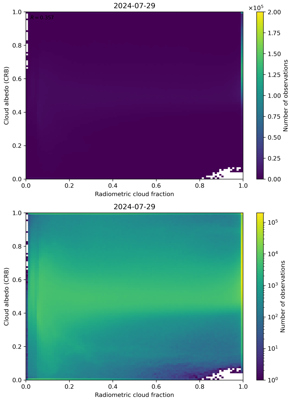
Figure 71: Scatter density plot of “Radiometric cloud fraction” against “Cloud albedo (CRB)” for 2024-07-28 to 2024-07-30.
