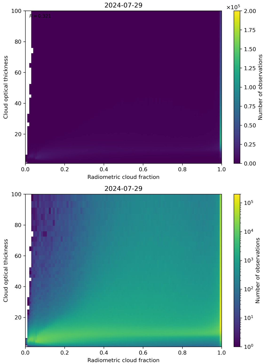
Figure 75: Scatter density plot of “Radiometric cloud fraction” against “Cloud optical thickness” for 2024-07-28 to 2024-07-30.
