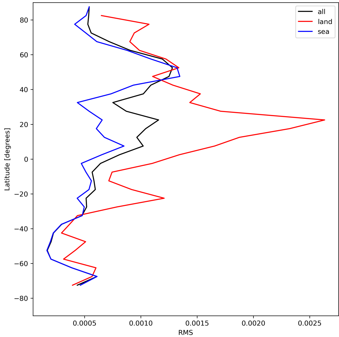
Figure 31: Zonal average of “RMS” for 2024-07-28 to 2024-07-30.
