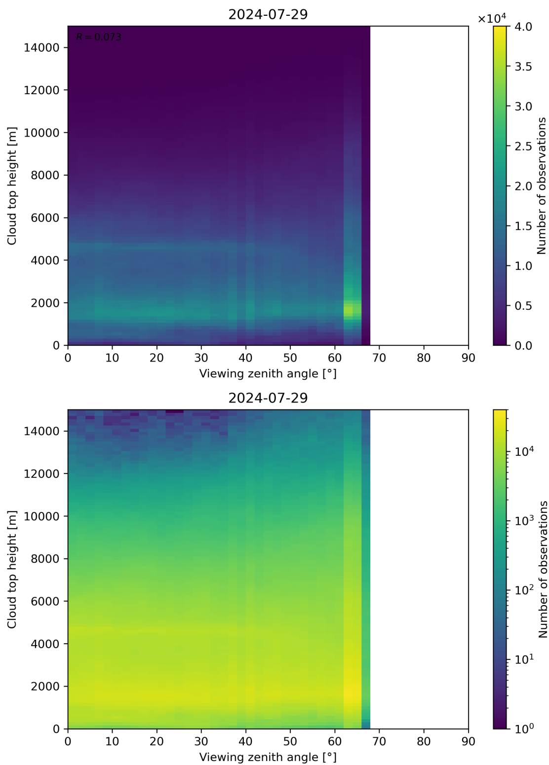
Figure 112: Scatter density plot of “Viewing zenith angle” against “Cloud top height” for 2024-07-28 to 2024-07-30.
