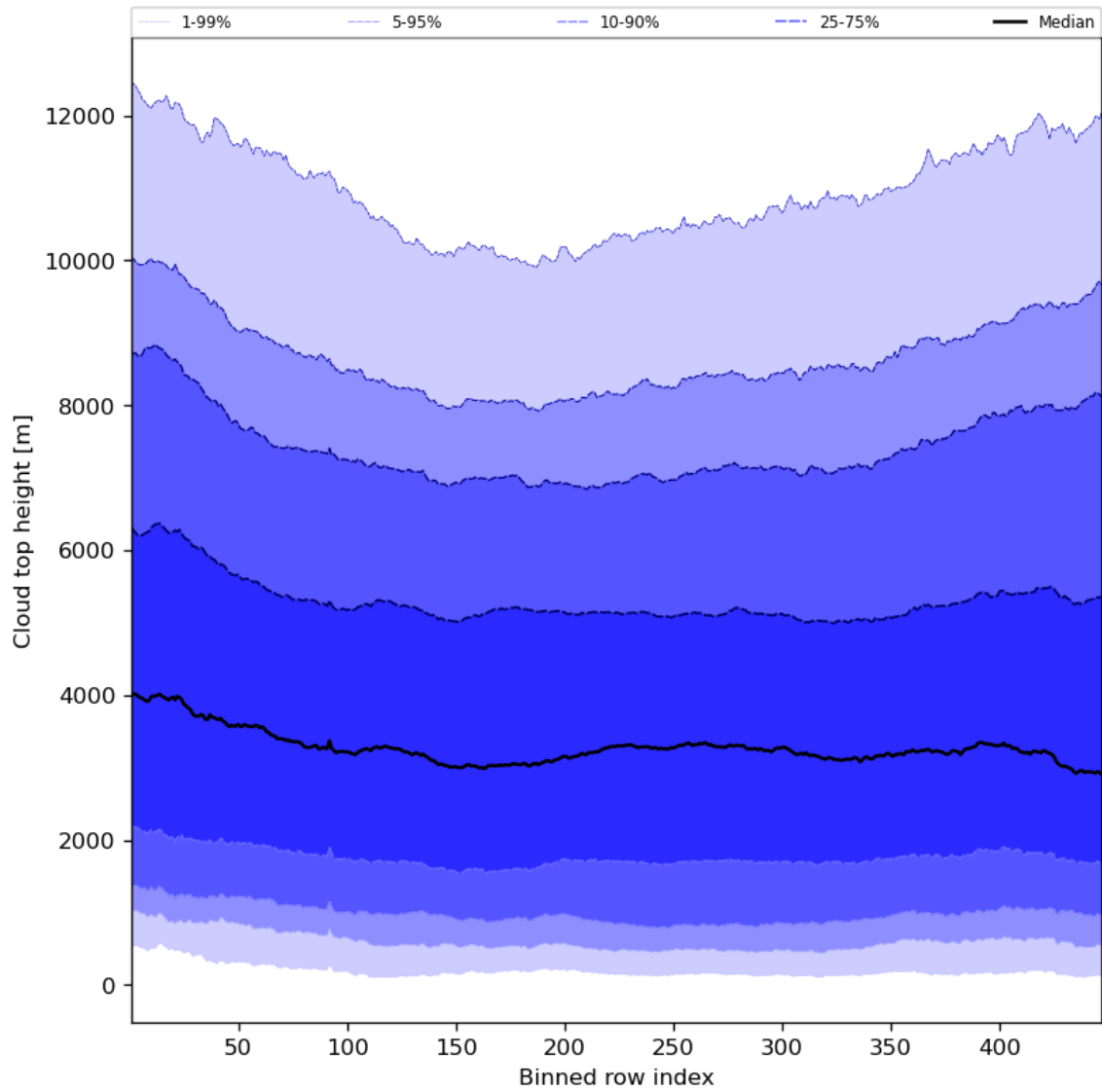
Figure 56: Along track statistics of “Cloud top height” for 2024-07-28 to 2024-07-30
