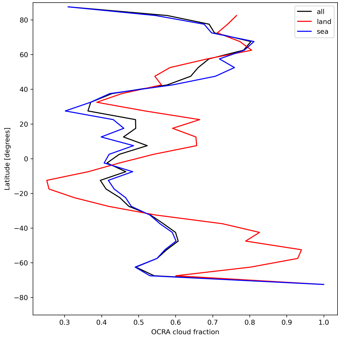
Figure 34: Zonal average of “OCRA cloud fraction” for 2024-07-31 to 2024-08-01.
