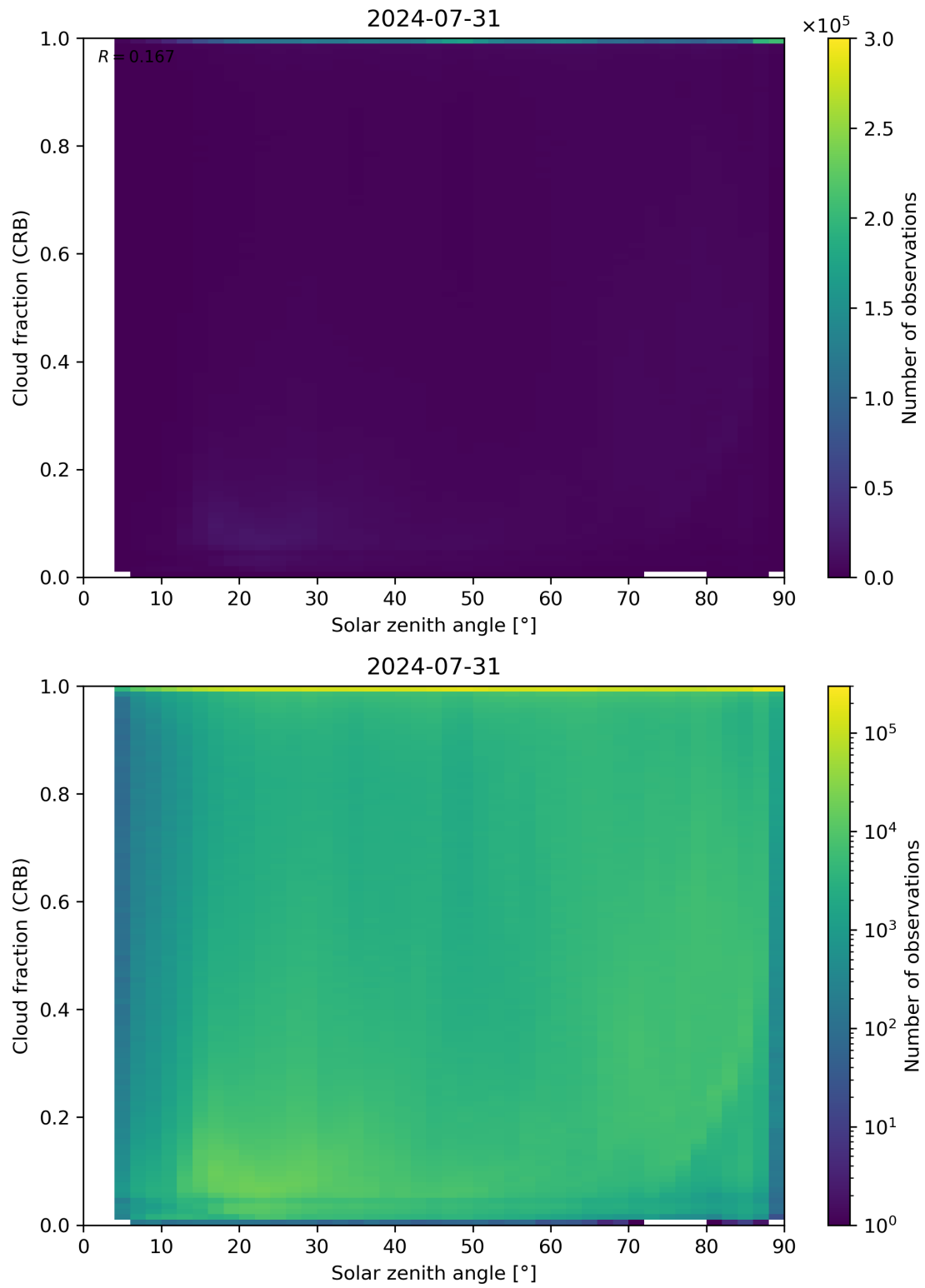
Figure 101: Scatter density plot of “Solar zenith angle” against “Cloud fraction (CRB)” for 2024-07-31 to 2024-08-01.
