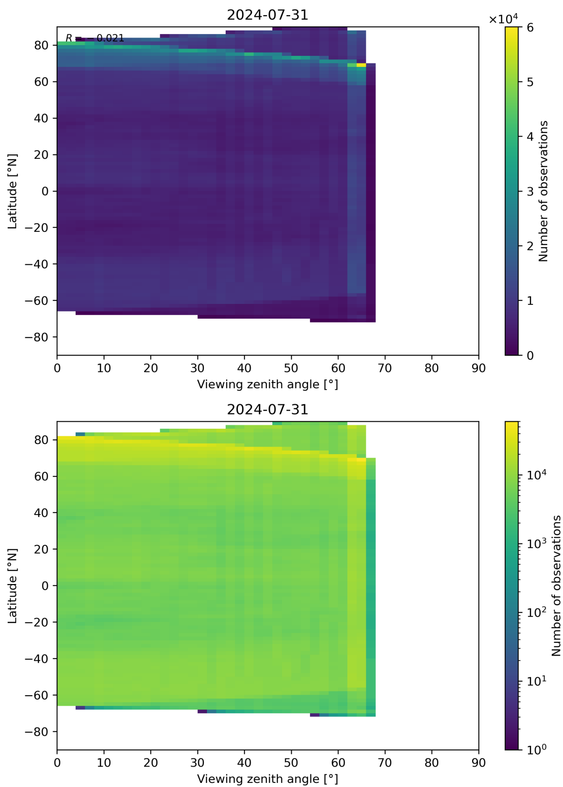
Figure 113: Scatter density plot of “Viewing zenith angle” against “Latitude” for 2024-07-31 to 2024-08-01.
