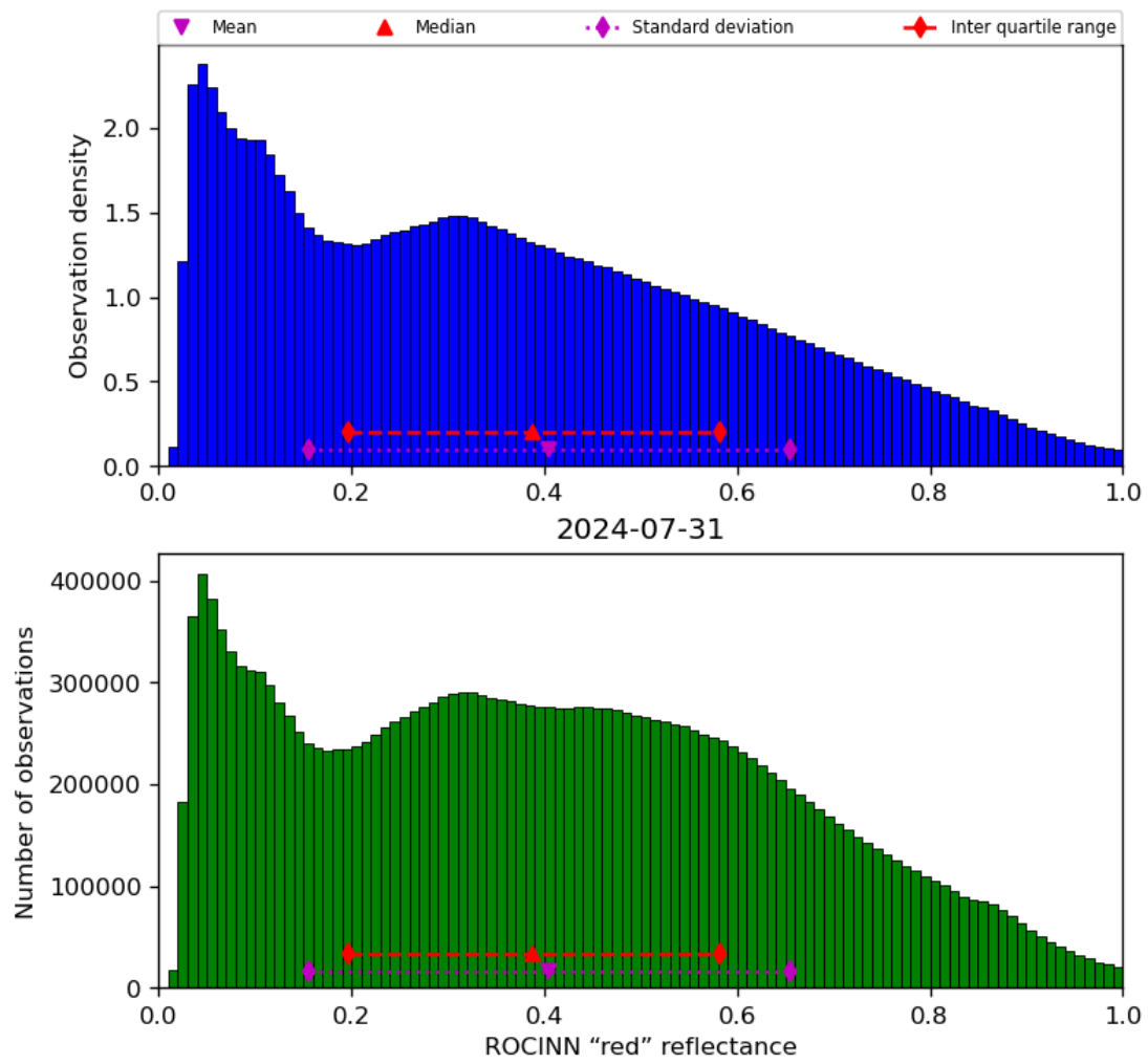
Figure 53: Histogram of “ROCINN “red” reflectance” for 2024-07-31 to 2024-08-01
