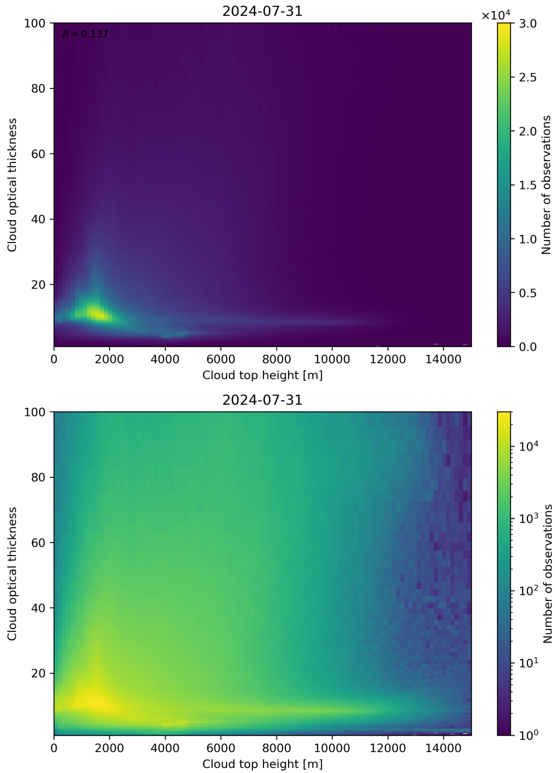
Figure 90: Scatter density plot of “Cloud top height” against “Cloud optical thickness” for 2024-07-31 to 2024-08-01.
