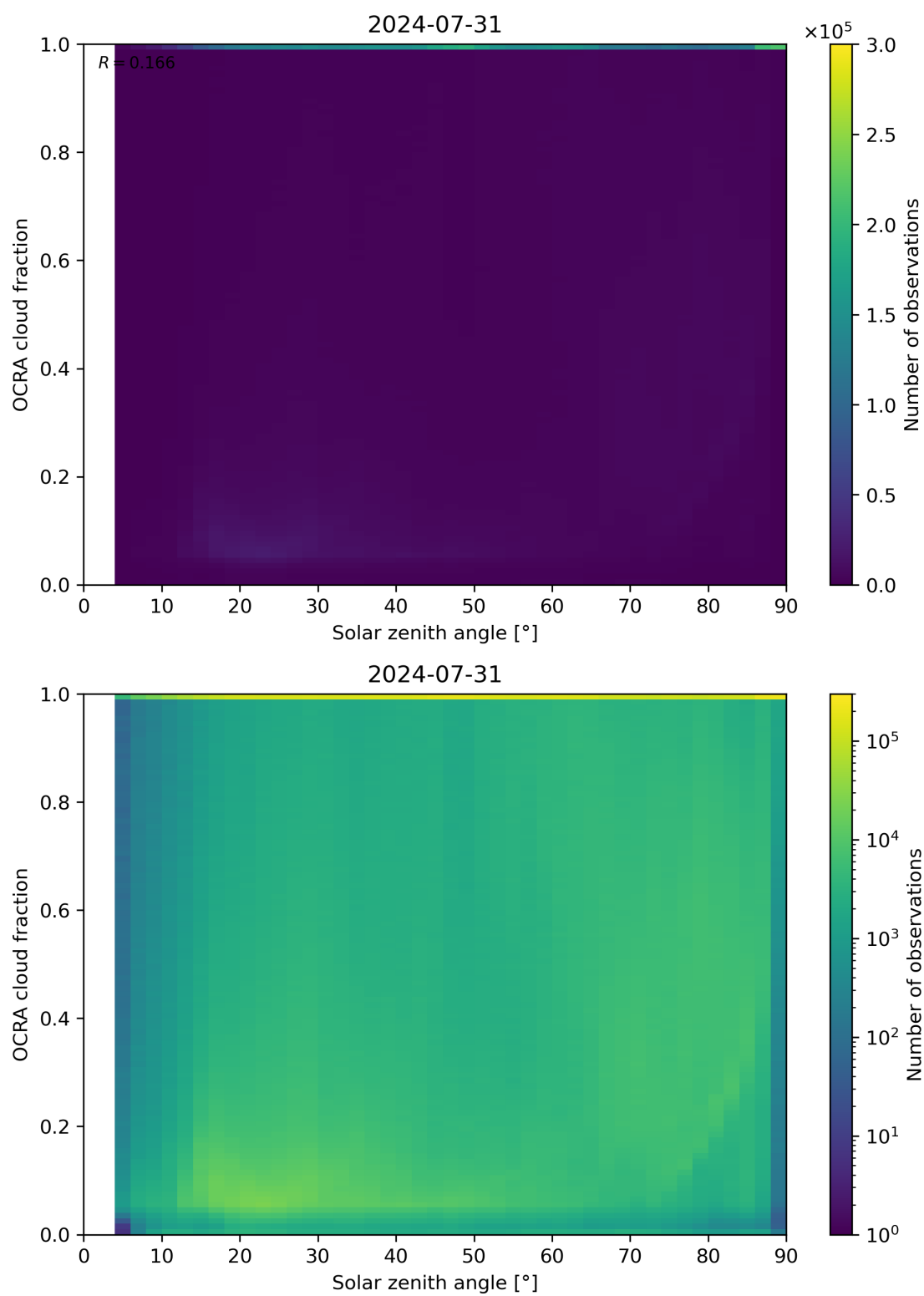
Figure 100: Scatter density plot of “Solar zenith angle” against “OCRA cloud fraction” for 2024-07-31 to 2024-08-01.
