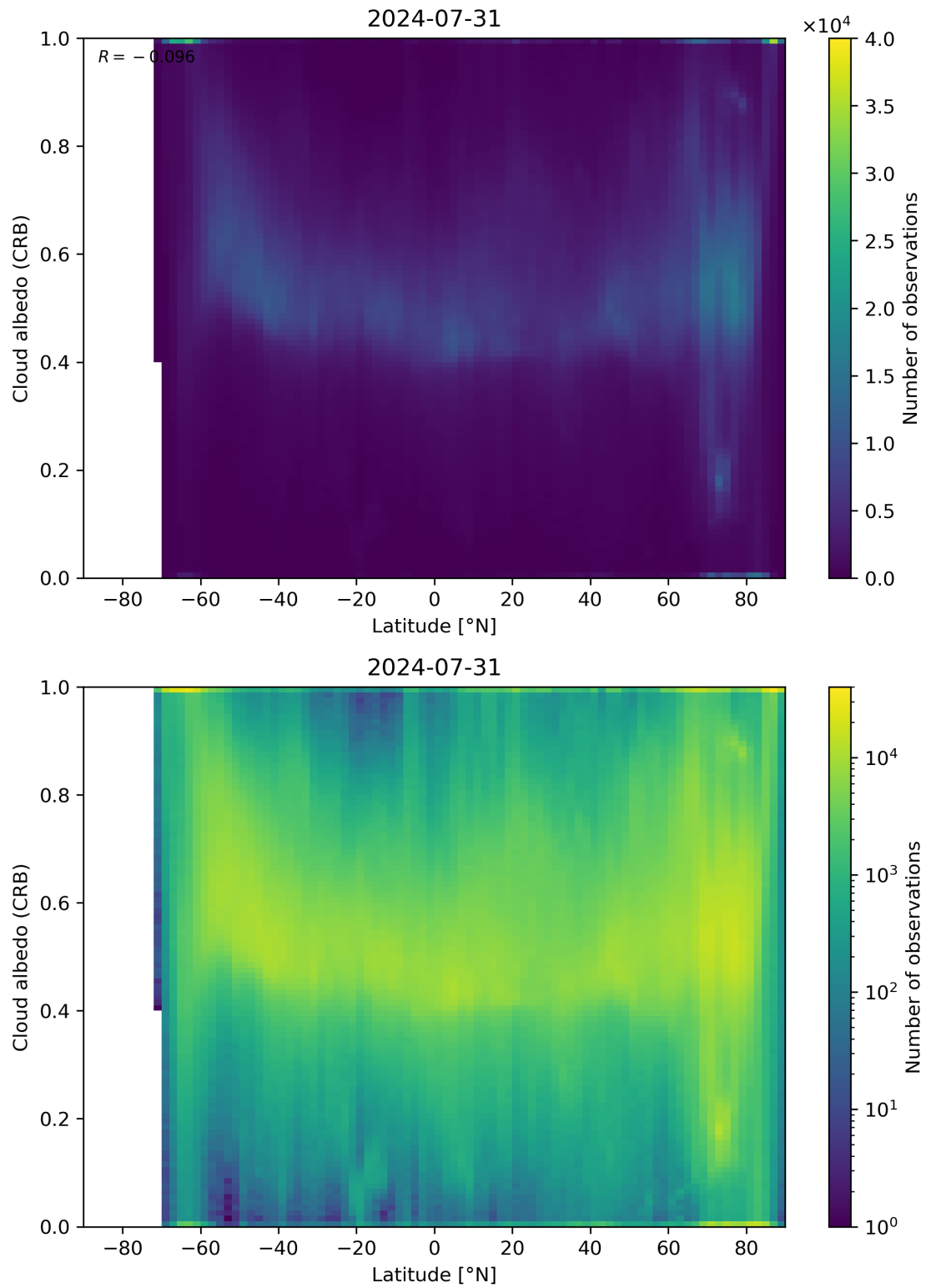
Figure 91: Scatter density plot of “Latitude” against “Cloud albedo (CRB)” for 2024-07-31 to 2024-08-01.
