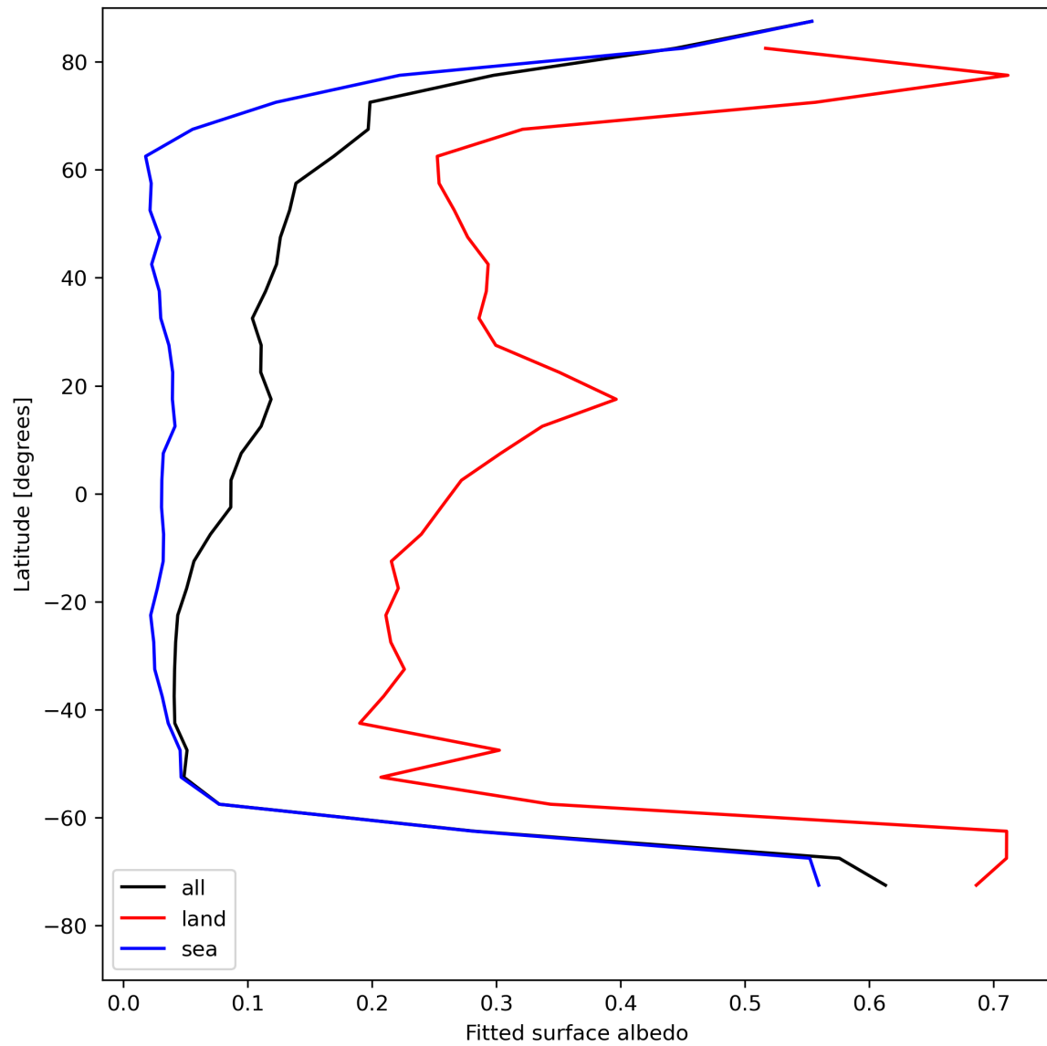
Figure 29: Zonal average of “Fitted surface albedo” for 2024-07-31 to 2024-08-01.
