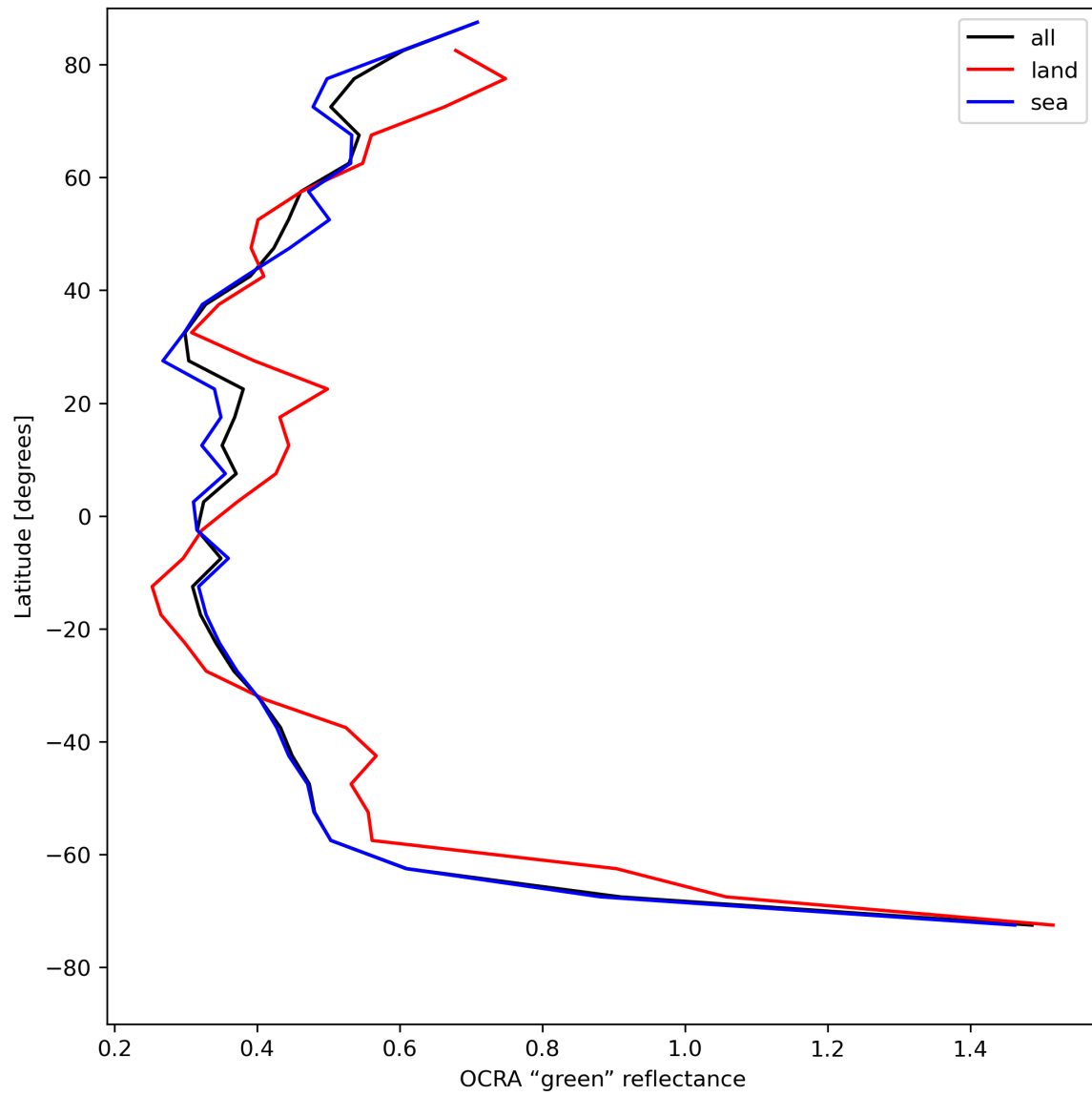
Figure 36: Zonal average of “OCRA “green” reflectance” for 2024-07-31 to 2024-08-01.
