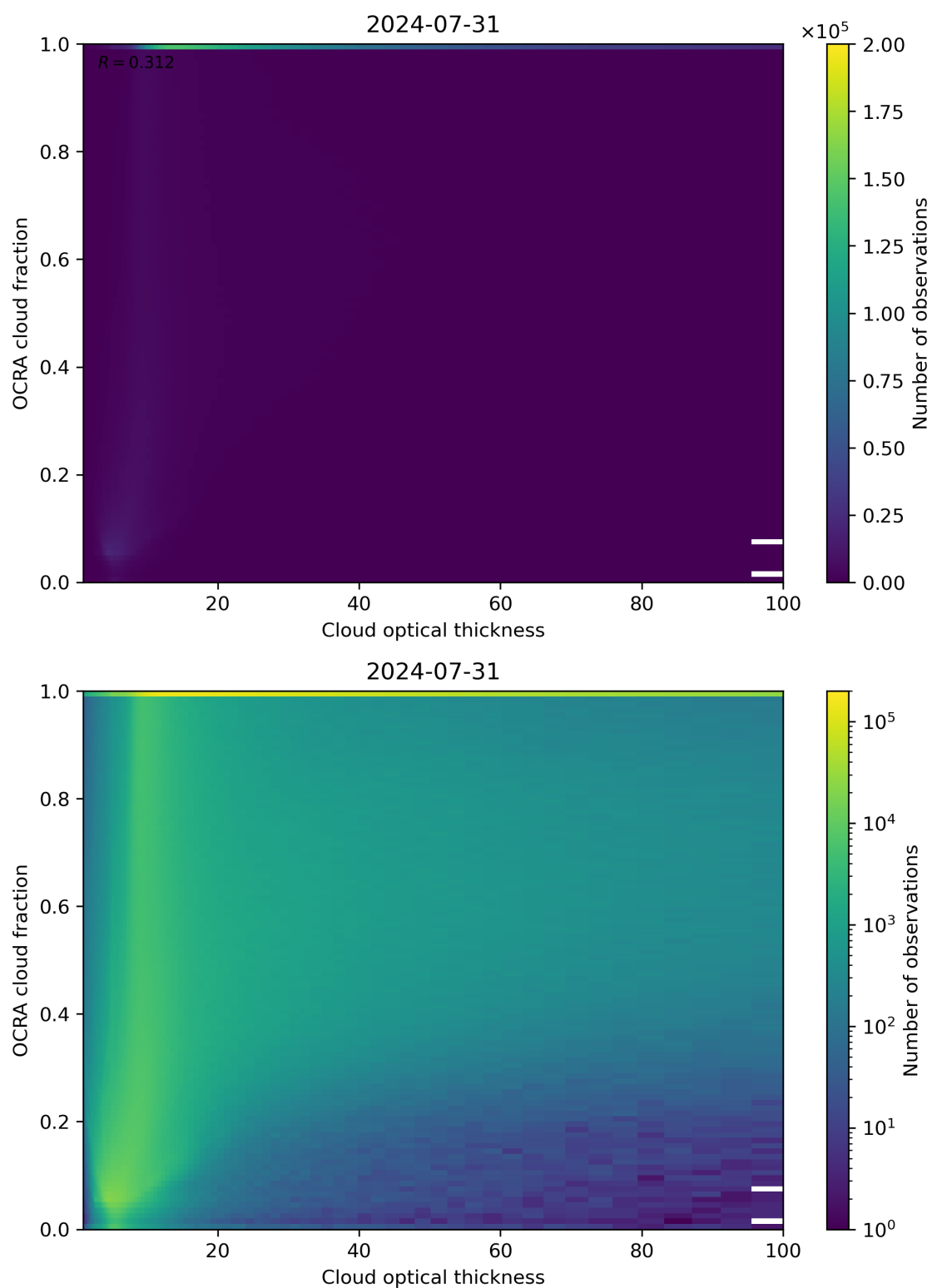
Figure 83: Scatter density plot of “Cloud optical thickness” against “OCRA cloud fraction” for 2024-07-31 to 2024-08-01.
