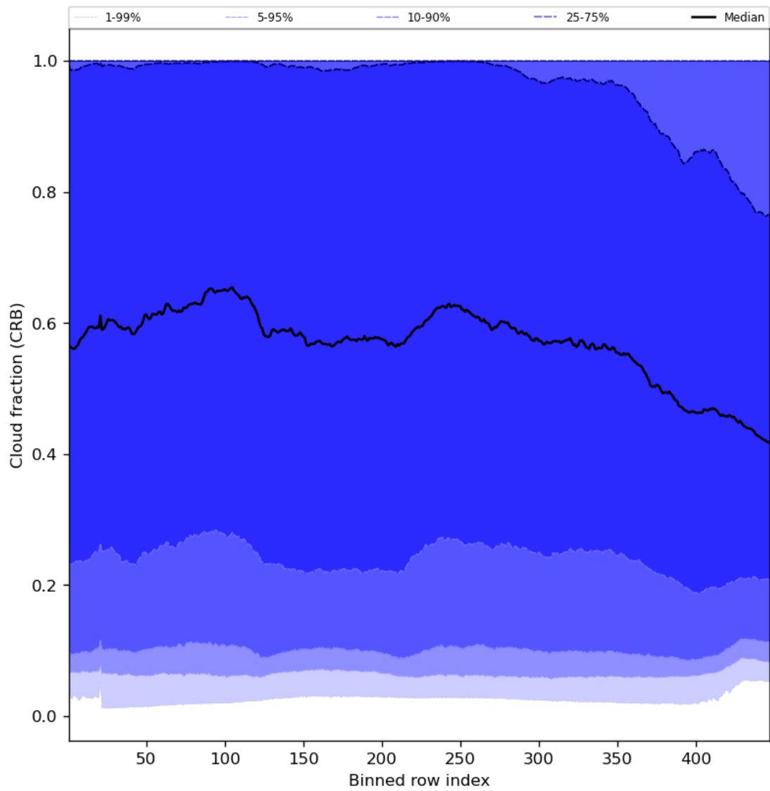
Figure 58: Along track statistics of “Cloud fraction (CRB)” for 2024-07-31 to 2024-08-01
