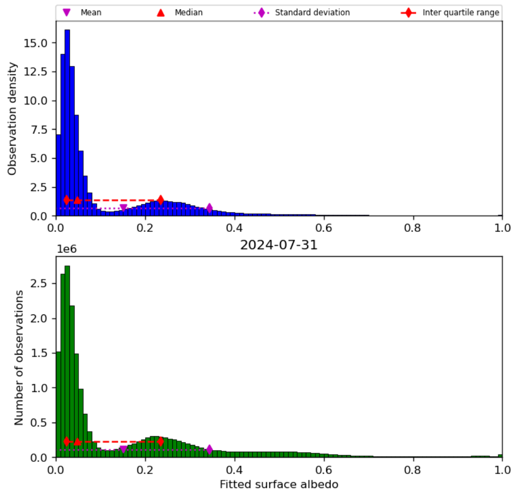
Figure 45: Histogram of “Fitted surface albedo” for 2024-07-31 to 2024-08-01
