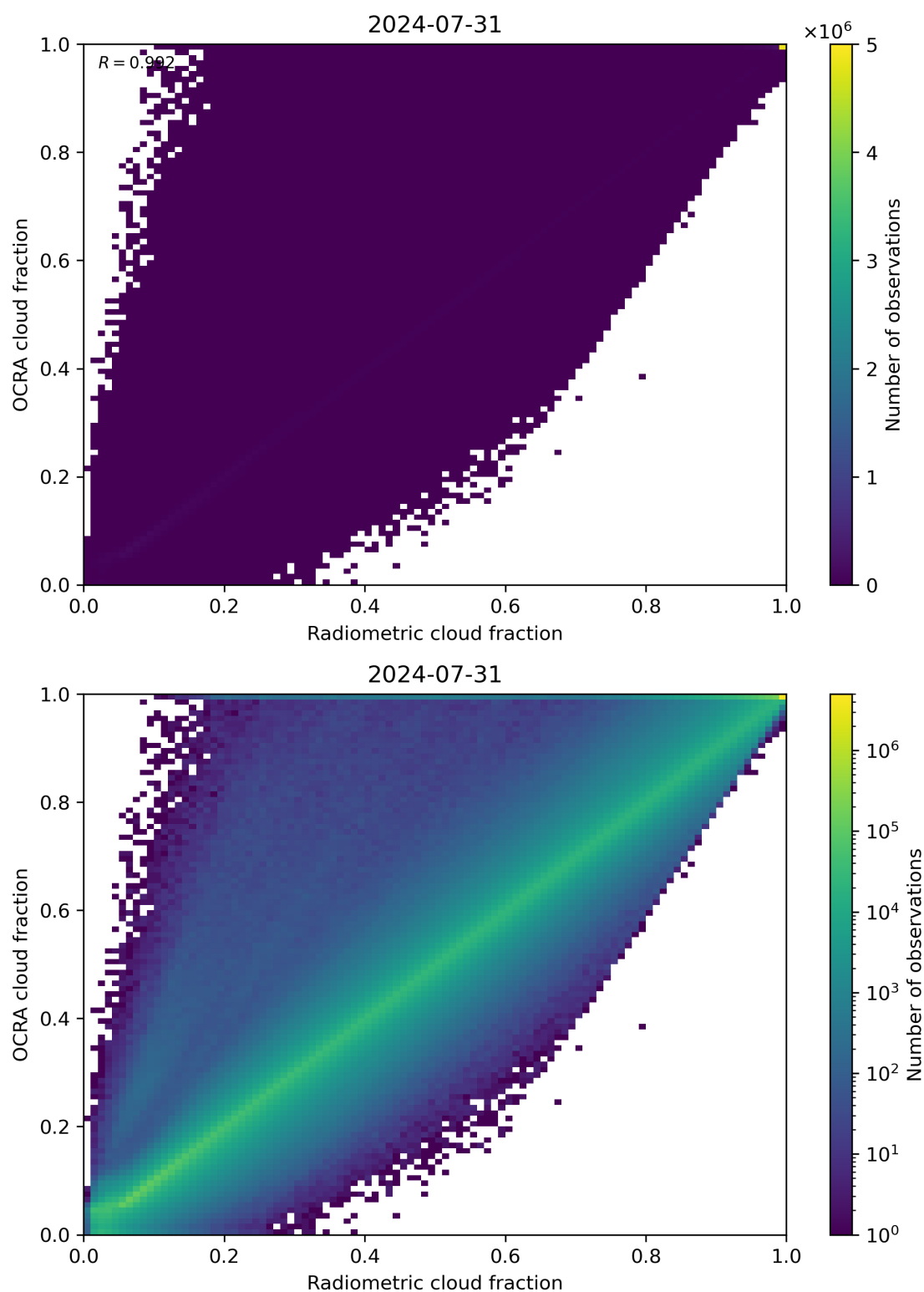
Figure 72: Scatter density plot of “Radiometric cloud fraction” against “OCRA cloud fraction” for 2024-07-31 to 2024-08-01.
