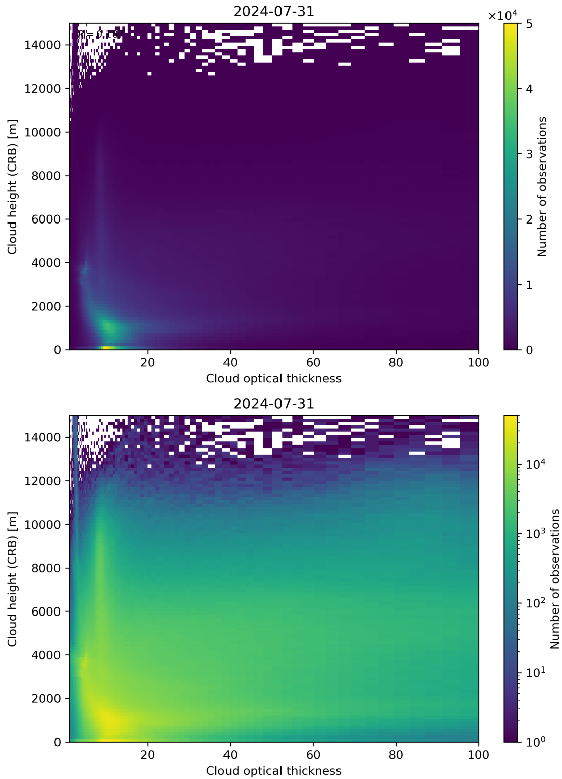
Figure 85: Scatter density plot of “Cloud optical thickness” against “Cloud height (CRB)” for 2024-07-31 to 2024-08-01.
