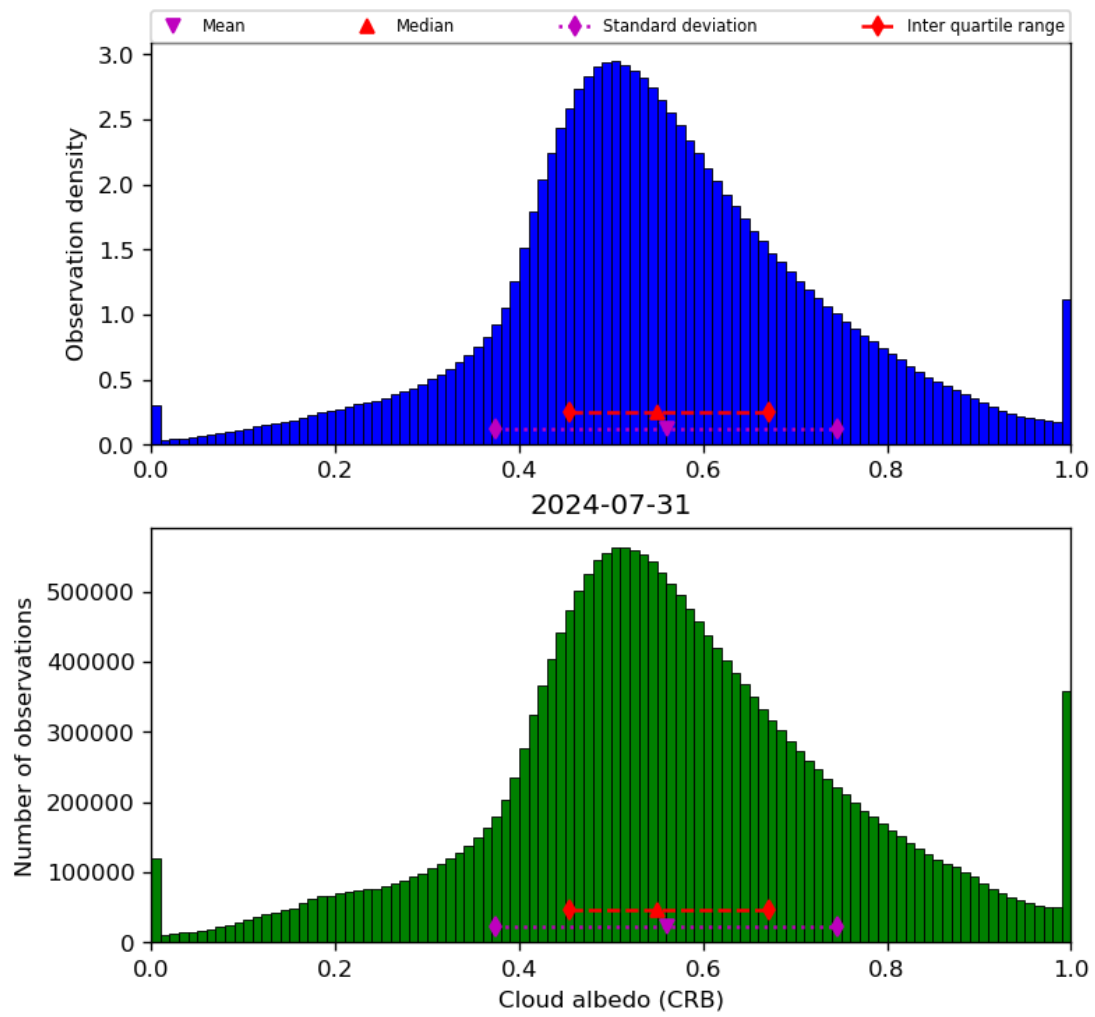
Figure 44: Histogram of “Cloud albedo (CRB)” for 2024-07-31 to 2024-08-01
