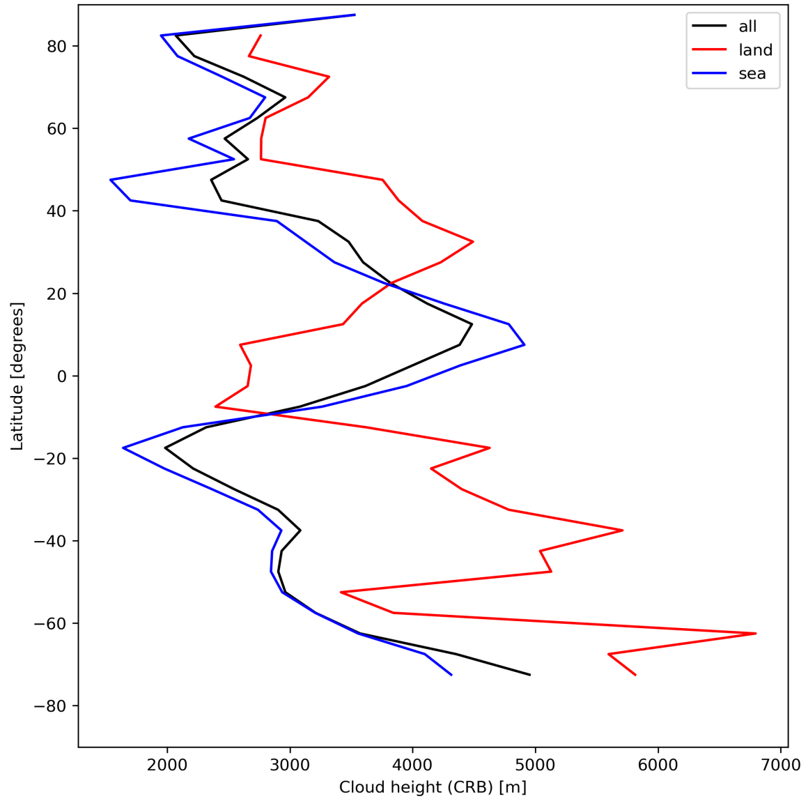
Figure 27: Zonal average of “Cloud height (CRB)” for 2024-07-31 to 2024-08-01.
