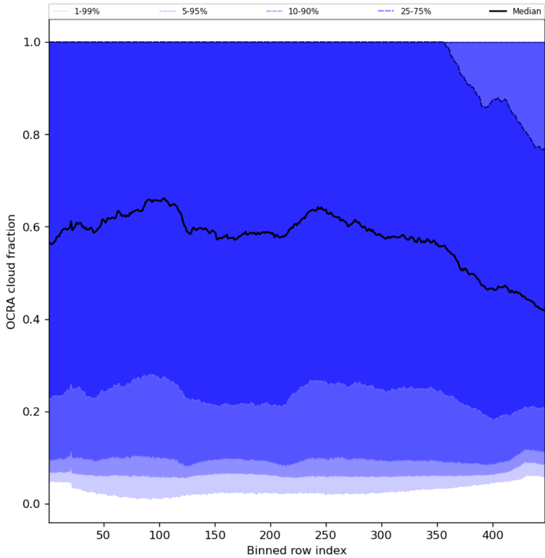
Figure 66: Along track statistics of “OCRA cloud fraction” for 2024-07-31 to 2024-08-01
