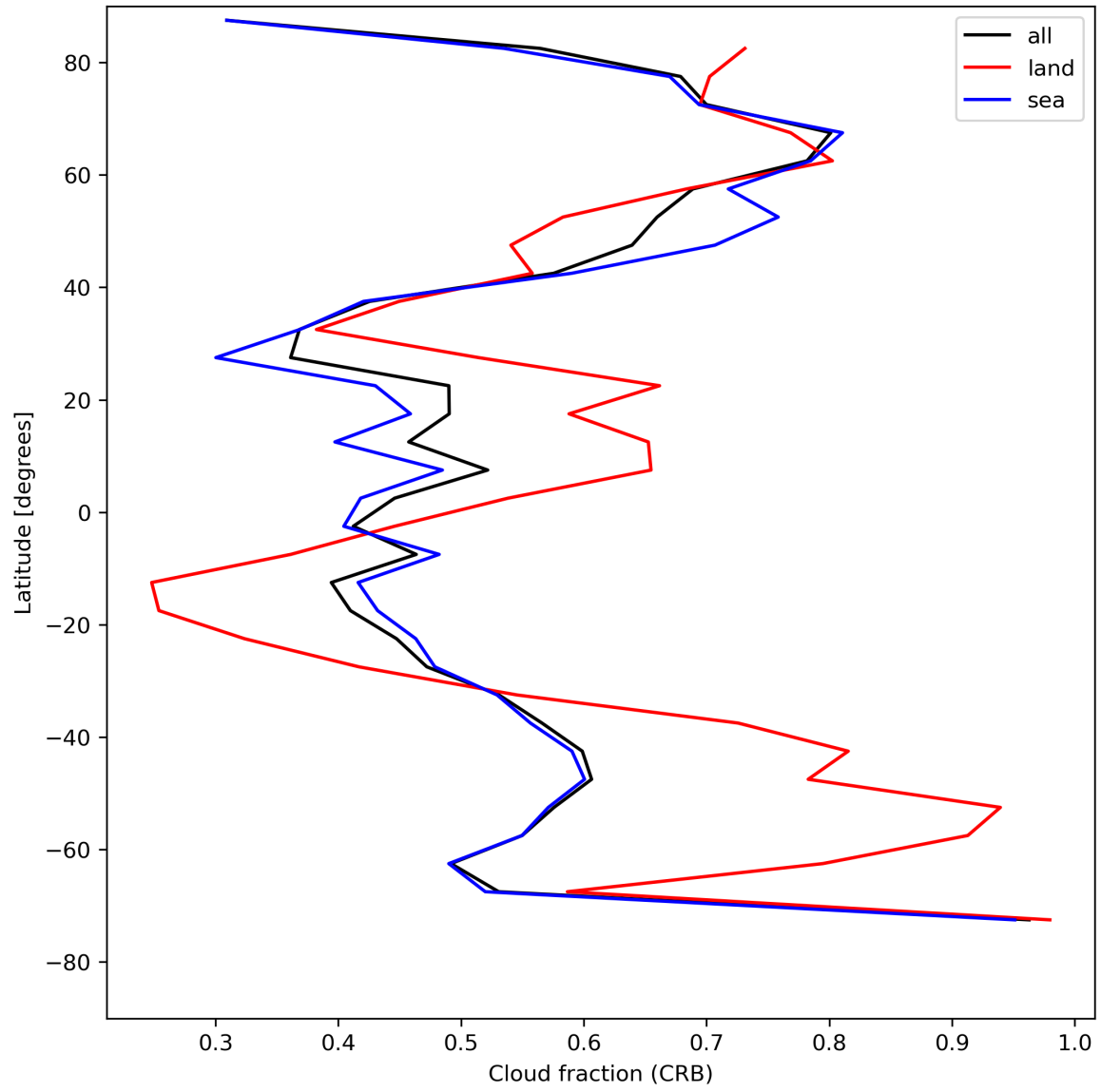
Figure 26: Zonal average of “Cloud fraction (CRB)” for 2024-07-31 to 2024-08-01.
