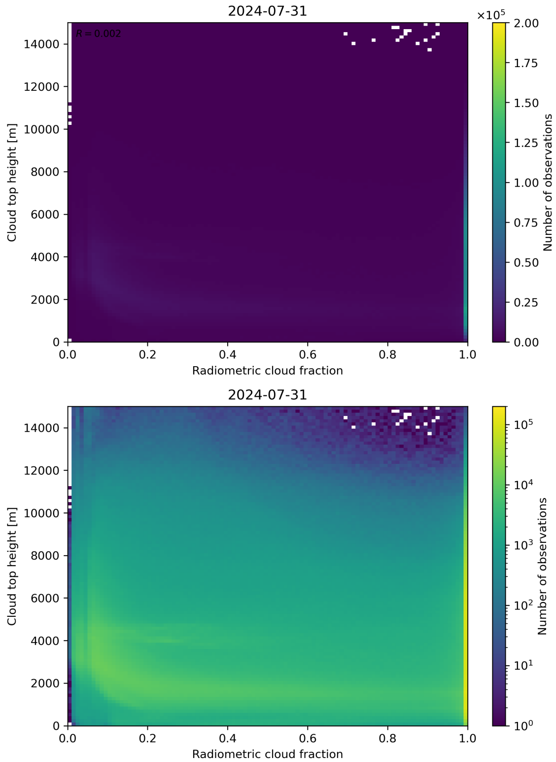
Figure 76: Scatter density plot of “Radiometric cloud fraction” against “Cloud top height” for 2024-07-31 to 2024-08-01.
