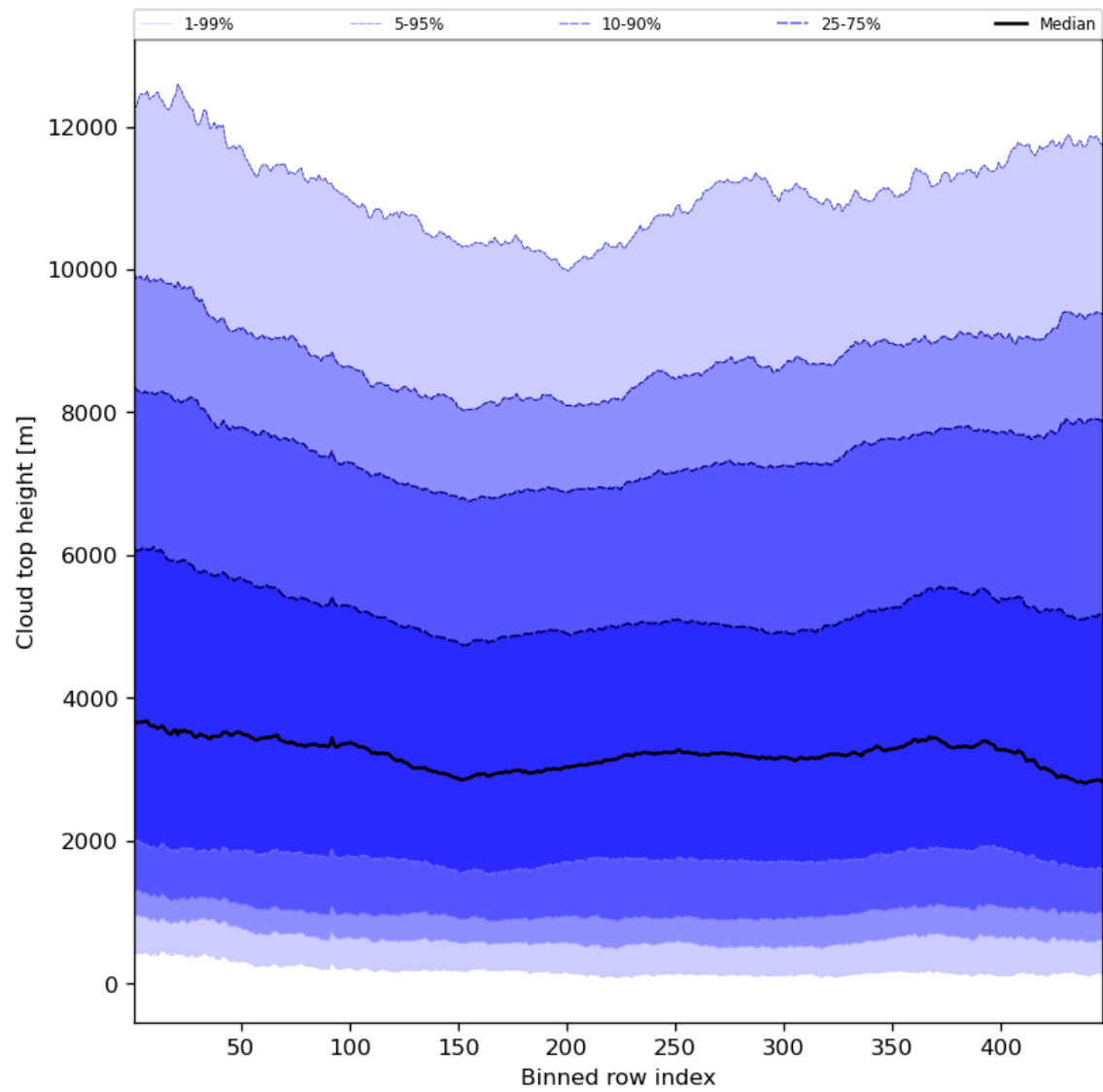
Figure 56: Along track statistics of “Cloud top height” for 2024-07-31 to 2024-08-01
