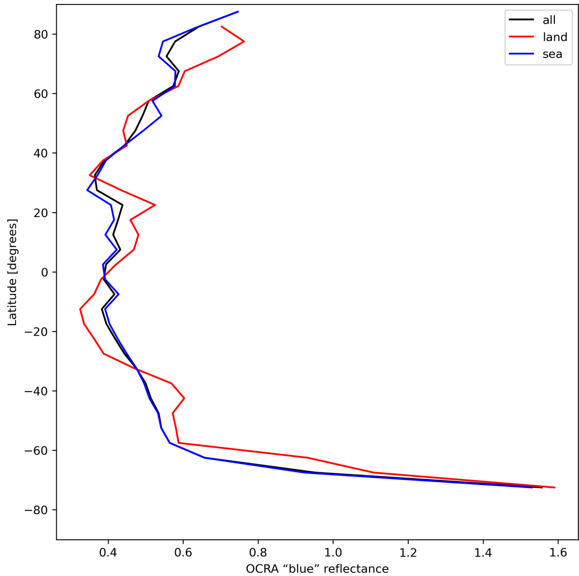
Figure 35: Zonal average of “OCRA “blue” reflectance” for 2024-07-31 to 2024-08-01.
