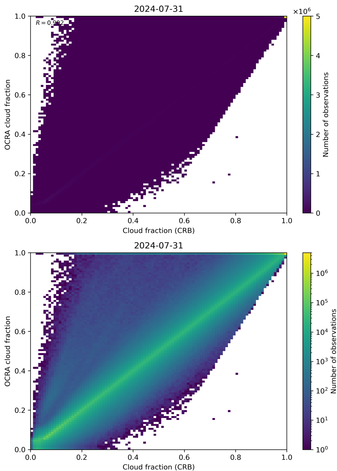
Figure 78: Scatter density plot of “Cloud fraction (CRB)” against “OCRA cloud fraction” for 2024-07-31 to 2024-08-01.
