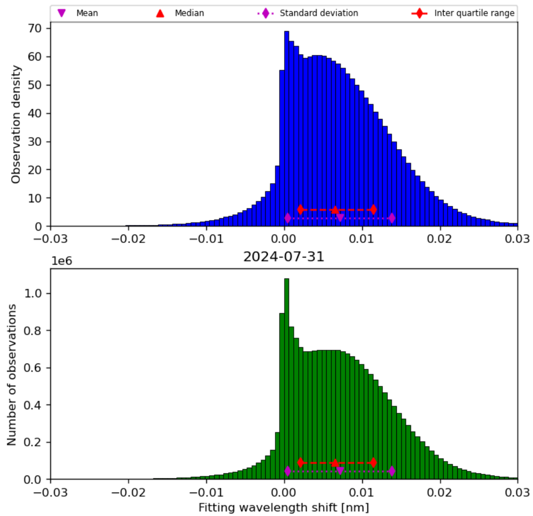
Figure 49: Histogram of “Fitting wavelength shift” for 2024-07-31 to 2024-08-01
