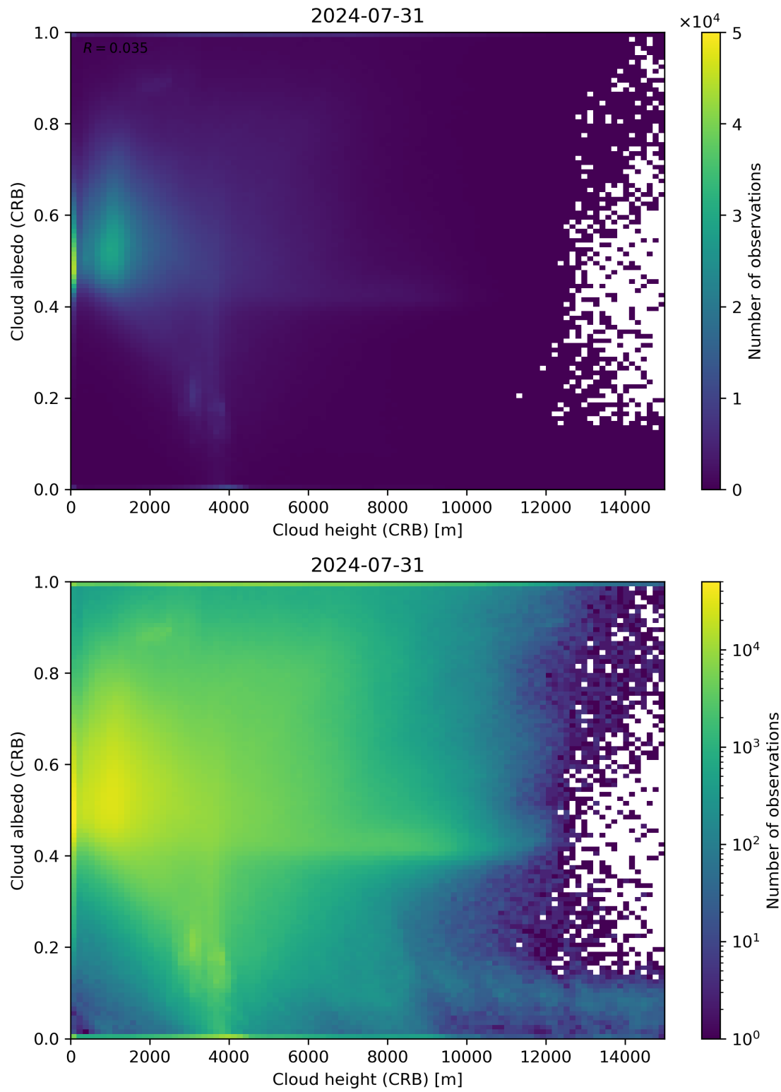
Figure 80: Scatter density plot of “Cloud height (CRB)” against “Cloud albedo (CRB)” for 2024-07-31 to 2024-08-01.
