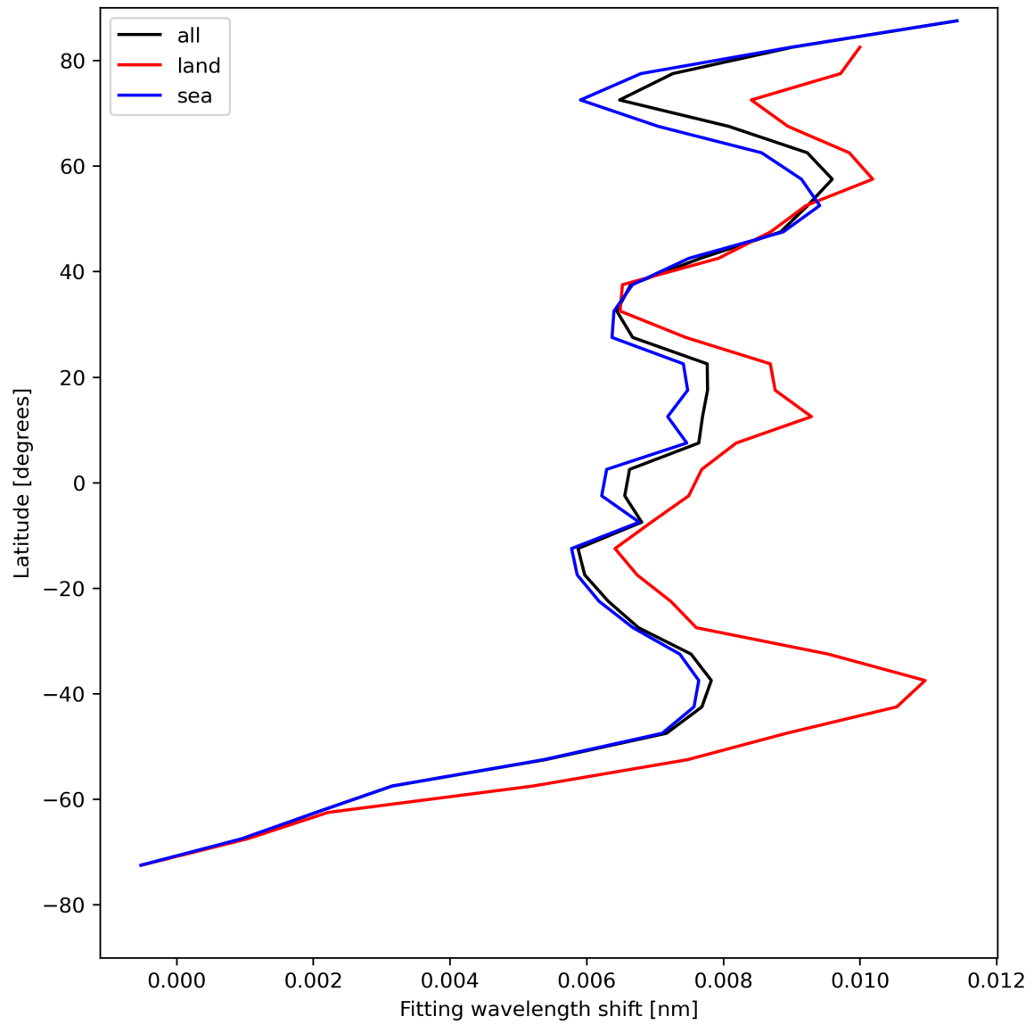
Figure 33: Zonal average of “Fitting wavelength shift” for 2024-07-31 to 2024-08-01.
