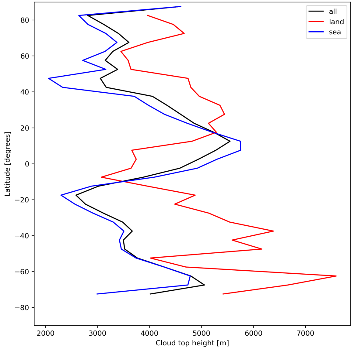
Figure 24: Zonal average of “Cloud top height” for 2024-07-31 to 2024-08-01.
