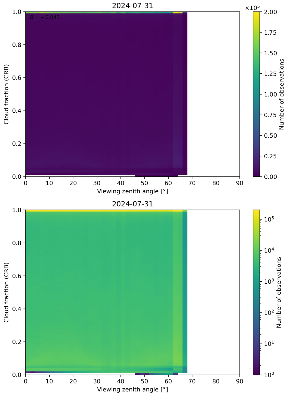
Figure 109: Scatter density plot of “Viewing zenith angle” against “Cloud fraction (CRB)” for 2024-07-31 to 2024-08-01.
