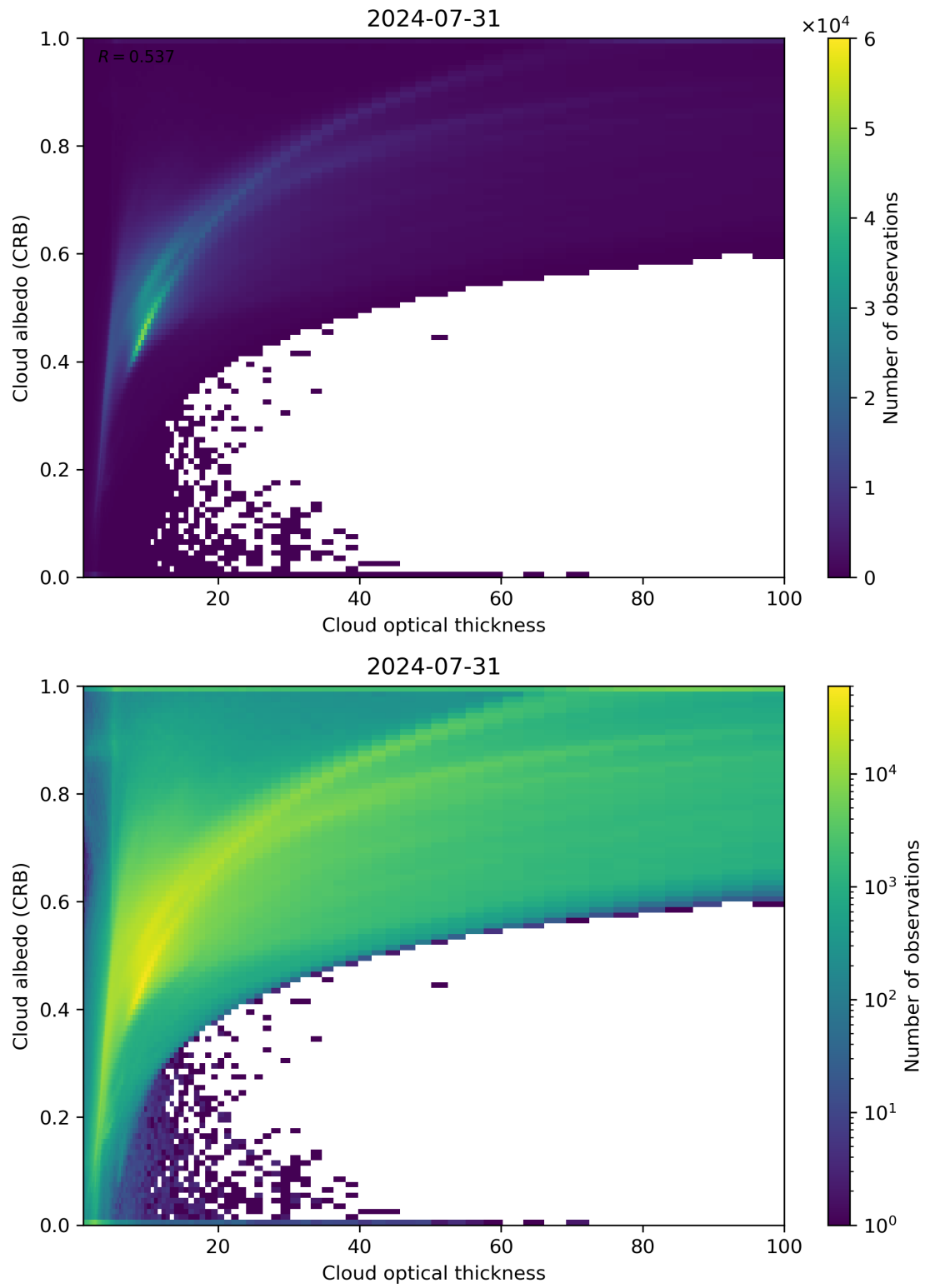
Figure 82: Scatter density plot of “Cloud optical thickness” against “Cloud albedo (CRB)” for 2024-07-31 to 2024-08-01.
