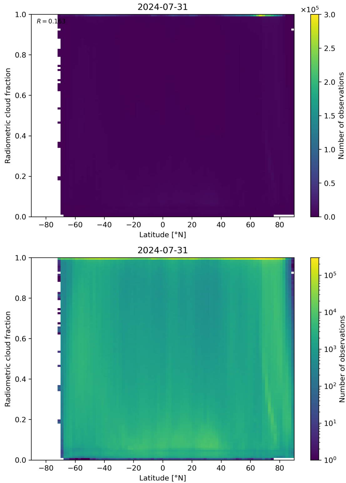
Figure 92: Scatter density plot of “Latitude” against “Radiometric cloud fraction” for 2024-07-31 to 2024-08-01.
