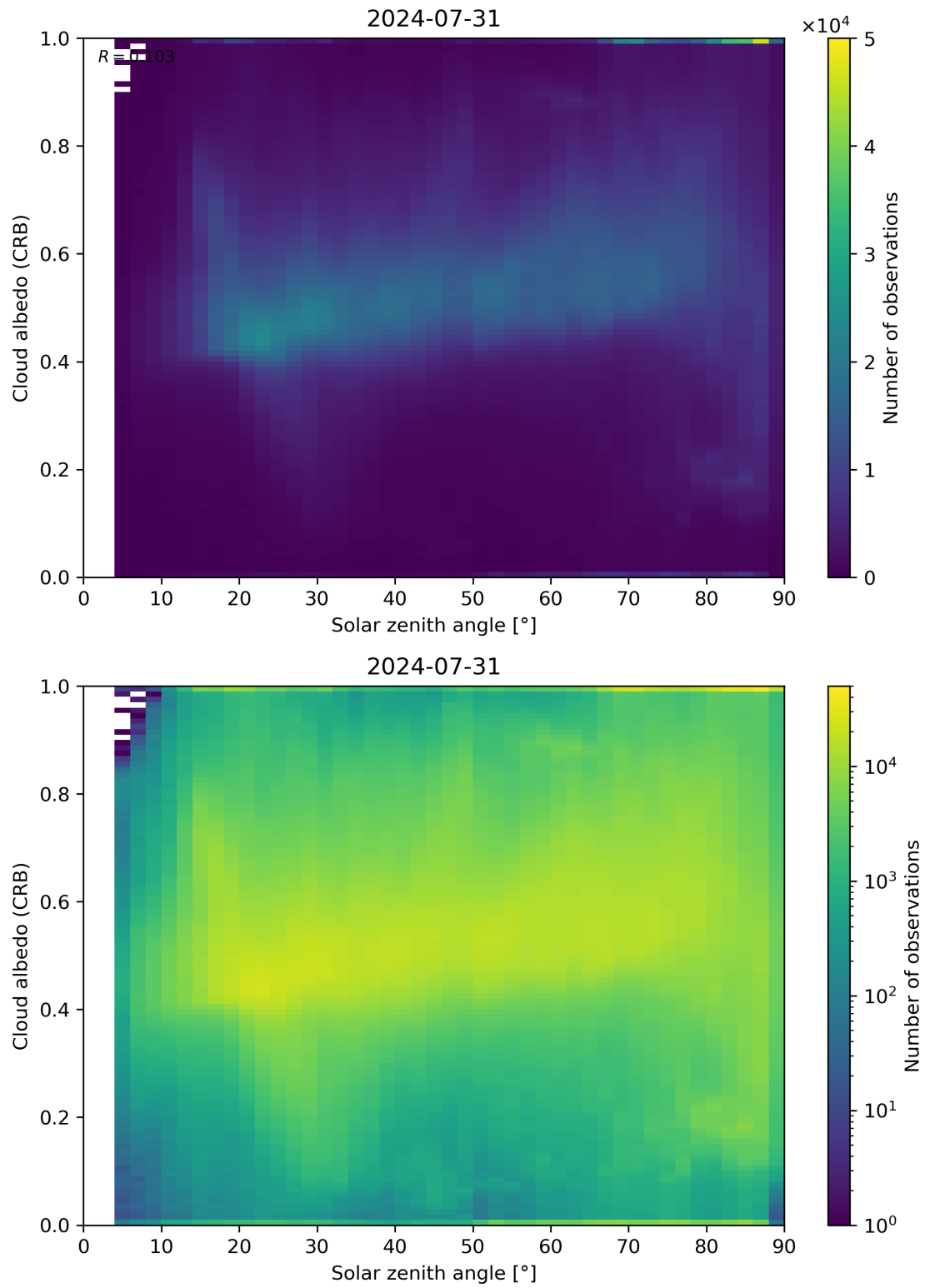
Figure 98: Scatter density plot of “Solar zenith angle” against “Cloud albedo (CRB)” for 2024-07-31 to 2024-08-01.
