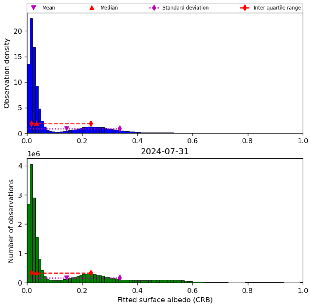
Figure 46: Histogram of “Fitted surface albedo (CRB)” for 2024-07-31 to 2024-08-01
