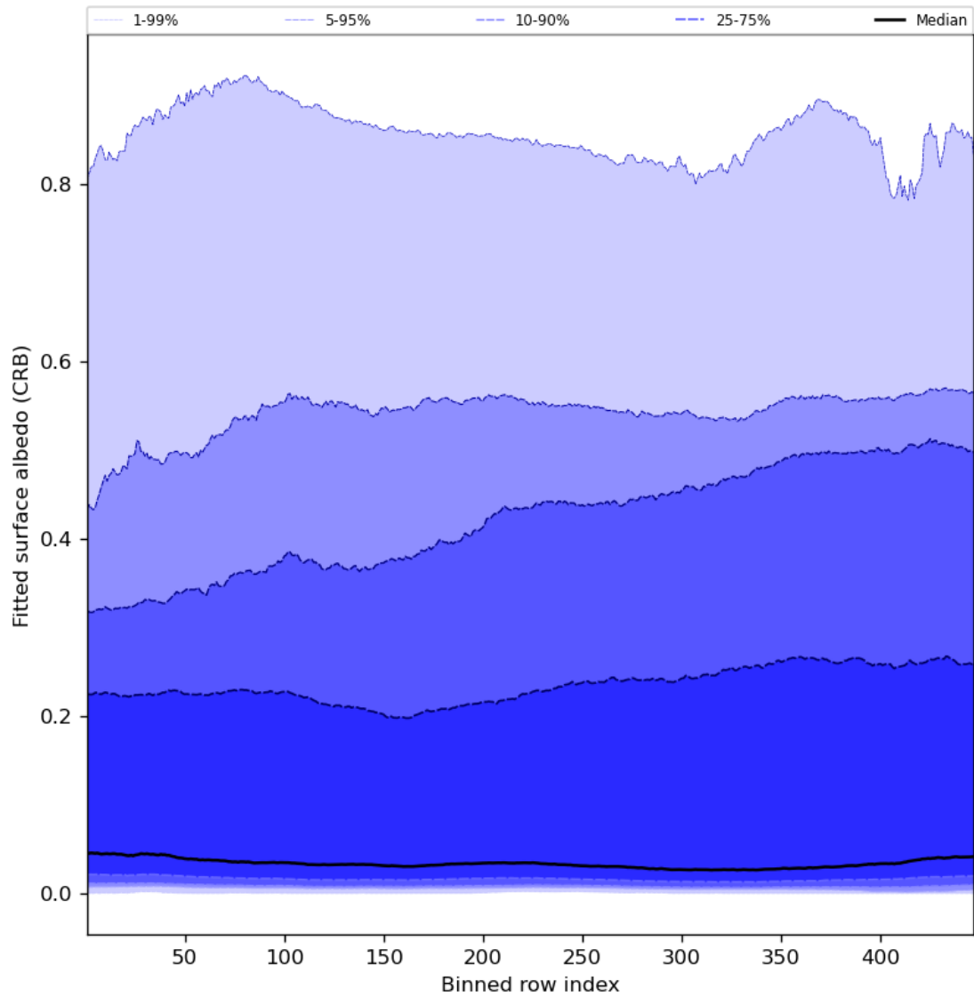
Figure 62: Along track statistics of “Fitted surface albedo (CRB)” for 2024-07-31 to 2024-08-01
