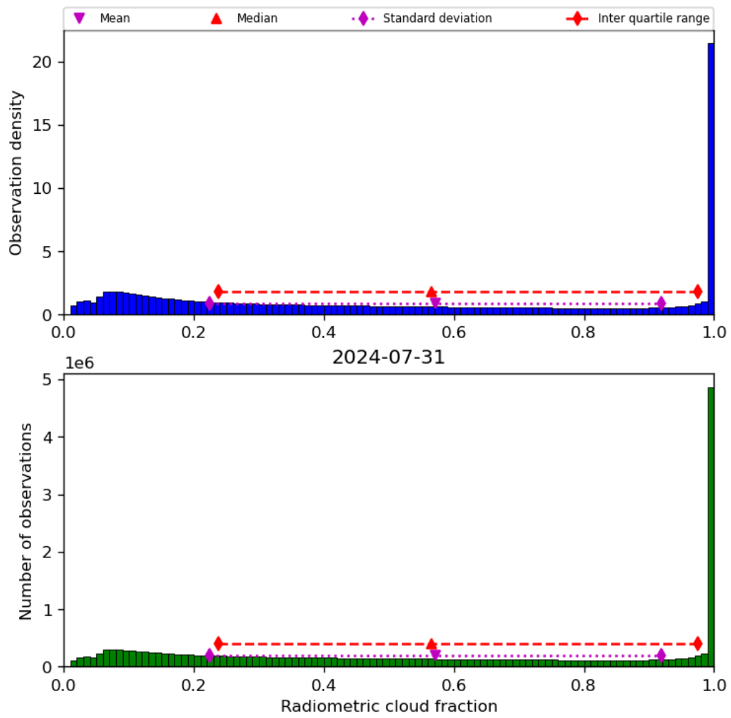
Figure 39: Histogram of “Radiometric cloud fraction” for 2024-07-31 to 2024-08-01
