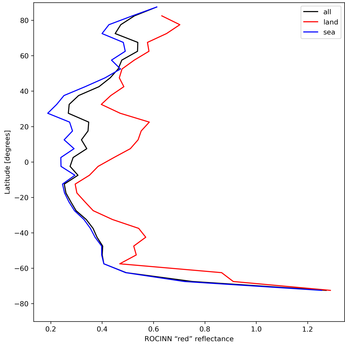
Figure 37: Zonal average of “ROCINN “red” reflectance” for 2024-07-31 to 2024-08-01.
