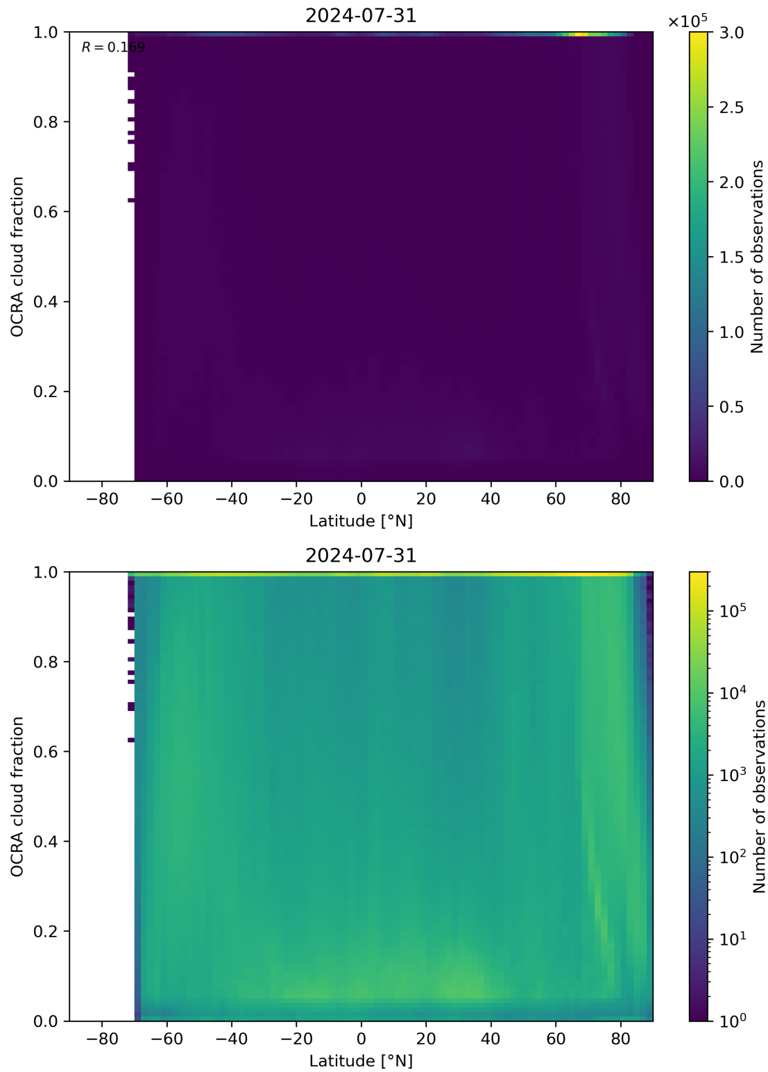
Figure 93: Scatter density plot of “Latitude” against “OCRA cloud fraction” for 2024-07-31 to 2024-08-01.
