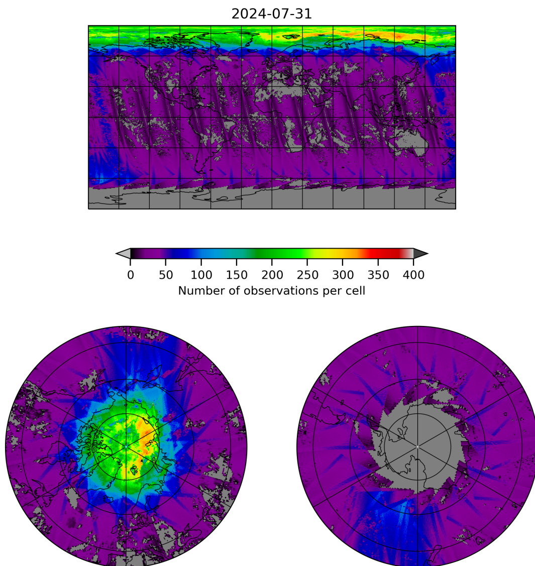
Figure 21: Map of the number of observations for 2024-07-31 to 2024-08-01
