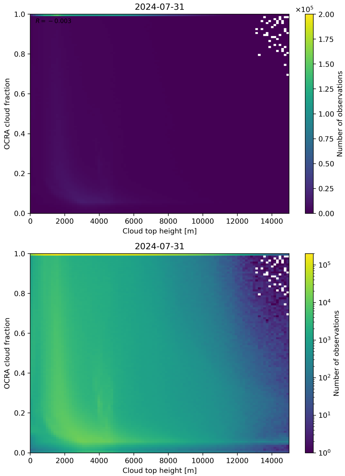
Figure 87: Scatter density plot of “Cloud top height” against “OCRA cloud fraction” for 2024-07-31 to 2024-08-01.
