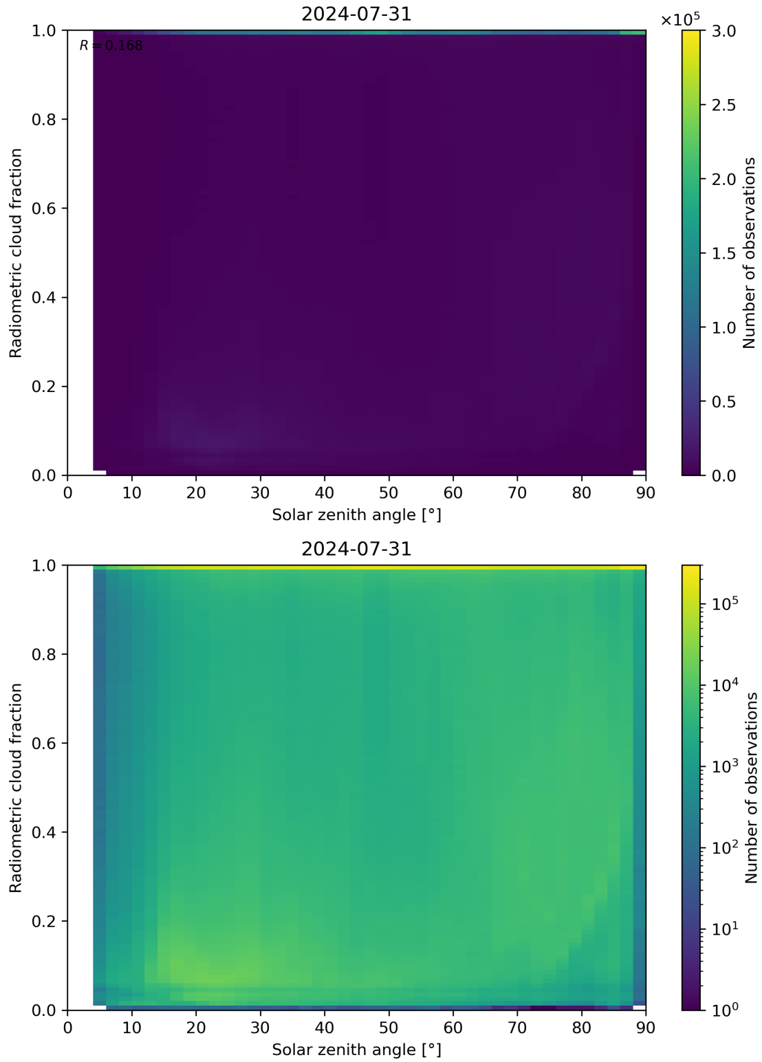
Figure 99: Scatter density plot of “Solar zenith angle” against “Radiometric cloud fraction” for 2024-07-31 to 2024-08-01.
