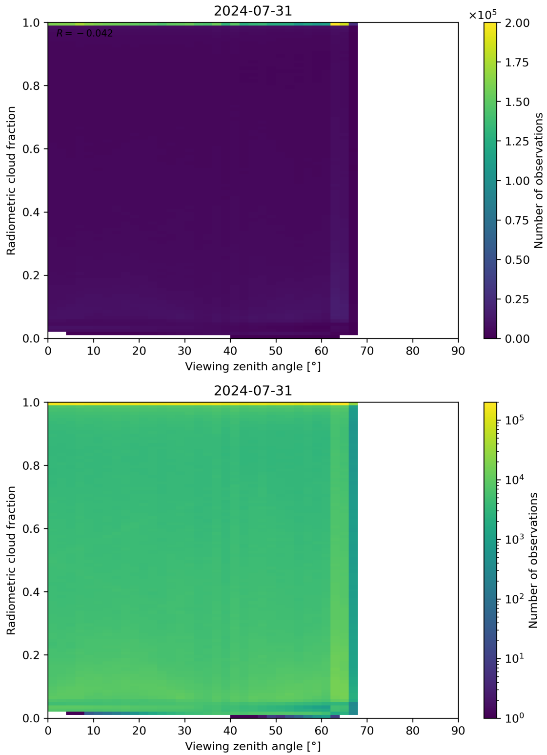
Figure 107: Scatter density plot of “Viewing zenith angle” against “Radiometric cloud fraction” for 2024-07-31 to 2024-08-01.
