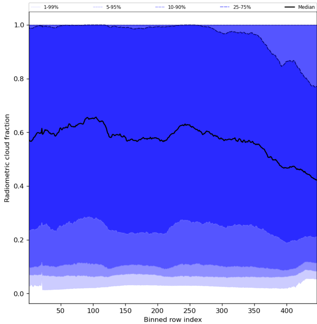
Figure 55: Along track statistics of “Radiometric cloud fraction” for 2024-07-31 to 2024-08-01
