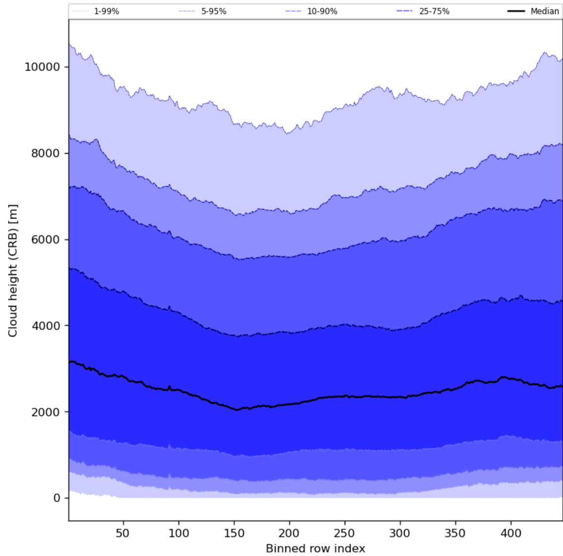
Figure 59: Along track statistics of “Cloud height (CRB)” for 2024-07-31 to 2024-08-01
