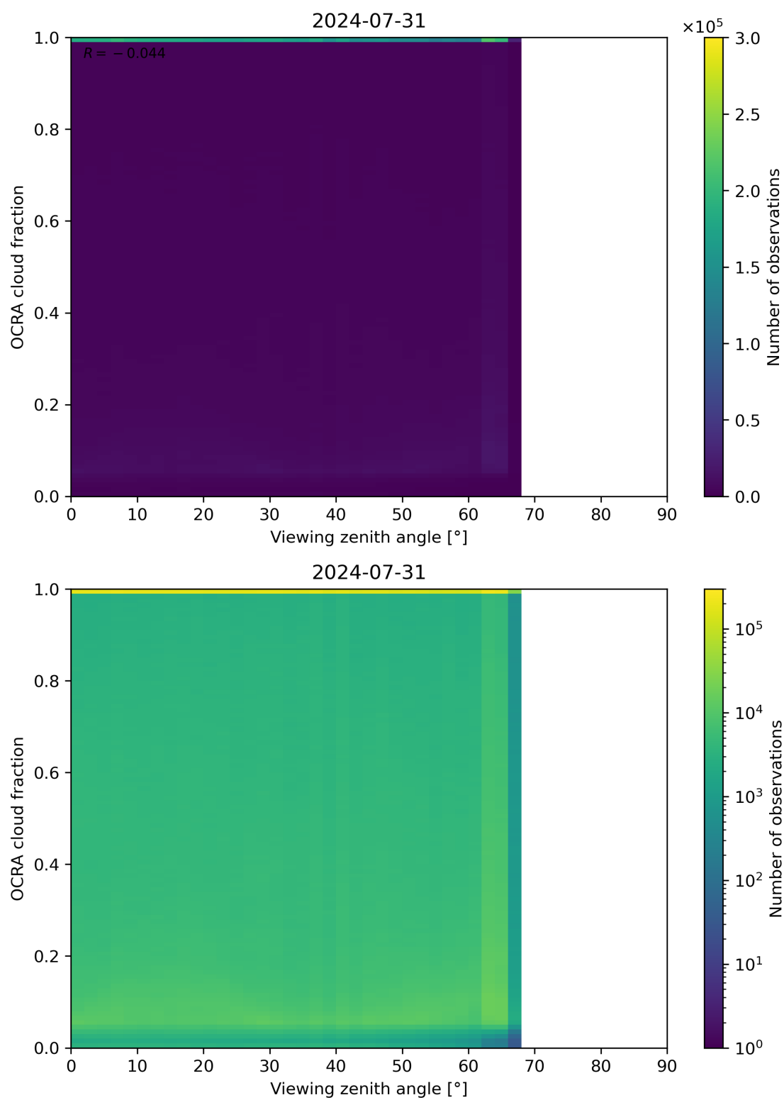
Figure 108: Scatter density plot of “Viewing zenith angle” against “OCRA cloud fraction” for 2024-07-31 to 2024-08-01.
