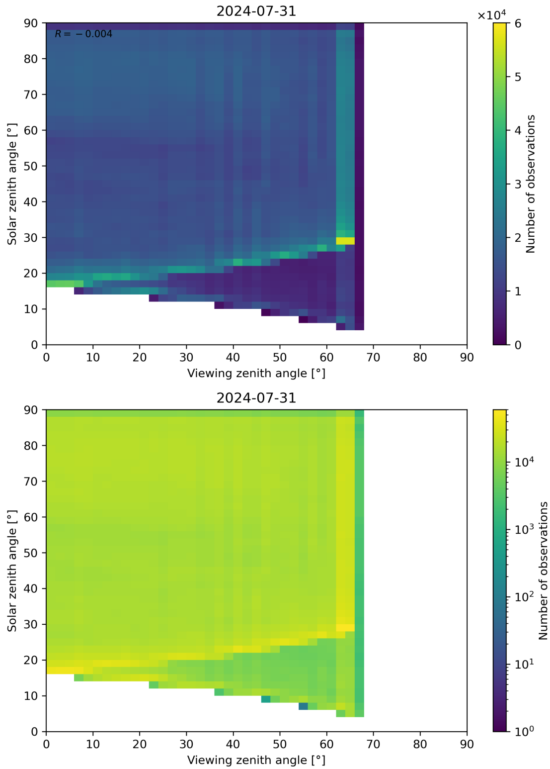
Figure 114: Scatter density plot of “Viewing zenith angle” against “Solar zenith angle” for 2024-07-31 to 2024-08-01.
