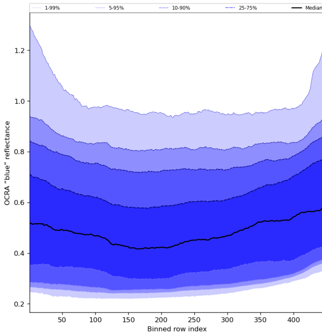
Figure 67: Along track statistics of “OCRA “blue” reflectance” for 2024-07-31 to 2024-08-01
