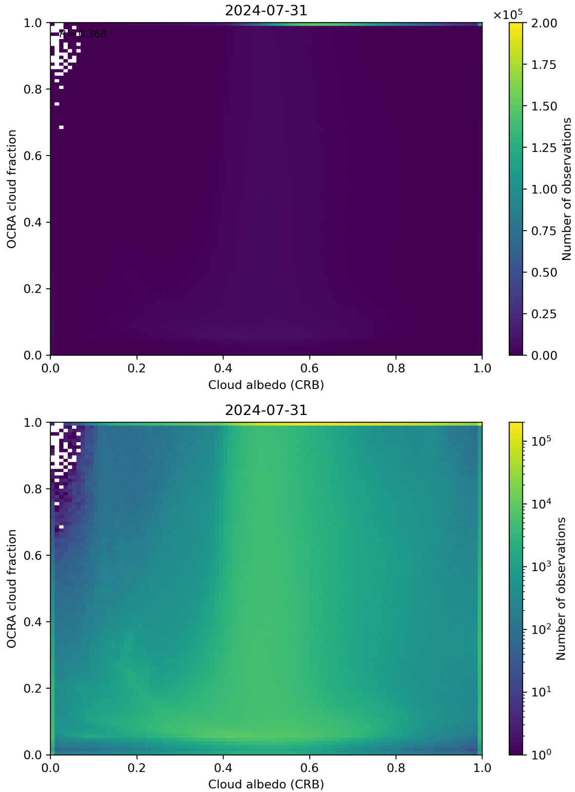
Figure 70: Scatter density plot of “Cloud albedo (CRB)” against “OCRA cloud fraction” for 2024-07-31 to 2024-08-01.
