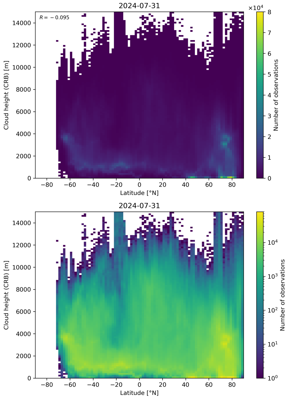
Figure 95: Scatter density plot of “Latitude” against “Cloud height (CRB)” for 2024-07-31 to 2024-08-01.
