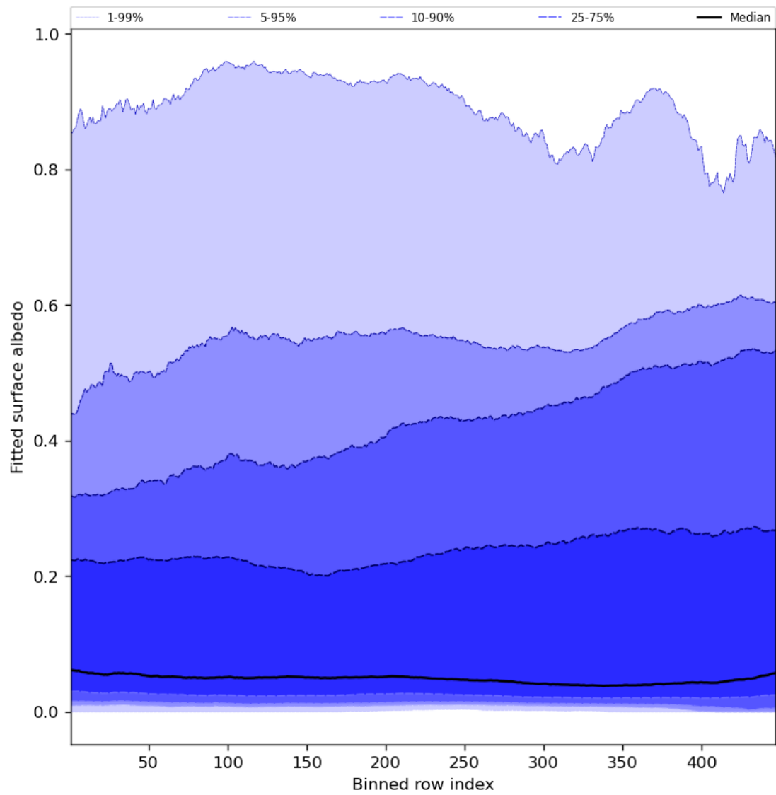
Figure 61: Along track statistics of “Fitted surface albedo” for 2024-07-31 to 2024-08-01
