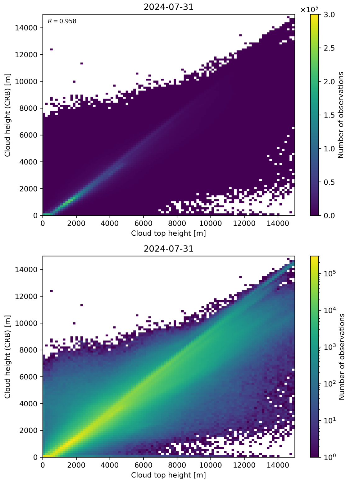
Figure 89: Scatter density plot of “Cloud top height” against “Cloud height (CRB)” for 2024-07-31 to 2024-08-01.
