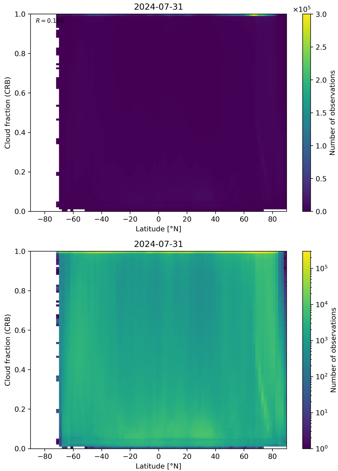
Figure 94: Scatter density plot of “Latitude” against “Cloud fraction (CRB)” for 2024-07-31 to 2024-08-01.
