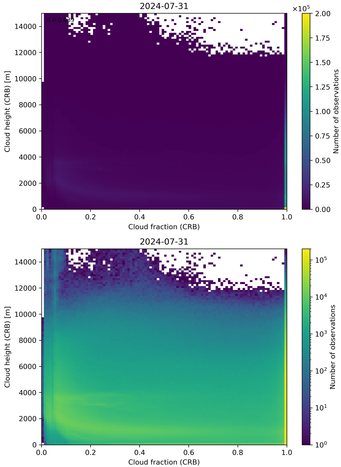
Figure 79: Scatter density plot of “Cloud fraction (CRB)” against “Cloud height (CRB)” for 2024-07-31 to 2024-08-01.
