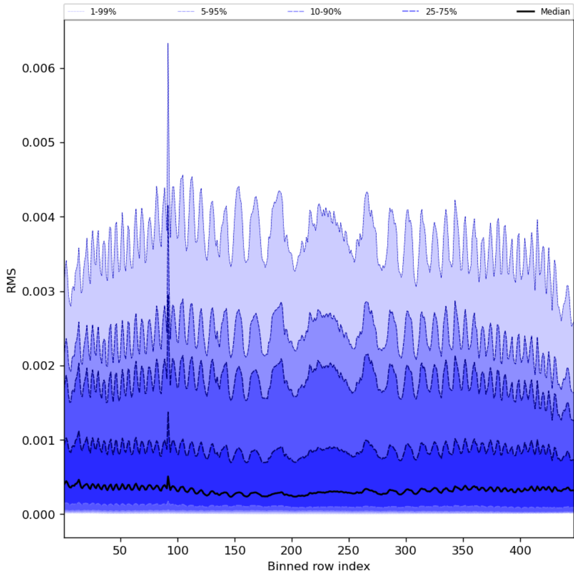
Figure 63: Along track statistics of “RMS” for 2024-07-31 to 2024-08-01
