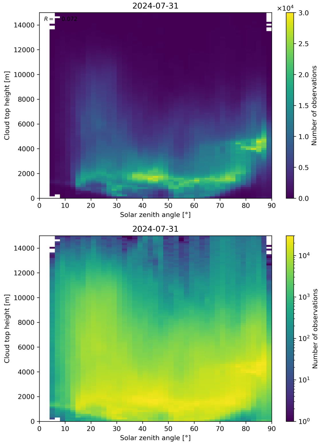
Figure 104: Scatter density plot of “Solar zenith angle” against “Cloud top height” for 2024-07-31 to 2024-08-01.
