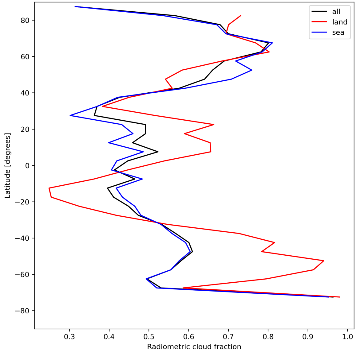
Figure 23: Zonal average of “Radiometric cloud fraction” for 2024-07-31 to 2024-08-01.
