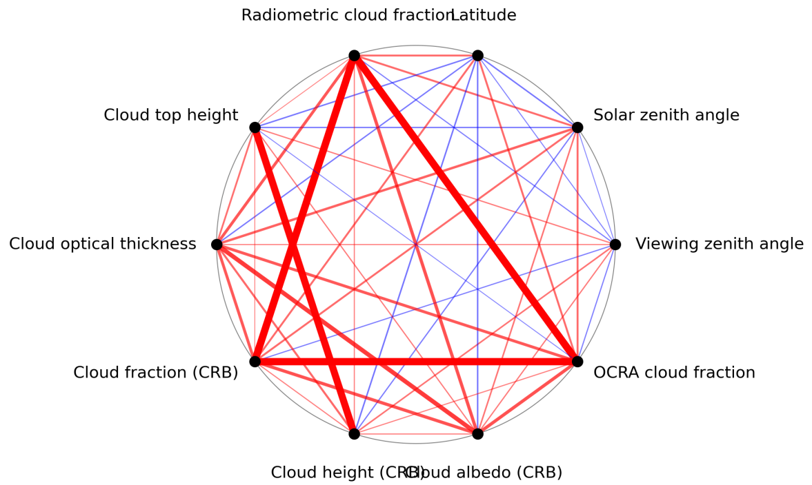
Figure 1: Map of correlation graph for 2024-07-31 to 2024-08-01.
