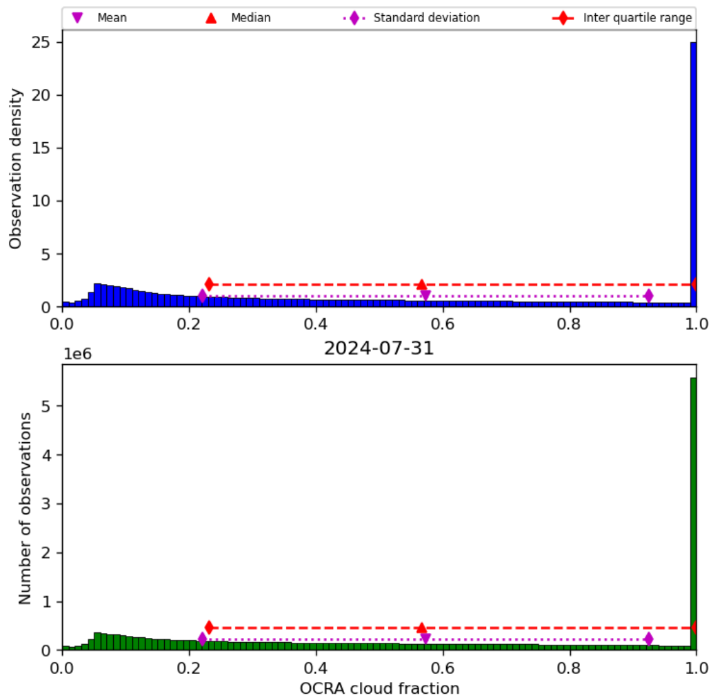
Figure 50: Histogram of “OCRA cloud fraction” for 2024-07-31 to 2024-08-01
