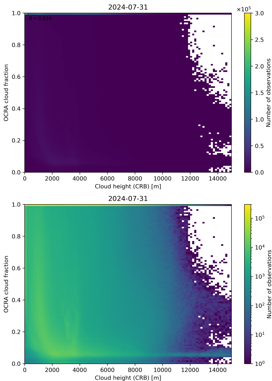
Figure 81: Scatter density plot of “Cloud height (CRB)” against “OCRA cloud fraction” for 2024-07-31 to 2024-08-01.
