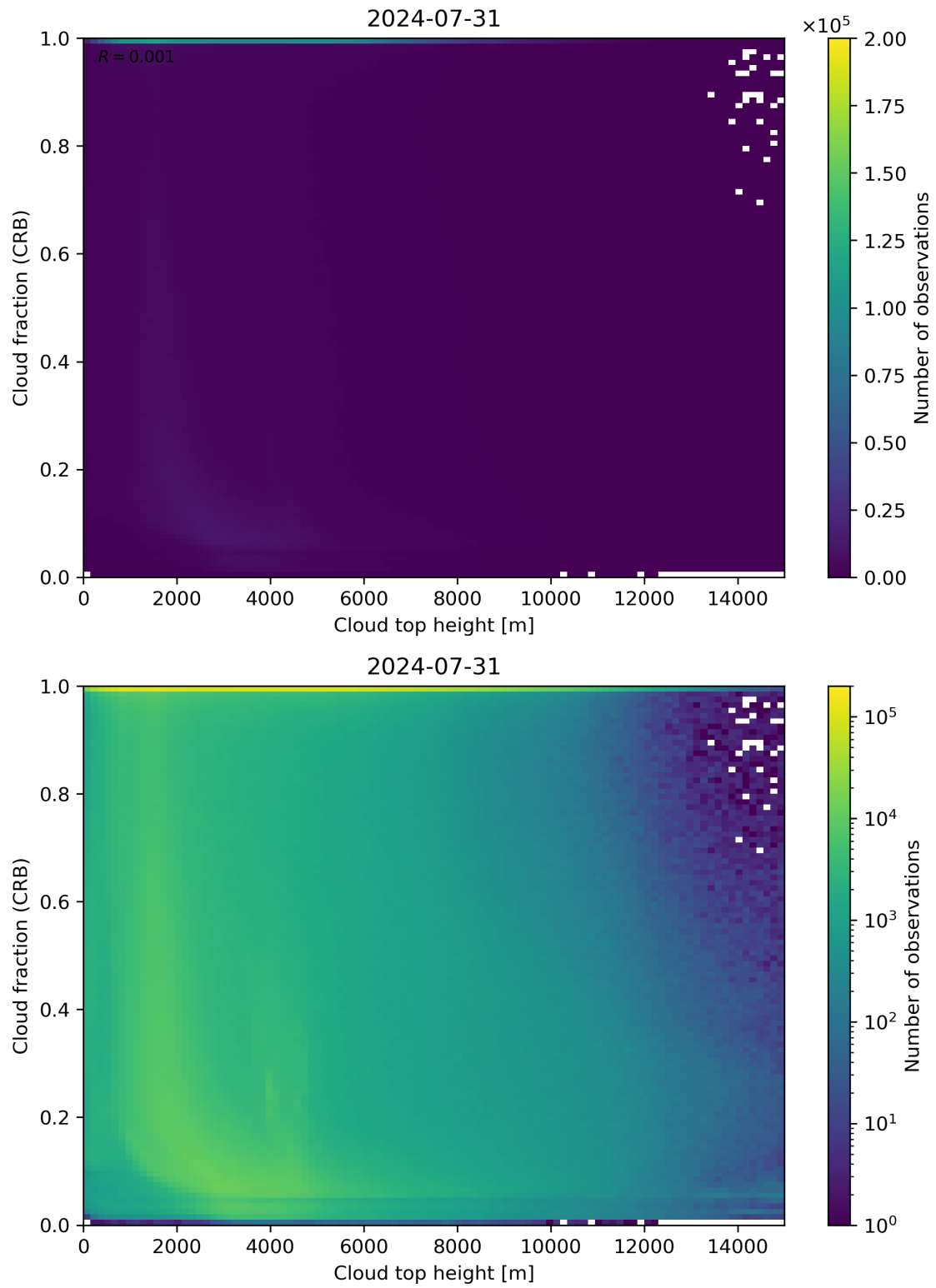
Figure 88: Scatter density plot of “Cloud top height” against “Cloud fraction (CRB)” for 2024-07-31 to 2024-08-01.
