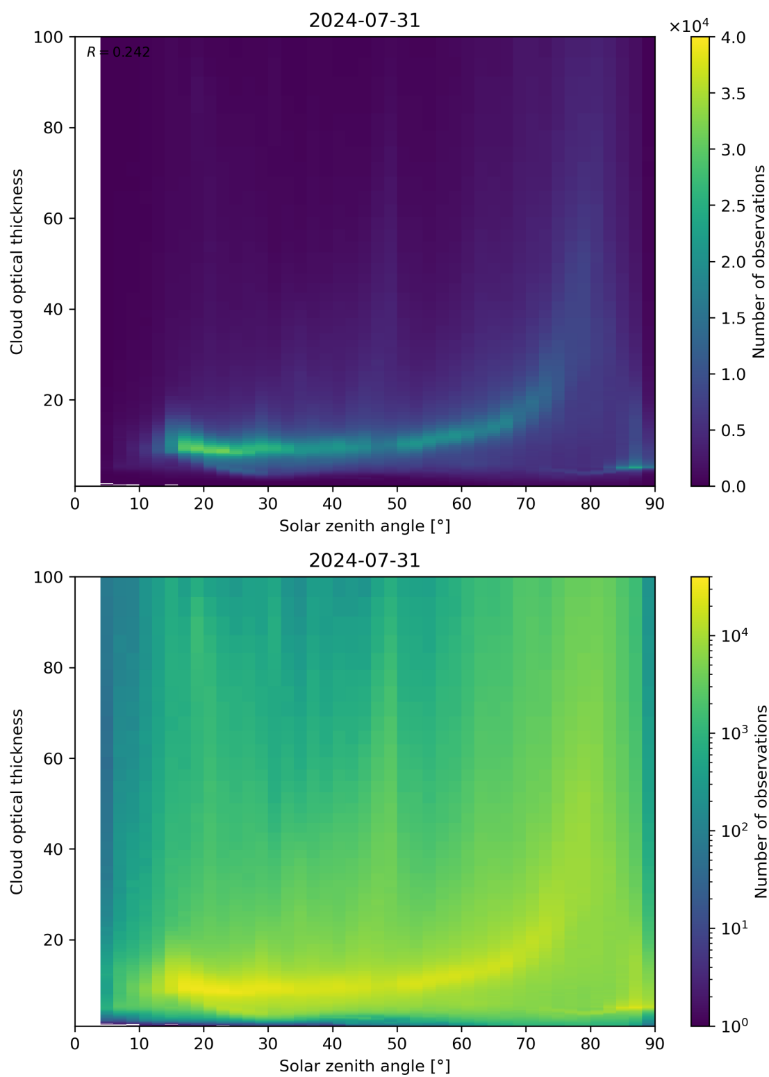
Figure 103: Scatter density plot of “Solar zenith angle” against “Cloud optical thickness” for 2024-07-31 to 2024-08-01.
