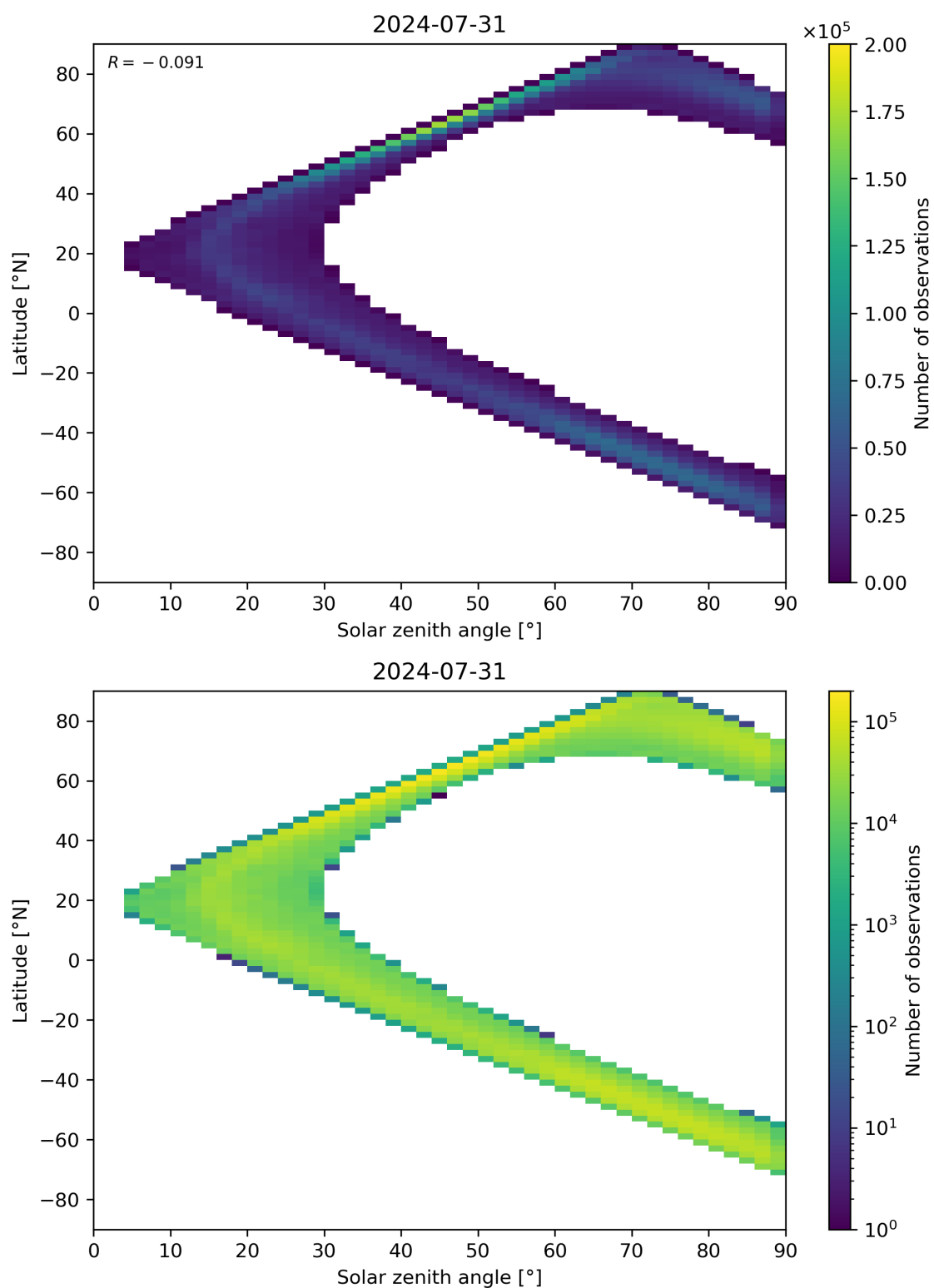
Figure 105: Scatter density plot of “Solar zenith angle” against “Latitude” for 2024-07-31 to 2024-08-01.
