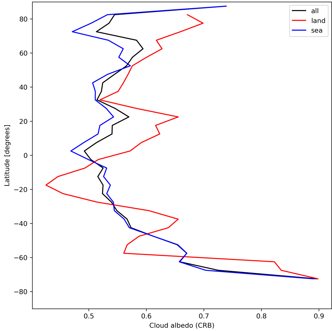
Figure 28: Zonal average of “Cloud albedo (CRB)” for 2024-07-31 to 2024-08-01.
