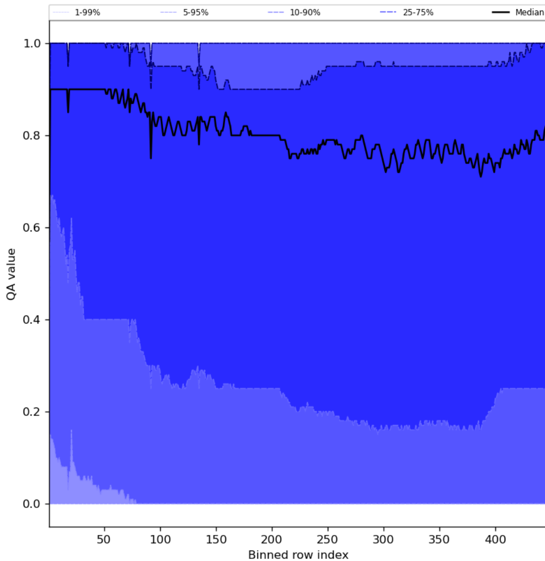
Figure 54: Along track statistics of “QA value” for 2024-07-31 to 2024-08-01
