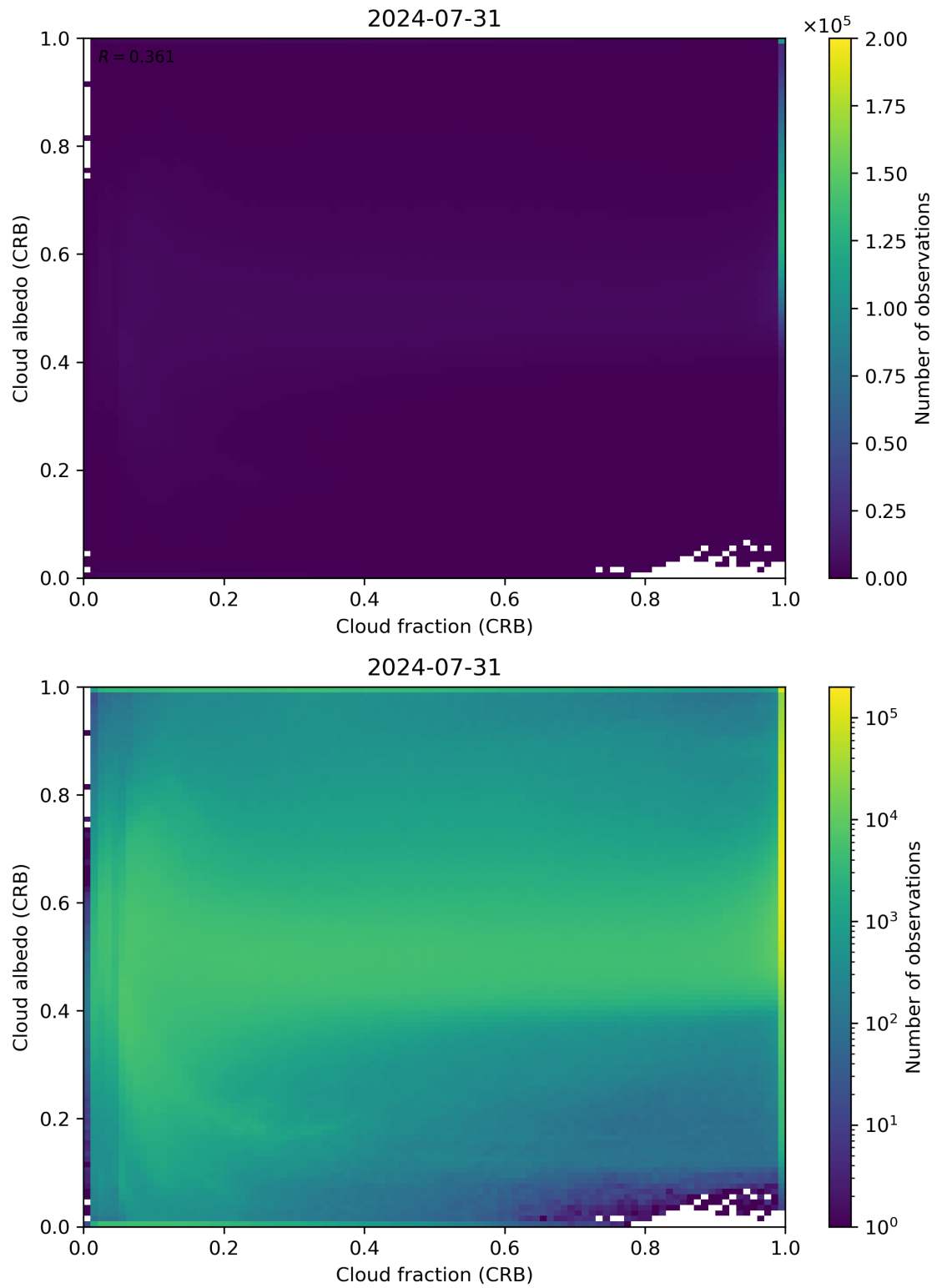
Figure 77: Scatter density plot of “Cloud fraction (CRB)” against “Cloud albedo (CRB)” for 2024-07-31 to 2024-08-01.
