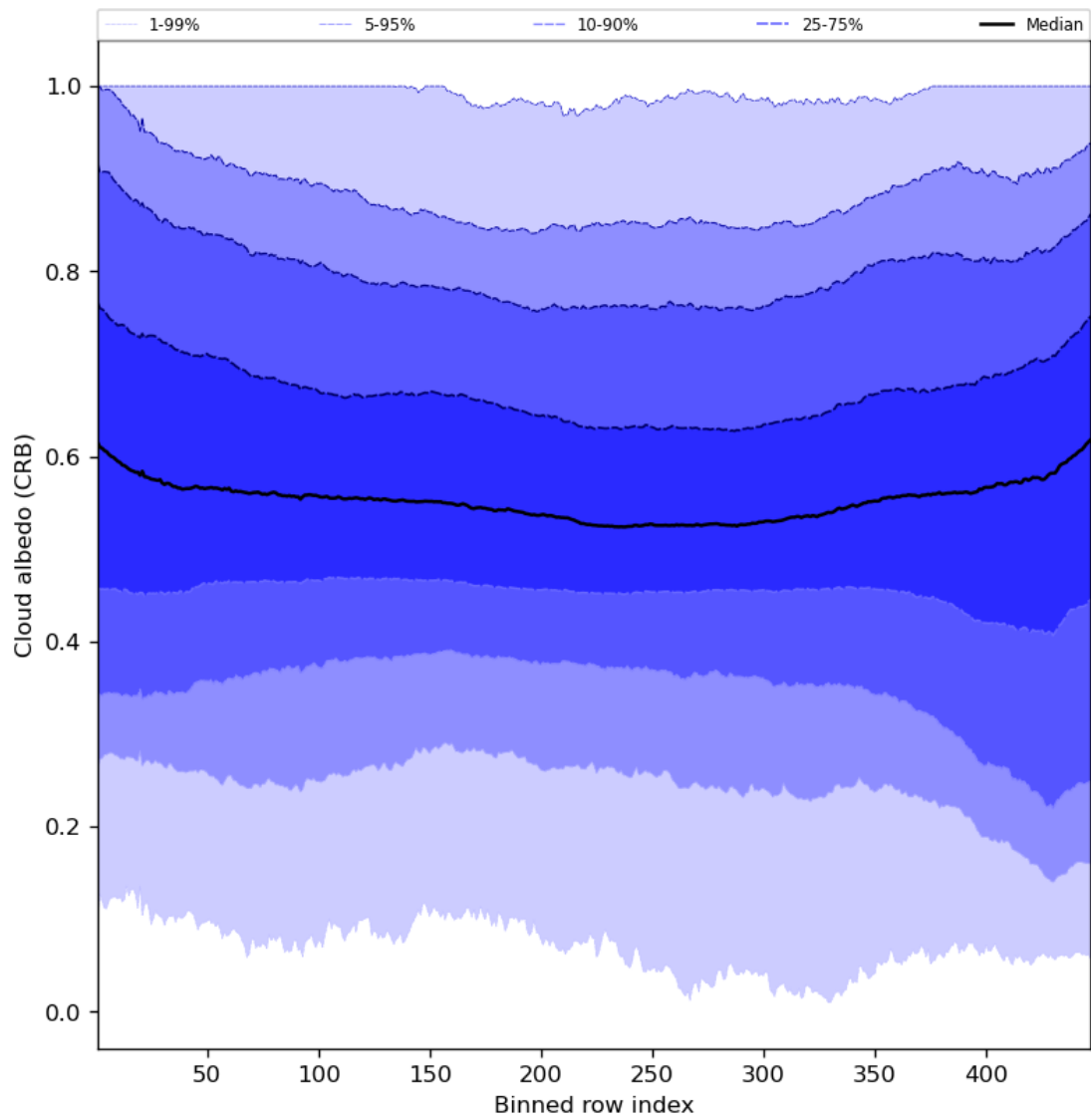
Figure 60: Along track statistics of “Cloud albedo (CRB)” for 2024-07-31 to 2024-08-01
