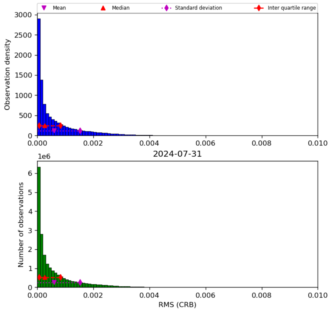
Figure 48: Histogram of “RMS (CRB)” for 2024-07-31 to 2024-08-01
