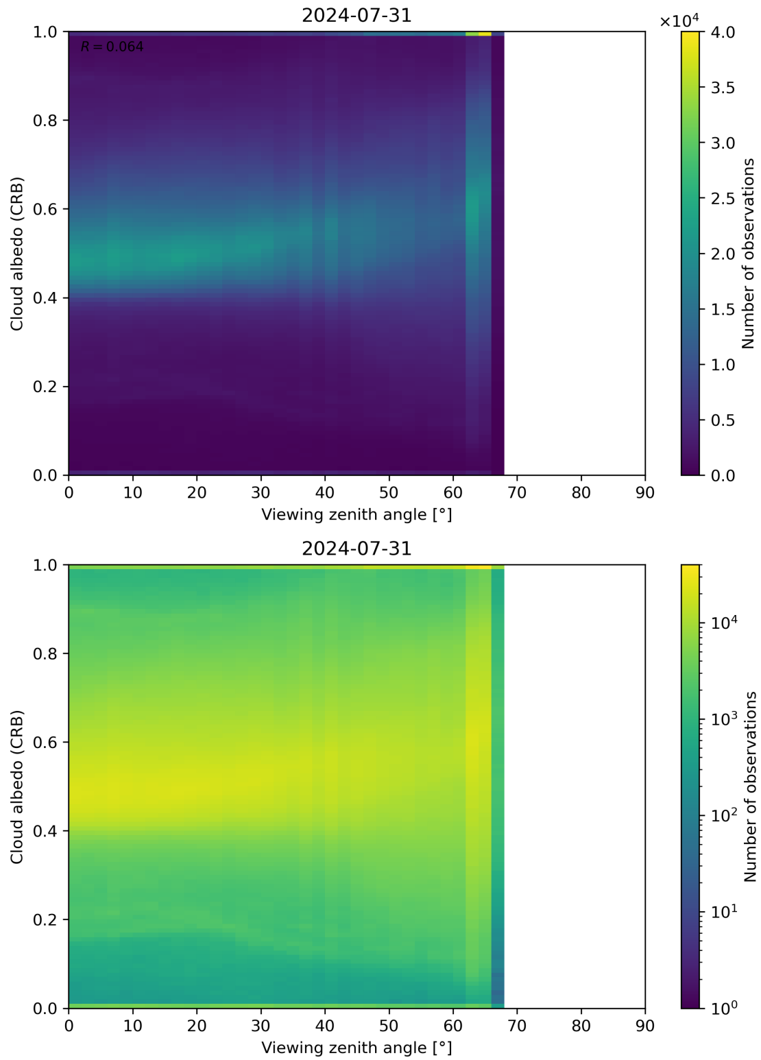
Figure 106: Scatter density plot of “Viewing zenith angle” against “Cloud albedo (CRB)” for 2024-07-31 to 2024-08-01.
