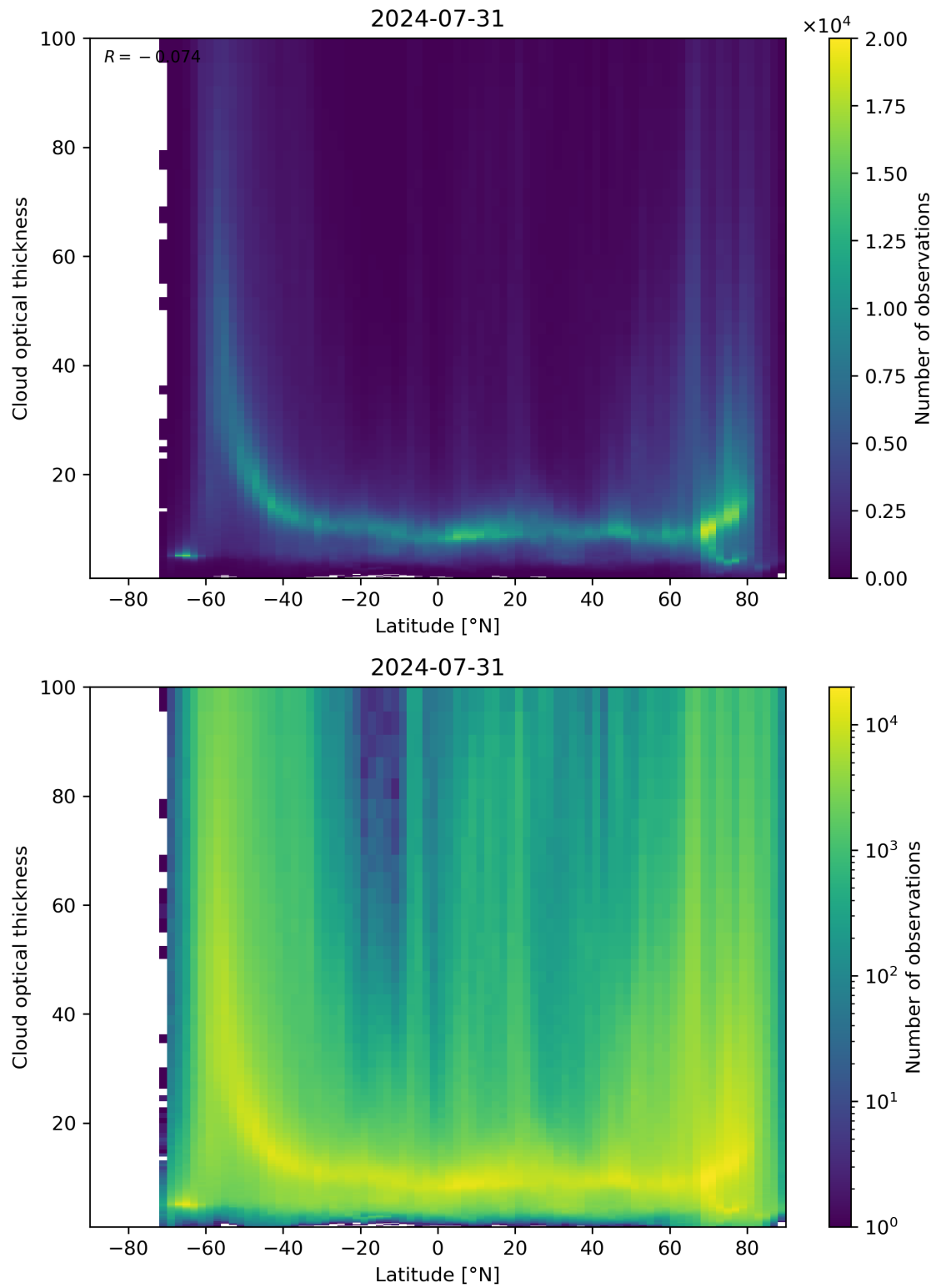
Figure 96: Scatter density plot of “Latitude” against “Cloud optical thickness” for 2024-07-31 to 2024-08-01.
