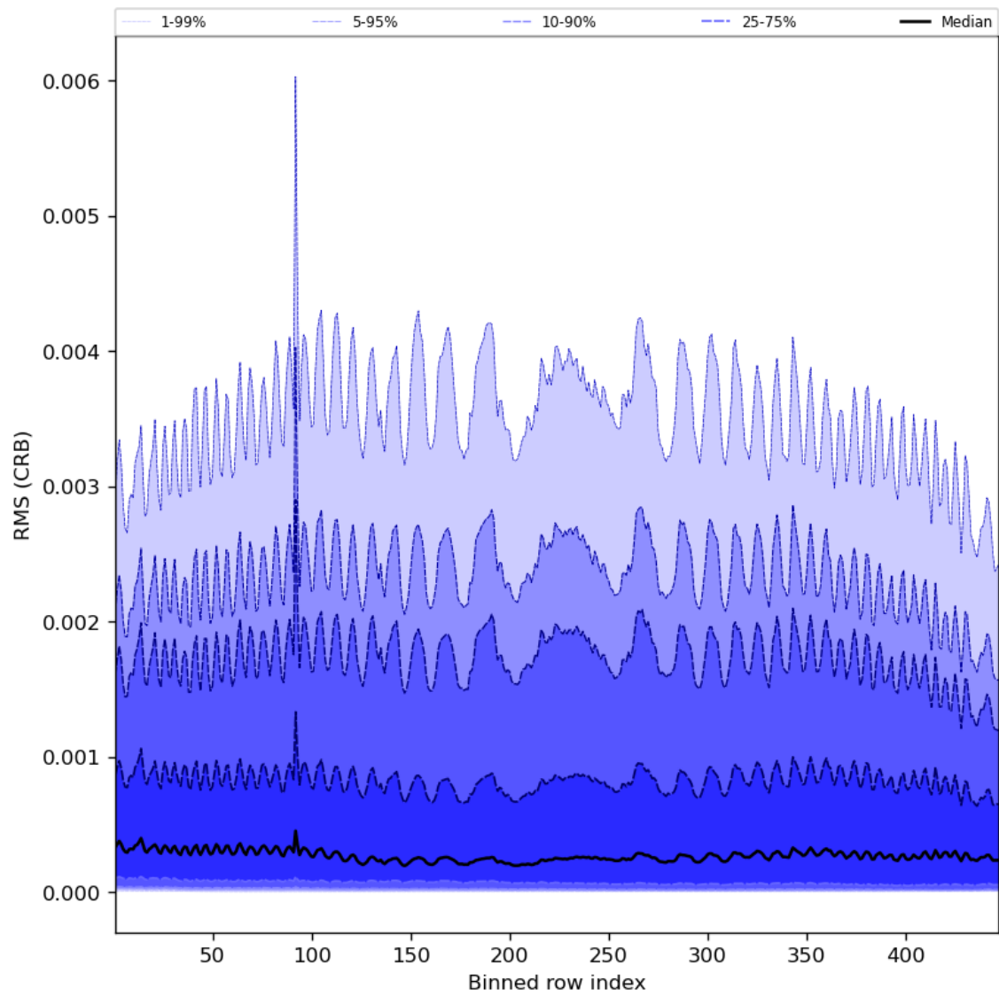
Figure 64: Along track statistics of “RMS (CRB)” for 2024-07-31 to 2024-08-01
