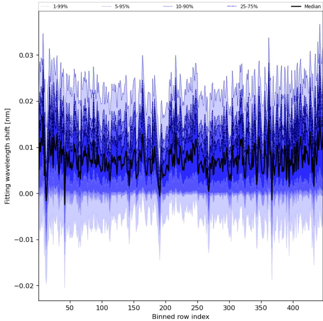
Figure 65: Along track statistics of “Fitting wavelength shift” for 2024-07-31 to 2024-08-01
