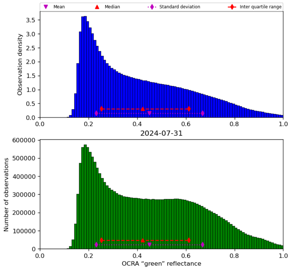
Figure 52: Histogram of “OCRA “green” reflectance” for 2024-07-31 to 2024-08-01
