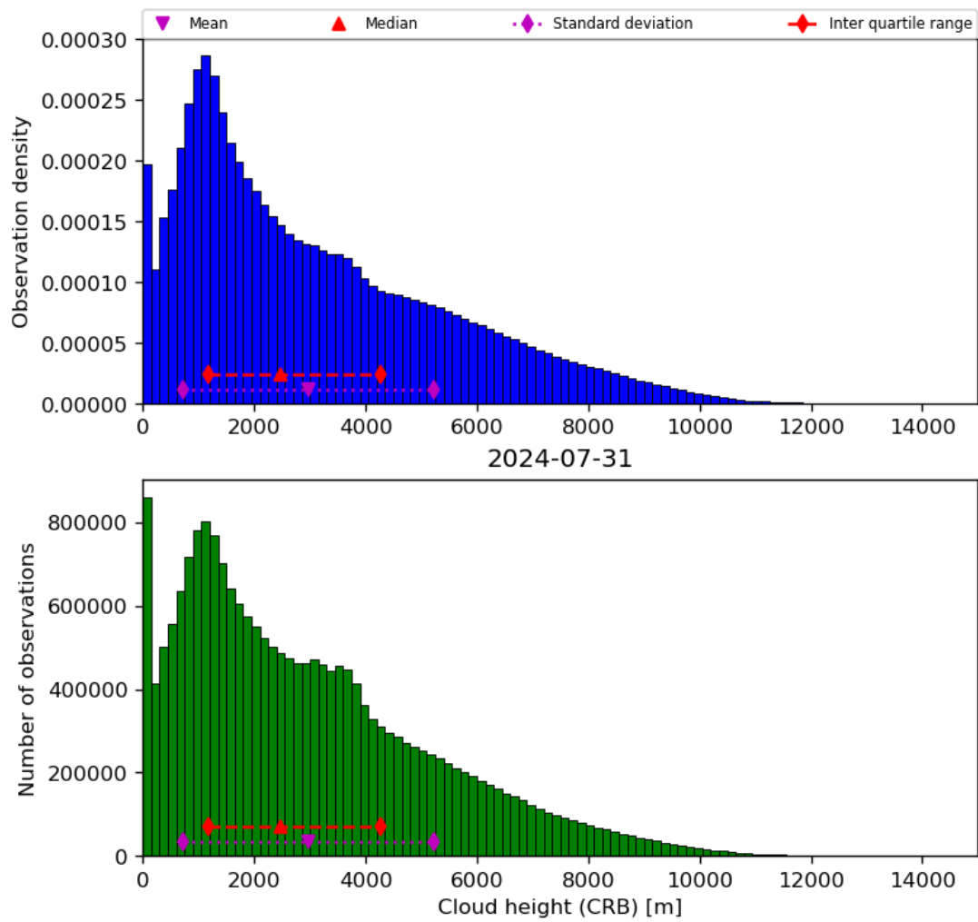
Figure 43: Histogram of “Cloud height (CRB)” for 2024-07-31 to 2024-08-01
