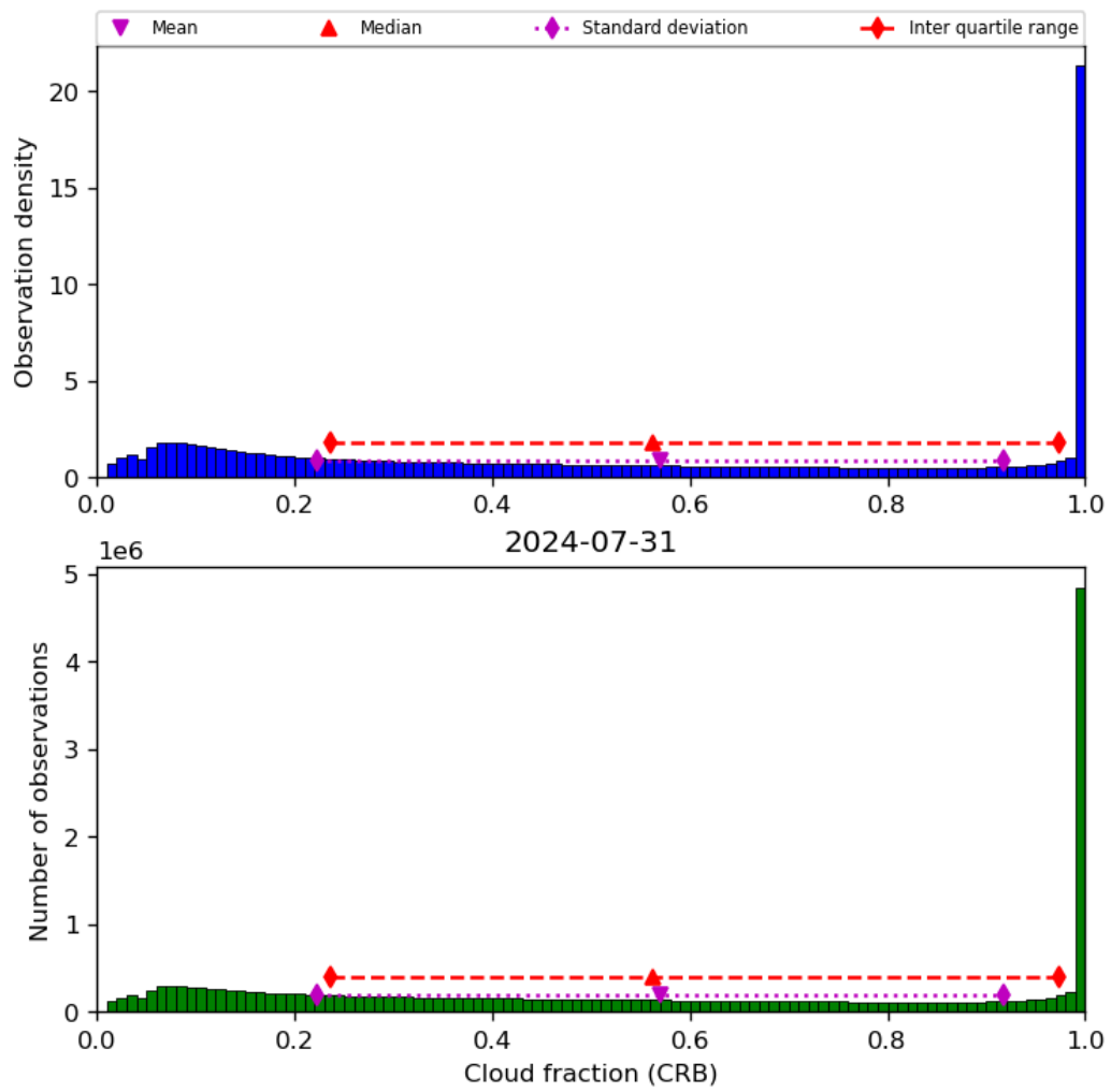
Figure 42: Histogram of “Cloud fraction (CRB)” for 2024-07-31 to 2024-08-01
