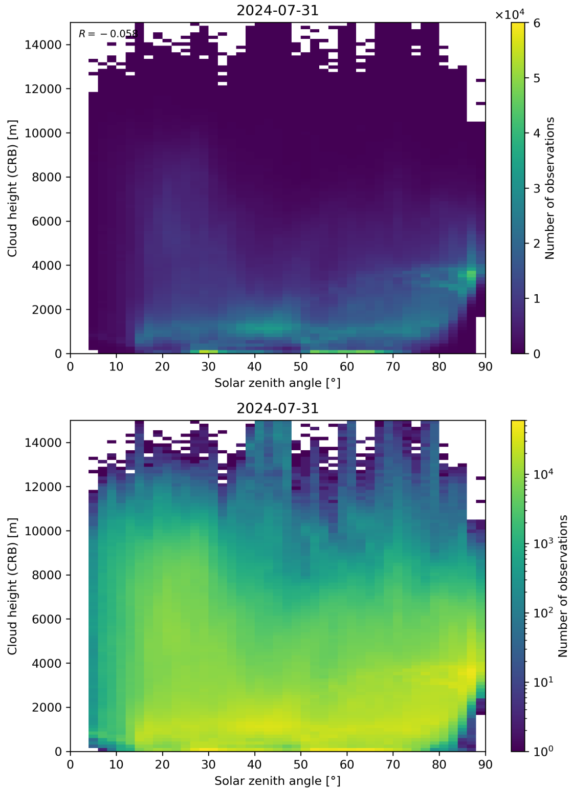
Figure 102: Scatter density plot of “Solar zenith angle” against “Cloud height (CRB)” for 2024-07-31 to 2024-08-01.
