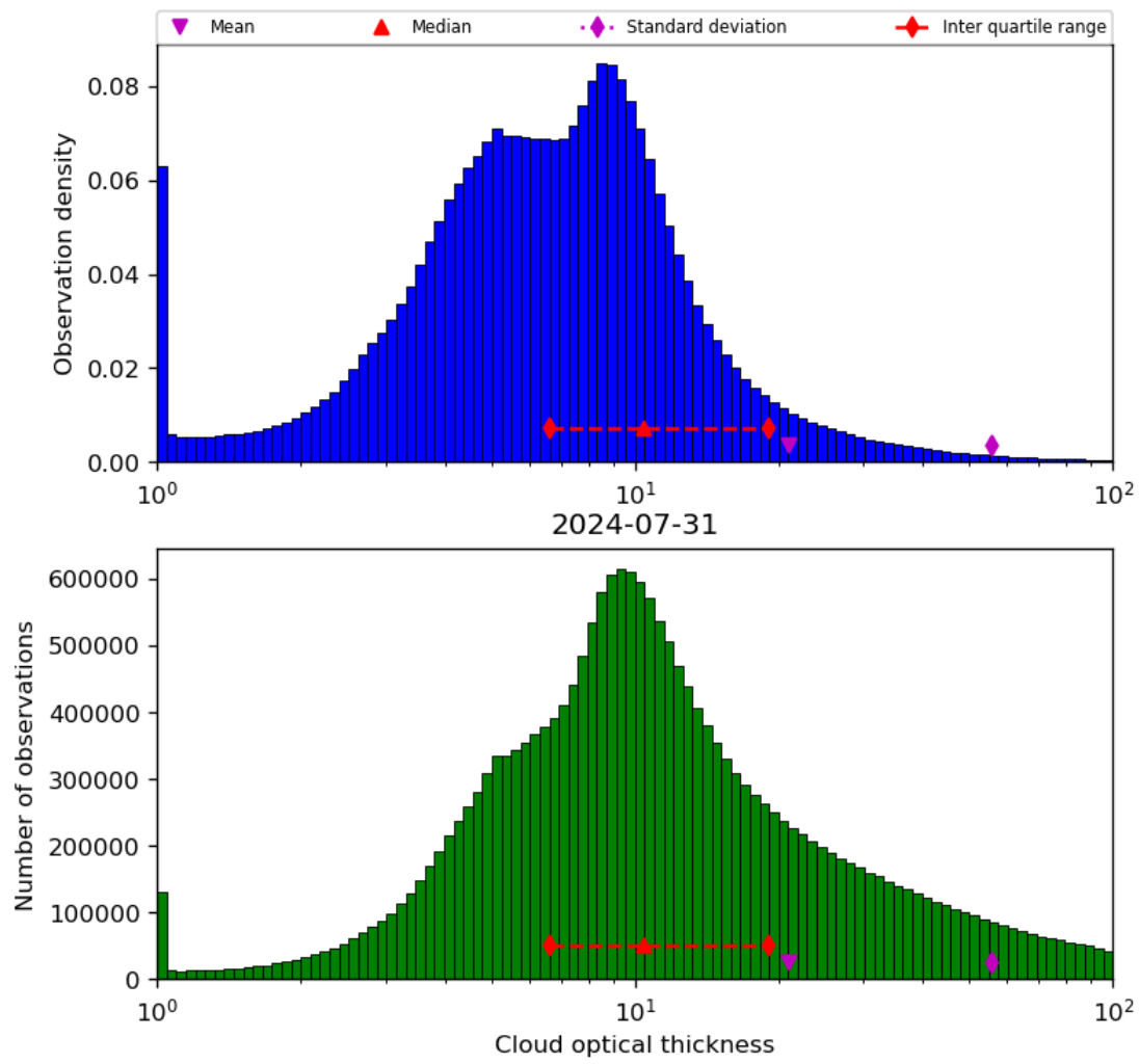
Figure 41: Histogram of “Cloud optical thickness” for 2024-07-31 to 2024-08-01
