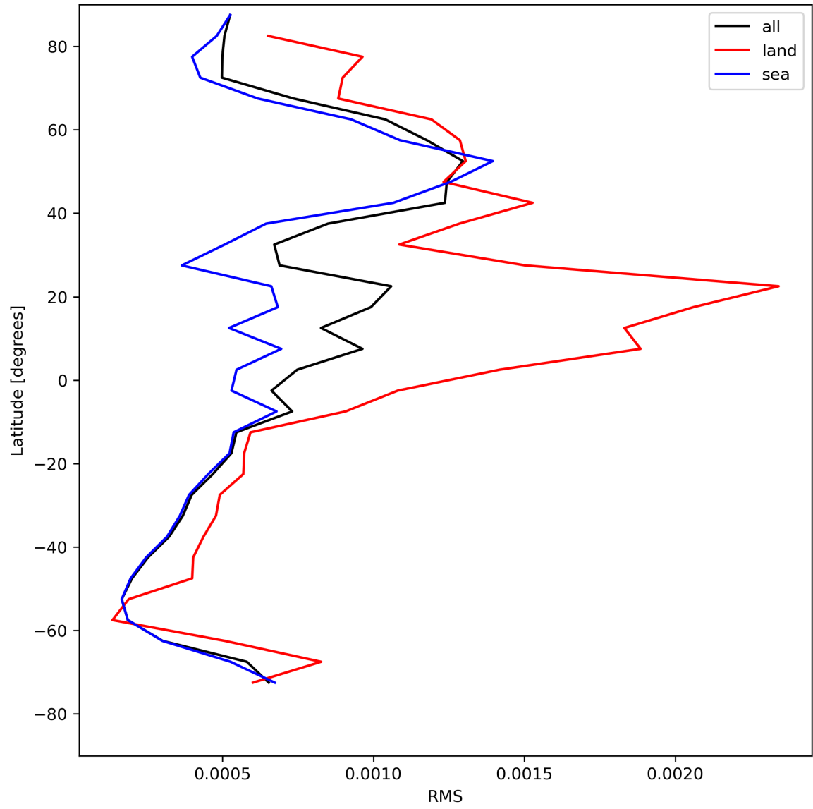
Figure 31: Zonal average of “RMS” for 2024-07-31 to 2024-08-01.
