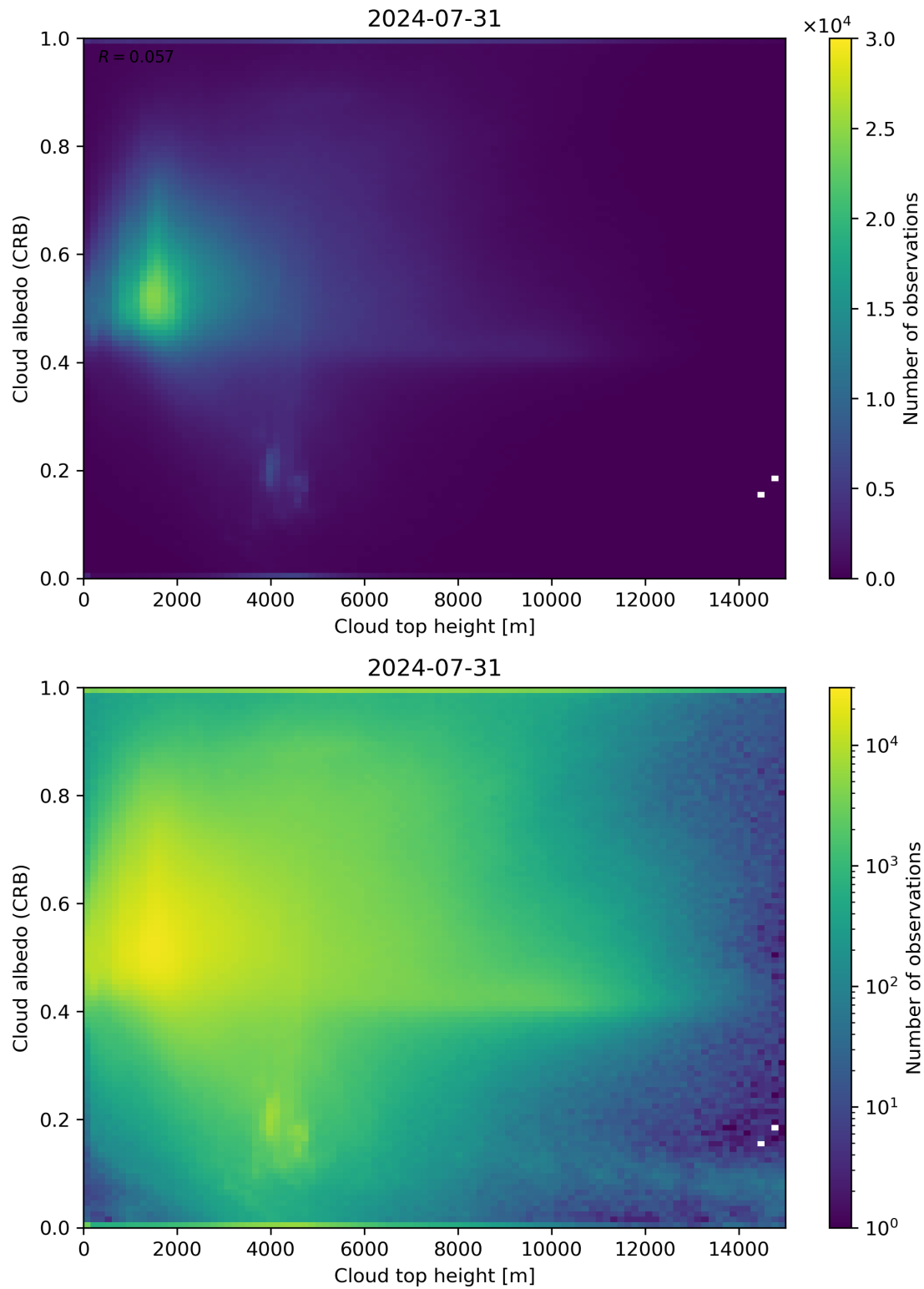
Figure 86: Scatter density plot of “Cloud top height” against “Cloud albedo (CRB)” for 2024-07-31 to 2024-08-01.
