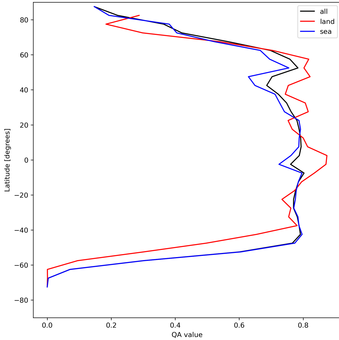
Figure 22: Zonal average of “QA value” for 2024-07-31 to 2024-08-01.
