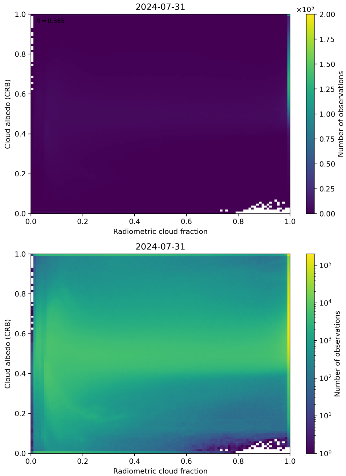
Figure 71: Scatter density plot of “Radiometric cloud fraction” against “Cloud albedo (CRB)” for 2024-07-31 to 2024-08-01.
