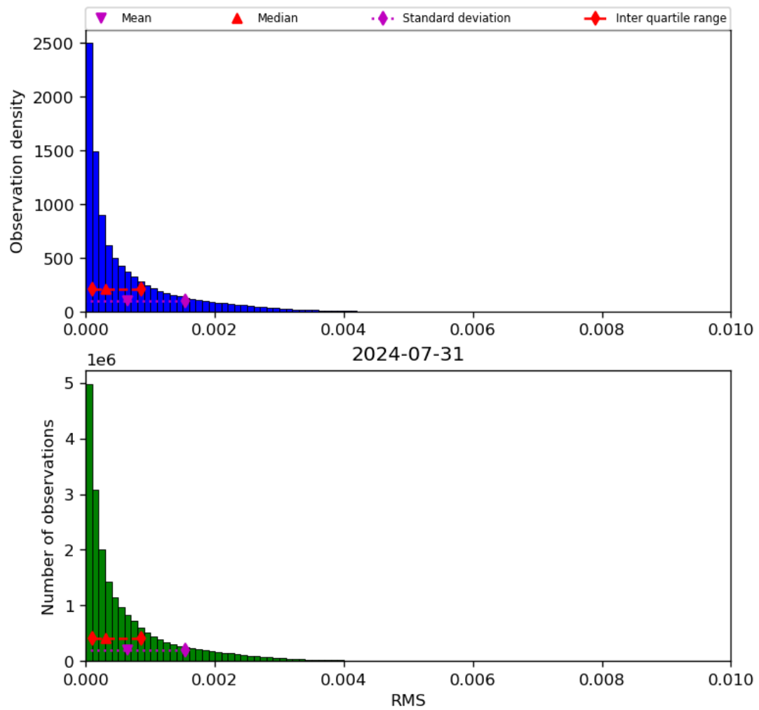
Figure 47: Histogram of “RMS” for 2024-07-31 to 2024-08-01
