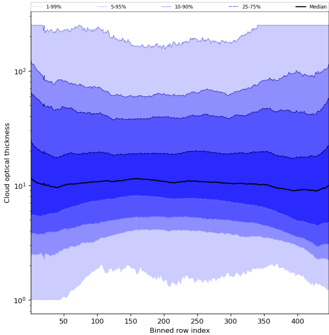
Figure 57: Along track statistics of “Cloud optical thickness” for 2024-07-31 to 2024-08-01
