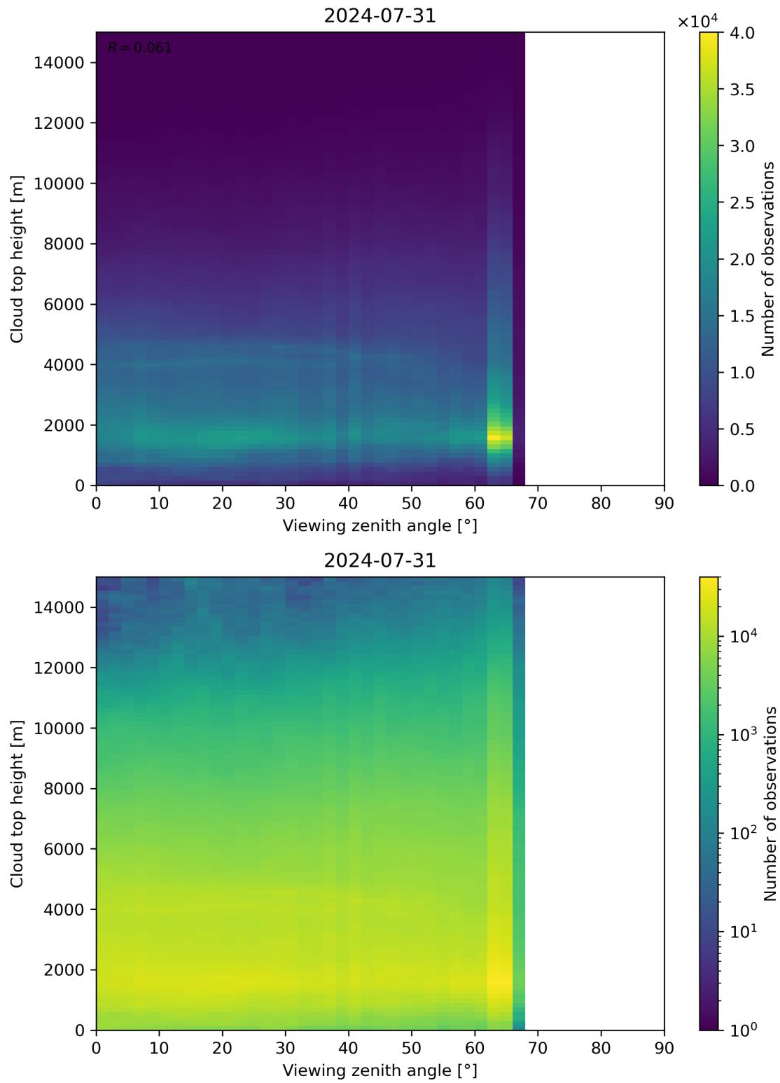
Figure 112: Scatter density plot of “Viewing zenith angle” against “Cloud top height” for 2024-07-31 to 2024-08-01.
