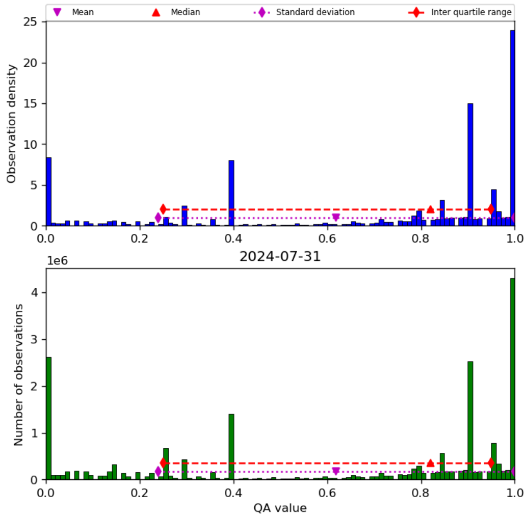
Figure 38: Histogram of “QA value” for 2024-07-31 to 2024-08-01
