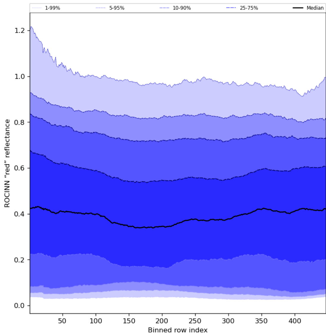
Figure 69: Along track statistics of “ROCINN “red” reflectance” for 2024-07-31 to 2024-08-01
