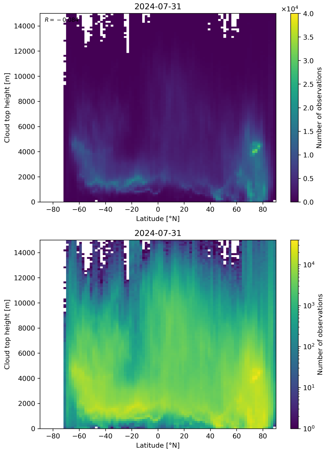
Figure 97: Scatter density plot of “Latitude” against “Cloud top height” for 2024-07-31 to 2024-08-01.
