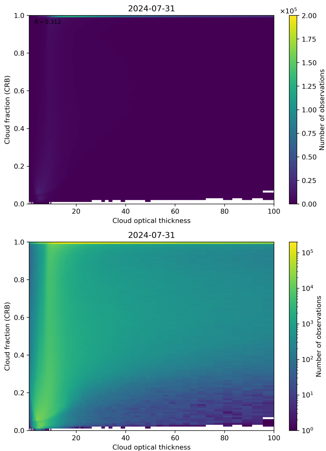
Figure 84: Scatter density plot of “Cloud optical thickness” against “Cloud fraction (CRB)” for 2024-07-31 to 2024-08-01.
