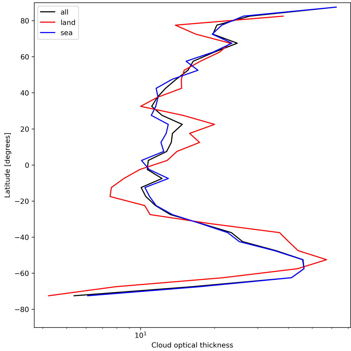
Figure 25: Zonal average of “Cloud optical thickness” for 2024-07-31 to 2024-08-01.
