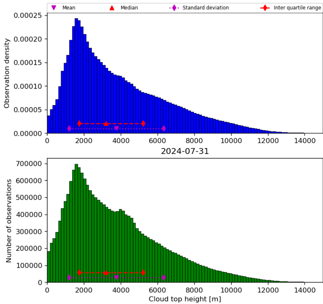
Figure 40: Histogram of “Cloud top height” for 2024-07-31 to 2024-08-01
