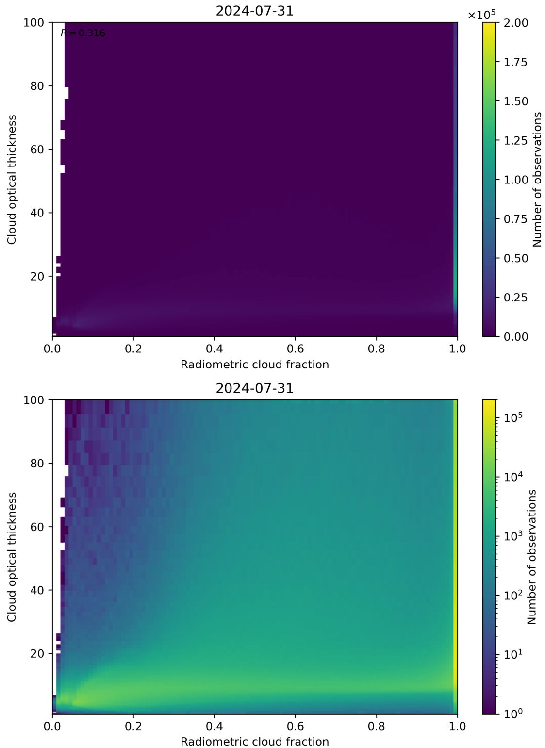
Figure 75: Scatter density plot of “Radiometric cloud fraction” against “Cloud optical thickness” for 2024-07-31 to 2024-08-01.
