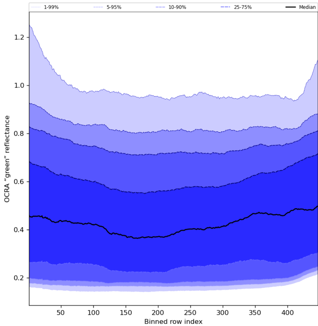
Figure 68: Along track statistics of “OCRA “green” reflectance” for 2024-07-31 to 2024-08-01
