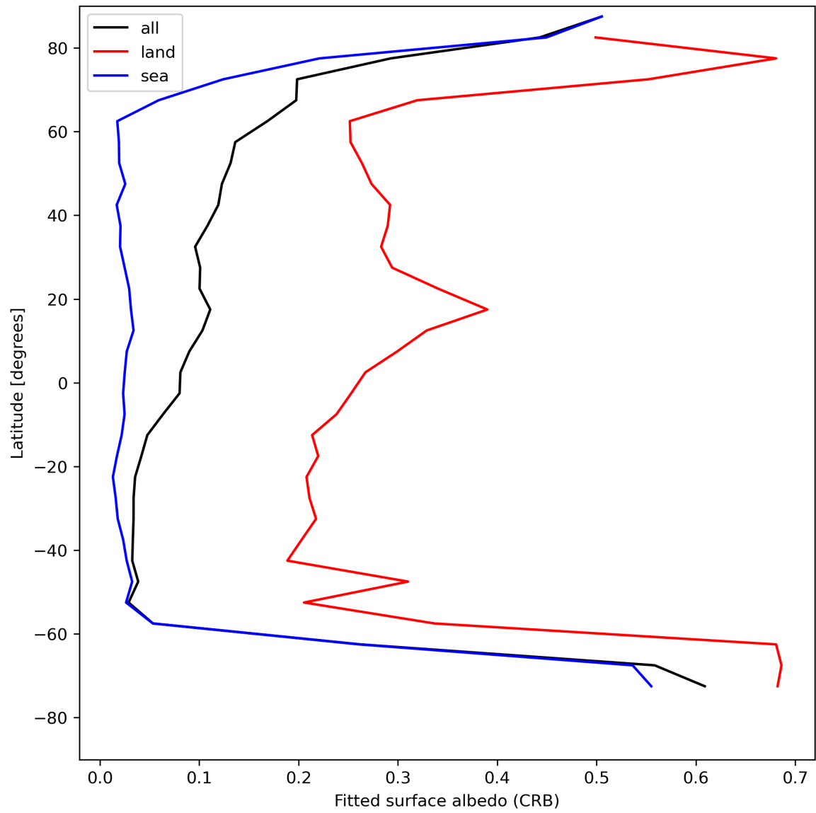
Figure 30: Zonal average of “Fitted surface albedo (CRB)” for 2024-07-31 to 2024-08-01.
