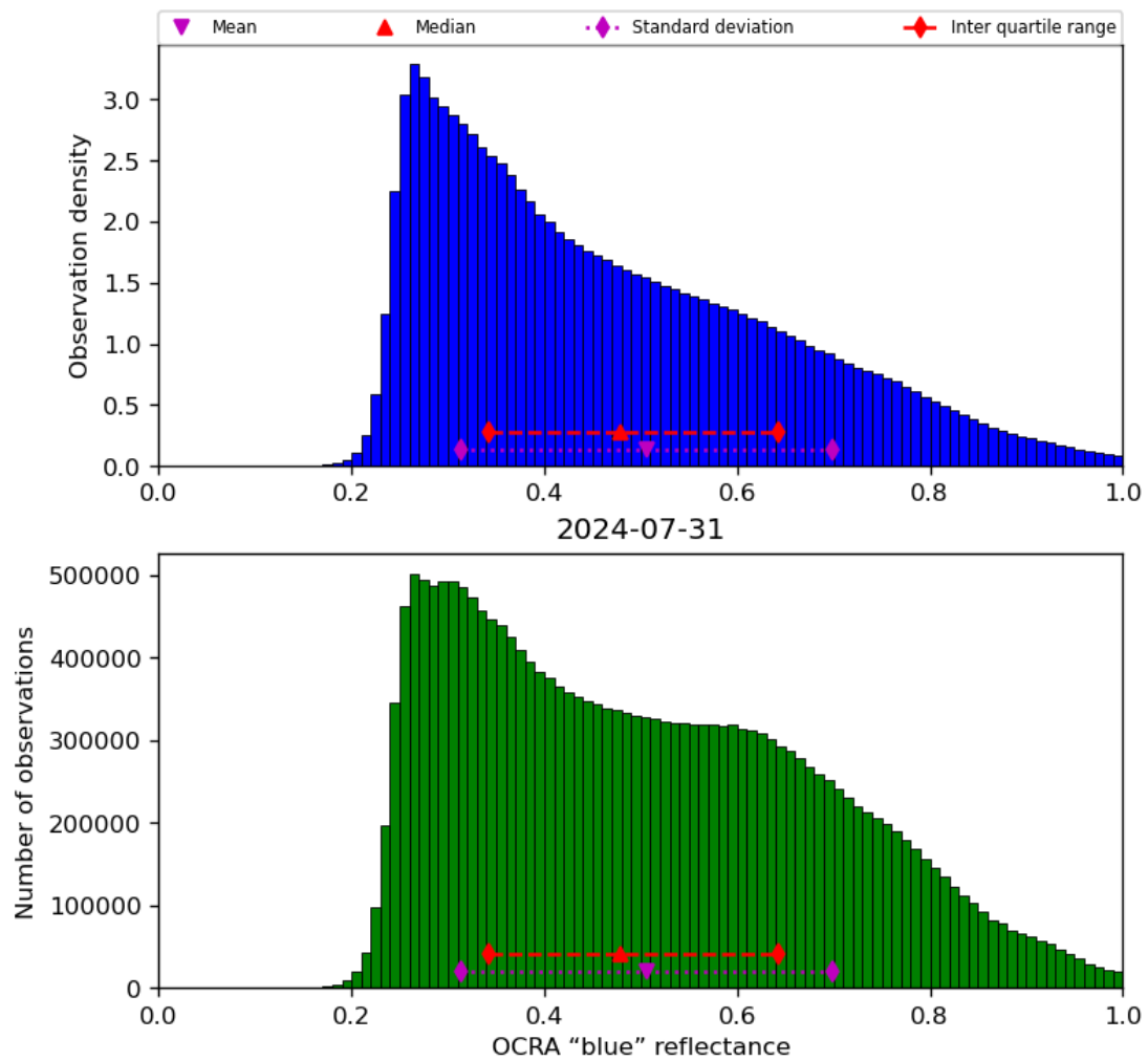
Figure 51: Histogram of “OCRA “blue” reflectance” for 2024-07-31 to 2024-08-01
