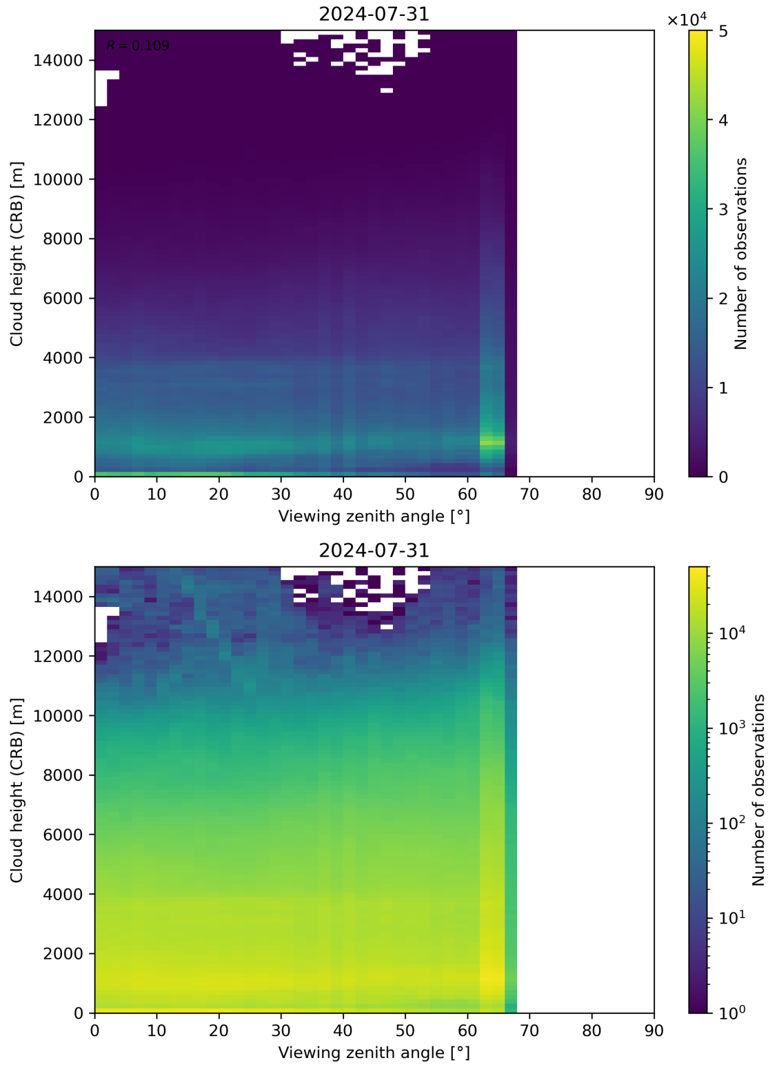
Figure 110: Scatter density plot of “Viewing zenith angle” against “Cloud height (CRB)” for 2024-07-31 to 2024-08-01.
