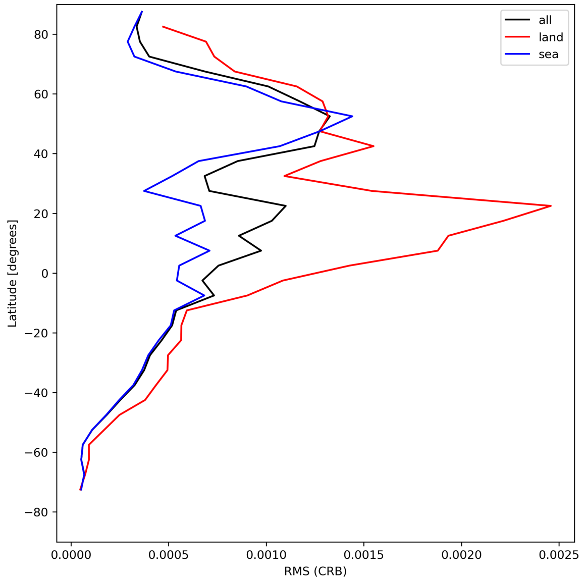
Figure 32: Zonal average of “RMS (CRB)” for 2024-07-31 to 2024-08-01.
