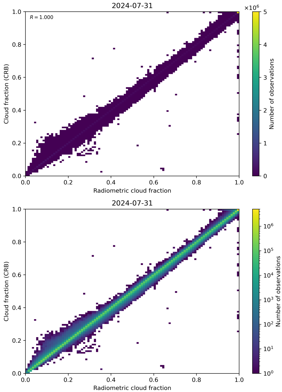
Figure 73: Scatter density plot of “Radiometric cloud fraction” against “Cloud fraction (CRB)” for 2024-07-31 to 2024-08-01.
