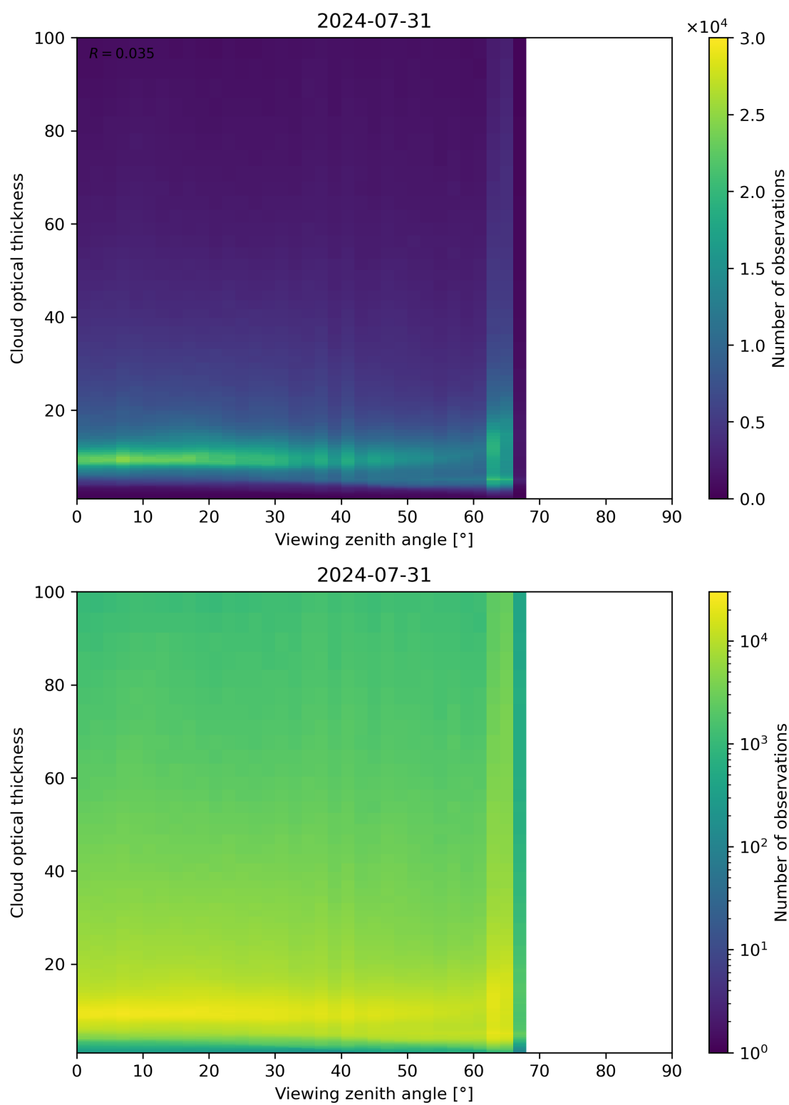
Figure 111: Scatter density plot of “Viewing zenith angle” against “Cloud optical thickness” for 2024-07-31 to 2024-08-01.
