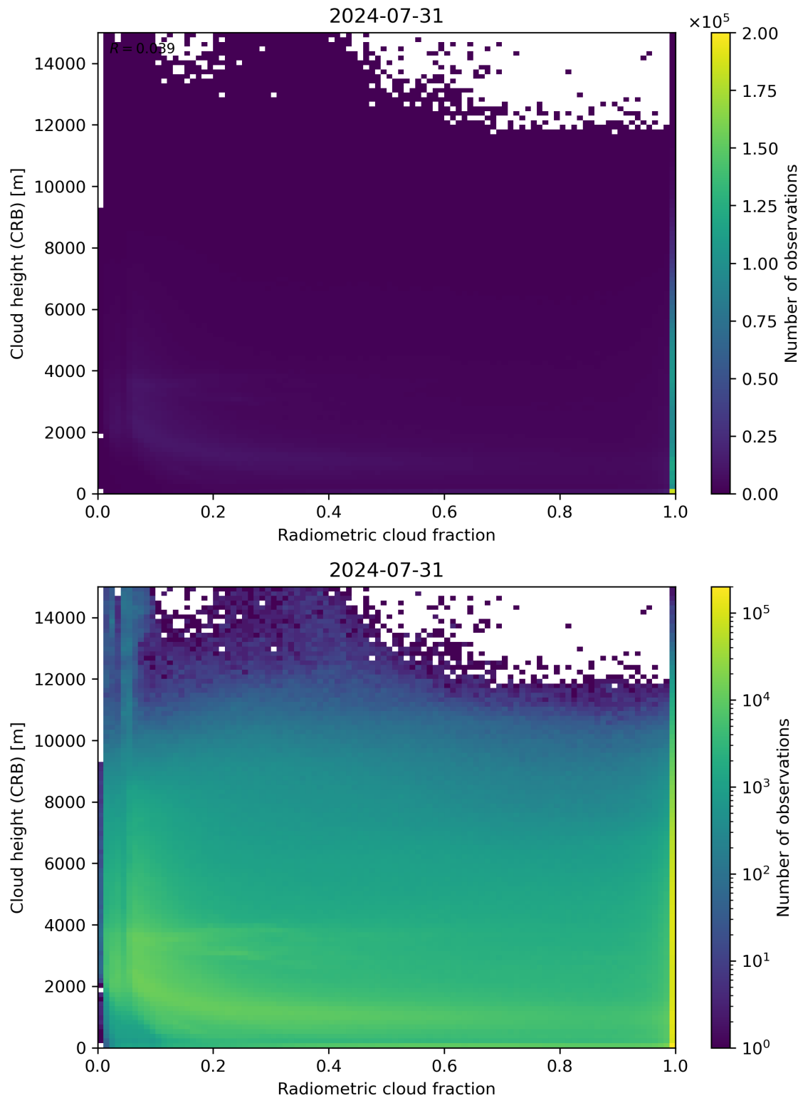
Figure 74: Scatter density plot of “Radiometric cloud fraction” against “Cloud height (CRB)” for 2024-07-31 to 2024-08-01.
