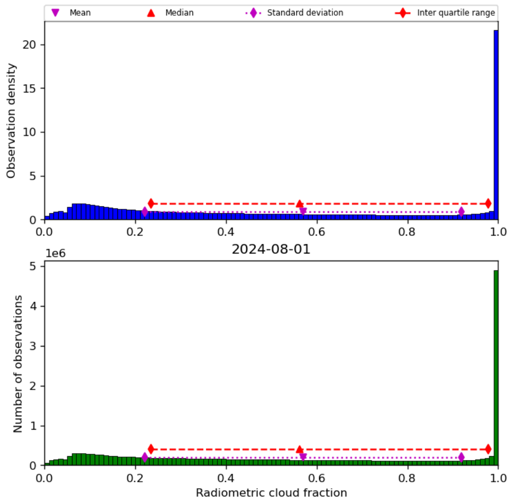
Figure 39: Histogram of “Radiometric cloud fraction” for 2024-07-31 to 2024-08-02
