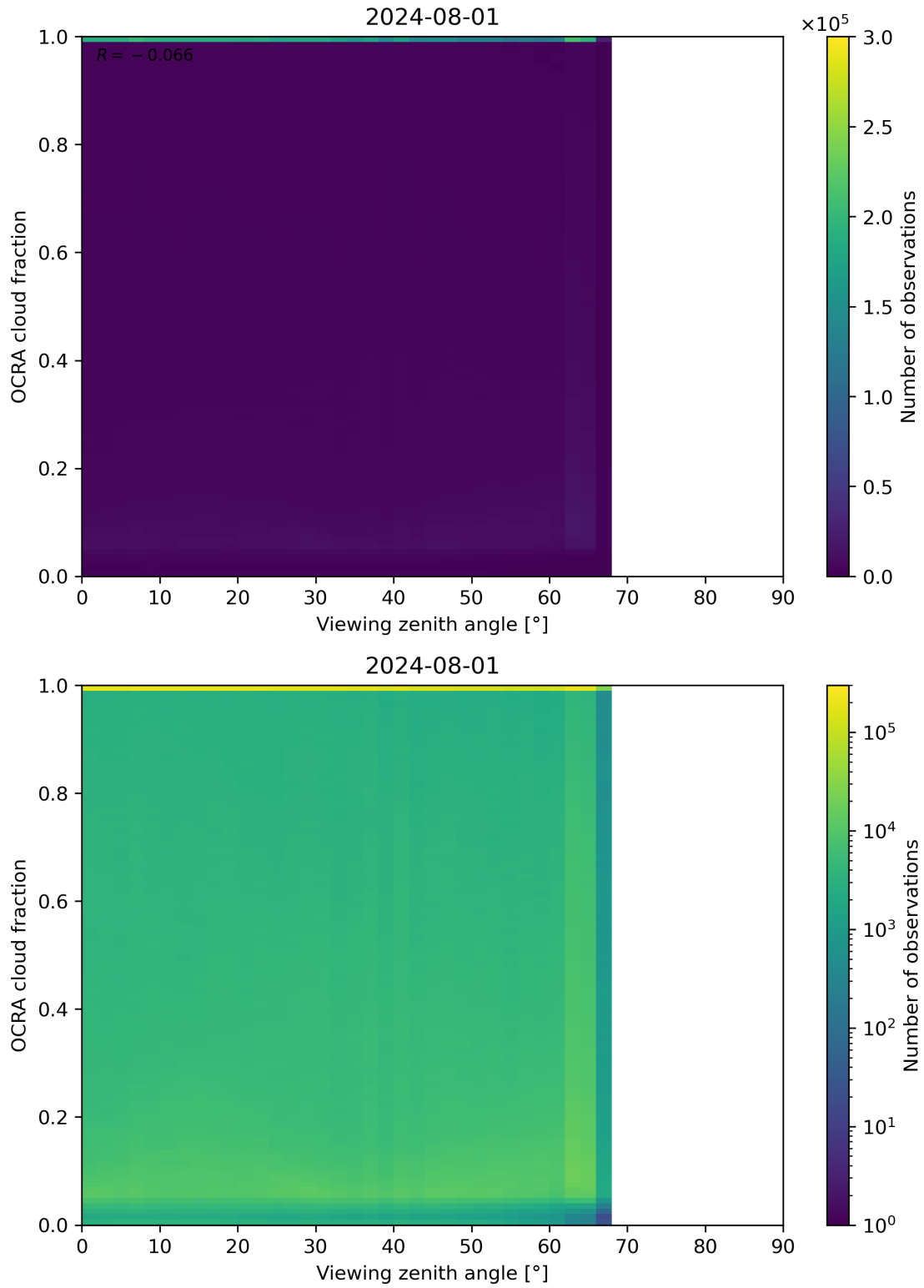
Figure 108: Scatter density plot of “Viewing zenith angle” against “OCRA cloud fraction” for 2024-07-31 to 2024-08-02.
