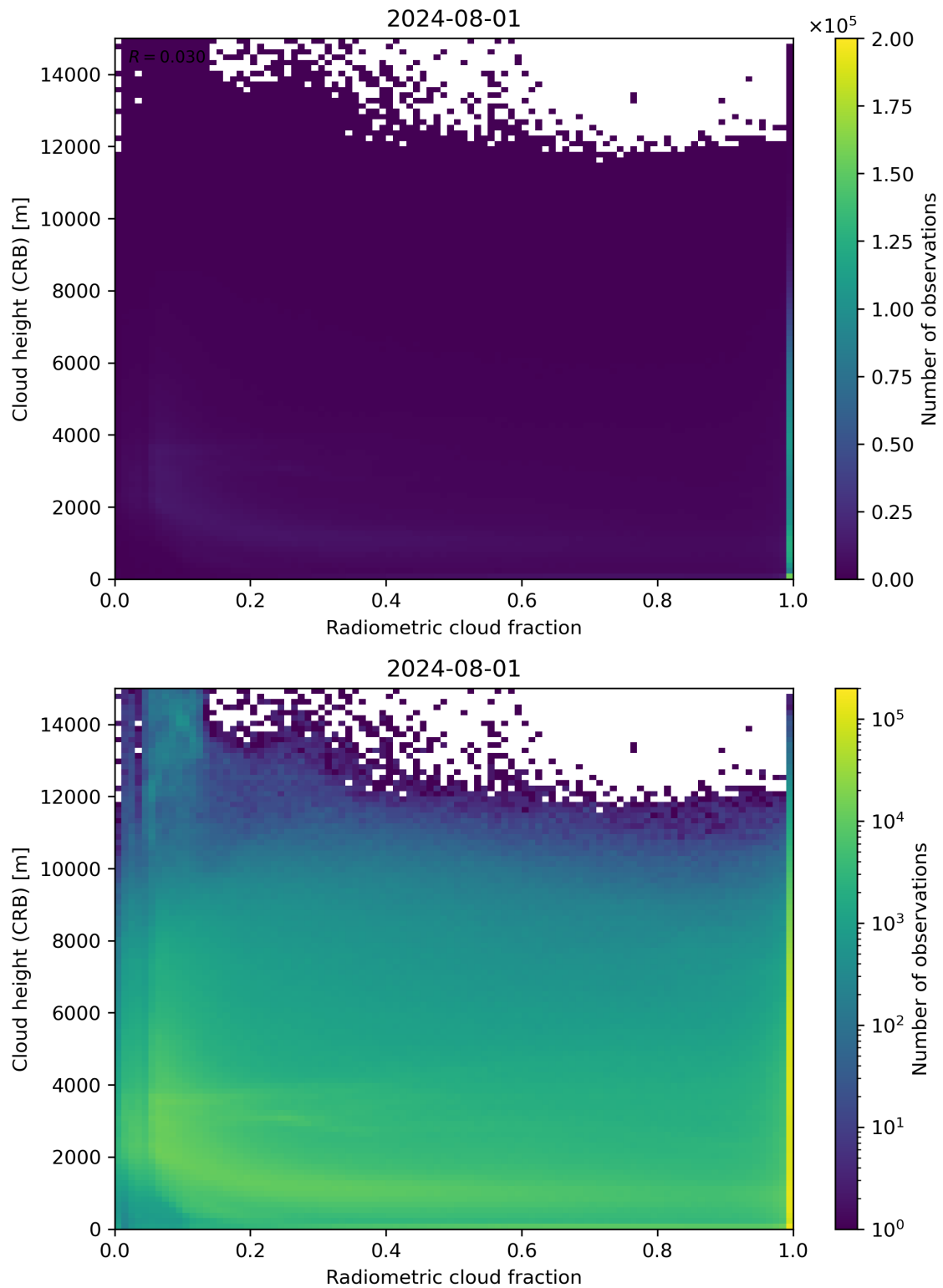
Figure 74: Scatter density plot of “Radiometric cloud fraction” against “Cloud height (CRB)” for 2024-07-31 to 2024-08-02.
