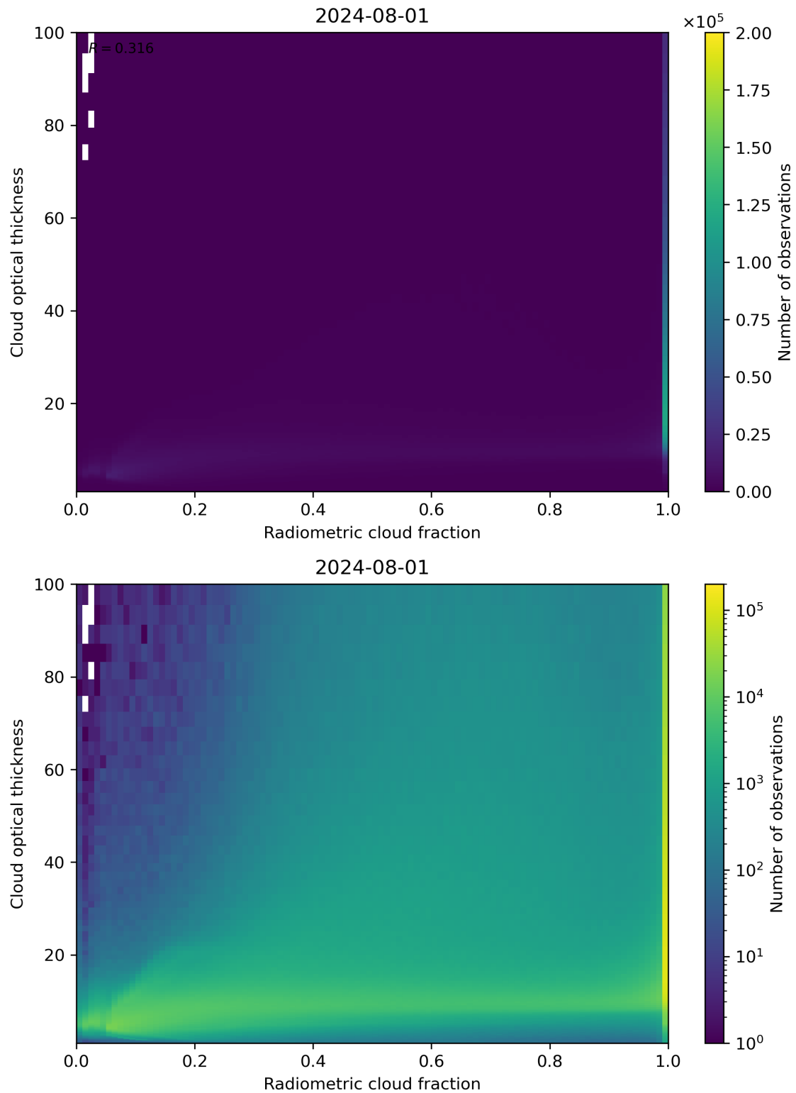
Figure 75: Scatter density plot of “Radiometric cloud fraction” against “Cloud optical thickness” for 2024-07-31 to 2024-08-02.
