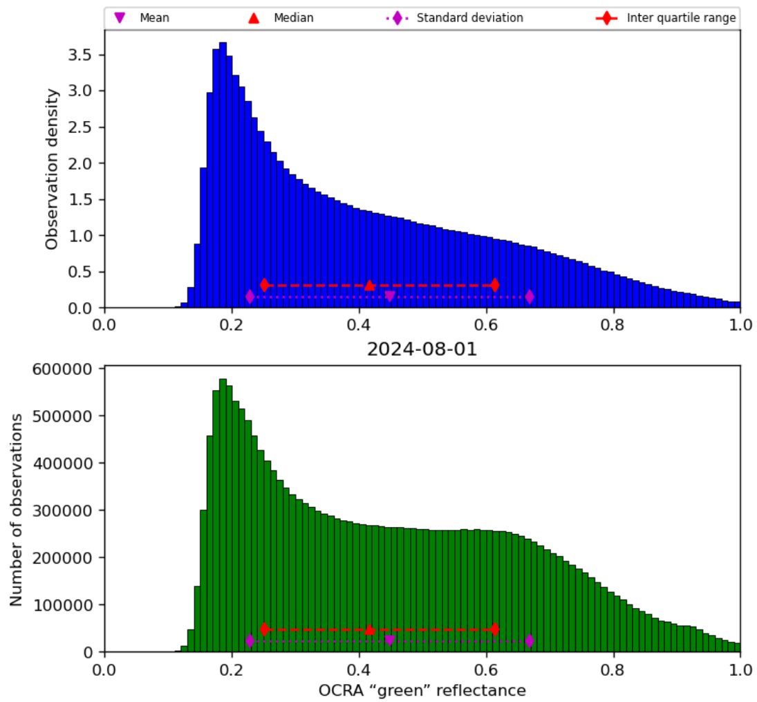
Figure 52: Histogram of “OCRA “green” reflectance” for 2024-07-31 to 2024-08-02
