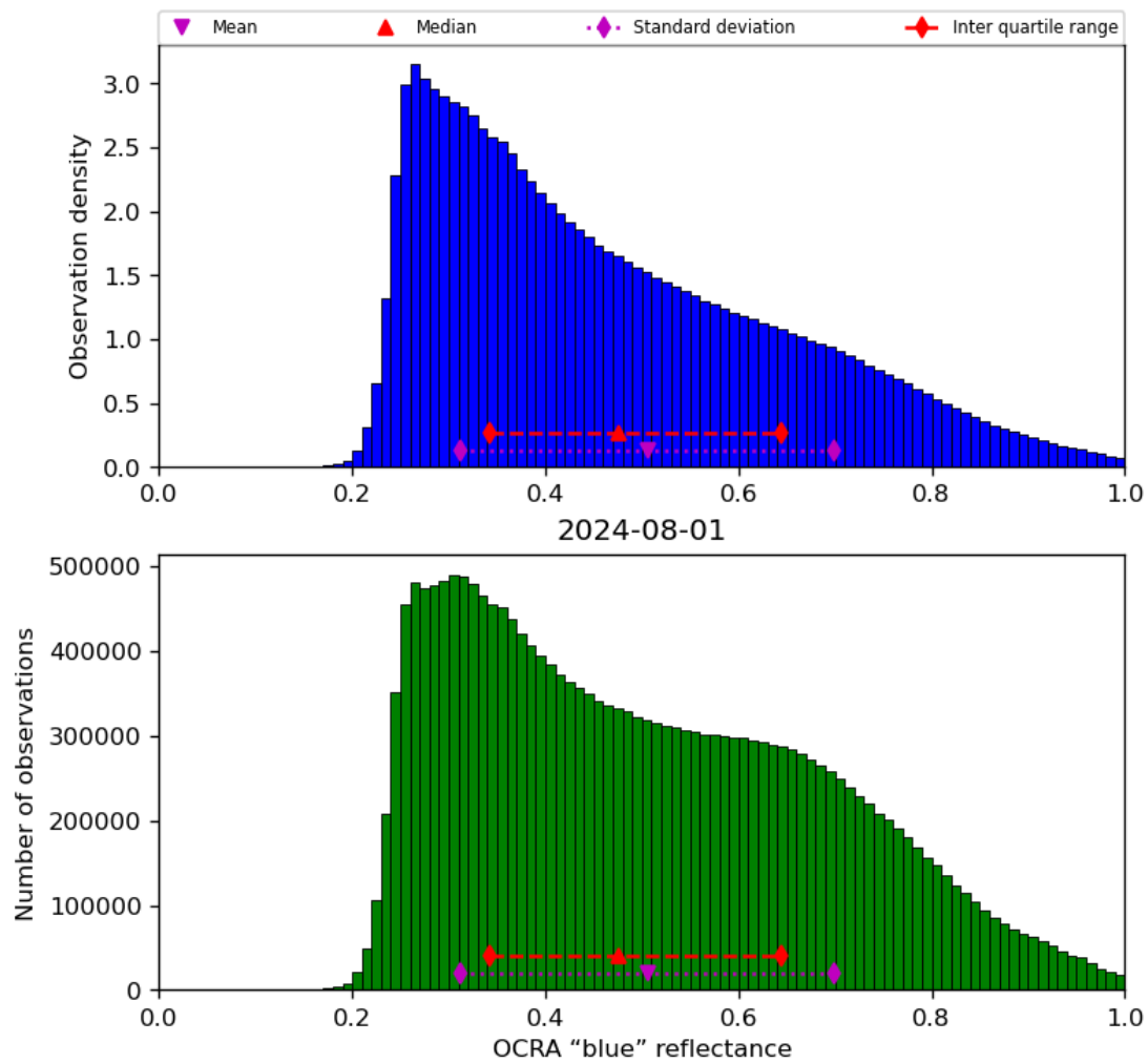
Figure 51: Histogram of “OCRA “blue” reflectance” for 2024-07-31 to 2024-08-02
