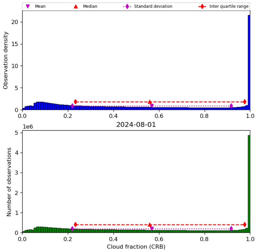
Figure 42: Histogram of “Cloud fraction (CRB)” for 2024-07-31 to 2024-08-02
