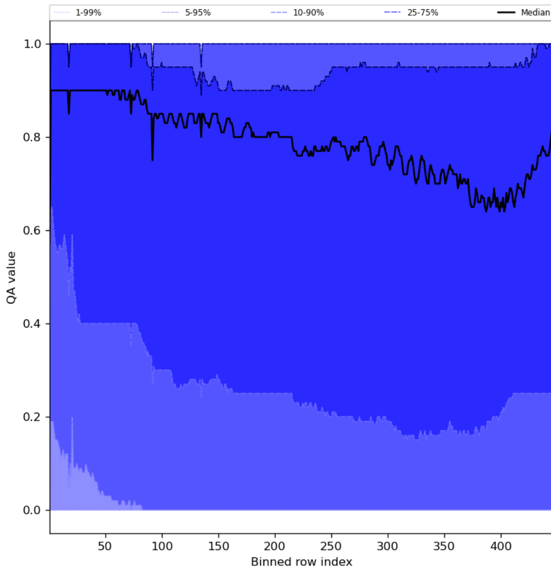
Figure 54: Along track statistics of “QA value” for 2024-07-31 to 2024-08-02
