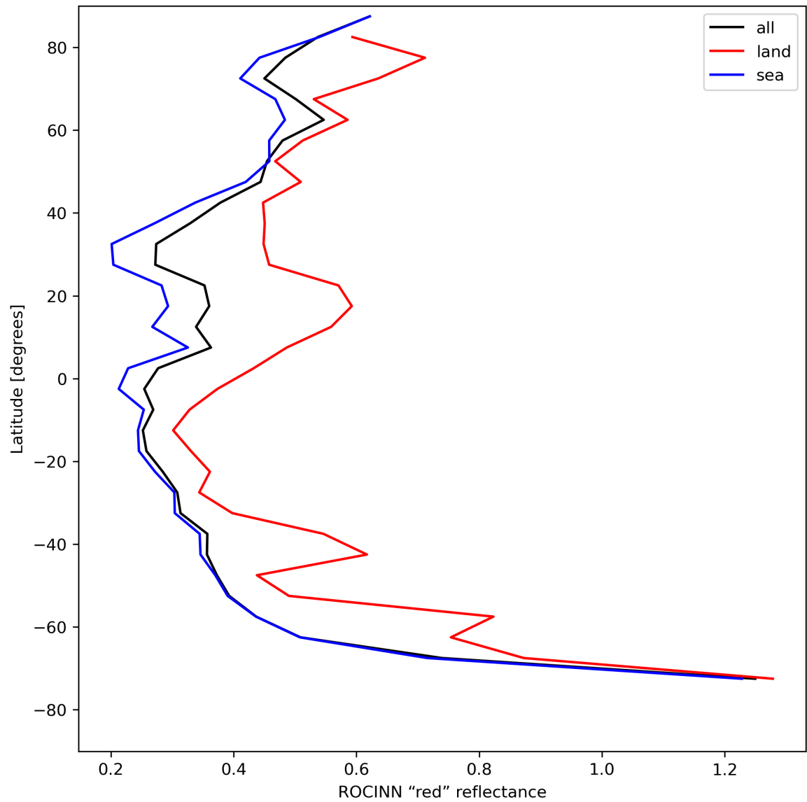
Figure 37: Zonal average of “ROCINN “red” reflectance” for 2024-07-31 to 2024-08-02.
