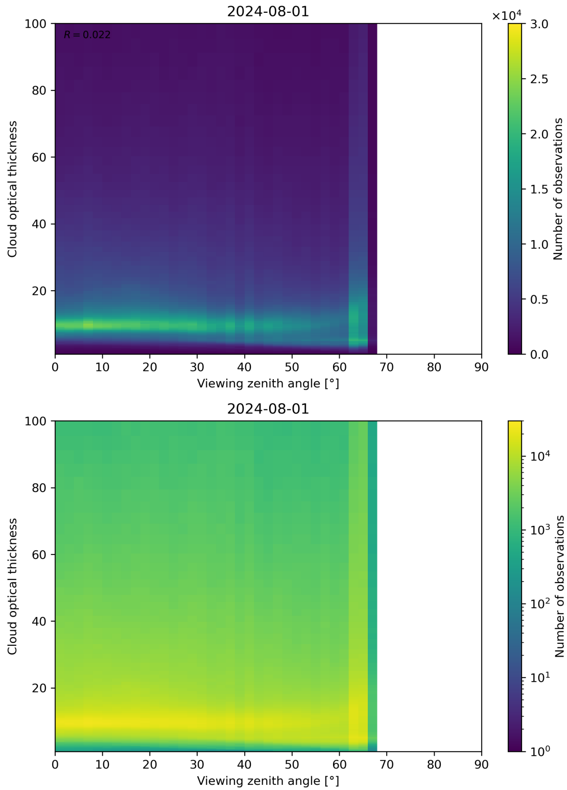
Figure 111: Scatter density plot of “Viewing zenith angle” against “Cloud optical thickness” for 2024-07-31 to 2024-08-02.
