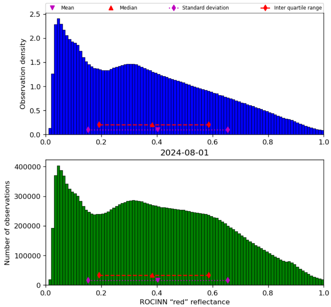
Figure 53: Histogram of “ROCINN “red” reflectance” for 2024-07-31 to 2024-08-02
