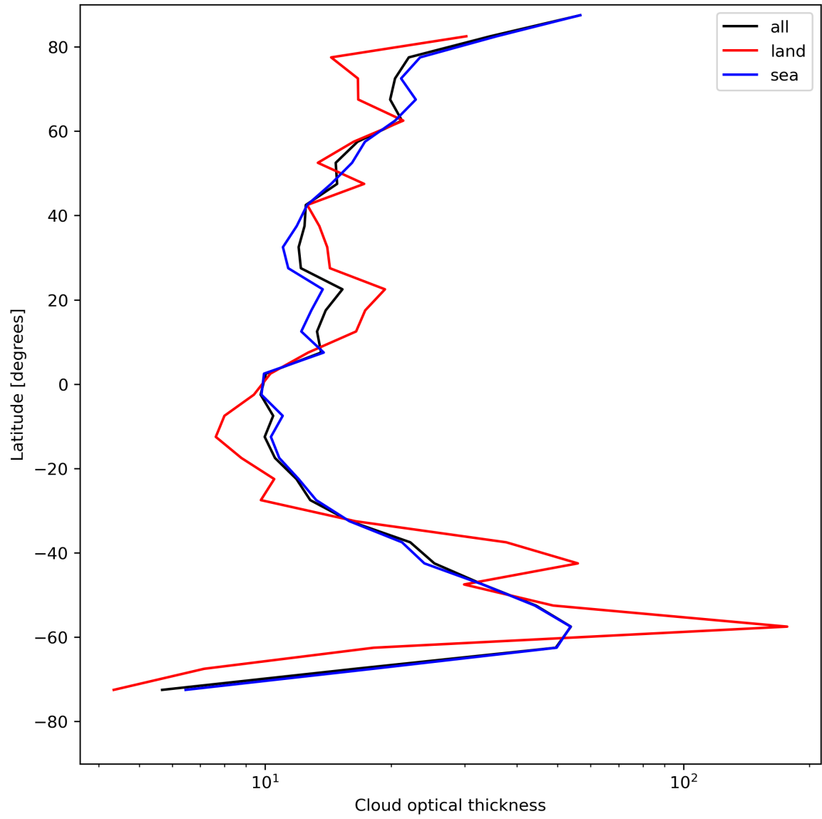
Figure 25: Zonal average of “Cloud optical thickness” for 2024-07-31 to 2024-08-02.
