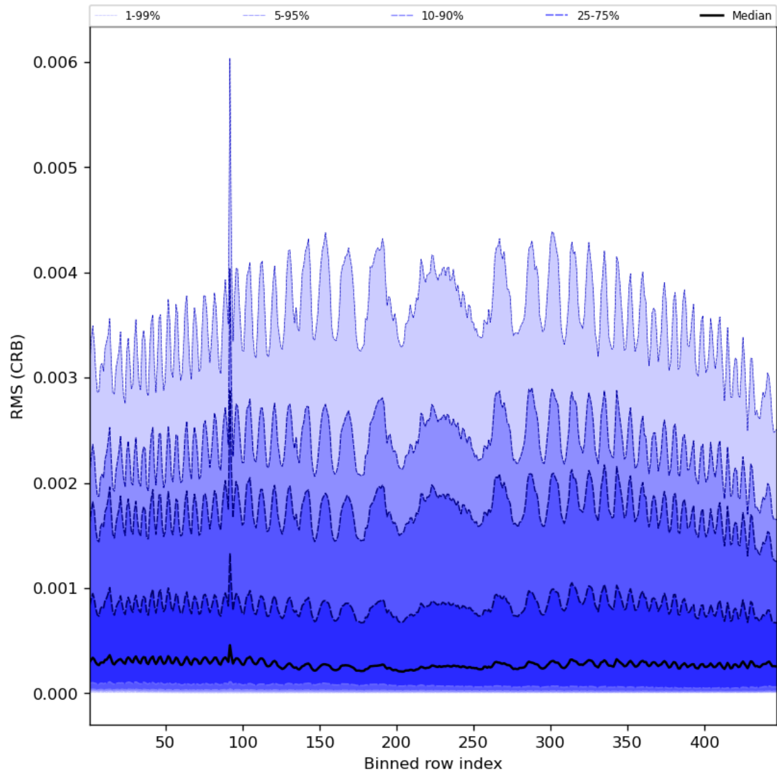
Figure 64: Along track statistics of “RMS (CRB)” for 2024-07-31 to 2024-08-02
