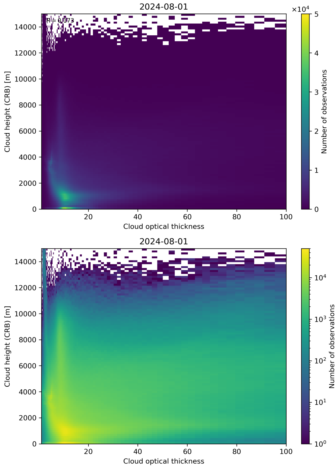
Figure 85: Scatter density plot of “Cloud optical thickness” against “Cloud height (CRB)” for 2024-07-31 to 2024-08-02.
