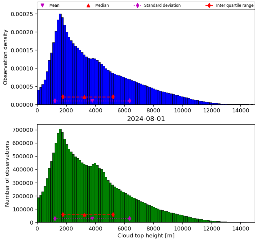
Figure 40: Histogram of “Cloud top height” for 2024-07-31 to 2024-08-02
