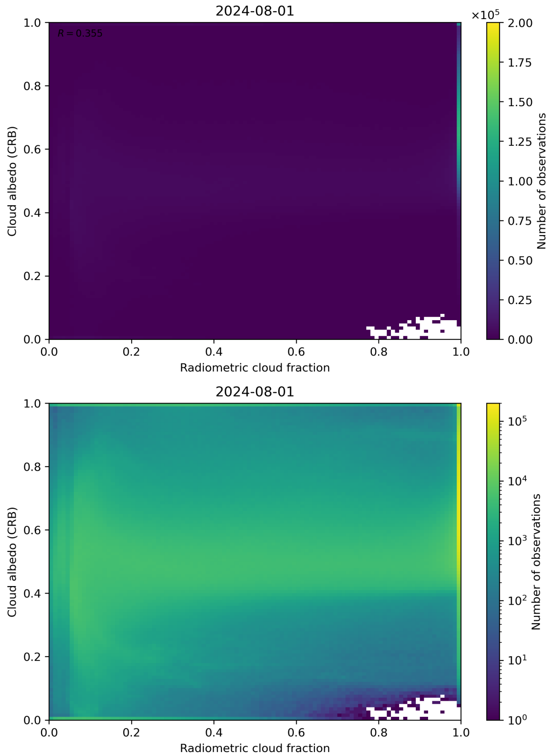
Figure 71: Scatter density plot of “Radiometric cloud fraction” against “Cloud albedo (CRB)” for 2024-07-31 to 2024-08-02.
