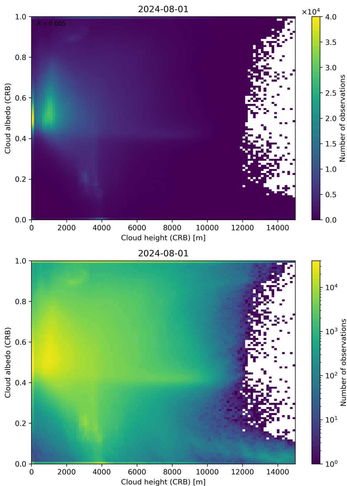
Figure 80: Scatter density plot of “Cloud height (CRB)” against “Cloud albedo (CRB)” for 2024-07-31 to 2024-08-02.
