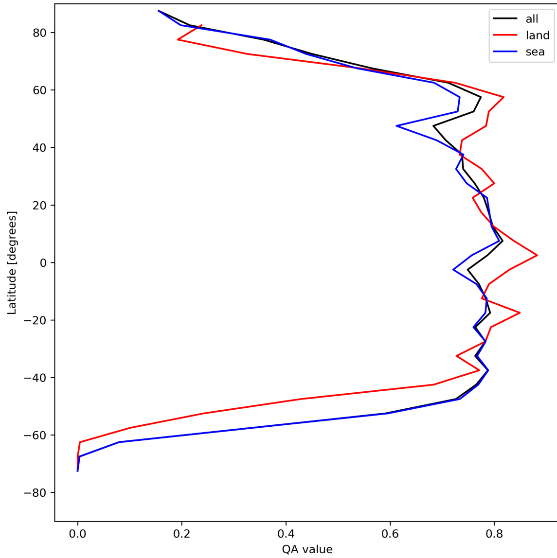
Figure 22: Zonal average of “QA value” for 2024-07-31 to 2024-08-02.
