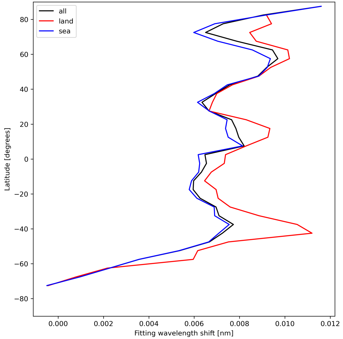
Figure 33: Zonal average of “Fitting wavelength shift” for 2024-07-31 to 2024-08-02.
