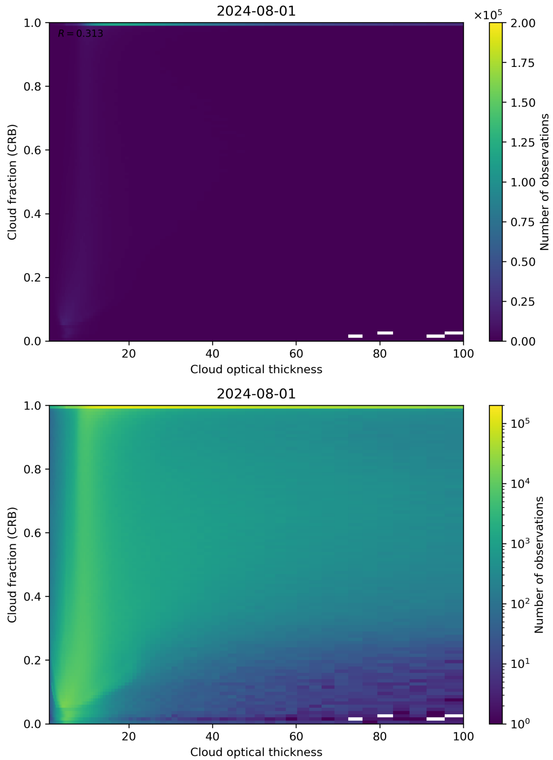
Figure 84: Scatter density plot of “Cloud optical thickness” against “Cloud fraction (CRB)” for 2024-07-31 to 2024-08-02.
