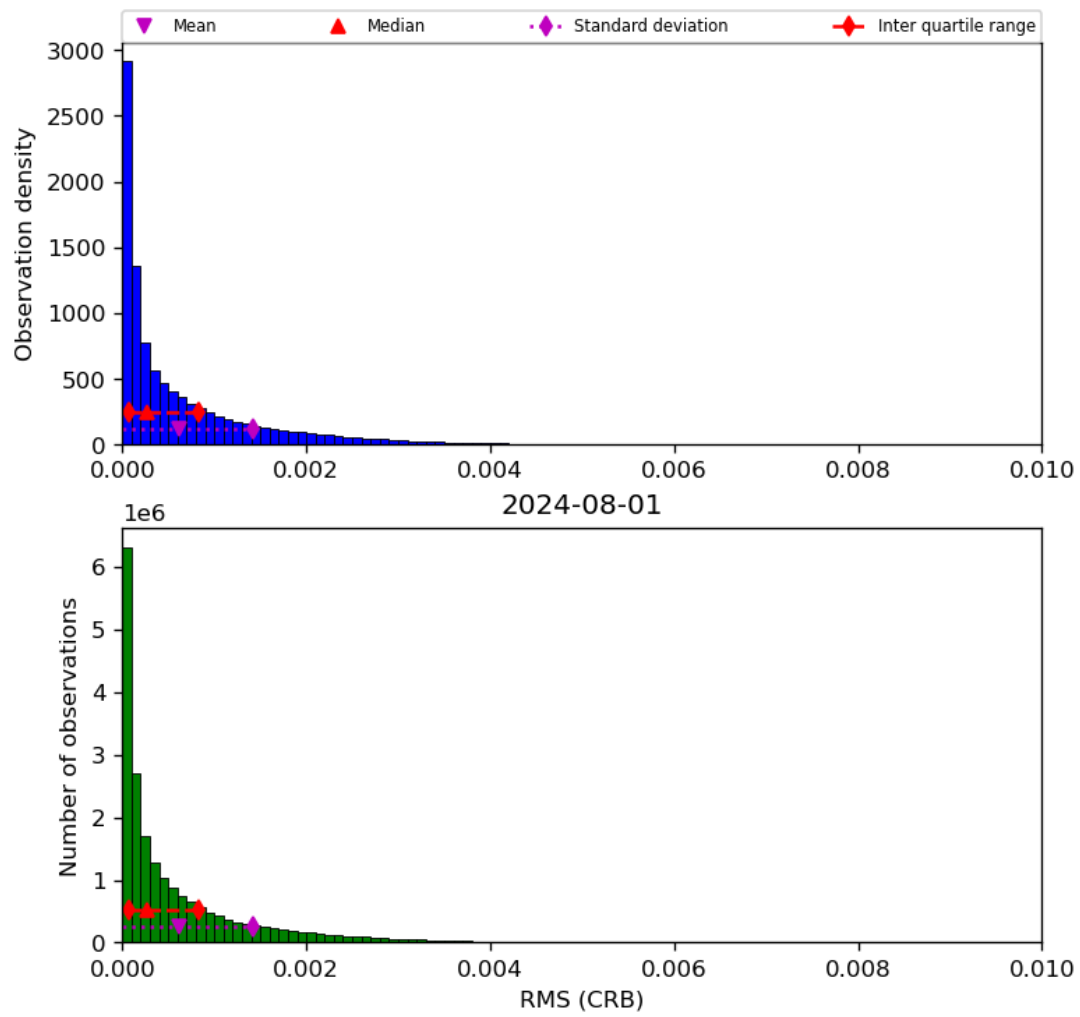
Figure 48: Histogram of “RMS (CRB)” for 2024-07-31 to 2024-08-02
