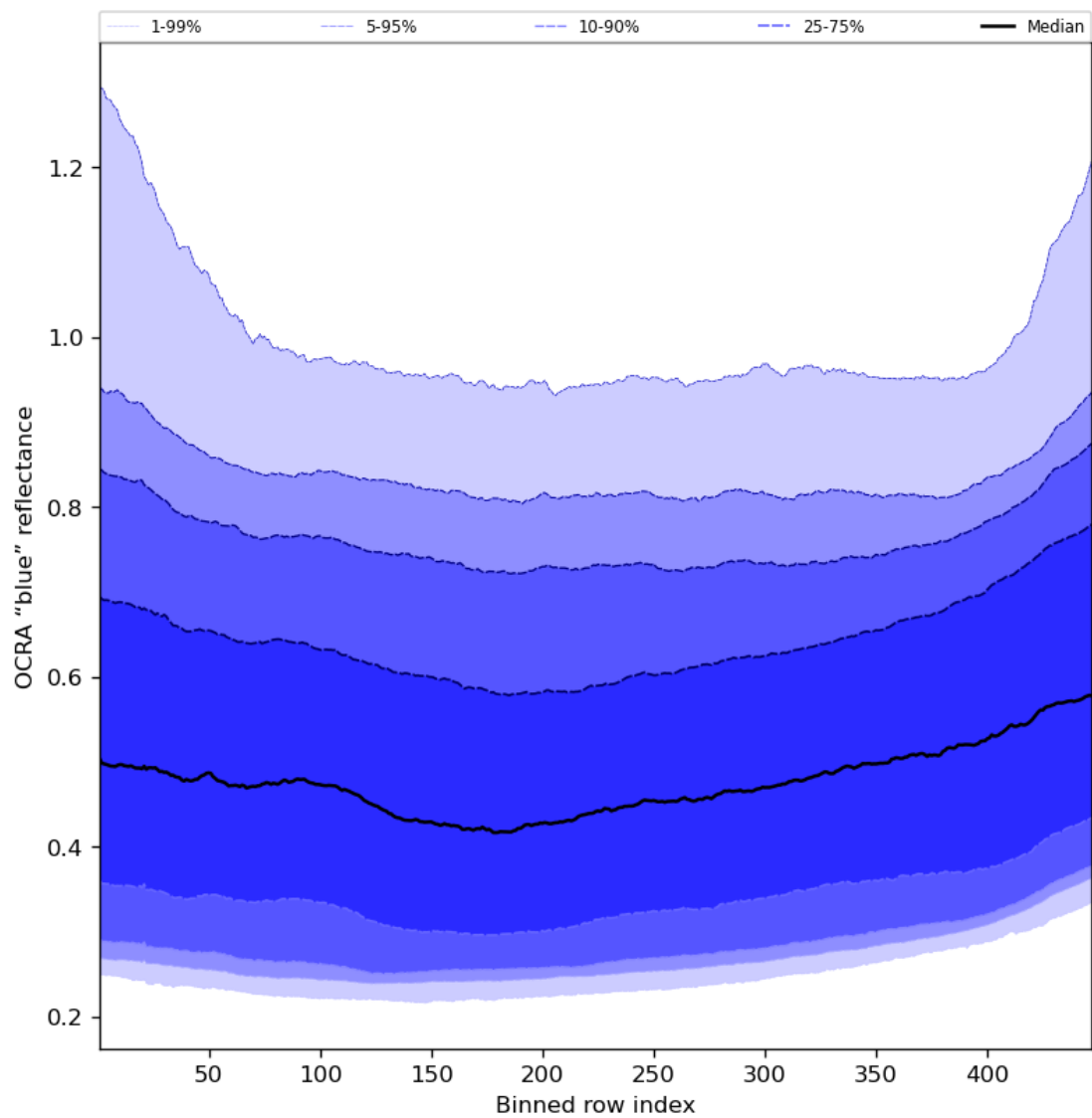
Figure 67: Along track statistics of “OCRA “blue” reflectance” for 2024-07-31 to 2024-08-02
