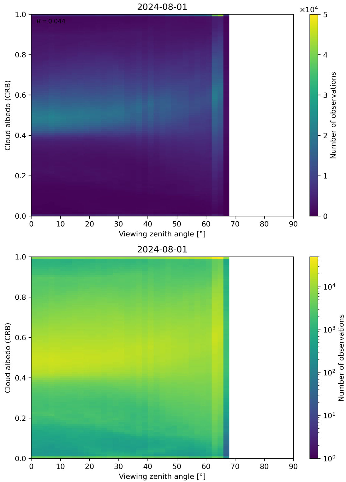
Figure 106: Scatter density plot of “Viewing zenith angle” against “Cloud albedo (CRB)” for 2024-07-31 to 2024-08-02.
