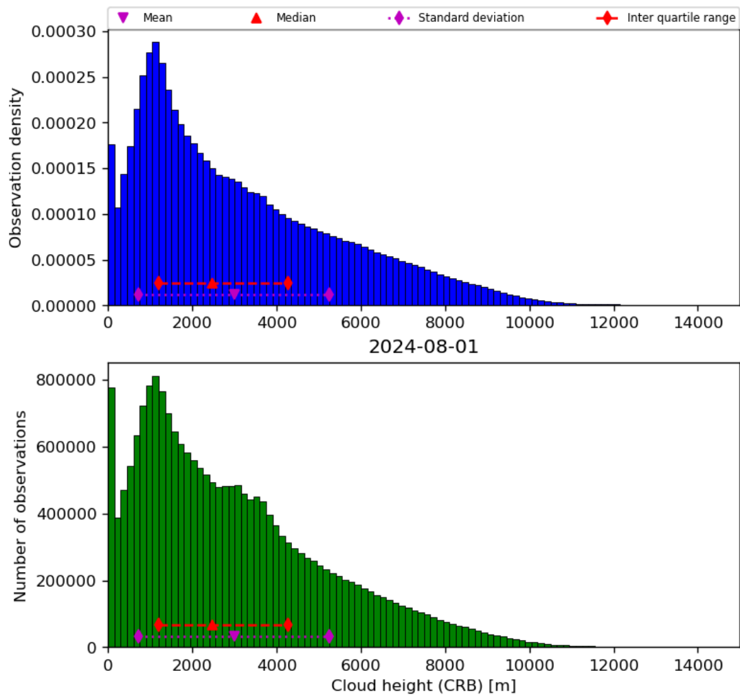
Figure 43: Histogram of “Cloud height (CRB)” for 2024-07-31 to 2024-08-02
