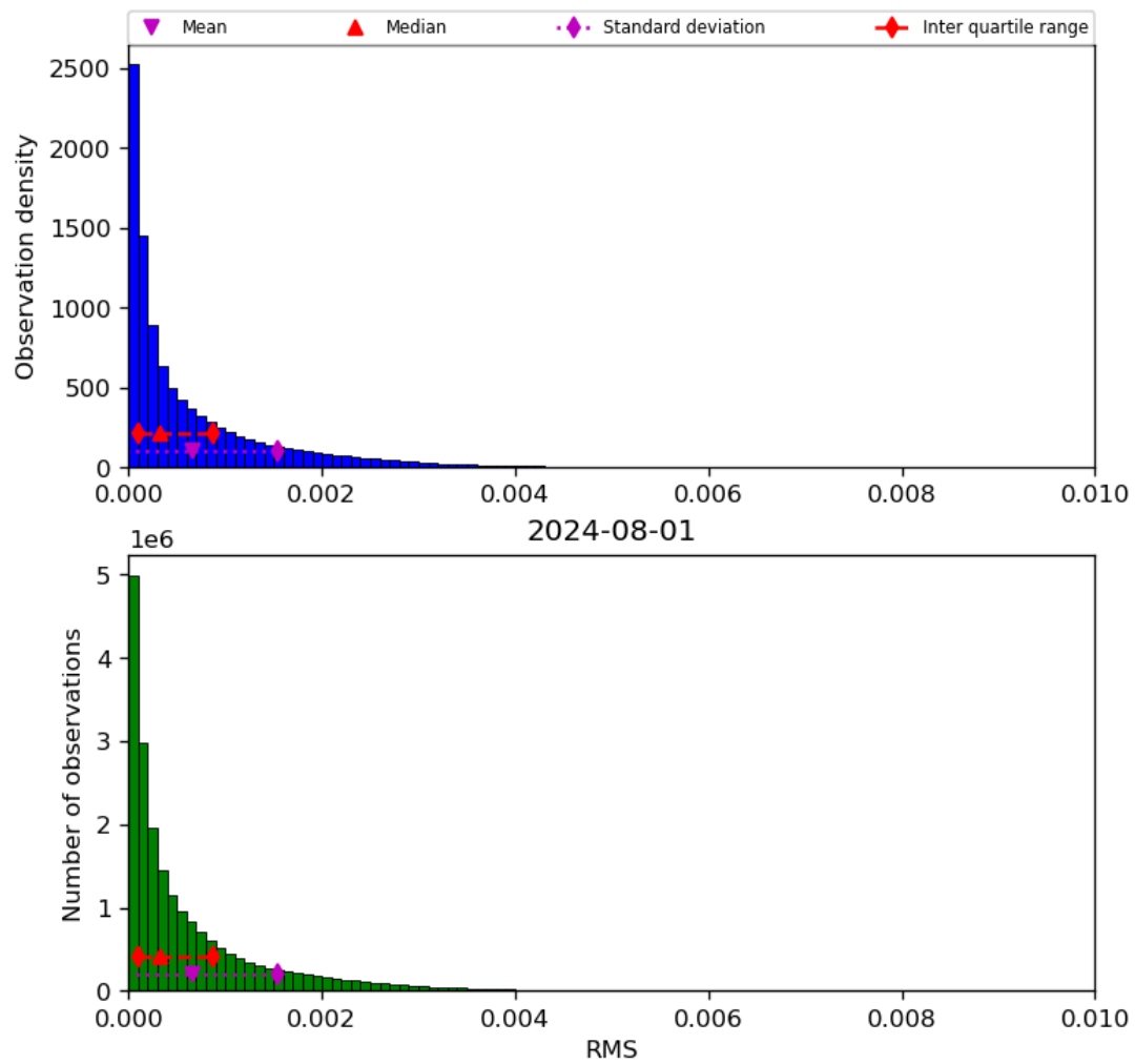
Figure 47: Histogram of “RMS” for 2024-07-31 to 2024-08-02
