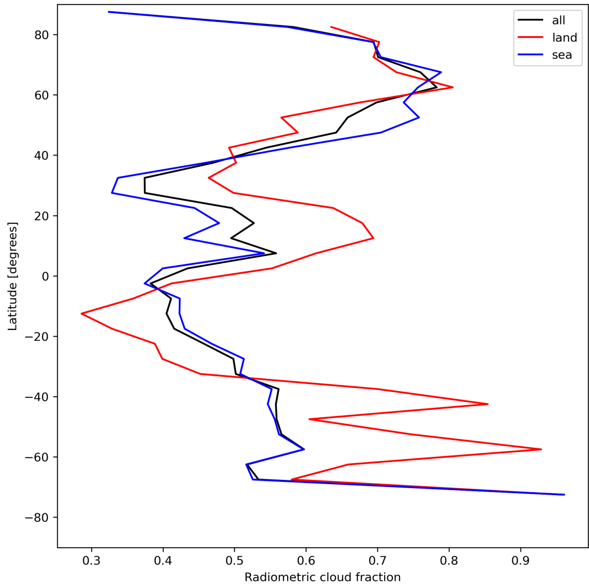
Figure 23: Zonal average of “Radiometric cloud fraction” for 2024-07-31 to 2024-08-02.
