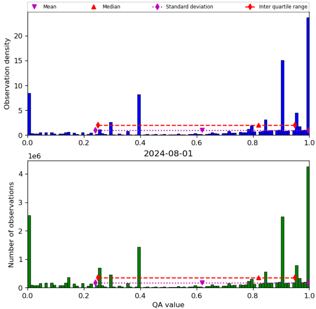
Figure 38: Histogram of “QA value” for 2024-07-31 to 2024-08-02
