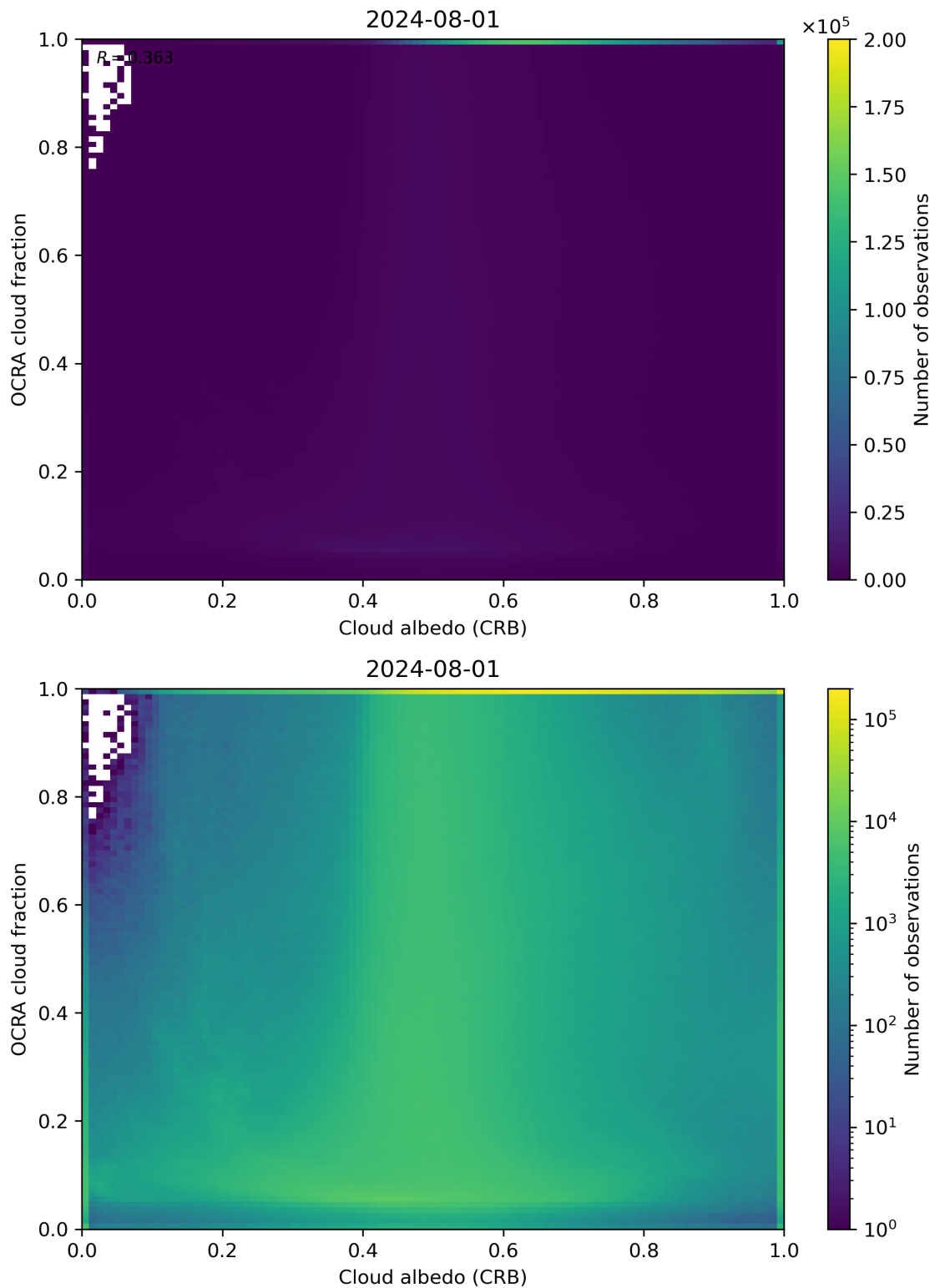
Figure 70: Scatter density plot of “Cloud albedo (CRB)” against “OCRA cloud fraction” for 2024-07-31 to 2024-08-02.
