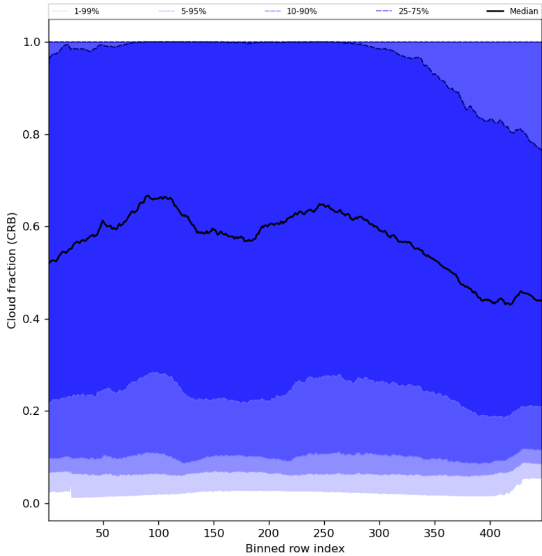
Figure 58: Along track statistics of “Cloud fraction (CRB)” for 2024-07-31 to 2024-08-02
