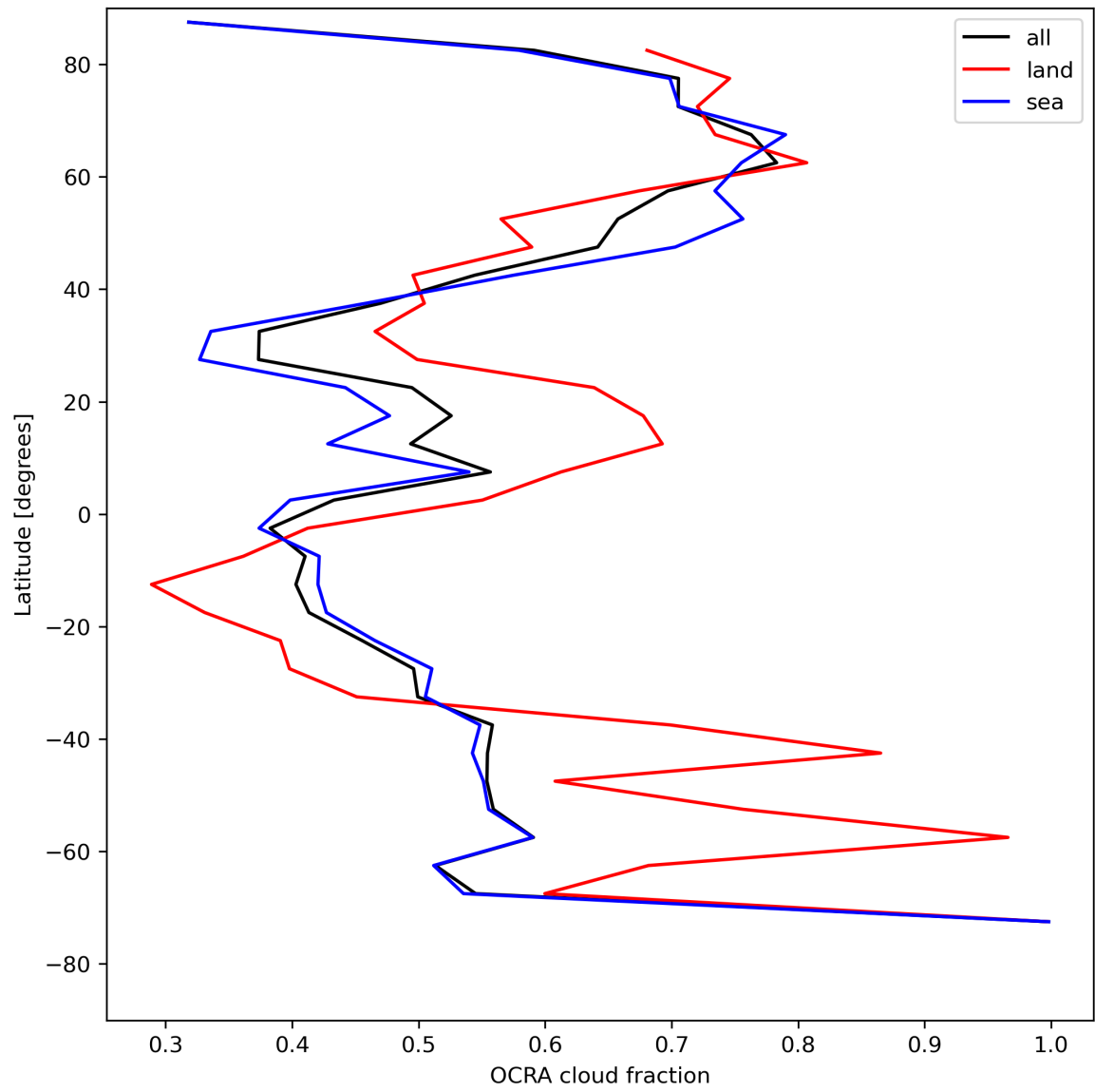
Figure 34: Zonal average of “OCRA cloud fraction” for 2024-07-31 to 2024-08-02.
