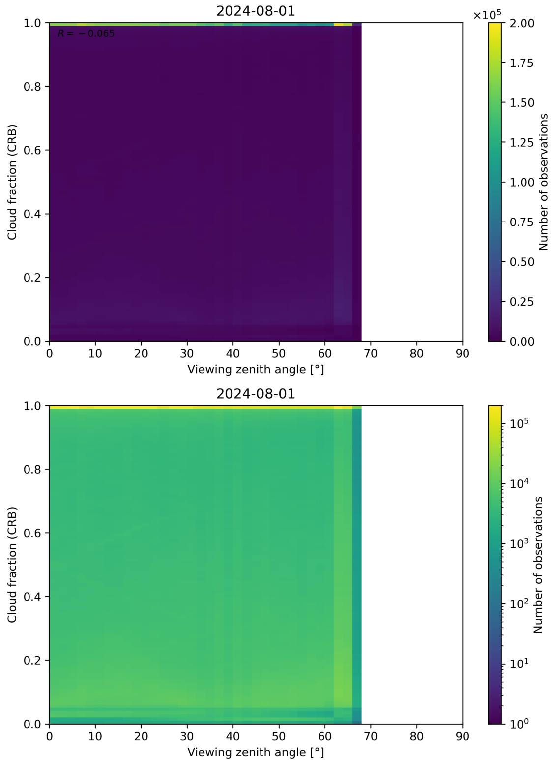
Figure 109: Scatter density plot of “Viewing zenith angle” against “Cloud fraction (CRB)” for 2024-07-31 to 2024-08-02.
