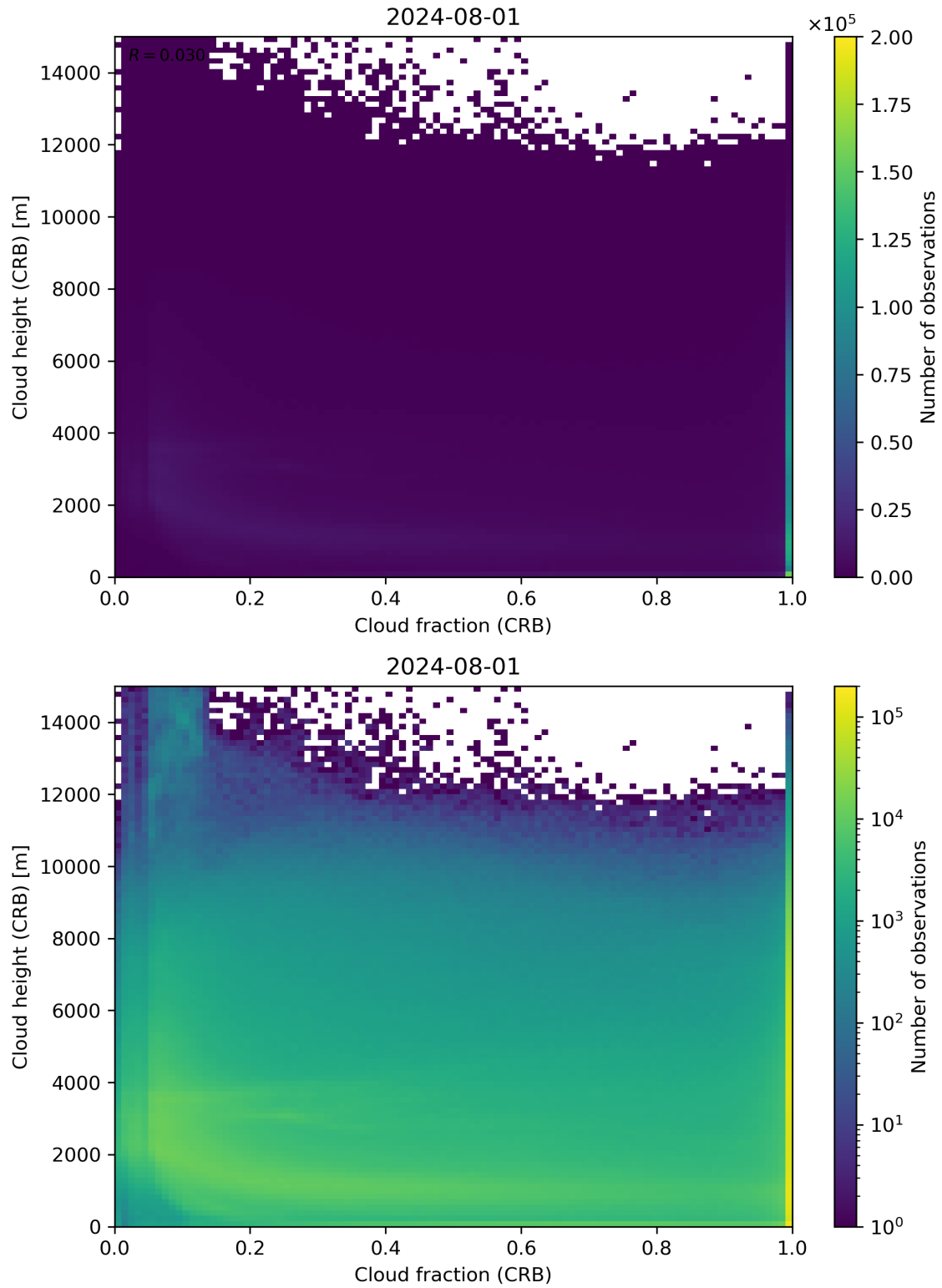
Figure 79: Scatter density plot of “Cloud fraction (CRB)” against “Cloud height (CRB)” for 2024-07-31 to 2024-08-02.
