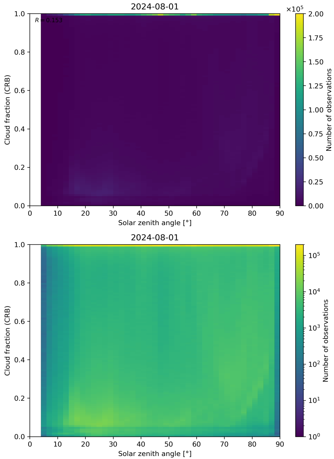
Figure 101: Scatter density plot of “Solar zenith angle” against “Cloud fraction (CRB)” for 2024-07-31 to 2024-08-02.
