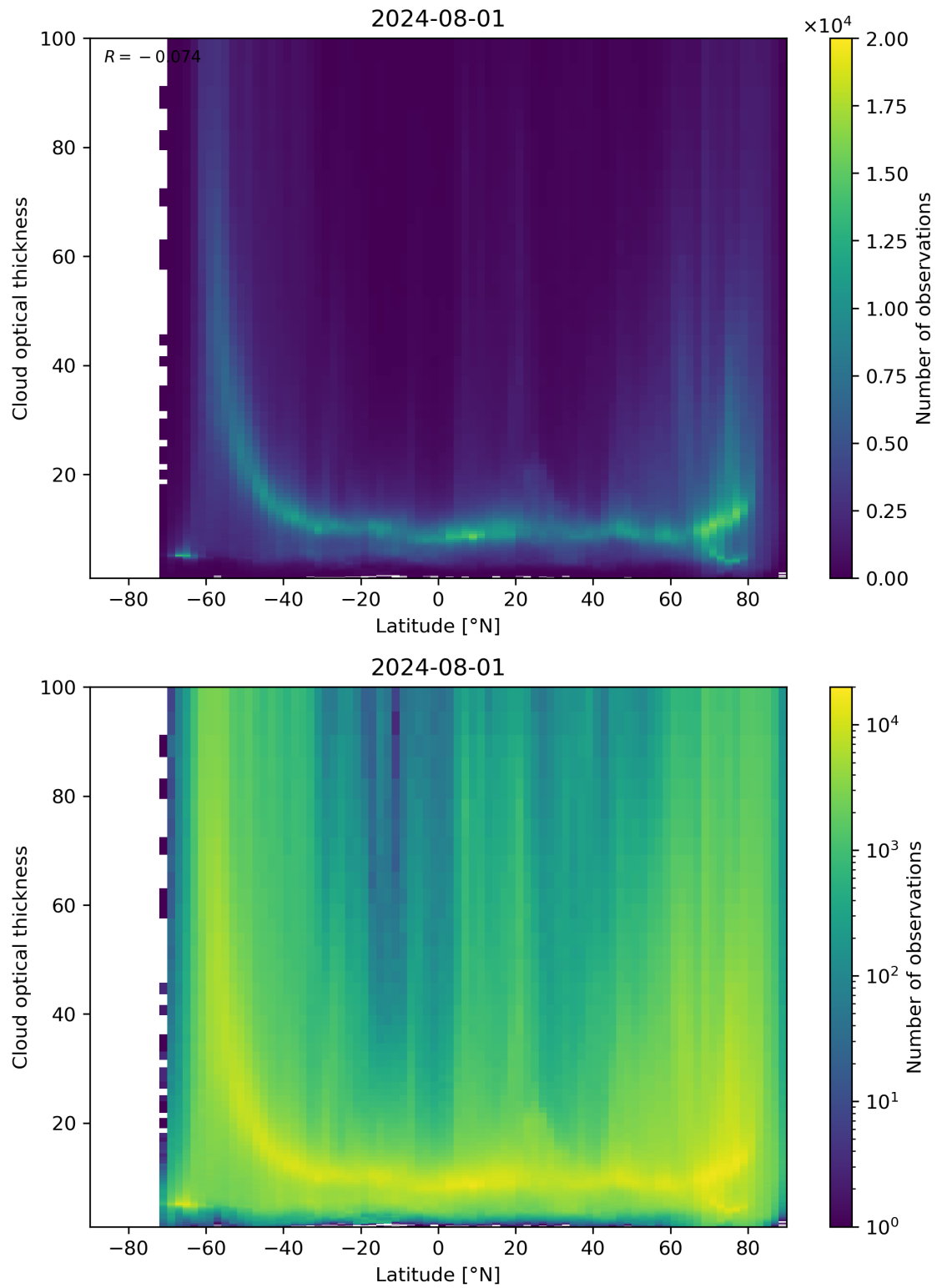
Figure 96: Scatter density plot of “Latitude” against “Cloud optical thickness” for 2024-07-31 to 2024-08-02.
