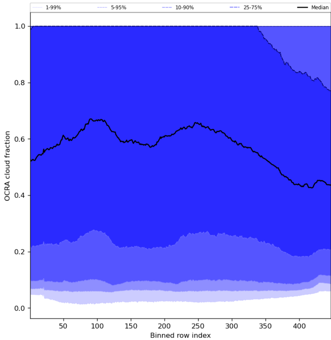
Figure 66: Along track statistics of “OCRA cloud fraction” for 2024-07-31 to 2024-08-02
