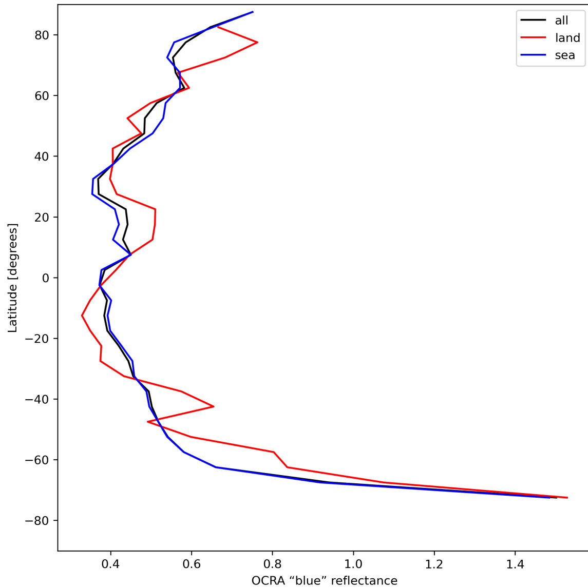
Figure 35: Zonal average of “OCRA “blue” reflectance” for 2024-07-31 to 2024-08-02.
