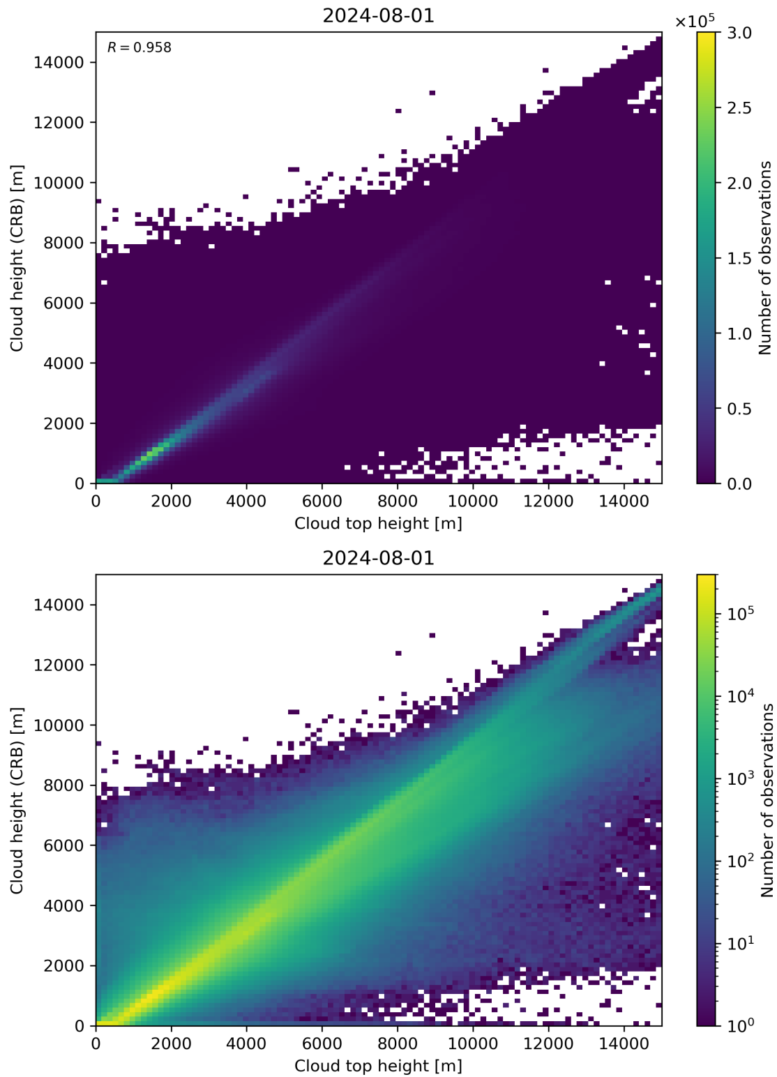
Figure 89: Scatter density plot of “Cloud top height” against “Cloud height (CRB)” for 2024-07-31 to 2024-08-02.
