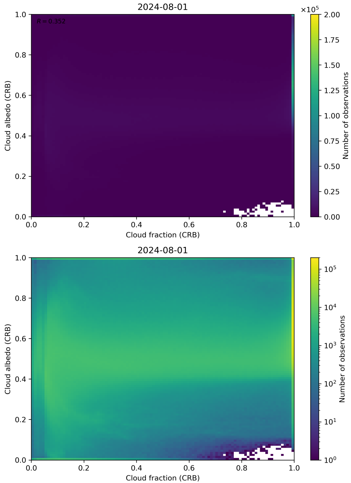
Figure 77: Scatter density plot of “Cloud fraction (CRB)” against “Cloud albedo (CRB)” for 2024-07-31 to 2024-08-02.
