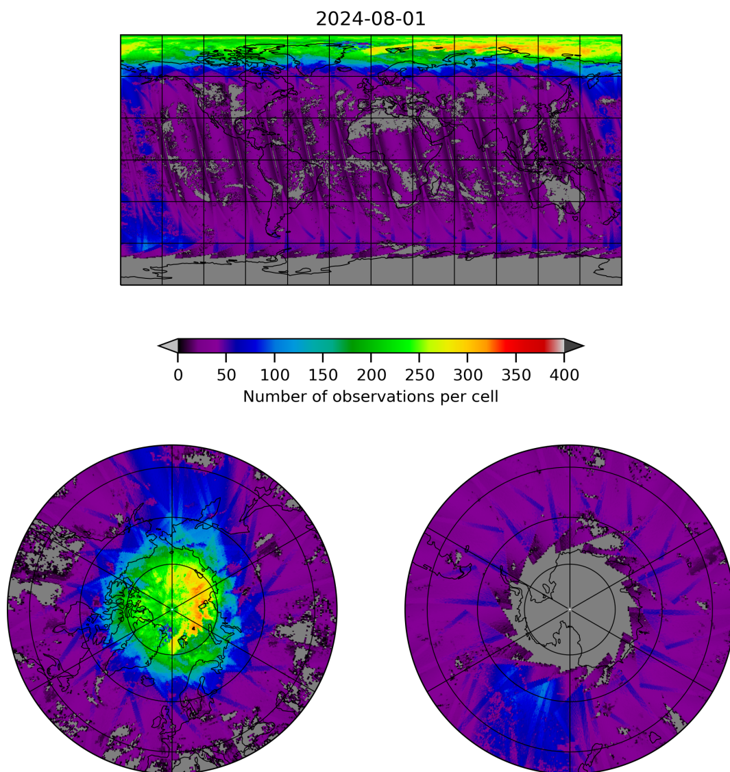
Figure 21: Map of the number of observations for 2024-07-31 to 2024-08-02
