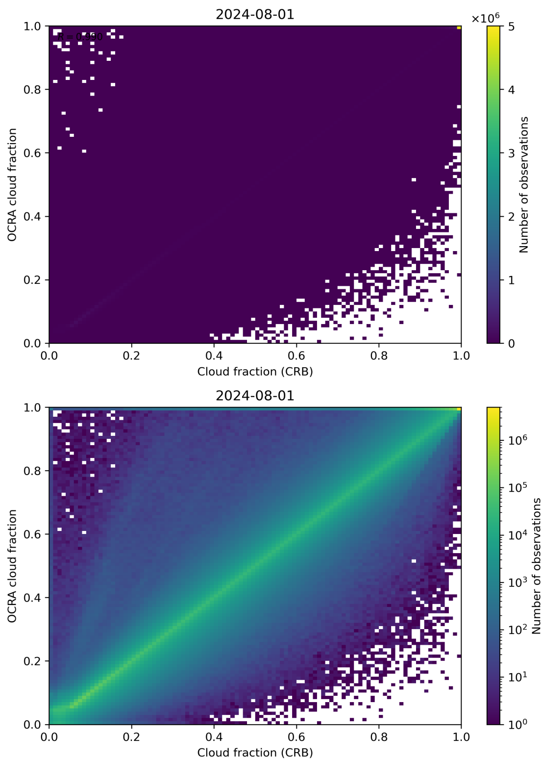
Figure 78: Scatter density plot of “Cloud fraction (CRB)” against “OCRA cloud fraction” for 2024-07-31 to 2024-08-02.
