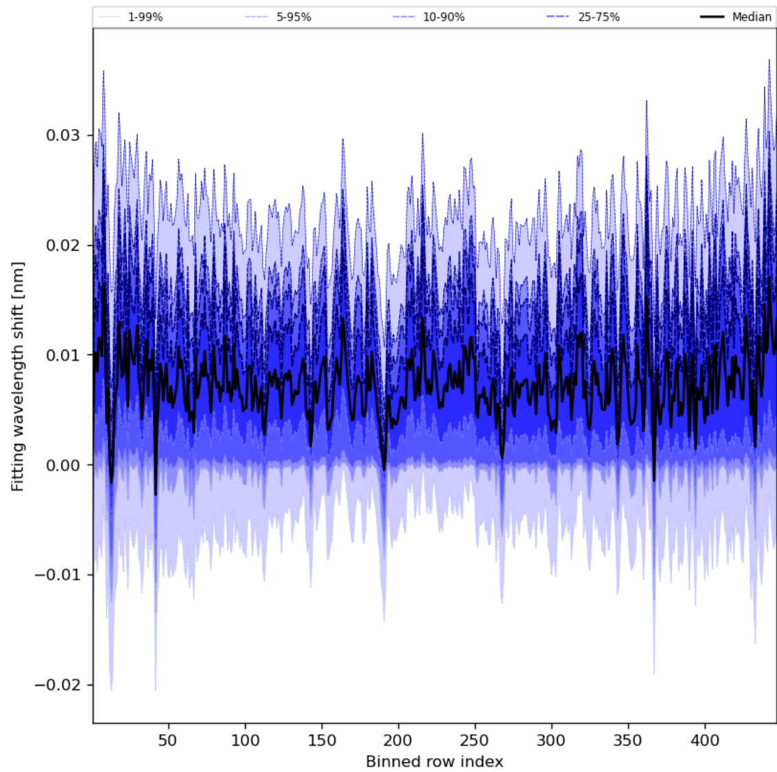
Figure 65: Along track statistics of “Fitting wavelength shift” for 2024-07-31 to 2024-08-02
