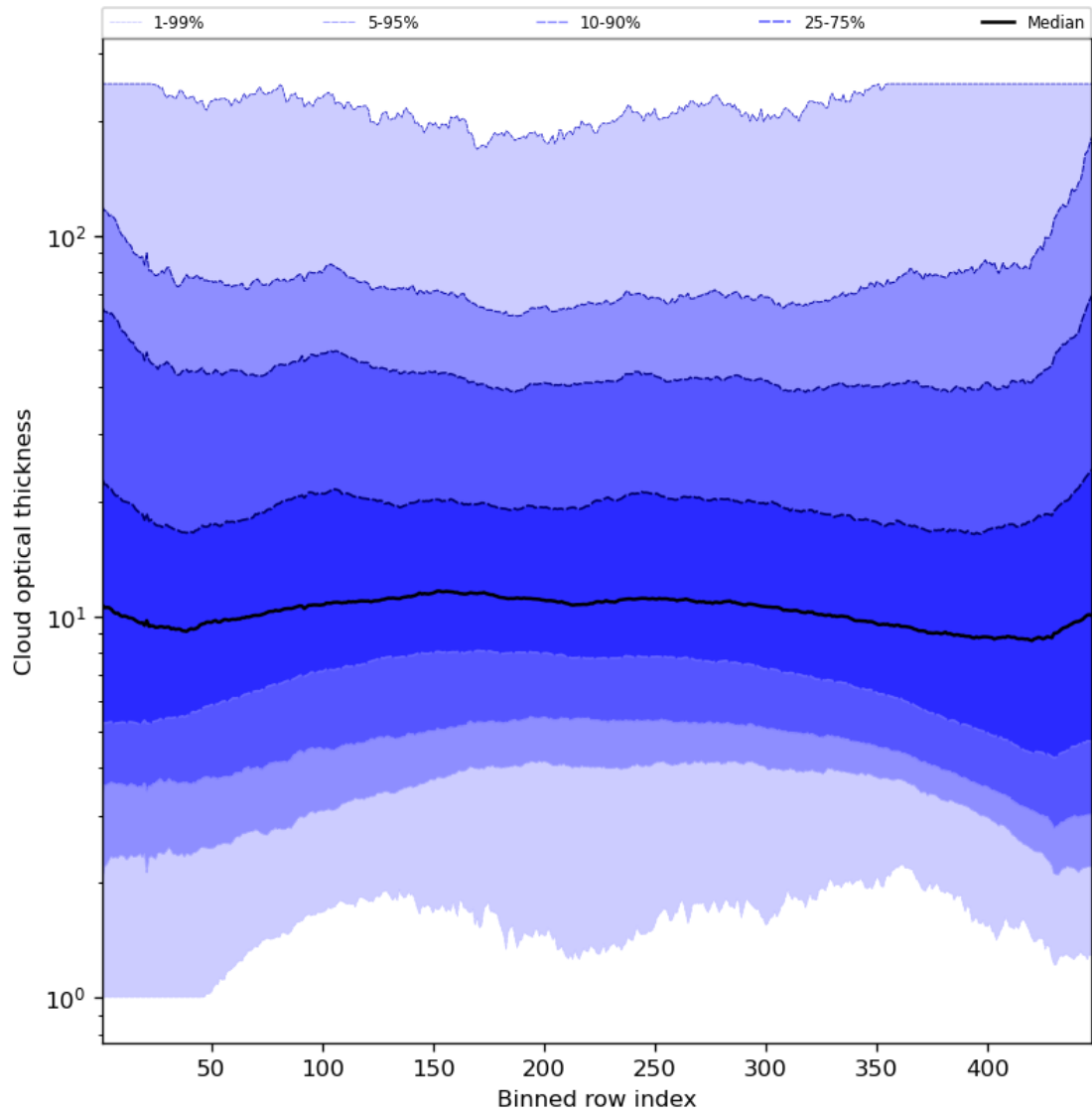
Figure 57: Along track statistics of “Cloud optical thickness” for 2024-07-31 to 2024-08-02
