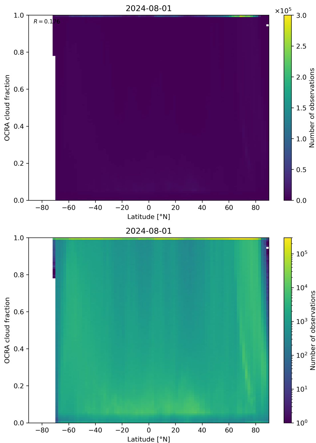
Figure 93: Scatter density plot of “Latitude” against “OCRA cloud fraction” for 2024-07-31 to 2024-08-02.
