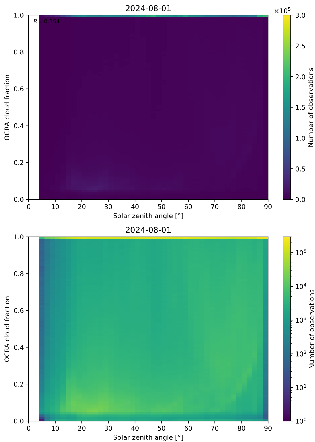
Figure 100: Scatter density plot of “Solar zenith angle” against “OCRA cloud fraction” for 2024-07-31 to 2024-08-02.
