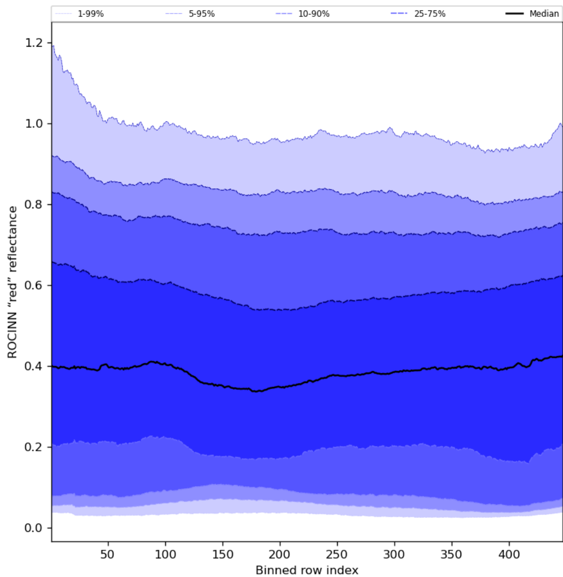
Figure 69: Along track statistics of "ROCINN "red" reflectance" for 2024-07-31 to 2024-08-02
