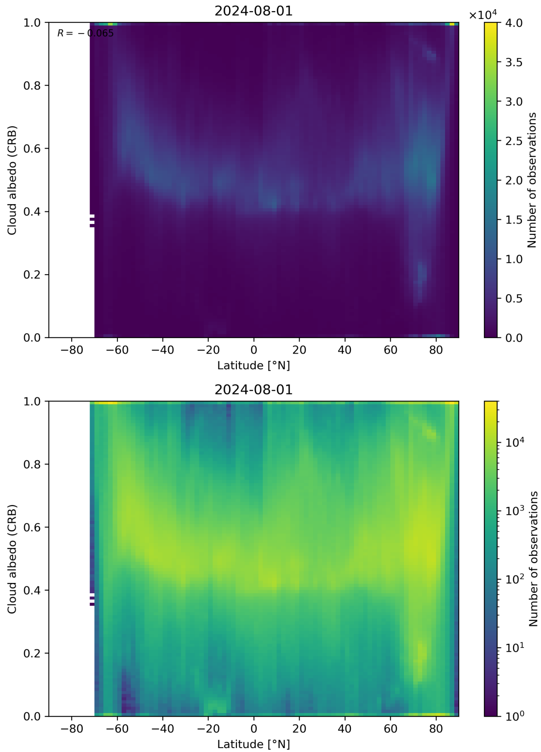
Figure 91: Scatter density plot of “Latitude” against “Cloud albedo (CRB)” for 2024-07-31 to 2024-08-02.
