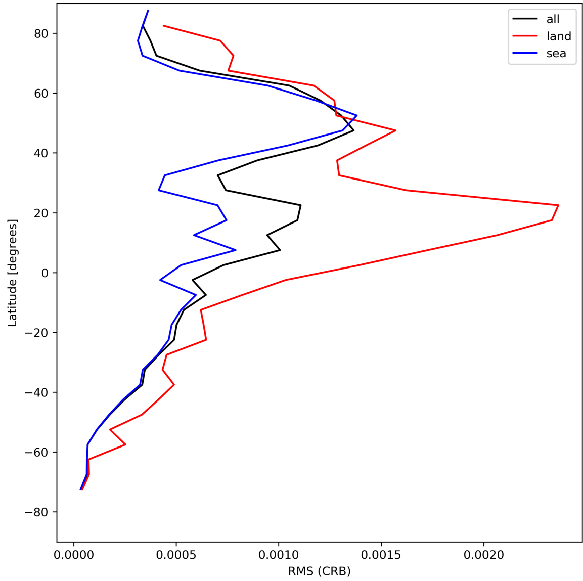
Figure 32: Zonal average of “RMS (CRB)” for 2024-07-31 to 2024-08-02.
