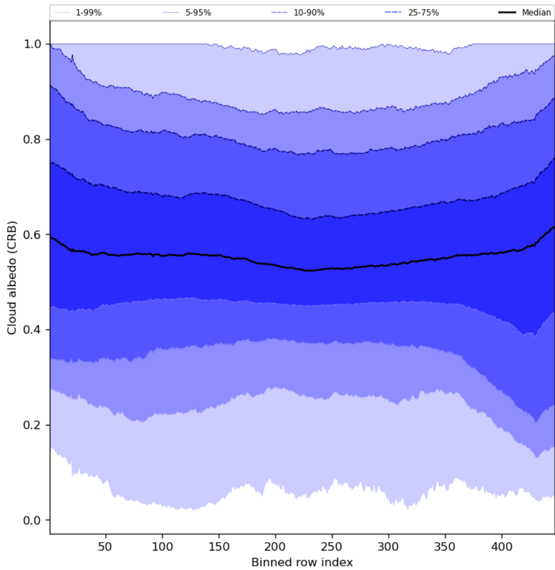
Figure 60: Along track statistics of “Cloud albedo (CRB)” for 2024-07-31 to 2024-08-02
