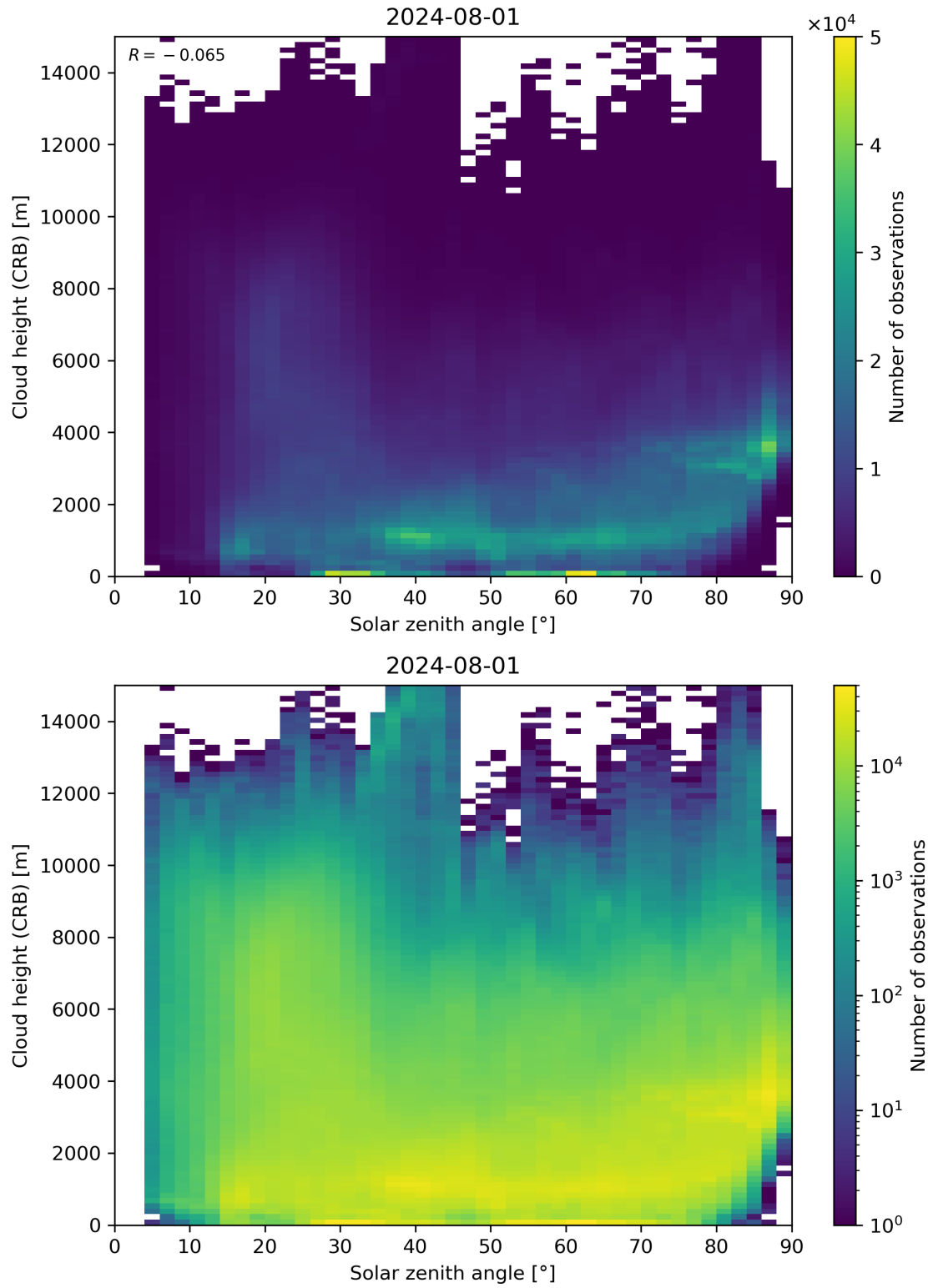
Figure 102: Scatter density plot of “Solar zenith angle” against “Cloud height (CRB)” for 2024-07-31 to 2024-08-02.
