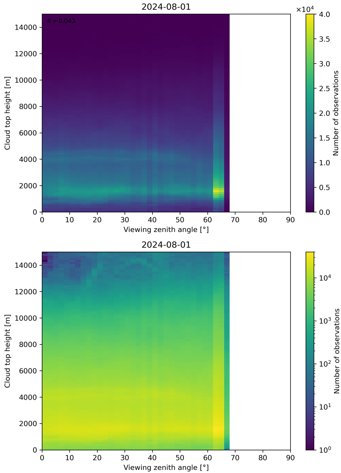
Figure 112: Scatter density plot of “Viewing zenith angle” against “Cloud top height” for 2024-07-31 to 2024-08-02.
