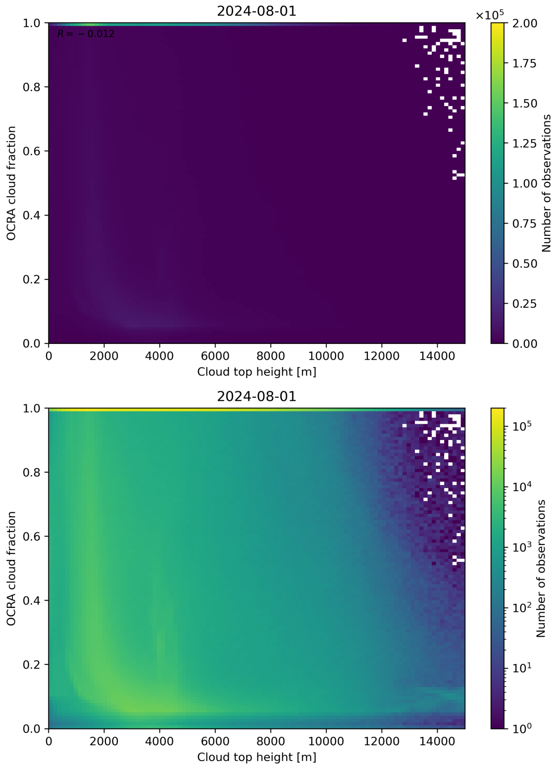
Figure 87: Scatter density plot of “Cloud top height” against “OCRA cloud fraction” for 2024-07-31 to 2024-08-02.
