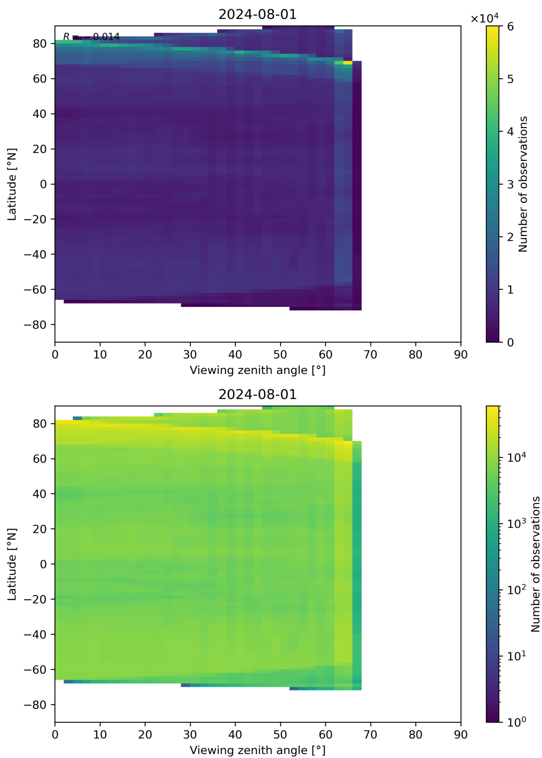
Figure 113: Scatter density plot of “Viewing zenith angle” against “Latitude” for 2024-07-31 to 2024-08-02.
