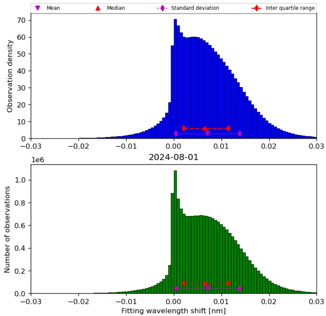
Figure 49: Histogram of “Fitting wavelength shift” for 2024-07-31 to 2024-08-02
