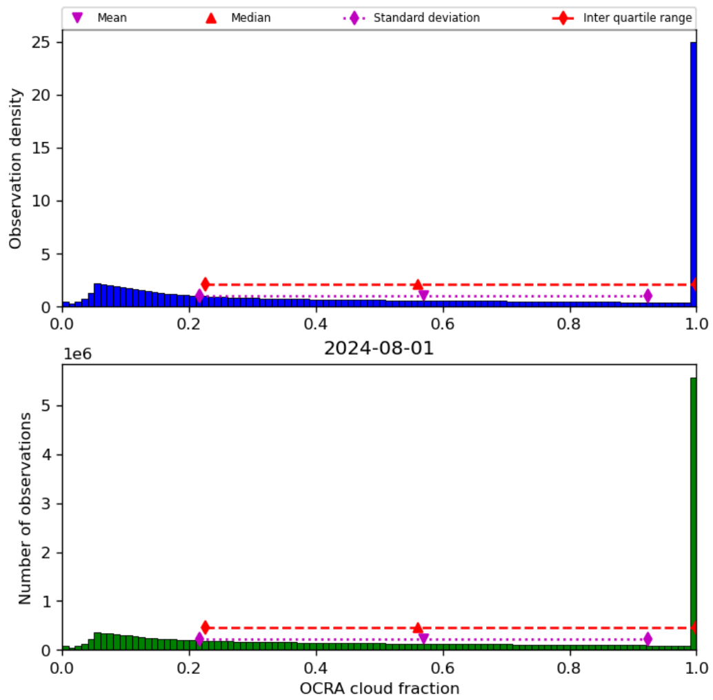
Figure 50: Histogram of “OCRA cloud fraction” for 2024-07-31 to 2024-08-02
