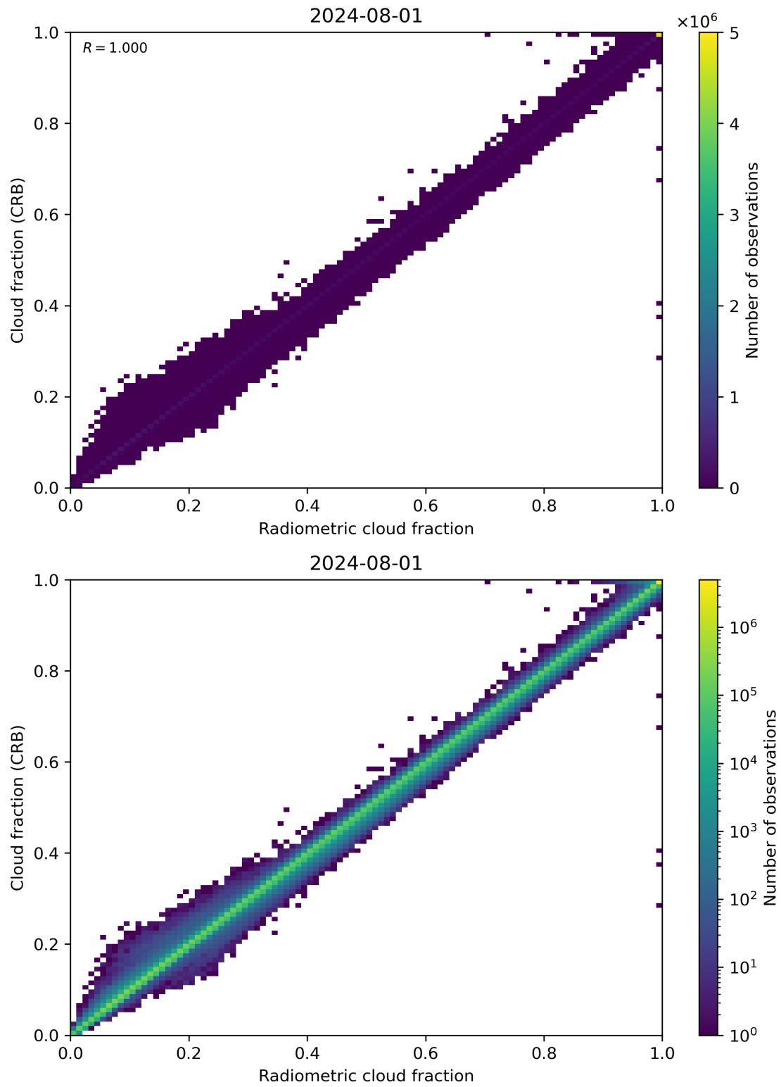
Figure 73: Scatter density plot of “Radiometric cloud fraction” against “Cloud fraction (CRB)” for 2024-07-31 to 2024-08-02.
