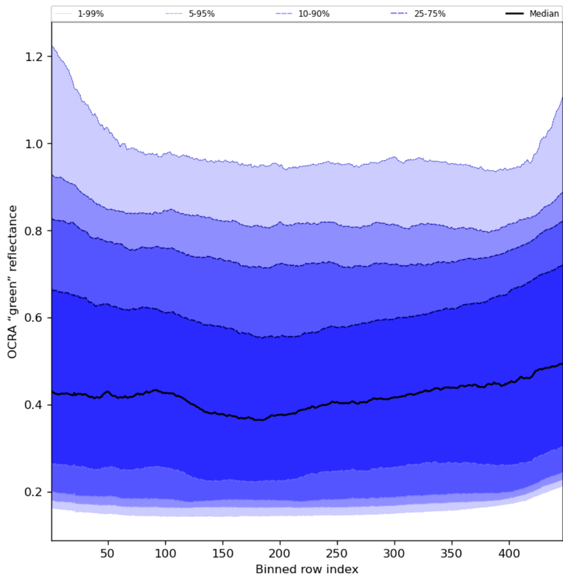
Figure 68: Along track statistics of "OCRA "green" reflectance" for 2024-07-31 to 2024-08-02
