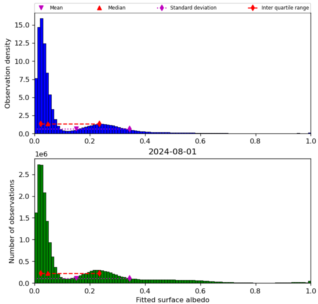
Figure 45: Histogram of “Fitted surface albedo” for 2024-07-31 to 2024-08-02
