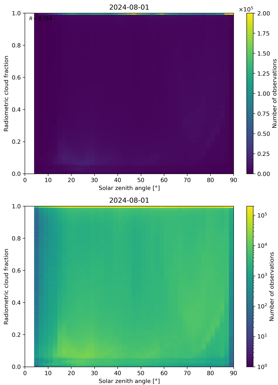
Figure 99: Scatter density plot of “Solar zenith angle” against “Radiometric cloud fraction” for 2024-07-31 to 2024-08-02.
