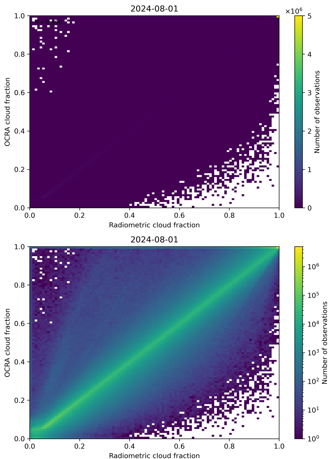
Figure 72: Scatter density plot of “Radiometric cloud fraction” against “OCRA cloud fraction” for 2024-07-31 to 2024-08-02.
