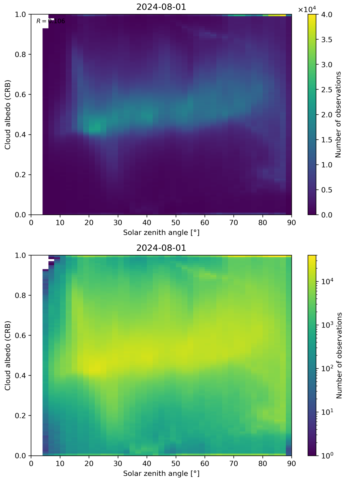
Figure 98: Scatter density plot of “Solar zenith angle” against “Cloud albedo (CRB)” for 2024-07-31 to 2024-08-02.
