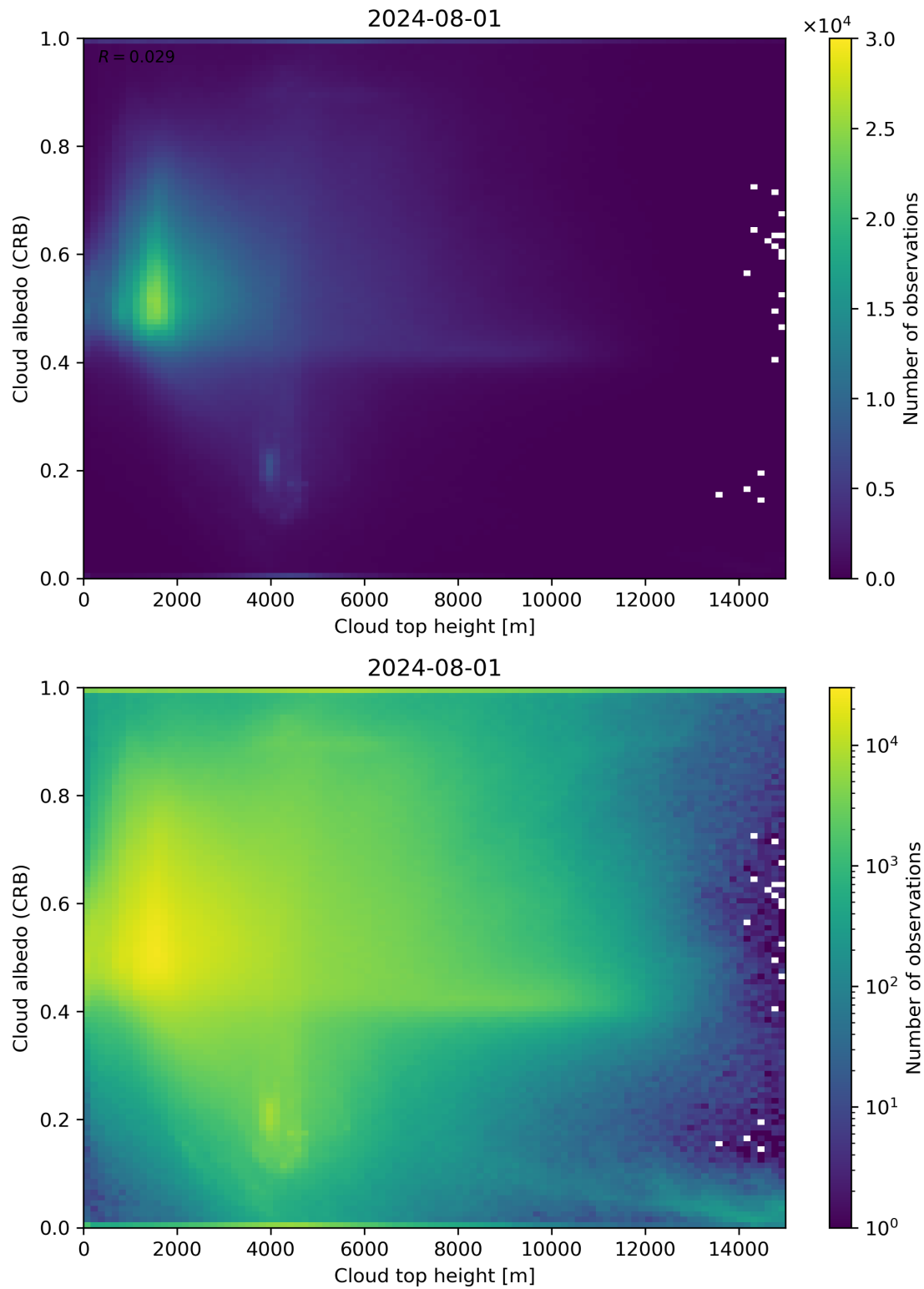
Figure 86: Scatter density plot of “Cloud top height” against “Cloud albedo (CRB)” for 2024-07-31 to 2024-08-02.
