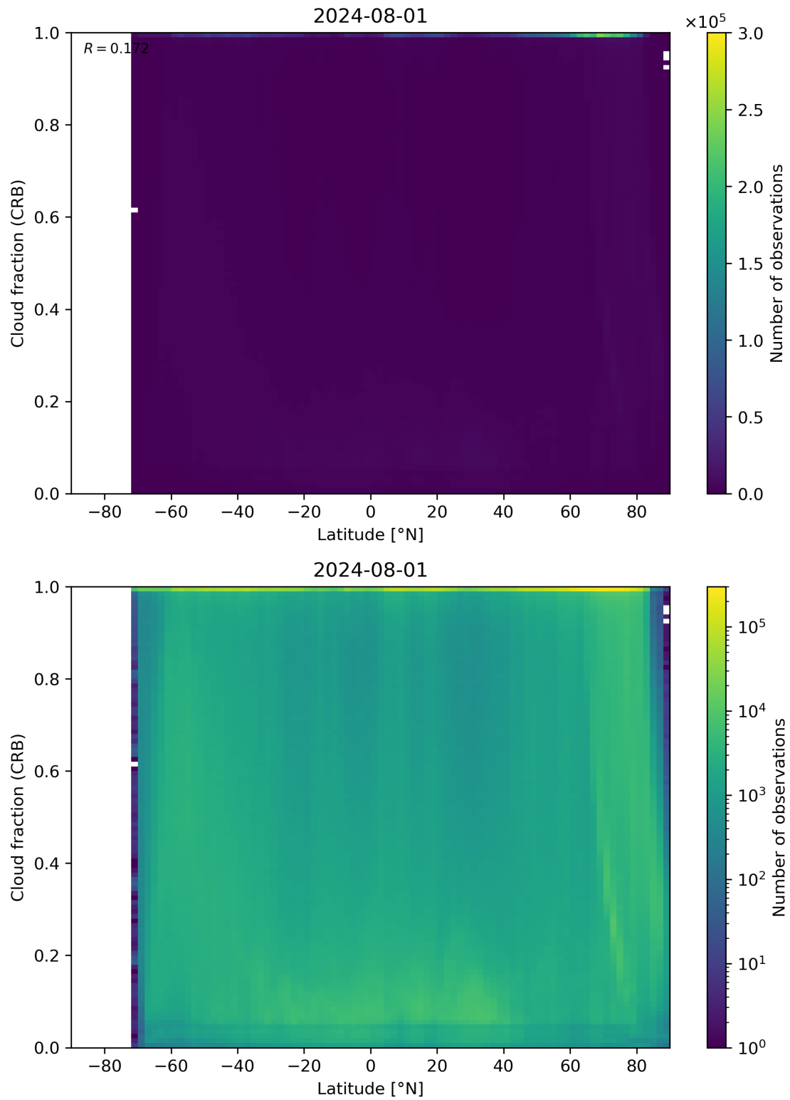
Figure 94: Scatter density plot of “Latitude” against “Cloud fraction (CRB)” for 2024-07-31 to 2024-08-02.
