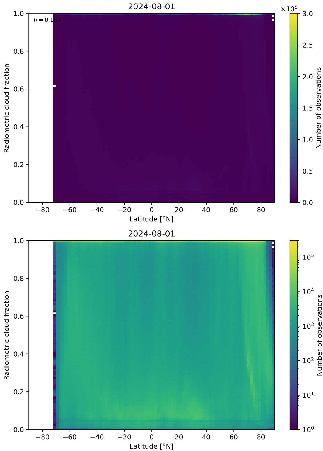
Figure 92: Scatter density plot of “Latitude” against “Radiometric cloud fraction” for 2024-07-31 to 2024-08-02.
