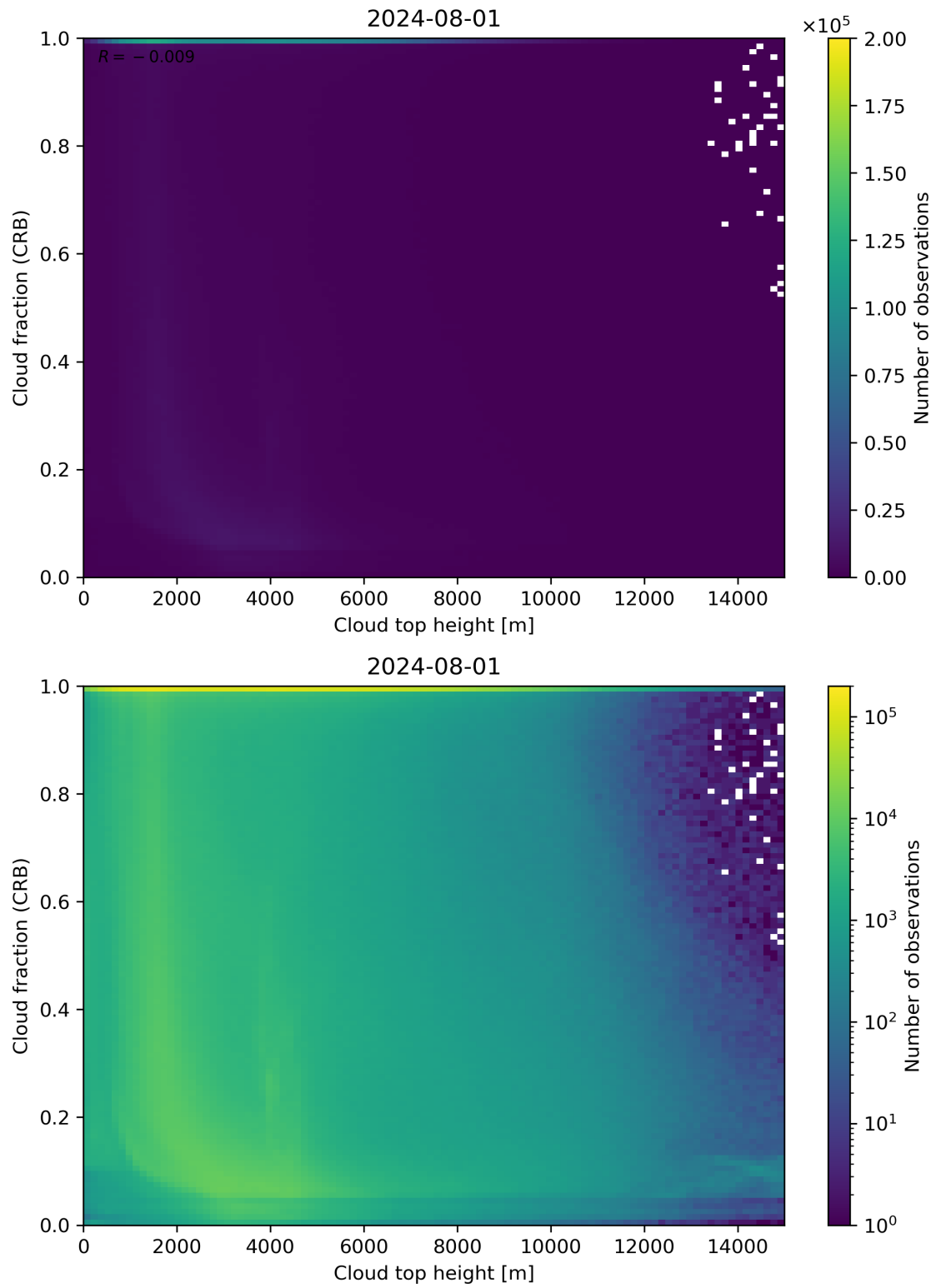
Figure 88: Scatter density plot of “Cloud top height” against “Cloud fraction (CRB)” for 2024-07-31 to 2024-08-02.
