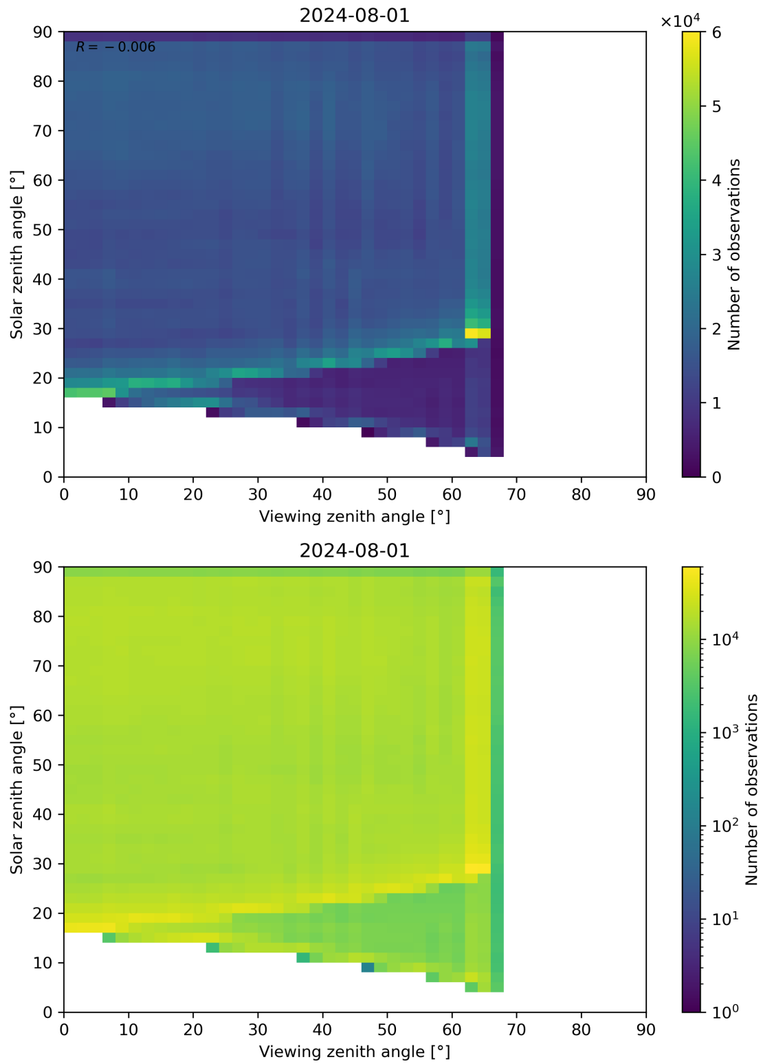
Figure 114: Scatter density plot of “Viewing zenith angle” against “Solar zenith angle” for 2024-07-31 to 2024-08-02.
