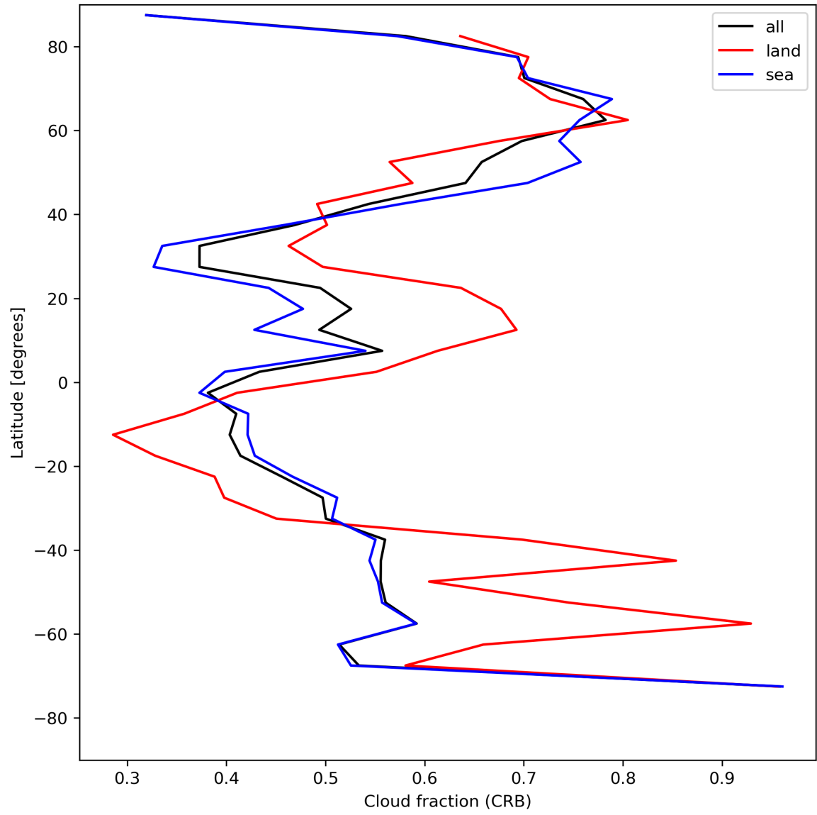
Figure 26: Zonal average of “Cloud fraction (CRB)” for 2024-07-31 to 2024-08-02.
