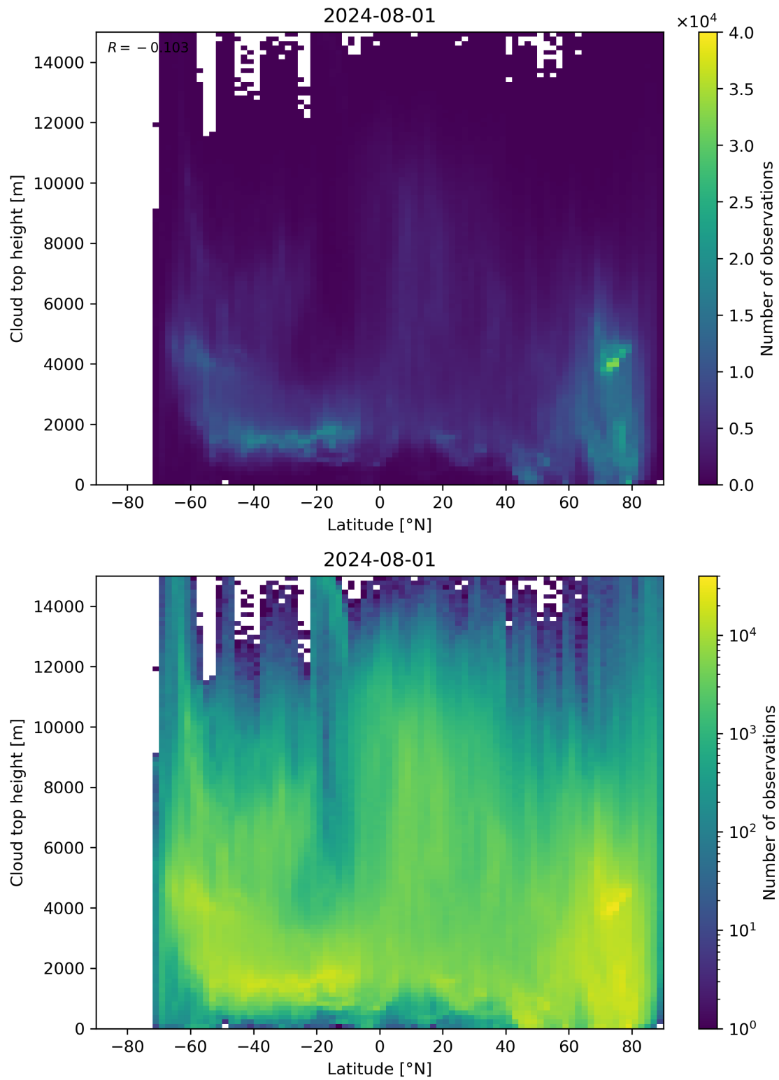
Figure 97: Scatter density plot of “Latitude” against “Cloud top height” for 2024-07-31 to 2024-08-02.
