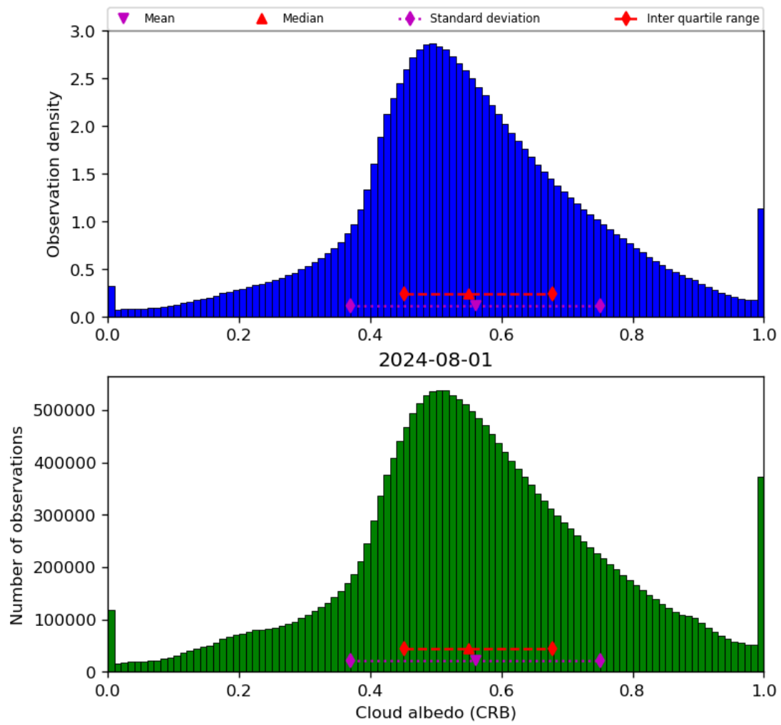
Figure 44: Histogram of “Cloud albedo (CRB)” for 2024-07-31 to 2024-08-02
