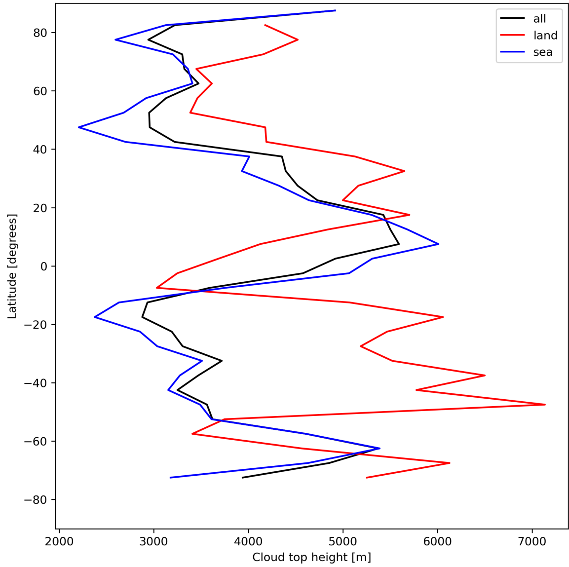
Figure 24: Zonal average of “Cloud top height” for 2024-07-31 to 2024-08-02.
