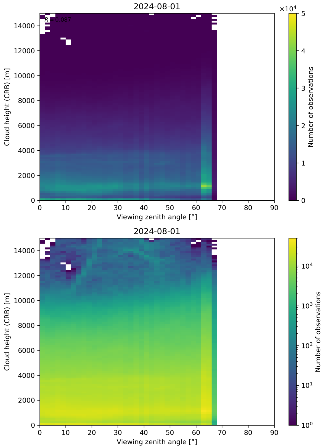
Figure 110: Scatter density plot of “Viewing zenith angle” against “Cloud height (CRB)” for 2024-07-31 to 2024-08-02.
