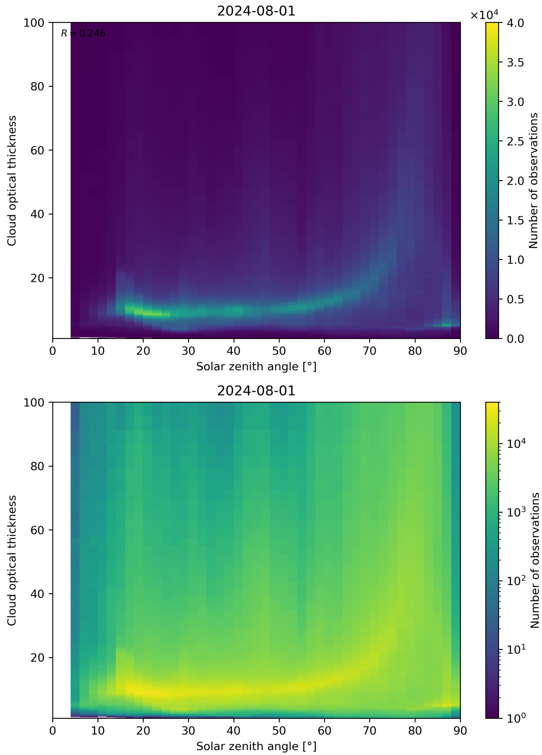
Figure 103: Scatter density plot of “Solar zenith angle” against “Cloud optical thickness” for 2024-07-31 to 2024-08-02.
