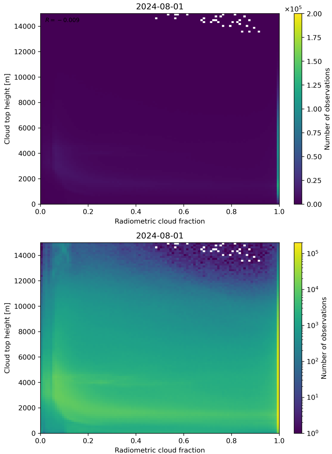
Figure 76: Scatter density plot of “Radiometric cloud fraction” against “Cloud top height” for 2024-07-31 to 2024-08-02.
