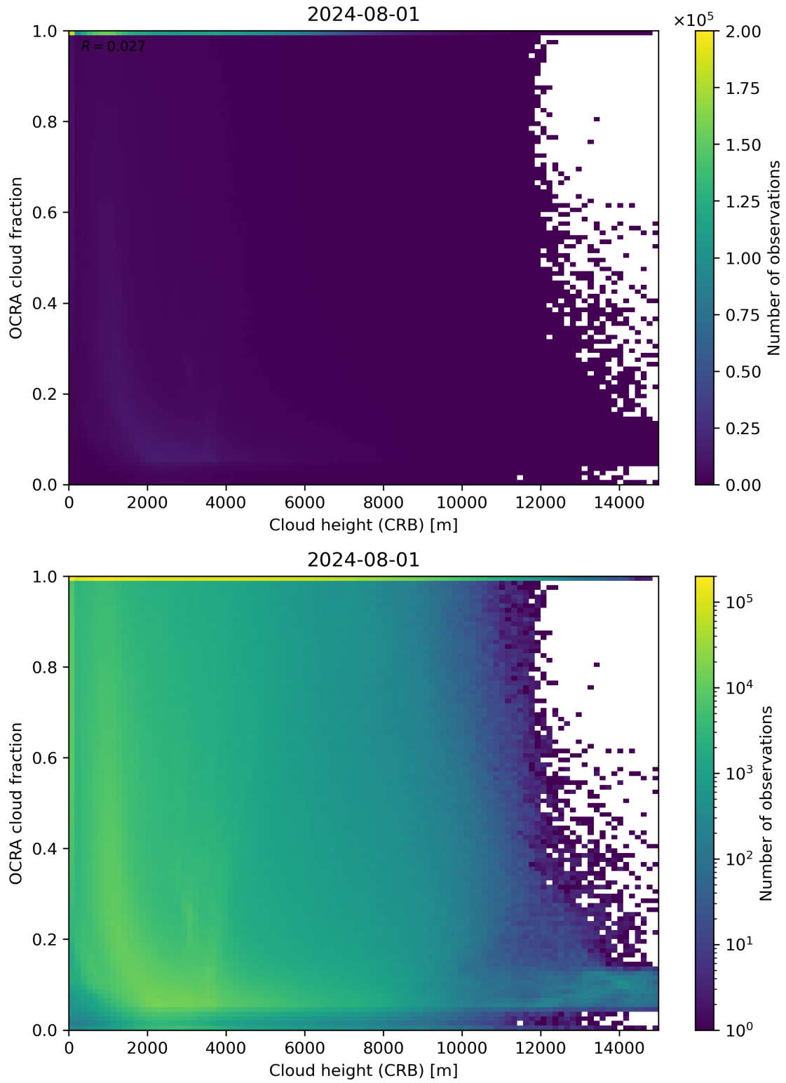
Figure 81: Scatter density plot of “Cloud height (CRB)” against “OCRA cloud fraction” for 2024-07-31 to 2024-08-02.
