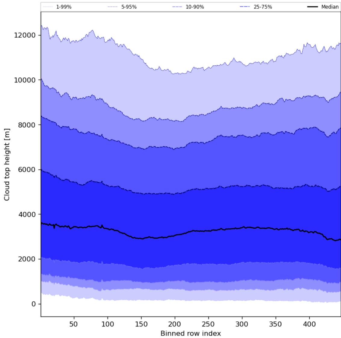
Figure 56: Along track statistics of “Cloud top height” for 2024-07-31 to 2024-08-02
