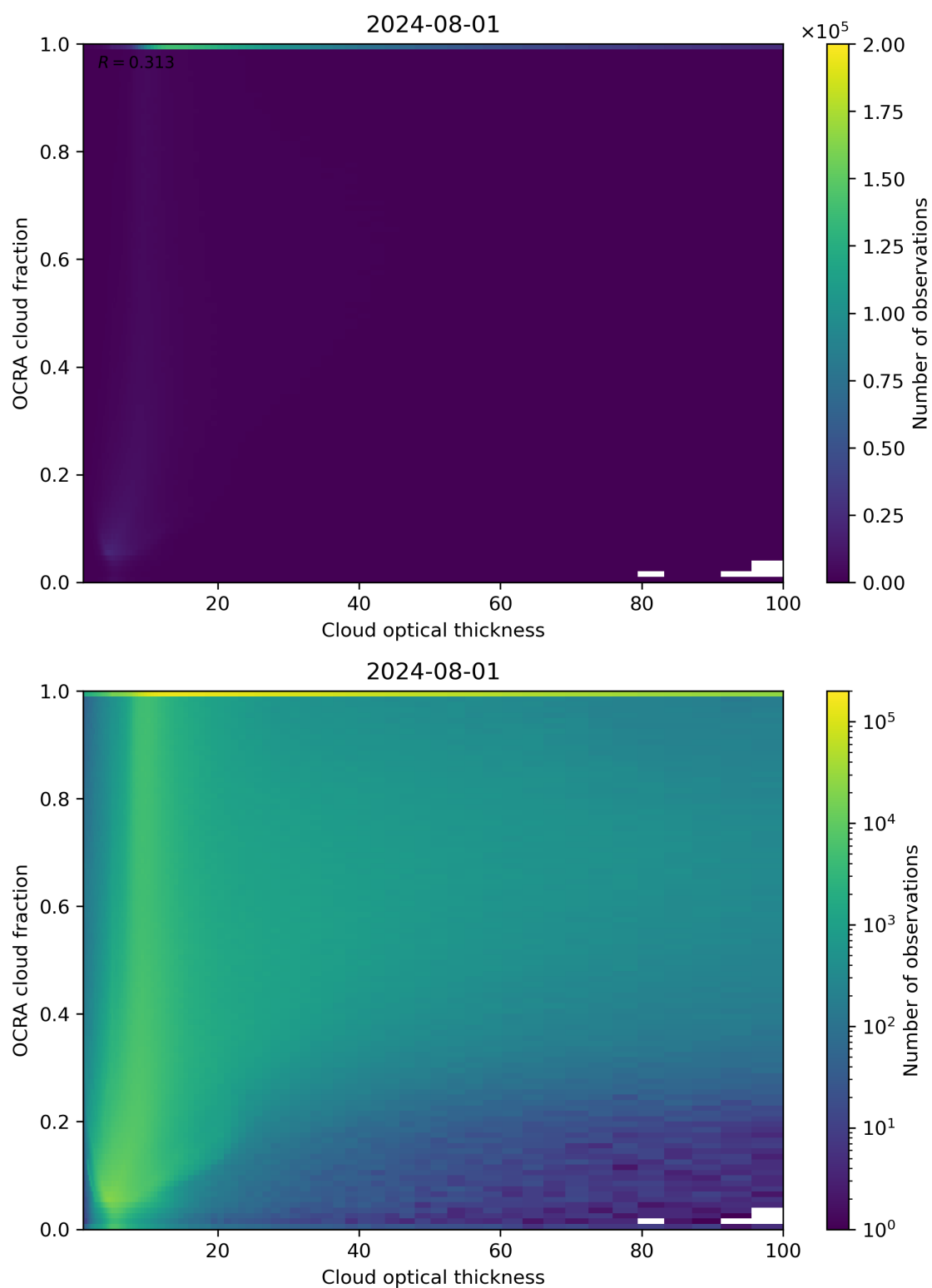
Figure 83: Scatter density plot of “Cloud optical thickness” against “OCRA cloud fraction” for 2024-07-31 to 2024-08-02.
