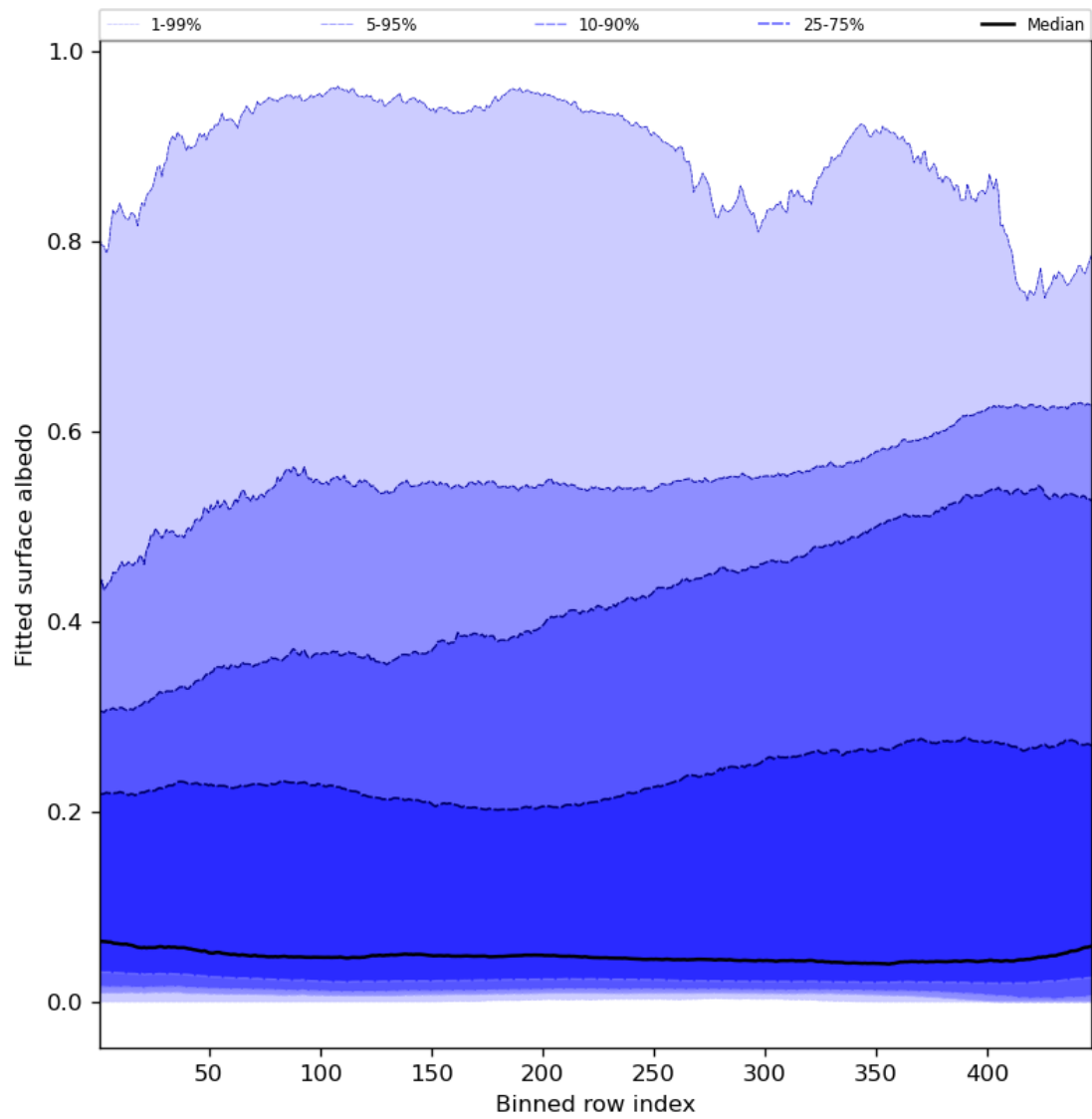
Figure 61: Along track statistics of “Fitted surface albedo” for 2024-07-31 to 2024-08-02
