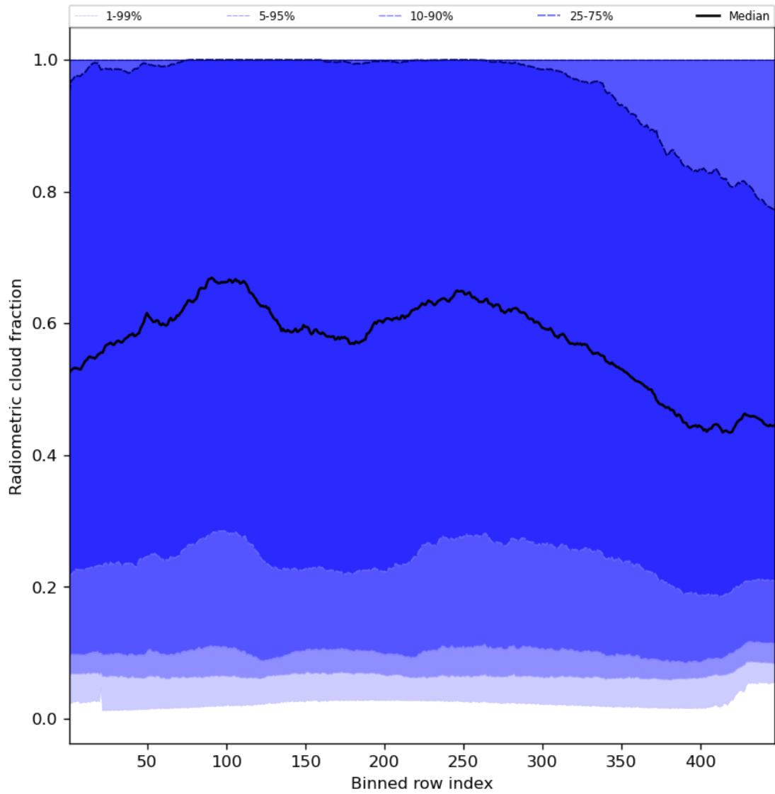
Figure 55: Along track statistics of “Radiometric cloud fraction” for 2024-07-31 to 2024-08-02
