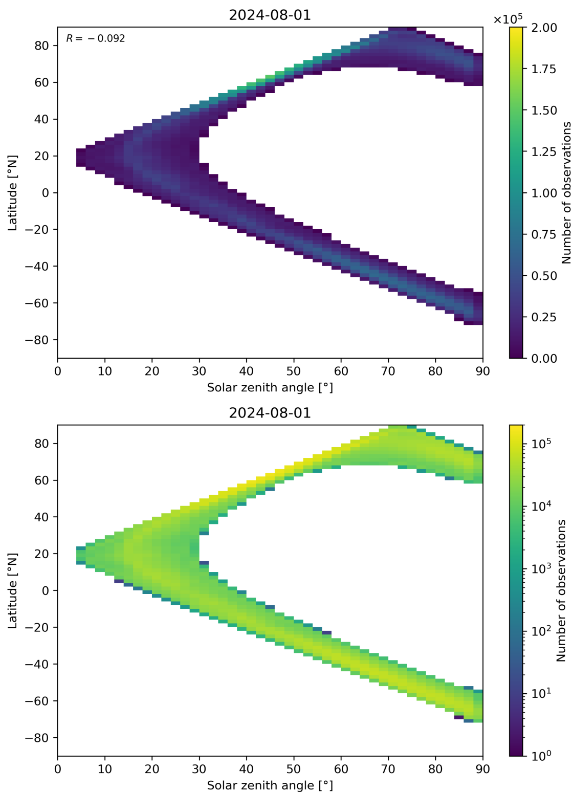
Figure 105: Scatter density plot of “Solar zenith angle” against “Latitude” for 2024-07-31 to 2024-08-02.
