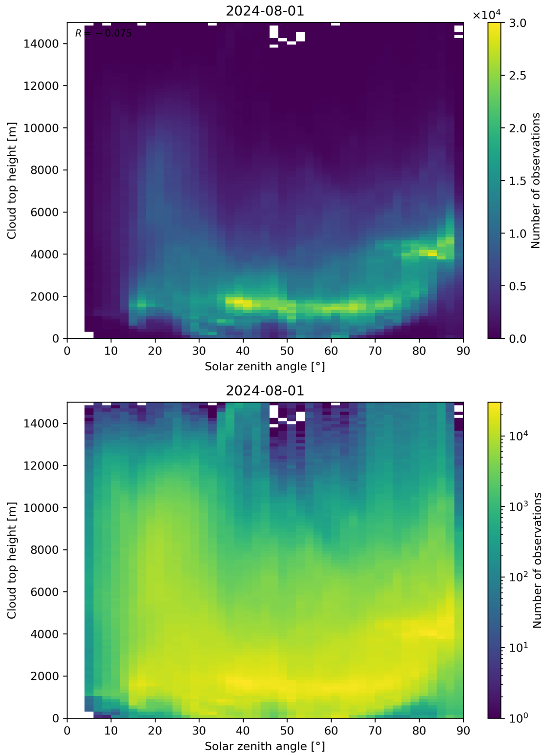
Figure 104: Scatter density plot of “Solar zenith angle” against “Cloud top height” for 2024-07-31 to 2024-08-02.
