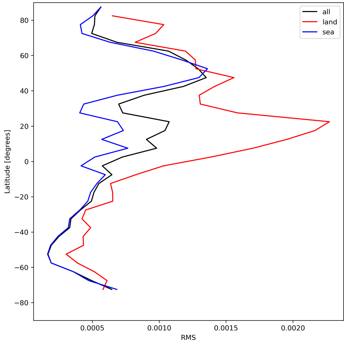
Figure 31: Zonal average of “RMS” for 2024-07-31 to 2024-08-02.
