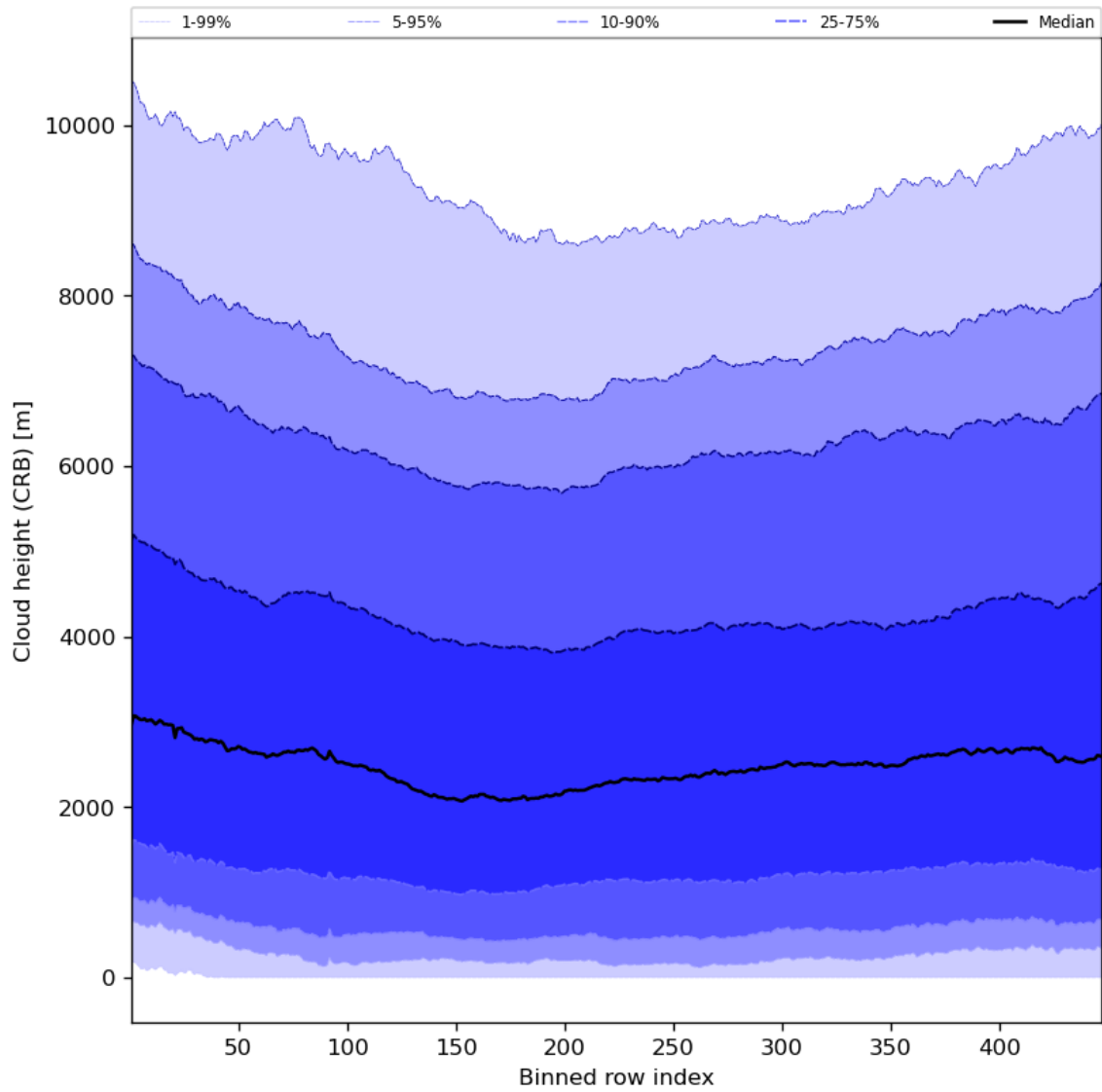
Figure 59: Along track statistics of “Cloud height (CRB)” for 2024-07-31 to 2024-08-02
