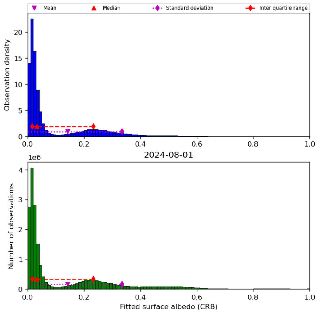
Figure 46: Histogram of “Fitted surface albedo (CRB)” for 2024-07-31 to 2024-08-02
