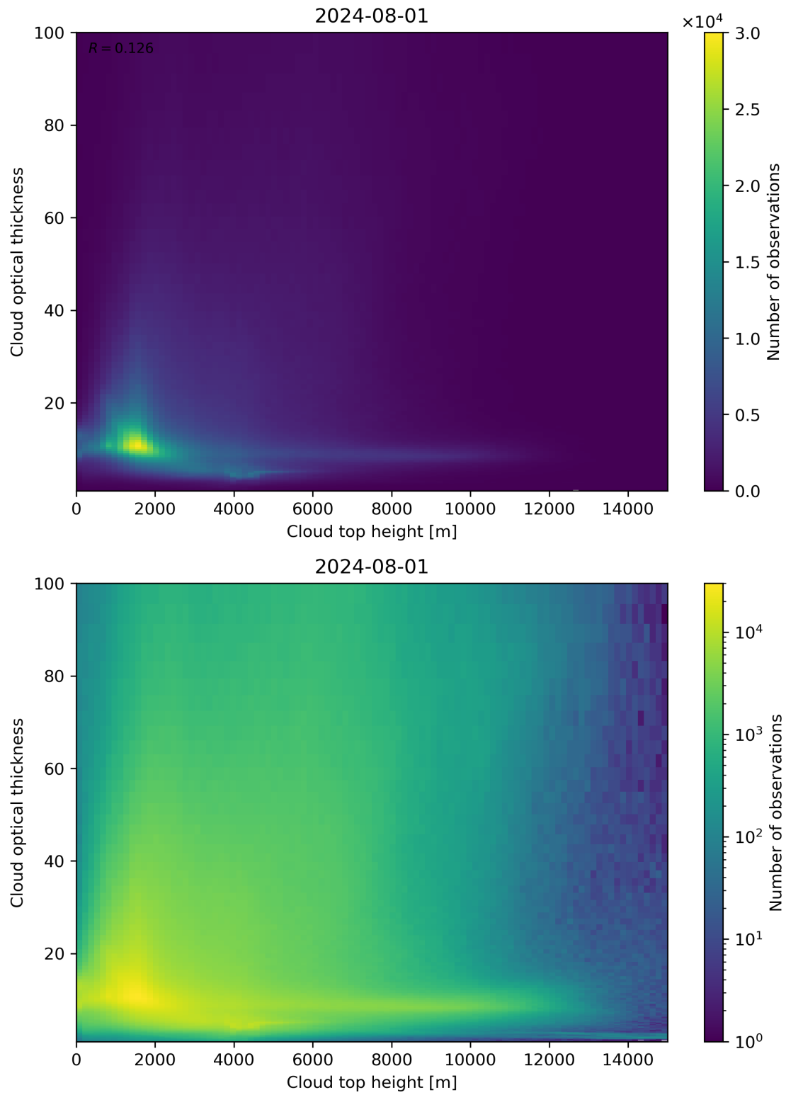
Figure 90: Scatter density plot of “Cloud top height” against “Cloud optical thickness” for 2024-07-31 to 2024-08-02.
