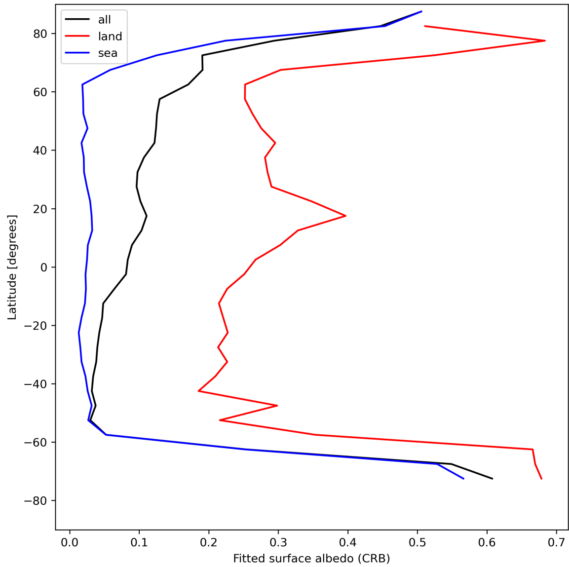
Figure 30: Zonal average of “Fitted surface albedo (CRB)” for 2024-07-31 to 2024-08-02.
