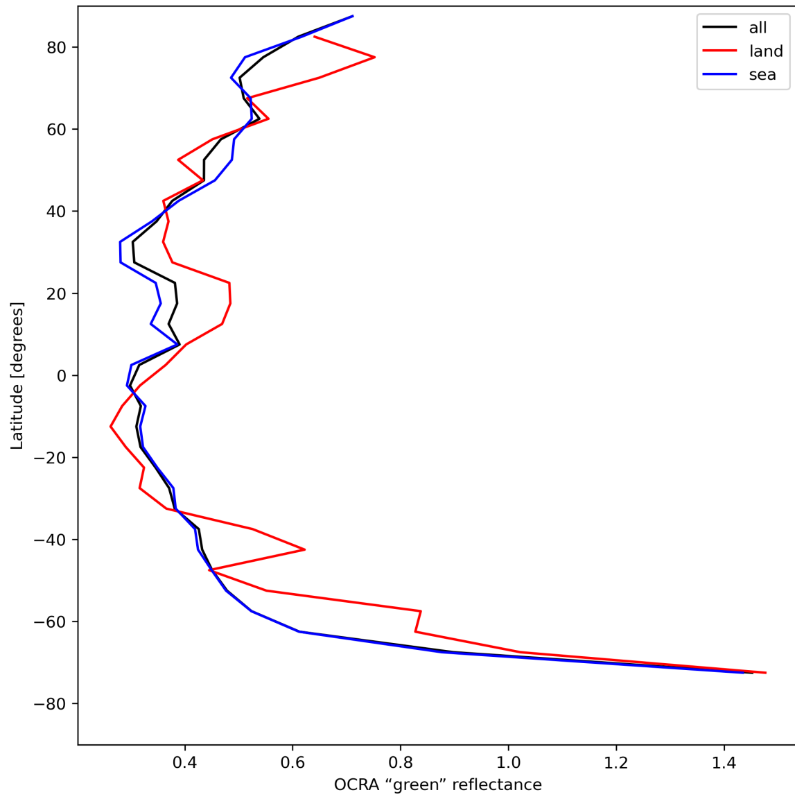
Figure 36: Zonal average of “OCRA “green” reflectance” for 2024-07-31 to 2024-08-02.
