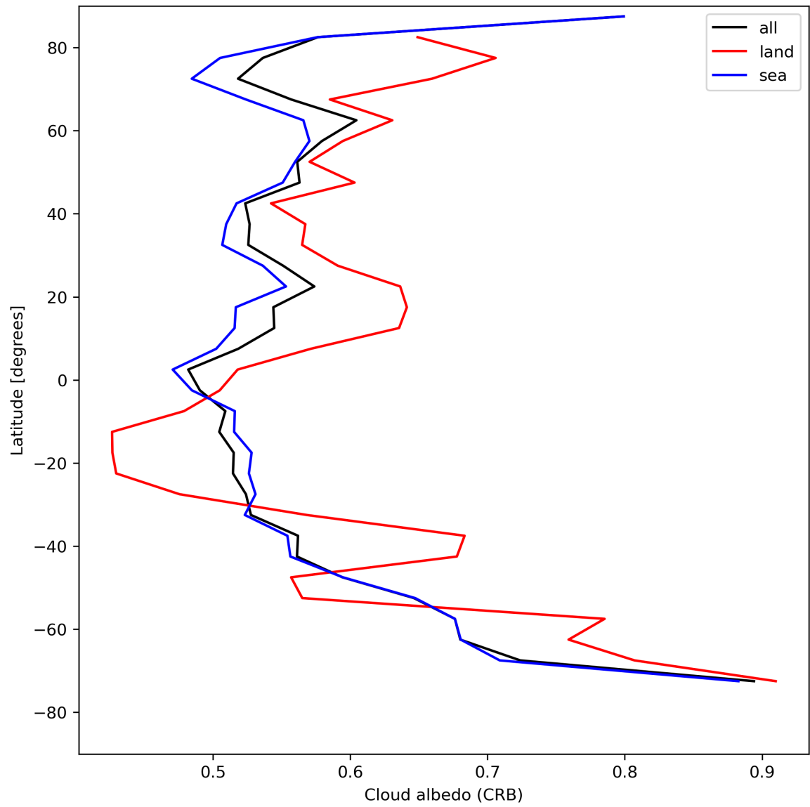
Figure 28: Zonal average of “Cloud albedo (CRB)” for 2024-07-31 to 2024-08-02.
