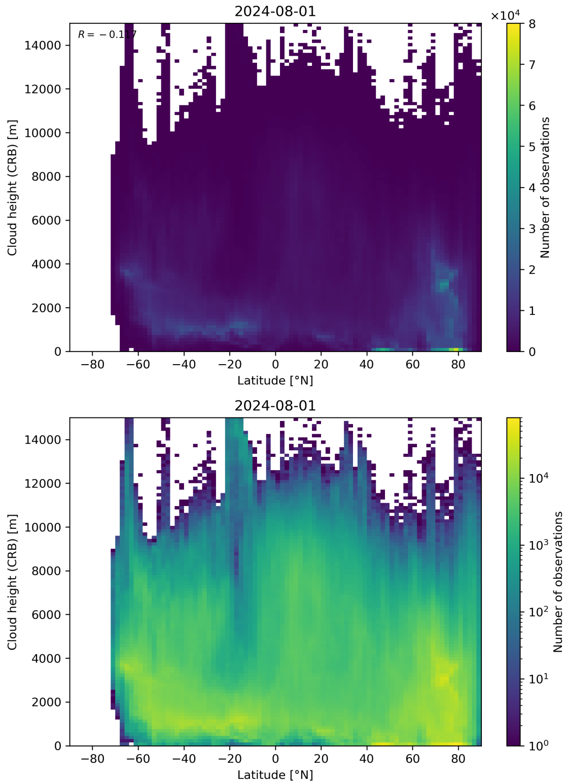
Figure 95: Scatter density plot of “Latitude” against “Cloud height (CRB)” for 2024-07-31 to 2024-08-02.
