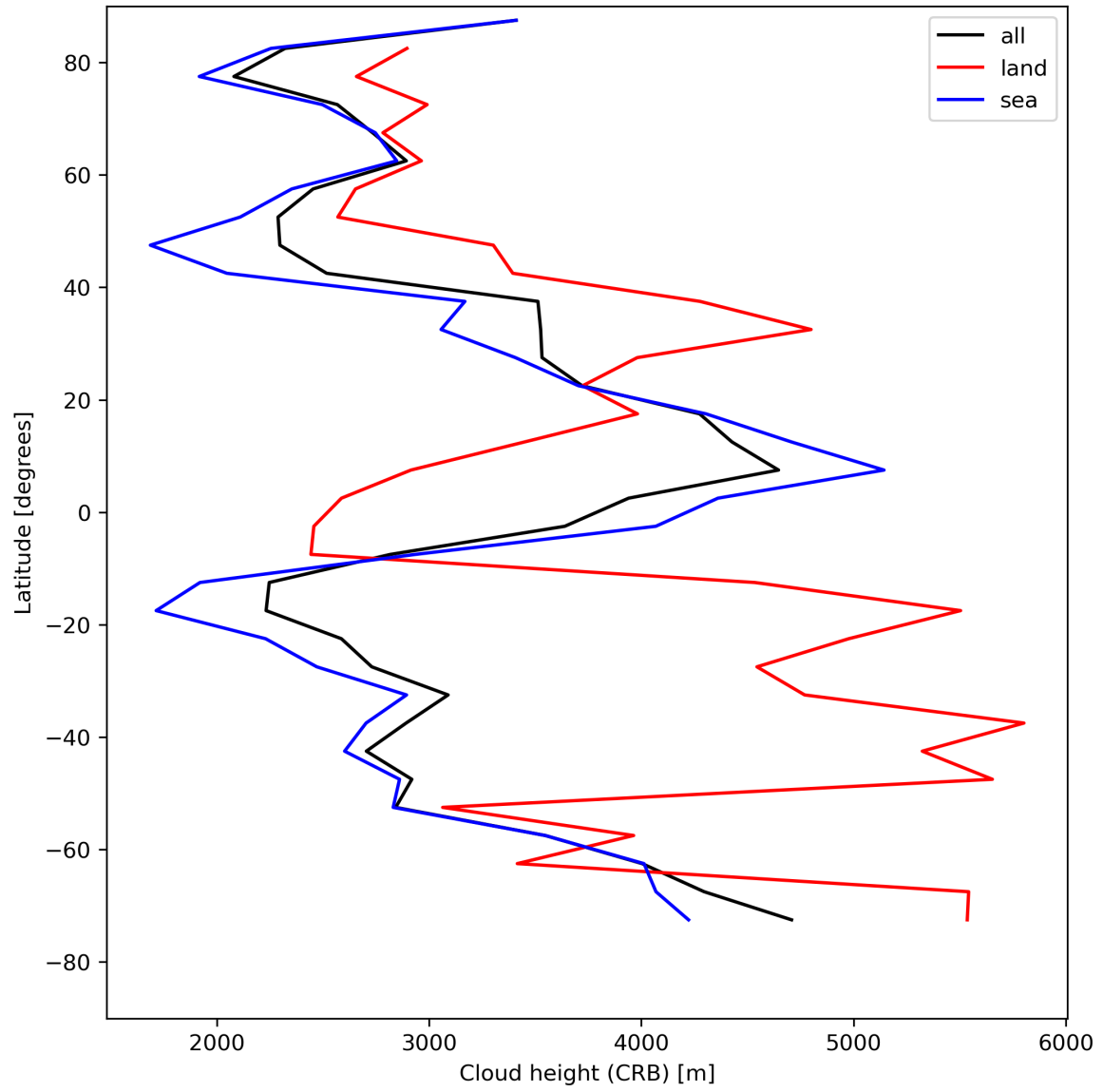
Figure 27: Zonal average of “Cloud height (CRB)” for 2024-07-31 to 2024-08-02.
