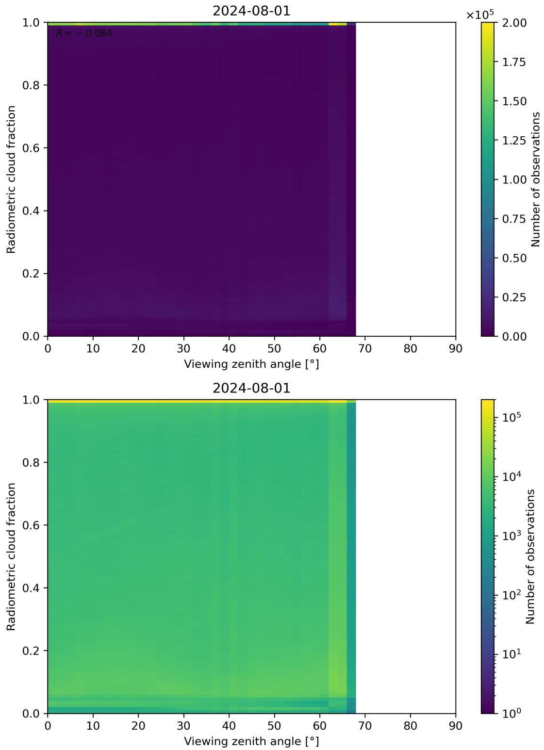
Figure 107: Scatter density plot of “Viewing zenith angle” against “Radiometric cloud fraction” for 2024-07-31 to 2024-08-02.
