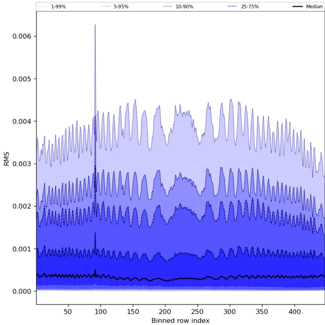
Figure 63: Along track statistics of “RMS” for 2024-07-31 to 2024-08-02
