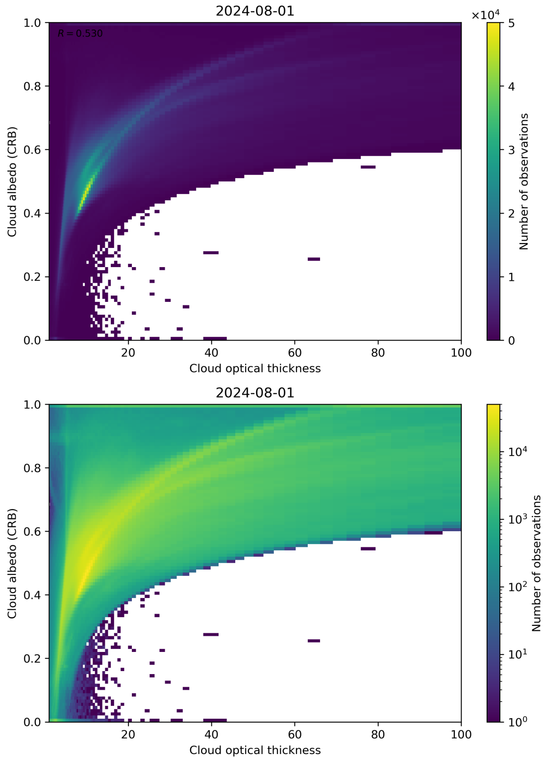
Figure 82: Scatter density plot of “Cloud optical thickness” against “Cloud albedo (CRB)” for 2024-07-31 to 2024-08-02.
