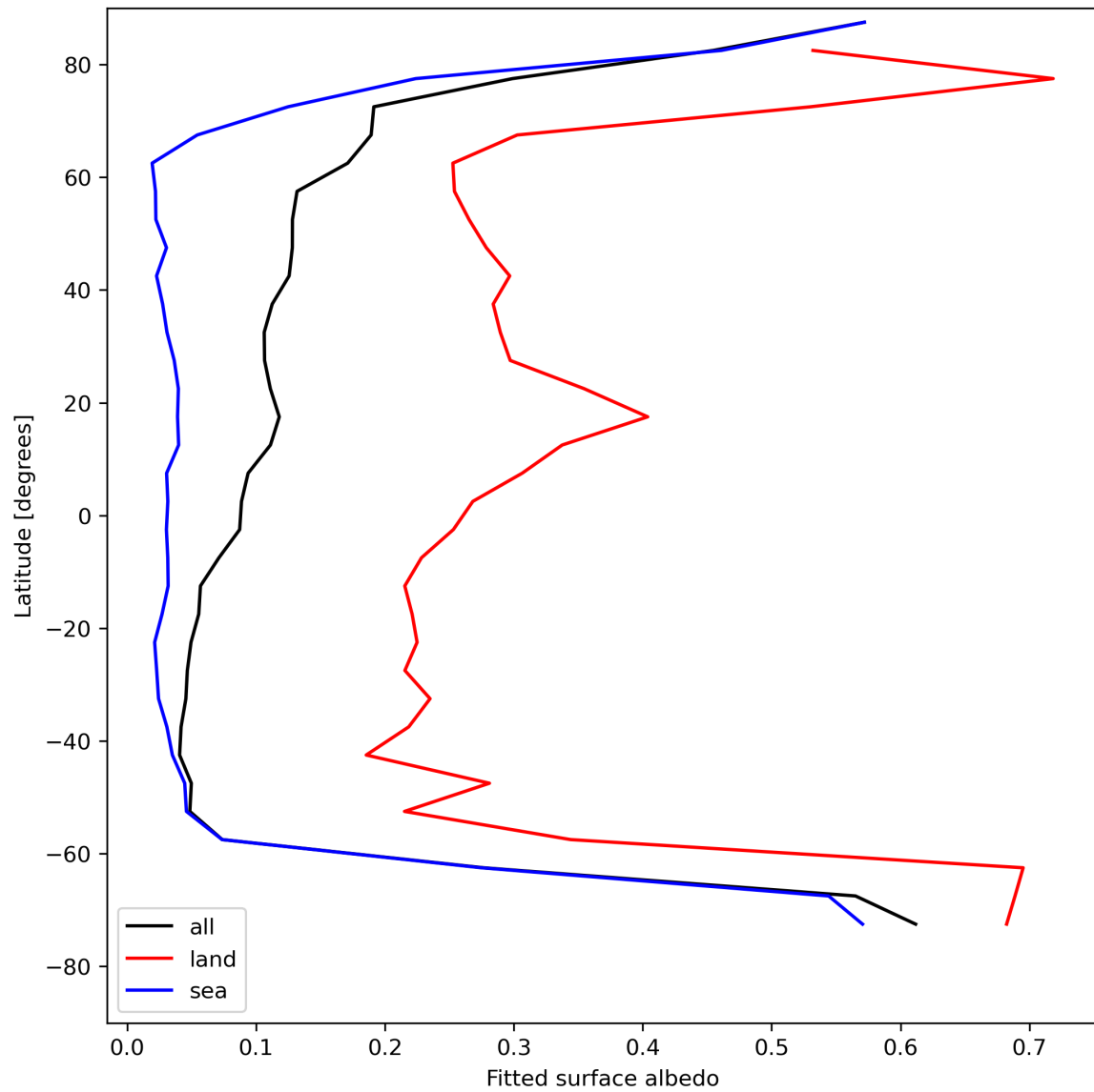
Figure 29: Zonal average of “Fitted surface albedo” for 2024-07-31 to 2024-08-02.
