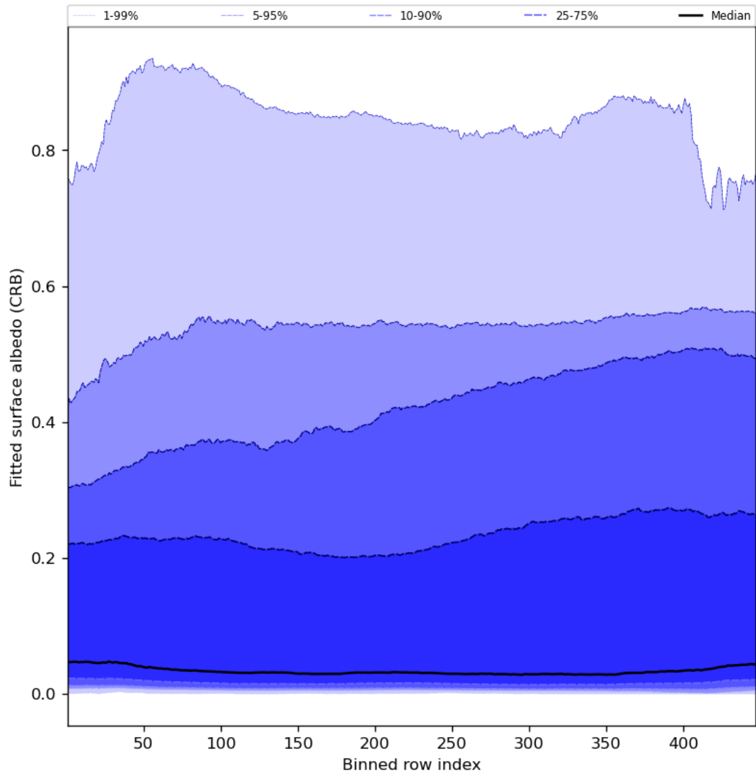
Figure 62: Along track statistics of “Fitted surface albedo (CRB)” for 2024-07-31 to 2024-08-02
