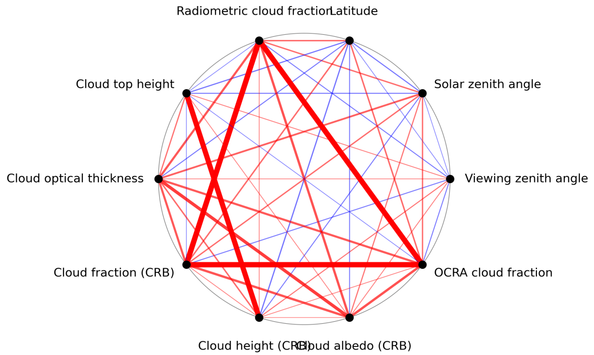
Figure 1: Map of correlation graph for 2024-07-31 to 2024-08-02.
