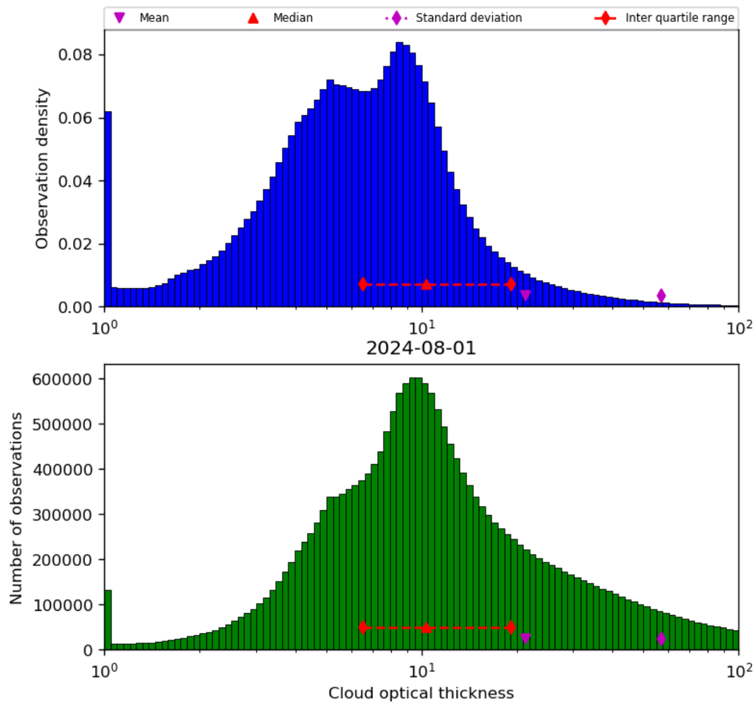
Figure 41: Histogram of “Cloud optical thickness” for 2024-07-31 to 2024-08-02
