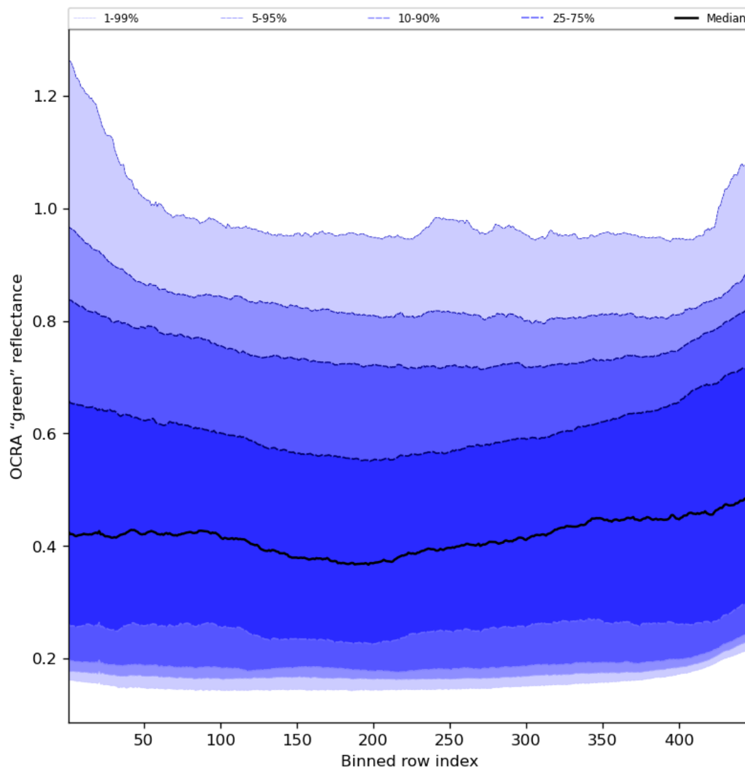
Figure 68: Along track statistics of “OCRA “green” reflectance” for 2024-08-06 to 2024-08-07
