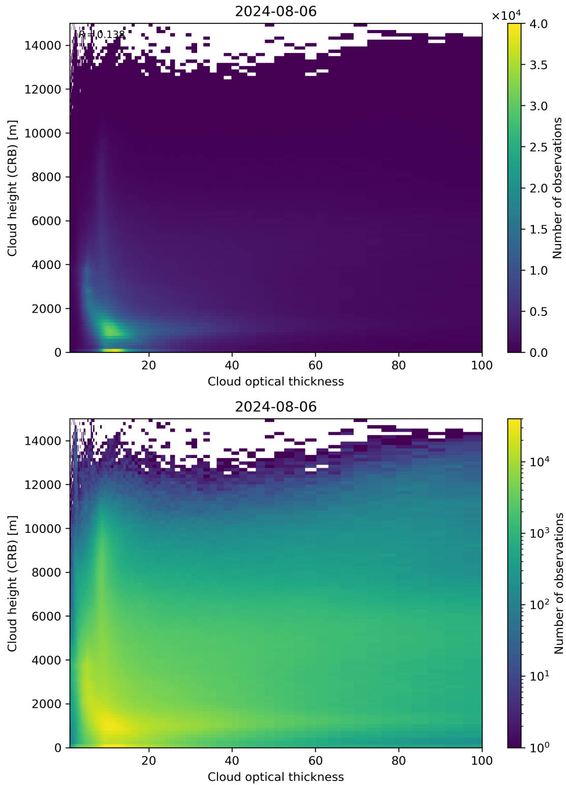
Figure 85: Scatter density plot of “Cloud optical thickness” against “Cloud height (CRB)” for 2024-08-06 to 2024-08-07.
