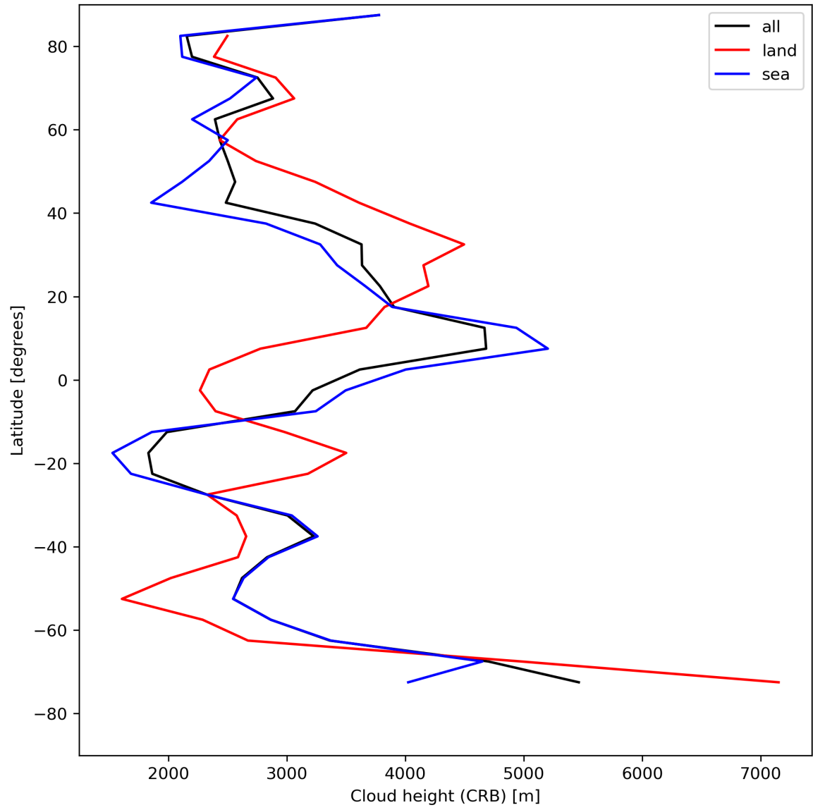
Figure 27: Zonal average of “Cloud height (CRB)” for 2024-08-06 to 2024-08-07.
