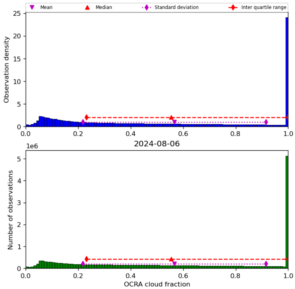
Figure 50: Histogram of “OCRA cloud fraction” for 2024-08-06 to 2024-08-07
