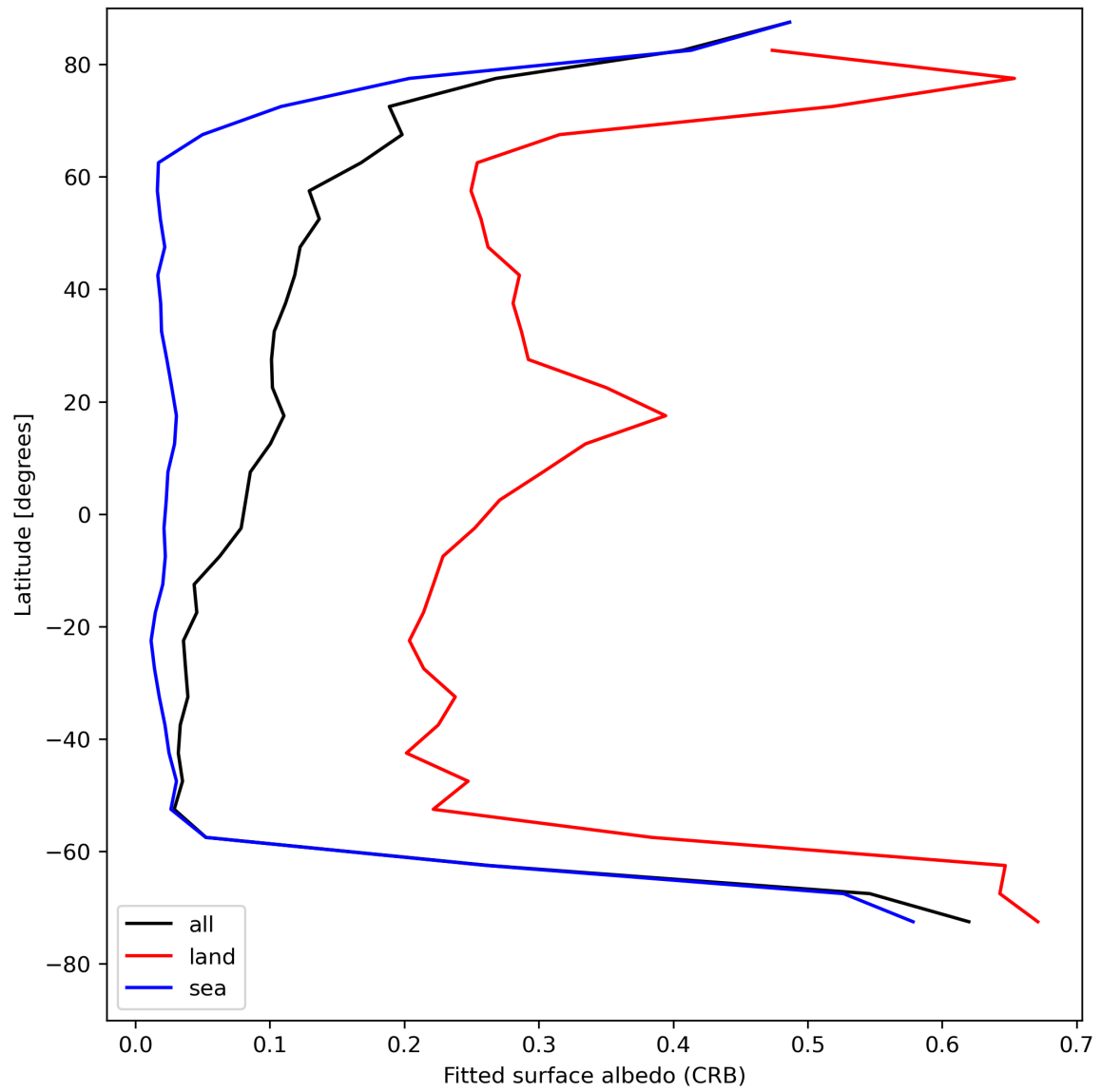
Figure 30: Zonal average of “Fitted surface albedo (CRB)” for 2024-08-06 to 2024-08-07.
