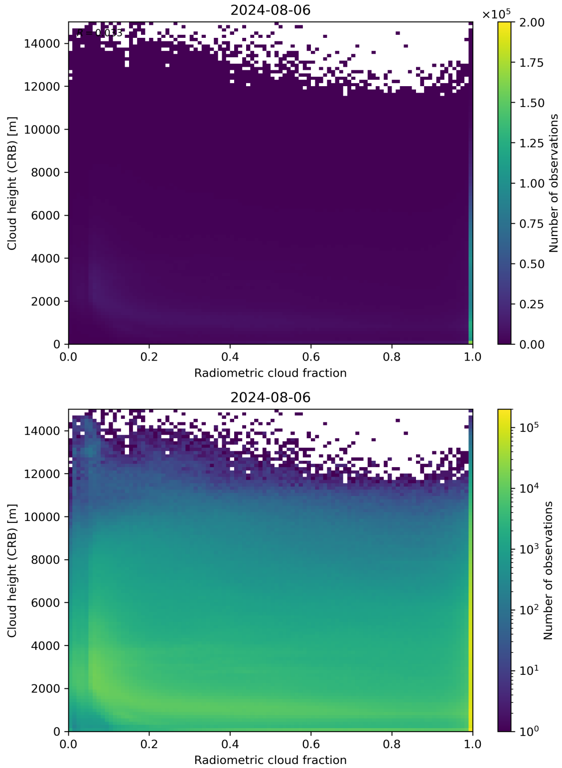
Figure 74: Scatter density plot of “Radiometric cloud fraction” against “Cloud height (CRB)” for 2024-08-06 to 2024-08-07.
