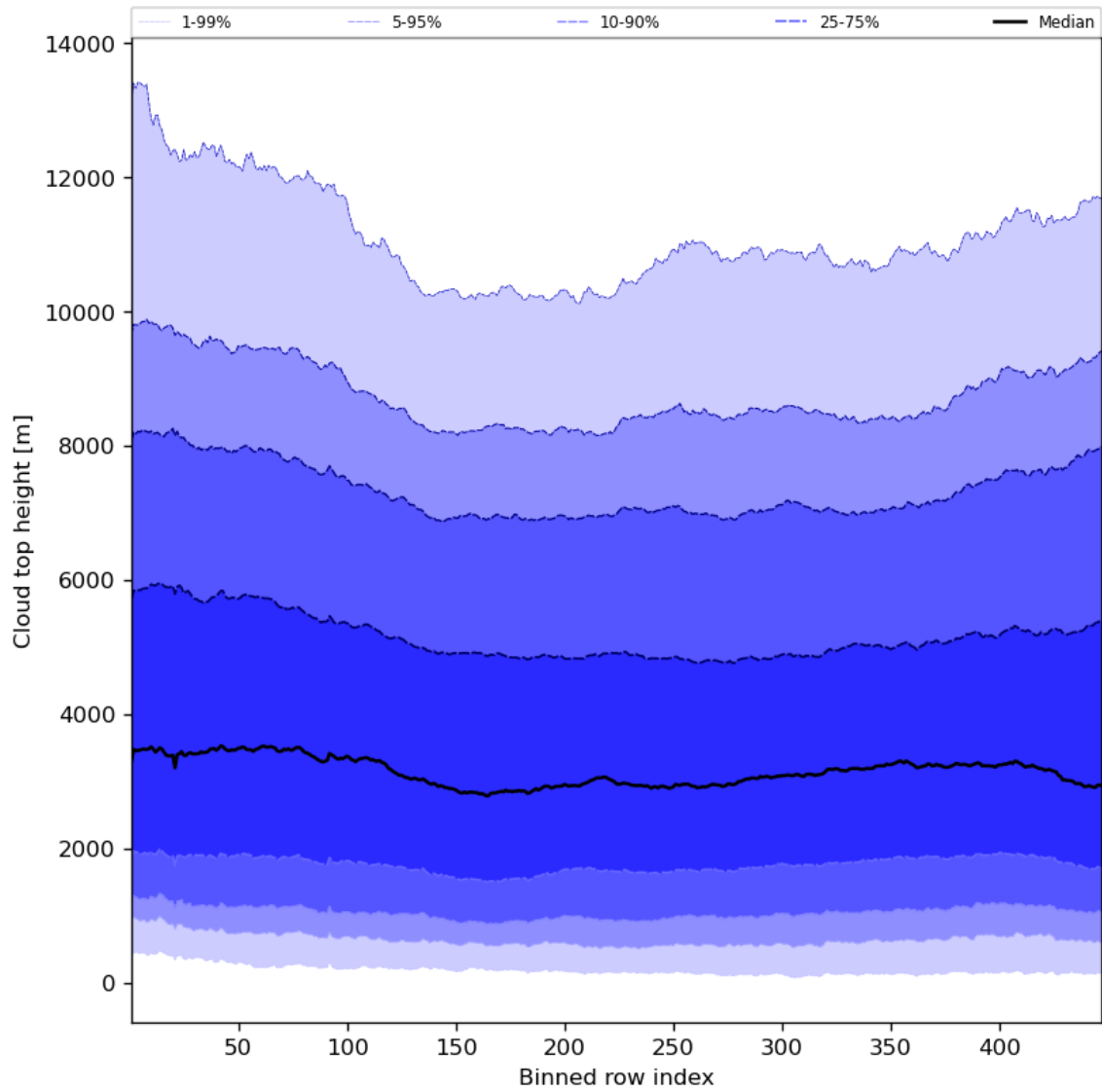
Figure 56: Along track statistics of “Cloud top height” for 2024-08-06 to 2024-08-07
