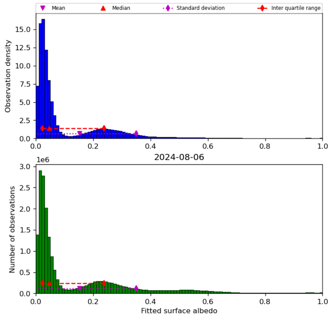
Figure 45: Histogram of “Fitted surface albedo” for 2024-08-06 to 2024-08-07
