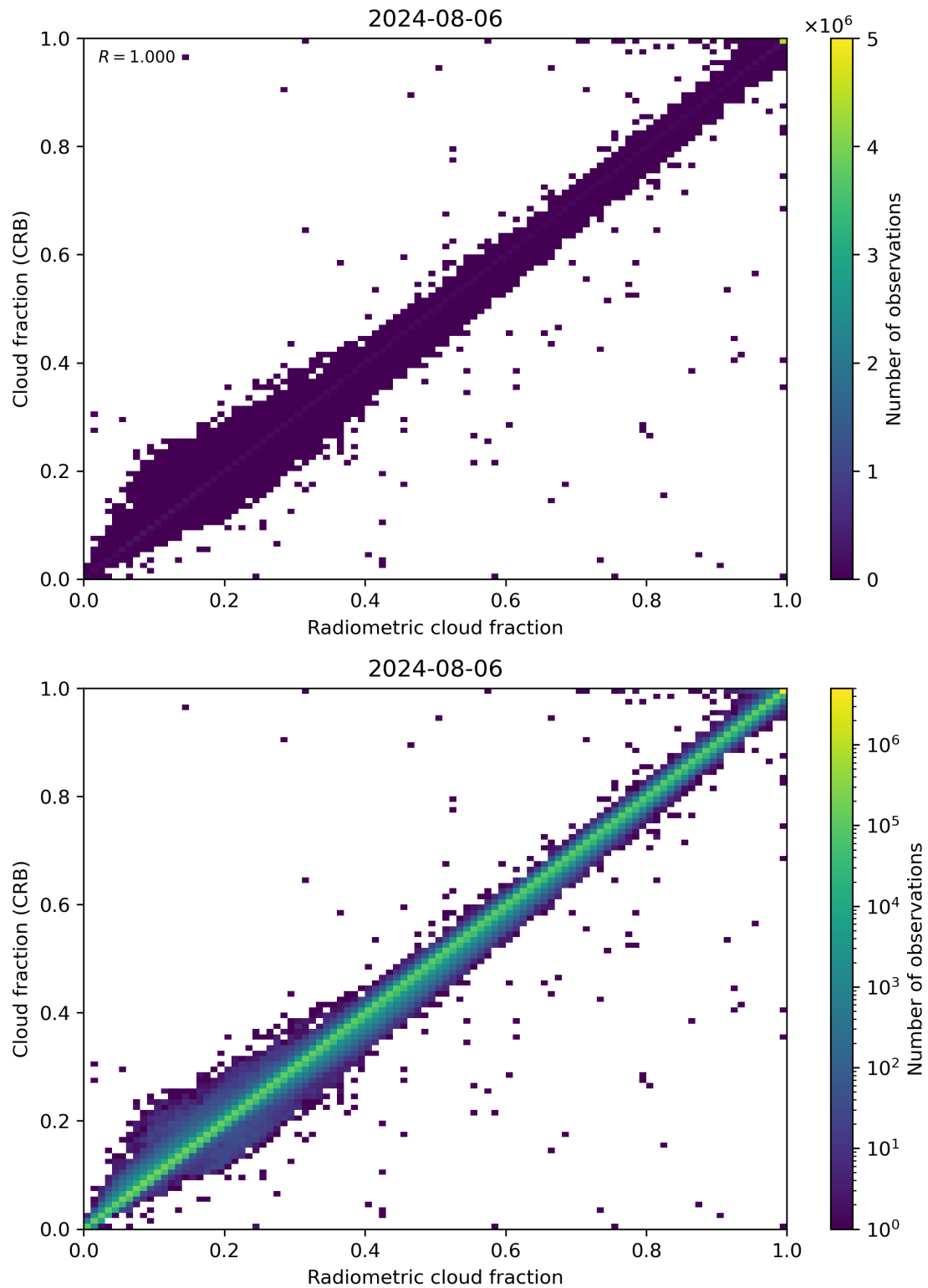
Figure 73: Scatter density plot of “Radiometric cloud fraction” against “Cloud fraction (CRB)” for 2024-08-06 to 2024-08-07.
