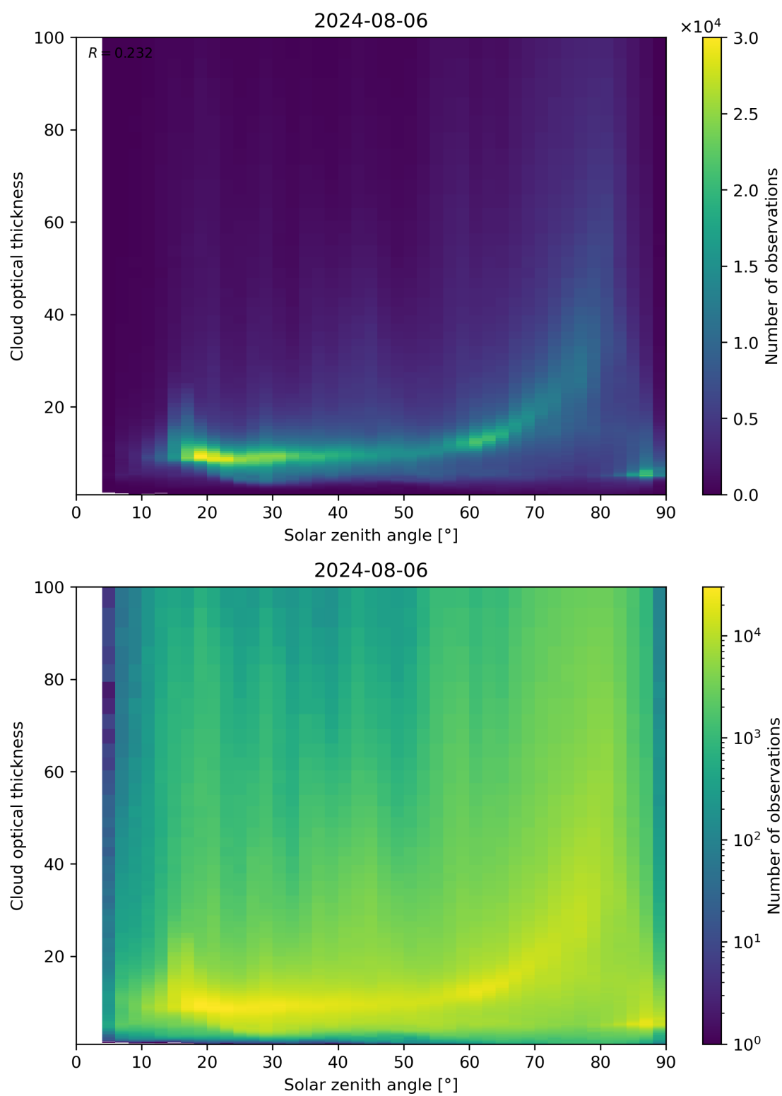
Figure 103: Scatter density plot of “Solar zenith angle” against “Cloud optical thickness” for 2024-08-06 to 2024-08-07.
