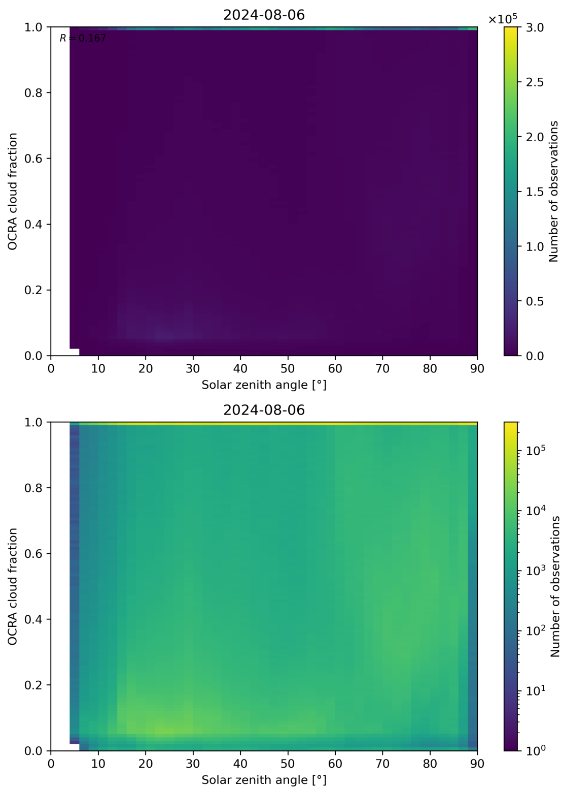
Figure 100: Scatter density plot of “Solar zenith angle” against “OCRA cloud fraction” for 2024-08-06 to 2024-08-07.
