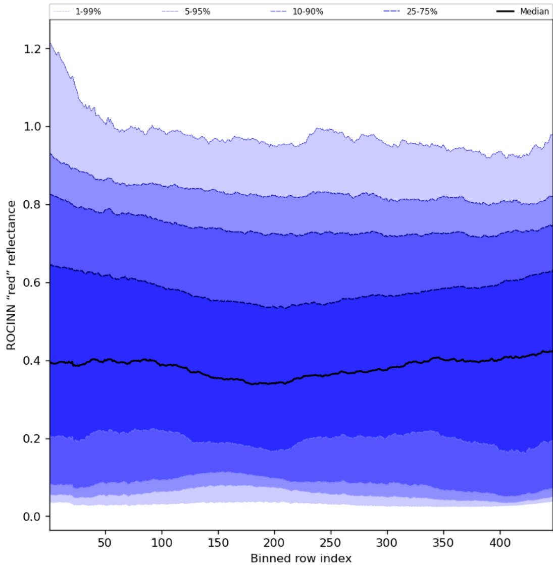
Figure 69: Along track statistics of “ROCINN “red” reflectance” for 2024-08-06 to 2024-08-07
