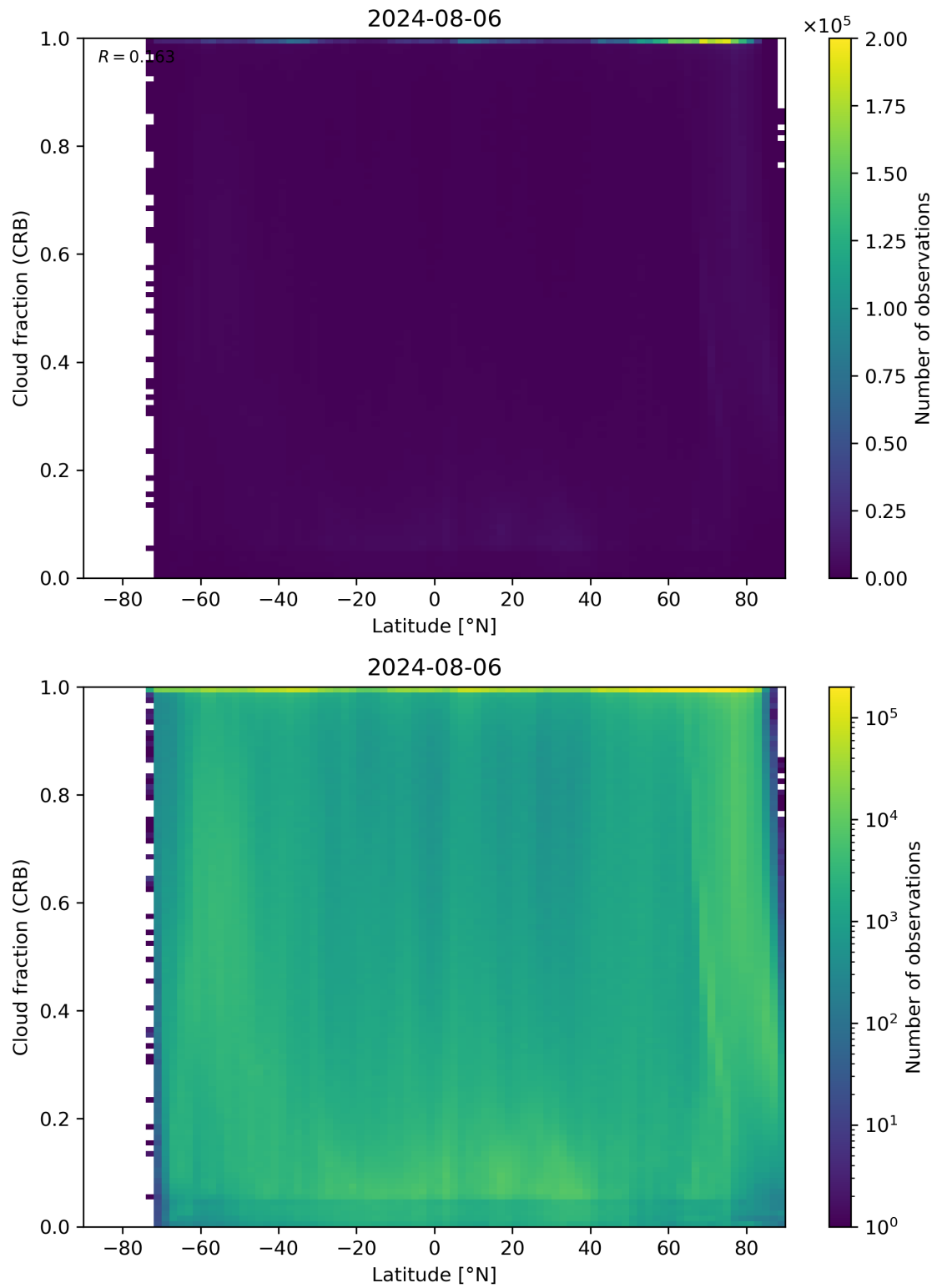
Figure 94: Scatter density plot of “Latitude” against “Cloud fraction (CRB)” for 2024-08-06 to 2024-08-07.
