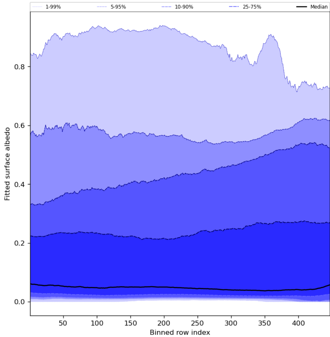
Figure 61: Along track statistics of “Fitted surface albedo” for 2024-08-06 to 2024-08-07
