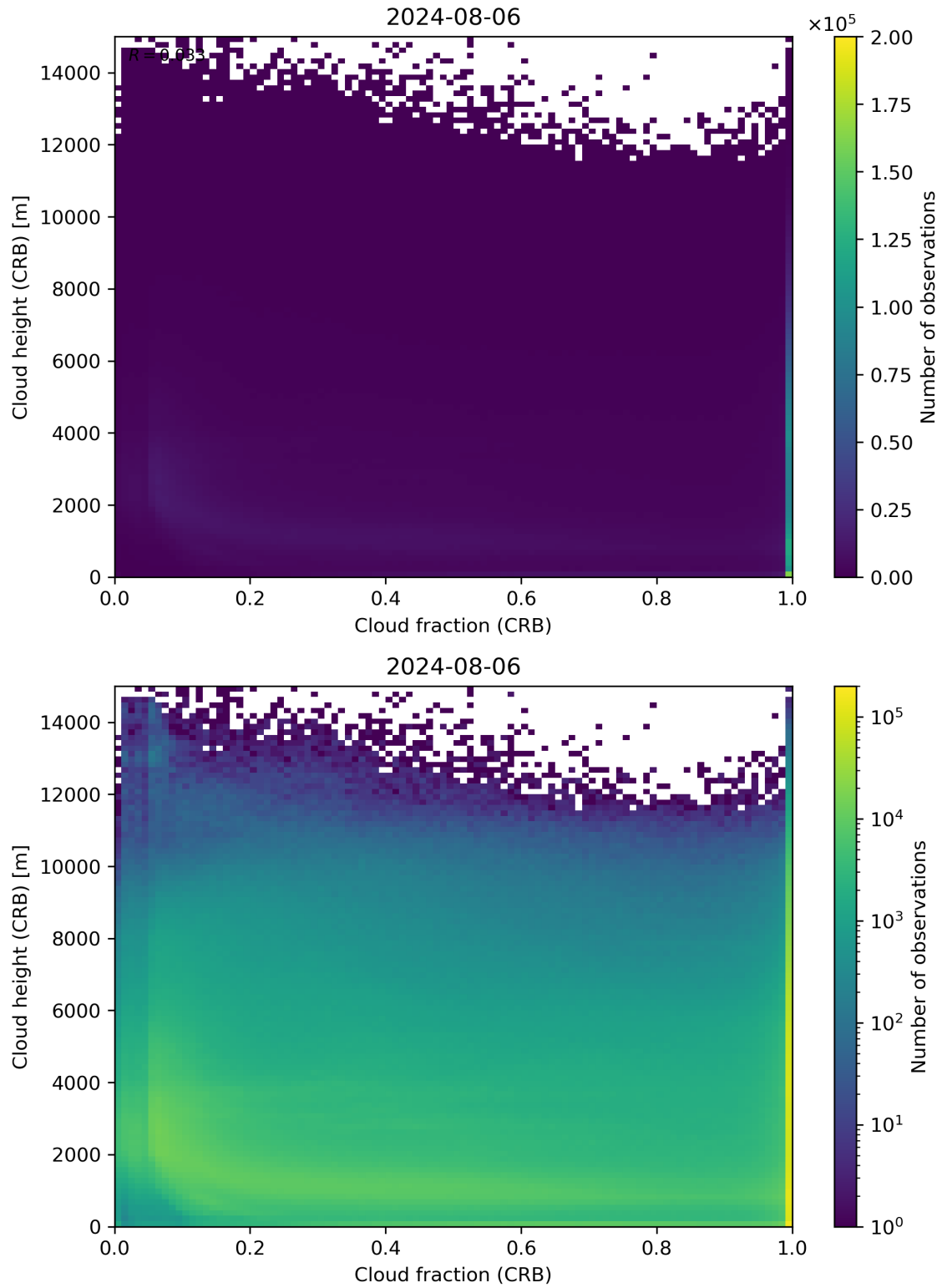
Figure 79: Scatter density plot of “Cloud fraction (CRB)” against “Cloud height (CRB)” for 2024-08-06 to 2024-08-07.
