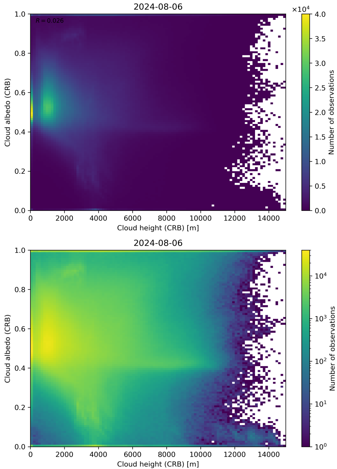
Figure 80: Scatter density plot of “Cloud height (CRB)” against “Cloud albedo (CRB)” for 2024-08-06 to 2024-08-07.
