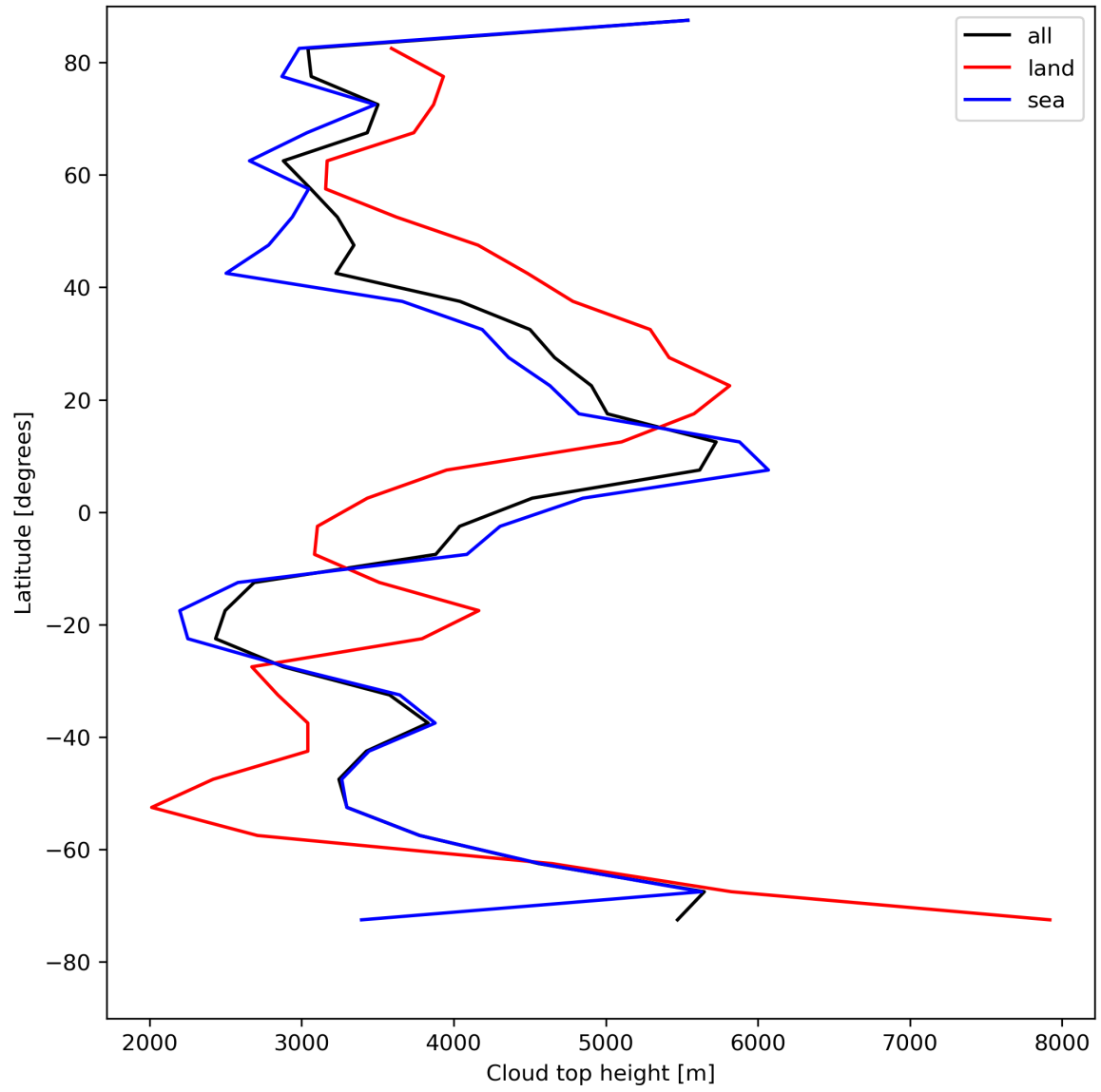
Figure 24: Zonal average of “Cloud top height” for 2024-08-06 to 2024-08-07.
