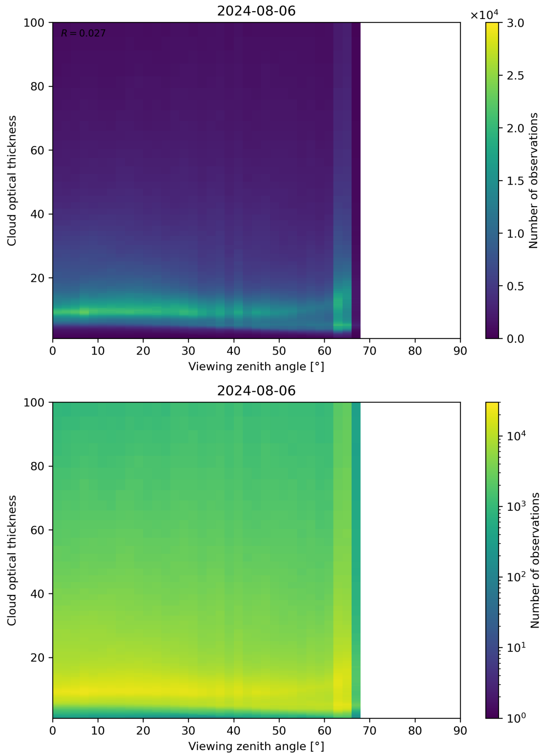
Figure 111: Scatter density plot of “Viewing zenith angle” against “Cloud optical thickness” for 2024-08-06 to 2024-08-07.
