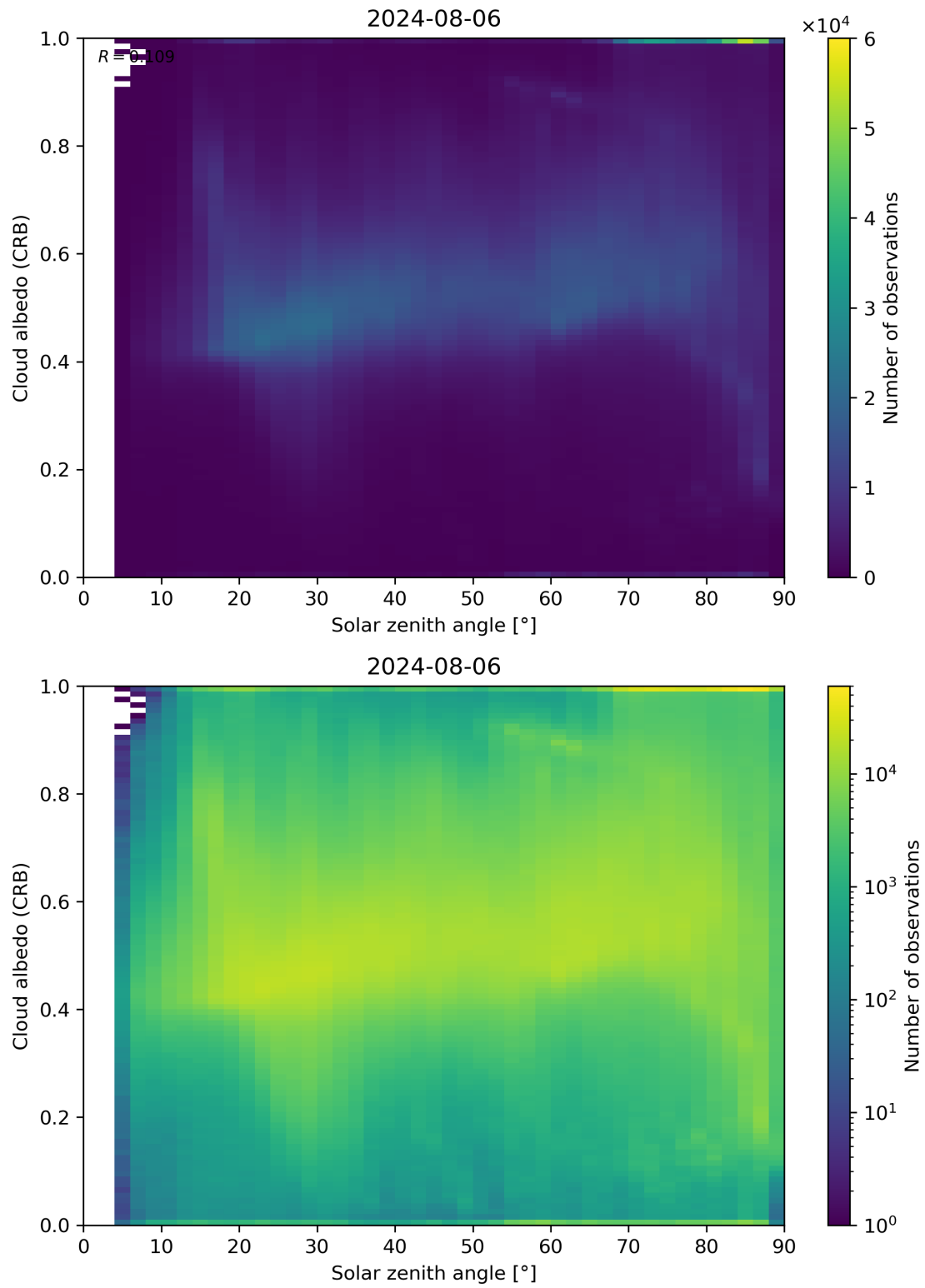
Figure 98: Scatter density plot of “Solar zenith angle” against “Cloud albedo (CRB)” for 2024-08-06 to 2024-08-07.
