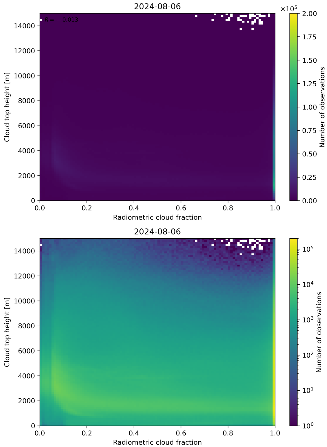
Figure 76: Scatter density plot of “Radiometric cloud fraction” against “Cloud top height” for 2024-08-06 to 2024-08-07.
