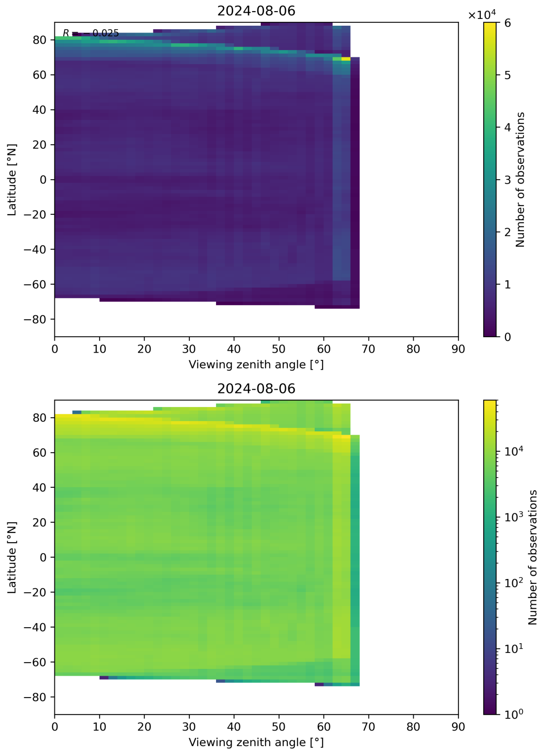
Figure 113: Scatter density plot of “Viewing zenith angle” against “Latitude” for 2024-08-06 to 2024-08-07.
