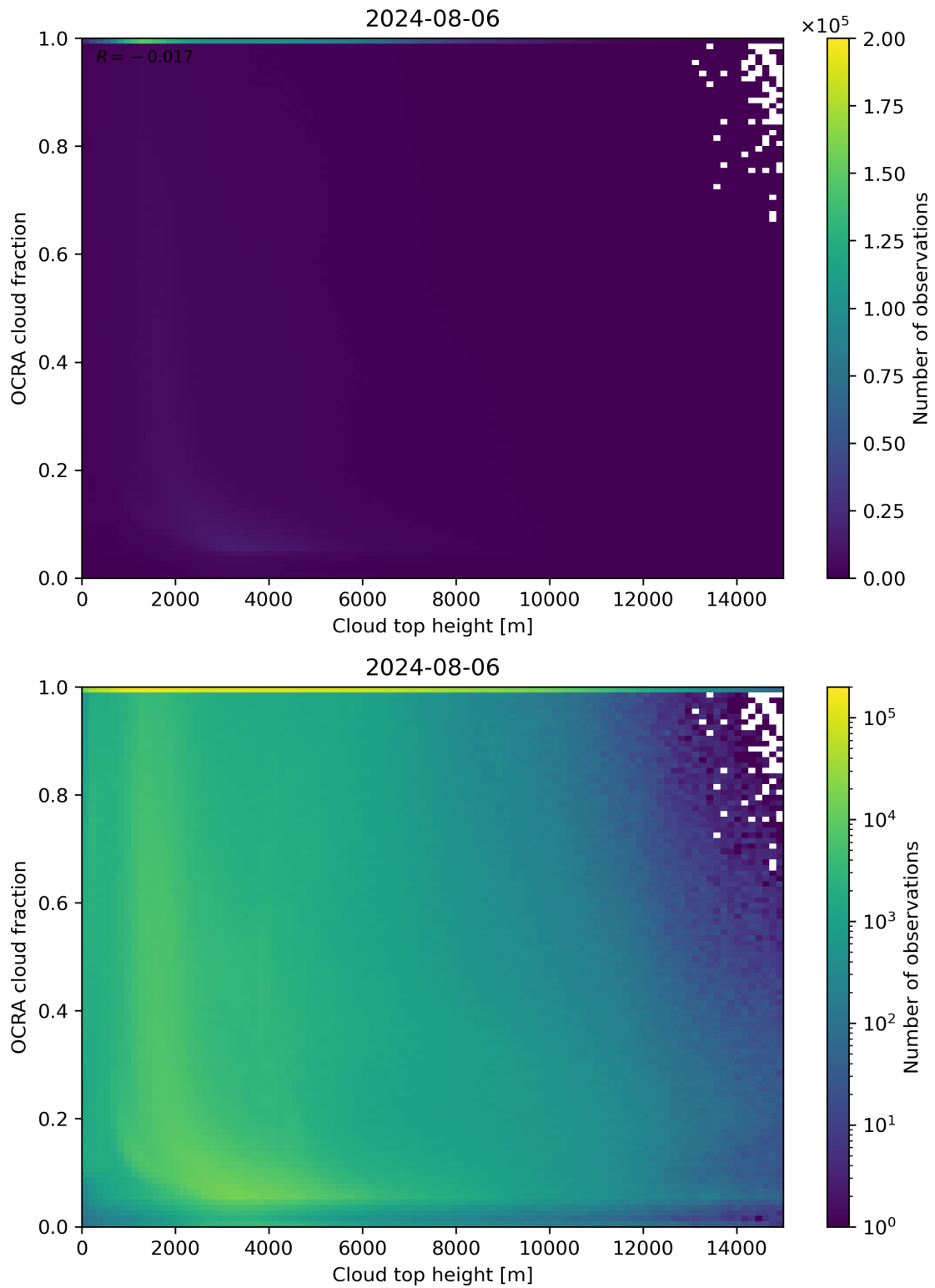
Figure 87: Scatter density plot of “Cloud top height” against “OCRA cloud fraction” for 2024-08-06 to 2024-08-07.
