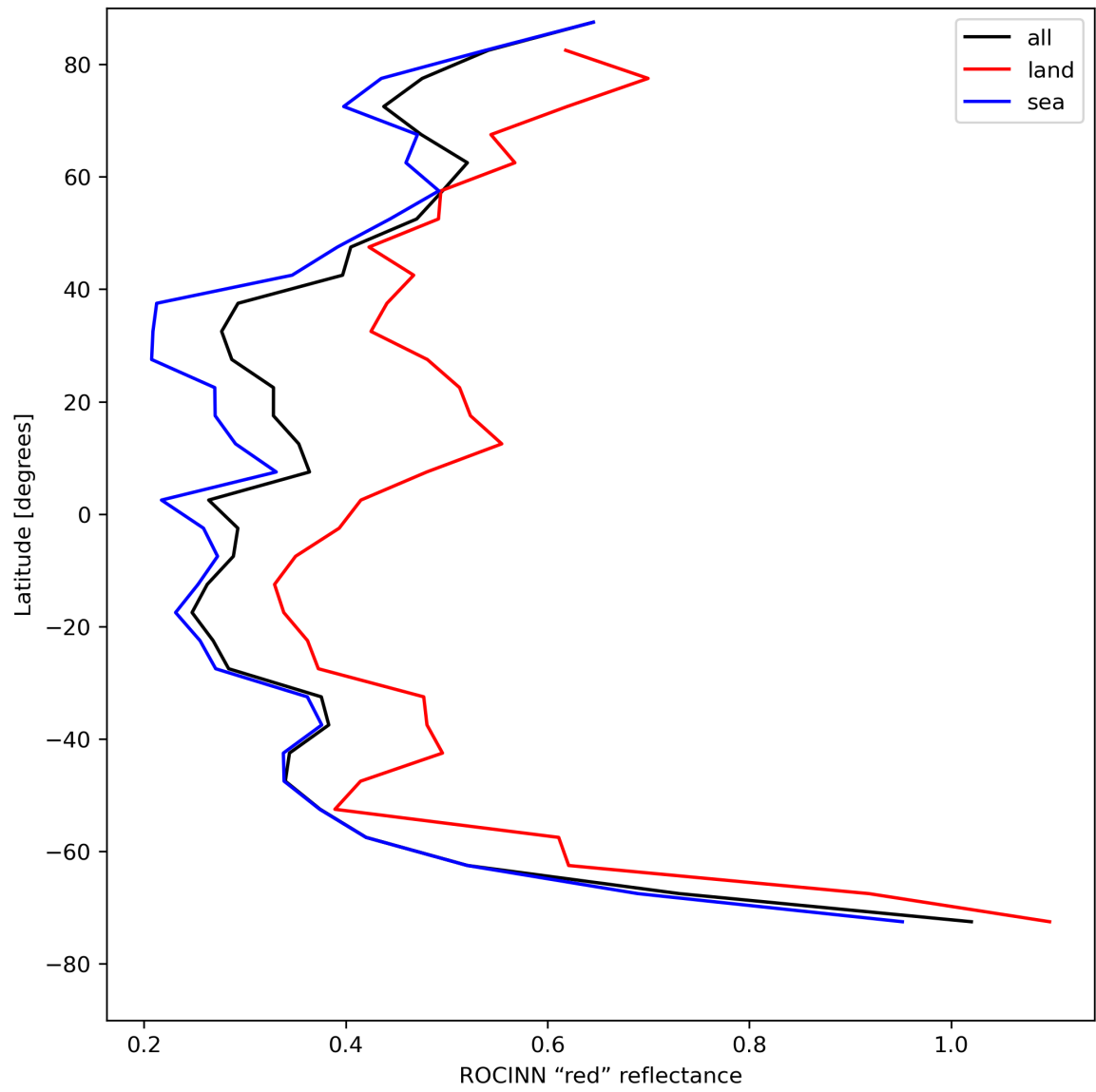
Figure 37: Zonal average of “ROCINN “red” reflectance” for 2024-08-06 to 2024-08-07.
