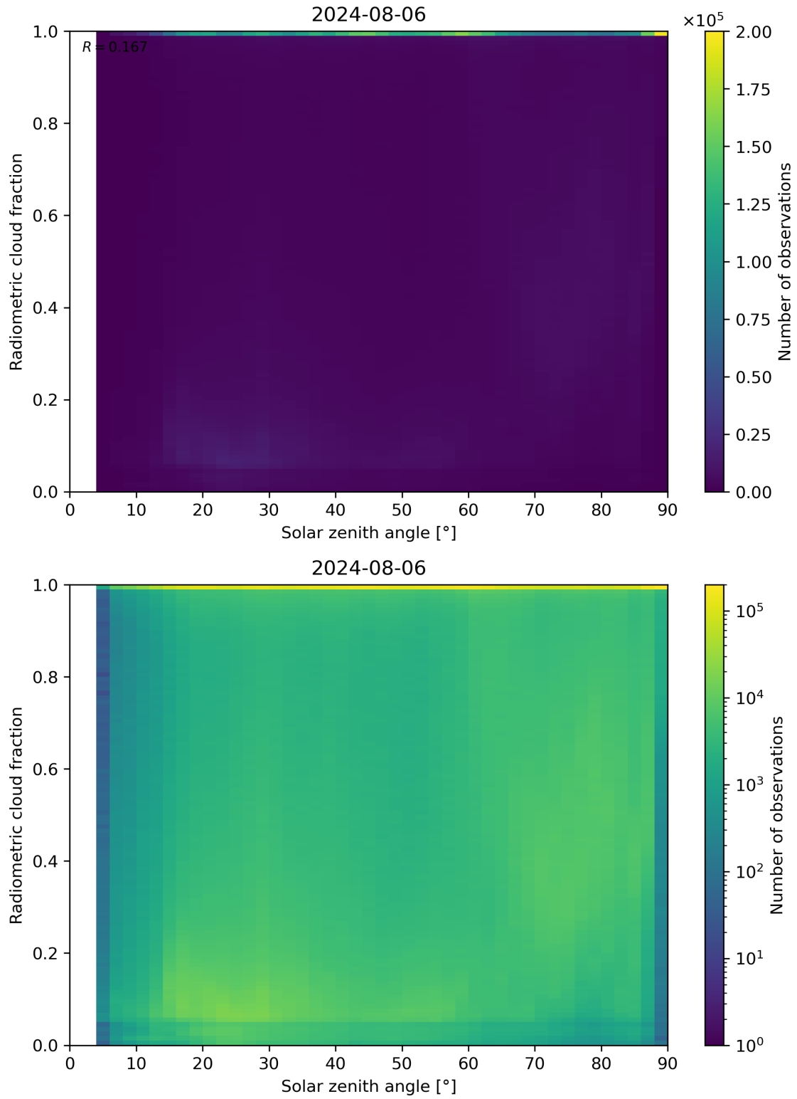
Figure 99: Scatter density plot of “Solar zenith angle” against “Radiometric cloud fraction” for 2024-08-06 to 2024-08-07.
