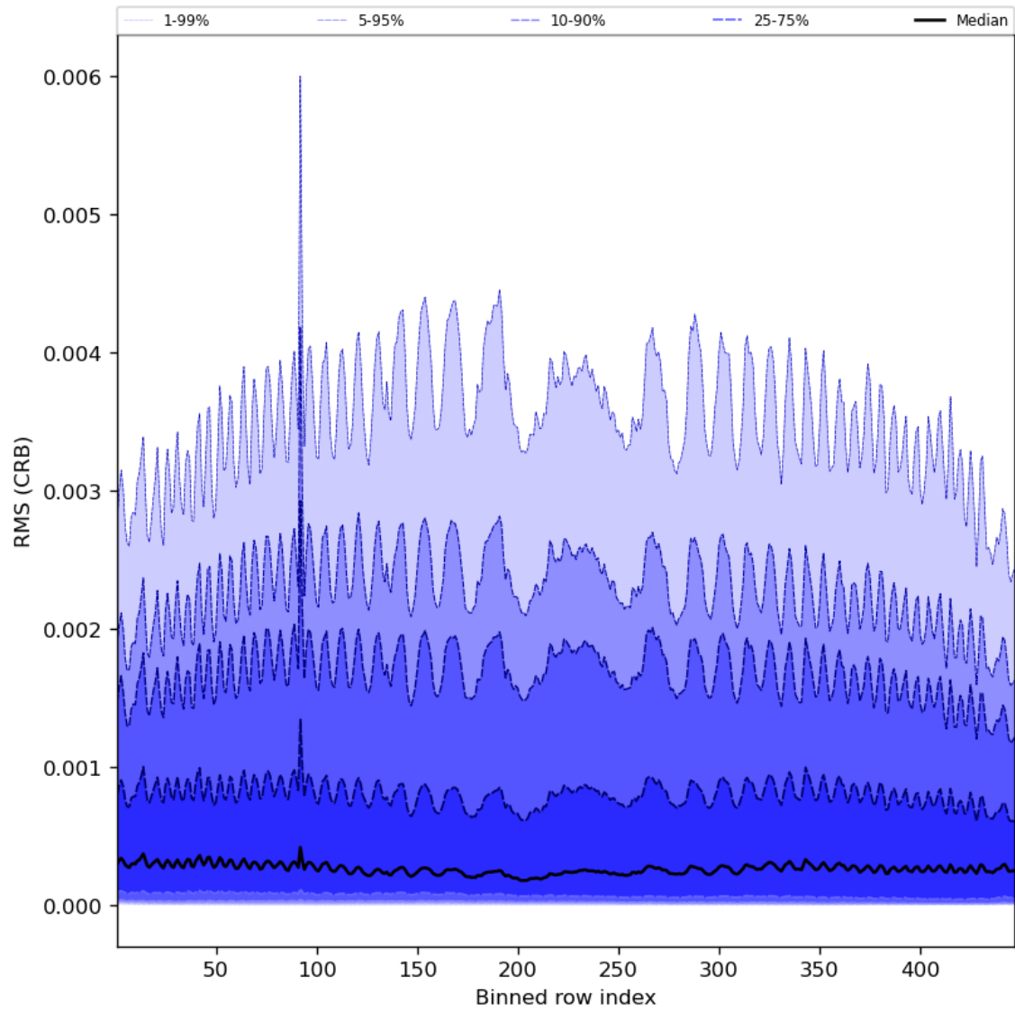
Figure 64: Along track statistics of “RMS (CRB)” for 2024-08-06 to 2024-08-07
