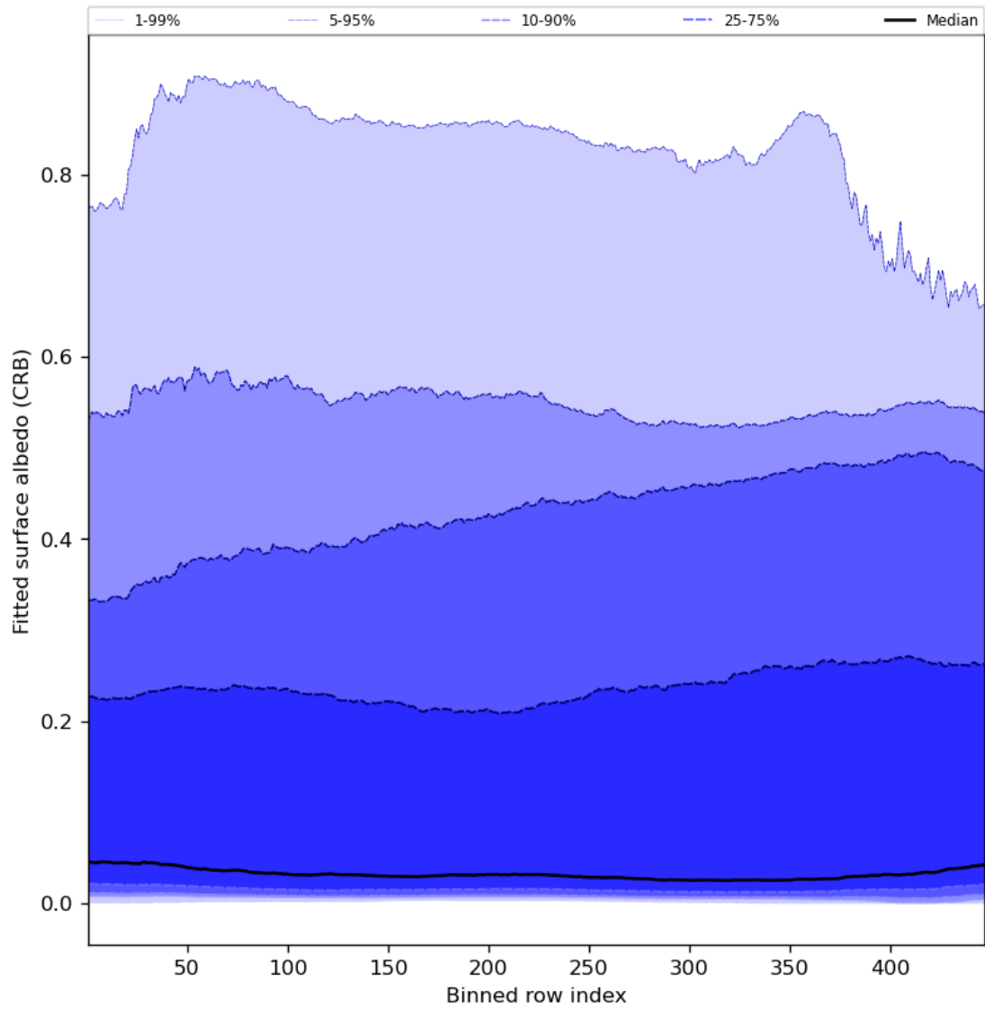
Figure 62: Along track statistics of “Fitted surface albedo (CRB)” for 2024-08-06 to 2024-08-07
