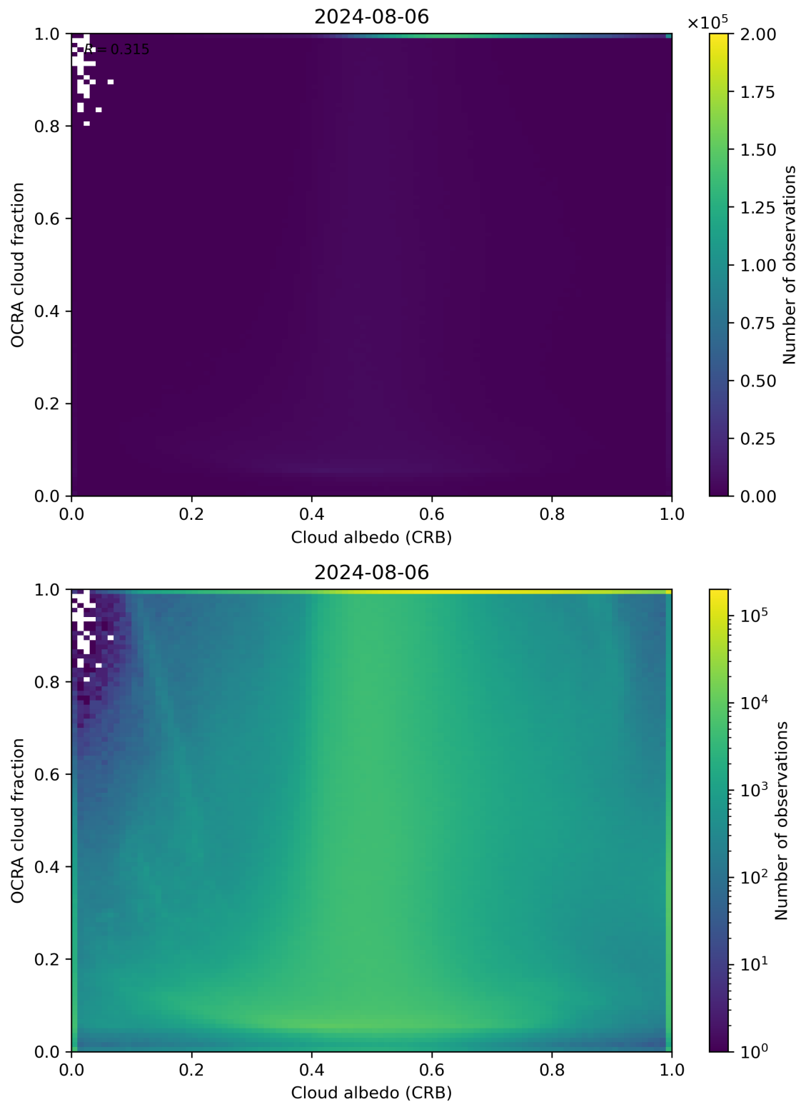
Figure 70: Scatter density plot of “Cloud albedo (CRB)” against “OCRA cloud fraction” for 2024-08-06 to 2024-08-07.
