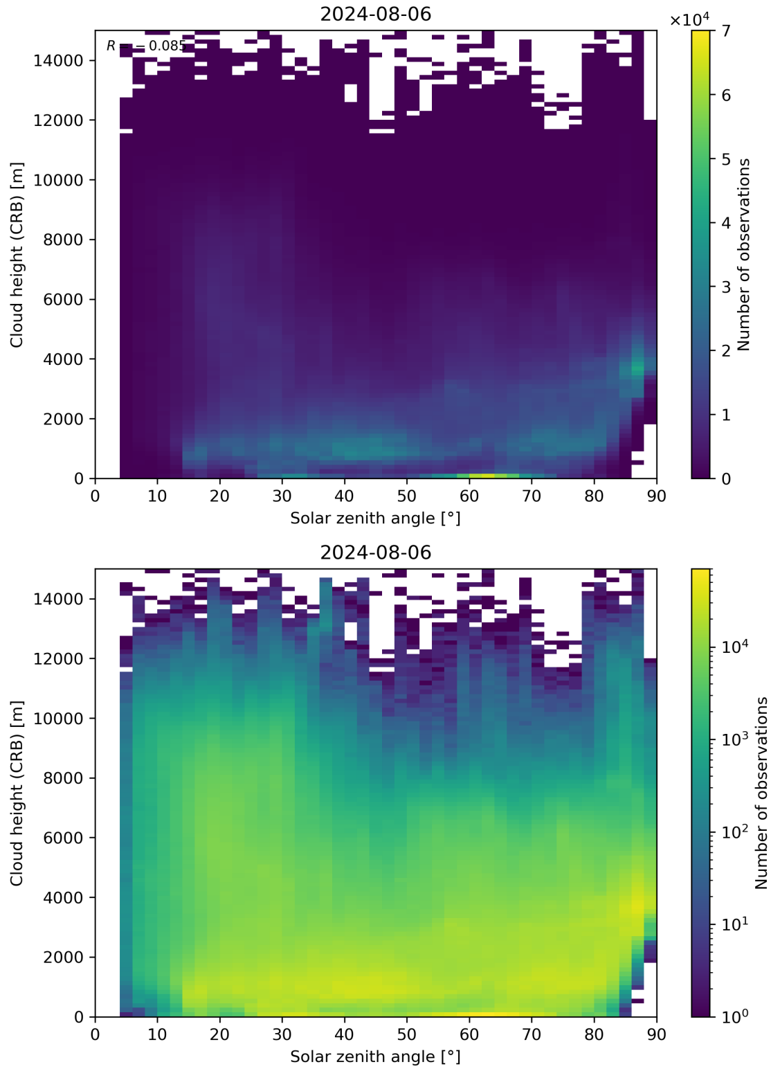
Figure 102: Scatter density plot of “Solar zenith angle” against “Cloud height (CRB)” for 2024-08-06 to 2024-08-07.
