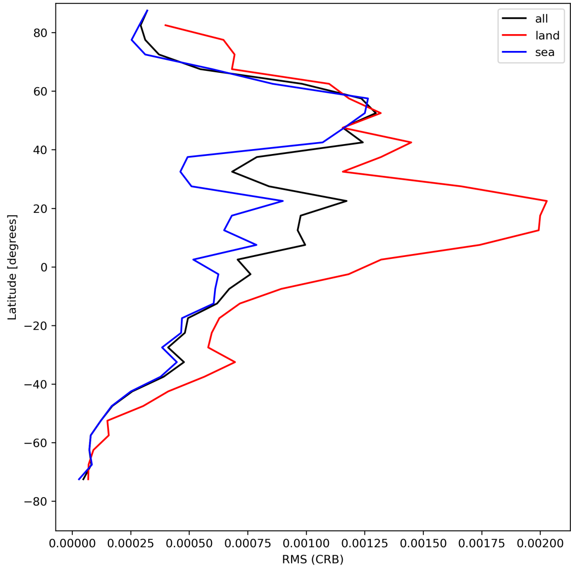
Figure 32: Zonal average of “RMS (CRB)” for 2024-08-06 to 2024-08-07.
