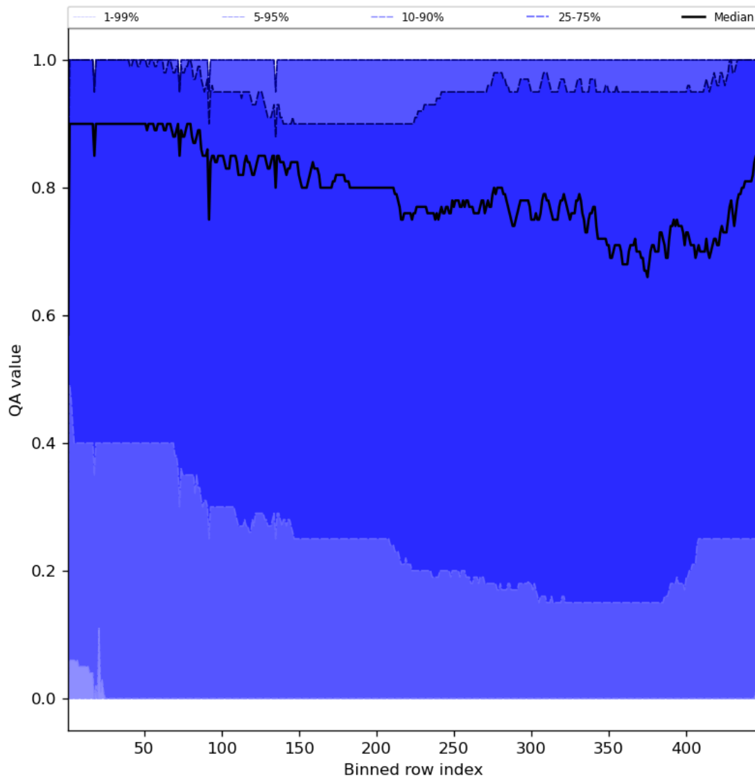
Figure 54: Along track statistics of “QA value” for 2024-08-06 to 2024-08-07
