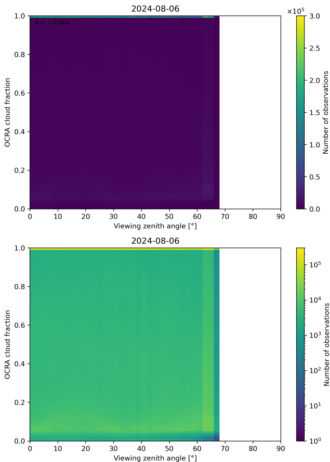
Figure 108: Scatter density plot of “Viewing zenith angle” against “OCRA cloud fraction” for 2024-08-06 to 2024-08-07.
