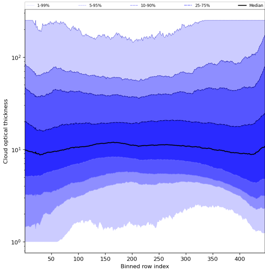
Figure 57: Along track statistics of “Cloud optical thickness” for 2024-08-06 to 2024-08-07
