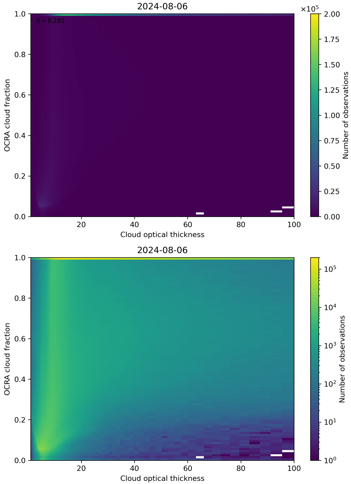
Figure 83: Scatter density plot of “Cloud optical thickness” against “OCRA cloud fraction” for 2024-08-06 to 2024-08-07.
