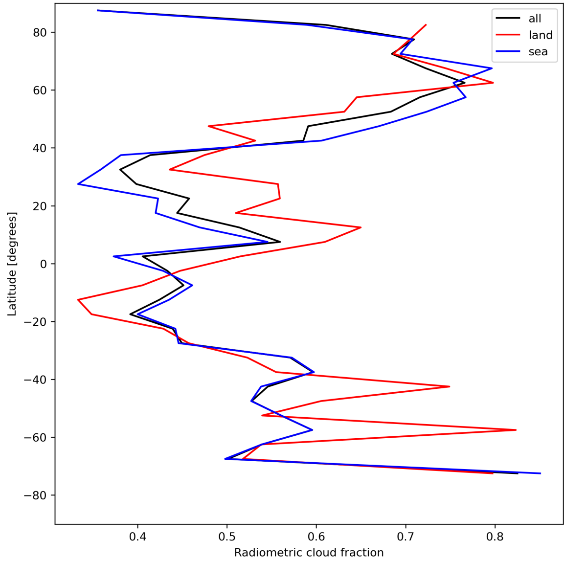
Figure 23: Zonal average of “Radiometric cloud fraction” for 2024-08-06 to 2024-08-07.
