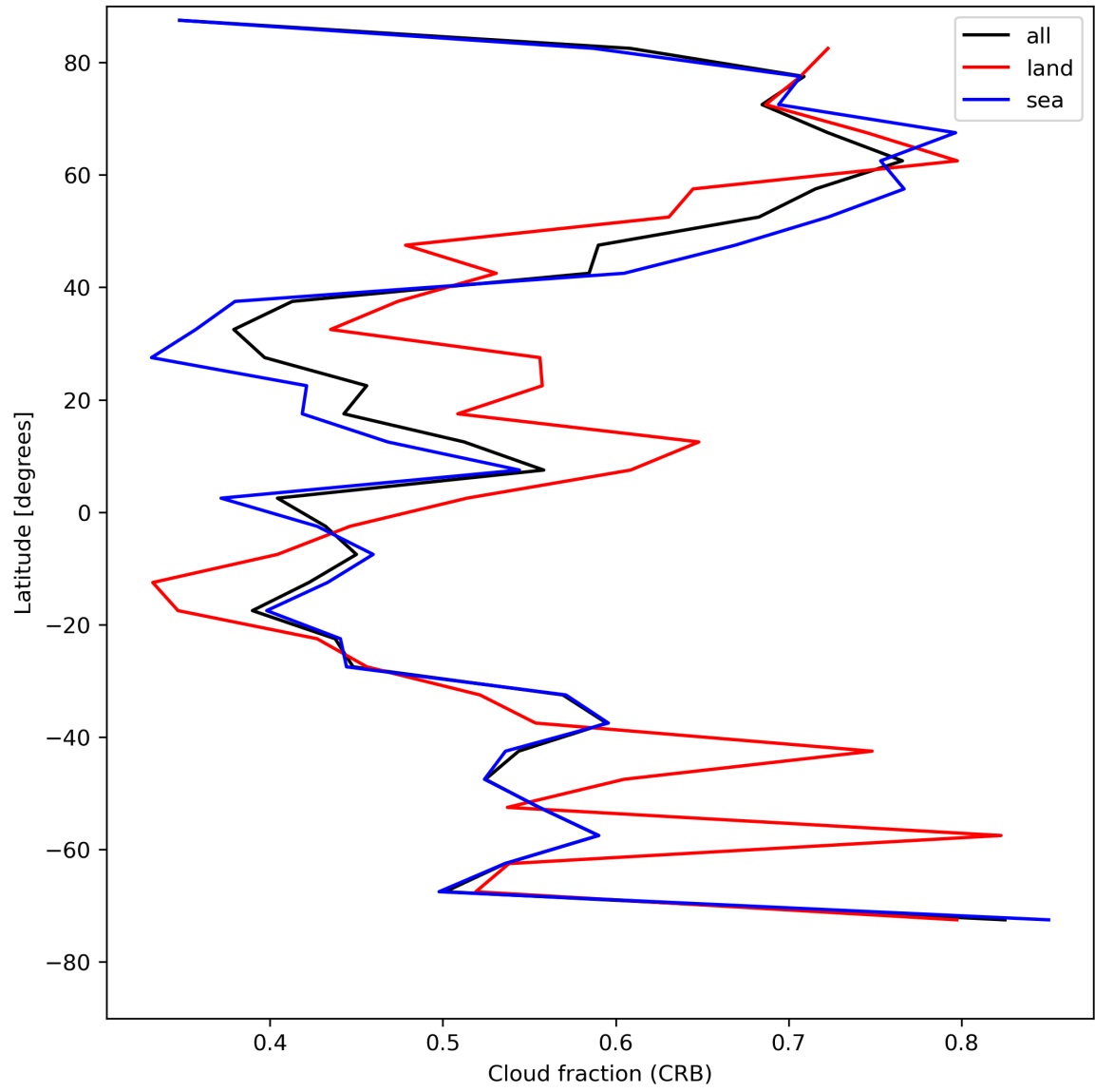
Figure 26: Zonal average of “Cloud fraction (CRB)” for 2024-08-06 to 2024-08-07.
