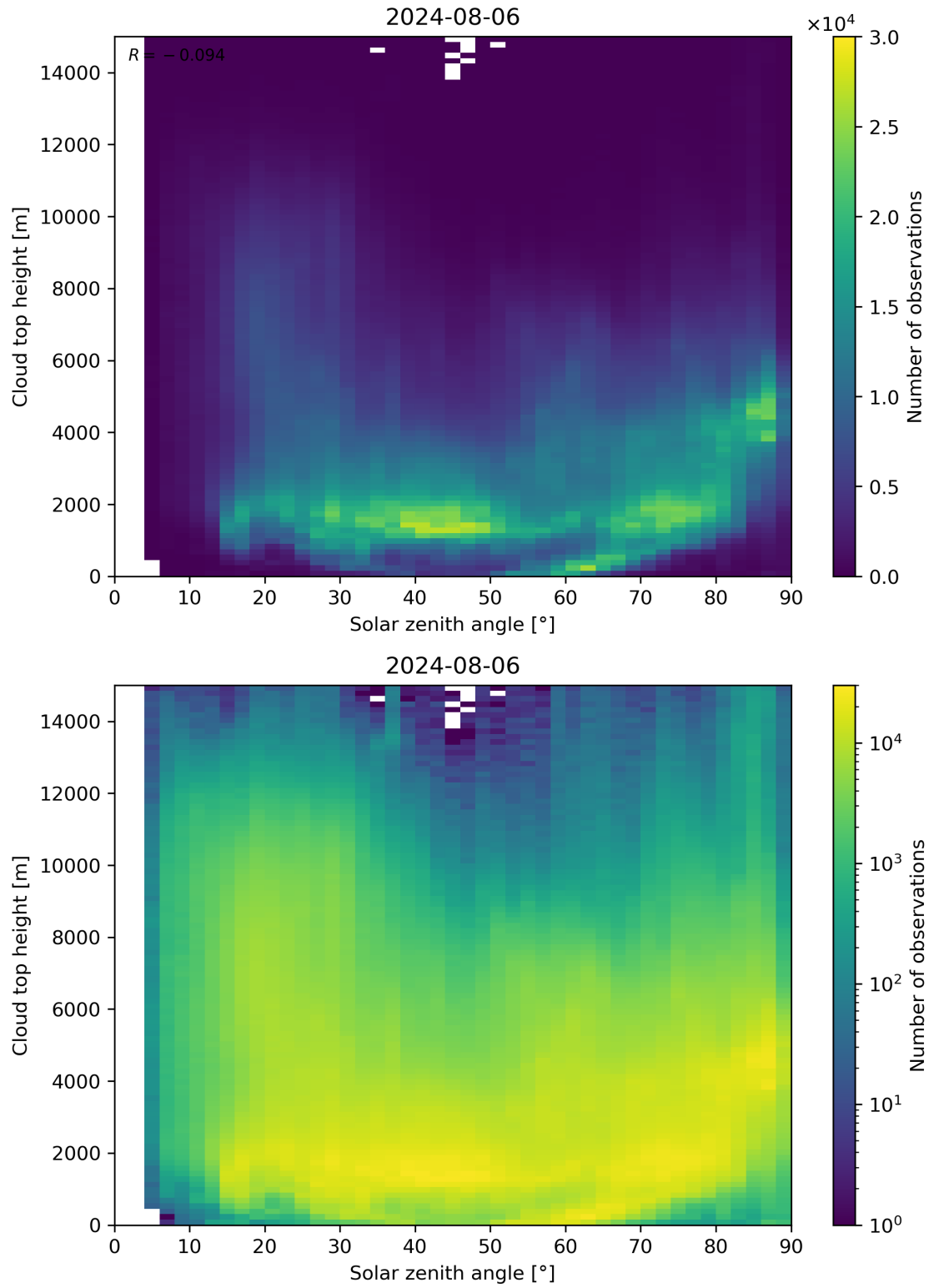
Figure 104: Scatter density plot of “Solar zenith angle” against “Cloud top height” for 2024-08-06 to 2024-08-07.
