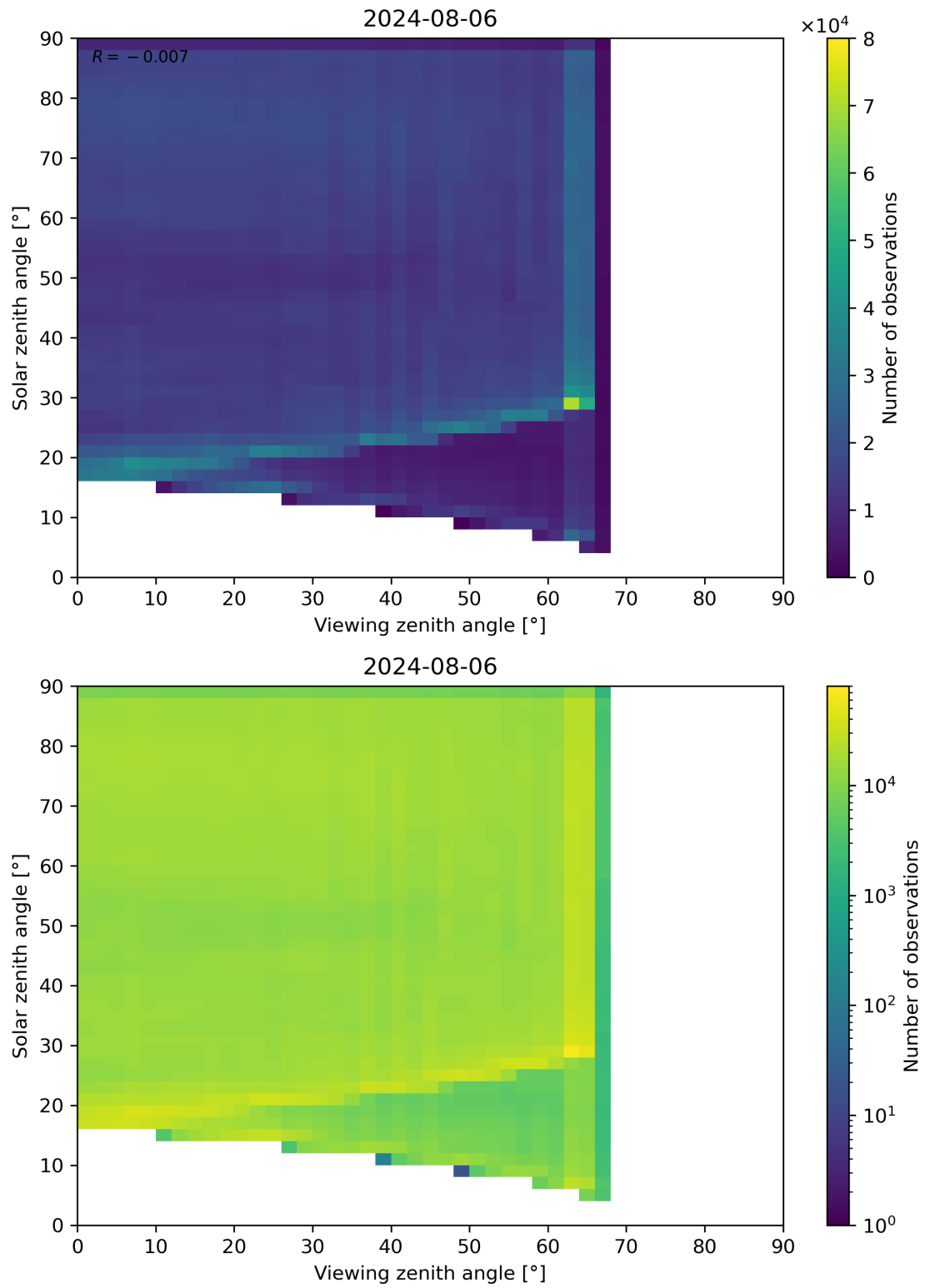
Figure 114: Scatter density plot of “Viewing zenith angle” against “Solar zenith angle” for 2024-08-06 to 2024-08-07.
