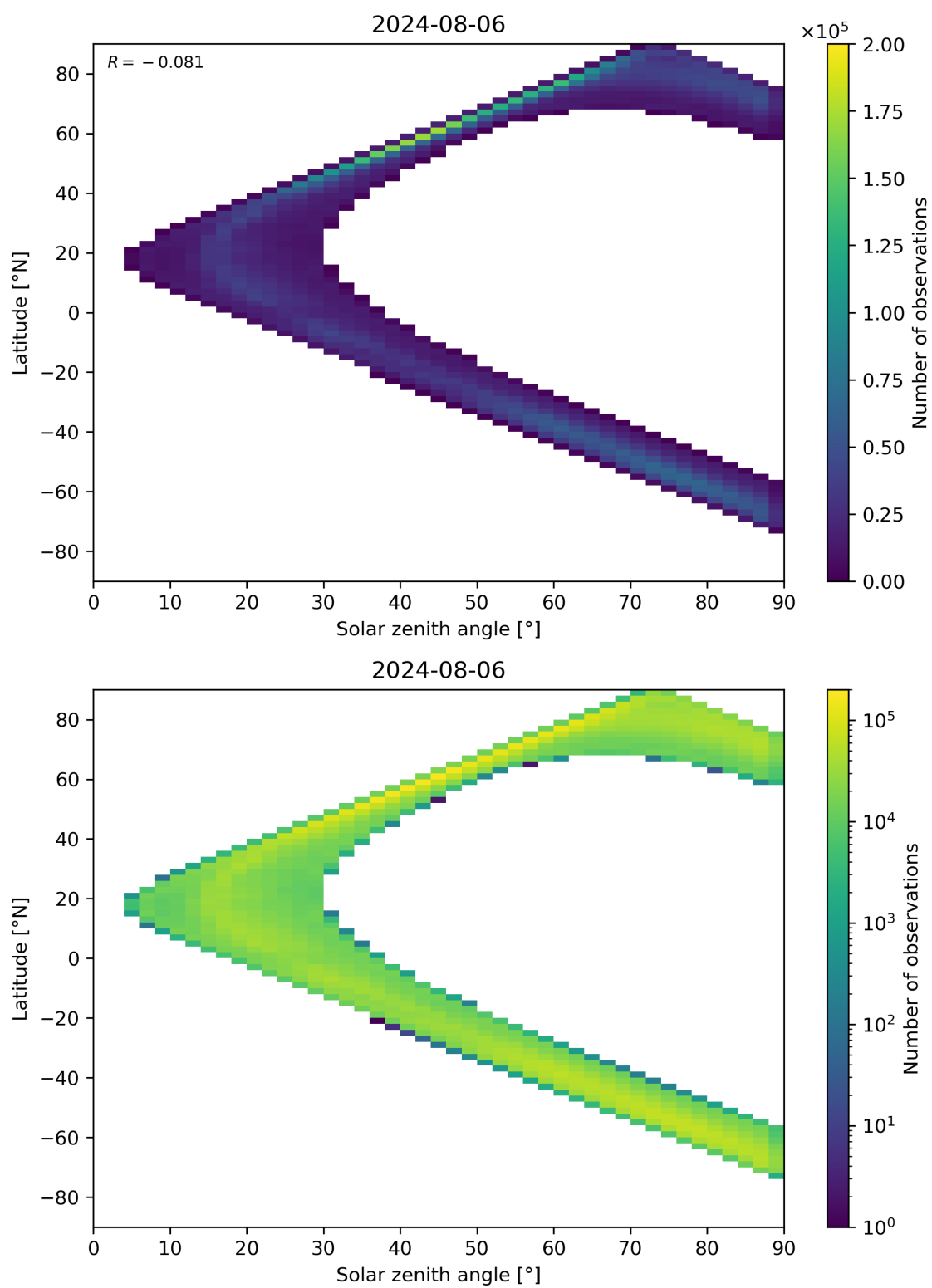
Figure 105: Scatter density plot of “Solar zenith angle” against “Latitude” for 2024-08-06 to 2024-08-07.
