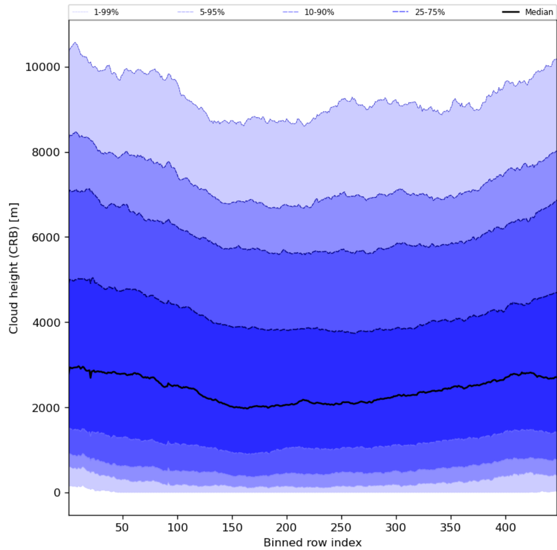
Figure 59: Along track statistics of “Cloud height (CRB)” for 2024-08-06 to 2024-08-07
