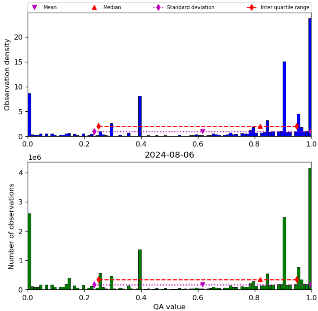
Figure 38: Histogram of “QA value” for 2024-08-06 to 2024-08-07
