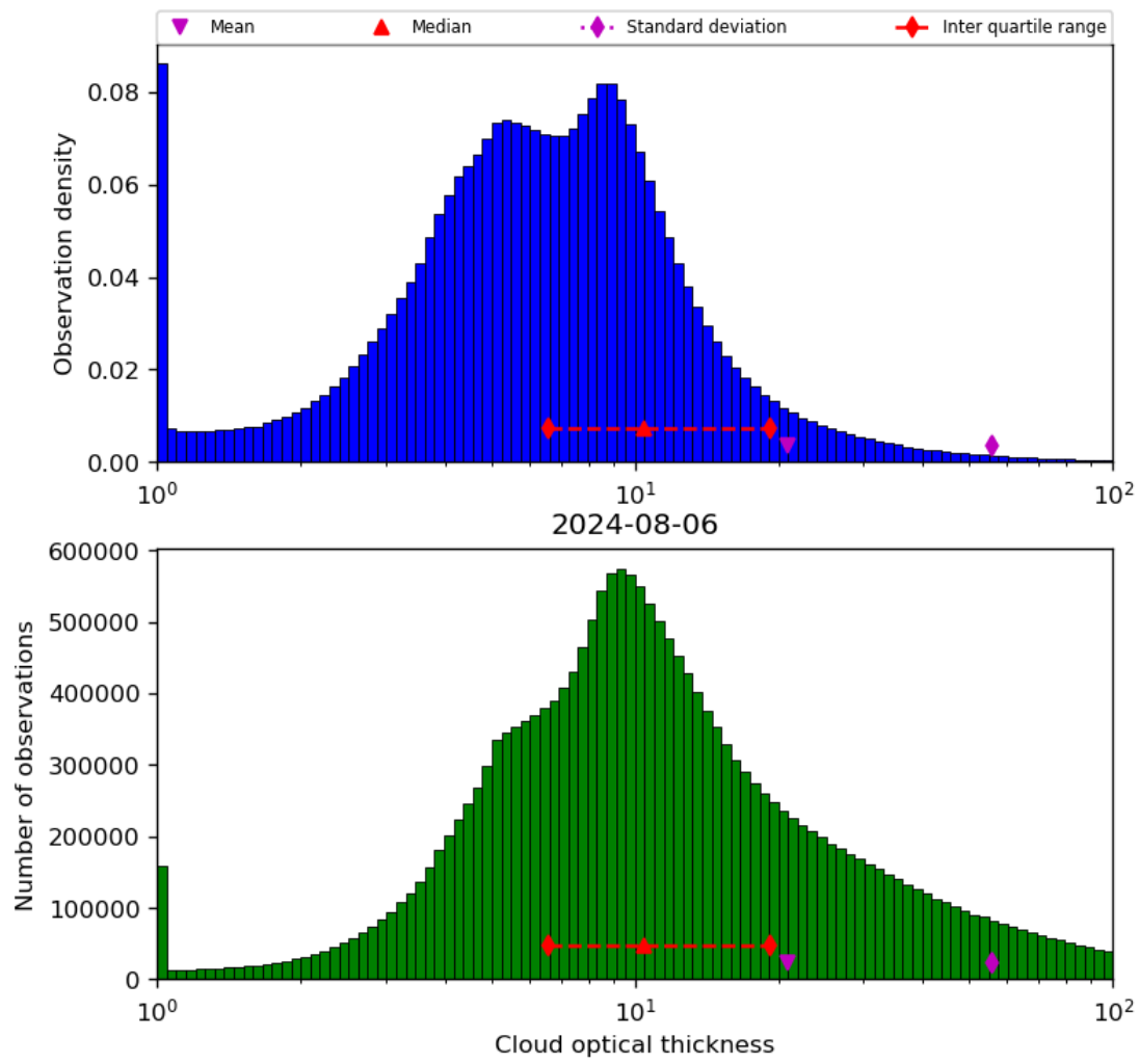
Figure 41: Histogram of “Cloud optical thickness” for 2024-08-06 to 2024-08-07
