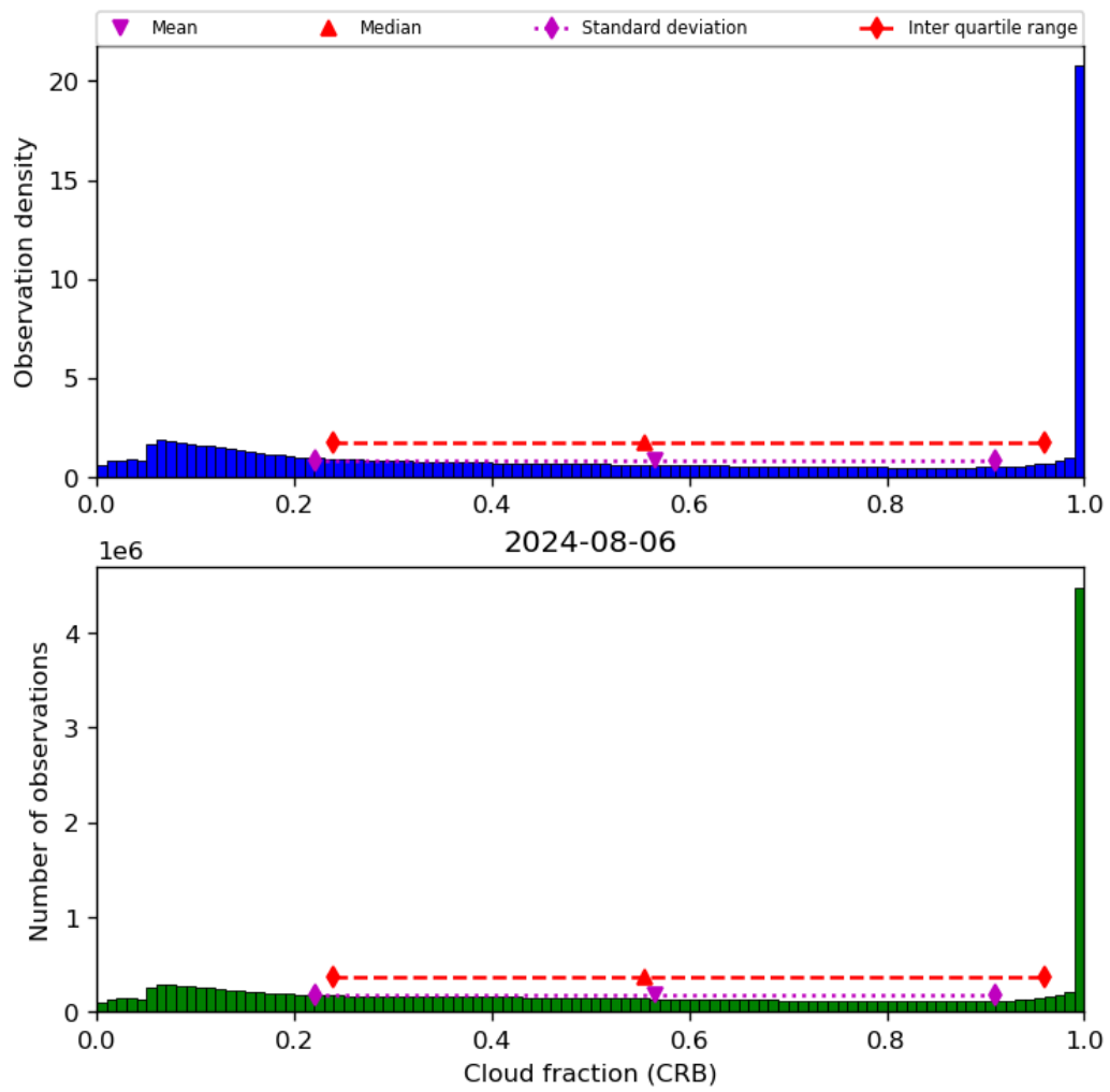
Figure 42: Histogram of “Cloud fraction (CRB)” for 2024-08-06 to 2024-08-07
