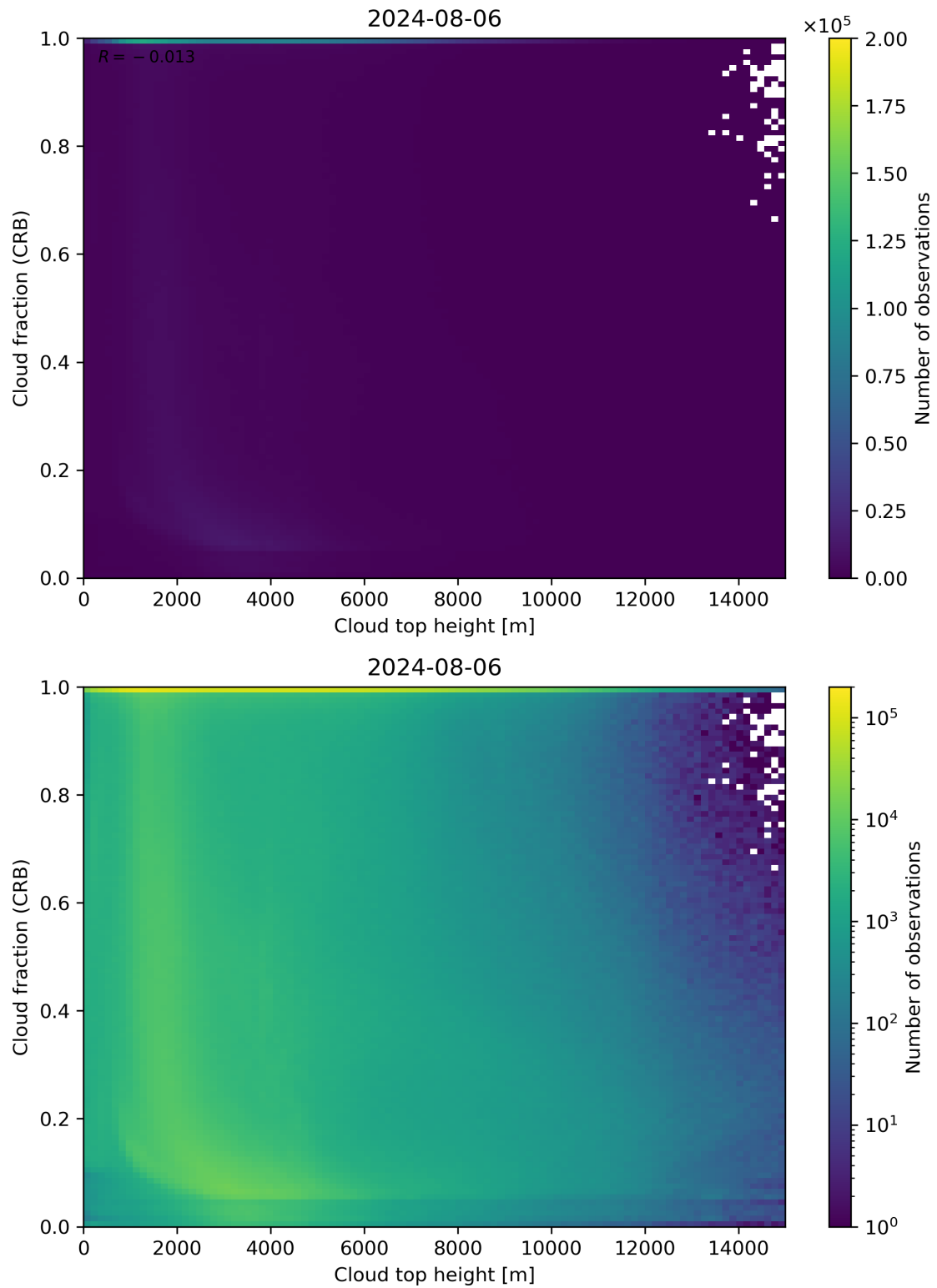
Figure 88: Scatter density plot of “Cloud top height” against “Cloud fraction (CRB)” for 2024-08-06 to 2024-08-07.
