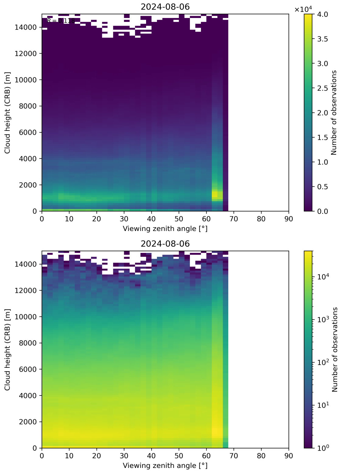
Figure 110: Scatter density plot of “Viewing zenith angle” against “Cloud height (CRB)” for 2024-08-06 to 2024-08-07.
