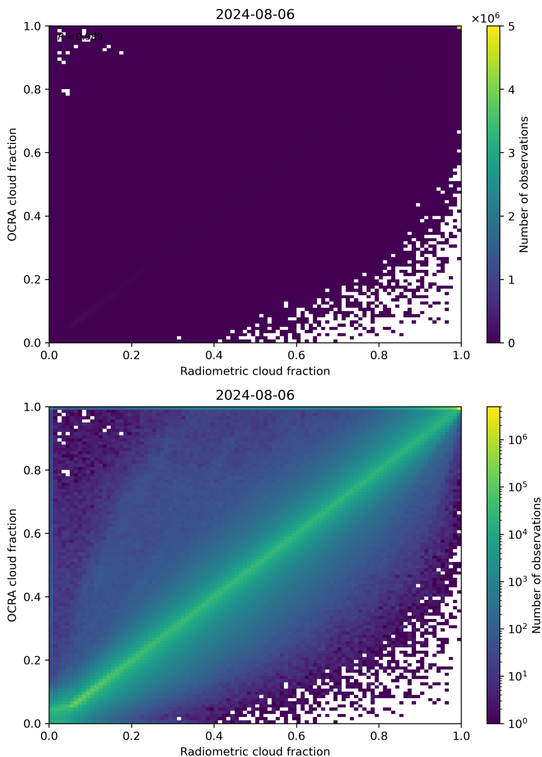
Figure 72: Scatter density plot of “Radiometric cloud fraction” against “OCRA cloud fraction” for 2024-08-06 to 2024-08-07.
