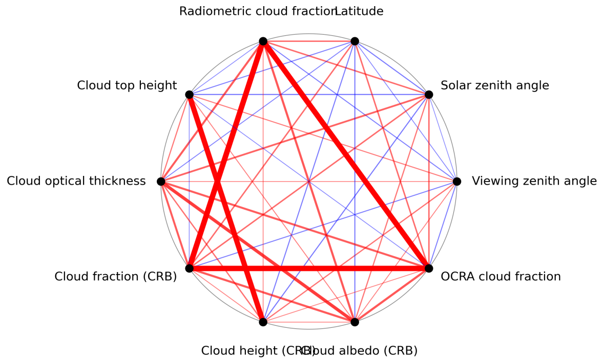
Figure 1: Map of correlation graph for 2024-08-06 to 2024-08-07.
