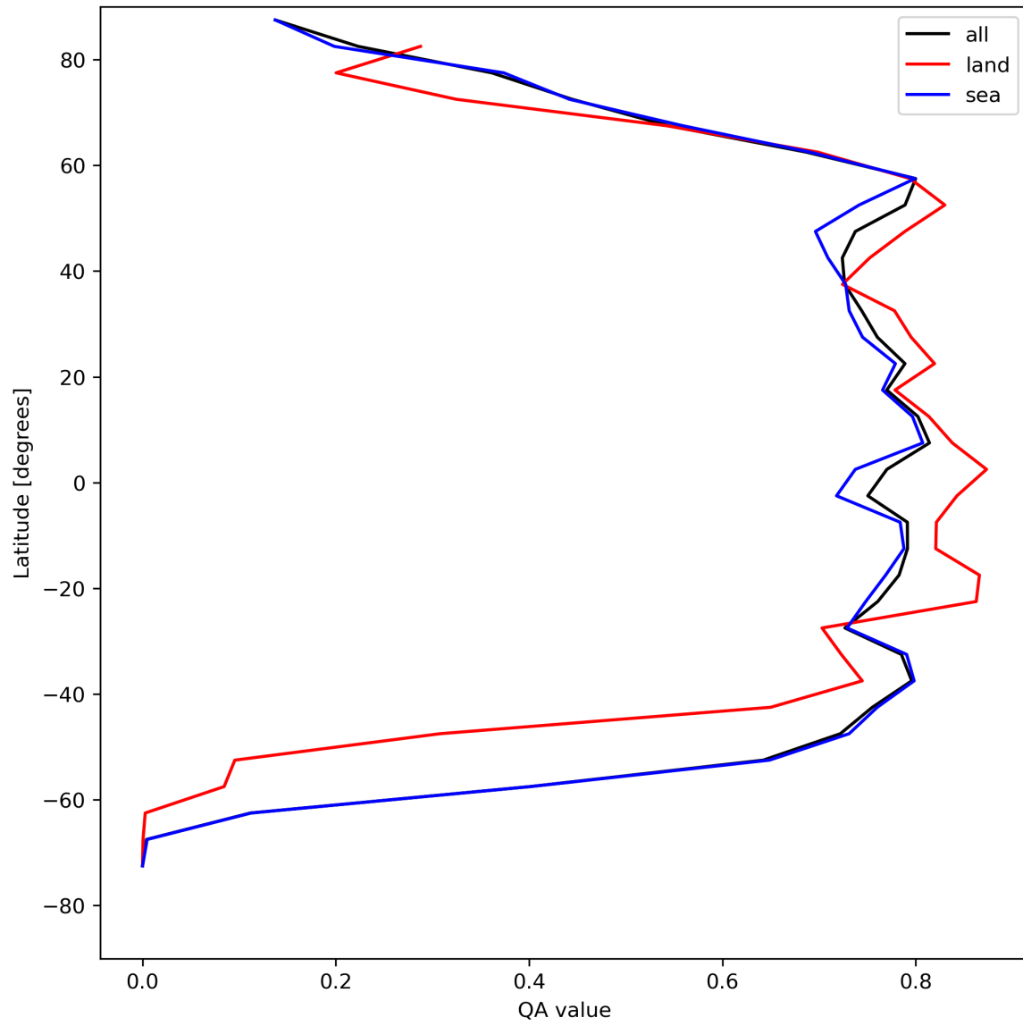
Figure 22: Zonal average of “QA value” for 2024-08-06 to 2024-08-07.
