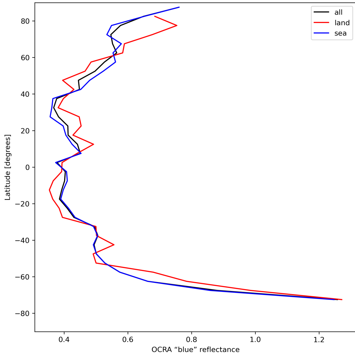
Figure 35: Zonal average of “OCRA “blue” reflectance” for 2024-08-06 to 2024-08-07.
