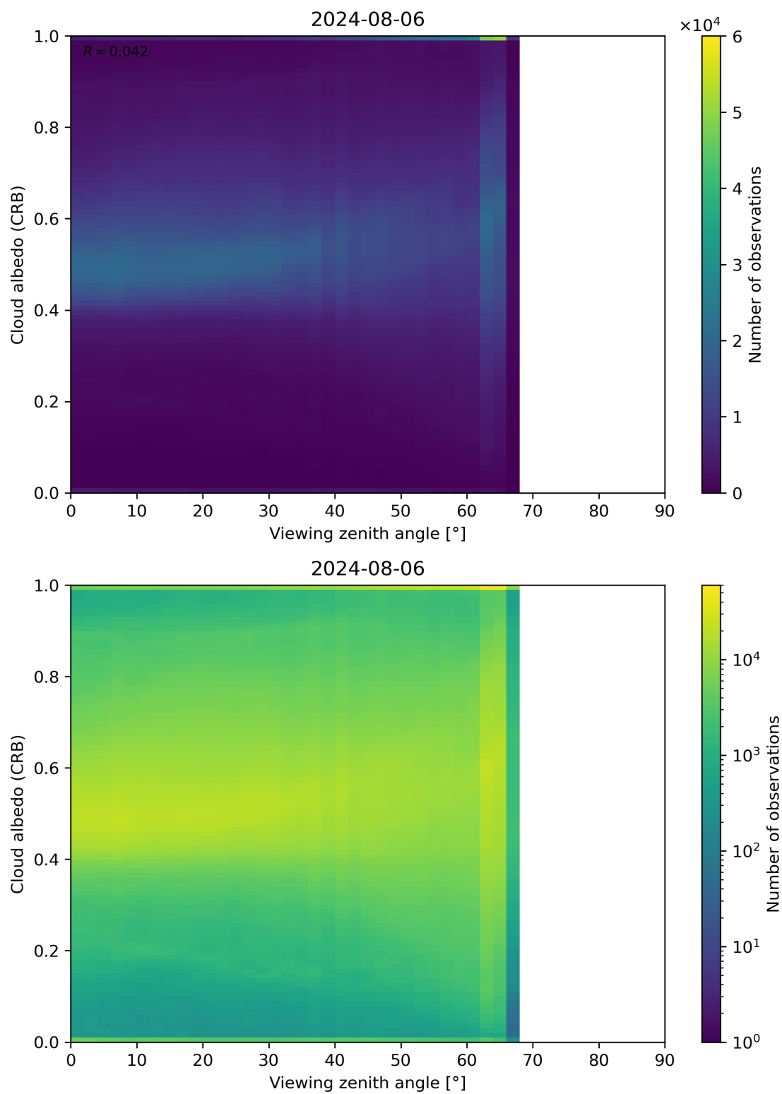
Figure 106: Scatter density plot of “Viewing zenith angle” against “Cloud albedo (CRB)” for 2024-08-06 to 2024-08-07.
