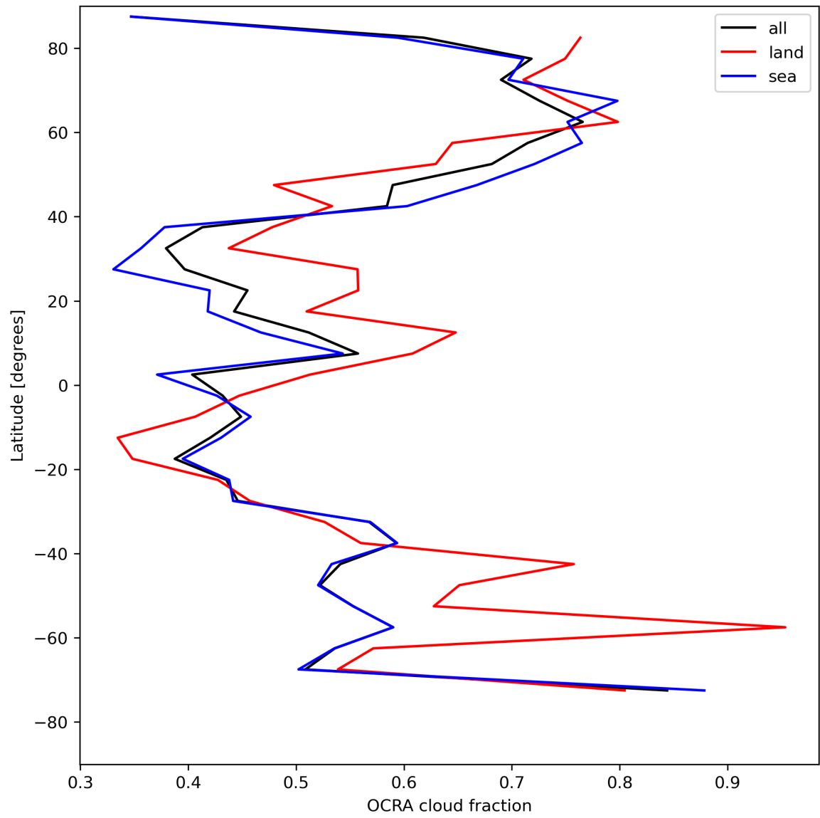
Figure 34: Zonal average of “OCRA cloud fraction” for 2024-08-06 to 2024-08-07.
