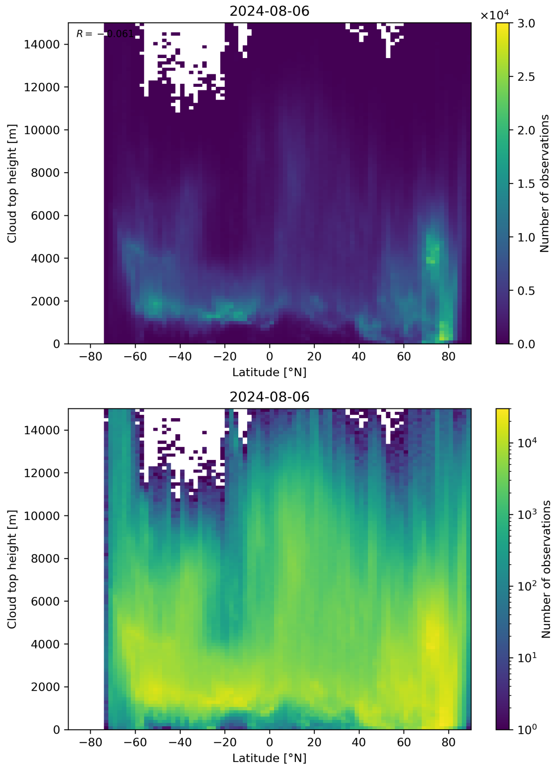
Figure 97: Scatter density plot of “Latitude” against “Cloud top height” for 2024-08-06 to 2024-08-07.
