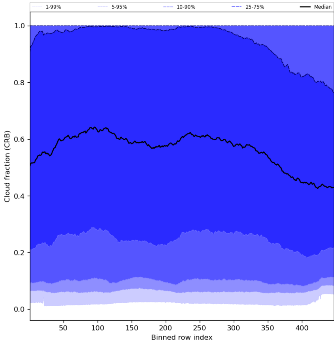
Figure 58: Along track statistics of “Cloud fraction (CRB)” for 2024-08-06 to 2024-08-07
