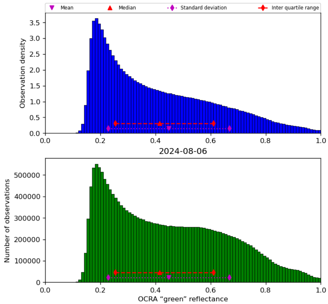
Figure 52: Histogram of “OCRA “green” reflectance” for 2024-08-06 to 2024-08-07
