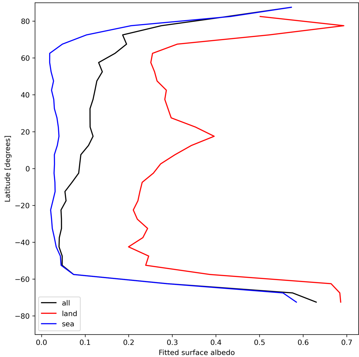
Figure 29: Zonal average of “Fitted surface albedo” for 2024-08-06 to 2024-08-07.
