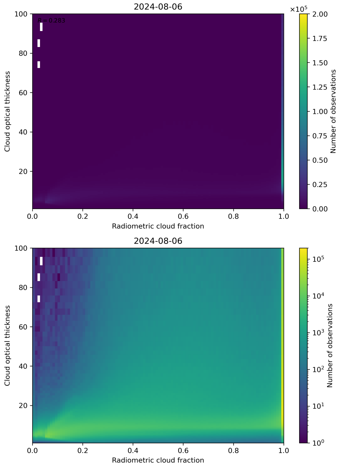
Figure 75: Scatter density plot of “Radiometric cloud fraction” against “Cloud optical thickness” for 2024-08-06 to 2024-08-07.
