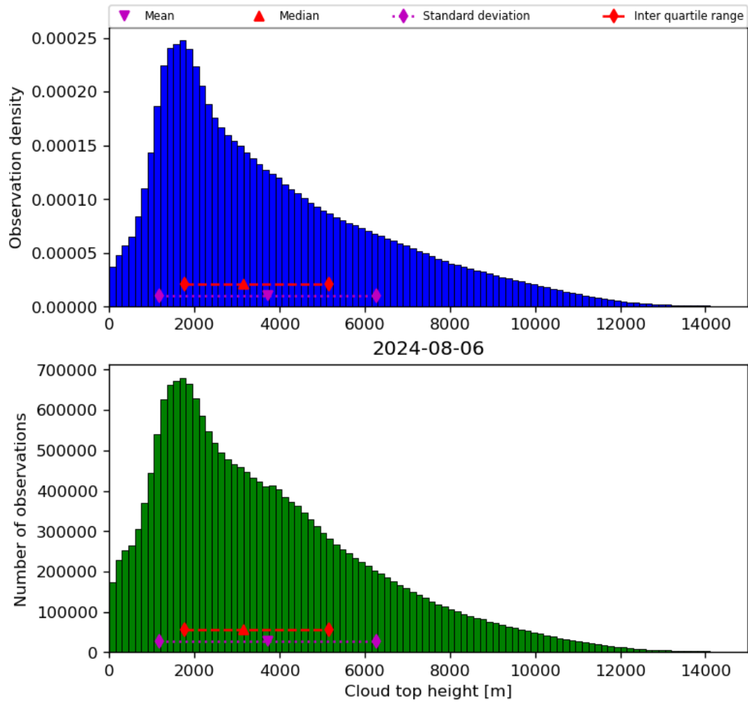
Figure 40: Histogram of “Cloud top height” for 2024-08-06 to 2024-08-07
