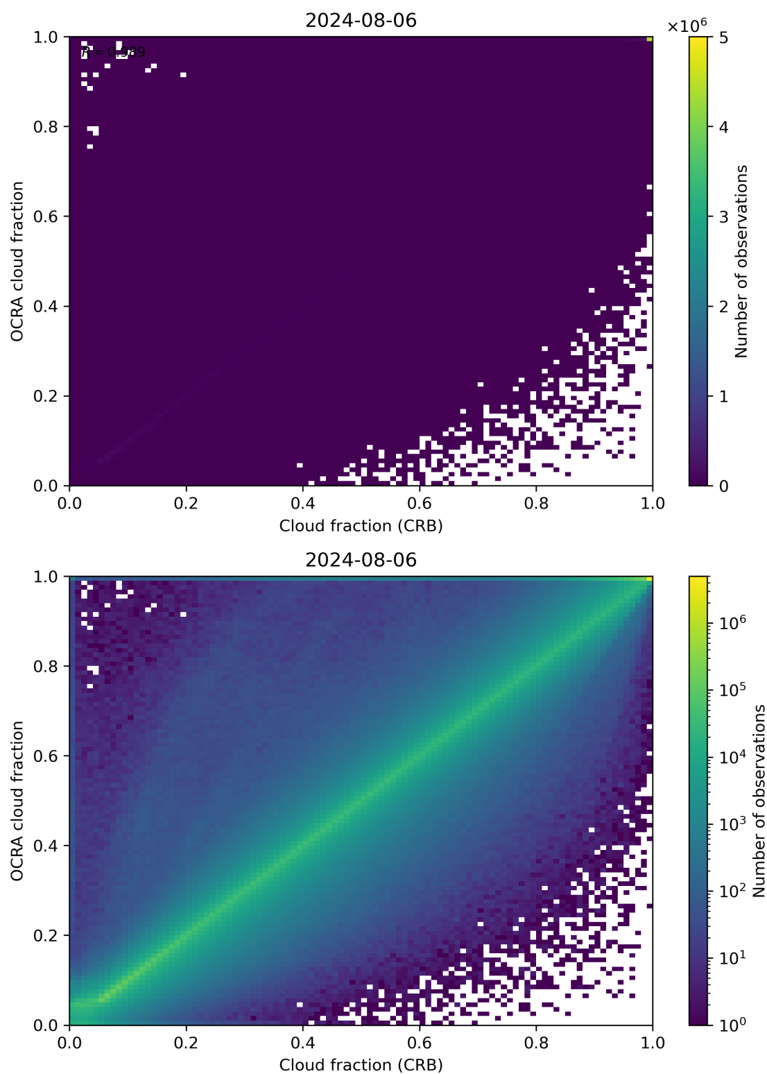
Figure 78: Scatter density plot of “Cloud fraction (CRB)” against “OCRA cloud fraction” for 2024-08-06 to 2024-08-07.
