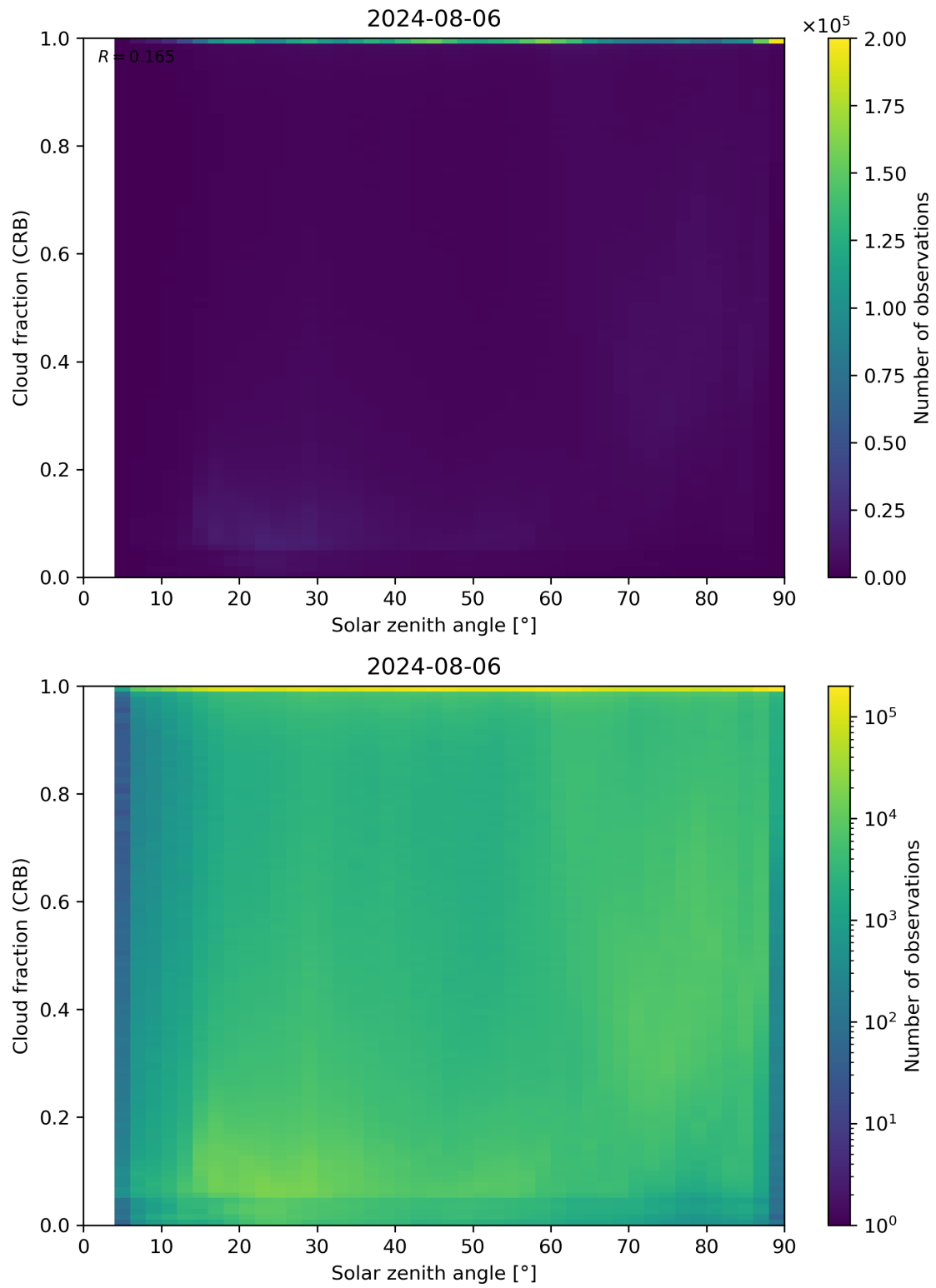
Figure 101: Scatter density plot of “Solar zenith angle” against “Cloud fraction (CRB)” for 2024-08-06 to 2024-08-07.
