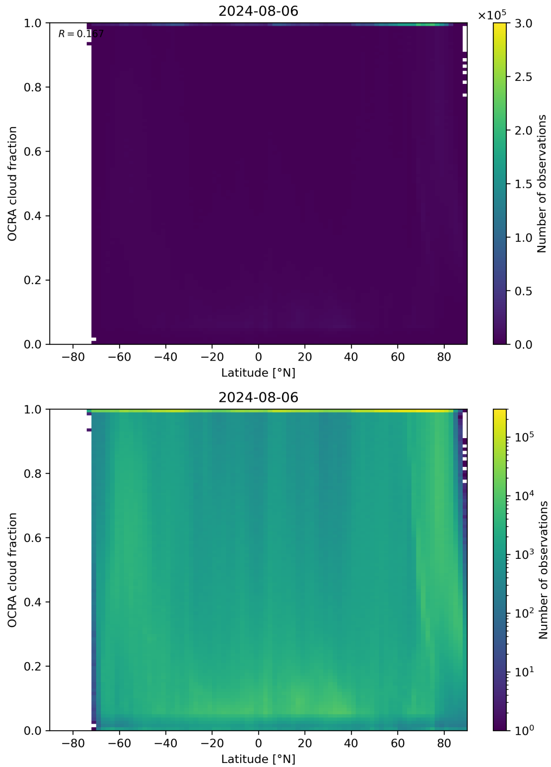
Figure 93: Scatter density plot of “Latitude” against “OCRA cloud fraction” for 2024-08-06 to 2024-08-07.
