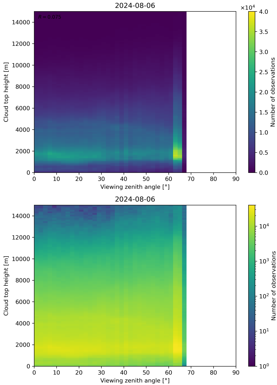
Figure 112: Scatter density plot of “Viewing zenith angle” against “Cloud top height” for 2024-08-06 to 2024-08-07.
