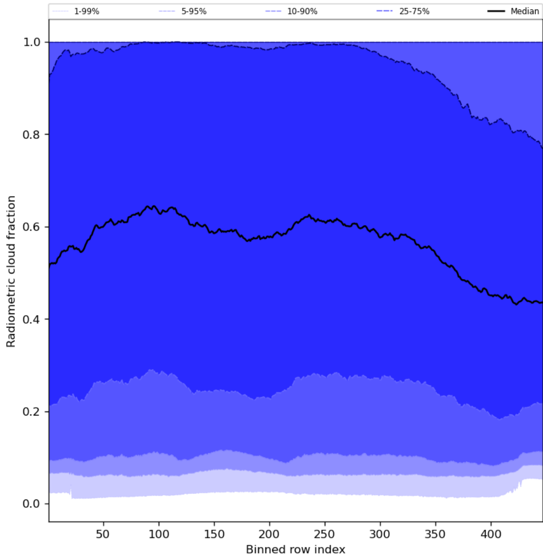
Figure 55: Along track statistics of “Radiometric cloud fraction” for 2024-08-06 to 2024-08-07
