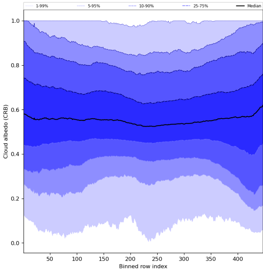
Figure 60: Along track statistics of “Cloud albedo (CRB)” for 2024-08-06 to 2024-08-07
