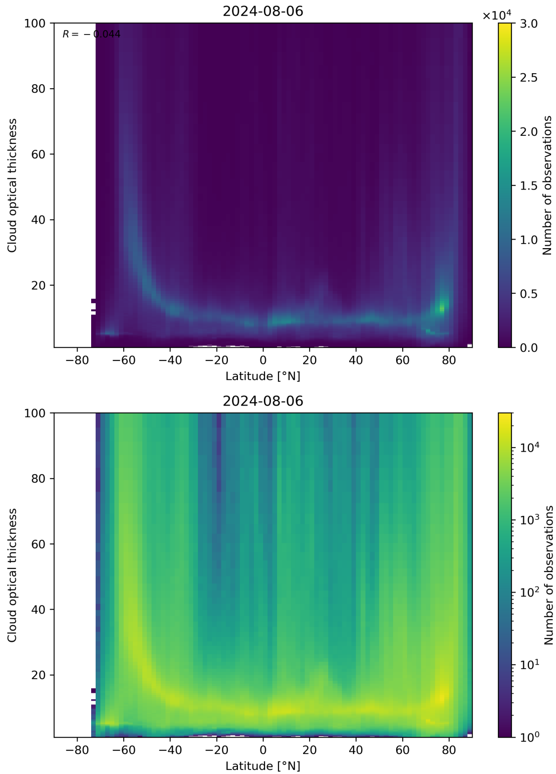
Figure 96: Scatter density plot of “Latitude” against “Cloud optical thickness” for 2024-08-06 to 2024-08-07.
