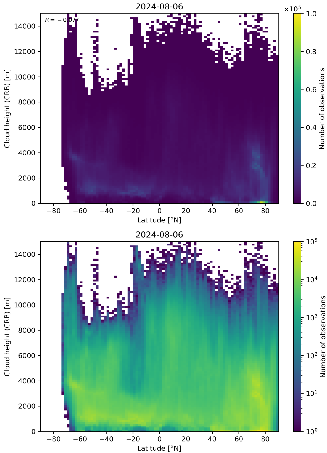
Figure 95: Scatter density plot of “Latitude” against “Cloud height (CRB)” for 2024-08-06 to 2024-08-07.
