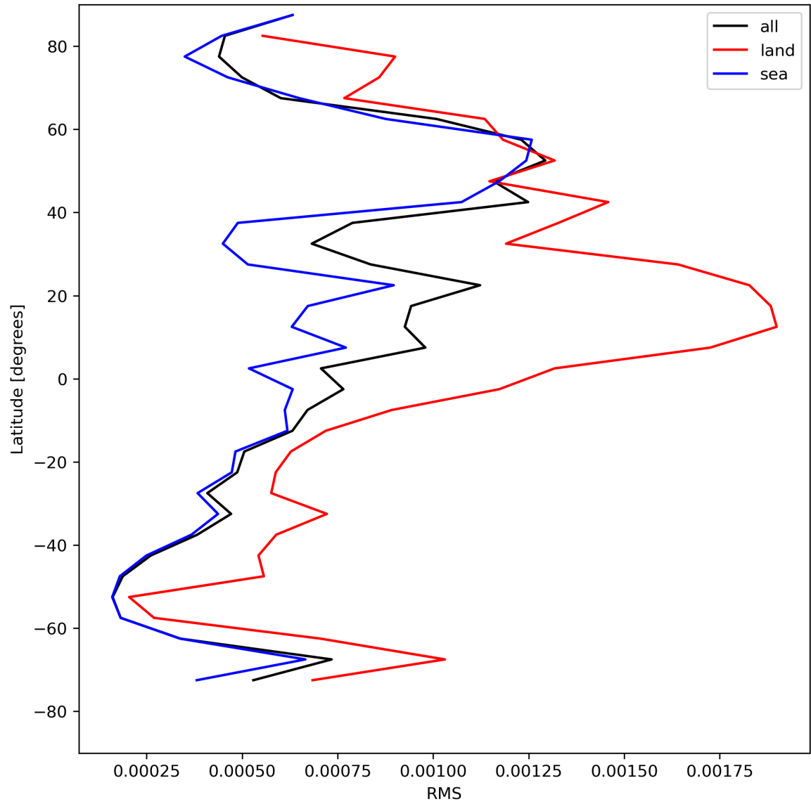
Figure 31: Zonal average of “RMS” for 2024-08-06 to 2024-08-07.
