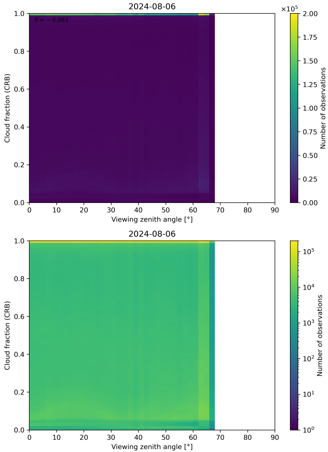
Figure 109: Scatter density plot of “Viewing zenith angle” against “Cloud fraction (CRB)” for 2024-08-06 to 2024-08-07.
