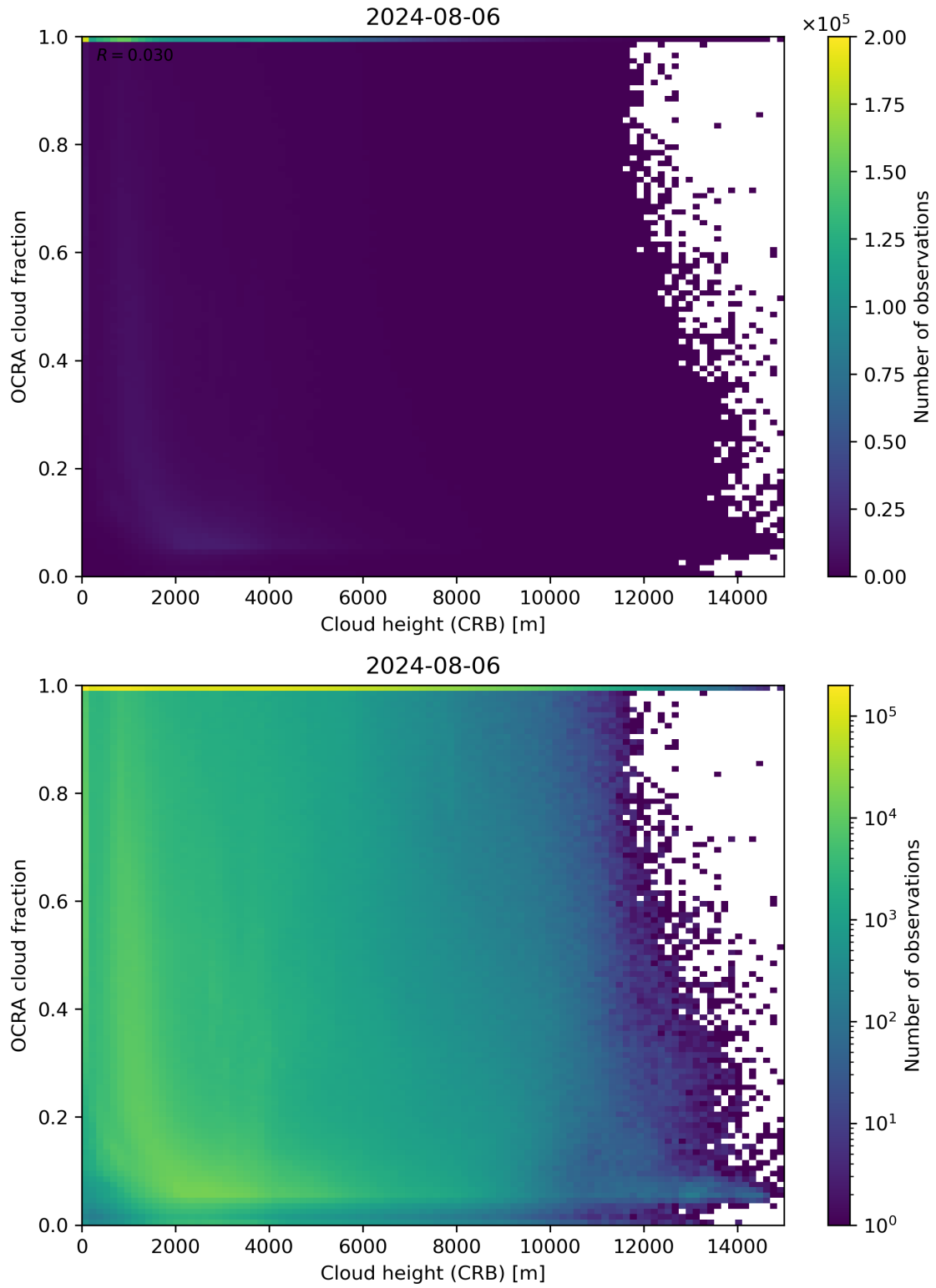
Figure 81: Scatter density plot of “Cloud height (CRB)” against “OCRA cloud fraction” for 2024-08-06 to 2024-08-07.
