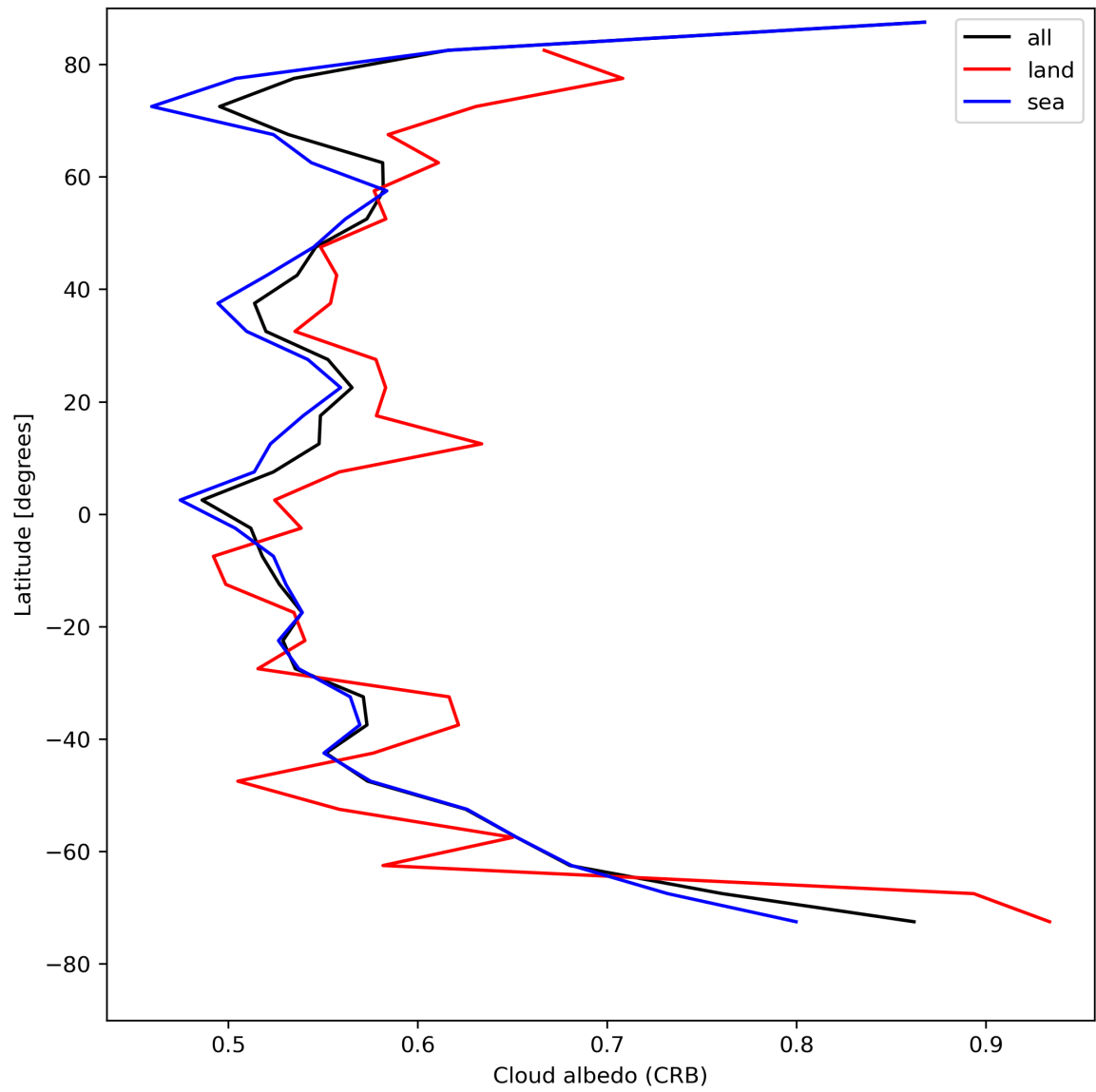
Figure 28: Zonal average of “Cloud albedo (CRB)” for 2024-08-06 to 2024-08-07.
