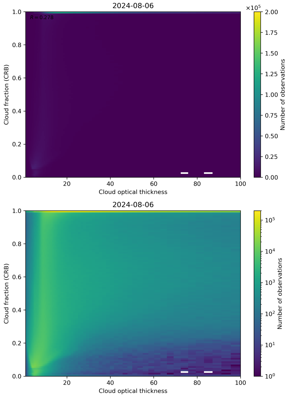
Figure 84: Scatter density plot of “Cloud optical thickness” against “Cloud fraction (CRB)” for 2024-08-06 to 2024-08-07.
