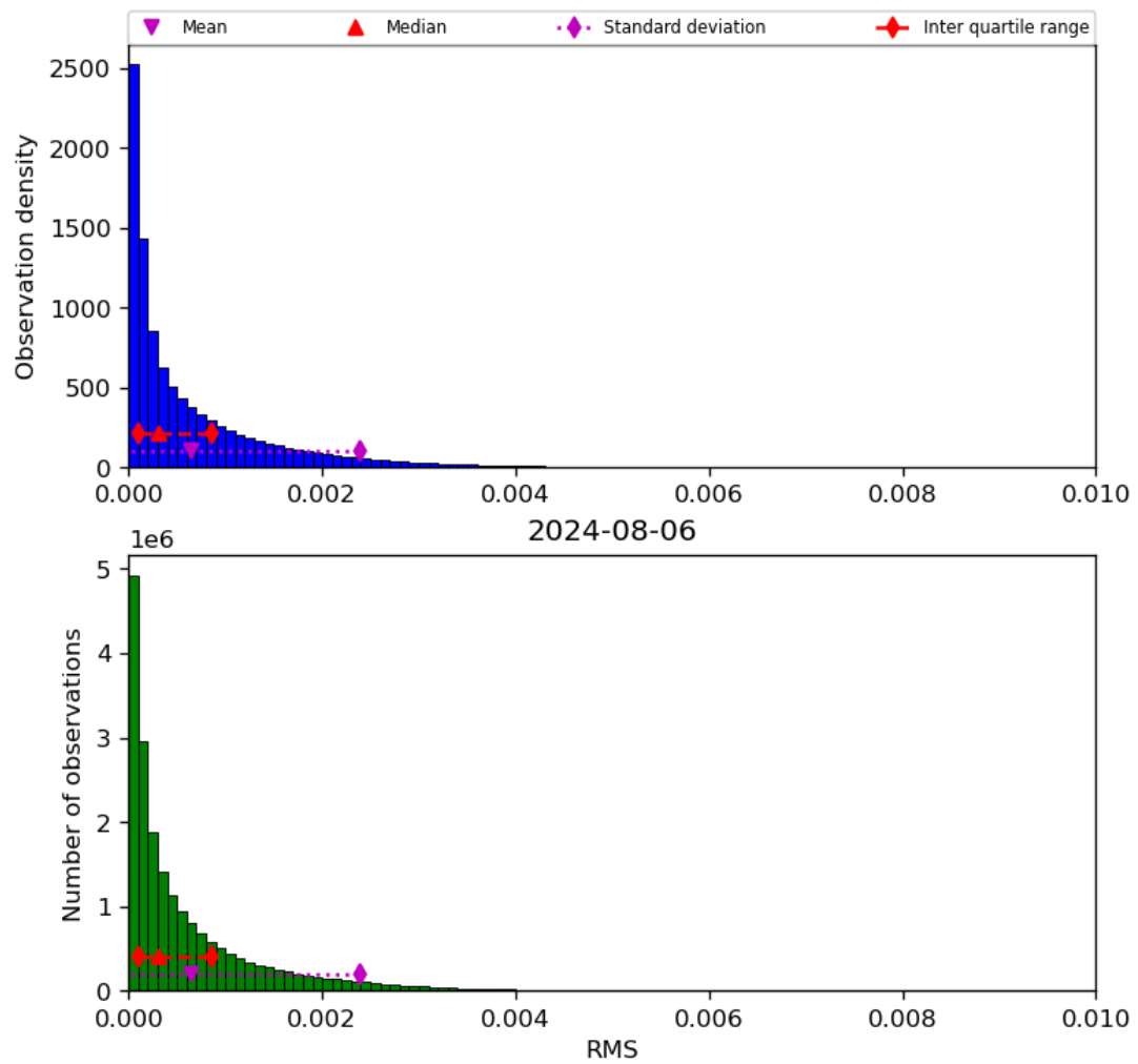
Figure 47: Histogram of “RMS” for 2024-08-06 to 2024-08-07
