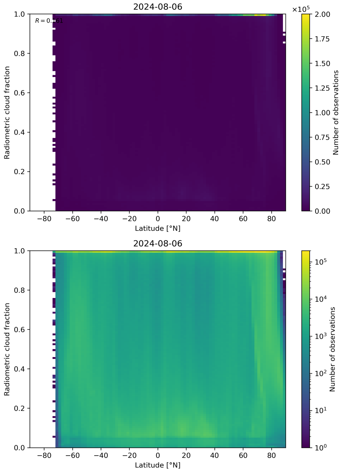
Figure 92: Scatter density plot of “Latitude” against “Radiometric cloud fraction” for 2024-08-06 to 2024-08-07.
