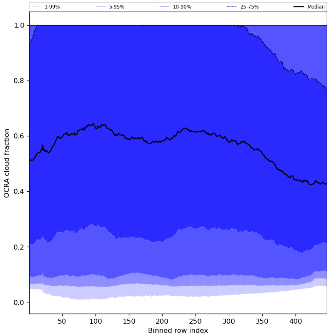
Figure 66: Along track statistics of “OCRA cloud fraction” for 2024-08-06 to 2024-08-07
