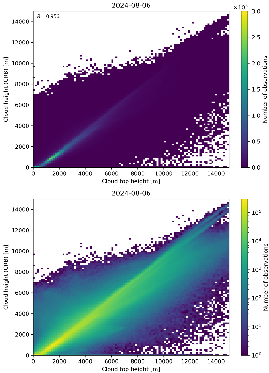
Figure 89: Scatter density plot of “Cloud top height” against “Cloud height (CRB)” for 2024-08-06 to 2024-08-07.
