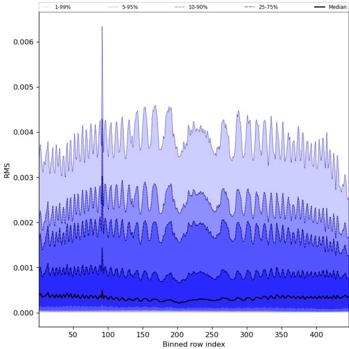
Figure 63: Along track statistics of “RMS” for 2024-08-06 to 2024-08-07
