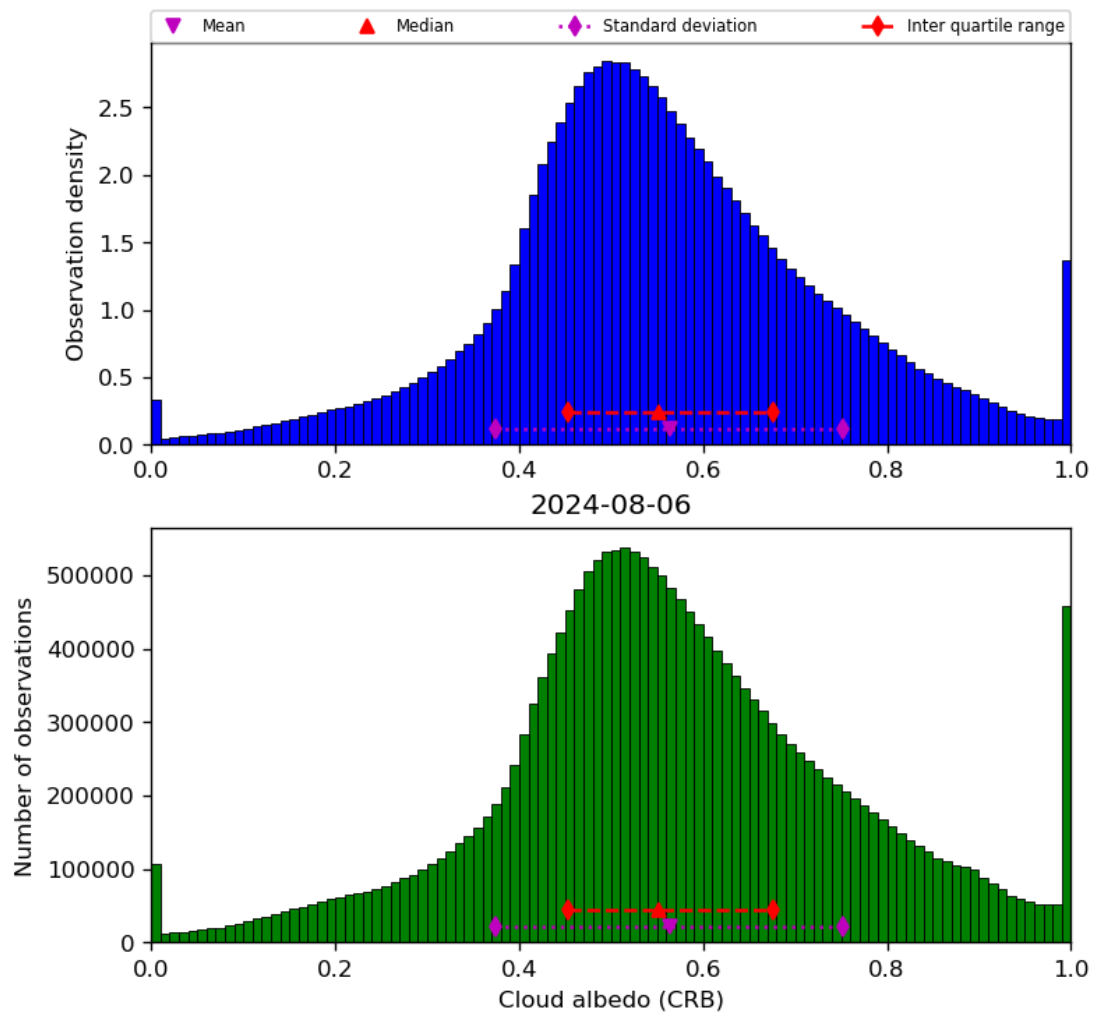
Figure 44: Histogram of “Cloud albedo (CRB)” for 2024-08-06 to 2024-08-07
