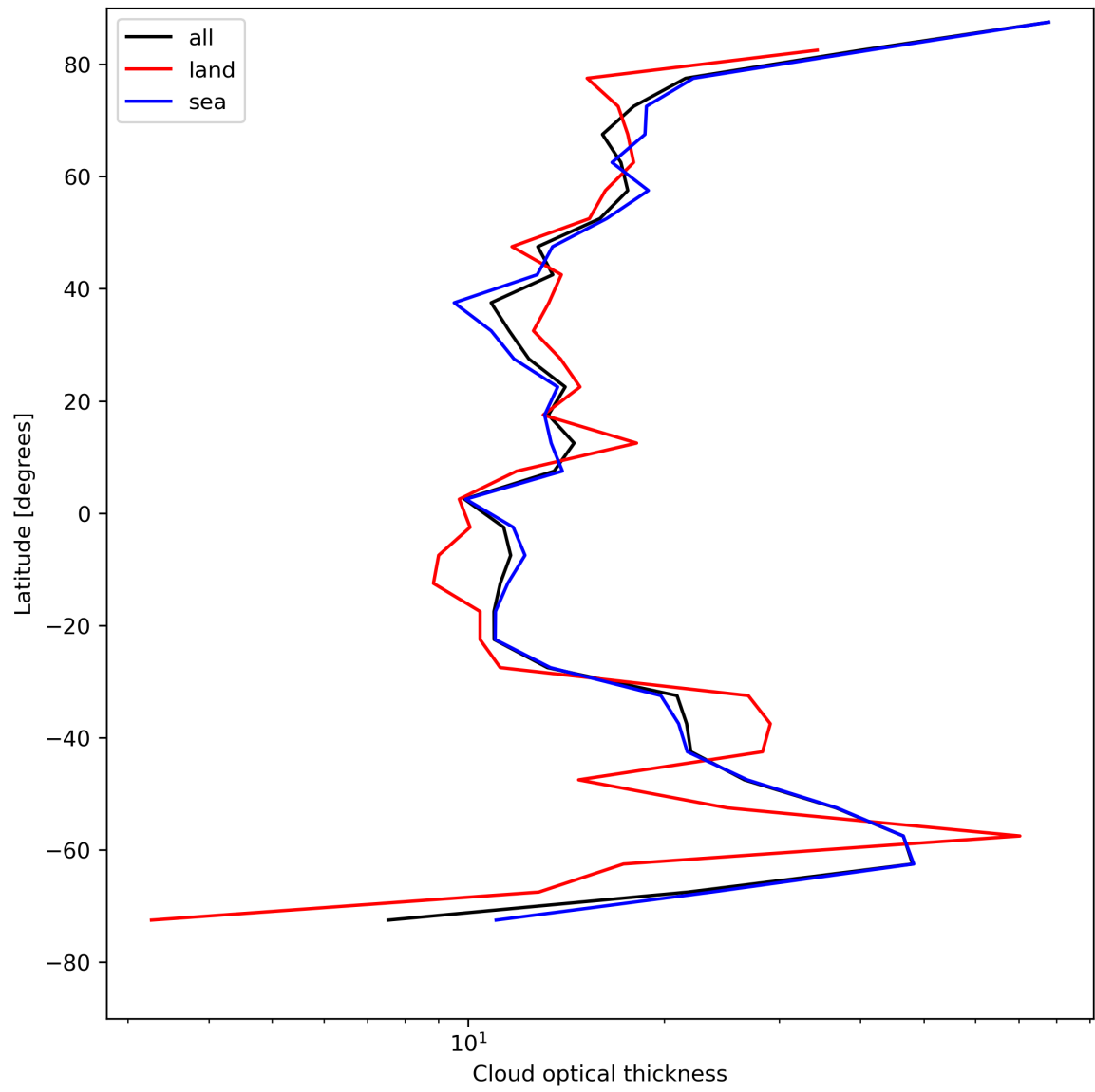
Figure 25: Zonal average of “Cloud optical thickness” for 2024-08-06 to 2024-08-07.
