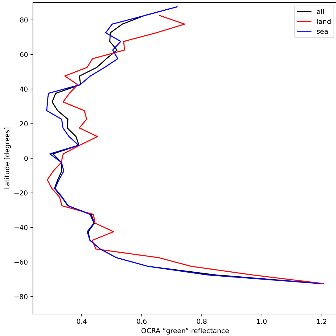
Figure 36: Zonal average of “OCRA “green” reflectance” for 2024-08-06 to 2024-08-07.
