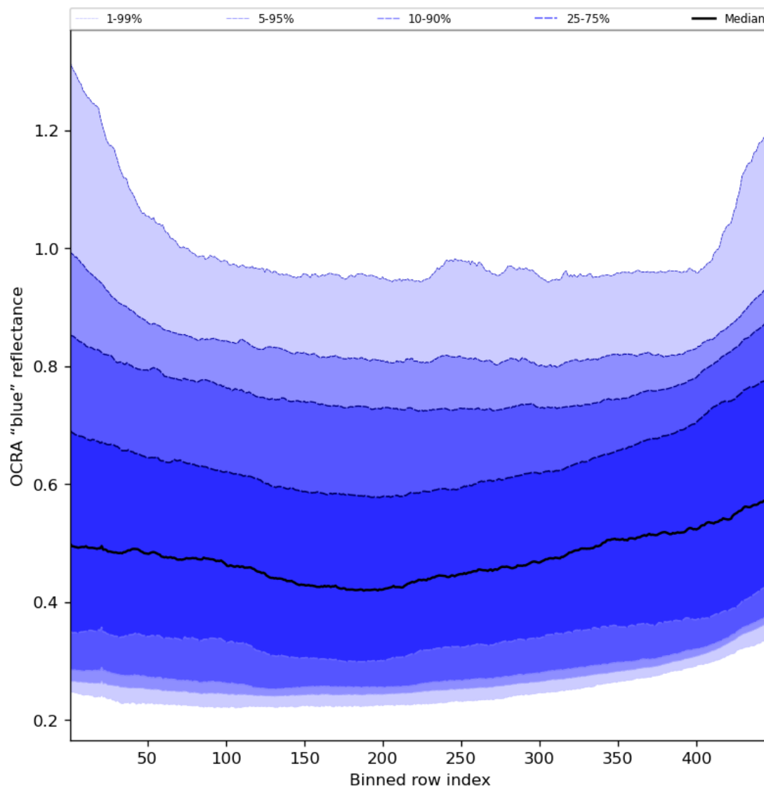
Figure 67: Along track statistics of “OCRA “blue” reflectance” for 2024-08-06 to 2024-08-07
