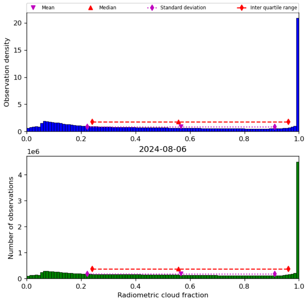
Figure 39: Histogram of “Radiometric cloud fraction” for 2024-08-06 to 2024-08-07
