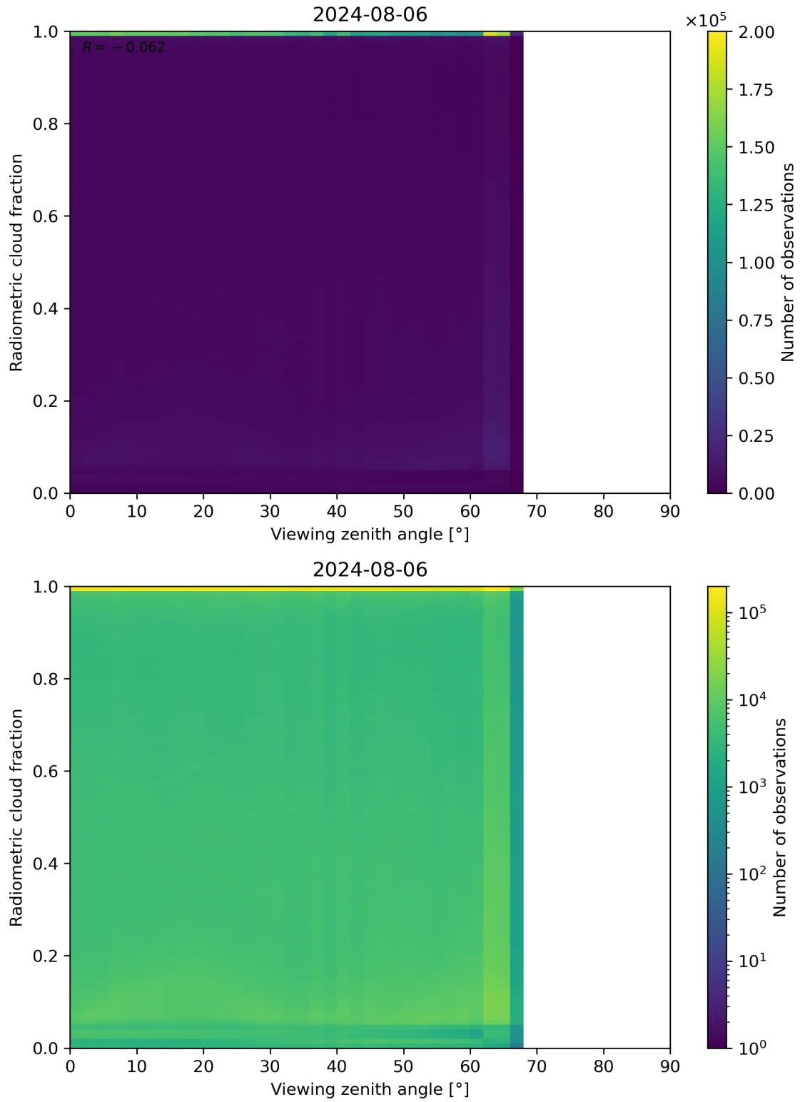
Figure 107: Scatter density plot of “Viewing zenith angle” against “Radiometric cloud fraction” for 2024-08-06 to 2024-08-07.
