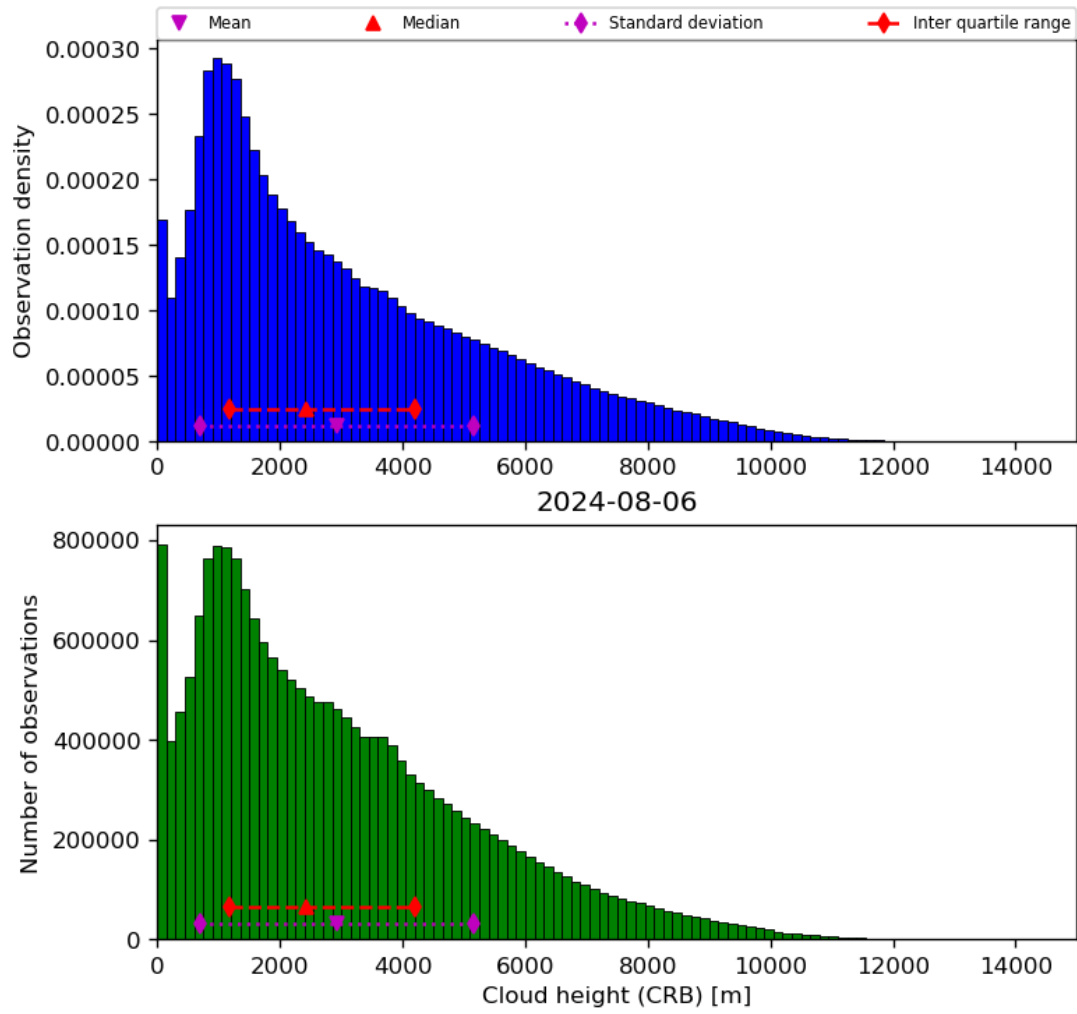
Figure 43: Histogram of “Cloud height (CRB)” for 2024-08-06 to 2024-08-07
