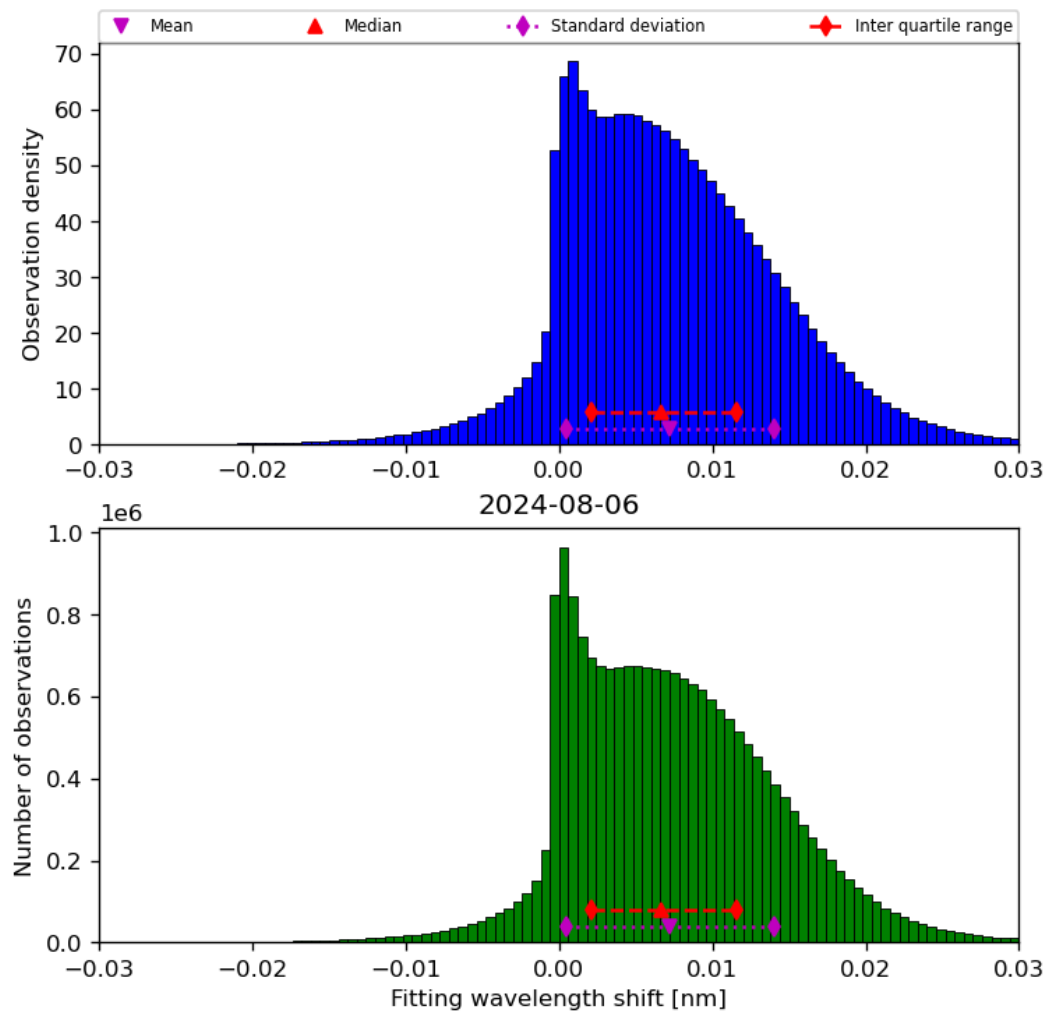
Figure 49: Histogram of “Fitting wavelength shift” for 2024-08-06 to 2024-08-07
