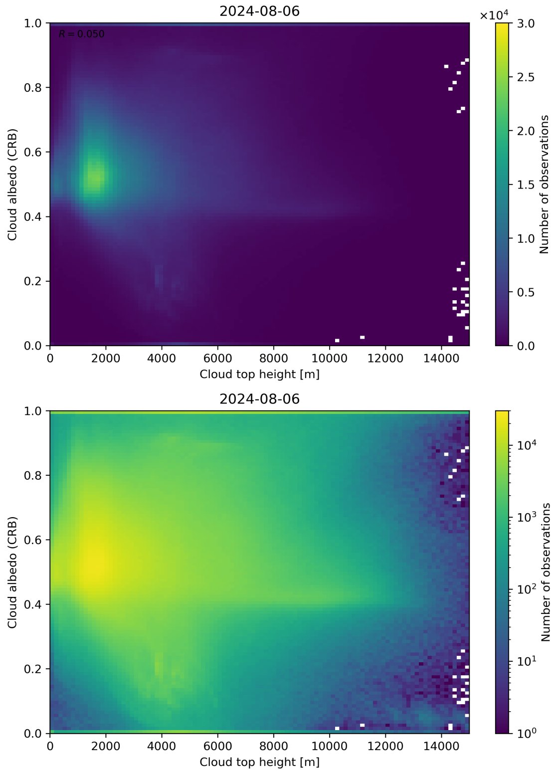
Figure 86: Scatter density plot of “Cloud top height” against “Cloud albedo (CRB)” for 2024-08-06 to 2024-08-07.
