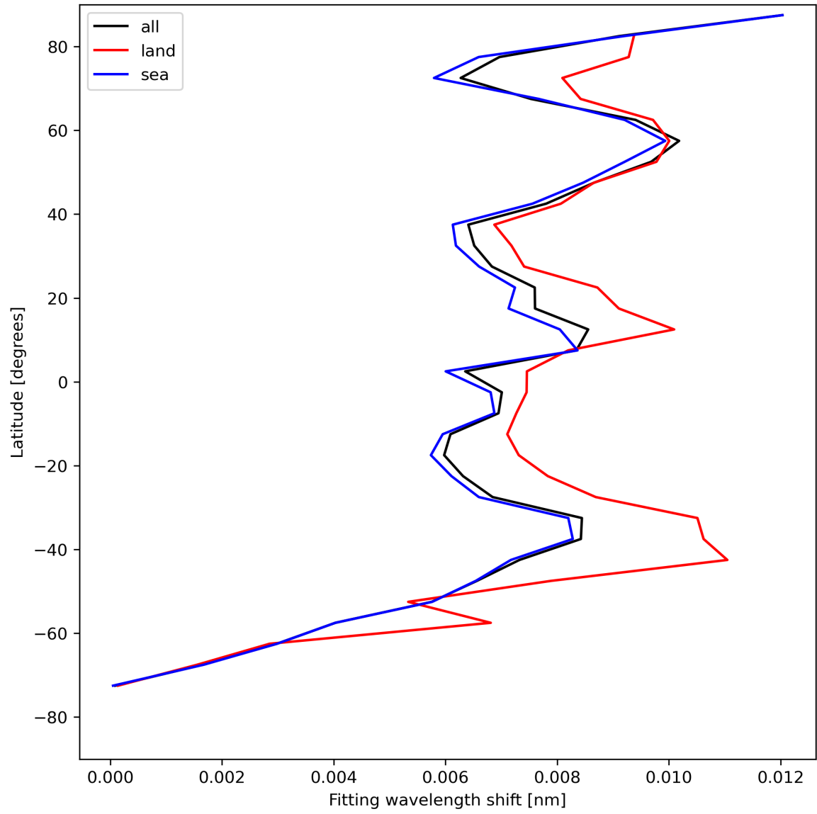
Figure 33: Zonal average of “Fitting wavelength shift” for 2024-08-06 to 2024-08-07.
