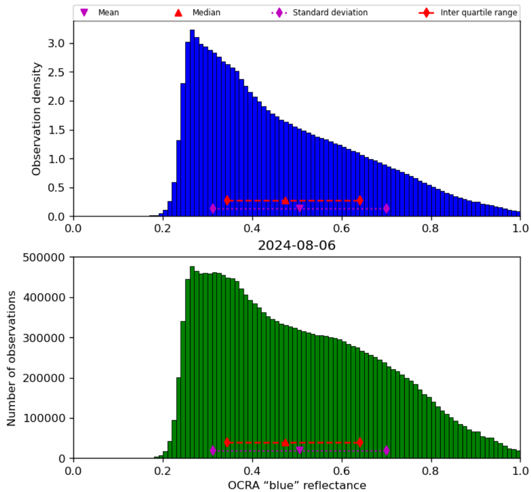
Figure 51: Histogram of “OCRA “blue” reflectance” for 2024-08-06 to 2024-08-07
