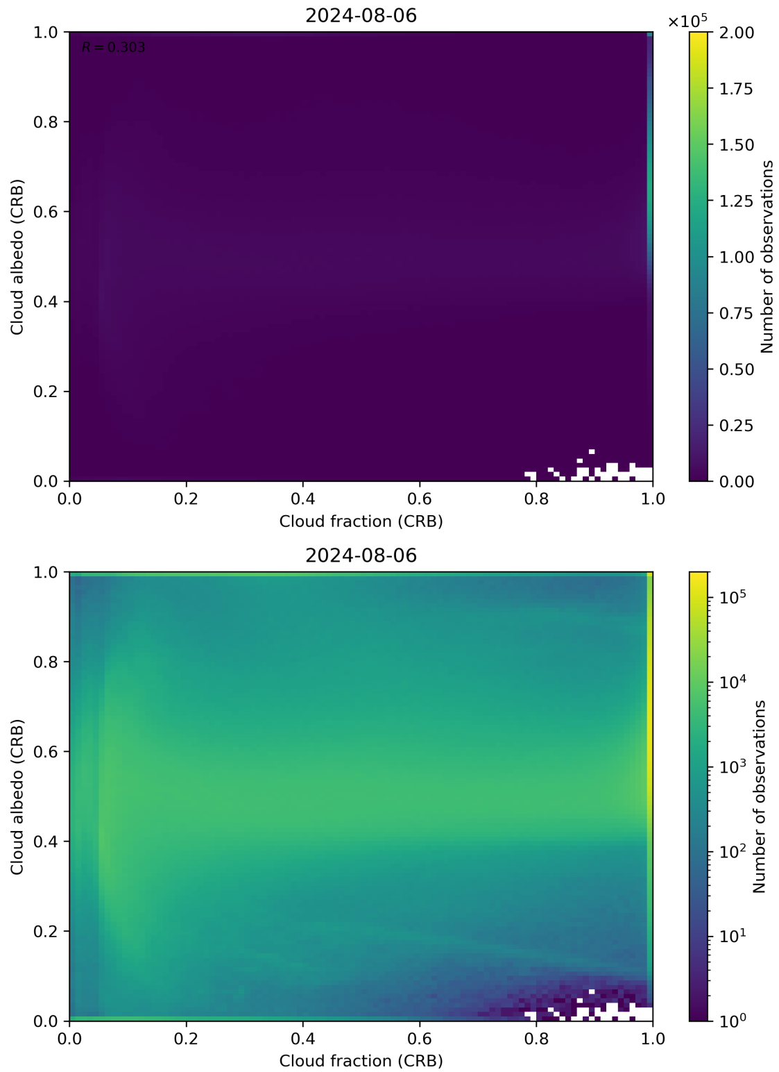
Figure 77: Scatter density plot of “Cloud fraction (CRB)” against “Cloud albedo (CRB)” for 2024-08-06 to 2024-08-07.
