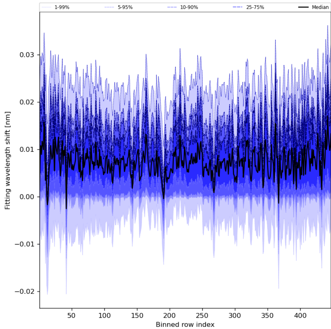
Figure 65: Along track statistics of “Fitting wavelength shift” for 2024-08-06 to 2024-08-07
