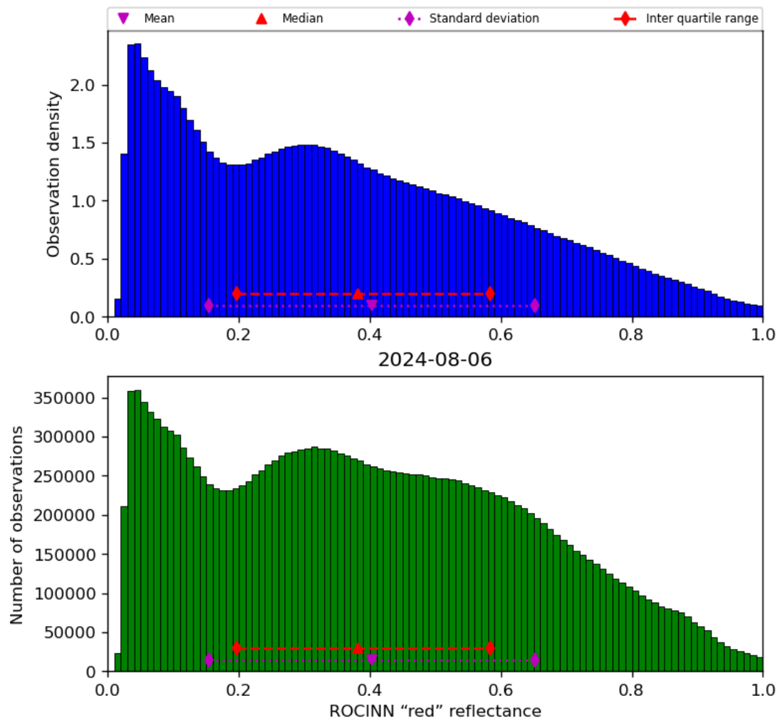
Figure 53: Histogram of “ROCINN “red” reflectance” for 2024-08-06 to 2024-08-07
