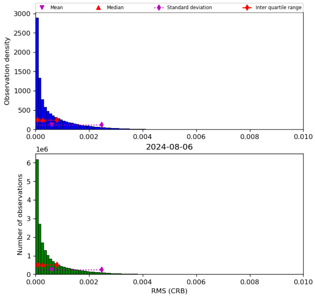
Figure 48: Histogram of “RMS (CRB)” for 2024-08-06 to 2024-08-07
