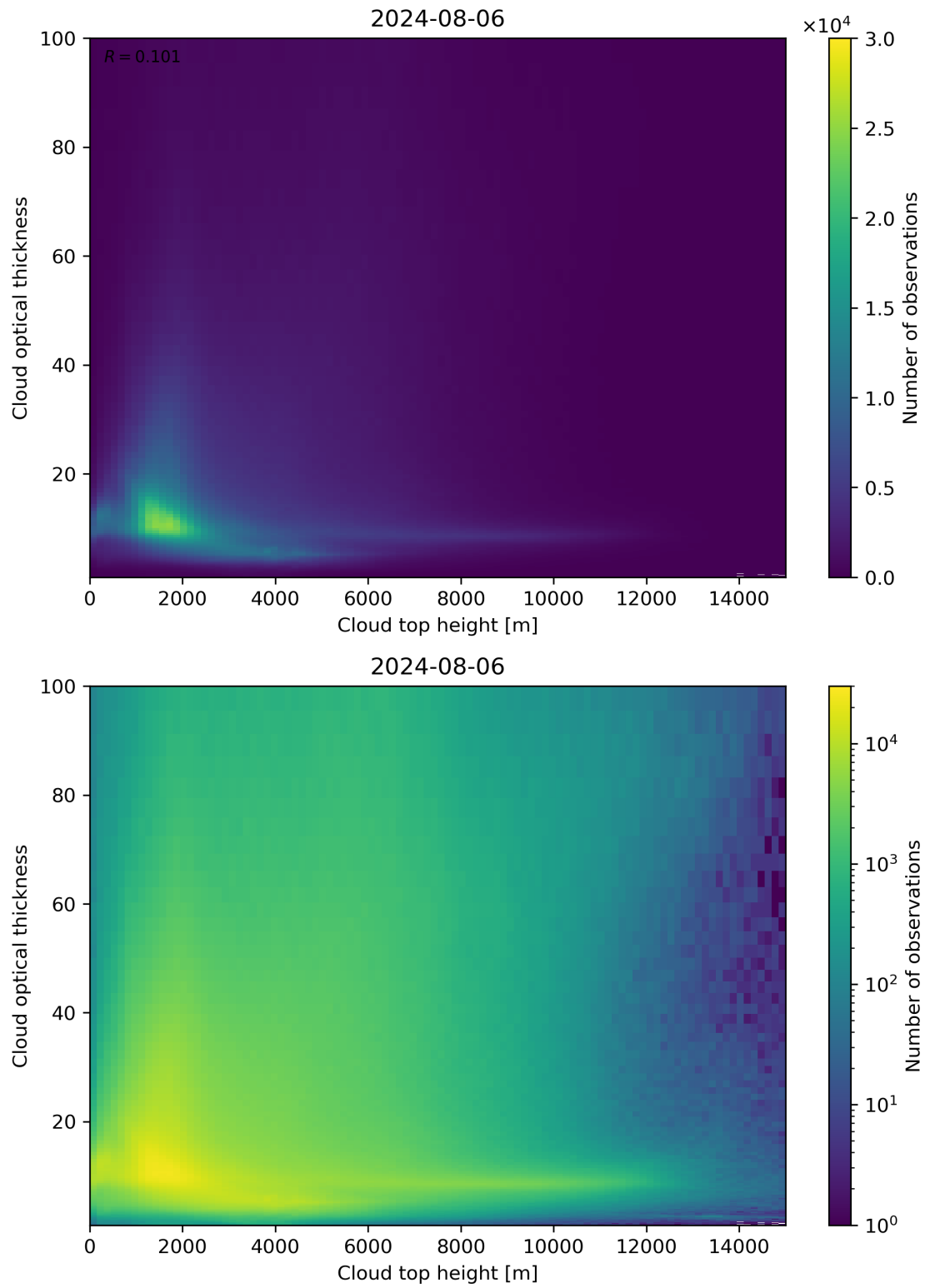
Figure 90: Scatter density plot of “Cloud top height” against “Cloud optical thickness” for 2024-08-06 to 2024-08-07.
