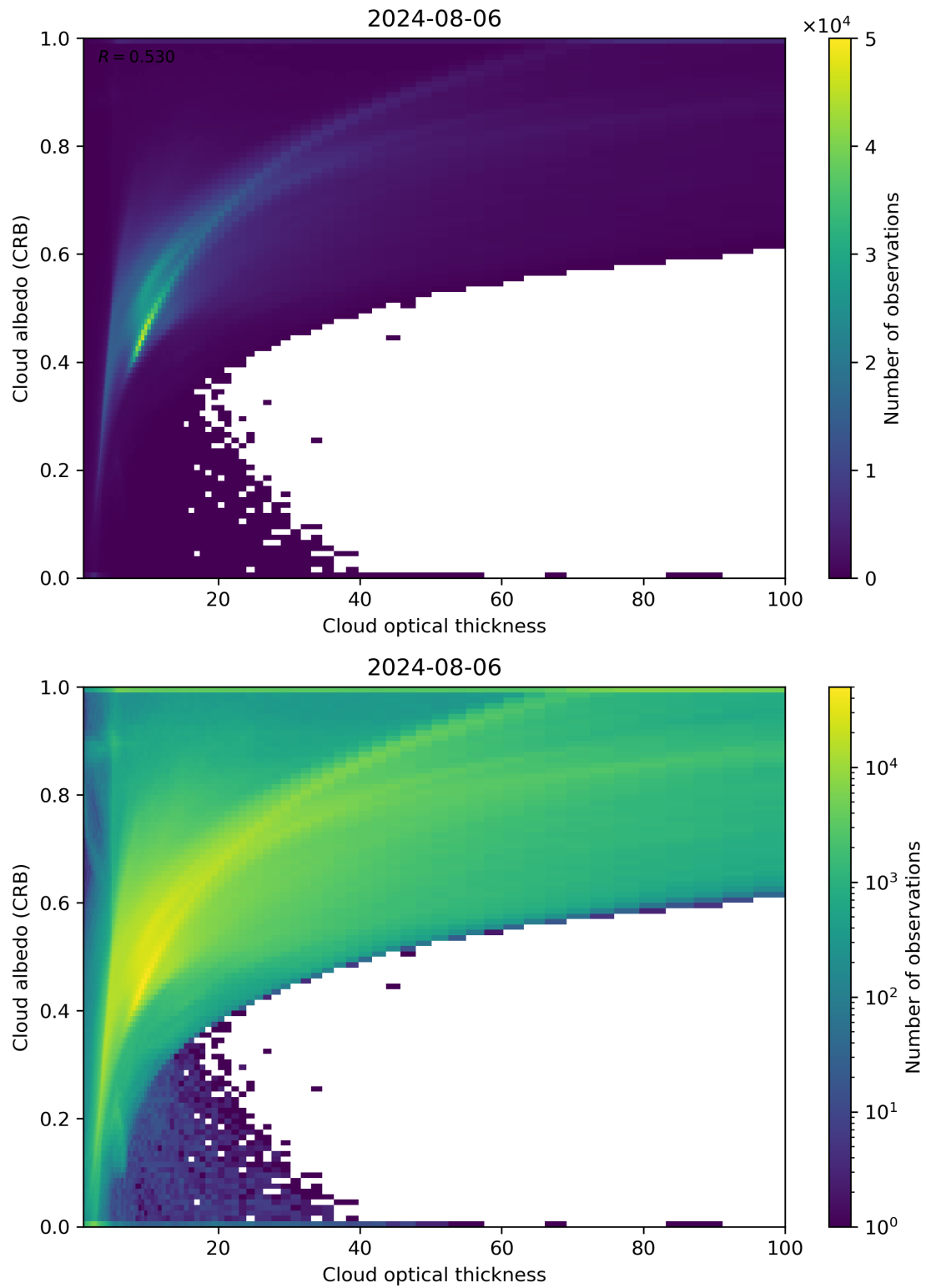
Figure 82: Scatter density plot of “Cloud optical thickness” against “Cloud albedo (CRB)” for 2024-08-06 to 2024-08-07.
