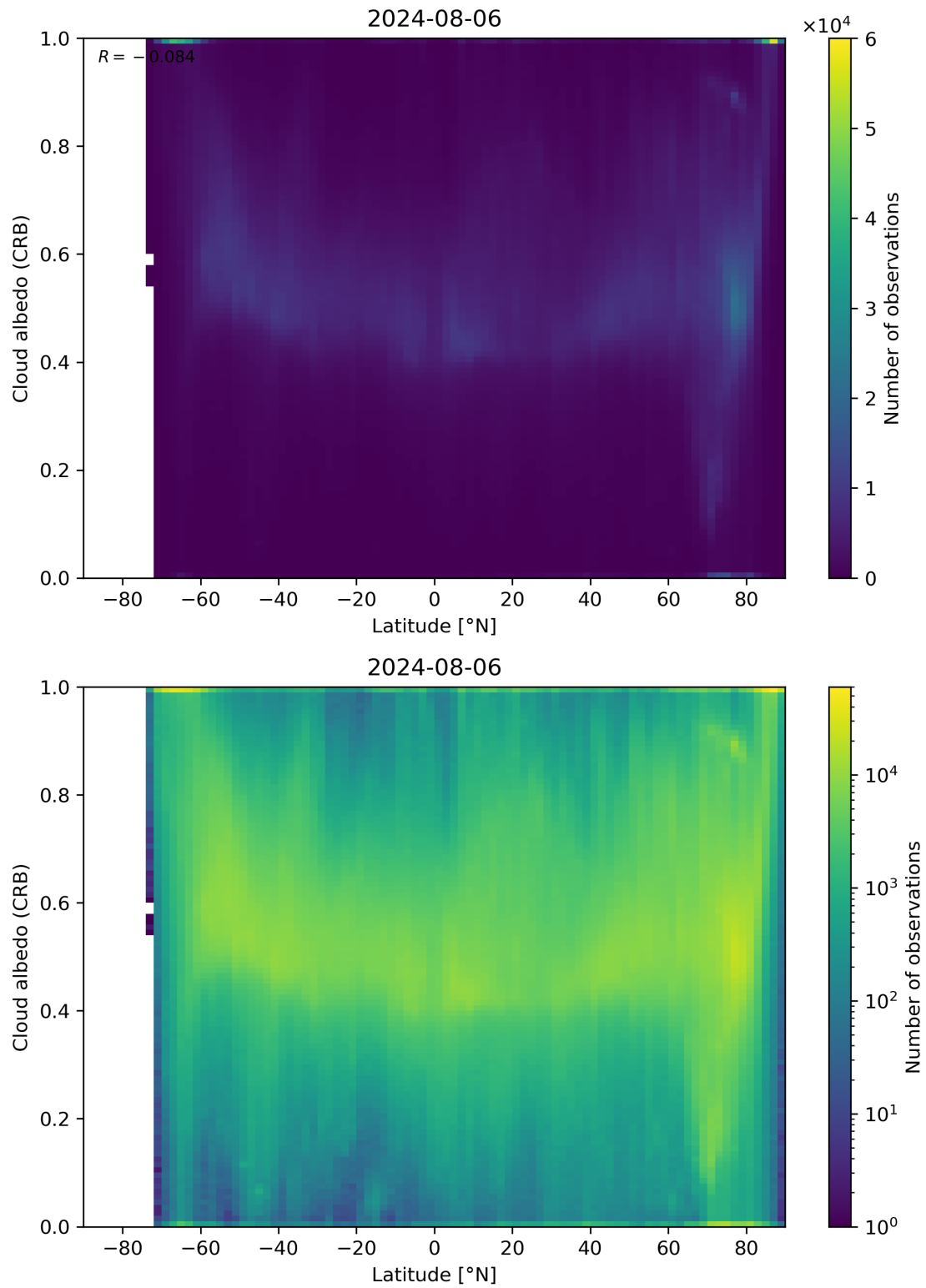
Figure 91: Scatter density plot of “Latitude” against “Cloud albedo (CRB)” for 2024-08-06 to 2024-08-07.
