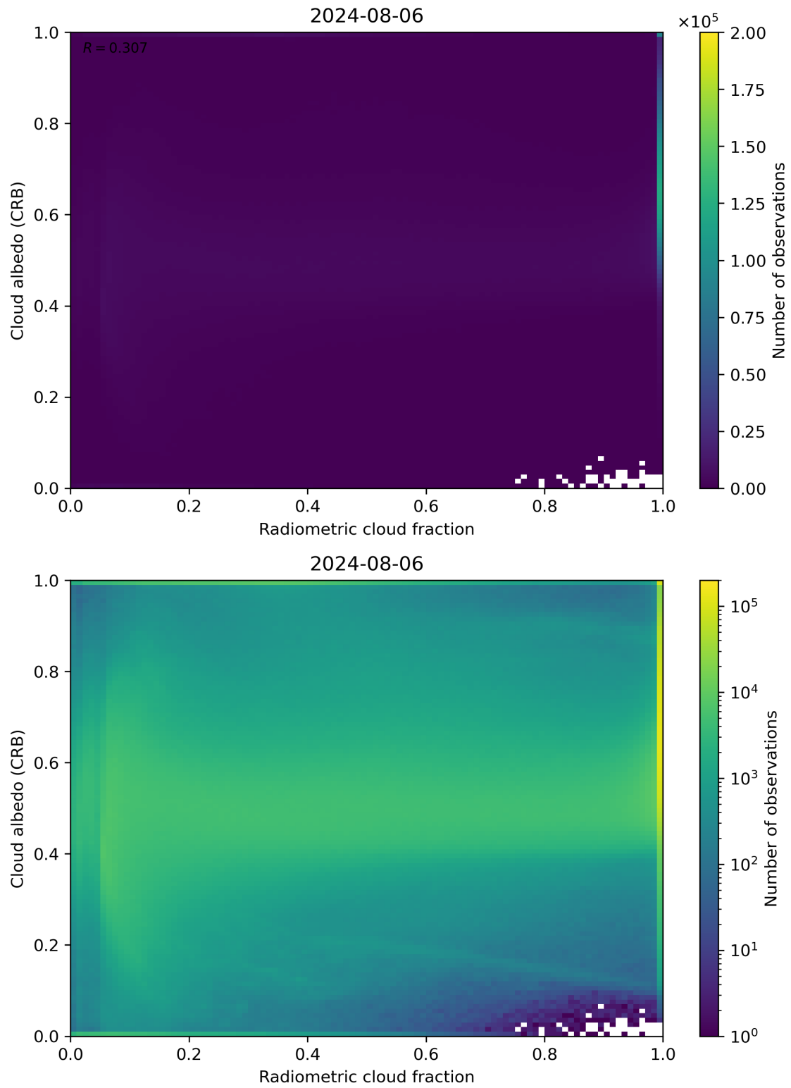
Figure 71: Scatter density plot of “Radiometric cloud fraction” against “Cloud albedo (CRB)” for 2024-08-06 to 2024-08-07.
