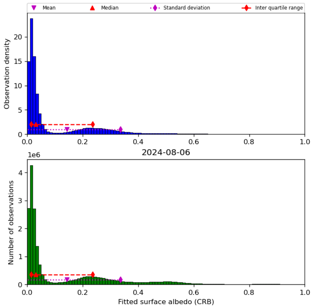
Figure 46: Histogram of “Fitted surface albedo (CRB)” for 2024-08-06 to 2024-08-07
