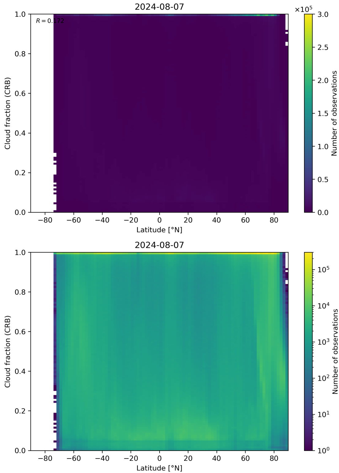
Figure 94: Scatter density plot of “Latitude” against “Cloud fraction (CRB)” for 2024-08-06 to 2024-08-08.
