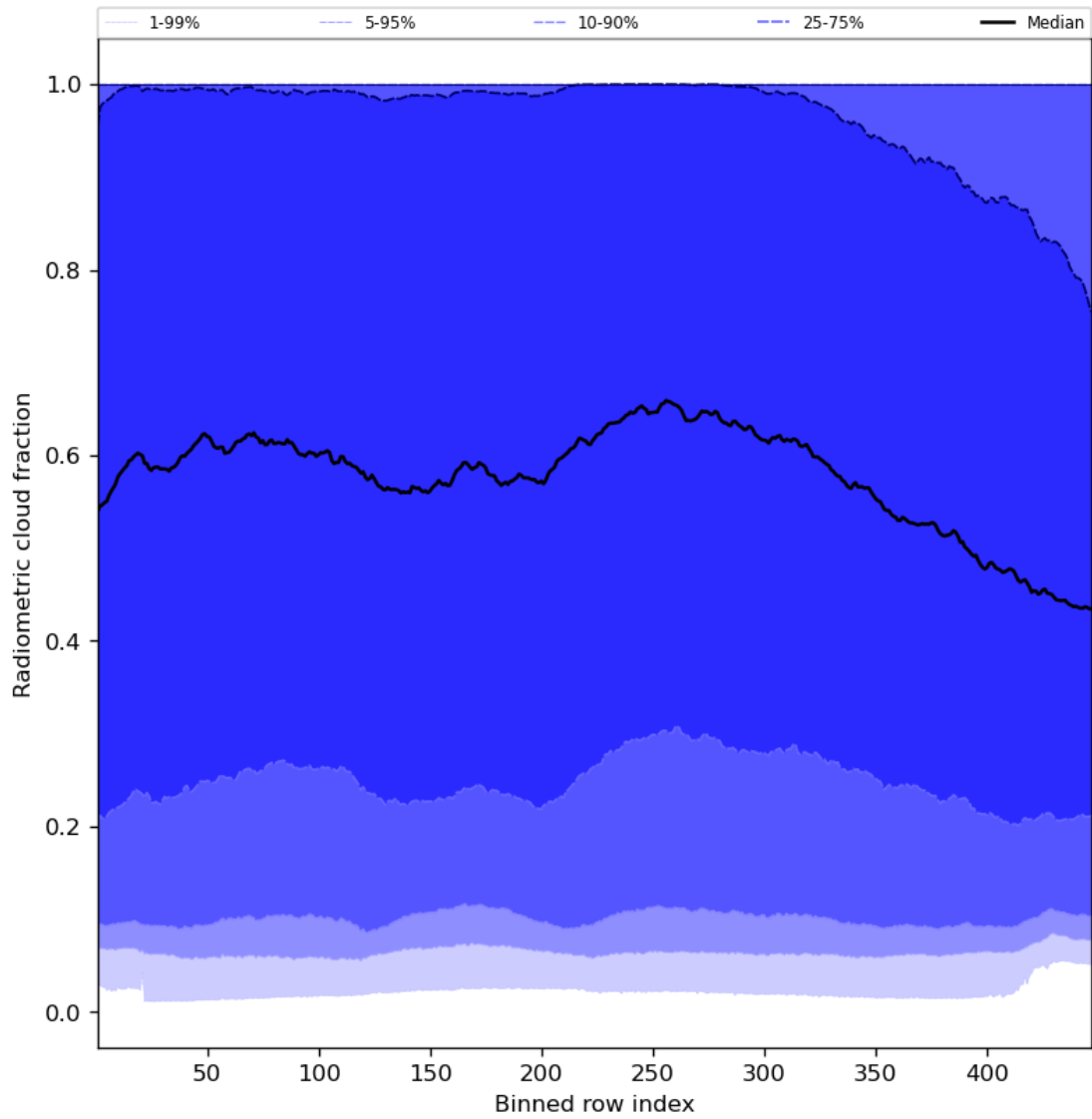
Figure 55: Along track statistics of “Radiometric cloud fraction” for 2024-08-06 to 2024-08-08
