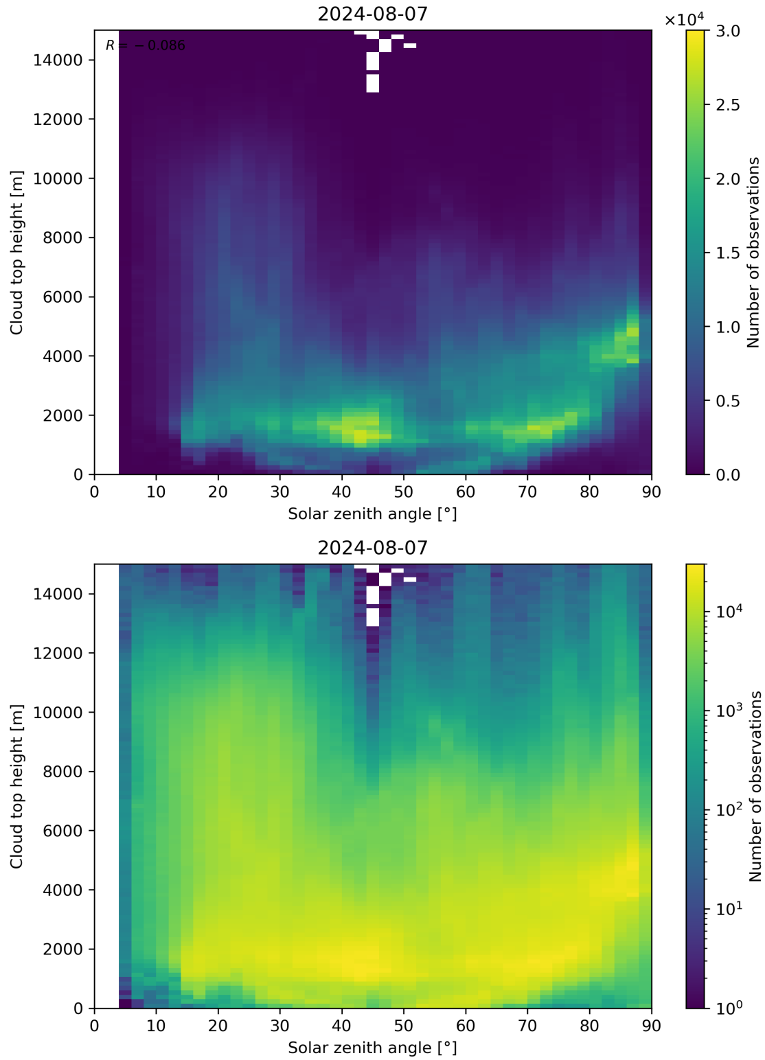
Figure 104: Scatter density plot of “Solar zenith angle” against “Cloud top height” for 2024-08-06 to 2024-08-08.
