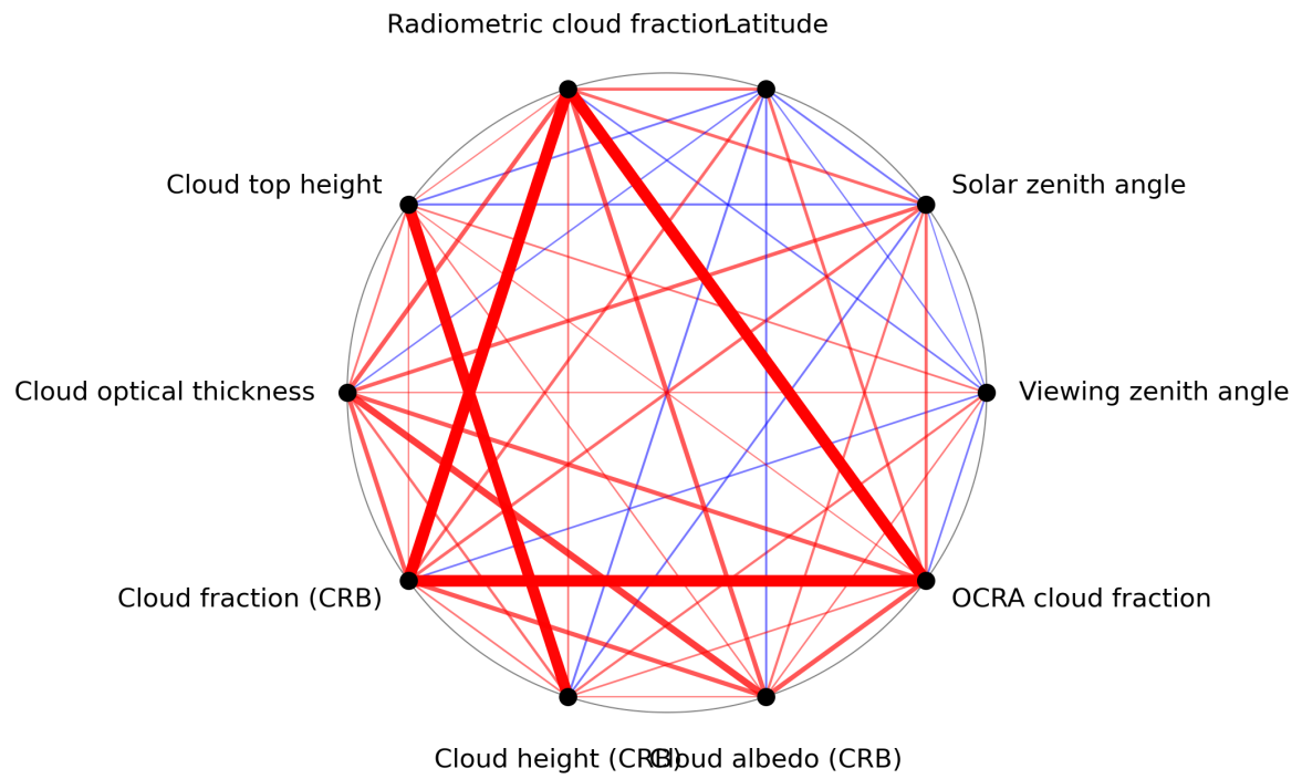
Figure 1: Map of correlation graph for 2024-08-06 to 2024-08-08.
