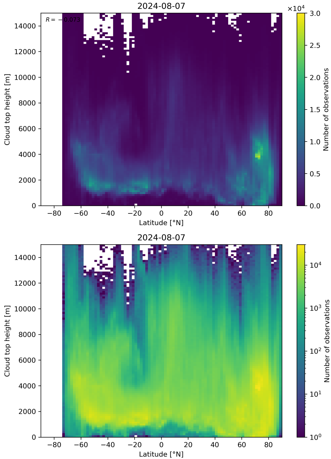
Figure 97: Scatter density plot of “Latitude” against “Cloud top height” for 2024-08-06 to 2024-08-08.
