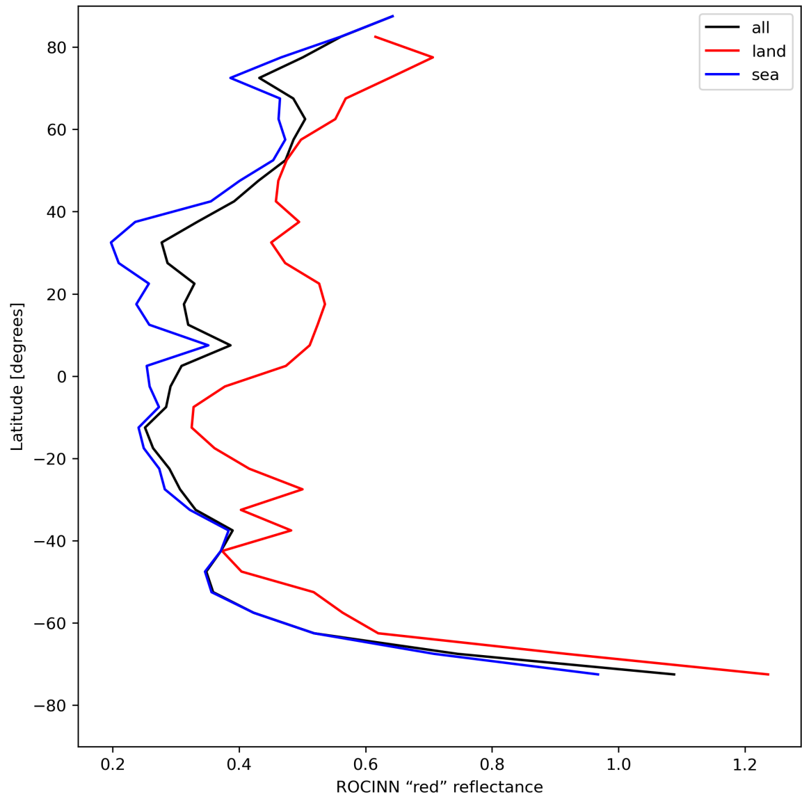
Figure 37: Zonal average of “ROCINN “red” reflectance” for 2024-08-06 to 2024-08-08.
