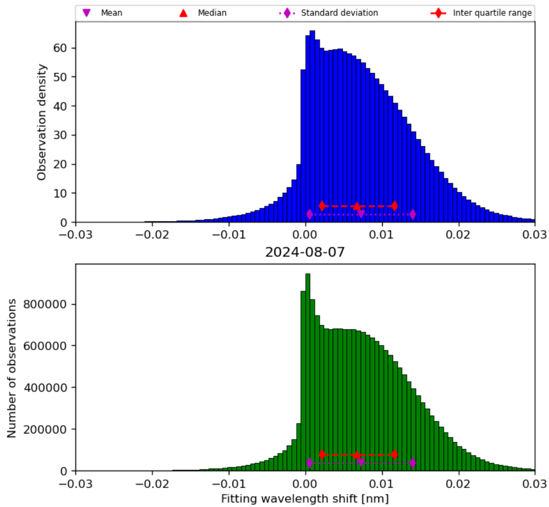
Figure 49: Histogram of “Fitting wavelength shift” for 2024-08-06 to 2024-08-08
