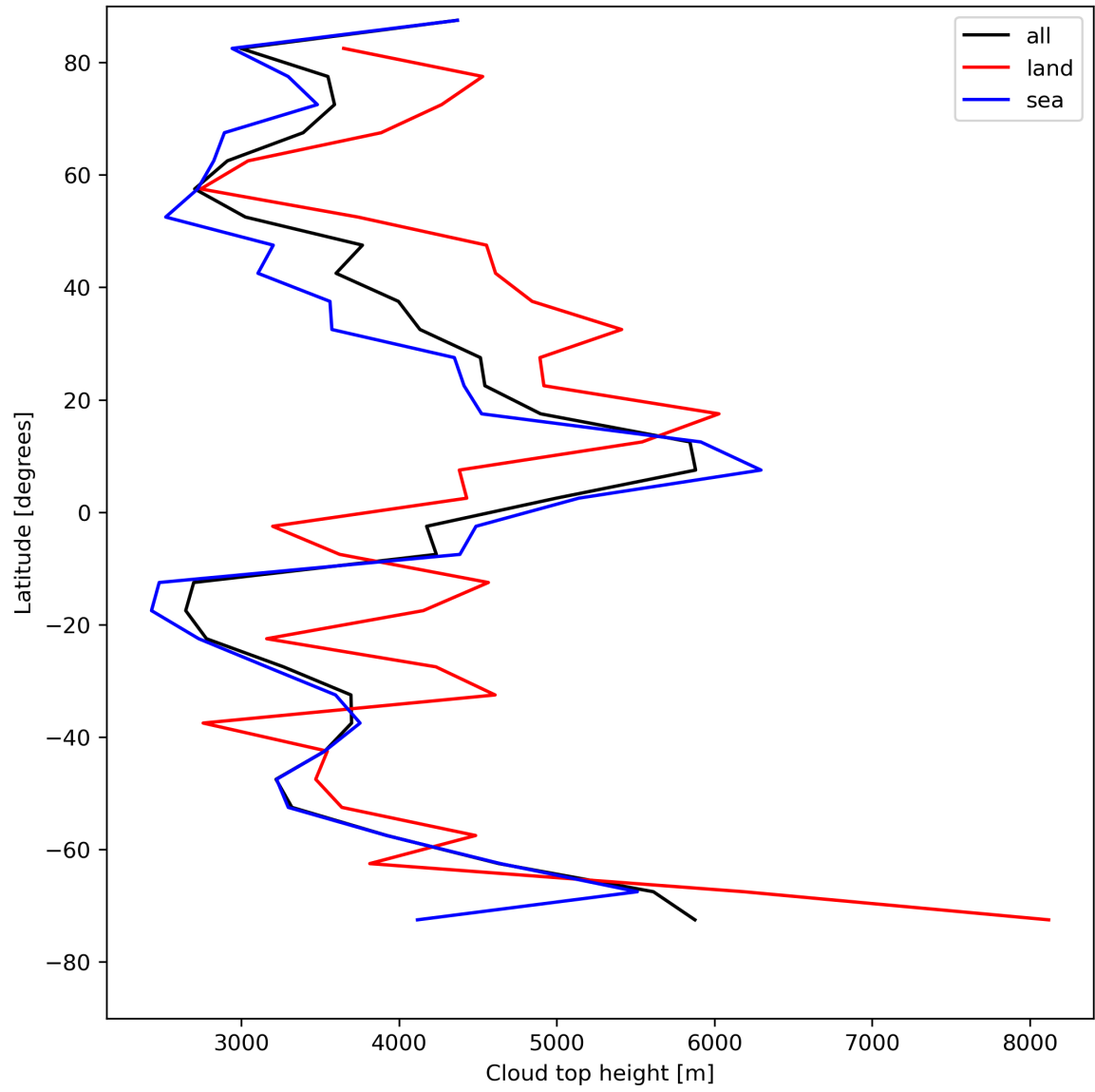
Figure 24: Zonal average of “Cloud top height” for 2024-08-06 to 2024-08-08.
