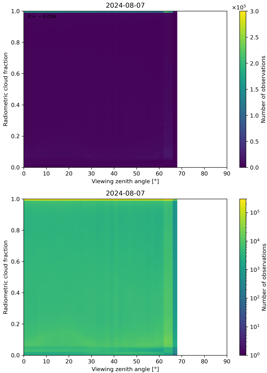
Figure 107: Scatter density plot of “Viewing zenith angle” against “Radiometric cloud fraction” for 2024-08-06 to 2024-08-08.
