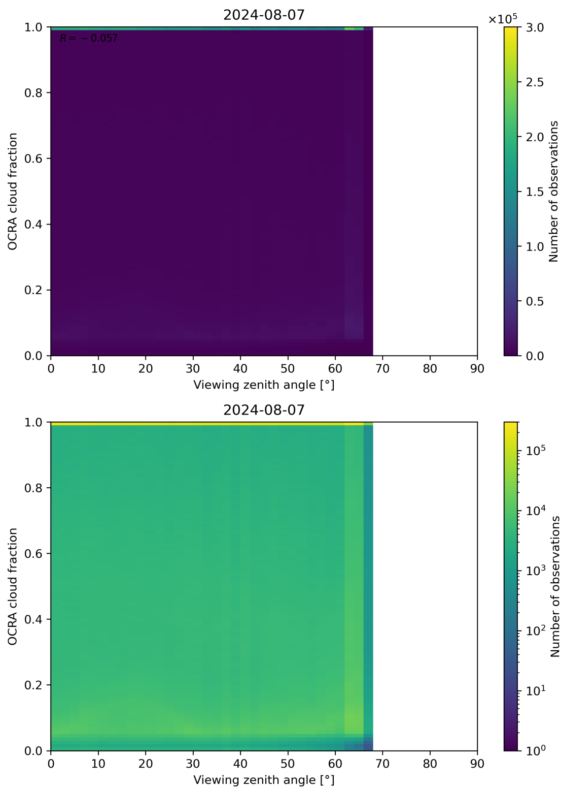
Figure 108: Scatter density plot of “Viewing zenith angle” against “OCRA cloud fraction” for 2024-08-06 to 2024-08-08.
