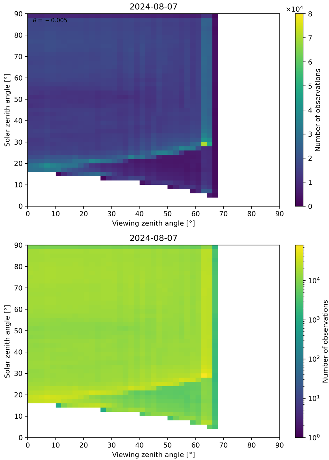
Figure 114: Scatter density plot of “Viewing zenith angle” against “Solar zenith angle” for 2024-08-06 to 2024-08-08.
