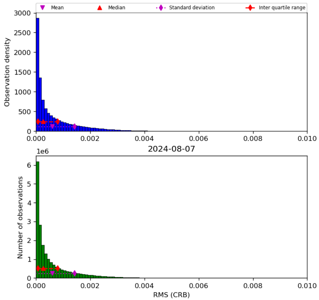
Figure 48: Histogram of “RMS (CRB)” for 2024-08-06 to 2024-08-08
