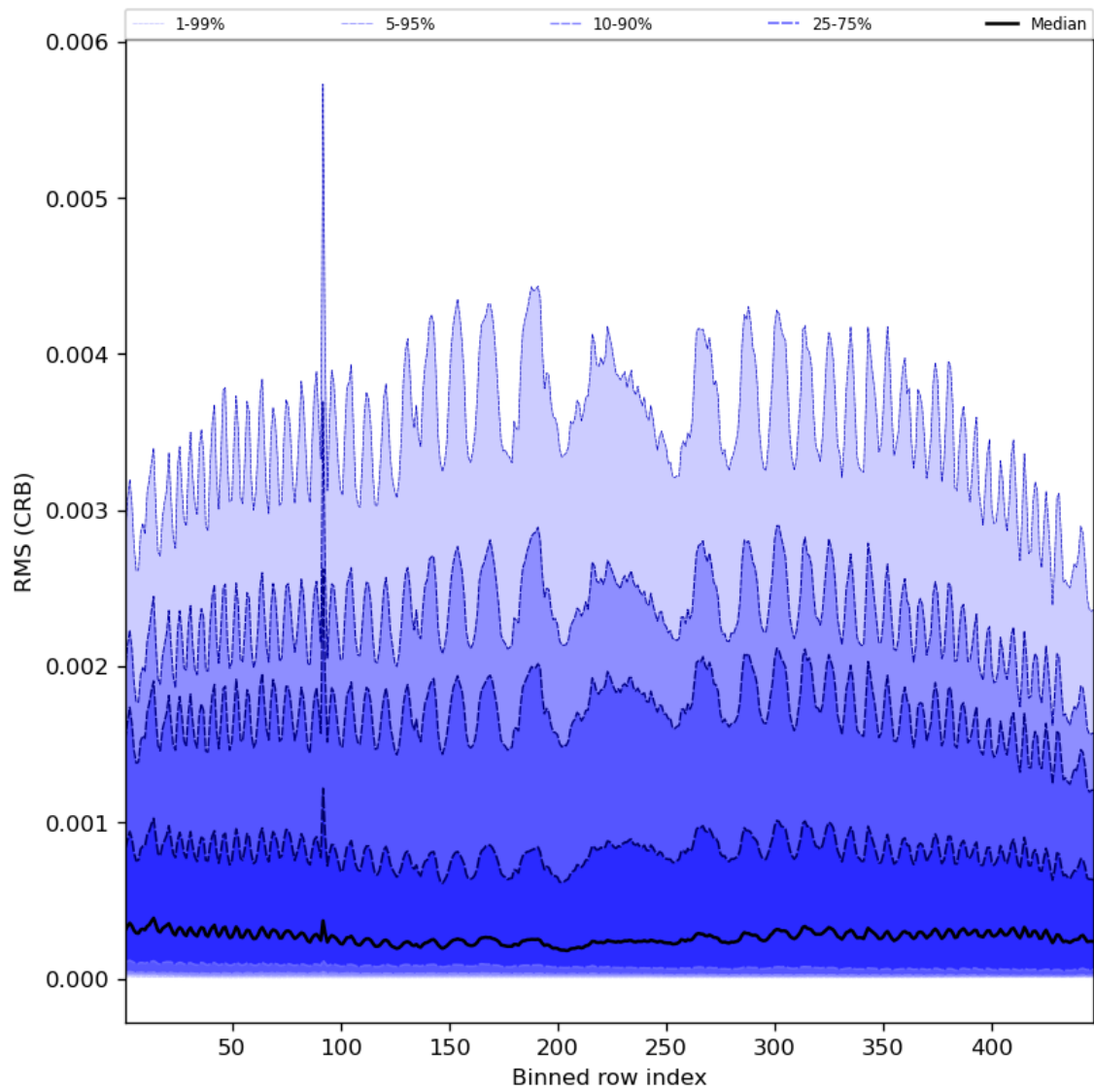
Figure 64: Along track statistics of “RMS (CRB)” for 2024-08-06 to 2024-08-08
