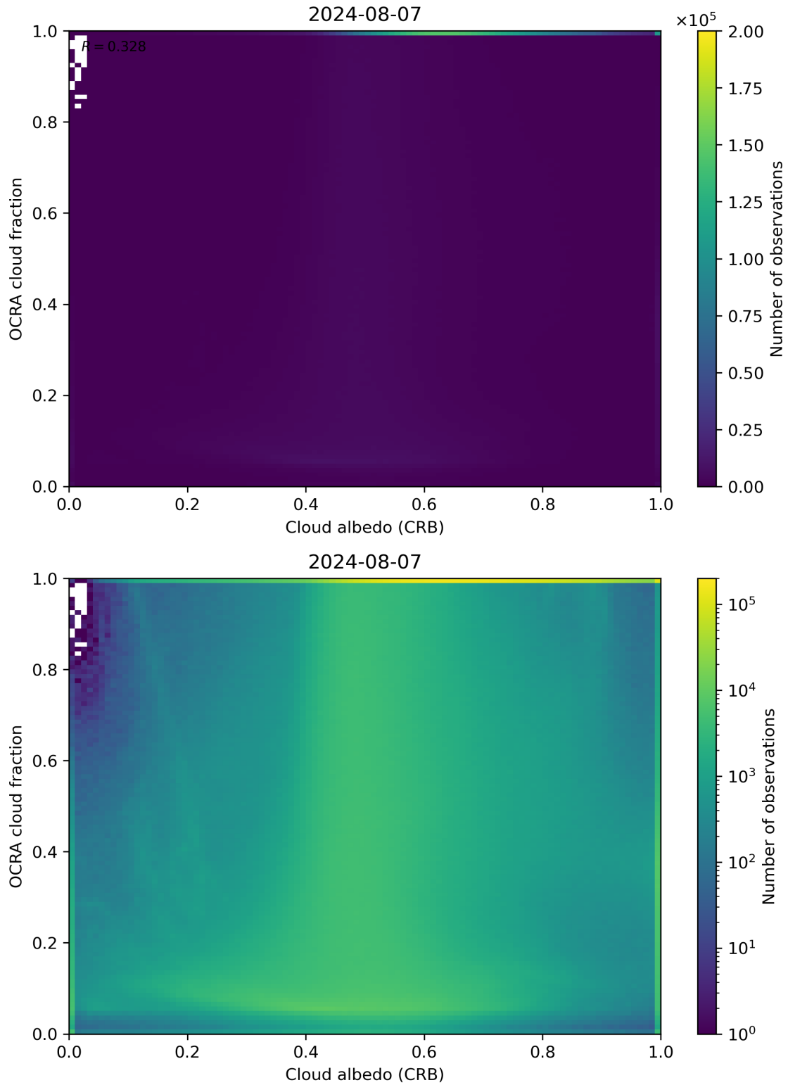
Figure 70: Scatter density plot of “Cloud albedo (CRB)” against “OCRA cloud fraction” for 2024-08-06 to 2024-08-08.
