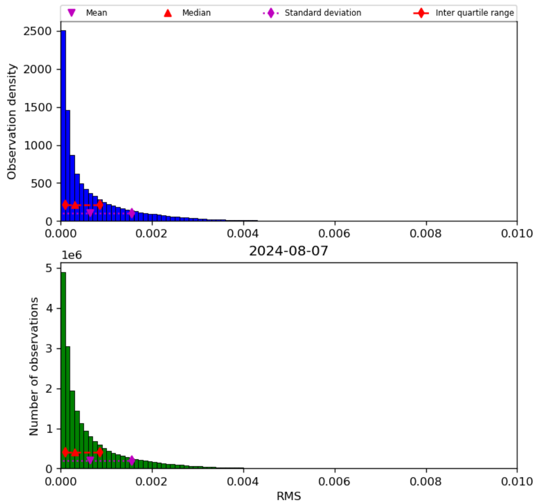
Figure 47: Histogram of “RMS” for 2024-08-06 to 2024-08-08
