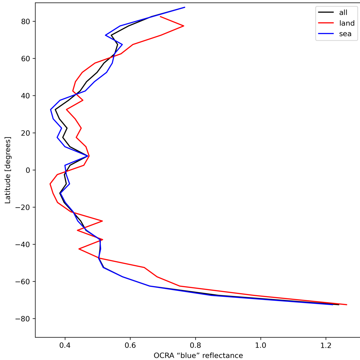
Figure 35: Zonal average of “OCRA “blue” reflectance” for 2024-08-06 to 2024-08-08.
