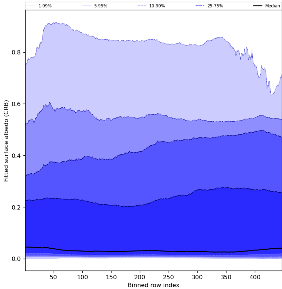
Figure 62: Along track statistics of “Fitted surface albedo (CRB)” for 2024-08-06 to 2024-08-08
