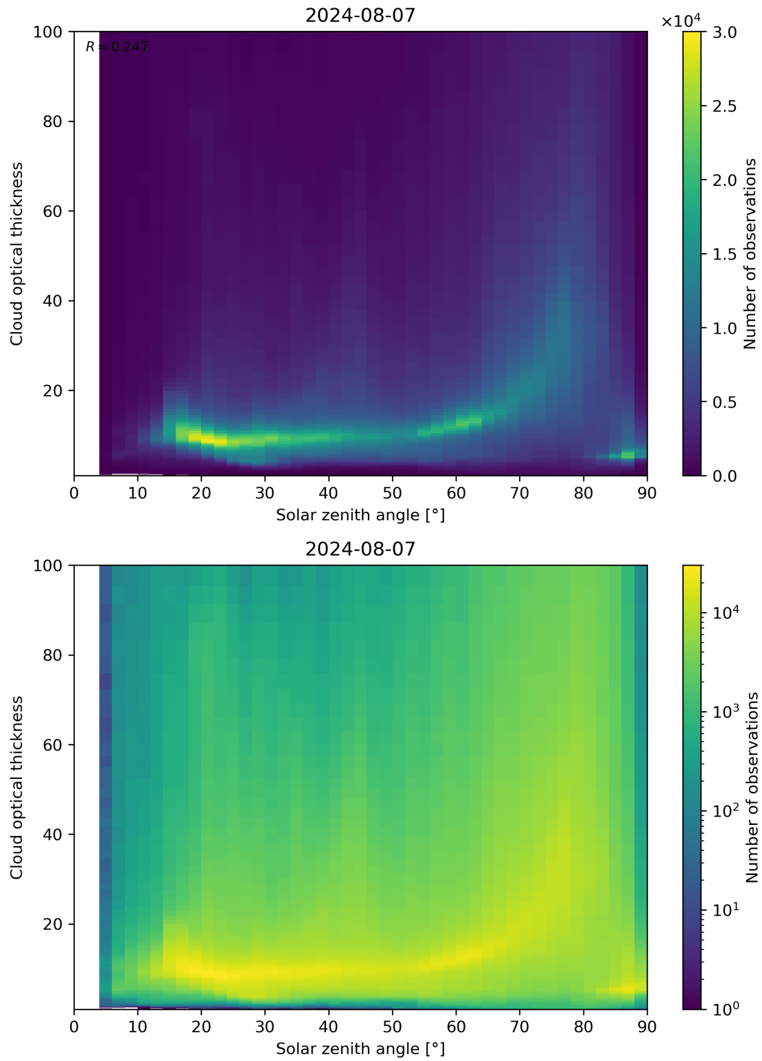
Figure 103: Scatter density plot of “Solar zenith angle” against “Cloud optical thickness” for 2024-08-06 to 2024-08-08.
