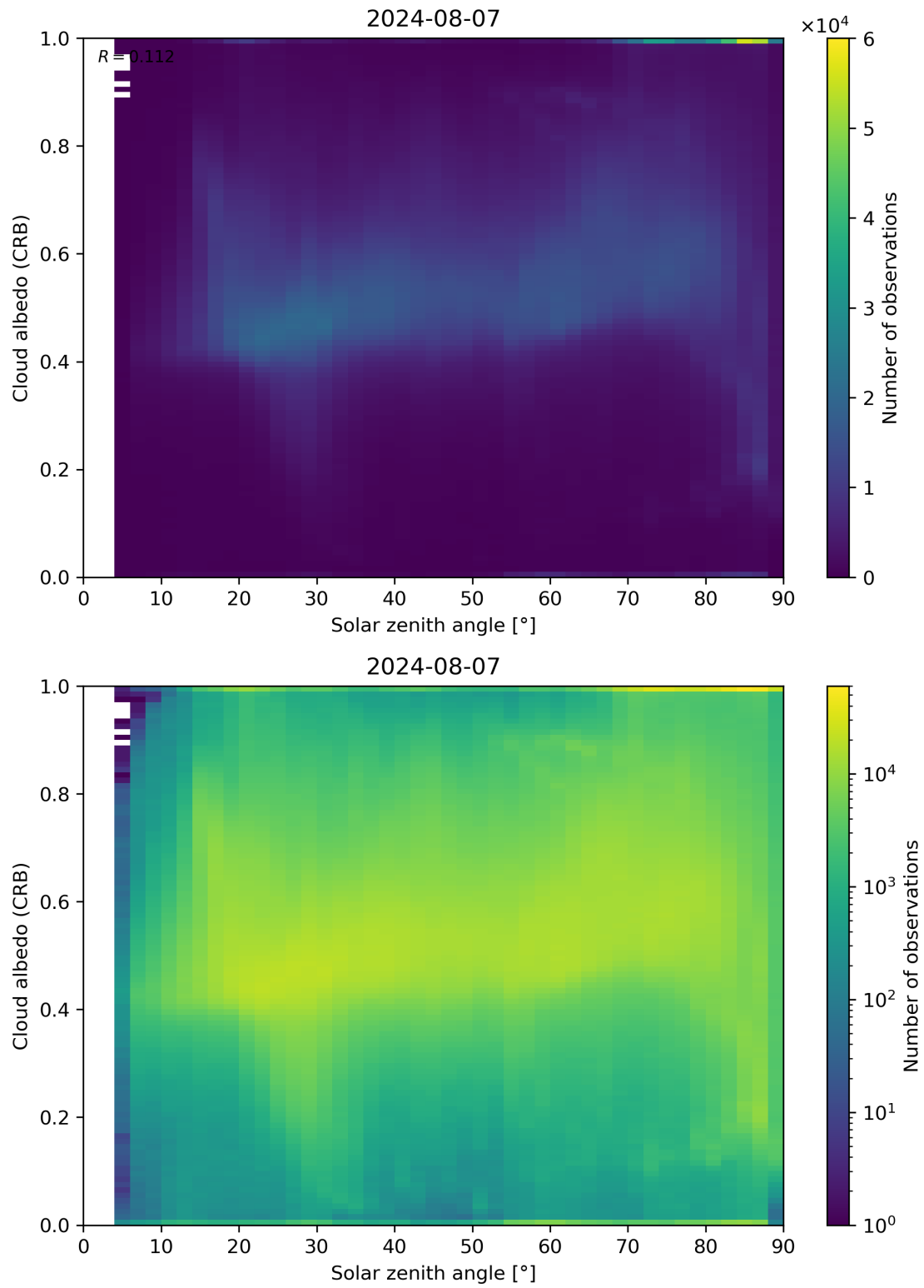
Figure 98: Scatter density plot of “Solar zenith angle” against “Cloud albedo (CRB)” for 2024-08-06 to 2024-08-08.
