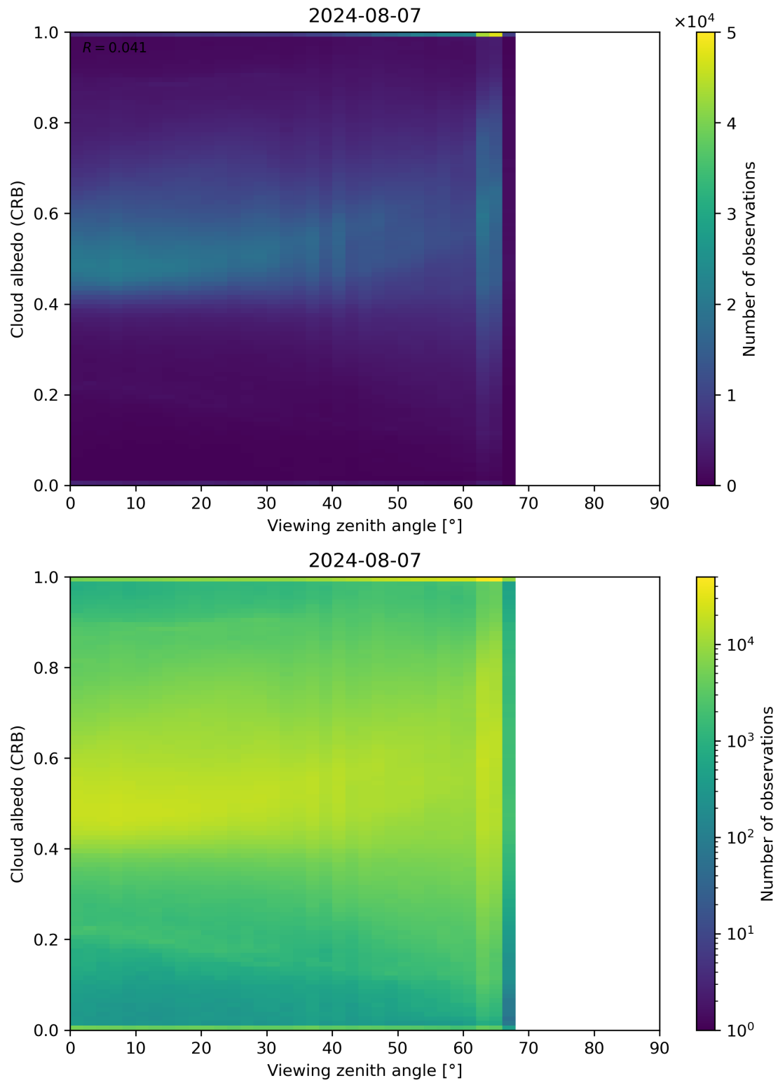
Figure 106: Scatter density plot of “Viewing zenith angle” against “Cloud albedo (CRB)” for 2024-08-06 to 2024-08-08.
