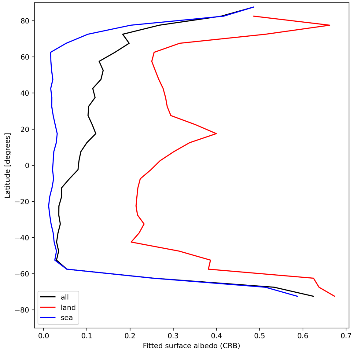
Figure 30: Zonal average of “Fitted surface albedo (CRB)” for 2024-08-06 to 2024-08-08.
