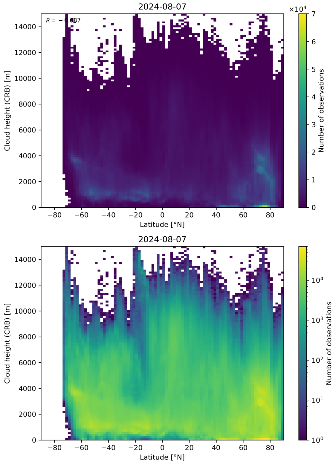
Figure 95: Scatter density plot of “Latitude” against “Cloud height (CRB)” for 2024-08-06 to 2024-08-08.
