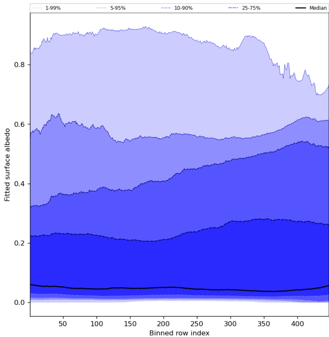
Figure 61: Along track statistics of “Fitted surface albedo” for 2024-08-06 to 2024-08-08
