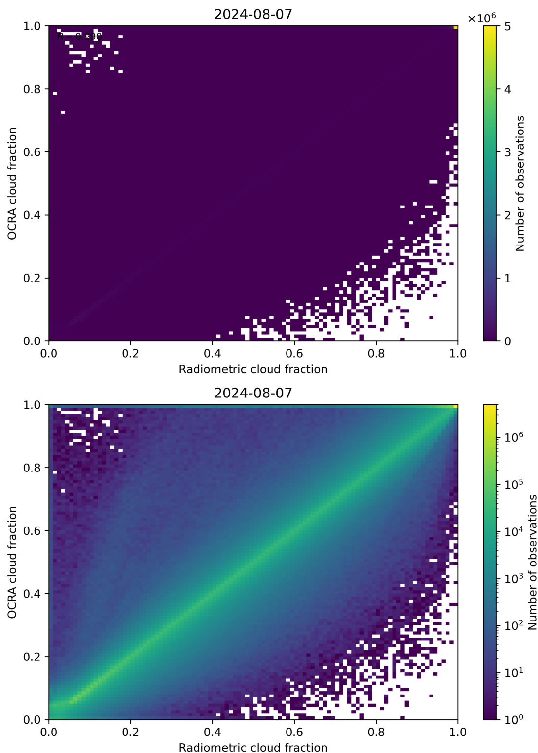
Figure 72: Scatter density plot of “Radiometric cloud fraction” against “OCRA cloud fraction” for 2024-08-06 to 2024-08-08.
