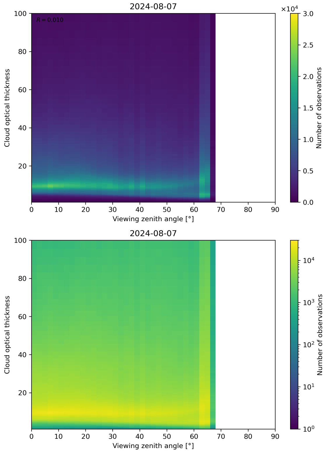
Figure 111: Scatter density plot of “Viewing zenith angle” against “Cloud optical thickness” for 2024-08-06 to 2024-08-08.
