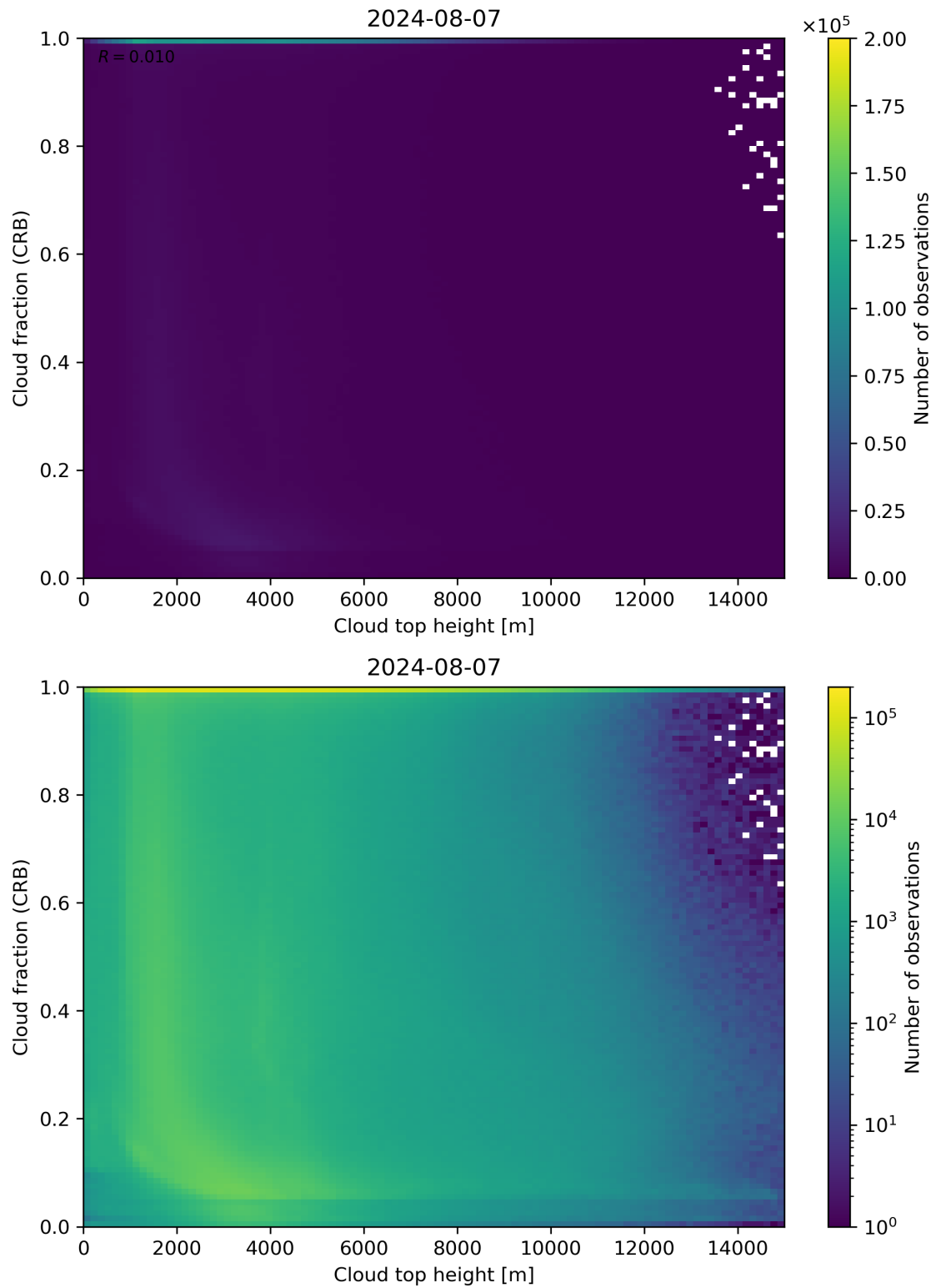
Figure 88: Scatter density plot of “Cloud top height” against “Cloud fraction (CRB)” for 2024-08-06 to 2024-08-08.
