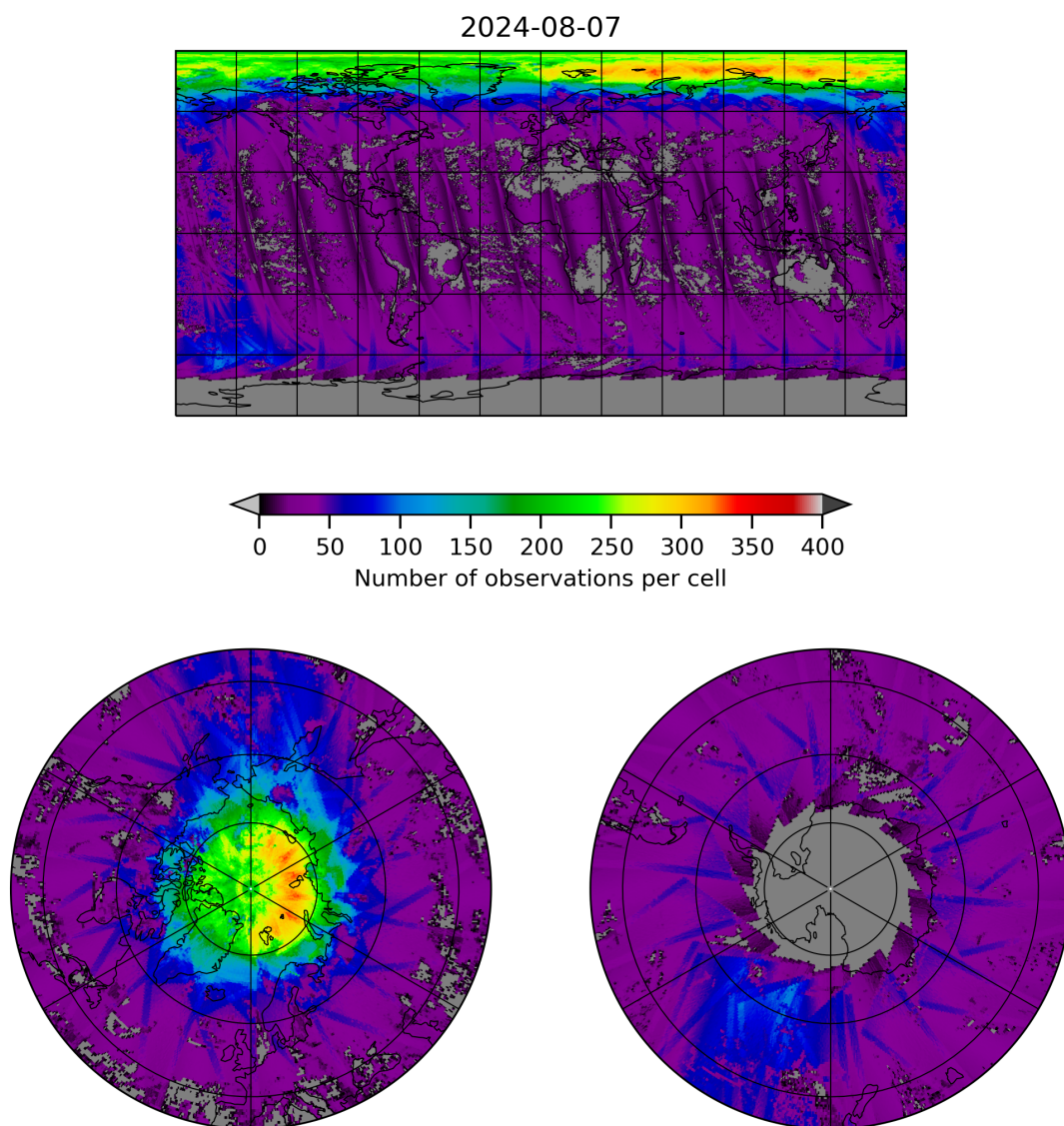
Figure 21: Map of the number of observations for 2024-08-06 to 2024-08-08
