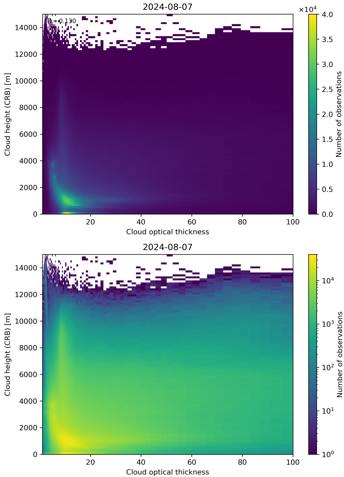
Figure 85: Scatter density plot of “Cloud optical thickness” against “Cloud height (CRB)” for 2024-08-06 to 2024-08-08.
