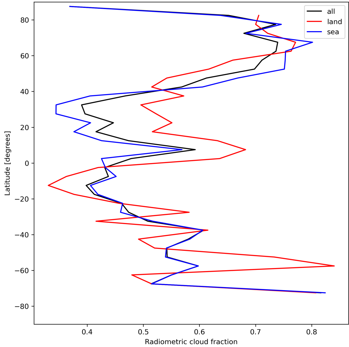
Figure 23: Zonal average of “Radiometric cloud fraction” for 2024-08-06 to 2024-08-08.
