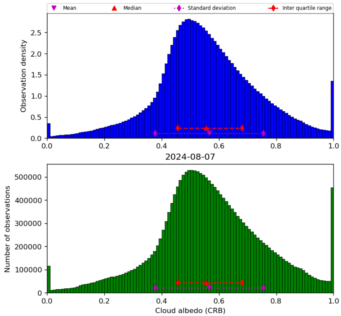
Figure 44: Histogram of “Cloud albedo (CRB)” for 2024-08-06 to 2024-08-08
