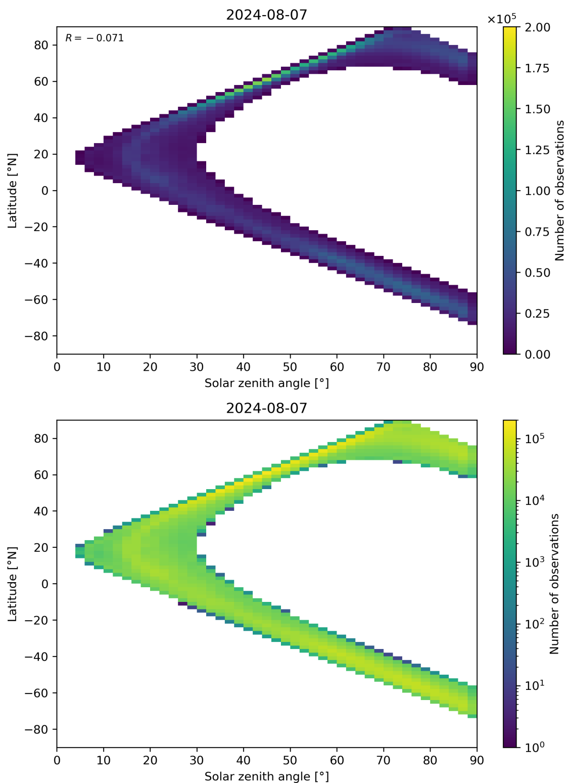
Figure 105: Scatter density plot of “Solar zenith angle” against “Latitude” for 2024-08-06 to 2024-08-08.
