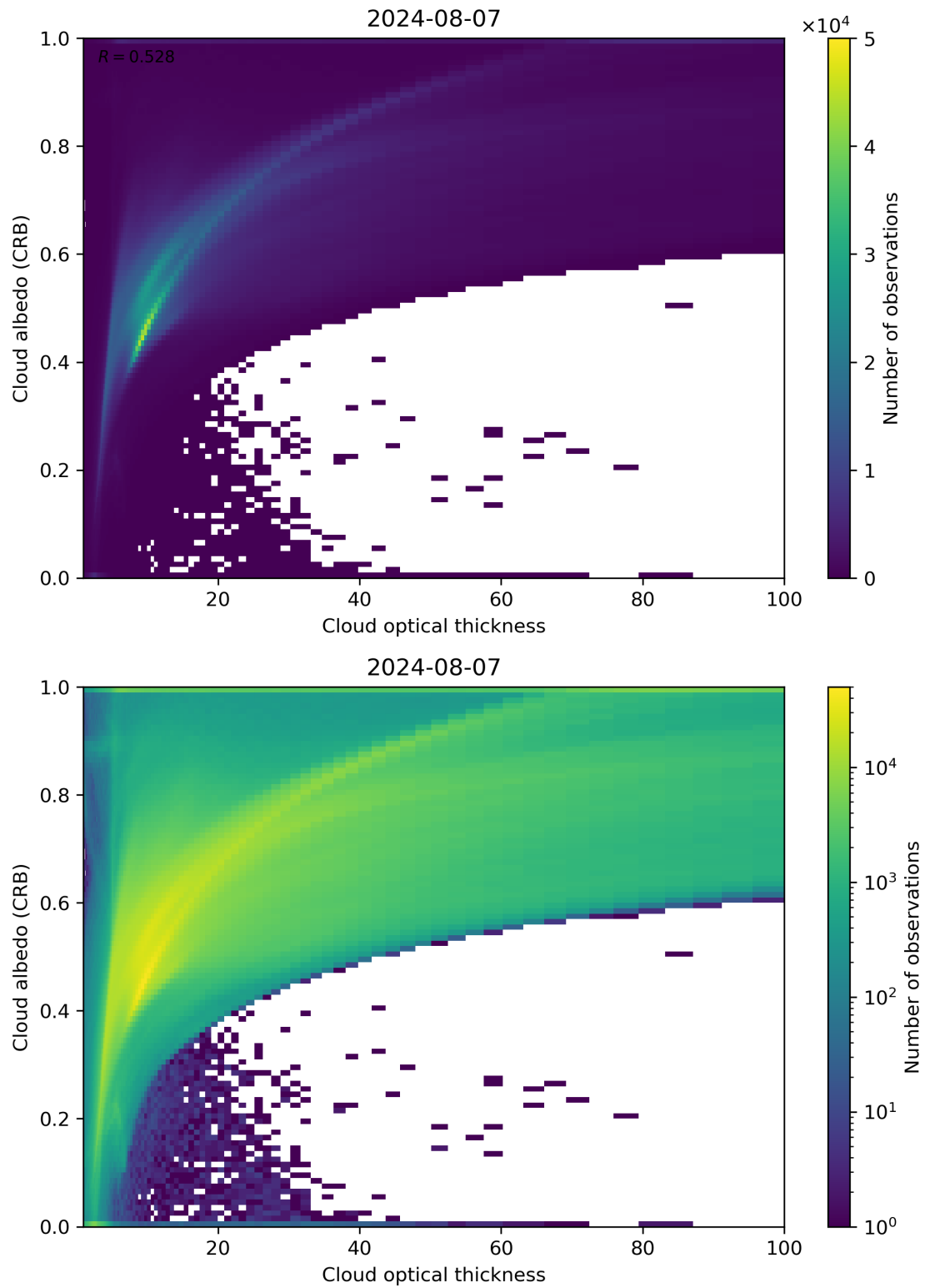
Figure 82: Scatter density plot of “Cloud optical thickness” against “Cloud albedo (CRB)” for 2024-08-06 to 2024-08-08.
