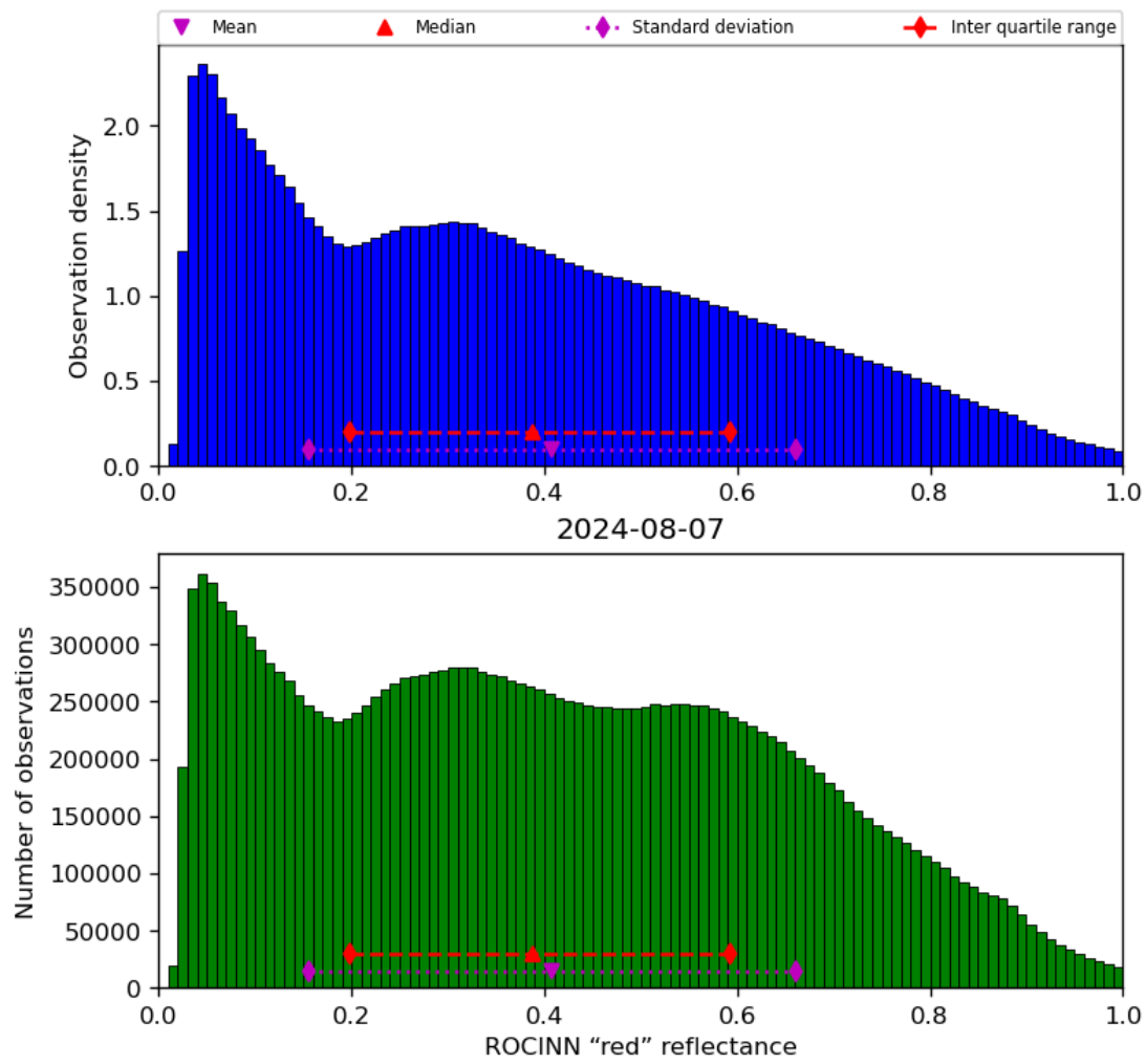
Figure 53: Histogram of “ROCINN “red” reflectance” for 2024-08-06 to 2024-08-08
