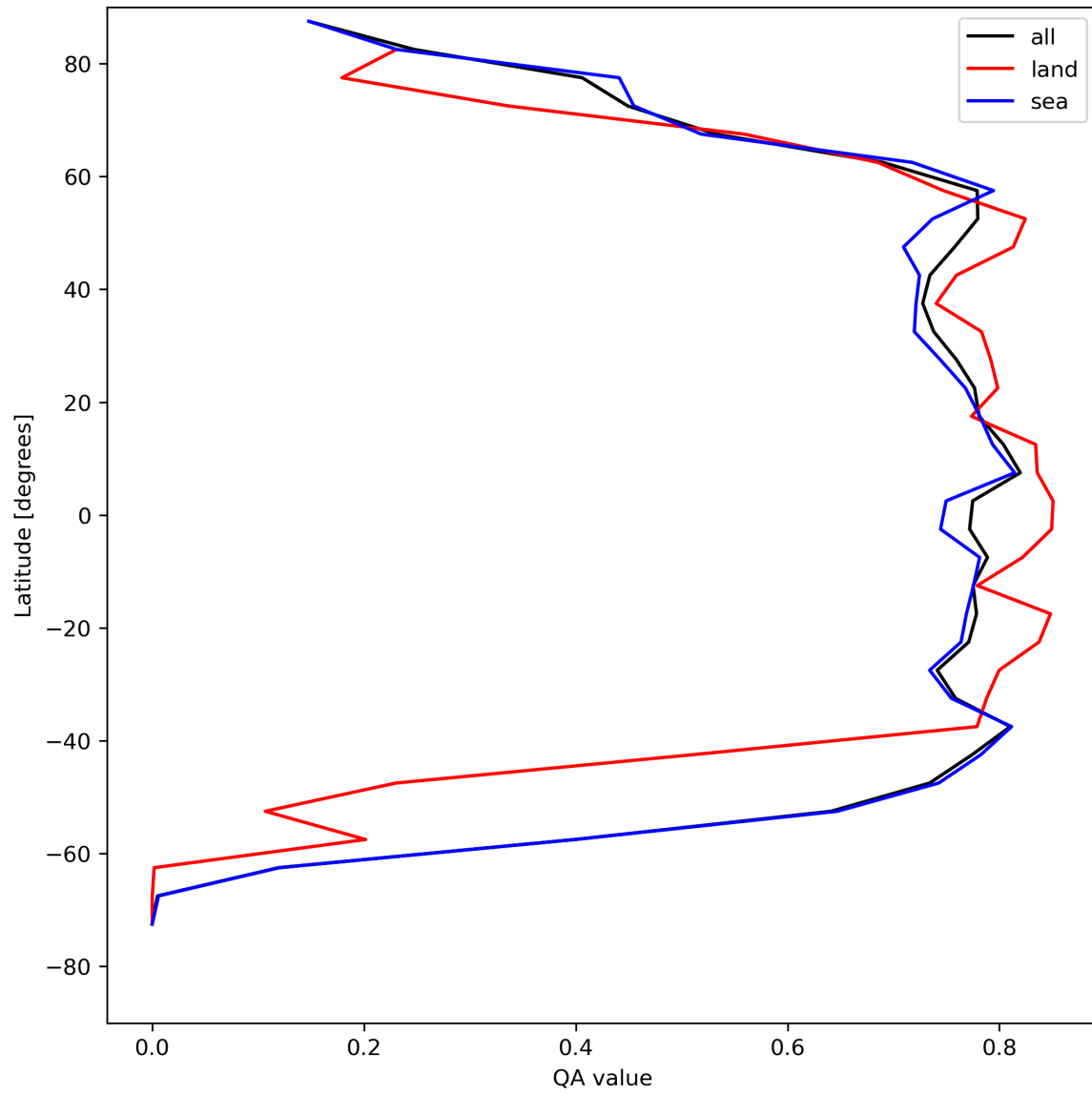
Figure 22: Zonal average of “QA value” for 2024-08-06 to 2024-08-08.
