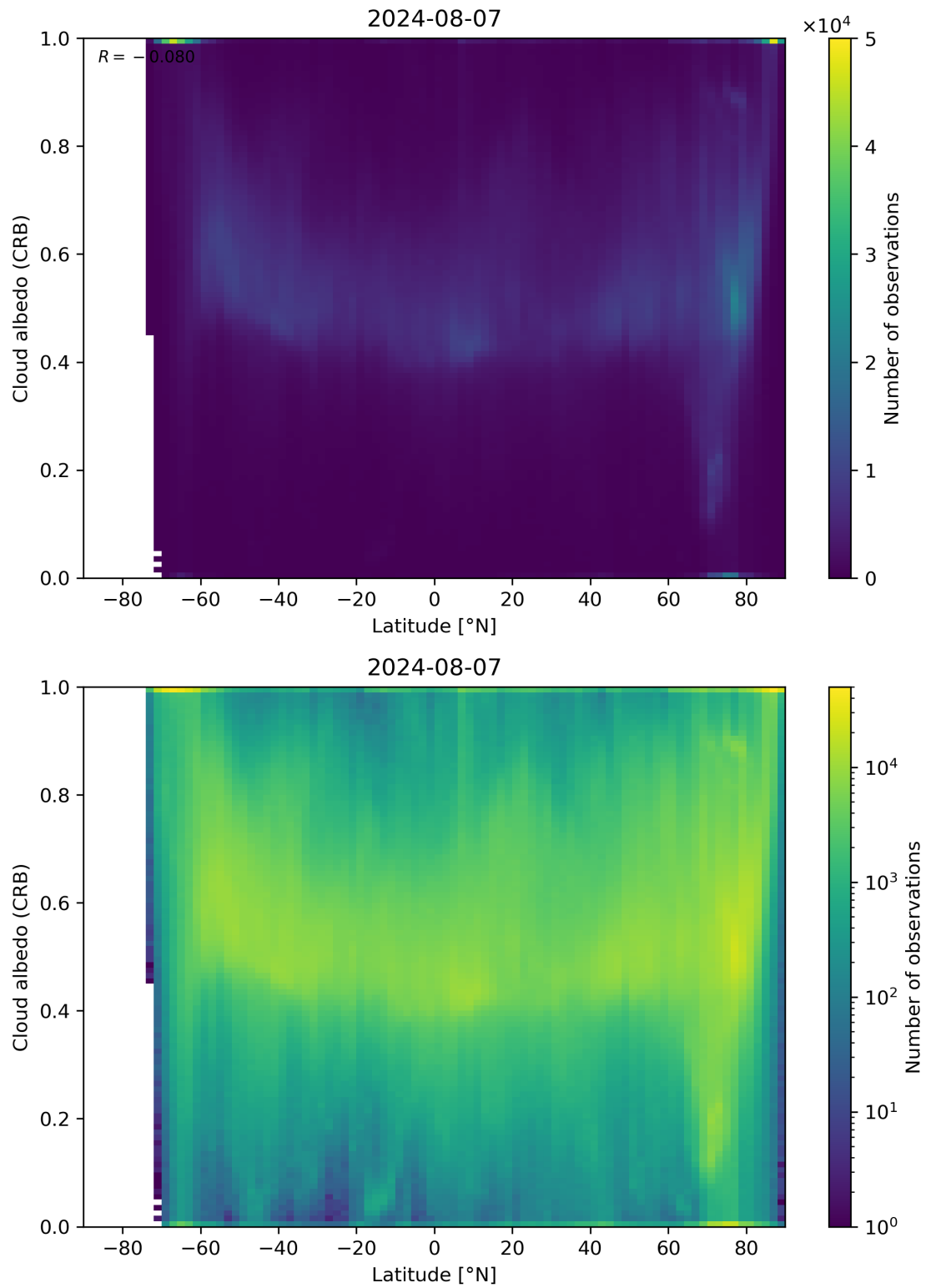
Figure 91: Scatter density plot of “Latitude” against “Cloud albedo (CRB)” for 2024-08-06 to 2024-08-08.
