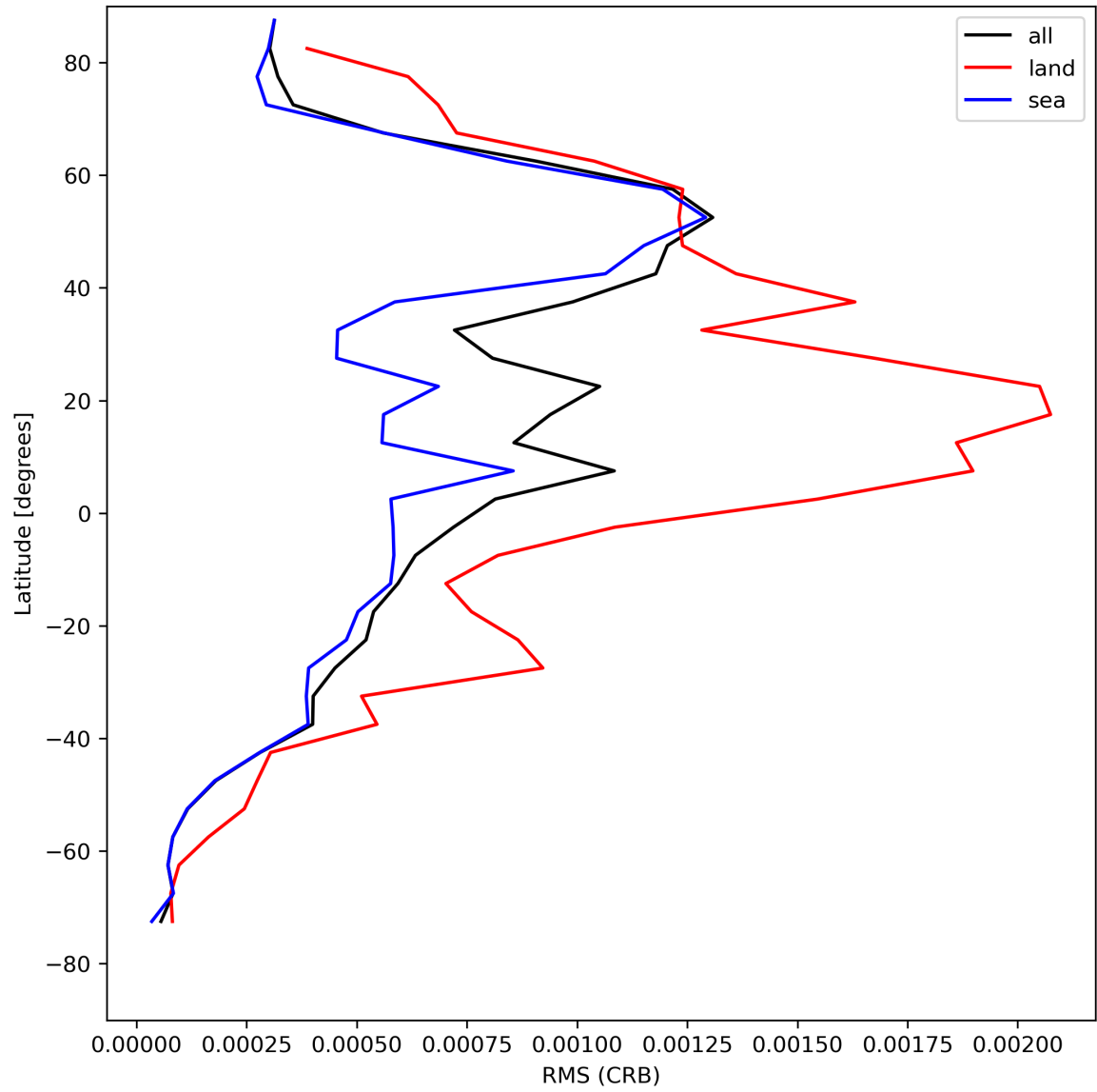
Figure 32: Zonal average of “RMS (CRB)” for 2024-08-06 to 2024-08-08.
