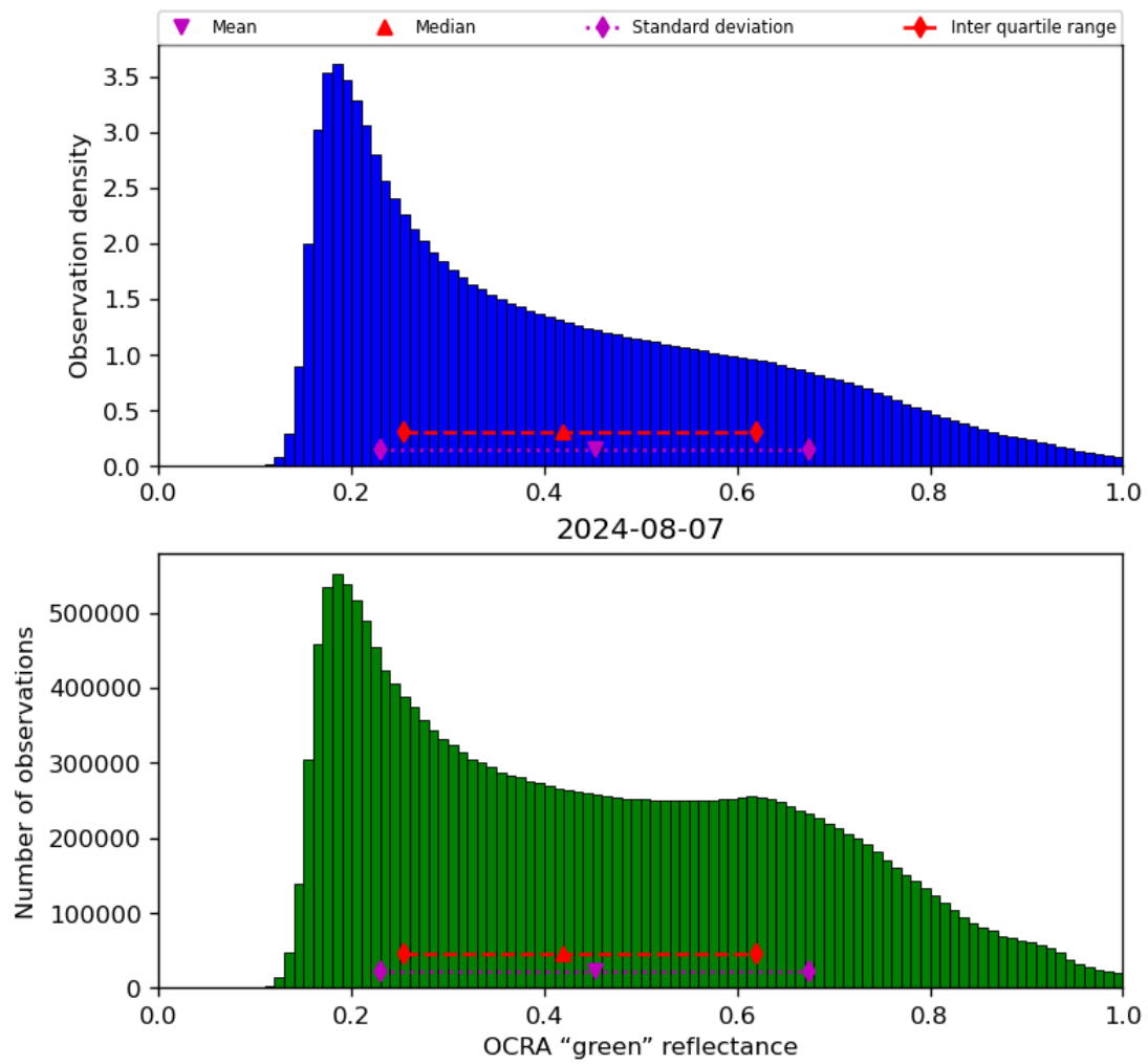
Figure 52: Histogram of “OCRA “green” reflectance” for 2024-08-06 to 2024-08-08
