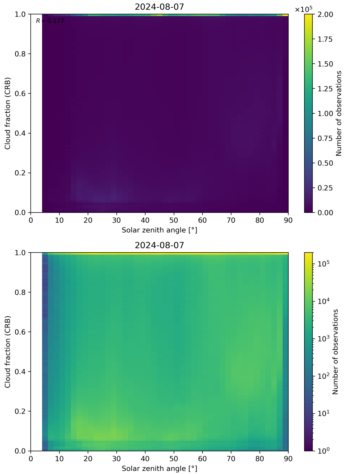
Figure 101: Scatter density plot of “Solar zenith angle” against “Cloud fraction (CRB)” for 2024-08-06 to 2024-08-08.
