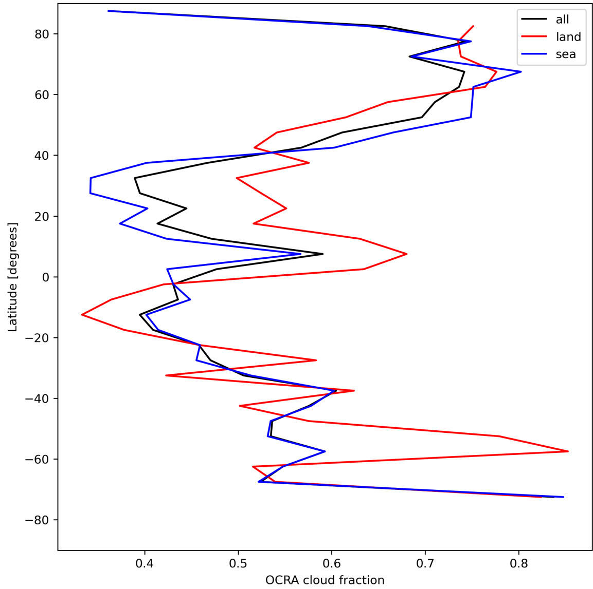
Figure 34: Zonal average of “OCRA cloud fraction” for 2024-08-06 to 2024-08-08.
