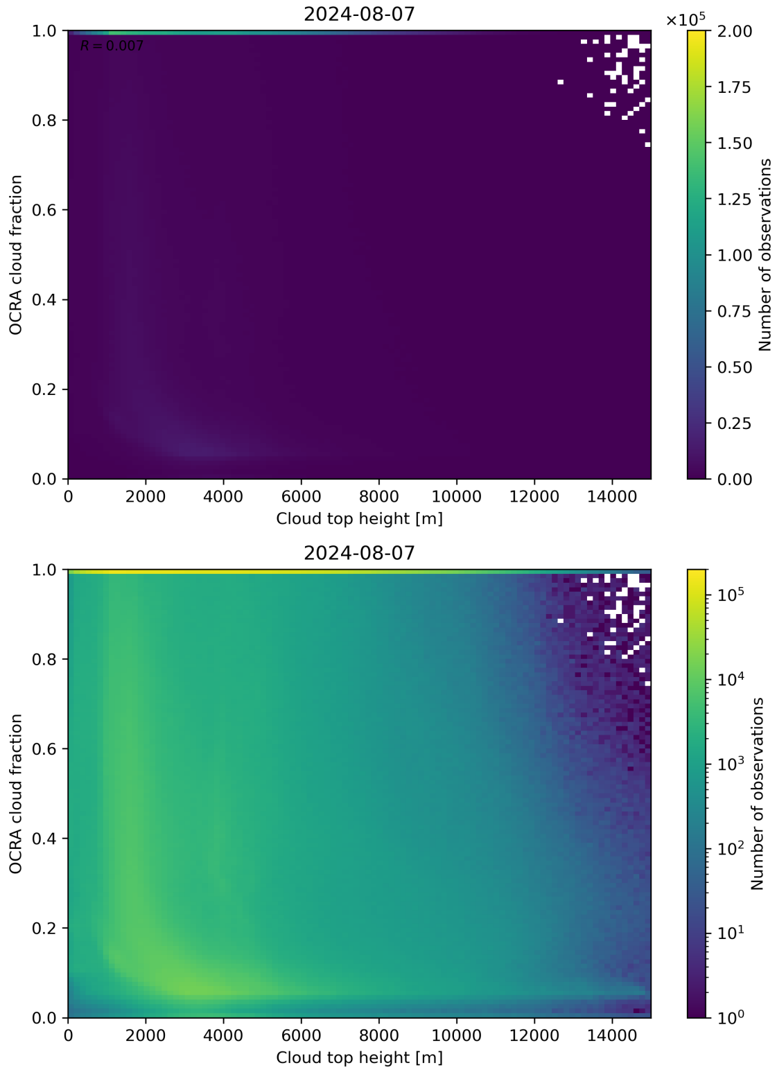
Figure 87: Scatter density plot of “Cloud top height” against “OCRA cloud fraction” for 2024-08-06 to 2024-08-08.
