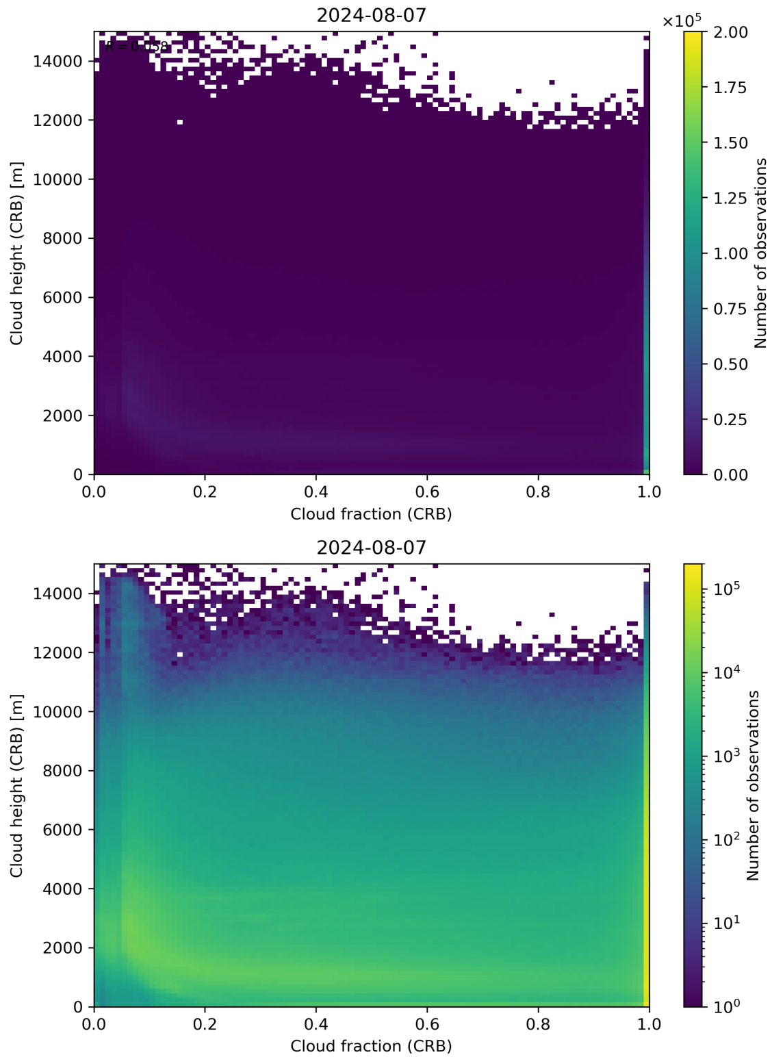
Figure 79: Scatter density plot of “Cloud fraction (CRB)” against “Cloud height (CRB)” for 2024-08-06 to 2024-08-08.
