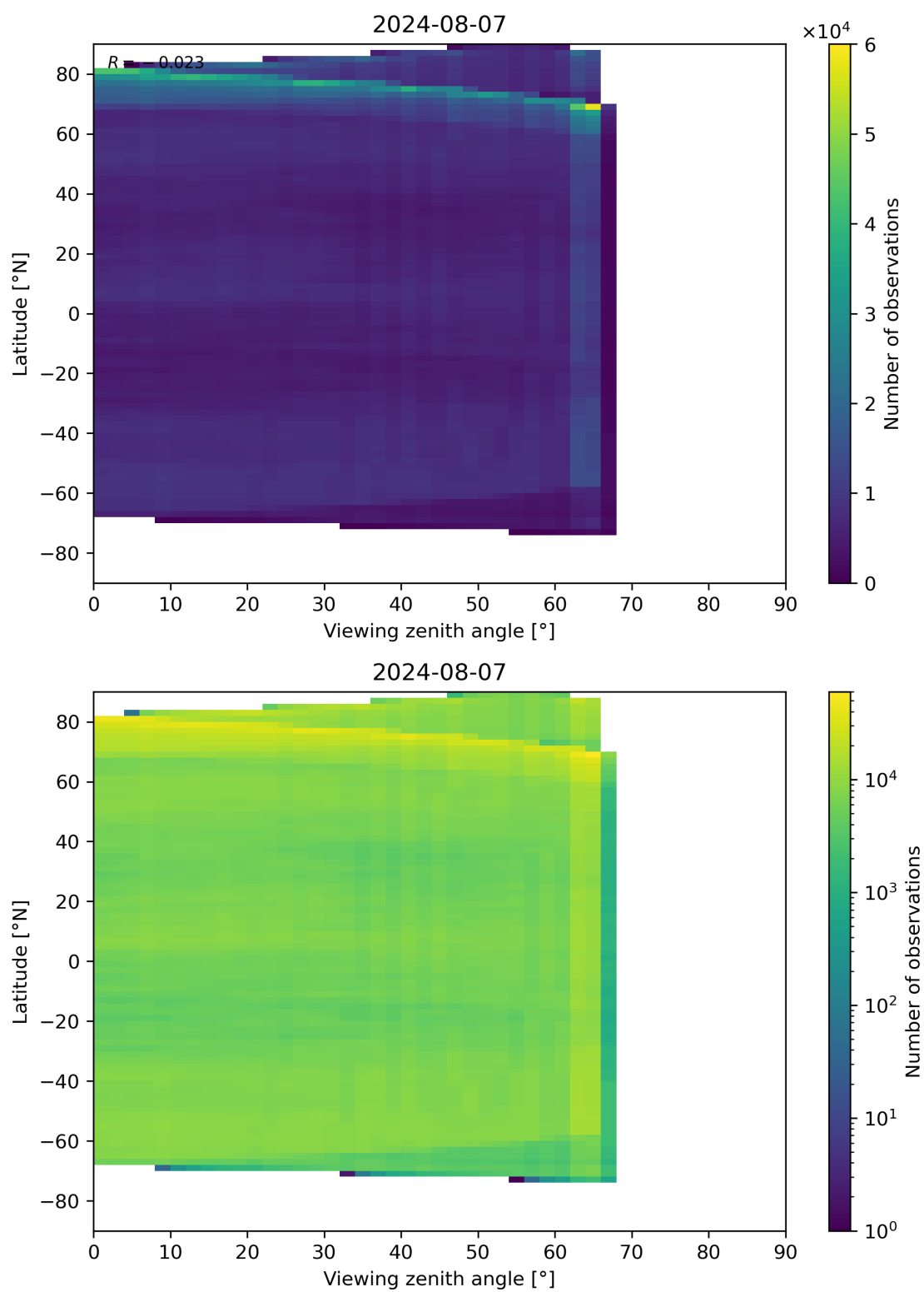
Figure 113: Scatter density plot of “Viewing zenith angle” against “Latitude” for 2024-08-06 to 2024-08-08.
