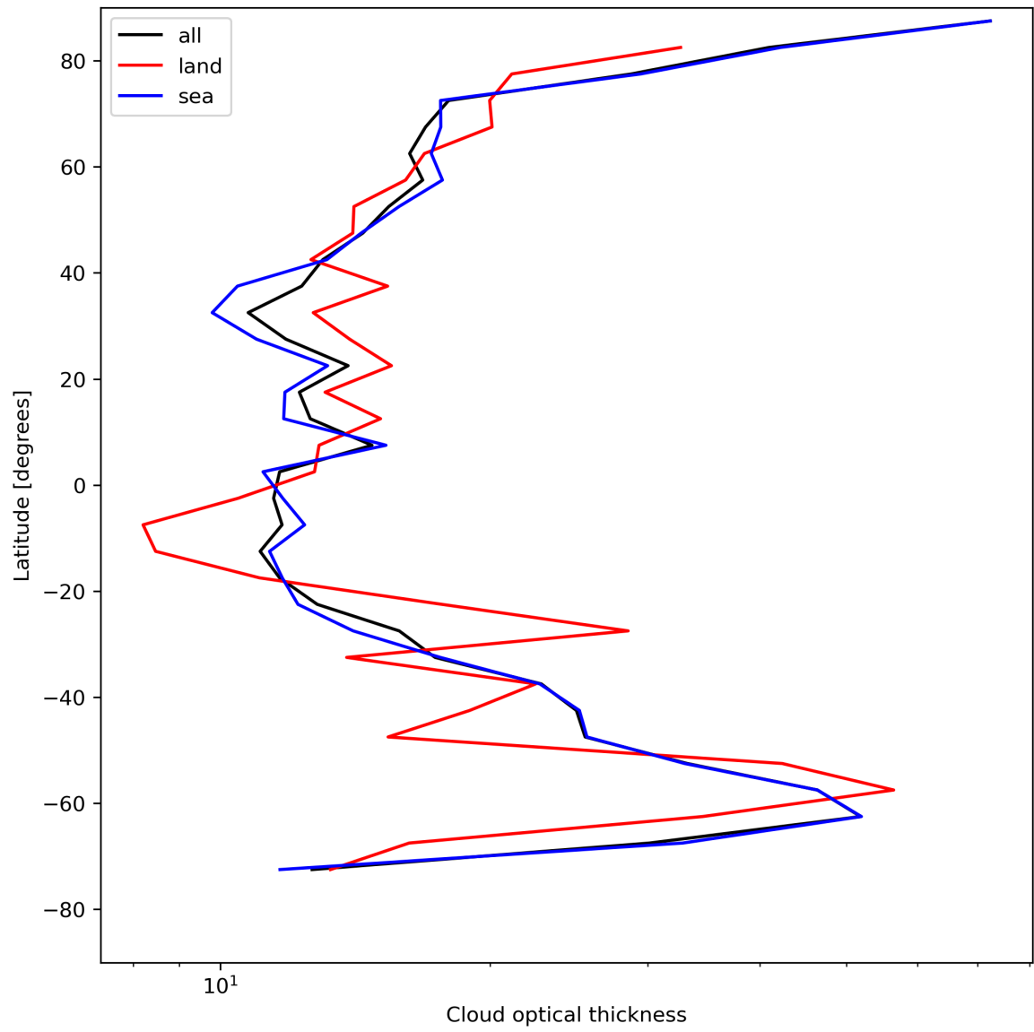
Figure 25: Zonal average of “Cloud optical thickness” for 2024-08-06 to 2024-08-08.
