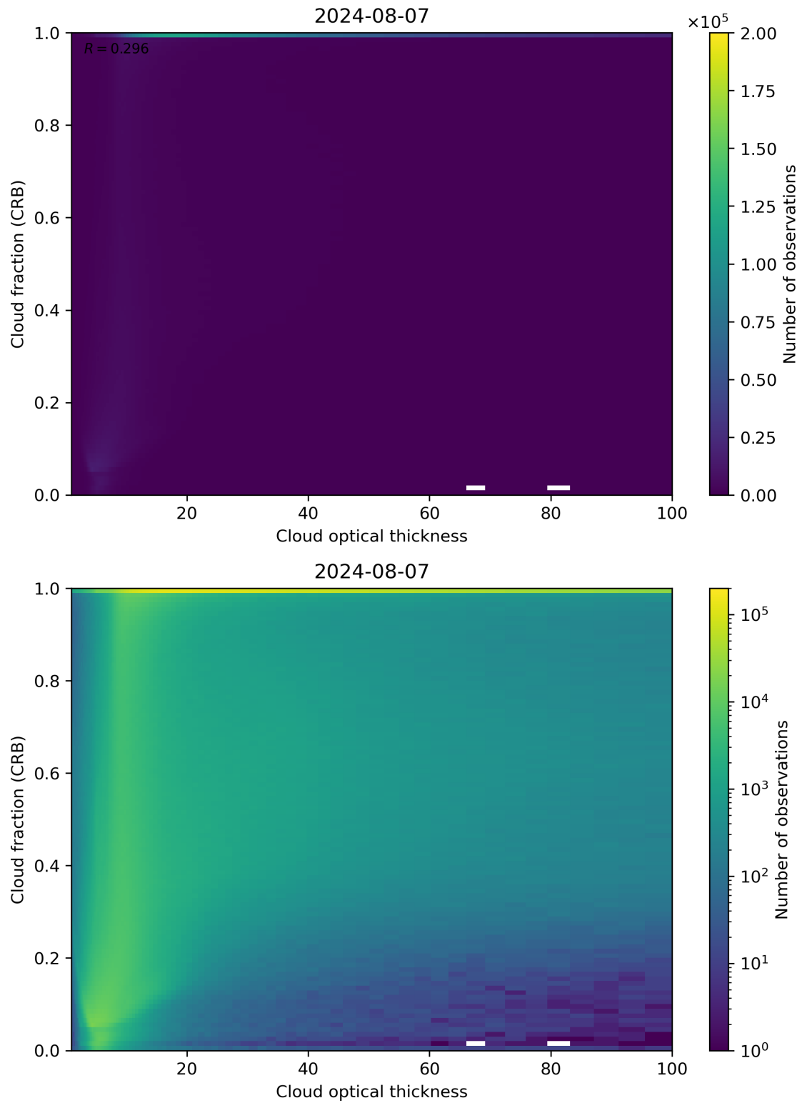
Figure 84: Scatter density plot of “Cloud optical thickness” against “Cloud fraction (CRB)” for 2024-08-06 to 2024-08-08.
