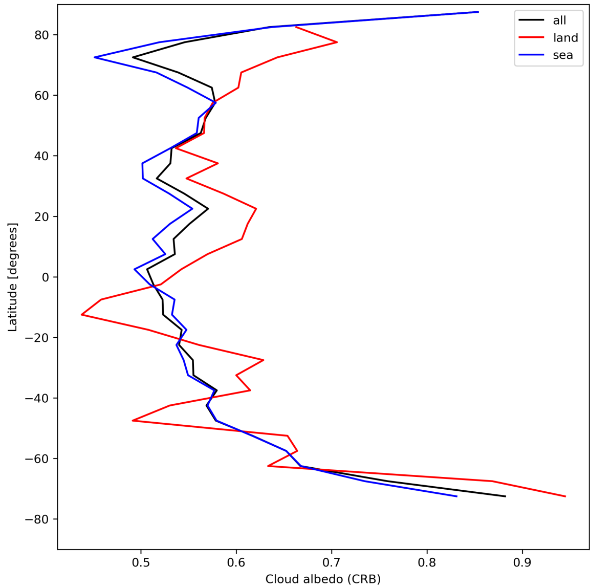
Figure 28: Zonal average of “Cloud albedo (CRB)” for 2024-08-06 to 2024-08-08.
