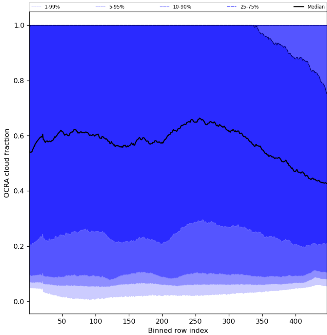
Figure 66: Along track statistics of “OCRA cloud fraction” for 2024-08-06 to 2024-08-08
