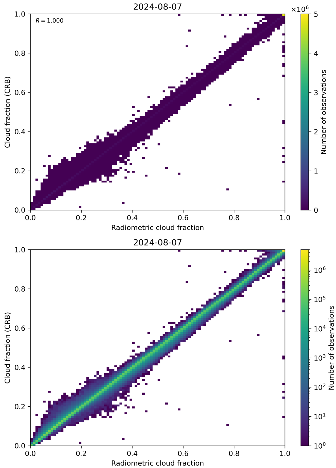
Figure 73: Scatter density plot of “Radiometric cloud fraction” against “Cloud fraction (CRB)” for 2024-08-06 to 2024-08-08.
