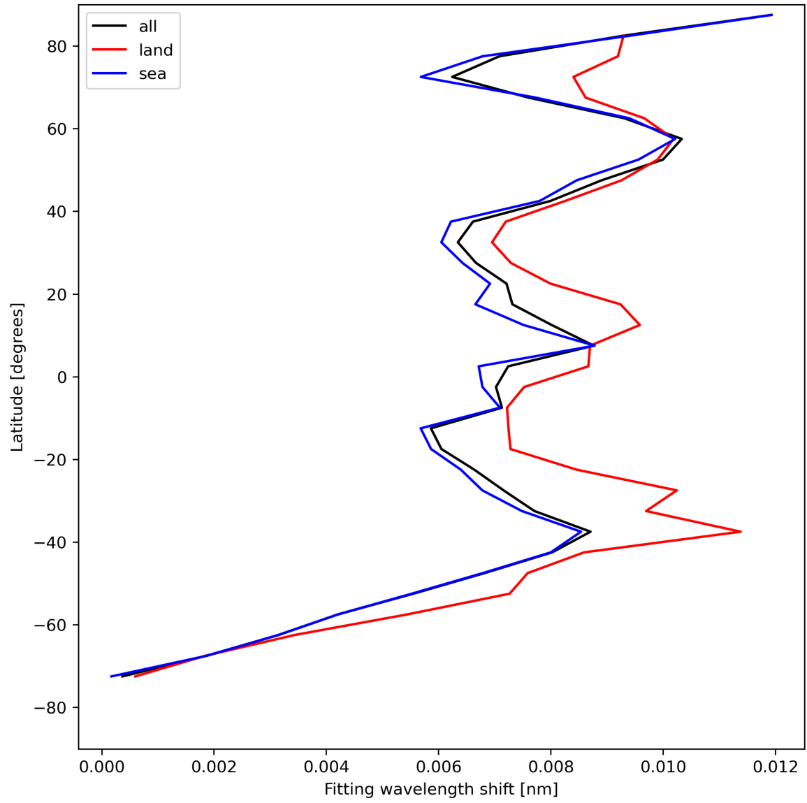
Figure 33: Zonal average of “Fitting wavelength shift” for 2024-08-06 to 2024-08-08.
