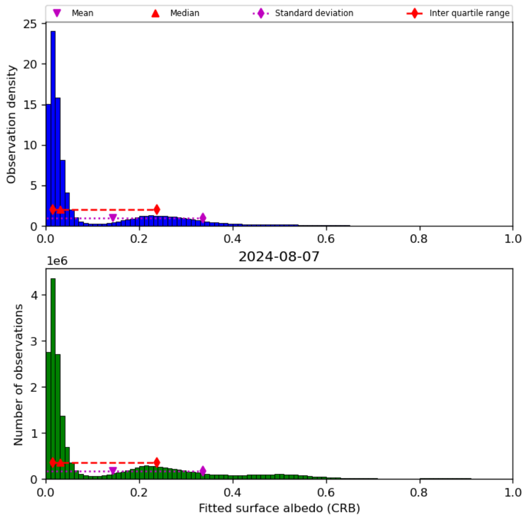
Figure 46: Histogram of “Fitted surface albedo (CRB)” for 2024-08-06 to 2024-08-08
