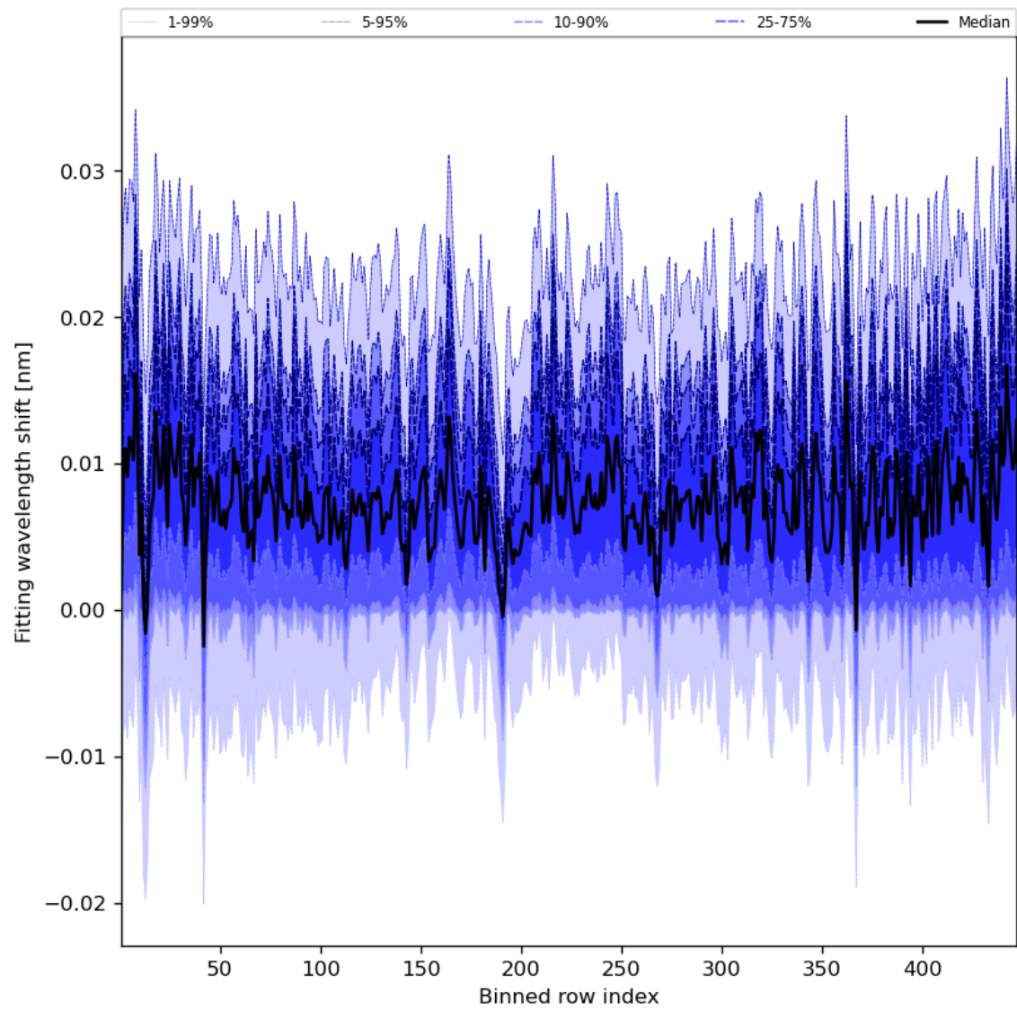
Figure 65: Along track statistics of “Fitting wavelength shift” for 2024-08-06 to 2024-08-08
