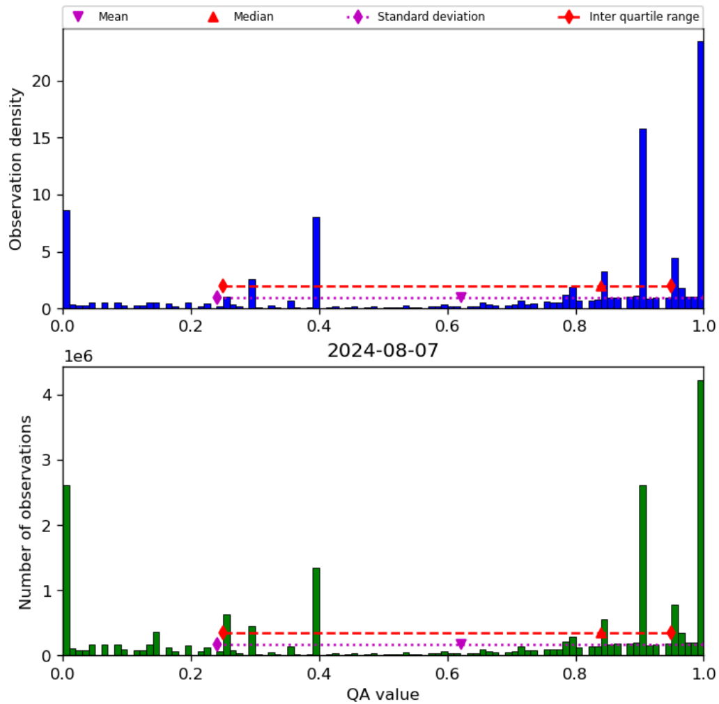
Figure 38: Histogram of “QA value” for 2024-08-06 to 2024-08-08
