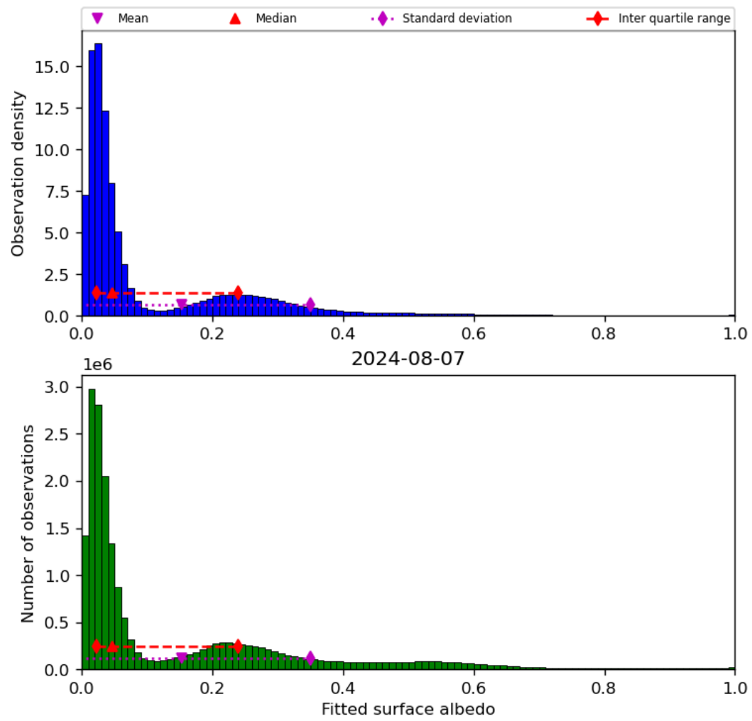
Figure 45: Histogram of “Fitted surface albedo” for 2024-08-06 to 2024-08-08
