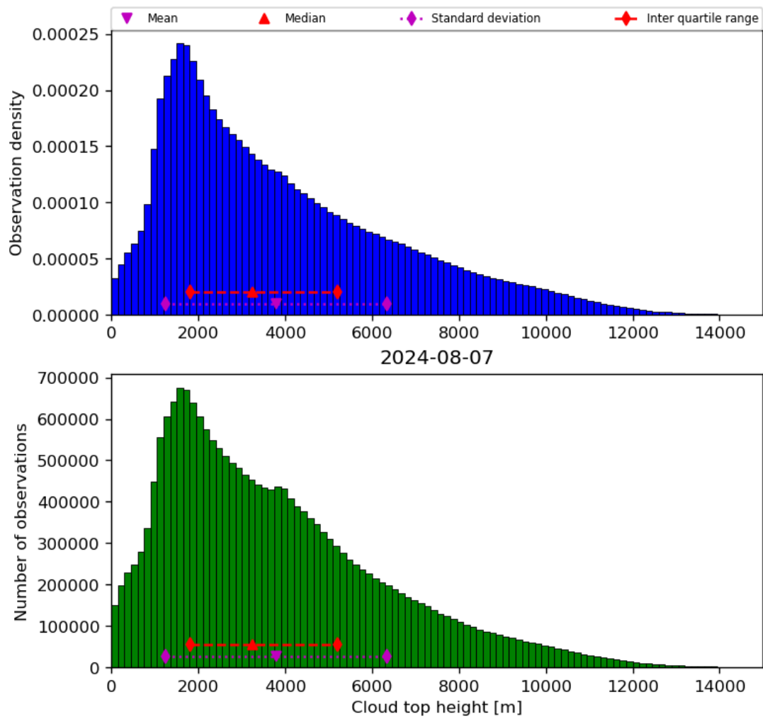
Figure 40: Histogram of “Cloud top height” for 2024-08-06 to 2024-08-08
