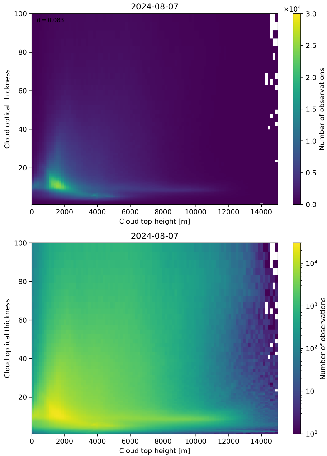
Figure 90: Scatter density plot of “Cloud top height” against “Cloud optical thickness” for 2024-08-06 to 2024-08-08.
