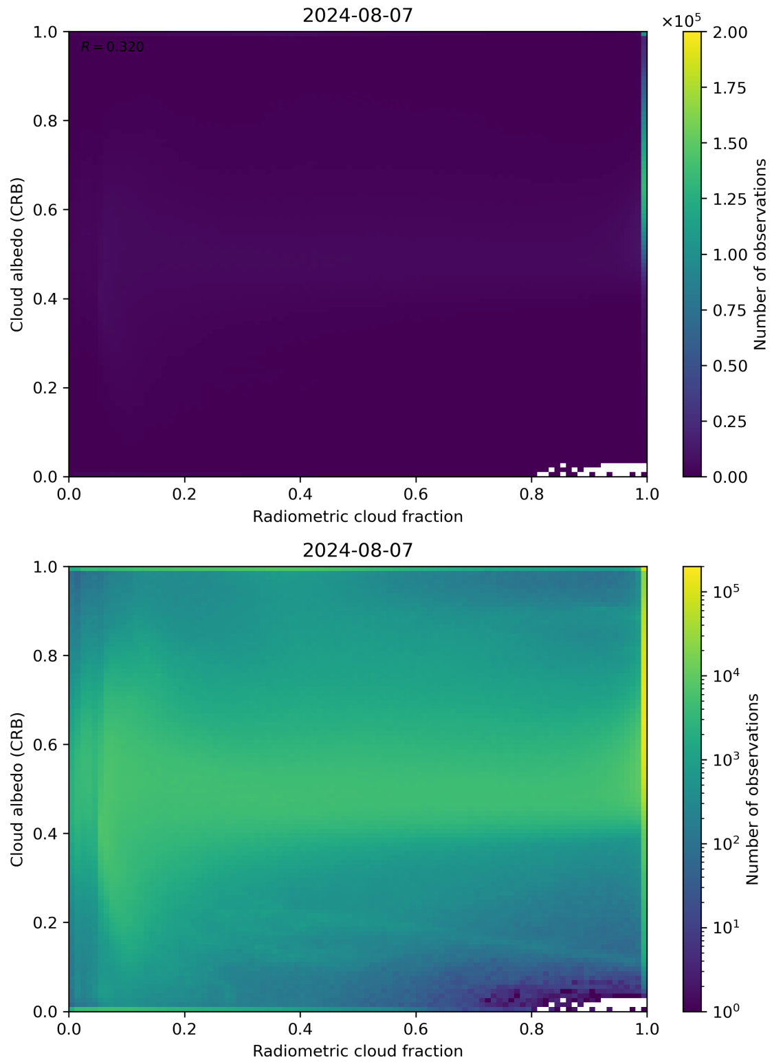
Figure 71: Scatter density plot of “Radiometric cloud fraction” against “Cloud albedo (CRB)” for 2024-08-06 to 2024-08-08.
