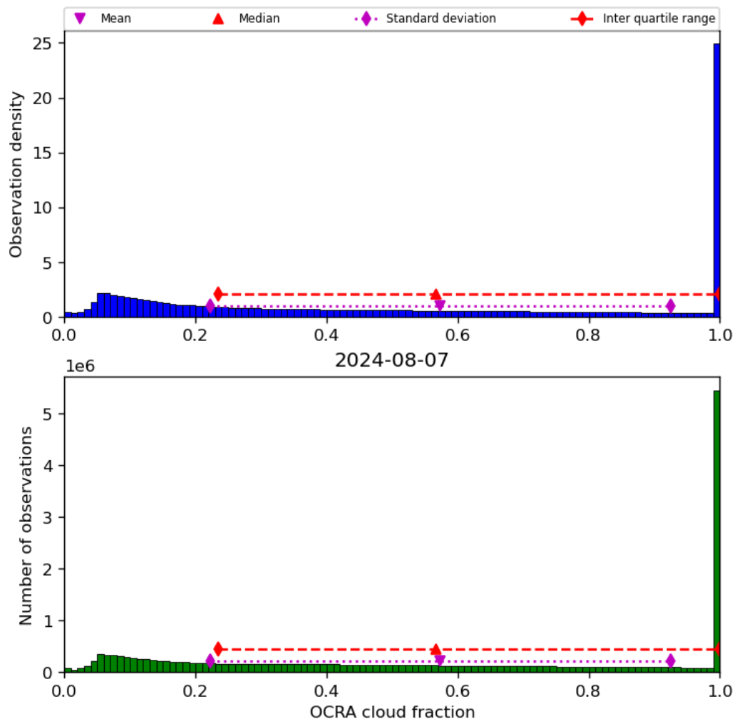
Figure 50: Histogram of “OCRA cloud fraction” for 2024-08-06 to 2024-08-08
