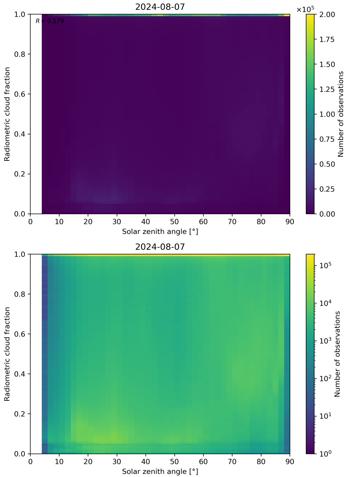
Figure 99: Scatter density plot of “Solar zenith angle” against “Radiometric cloud fraction” for 2024-08-06 to 2024-08-08.
