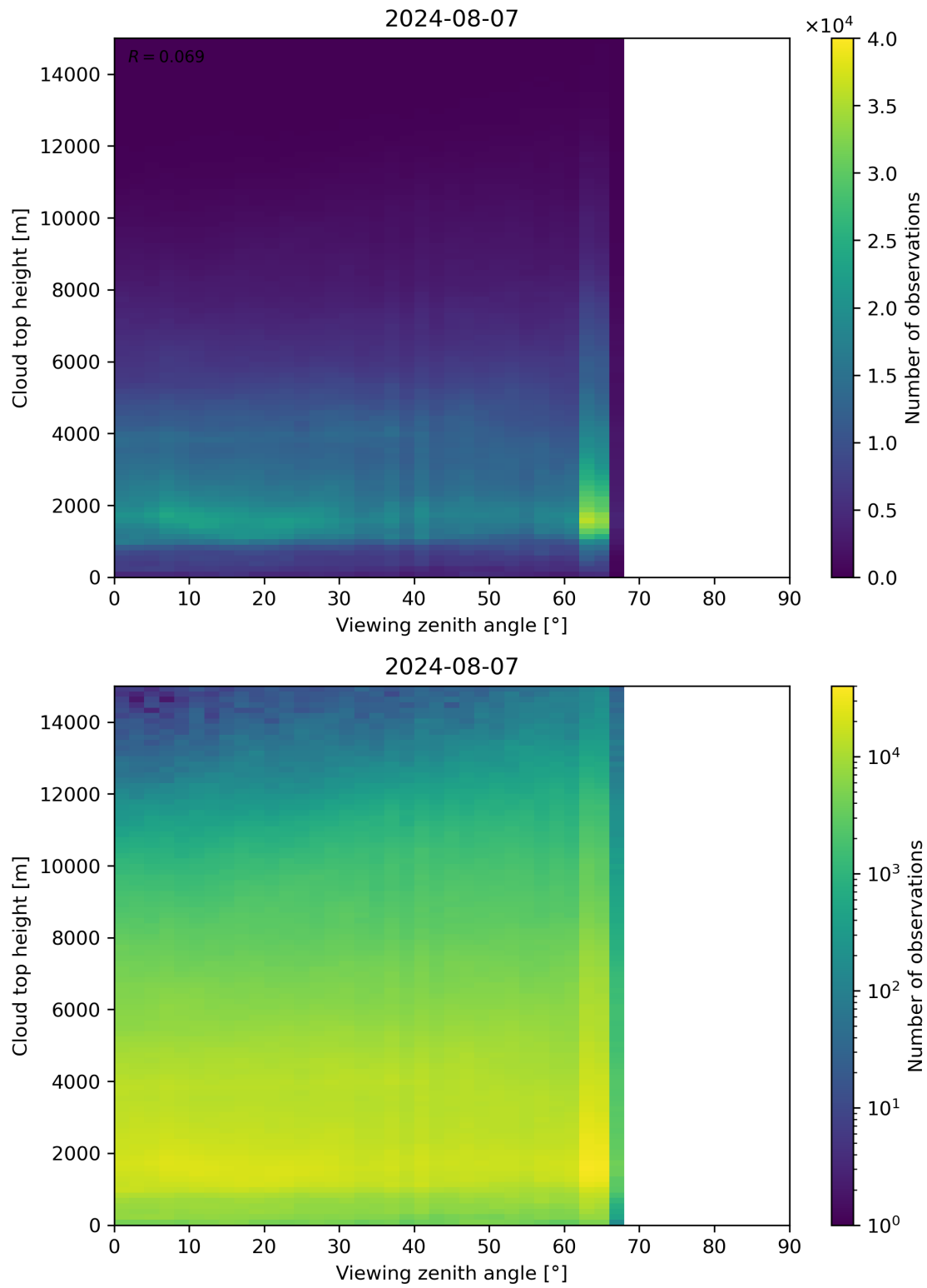
Figure 112: Scatter density plot of “Viewing zenith angle” against “Cloud top height” for 2024-08-06 to 2024-08-08.
