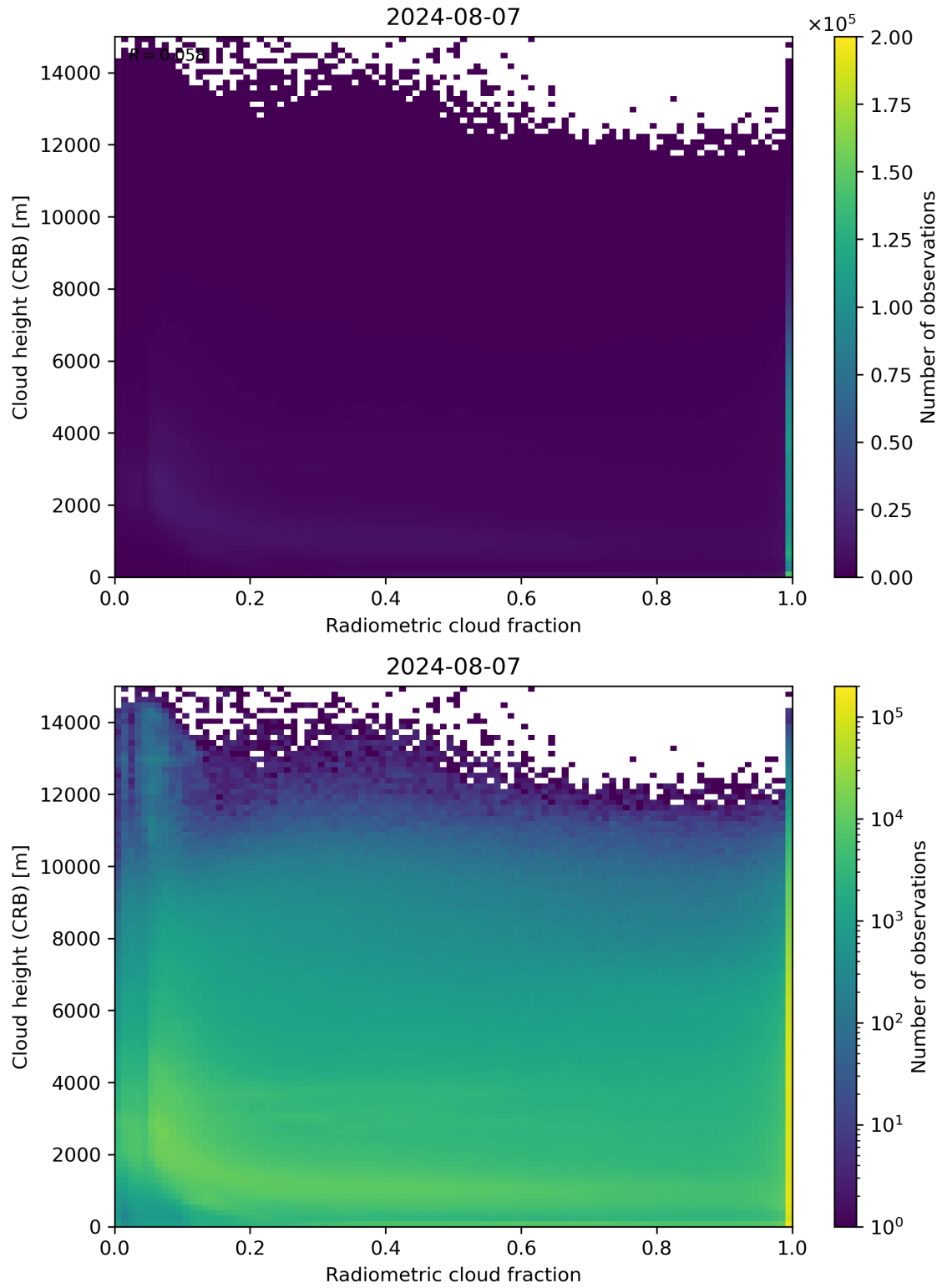
Figure 74: Scatter density plot of “Radiometric cloud fraction” against “Cloud height (CRB)” for 2024-08-06 to 2024-08-08.
