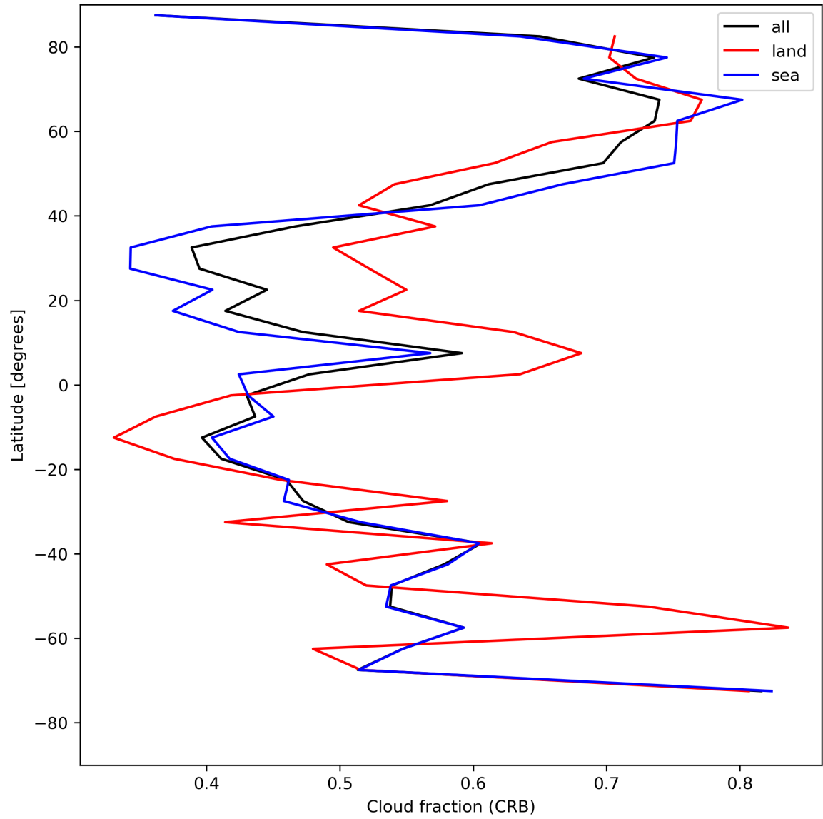
Figure 26: Zonal average of “Cloud fraction (CRB)” for 2024-08-06 to 2024-08-08.
