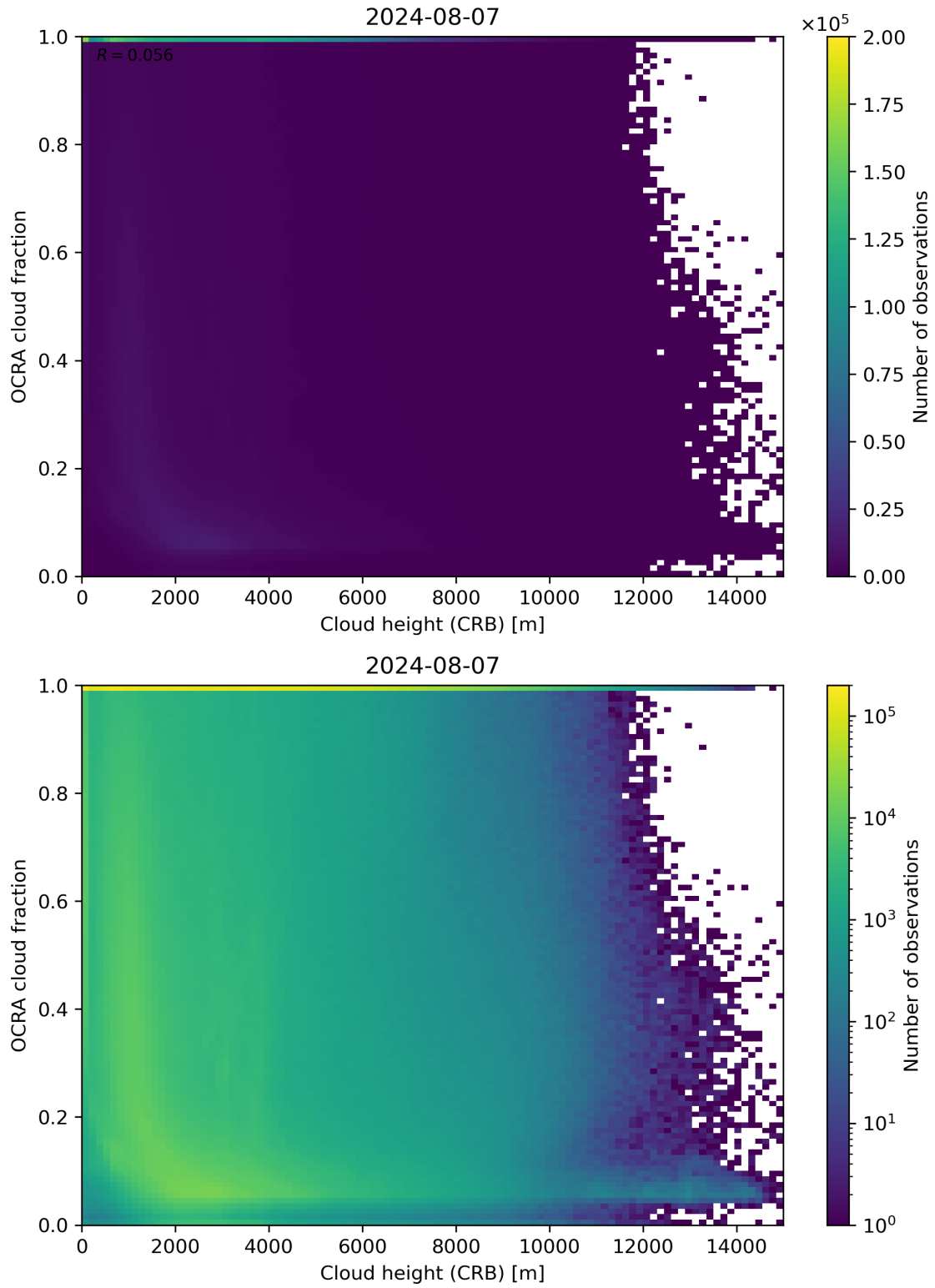
Figure 81: Scatter density plot of “Cloud height (CRB)” against “OCRA cloud fraction” for 2024-08-06 to 2024-08-08.
