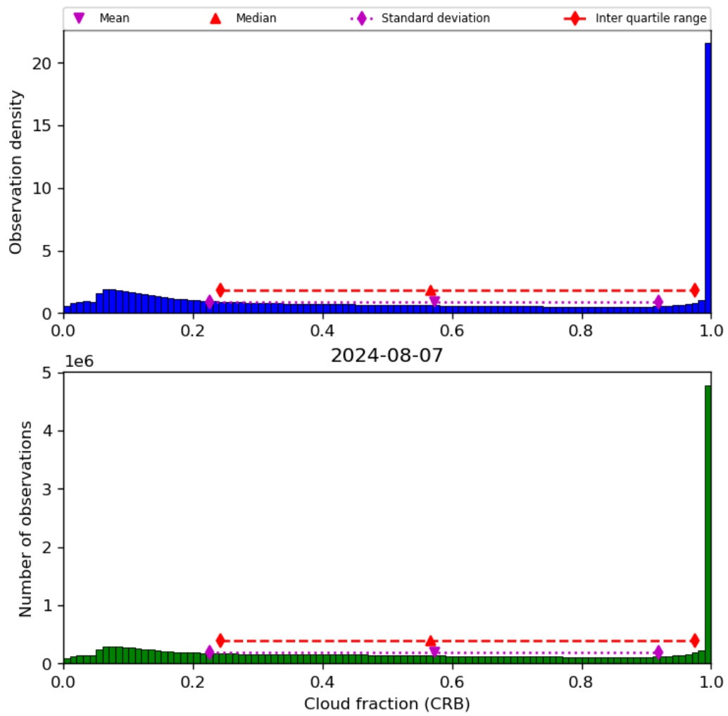
Figure 42: Histogram of “Cloud fraction (CRB)” for 2024-08-06 to 2024-08-08
