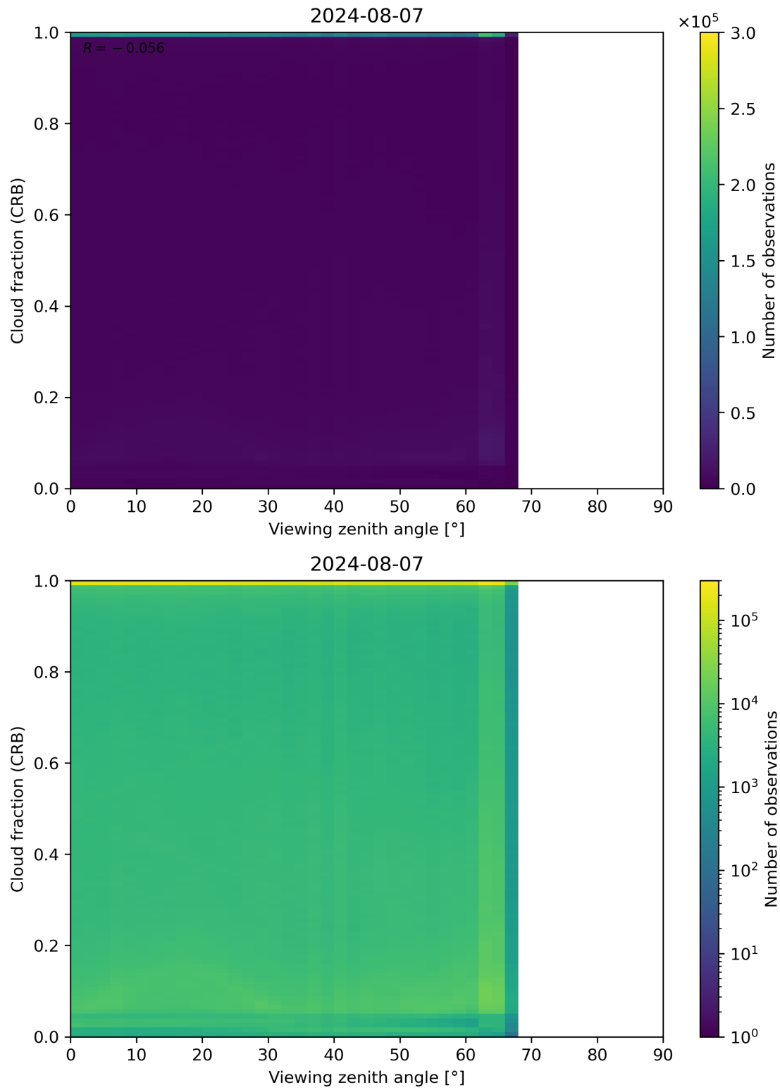
Figure 109: Scatter density plot of “Viewing zenith angle” against “Cloud fraction (CRB)” for 2024-08-06 to 2024-08-08.
