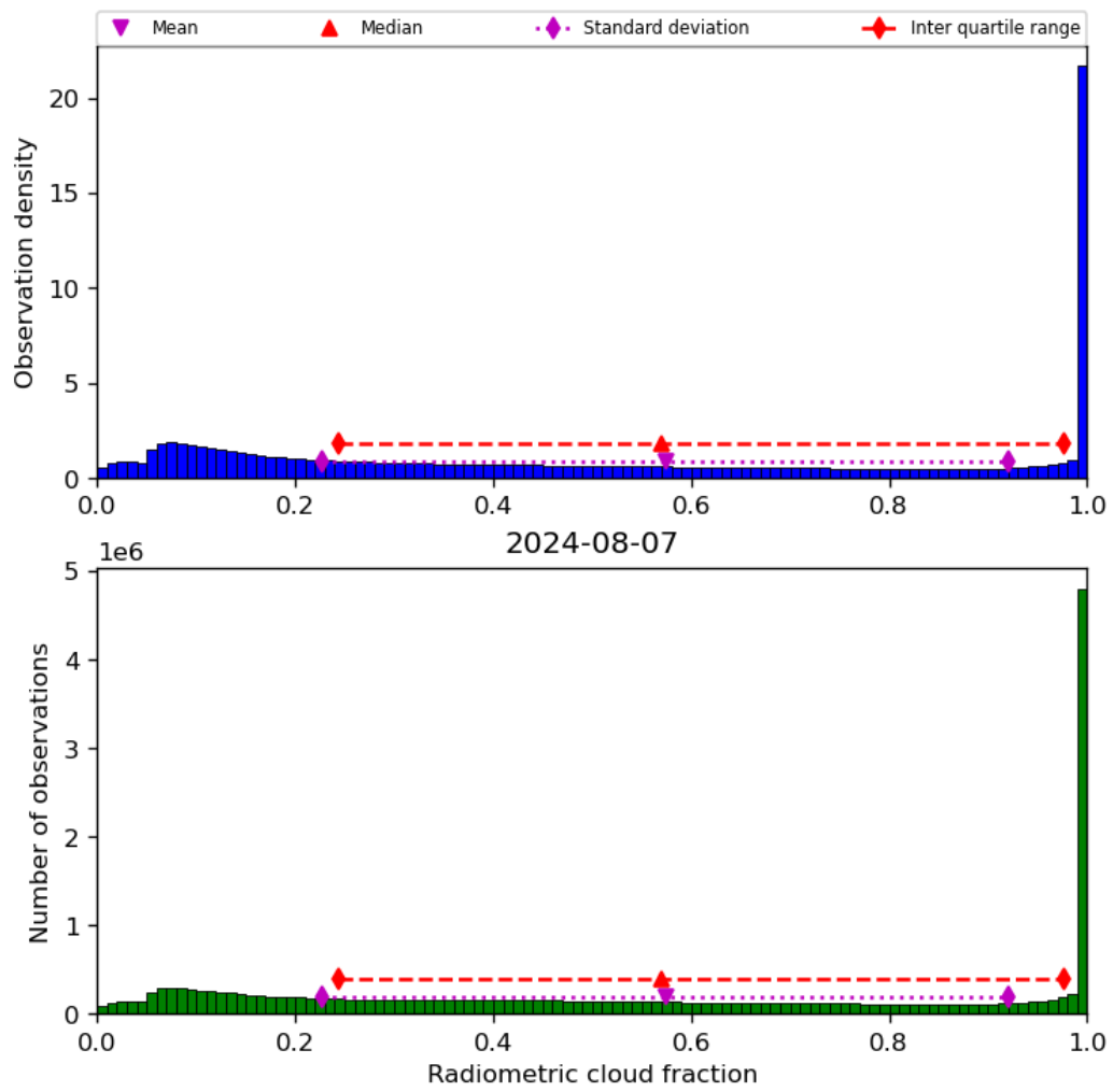
Figure 39: Histogram of “Radiometric cloud fraction” for 2024-08-06 to 2024-08-08
