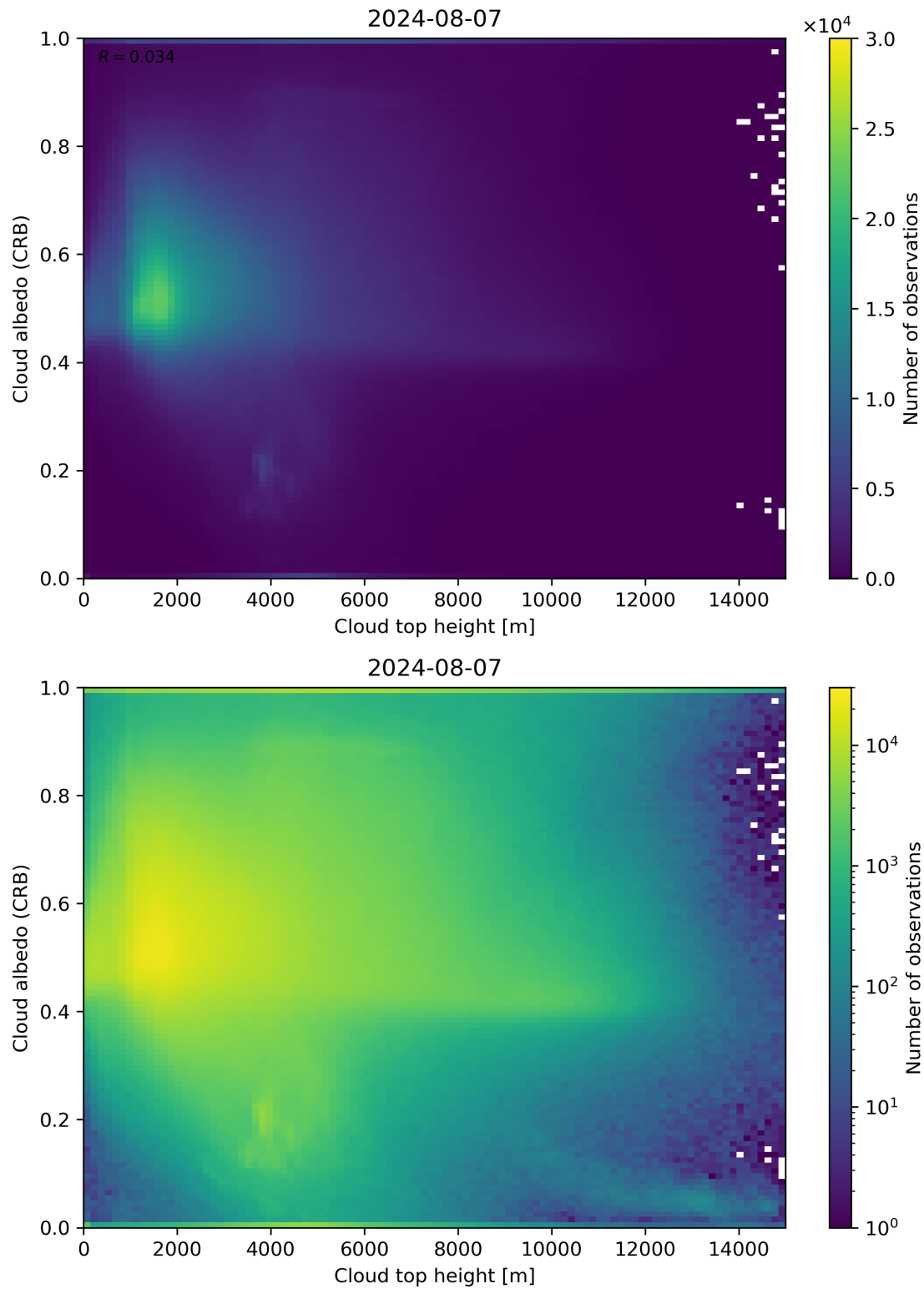
Figure 86: Scatter density plot of “Cloud top height” against “Cloud albedo (CRB)” for 2024-08-06 to 2024-08-08.
