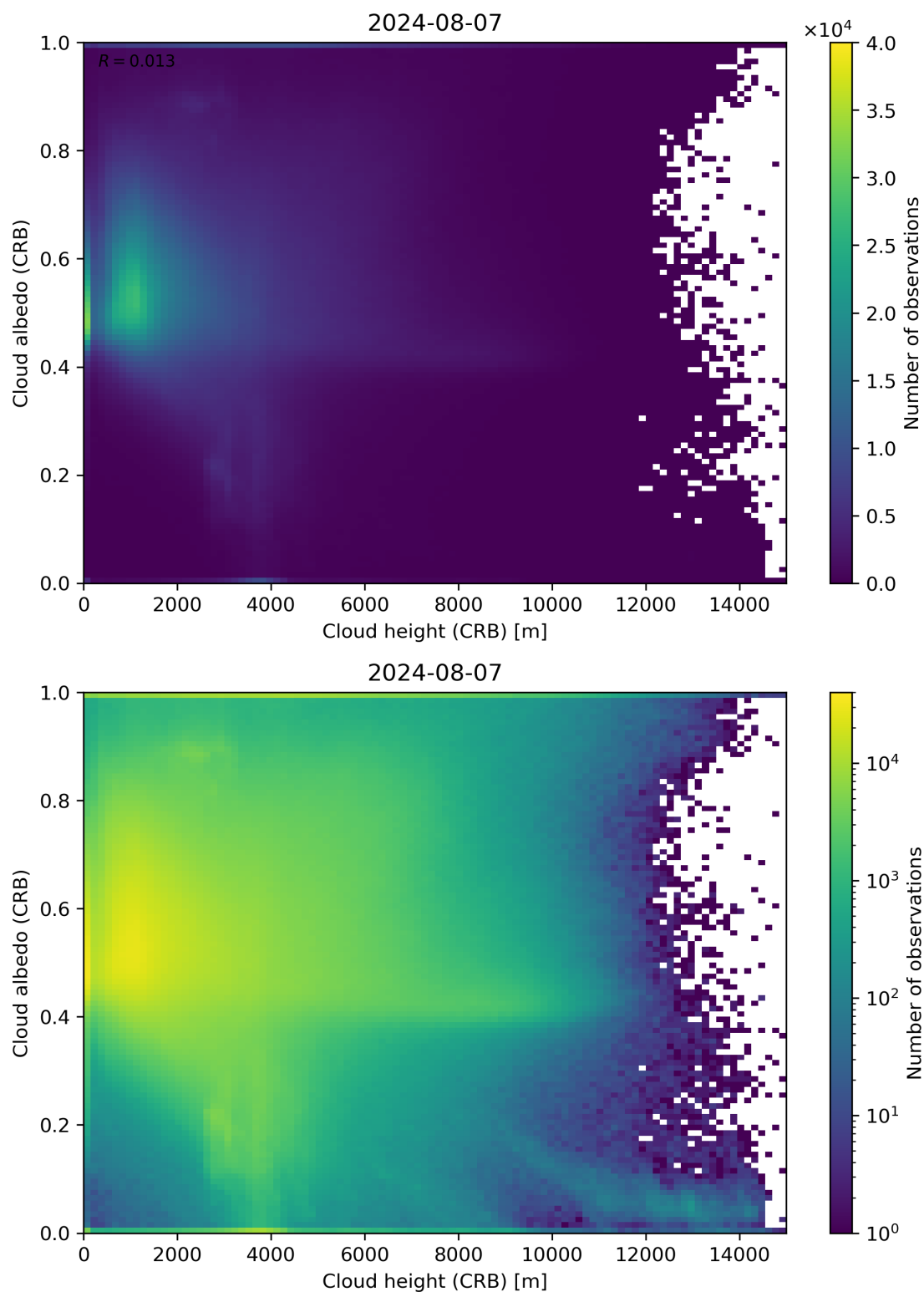
Figure 80: Scatter density plot of “Cloud height (CRB)” against “Cloud albedo (CRB)” for 2024-08-06 to 2024-08-08.
