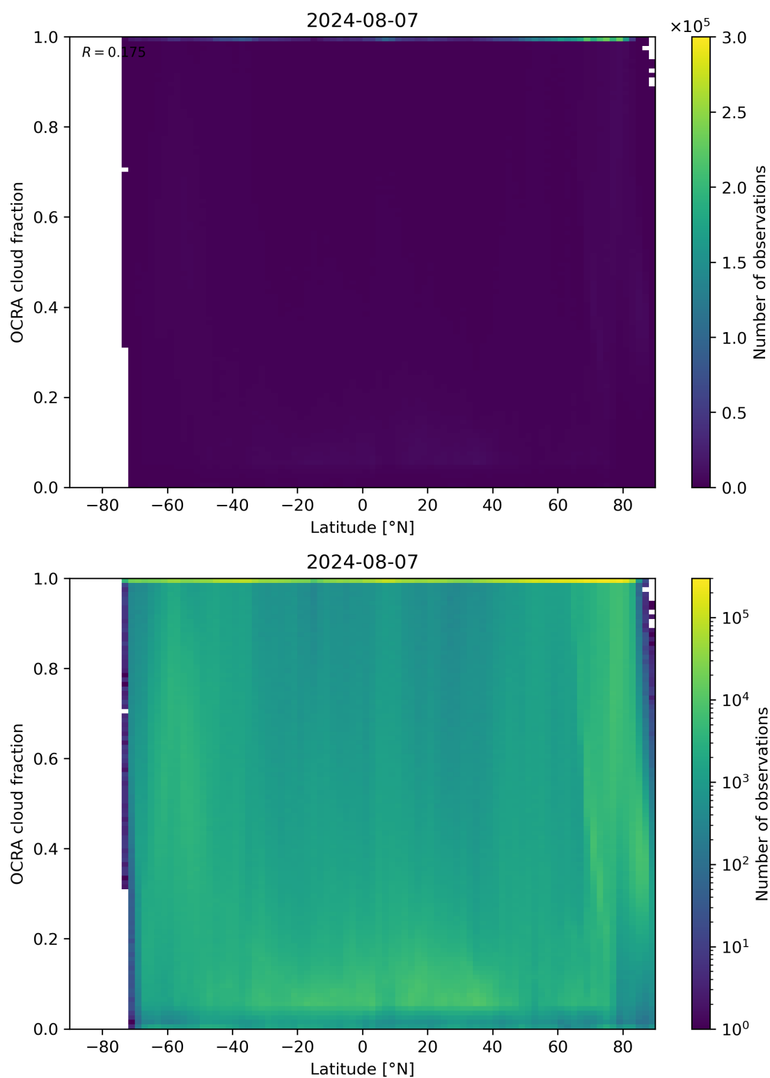
Figure 93: Scatter density plot of “Latitude” against “OCRA cloud fraction” for 2024-08-06 to 2024-08-08.
