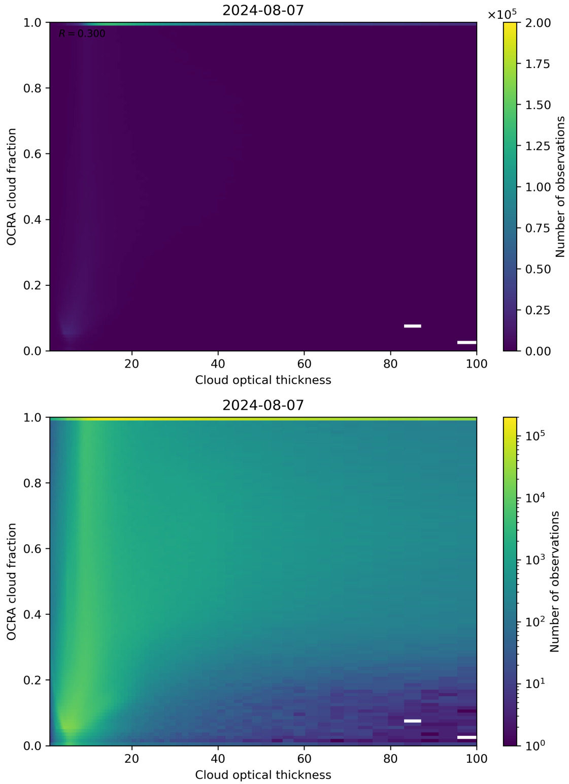
Figure 83: Scatter density plot of “Cloud optical thickness” against “OCRA cloud fraction” for 2024-08-06 to 2024-08-08.
