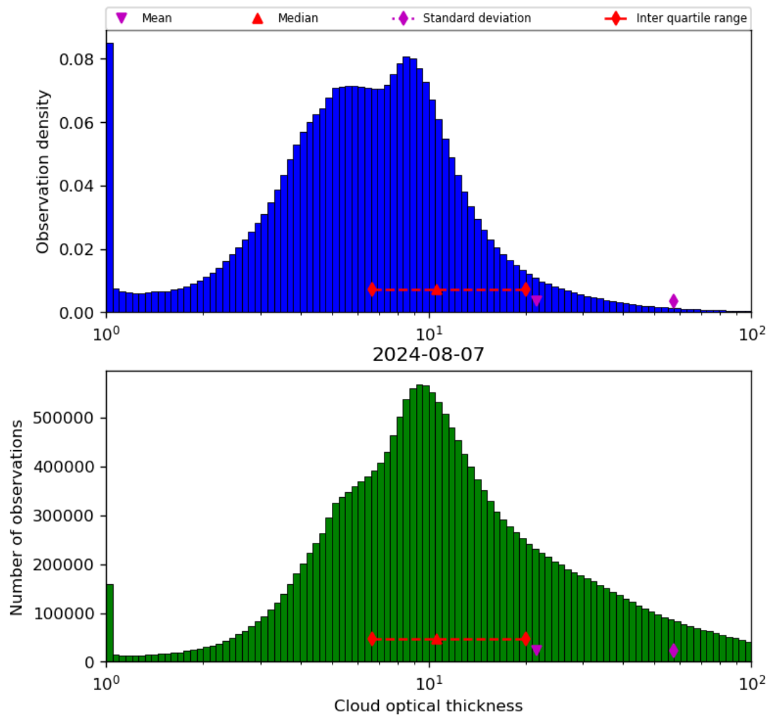
Figure 41: Histogram of “Cloud optical thickness” for 2024-08-06 to 2024-08-08
