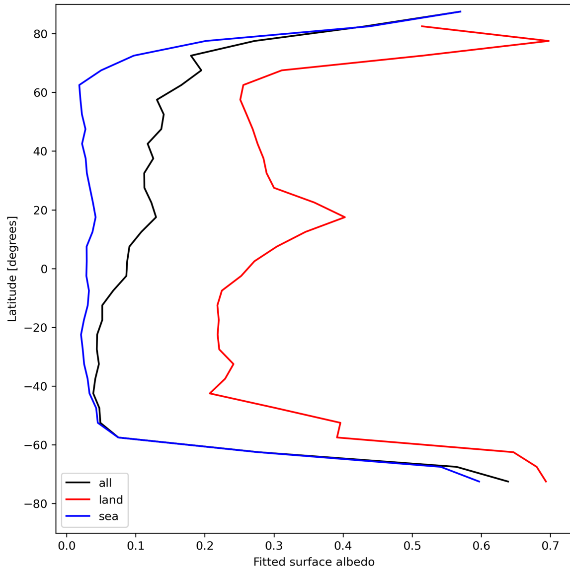
Figure 29: Zonal average of “Fitted surface albedo” for 2024-08-06 to 2024-08-08.
