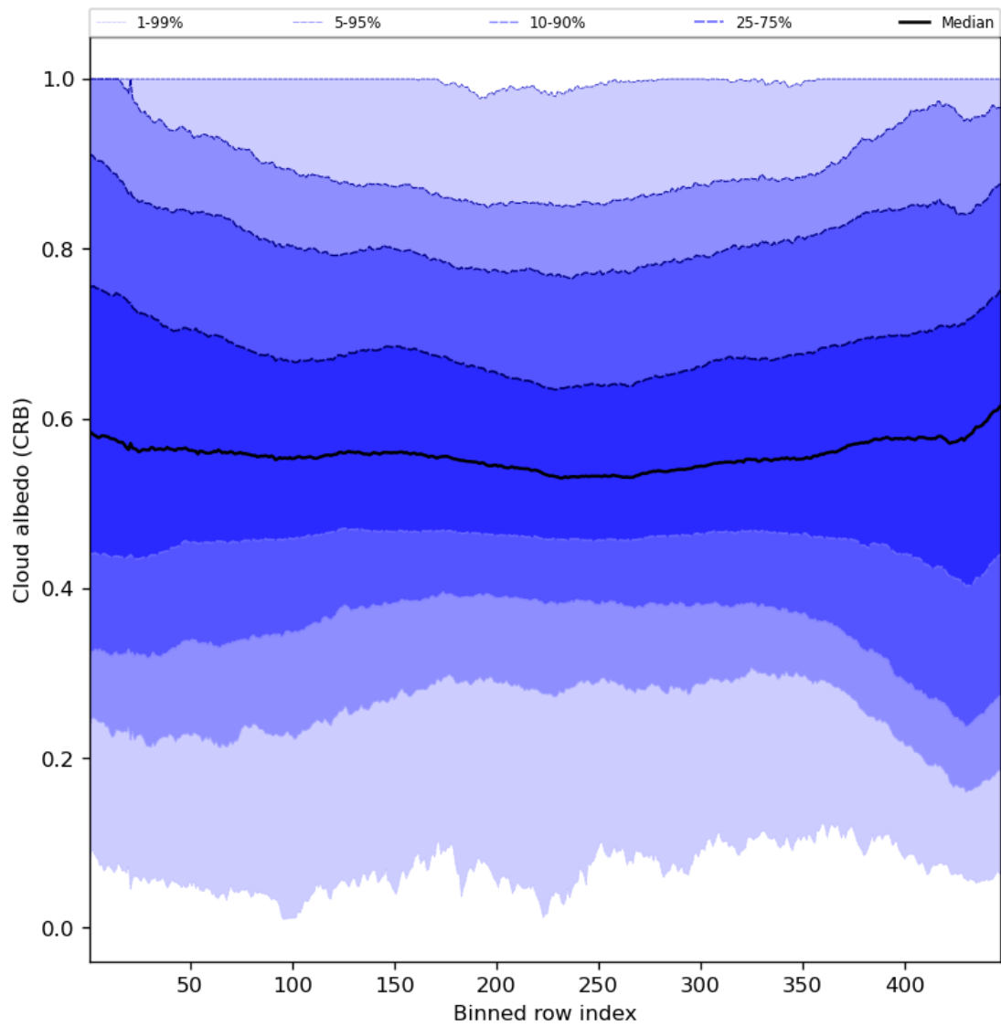
Figure 60: Along track statistics of “Cloud albedo (CRB)” for 2024-08-06 to 2024-08-08
