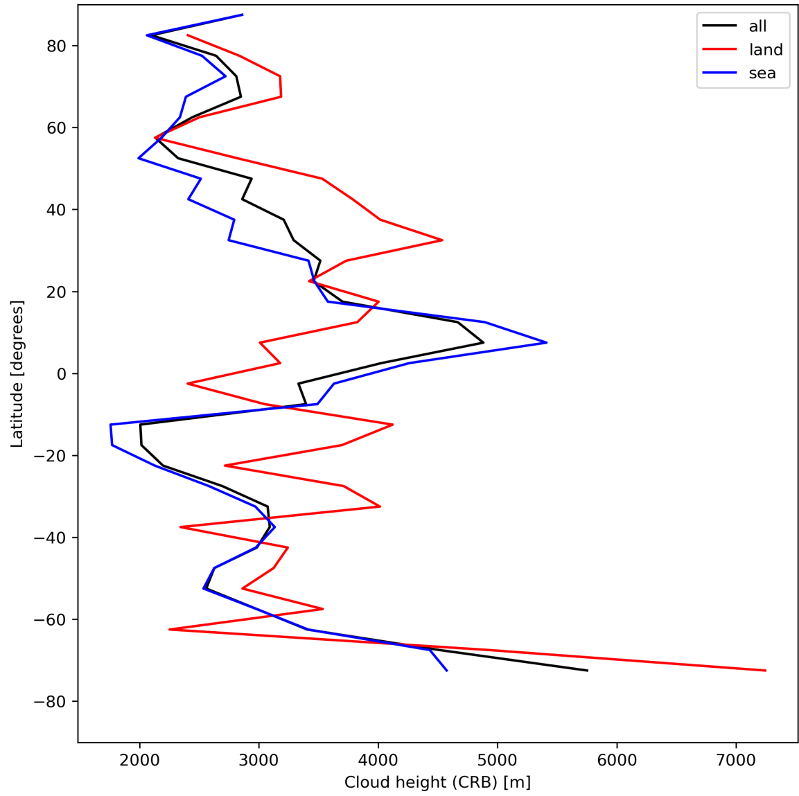
Figure 27: Zonal average of “Cloud height (CRB)” for 2024-08-06 to 2024-08-08.
