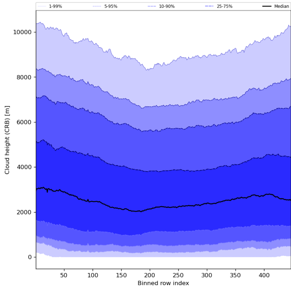
Figure 59: Along track statistics of “Cloud height (CRB)” for 2024-08-06 to 2024-08-08
