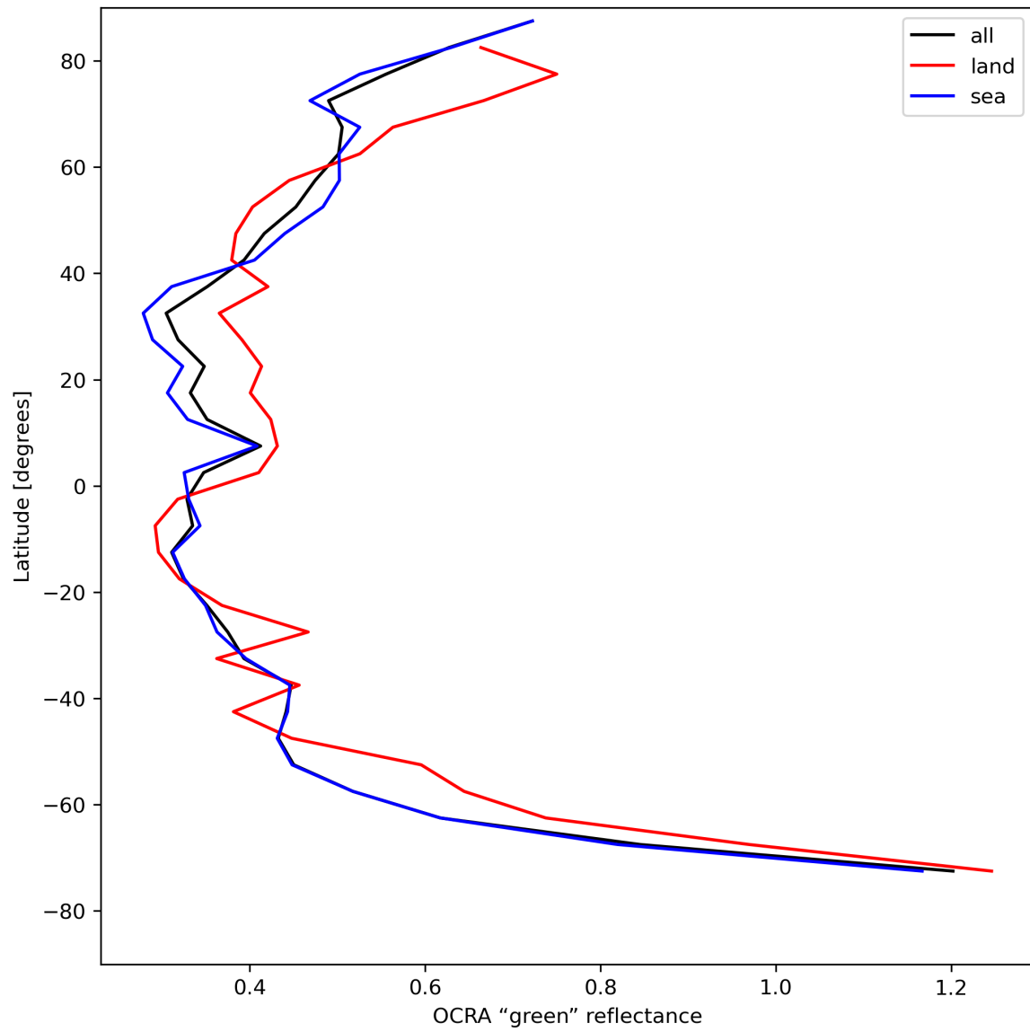
Figure 36: Zonal average of “OCRA “green” reflectance” for 2024-08-06 to 2024-08-08.
