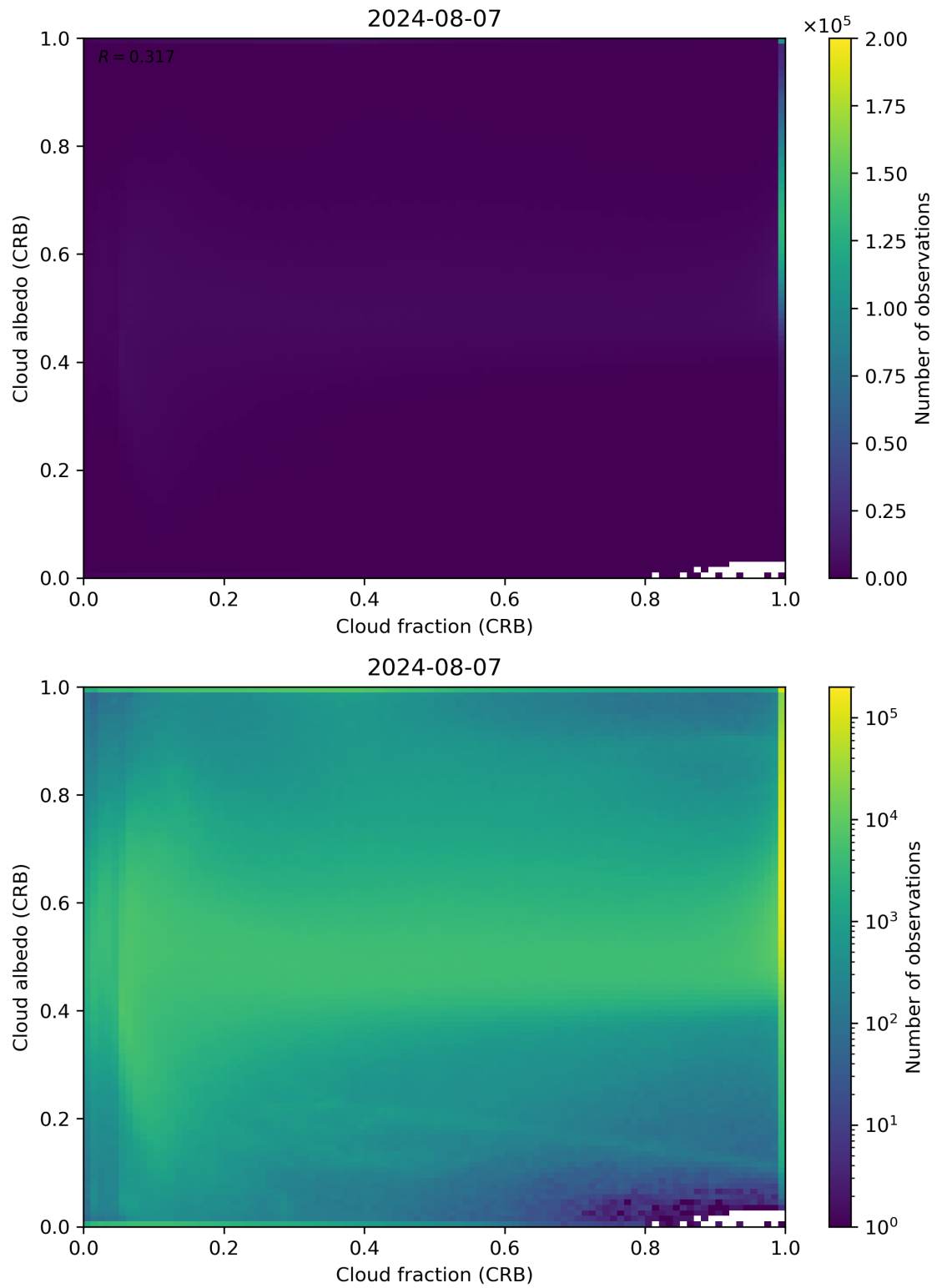
Figure 77: Scatter density plot of “Cloud fraction (CRB)” against “Cloud albedo (CRB)” for 2024-08-06 to 2024-08-08.
