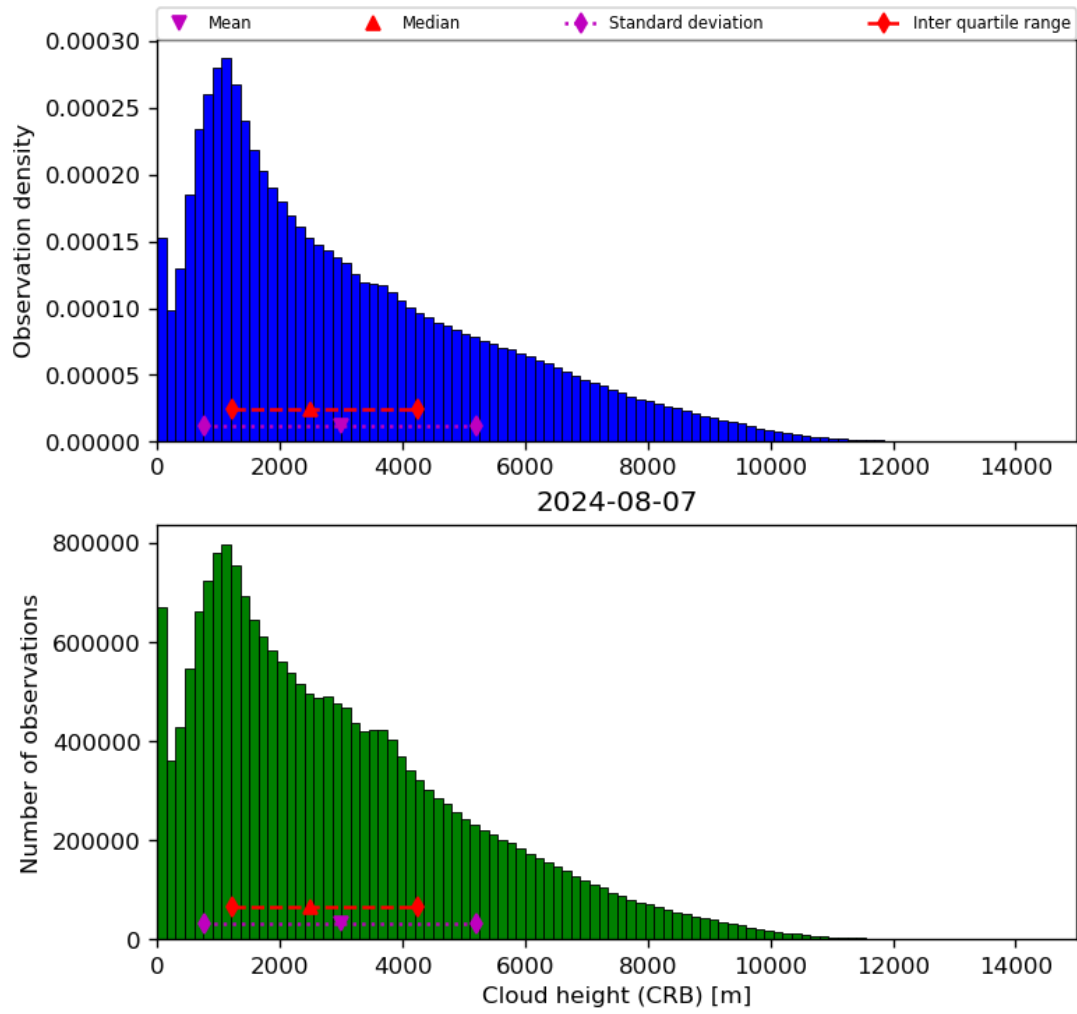
Figure 43: Histogram of “Cloud height (CRB)” for 2024-08-06 to 2024-08-08
