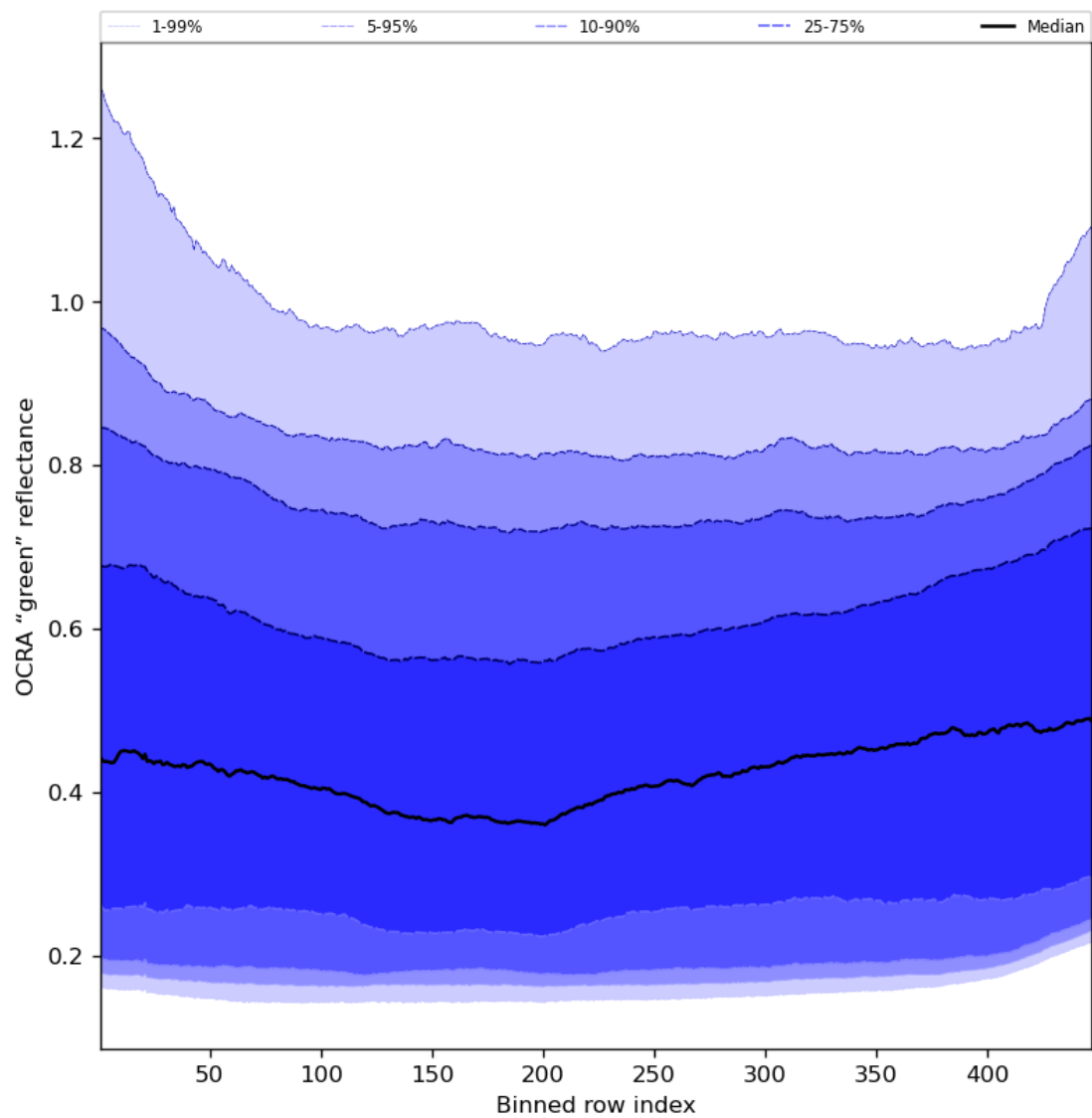
Figure 68: Along track statistics of “OCRA “green” reflectance” for 2024-08-06 to 2024-08-08
