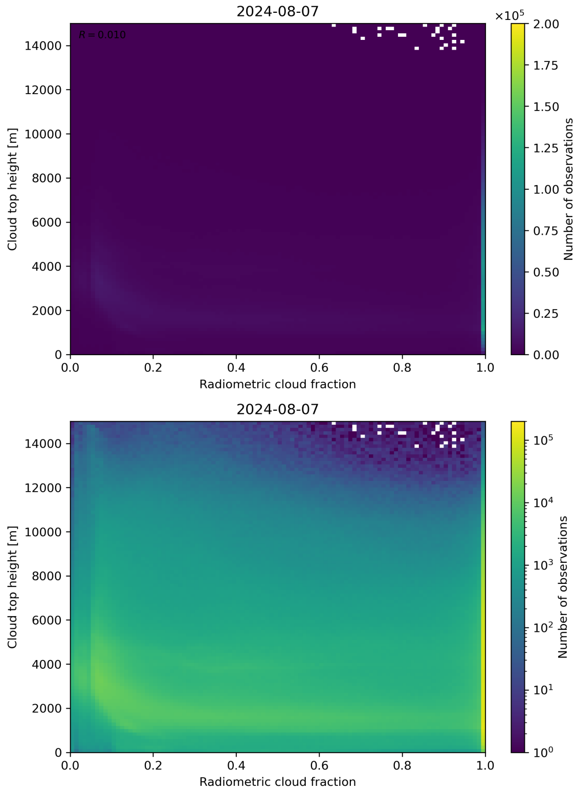
Figure 76: Scatter density plot of “Radiometric cloud fraction” against “Cloud top height” for 2024-08-06 to 2024-08-08.
