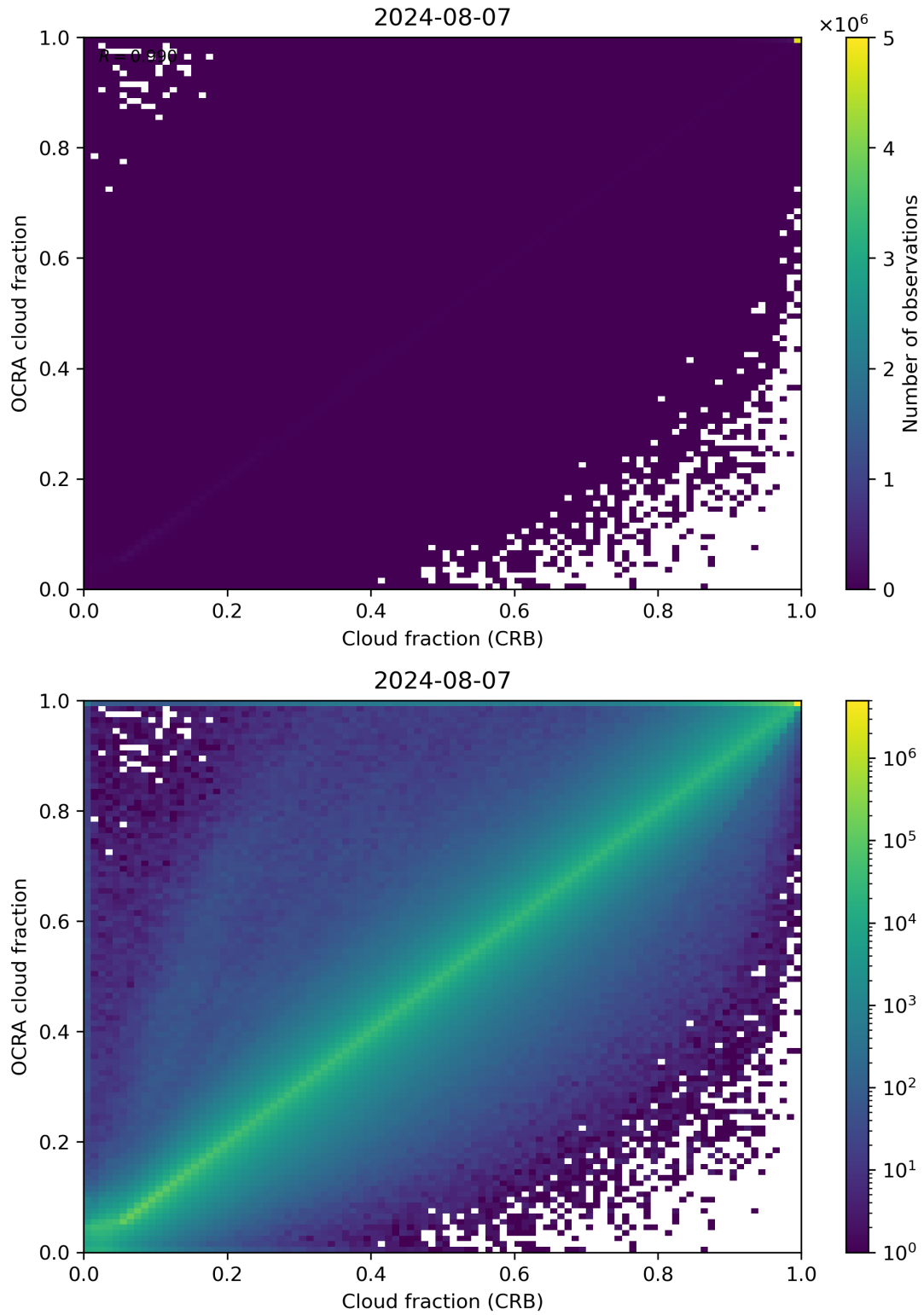
Figure 78: Scatter density plot of “Cloud fraction (CRB)” against “OCRA cloud fraction” for 2024-08-06 to 2024-08-08.
