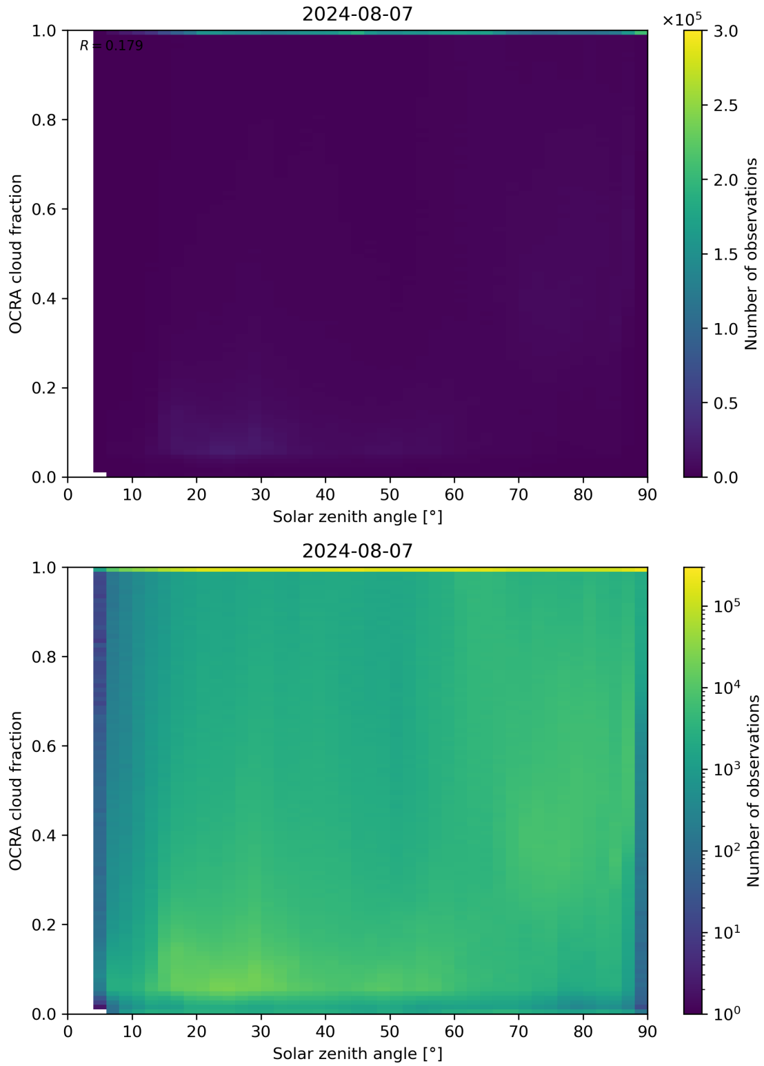
Figure 100: Scatter density plot of “Solar zenith angle” against “OCRA cloud fraction” for 2024-08-06 to 2024-08-08.
