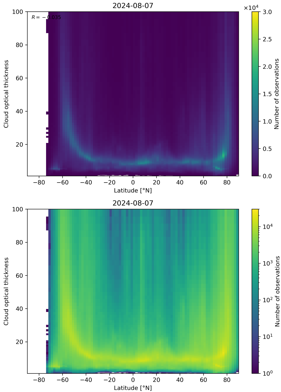
Figure 96: Scatter density plot of “Latitude” against “Cloud optical thickness” for 2024-08-06 to 2024-08-08.
