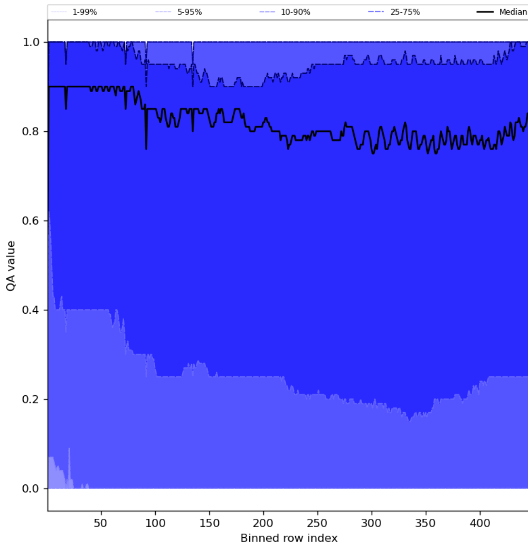
Figure 54: Along track statistics of “QA value” for 2024-08-06 to 2024-08-08
