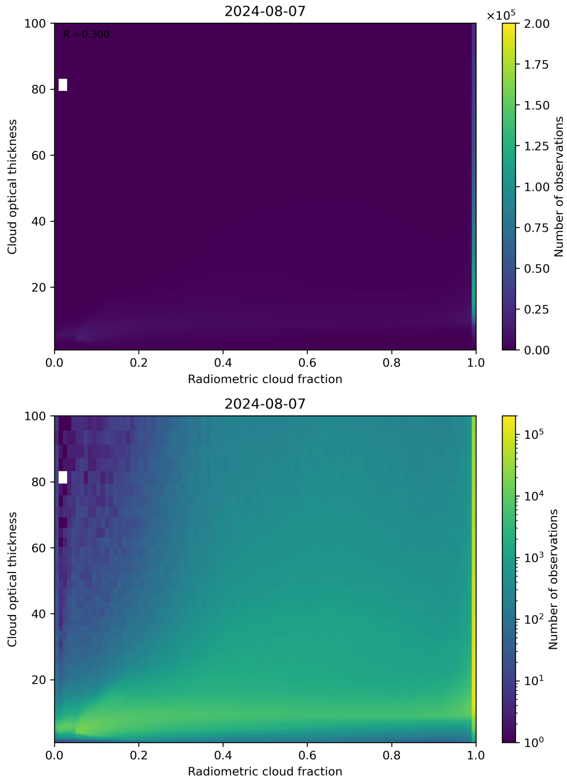
Figure 75: Scatter density plot of “Radiometric cloud fraction” against “Cloud optical thickness” for 2024-08-06 to 2024-08-08.
