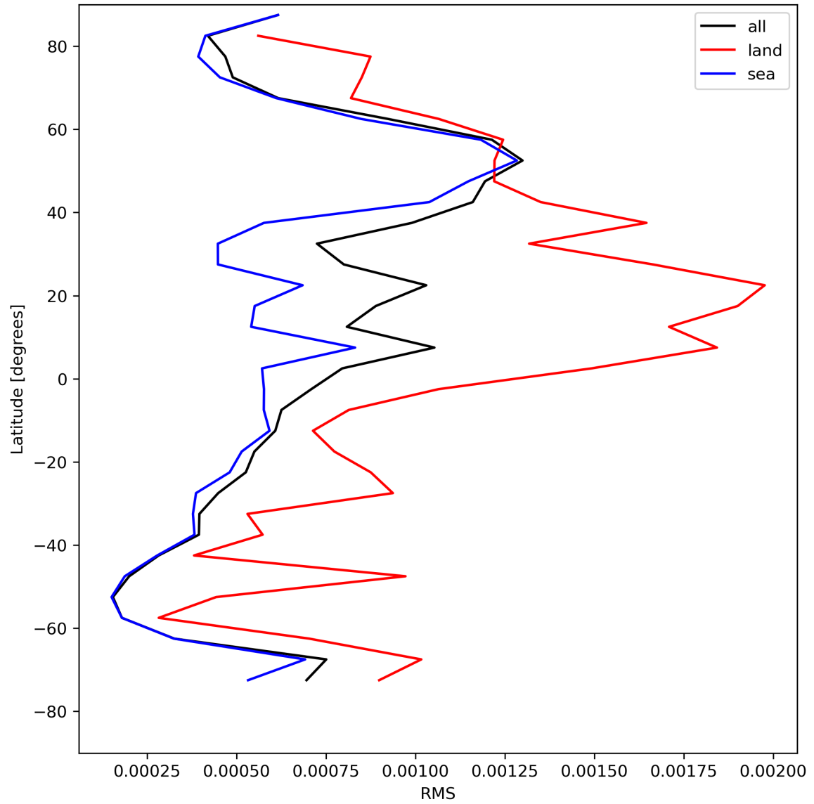
Figure 31: Zonal average of “RMS” for 2024-08-06 to 2024-08-08.
