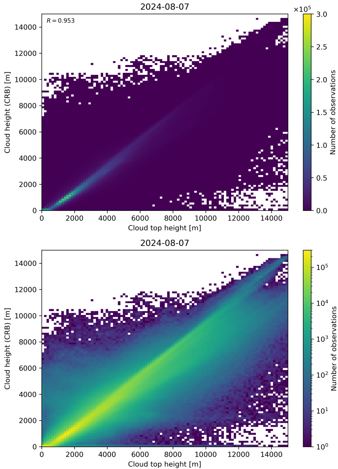
Figure 89: Scatter density plot of “Cloud top height” against “Cloud height (CRB)” for 2024-08-06 to 2024-08-08.
