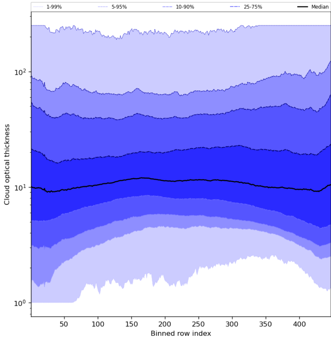
Figure 57: Along track statistics of “Cloud optical thickness” for 2024-08-06 to 2024-08-08
