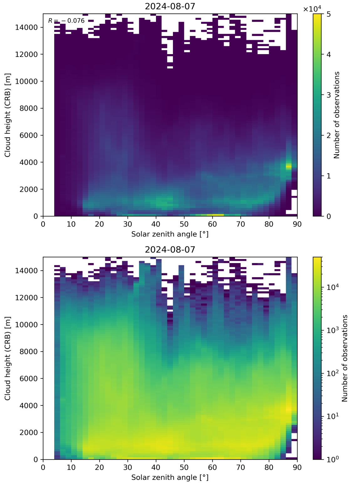
Figure 102: Scatter density plot of “Solar zenith angle” against “Cloud height (CRB)” for 2024-08-06 to 2024-08-08.
