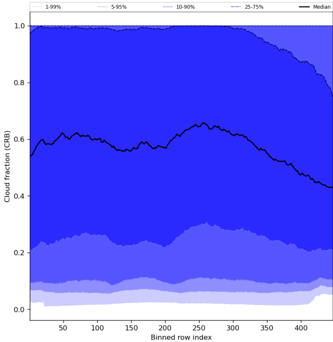
Figure 58: Along track statistics of “Cloud fraction (CRB)” for 2024-08-06 to 2024-08-08
