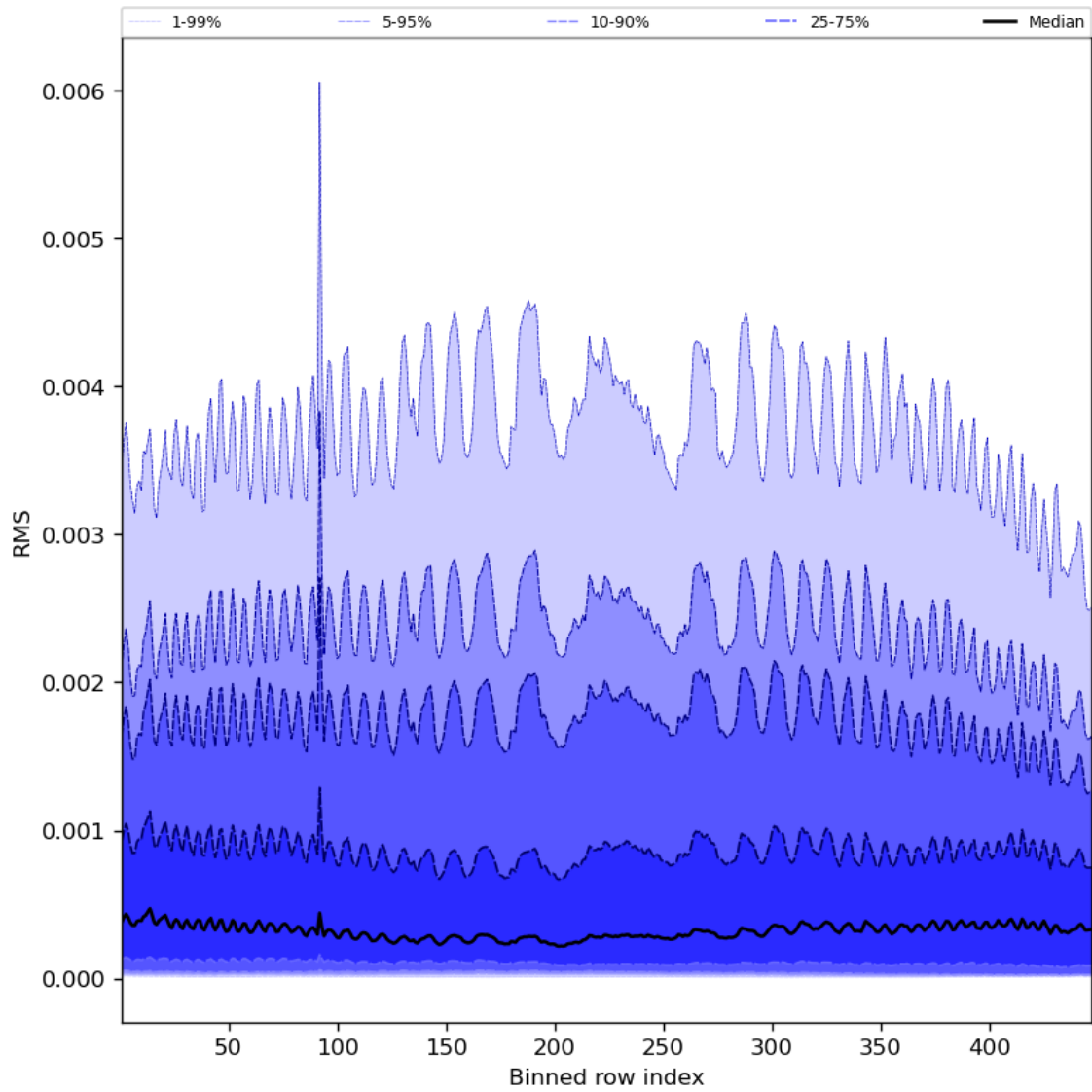
Figure 63: Along track statistics of “RMS” for 2024-08-06 to 2024-08-08
