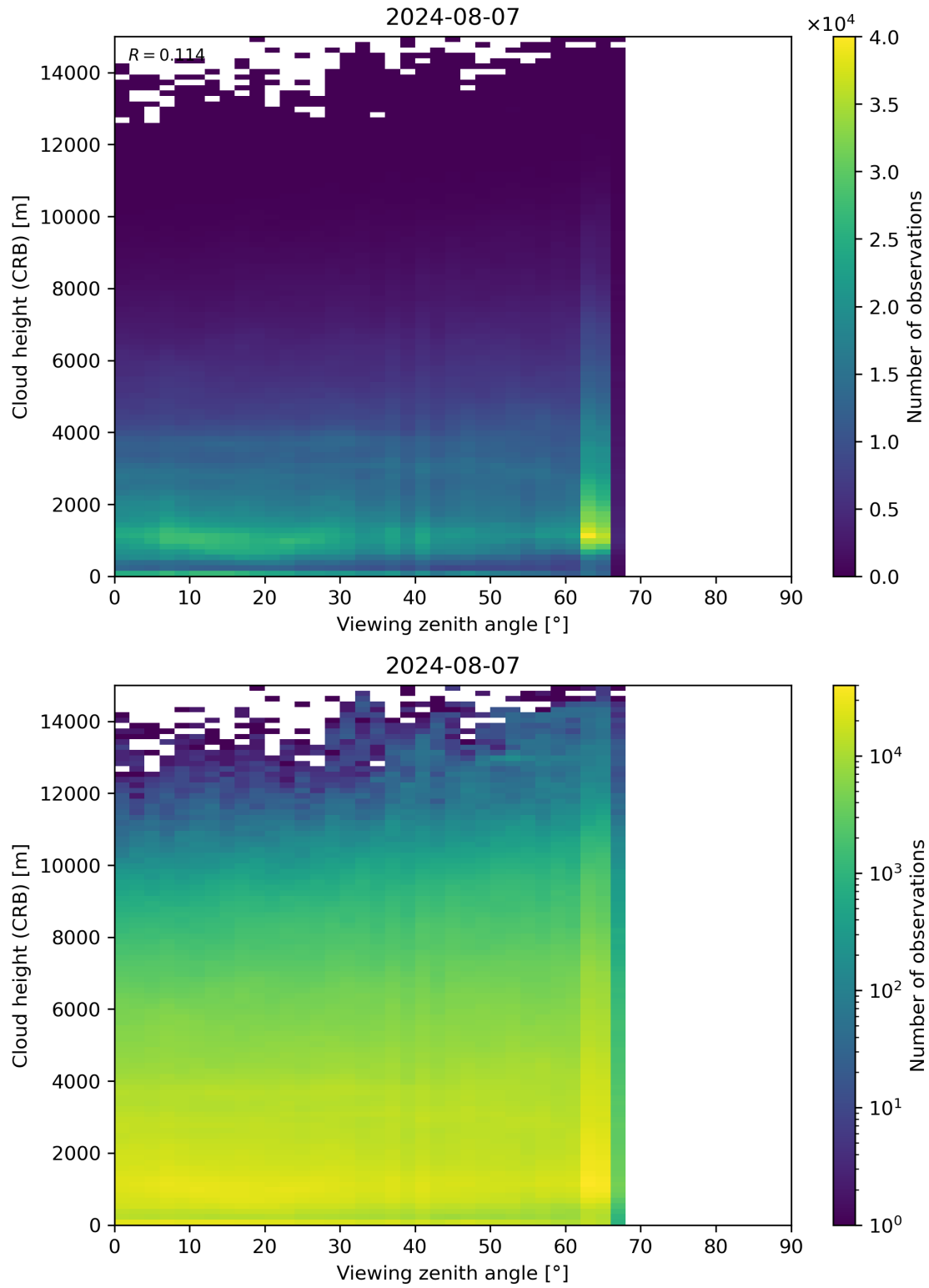
Figure 110: Scatter density plot of “Viewing zenith angle” against “Cloud height (CRB)” for 2024-08-06 to 2024-08-08.
