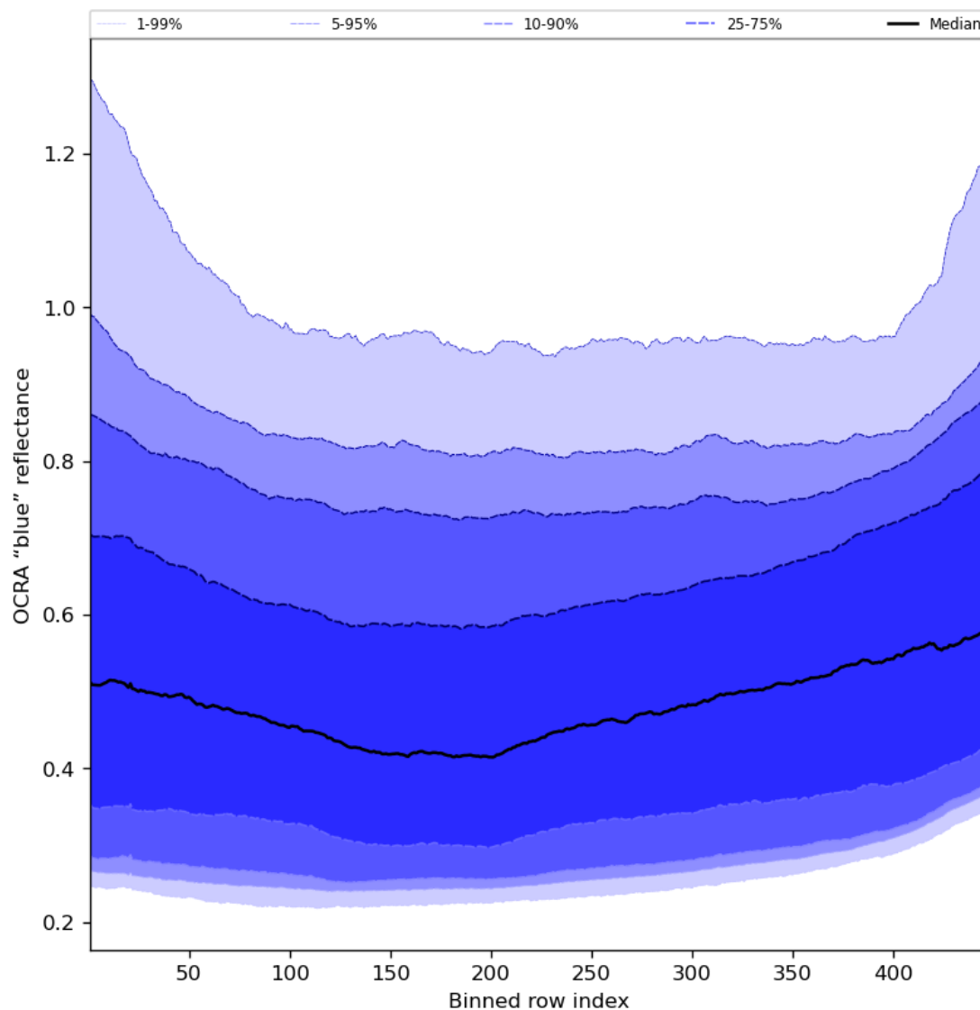
Figure 67: Along track statistics of “OCRA “blue” reflectance” for 2024-08-06 to 2024-08-08
