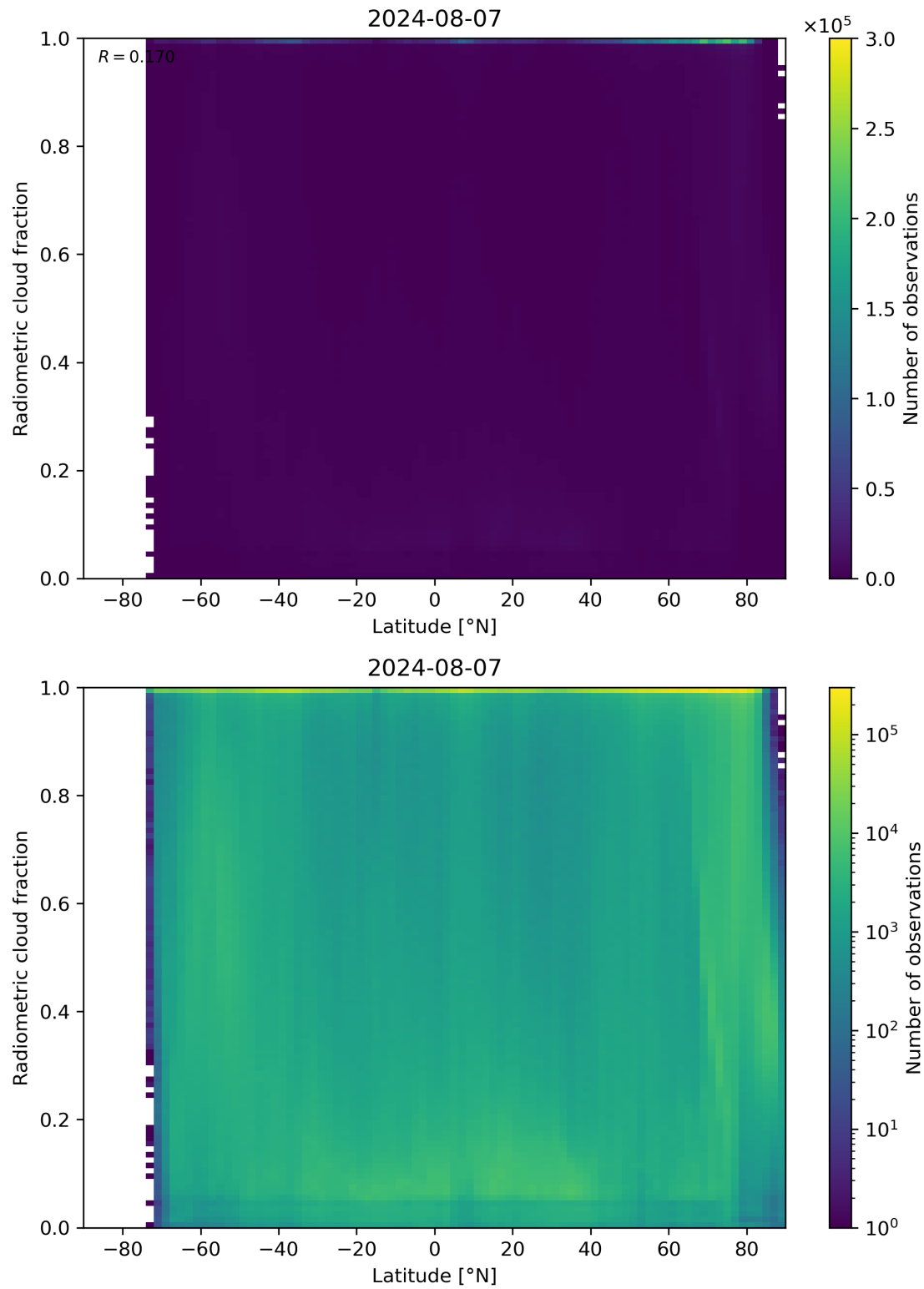
Figure 92: Scatter density plot of “Latitude” against “Radiometric cloud fraction” for 2024-08-06 to 2024-08-08.
