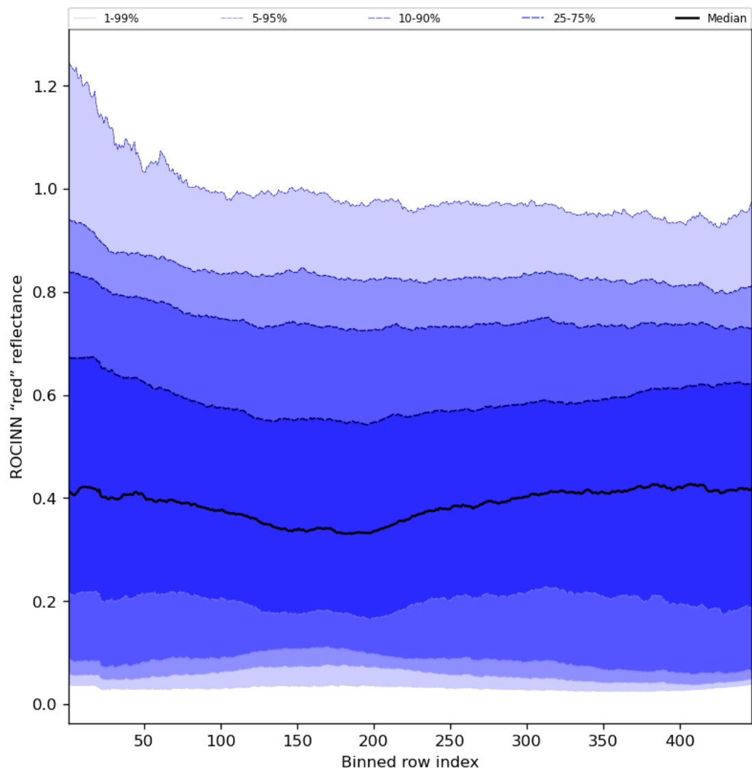
Figure 69: Along track statistics of “ROCINN “red” reflectance” for 2024-08-06 to 2024-08-08
