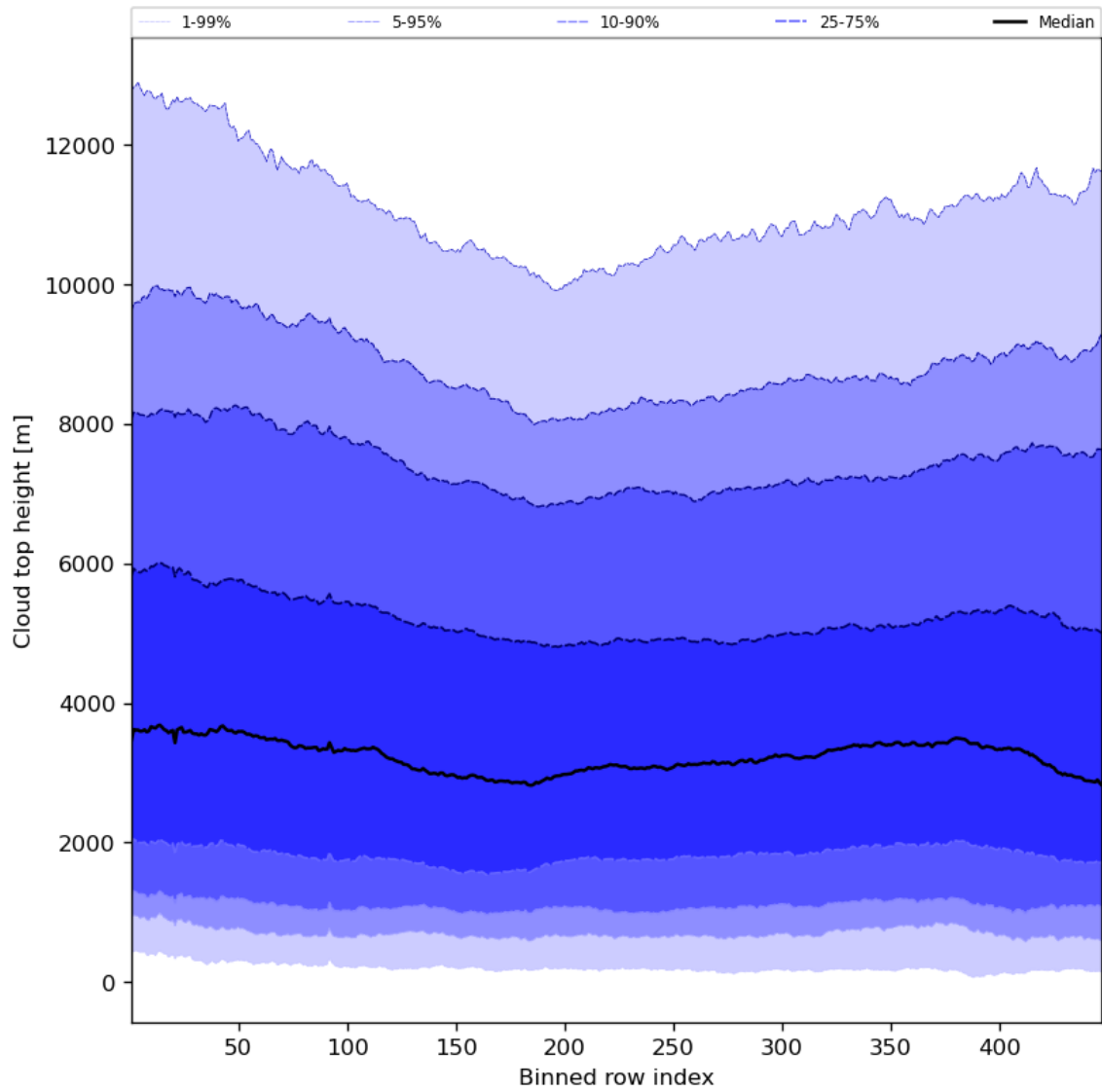
Figure 56: Along track statistics of “Cloud top height” for 2024-08-06 to 2024-08-08
