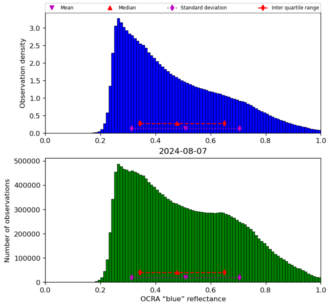
Figure 51: Histogram of “OCRA “blue” reflectance” for 2024-08-06 to 2024-08-08
