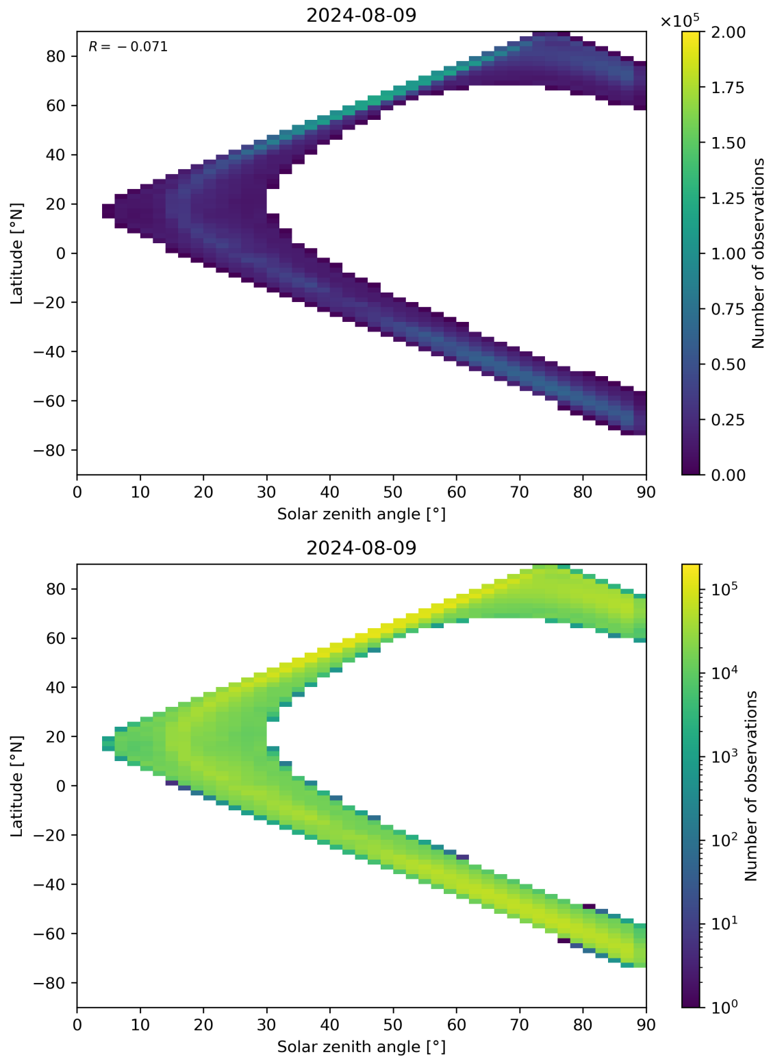
Figure 105: Scatter density plot of “Solar zenith angle” against “Latitude” for 2024-08-08 to 2024-08-10.
