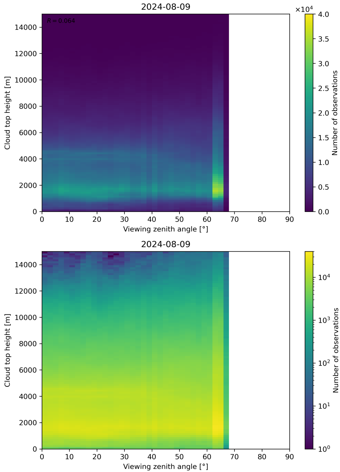
Figure 112: Scatter density plot of “Viewing zenith angle” against “Cloud top height” for 2024-08-08 to 2024-08-10.
