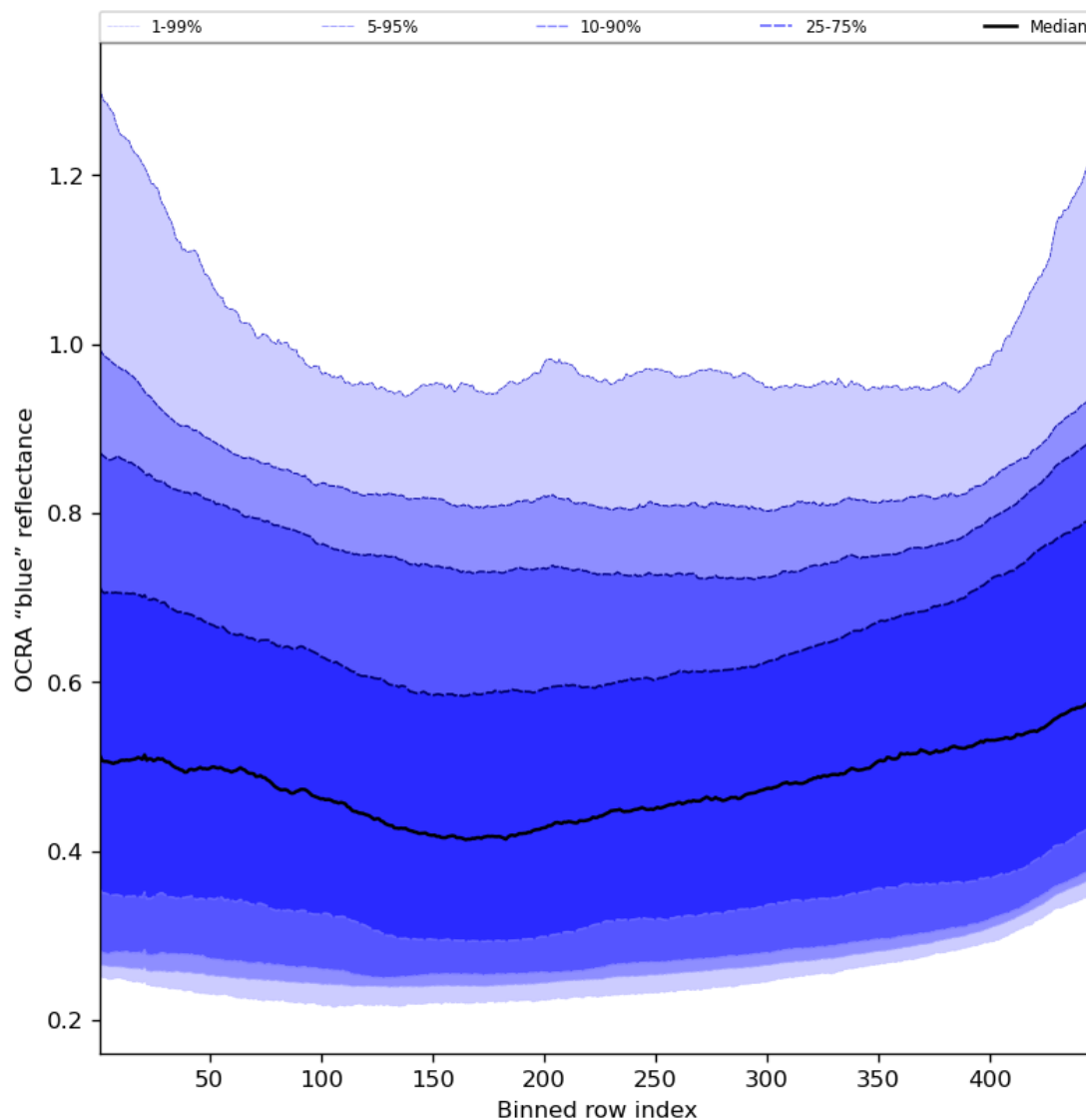
Figure 67: Along track statistics of “OCRA “blue” reflectance” for 2024-08-08 to 2024-08-10
