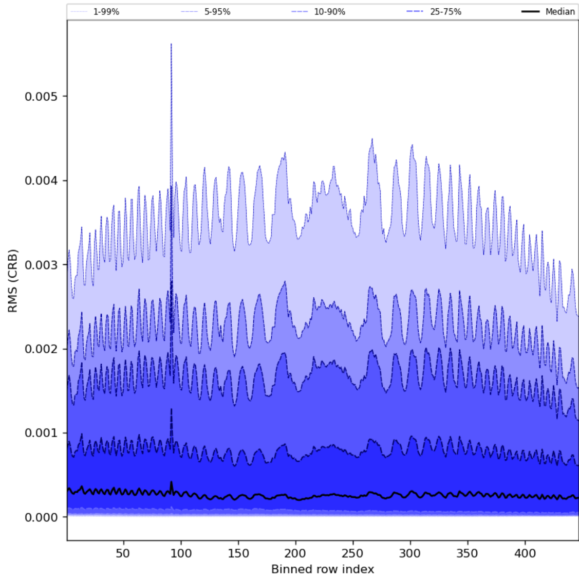
Figure 64: Along track statistics of “RMS (CRB)” for 2024-08-08 to 2024-08-10
