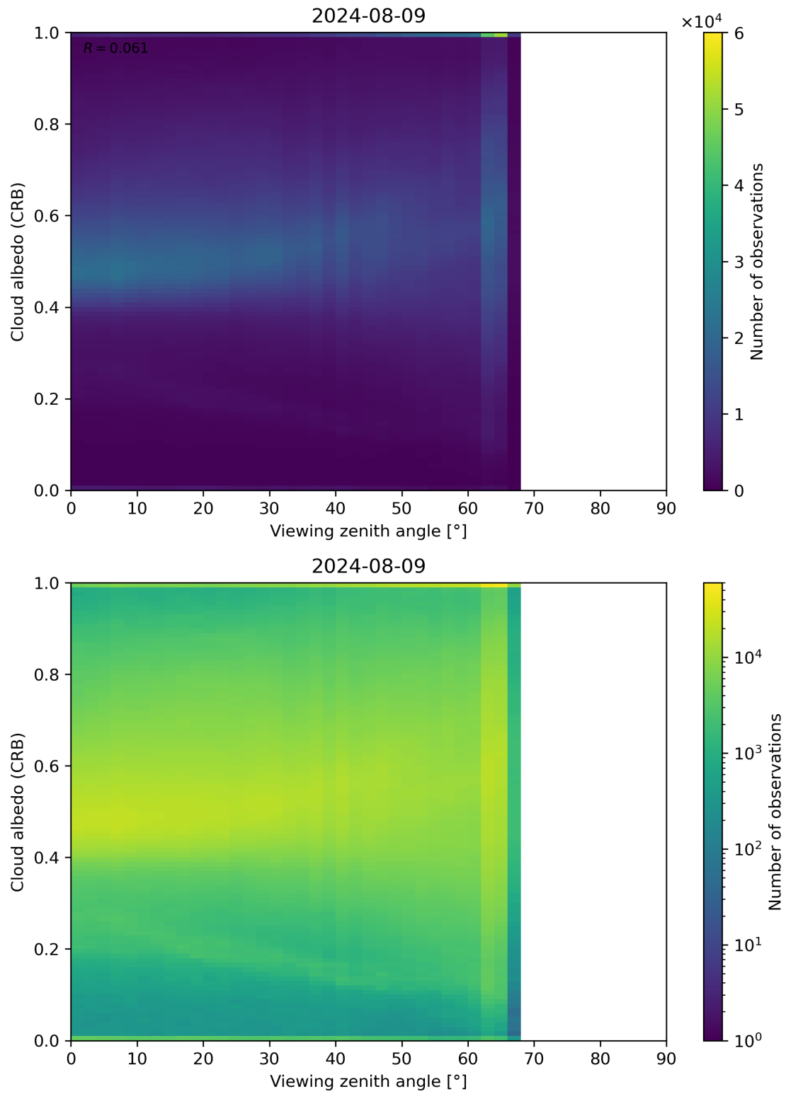
Figure 106: Scatter density plot of “Viewing zenith angle” against “Cloud albedo (CRB)” for 2024-08-08 to 2024-08-10.
