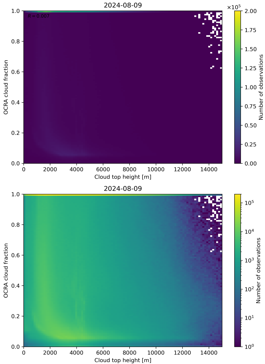
Figure 87: Scatter density plot of “Cloud top height” against “OCRA cloud fraction” for 2024-08-08 to 2024-08-10.
