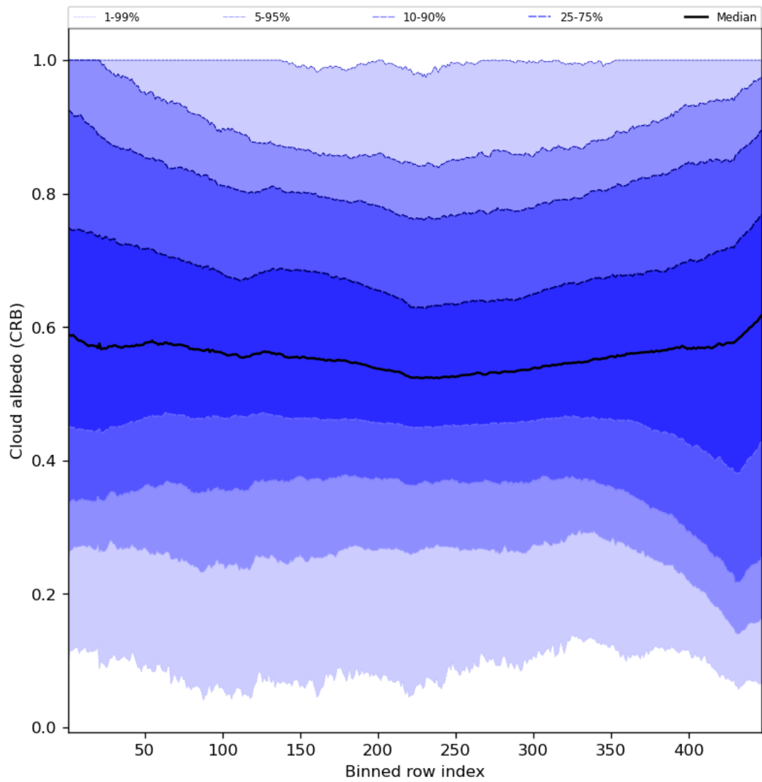
Figure 60: Along track statistics of “Cloud albedo (CRB)” for 2024-08-08 to 2024-08-10
