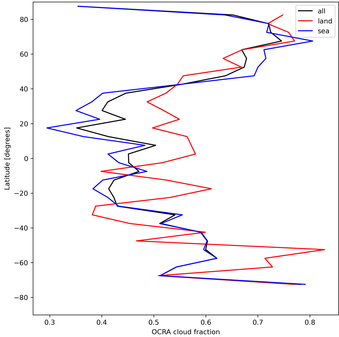
Figure 34: Zonal average of “OCRA cloud fraction” for 2024-08-08 to 2024-08-10.
