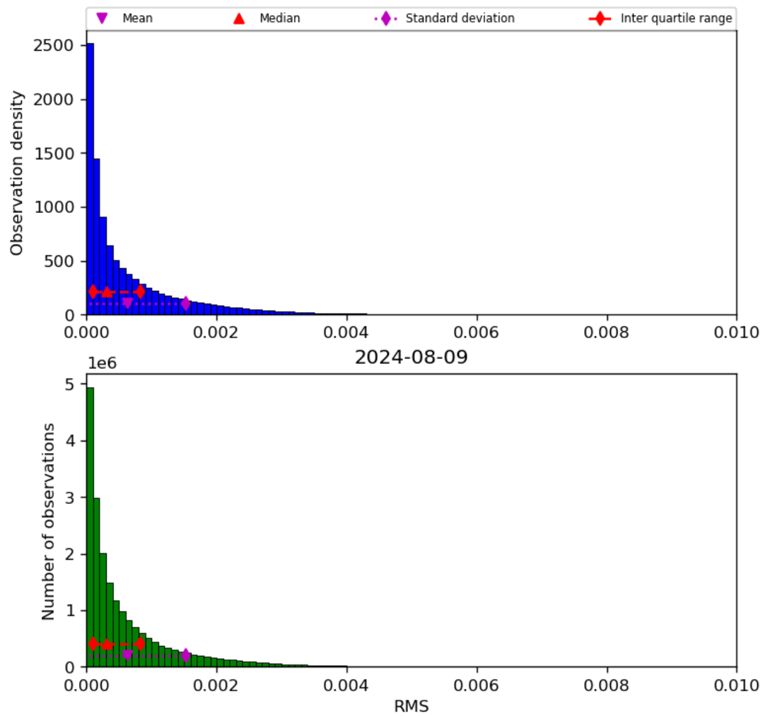
Figure 47: Histogram of “RMS” for 2024-08-08 to 2024-08-10
