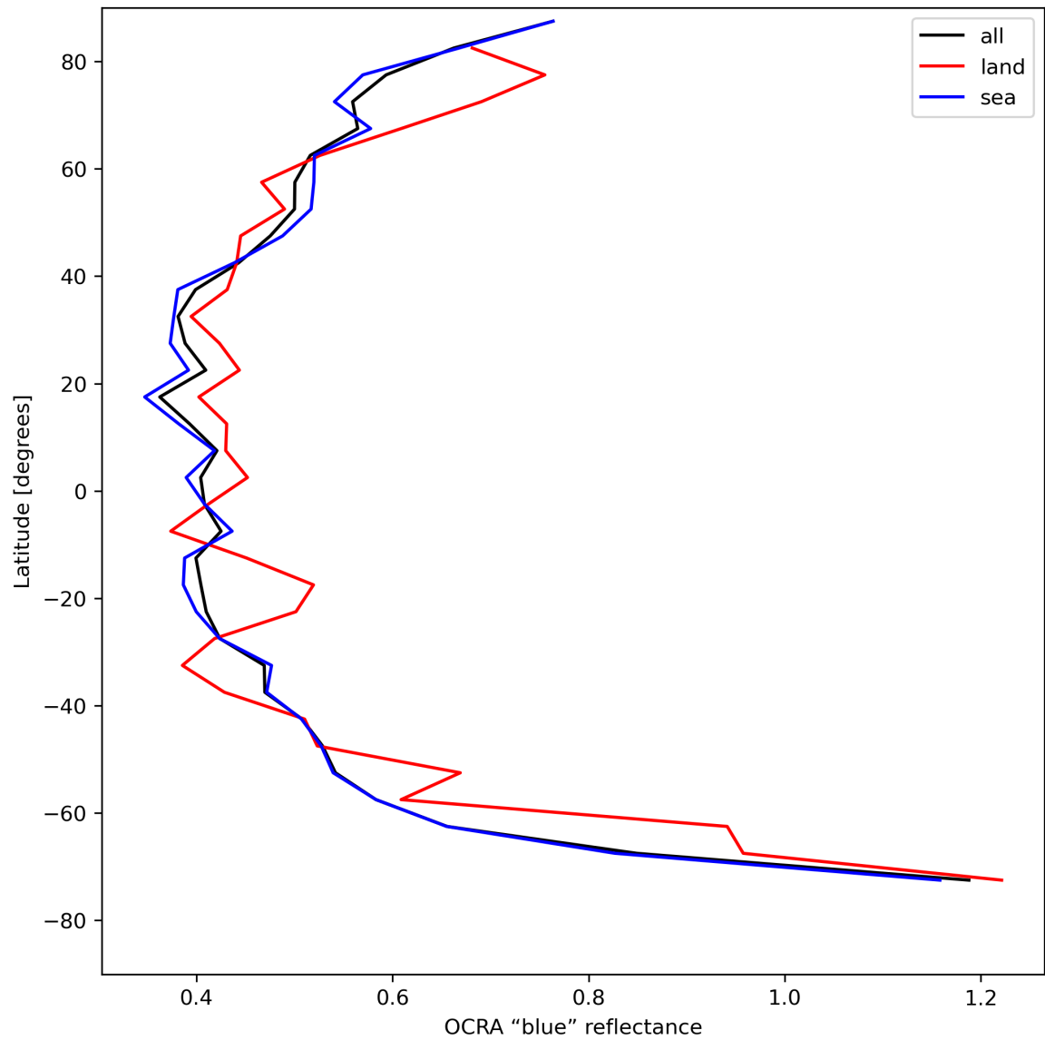
Figure 35: Zonal average of “OCRA “blue” reflectance” for 2024-08-08 to 2024-08-10.
