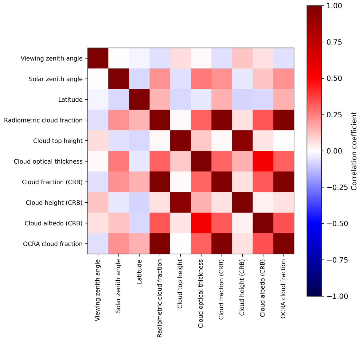
Figure 2: Map of correlation matrix for 2024-08-08 to 2024-08-10.
