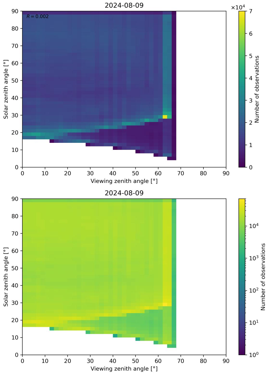
Figure 114: Scatter density plot of “Viewing zenith angle” against “Solar zenith angle” for 2024-08-08 to 2024-08-10.
