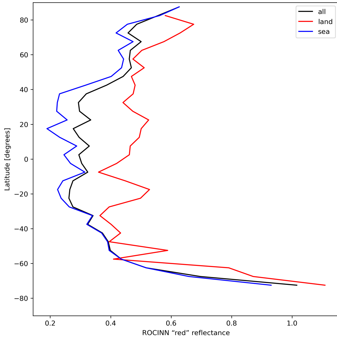
Figure 37: Zonal average of “ROCINN “red” reflectance” for 2024-08-08 to 2024-08-10.
