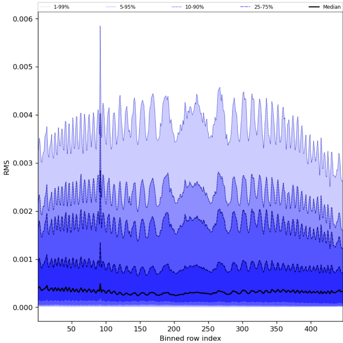
Figure 63: Along track statistics of “RMS” for 2024-08-08 to 2024-08-10
