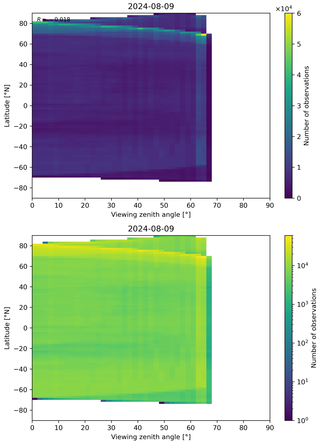
Figure 113: Scatter density plot of “Viewing zenith angle” against “Latitude” for 2024-08-08 to 2024-08-10.
