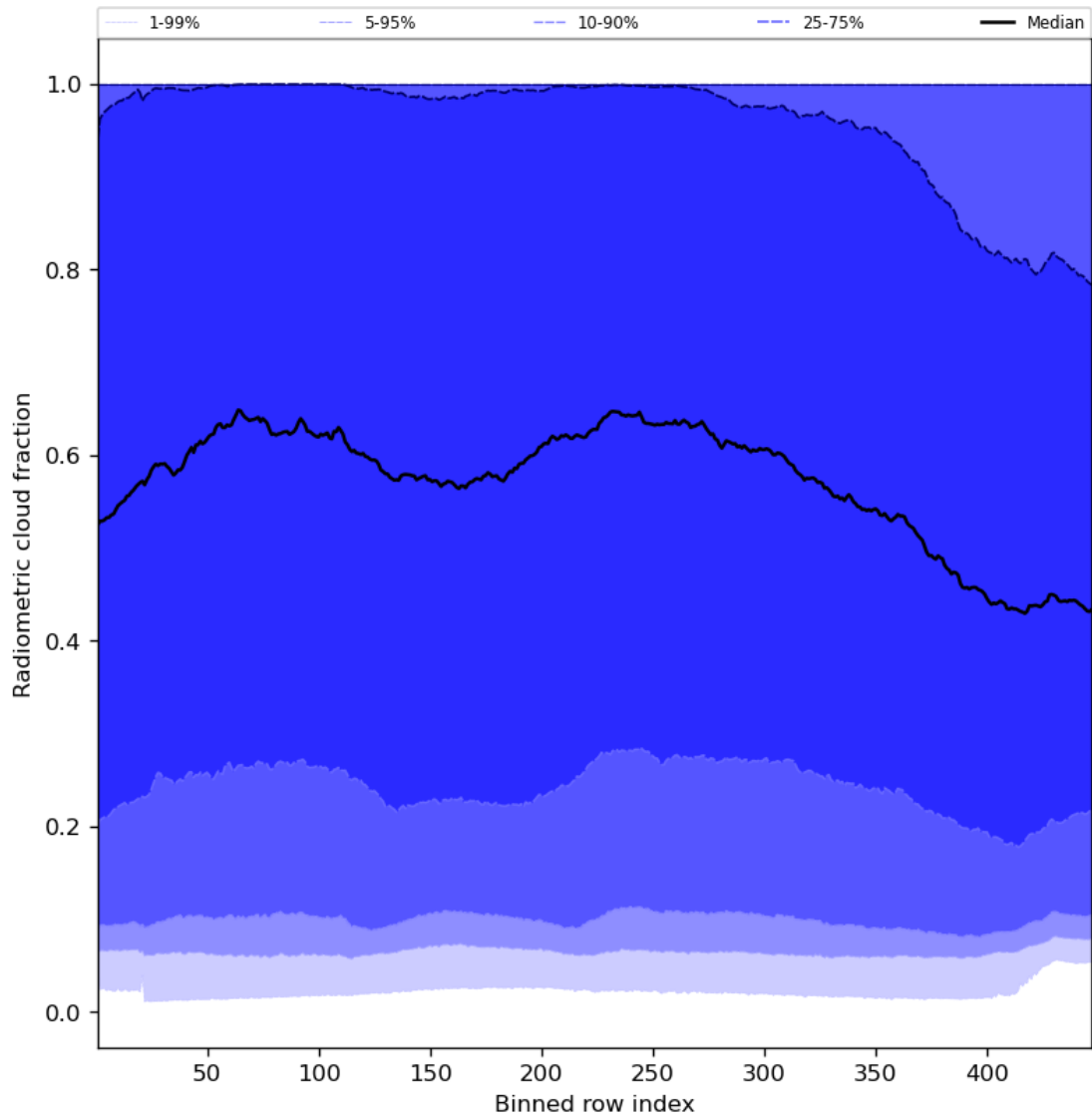
Figure 55: Along track statistics of “Radiometric cloud fraction” for 2024-08-08 to 2024-08-10
