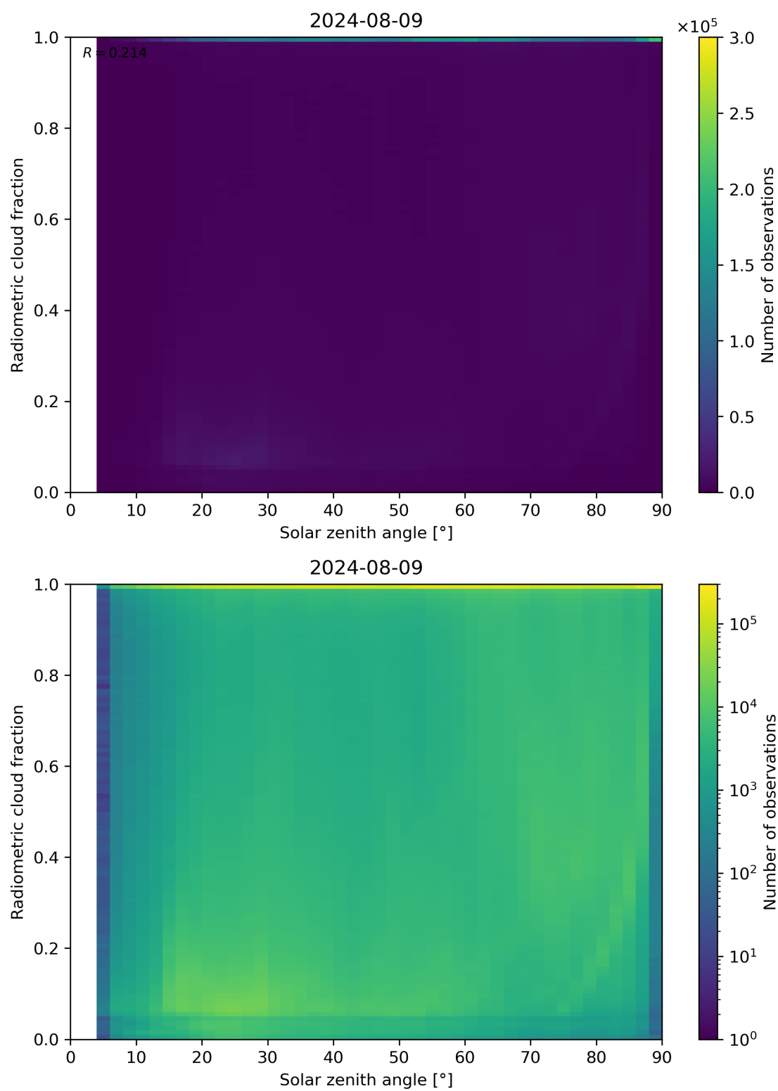
Figure 99: Scatter density plot of “Solar zenith angle” against “Radiometric cloud fraction” for 2024-08-08 to 2024-08-10.
