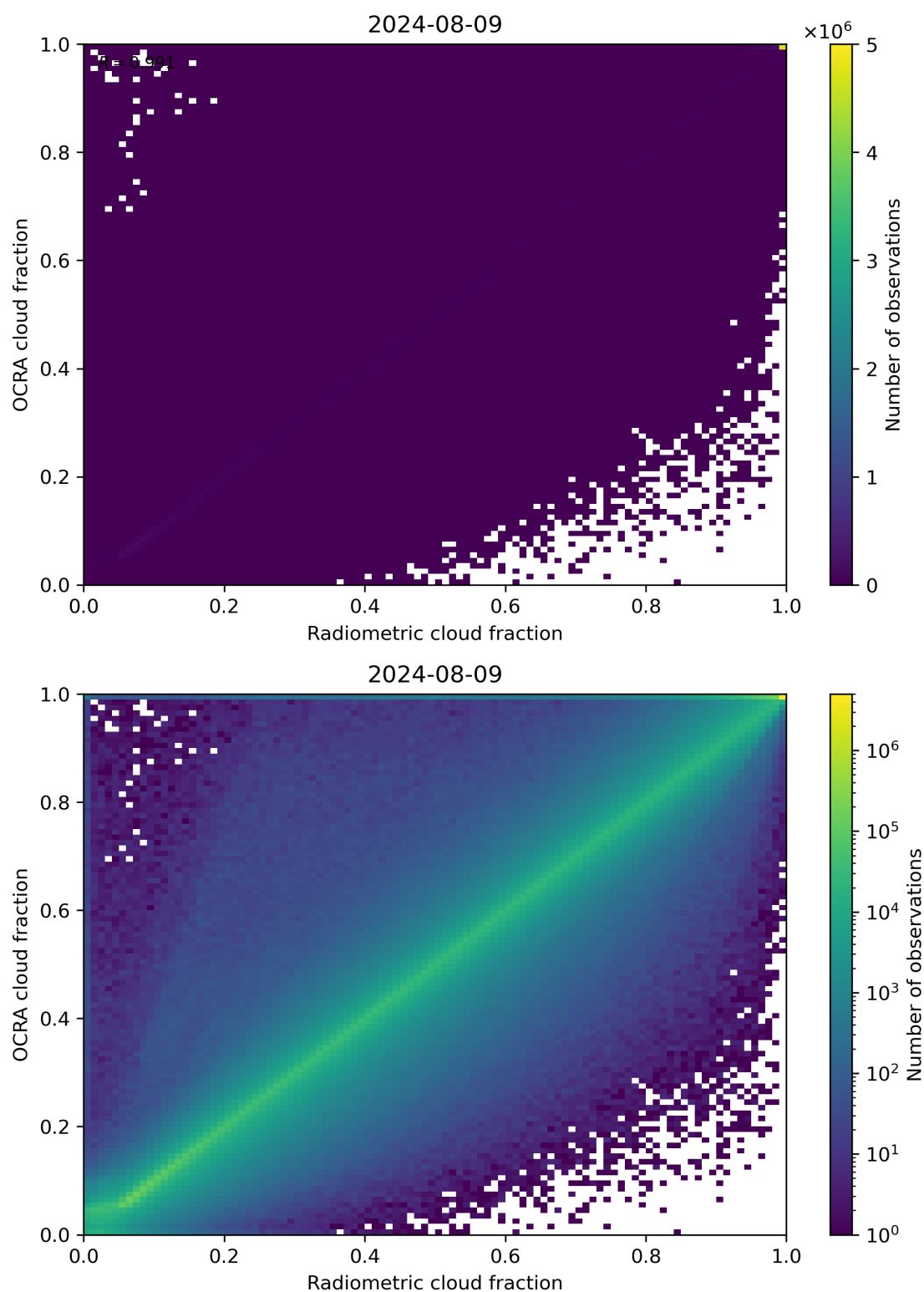
Figure 72: Scatter density plot of “Radiometric cloud fraction” against “OCRA cloud fraction” for 2024-08-08 to 2024-08-10.
