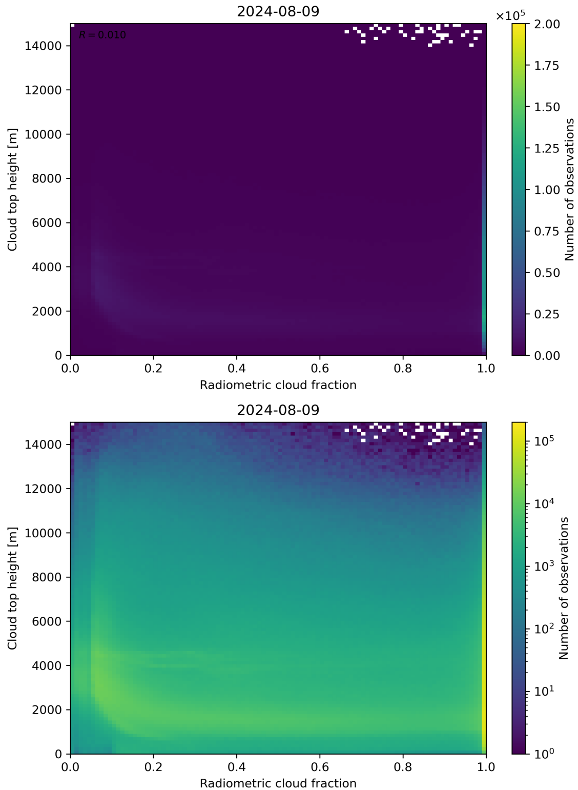
Figure 76: Scatter density plot of “Radiometric cloud fraction” against “Cloud top height” for 2024-08-08 to 2024-08-10.
