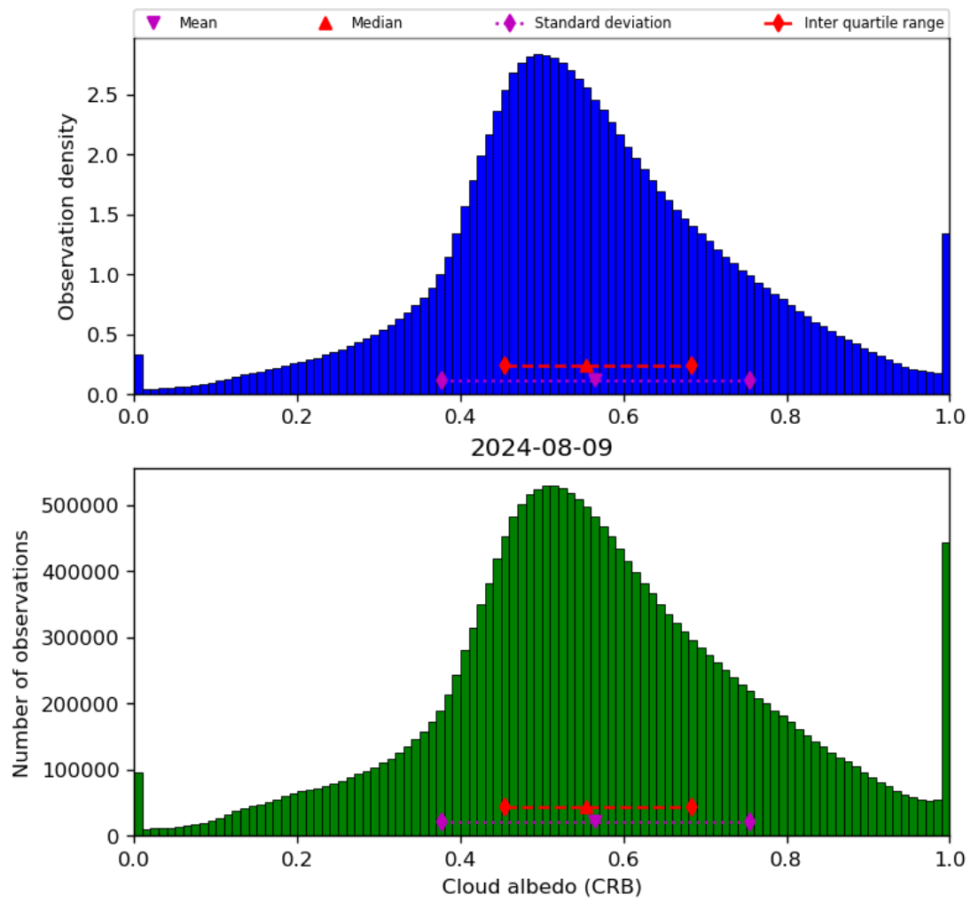
Figure 44: Histogram of “Cloud albedo (CRB)” for 2024-08-08 to 2024-08-10
