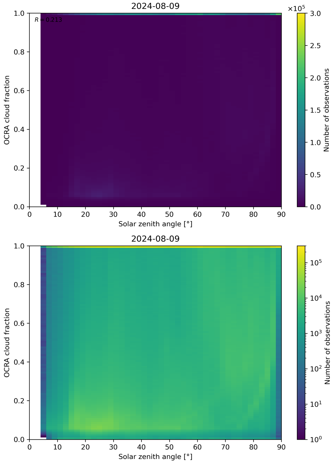
Figure 100: Scatter density plot of “Solar zenith angle” against “OCRA cloud fraction” for 2024-08-08 to 2024-08-10.
