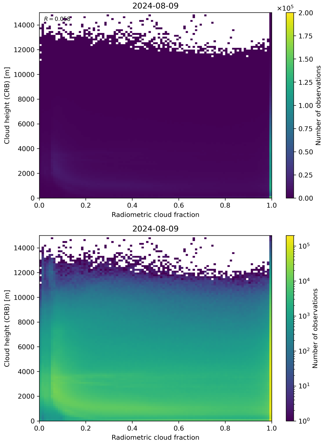
Figure 74: Scatter density plot of “Radiometric cloud fraction” against “Cloud height (CRB)” for 2024-08-08 to 2024-08-10.
