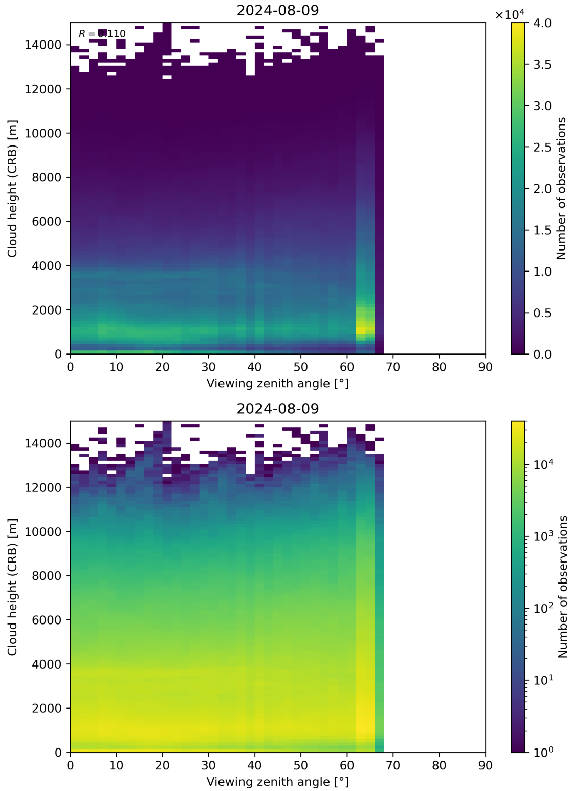
Figure 110: Scatter density plot of “Viewing zenith angle” against “Cloud height (CRB)” for 2024-08-08 to 2024-08-10.
