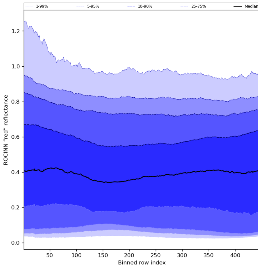
Figure 69: Along track statistics of “ROCINN “red” reflectance” for 2024-08-08 to 2024-08-10
