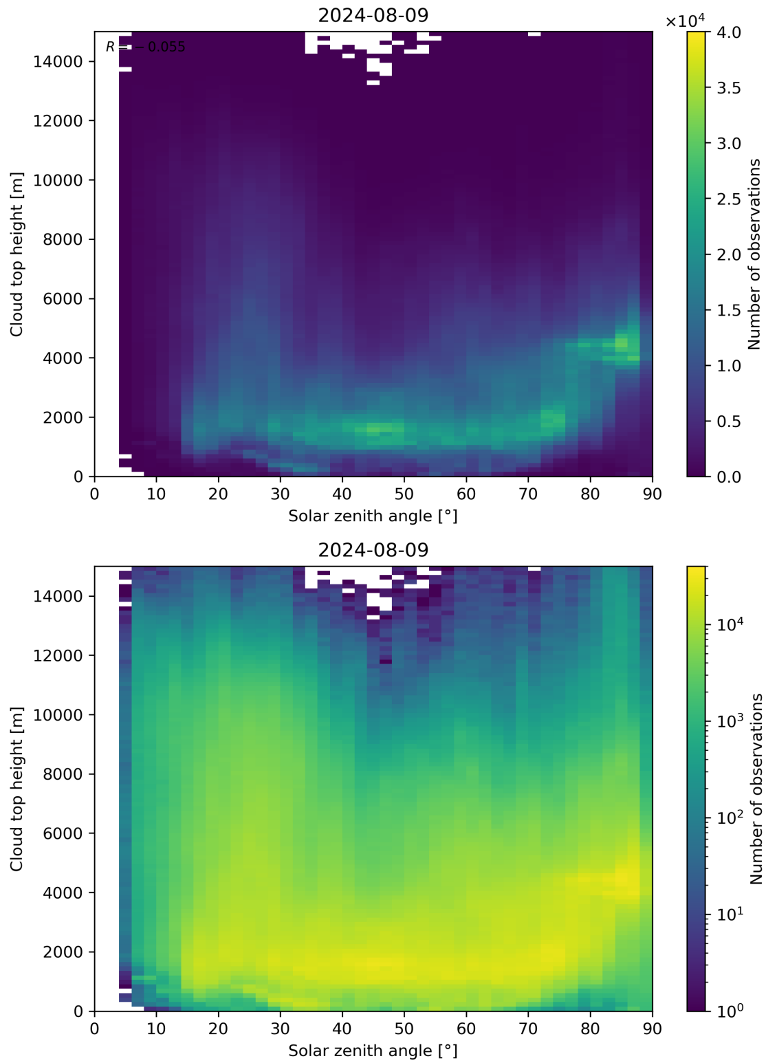
Figure 104: Scatter density plot of “Solar zenith angle” against “Cloud top height” for 2024-08-08 to 2024-08-10.
