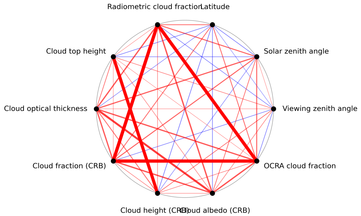
Figure 1: Map of correlation graph for 2024-08-08 to 2024-08-10.
