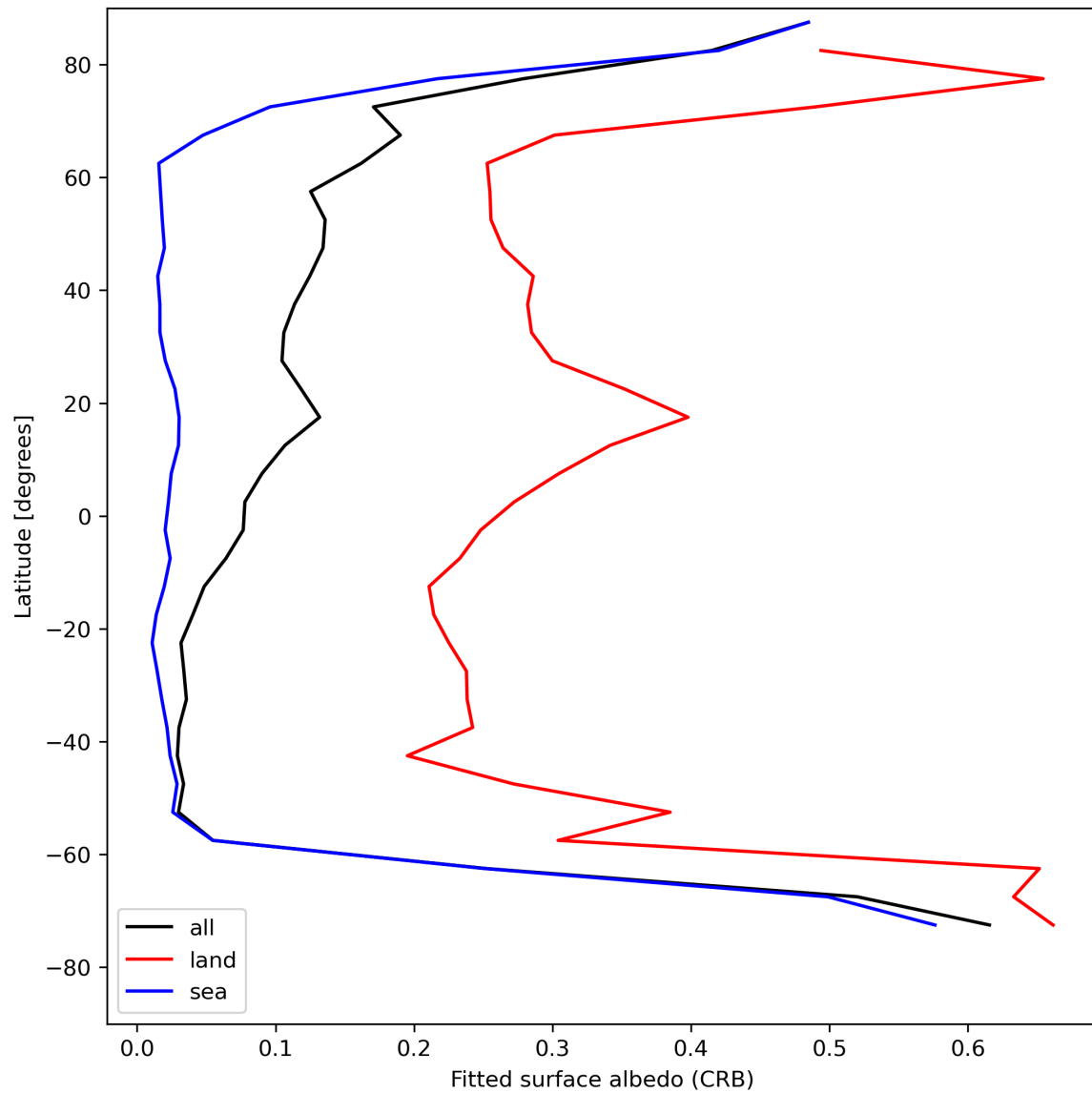
Figure 30: Zonal average of “Fitted surface albedo (CRB)” for 2024-08-08 to 2024-08-10.
