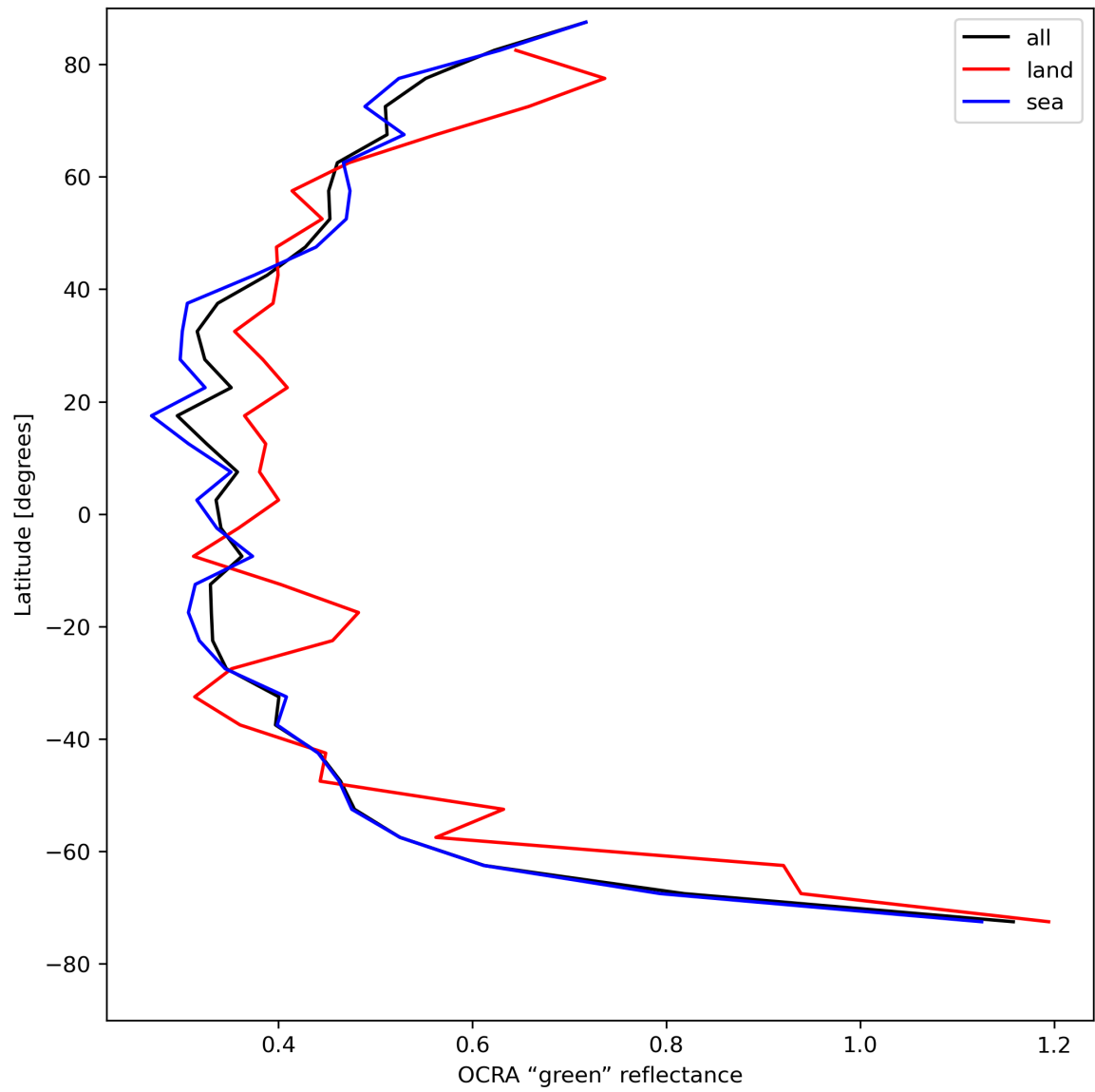
Figure 36: Zonal average of “OCRA “green” reflectance” for 2024-08-08 to 2024-08-10.
