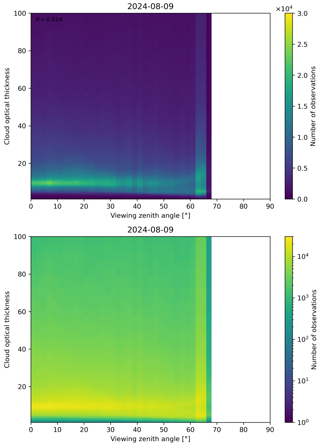
Figure 111: Scatter density plot of “Viewing zenith angle” against “Cloud optical thickness” for 2024-08-08 to 2024-08-10.
