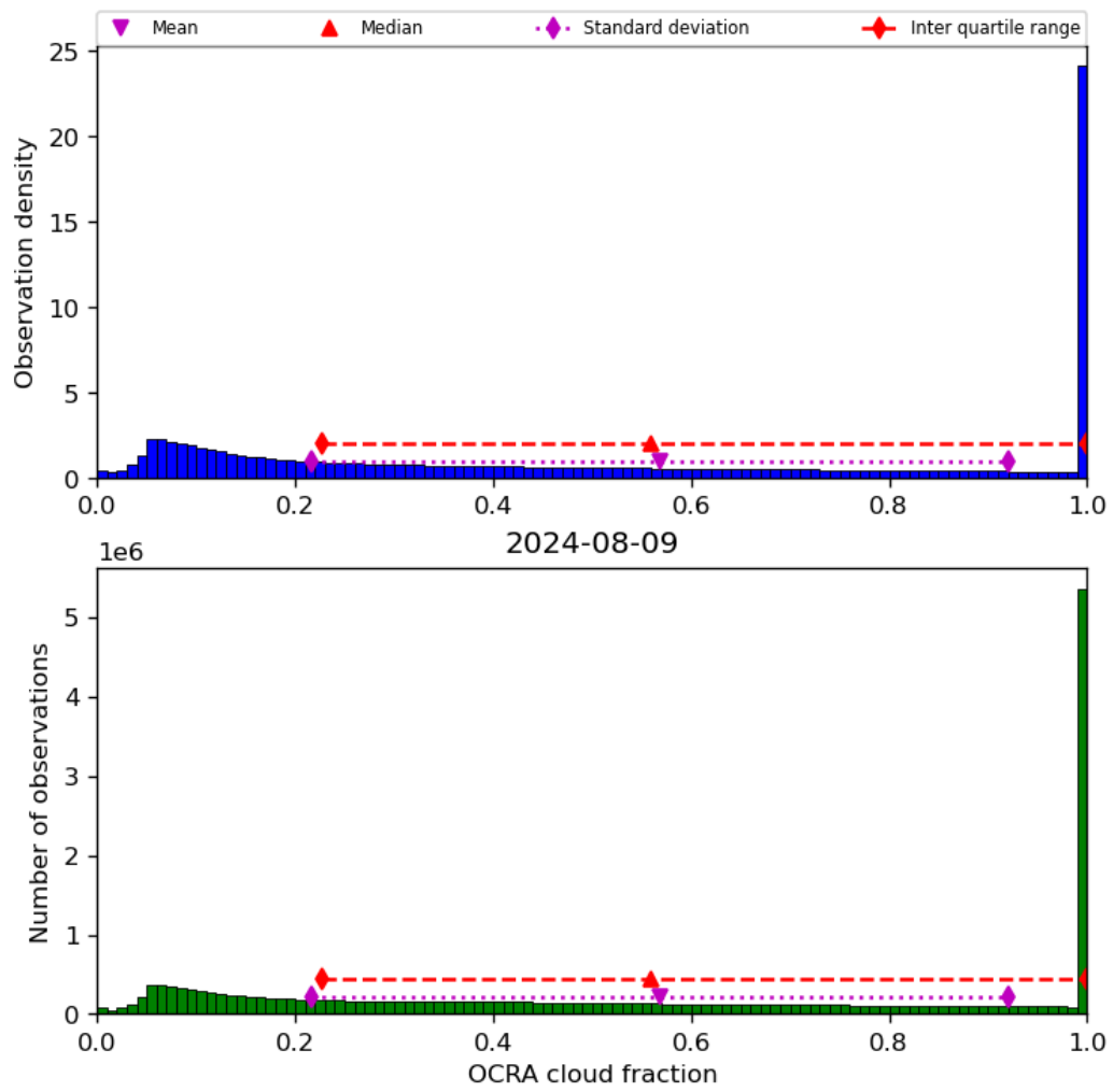
Figure 50: Histogram of “OCRA cloud fraction” for 2024-08-08 to 2024-08-10
