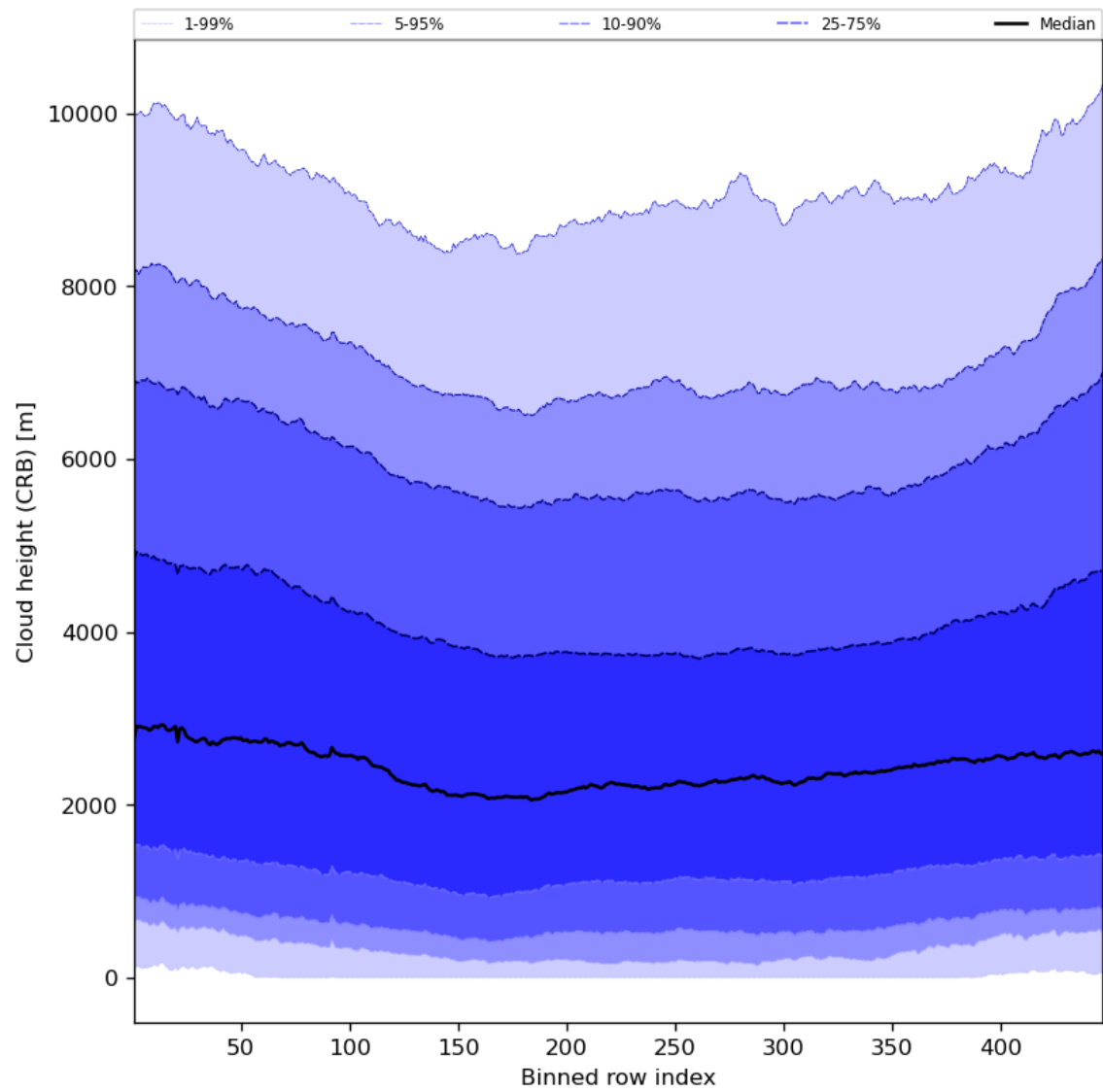
Figure 59: Along track statistics of “Cloud height (CRB)” for 2024-08-08 to 2024-08-10
