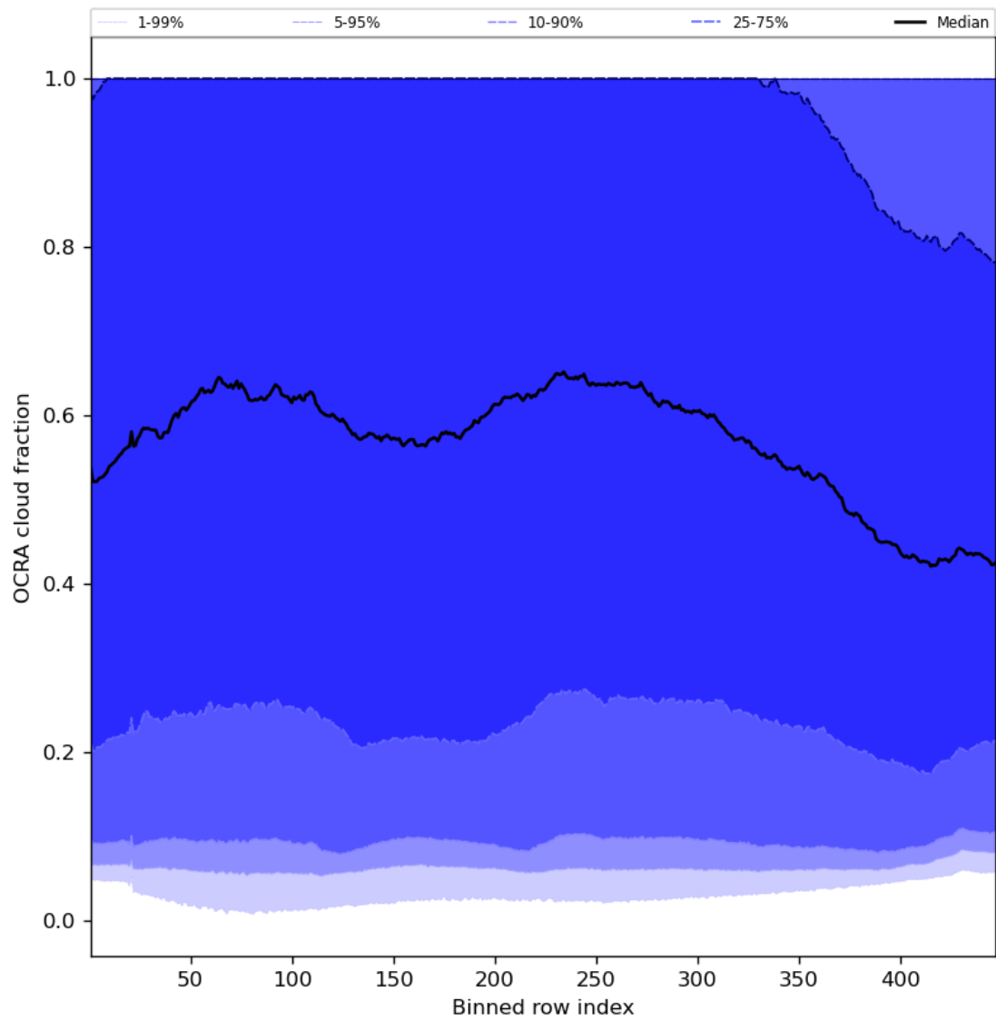
Figure 66: Along track statistics of “OCRA cloud fraction” for 2024-08-08 to 2024-08-10
