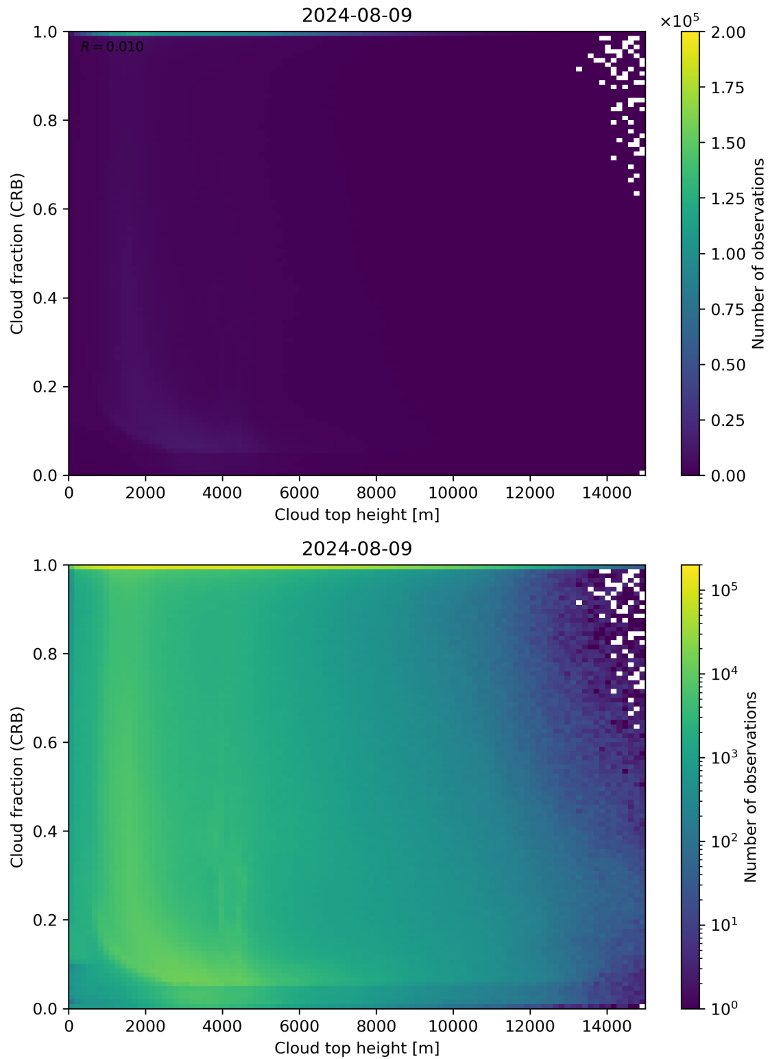
Figure 88: Scatter density plot of “Cloud top height” against “Cloud fraction (CRB)” for 2024-08-08 to 2024-08-10.
