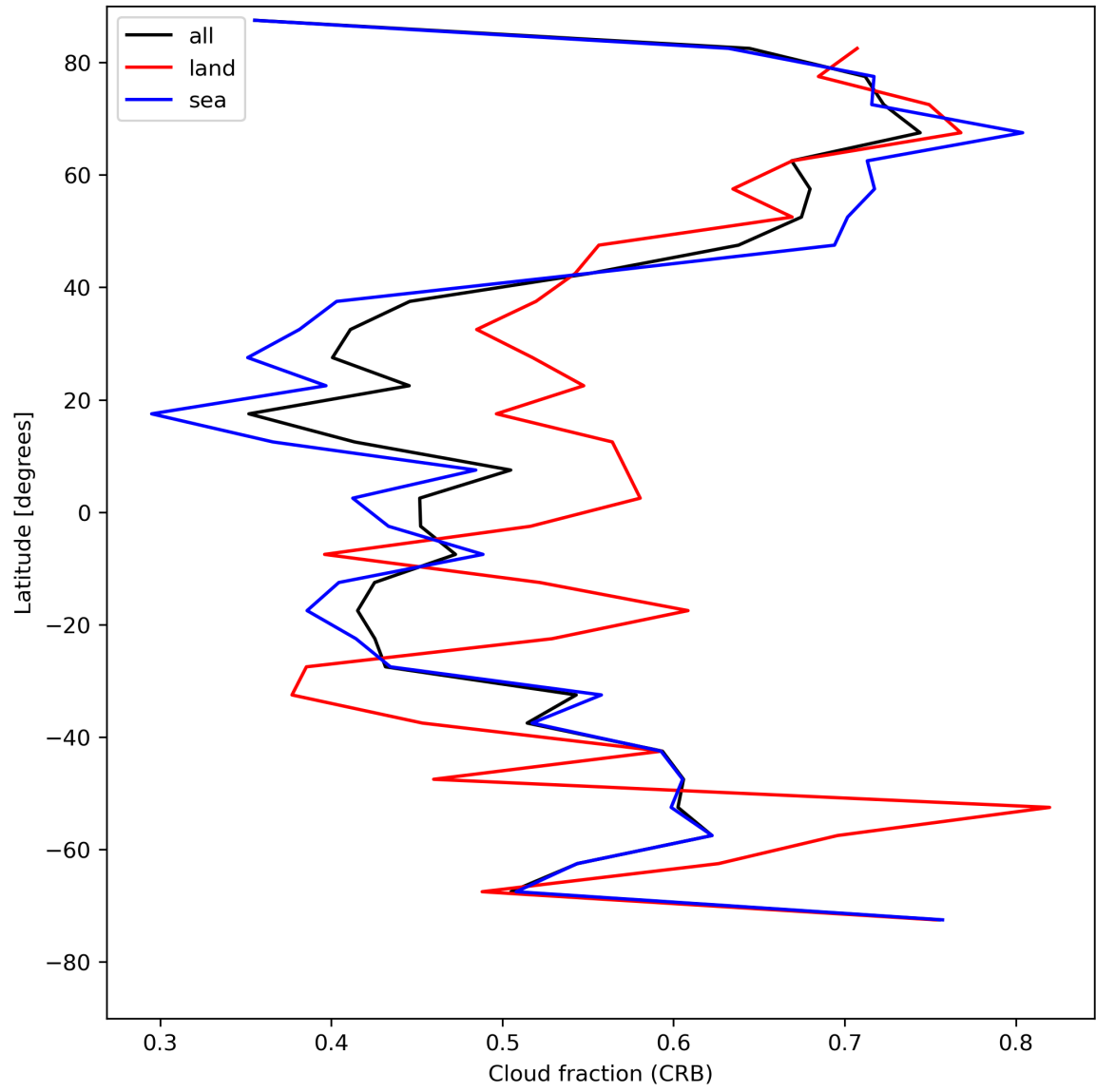
Figure 26: Zonal average of “Cloud fraction (CRB)” for 2024-08-08 to 2024-08-10.
