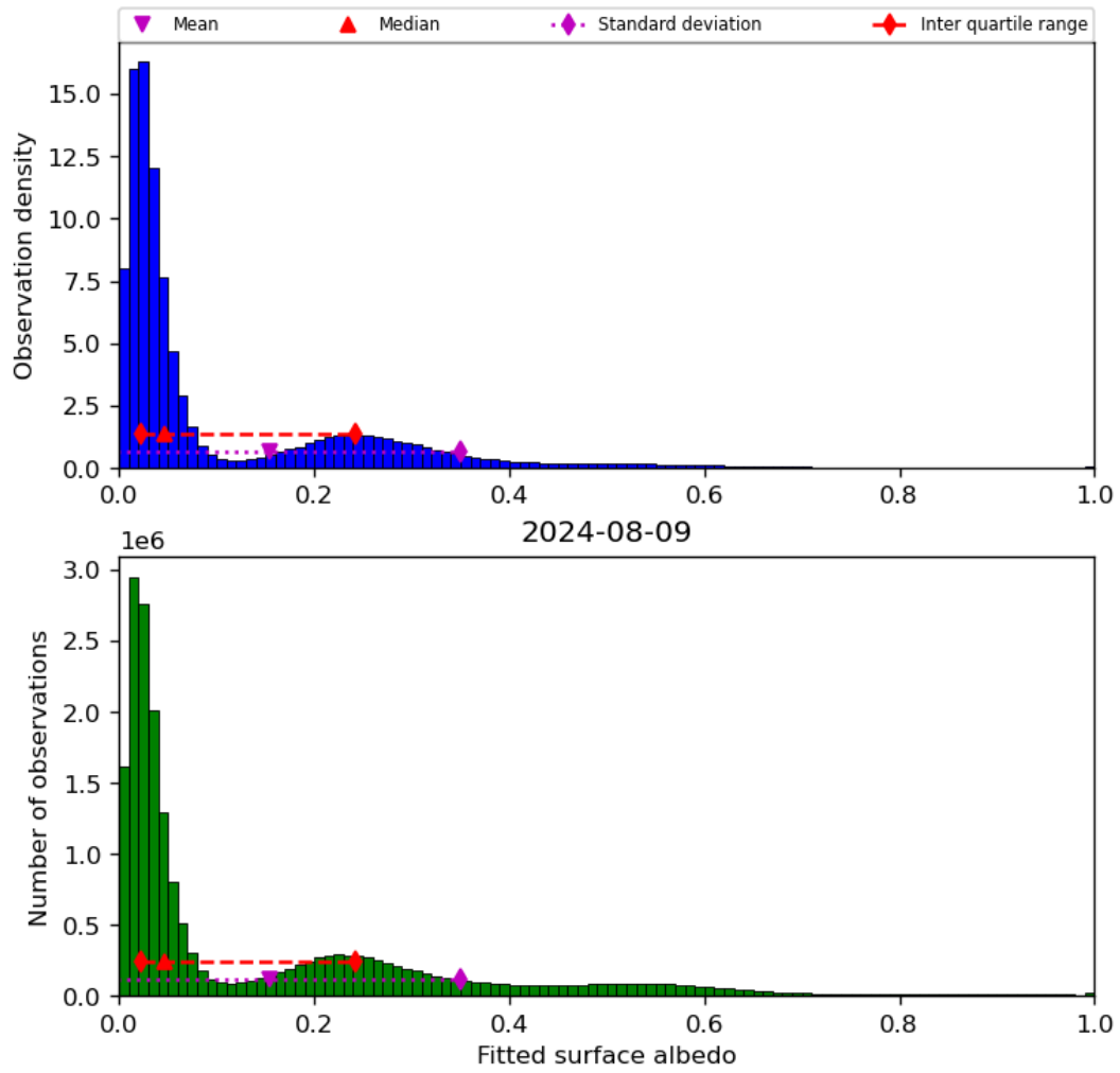
Figure 45: Histogram of “Fitted surface albedo” for 2024-08-08 to 2024-08-10
