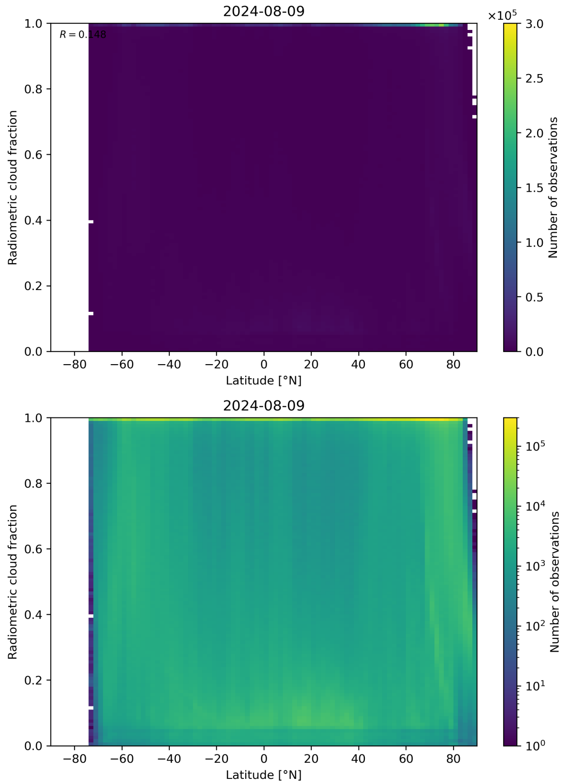
Figure 92: Scatter density plot of “Latitude” against “Radiometric cloud fraction” for 2024-08-08 to 2024-08-10.
