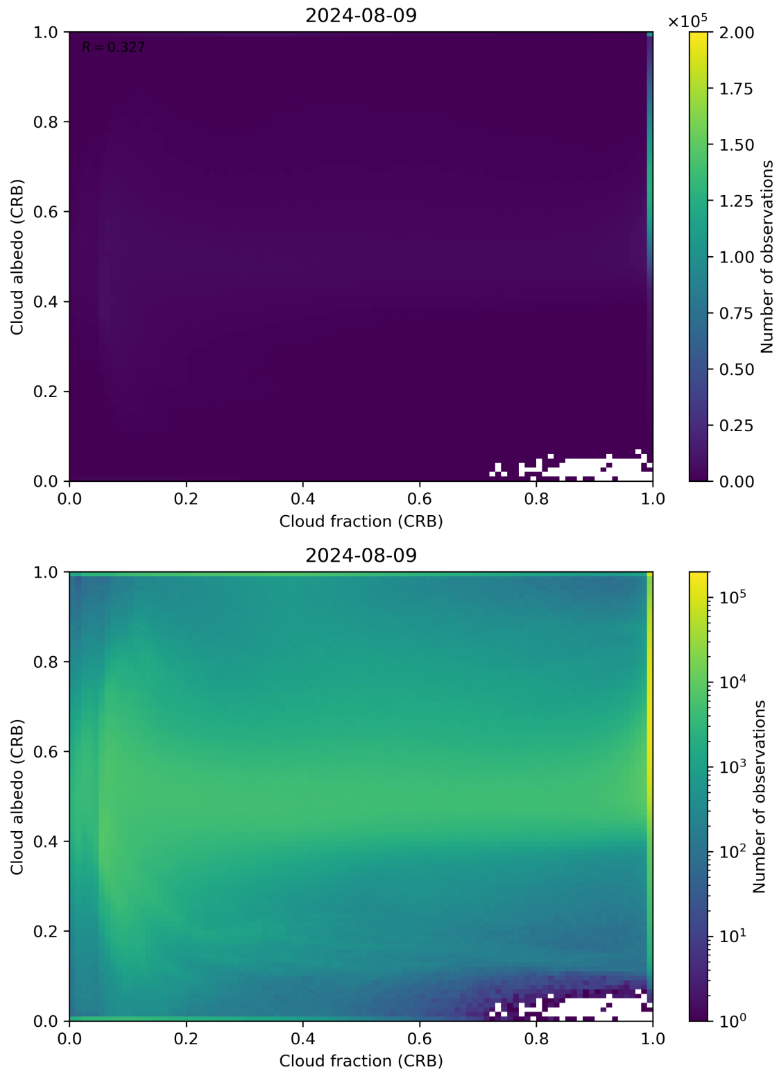
Figure 77: Scatter density plot of “Cloud fraction (CRB)” against “Cloud albedo (CRB)” for 2024-08-08 to 2024-08-10.
