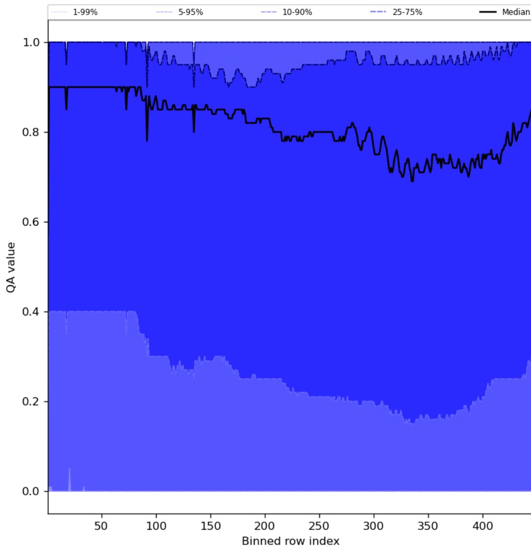
Figure 54: Along track statistics of “QA value” for 2024-08-08 to 2024-08-10
