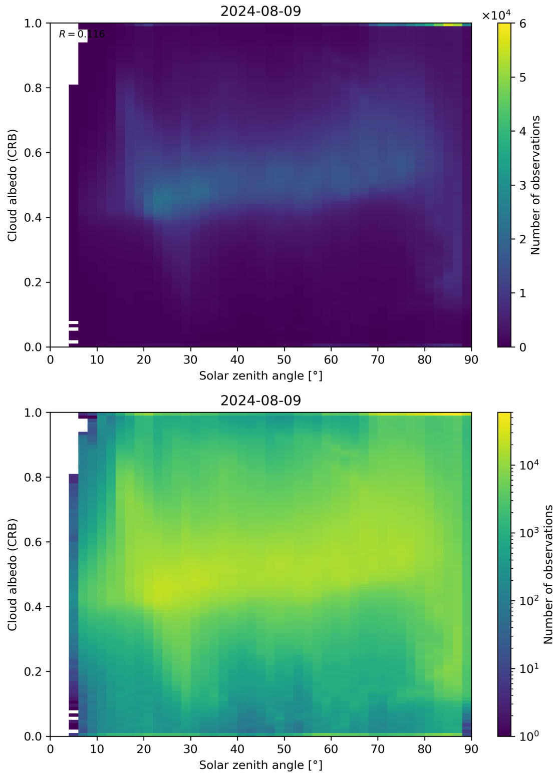
Figure 98: Scatter density plot of “Solar zenith angle” against “Cloud albedo (CRB)” for 2024-08-08 to 2024-08-10.
