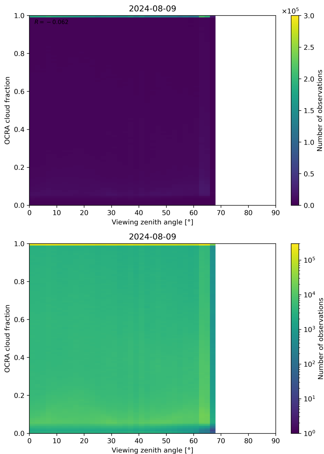
Figure 108: Scatter density plot of “Viewing zenith angle” against “OCRA cloud fraction” for 2024-08-08 to 2024-08-10.
