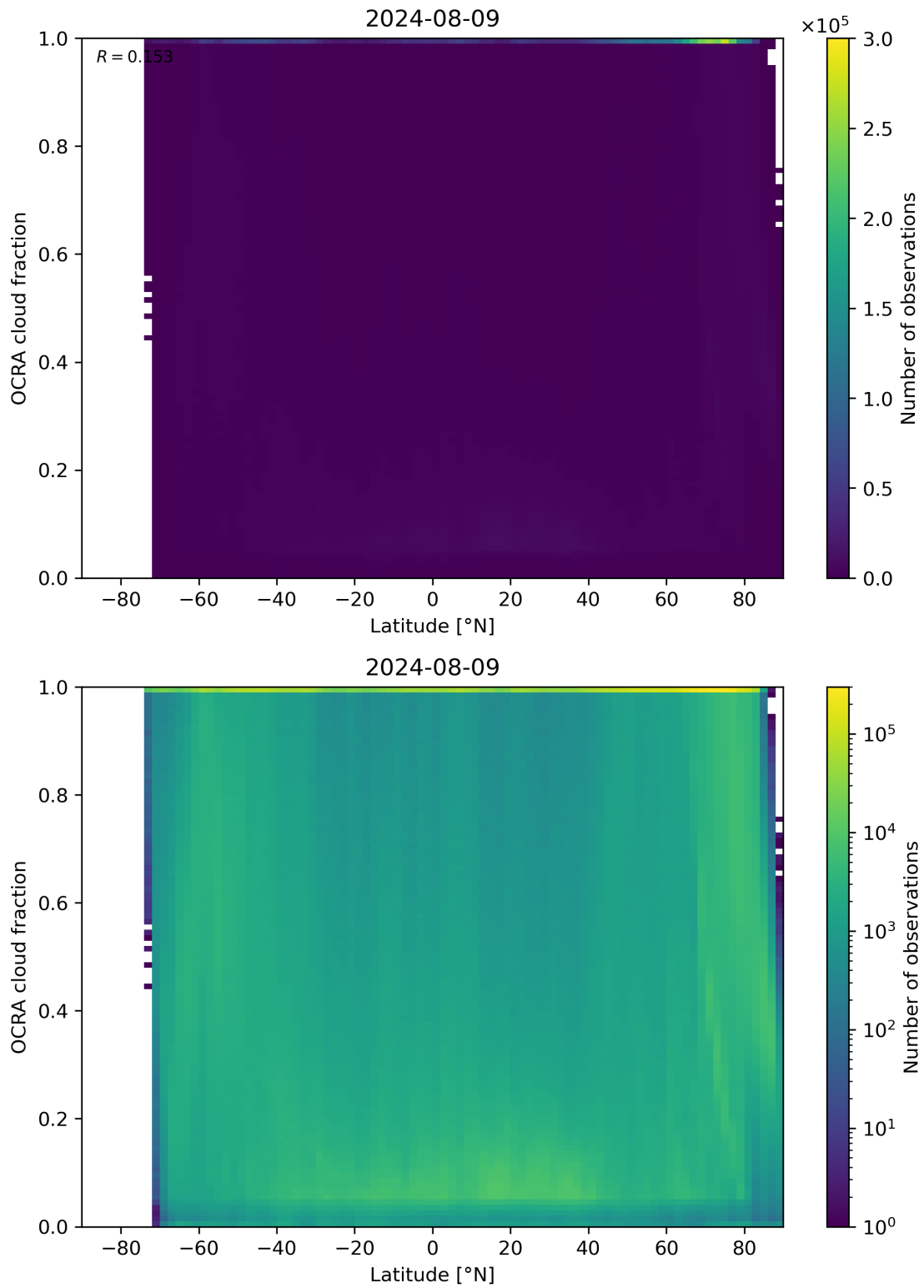
Figure 93: Scatter density plot of “Latitude” against “OCRA cloud fraction” for 2024-08-08 to 2024-08-10.
