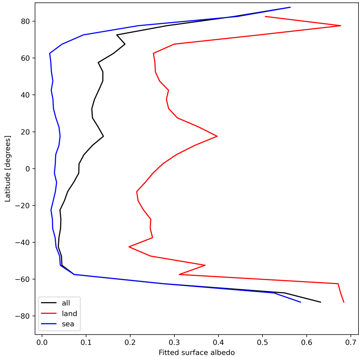
Figure 29: Zonal average of “Fitted surface albedo” for 2024-08-08 to 2024-08-10.
