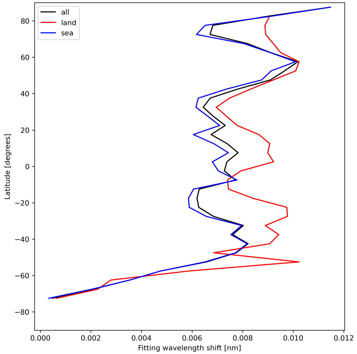
Figure 33: Zonal average of “Fitting wavelength shift” for 2024-08-08 to 2024-08-10.
