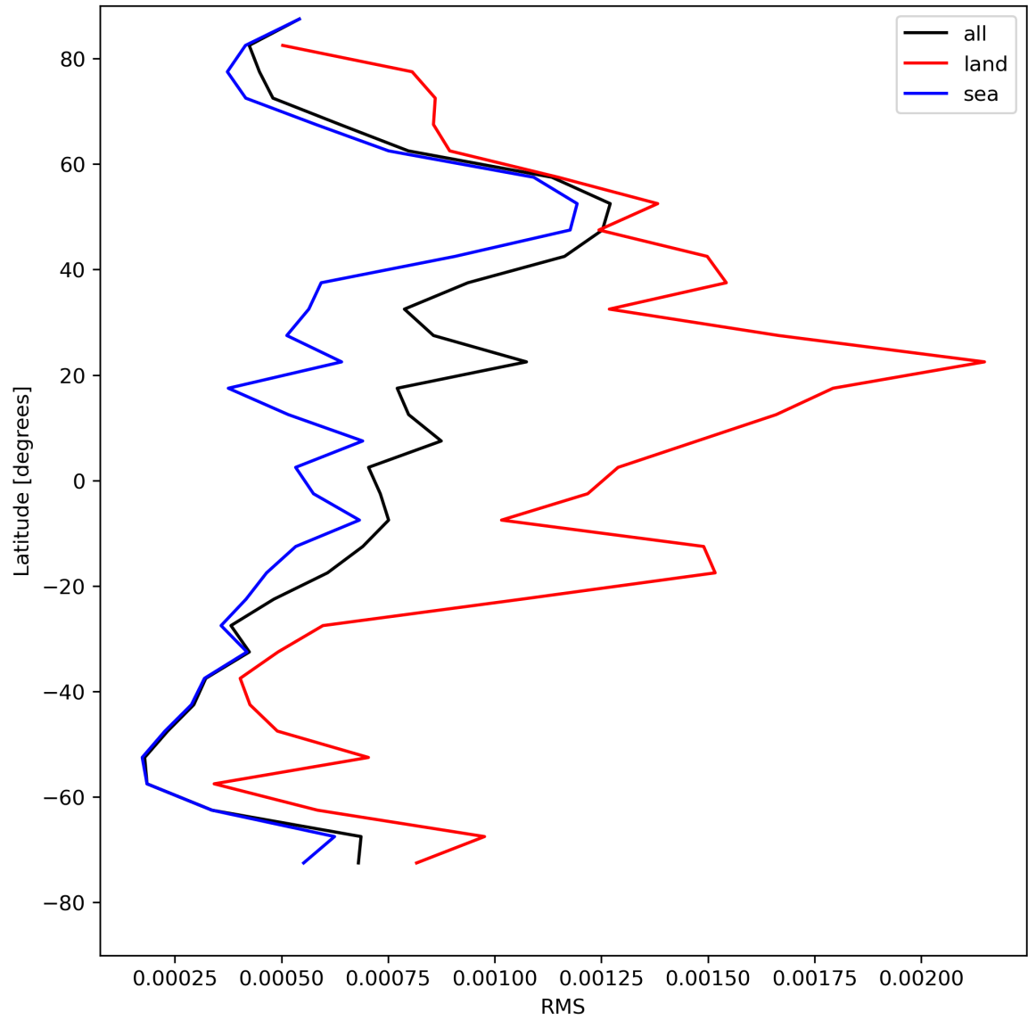
Figure 31: Zonal average of “RMS” for 2024-08-08 to 2024-08-10.
