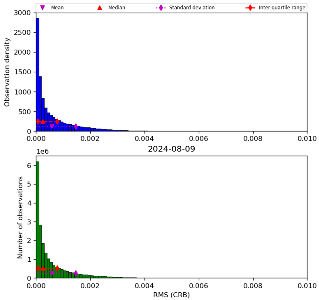
Figure 48: Histogram of “RMS (CRB)” for 2024-08-08 to 2024-08-10
