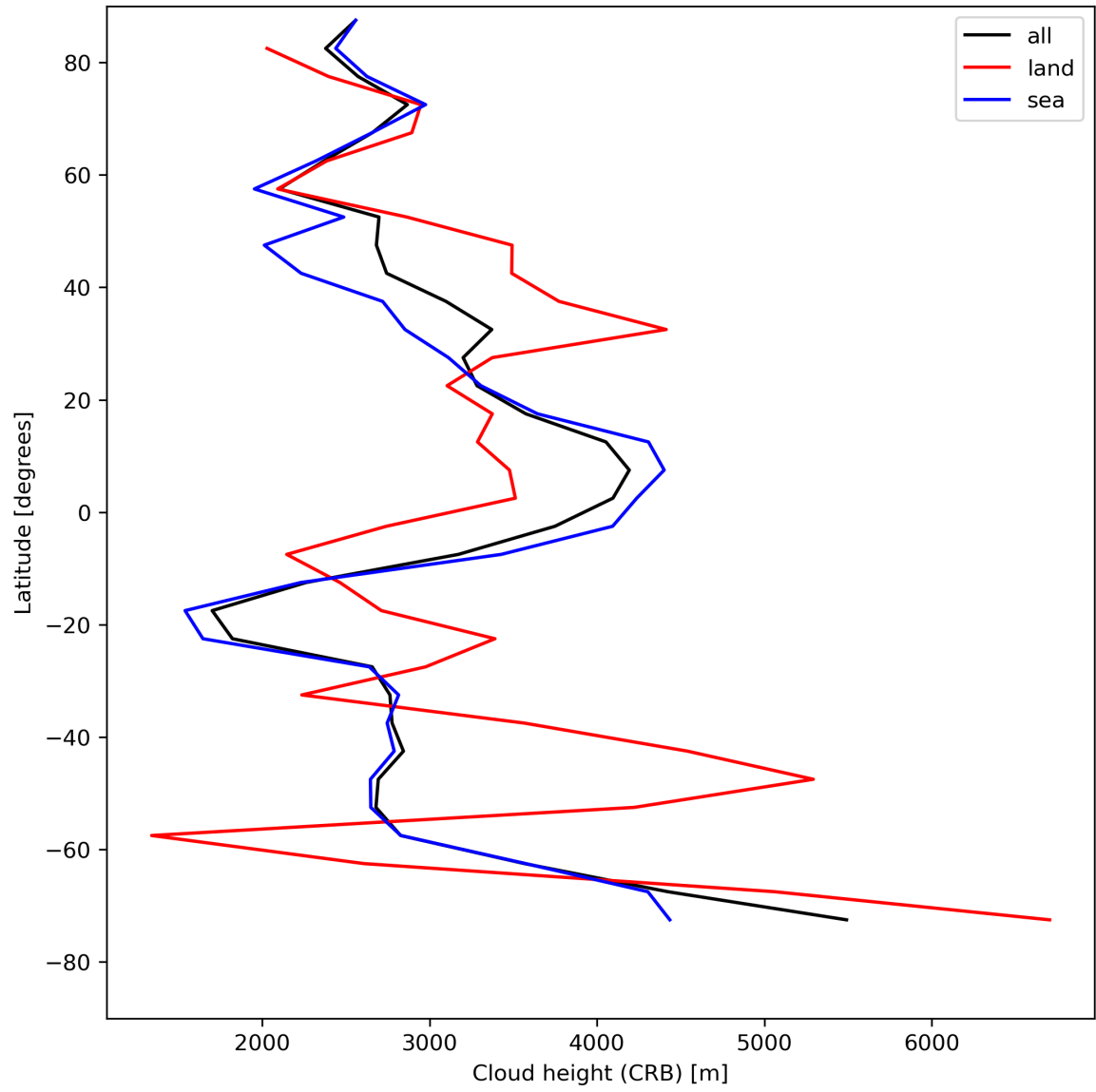
Figure 27: Zonal average of “Cloud height (CRB)” for 2024-08-08 to 2024-08-10.
