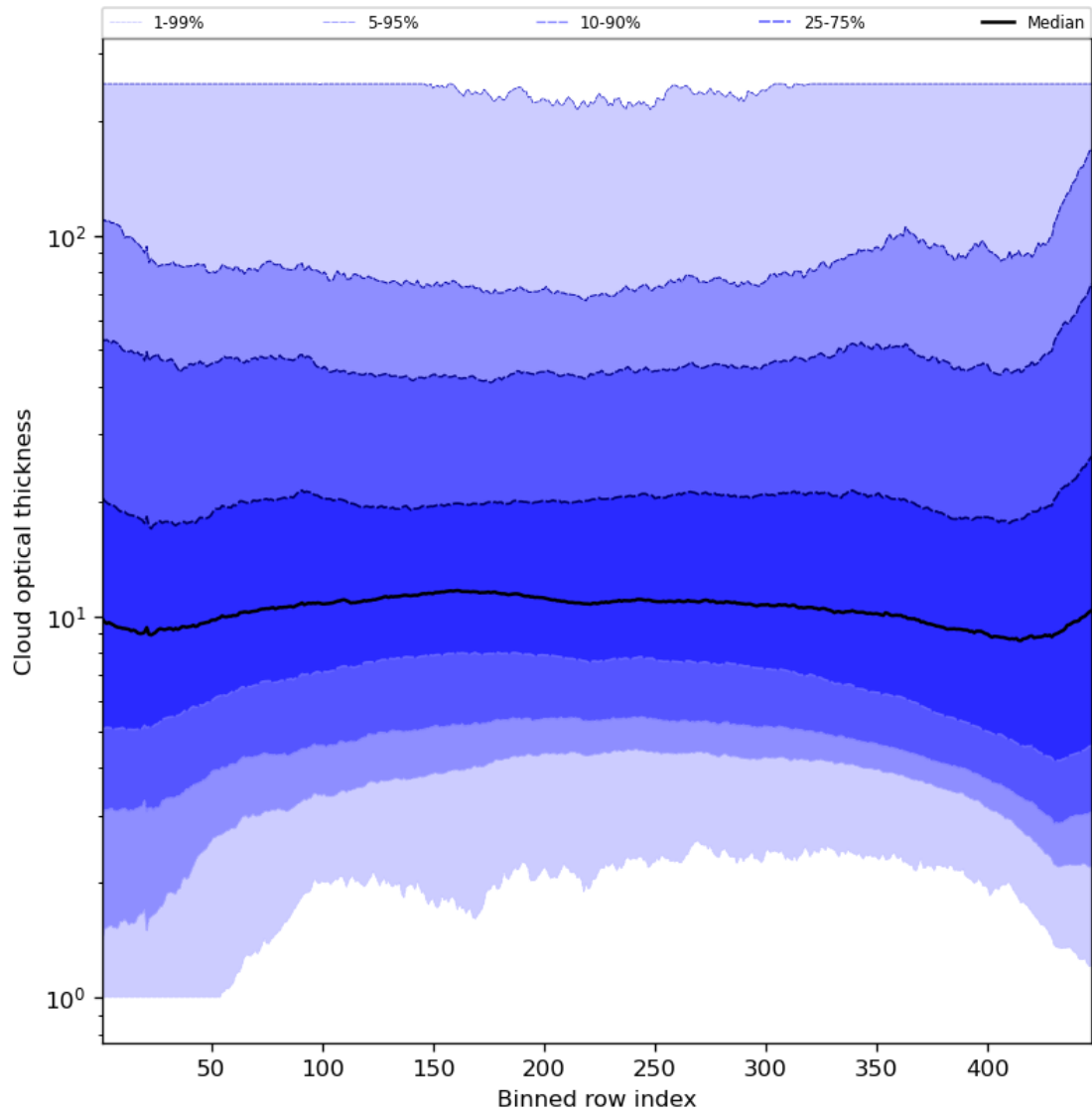
Figure 57: Along track statistics of “Cloud optical thickness” for 2024-08-08 to 2024-08-10
