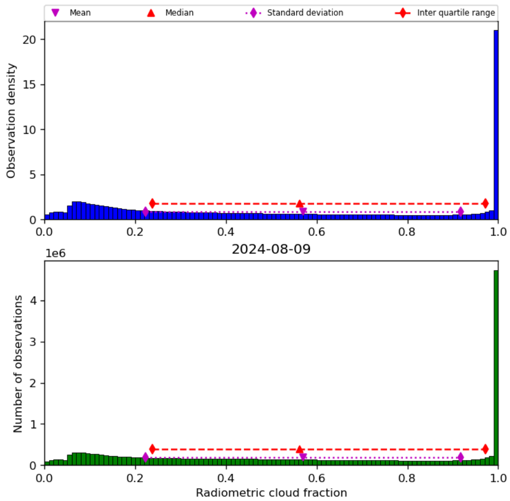
Figure 39: Histogram of “Radiometric cloud fraction” for 2024-08-08 to 2024-08-10
