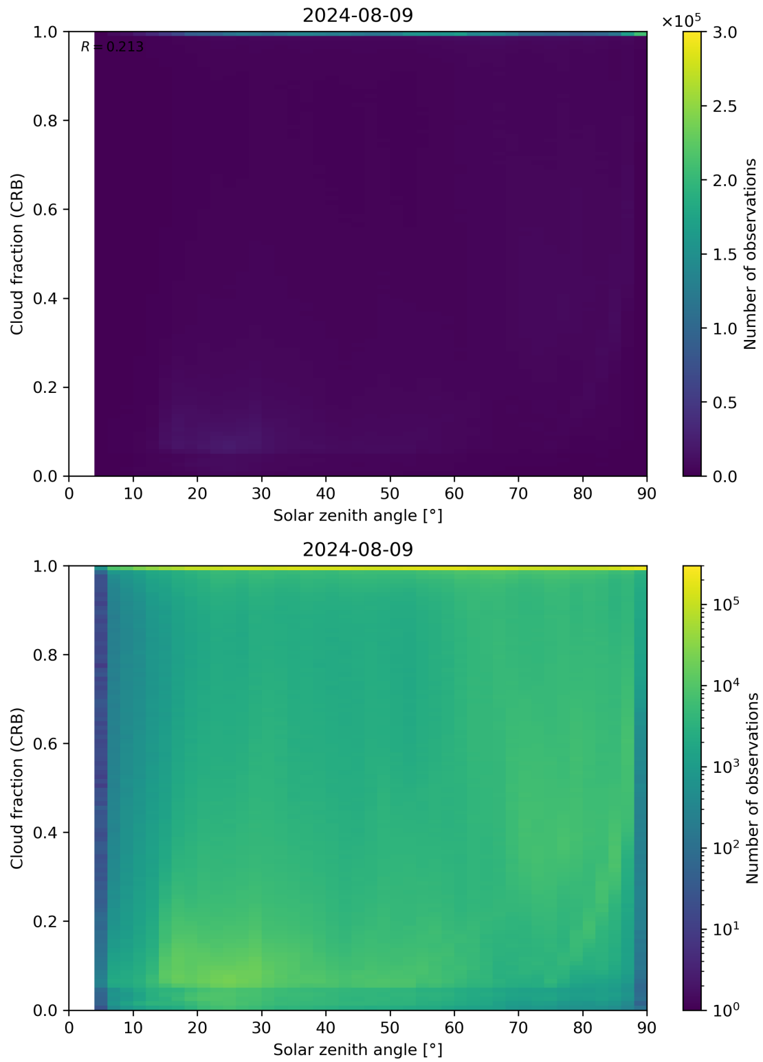
Figure 101: Scatter density plot of “Solar zenith angle” against “Cloud fraction (CRB)” for 2024-08-08 to 2024-08-10.
