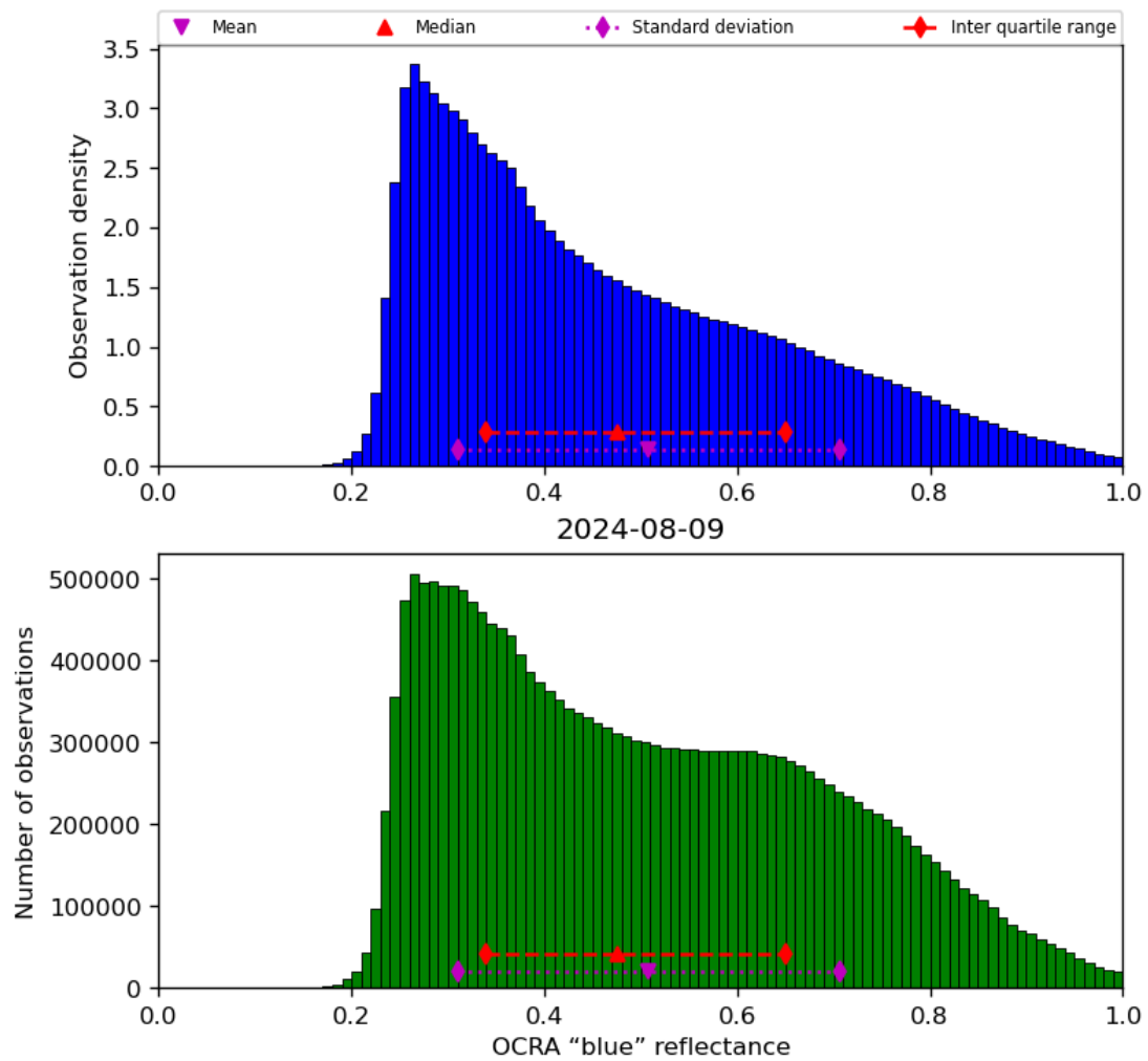
Figure 51: Histogram of “OCRA “blue” reflectance” for 2024-08-08 to 2024-08-10
