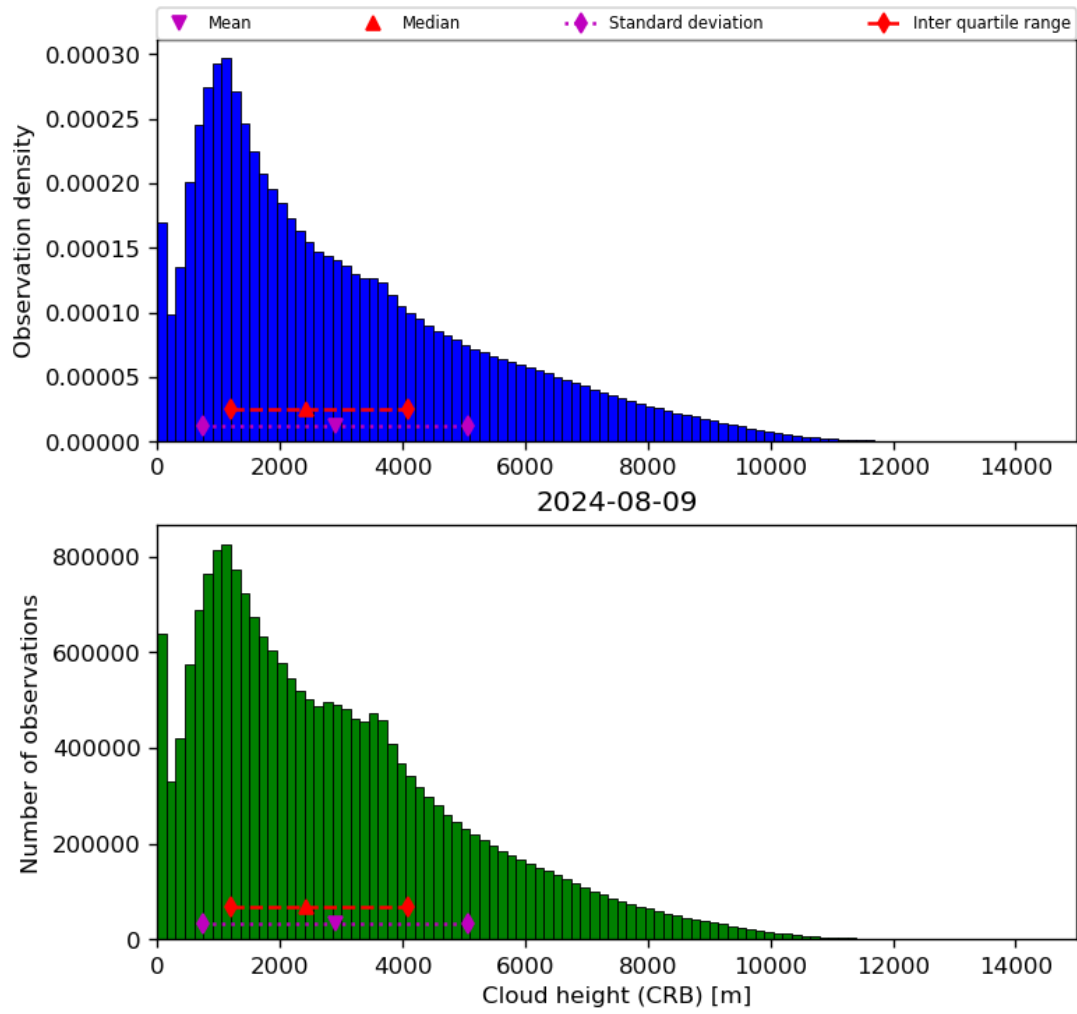
Figure 43: Histogram of “Cloud height (CRB)” for 2024-08-08 to 2024-08-10
