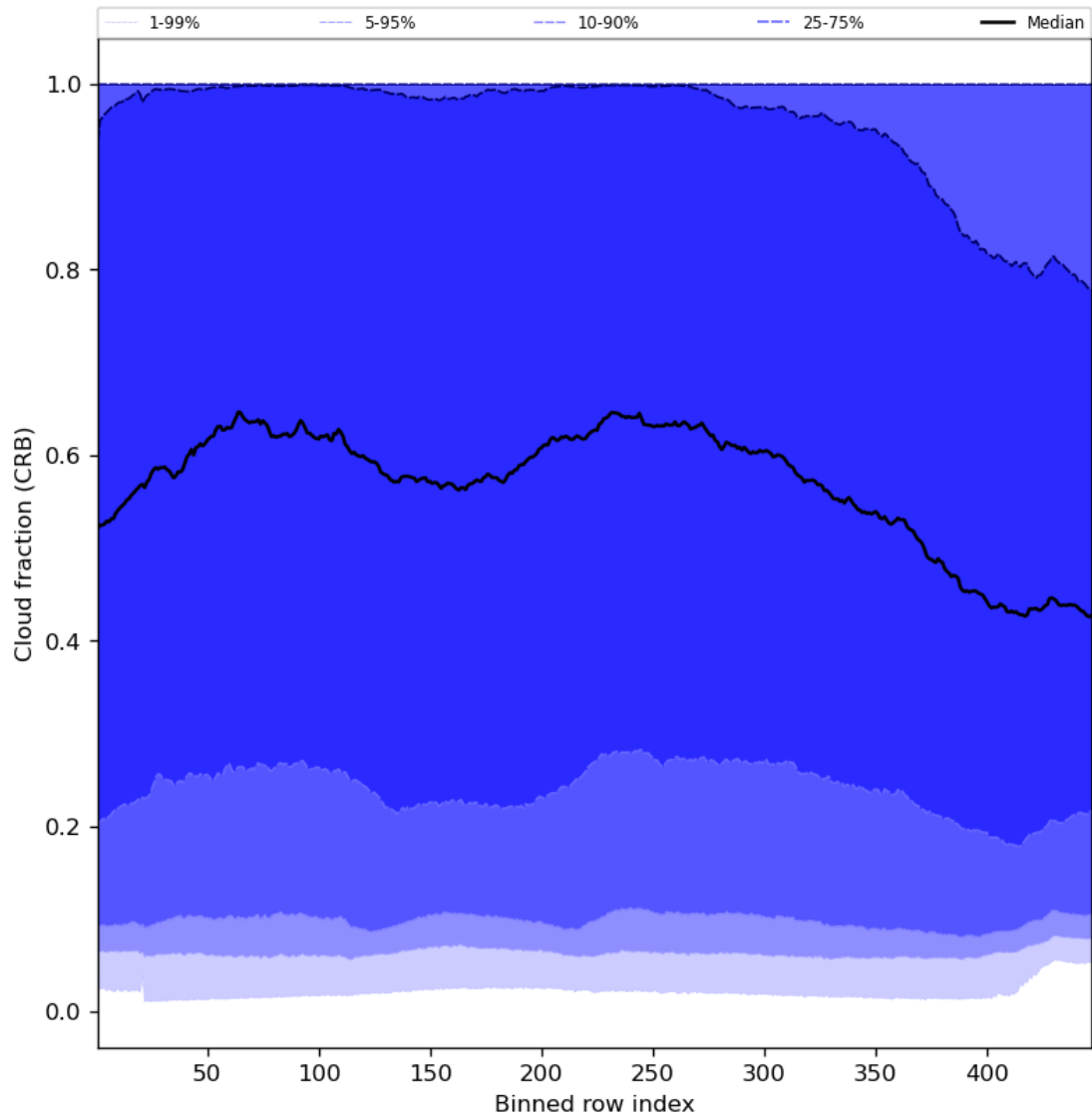
Figure 58: Along track statistics of “Cloud fraction (CRB)” for 2024-08-08 to 2024-08-10
