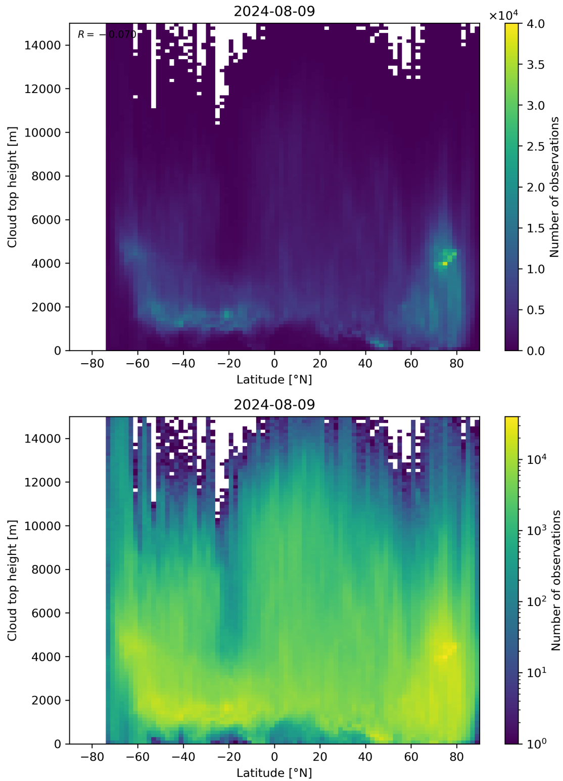
Figure 97: Scatter density plot of “Latitude” against “Cloud top height” for 2024-08-08 to 2024-08-10.
