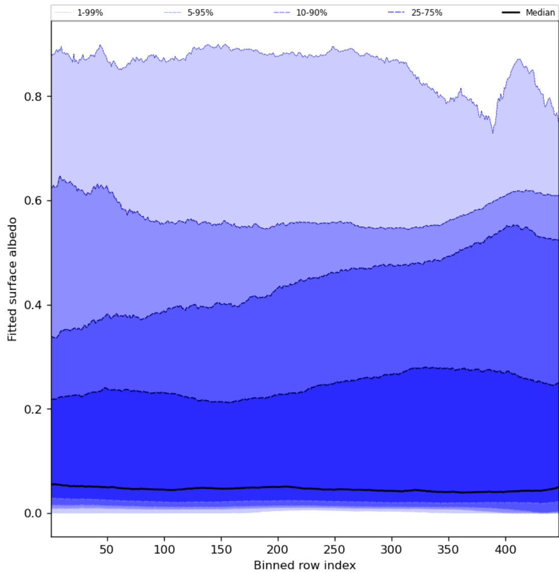
Figure 61: Along track statistics of “Fitted surface albedo” for 2024-08-08 to 2024-08-10
