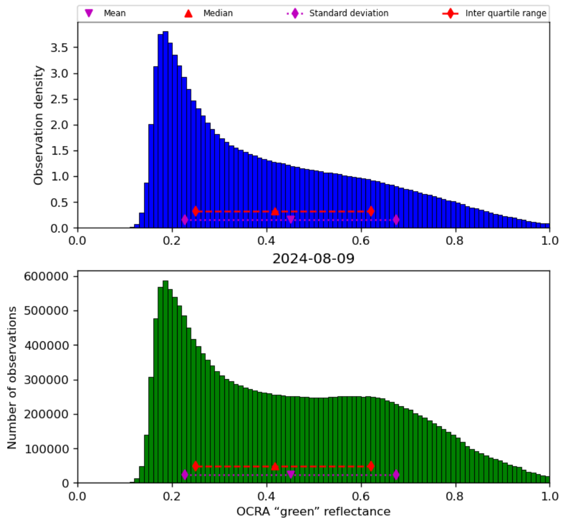
Figure 52: Histogram of “OCRA “green” reflectance” for 2024-08-08 to 2024-08-10
