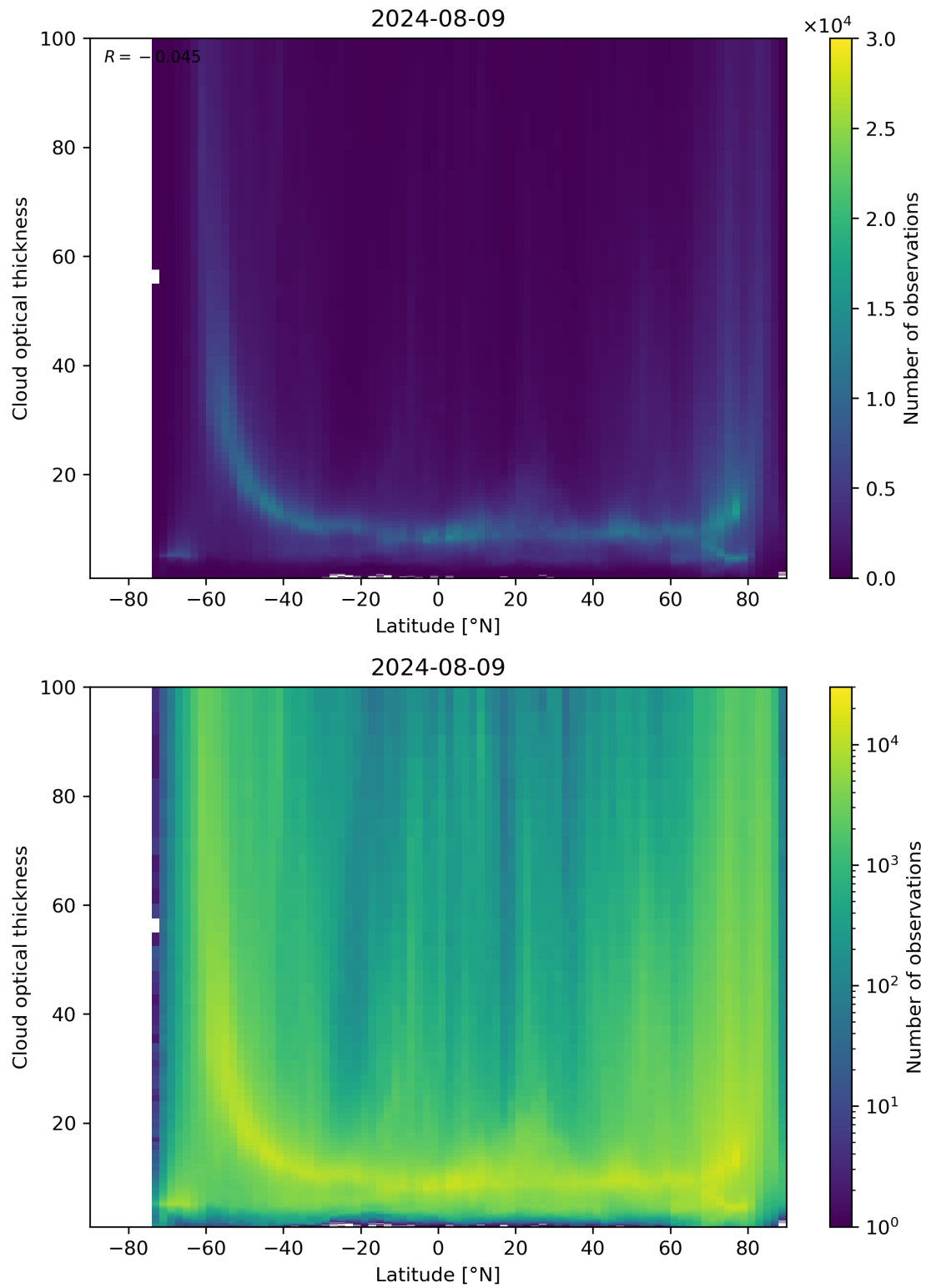
Figure 96: Scatter density plot of “Latitude” against “Cloud optical thickness” for 2024-08-08 to 2024-08-10.
