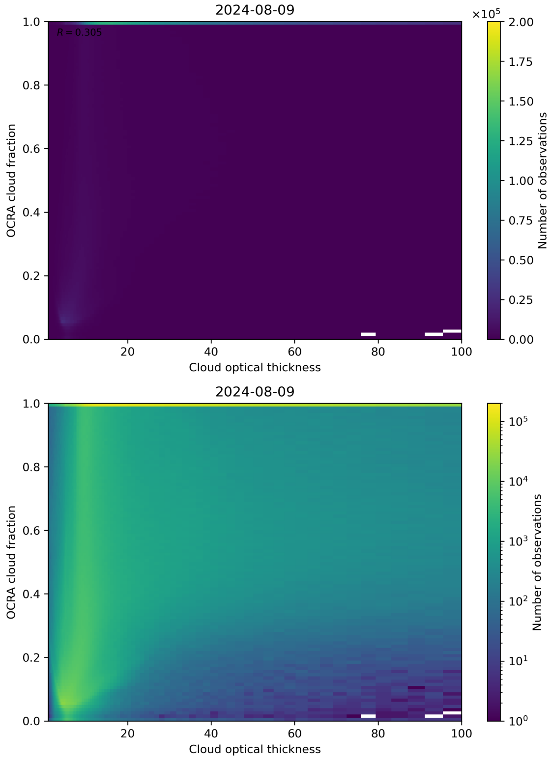
Figure 83: Scatter density plot of “Cloud optical thickness” against “OCRA cloud fraction” for 2024-08-08 to 2024-08-10.
