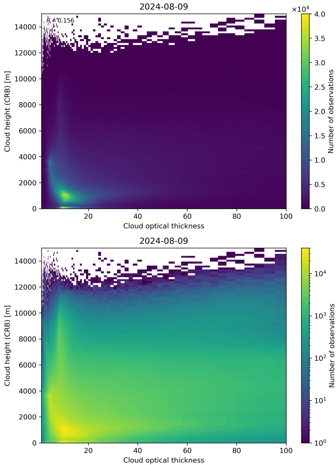
Figure 85: Scatter density plot of “Cloud optical thickness” against “Cloud height (CRB)” for 2024-08-08 to 2024-08-10.
