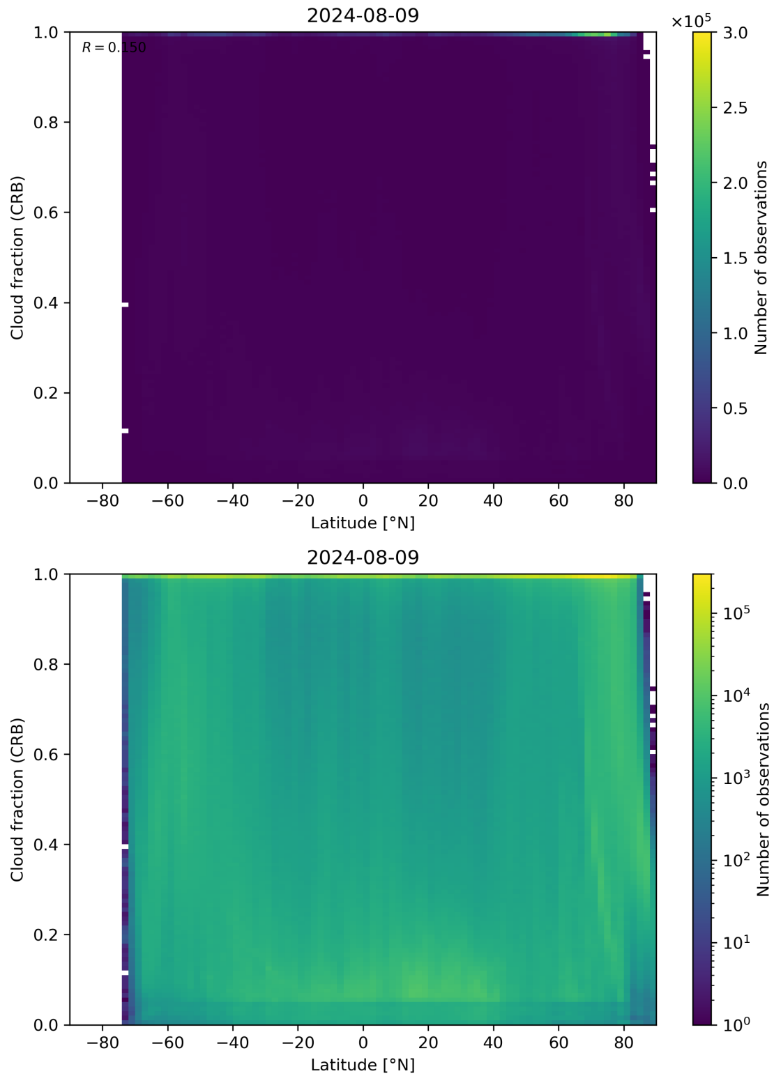
Figure 94: Scatter density plot of “Latitude” against “Cloud fraction (CRB)” for 2024-08-08 to 2024-08-10.
