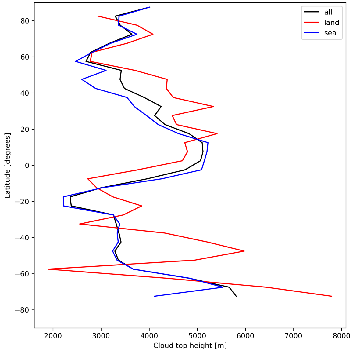
Figure 24: Zonal average of “Cloud top height” for 2024-08-08 to 2024-08-10.
