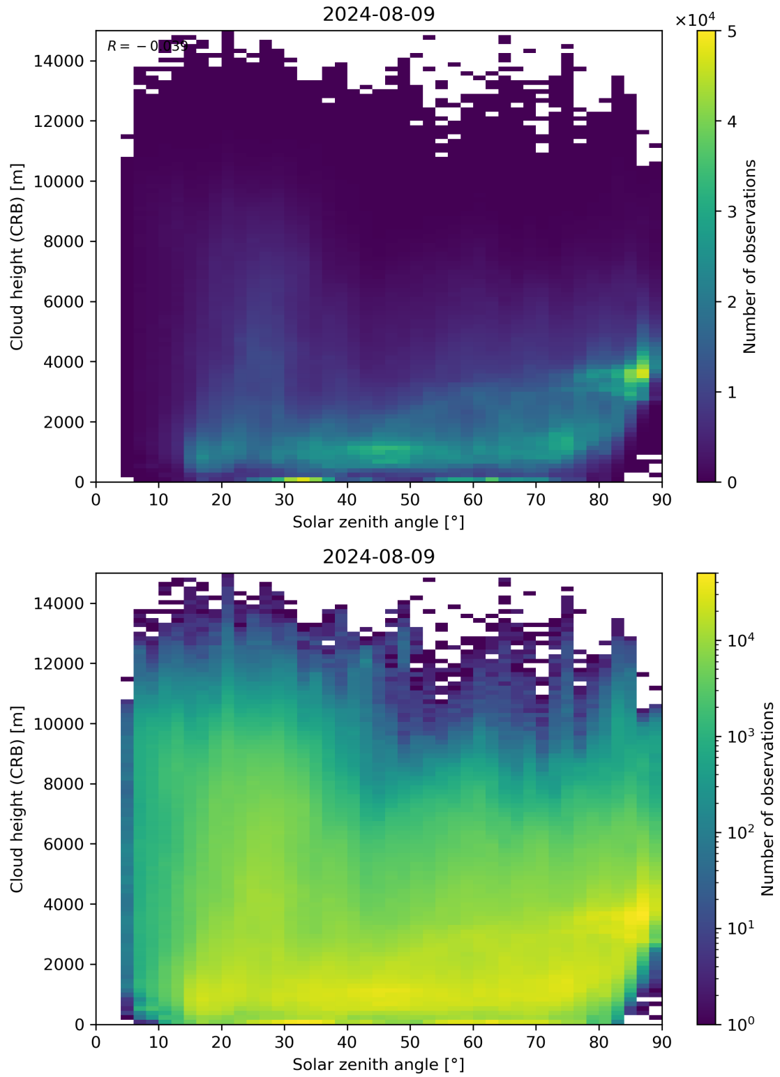
Figure 102: Scatter density plot of “Solar zenith angle” against “Cloud height (CRB)” for 2024-08-08 to 2024-08-10.
