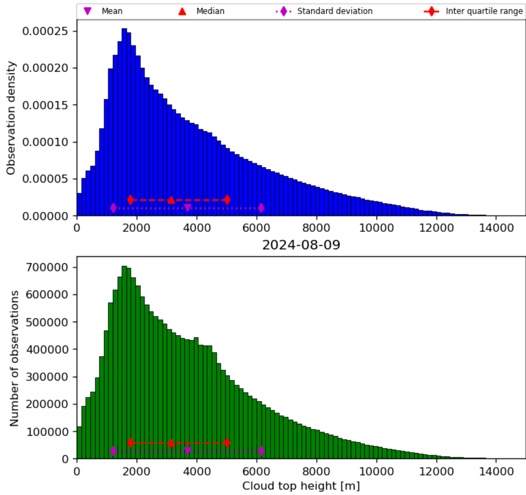
Figure 40: Histogram of “Cloud top height” for 2024-08-08 to 2024-08-10
