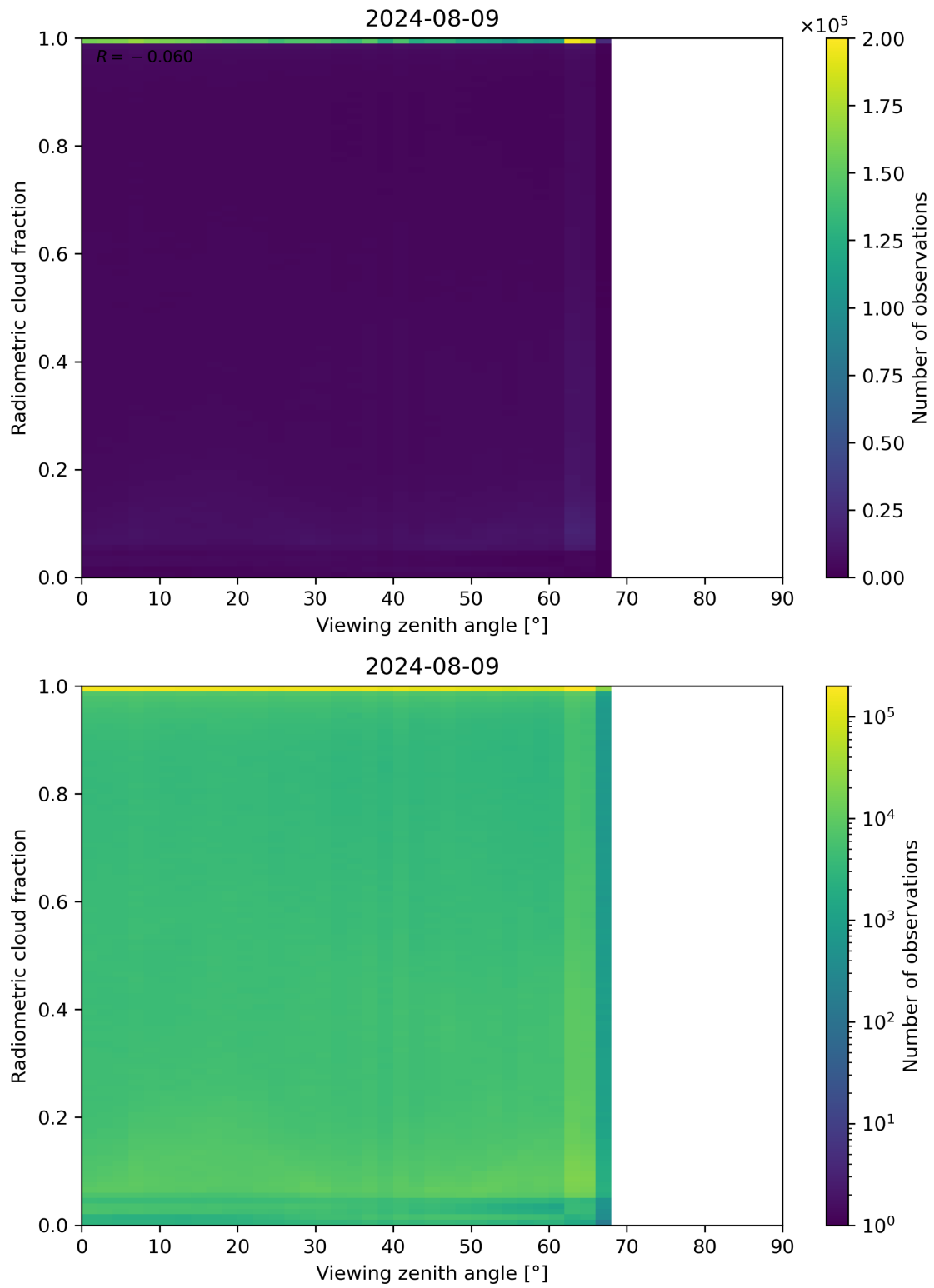
Figure 107: Scatter density plot of “Viewing zenith angle” against “Radiometric cloud fraction” for 2024-08-08 to 2024-08-10.
