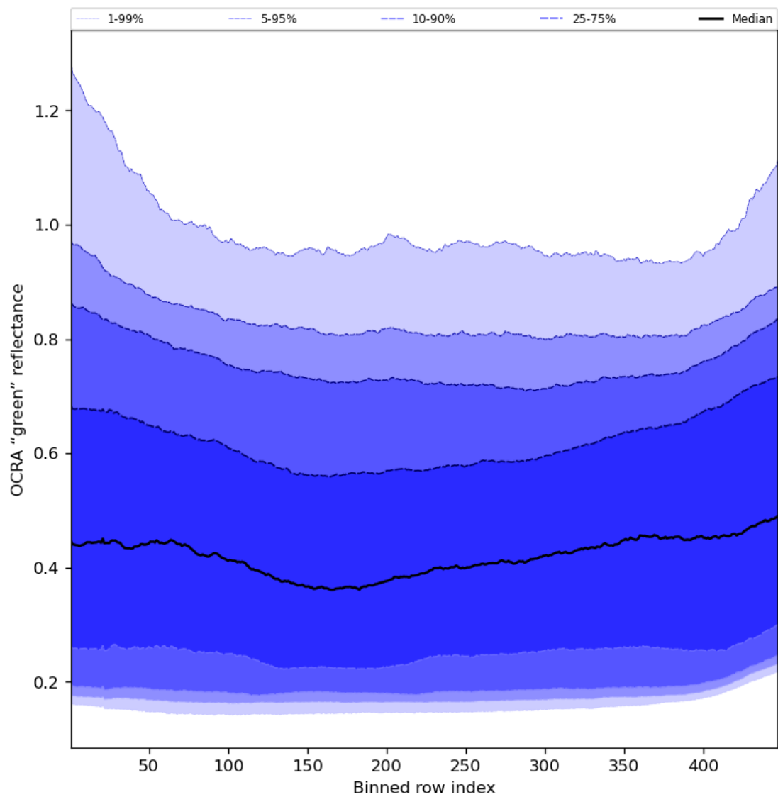
Figure 68: Along track statistics of “OCRA “green” reflectance” for 2024-08-08 to 2024-08-10
