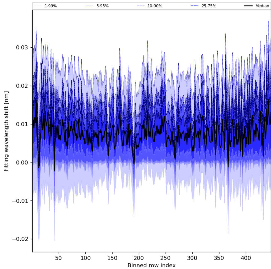
Figure 65: Along track statistics of “Fitting wavelength shift” for 2024-08-08 to 2024-08-10
