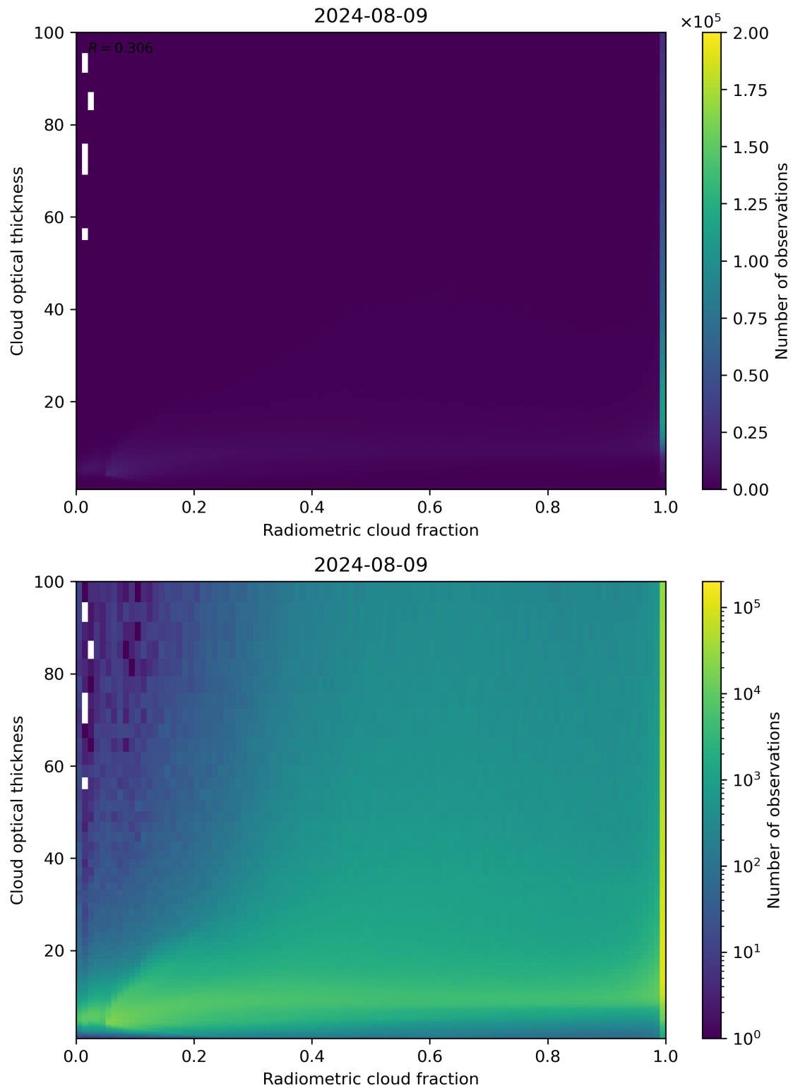
Figure 75: Scatter density plot of “Radiometric cloud fraction” against “Cloud optical thickness” for 2024-08-08 to 2024-08-10.
