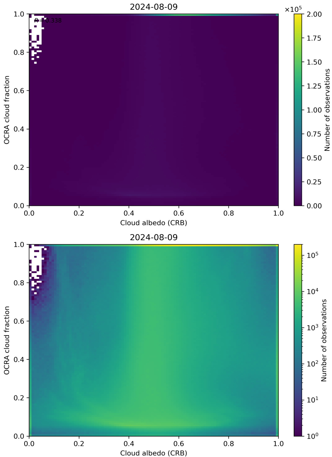
Figure 70: Scatter density plot of “Cloud albedo (CRB)” against “OCRA cloud fraction” for 2024-08-08 to 2024-08-10.
