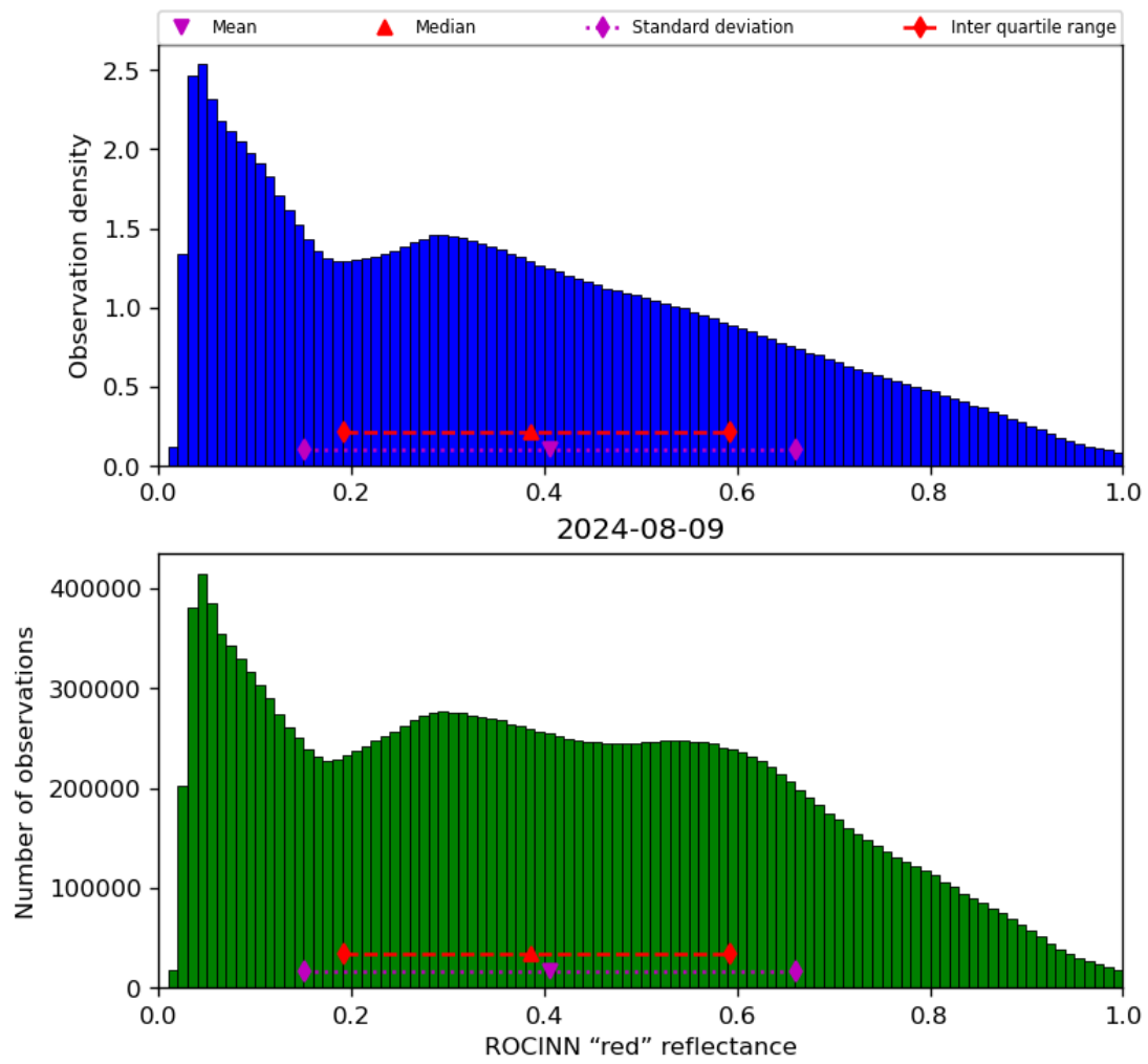
Figure 53: Histogram of “ROCINN “red” reflectance” for 2024-08-08 to 2024-08-10
