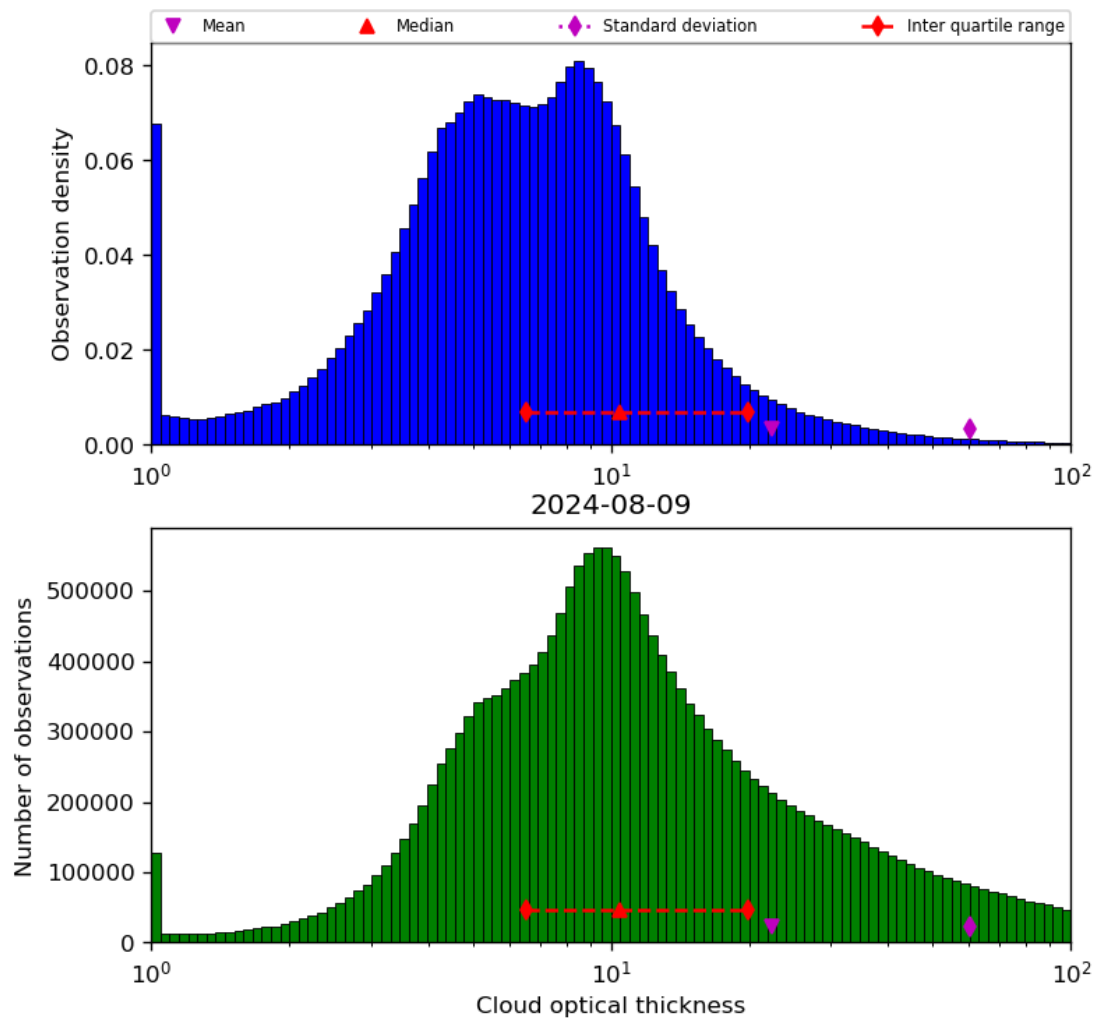
Figure 41: Histogram of “Cloud optical thickness” for 2024-08-08 to 2024-08-10
