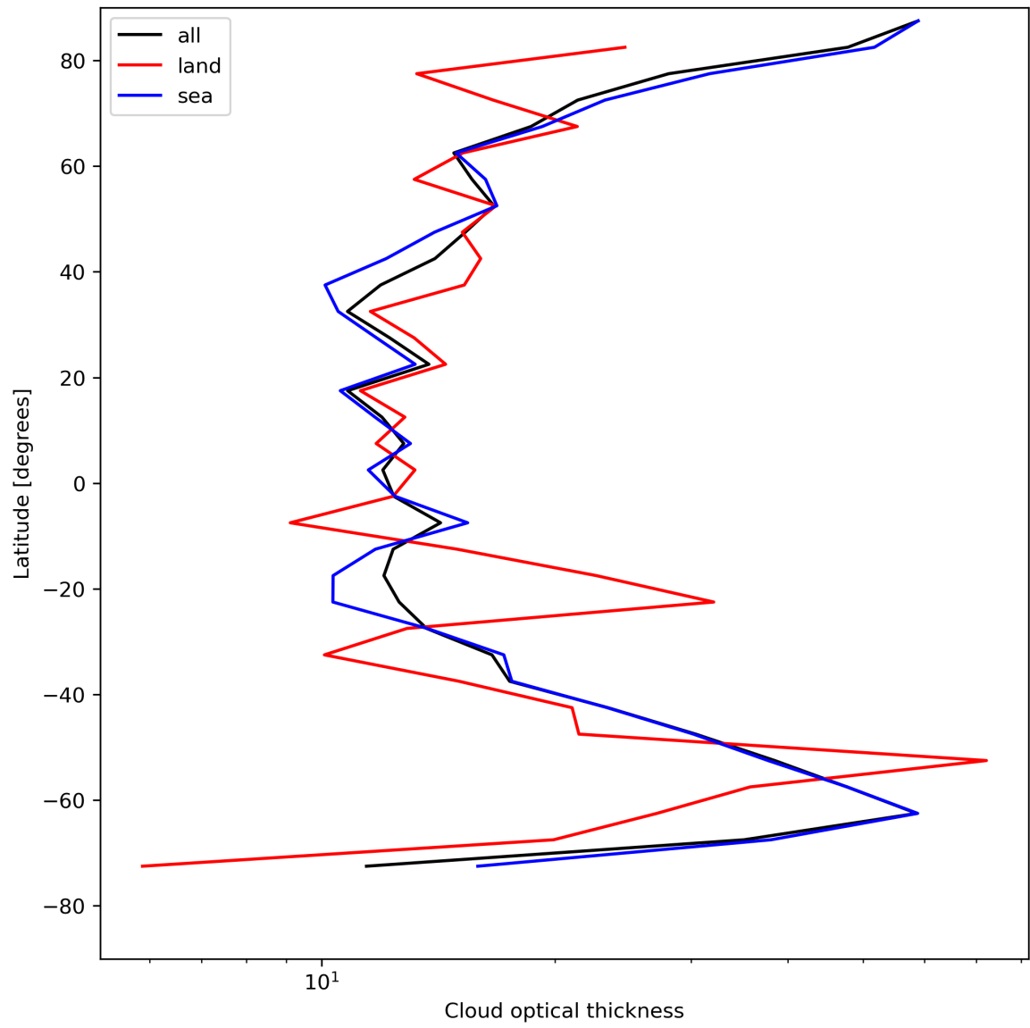
Figure 25: Zonal average of “Cloud optical thickness” for 2024-08-08 to 2024-08-10.
