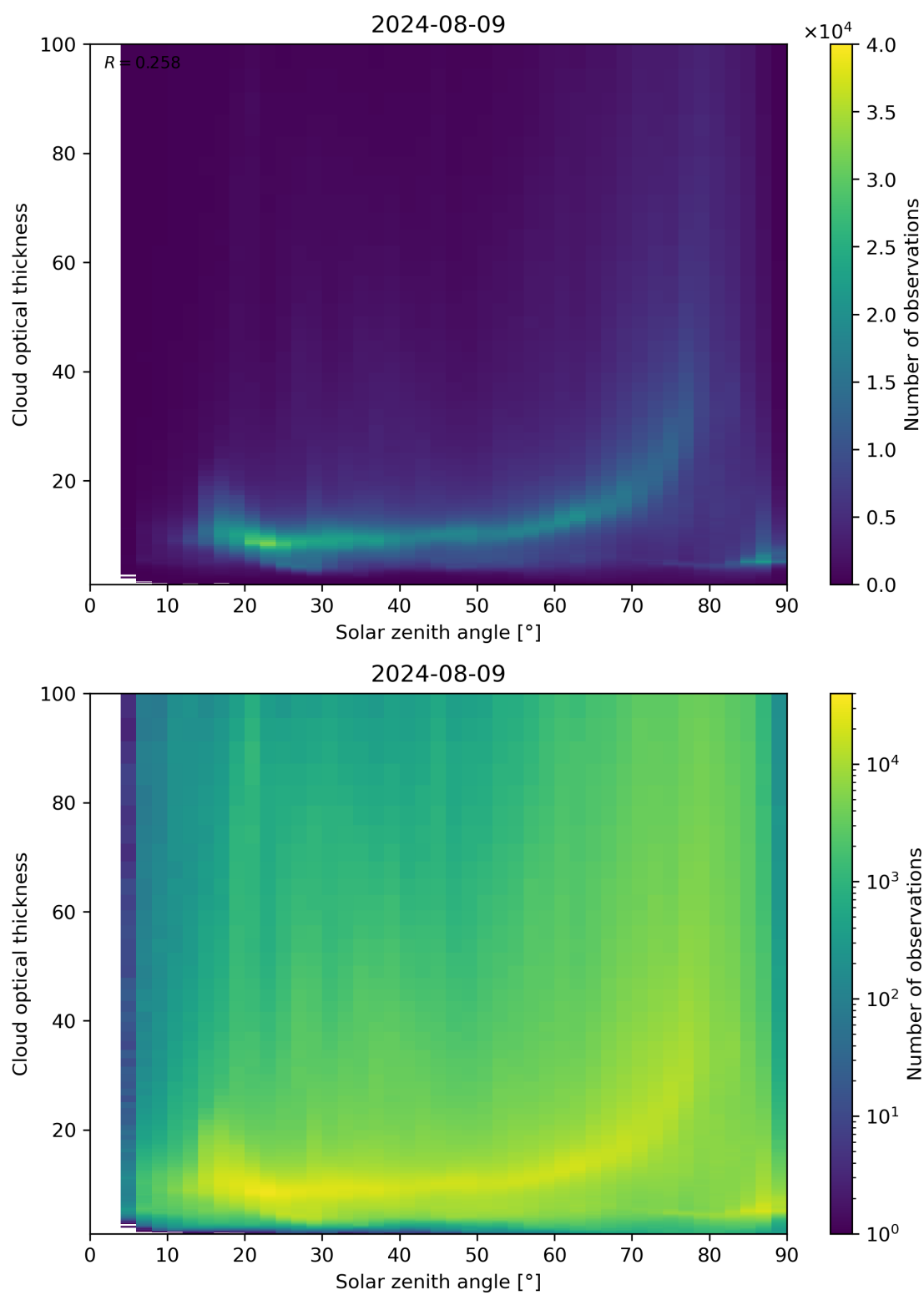
Figure 103: Scatter density plot of “Solar zenith angle” against “Cloud optical thickness” for 2024-08-08 to 2024-08-10.
