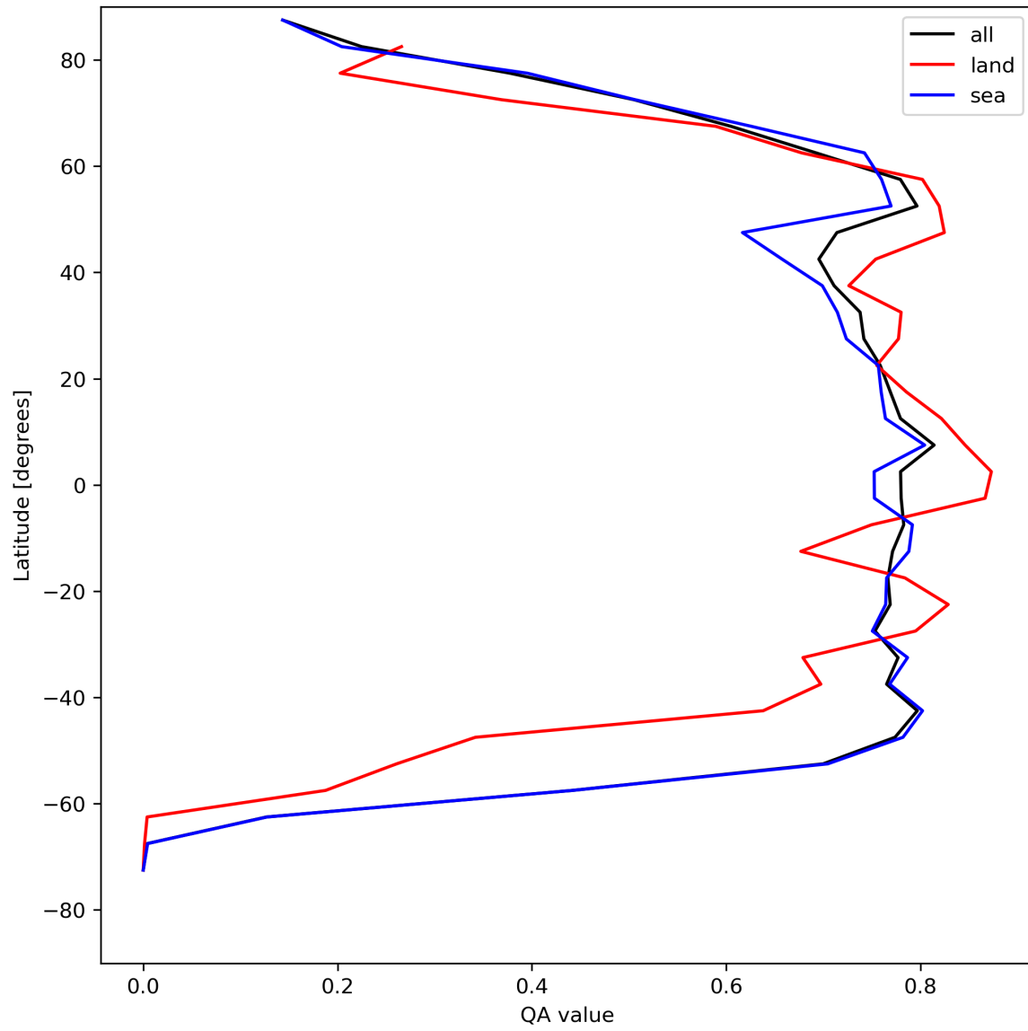
Figure 22: Zonal average of “QA value” for 2024-08-08 to 2024-08-10.
