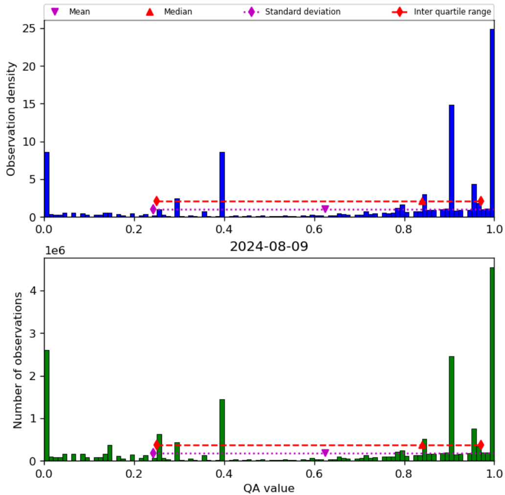
Figure 38: Histogram of “QA value” for 2024-08-08 to 2024-08-10
