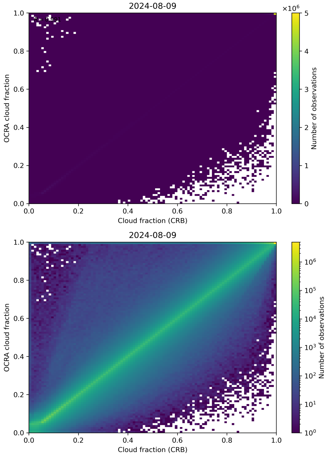
Figure 78: Scatter density plot of “Cloud fraction (CRB)” against “OCRA cloud fraction” for 2024-08-08 to 2024-08-10.
