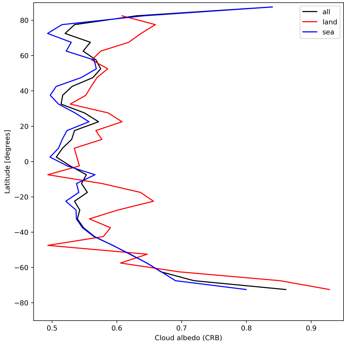
Figure 28: Zonal average of “Cloud albedo (CRB)” for 2024-08-08 to 2024-08-10.
