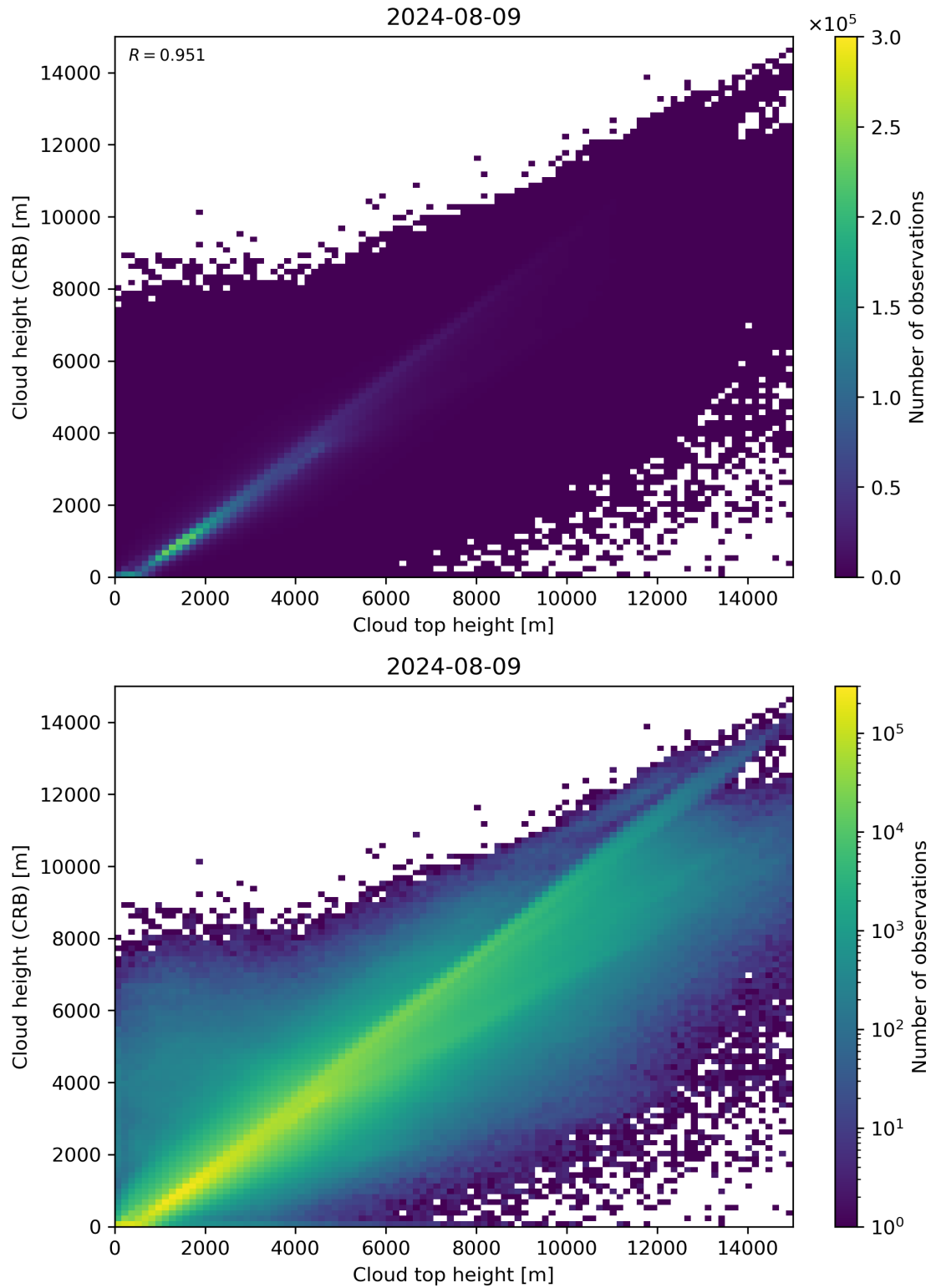
Figure 89: Scatter density plot of “Cloud top height” against “Cloud height (CRB)” for 2024-08-08 to 2024-08-10.
