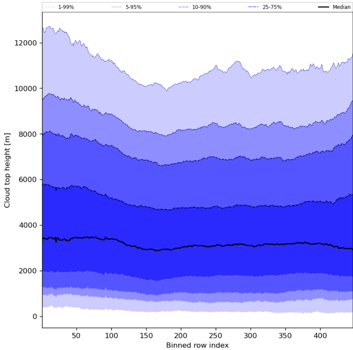
Figure 56: Along track statistics of “Cloud top height” for 2024-08-08 to 2024-08-10
