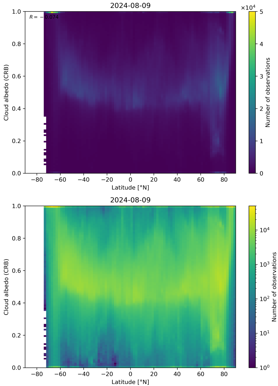
Figure 91: Scatter density plot of “Latitude” against “Cloud albedo (CRB)” for 2024-08-08 to 2024-08-10.
