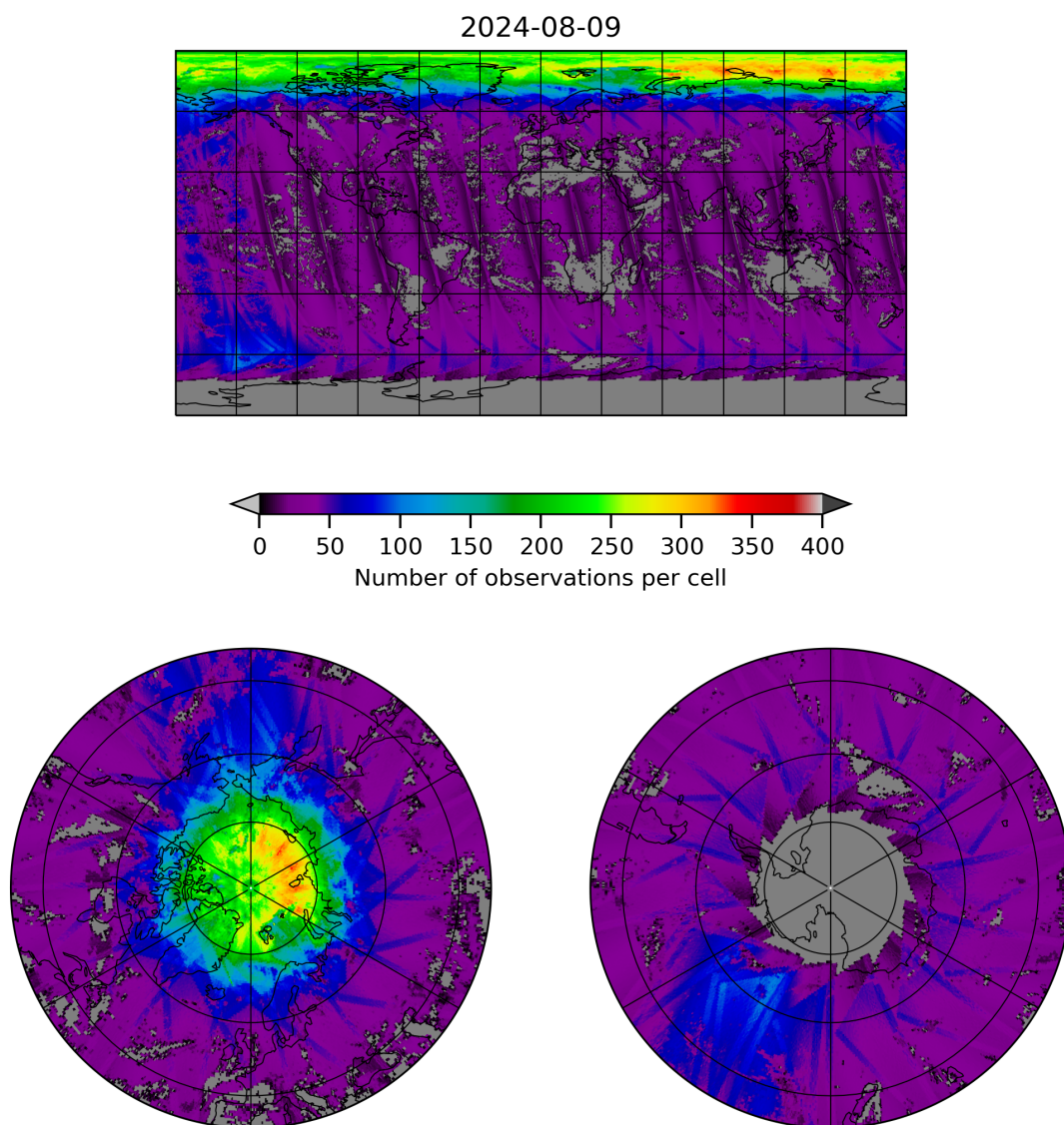
Figure 21: Map of the number of observations for 2024-08-08 to 2024-08-10
