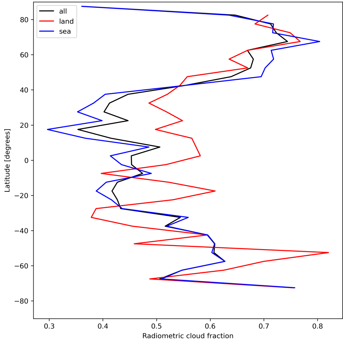
Figure 23: Zonal average of “Radiometric cloud fraction” for 2024-08-08 to 2024-08-10.
