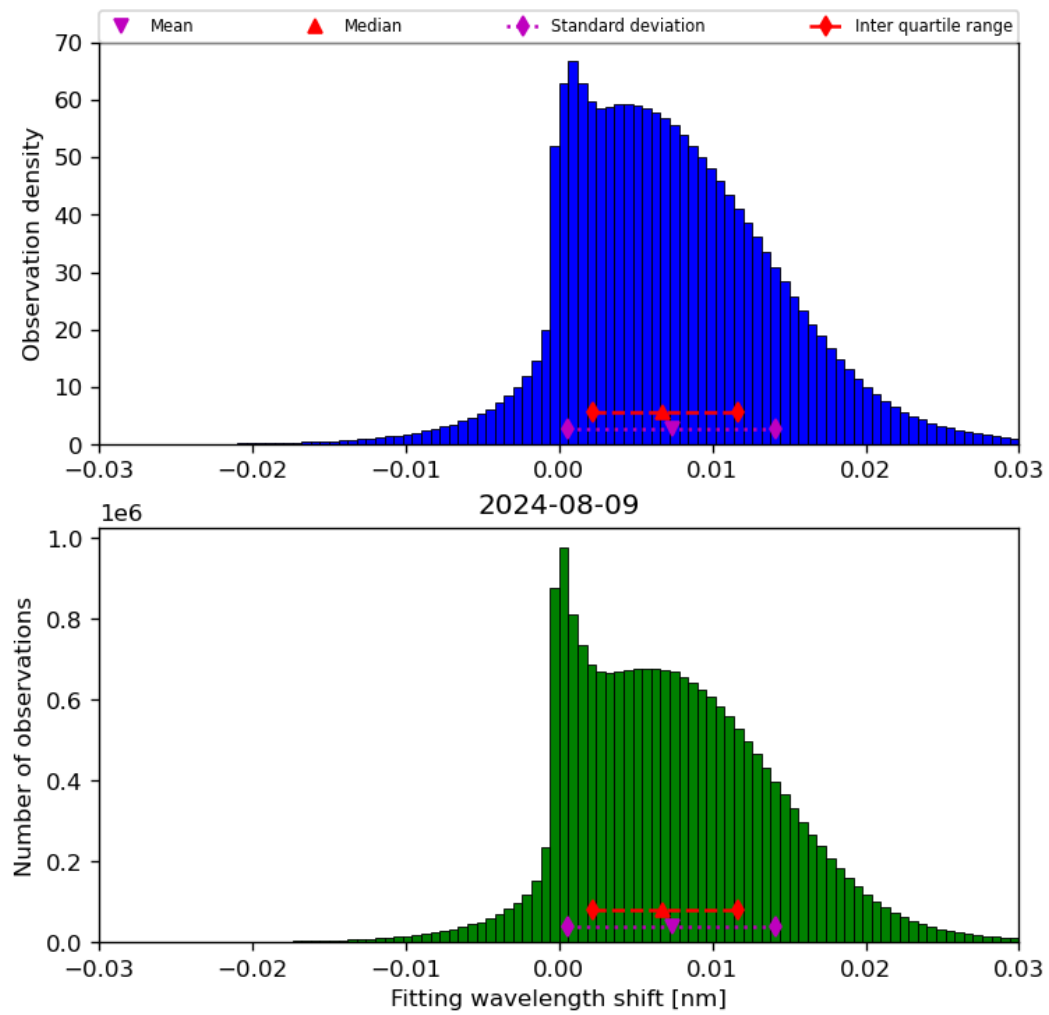
Figure 49: Histogram of “Fitting wavelength shift” for 2024-08-08 to 2024-08-10
