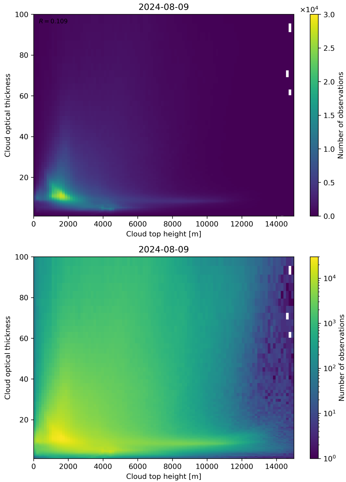
Figure 90: Scatter density plot of “Cloud top height” against “Cloud optical thickness” for 2024-08-08 to 2024-08-10.
