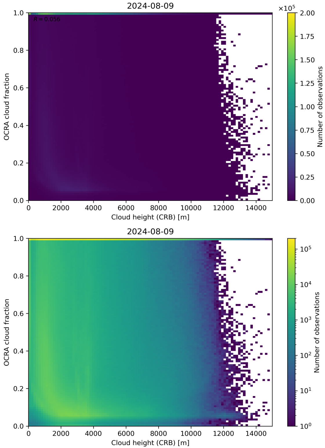
Figure 81: Scatter density plot of “Cloud height (CRB)” against “OCRA cloud fraction” for 2024-08-08 to 2024-08-10.
