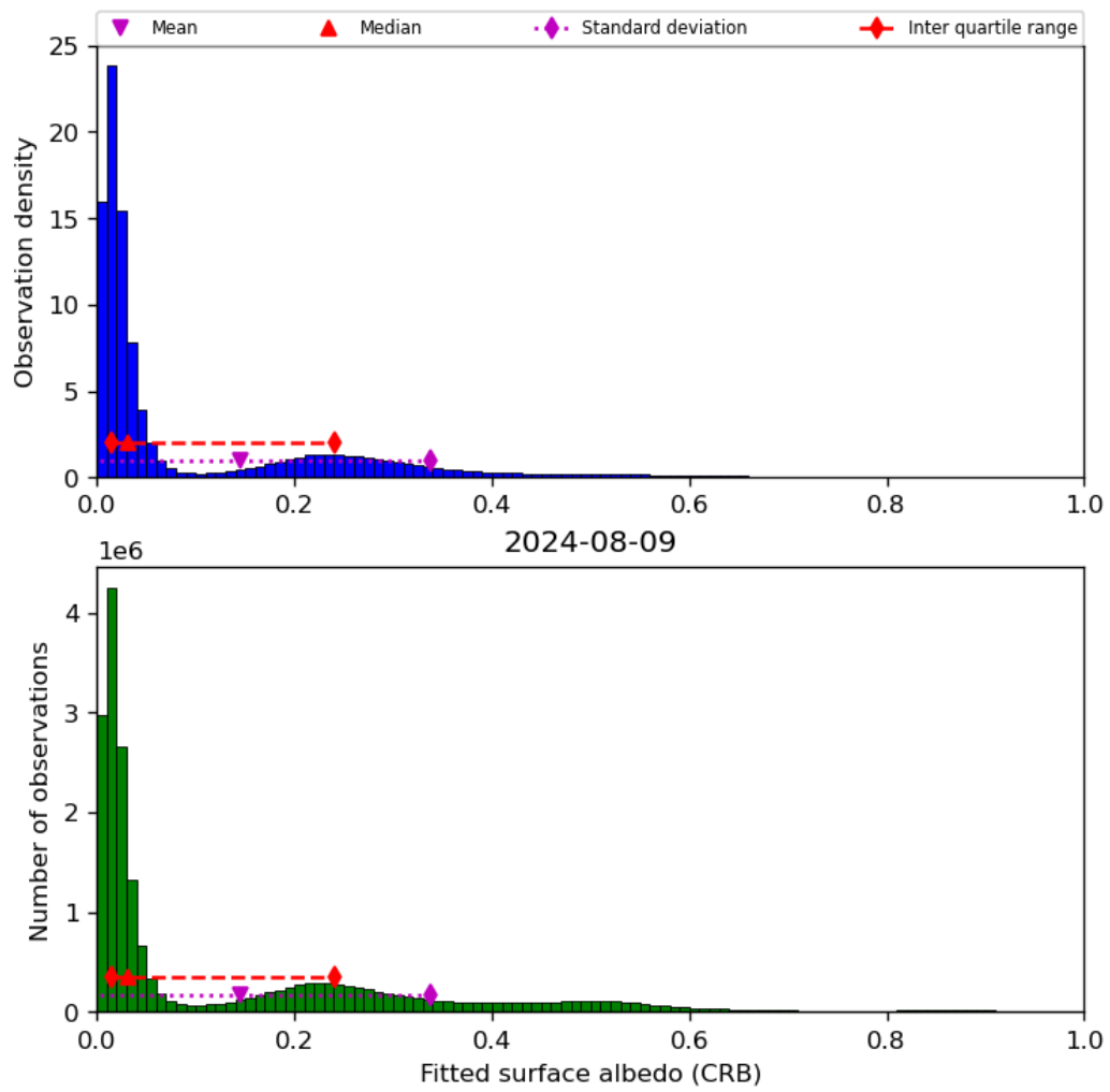
Figure 46: Histogram of “Fitted surface albedo (CRB)” for 2024-08-08 to 2024-08-10
