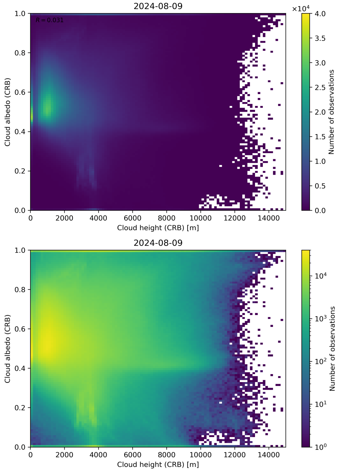
Figure 80: Scatter density plot of “Cloud height (CRB)” against “Cloud albedo (CRB)” for 2024-08-08 to 2024-08-10.
