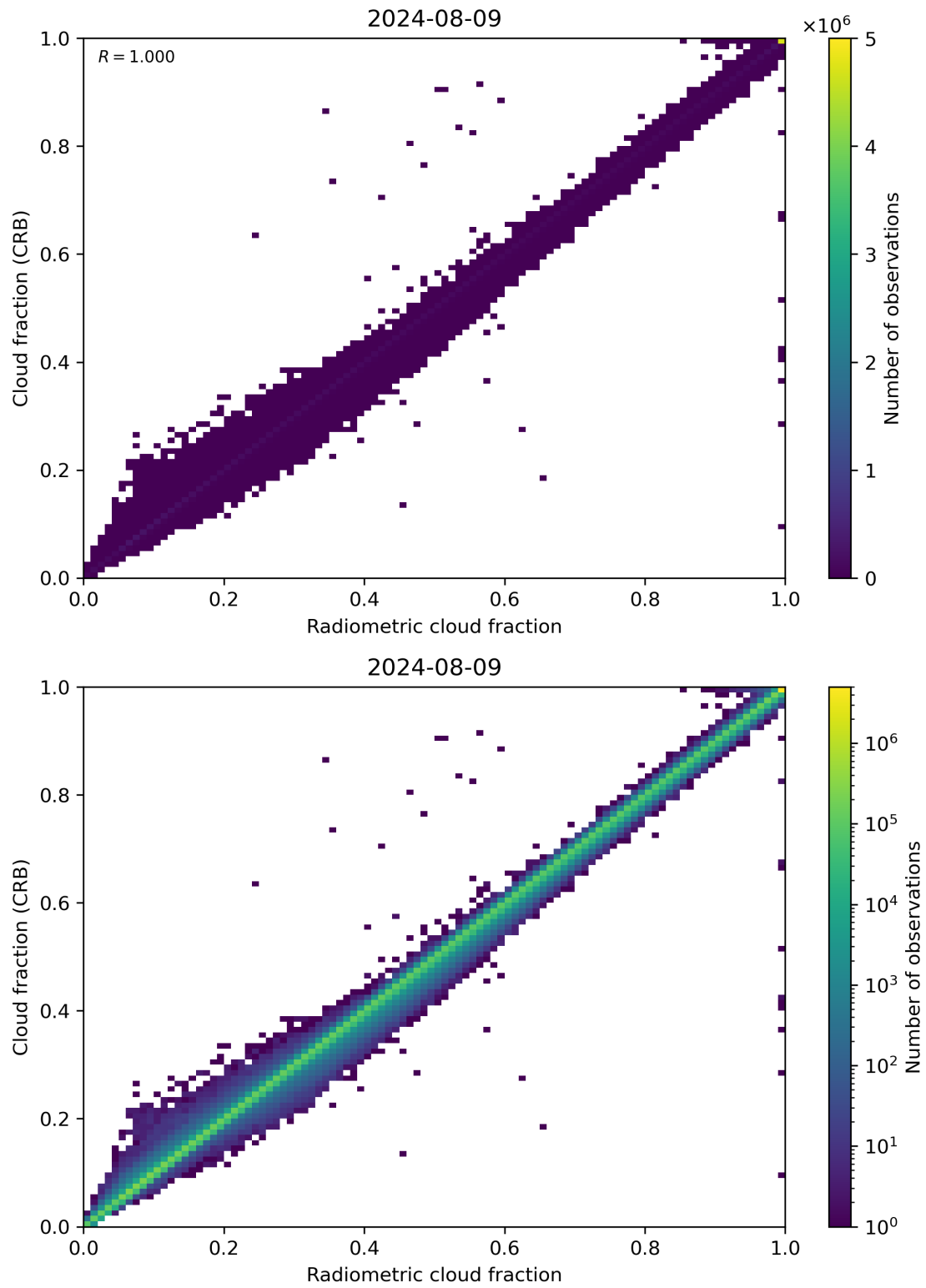
Figure 73: Scatter density plot of “Radiometric cloud fraction” against “Cloud fraction (CRB)” for 2024-08-08 to 2024-08-10.
