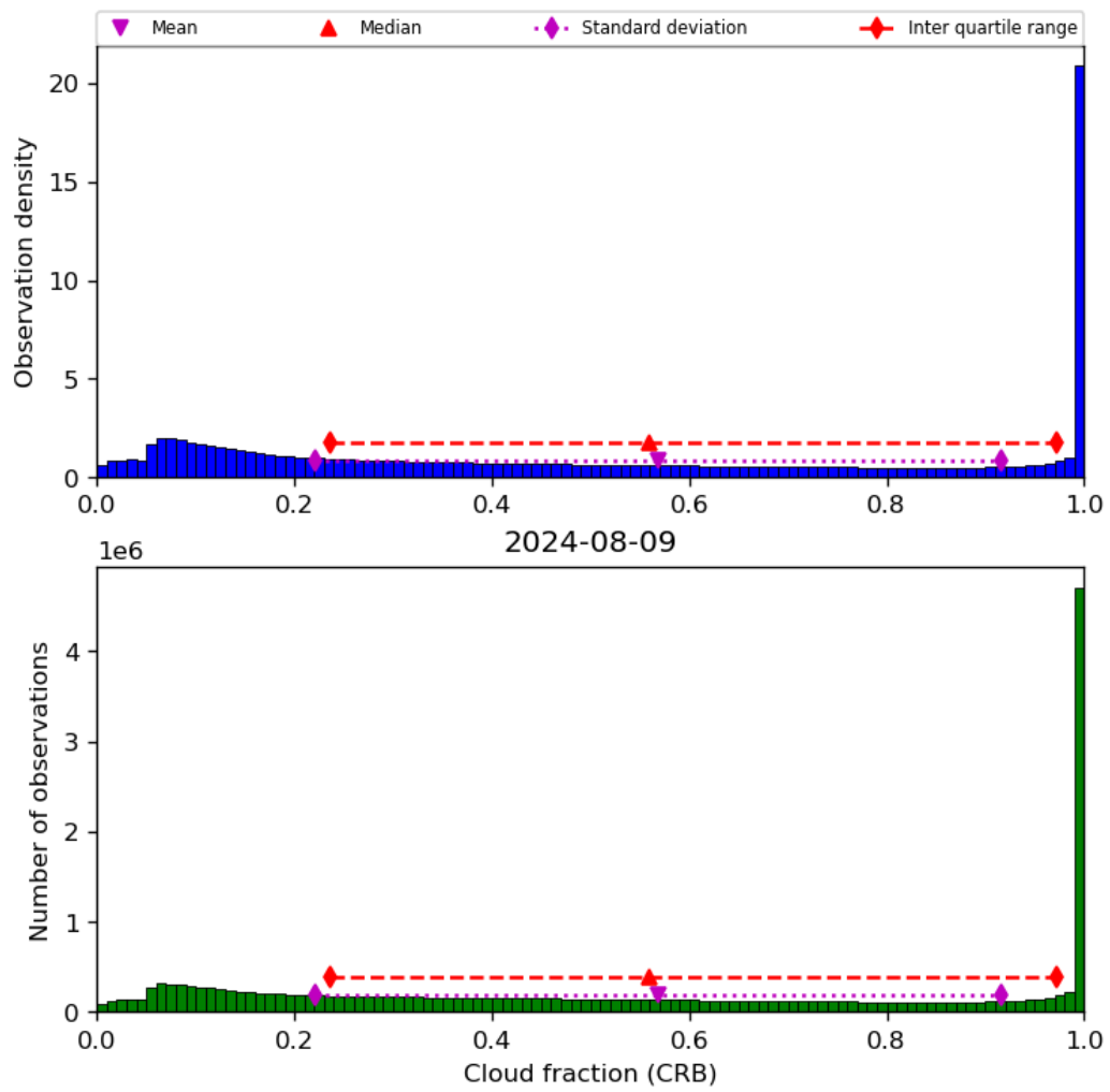
Figure 42: Histogram of “Cloud fraction (CRB)” for 2024-08-08 to 2024-08-10
