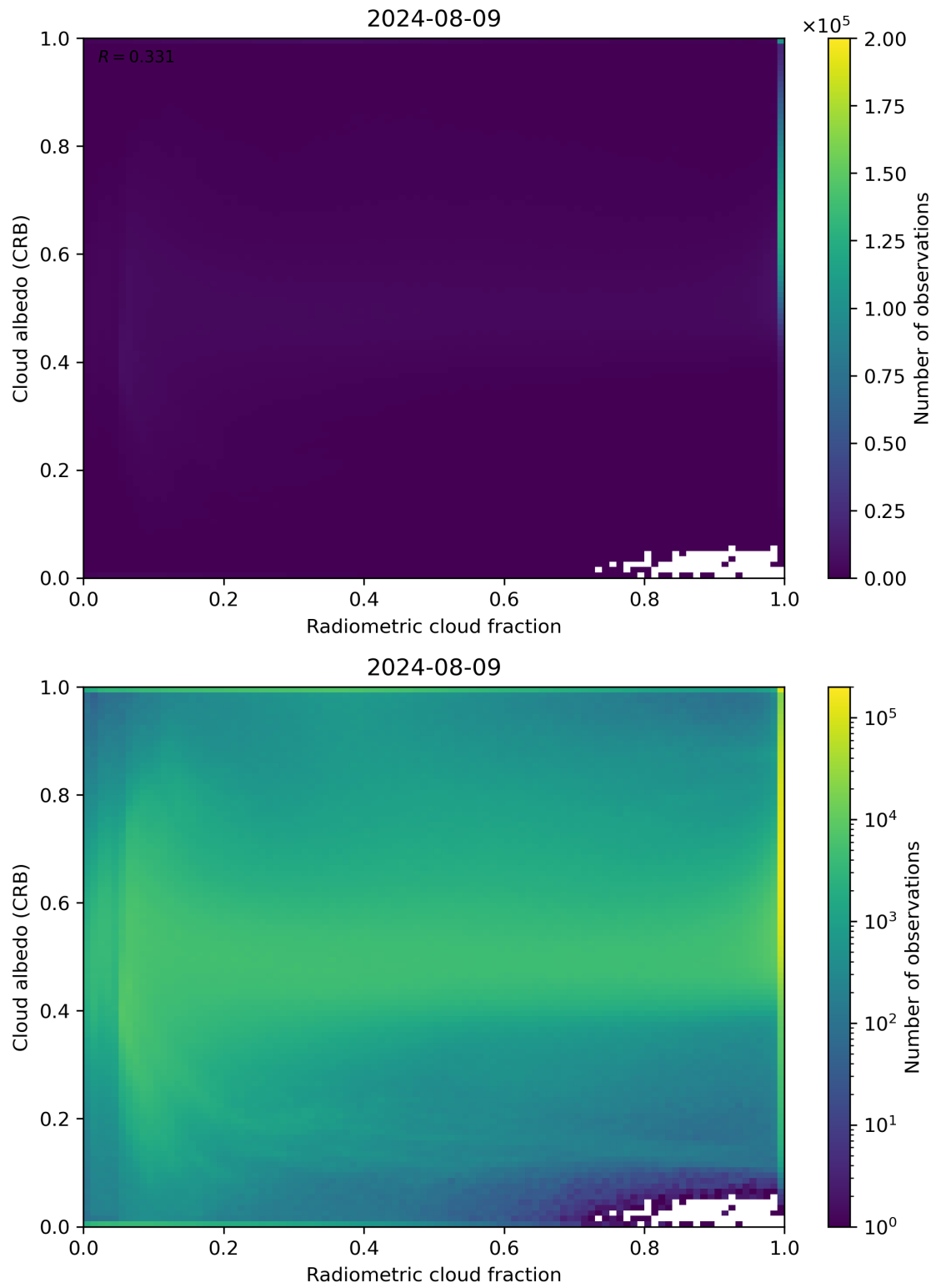
Figure 71: Scatter density plot of “Radiometric cloud fraction” against “Cloud albedo (CRB)” for 2024-08-08 to 2024-08-10.
