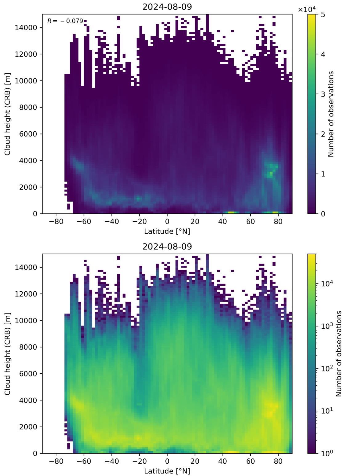
Figure 95: Scatter density plot of “Latitude” against “Cloud height (CRB)” for 2024-08-08 to 2024-08-10.
