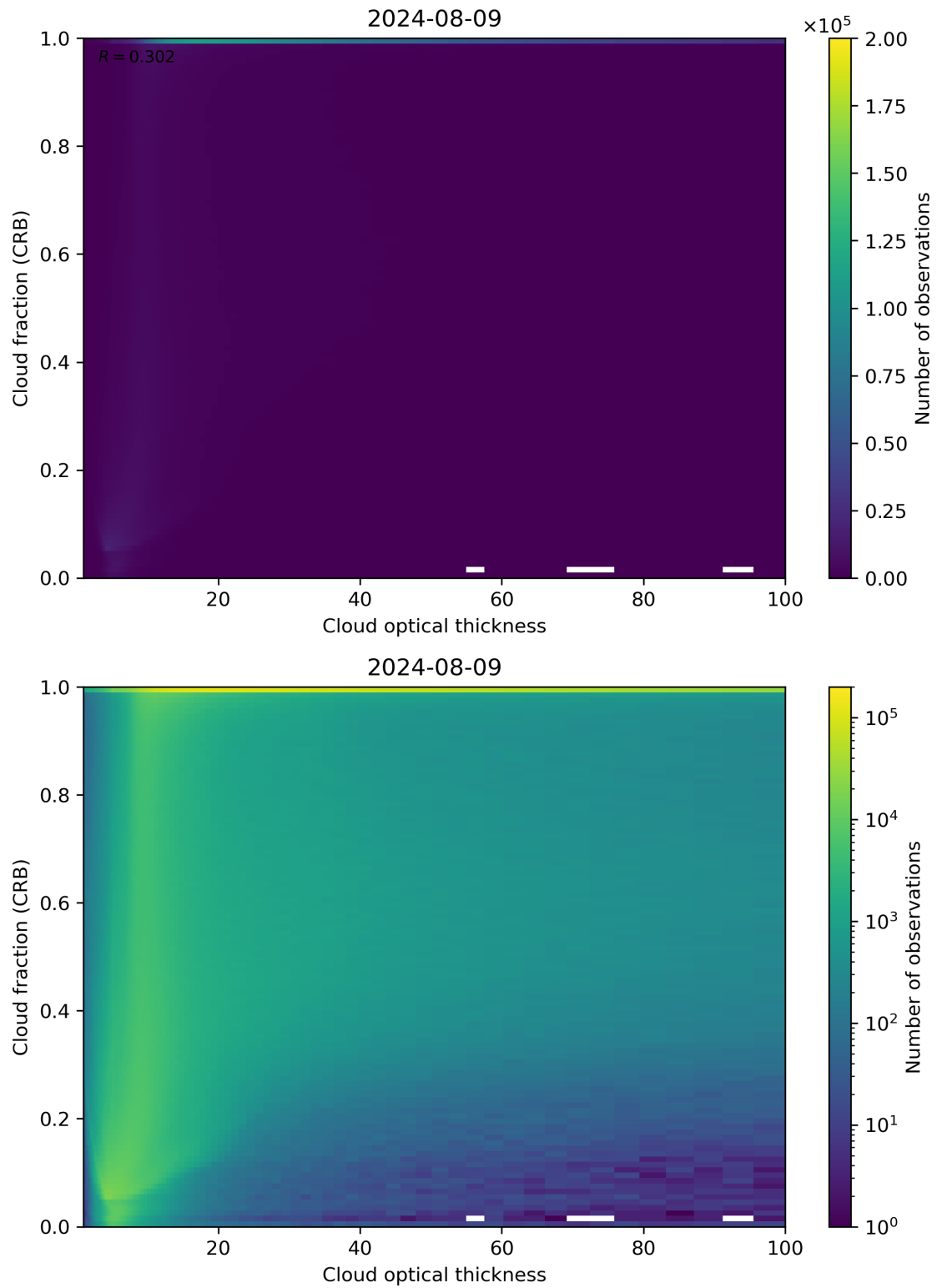
Figure 84: Scatter density plot of “Cloud optical thickness” against “Cloud fraction (CRB)” for 2024-08-08 to 2024-08-10.
