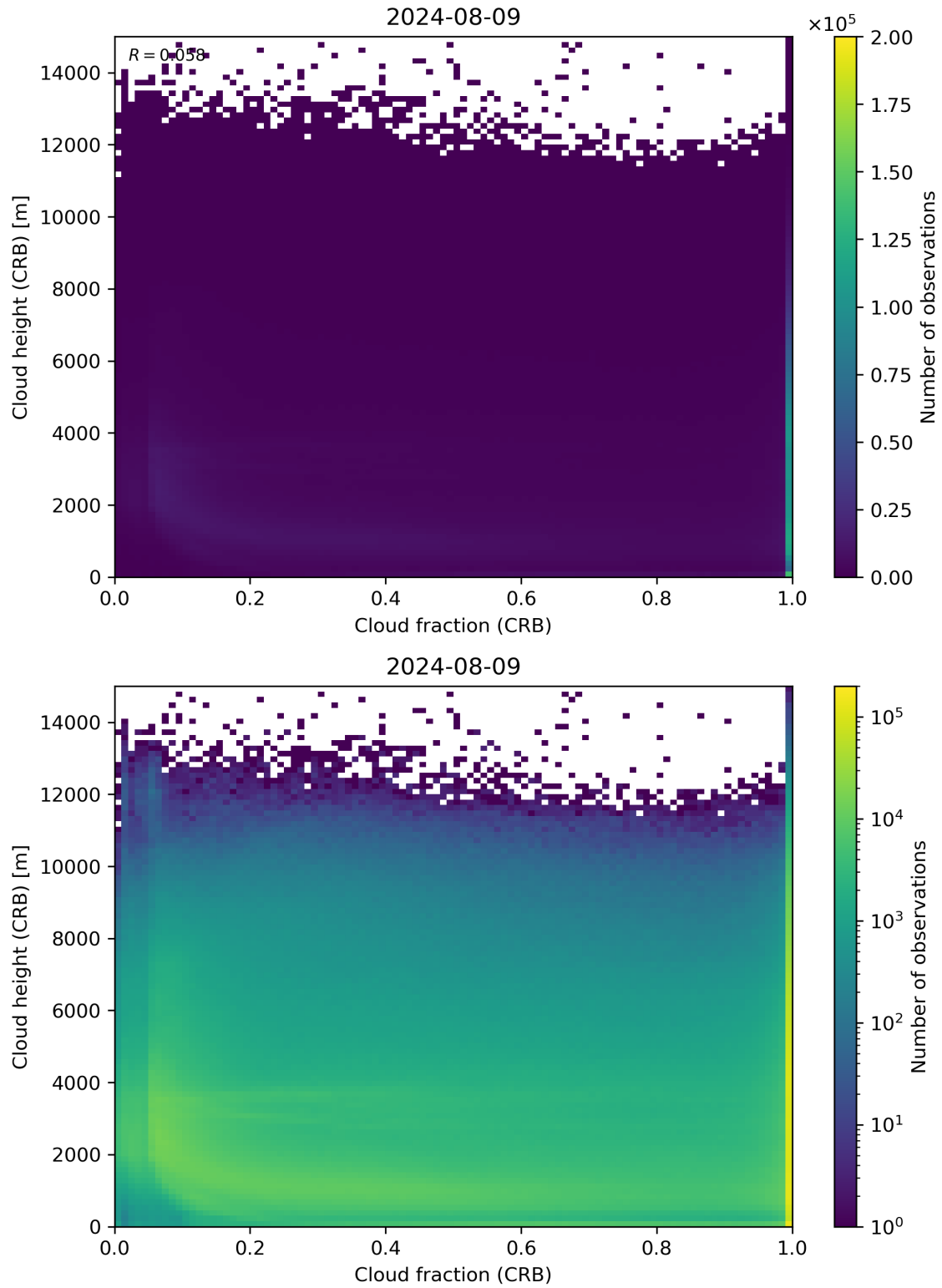
Figure 79: Scatter density plot of “Cloud fraction (CRB)” against “Cloud height (CRB)” for 2024-08-08 to 2024-08-10.
