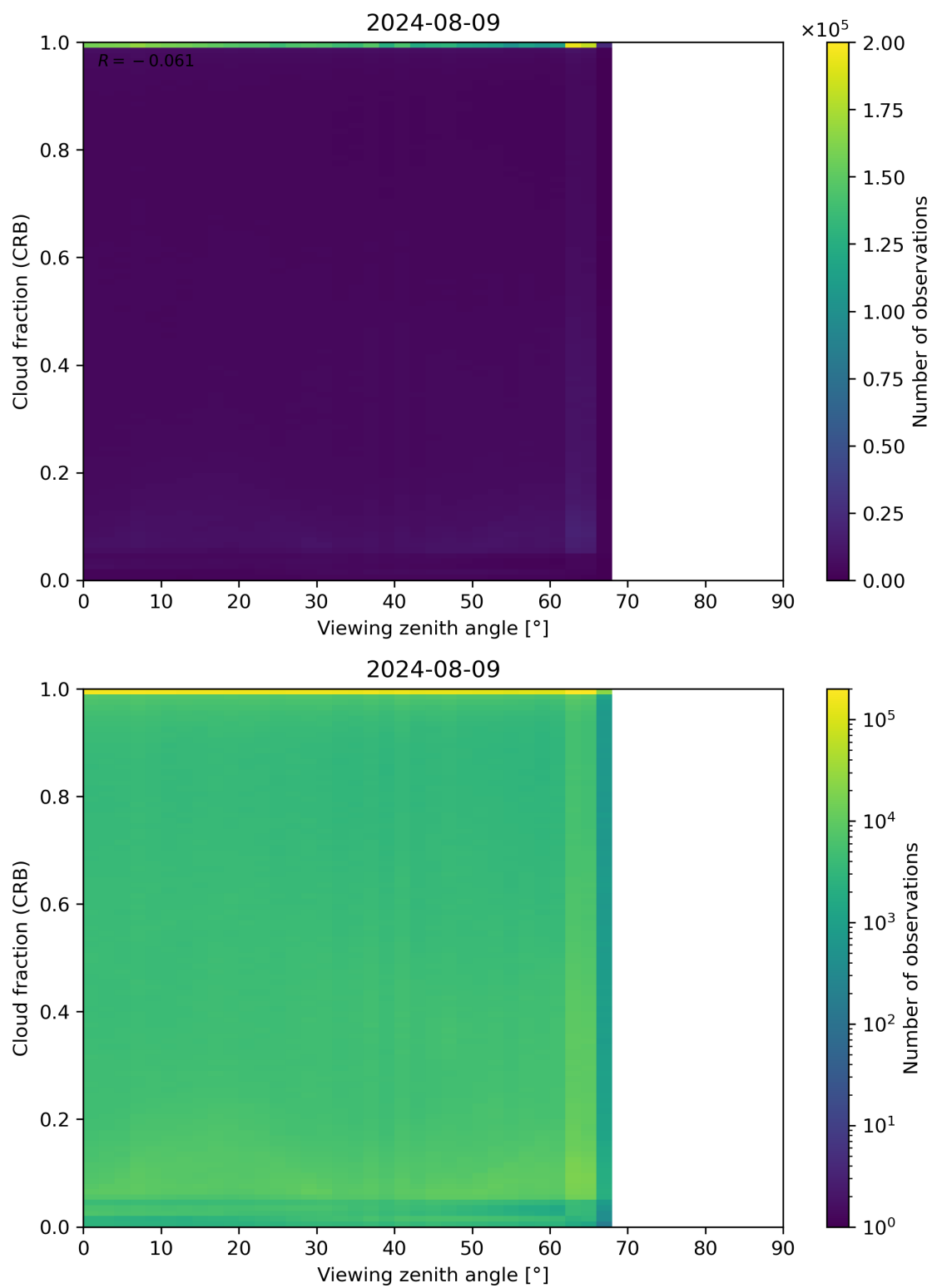
Figure 109: Scatter density plot of “Viewing zenith angle” against “Cloud fraction (CRB)” for 2024-08-08 to 2024-08-10.
