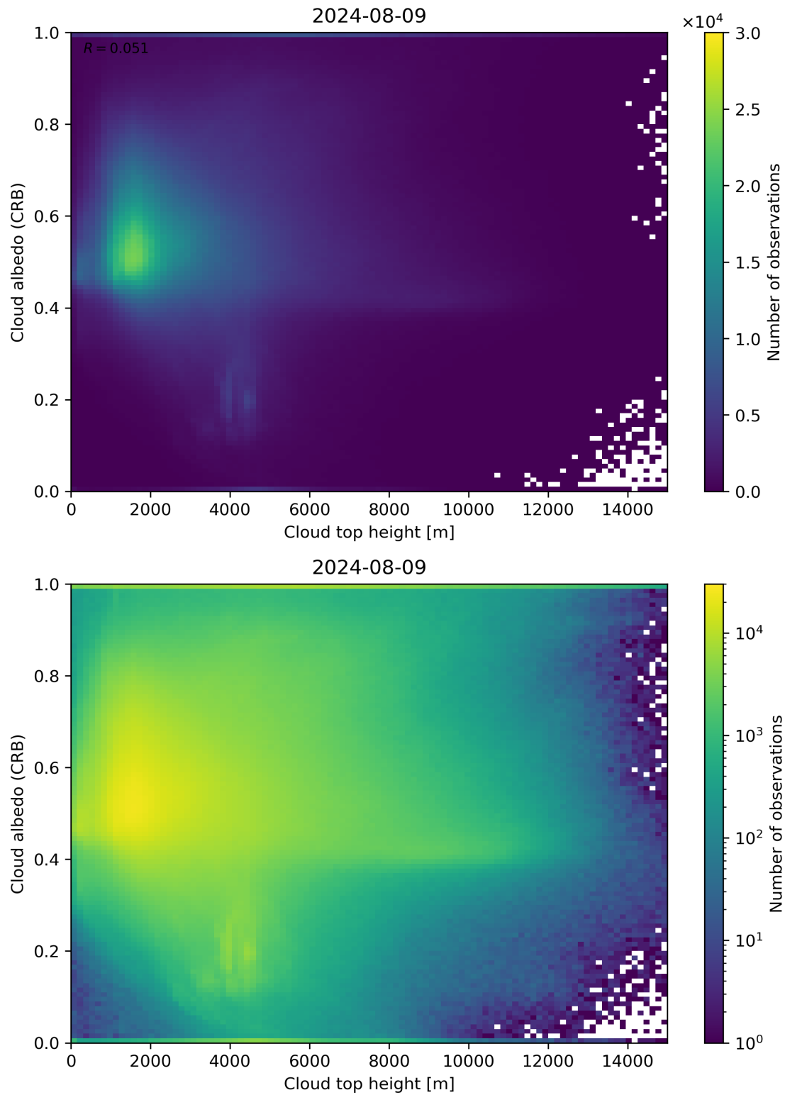
Figure 86: Scatter density plot of “Cloud top height” against “Cloud albedo (CRB)” for 2024-08-08 to 2024-08-10.
