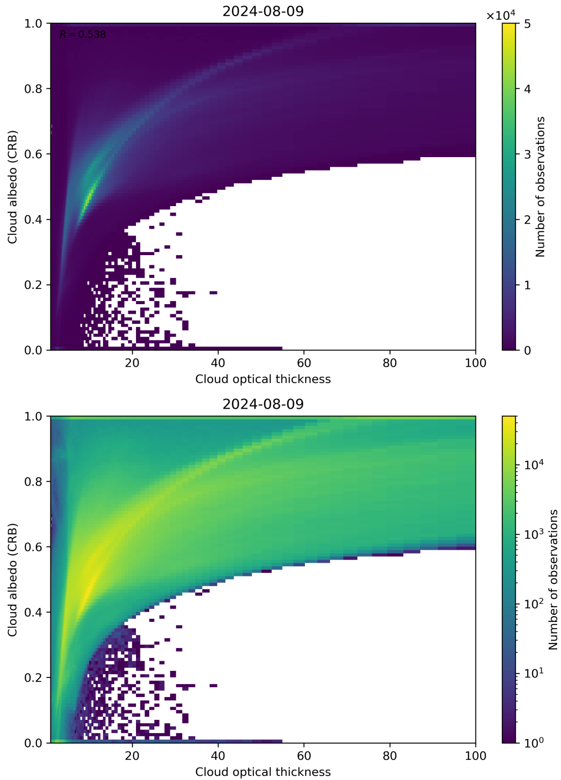
Figure 82: Scatter density plot of “Cloud optical thickness” against “Cloud albedo (CRB)” for 2024-08-08 to 2024-08-10.
