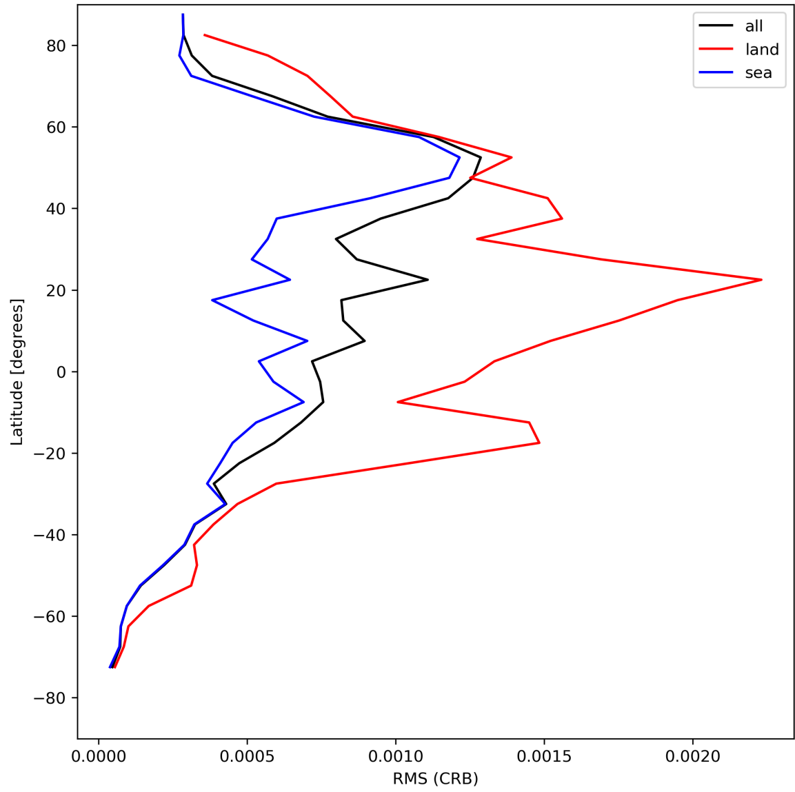
Figure 32: Zonal average of “RMS (CRB)” for 2024-08-08 to 2024-08-10.
