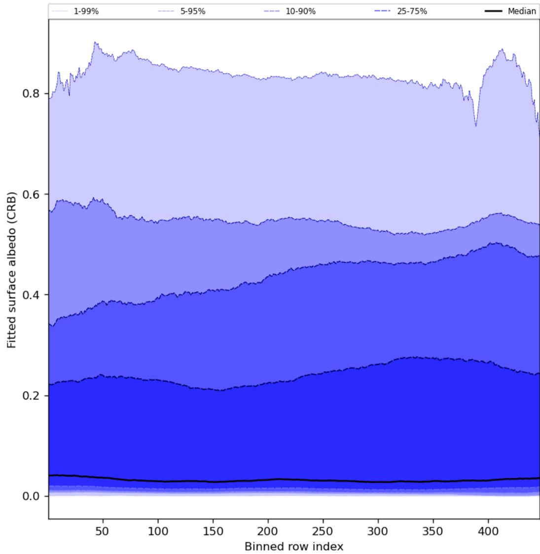
Figure 62: Along track statistics of “Fitted surface albedo (CRB)” for 2024-08-08 to 2024-08-10
