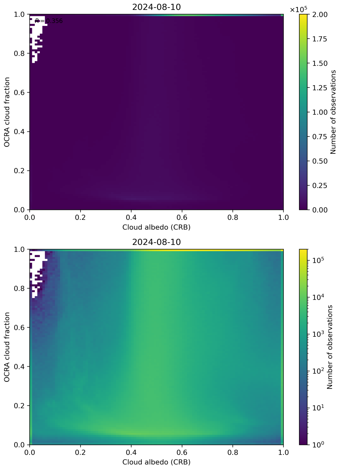
Figure 70: Scatter density plot of “Cloud albedo (CRB)” against “OCRA cloud fraction” for 2024-08-09 to 2024-08-11.
