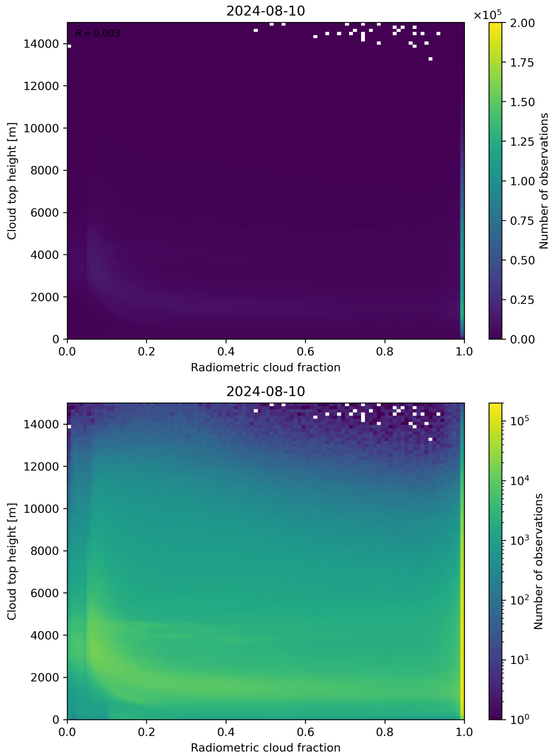
Figure 76: Scatter density plot of “Radiometric cloud fraction” against “Cloud top height” for 2024-08-09 to 2024-08-11.
