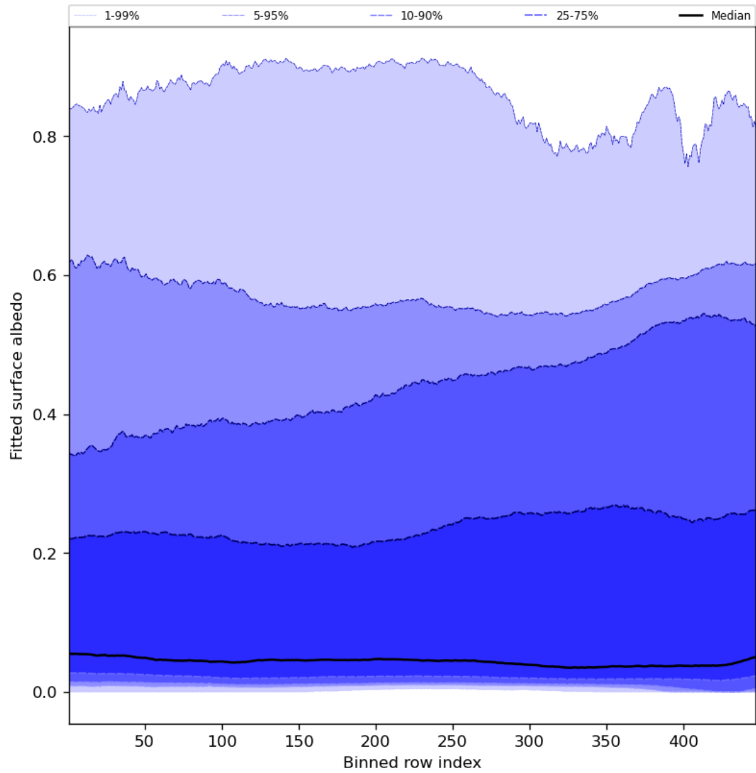
Figure 61: Along track statistics of “Fitted surface albedo” for 2024-08-09 to 2024-08-11
