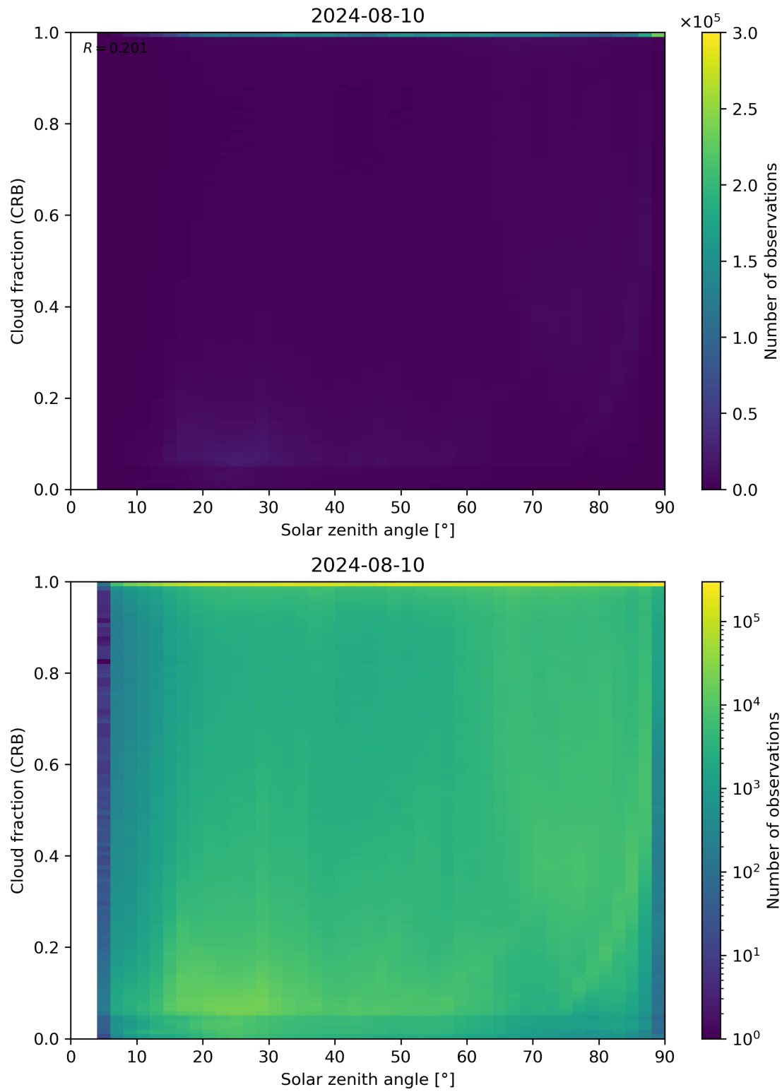
Figure 101: Scatter density plot of “Solar zenith angle” against “Cloud fraction (CRB)” for 2024-08-09 to 2024-08-11.
