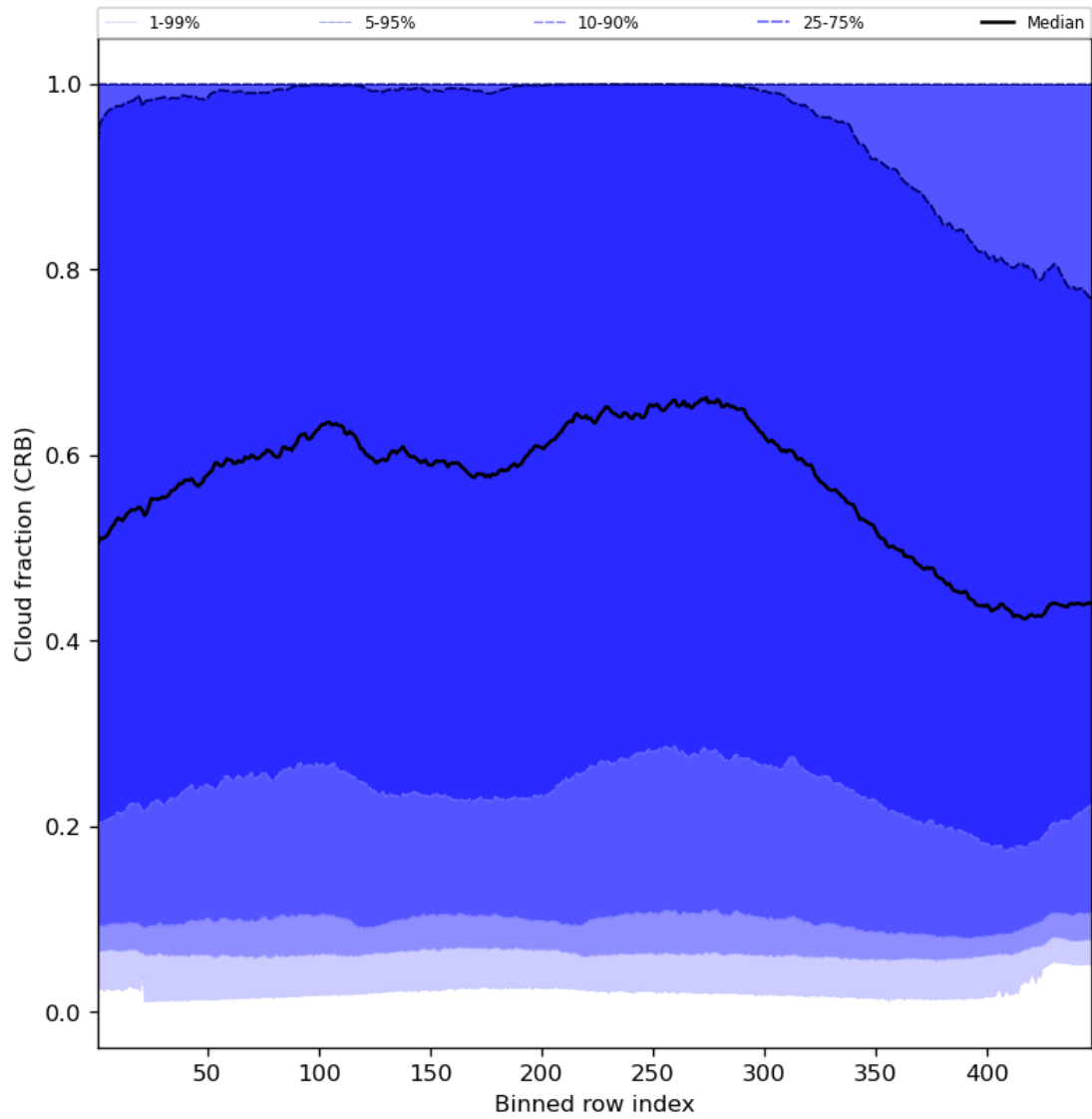
Figure 58: Along track statistics of “Cloud fraction (CRB)” for 2024-08-09 to 2024-08-11
