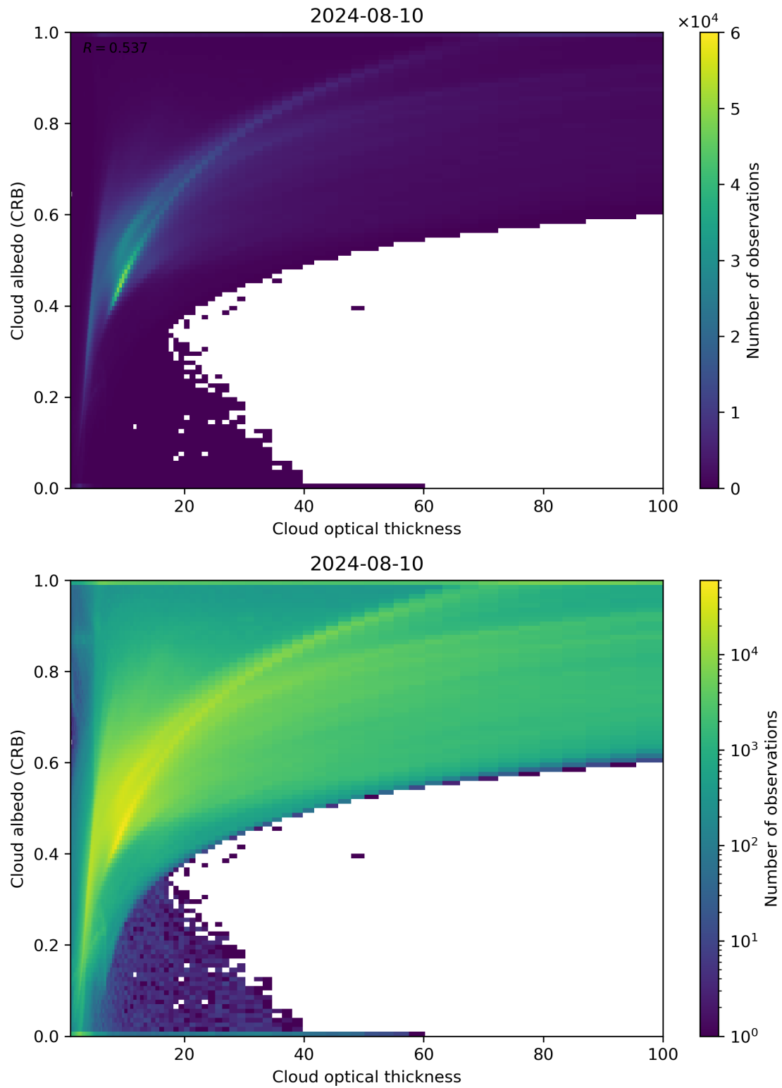
Figure 82: Scatter density plot of “Cloud optical thickness” against “Cloud albedo (CRB)” for 2024-08-09 to 2024-08-11.
