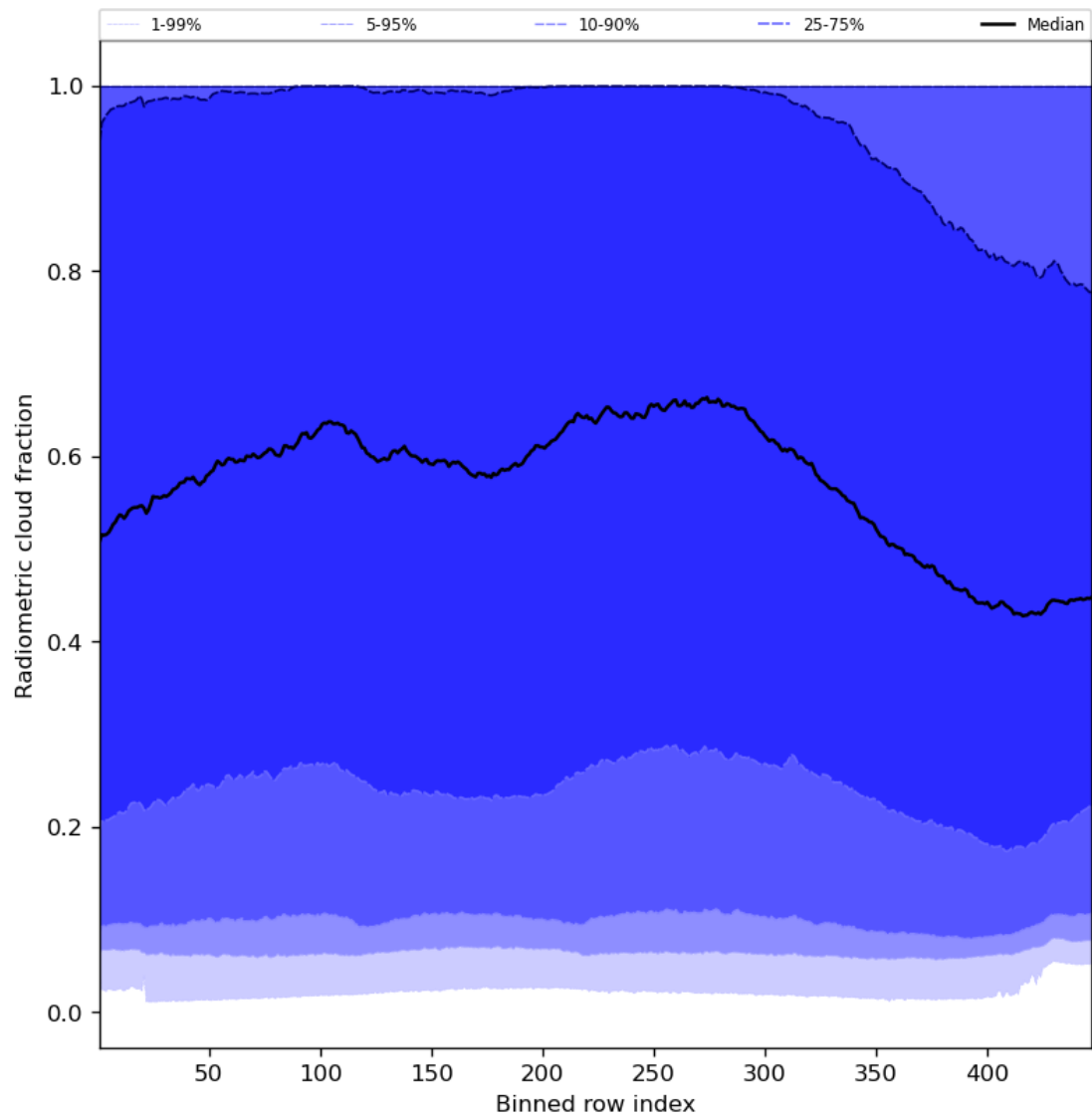
Figure 55: Along track statistics of “Radiometric cloud fraction” for 2024-08-09 to 2024-08-11
