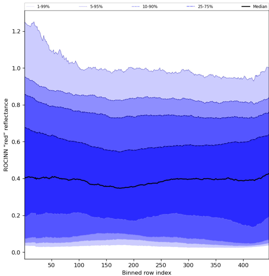
Figure 69: Along track statistics of “ROCINN “red” reflectance” for 2024-08-09 to 2024-08-11
