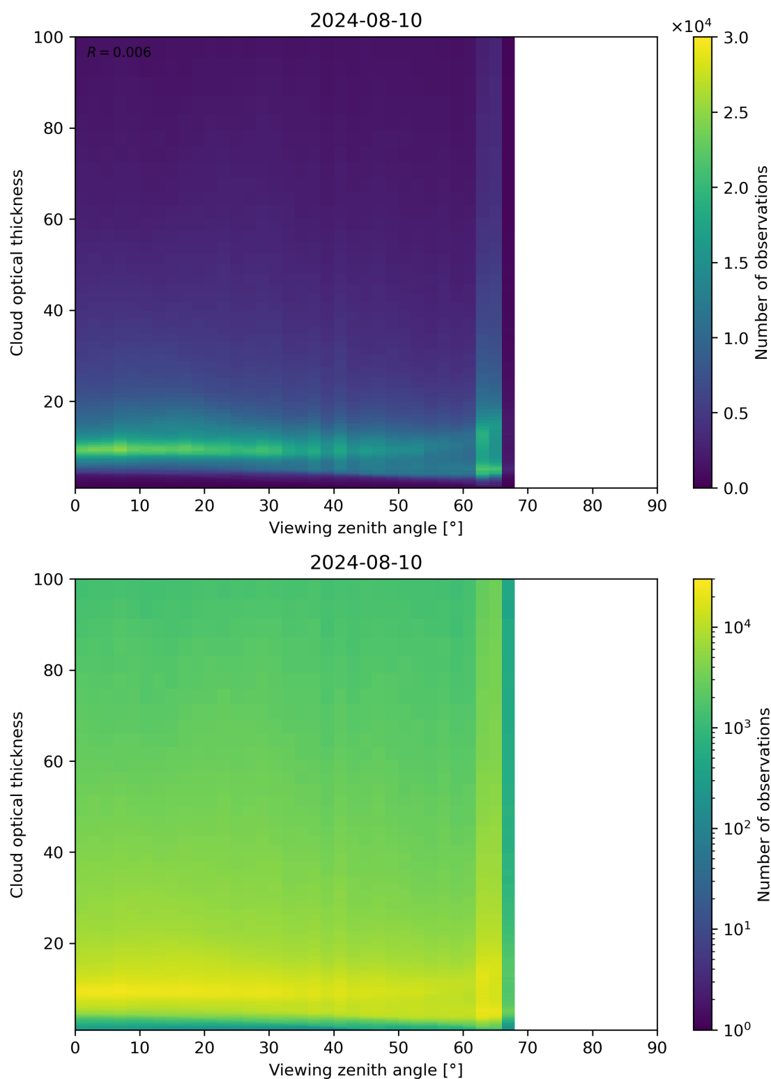
Figure 111: Scatter density plot of “Viewing zenith angle” against “Cloud optical thickness” for 2024-08-09 to 2024-08-11.
