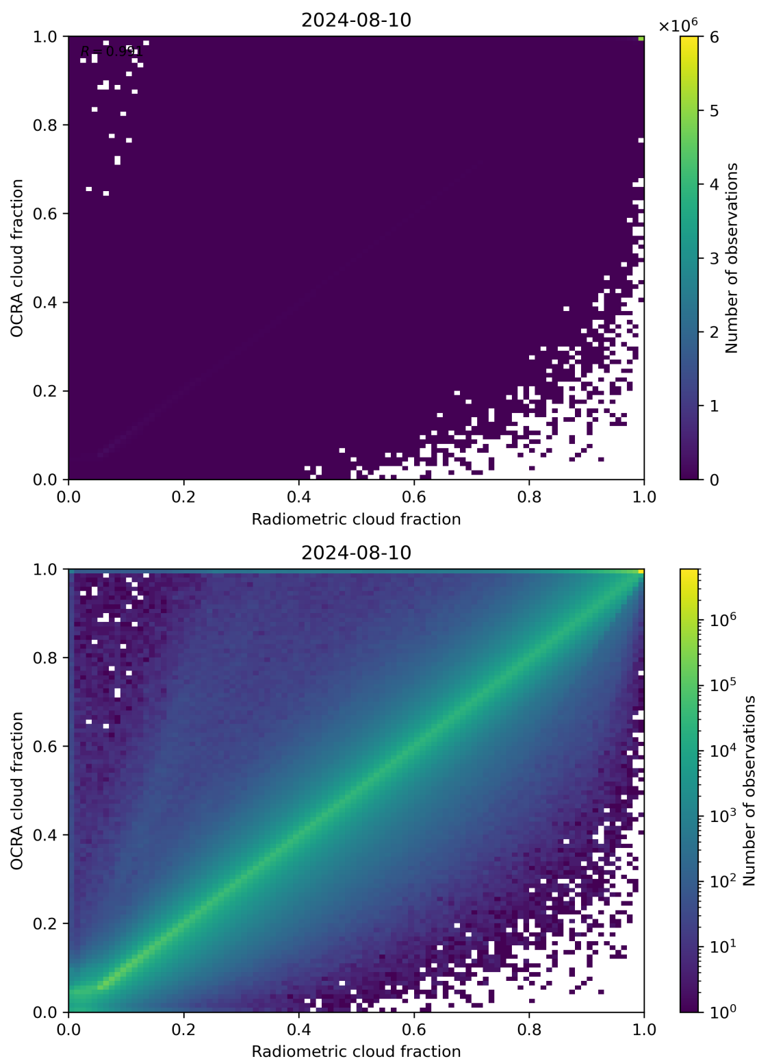
Figure 72: Scatter density plot of “Radiometric cloud fraction” against “OCRA cloud fraction” for 2024-08-09 to 2024-08-11.
