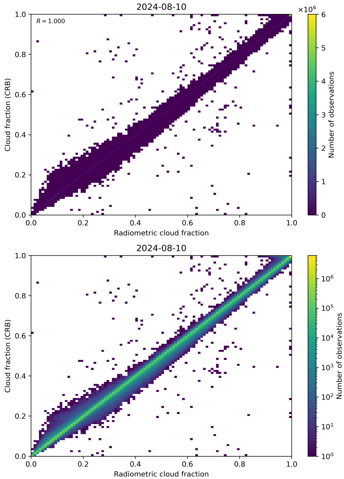
Figure 73: Scatter density plot of “Radiometric cloud fraction” against “Cloud fraction (CRB)” for 2024-08-09 to 2024-08-11.
