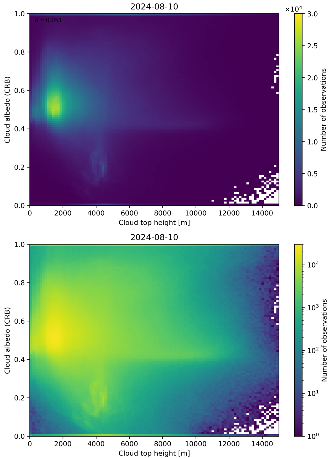
Figure 86: Scatter density plot of “Cloud top height” against “Cloud albedo (CRB)” for 2024-08-09 to 2024-08-11.
