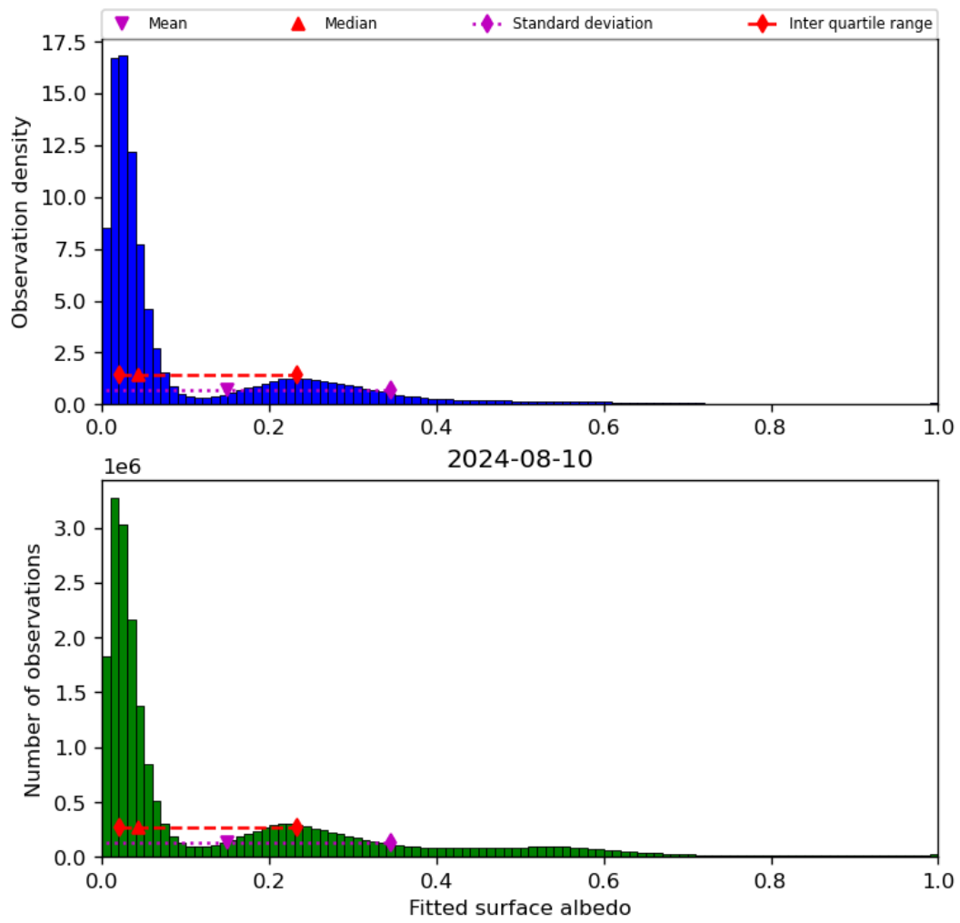
Figure 45: Histogram of “Fitted surface albedo” for 2024-08-09 to 2024-08-11
