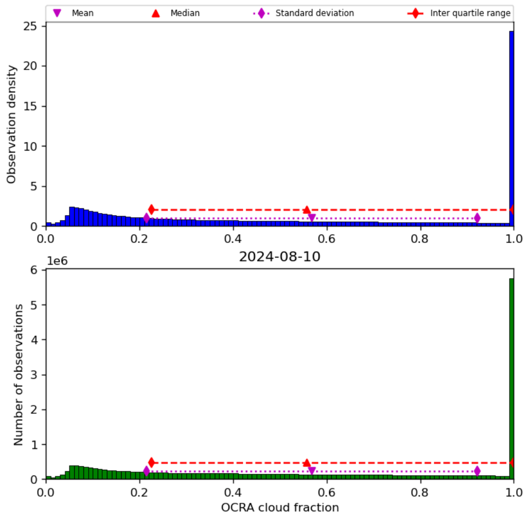
Figure 50: Histogram of “OCRA cloud fraction” for 2024-08-09 to 2024-08-11
