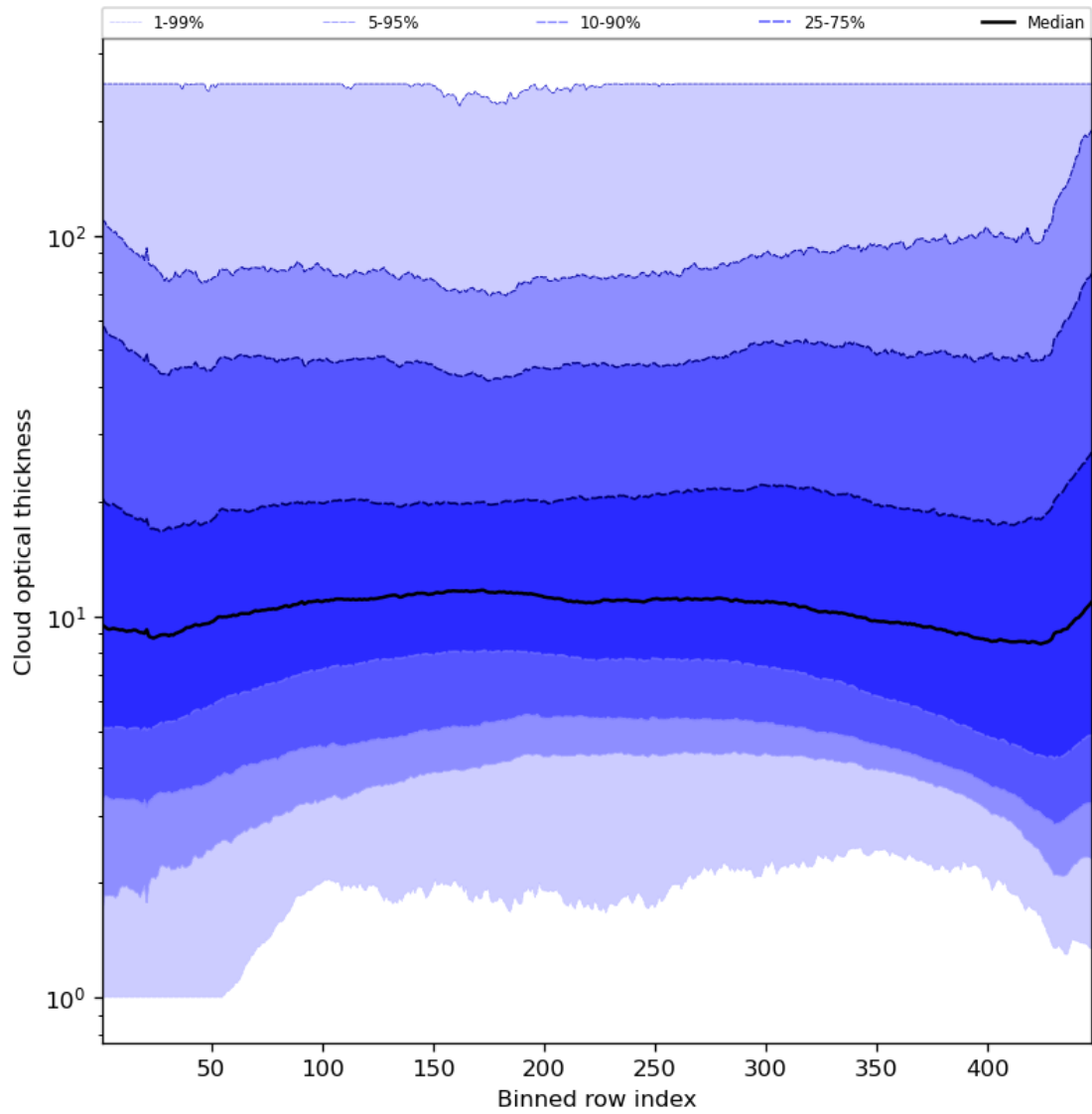
Figure 57: Along track statistics of “Cloud optical thickness” for 2024-08-09 to 2024-08-11
