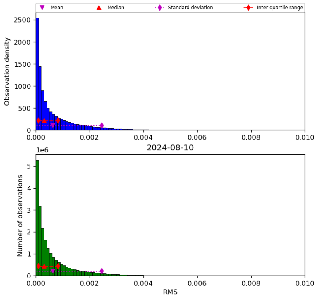
Figure 47: Histogram of “RMS” for 2024-08-09 to 2024-08-11
