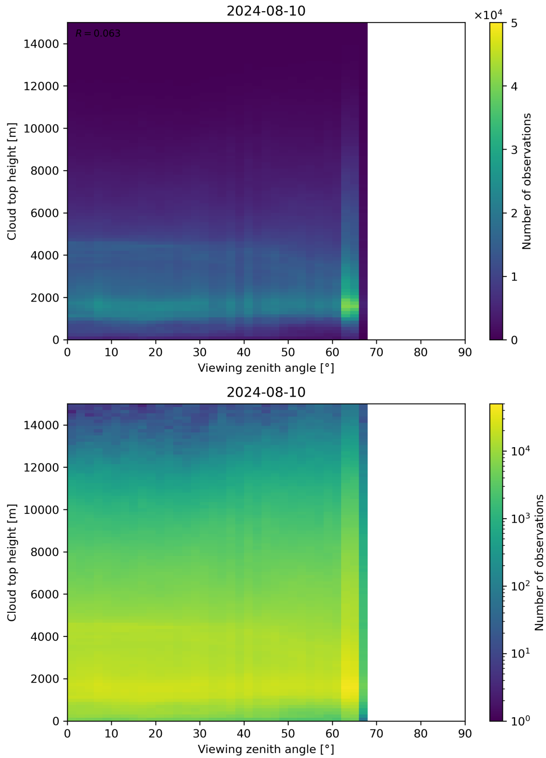
Figure 112: Scatter density plot of “Viewing zenith angle” against “Cloud top height” for 2024-08-09 to 2024-08-11.
