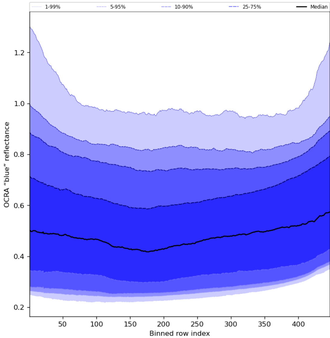
Figure 67: Along track statistics of “OCRA “blue” reflectance” for 2024-08-09 to 2024-08-11
