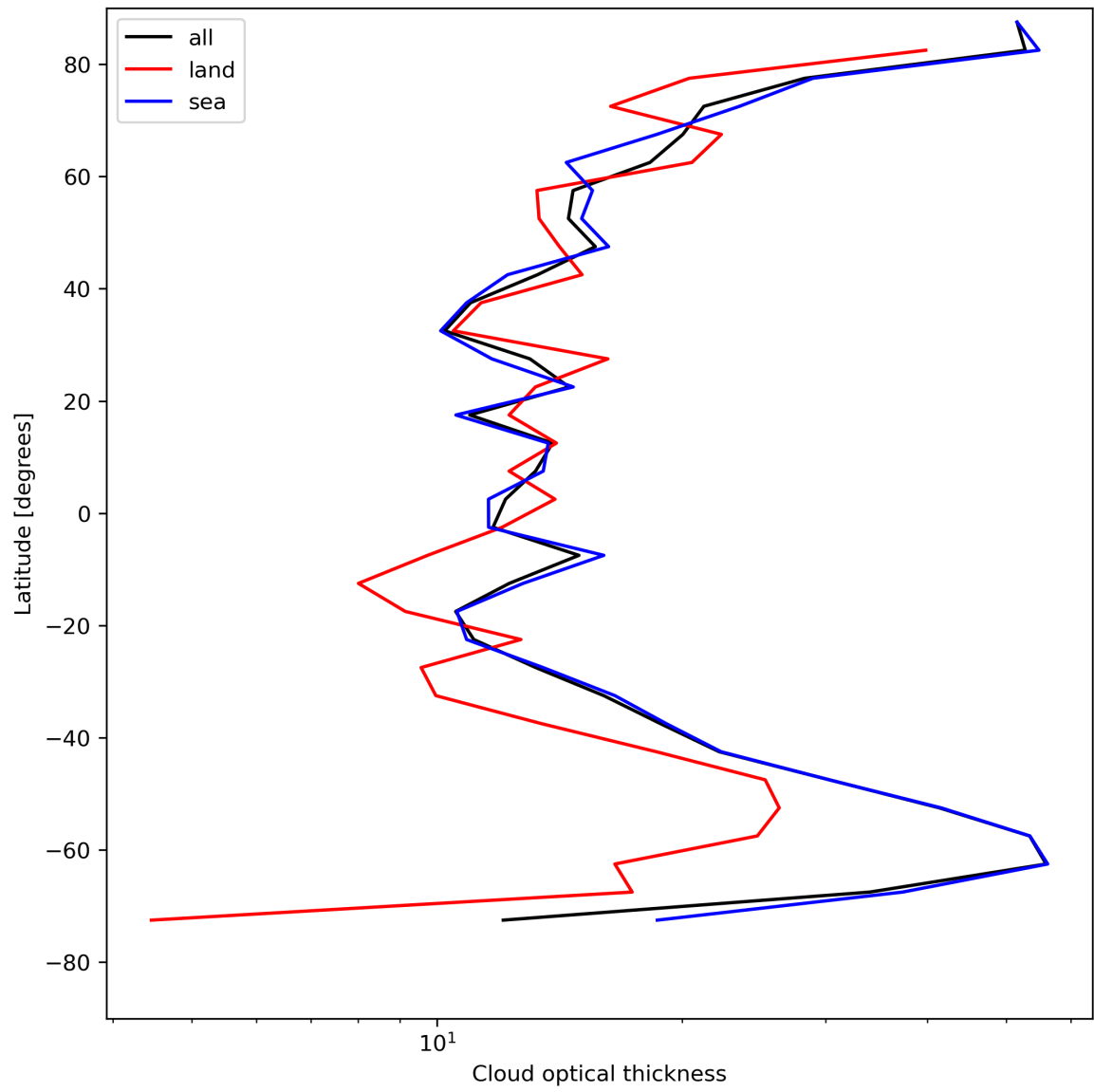
Figure 25: Zonal average of “Cloud optical thickness” for 2024-08-09 to 2024-08-11.
