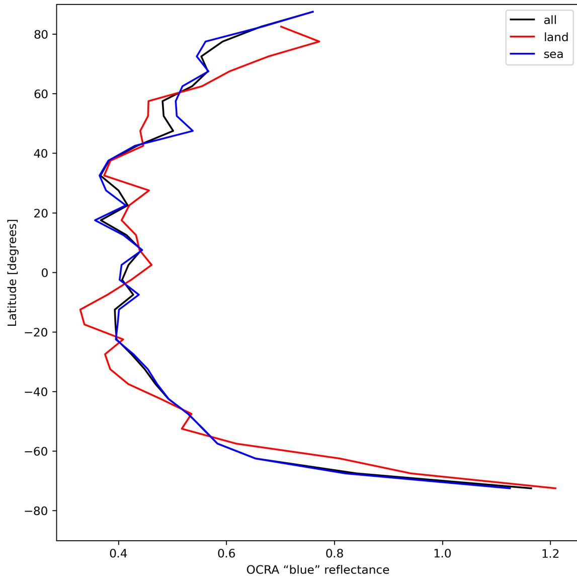
Figure 35: Zonal average of “OCRA “blue” reflectance” for 2024-08-09 to 2024-08-11.
