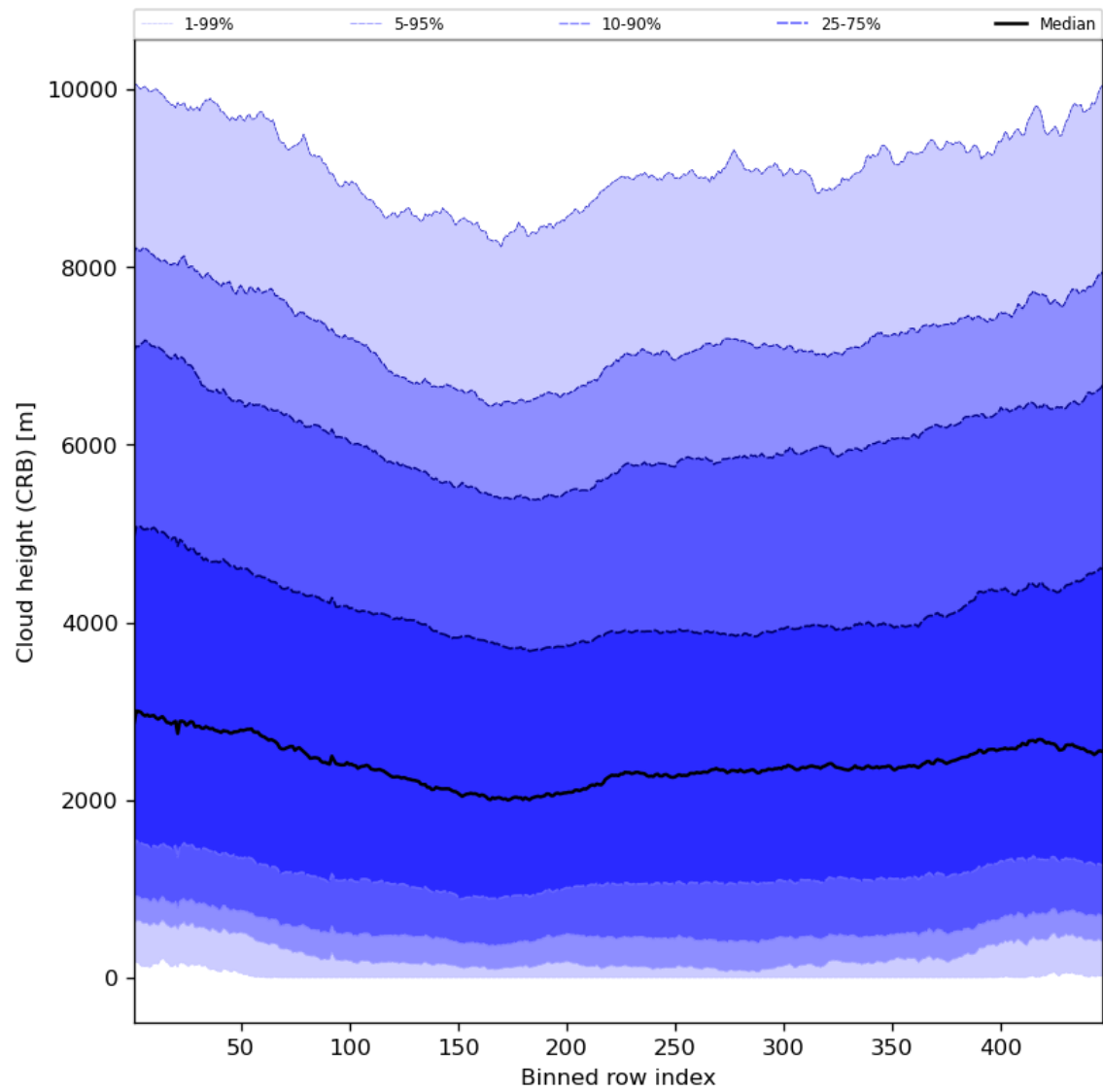
Figure 59: Along track statistics of “Cloud height (CRB)” for 2024-08-09 to 2024-08-11
