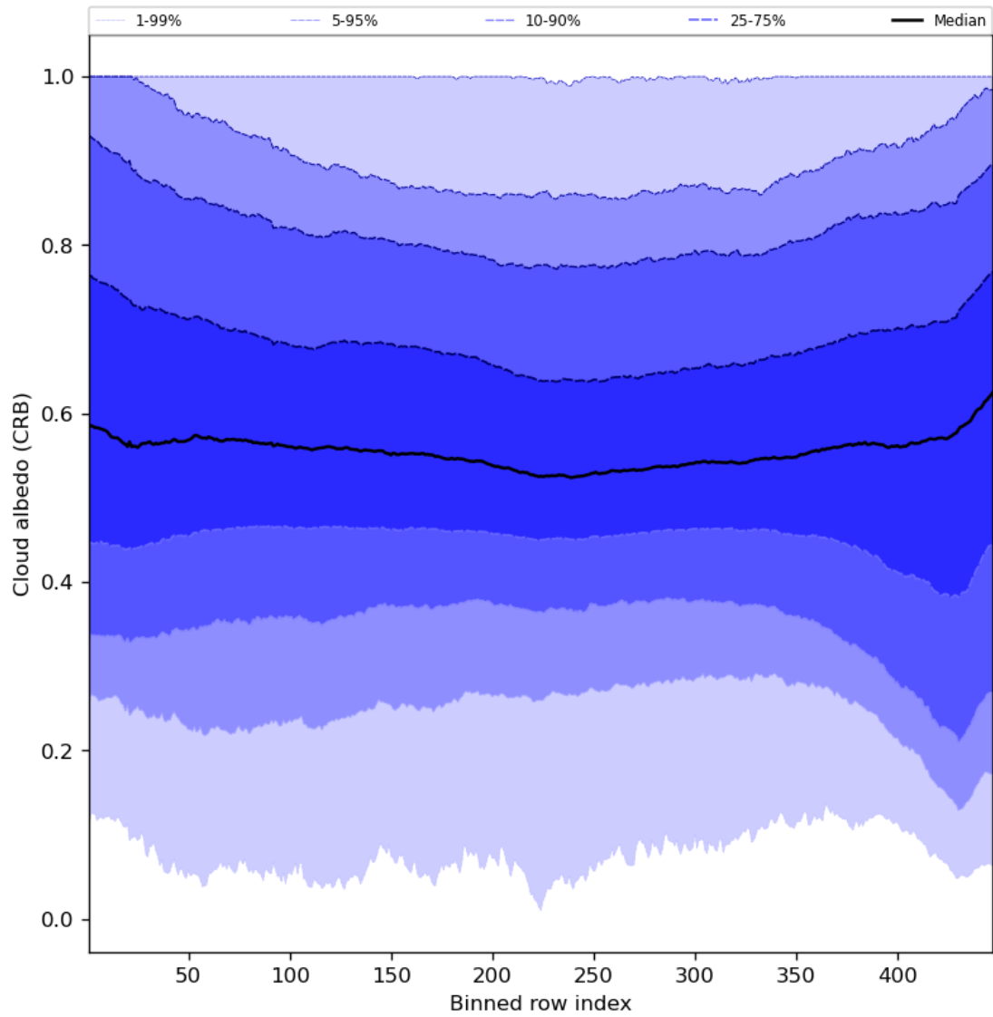
Figure 60: Along track statistics of “Cloud albedo (CRB)” for 2024-08-09 to 2024-08-11
