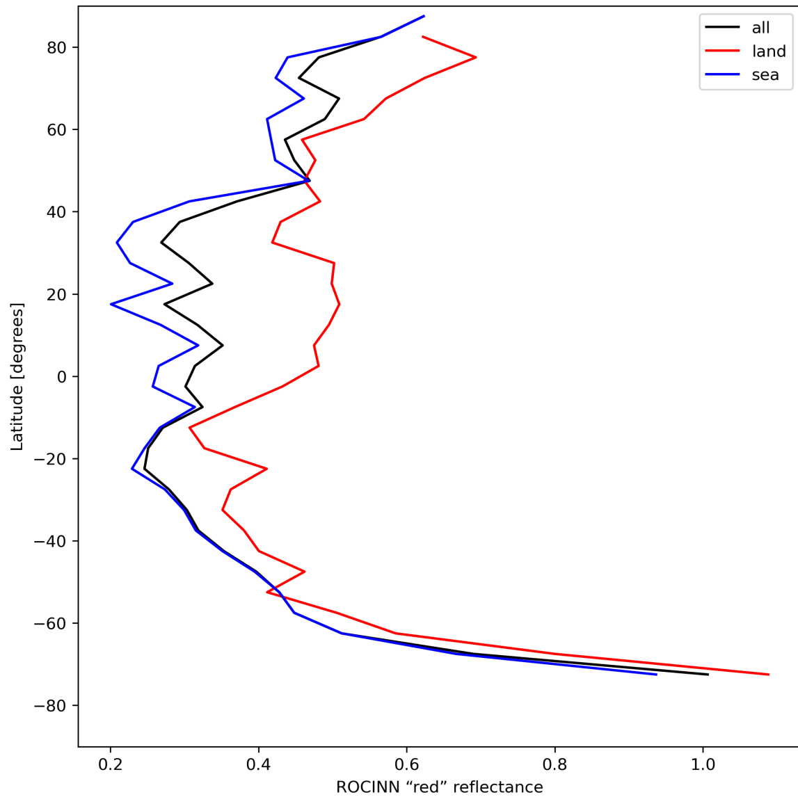
Figure 37: Zonal average of “ROCINN “red” reflectance” for 2024-08-09 to 2024-08-11.
