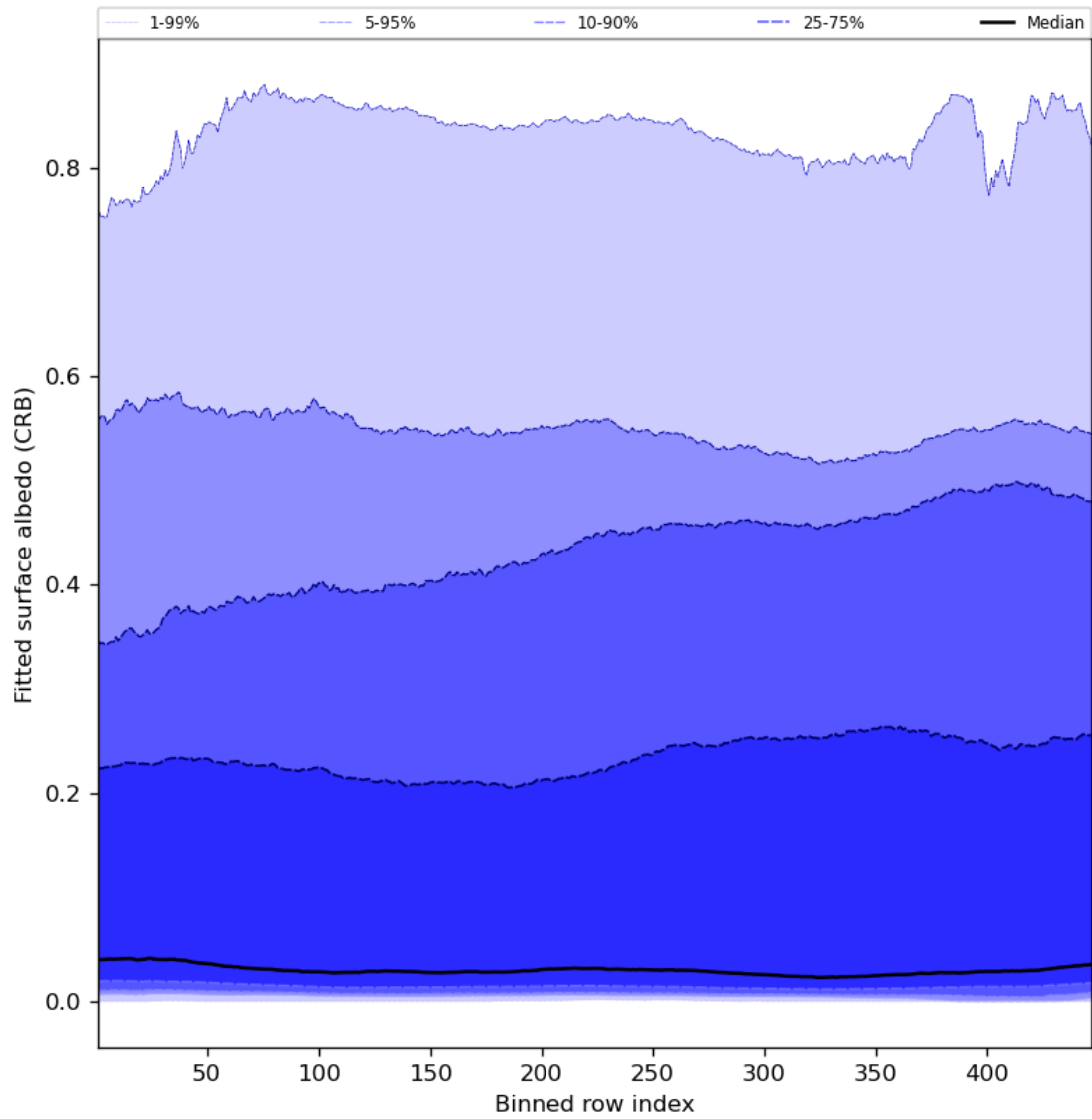
Figure 62: Along track statistics of “Fitted surface albedo (CRB)” for 2024-08-09 to 2024-08-11
