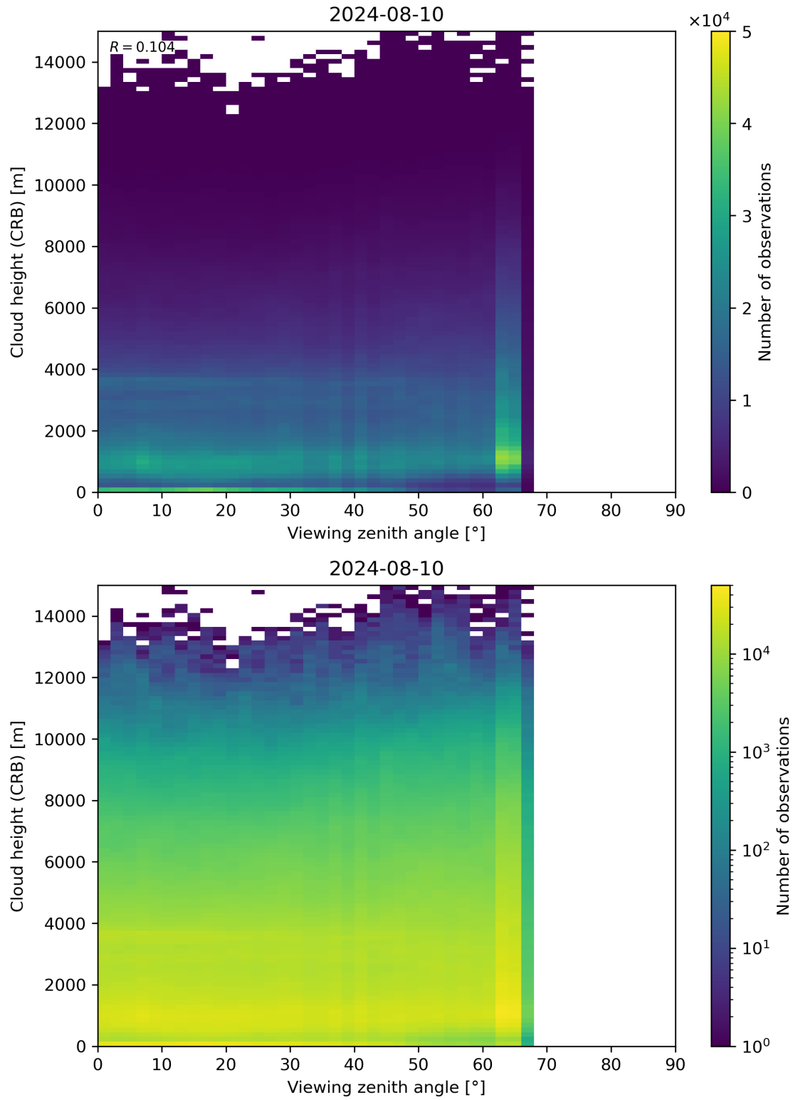
Figure 110: Scatter density plot of “Viewing zenith angle” against “Cloud height (CRB)” for 2024-08-09 to 2024-08-11.
