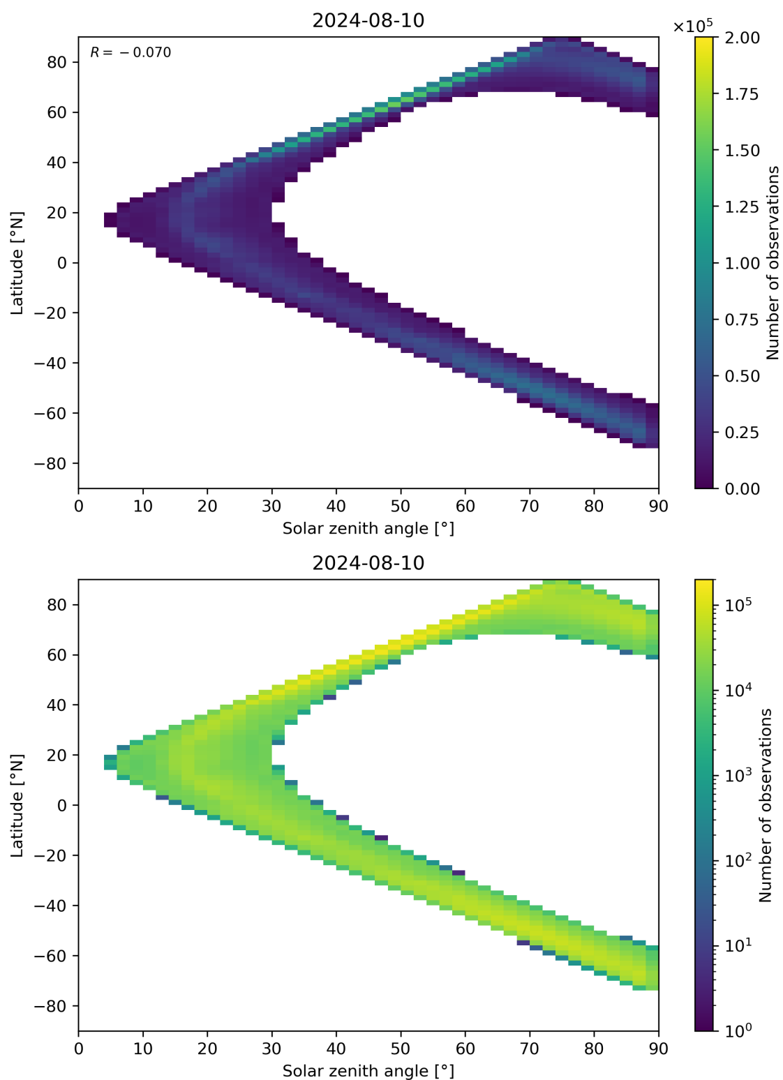
Figure 105: Scatter density plot of “Solar zenith angle” against “Latitude” for 2024-08-09 to 2024-08-11.
