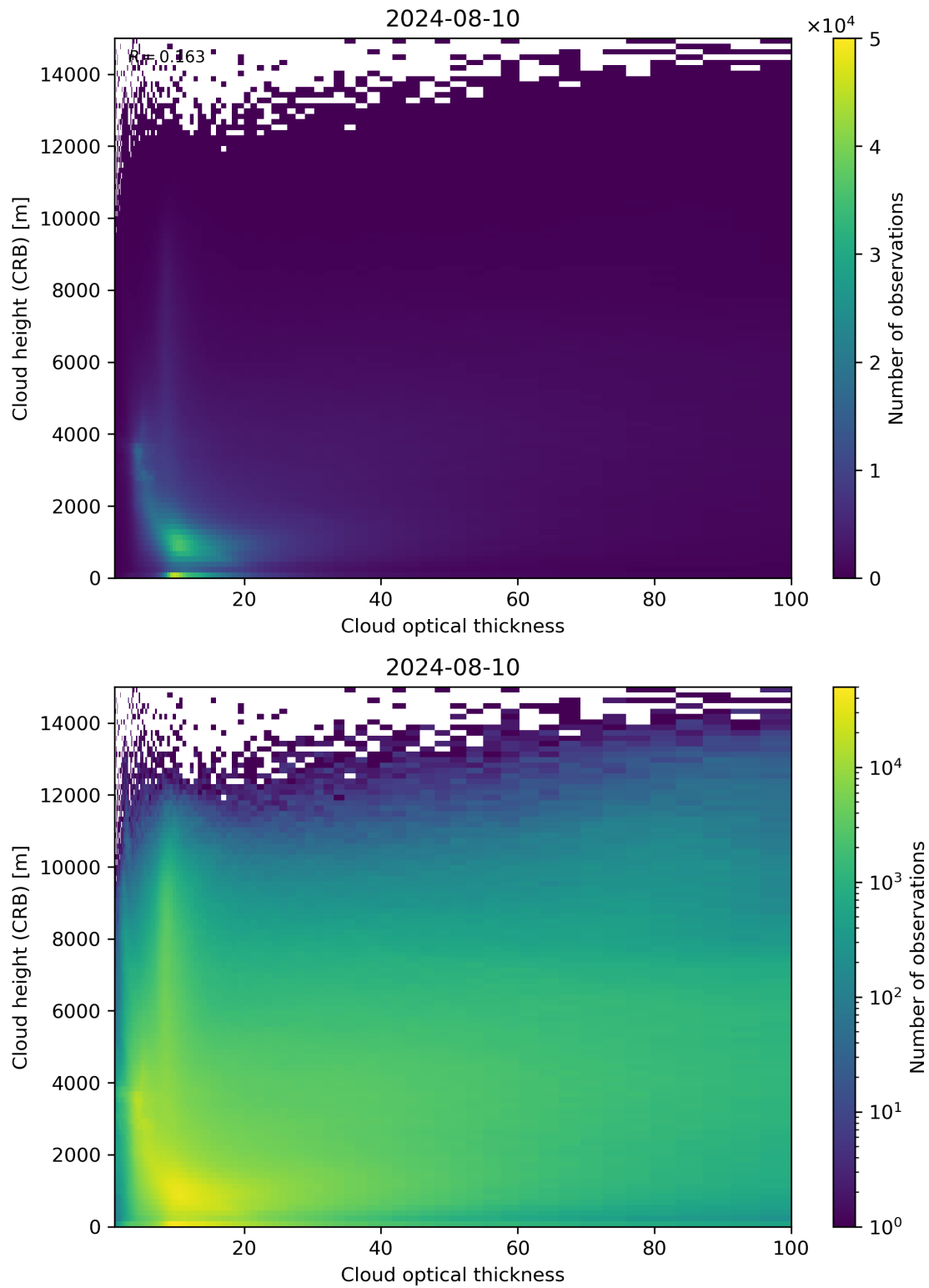
Figure 85: Scatter density plot of “Cloud optical thickness” against “Cloud height (CRB)” for 2024-08-09 to 2024-08-11.
