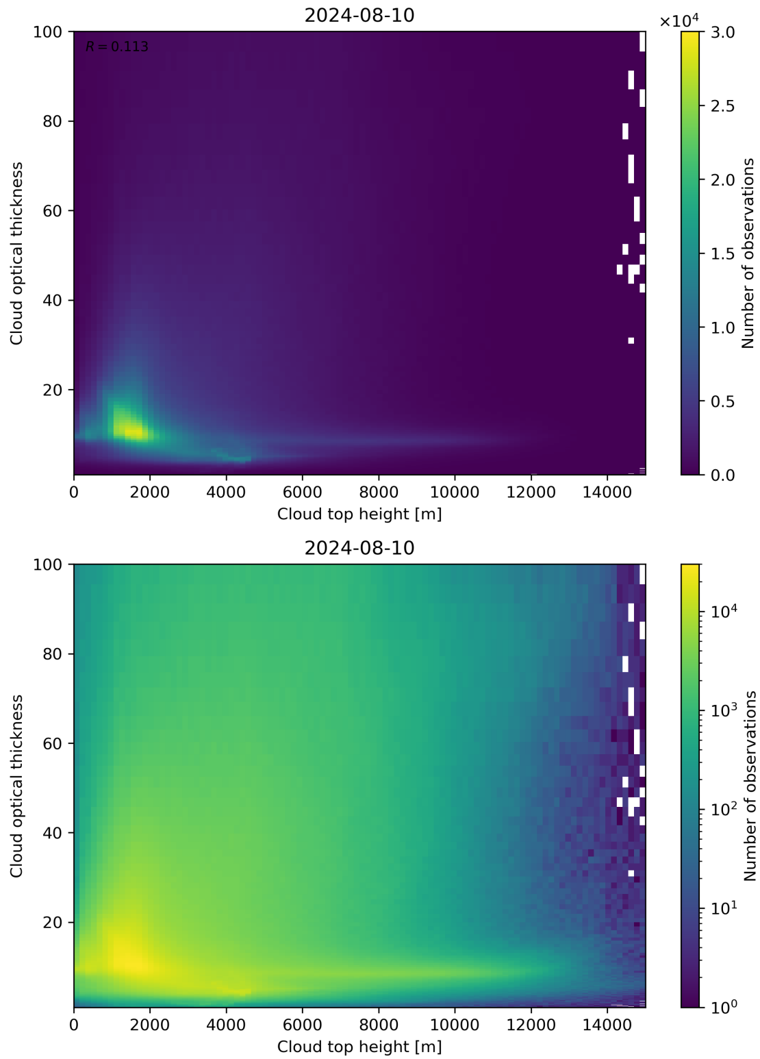
Figure 90: Scatter density plot of “Cloud top height” against “Cloud optical thickness” for 2024-08-09 to 2024-08-11.
