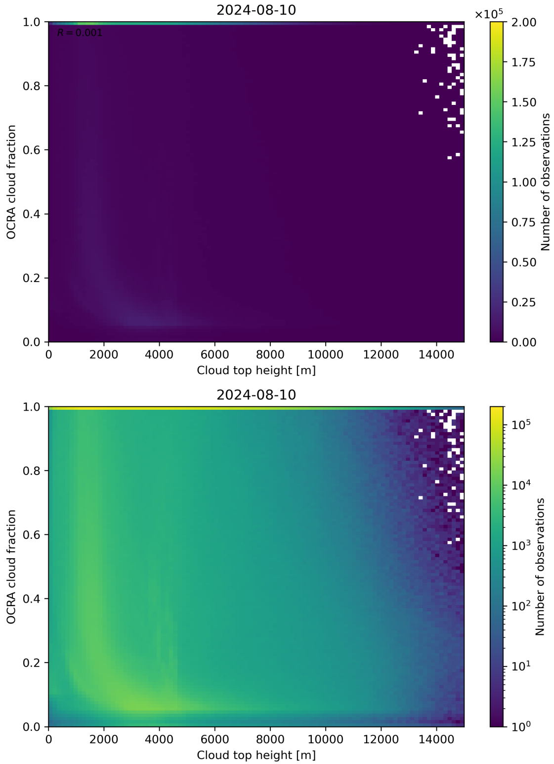
Figure 87: Scatter density plot of “Cloud top height” against “OCRA cloud fraction” for 2024-08-09 to 2024-08-11.
