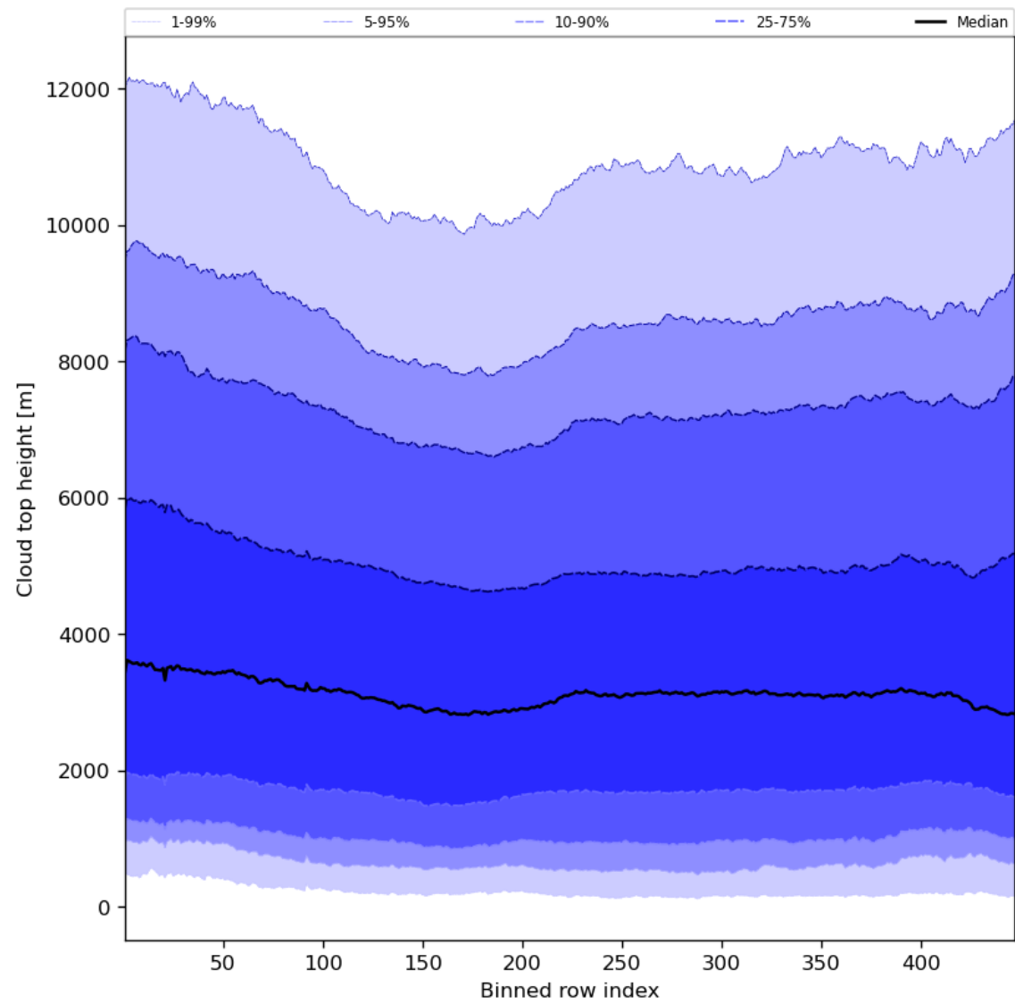
Figure 56: Along track statistics of “Cloud top height” for 2024-08-09 to 2024-08-11
