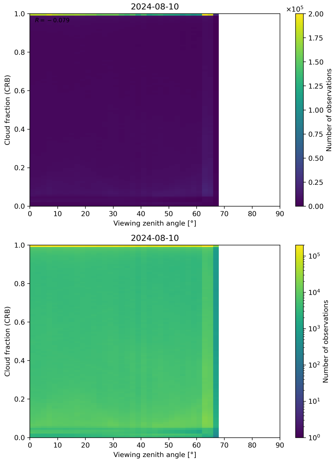
Figure 109: Scatter density plot of “Viewing zenith angle” against “Cloud fraction (CRB)” for 2024-08-09 to 2024-08-11.
