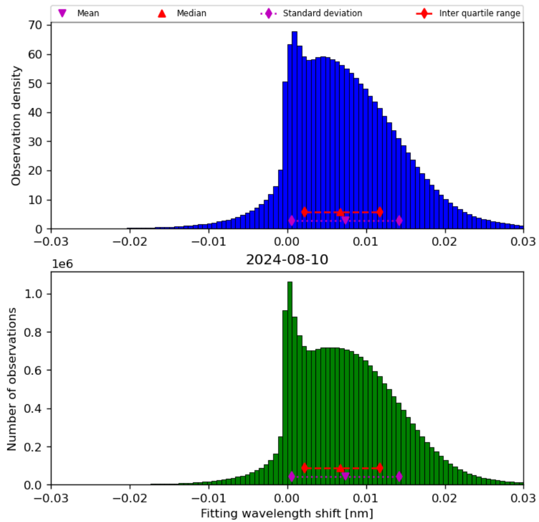
Figure 49: Histogram of “Fitting wavelength shift” for 2024-08-09 to 2024-08-11
