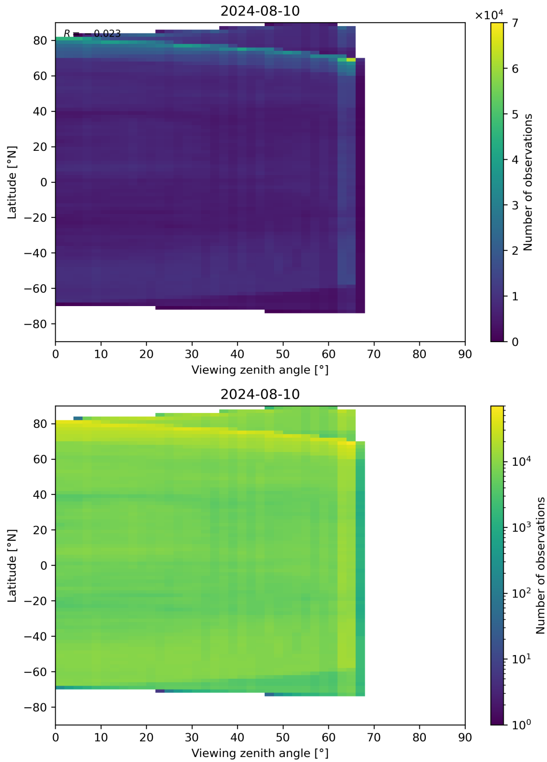
Figure 113: Scatter density plot of “Viewing zenith angle” against “Latitude” for 2024-08-09 to 2024-08-11.
