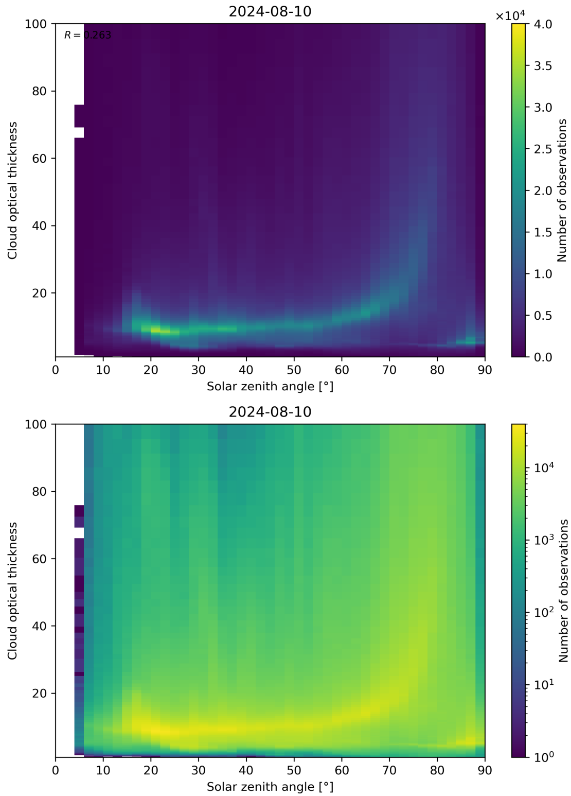
Figure 103: Scatter density plot of “Solar zenith angle” against “Cloud optical thickness” for 2024-08-09 to 2024-08-11.
