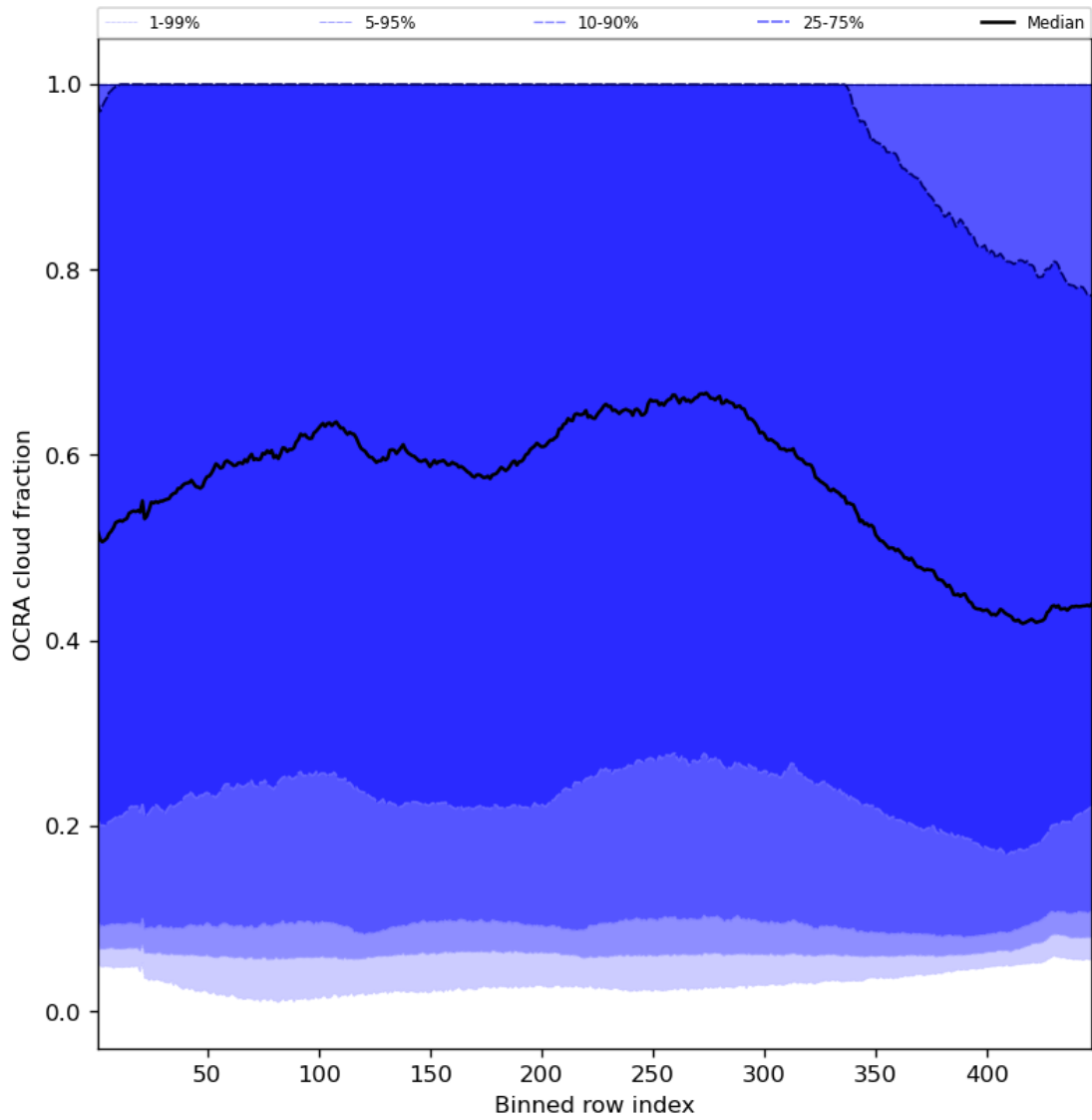
Figure 66: Along track statistics of “OCRA cloud fraction” for 2024-08-09 to 2024-08-11
