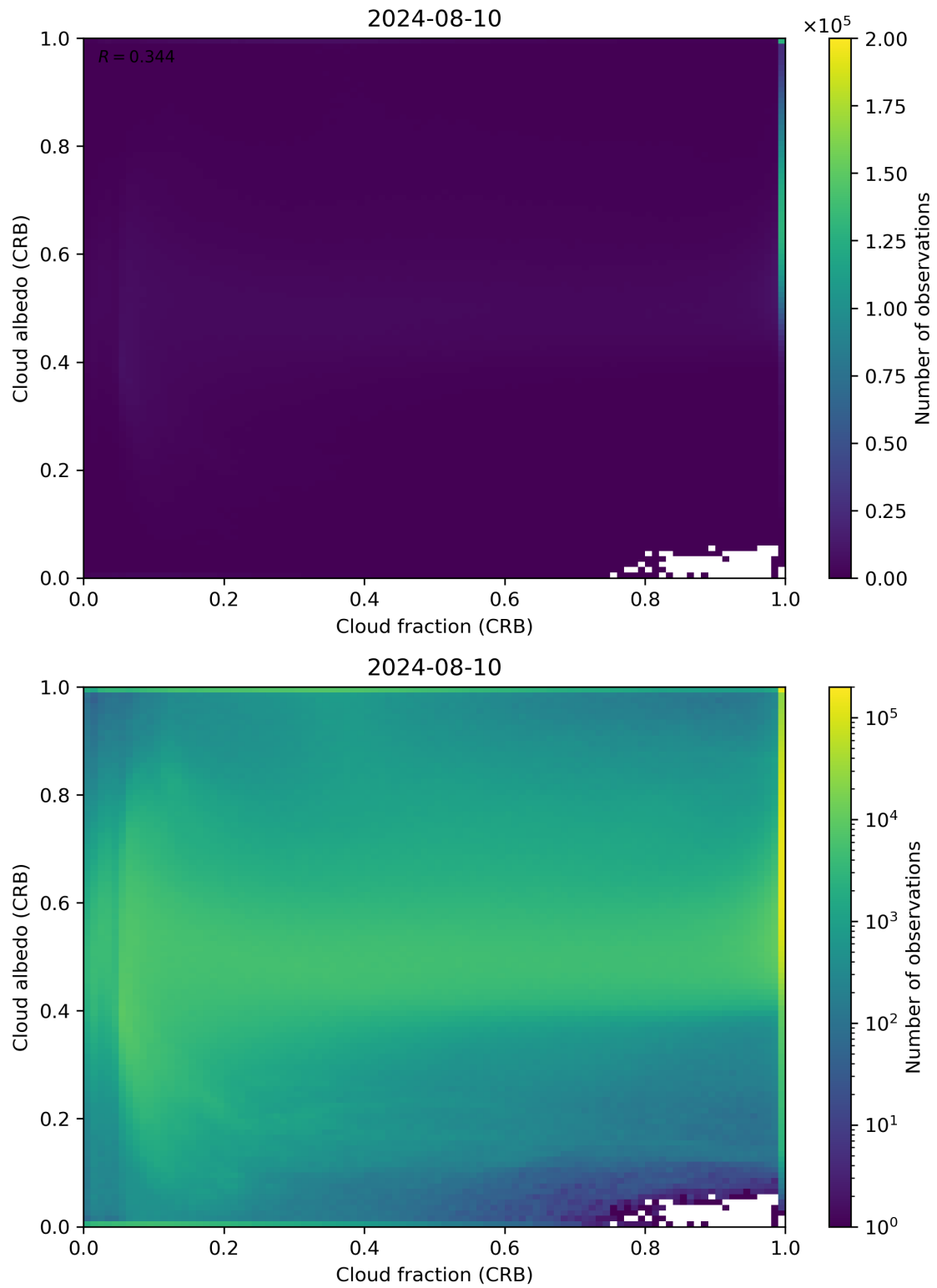
Figure 77: Scatter density plot of “Cloud fraction (CRB)” against “Cloud albedo (CRB)” for 2024-08-09 to 2024-08-11.
