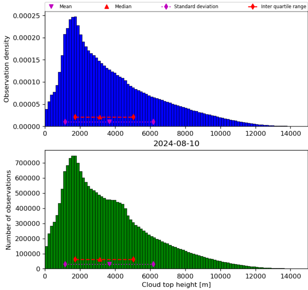
Figure 40: Histogram of “Cloud top height” for 2024-08-09 to 2024-08-11
