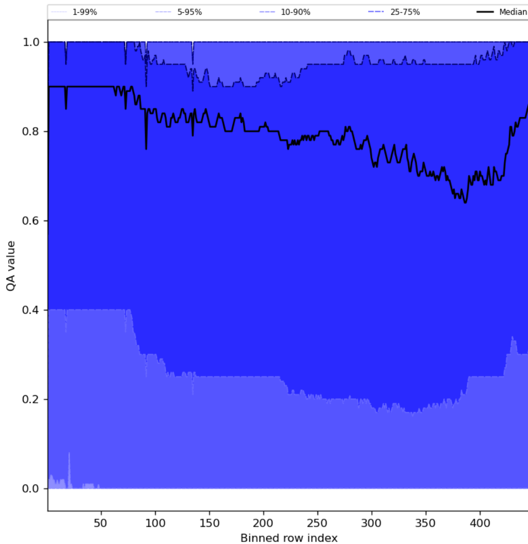
Figure 54: Along track statistics of “QA value” for 2024-08-09 to 2024-08-11
