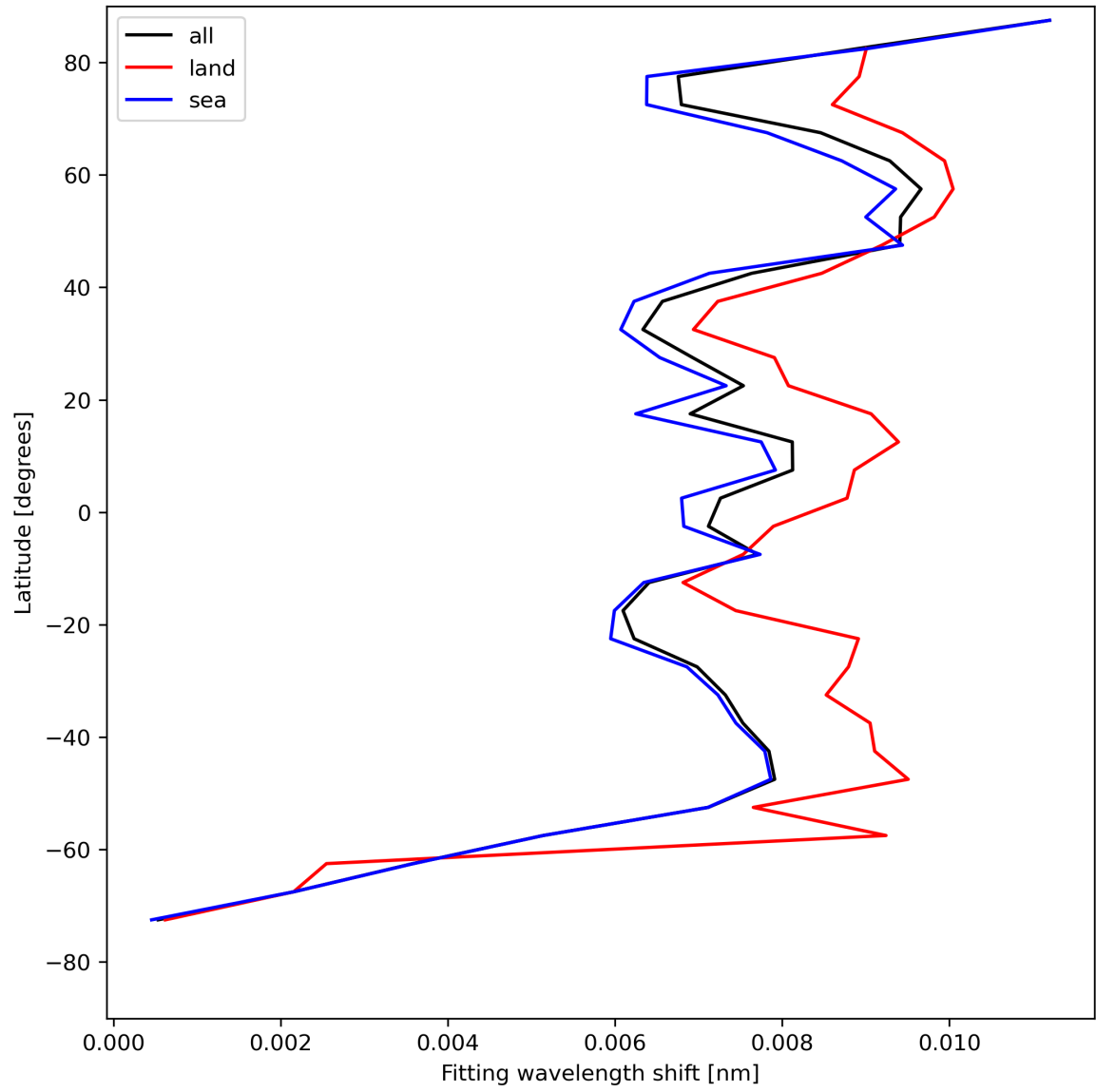
Figure 33: Zonal average of “Fitting wavelength shift” for 2024-08-09 to 2024-08-11.
