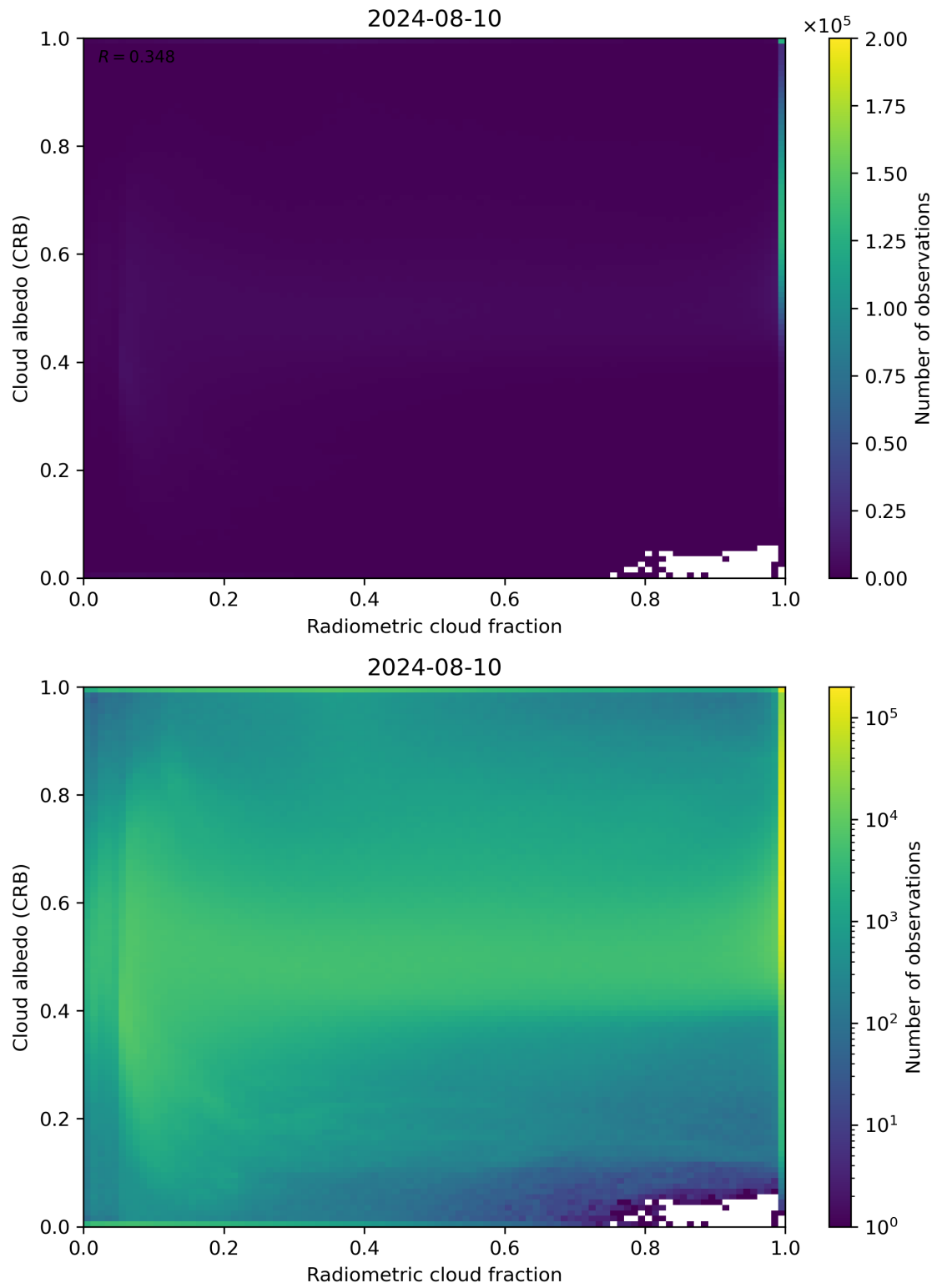
Figure 71: Scatter density plot of “Radiometric cloud fraction” against “Cloud albedo (CRB)” for 2024-08-09 to 2024-08-11.
