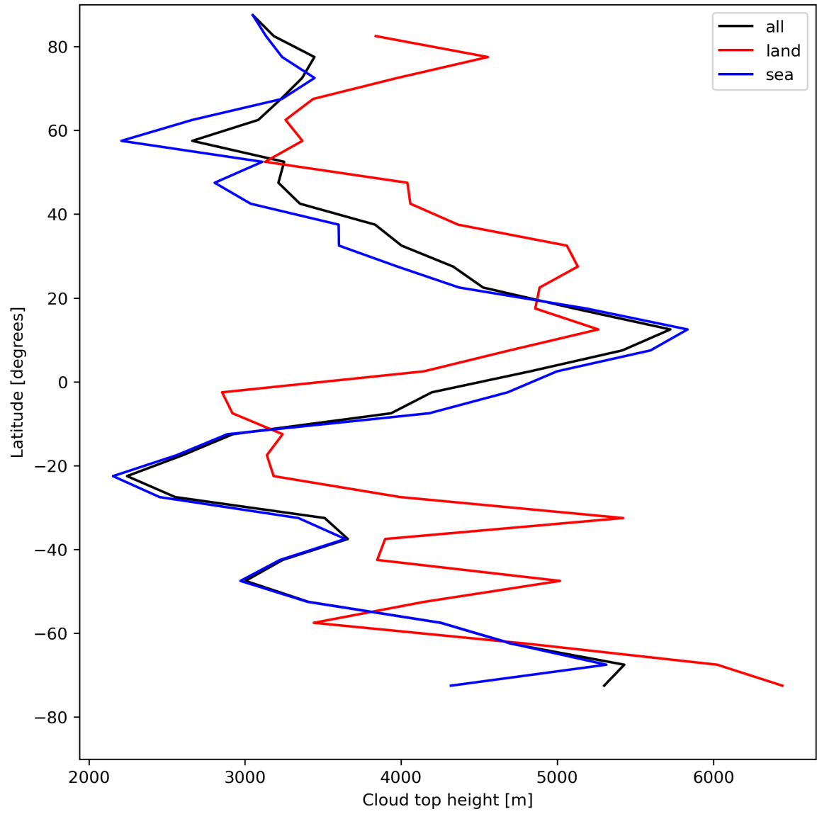
Figure 24: Zonal average of “Cloud top height” for 2024-08-09 to 2024-08-11.
