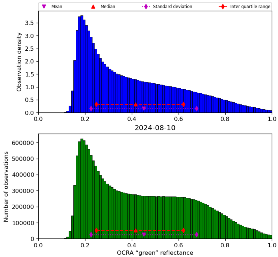
Figure 52: Histogram of “OCRA “green” reflectance” for 2024-08-09 to 2024-08-11
