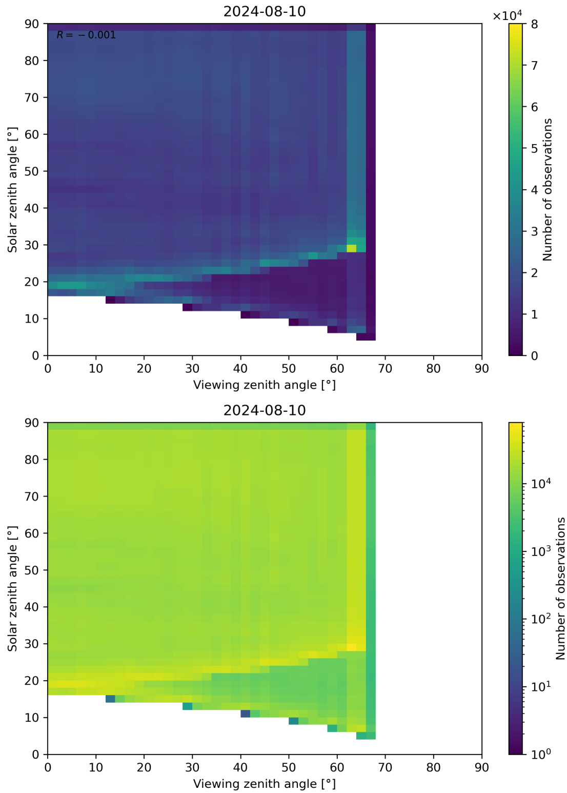
Figure 114: Scatter density plot of “Viewing zenith angle” against “Solar zenith angle” for 2024-08-09 to 2024-08-11.
