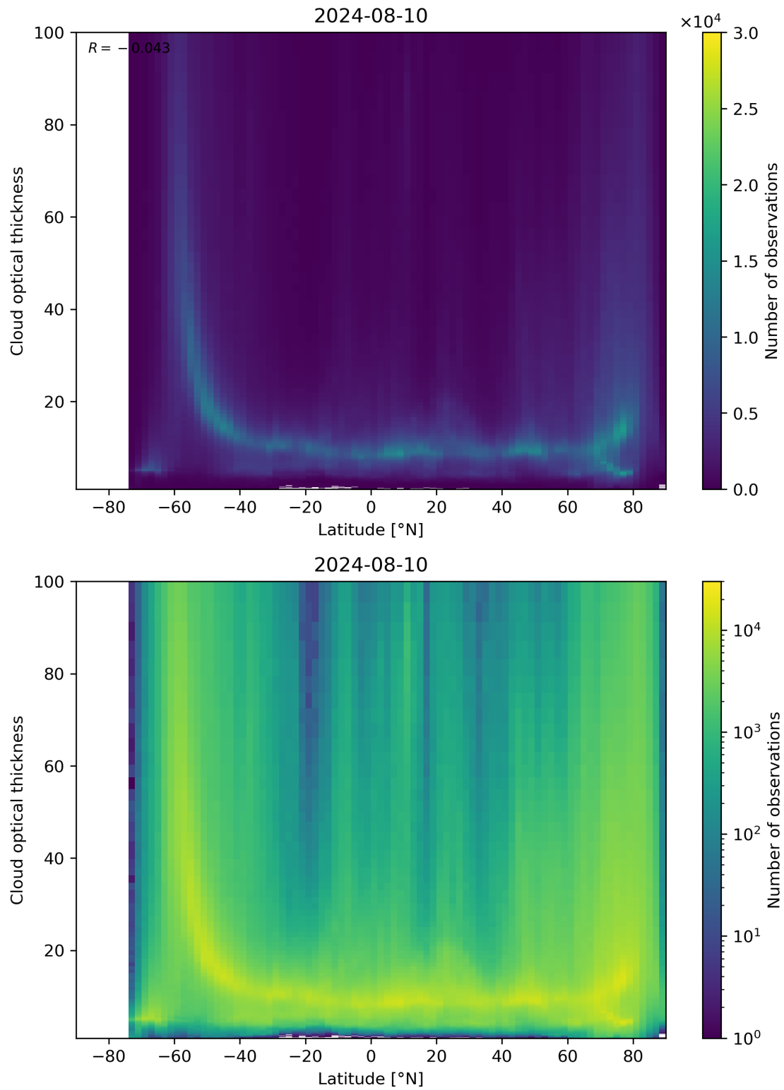
Figure 96: Scatter density plot of “Latitude” against “Cloud optical thickness” for 2024-08-09 to 2024-08-11.
