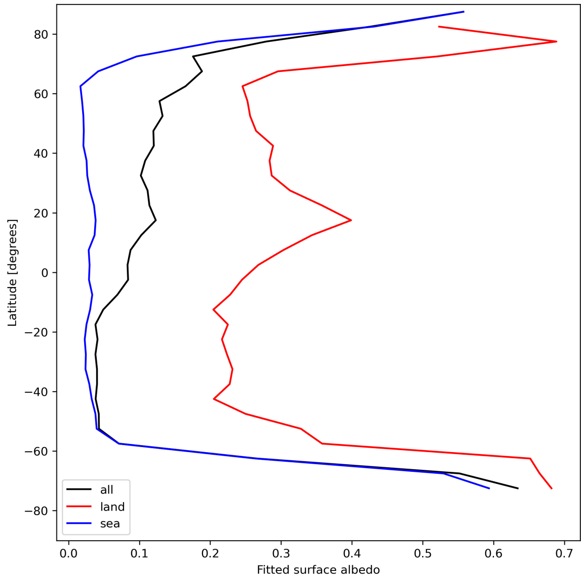
Figure 29: Zonal average of “Fitted surface albedo” for 2024-08-09 to 2024-08-11.
