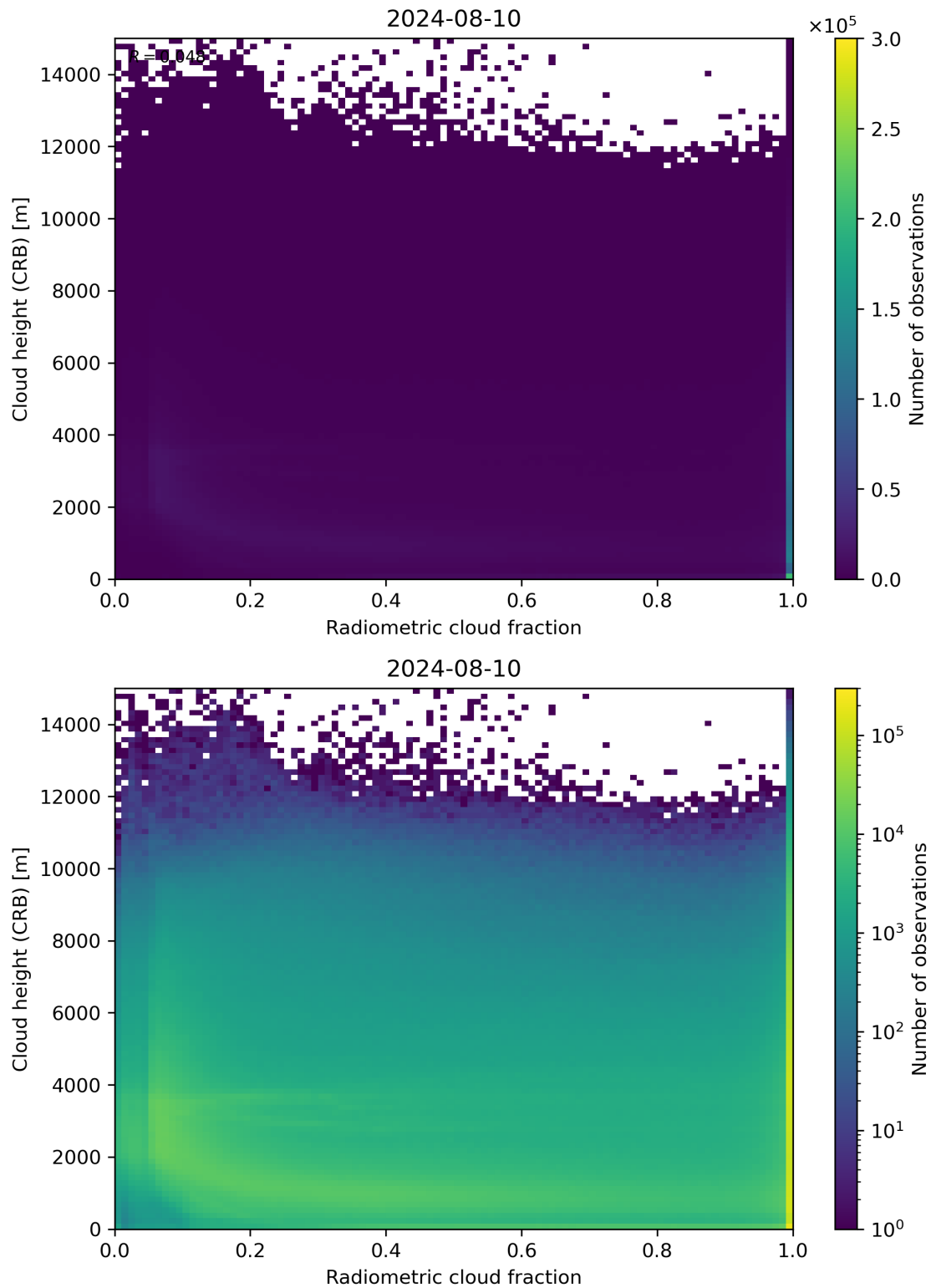
Figure 74: Scatter density plot of “Radiometric cloud fraction” against “Cloud height (CRB)” for 2024-08-09 to 2024-08-11.
