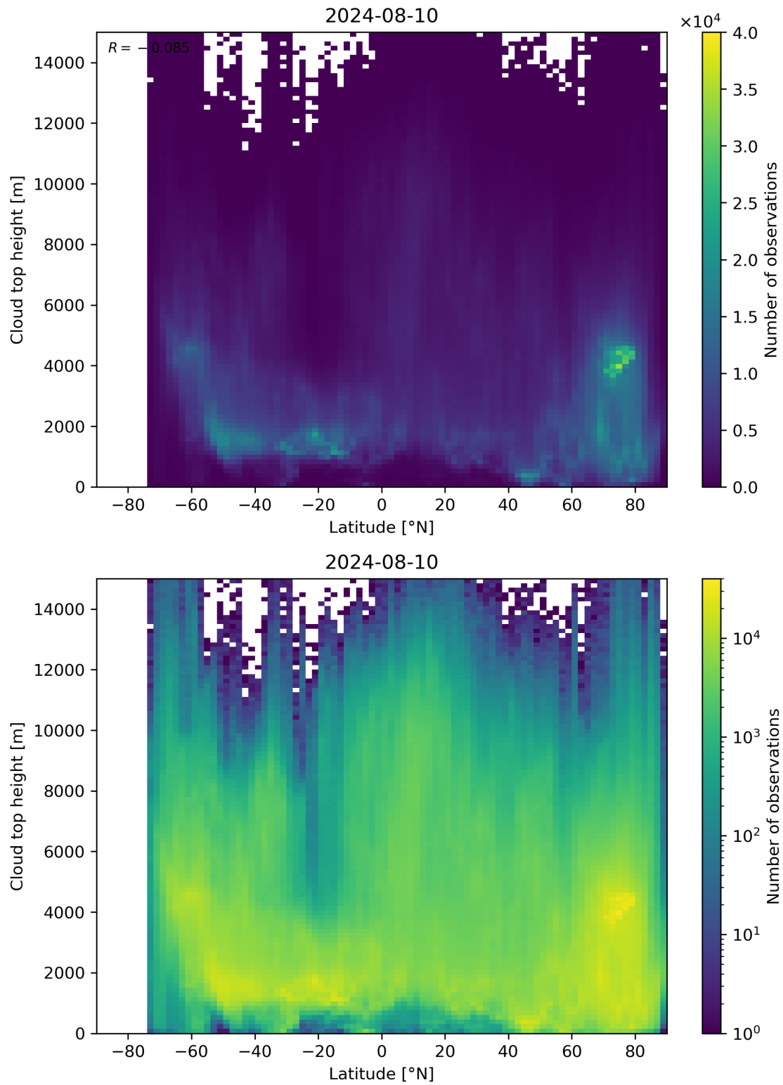
Figure 97: Scatter density plot of “Latitude” against “Cloud top height” for 2024-08-09 to 2024-08-11.
