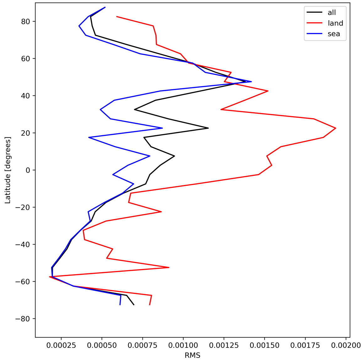
Figure 31: Zonal average of “RMS” for 2024-08-09 to 2024-08-11.
