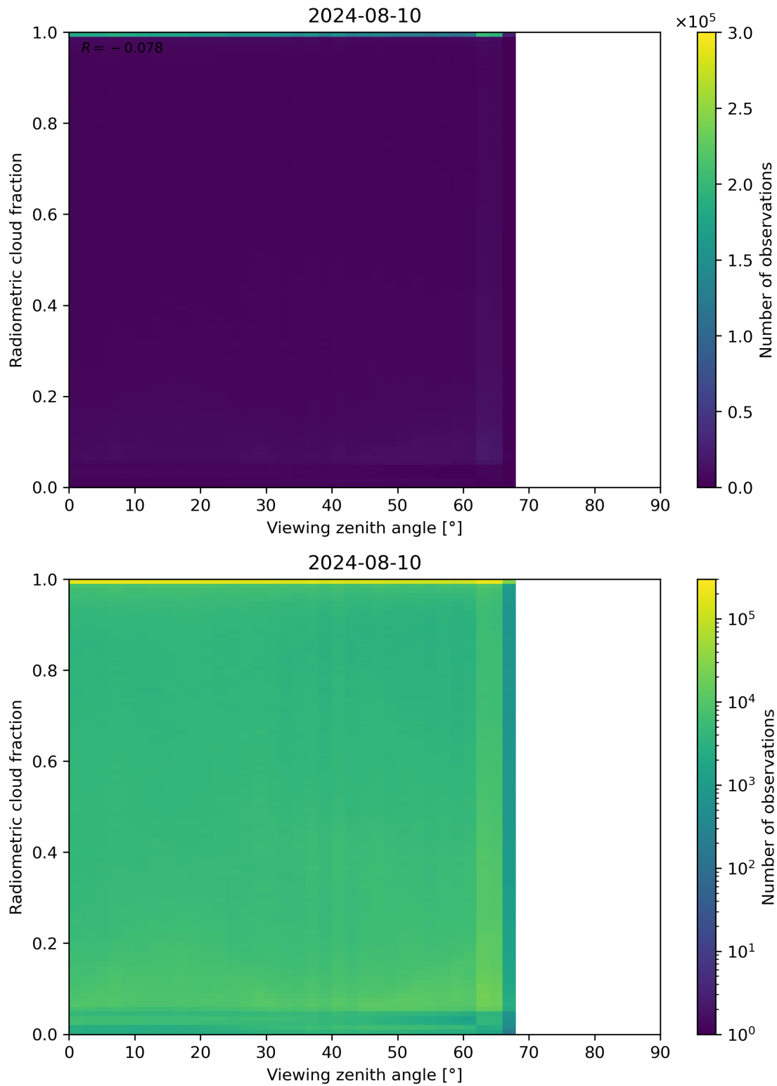
Figure 107: Scatter density plot of “Viewing zenith angle” against “Radiometric cloud fraction” for 2024-08-09 to 2024-08-11.
