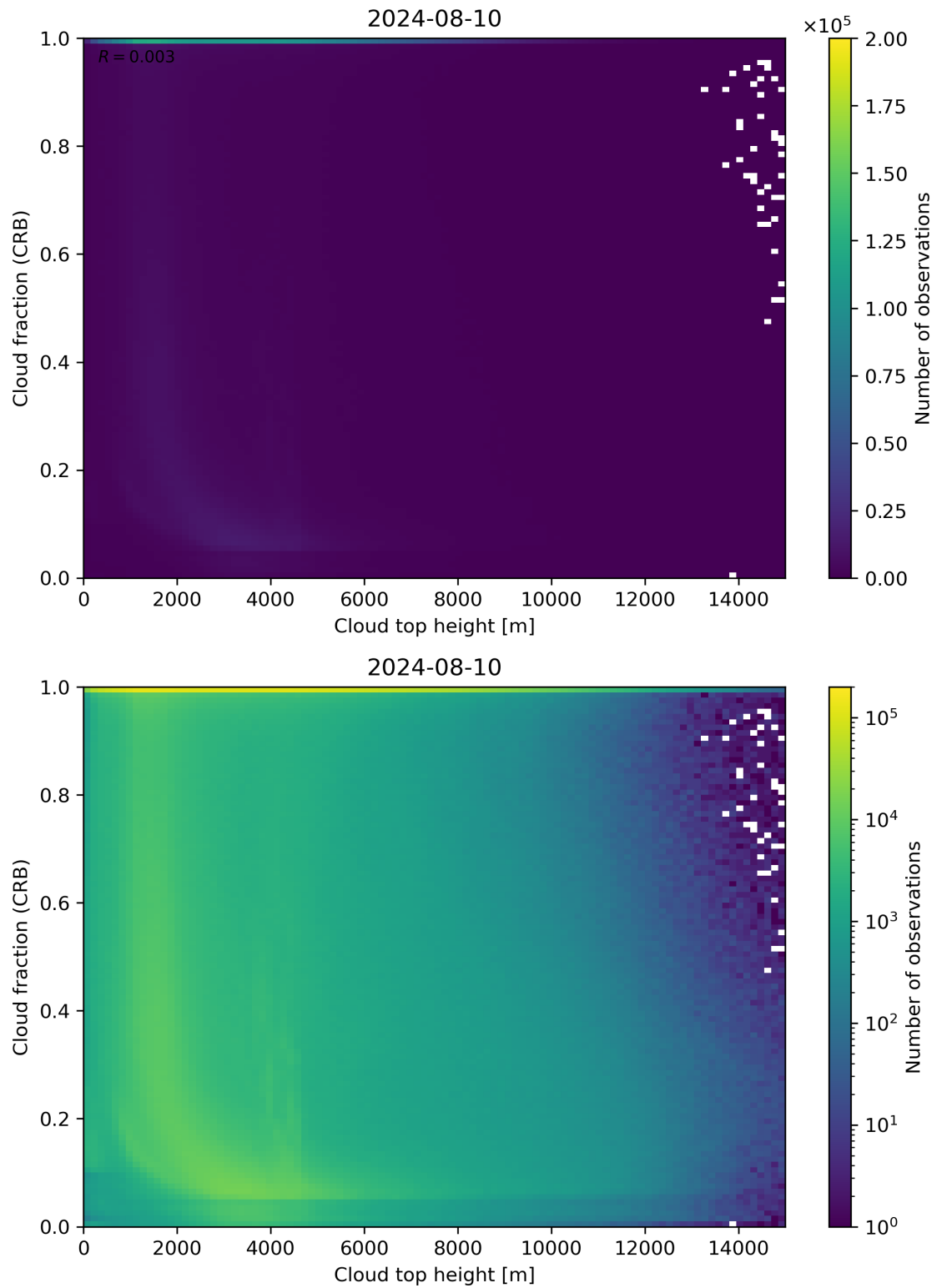
Figure 88: Scatter density plot of “Cloud top height” against “Cloud fraction (CRB)” for 2024-08-09 to 2024-08-11.
