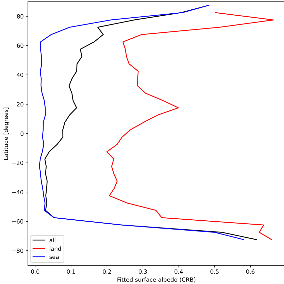
Figure 30: Zonal average of “Fitted surface albedo (CRB)” for 2024-08-09 to 2024-08-11.
