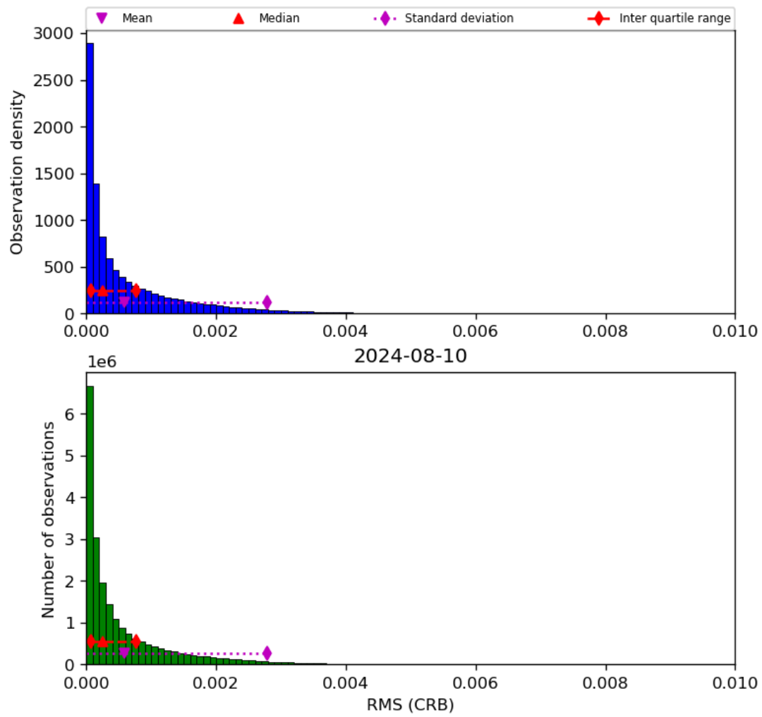
Figure 48: Histogram of “RMS (CRB)” for 2024-08-09 to 2024-08-11
