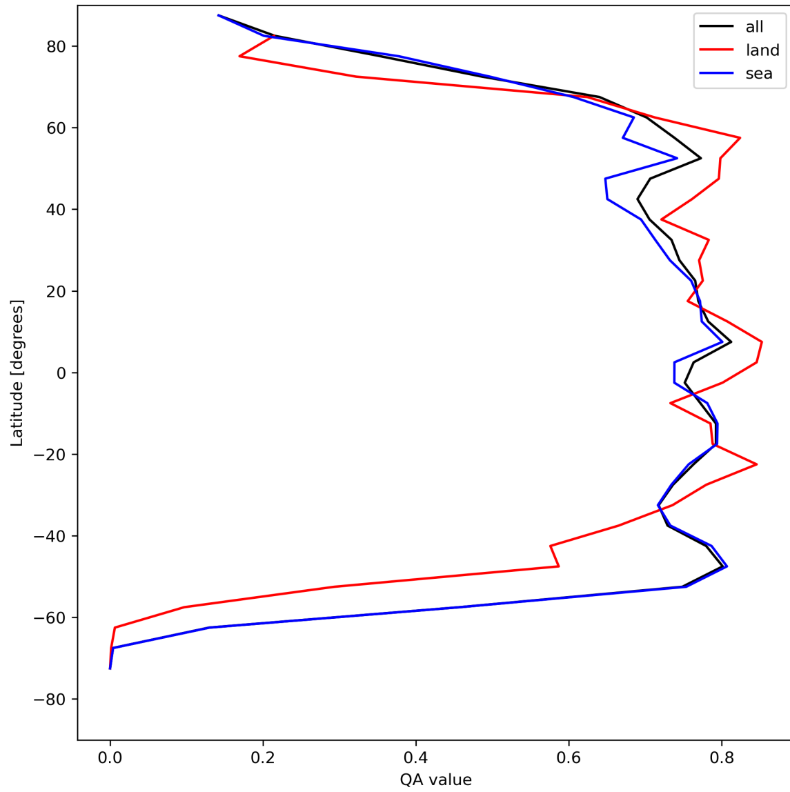
Figure 22: Zonal average of “QA value” for 2024-08-09 to 2024-08-11.
