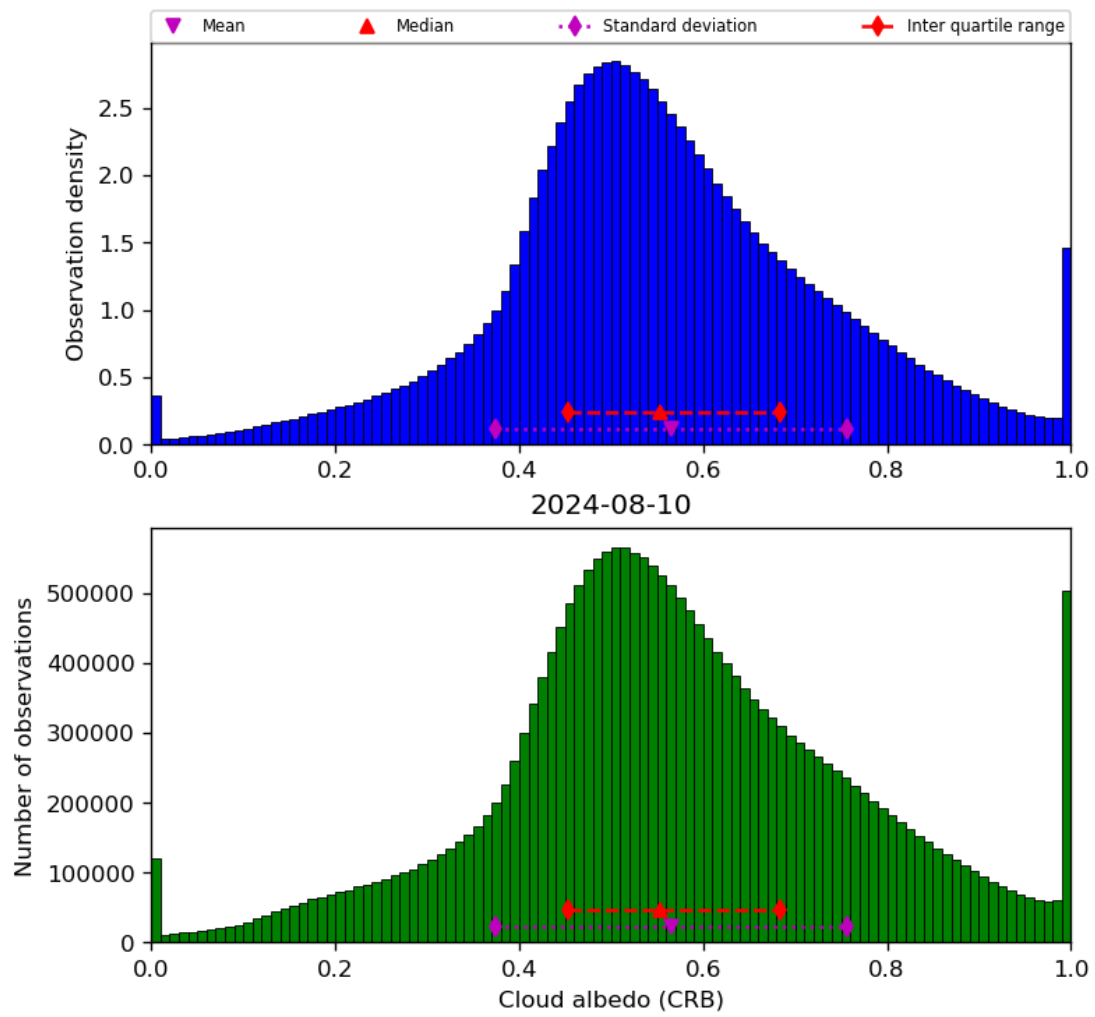
Figure 44: Histogram of “Cloud albedo (CRB)” for 2024-08-09 to 2024-08-11
