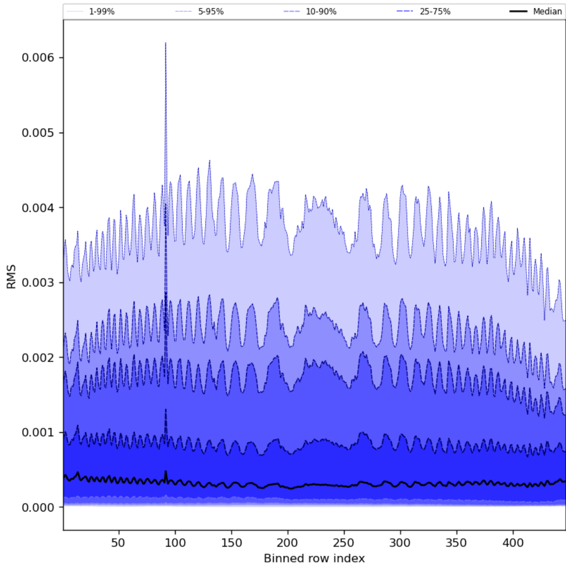
Figure 63: Along track statistics of “RMS” for 2024-08-09 to 2024-08-11
