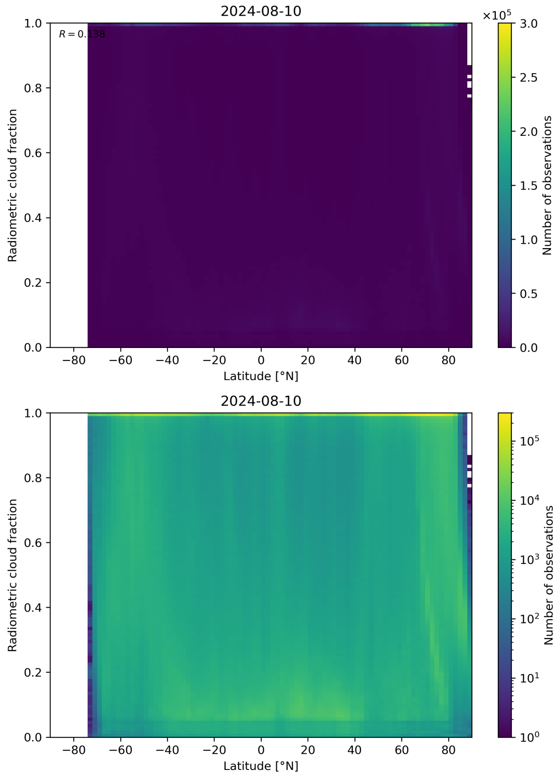
Figure 92: Scatter density plot of “Latitude” against “Radiometric cloud fraction” for 2024-08-09 to 2024-08-11.
