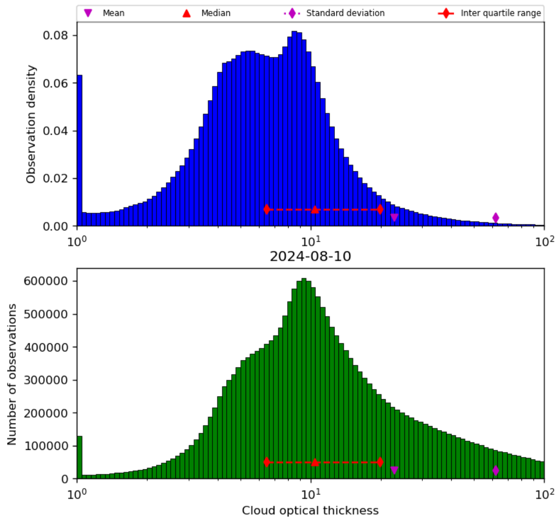
Figure 41: Histogram of “Cloud optical thickness” for 2024-08-09 to 2024-08-11
