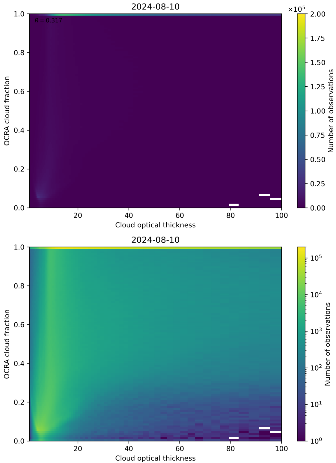
Figure 83: Scatter density plot of “Cloud optical thickness” against “OCRA cloud fraction” for 2024-08-09 to 2024-08-11.
