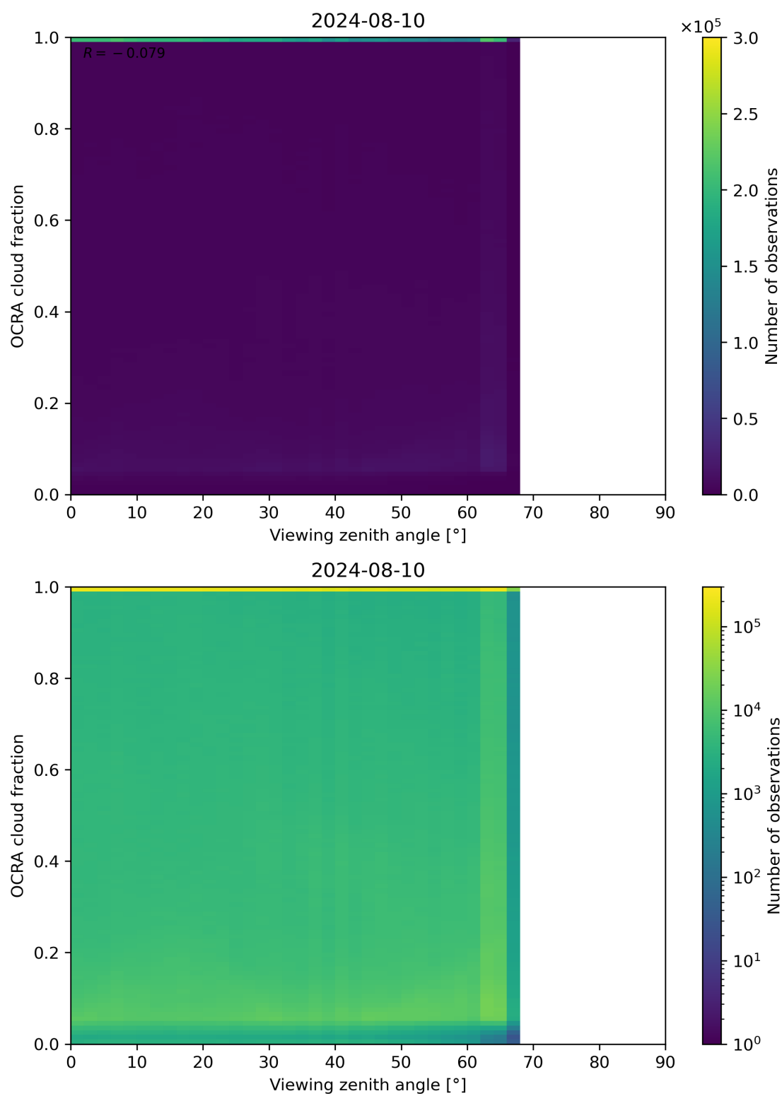
Figure 108: Scatter density plot of “Viewing zenith angle” against “OCRA cloud fraction” for 2024-08-09 to 2024-08-11.
