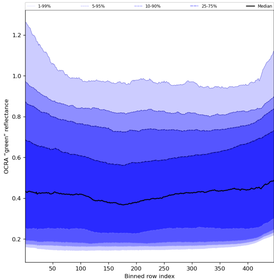
Figure 68: Along track statistics of “OCRA “green” reflectance” for 2024-08-09 to 2024-08-11
