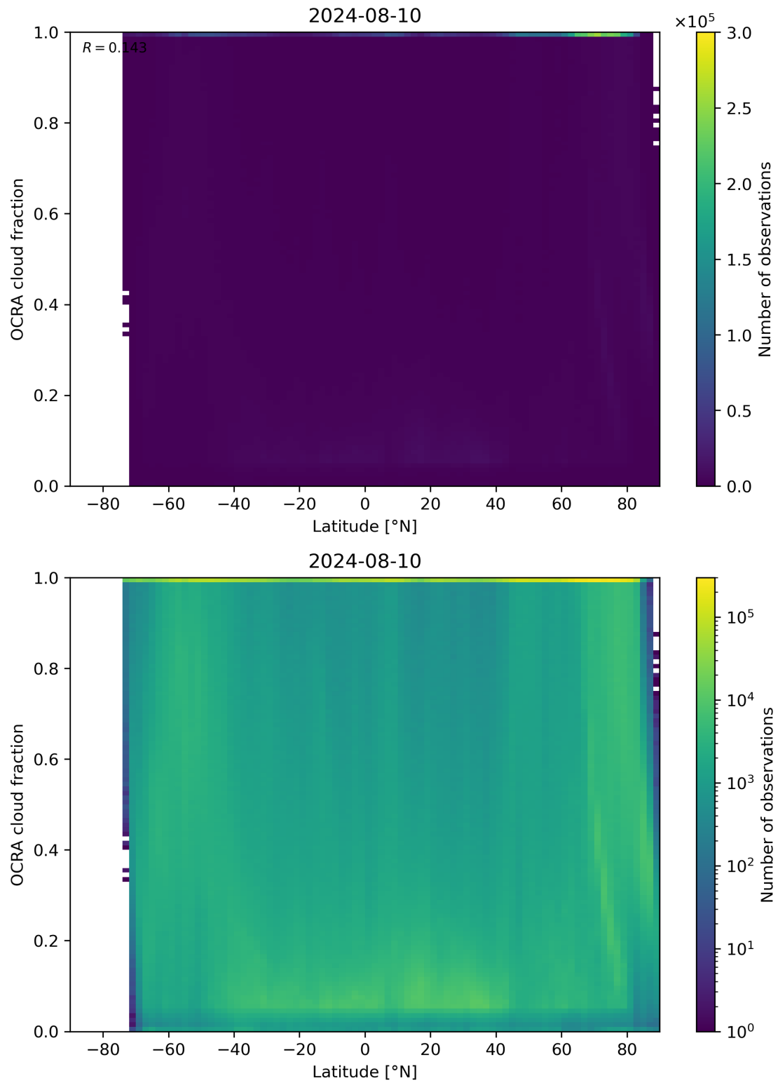
Figure 93: Scatter density plot of “Latitude” against “OCRA cloud fraction” for 2024-08-09 to 2024-08-11.
