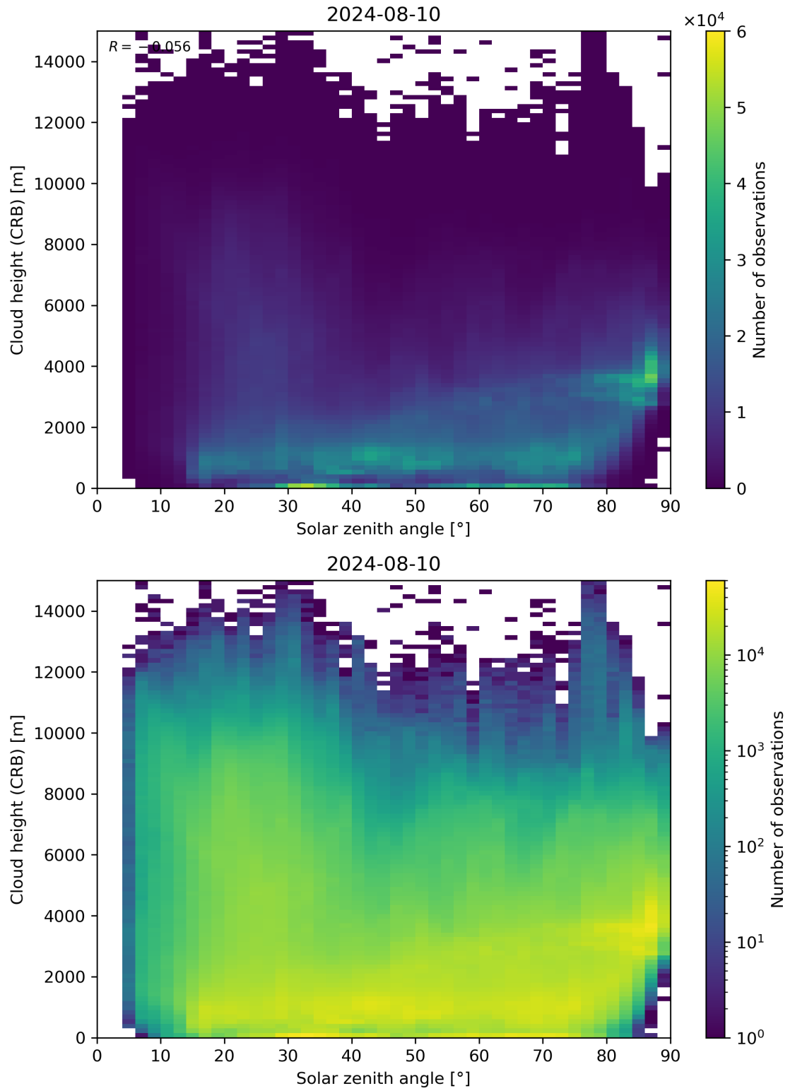
Figure 102: Scatter density plot of “Solar zenith angle” against “Cloud height (CRB)” for 2024-08-09 to 2024-08-11.
