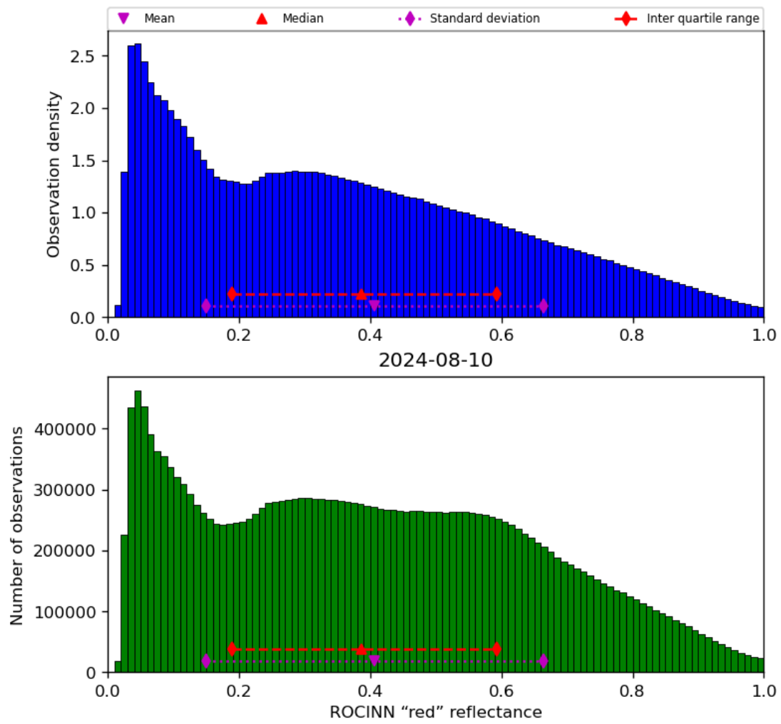
Figure 53: Histogram of “ROCINN “red” reflectance” for 2024-08-09 to 2024-08-11
