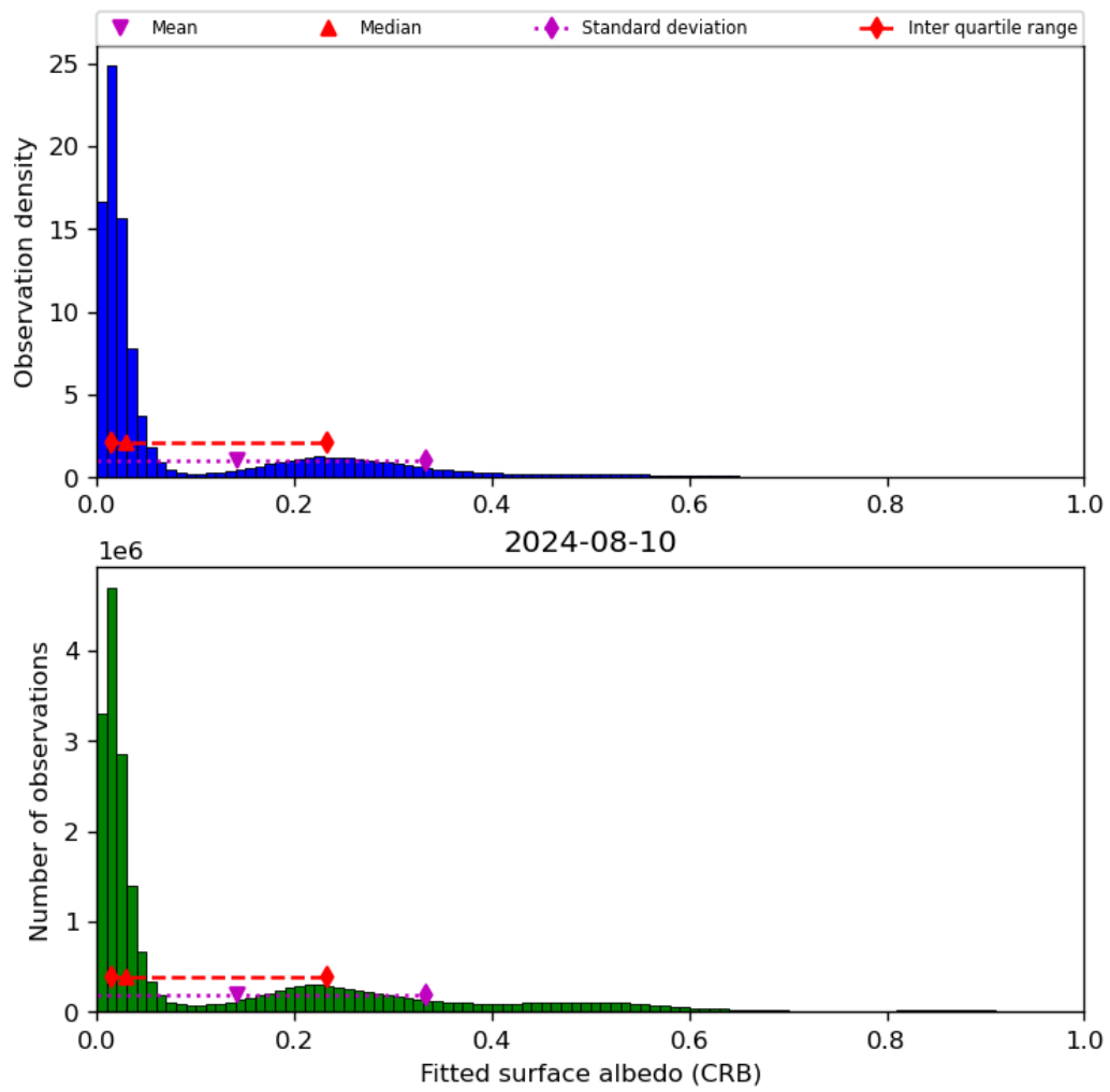
Figure 46: Histogram of “Fitted surface albedo (CRB)” for 2024-08-09 to 2024-08-11
