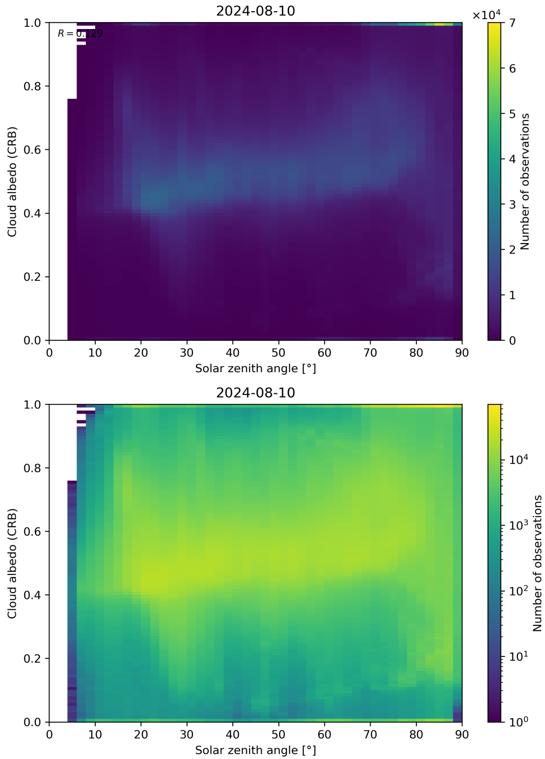
Figure 98: Scatter density plot of “Solar zenith angle” against “Cloud albedo (CRB)” for 2024-08-09 to 2024-08-11.
