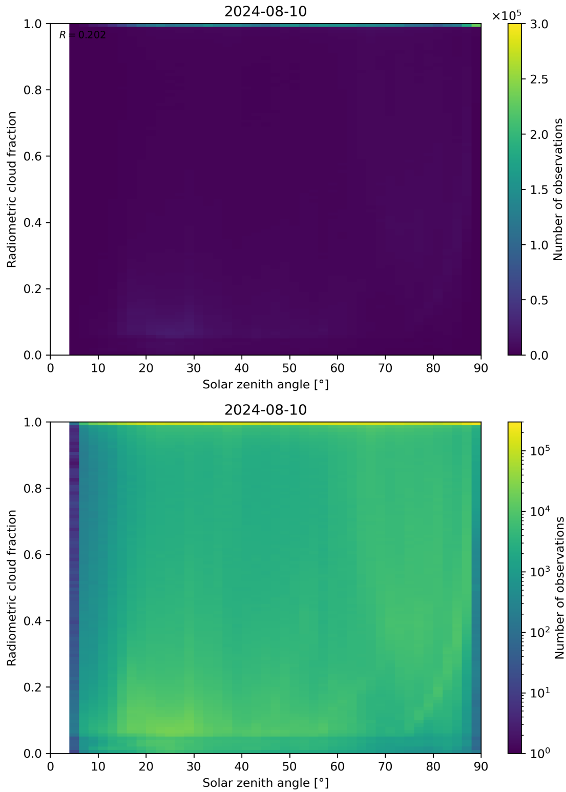
Figure 99: Scatter density plot of “Solar zenith angle” against “Radiometric cloud fraction” for 2024-08-09 to 2024-08-11.
