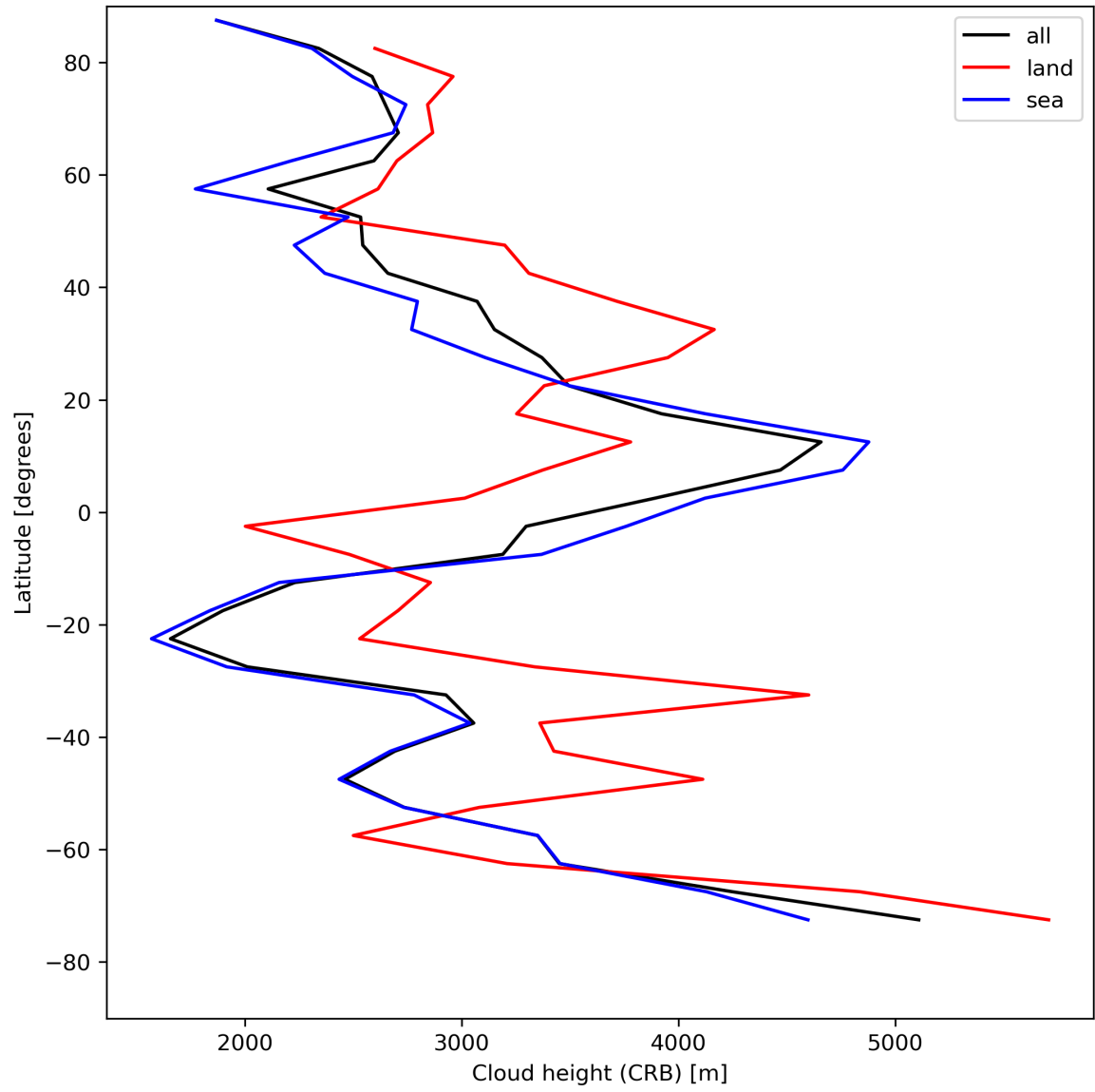
Figure 27: Zonal average of “Cloud height (CRB)” for 2024-08-09 to 2024-08-11.
