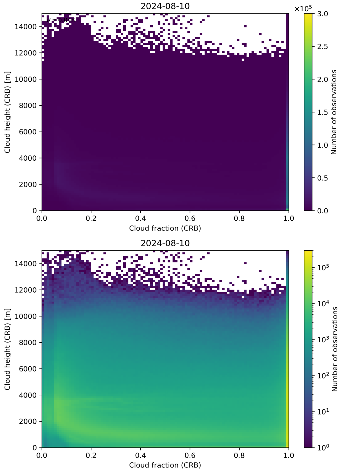
Figure 79: Scatter density plot of “Cloud fraction (CRB)” against “Cloud height (CRB)” for 2024-08-09 to 2024-08-11.
