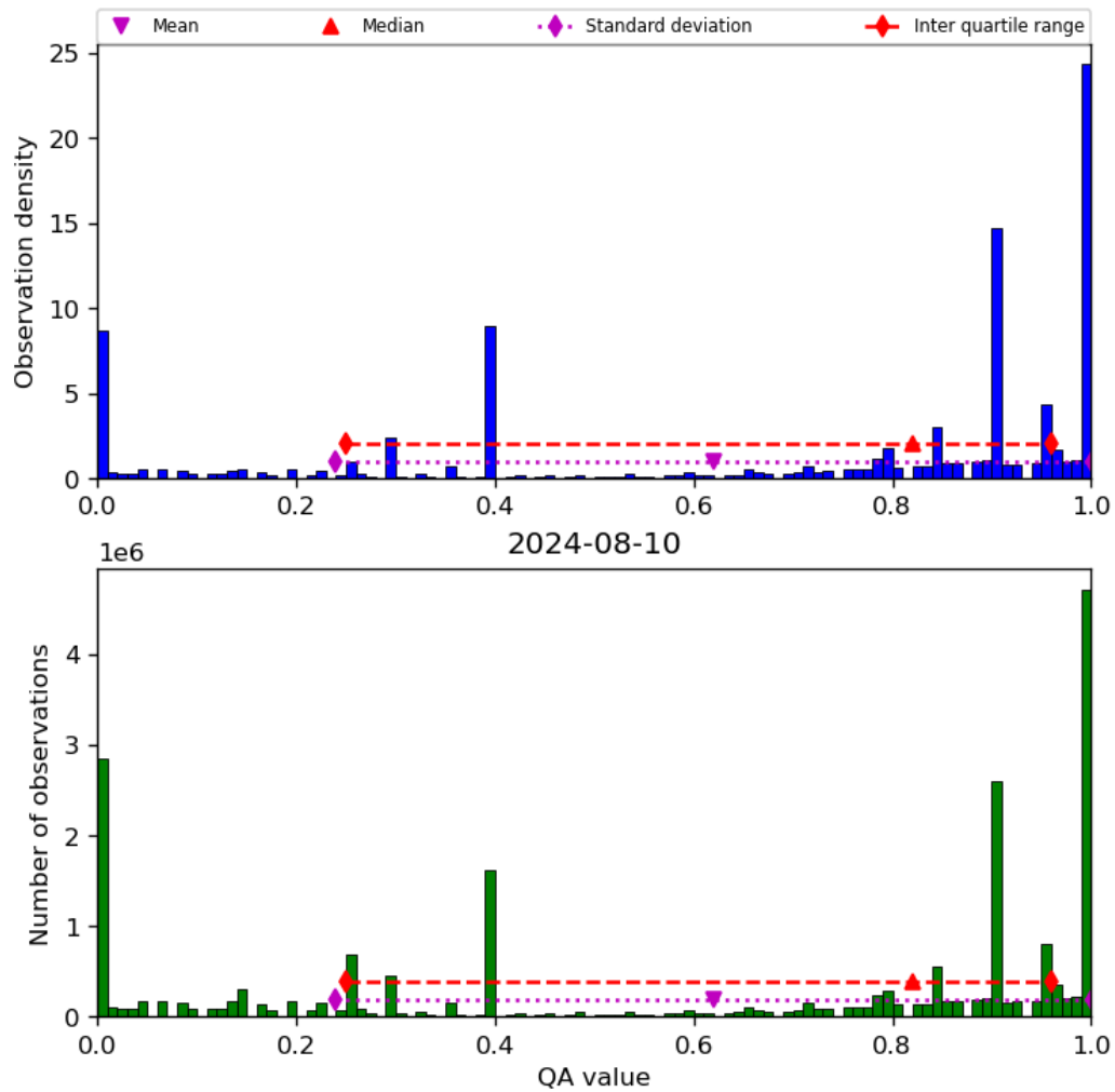
Figure 38: Histogram of “QA value” for 2024-08-09 to 2024-08-11
