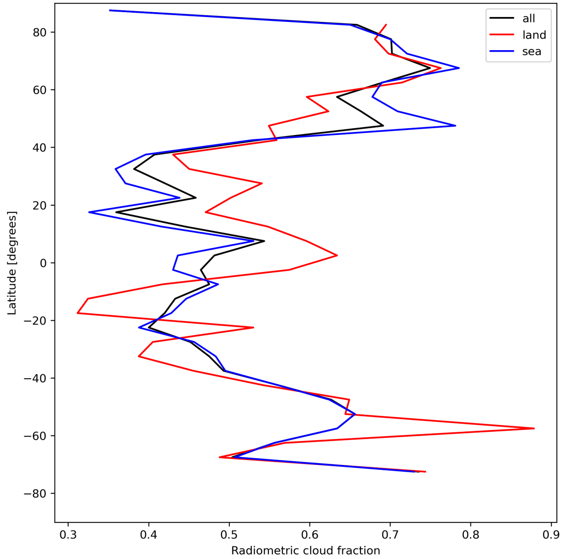
Figure 23: Zonal average of “Radiometric cloud fraction” for 2024-08-09 to 2024-08-11.
