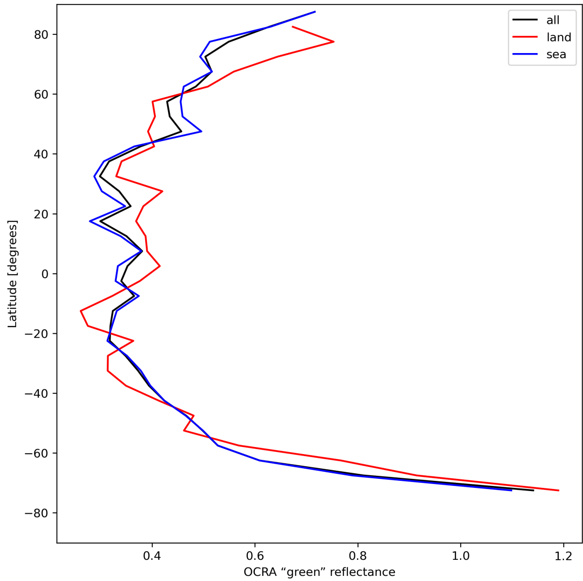
Figure 36: Zonal average of “OCRA “green” reflectance” for 2024-08-09 to 2024-08-11.
