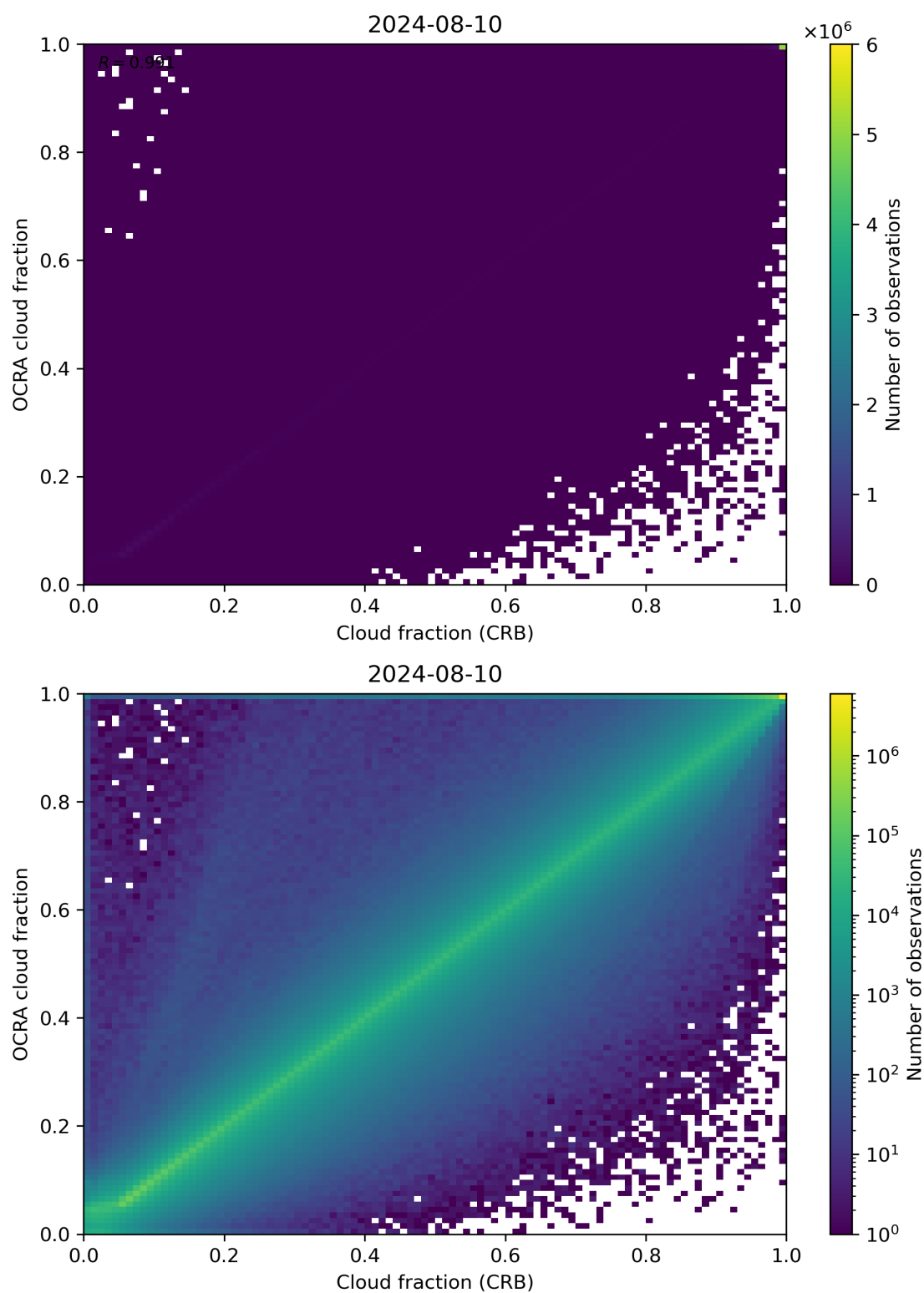
Figure 78: Scatter density plot of “Cloud fraction (CRB)” against “OCRA cloud fraction” for 2024-08-09 to 2024-08-11.
