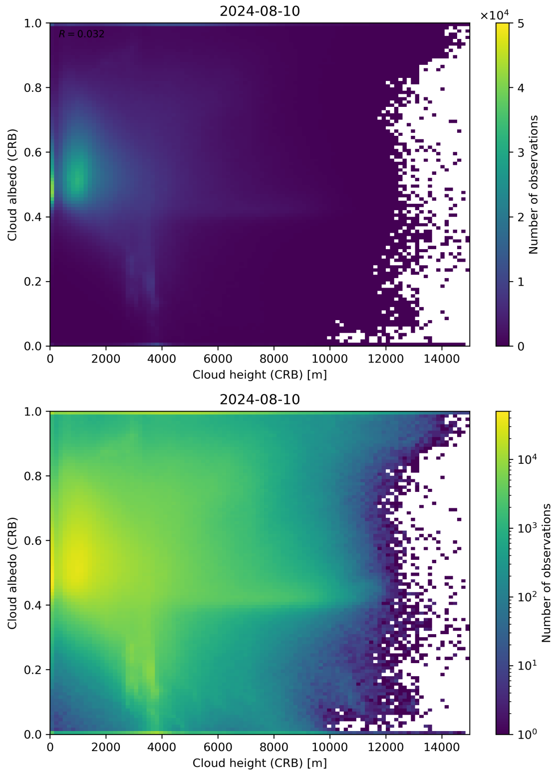
Figure 80: Scatter density plot of “Cloud height (CRB)” against “Cloud albedo (CRB)” for 2024-08-09 to 2024-08-11.
