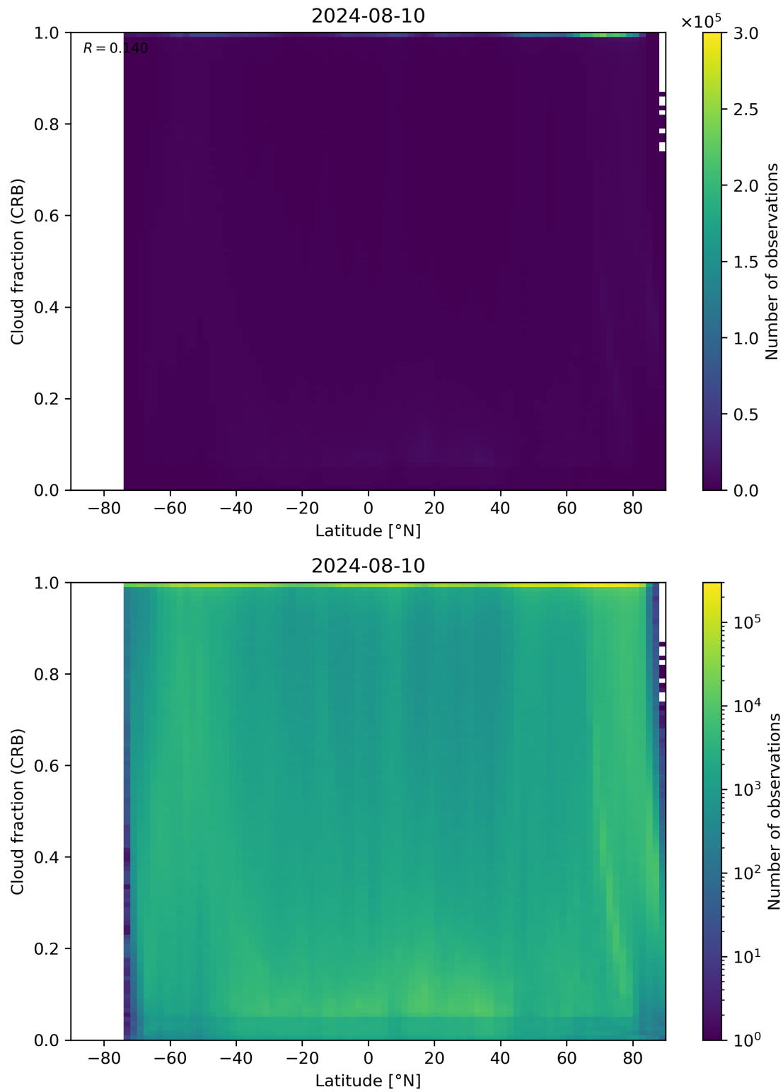
Figure 94: Scatter density plot of “Latitude” against “Cloud fraction (CRB)” for 2024-08-09 to 2024-08-11.
