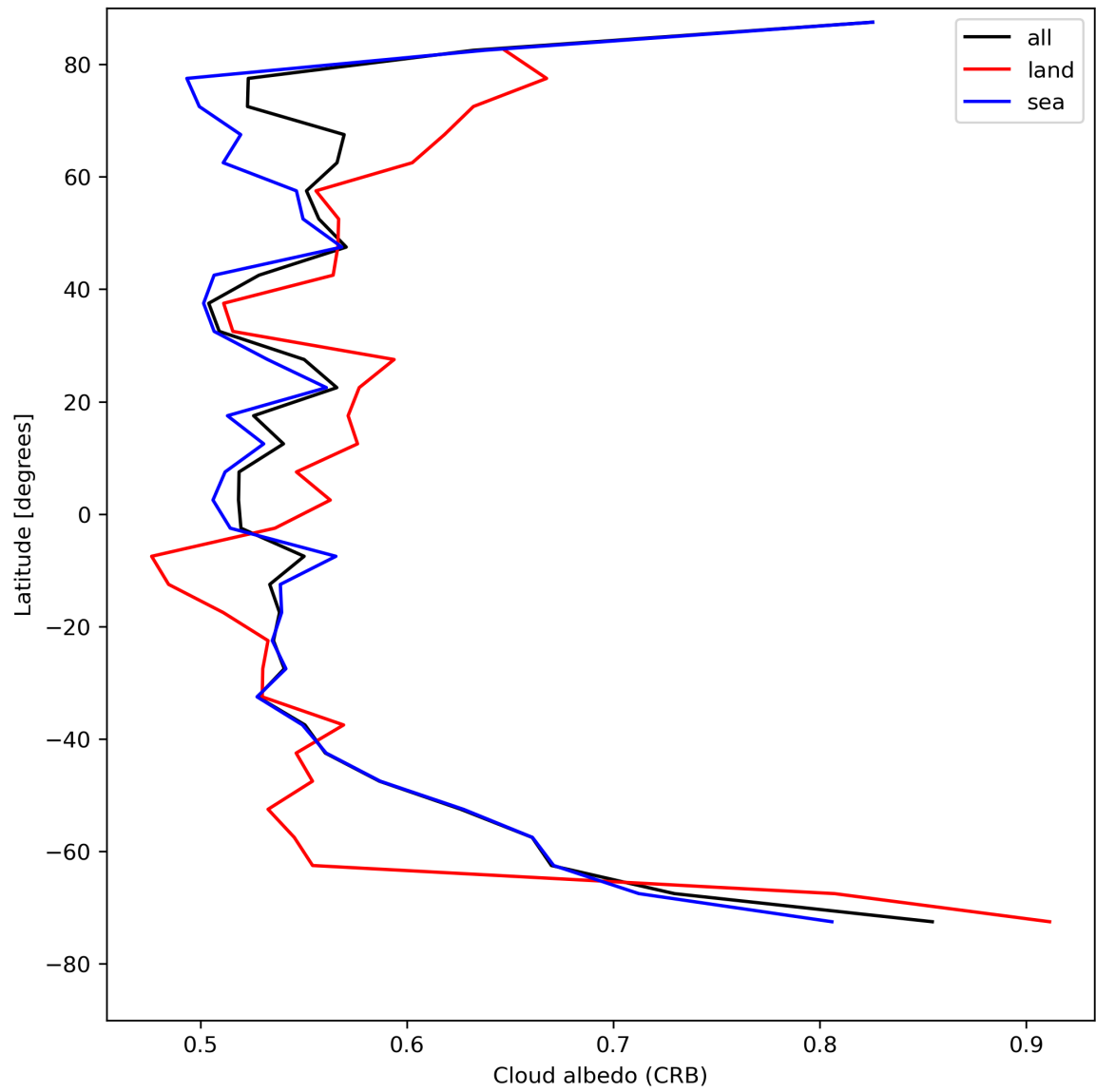
Figure 28: Zonal average of “Cloud albedo (CRB)” for 2024-08-09 to 2024-08-11.
