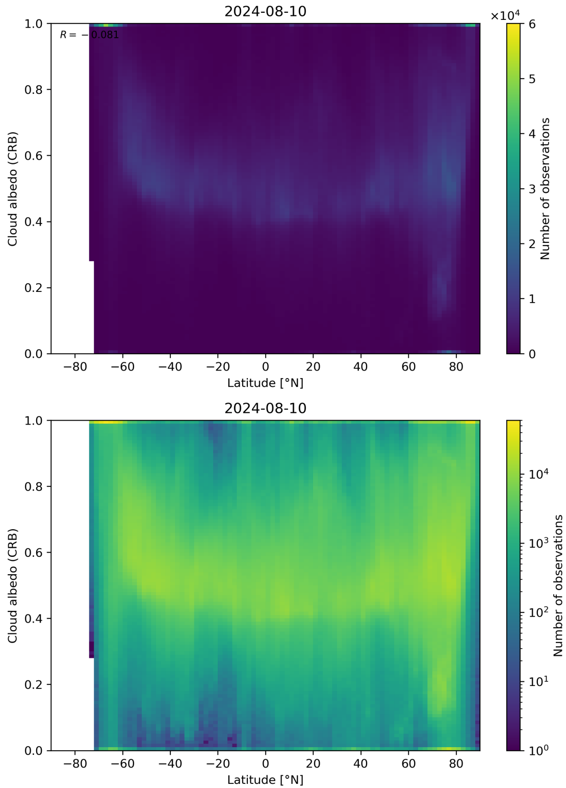
Figure 91: Scatter density plot of “Latitude” against “Cloud albedo (CRB)” for 2024-08-09 to 2024-08-11.
