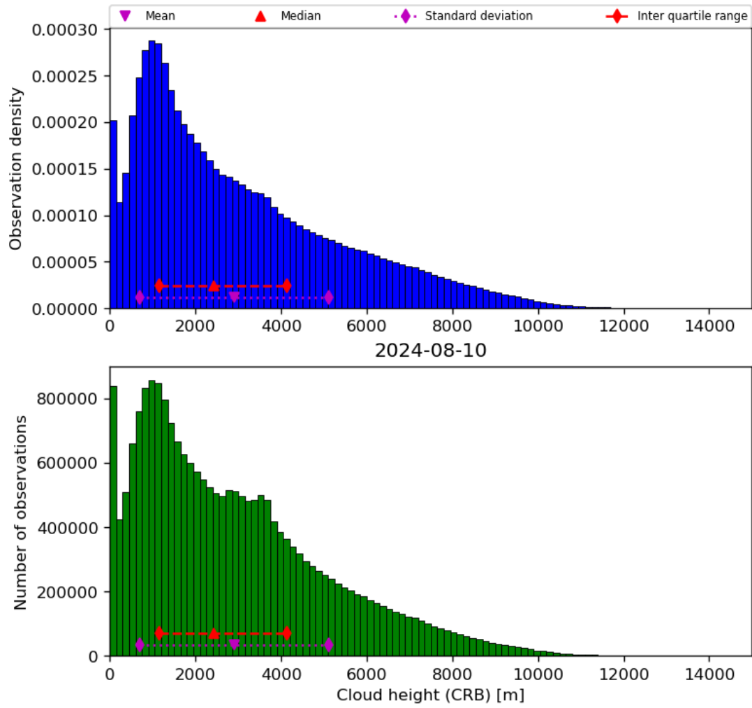
Figure 43: Histogram of “Cloud height (CRB)” for 2024-08-09 to 2024-08-11
