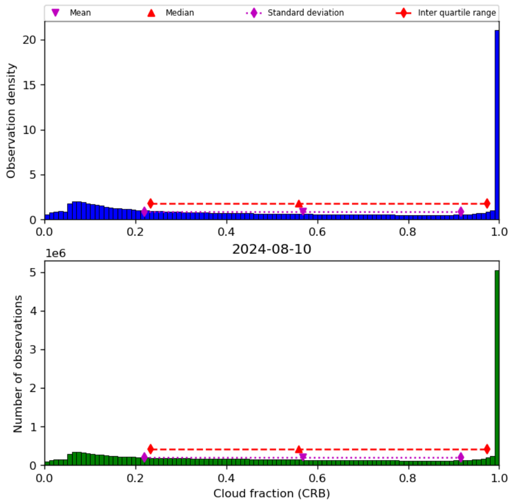
Figure 42: Histogram of “Cloud fraction (CRB)” for 2024-08-09 to 2024-08-11
