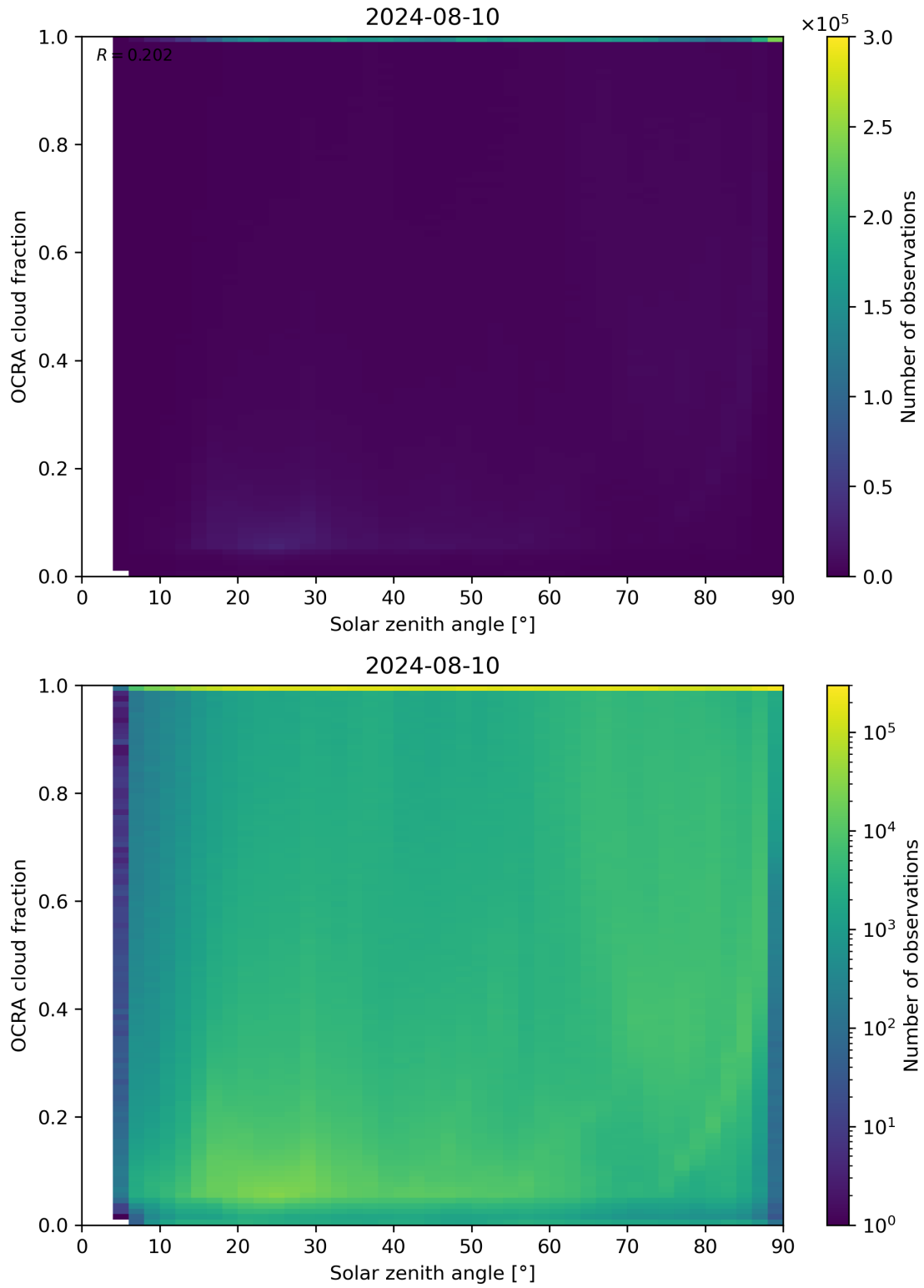
Figure 100: Scatter density plot of “Solar zenith angle” against “OCRA cloud fraction” for 2024-08-09 to 2024-08-11.
