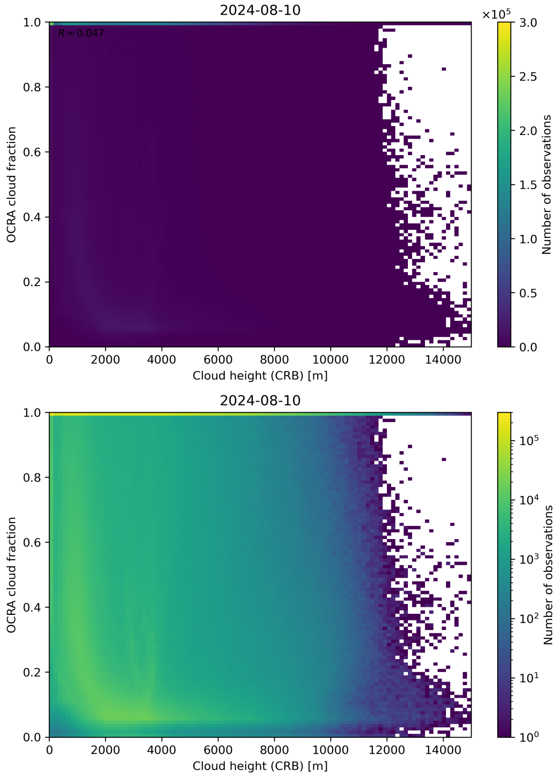
Figure 81: Scatter density plot of “Cloud height (CRB)” against “OCRA cloud fraction” for 2024-08-09 to 2024-08-11.
