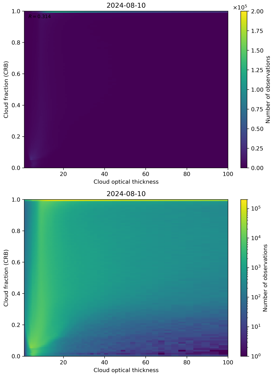
Figure 84: Scatter density plot of “Cloud optical thickness” against “Cloud fraction (CRB)” for 2024-08-09 to 2024-08-11.
