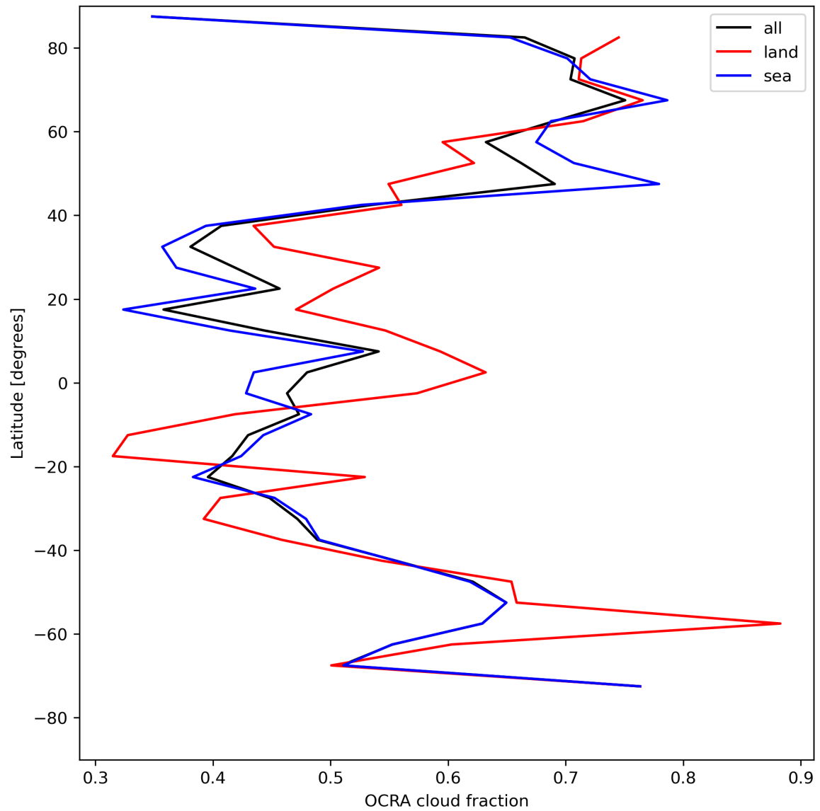
Figure 34: Zonal average of “OCRA cloud fraction” for 2024-08-09 to 2024-08-11.
