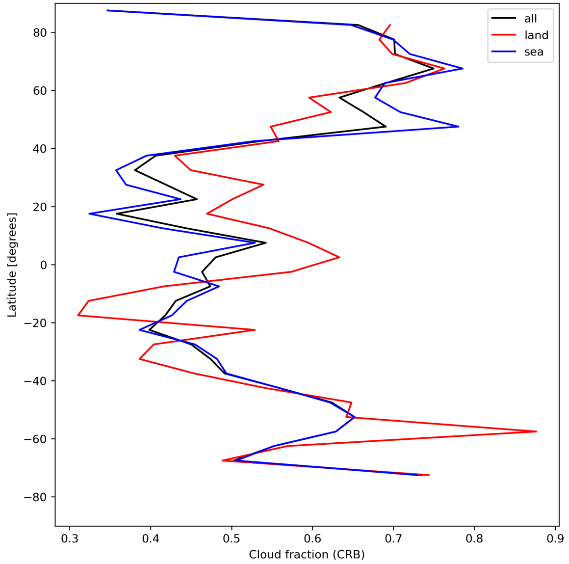
Figure 26: Zonal average of “Cloud fraction (CRB)” for 2024-08-09 to 2024-08-11.
