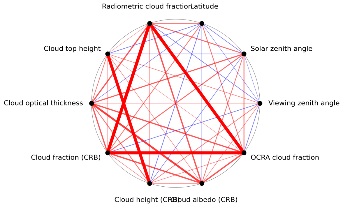
Figure 1: Map of correlation graph for 2024-08-09 to 2024-08-11.
