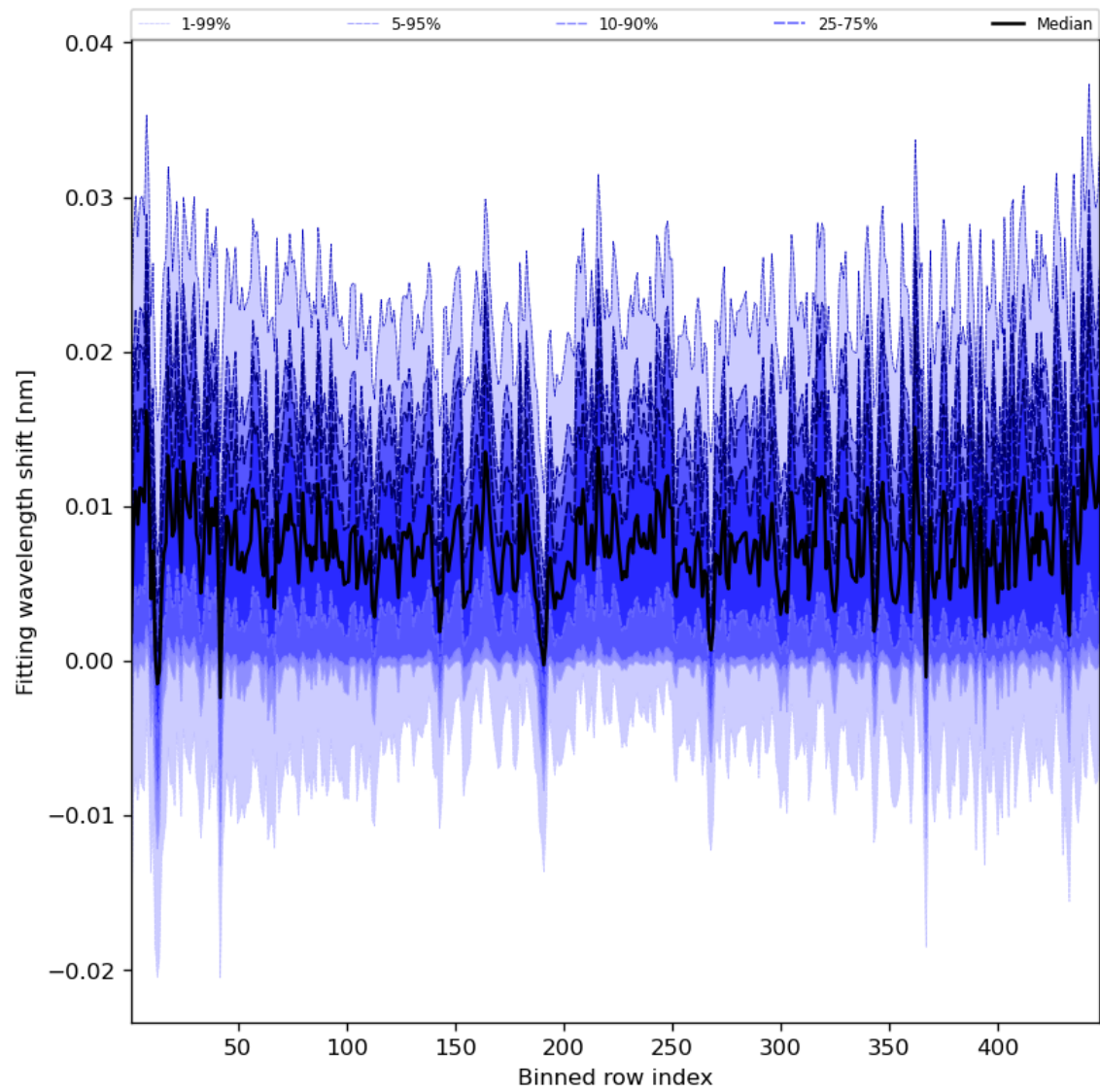
Figure 65: Along track statistics of “Fitting wavelength shift” for 2024-08-09 to 2024-08-11
