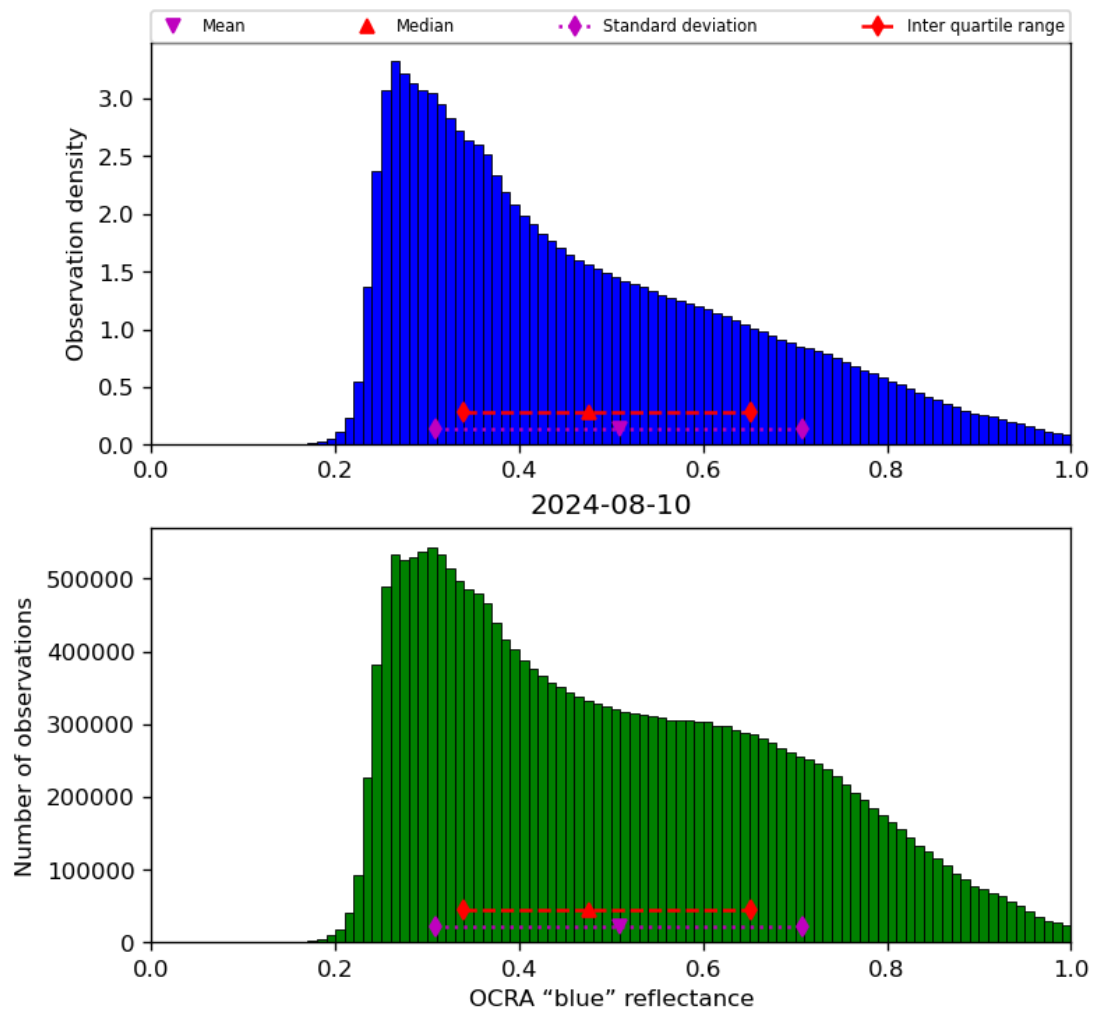
Figure 51: Histogram of “OCRA “blue” reflectance” for 2024-08-09 to 2024-08-11
