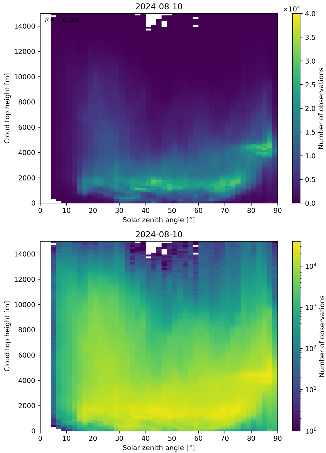
Figure 104: Scatter density plot of “Solar zenith angle” against “Cloud top height” for 2024-08-09 to 2024-08-11.
