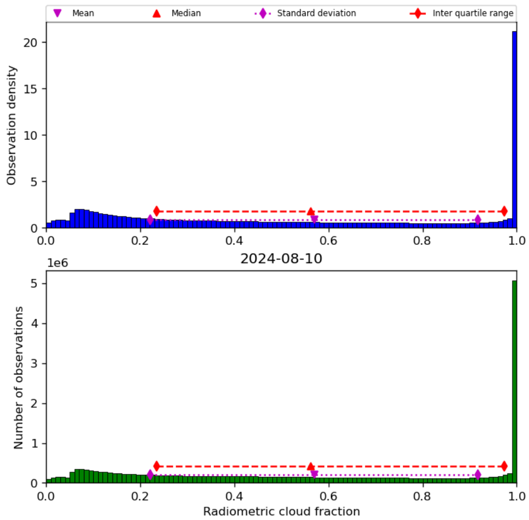
Figure 39: Histogram of “Radiometric cloud fraction” for 2024-08-09 to 2024-08-11
