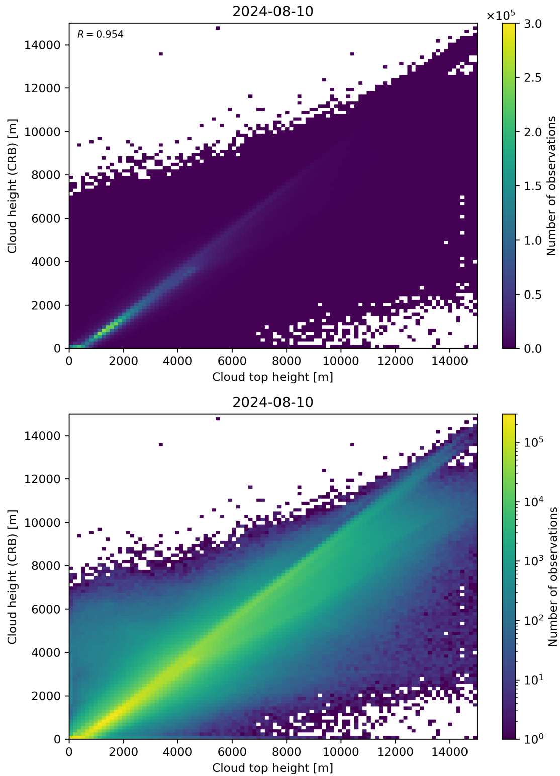
Figure 89: Scatter density plot of “Cloud top height” against “Cloud height (CRB)” for 2024-08-09 to 2024-08-11.
