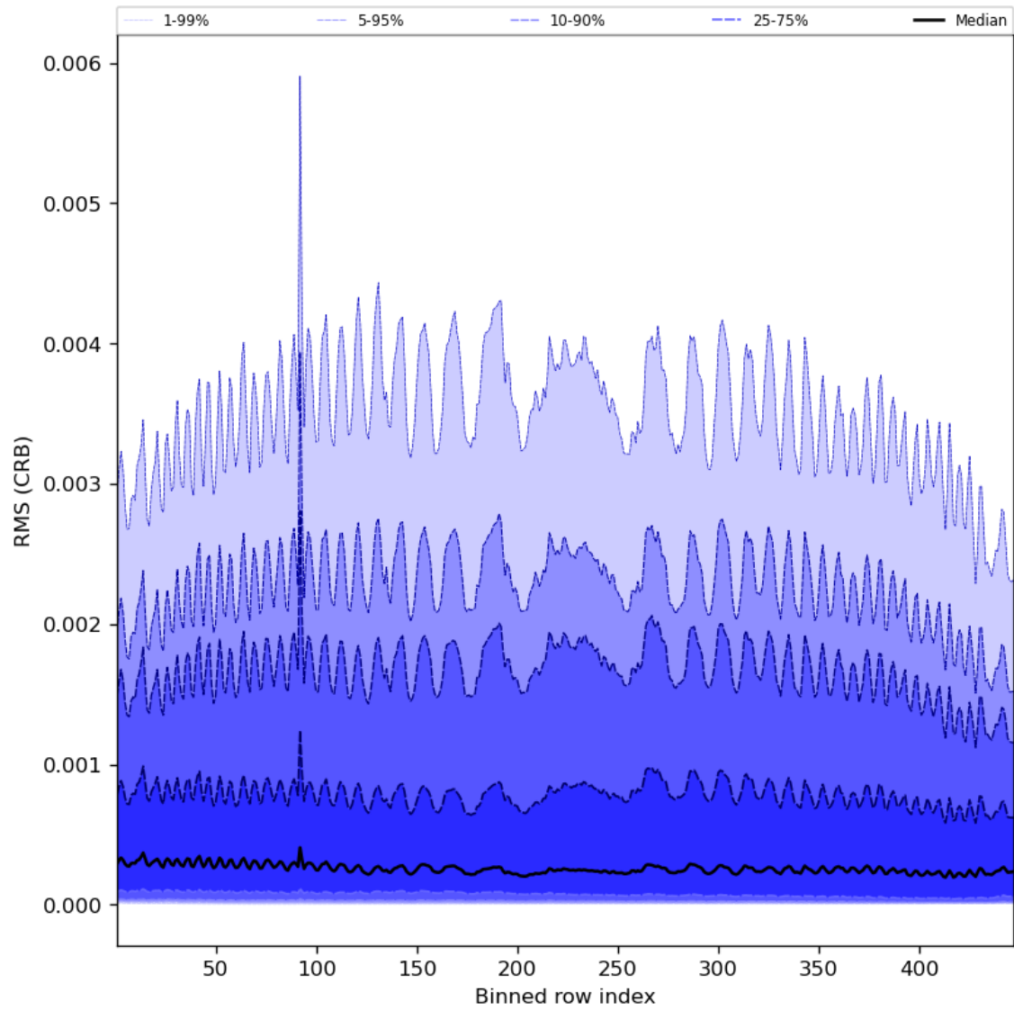
Figure 64: Along track statistics of “RMS (CRB)” for 2024-08-09 to 2024-08-11
