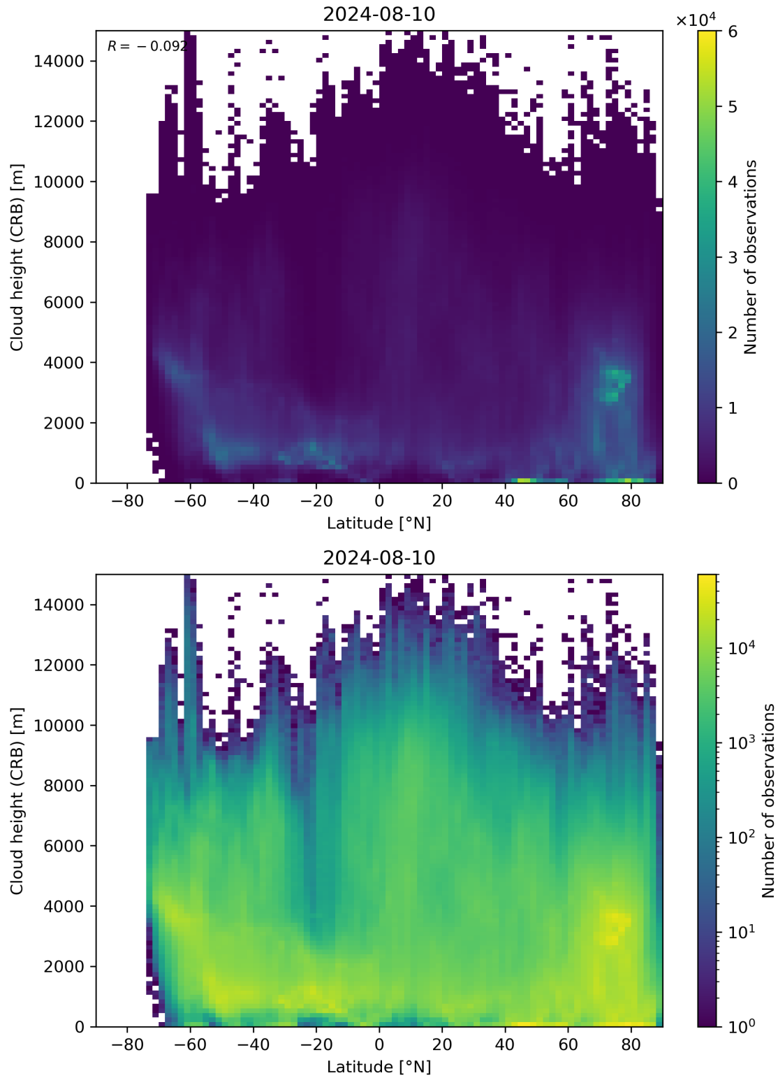
Figure 95: Scatter density plot of “Latitude” against “Cloud height (CRB)” for 2024-08-09 to 2024-08-11.
