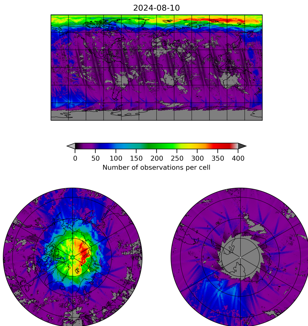
Figure 21: Map of the number of observations for 2024-08-09 to 2024-08-11
