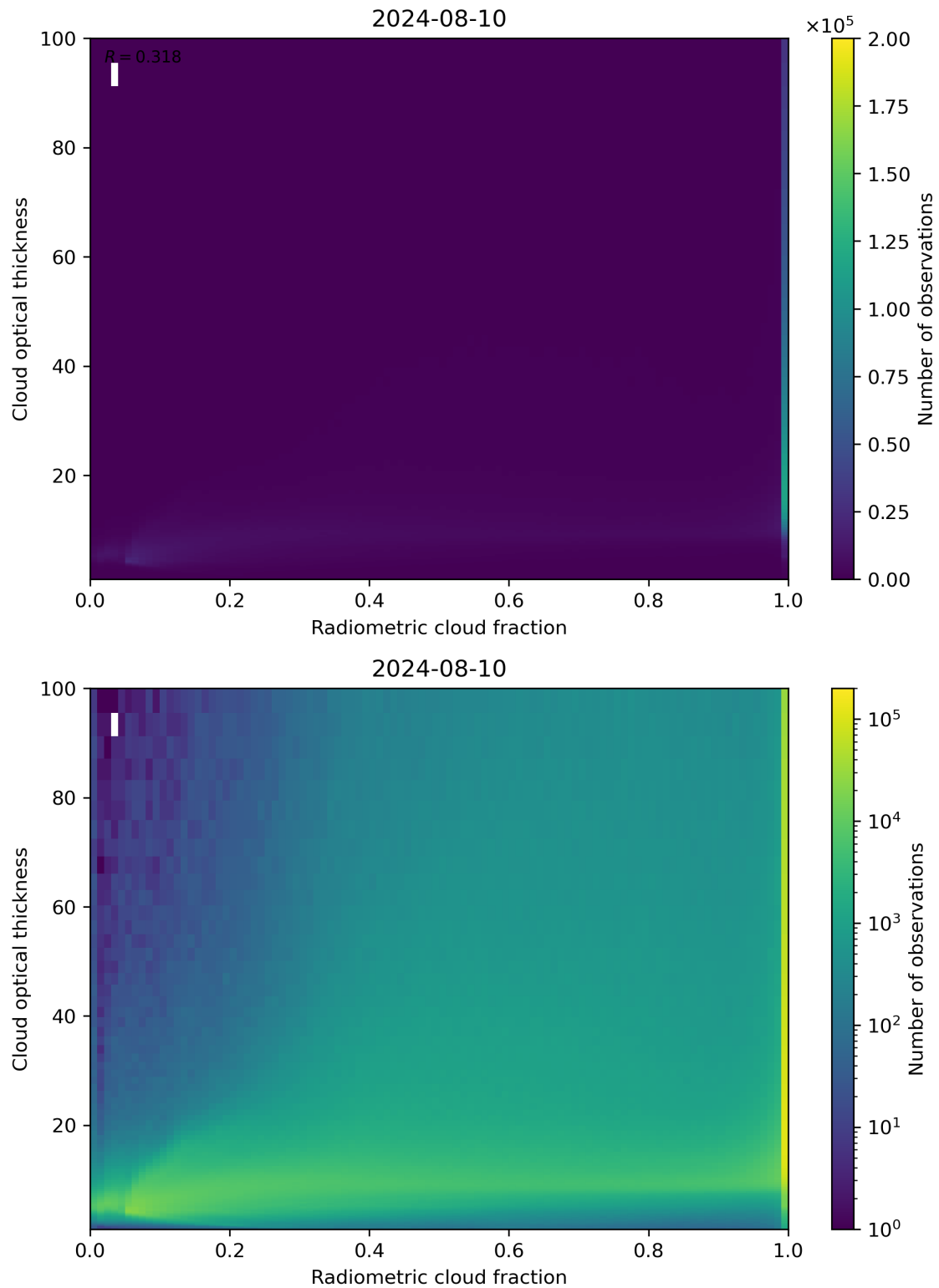
Figure 75: Scatter density plot of “Radiometric cloud fraction” against “Cloud optical thickness” for 2024-08-09 to 2024-08-11.
