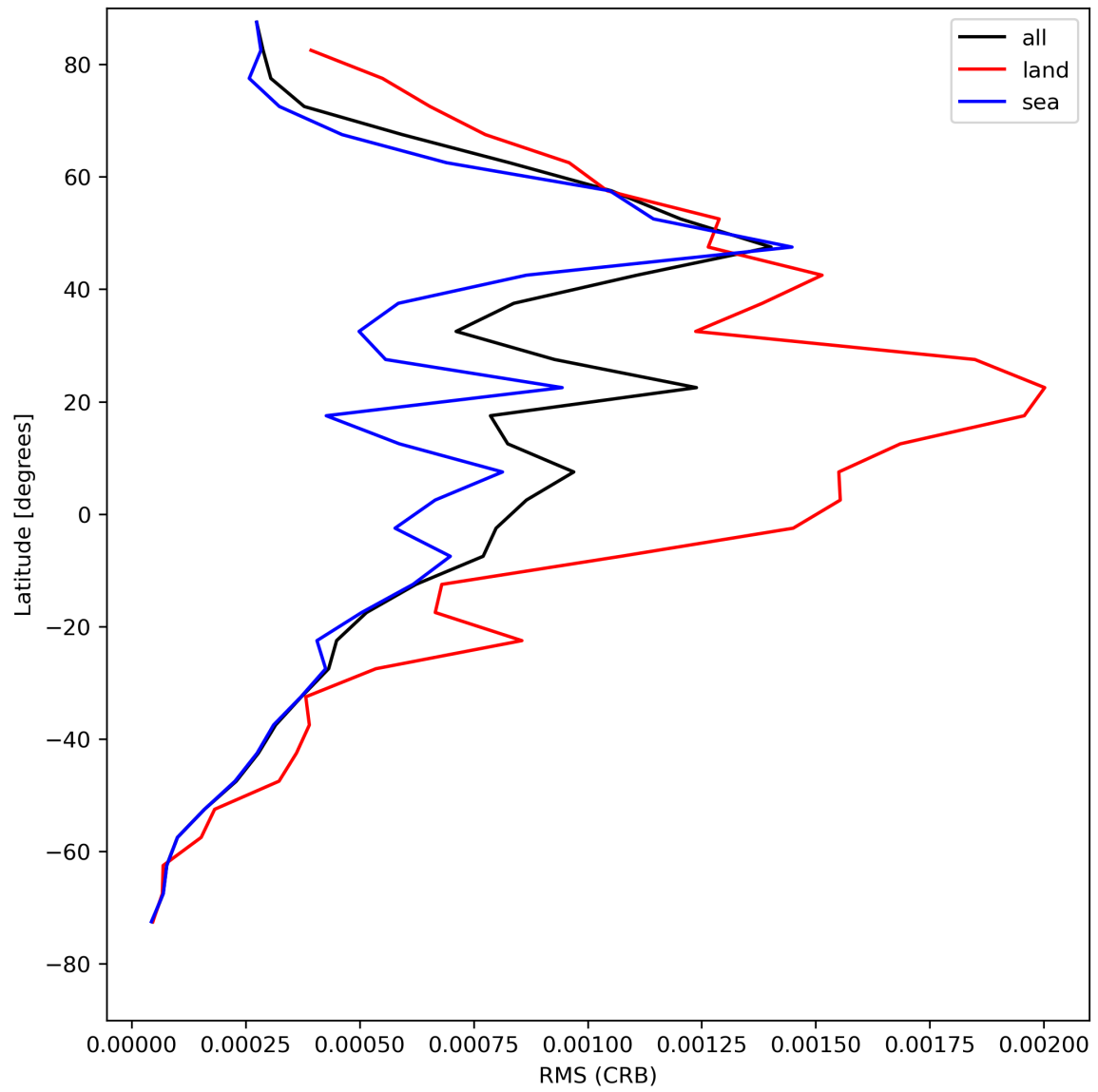
Figure 32: Zonal average of “RMS (CRB)” for 2024-08-09 to 2024-08-11.
