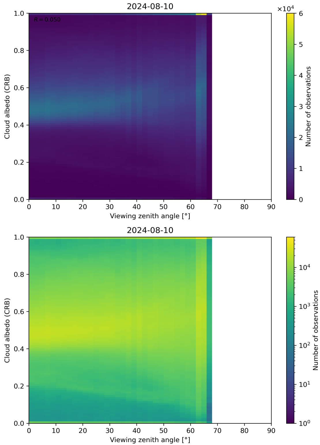
Figure 106: Scatter density plot of “Viewing zenith angle” against “Cloud albedo (CRB)” for 2024-08-09 to 2024-08-11.
