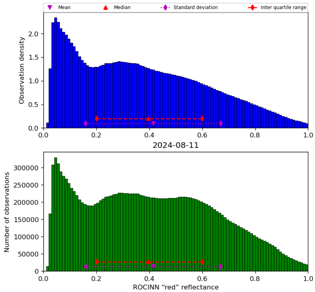
Figure 53: Histogram of “ROCINN “red” reflectance” for 2024-08-11 to 2024-08-11
