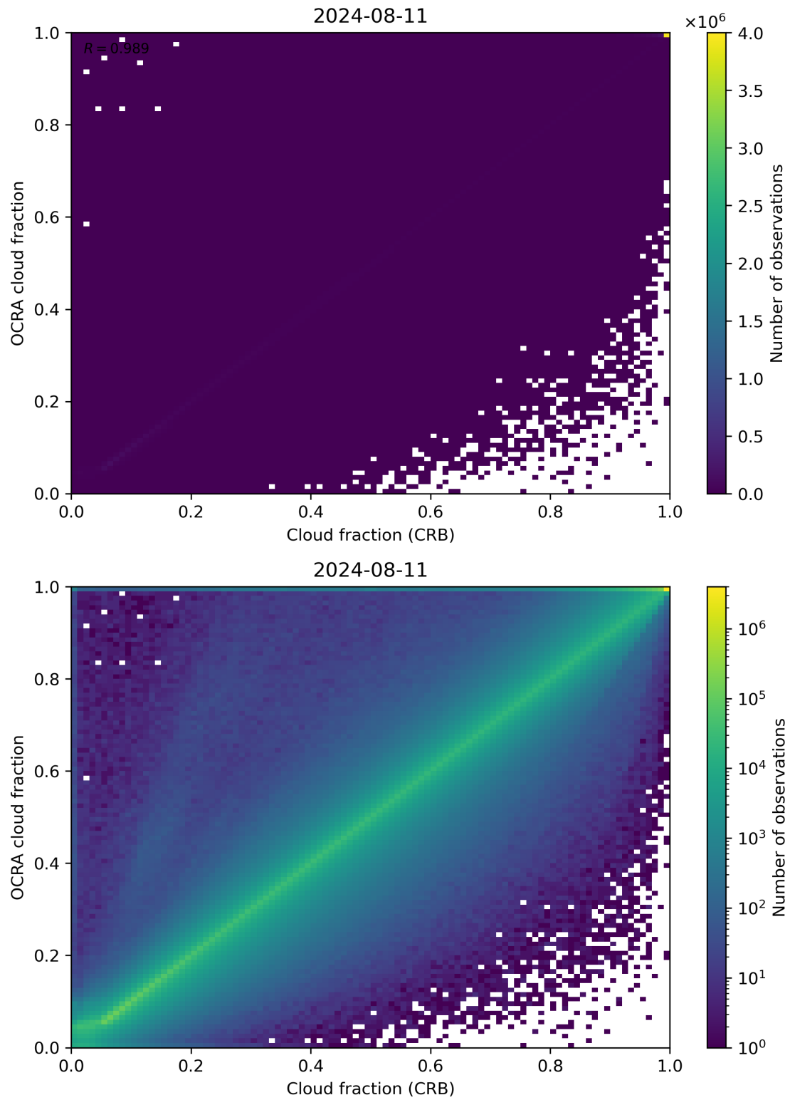
Figure 78: Scatter density plot of “Cloud fraction (CRB)” against “OCRA cloud fraction” for 2024-08-11 to 2024-08-11.
