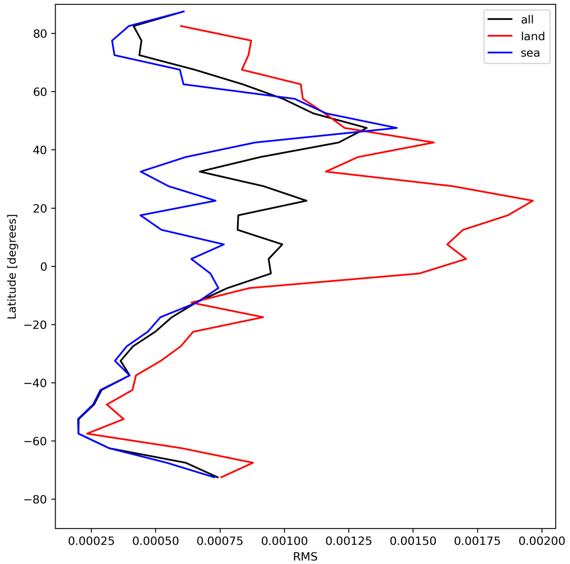
Figure 31: Zonal average of “RMS” for 2024-08-11 to 2024-08-11.
