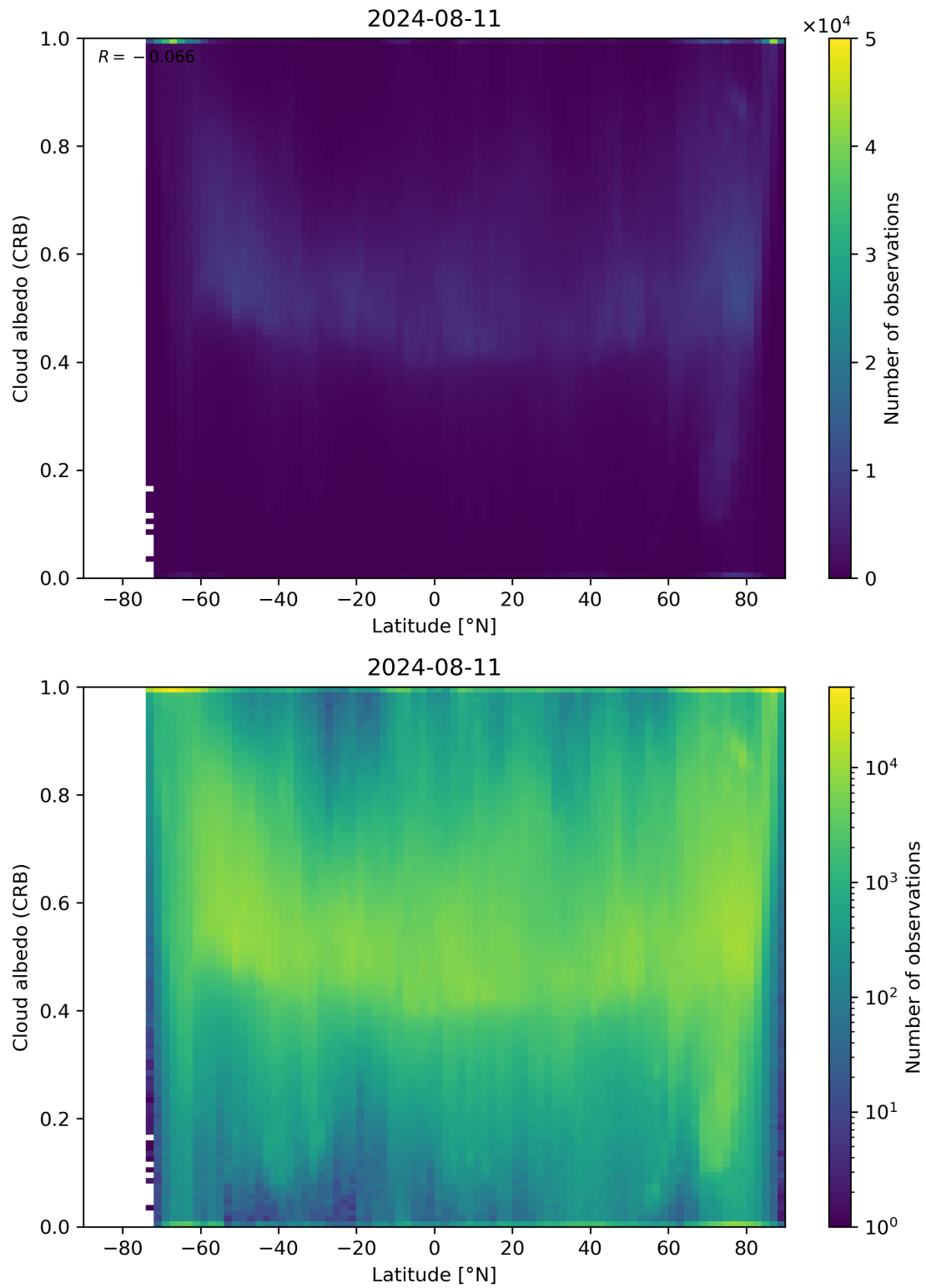
Figure 91: Scatter density plot of “Latitude” against “Cloud albedo (CRB)” for 2024-08-11 to 2024-08-11.
