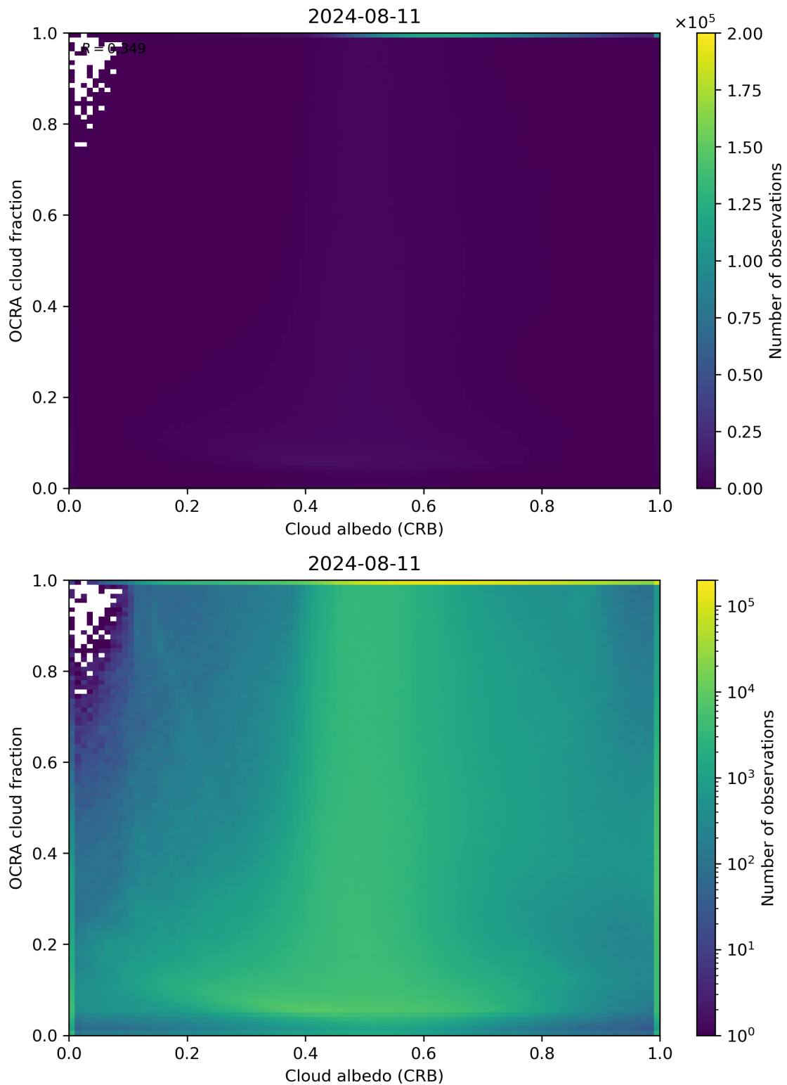
Figure 70: Scatter density plot of “Cloud albedo (CRB)” against “OCRA cloud fraction” for 2024-08-11 to 2024-08-11.
