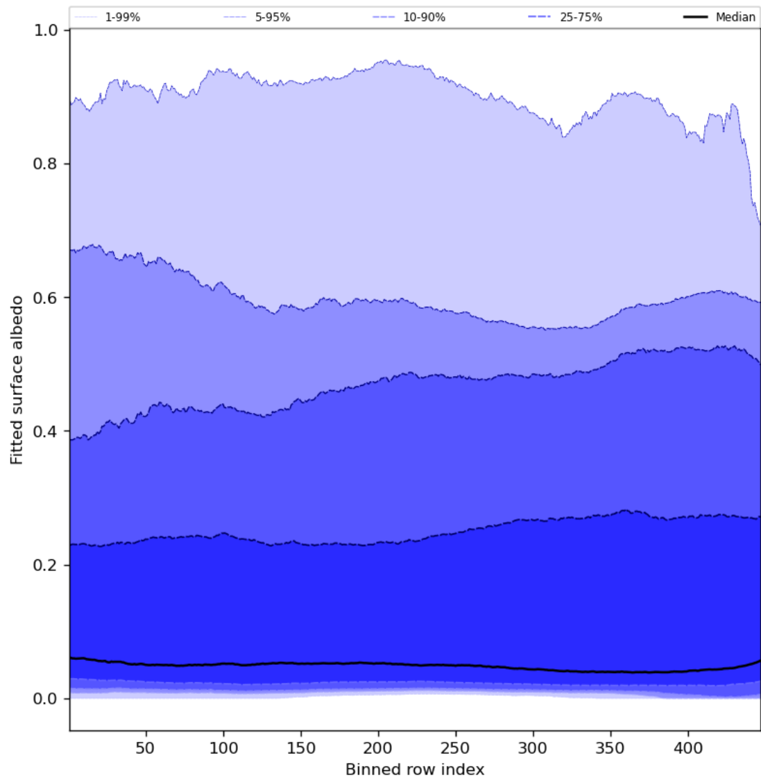
Figure 61: Along track statistics of “Fitted surface albedo” for 2024-08-11 to 2024-08-11
