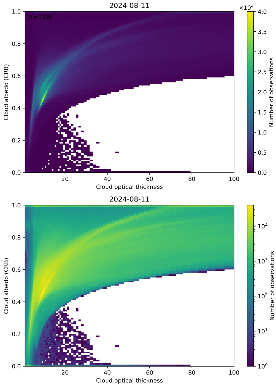
Figure 82: Scatter density plot of “Cloud optical thickness” against “Cloud albedo (CRB)” for 2024-08-11 to 2024-08-11.
