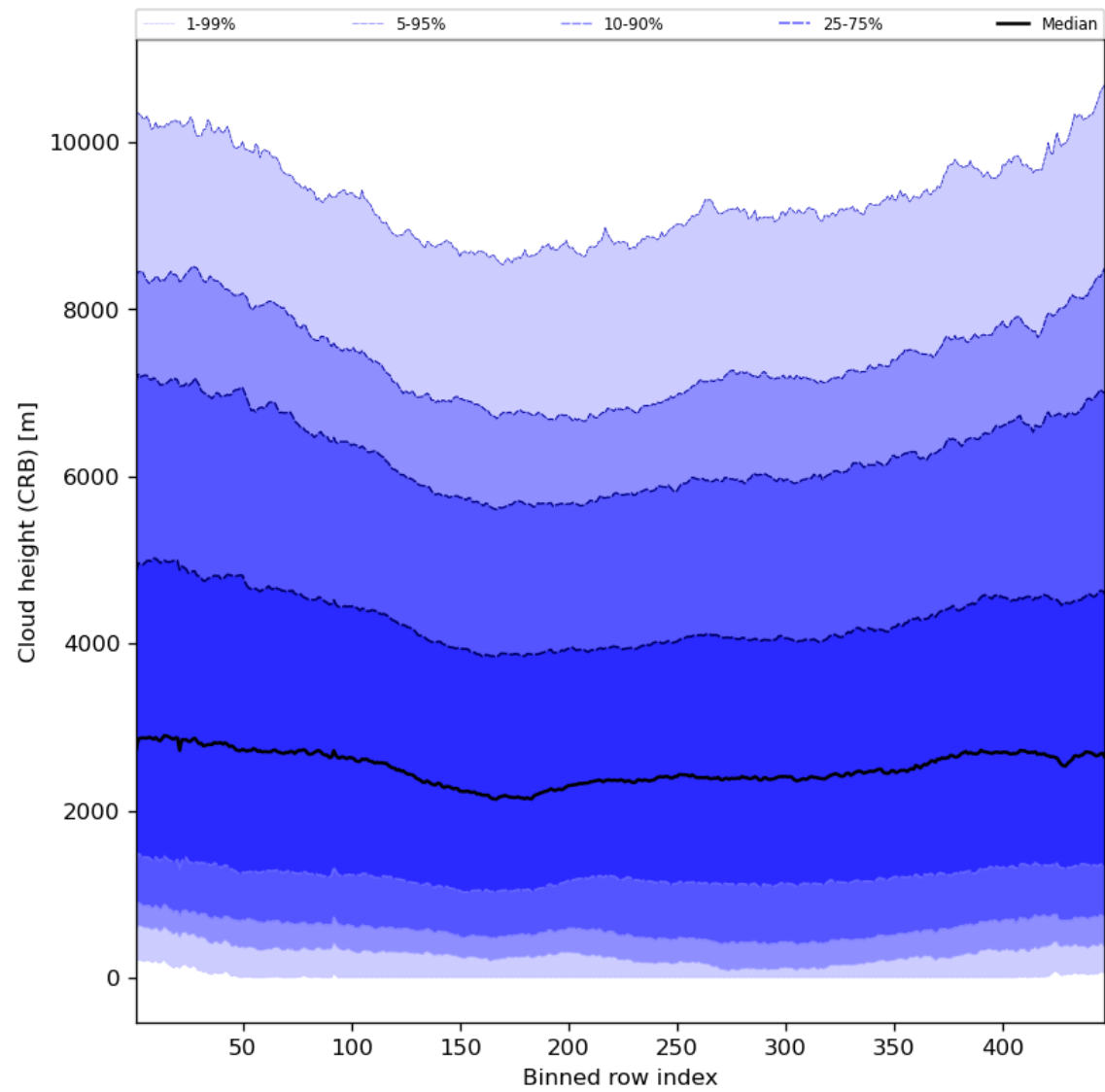
Figure 59: Along track statistics of “Cloud height (CRB)” for 2024-08-11 to 2024-08-11
