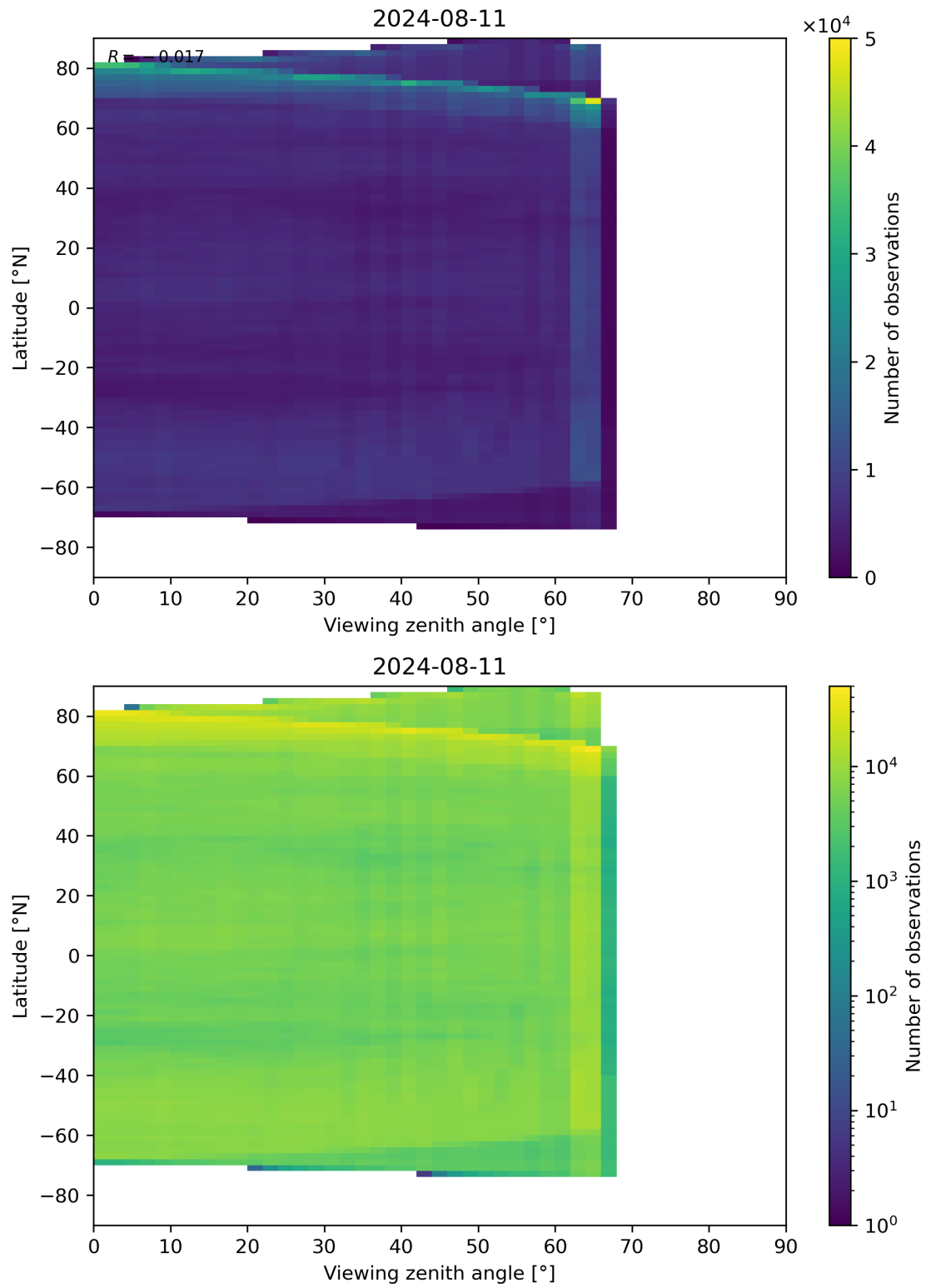
Figure 113: Scatter density plot of “Viewing zenith angle” against “Latitude” for 2024-08-11 to 2024-08-11.
