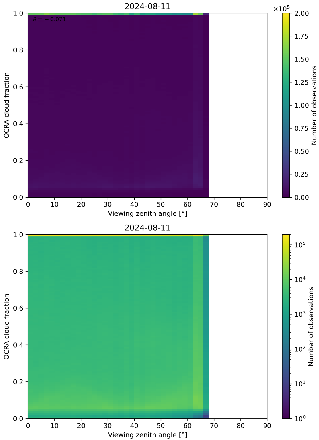
Figure 108: Scatter density plot of “Viewing zenith angle” against “OCRA cloud fraction” for 2024-08-11 to 2024-08-11.
