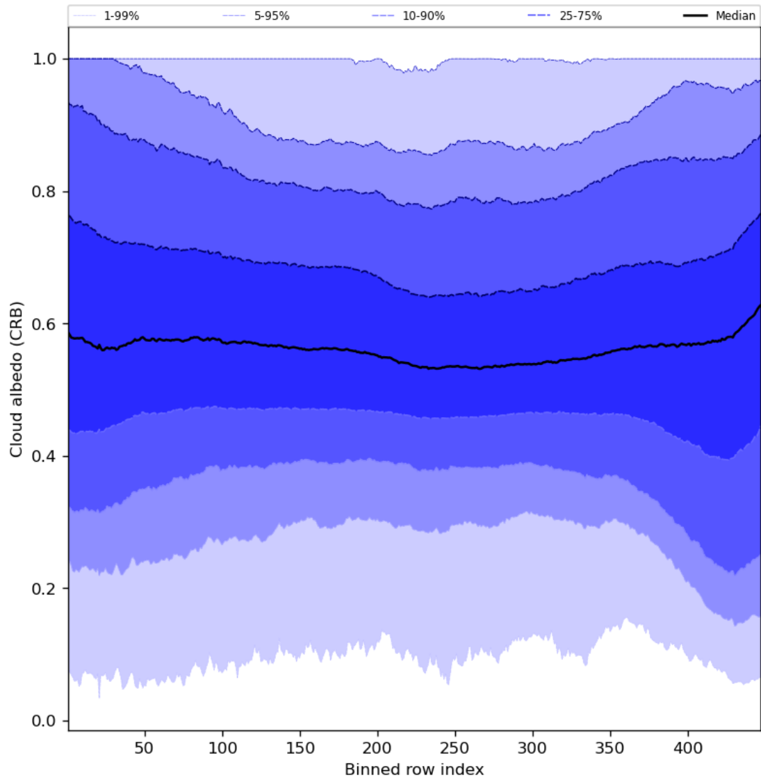
Figure 60: Along track statistics of “Cloud albedo (CRB)” for 2024-08-11 to 2024-08-11
