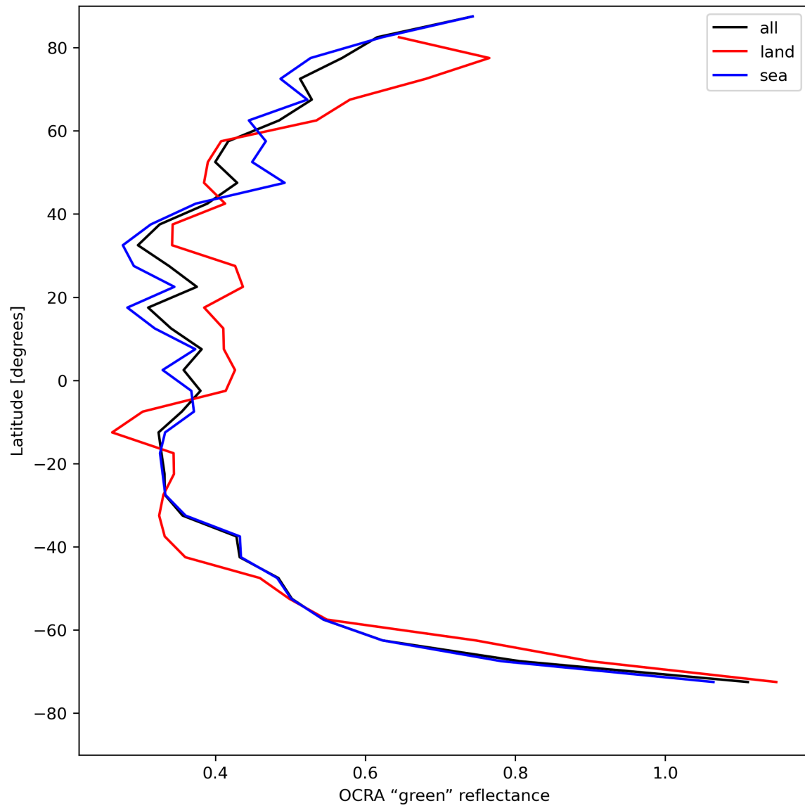
Figure 36: Zonal average of “OCRA “green” reflectance” for 2024-08-11 to 2024-08-11.
