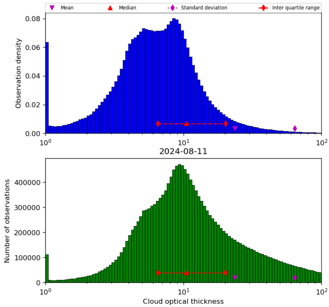
Figure 41: Histogram of “Cloud optical thickness” for 2024-08-11 to 2024-08-11
