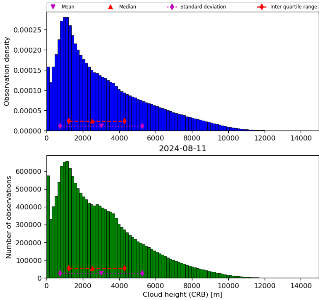
Figure 43: Histogram of “Cloud height (CRB)” for 2024-08-11 to 2024-08-11
