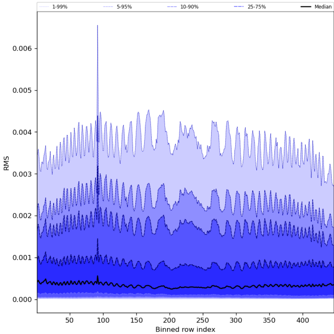
Figure 63: Along track statistics of “RMS” for 2024-08-11 to 2024-08-11
