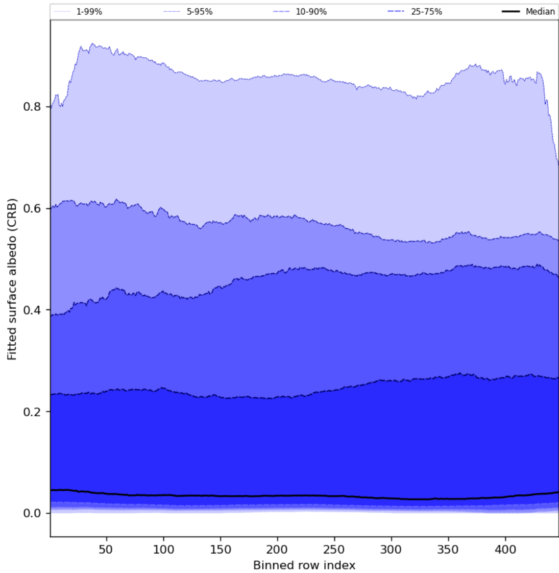
Figure 62: Along track statistics of “Fitted surface albedo (CRB)” for 2024-08-11 to 2024-08-11
