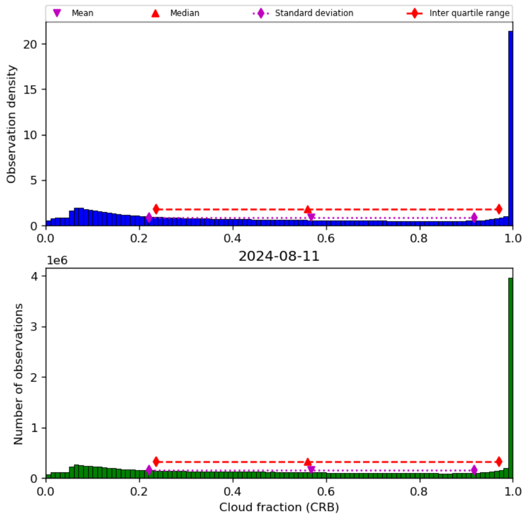
Figure 42: Histogram of “Cloud fraction (CRB)” for 2024-08-11 to 2024-08-11
