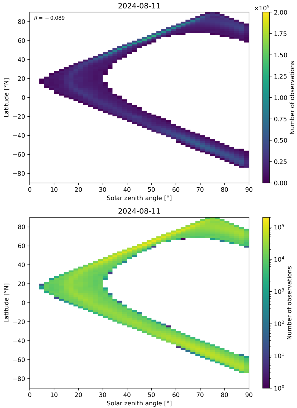
Figure 105: Scatter density plot of “Solar zenith angle” against “Latitude” for 2024-08-11 to 2024-08-11.
