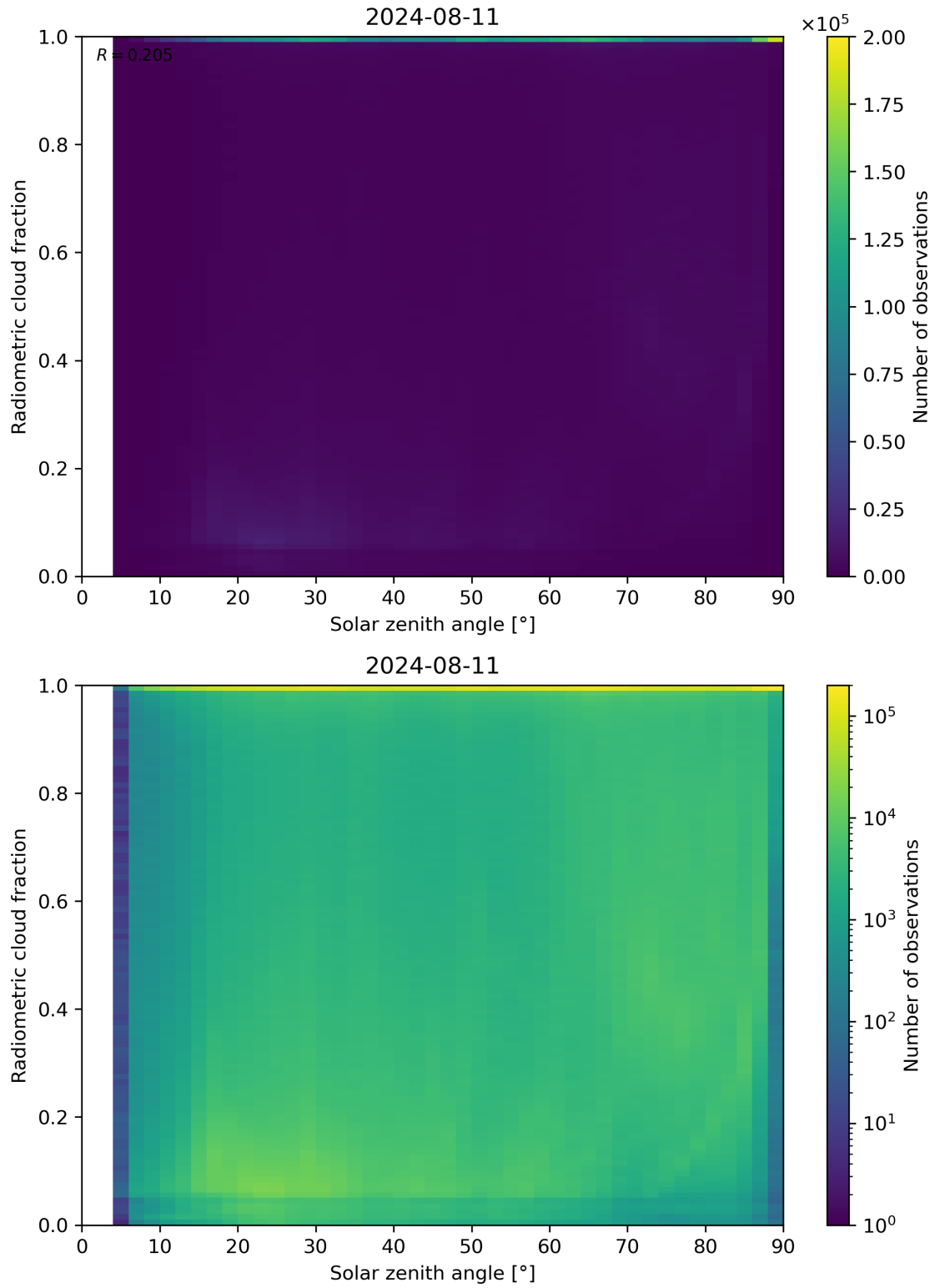
Figure 99: Scatter density plot of “Solar zenith angle” against “Radiometric cloud fraction” for 2024-08-11 to 2024-08-11.
