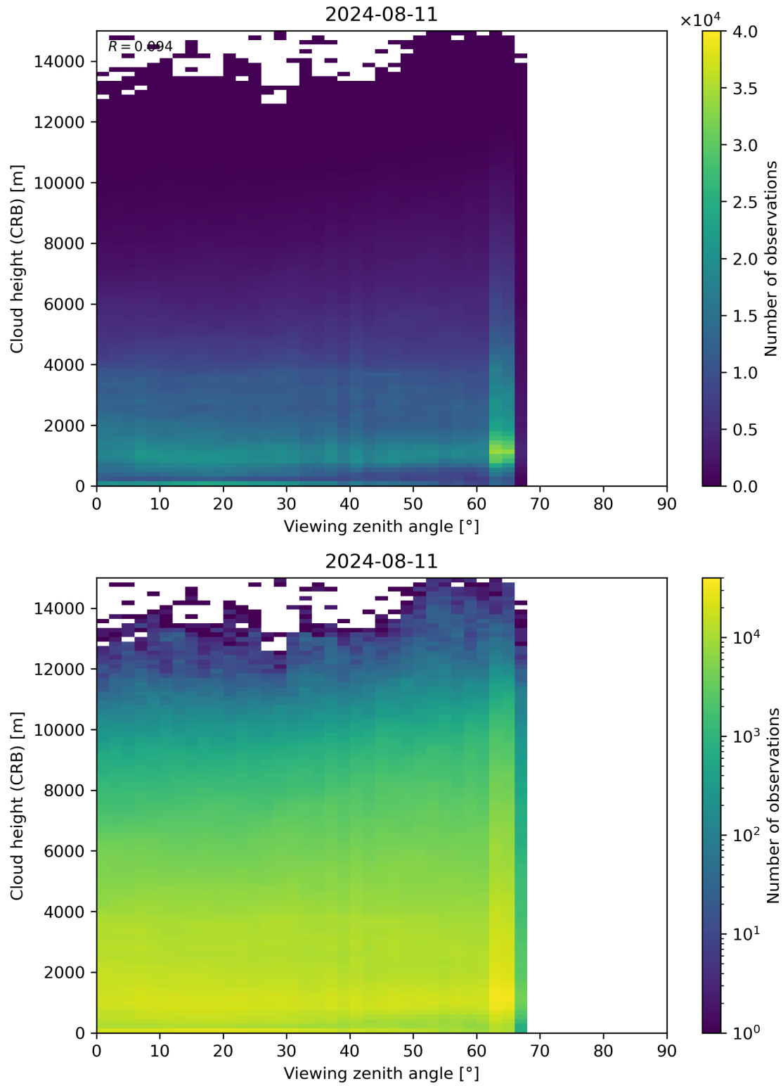
Figure 110: Scatter density plot of “Viewing zenith angle” against “Cloud height (CRB)” for 2024-08-11 to 2024-08-11.
