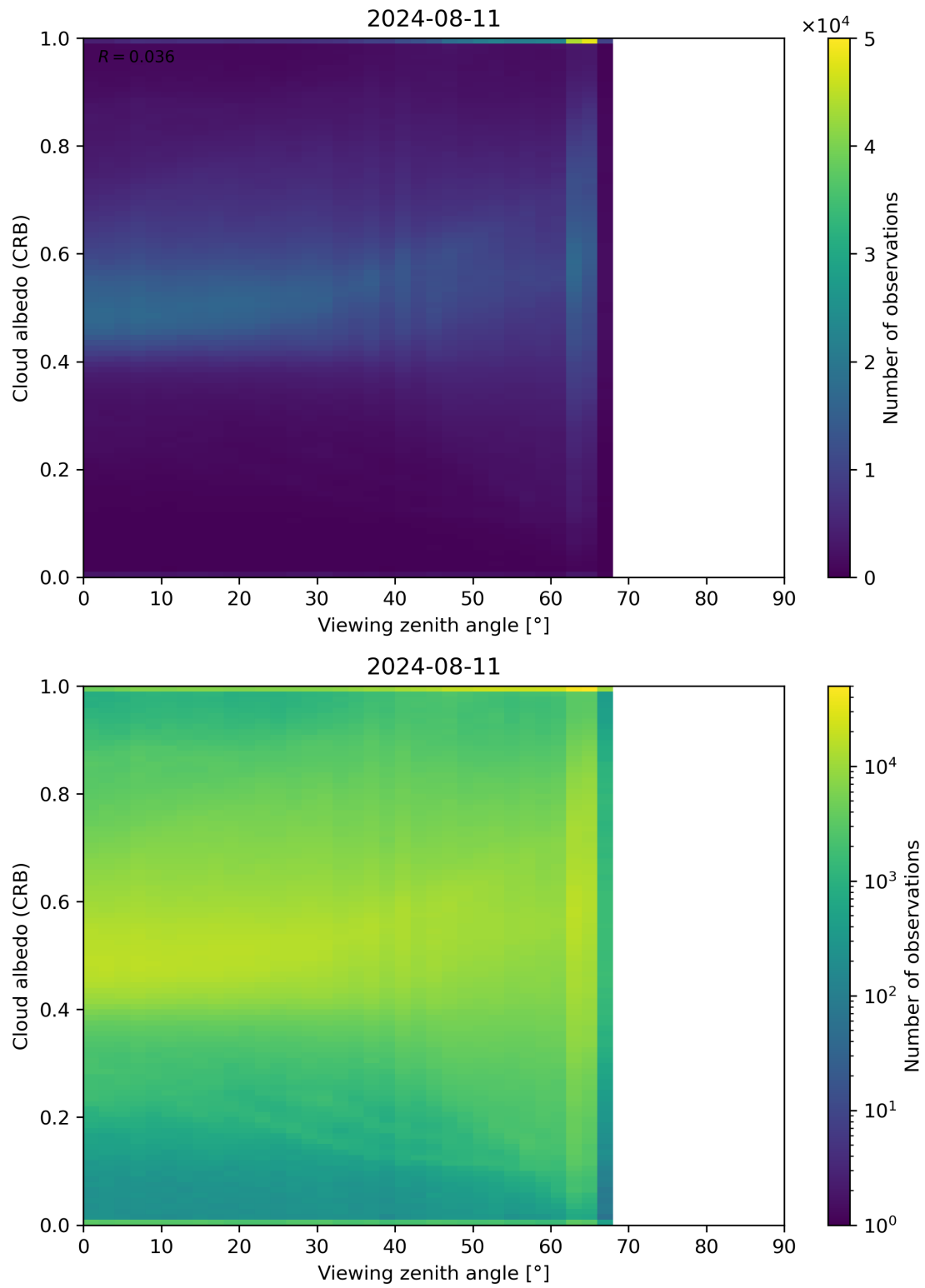
Figure 106: Scatter density plot of “Viewing zenith angle” against “Cloud albedo (CRB)” for 2024-08-11 to 2024-08-11.
