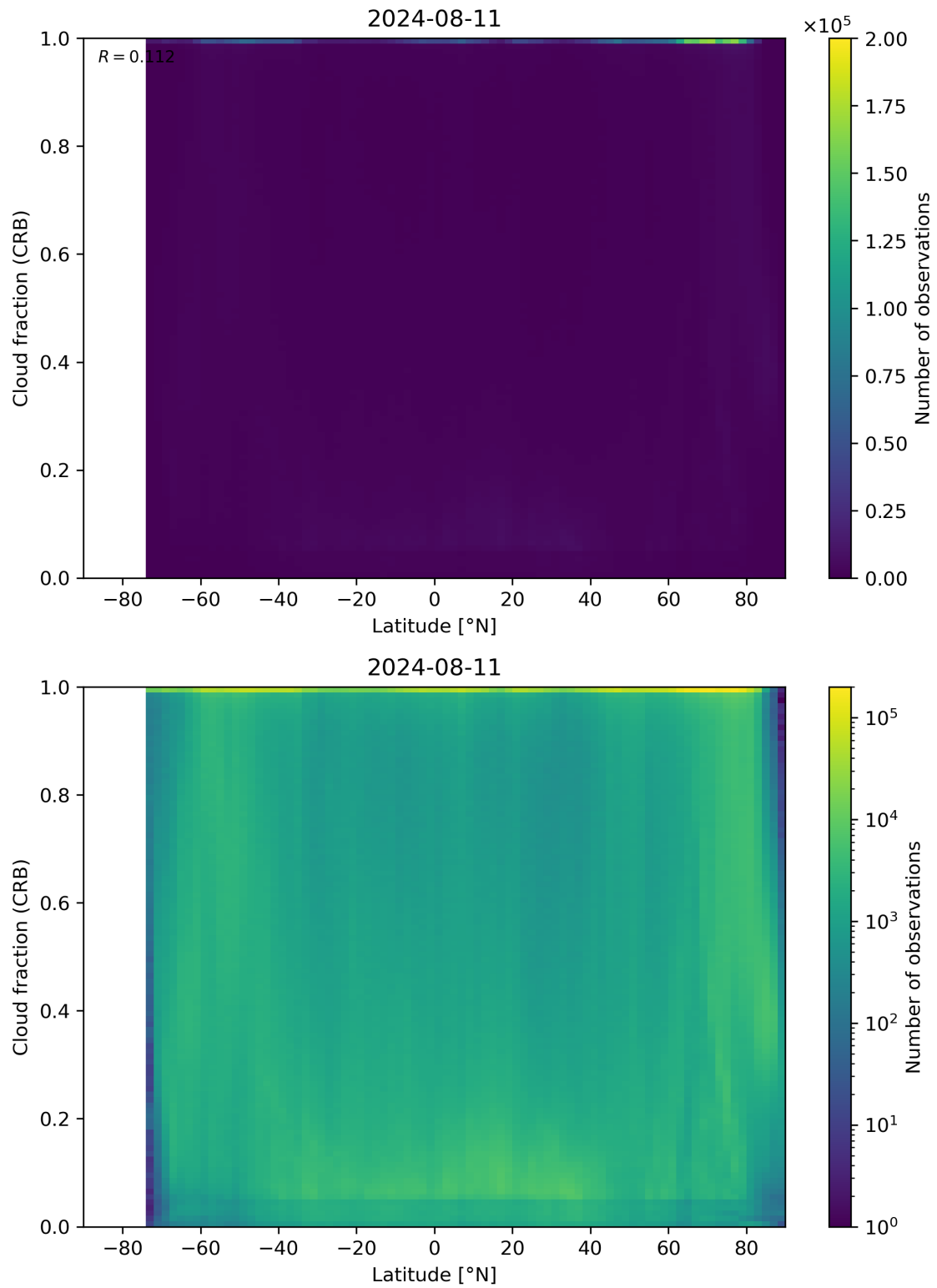
Figure 94: Scatter density plot of “Latitude” against “Cloud fraction (CRB)” for 2024-08-11 to 2024-08-11.
