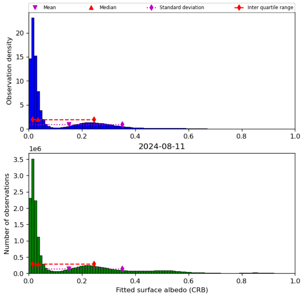
Figure 46: Histogram of “Fitted surface albedo (CRB)” for 2024-08-11 to 2024-08-11
