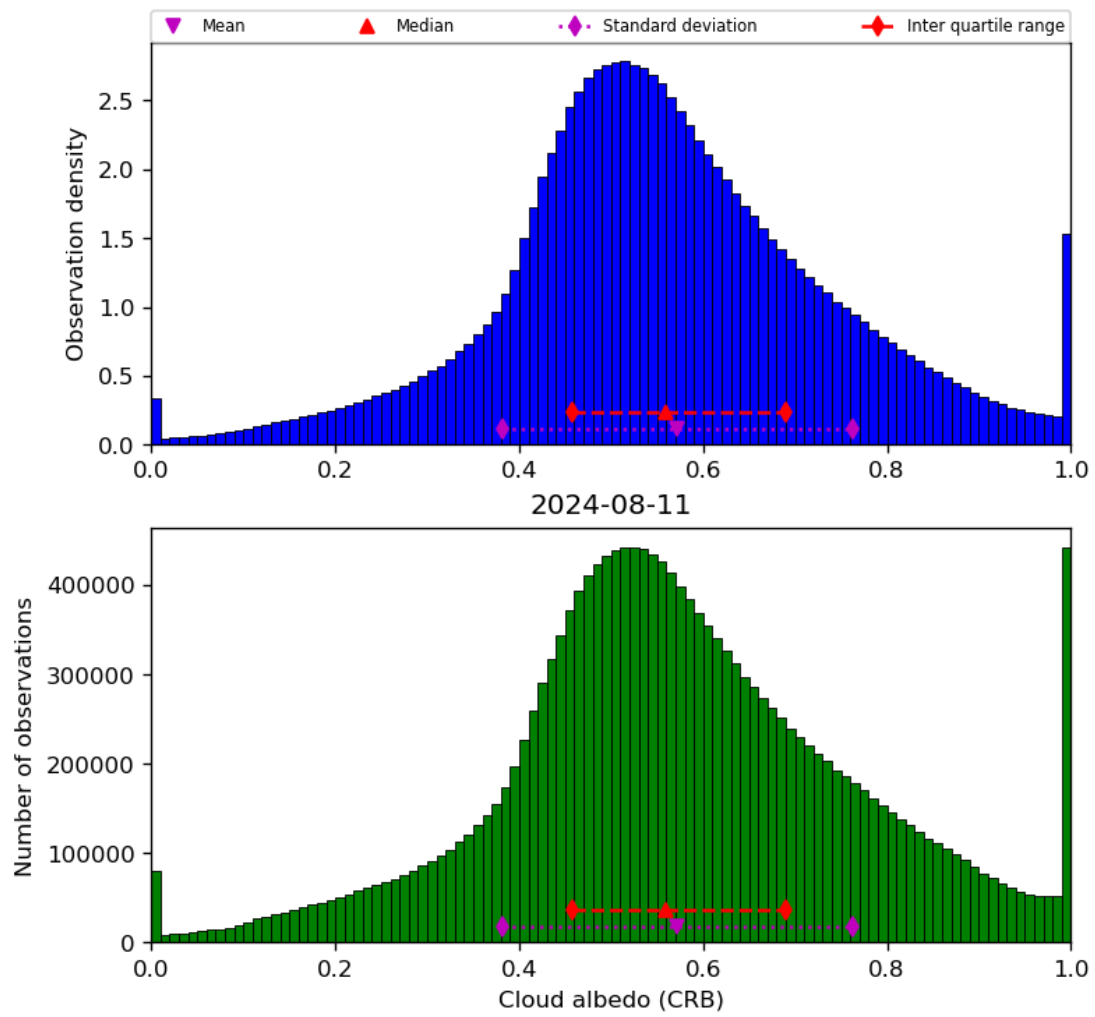
Figure 44: Histogram of “Cloud albedo (CRB)” for 2024-08-11 to 2024-08-11
