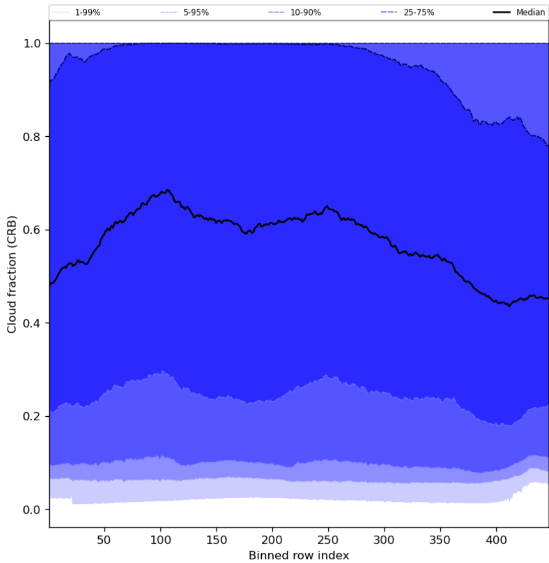
Figure 58: Along track statistics of “Cloud fraction (CRB)” for 2024-08-11 to 2024-08-11
