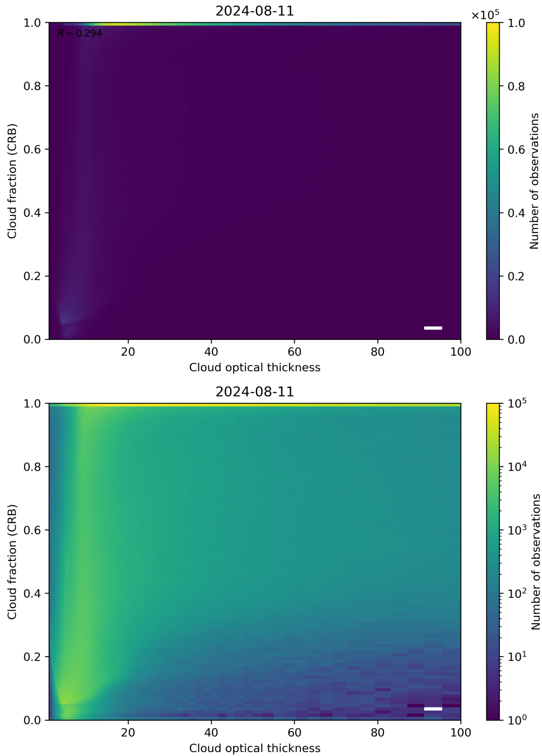
Figure 84: Scatter density plot of “Cloud optical thickness” against “Cloud fraction (CRB)” for 2024-08-11 to 2024-08-11.
