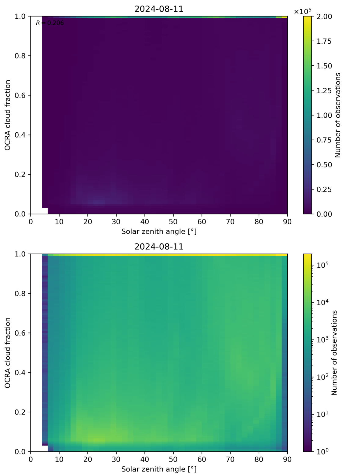
Figure 100: Scatter density plot of “Solar zenith angle” against “OCRA cloud fraction” for 2024-08-11 to 2024-08-11.
