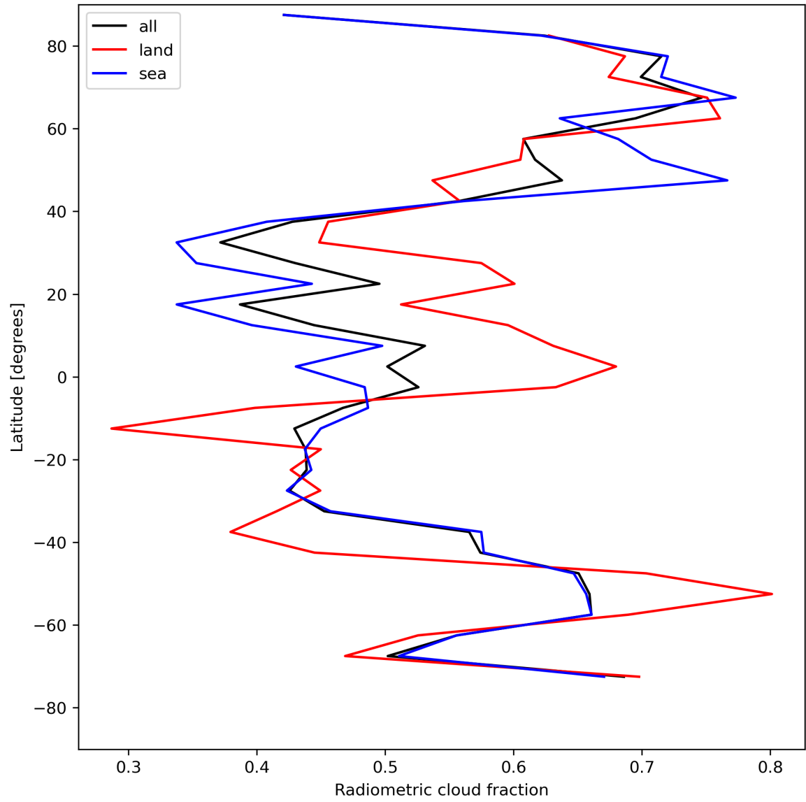
Figure 23: Zonal average of “Radiometric cloud fraction” for 2024-08-11 to 2024-08-11.
