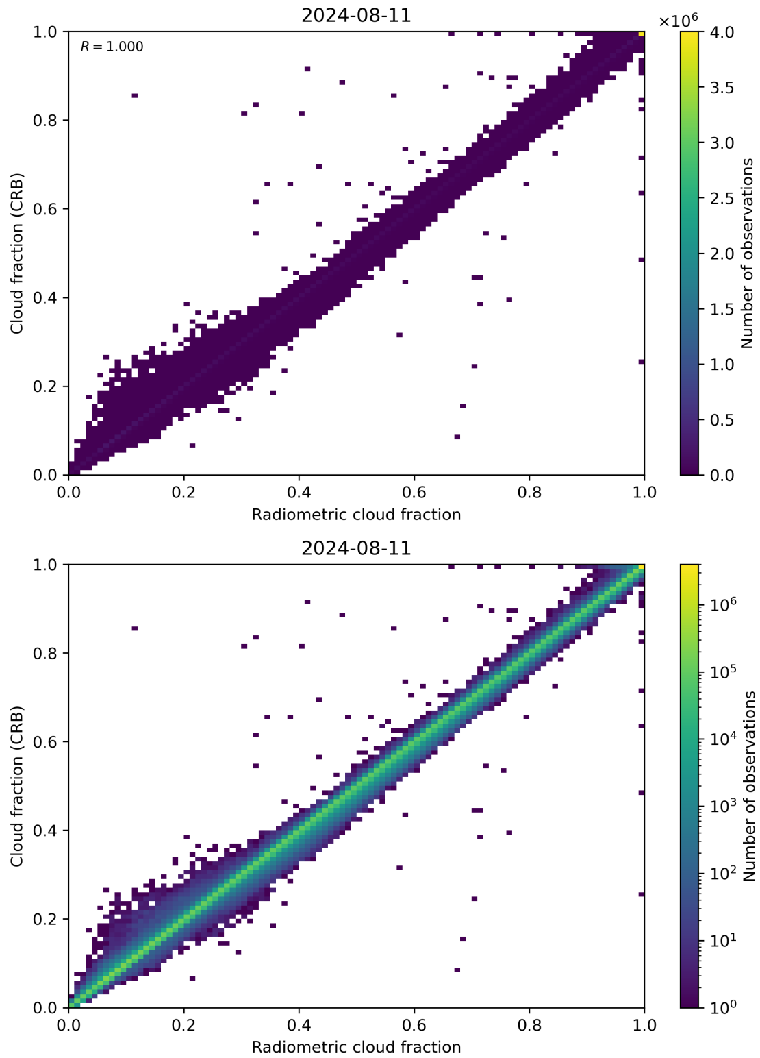
Figure 73: Scatter density plot of “Radiometric cloud fraction” against “Cloud fraction (CRB)” for 2024-08-11 to 2024-08-11.
