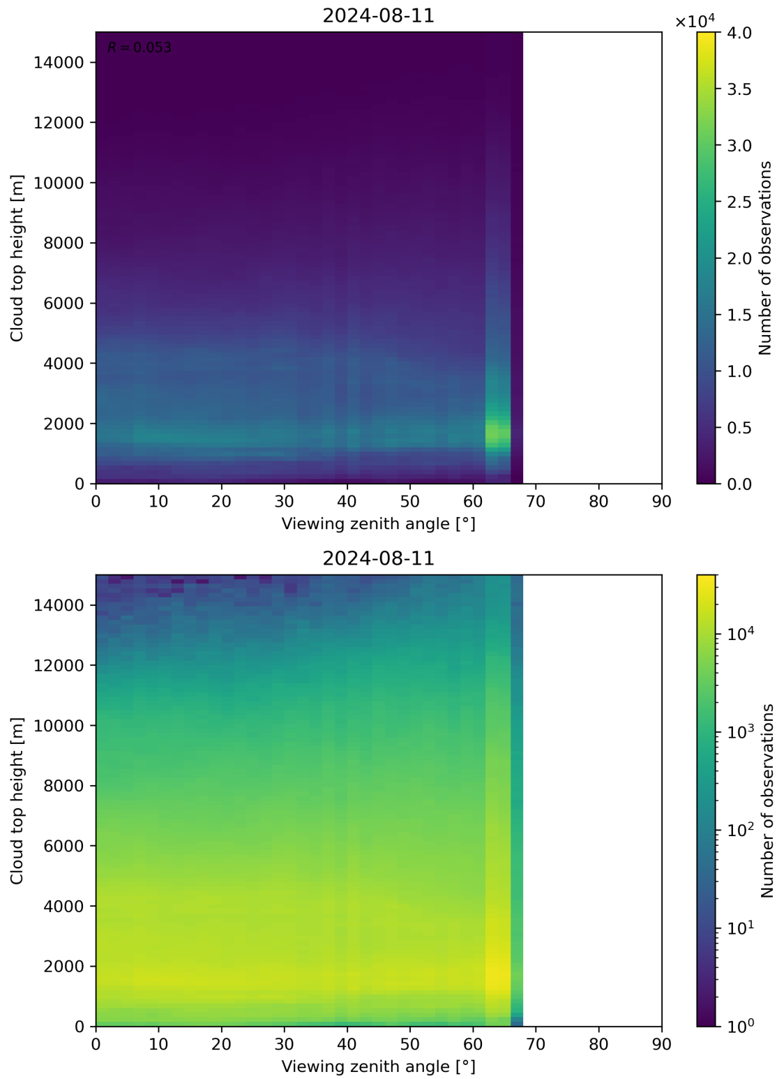
Figure 112: Scatter density plot of “Viewing zenith angle” against “Cloud top height” for 2024-08-11 to 2024-08-11.
