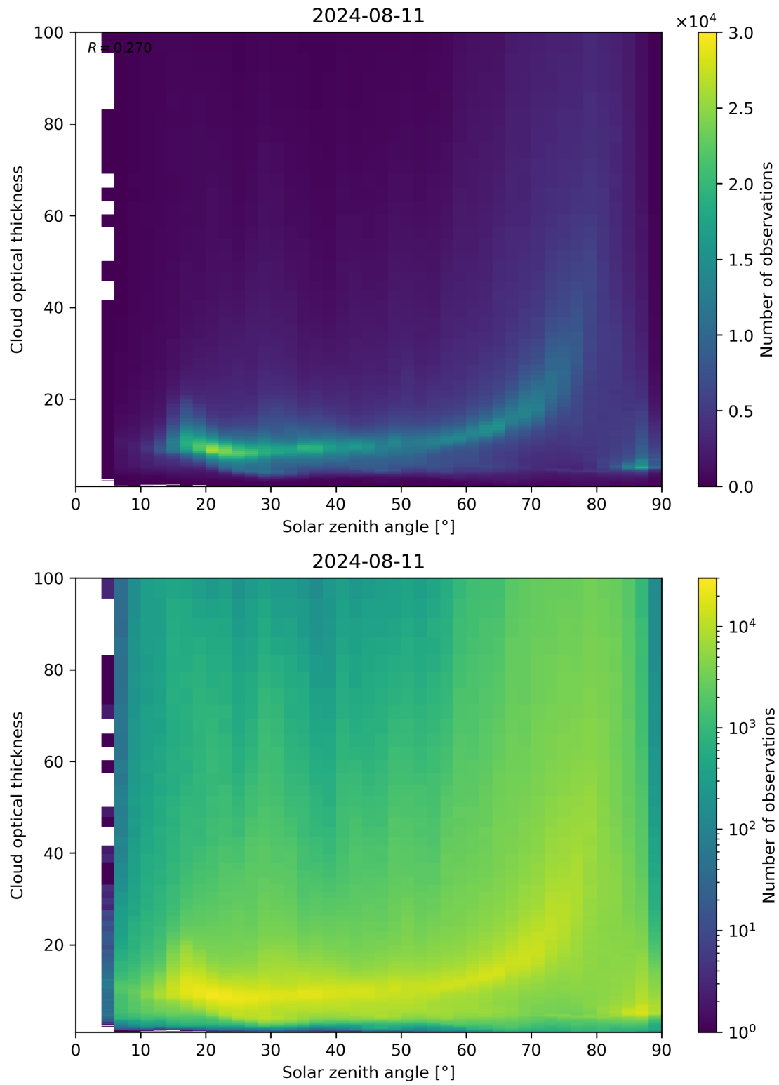
Figure 103: Scatter density plot of “Solar zenith angle” against “Cloud optical thickness” for 2024-08-11 to 2024-08-11.
