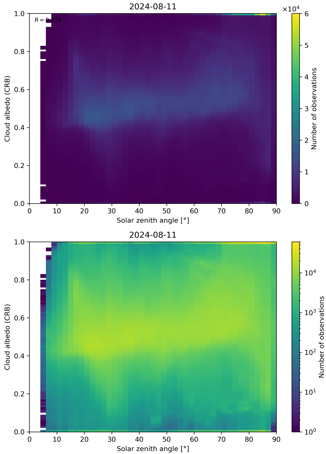
Figure 98: Scatter density plot of “Solar zenith angle” against “Cloud albedo (CRB)” for 2024-08-11 to 2024-08-11.
