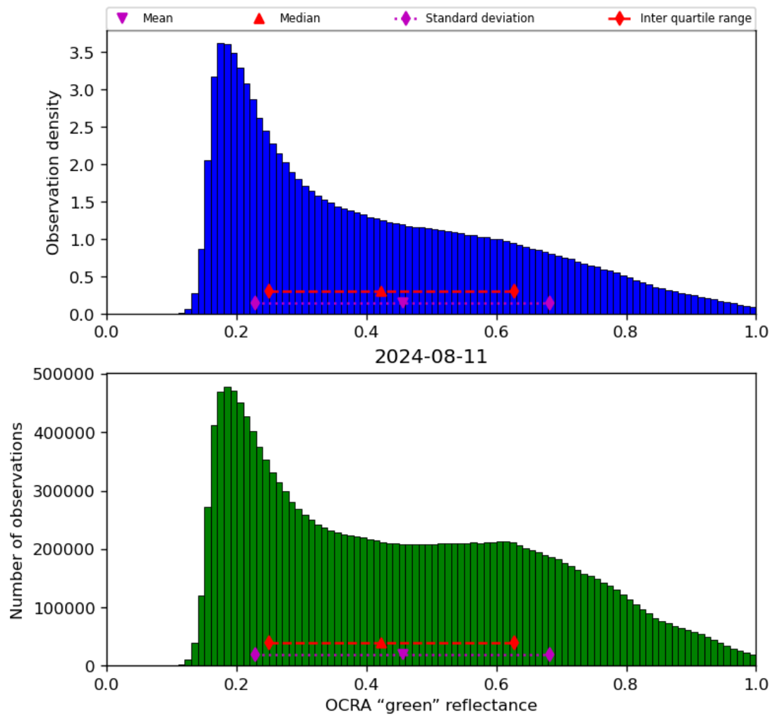
Figure 52: Histogram of “OCRA “green” reflectance” for 2024-08-11 to 2024-08-11
