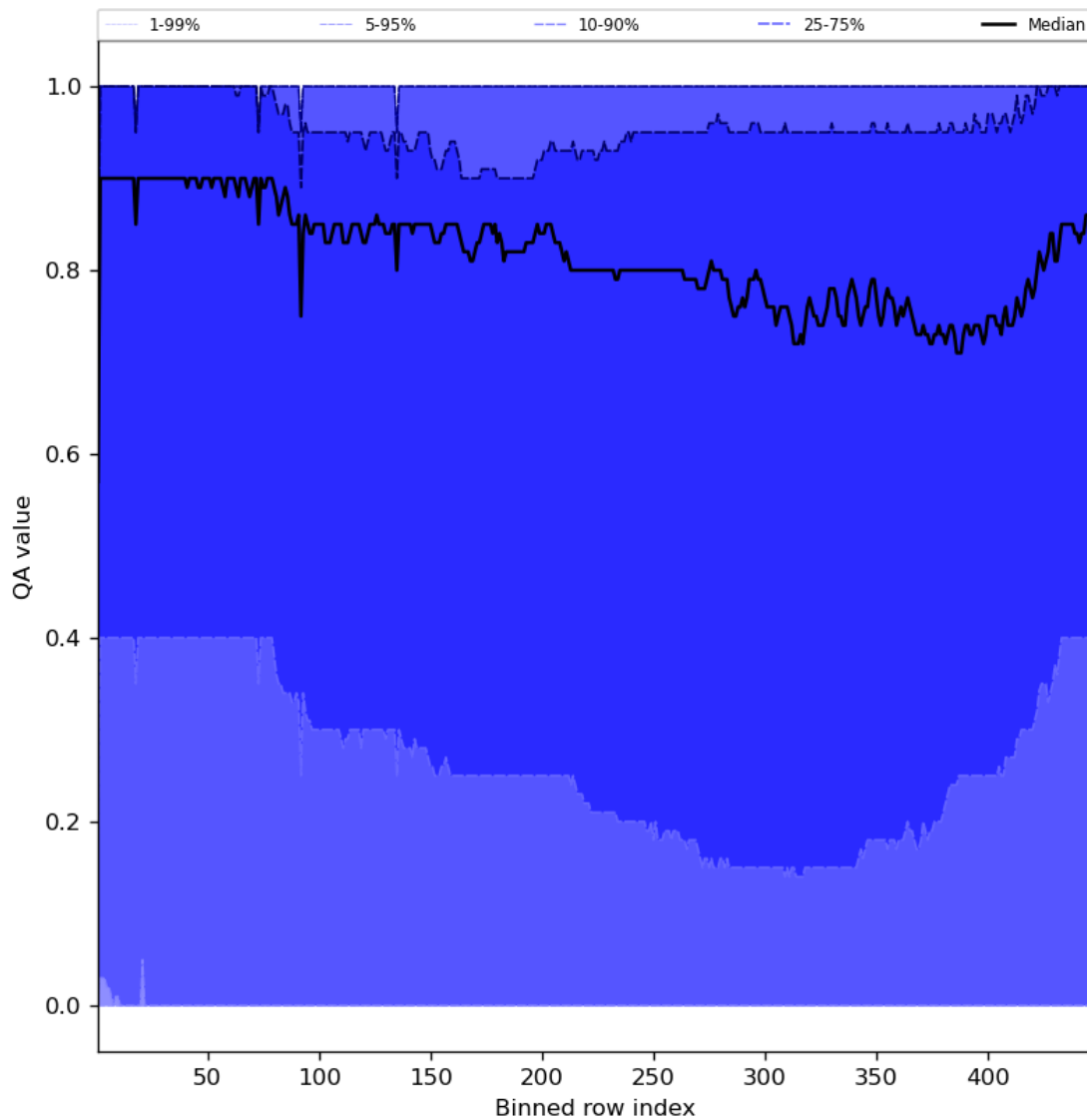
Figure 54: Along track statistics of “QA value” for 2024-08-11 to 2024-08-11
