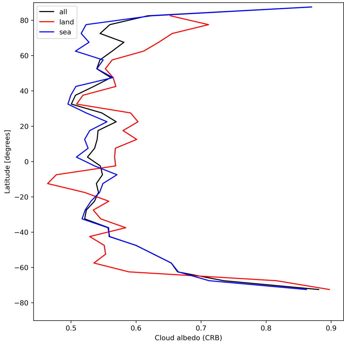
Figure 28: Zonal average of “Cloud albedo (CRB)” for 2024-08-11 to 2024-08-11.
