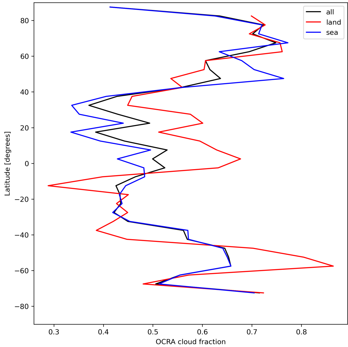
Figure 34: Zonal average of “OCRA cloud fraction” for 2024-08-11 to 2024-08-11.
