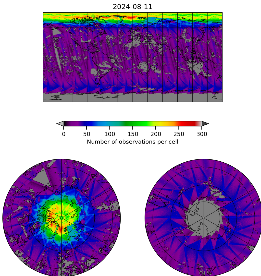
Figure 21: Map of the number of observations for 2024-08-11 to 2024-08-11
