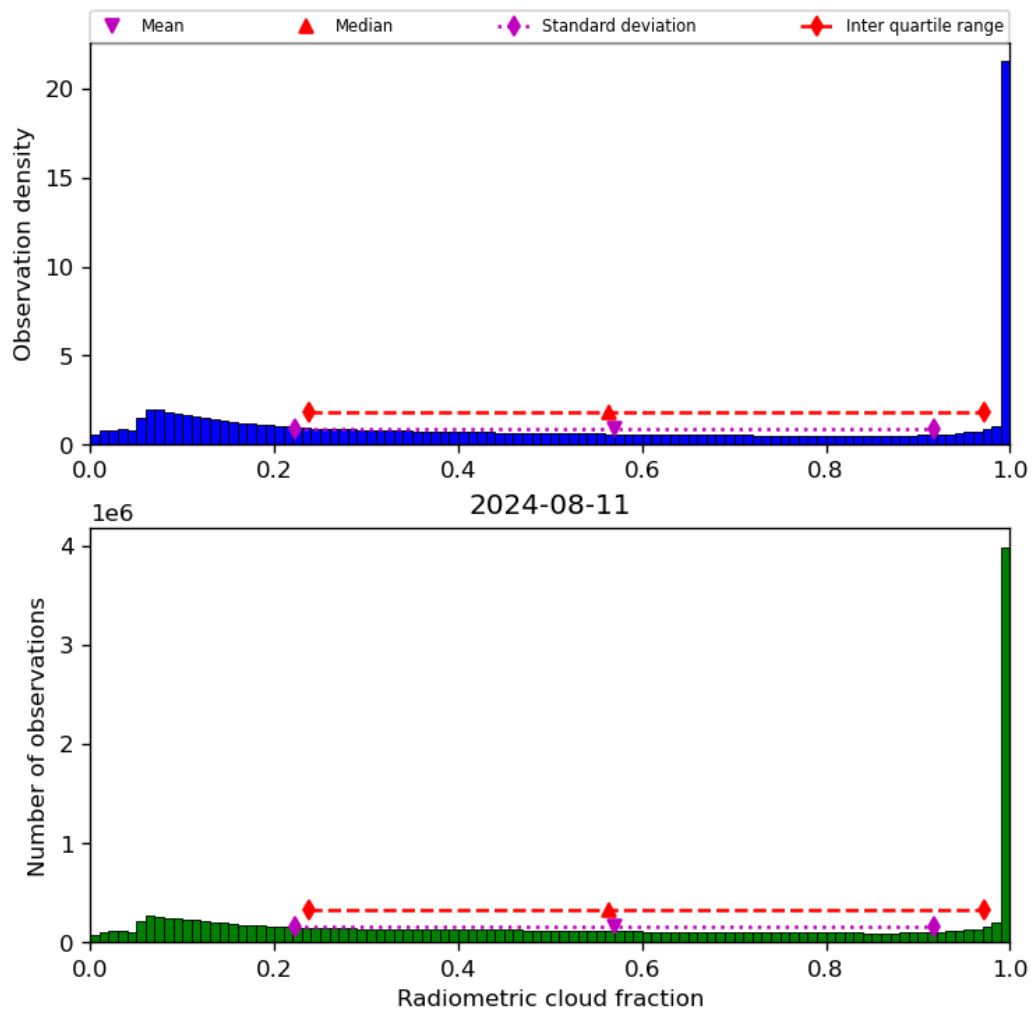
Figure 39: Histogram of “Radiometric cloud fraction” for 2024-08-11 to 2024-08-11
