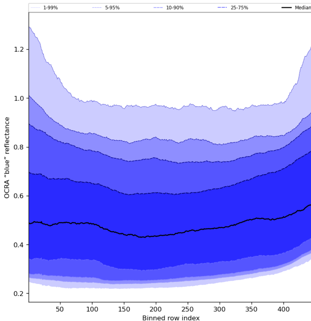
Figure 67: Along track statistics of “OCRA “blue” reflectance” for 2024-08-11 to 2024-08-11
