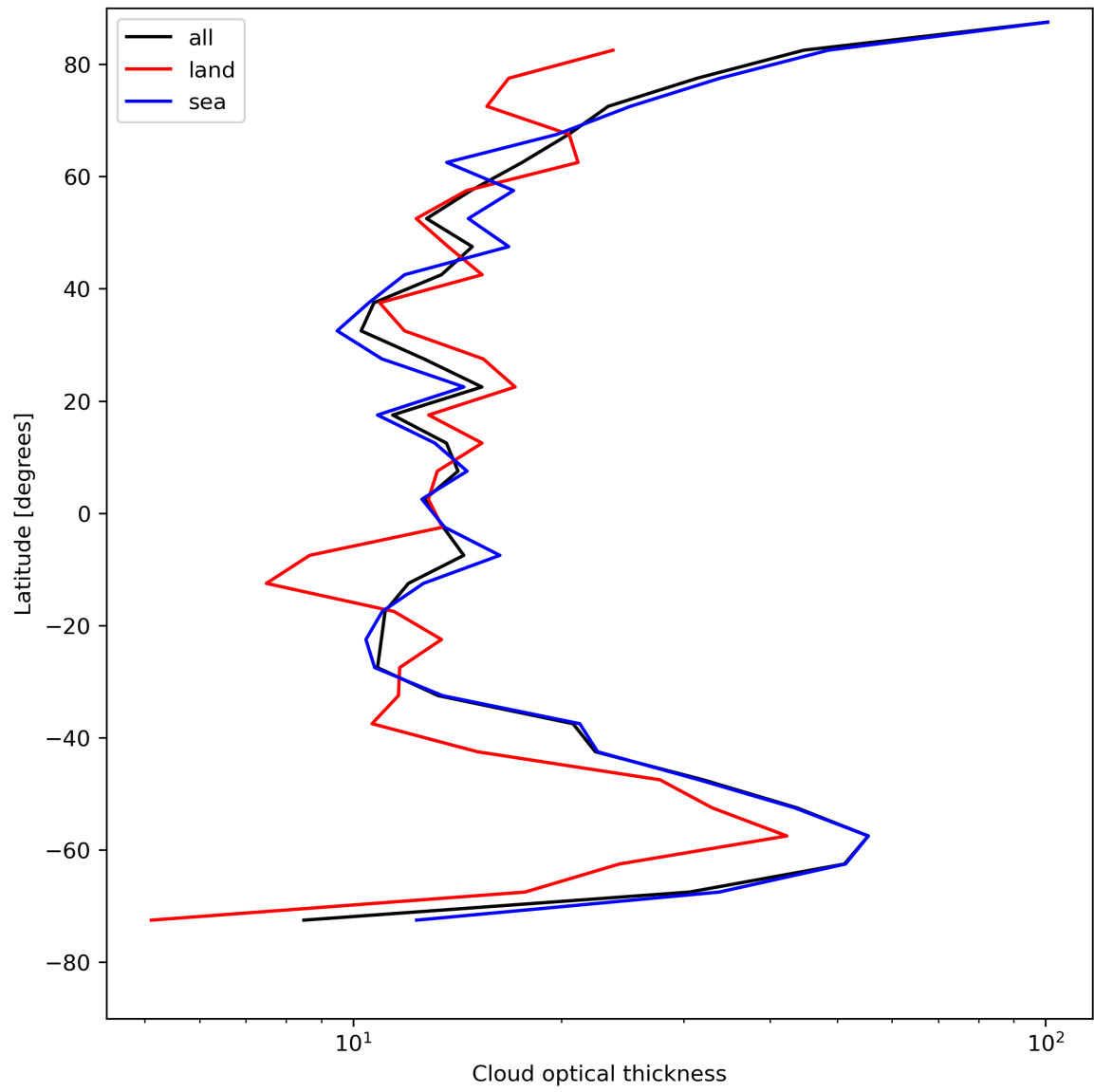
Figure 25: Zonal average of “Cloud optical thickness” for 2024-08-11 to 2024-08-11.
