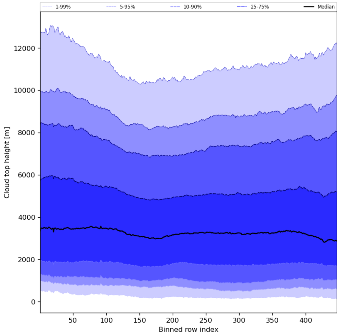
Figure 56: Along track statistics of “Cloud top height” for 2024-08-11 to 2024-08-11
