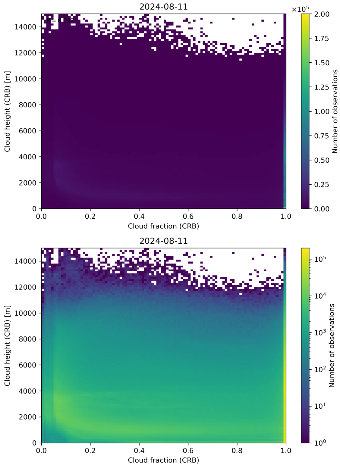
Figure 79: Scatter density plot of “Cloud fraction (CRB)” against “Cloud height (CRB)” for 2024-08-11 to 2024-08-11.
