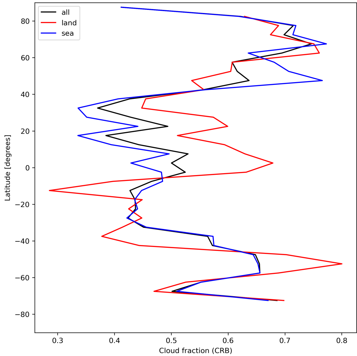
Figure 26: Zonal average of “Cloud fraction (CRB)” for 2024-08-11 to 2024-08-11.
