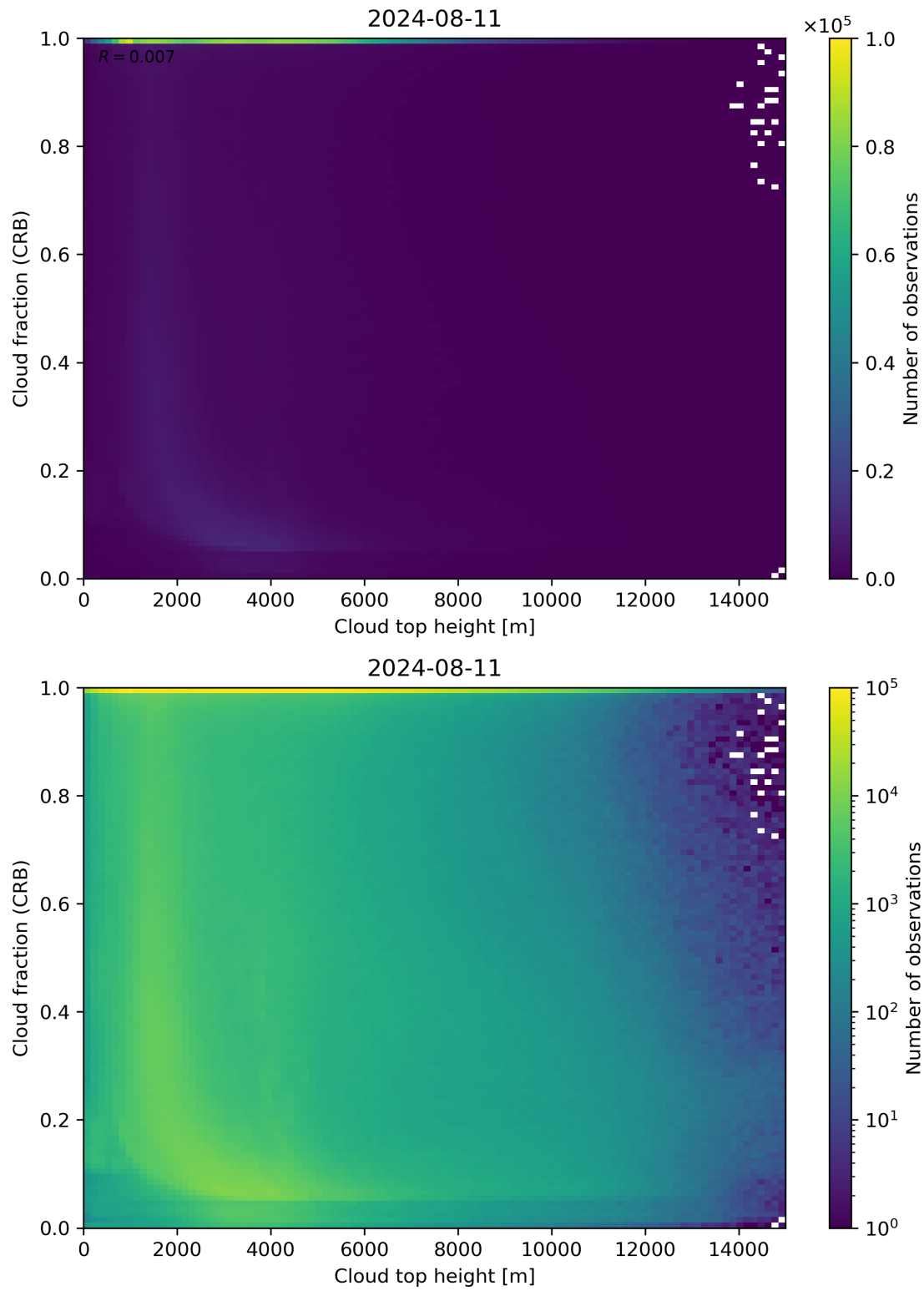
Figure 88: Scatter density plot of “Cloud top height” against “Cloud fraction (CRB)” for 2024-08-11 to 2024-08-11.
