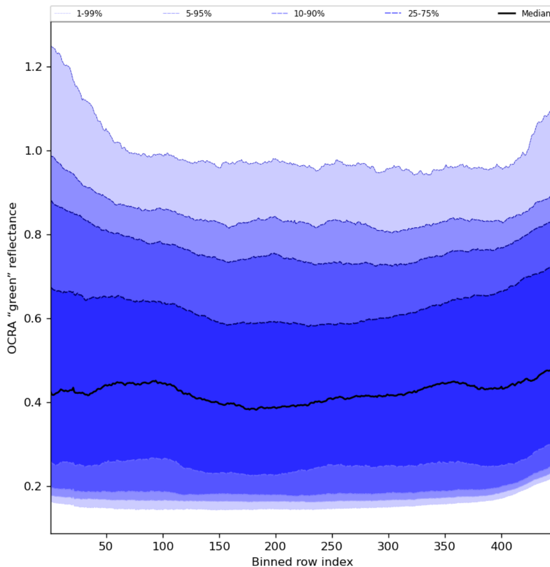
Figure 68: Along track statistics of “OCRA “green” reflectance” for 2024-08-11 to 2024-08-11
