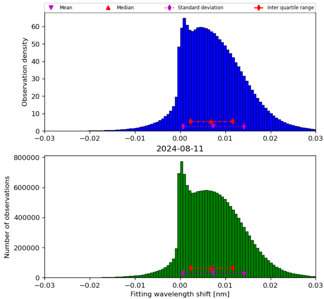
Figure 49: Histogram of “Fitting wavelength shift” for 2024-08-11 to 2024-08-11
