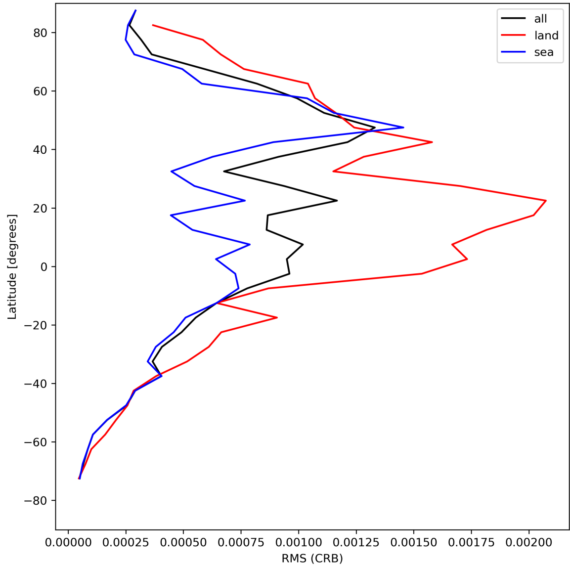
Figure 32: Zonal average of “RMS (CRB)” for 2024-08-11 to 2024-08-11.
