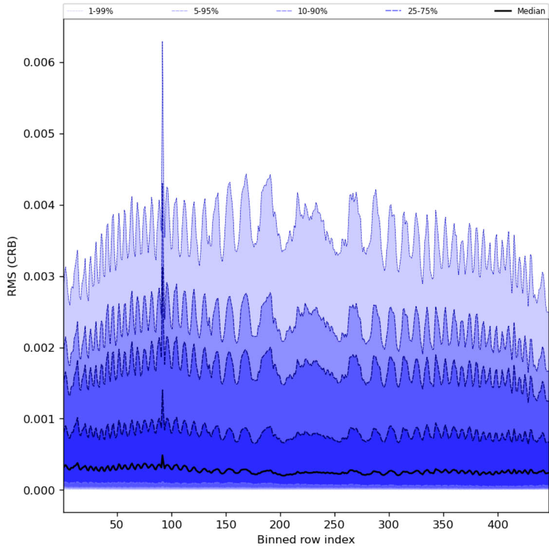
Figure 64: Along track statistics of “RMS (CRB)” for 2024-08-11 to 2024-08-11
