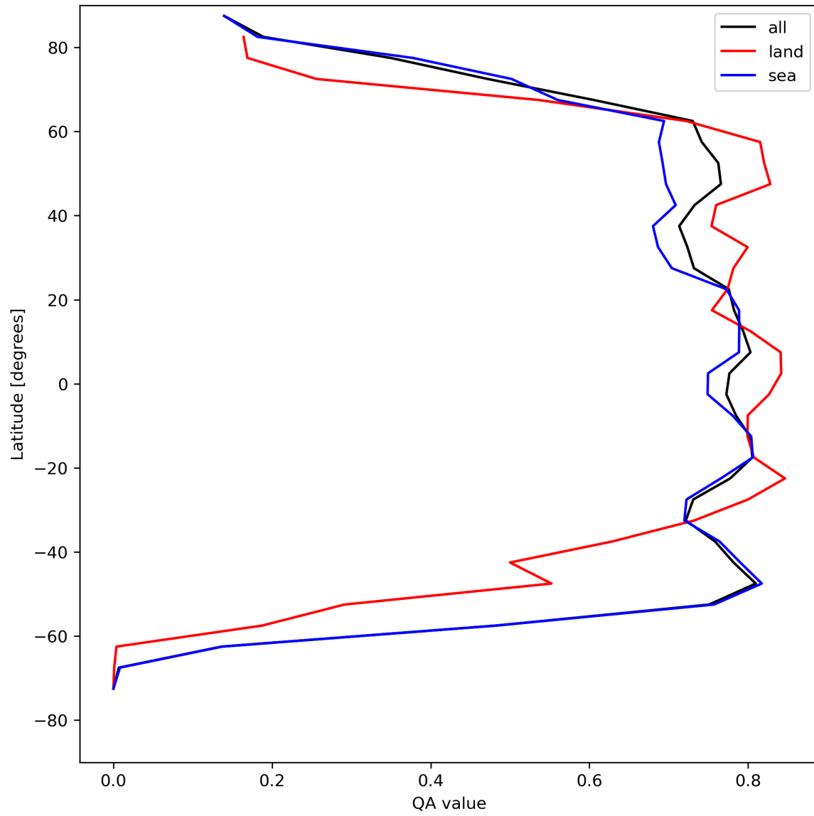
Figure 22: Zonal average of “QA value” for 2024-08-11 to 2024-08-11.
