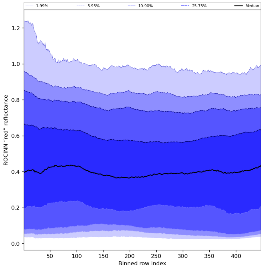
Figure 69: Along track statistics of "ROCINN "red" reflectance" for 2024-08-11 to 2024-08-11
