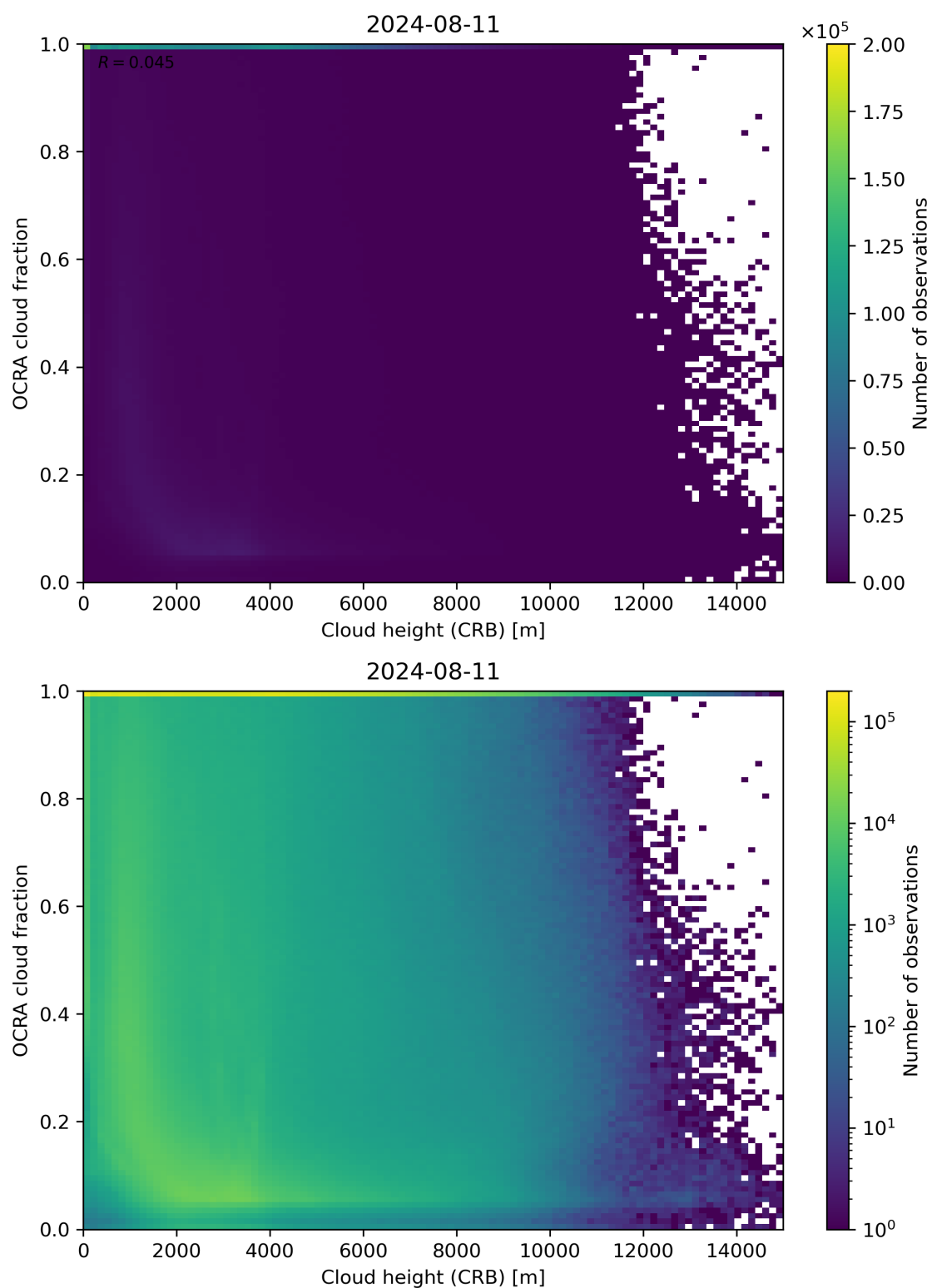
Figure 81: Scatter density plot of “Cloud height (CRB)” against “OCRA cloud fraction” for 2024-08-11 to 2024-08-11.
