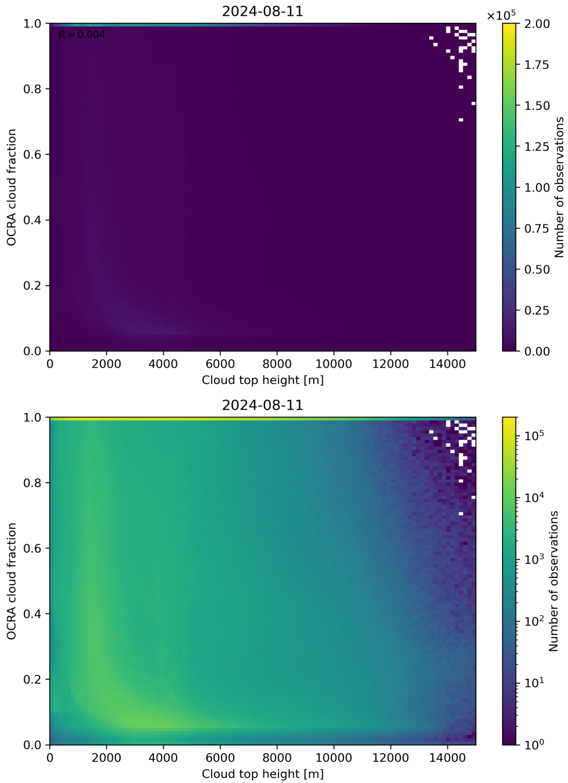
Figure 87: Scatter density plot of “Cloud top height” against “OCRA cloud fraction” for 2024-08-11 to 2024-08-11.
