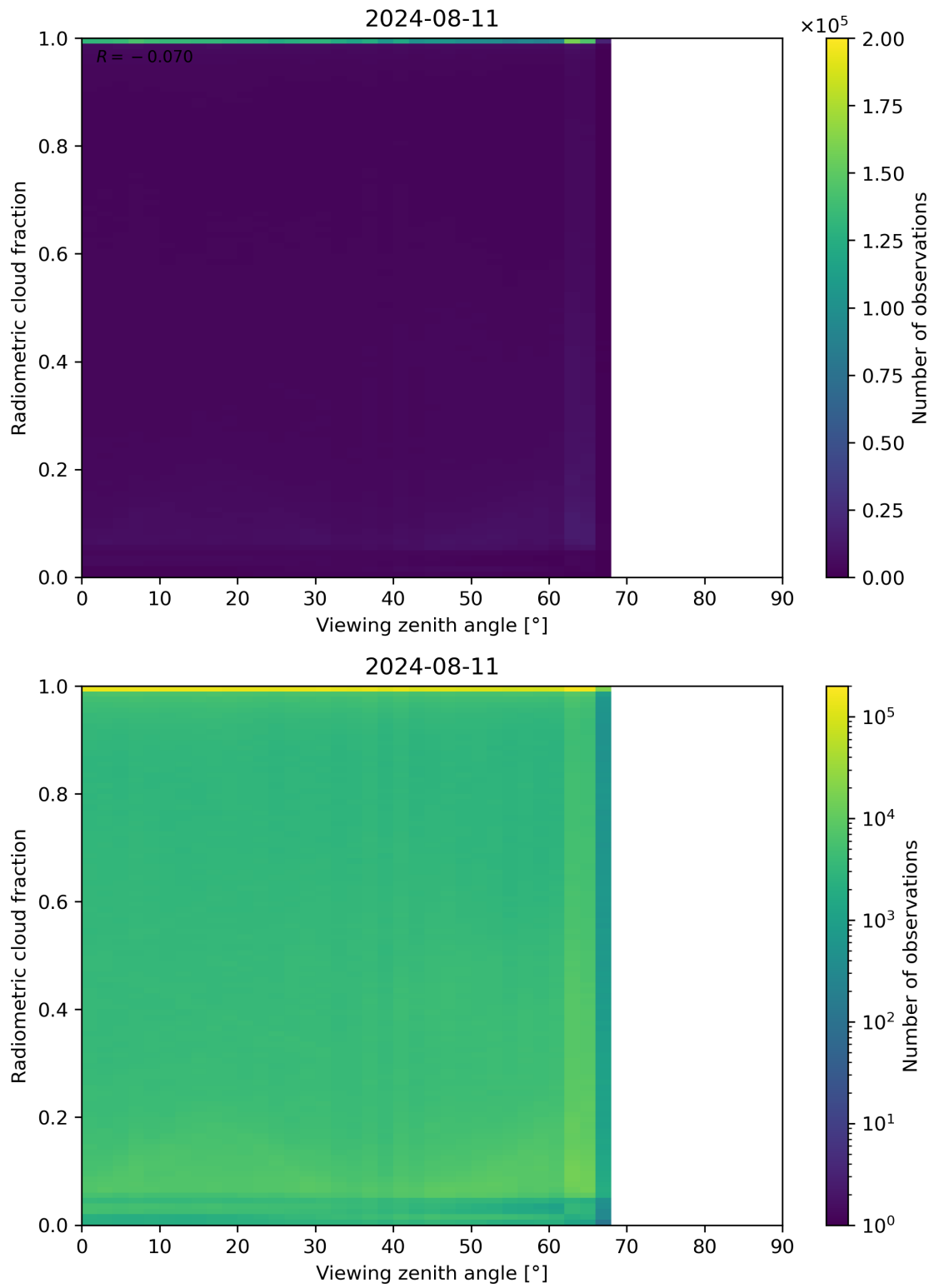
Figure 107: Scatter density plot of “Viewing zenith angle” against “Radiometric cloud fraction” for 2024-08-11 to 2024-08-11.
