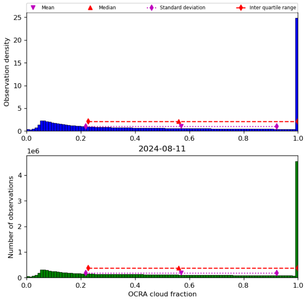
Figure 50: Histogram of “OCRA cloud fraction” for 2024-08-11 to 2024-08-11
