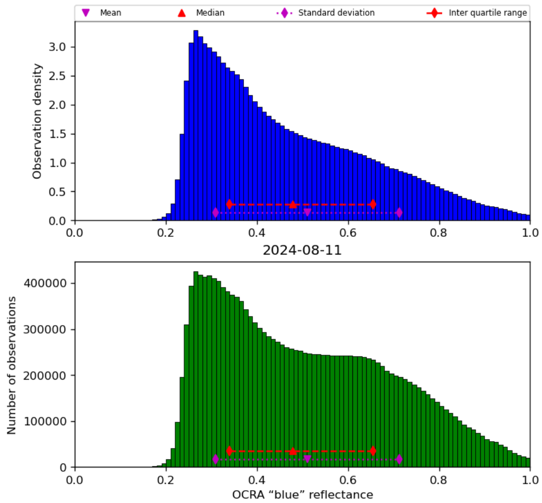
Figure 51: Histogram of “OCRA “blue” reflectance” for 2024-08-11 to 2024-08-11
