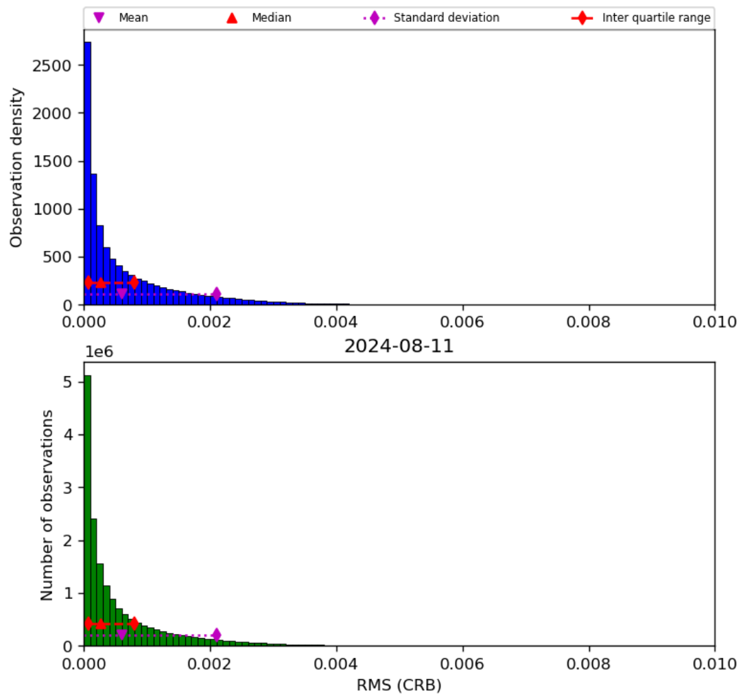
Figure 48: Histogram of “RMS (CRB)” for 2024-08-11 to 2024-08-11
