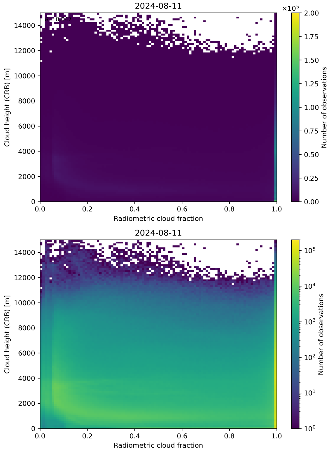
Figure 74: Scatter density plot of “Radiometric cloud fraction” against “Cloud height (CRB)” for 2024-08-11 to 2024-08-11.
