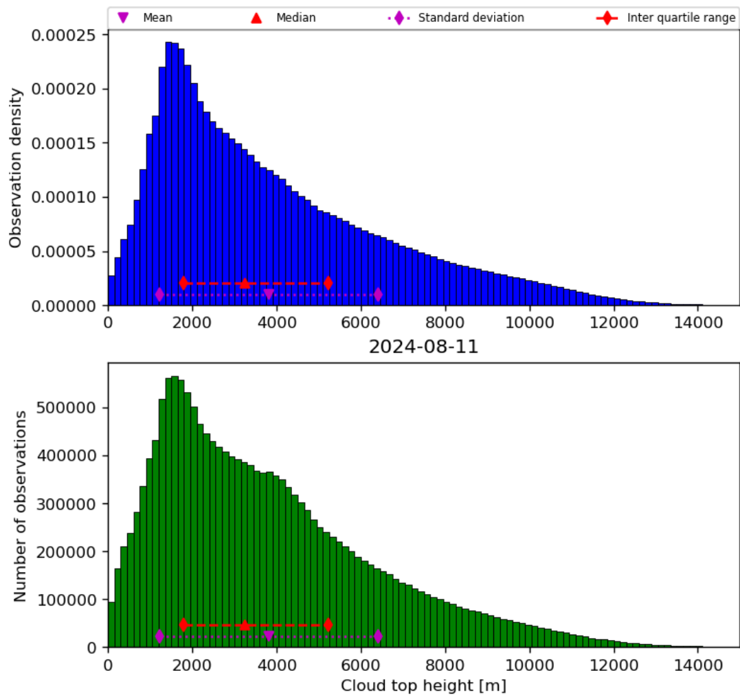
Figure 40: Histogram of “Cloud top height” for 2024-08-11 to 2024-08-11
