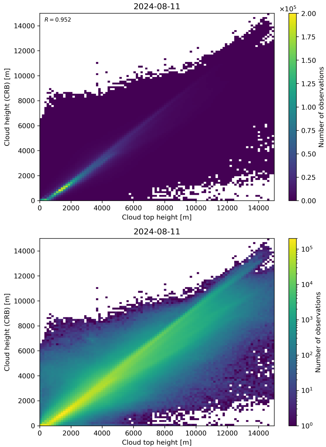
Figure 89: Scatter density plot of “Cloud top height” against “Cloud height (CRB)” for 2024-08-11 to 2024-08-11.
