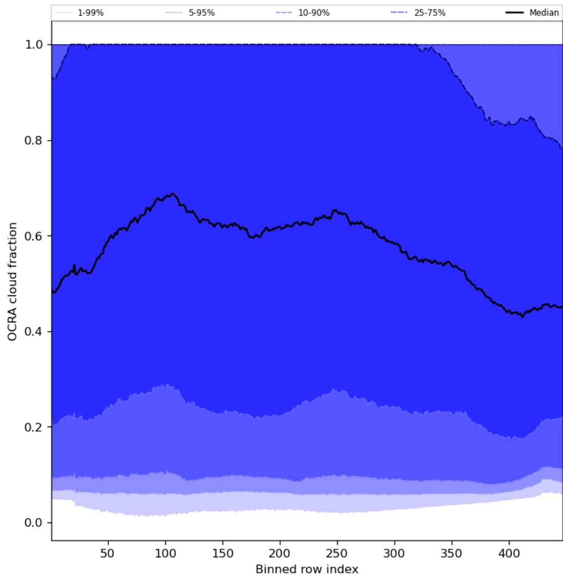
Figure 66: Along track statistics of “OCRA cloud fraction” for 2024-08-11 to 2024-08-11
