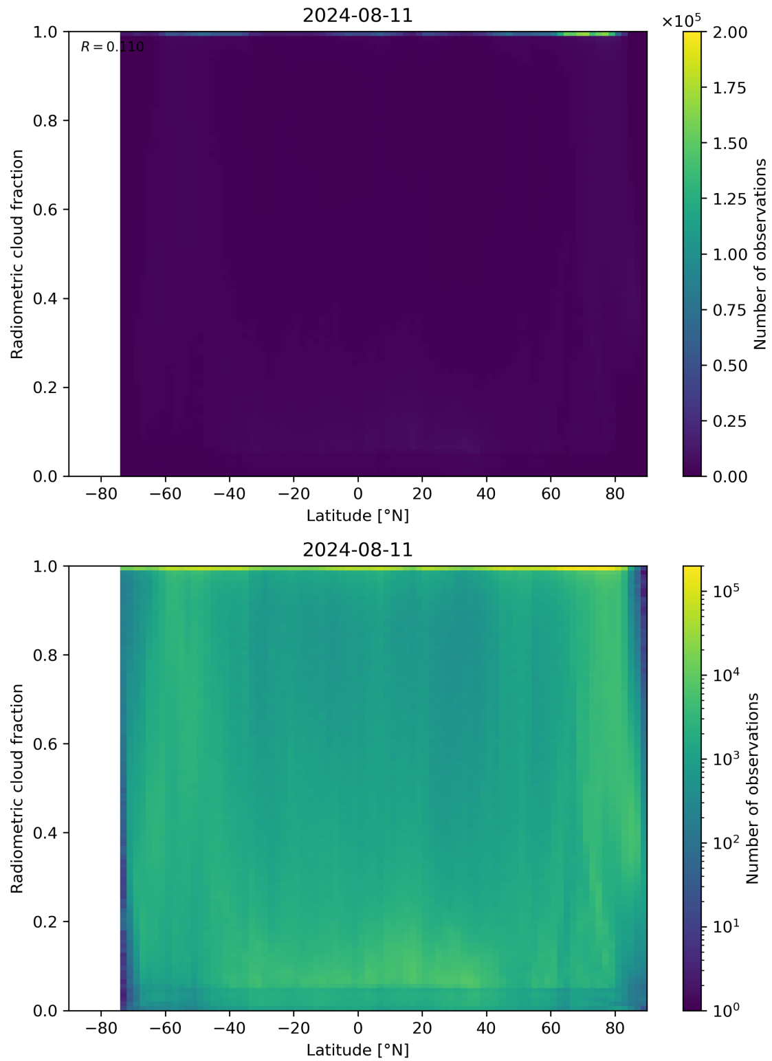
Figure 92: Scatter density plot of “Latitude” against “Radiometric cloud fraction” for 2024-08-11 to 2024-08-11.
