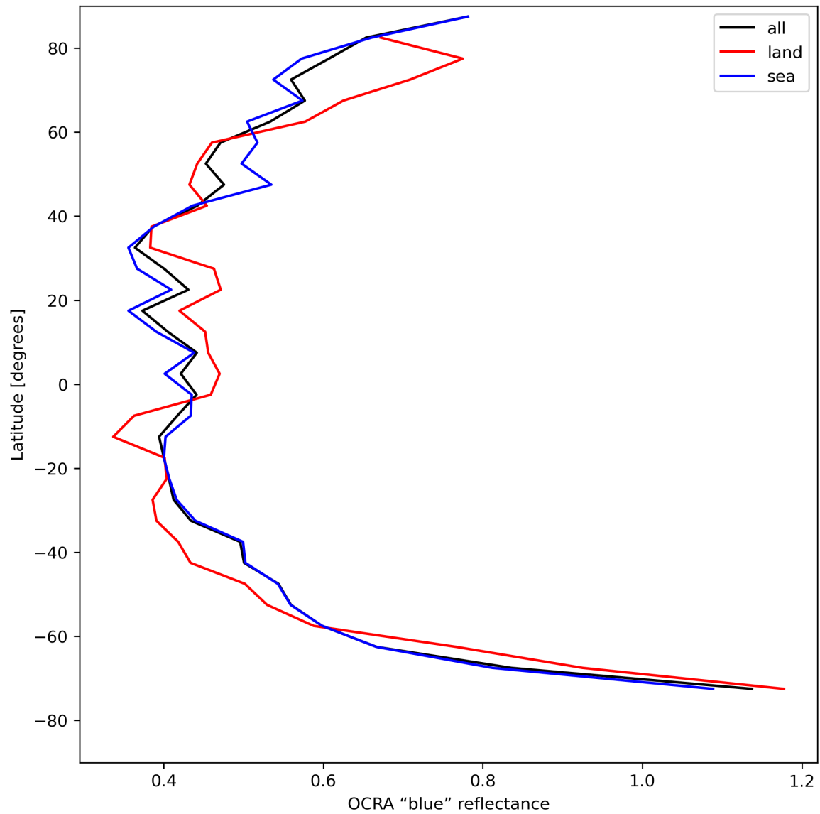
Figure 35: Zonal average of “OCRA “blue” reflectance” for 2024-08-11 to 2024-08-11.
