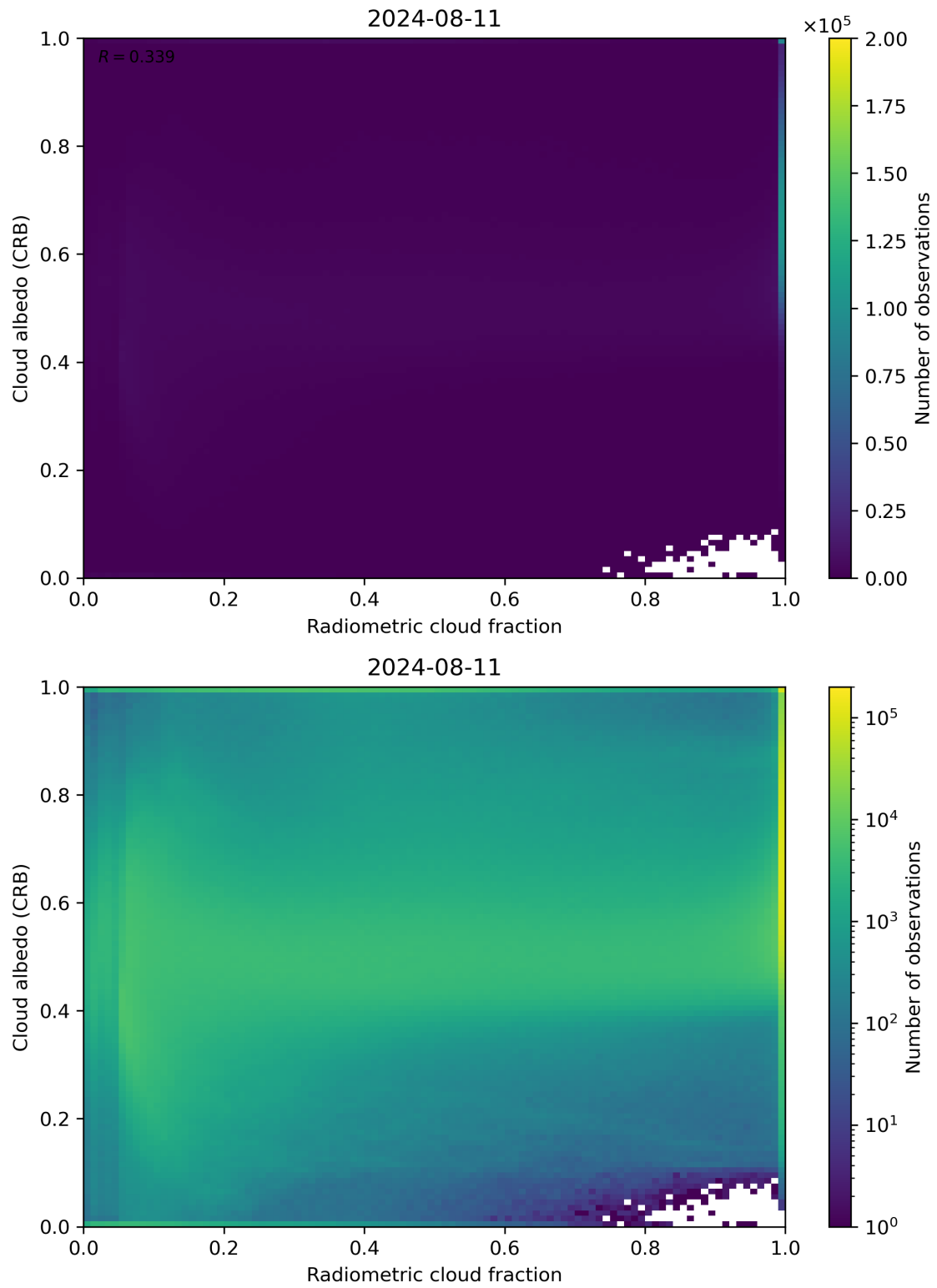
Figure 71: Scatter density plot of “Radiometric cloud fraction” against “Cloud albedo (CRB)” for 2024-08-11 to 2024-08-11.
