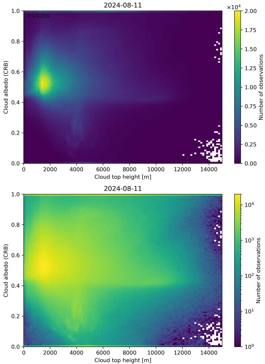
Figure 86: Scatter density plot of “Cloud top height” against “Cloud albedo (CRB)” for 2024-08-11 to 2024-08-11.
