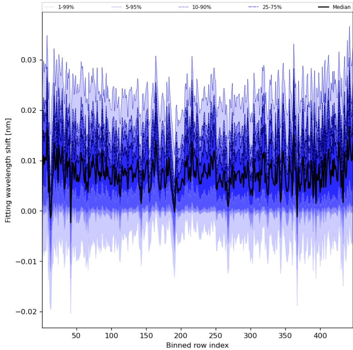
Figure 65: Along track statistics of “Fitting wavelength shift” for 2024-08-11 to 2024-08-11
