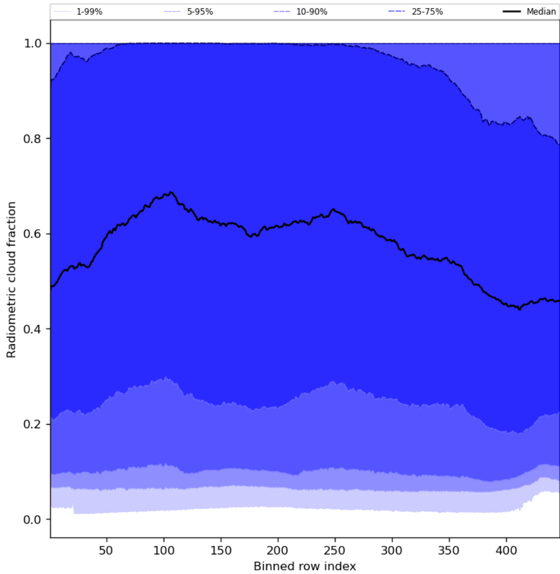
Figure 55: Along track statistics of “Radiometric cloud fraction” for 2024-08-11 to 2024-08-11
