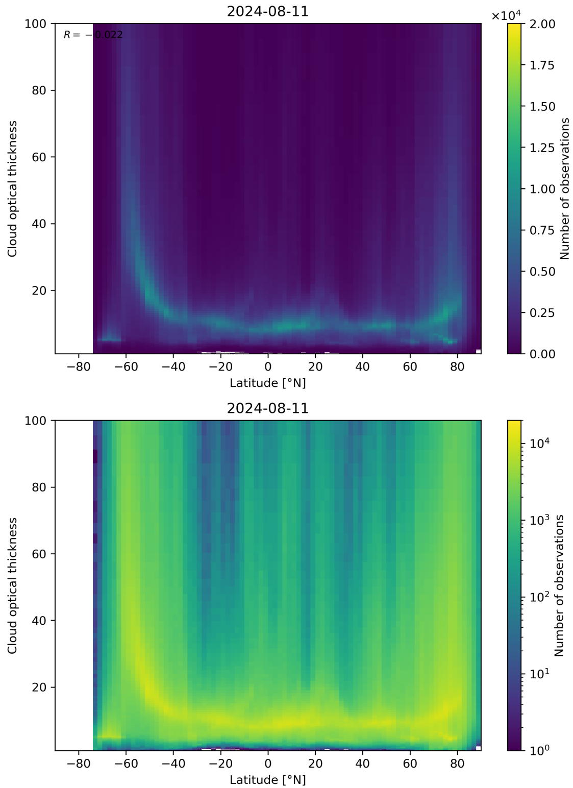
Figure 96: Scatter density plot of “Latitude” against “Cloud optical thickness” for 2024-08-11 to 2024-08-11.
