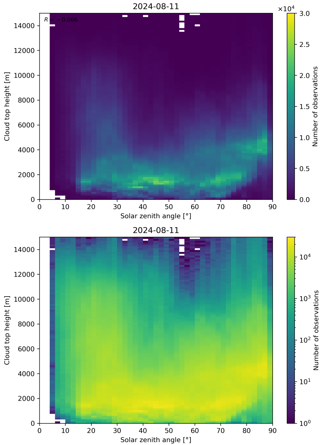
Figure 104: Scatter density plot of “Solar zenith angle” against “Cloud top height” for 2024-08-11 to 2024-08-11.
