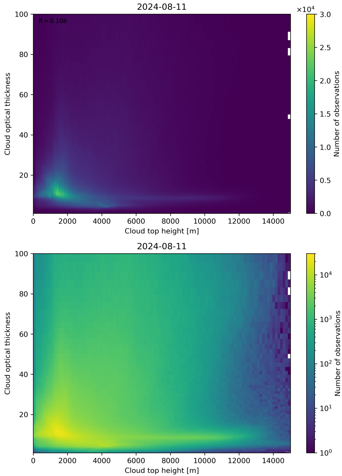
Figure 90: Scatter density plot of “Cloud top height” against “Cloud optical thickness” for 2024-08-11 to 2024-08-11.
