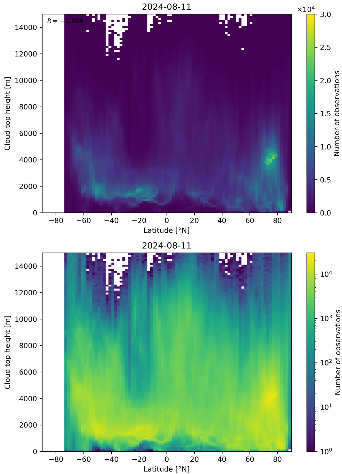
Figure 97: Scatter density plot of “Latitude” against “Cloud top height” for 2024-08-11 to 2024-08-11.
