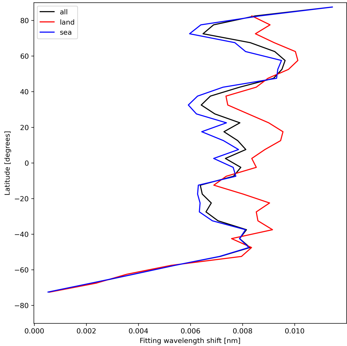
Figure 33: Zonal average of “Fitting wavelength shift” for 2024-08-11 to 2024-08-11.
