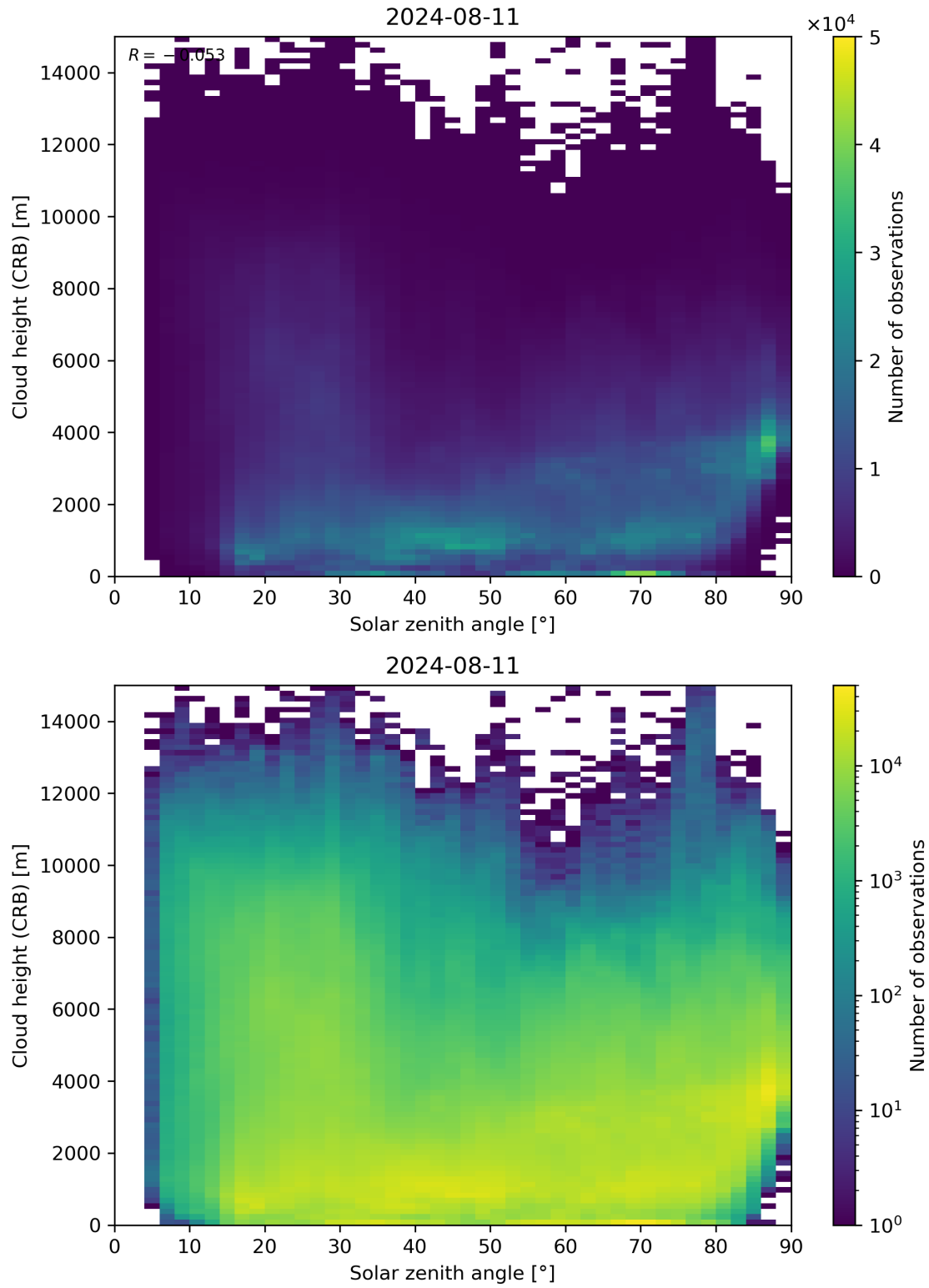
Figure 102: Scatter density plot of “Solar zenith angle” against “Cloud height (CRB)” for 2024-08-11 to 2024-08-11.
