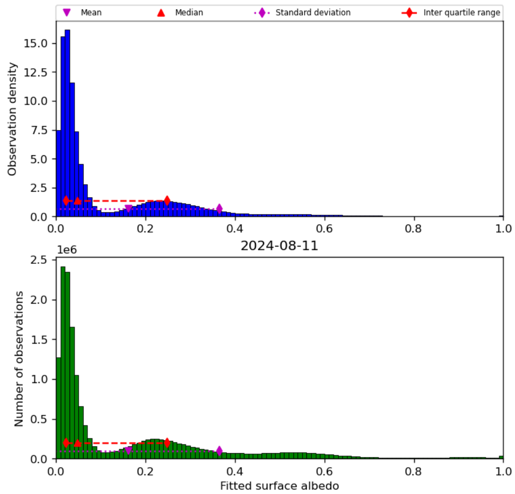
Figure 45: Histogram of “Fitted surface albedo” for 2024-08-11 to 2024-08-11
