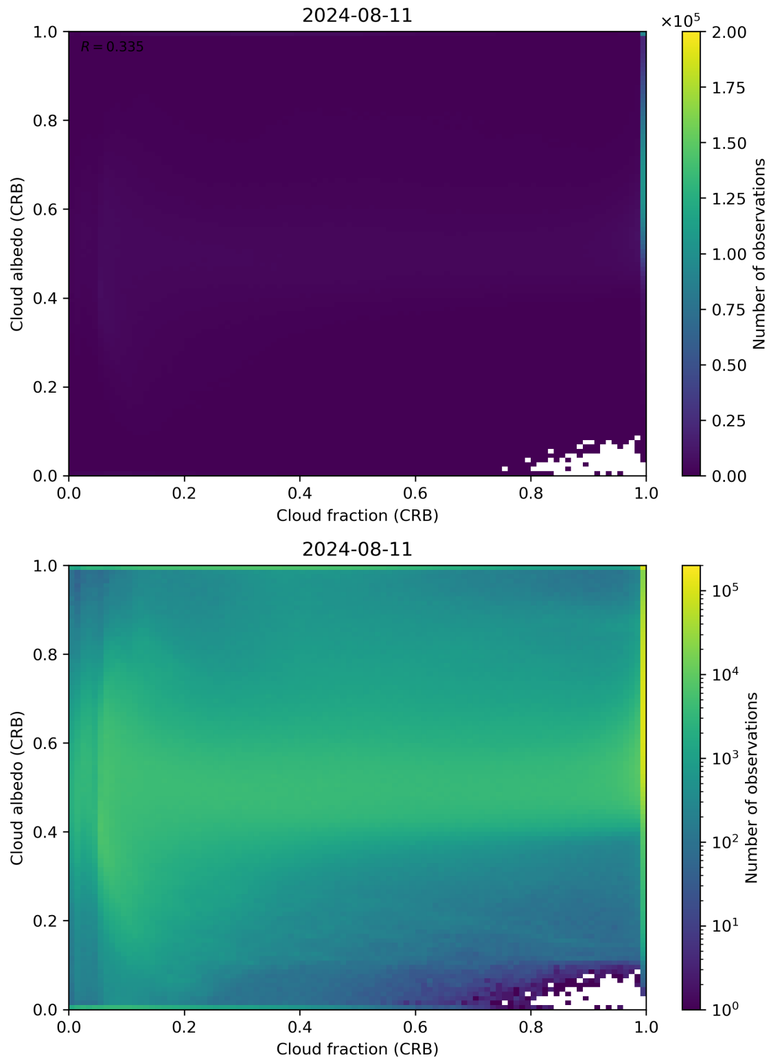
Figure 77: Scatter density plot of “Cloud fraction (CRB)” against “Cloud albedo (CRB)” for 2024-08-11 to 2024-08-11.
