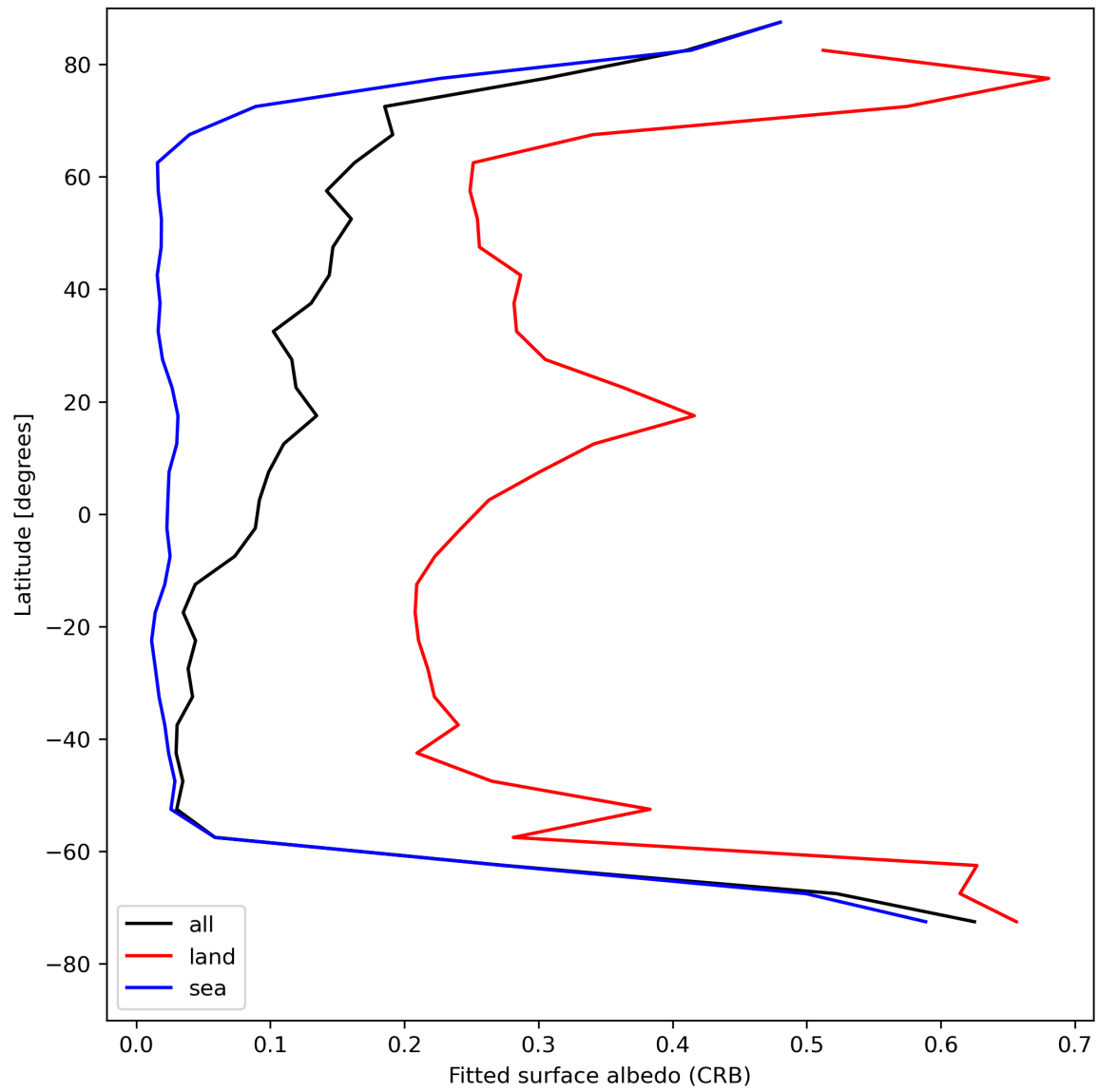
Figure 30: Zonal average of “Fitted surface albedo (CRB)” for 2024-08-11 to 2024-08-11.
