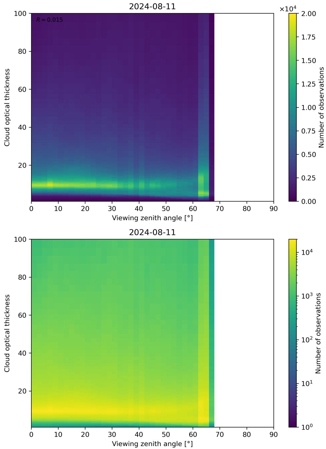
Figure 111: Scatter density plot of “Viewing zenith angle” against “Cloud optical thickness” for 2024-08-11 to 2024-08-11.
