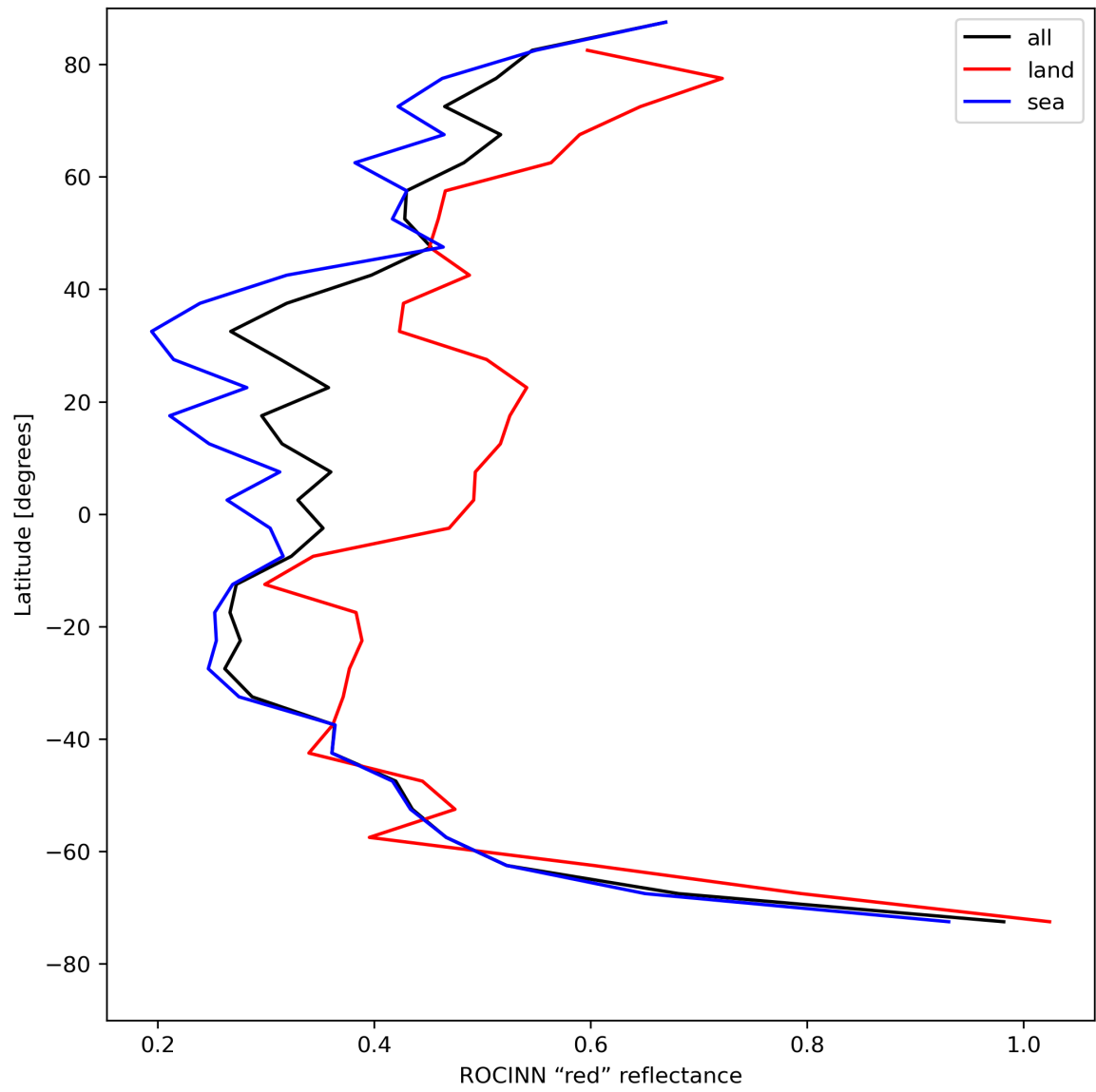
Figure 37: Zonal average of “ROCINN “red” reflectance” for 2024-08-11 to 2024-08-11.
