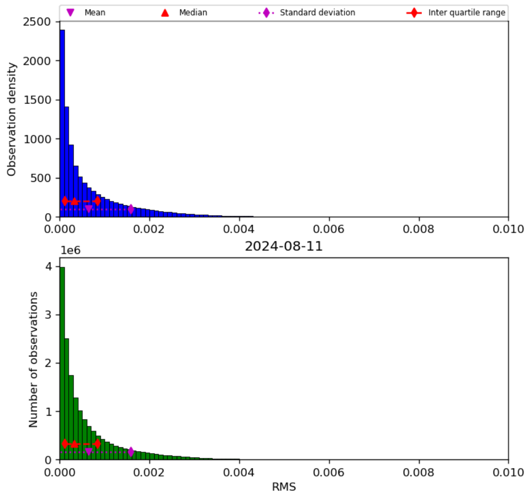
Figure 47: Histogram of “RMS” for 2024-08-11 to 2024-08-11
