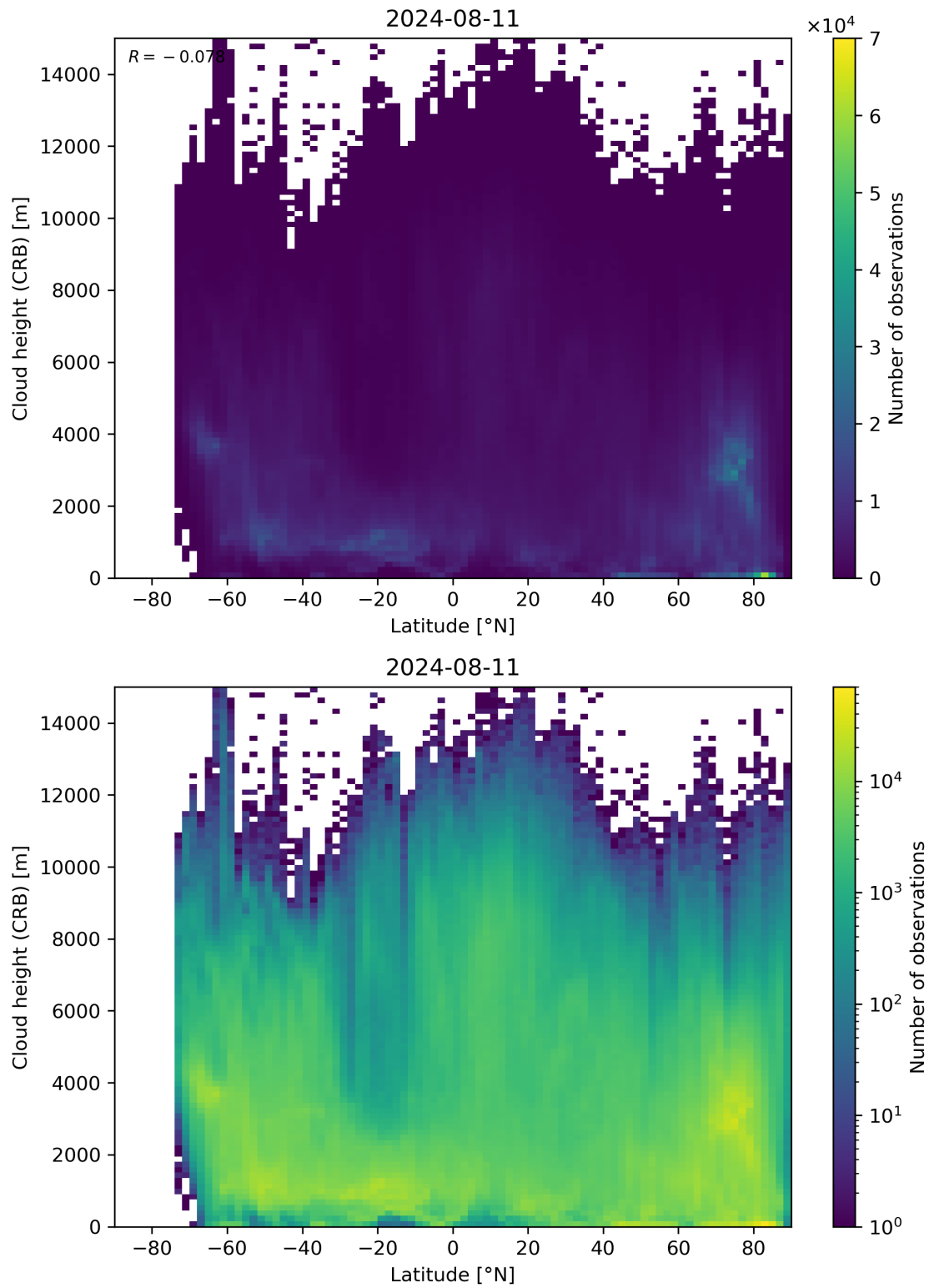
Figure 95: Scatter density plot of “Latitude” against “Cloud height (CRB)” for 2024-08-11 to 2024-08-11.
