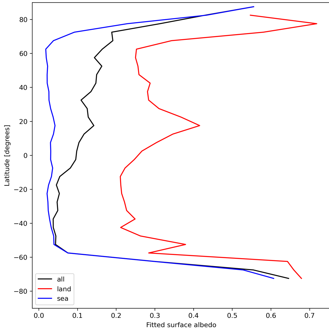
Figure 29: Zonal average of “Fitted surface albedo” for 2024-08-11 to 2024-08-11.
