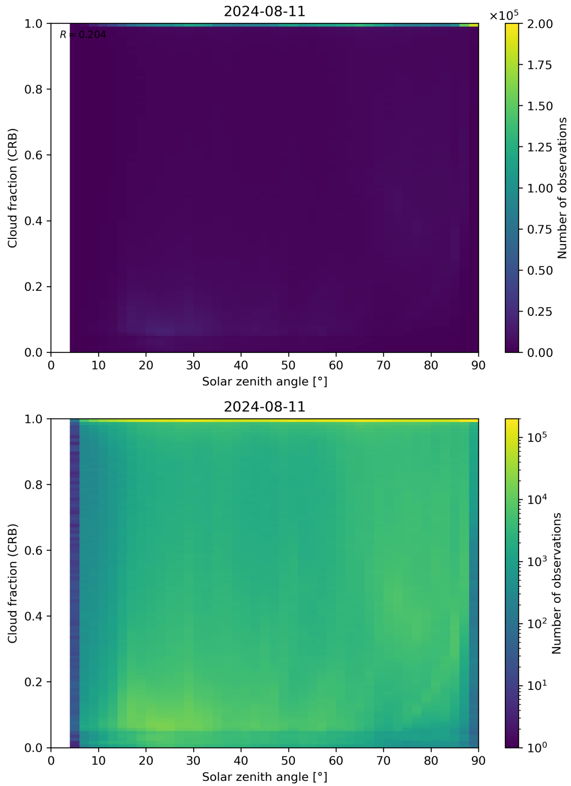
Figure 101: Scatter density plot of “Solar zenith angle” against “Cloud fraction (CRB)” for 2024-08-11 to 2024-08-11.
