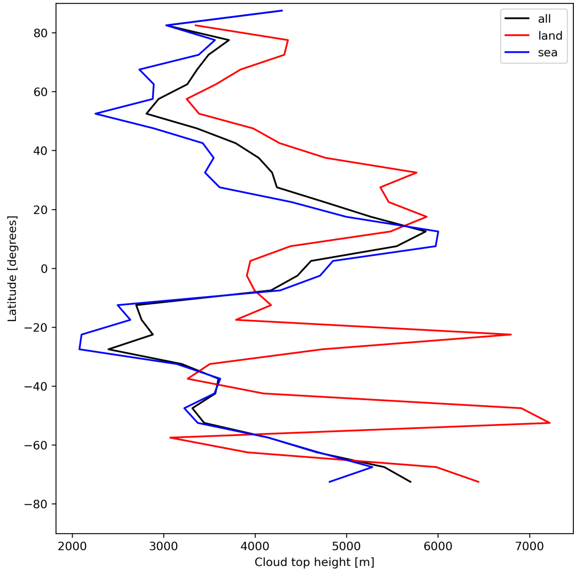
Figure 24: Zonal average of “Cloud top height” for 2024-08-11 to 2024-08-11.
