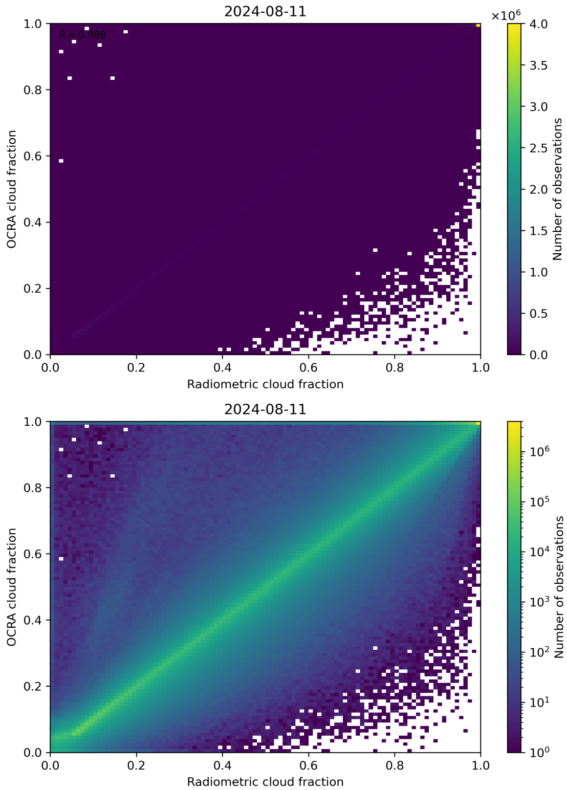
Figure 72: Scatter density plot of “Radiometric cloud fraction” against “OCRA cloud fraction” for 2024-08-11 to 2024-08-11.
