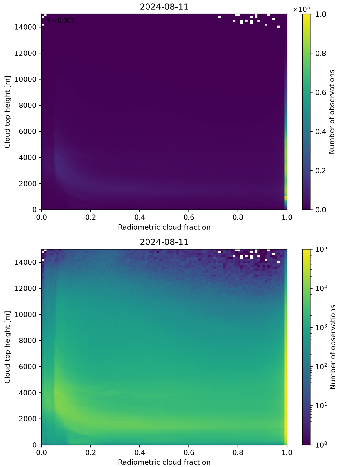
Figure 76: Scatter density plot of “Radiometric cloud fraction” against “Cloud top height” for 2024-08-11 to 2024-08-11.
