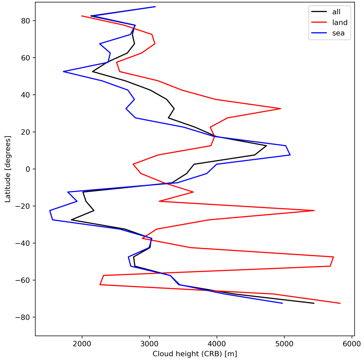
Figure 27: Zonal average of “Cloud height (CRB)” for 2024-08-11 to 2024-08-11.
