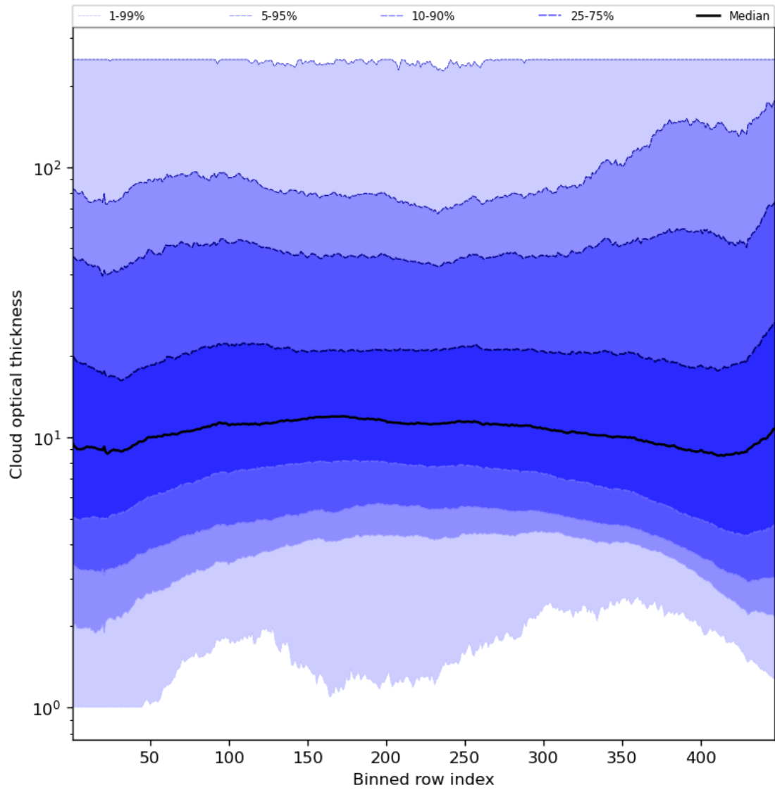
Figure 57: Along track statistics of “Cloud optical thickness” for 2024-08-11 to 2024-08-11
