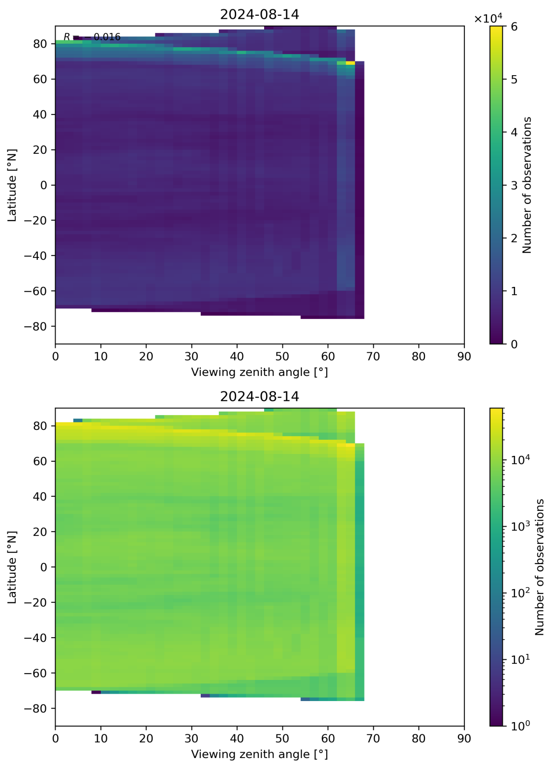
Figure 113: Scatter density plot of “Viewing zenith angle” against “Latitude” for 2024-08-13 to 2024-08-15.
