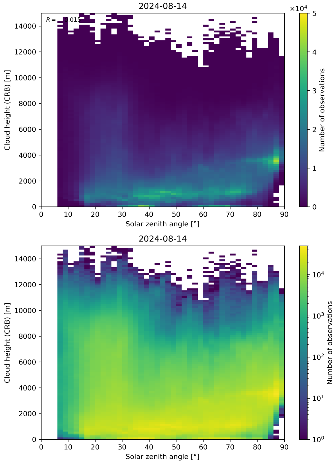
Figure 102: Scatter density plot of “Solar zenith angle” against “Cloud height (CRB)” for 2024-08-13 to 2024-08-15.
