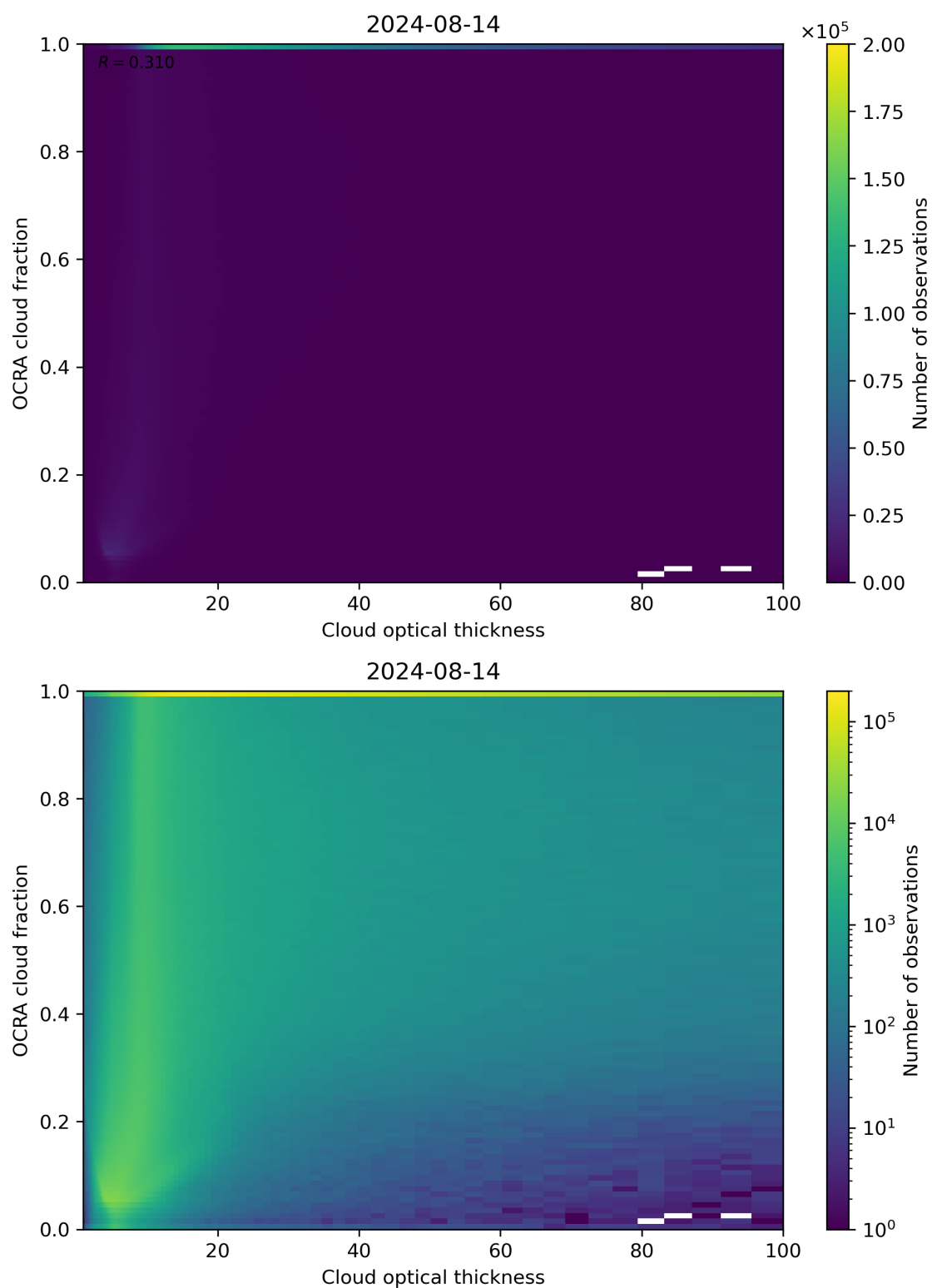
Figure 83: Scatter density plot of “Cloud optical thickness” against “OCRA cloud fraction” for 2024-08-13 to 2024-08-15.
