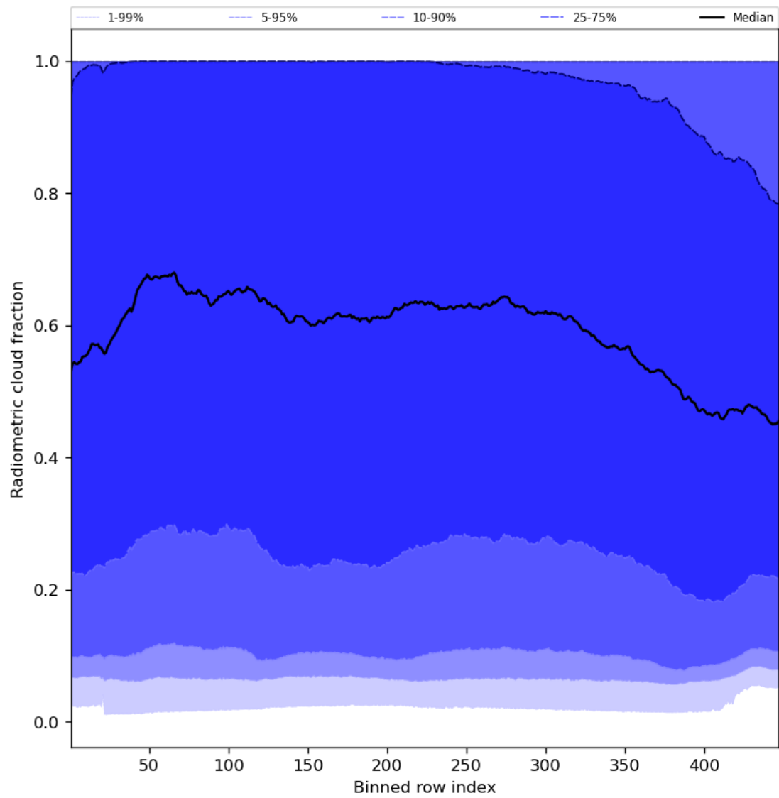
Figure 55: Along track statistics of “Radiometric cloud fraction” for 2024-08-13 to 2024-08-15
