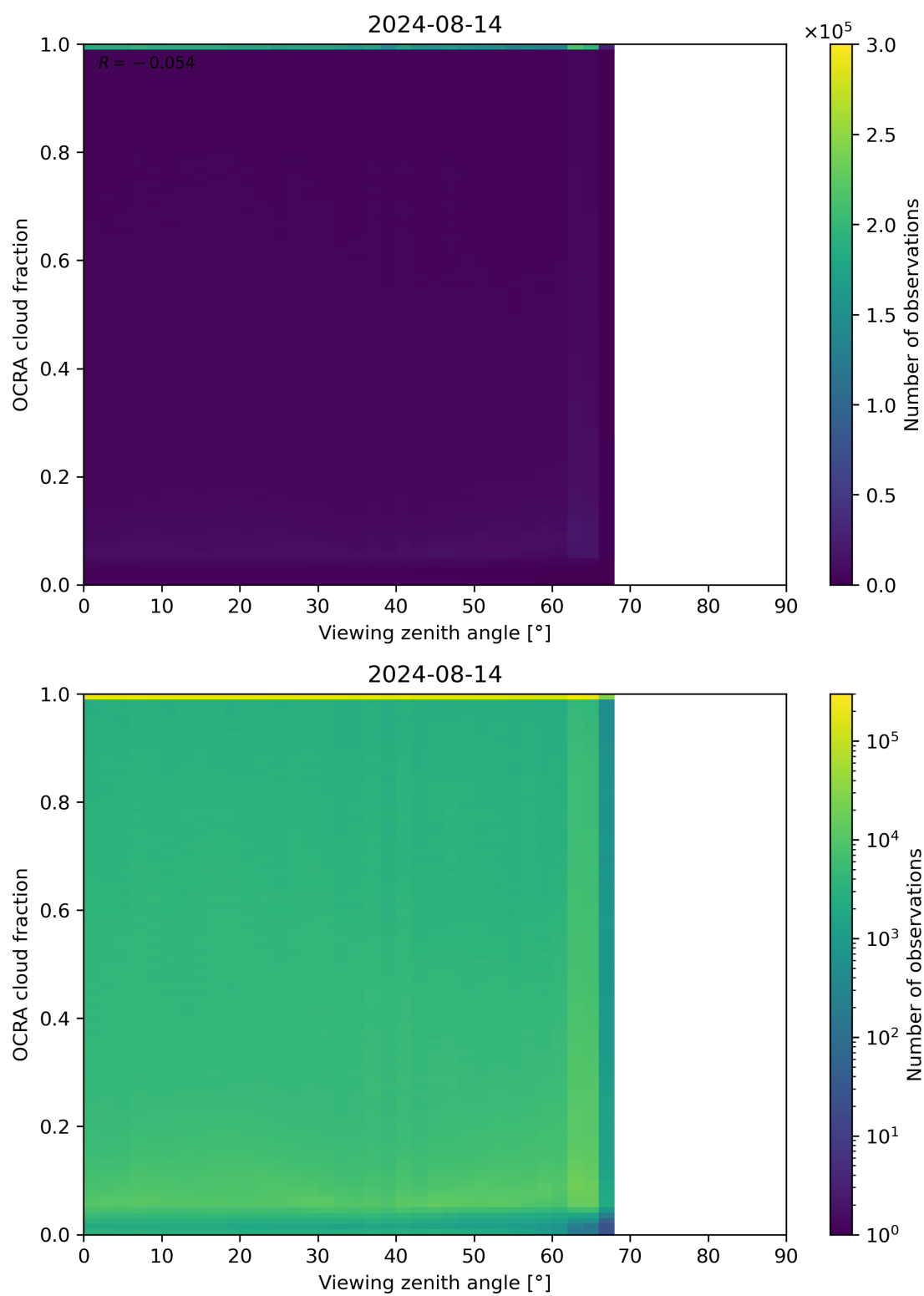
Figure 108: Scatter density plot of “Viewing zenith angle” against “OCRA cloud fraction” for 2024-08-13 to 2024-08-15.
