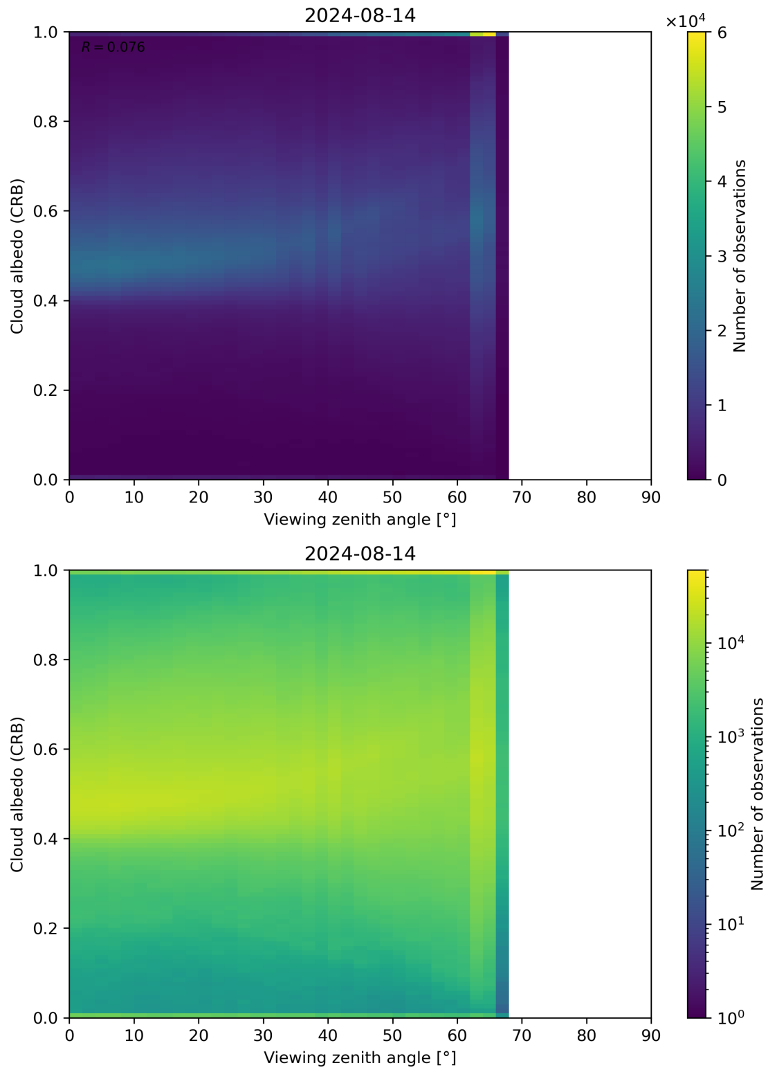
Figure 106: Scatter density plot of “Viewing zenith angle” against “Cloud albedo (CRB)” for 2024-08-13 to 2024-08-15.
