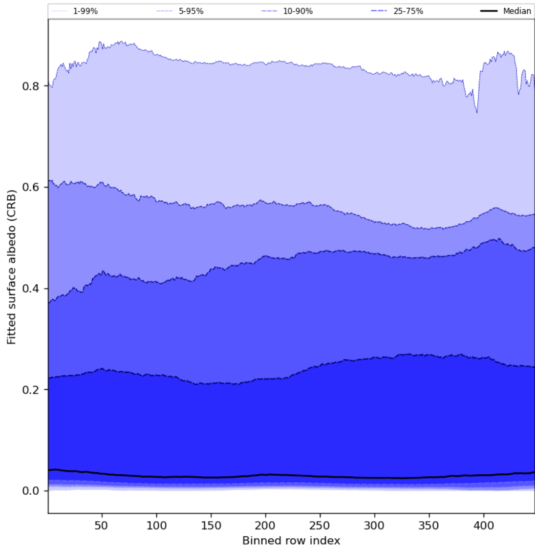
Figure 62: Along track statistics of “Fitted surface albedo (CRB)” for 2024-08-13 to 2024-08-15
