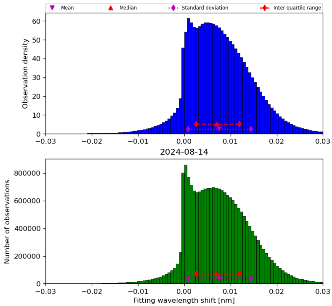
Figure 49: Histogram of “Fitting wavelength shift” for 2024-08-13 to 2024-08-15
