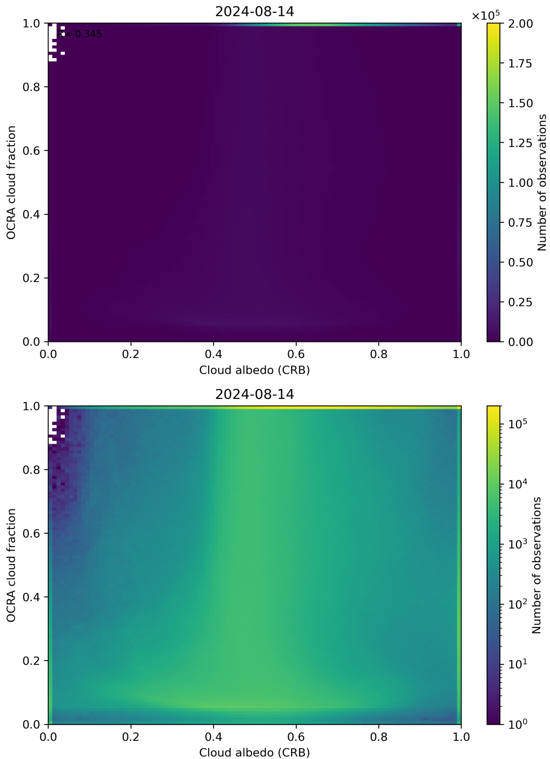
Figure 70: Scatter density plot of “Cloud albedo (CRB)” against “OCRA cloud fraction” for 2024-08-13 to 2024-08-15.
