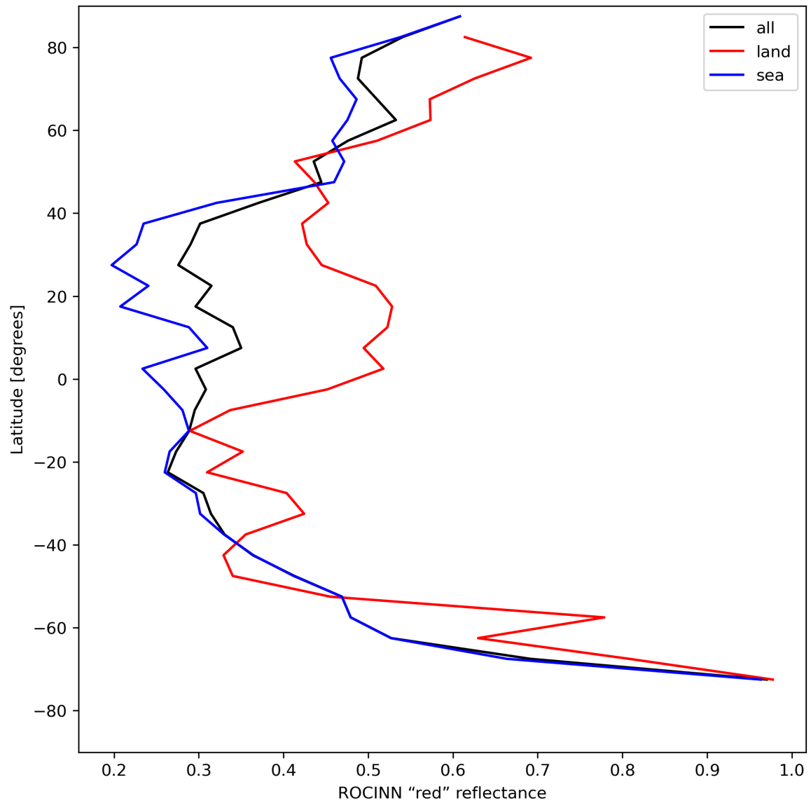
Figure 37: Zonal average of “ROCINN “red” reflectance” for 2024-08-13 to 2024-08-15.
