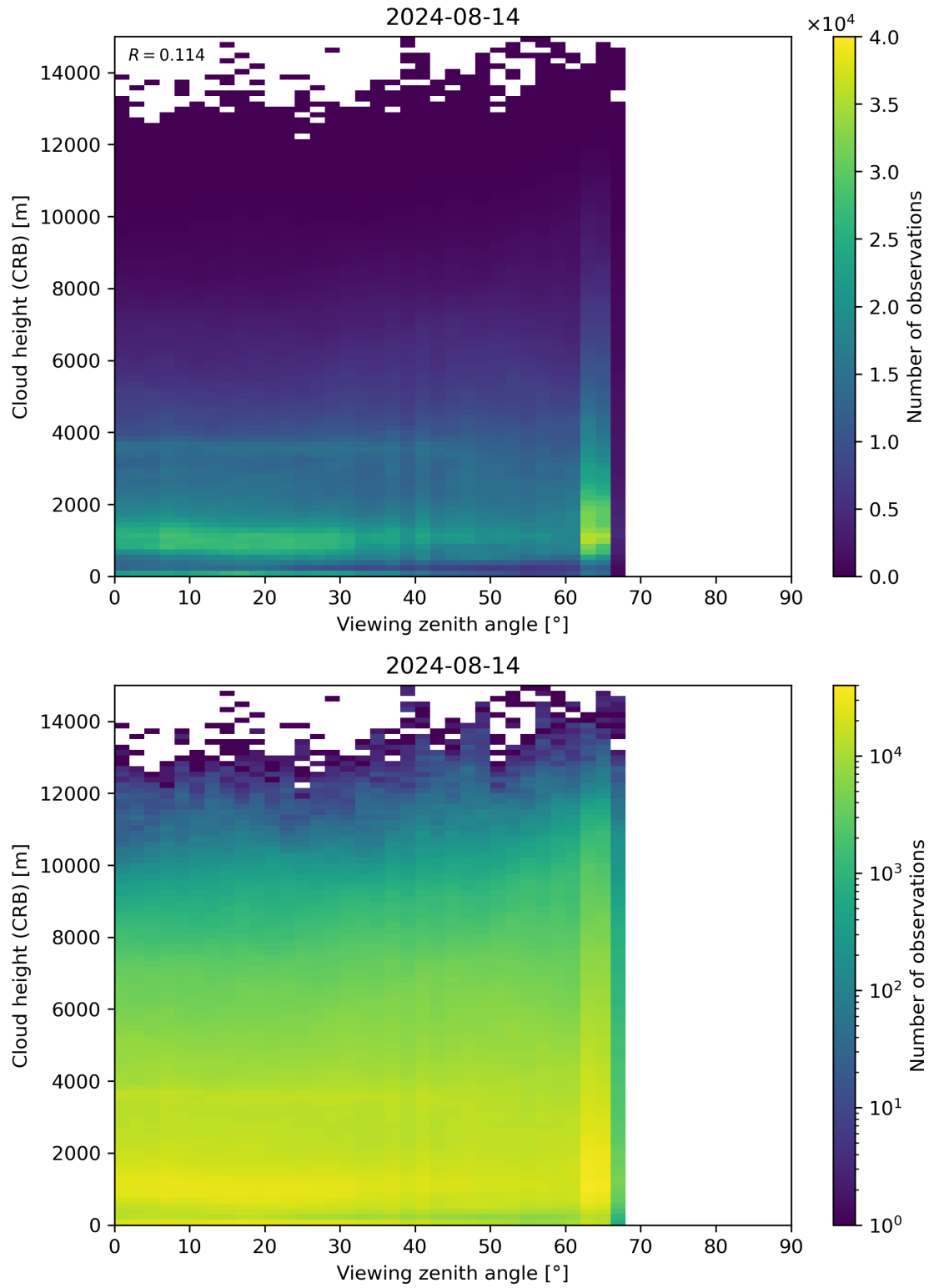
Figure 110: Scatter density plot of “Viewing zenith angle” against “Cloud height (CRB)” for 2024-08-13 to 2024-08-15.
