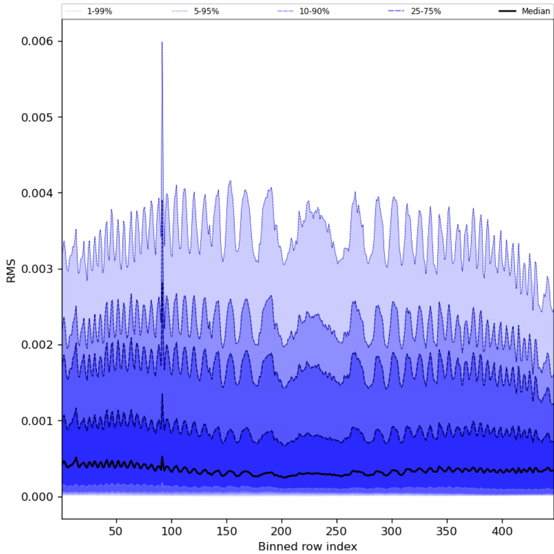
Figure 63: Along track statistics of “RMS” for 2024-08-13 to 2024-08-15
