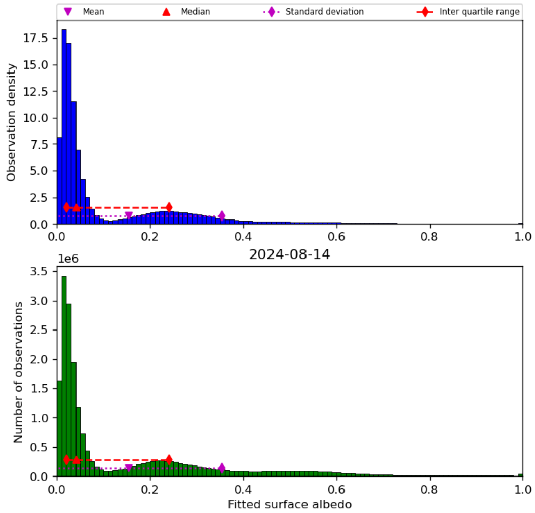
Figure 45: Histogram of “Fitted surface albedo” for 2024-08-13 to 2024-08-15
