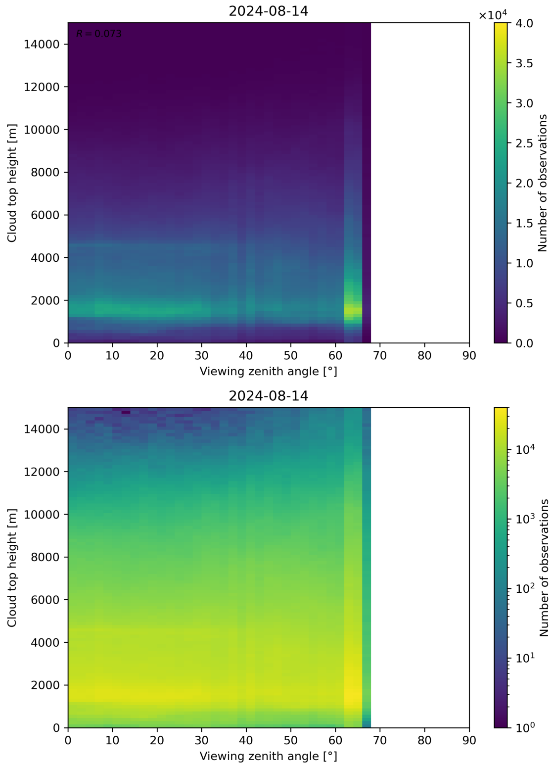
Figure 112: Scatter density plot of “Viewing zenith angle” against “Cloud top height” for 2024-08-13 to 2024-08-15.
