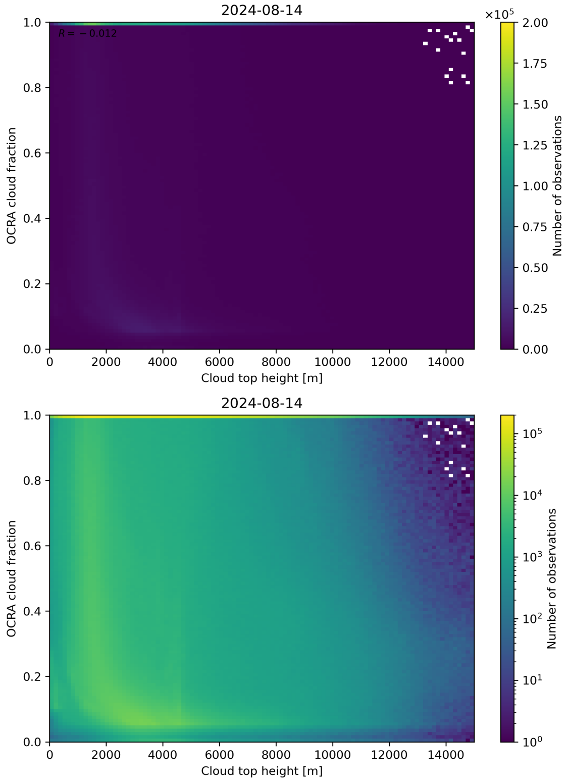
Figure 87: Scatter density plot of “Cloud top height” against “OCRA cloud fraction” for 2024-08-13 to 2024-08-15.
