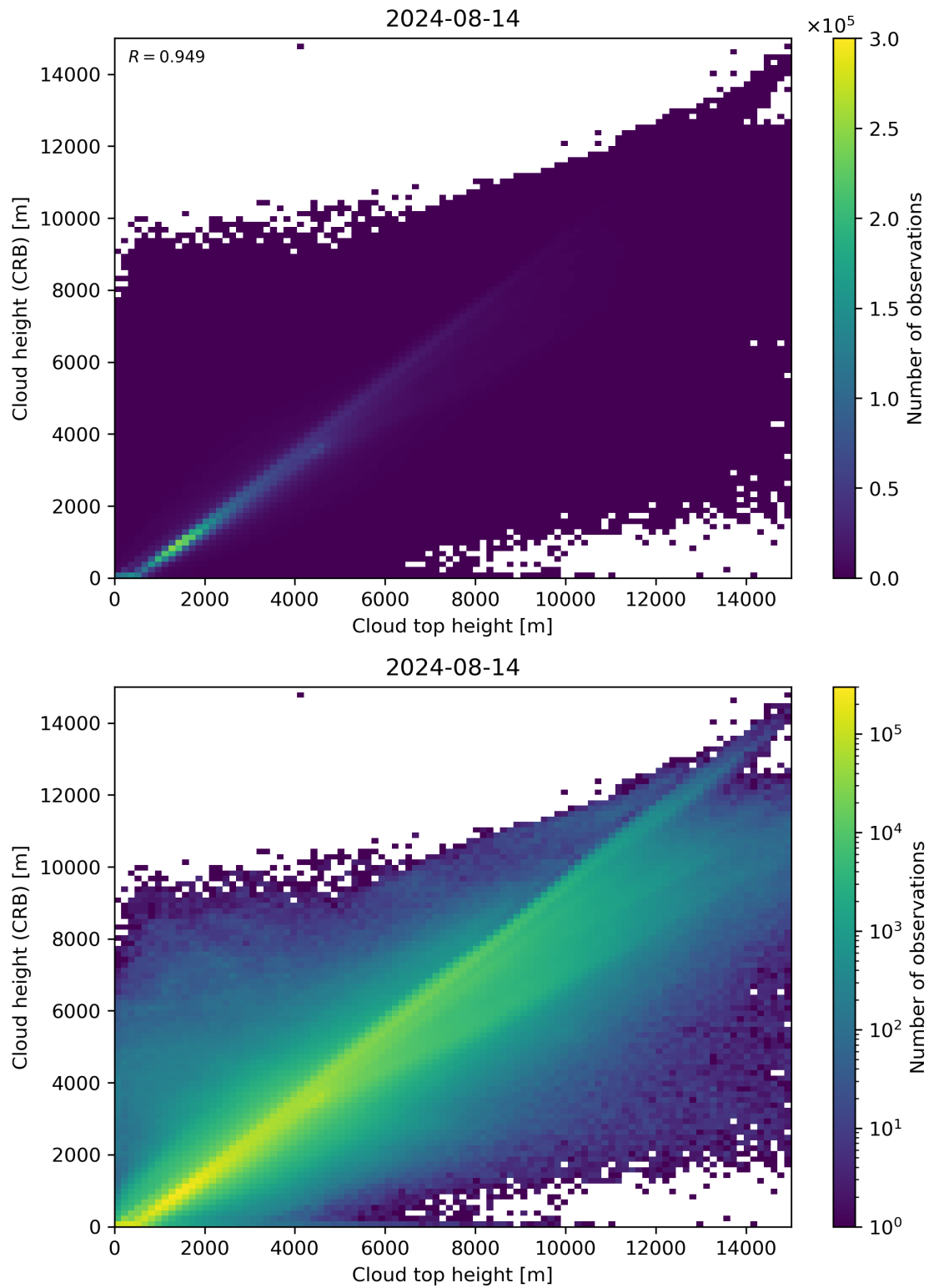
Figure 89: Scatter density plot of “Cloud top height” against “Cloud height (CRB)” for 2024-08-13 to 2024-08-15.
