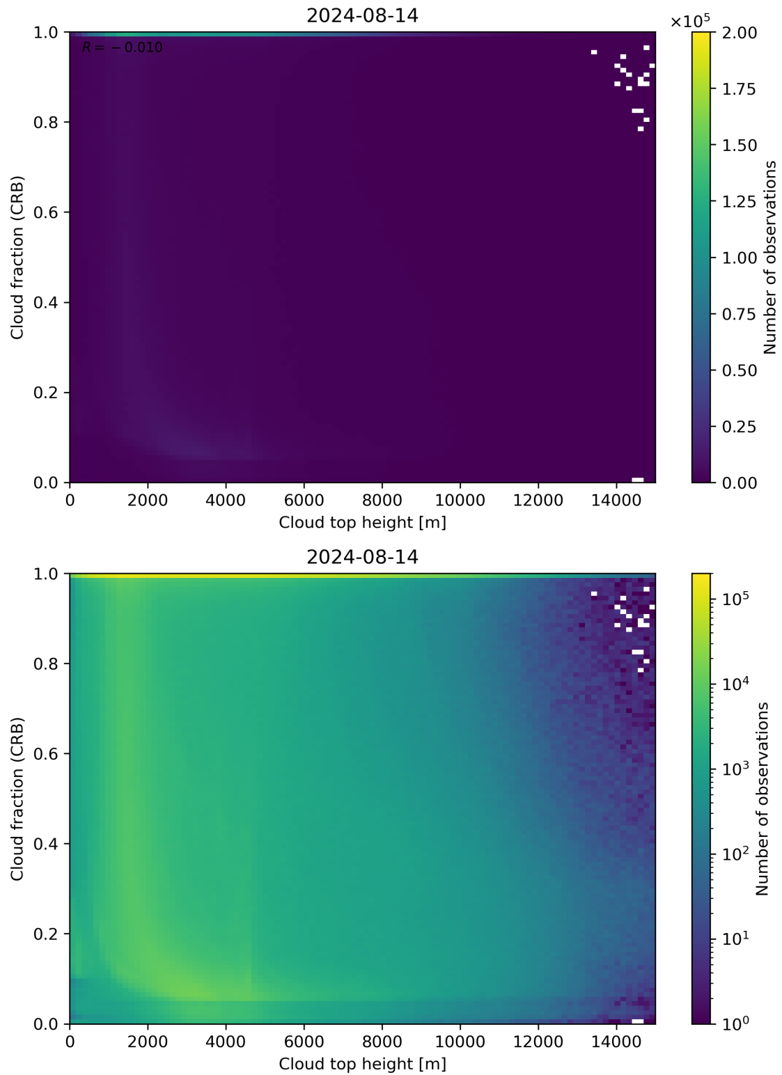
Figure 88: Scatter density plot of “Cloud top height” against “Cloud fraction (CRB)” for 2024-08-13 to 2024-08-15.
