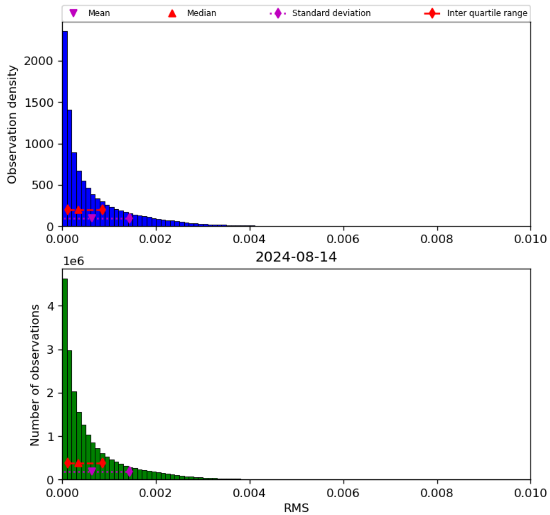
Figure 47: Histogram of “RMS” for 2024-08-13 to 2024-08-15
