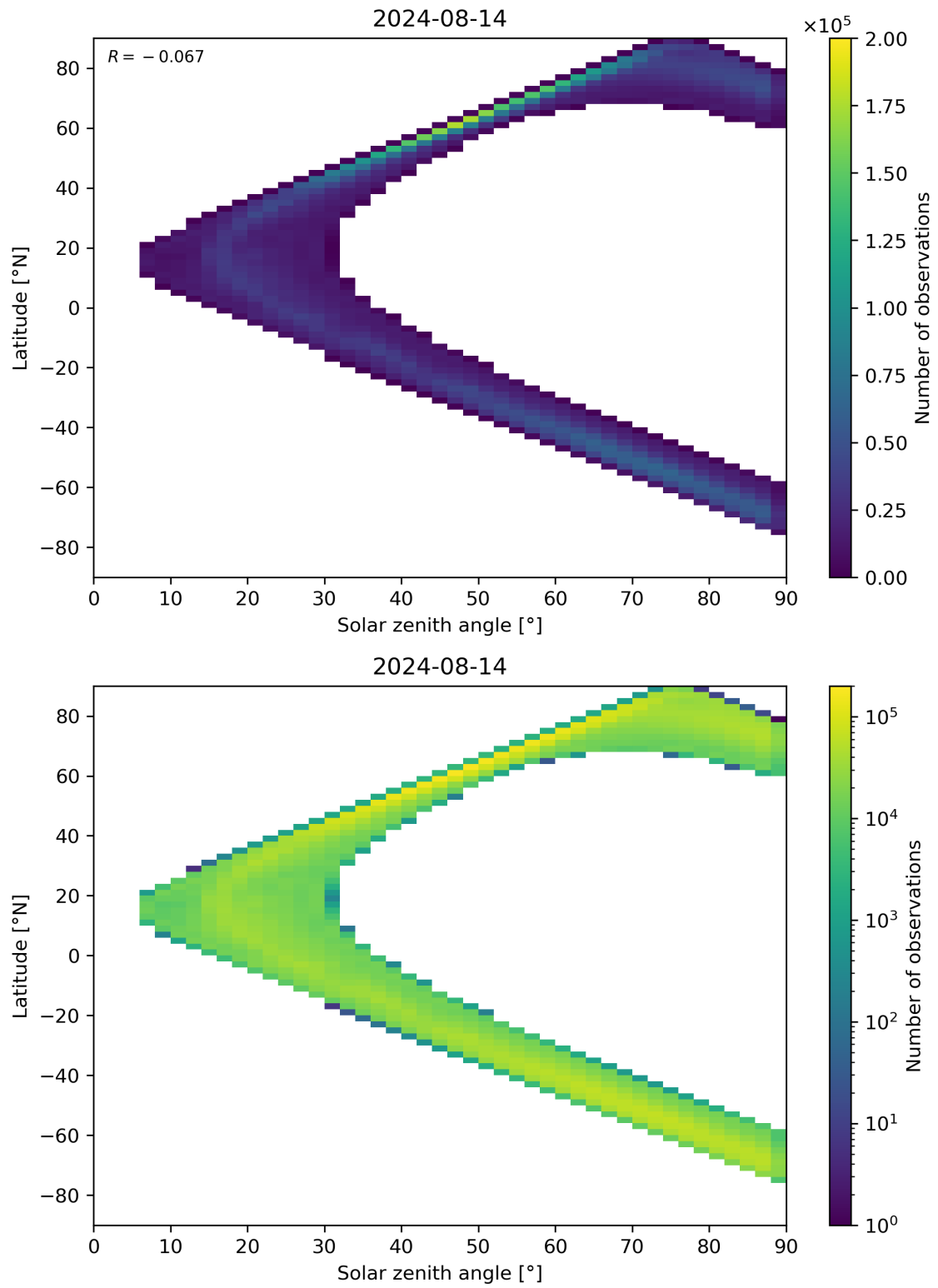
Figure 105: Scatter density plot of “Solar zenith angle” against “Latitude” for 2024-08-13 to 2024-08-15.
