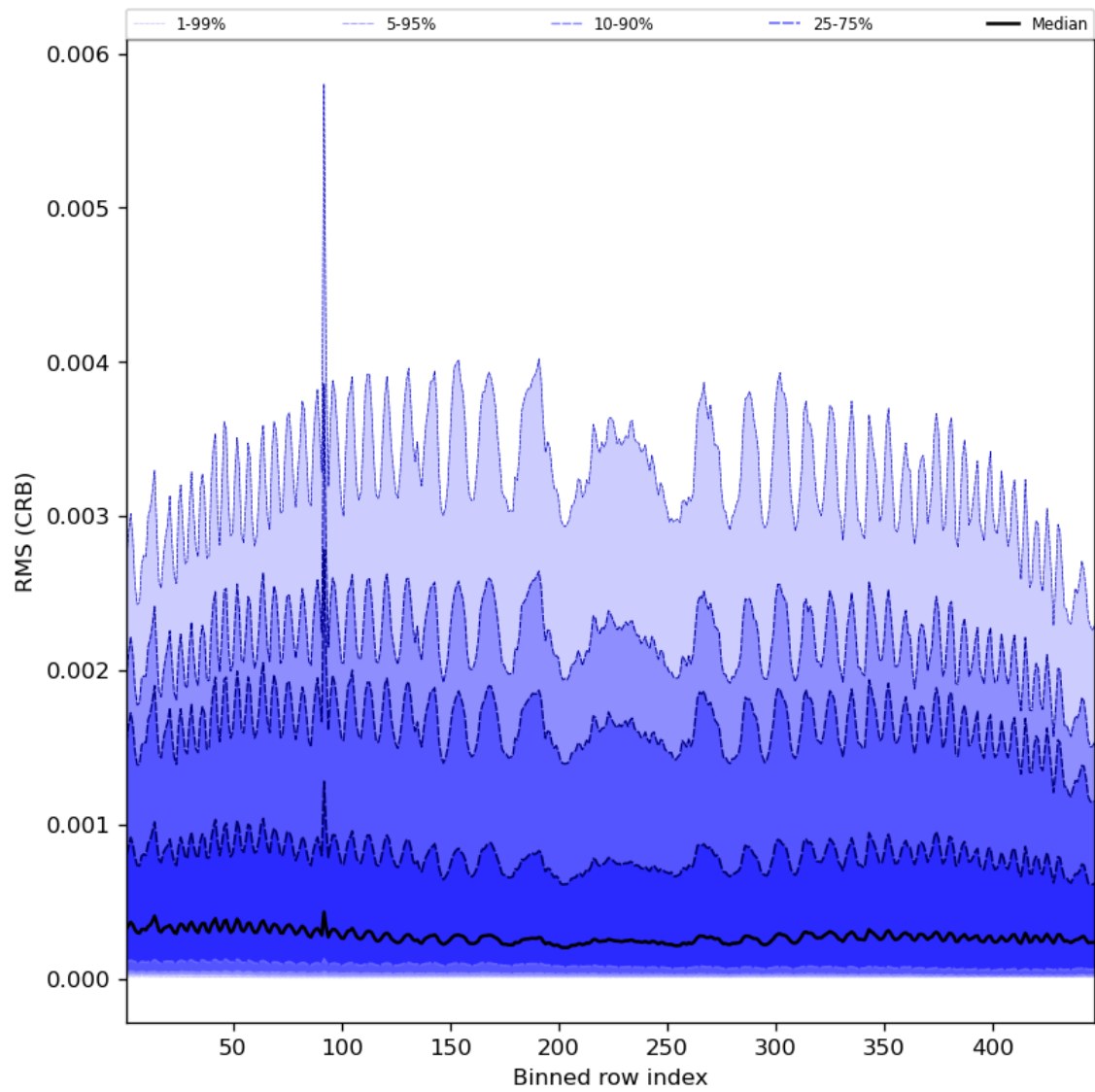
Figure 64: Along track statistics of “RMS (CRB)” for 2024-08-13 to 2024-08-15
