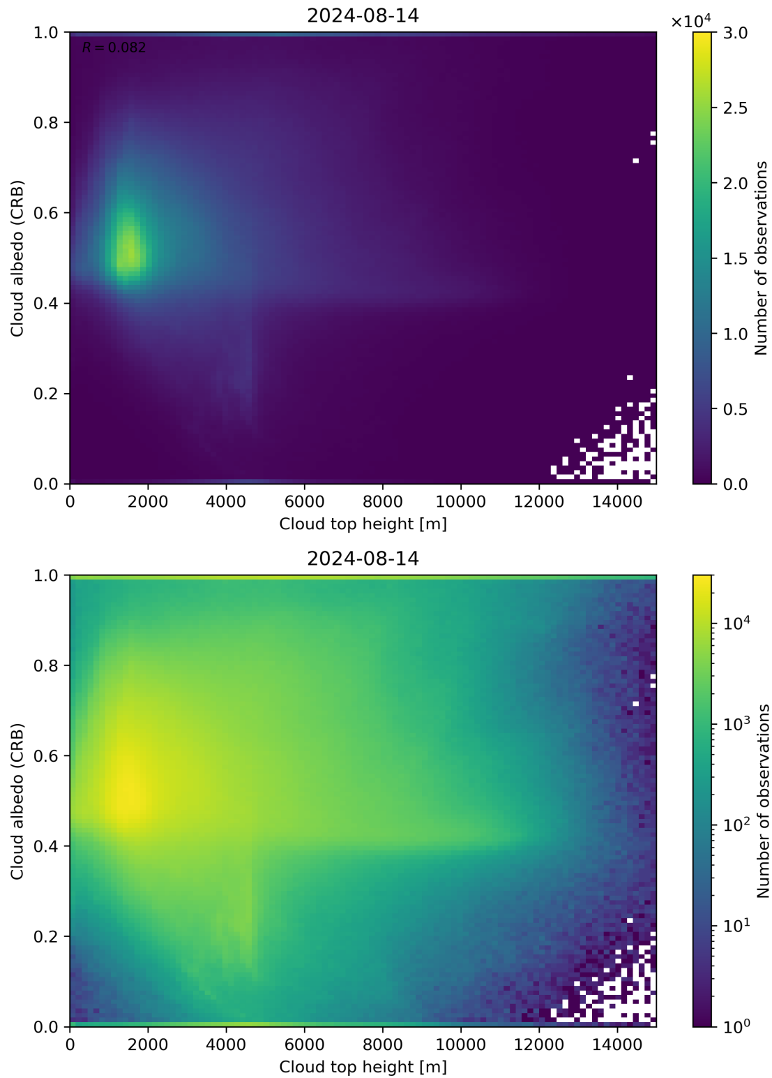
Figure 86: Scatter density plot of “Cloud top height” against “Cloud albedo (CRB)” for 2024-08-13 to 2024-08-15.
