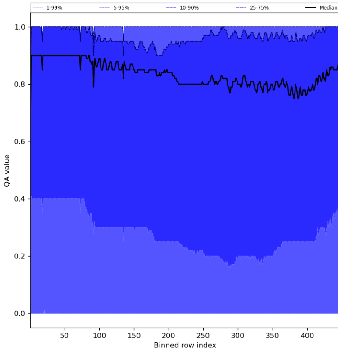
Figure 54: Along track statistics of “QA value” for 2024-08-13 to 2024-08-15
