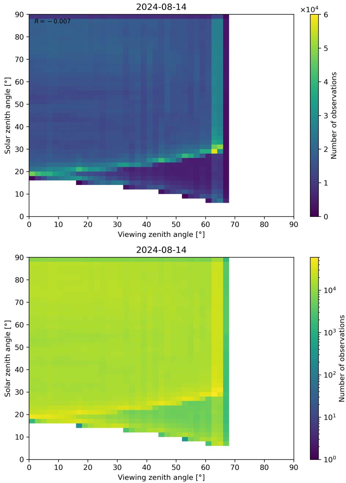
Figure 114: Scatter density plot of “Viewing zenith angle” against “Solar zenith angle” for 2024-08-13 to 2024-08-15.
