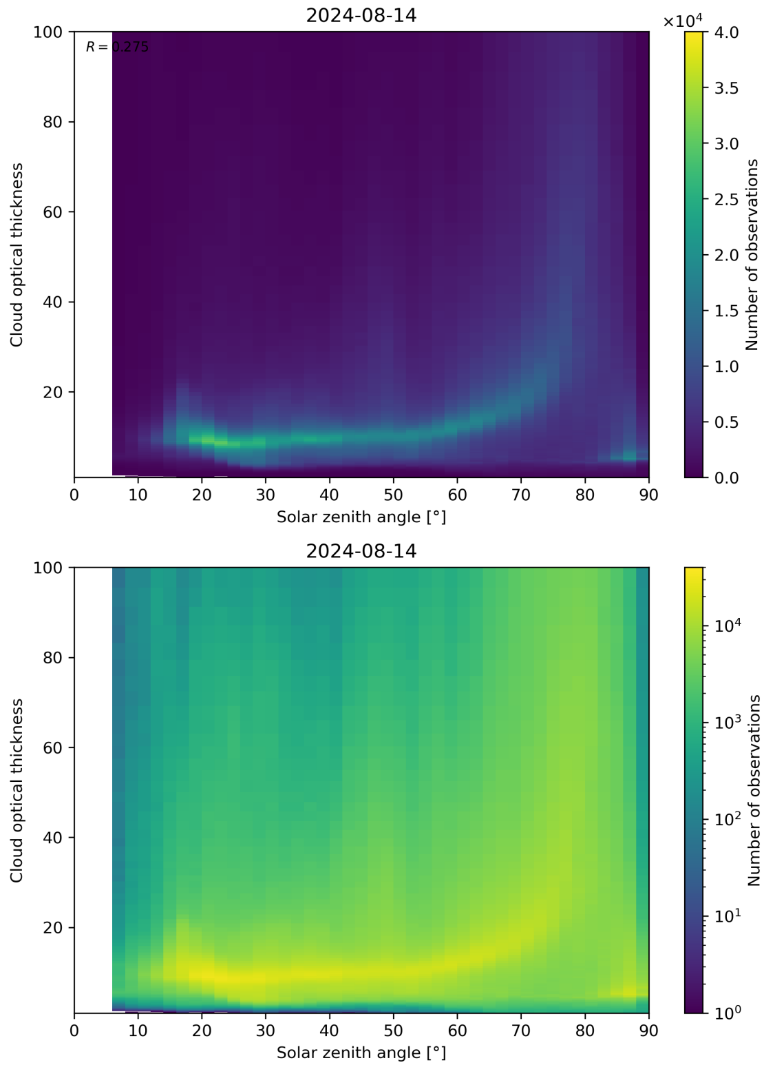
Figure 103: Scatter density plot of “Solar zenith angle” against “Cloud optical thickness” for 2024-08-13 to 2024-08-15.
