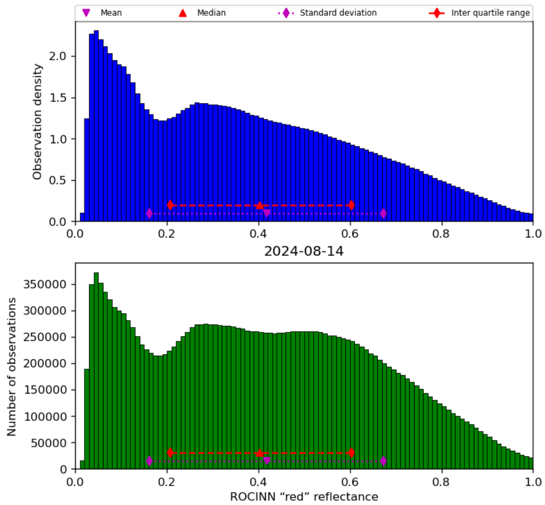
Figure 53: Histogram of “ROCINN “red” reflectance” for 2024-08-13 to 2024-08-15
