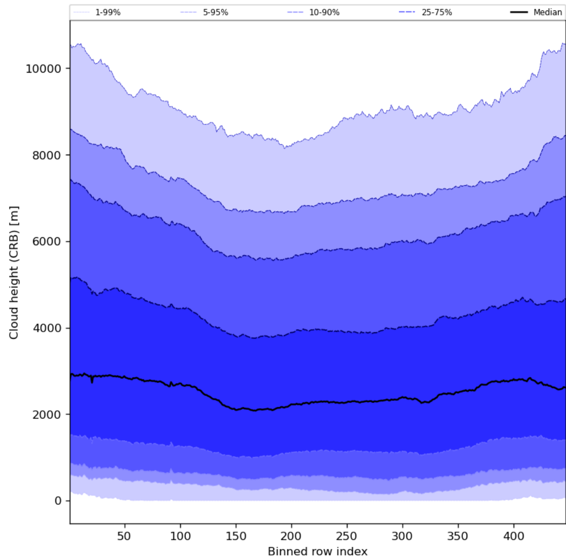
Figure 59: Along track statistics of “Cloud height (CRB)” for 2024-08-13 to 2024-08-15
