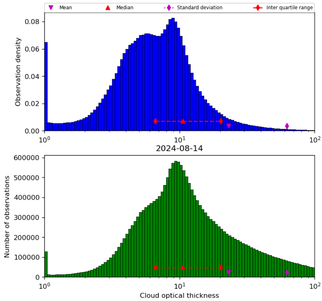
Figure 41: Histogram of “Cloud optical thickness” for 2024-08-13 to 2024-08-15
