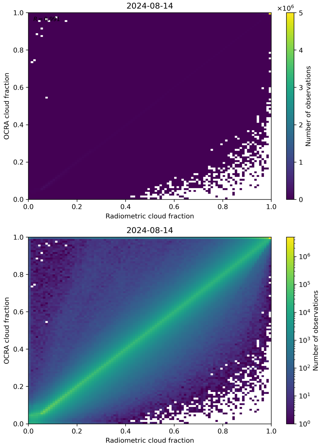
Figure 72: Scatter density plot of “Radiometric cloud fraction” against “OCRA cloud fraction” for 2024-08-13 to 2024-08-15.
