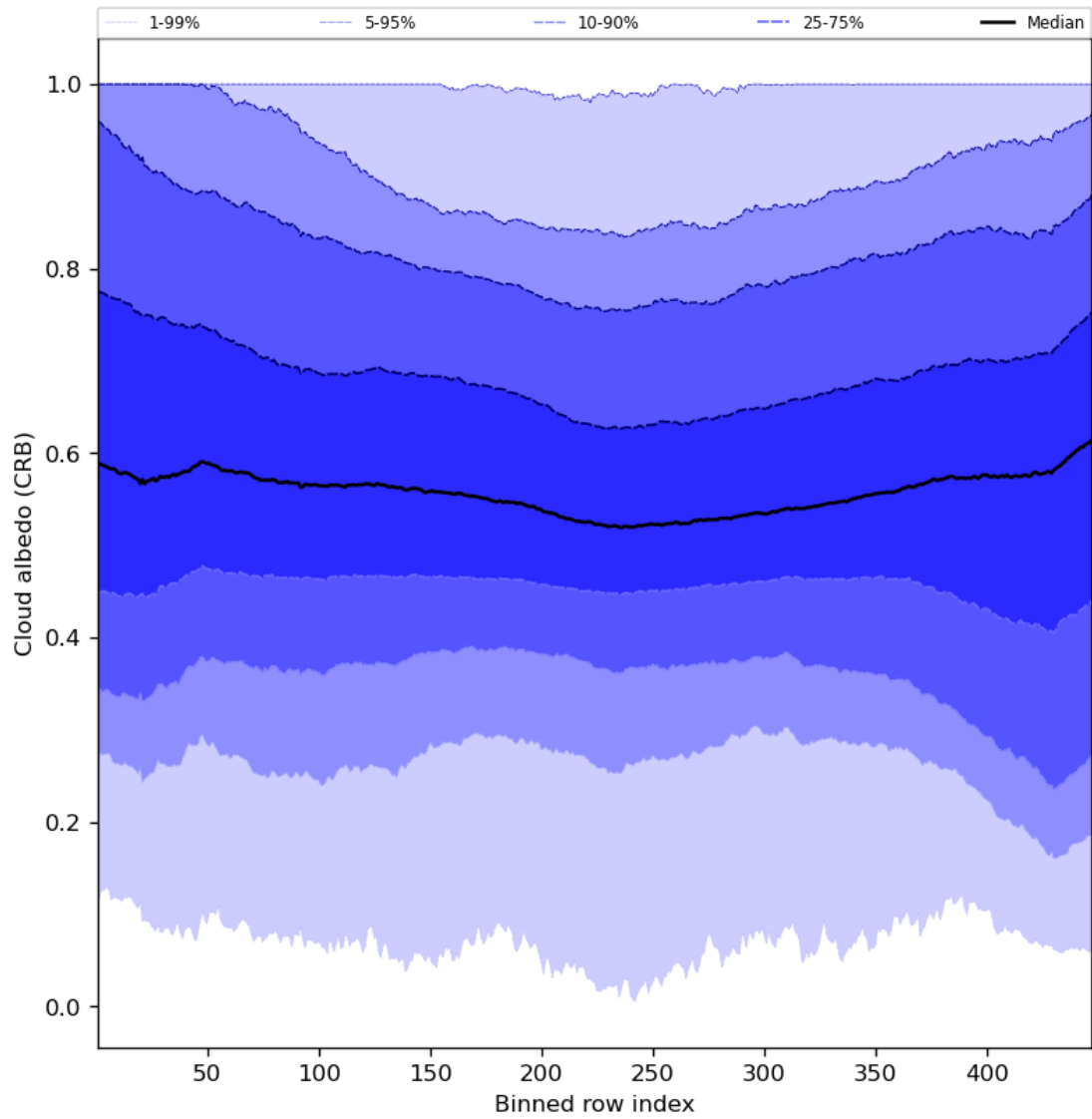
Figure 60: Along track statistics of “Cloud albedo (CRB)” for 2024-08-13 to 2024-08-15
