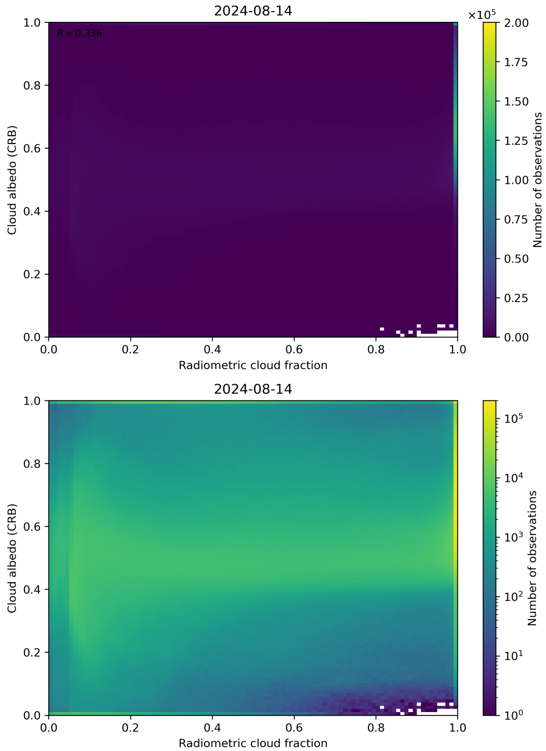
Figure 71: Scatter density plot of “Radiometric cloud fraction” against “Cloud albedo (CRB)” for 2024-08-13 to 2024-08-15.
