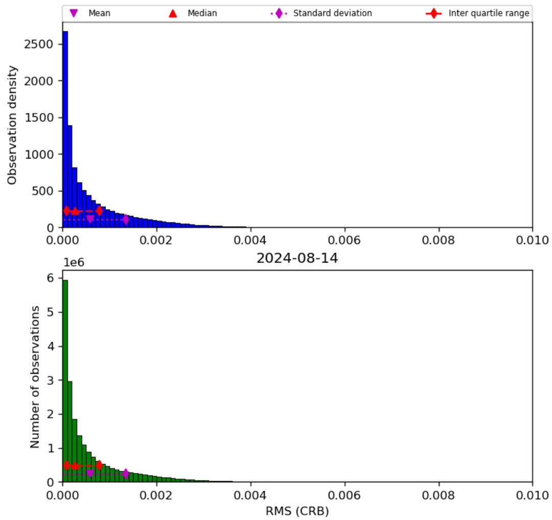
Figure 48: Histogram of “RMS (CRB)” for 2024-08-13 to 2024-08-15
