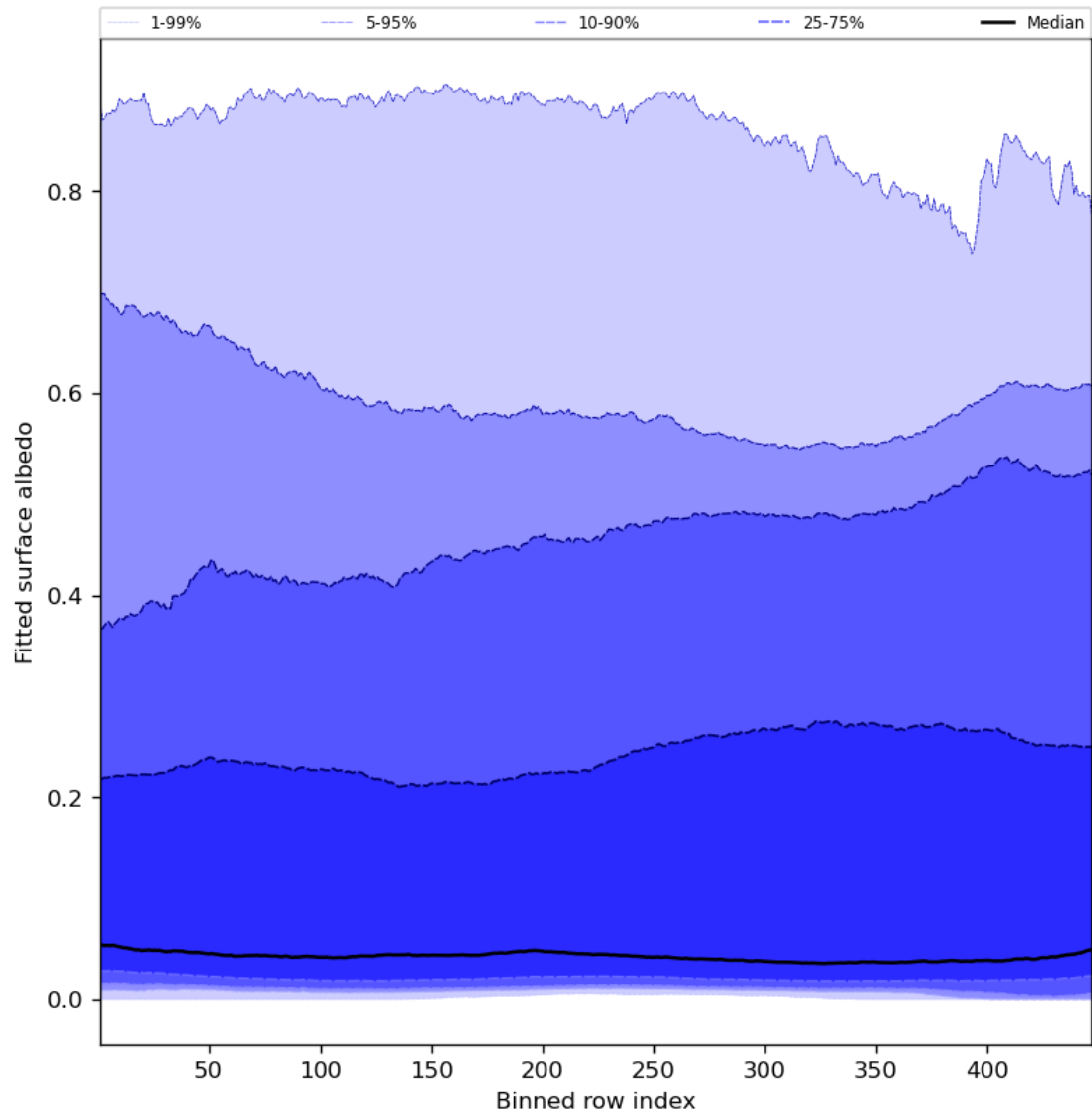
Figure 61: Along track statistics of “Fitted surface albedo” for 2024-08-13 to 2024-08-15
