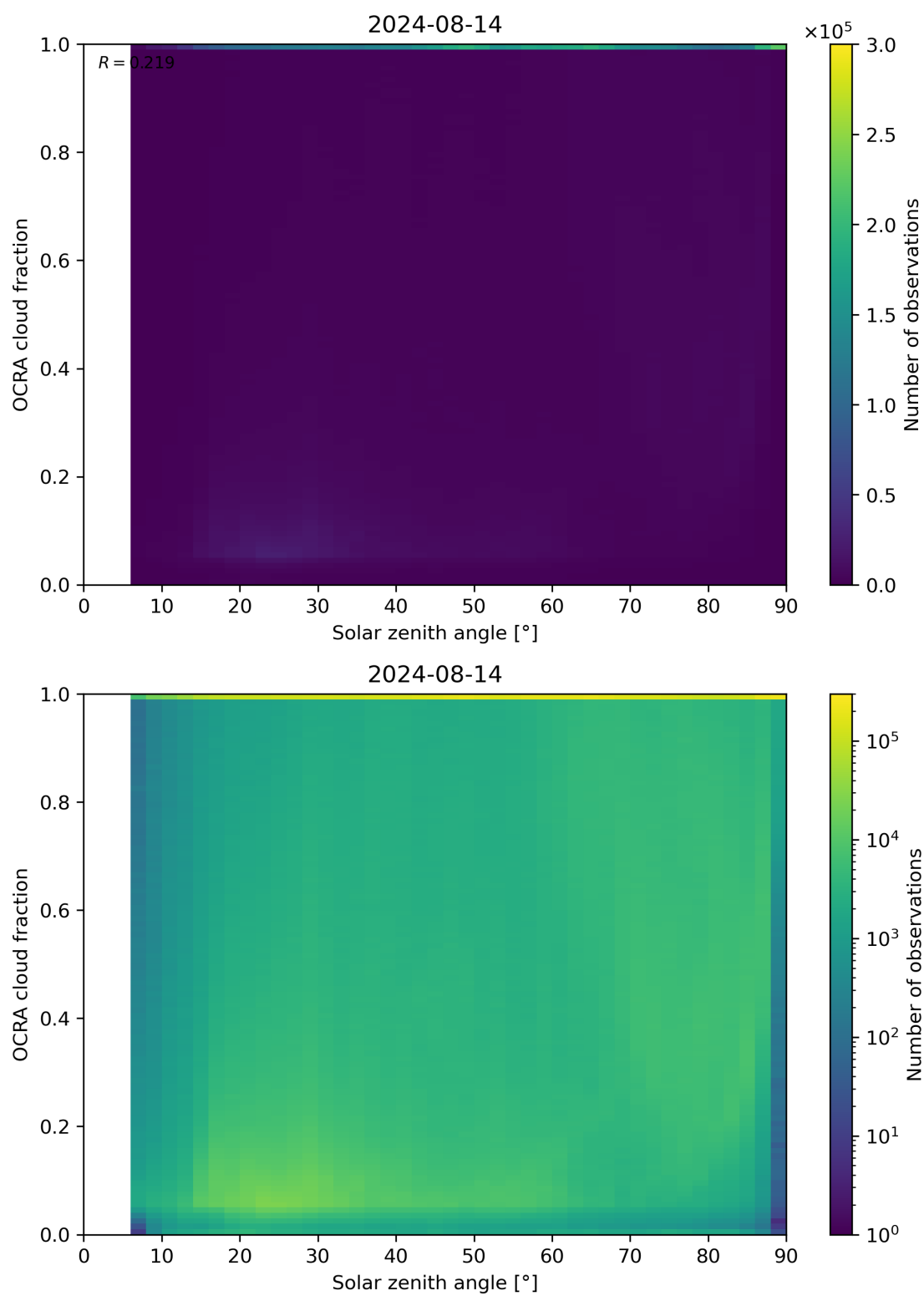
Figure 100: Scatter density plot of “Solar zenith angle” against “OCRA cloud fraction” for 2024-08-13 to 2024-08-15.
