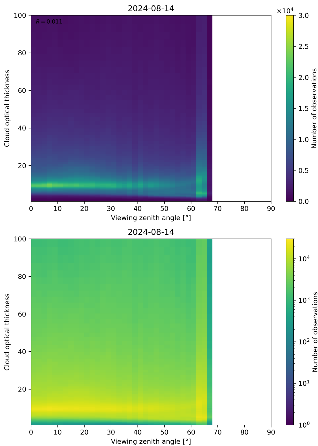
Figure 111: Scatter density plot of “Viewing zenith angle” against “Cloud optical thickness” for 2024-08-13 to 2024-08-15.
