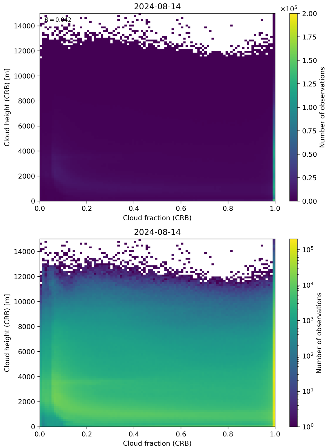
Figure 79: Scatter density plot of “Cloud fraction (CRB)” against “Cloud height (CRB)” for 2024-08-13 to 2024-08-15.
