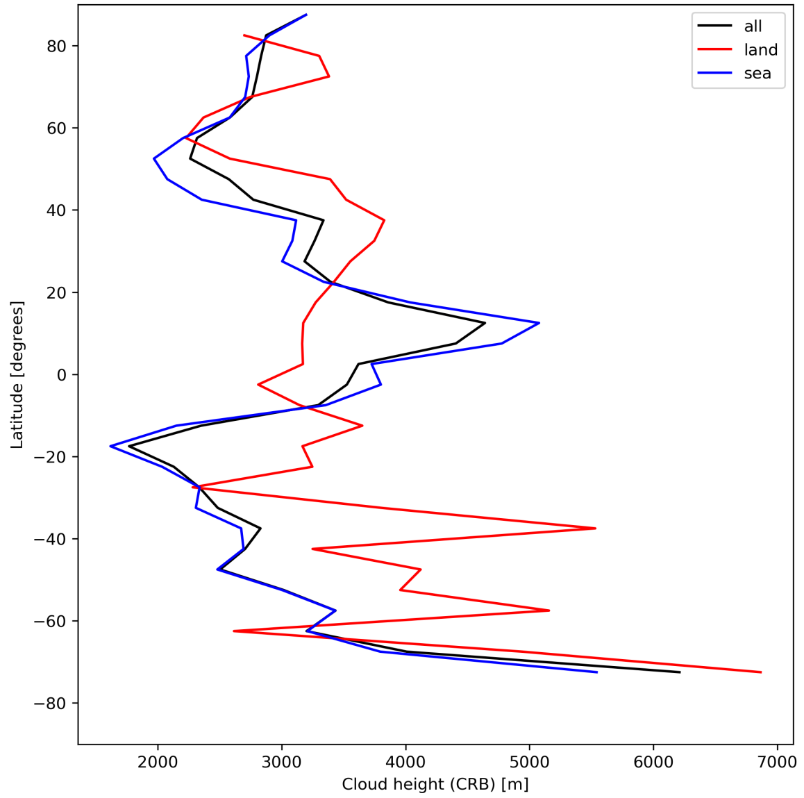
Figure 27: Zonal average of “Cloud height (CRB)” for 2024-08-13 to 2024-08-15.
