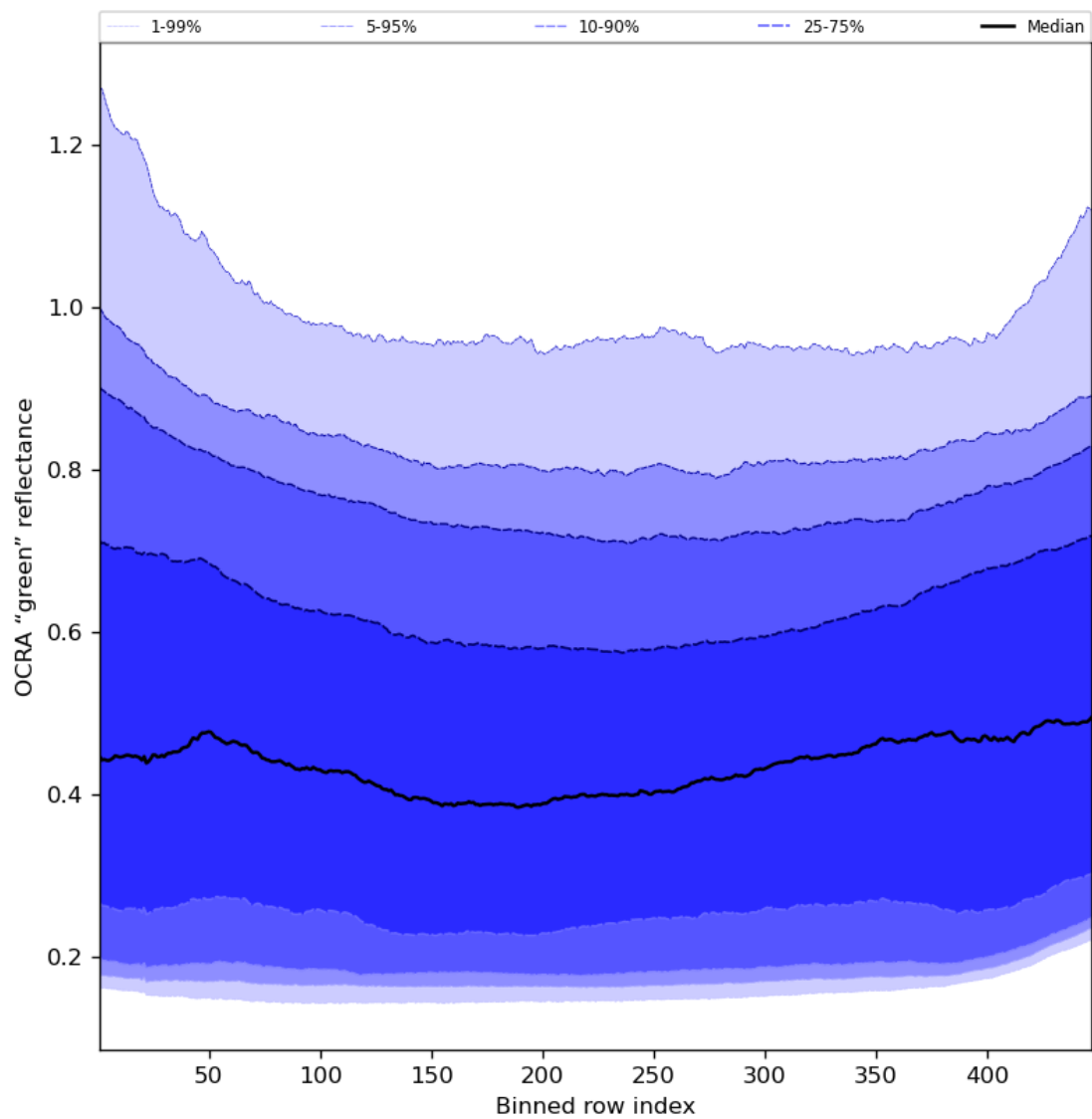
Figure 68: Along track statistics of “OCRA “green” reflectance” for 2024-08-13 to 2024-08-15
