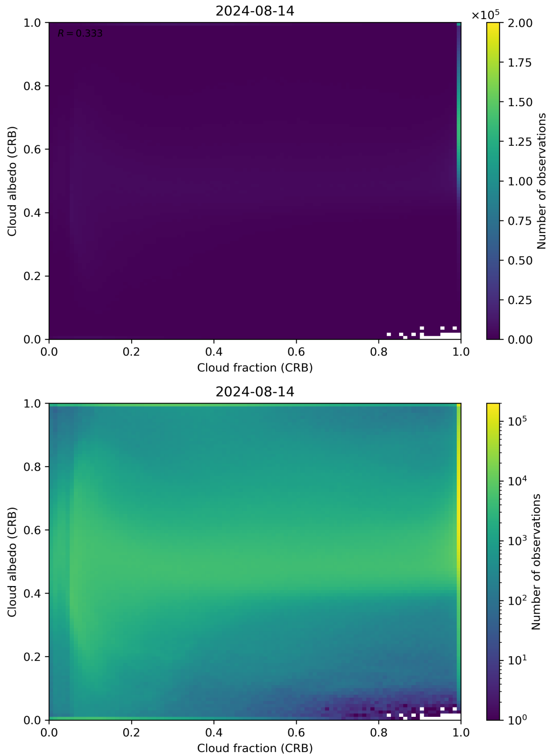
Figure 77: Scatter density plot of “Cloud fraction (CRB)” against “Cloud albedo (CRB)” for 2024-08-13 to 2024-08-15.
