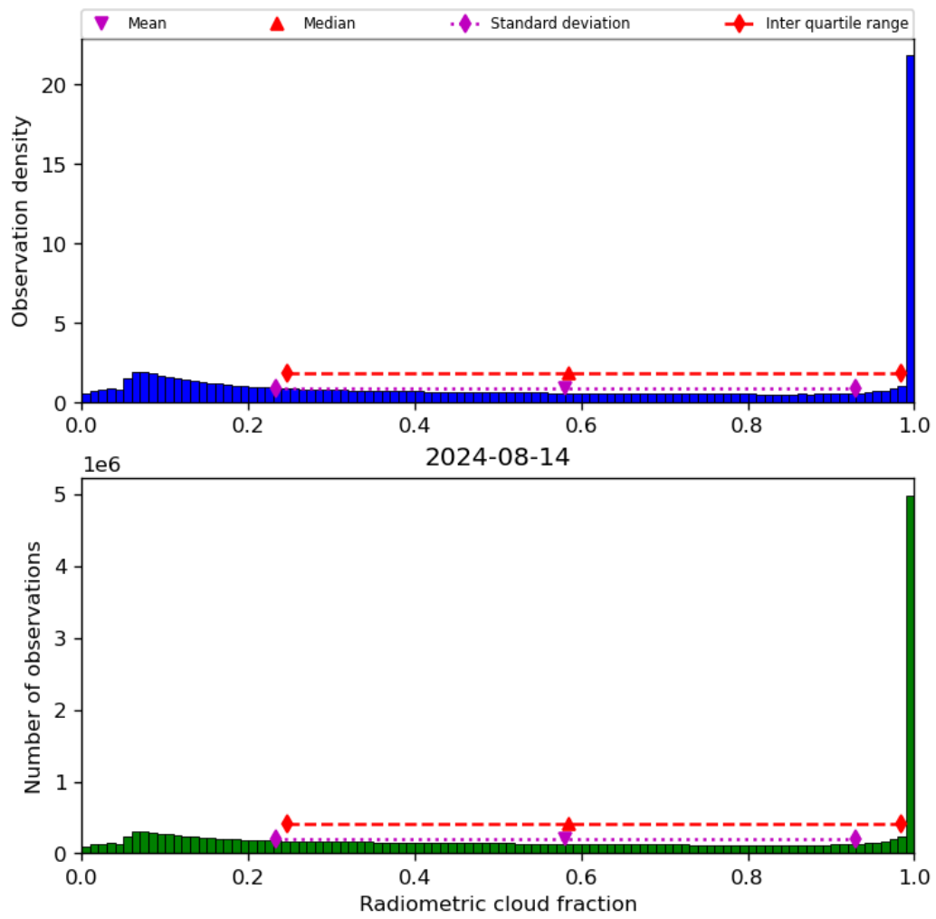
Figure 39: Histogram of “Radiometric cloud fraction” for 2024-08-13 to 2024-08-15
