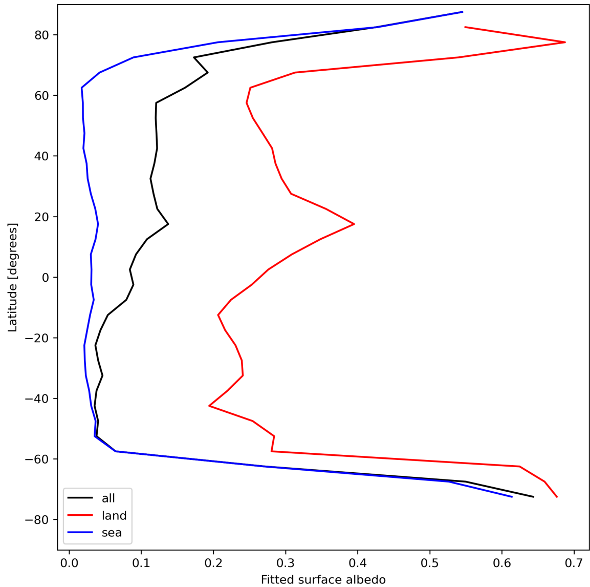
Figure 29: Zonal average of “Fitted surface albedo” for 2024-08-13 to 2024-08-15.
