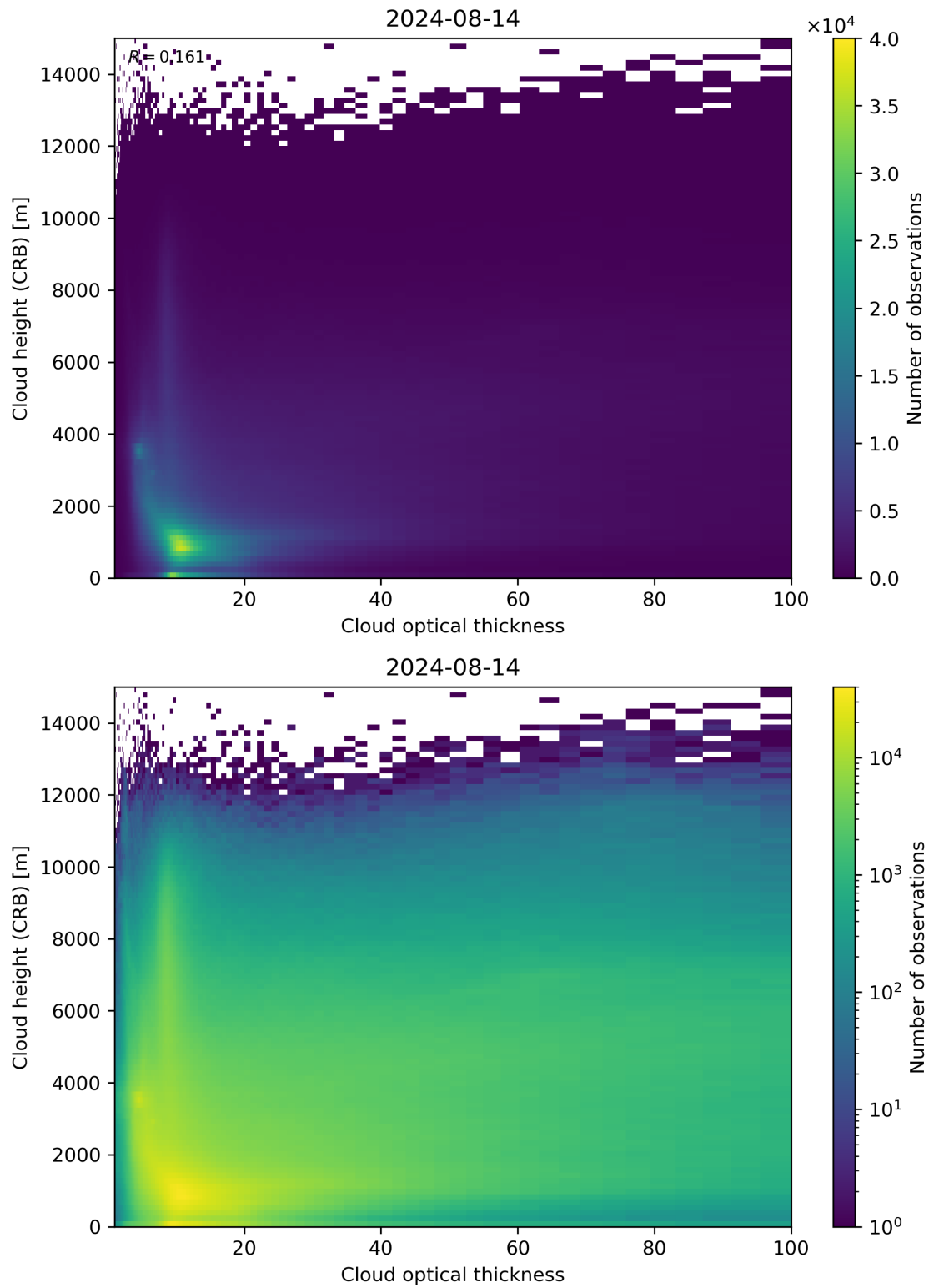
Figure 85: Scatter density plot of “Cloud optical thickness” against “Cloud height (CRB)” for 2024-08-13 to 2024-08-15.
