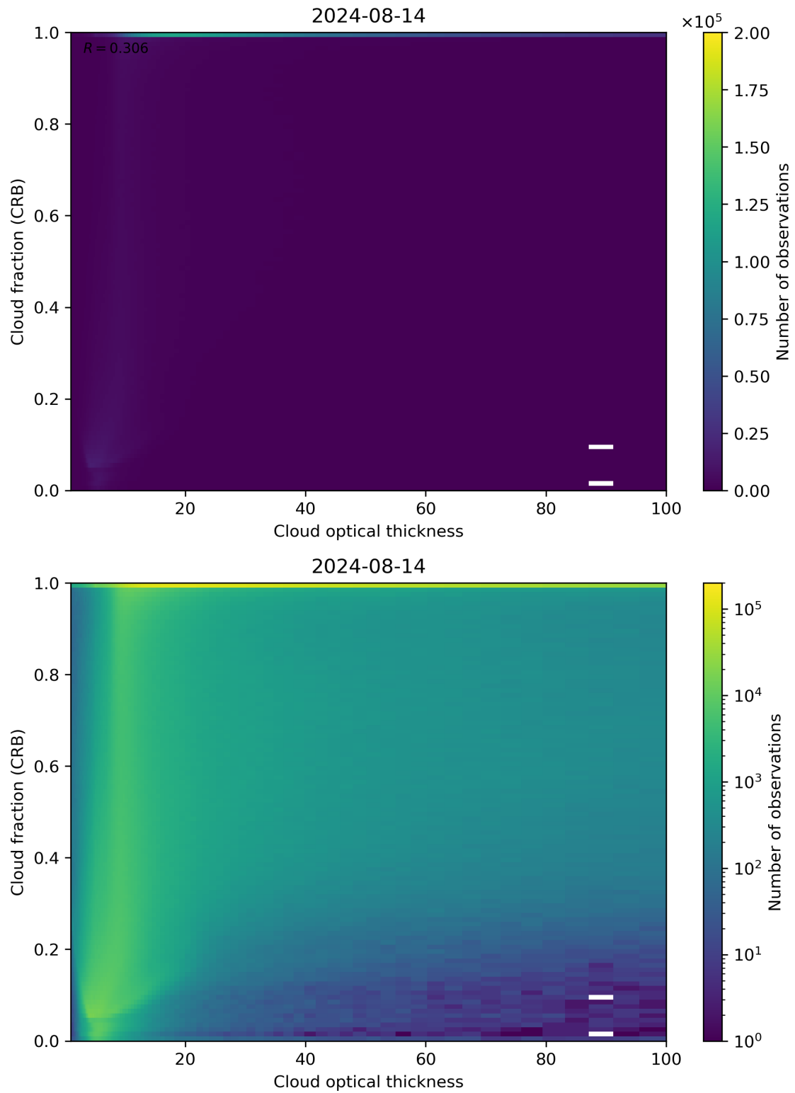
Figure 84: Scatter density plot of “Cloud optical thickness” against “Cloud fraction (CRB)” for 2024-08-13 to 2024-08-15.
