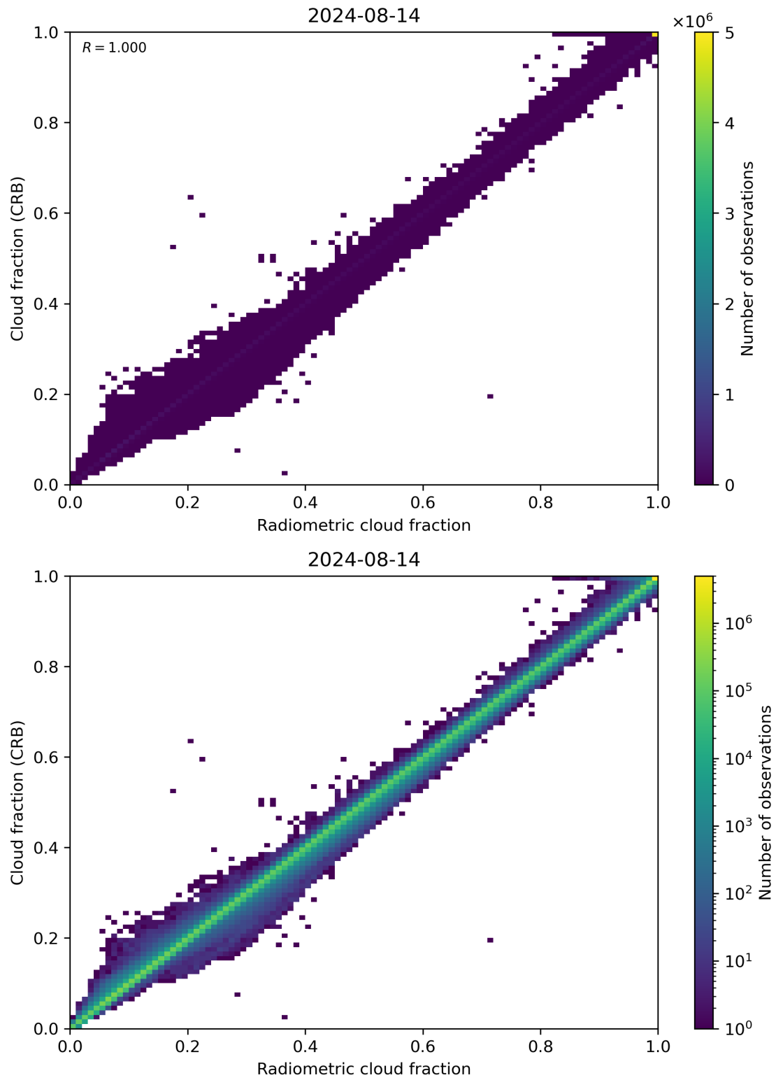
Figure 73: Scatter density plot of “Radiometric cloud fraction” against “Cloud fraction (CRB)” for 2024-08-13 to 2024-08-15.
