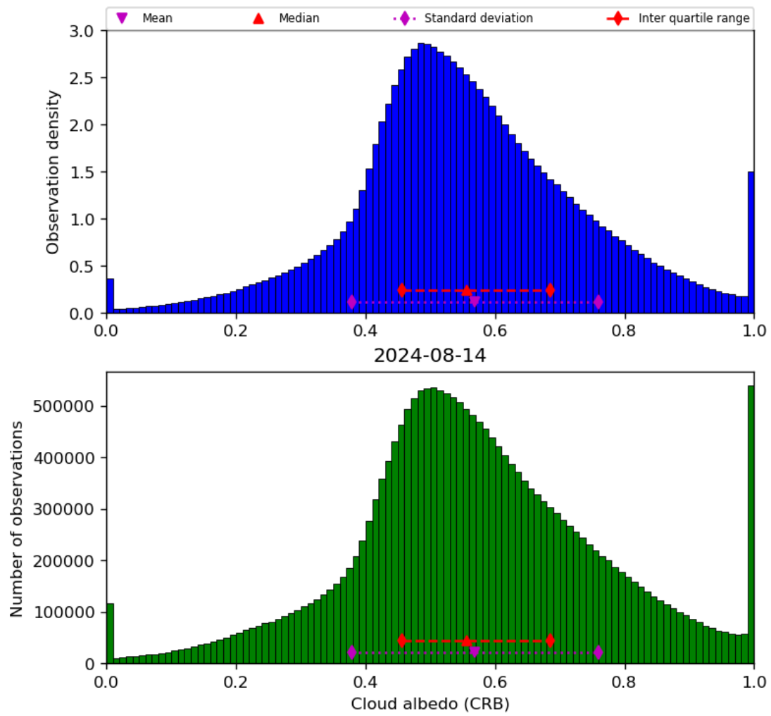
Figure 44: Histogram of “Cloud albedo (CRB)” for 2024-08-13 to 2024-08-15
