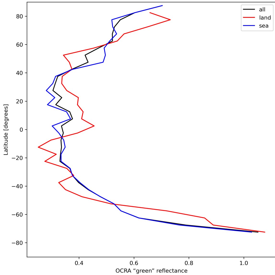
Figure 36: Zonal average of “OCRA “green” reflectance” for 2024-08-13 to 2024-08-15.
