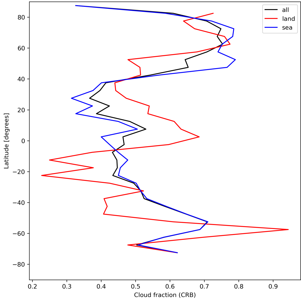
Figure 26: Zonal average of “Cloud fraction (CRB)” for 2024-08-13 to 2024-08-15.
