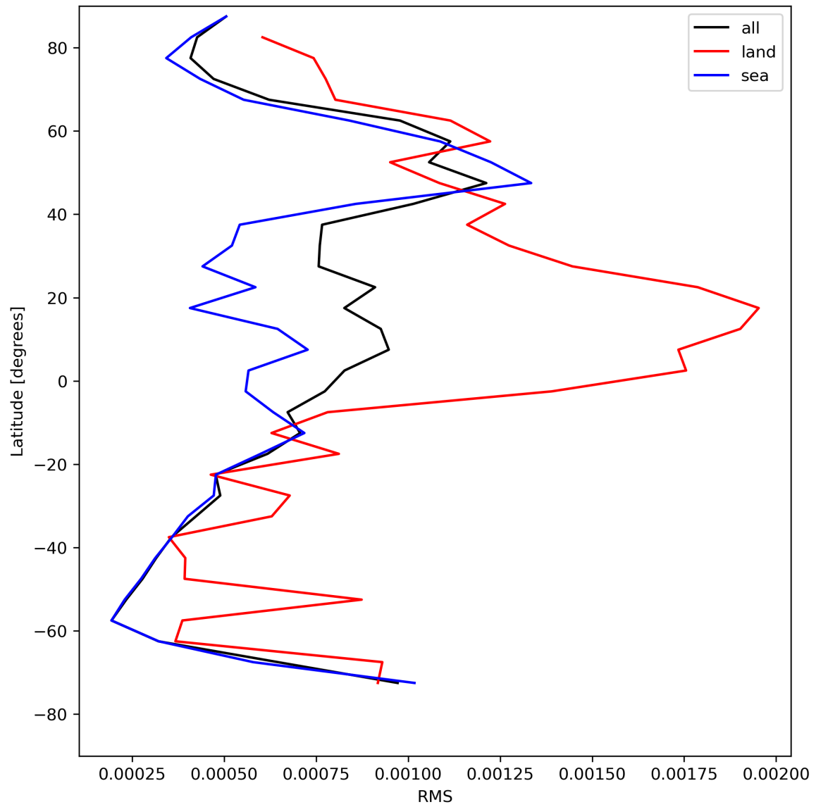
Figure 31: Zonal average of “RMS” for 2024-08-13 to 2024-08-15.
