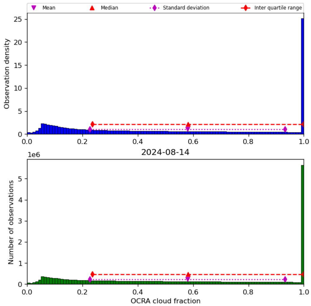
Figure 50: Histogram of “OCRA cloud fraction” for 2024-08-13 to 2024-08-15
