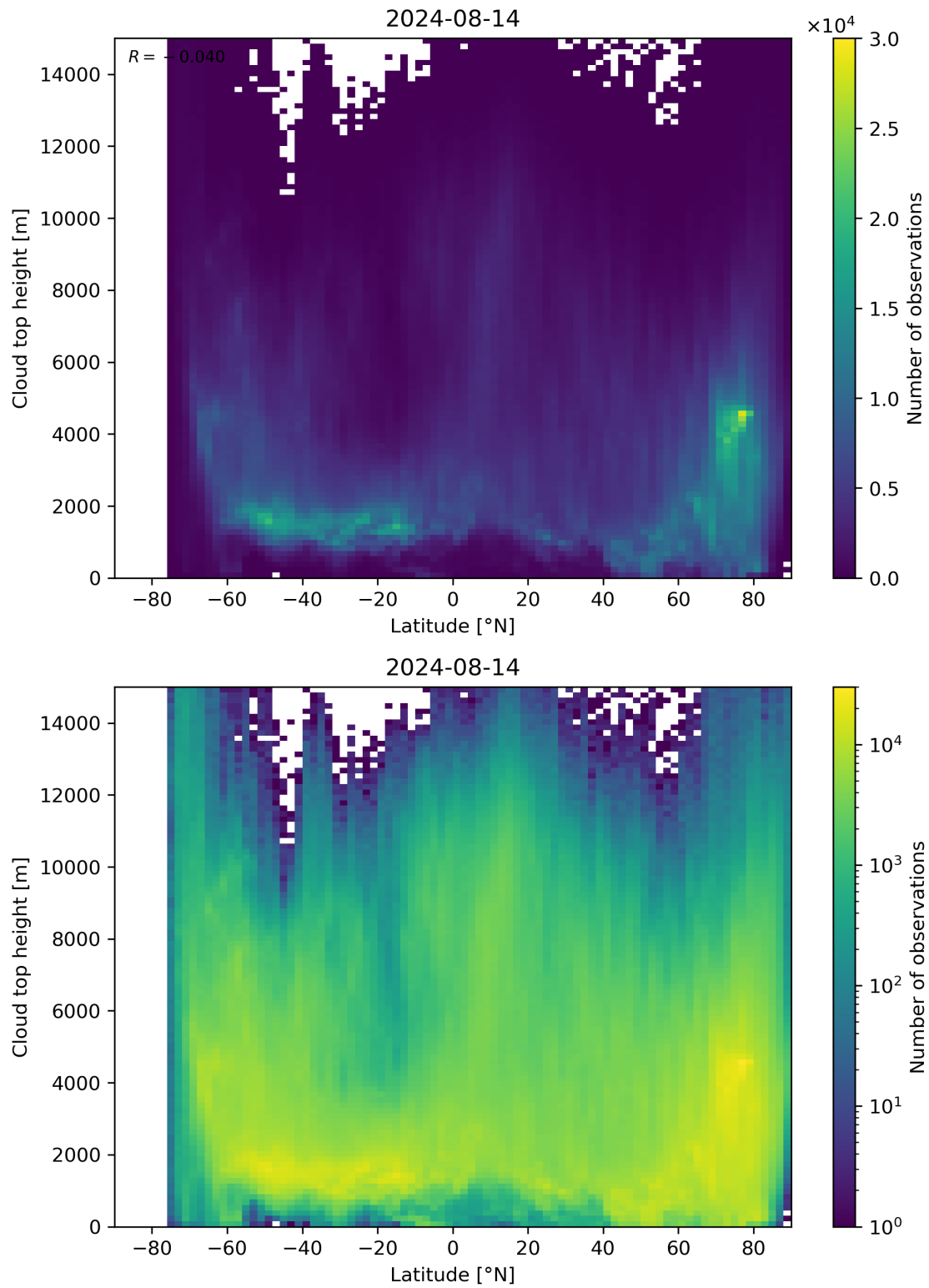
Figure 97: Scatter density plot of “Latitude” against “Cloud top height” for 2024-08-13 to 2024-08-15.
