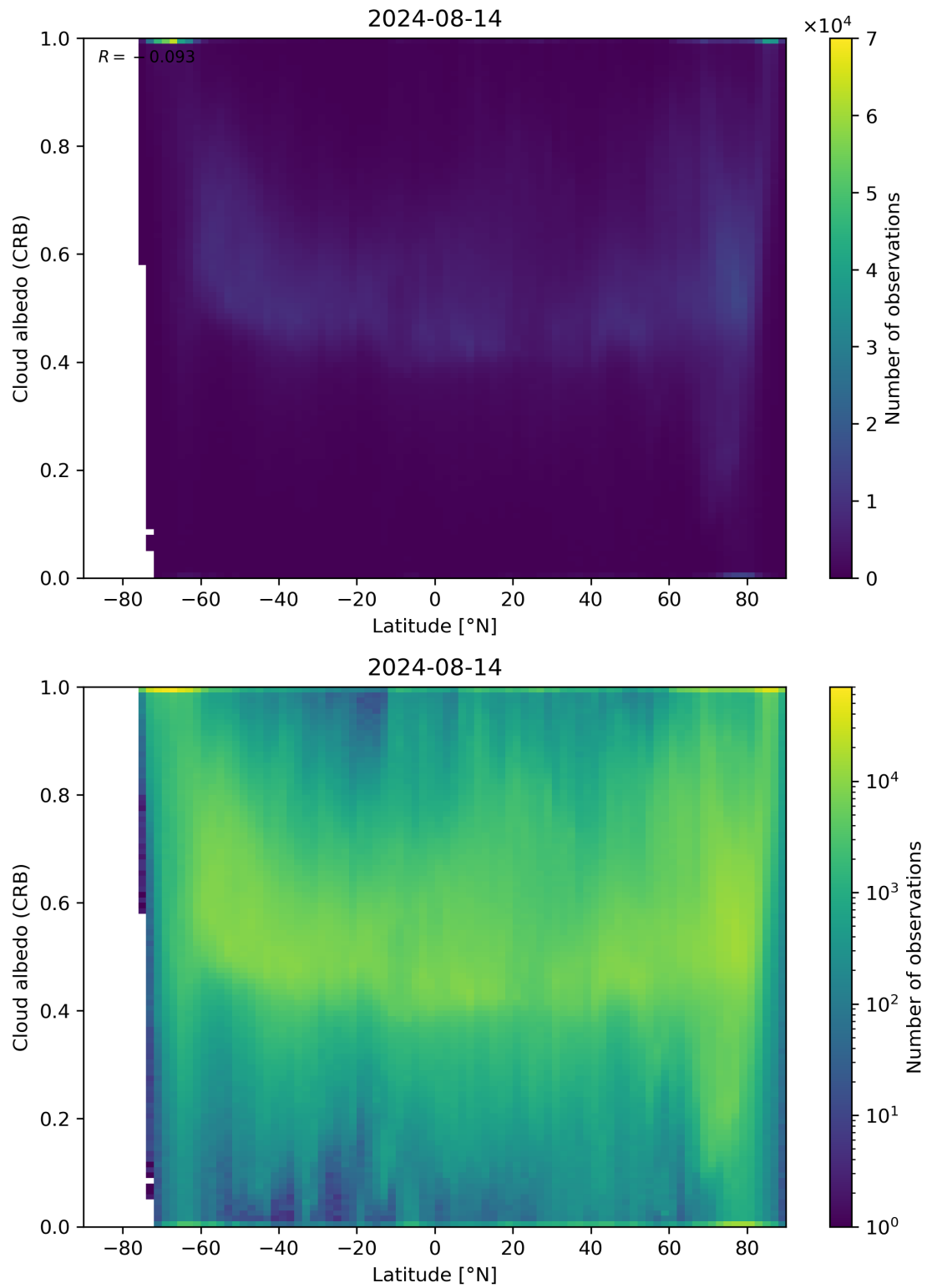
Figure 91: Scatter density plot of “Latitude” against “Cloud albedo (CRB)” for 2024-08-13 to 2024-08-15.
