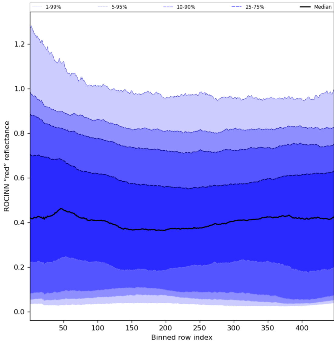
Figure 69: Along track statistics of “ROCINN “red” reflectance” for 2024-08-13 to 2024-08-15
