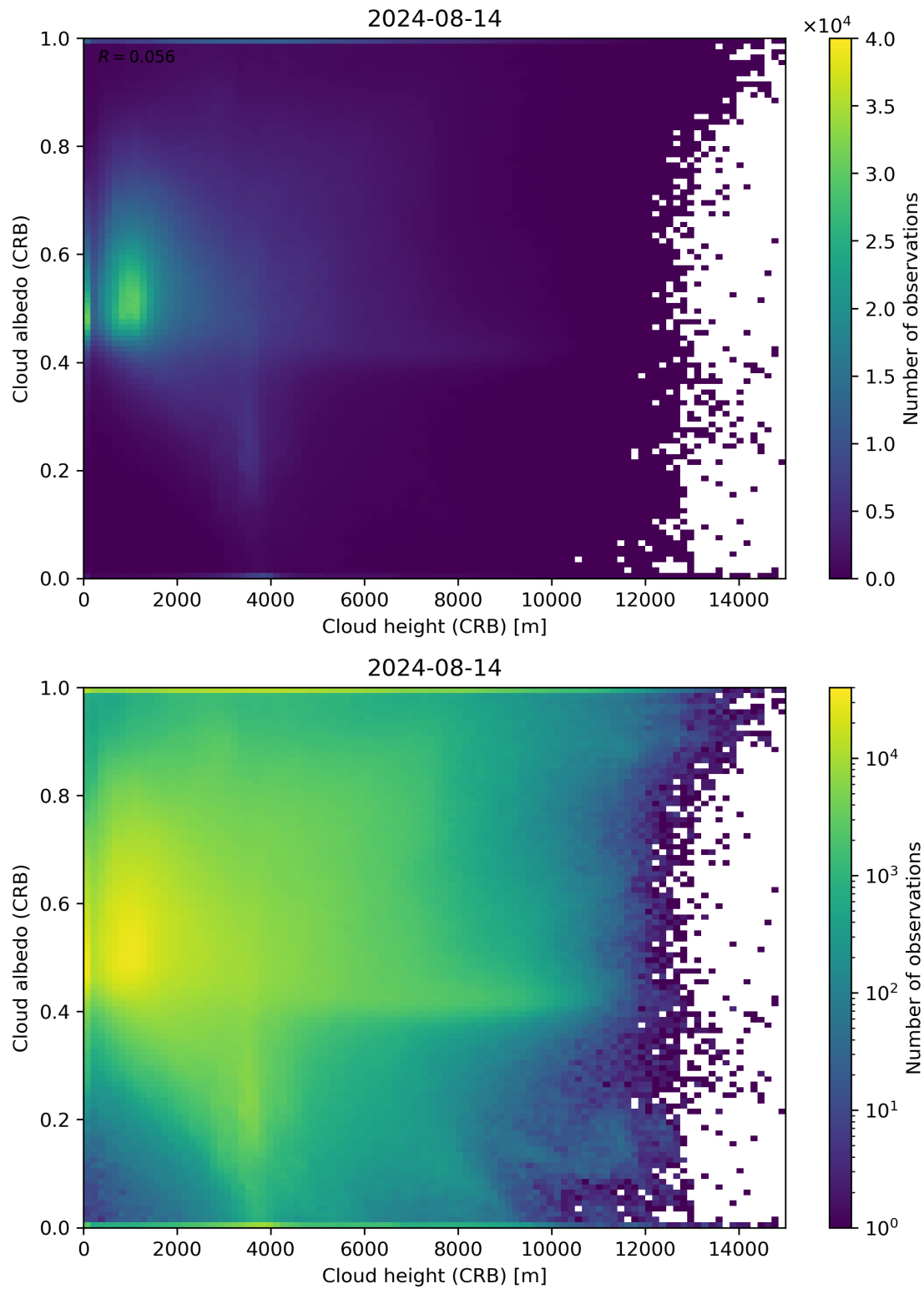
Figure 80: Scatter density plot of “Cloud height (CRB)” against “Cloud albedo (CRB)” for 2024-08-13 to 2024-08-15.
