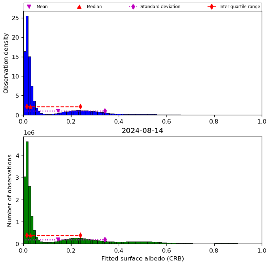
Figure 46: Histogram of “Fitted surface albedo (CRB)” for 2024-08-13 to 2024-08-15
