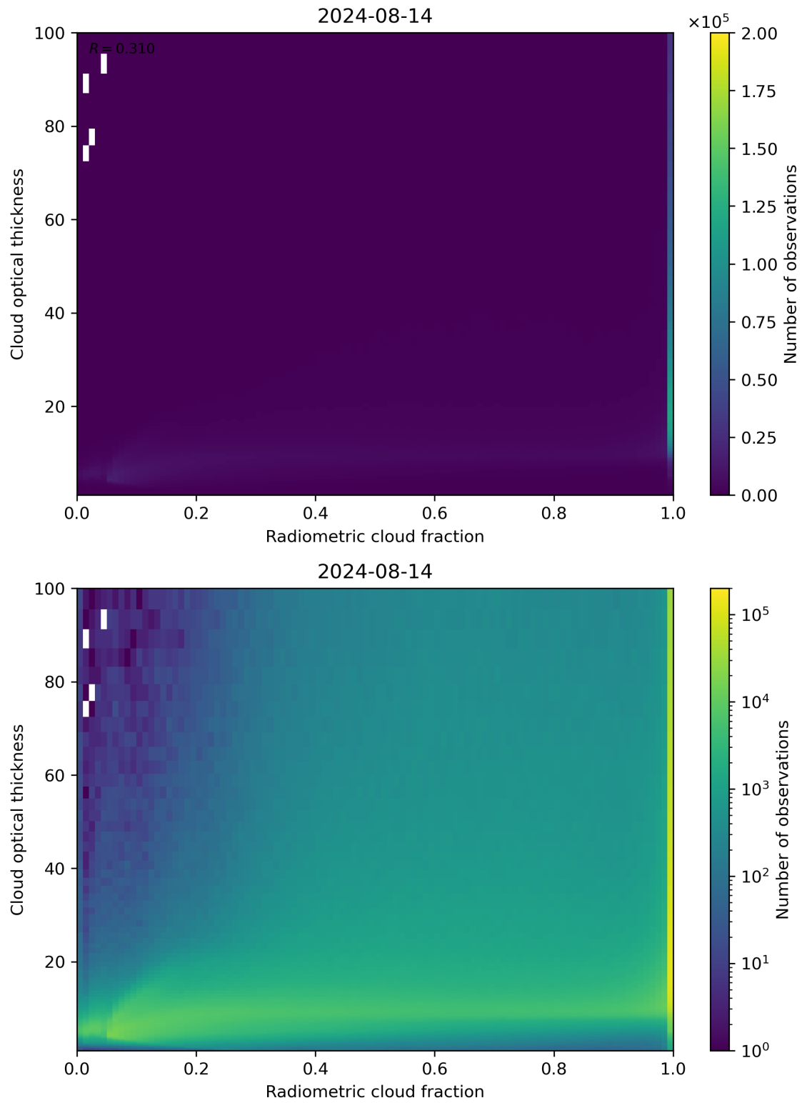
Figure 75: Scatter density plot of “Radiometric cloud fraction” against “Cloud optical thickness” for 2024-08-13 to 2024-08-15.
