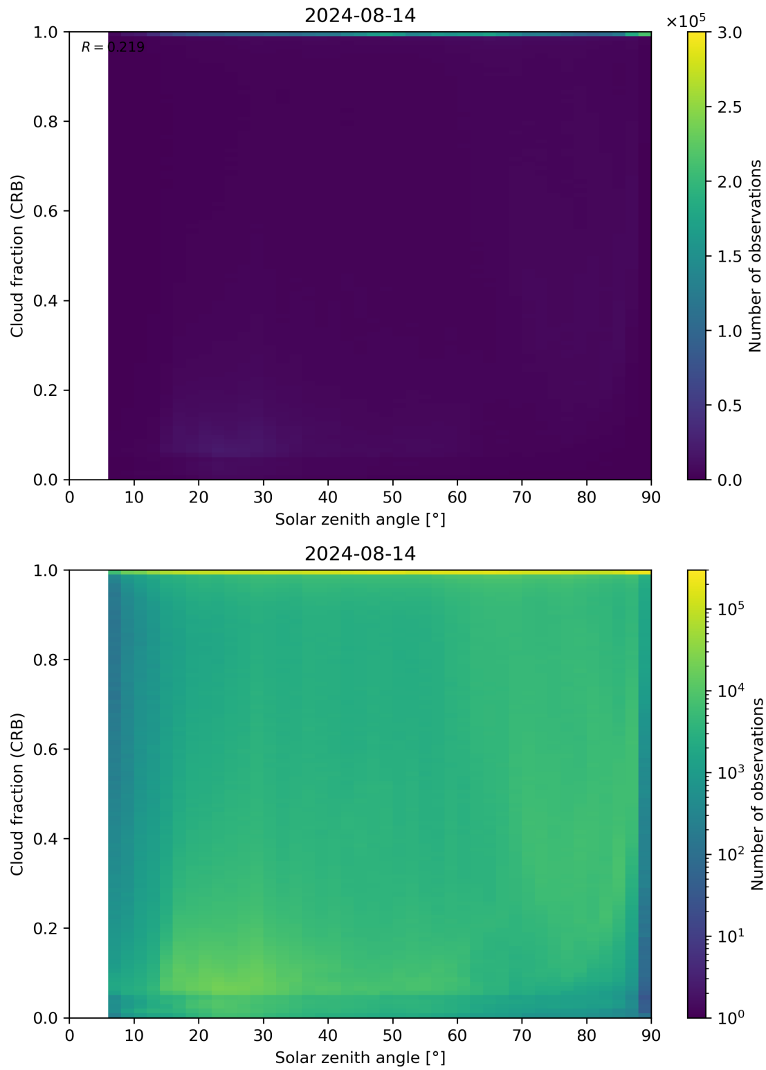
Figure 101: Scatter density plot of “Solar zenith angle” against “Cloud fraction (CRB)” for 2024-08-13 to 2024-08-15.
