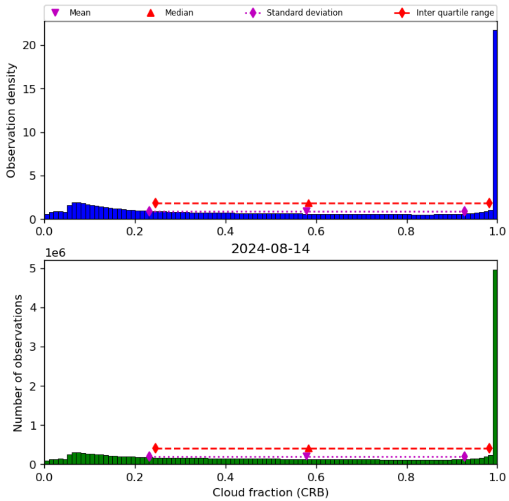
Figure 42: Histogram of “Cloud fraction (CRB)” for 2024-08-13 to 2024-08-15
