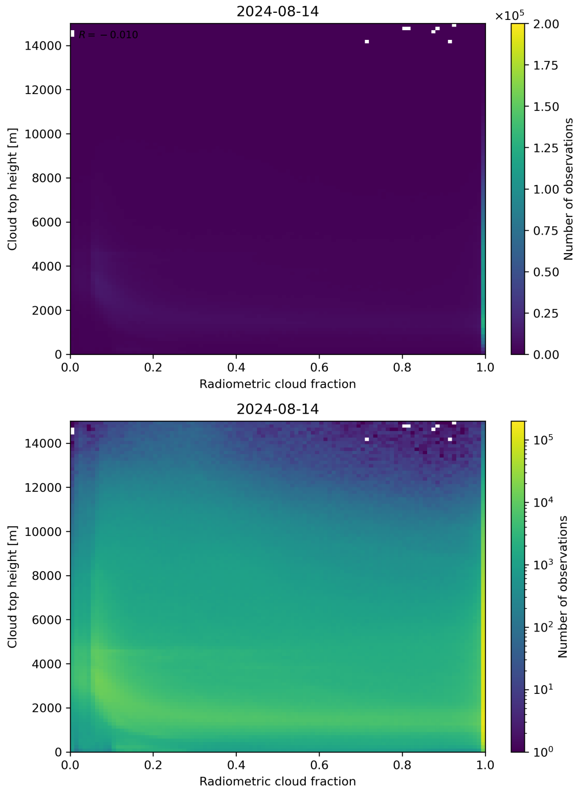
Figure 76: Scatter density plot of “Radiometric cloud fraction” against “Cloud top height” for 2024-08-13 to 2024-08-15.
