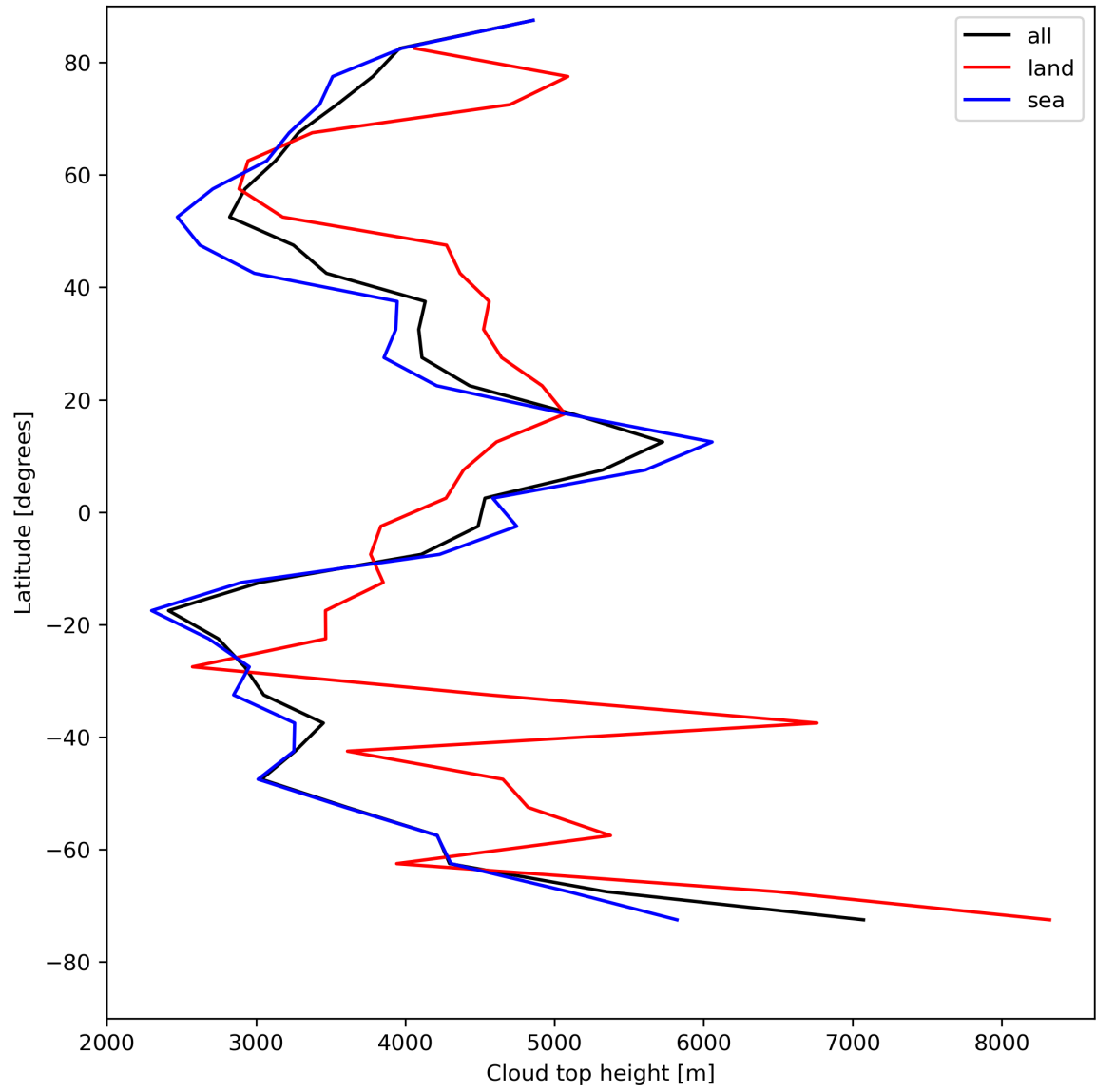
Figure 24: Zonal average of “Cloud top height” for 2024-08-13 to 2024-08-15.
