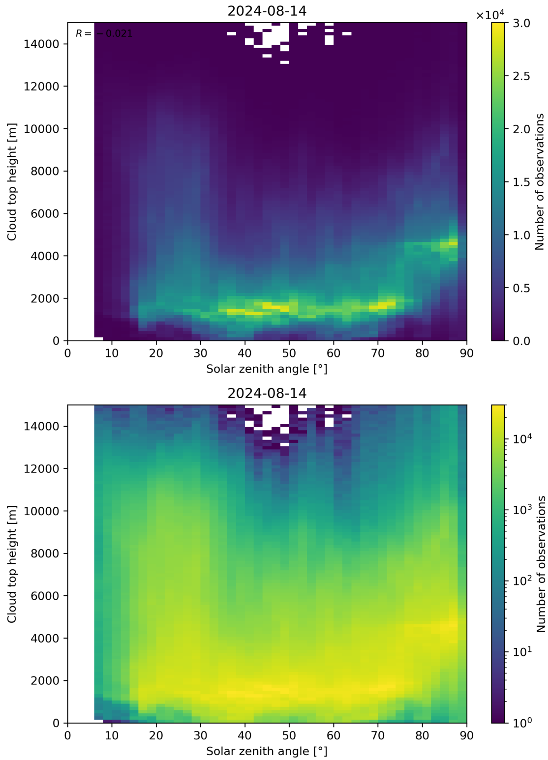
Figure 104: Scatter density plot of “Solar zenith angle” against “Cloud top height” for 2024-08-13 to 2024-08-15.
