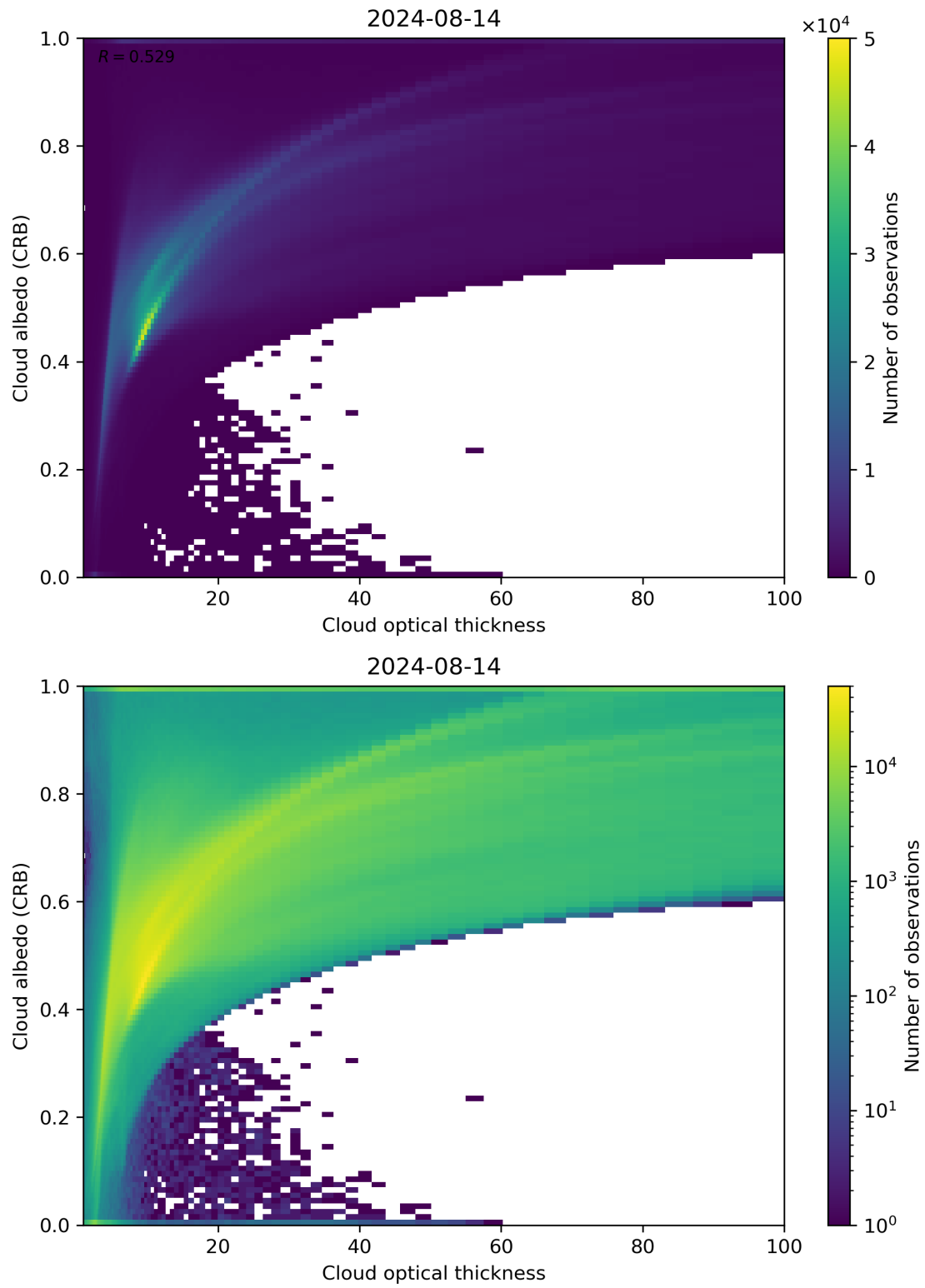
Figure 82: Scatter density plot of “Cloud optical thickness” against “Cloud albedo (CRB)” for 2024-08-13 to 2024-08-15.
