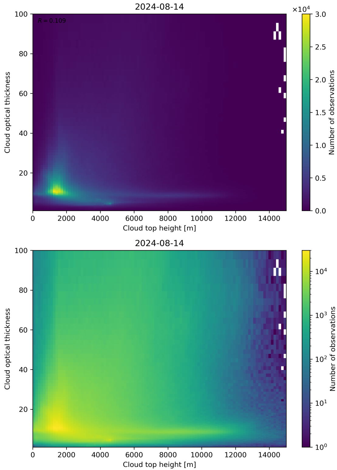
Figure 90: Scatter density plot of “Cloud top height” against “Cloud optical thickness” for 2024-08-13 to 2024-08-15.
