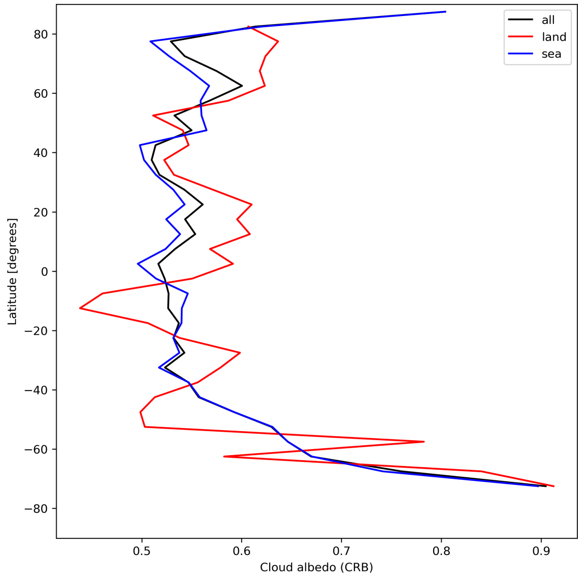
Figure 28: Zonal average of “Cloud albedo (CRB)” for 2024-08-13 to 2024-08-15.
