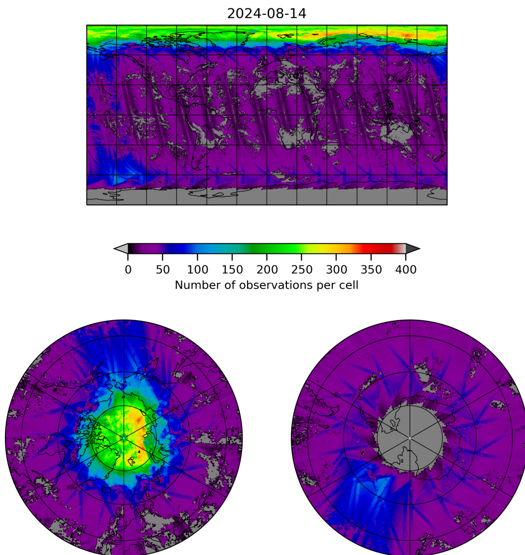
Figure 21: Map of the number of observations for 2024-08-13 to 2024-08-15
