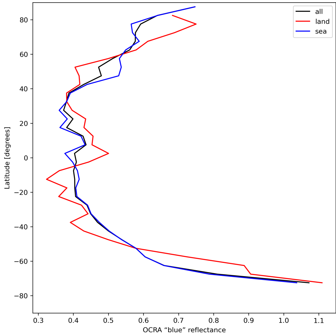
Figure 35: Zonal average of “OCRA “blue” reflectance” for 2024-08-13 to 2024-08-15.
