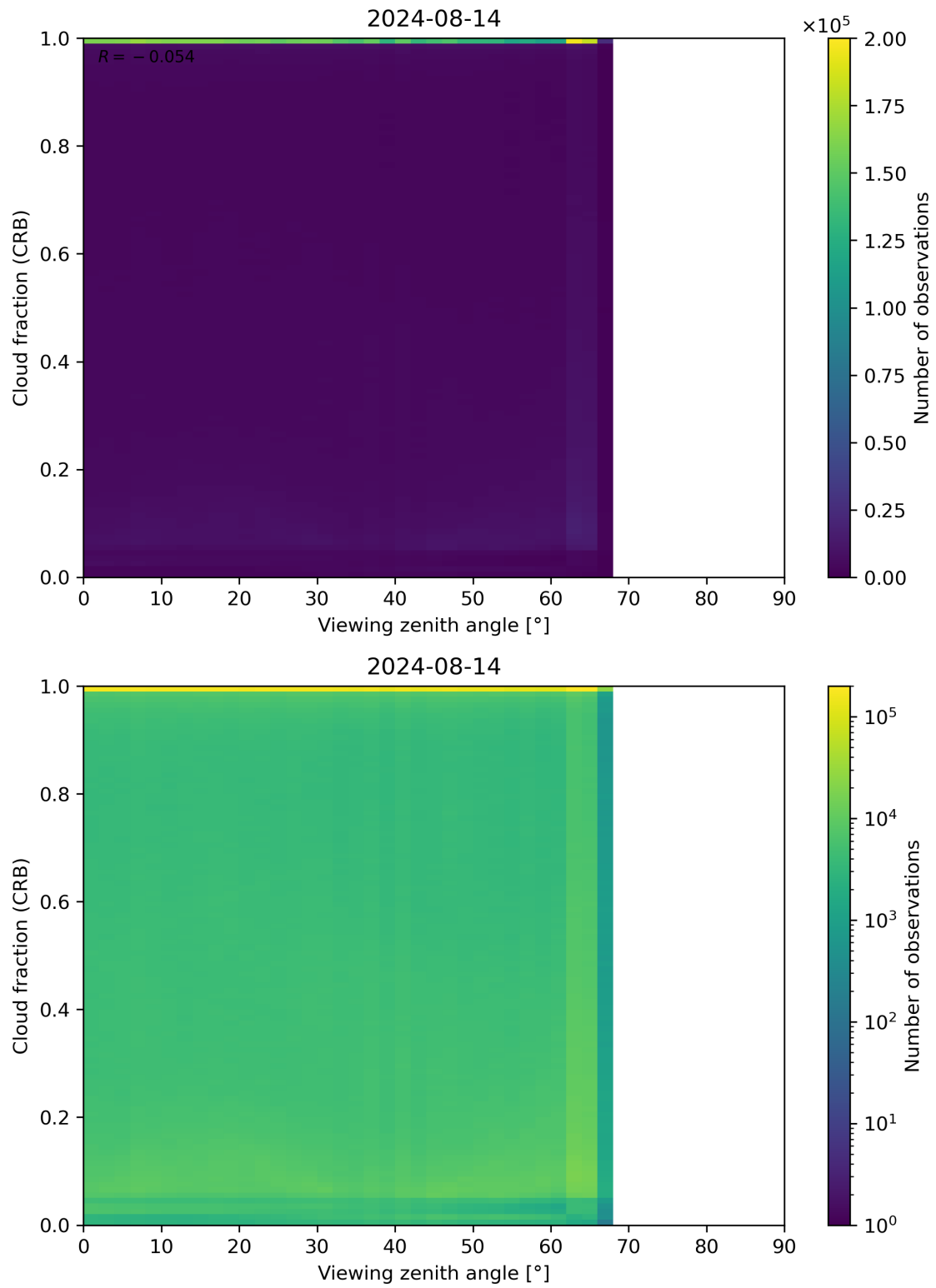
Figure 109: Scatter density plot of “Viewing zenith angle” against “Cloud fraction (CRB)” for 2024-08-13 to 2024-08-15.
