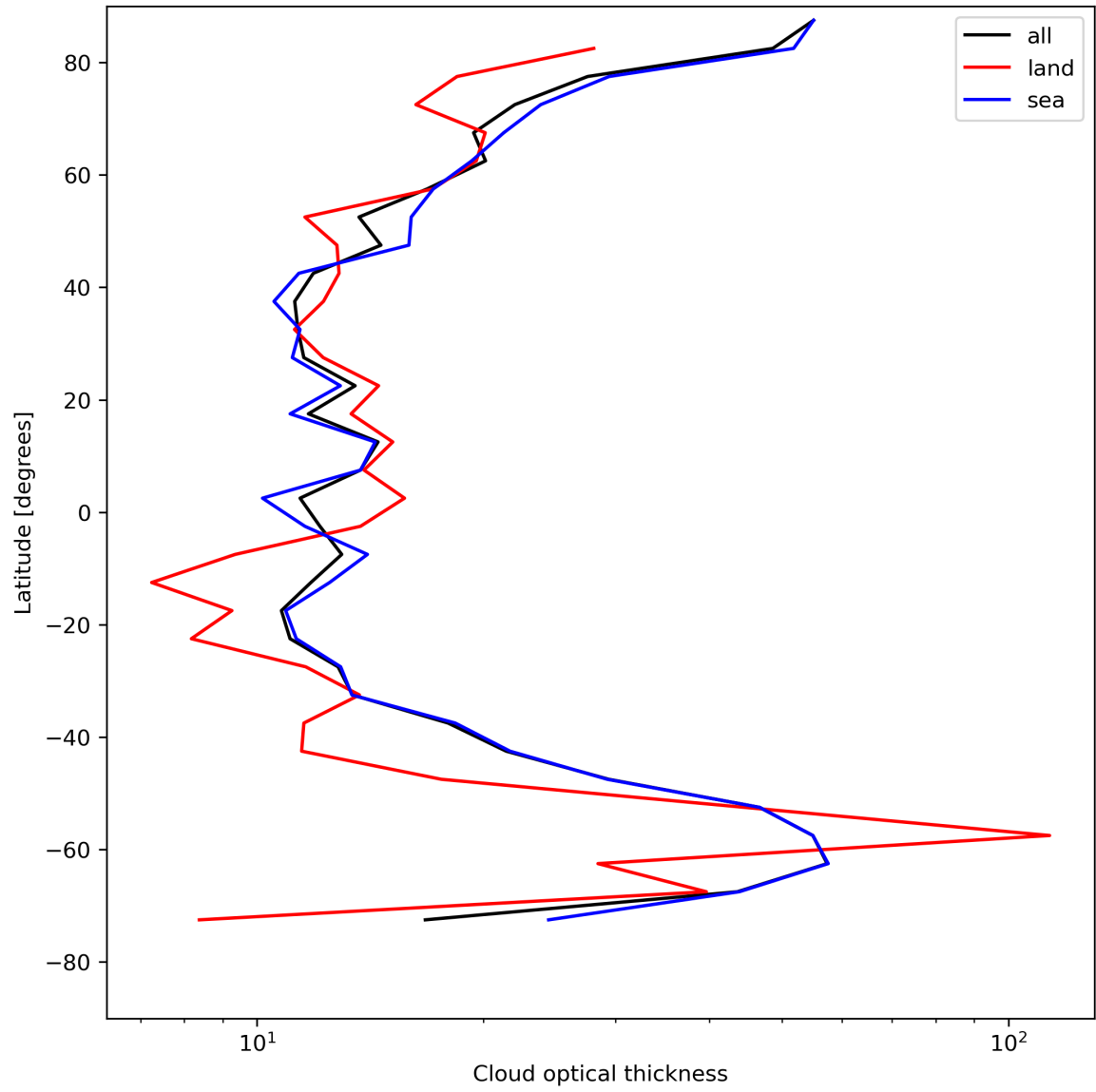
Figure 25: Zonal average of “Cloud optical thickness” for 2024-08-13 to 2024-08-15.
