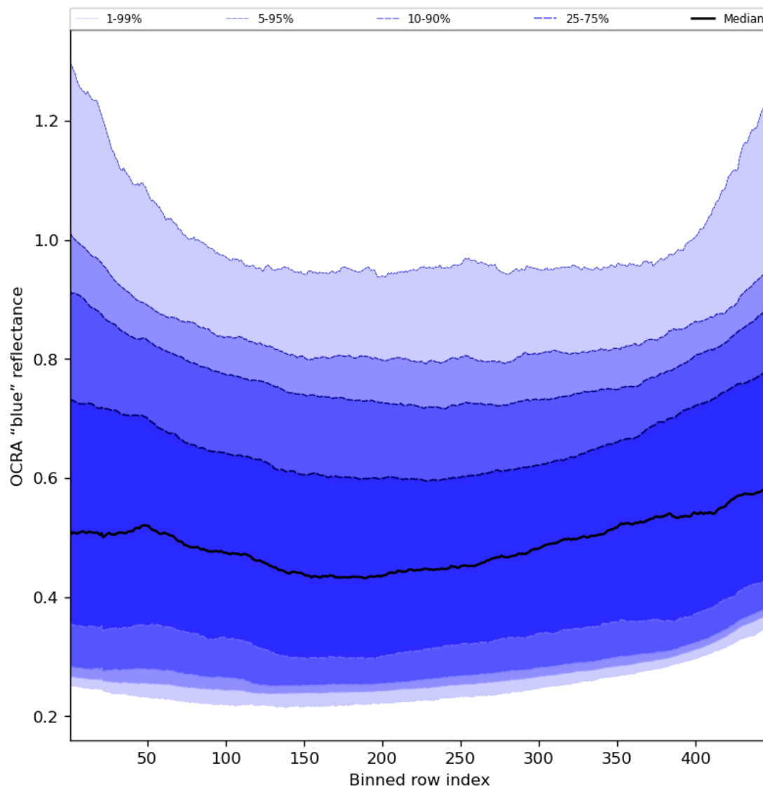
Figure 67: Along track statistics of “OCRA “blue” reflectance” for 2024-08-13 to 2024-08-15
