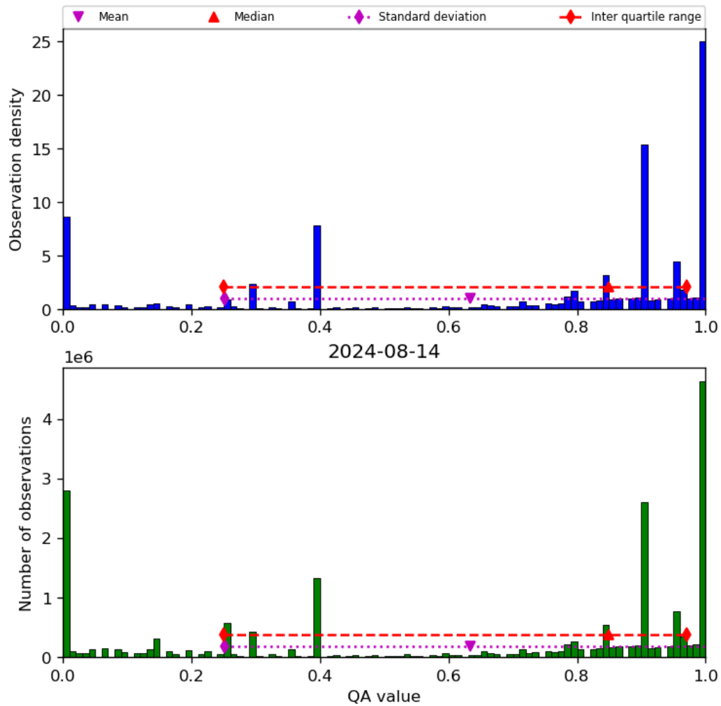
Figure 38: Histogram of “QA value” for 2024-08-13 to 2024-08-15
