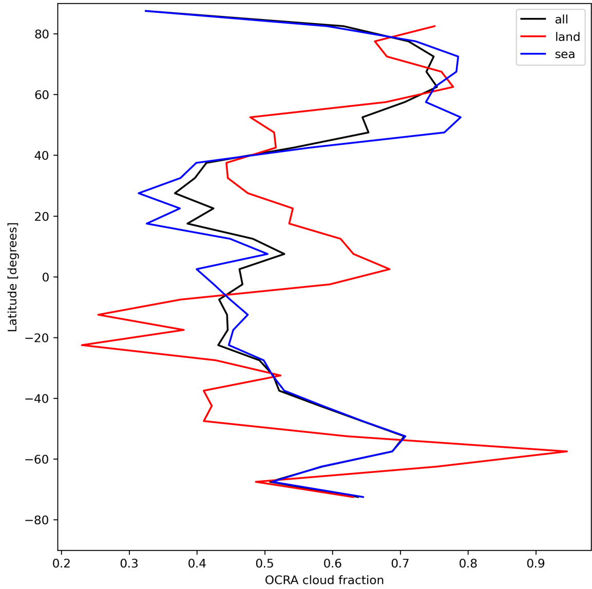
Figure 34: Zonal average of “OCRA cloud fraction” for 2024-08-13 to 2024-08-15.
