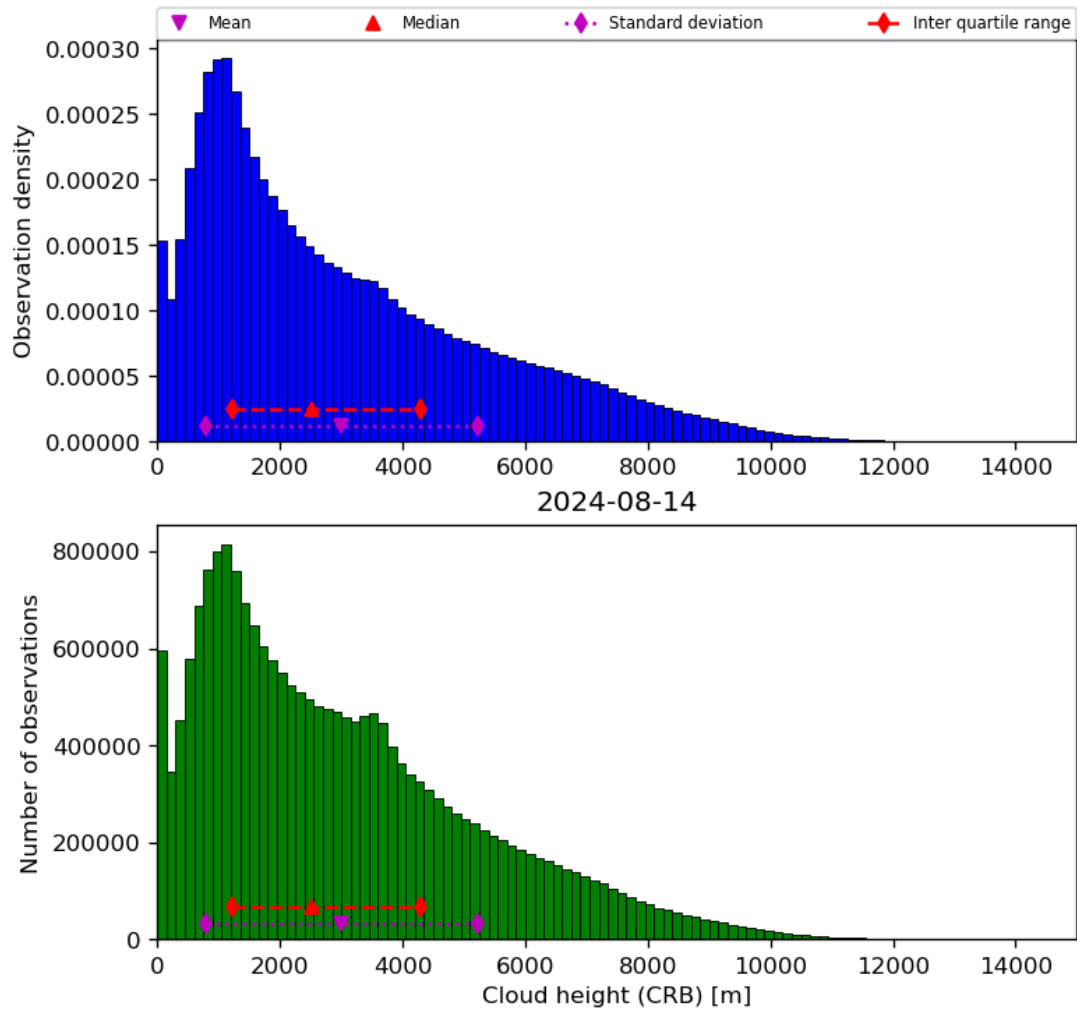
Figure 43: Histogram of “Cloud height (CRB)” for 2024-08-13 to 2024-08-15
