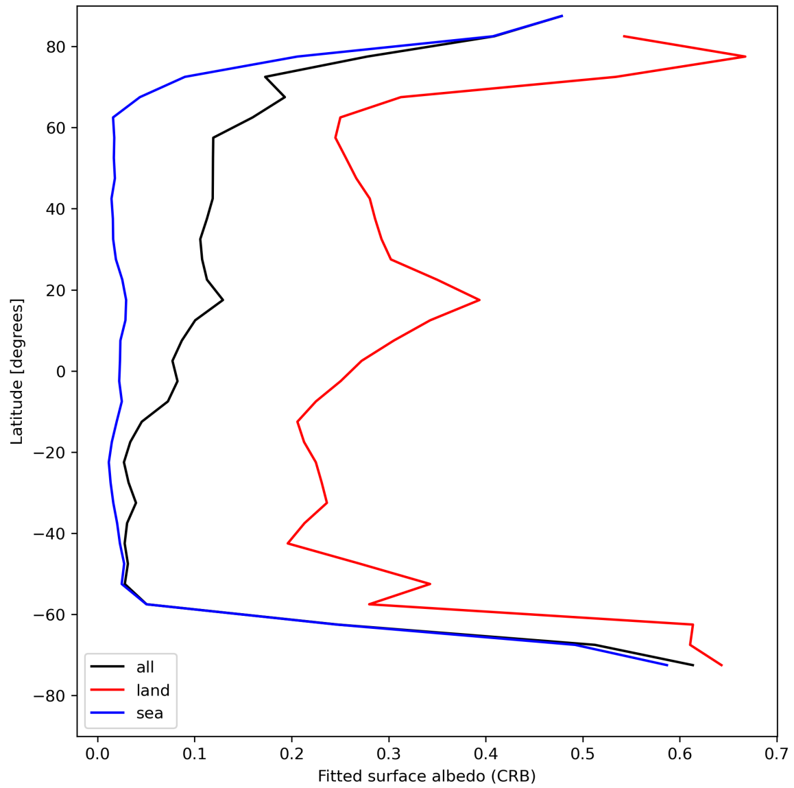
Figure 30: Zonal average of “Fitted surface albedo (CRB)” for 2024-08-13 to 2024-08-15.
