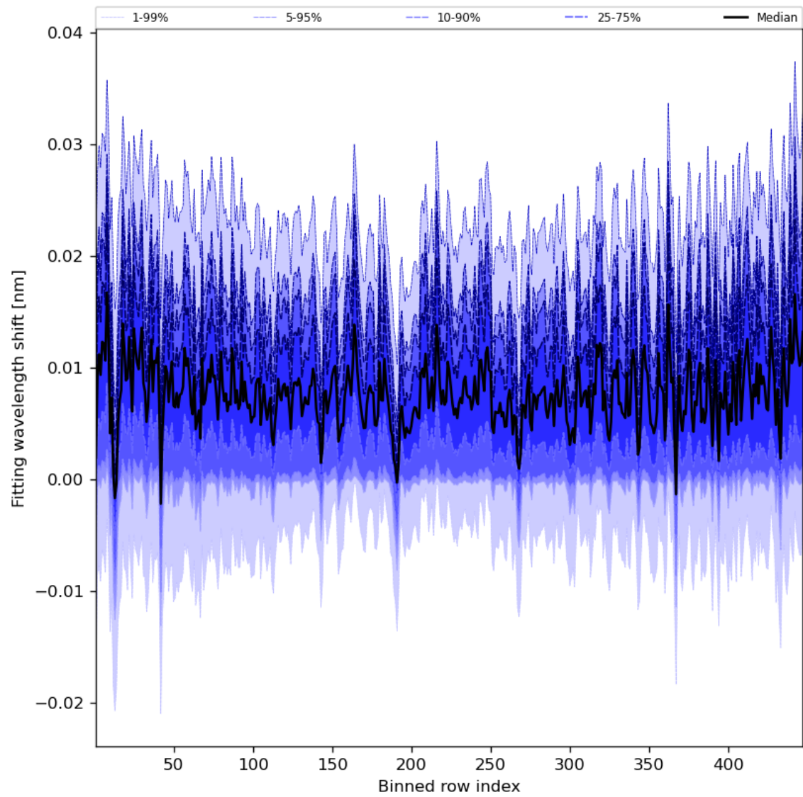
Figure 65: Along track statistics of “Fitting wavelength shift” for 2024-08-13 to 2024-08-15
