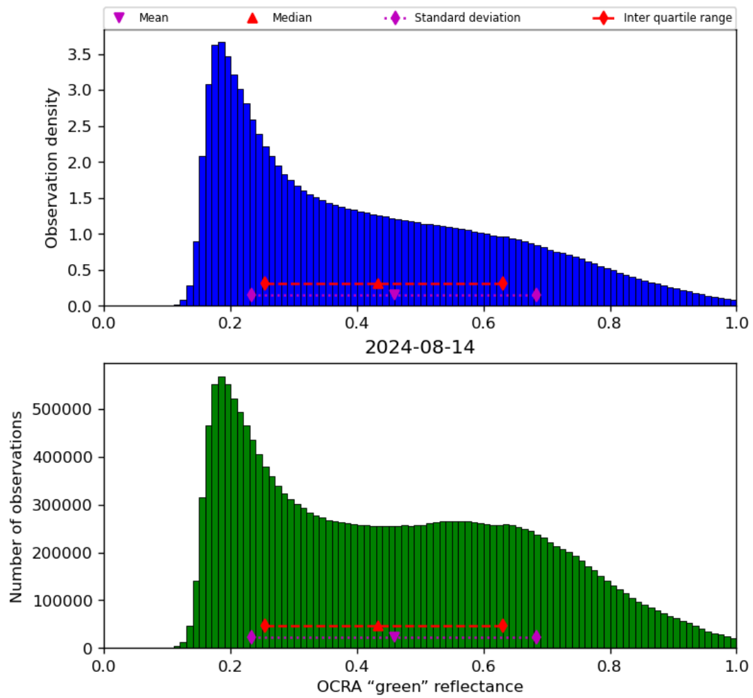
Figure 52: Histogram of “OCRA “green” reflectance” for 2024-08-13 to 2024-08-15
