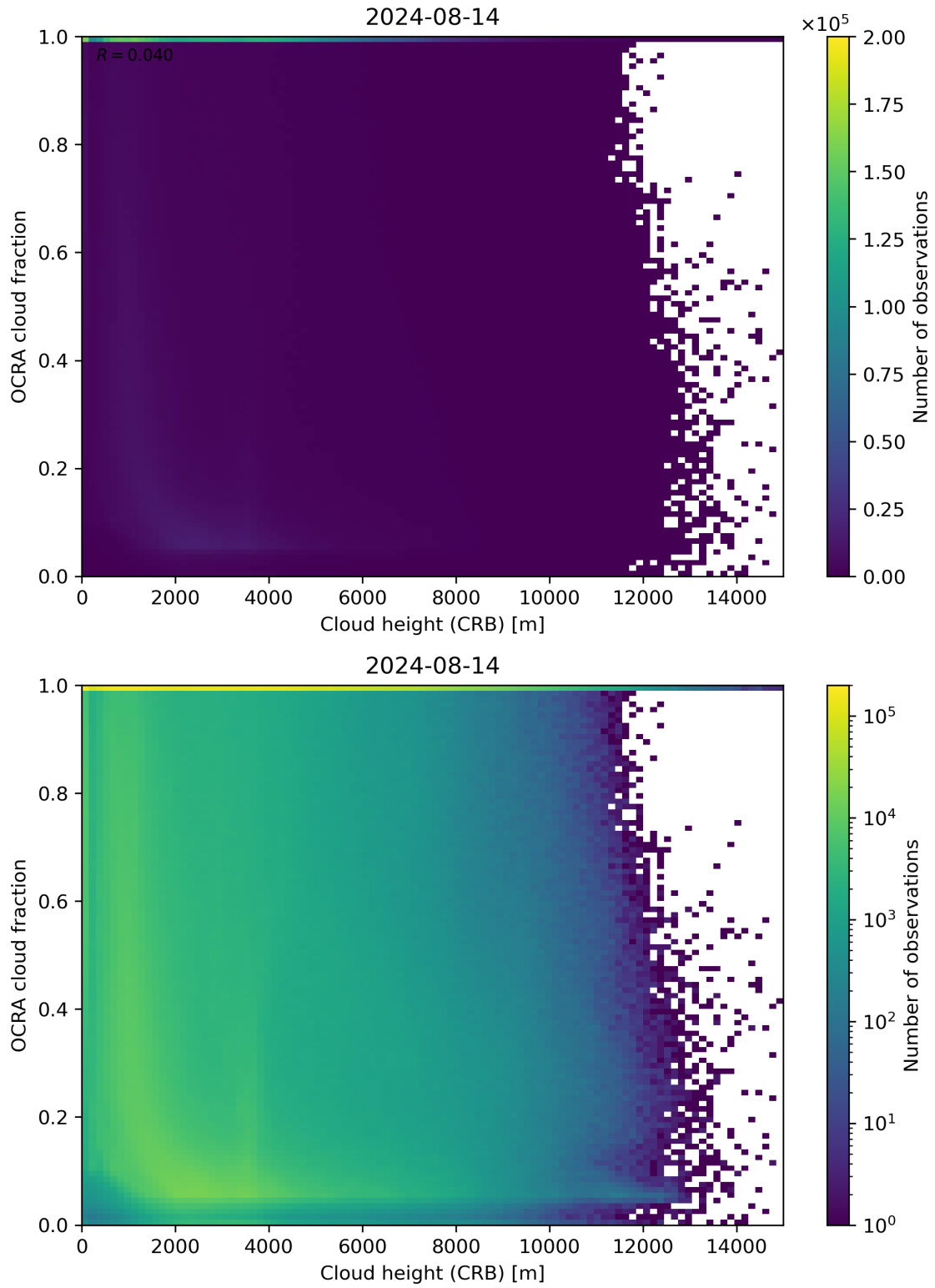
Figure 81: Scatter density plot of “Cloud height (CRB)” against “OCRA cloud fraction” for 2024-08-13 to 2024-08-15.
