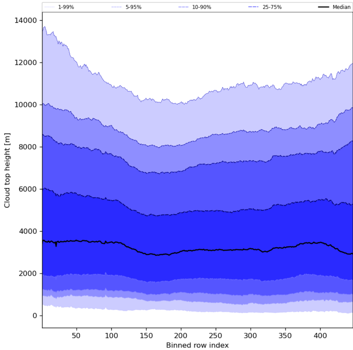
Figure 56: Along track statistics of “Cloud top height” for 2024-08-13 to 2024-08-15
