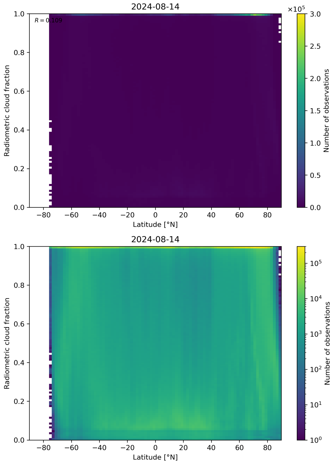
Figure 92: Scatter density plot of “Latitude” against “Radiometric cloud fraction” for 2024-08-13 to 2024-08-15.
