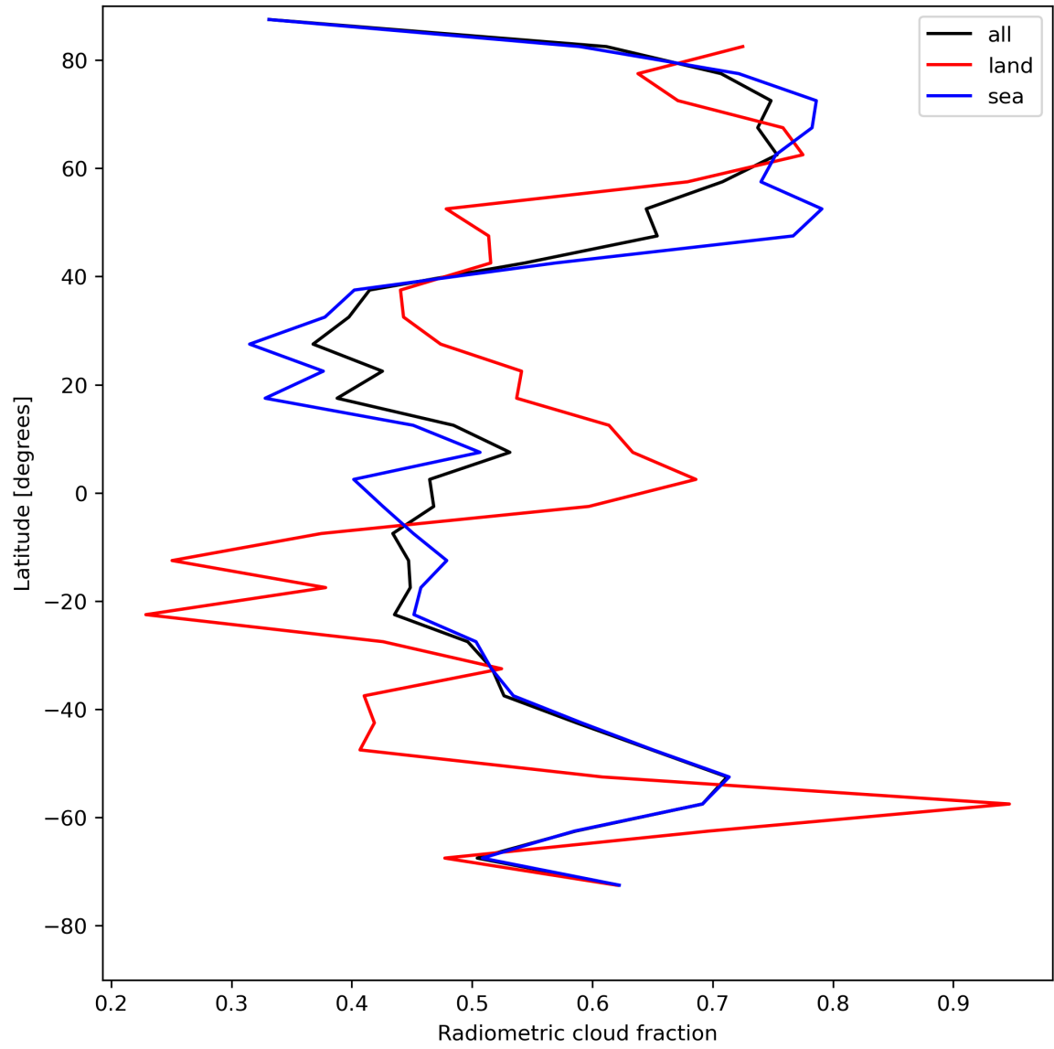
Figure 23: Zonal average of “Radiometric cloud fraction” for 2024-08-13 to 2024-08-15.
