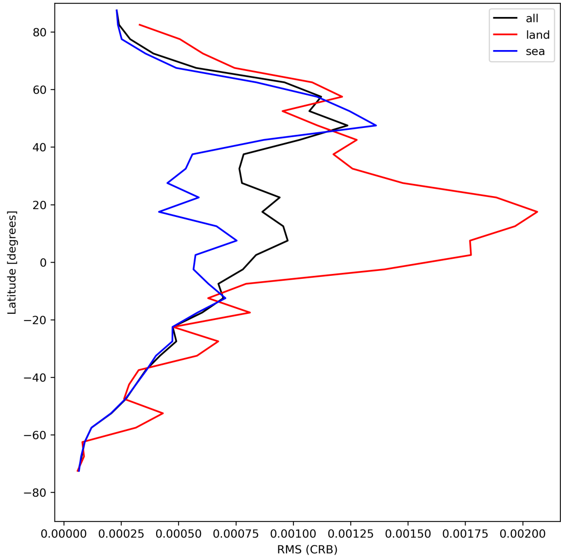
Figure 32: Zonal average of “RMS (CRB)” for 2024-08-13 to 2024-08-15.
