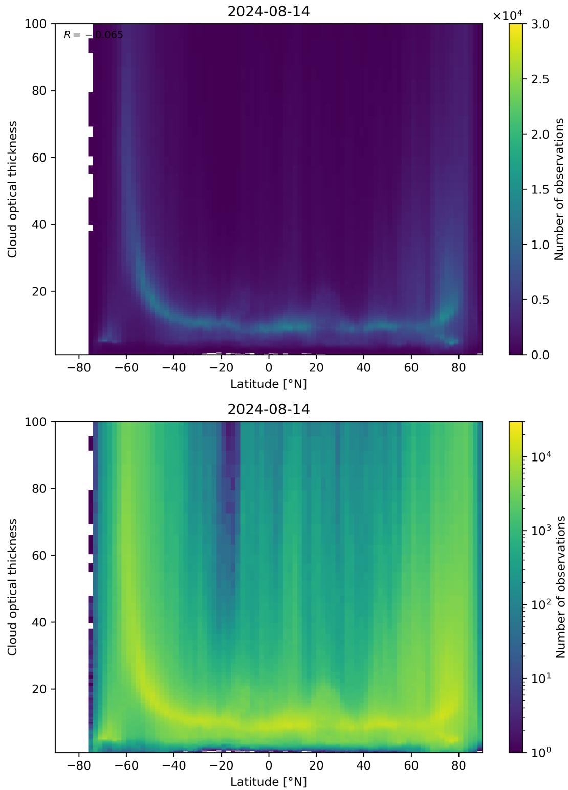
Figure 96: Scatter density plot of “Latitude” against “Cloud optical thickness” for 2024-08-13 to 2024-08-15.
