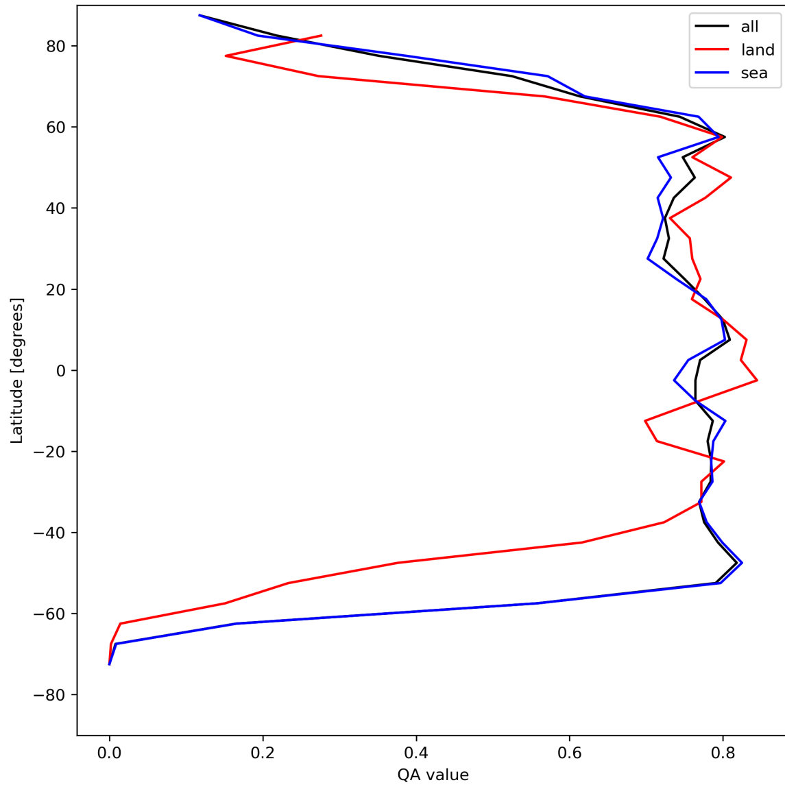
Figure 22: Zonal average of “QA value” for 2024-08-13 to 2024-08-15.
