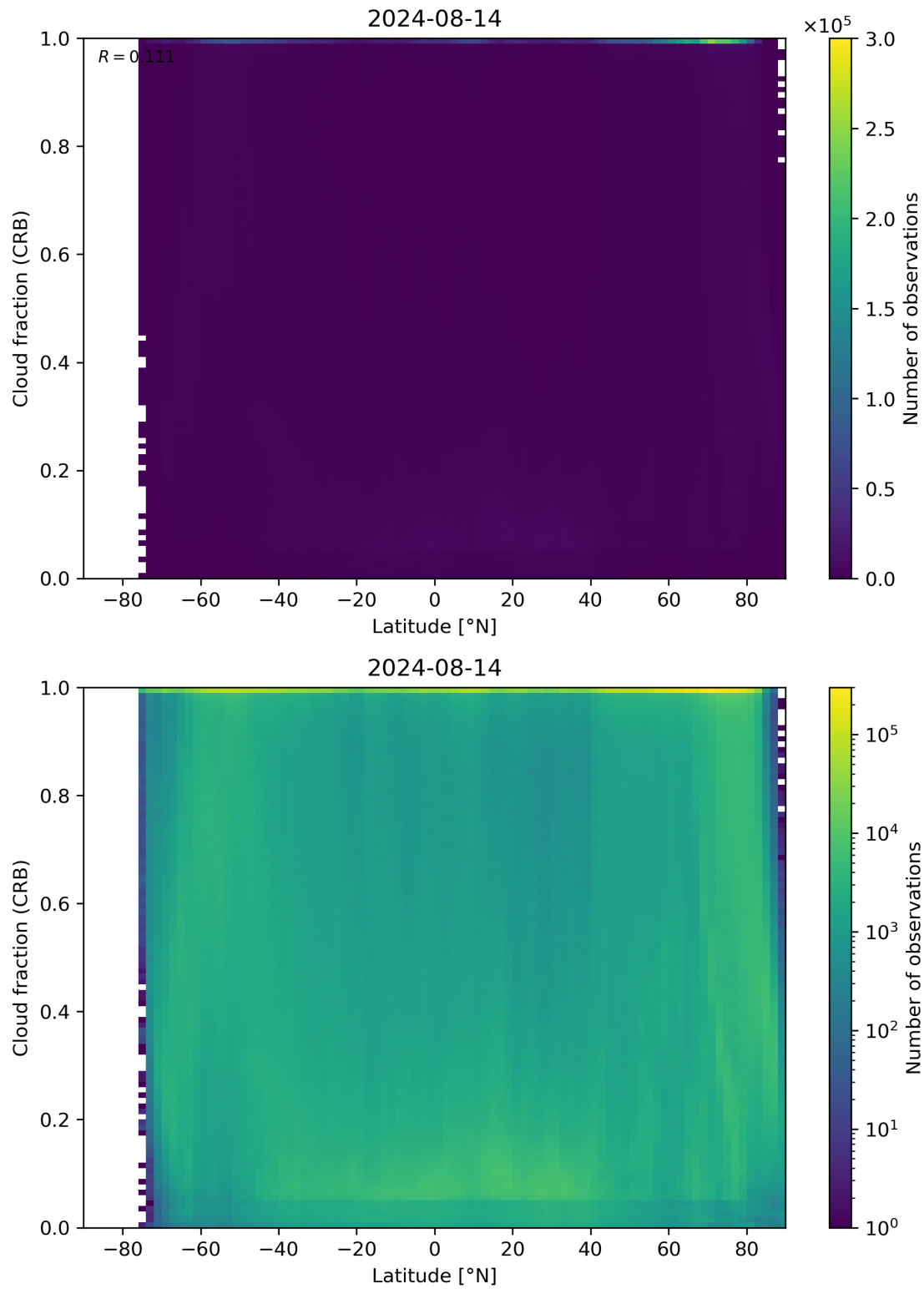
Figure 94: Scatter density plot of “Latitude” against “Cloud fraction (CRB)” for 2024-08-13 to 2024-08-15.
