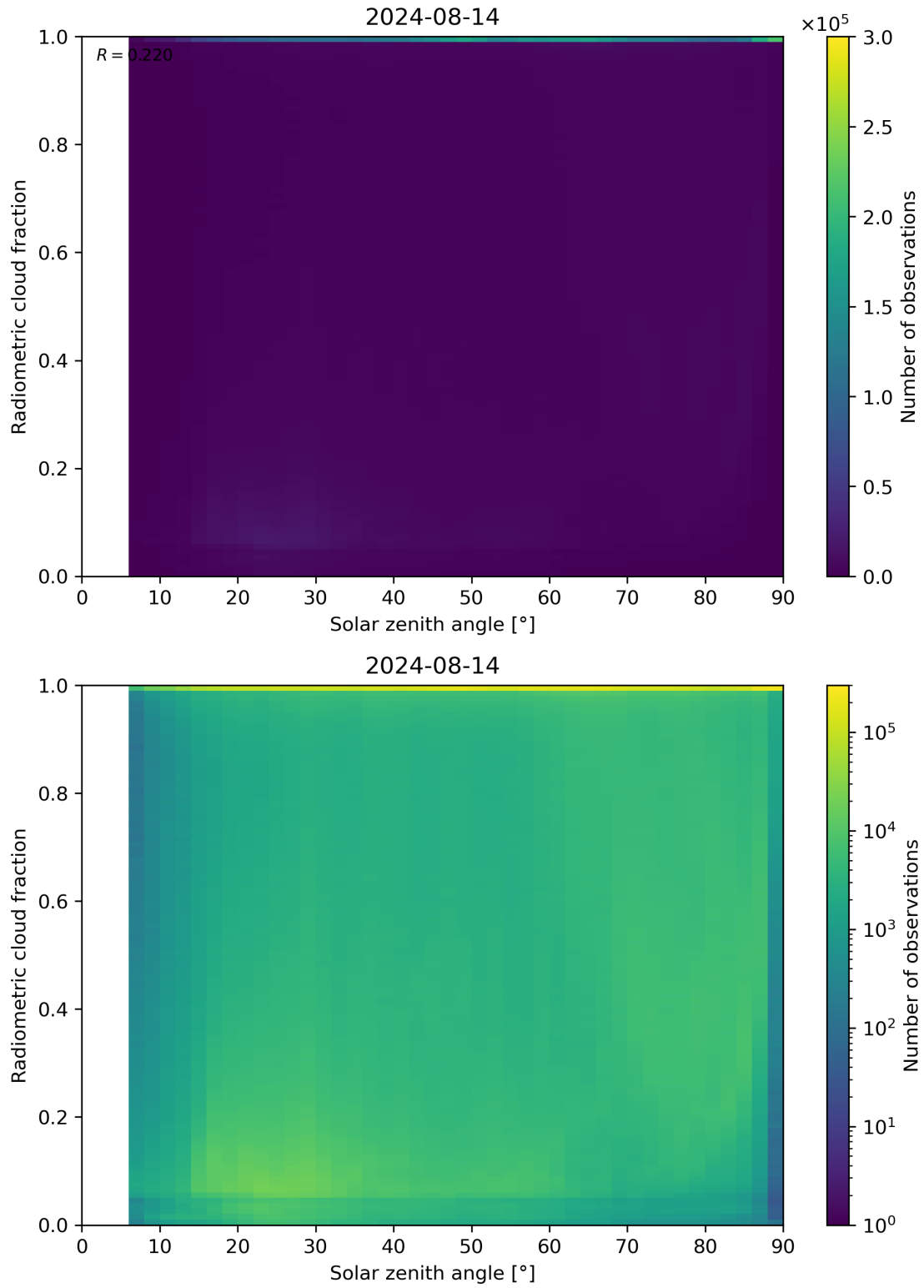
Figure 99: Scatter density plot of “Solar zenith angle” against “Radiometric cloud fraction” for 2024-08-13 to 2024-08-15.
