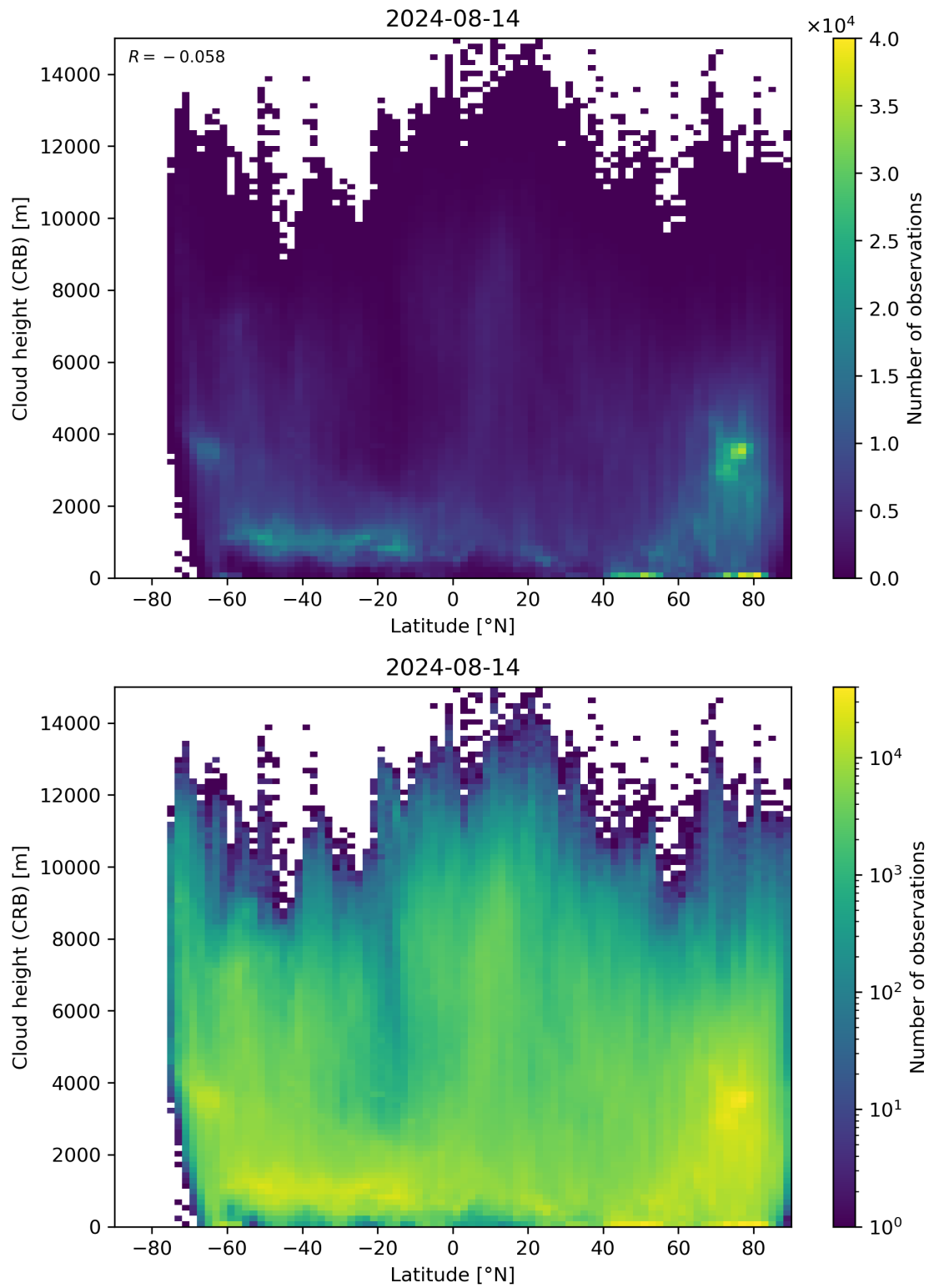
Figure 95: Scatter density plot of “Latitude” against “Cloud height (CRB)” for 2024-08-13 to 2024-08-15.
