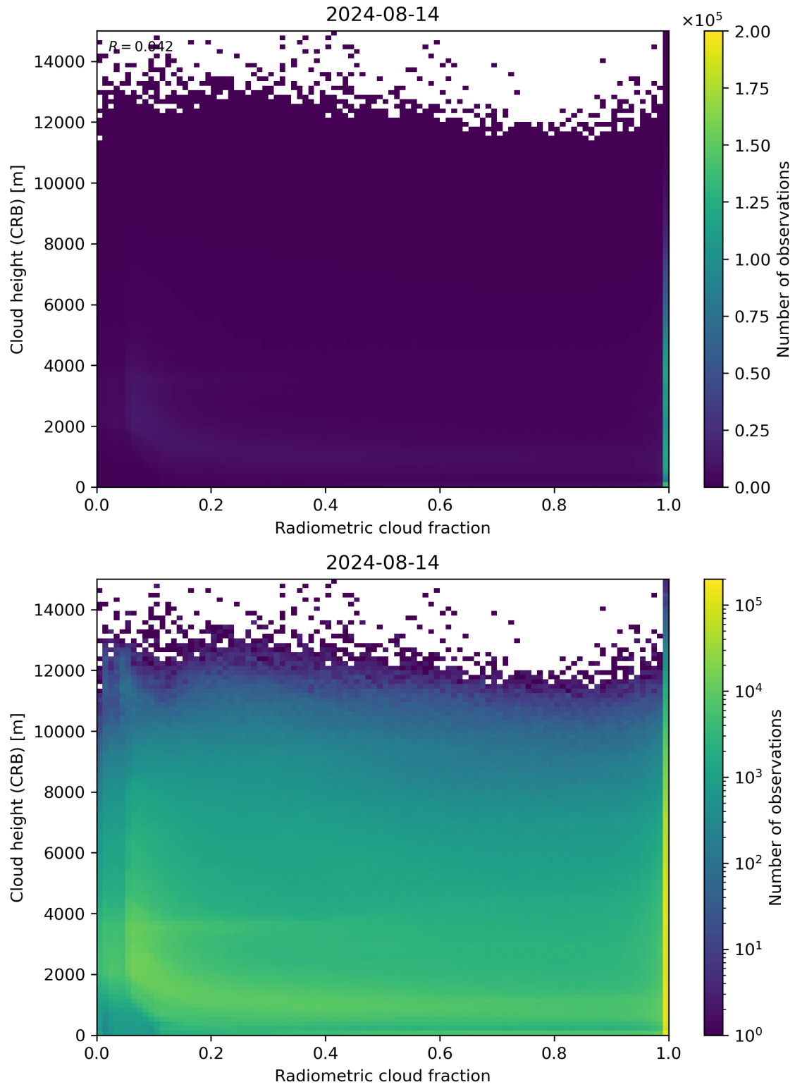
Figure 74: Scatter density plot of “Radiometric cloud fraction” against “Cloud height (CRB)” for 2024-08-13 to 2024-08-15.
