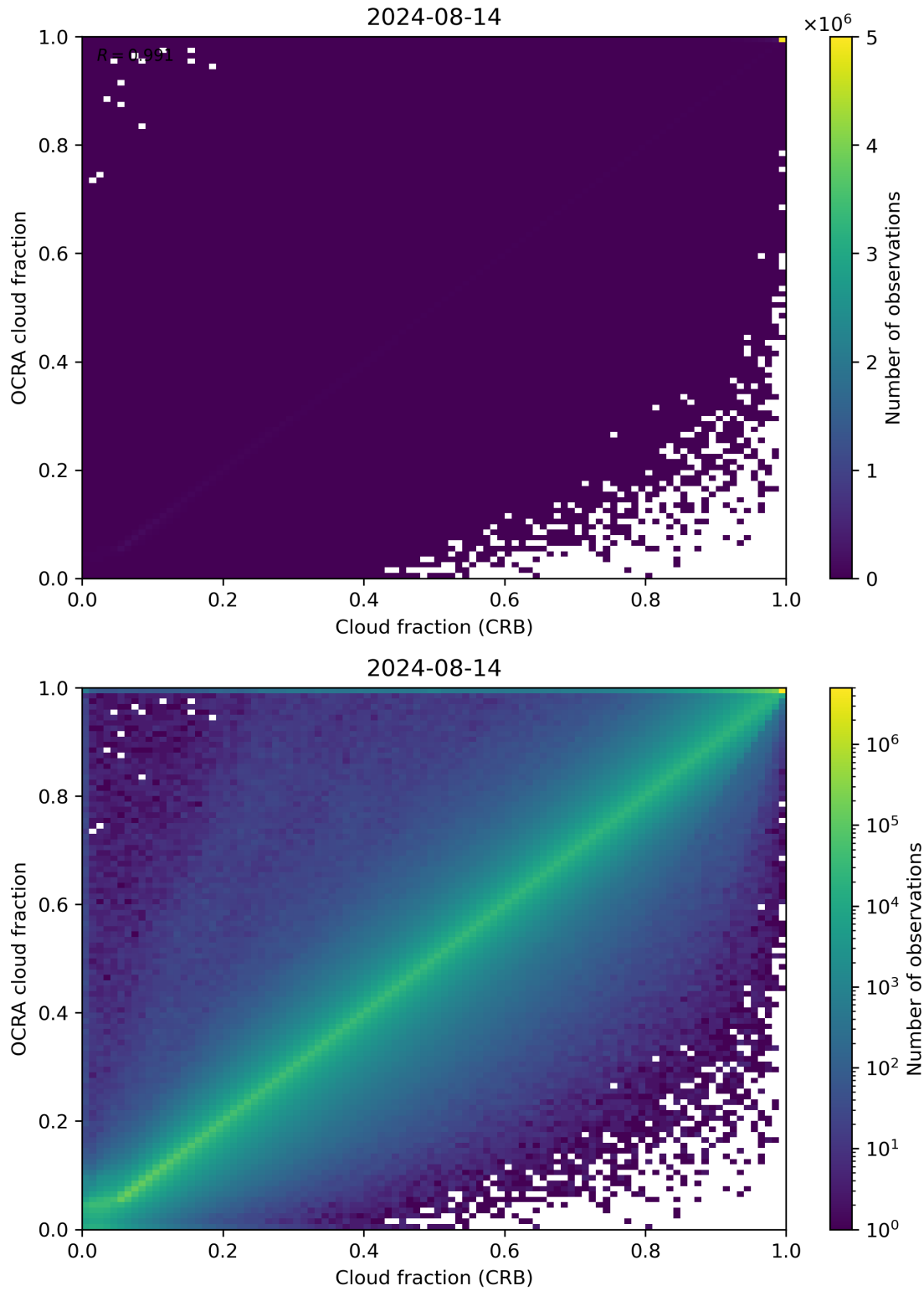
Figure 78: Scatter density plot of “Cloud fraction (CRB)” against “OCRA cloud fraction” for 2024-08-13 to 2024-08-15.
