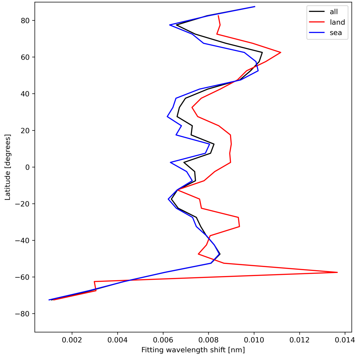
Figure 33: Zonal average of “Fitting wavelength shift” for 2024-08-13 to 2024-08-15.
