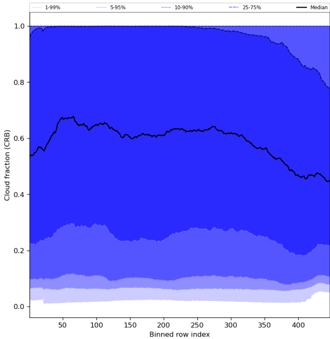
Figure 58: Along track statistics of “Cloud fraction (CRB)” for 2024-08-13 to 2024-08-15
