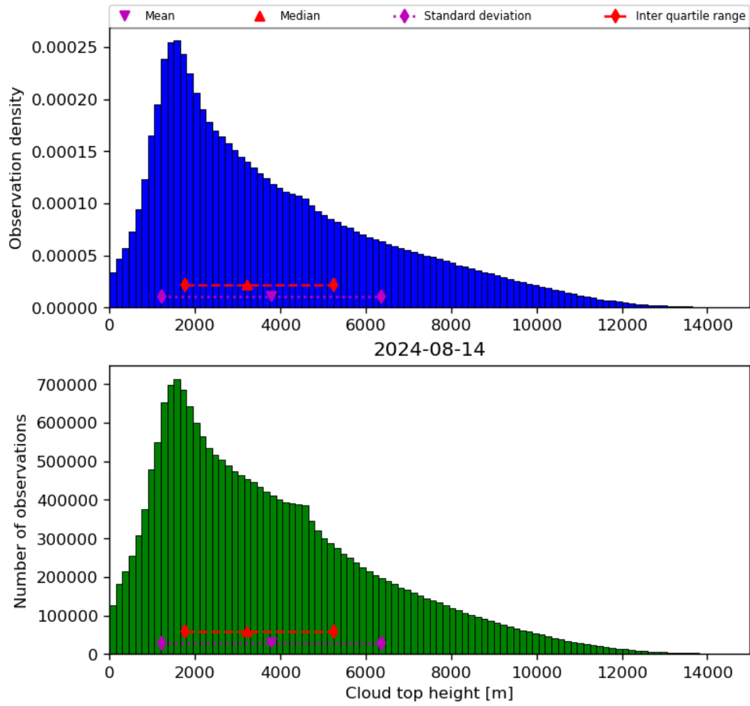
Figure 40: Histogram of “Cloud top height” for 2024-08-13 to 2024-08-15
