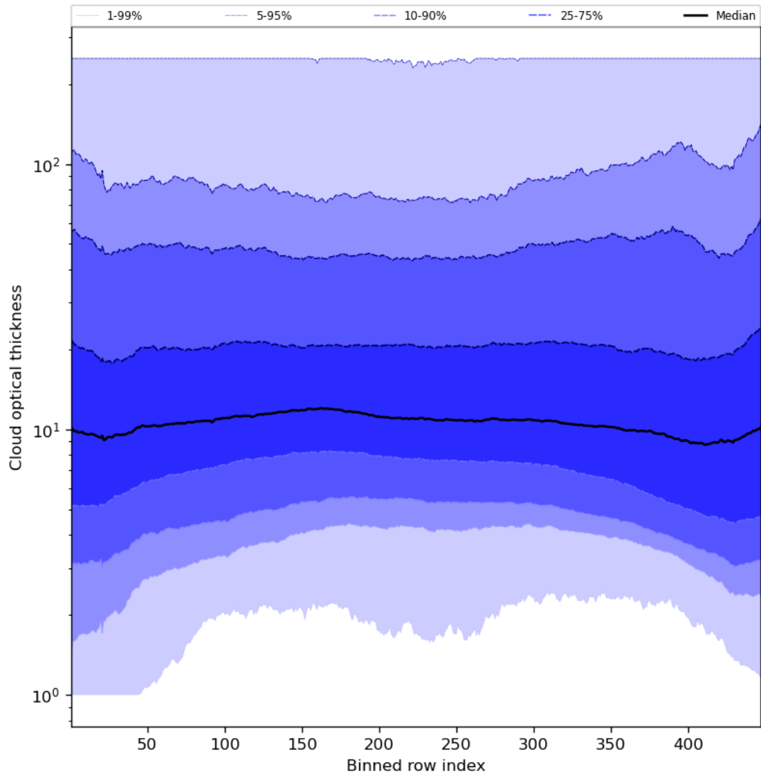
Figure 57: Along track statistics of “Cloud optical thickness” for 2024-08-13 to 2024-08-15
