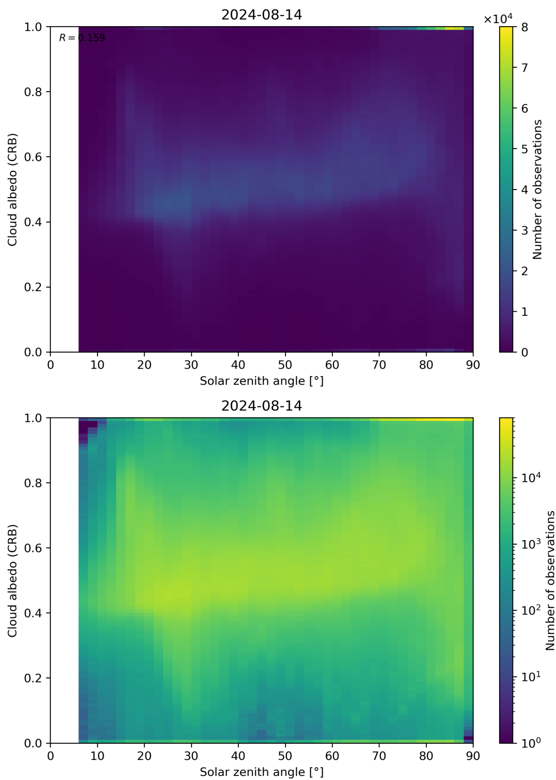
Figure 98: Scatter density plot of “Solar zenith angle” against “Cloud albedo (CRB)” for 2024-08-13 to 2024-08-15.
