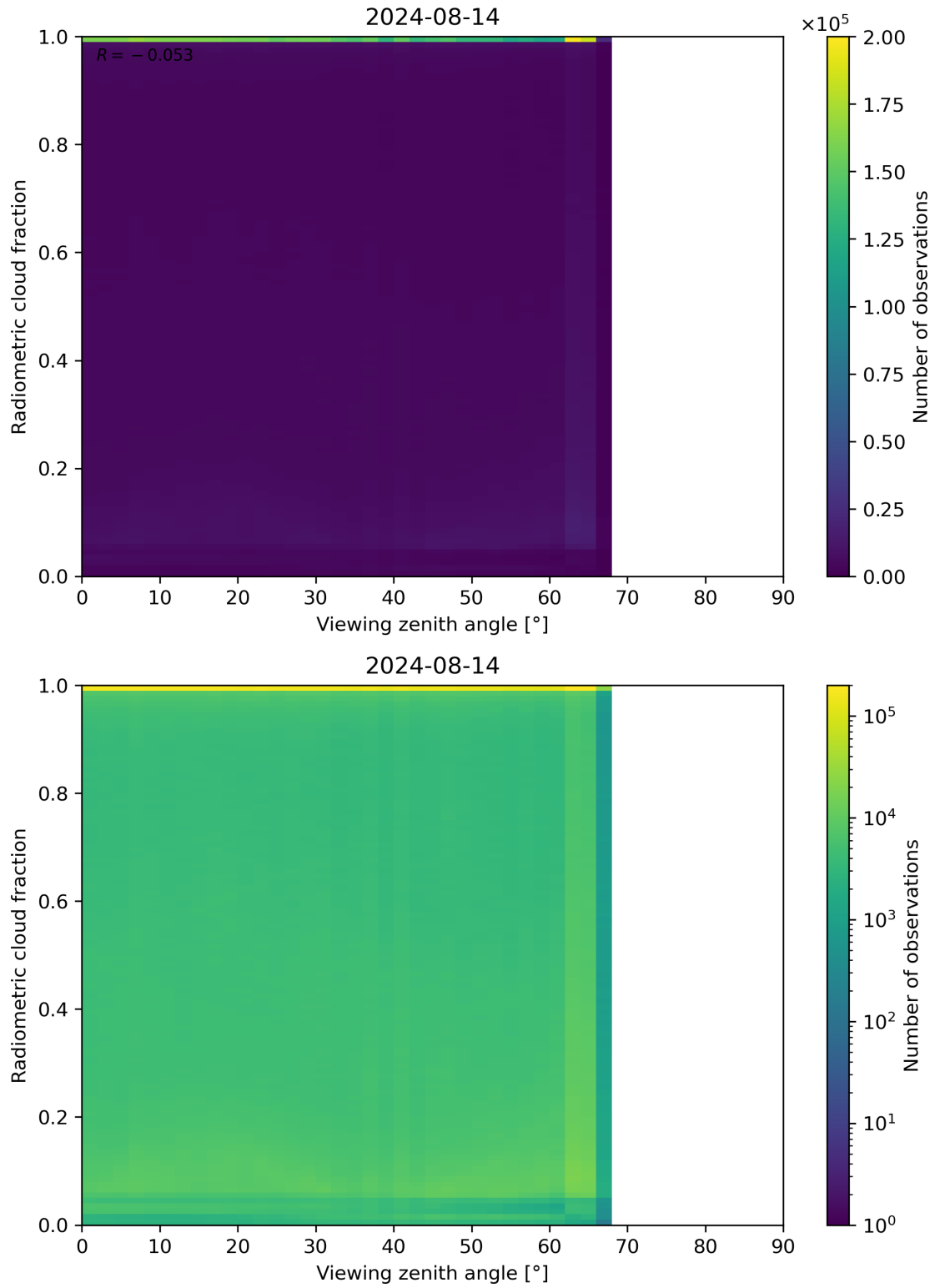
Figure 107: Scatter density plot of “Viewing zenith angle” against “Radiometric cloud fraction” for 2024-08-13 to 2024-08-15.
