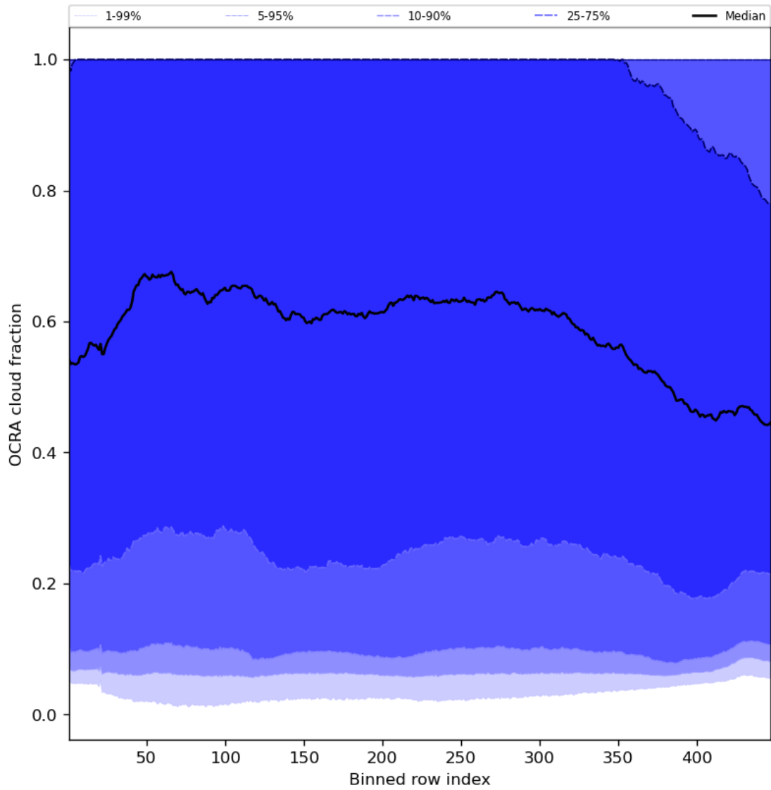
Figure 66: Along track statistics of “OCRA cloud fraction” for 2024-08-13 to 2024-08-15
