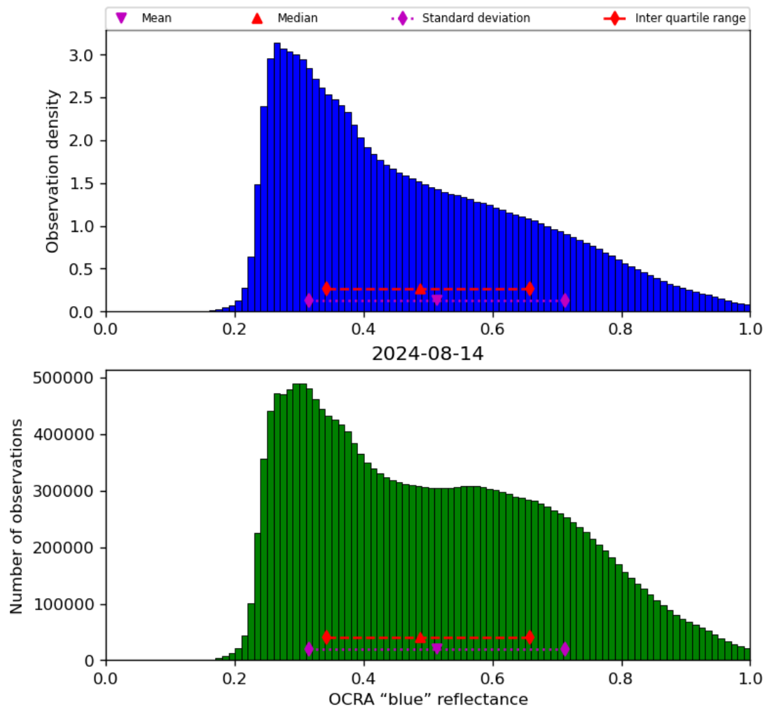
Figure 51: Histogram of “OCRA “blue” reflectance” for 2024-08-13 to 2024-08-15
