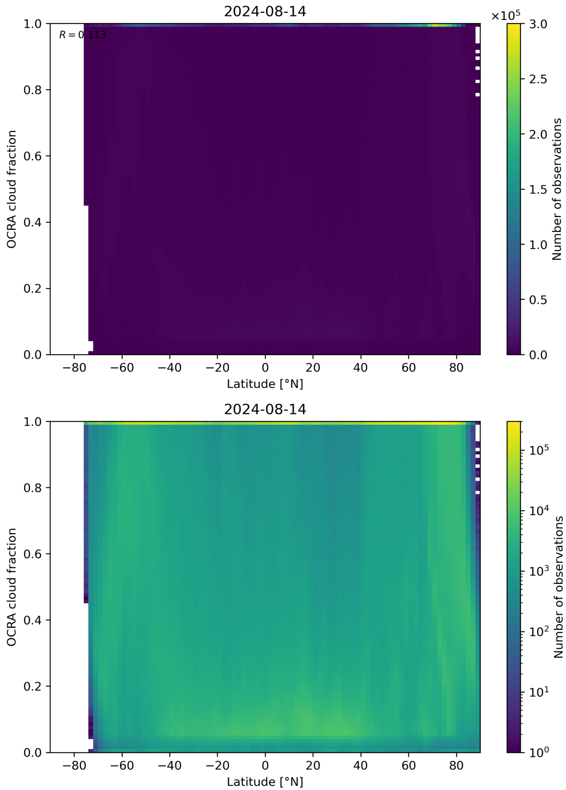
Figure 93: Scatter density plot of “Latitude” against “OCRA cloud fraction” for 2024-08-13 to 2024-08-15.
