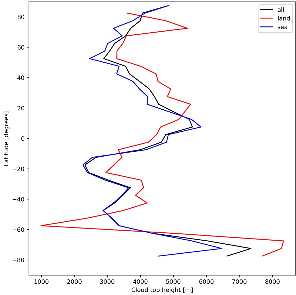
Figure 24: Zonal average of “Cloud top height” for 2024-08-16 to 2024-08-18.
