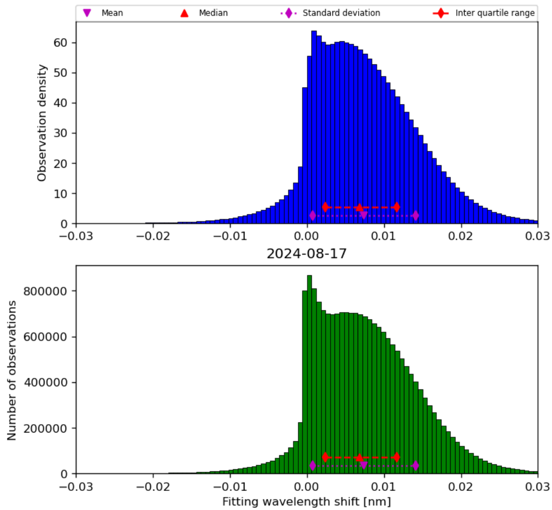
Figure 49: Histogram of “Fitting wavelength shift” for 2024-08-16 to 2024-08-18
