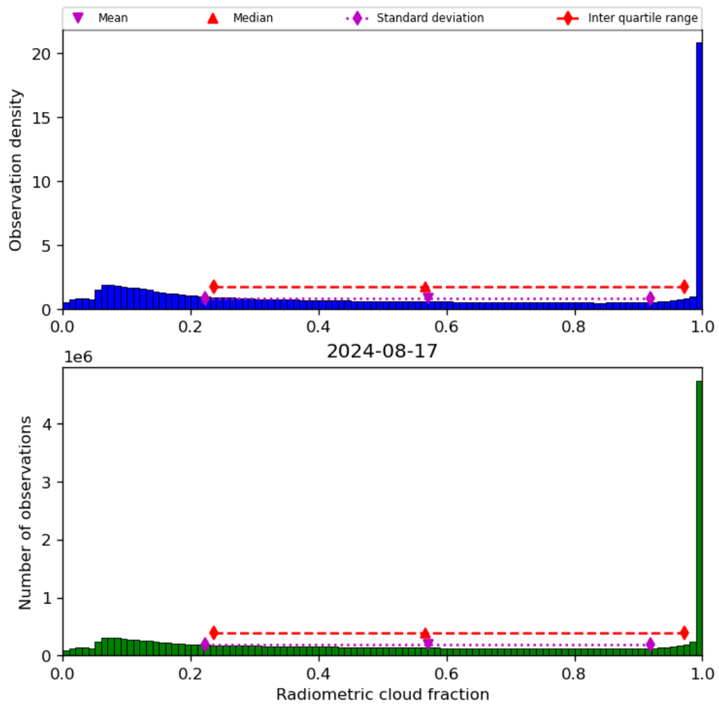
Figure 39: Histogram of “Radiometric cloud fraction” for 2024-08-16 to 2024-08-18
