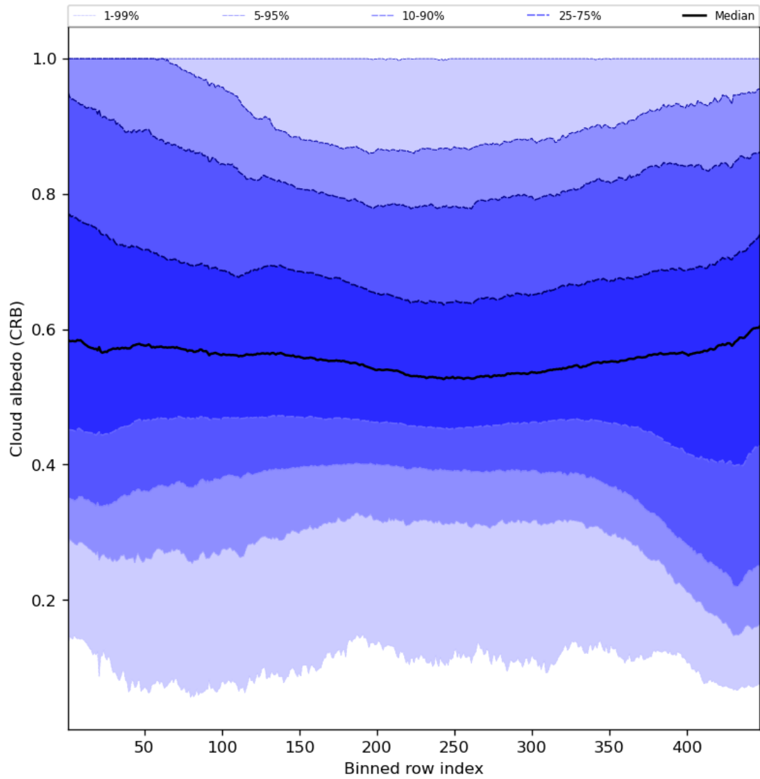
Figure 60: Along track statistics of “Cloud albedo (CRB)” for 2024-08-16 to 2024-08-18
