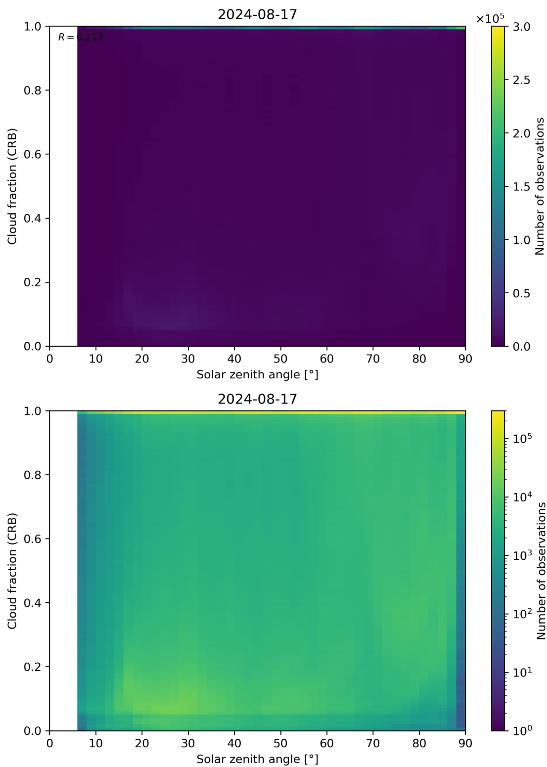
Figure 101: Scatter density plot of “Solar zenith angle” against “Cloud fraction (CRB)” for 2024-08-16 to 2024-08-18.
