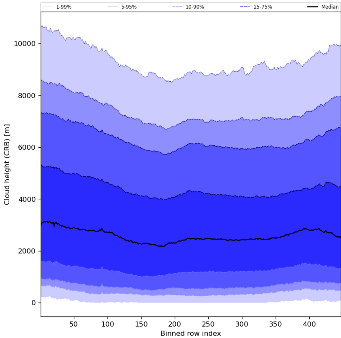
Figure 59: Along track statistics of “Cloud height (CRB)” for 2024-08-16 to 2024-08-18
