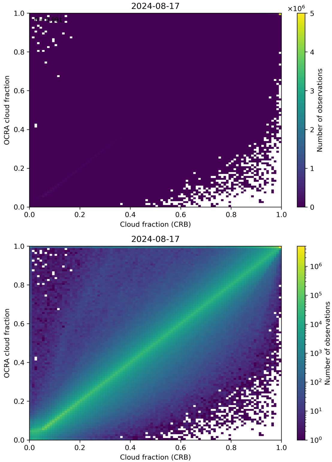
Figure 78: Scatter density plot of “Cloud fraction (CRB)” against “OCRA cloud fraction” for 2024-08-16 to 2024-08-18.
