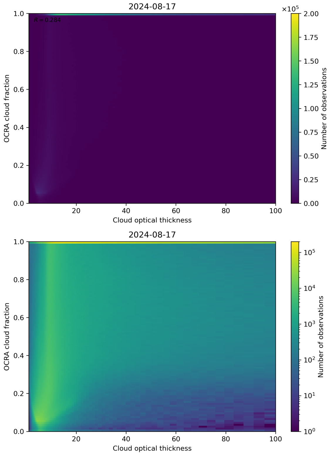
Figure 83: Scatter density plot of “Cloud optical thickness” against “OCRA cloud fraction” for 2024-08-16 to 2024-08-18.
