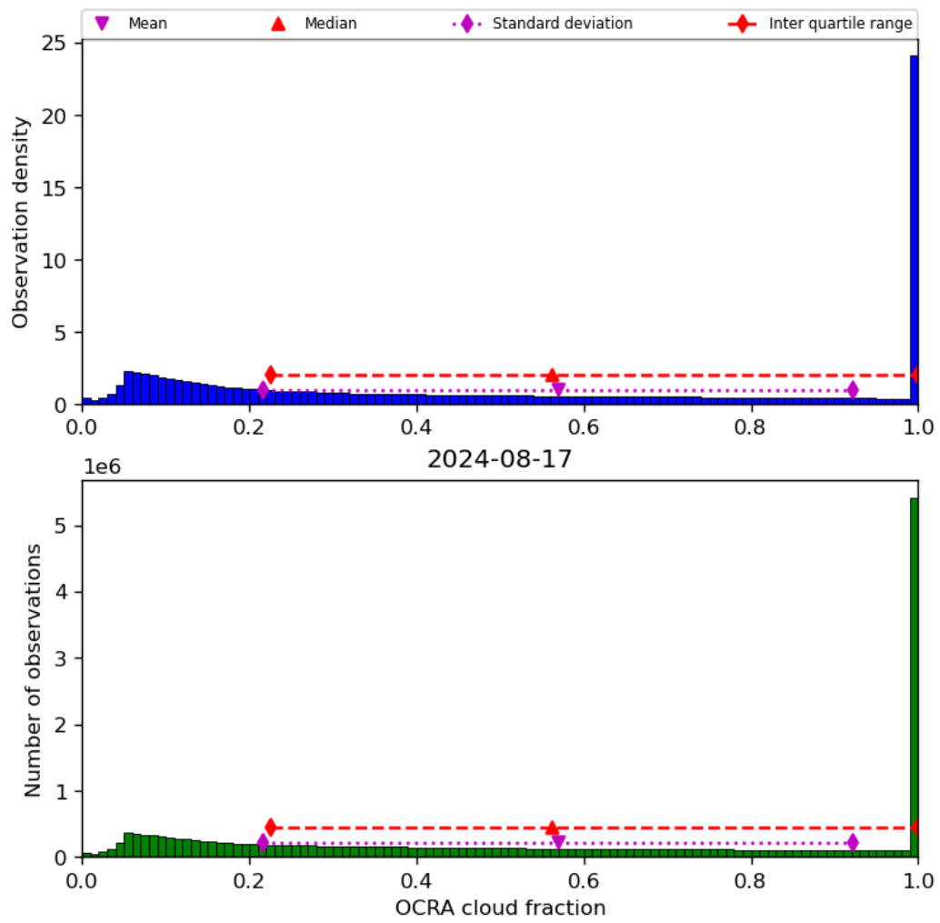
Figure 50: Histogram of “OCRA cloud fraction” for 2024-08-16 to 2024-08-18
