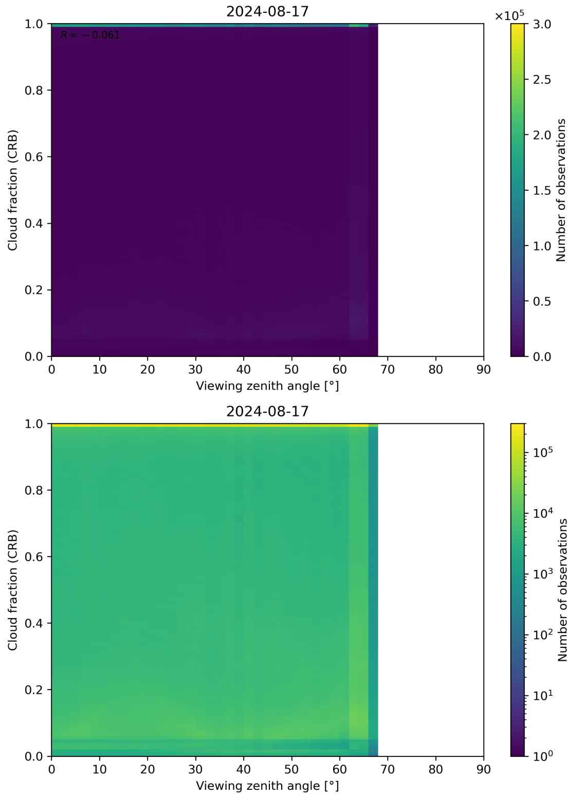
Figure 109: Scatter density plot of “Viewing zenith angle” against “Cloud fraction (CRB)” for 2024-08-16 to 2024-08-18.
