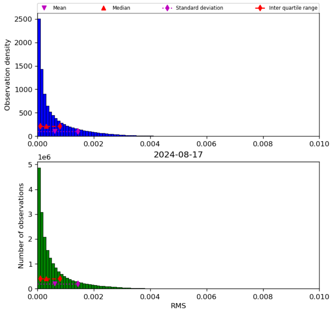
Figure 47: Histogram of “RMS” for 2024-08-16 to 2024-08-18
