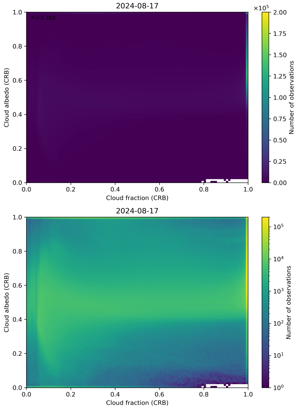
Figure 77: Scatter density plot of “Cloud fraction (CRB)” against “Cloud albedo (CRB)” for 2024-08-16 to 2024-08-18.
