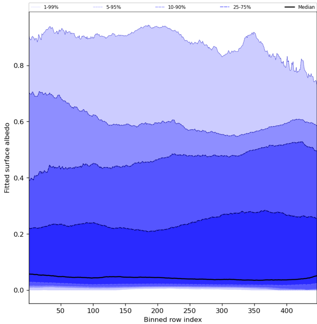
Figure 61: Along track statistics of “Fitted surface albedo” for 2024-08-16 to 2024-08-18
