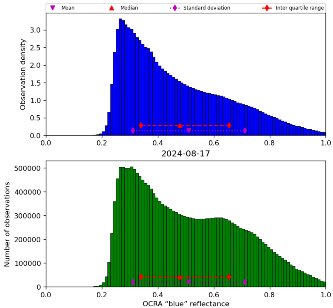
Figure 51: Histogram of “OCRA “blue” reflectance” for 2024-08-16 to 2024-08-18
