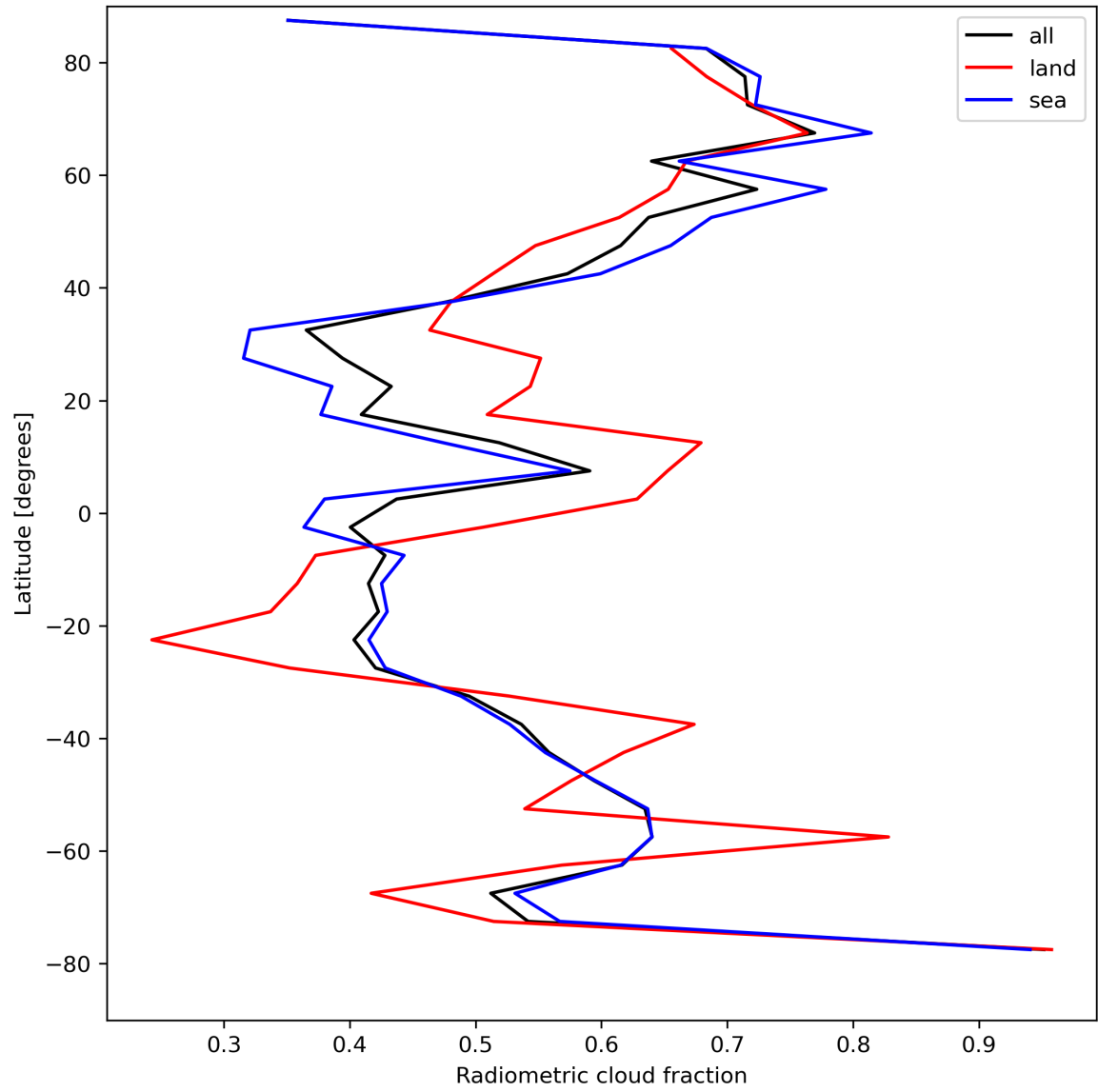
Figure 23: Zonal average of “Radiometric cloud fraction” for 2024-08-16 to 2024-08-18.
