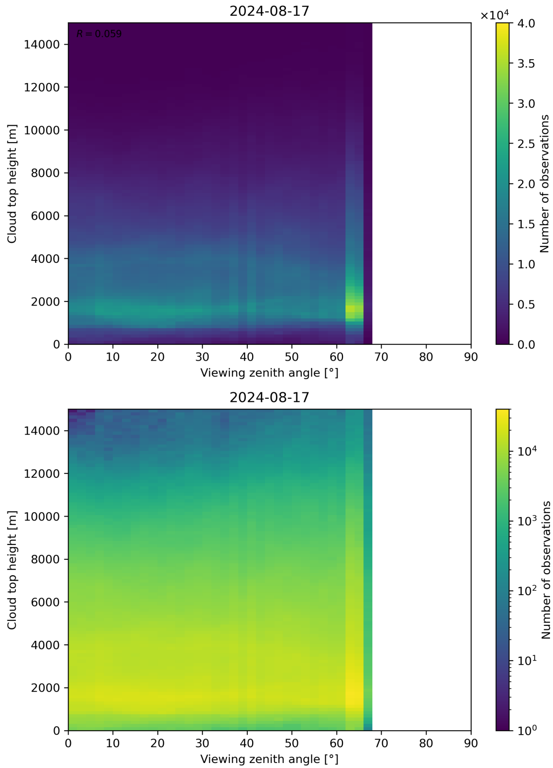
Figure 112: Scatter density plot of “Viewing zenith angle” against “Cloud top height” for 2024-08-16 to 2024-08-18.
