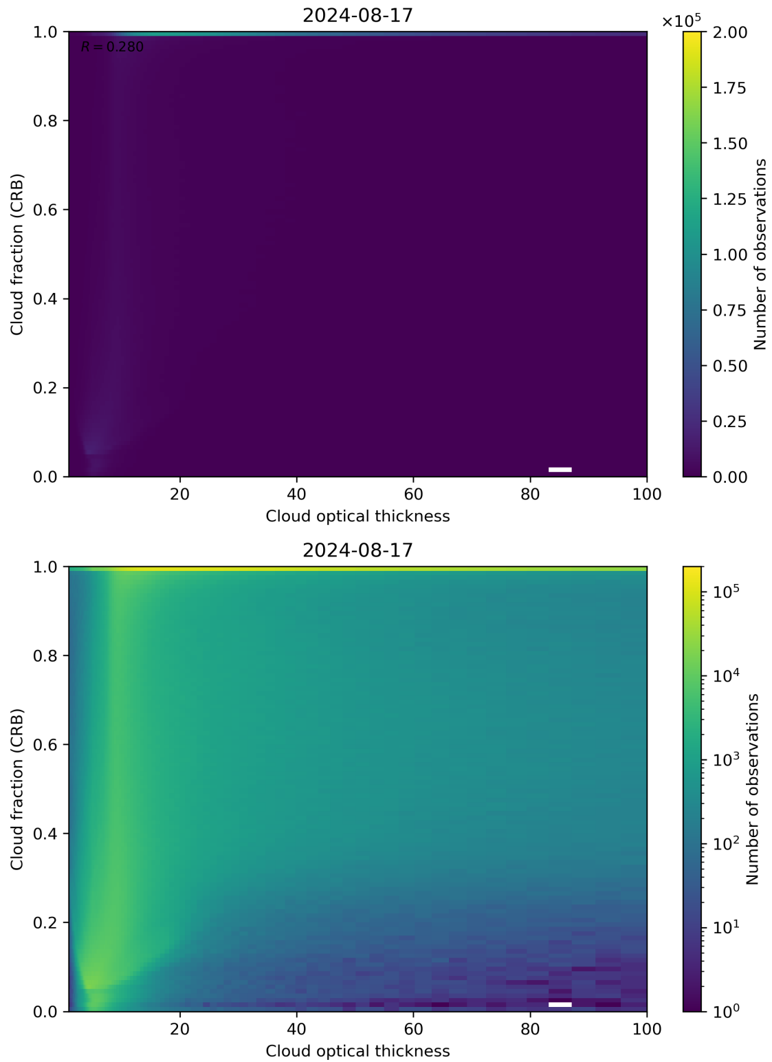
Figure 84: Scatter density plot of “Cloud optical thickness” against “Cloud fraction (CRB)” for 2024-08-16 to 2024-08-18.
