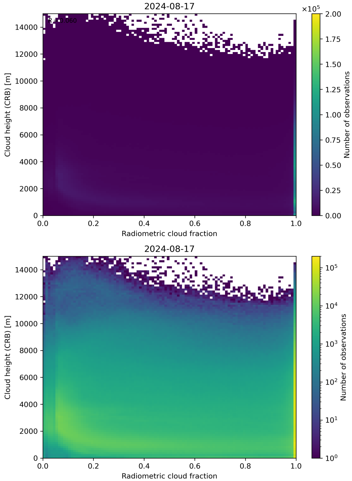
Figure 74: Scatter density plot of “Radiometric cloud fraction” against “Cloud height (CRB)” for 2024-08-16 to 2024-08-18.
