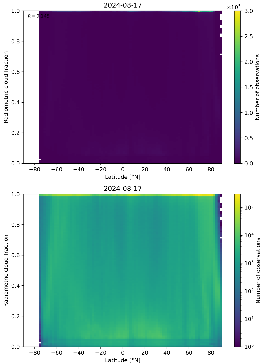
Figure 92: Scatter density plot of “Latitude” against “Radiometric cloud fraction” for 2024-08-16 to 2024-08-18.
