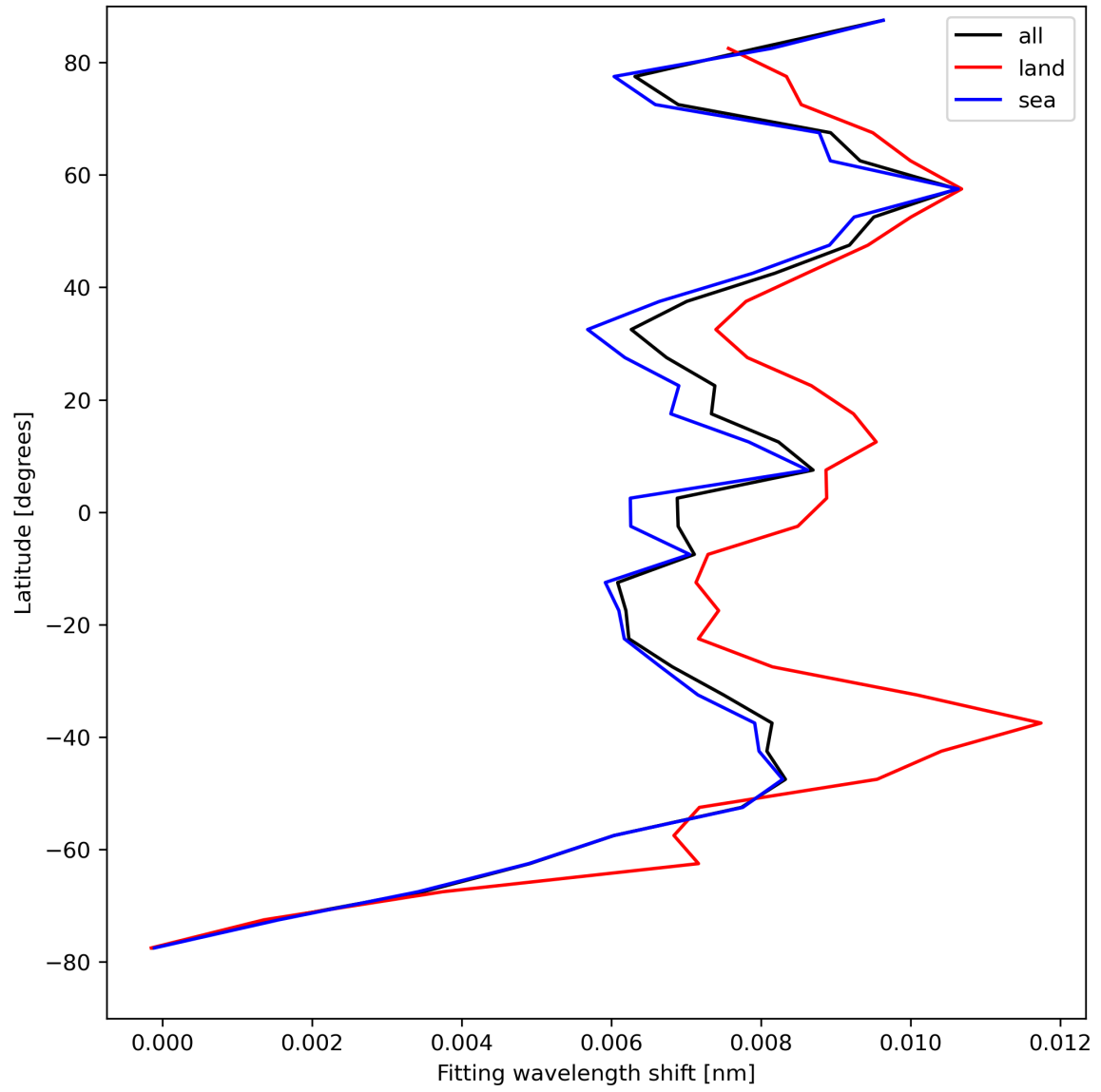
Figure 33: Zonal average of “Fitting wavelength shift” for 2024-08-16 to 2024-08-18.
