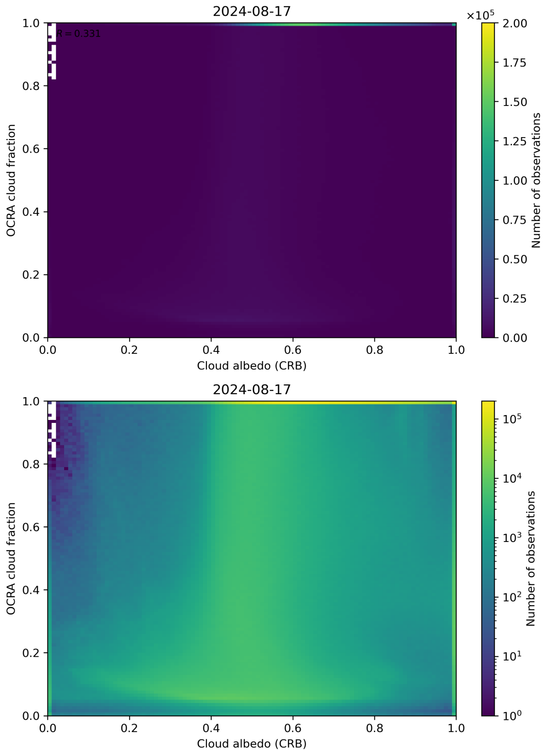
Figure 70: Scatter density plot of “Cloud albedo (CRB)” against “OCRA cloud fraction” for 2024-08-16 to 2024-08-18.
