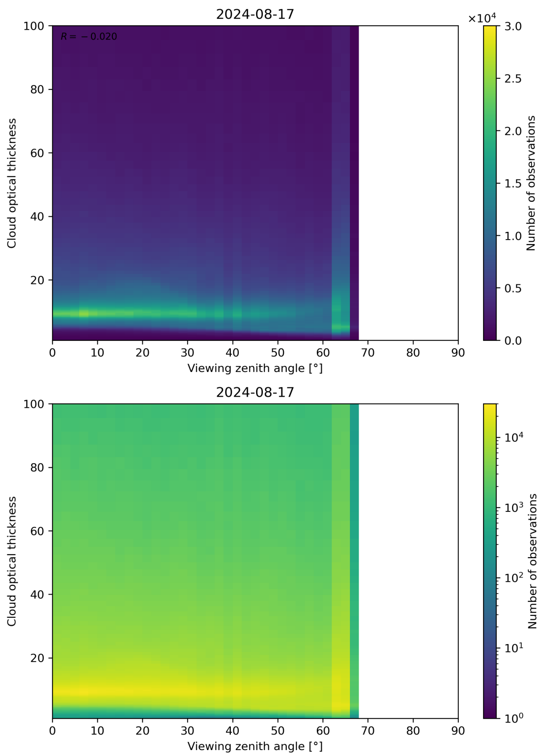
Figure 111: Scatter density plot of “Viewing zenith angle” against “Cloud optical thickness” for 2024-08-16 to 2024-08-18.
