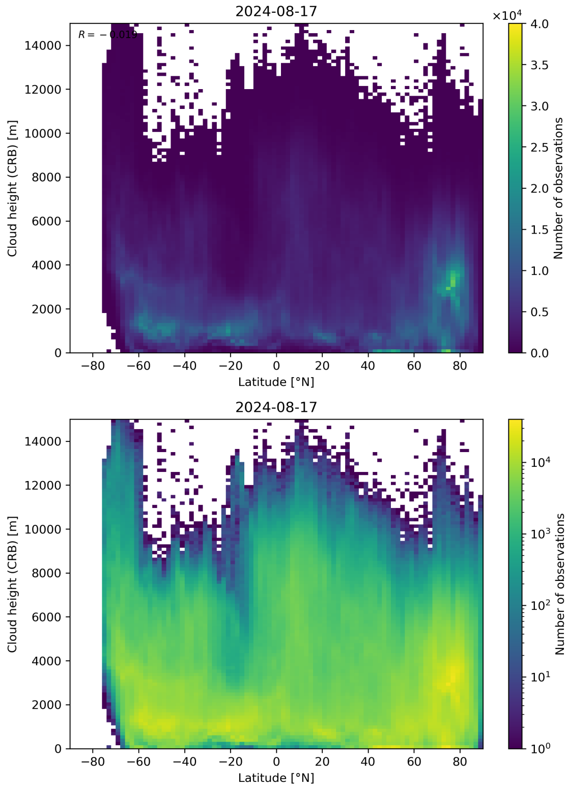
Figure 95: Scatter density plot of “Latitude” against “Cloud height (CRB)” for 2024-08-16 to 2024-08-18.
