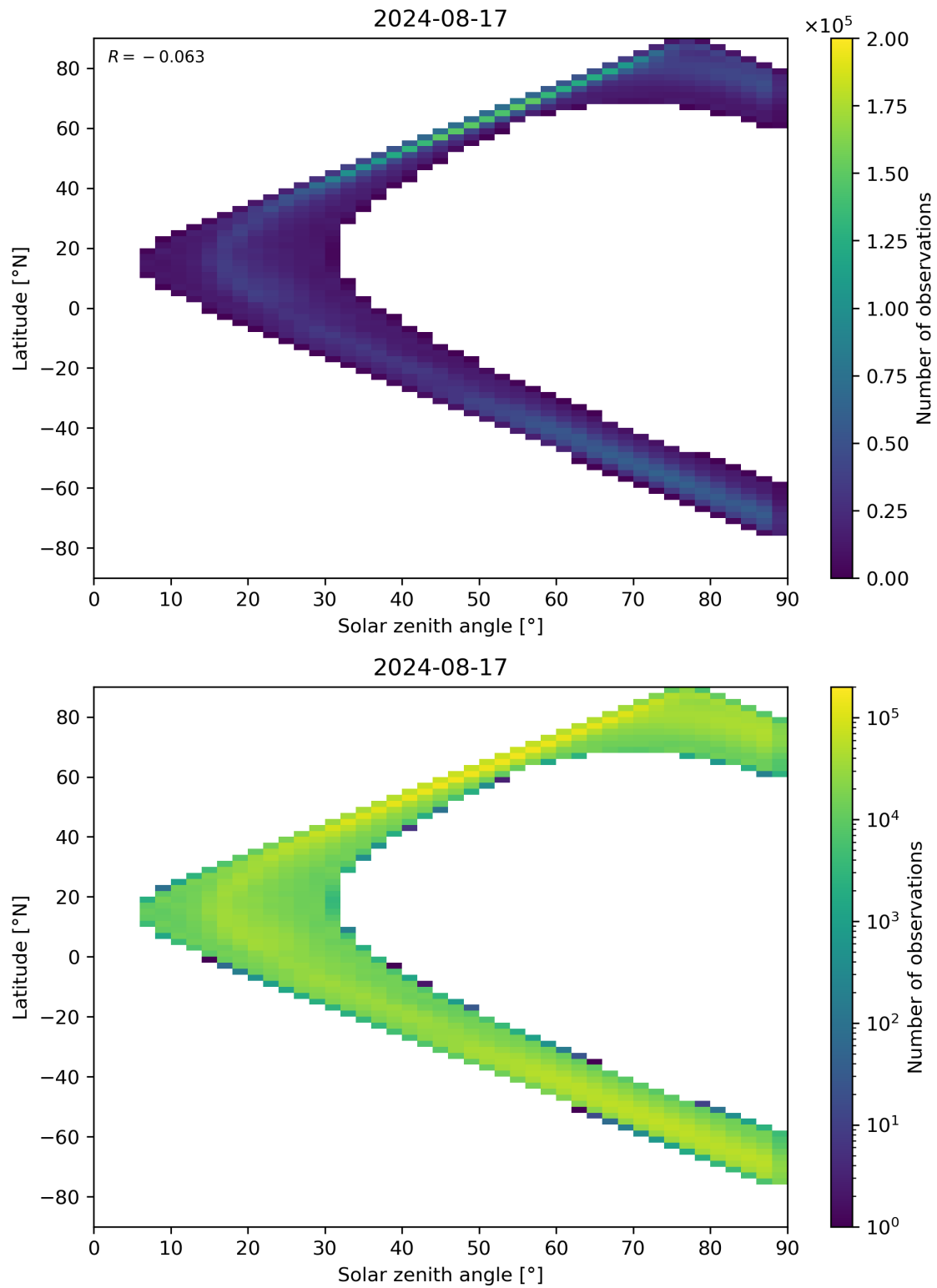
Figure 105: Scatter density plot of “Solar zenith angle” against “Latitude” for 2024-08-16 to 2024-08-18.
