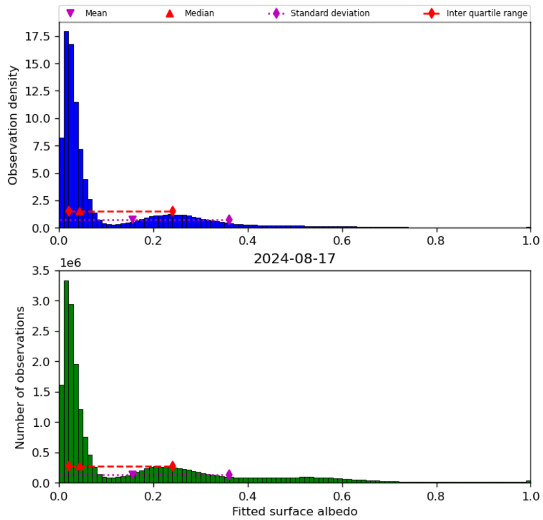
Figure 45: Histogram of “Fitted surface albedo” for 2024-08-16 to 2024-08-18
