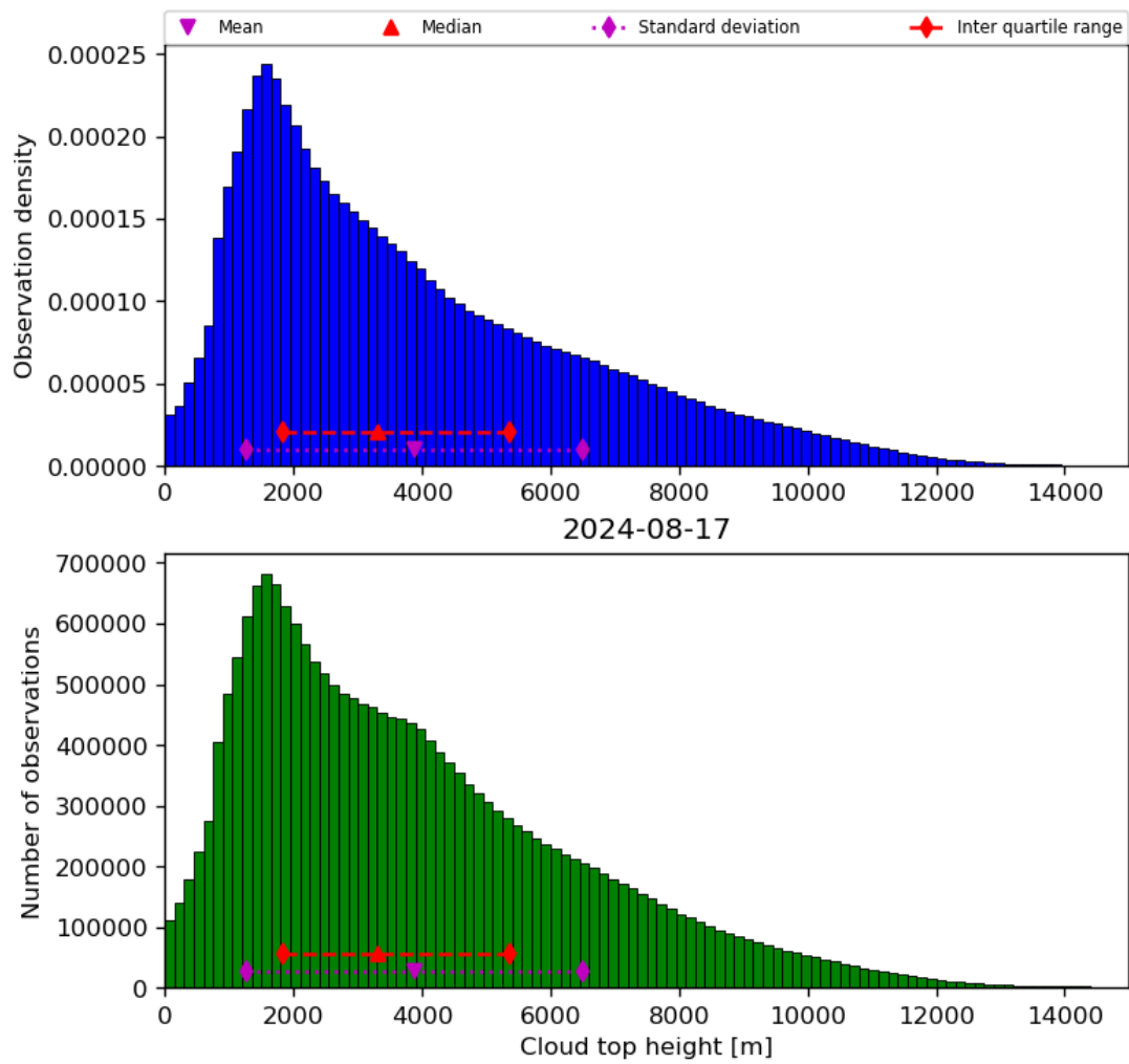
Figure 40: Histogram of “Cloud top height” for 2024-08-16 to 2024-08-18
