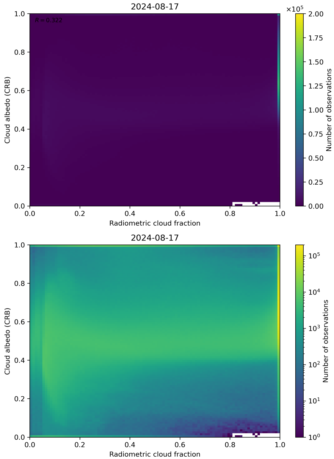
Figure 71: Scatter density plot of “Radiometric cloud fraction” against “Cloud albedo (CRB)” for 2024-08-16 to 2024-08-18.
