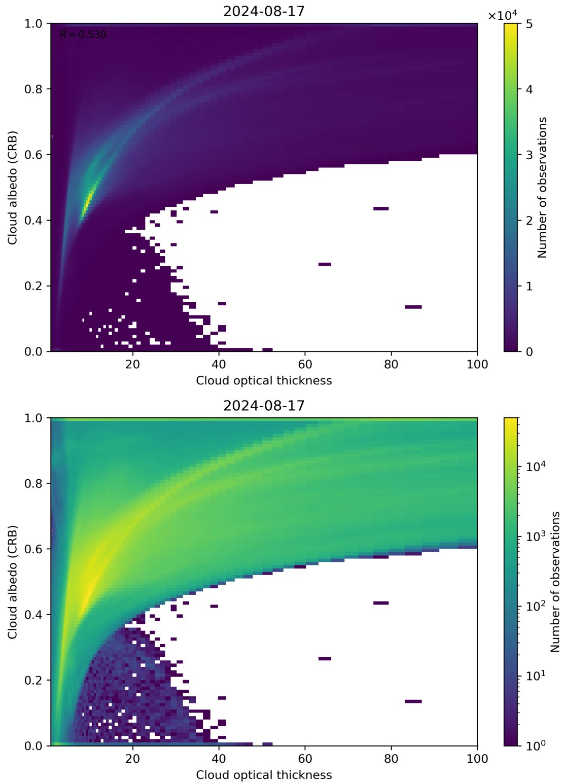
Figure 82: Scatter density plot of “Cloud optical thickness” against “Cloud albedo (CRB)” for 2024-08-16 to 2024-08-18.
