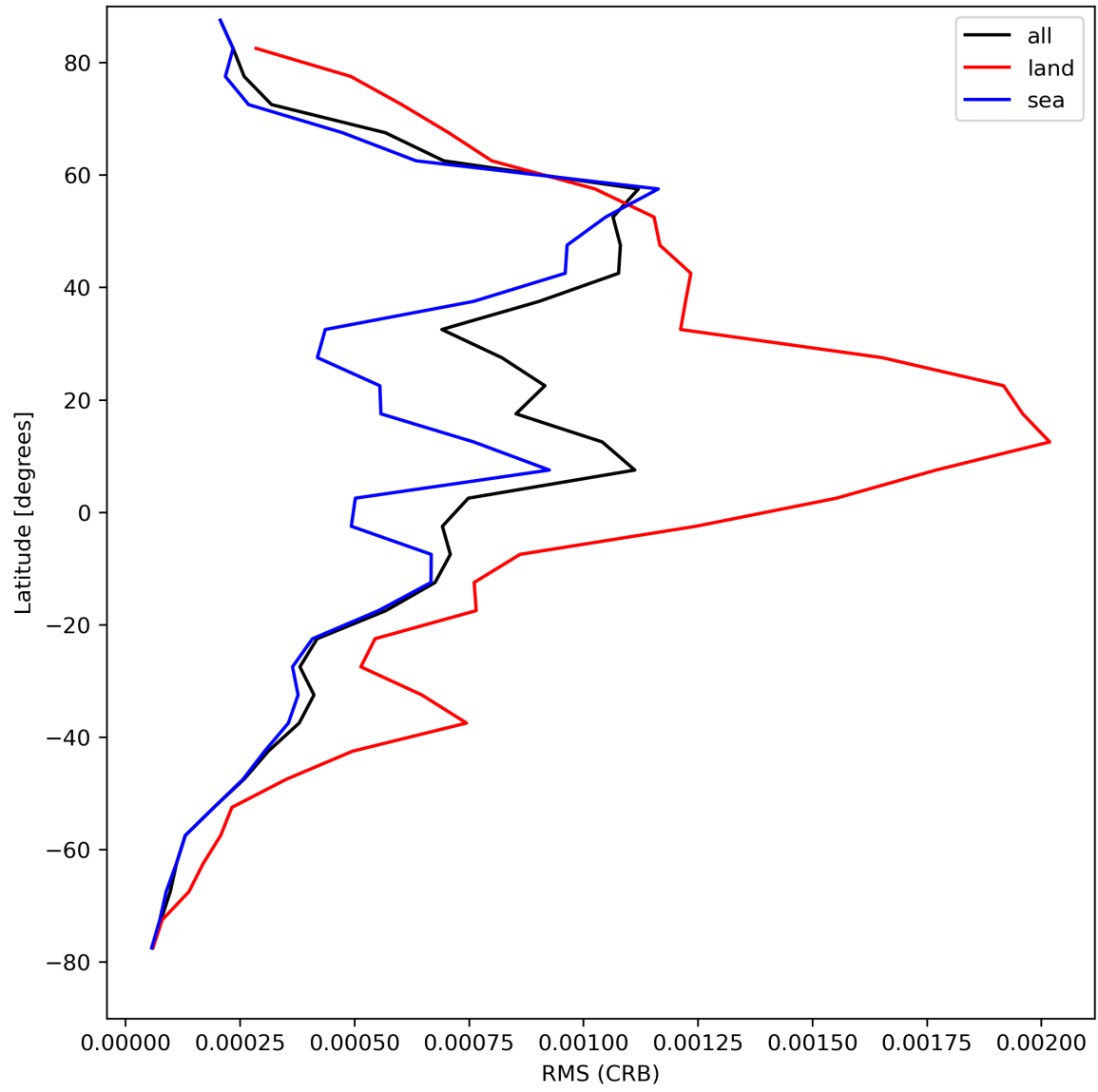
Figure 32: Zonal average of “RMS (CRB)” for 2024-08-16 to 2024-08-18.
