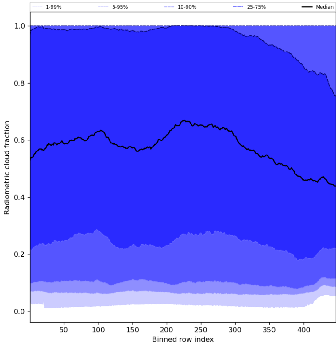
Figure 55: Along track statistics of “Radiometric cloud fraction” for 2024-08-16 to 2024-08-18
