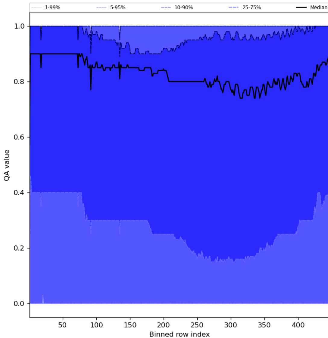
Figure 54: Along track statistics of “QA value” for 2024-08-17 to 2024-08-19
