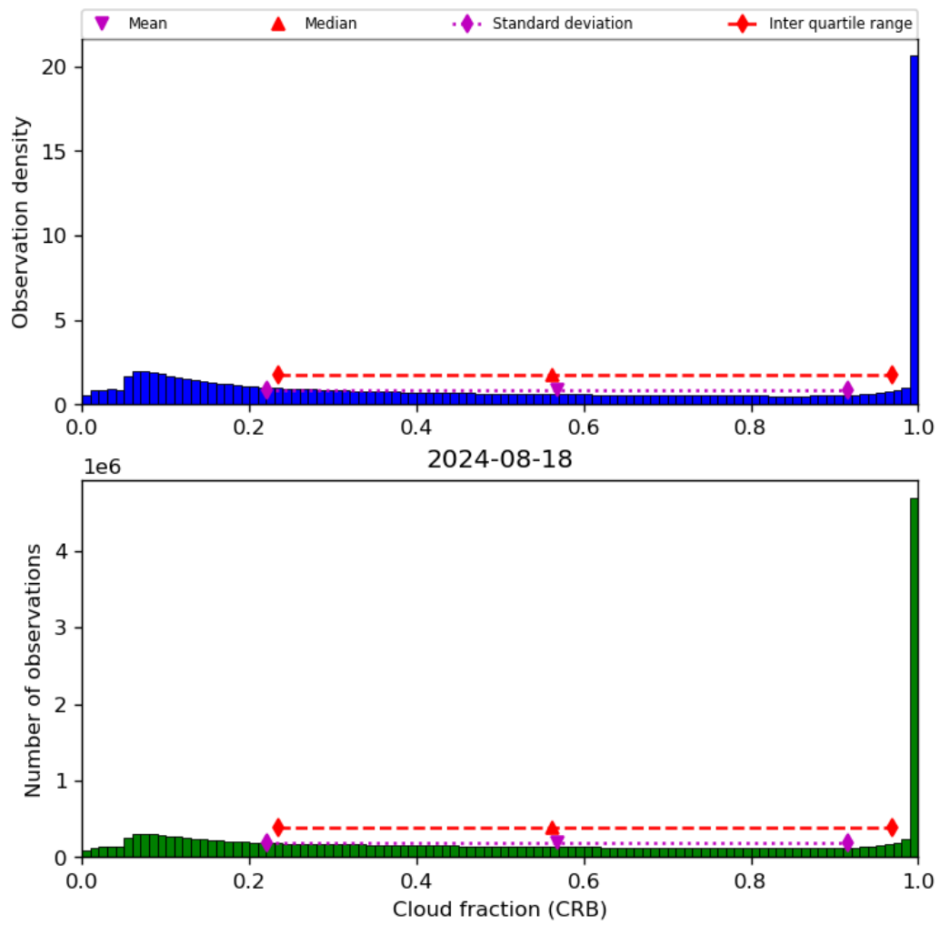
Figure 42: Histogram of “Cloud fraction (CRB)” for 2024-08-17 to 2024-08-19
