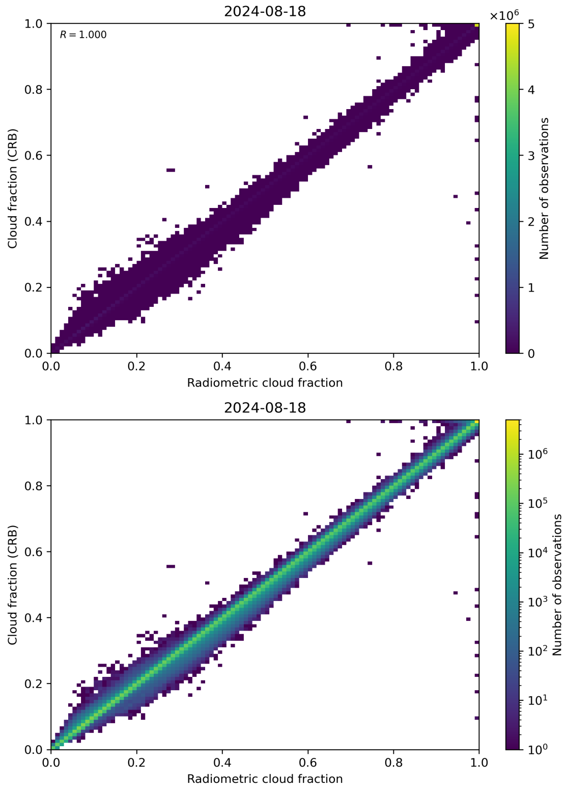
Figure 73: Scatter density plot of “Radiometric cloud fraction” against “Cloud fraction (CRB)” for 2024-08-17 to 2024-08-19.
