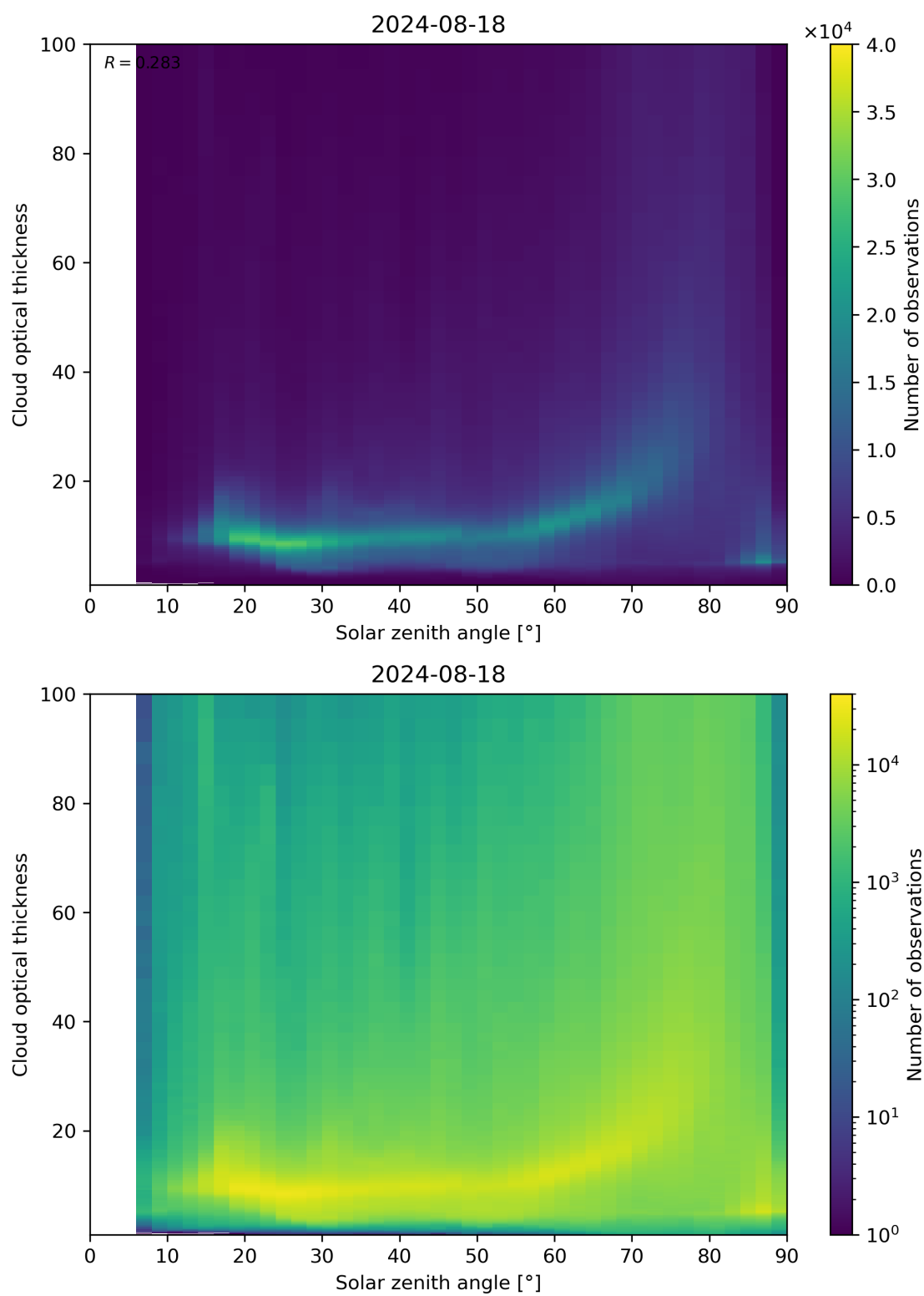
Figure 103: Scatter density plot of “Solar zenith angle” against “Cloud optical thickness” for 2024-08-17 to 2024-08-19.
