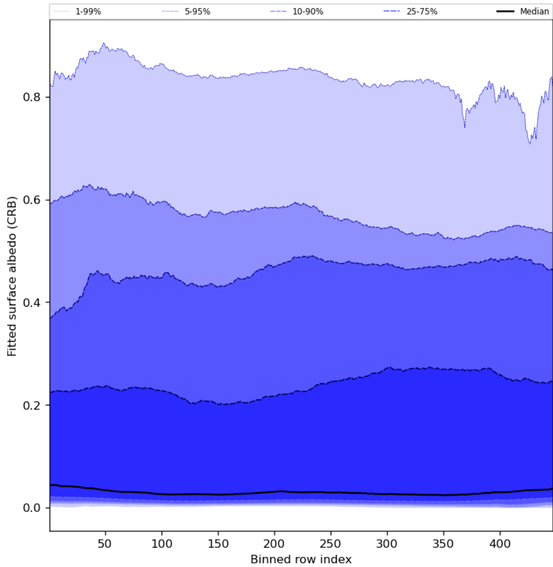
Figure 62: Along track statistics of “Fitted surface albedo (CRB)” for 2024-08-17 to 2024-08-19
