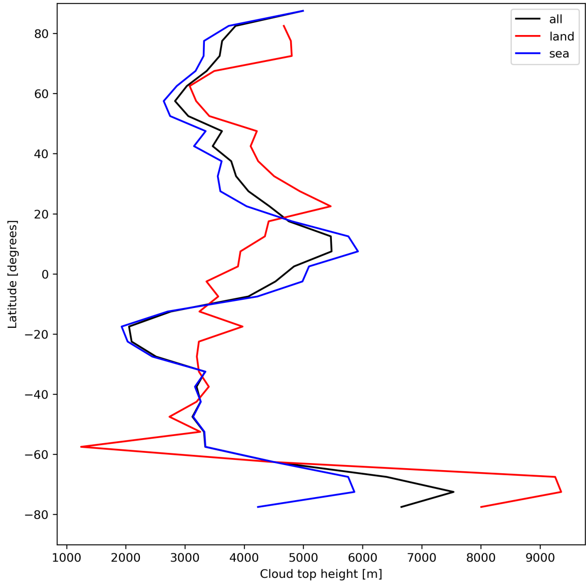
Figure 24: Zonal average of “Cloud top height” for 2024-08-17 to 2024-08-19.
