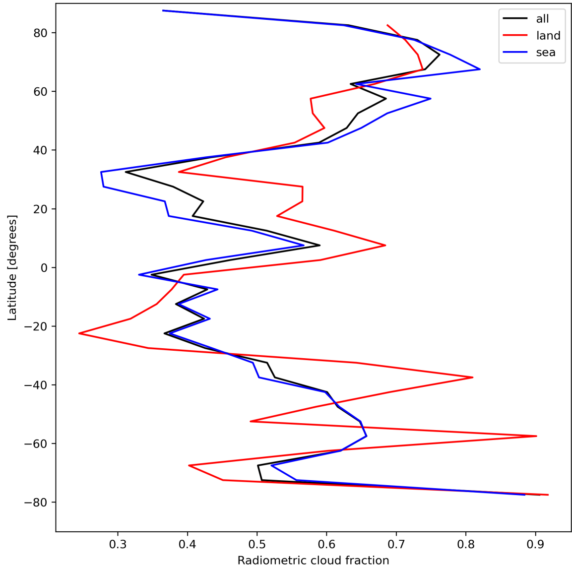
Figure 23: Zonal average of “Radiometric cloud fraction” for 2024-08-17 to 2024-08-19.
