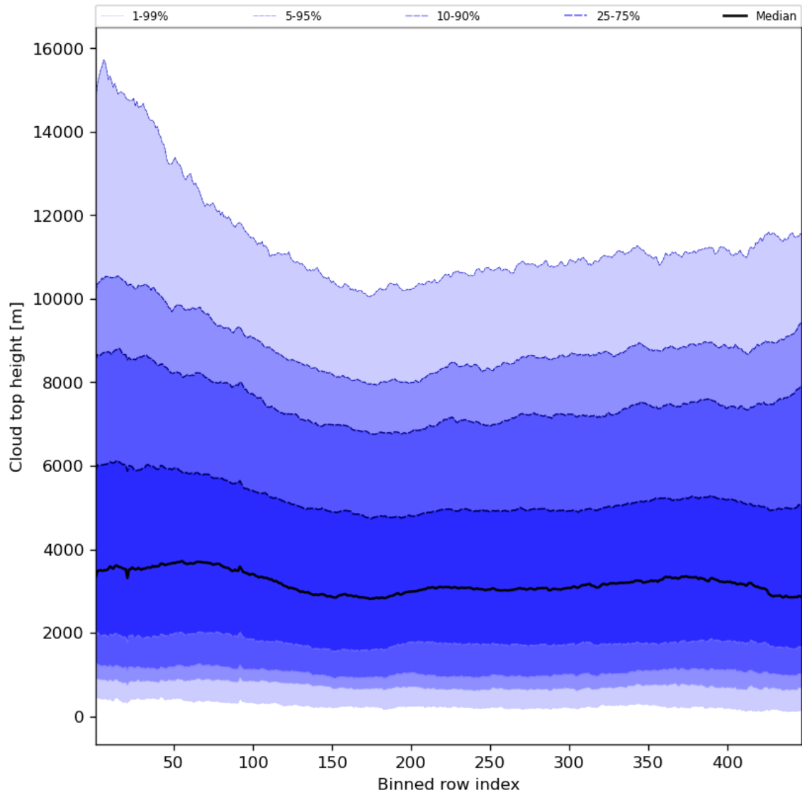
Figure 56: Along track statistics of “Cloud top height” for 2024-08-17 to 2024-08-19
