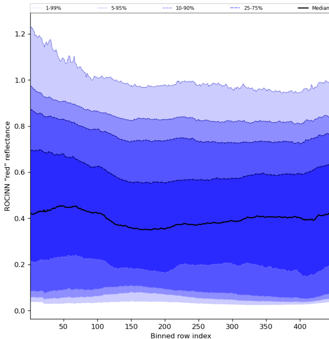
Figure 69: Along track statistics of “ROCINN “red” reflectance” for 2024-08-17 to 2024-08-19
