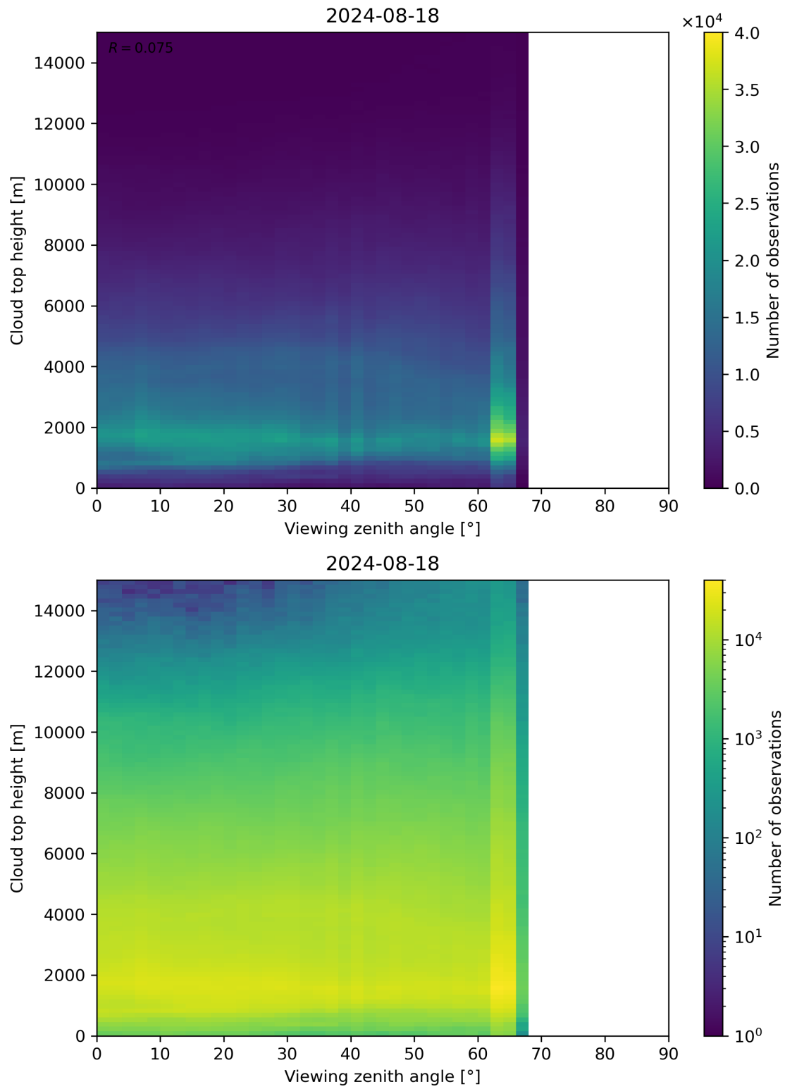
Figure 112: Scatter density plot of “Viewing zenith angle” against “Cloud top height” for 2024-08-17 to 2024-08-19.
