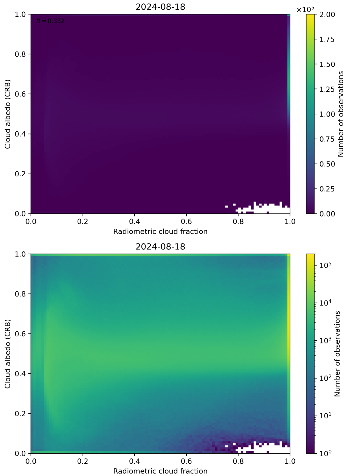
Figure 71: Scatter density plot of “Radiometric cloud fraction” against “Cloud albedo (CRB)” for 2024-08-17 to 2024-08-19.
