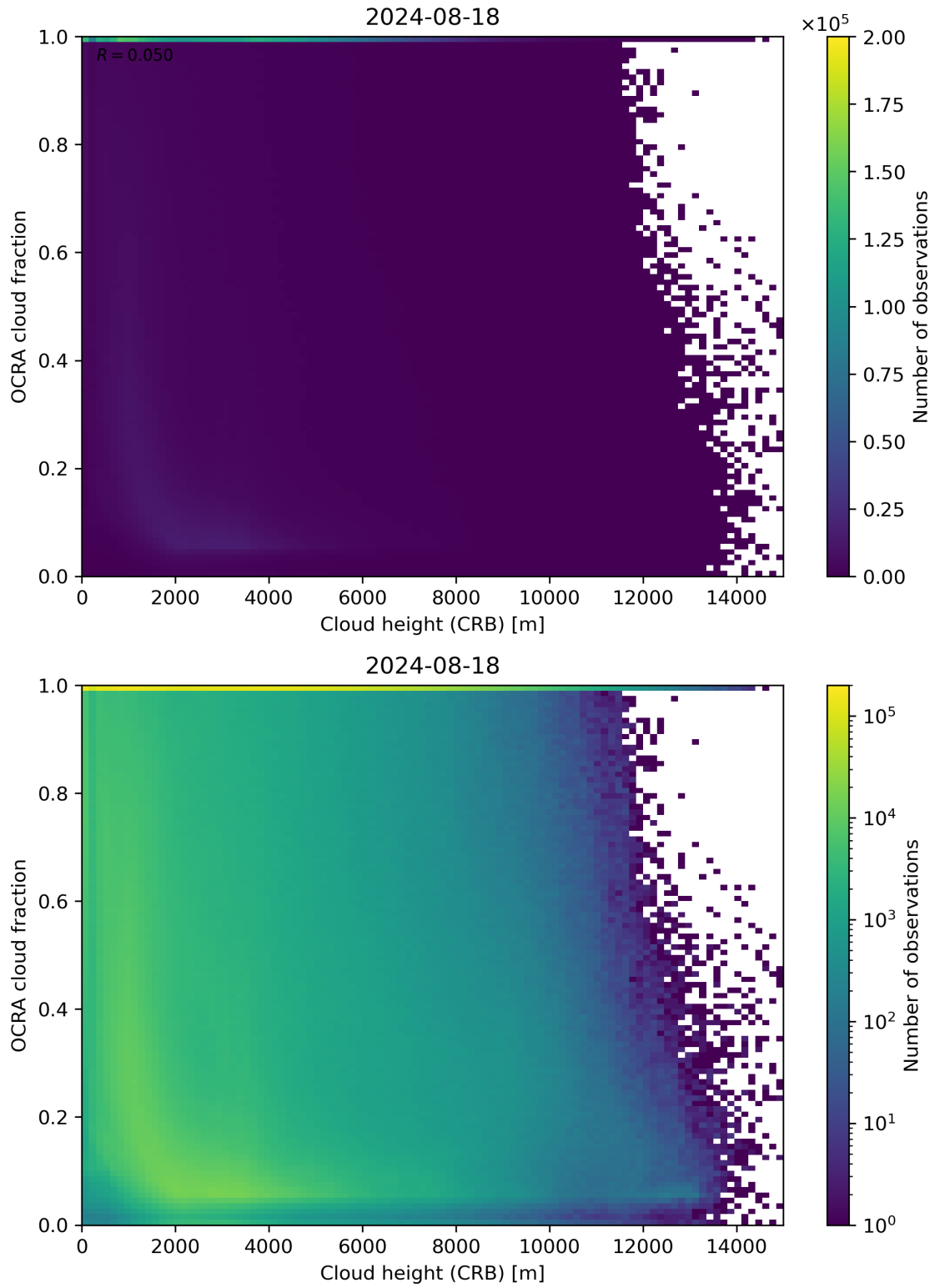
Figure 81: Scatter density plot of “Cloud height (CRB)” against “OCRA cloud fraction” for 2024-08-17 to 2024-08-19.
