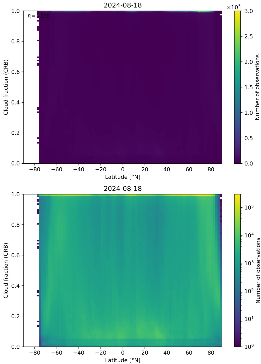
Figure 94: Scatter density plot of “Latitude” against “Cloud fraction (CRB)” for 2024-08-17 to 2024-08-19.
