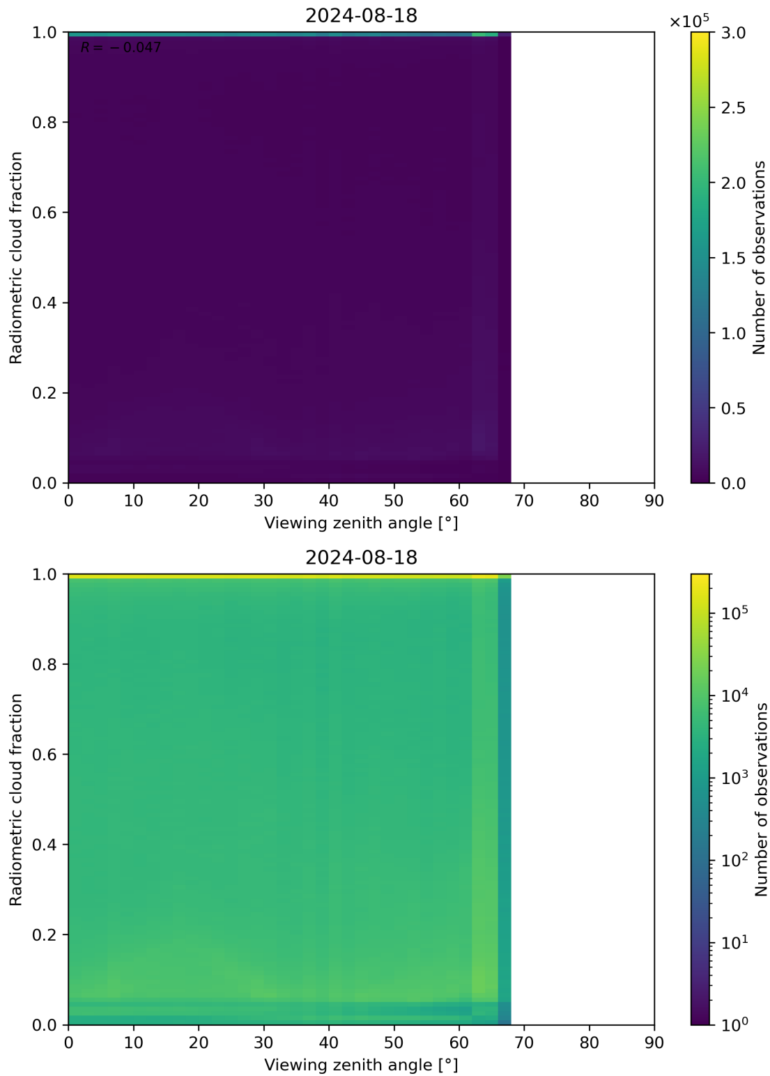
Figure 107: Scatter density plot of “Viewing zenith angle” against “Radiometric cloud fraction” for 2024-08-17 to 2024-08-19.
