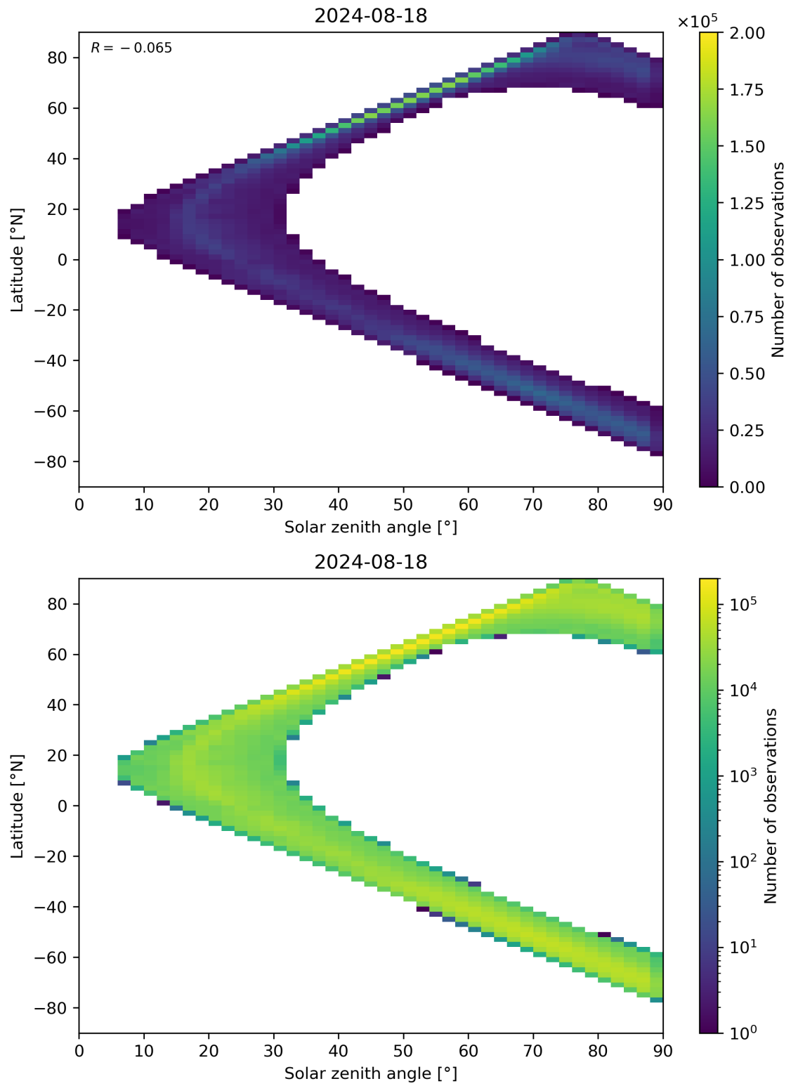
Figure 105: Scatter density plot of “Solar zenith angle” against “Latitude” for 2024-08-17 to 2024-08-19.
