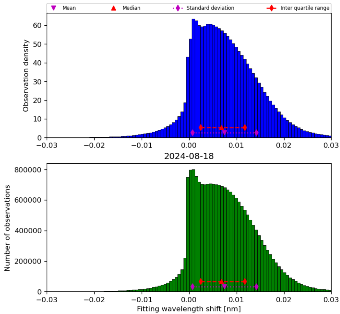
Figure 49: Histogram of “Fitting wavelength shift” for 2024-08-17 to 2024-08-19
