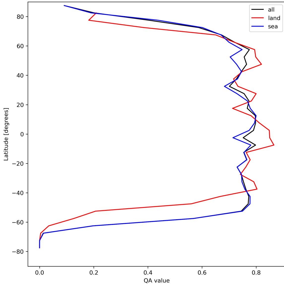
Figure 22: Zonal average of “QA value” for 2024-08-17 to 2024-08-19.
