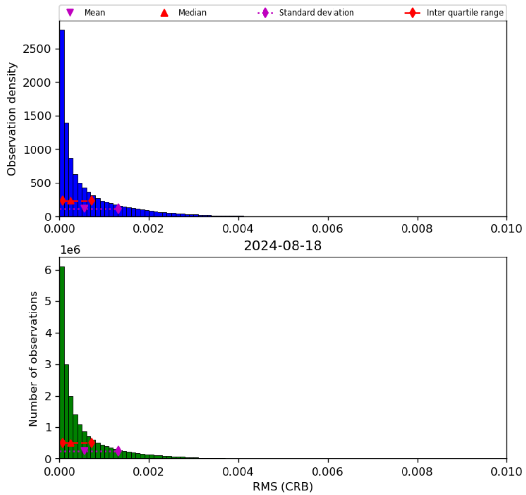
Figure 48: Histogram of “RMS (CRB)” for 2024-08-17 to 2024-08-19
