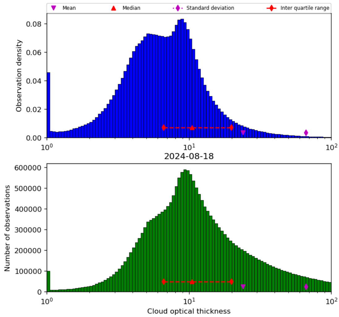
Figure 41: Histogram of “Cloud optical thickness” for 2024-08-17 to 2024-08-19
