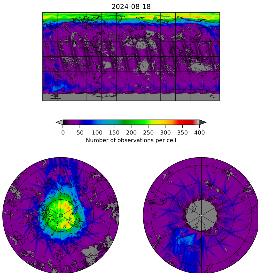
Figure 21: Map of the number of observations for 2024-08-17 to 2024-08-19
