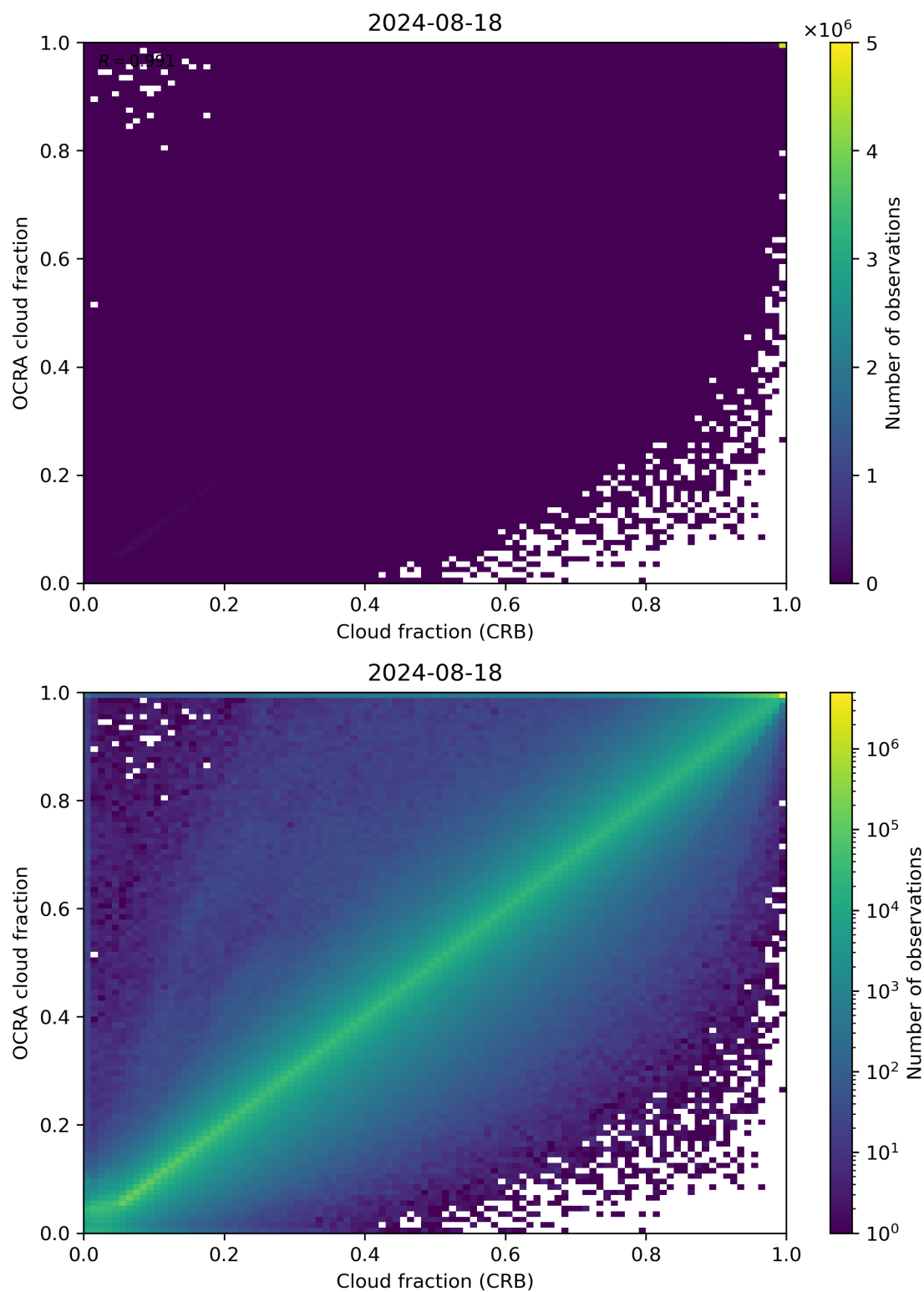
Figure 78: Scatter density plot of “Cloud fraction (CRB)” against “OCRA cloud fraction” for 2024-08-17 to 2024-08-19.
