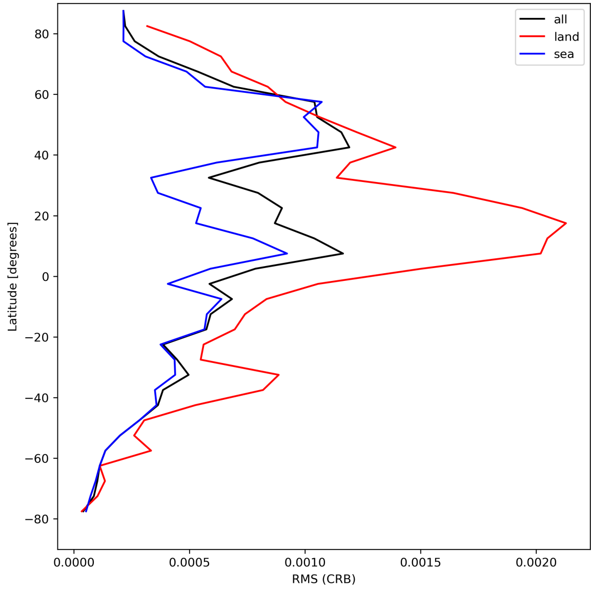
Figure 32: Zonal average of “RMS (CRB)” for 2024-08-17 to 2024-08-19.
