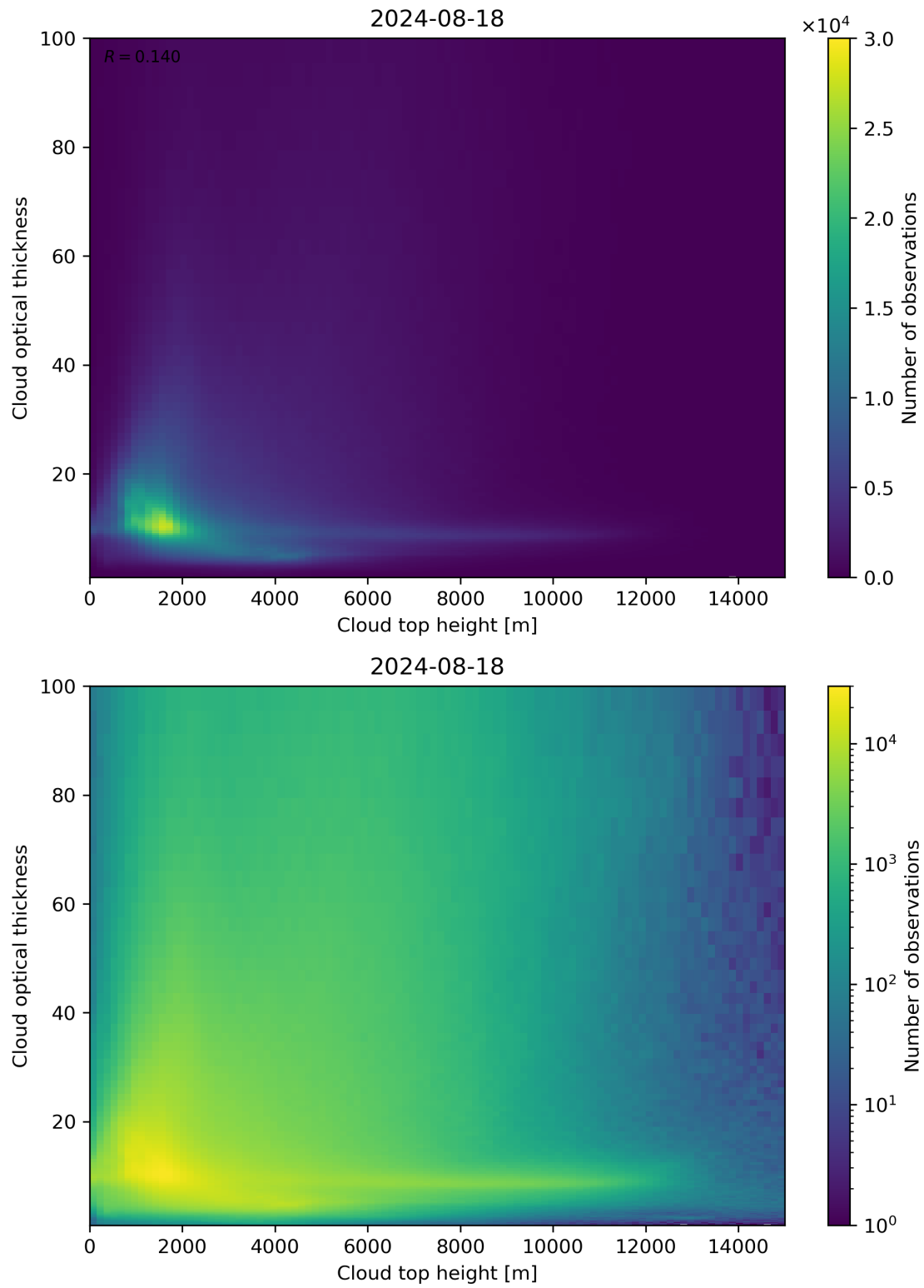
Figure 90: Scatter density plot of “Cloud top height” against “Cloud optical thickness” for 2024-08-17 to 2024-08-19.
