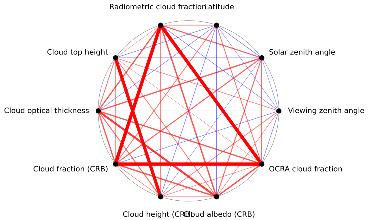
Figure 1: Map of correlation graph for 2024-08-17 to 2024-08-19.
