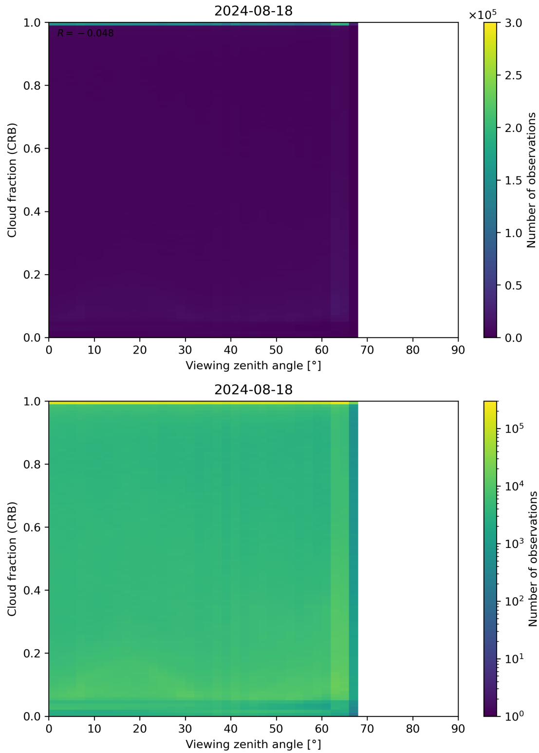
Figure 109: Scatter density plot of “Viewing zenith angle” against “Cloud fraction (CRB)” for 2024-08-17 to 2024-08-19.
