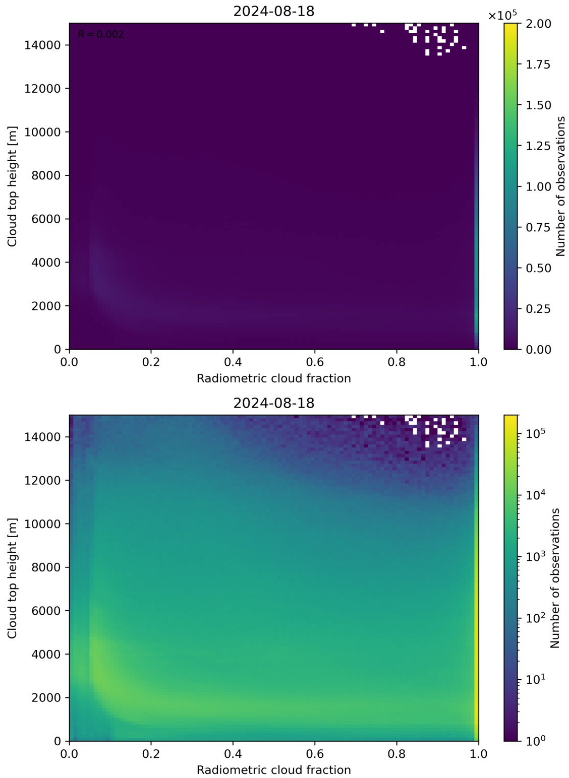
Figure 76: Scatter density plot of “Radiometric cloud fraction” against “Cloud top height” for 2024-08-17 to 2024-08-19.
