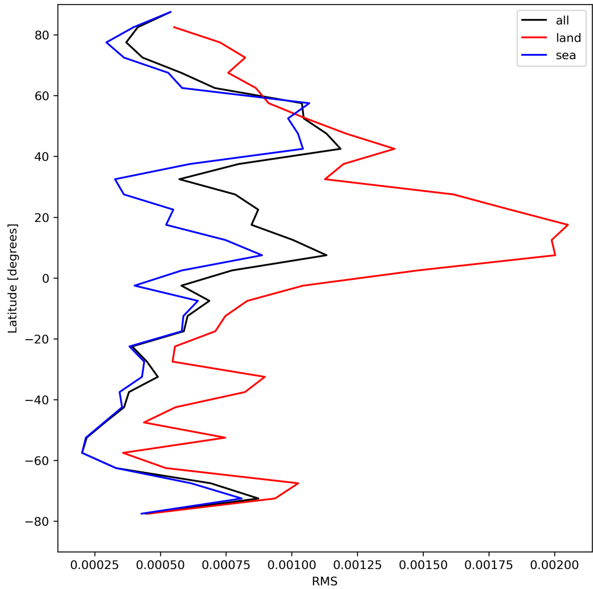
Figure 31: Zonal average of “RMS” for 2024-08-17 to 2024-08-19.
