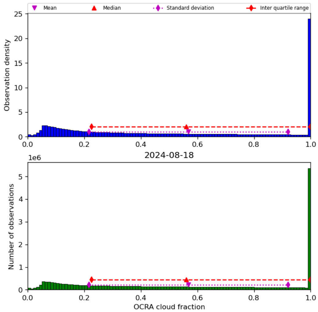
Figure 50: Histogram of “OCRA cloud fraction” for 2024-08-17 to 2024-08-19
