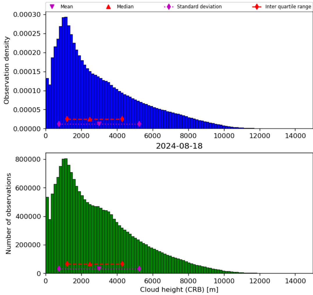
Figure 43: Histogram of “Cloud height (CRB)” for 2024-08-17 to 2024-08-19
