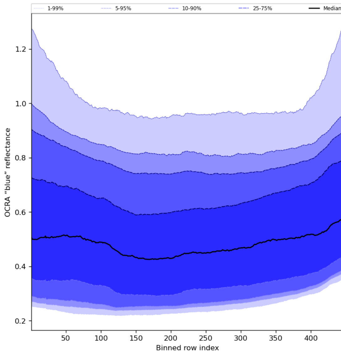
Figure 67: Along track statistics of “OCRA “blue” reflectance” for 2024-08-17 to 2024-08-19
