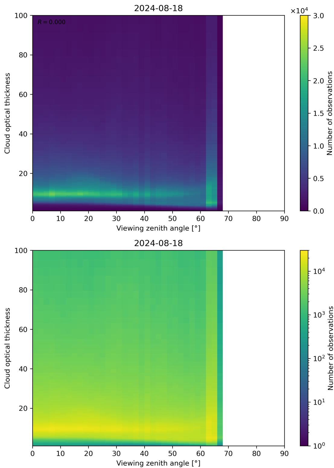
Figure 111: Scatter density plot of “Viewing zenith angle” against “Cloud optical thickness” for 2024-08-17 to 2024-08-19.
