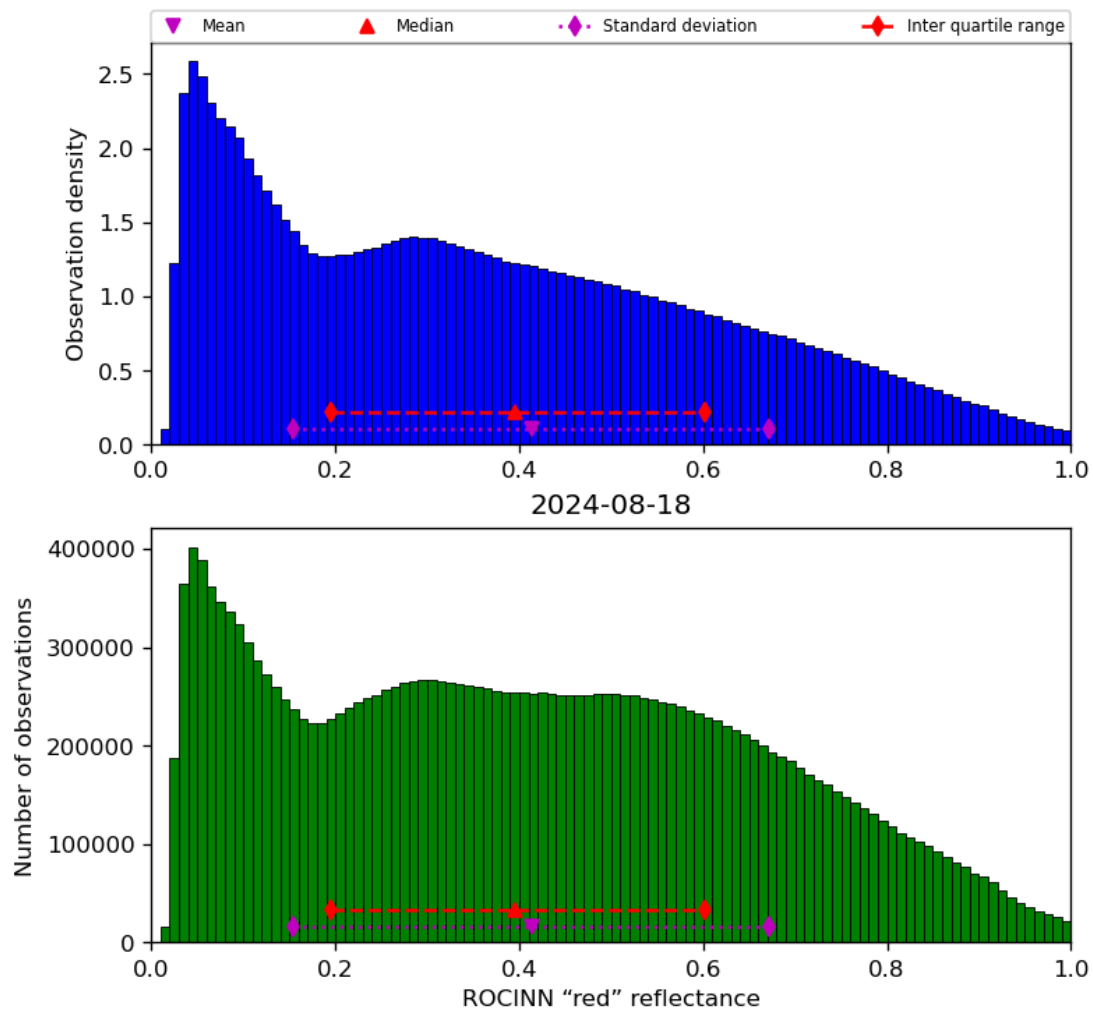
Figure 53: Histogram of “ROCINN “red” reflectance” for 2024-08-17 to 2024-08-19
