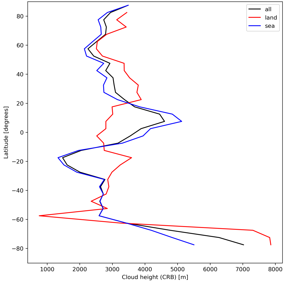
Figure 27: Zonal average of “Cloud height (CRB)” for 2024-08-17 to 2024-08-19.
