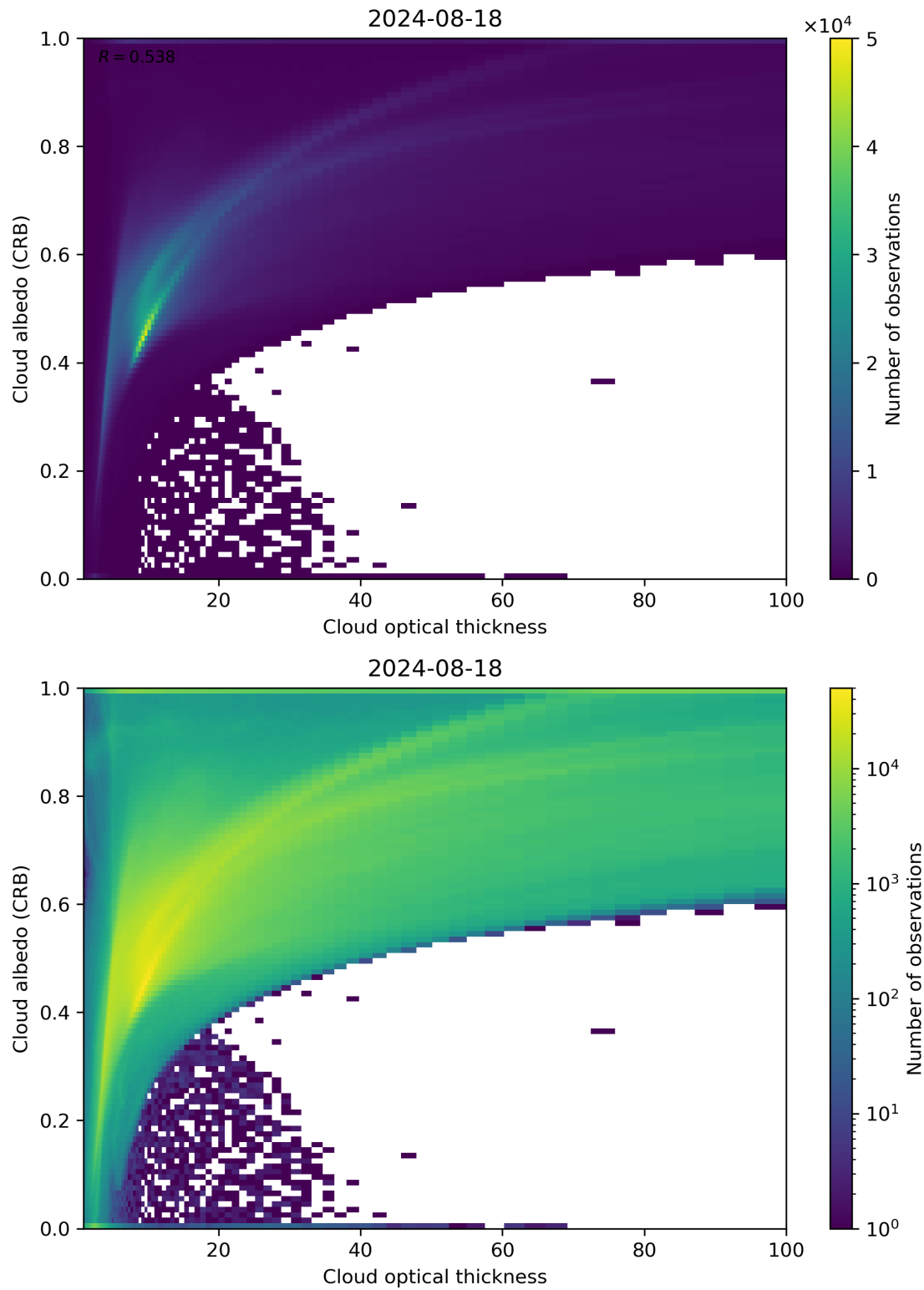
Figure 82: Scatter density plot of “Cloud optical thickness” against “Cloud albedo (CRB)” for 2024-08-17 to 2024-08-19.
