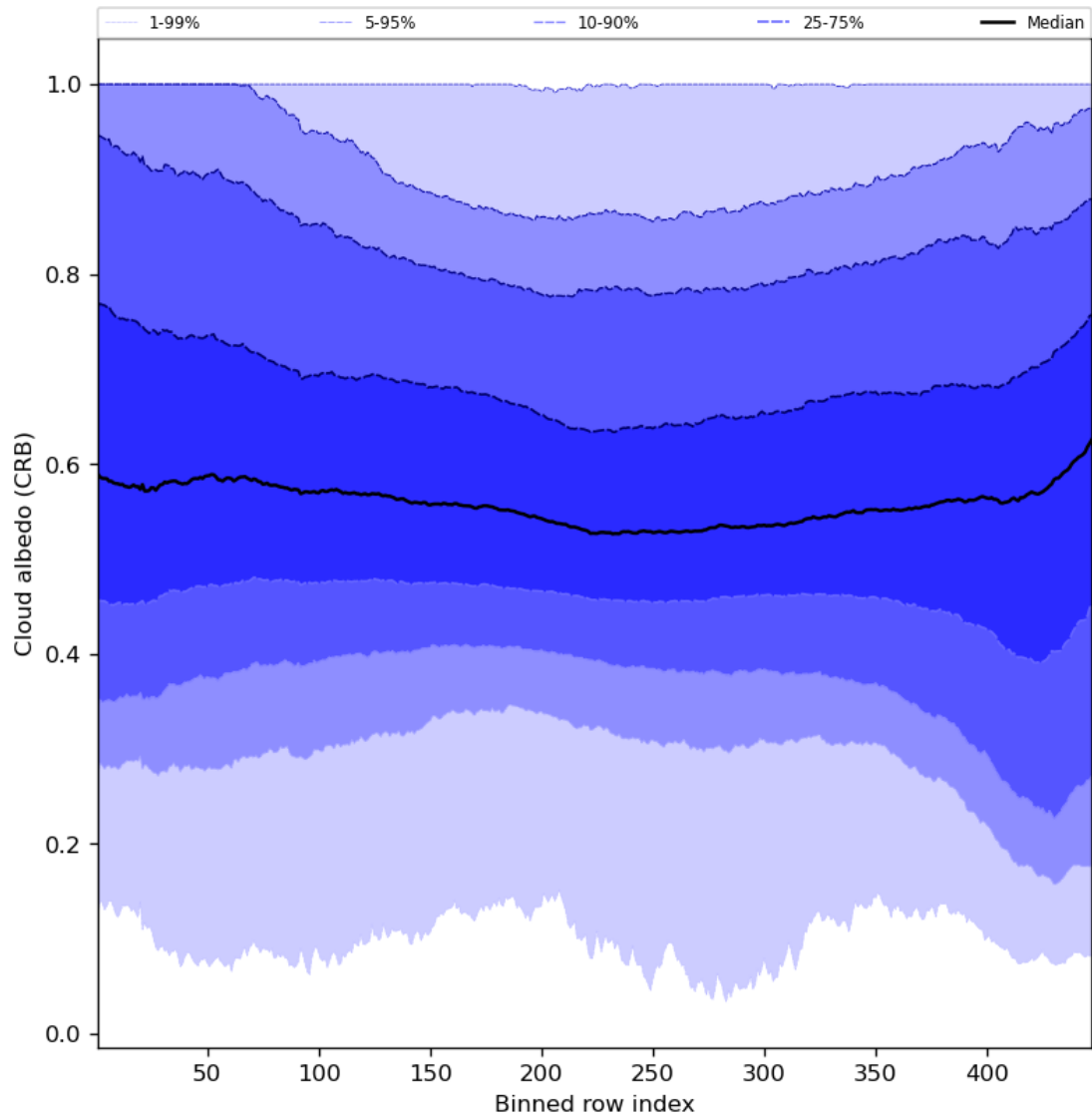
Figure 60: Along track statistics of “Cloud albedo (CRB)” for 2024-08-17 to 2024-08-19
