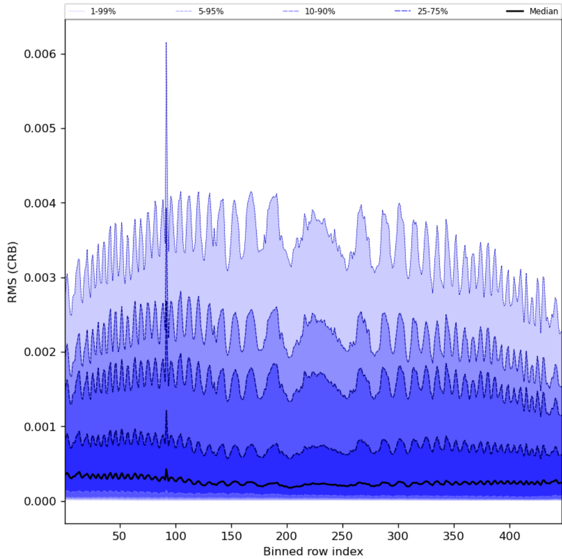
Figure 64: Along track statistics of “RMS (CRB)” for 2024-08-17 to 2024-08-19
