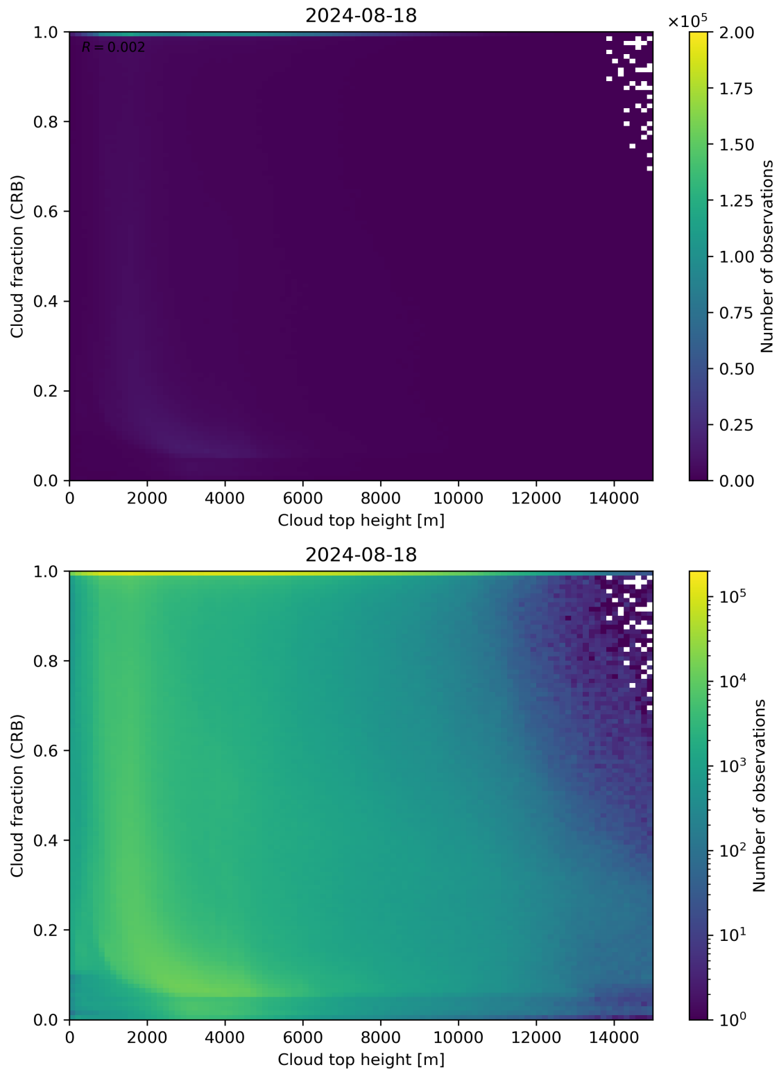
Figure 88: Scatter density plot of “Cloud top height” against “Cloud fraction (CRB)” for 2024-08-17 to 2024-08-19.
