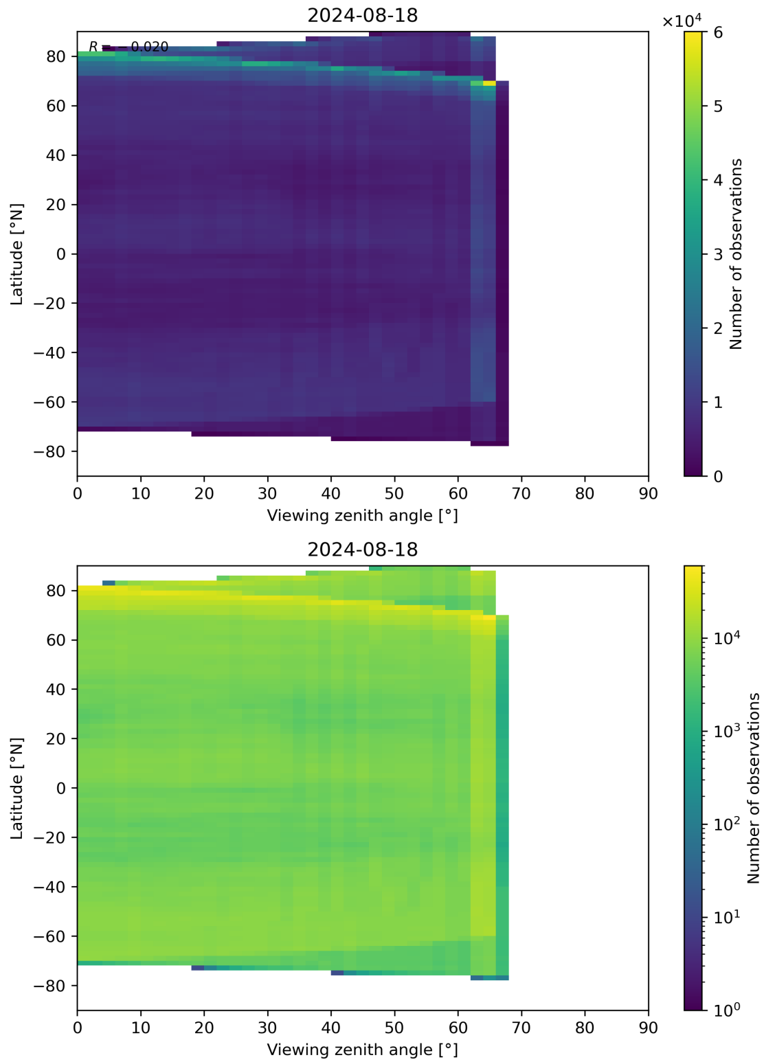
Figure 113: Scatter density plot of “Viewing zenith angle” against “Latitude” for 2024-08-17 to 2024-08-19.
