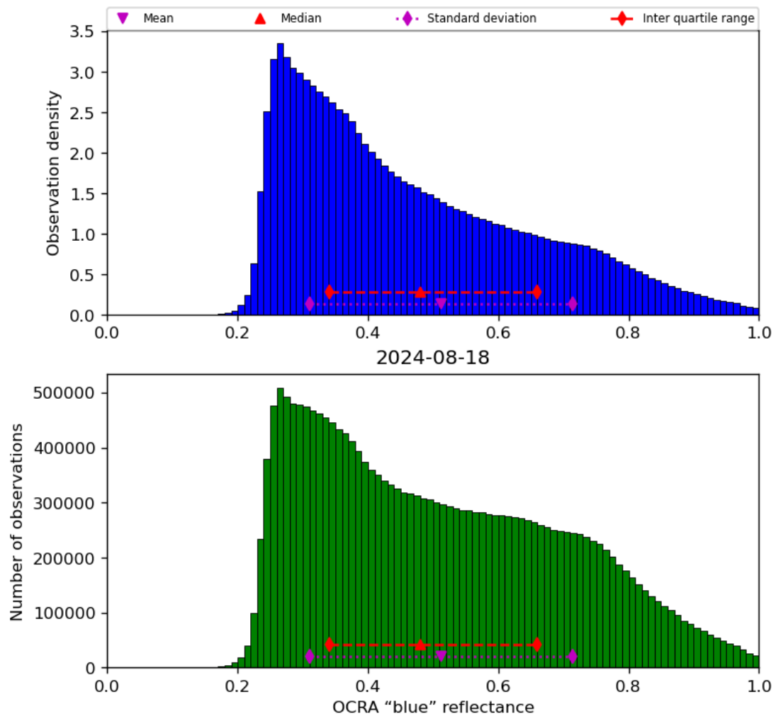
Figure 51: Histogram of “OCRA “blue” reflectance” for 2024-08-17 to 2024-08-19
