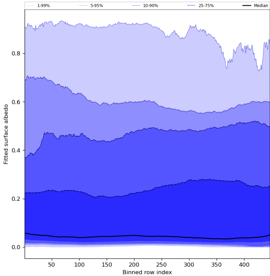
Figure 61: Along track statistics of “Fitted surface albedo” for 2024-08-17 to 2024-08-19
