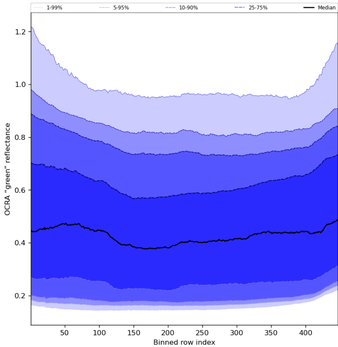
Figure 68: Along track statistics of “OCRA “green” reflectance” for 2024-08-17 to 2024-08-19
