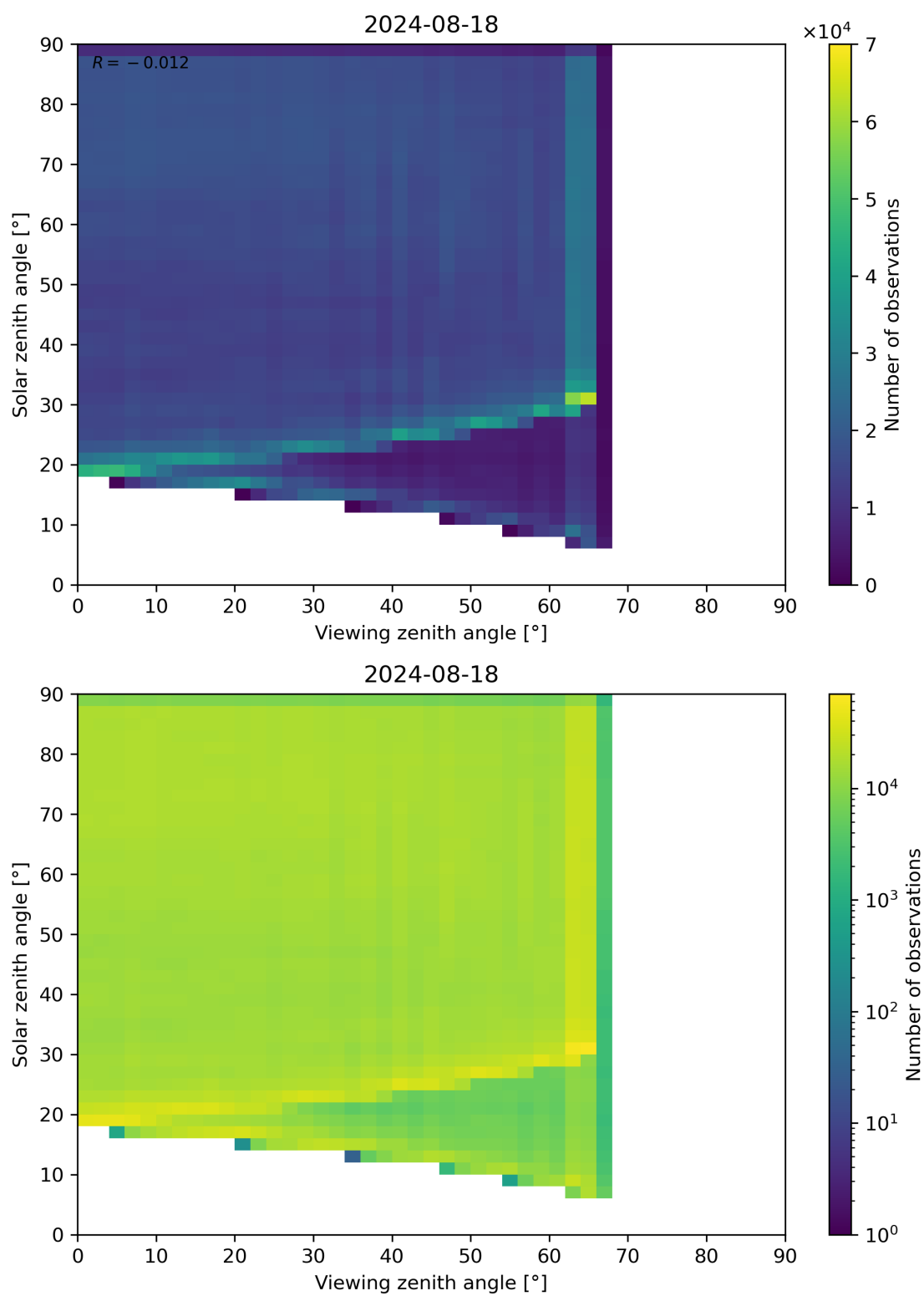
Figure 114: Scatter density plot of “Viewing zenith angle” against “Solar zenith angle” for 2024-08-17 to 2024-08-19.
