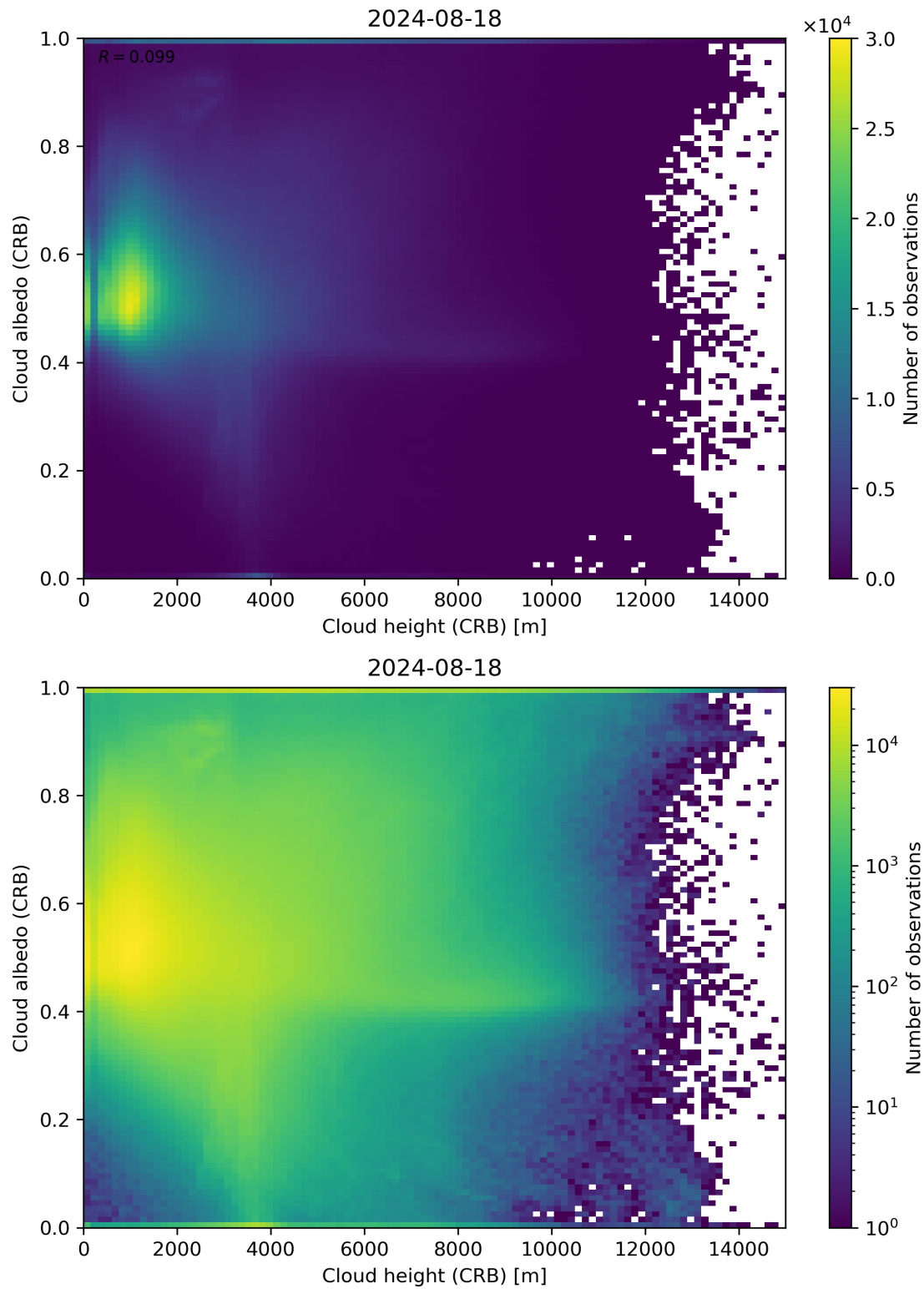
Figure 80: Scatter density plot of “Cloud height (CRB)” against “Cloud albedo (CRB)” for 2024-08-17 to 2024-08-19.
