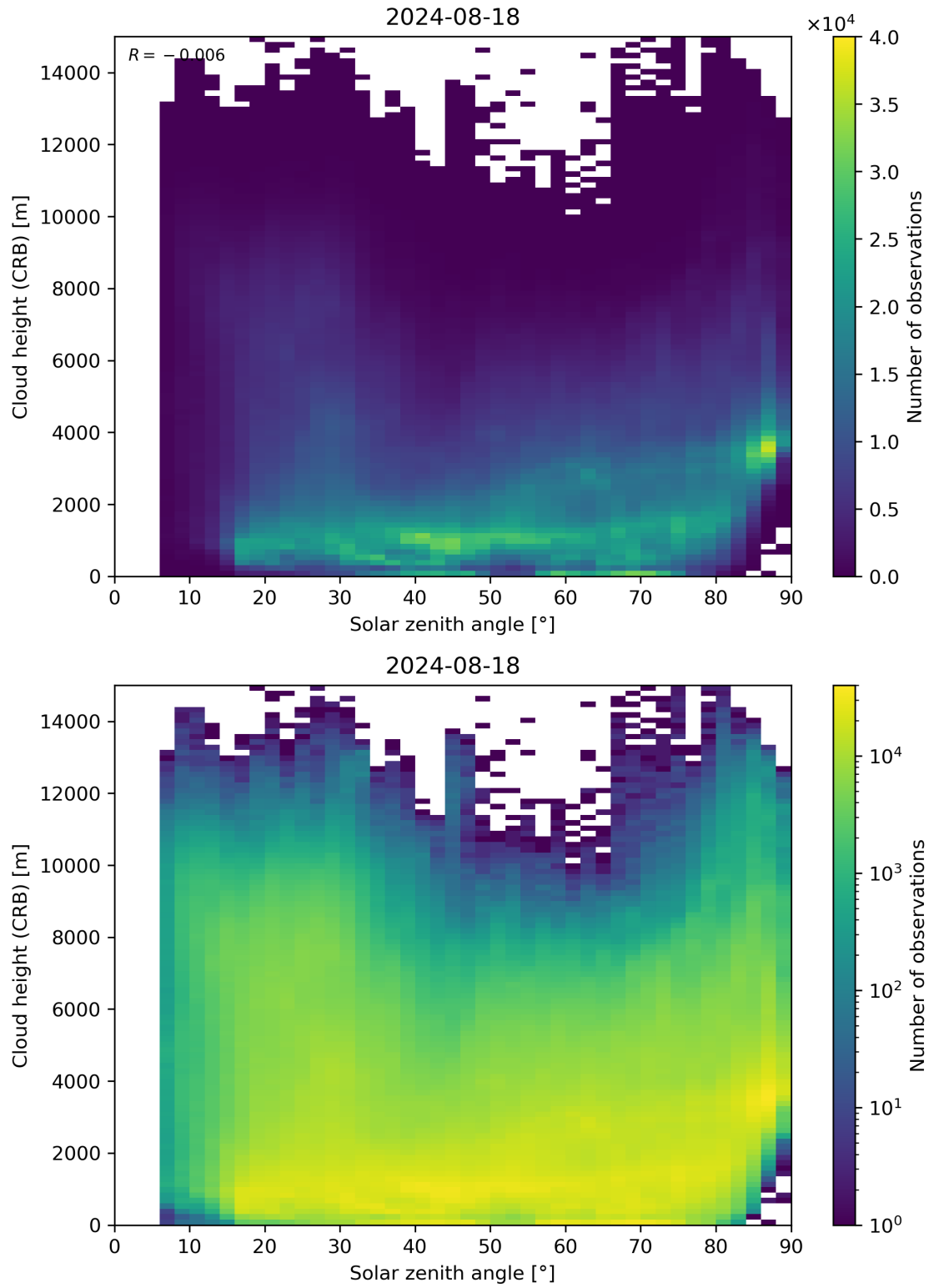
Figure 102: Scatter density plot of “Solar zenith angle” against “Cloud height (CRB)” for 2024-08-17 to 2024-08-19.
