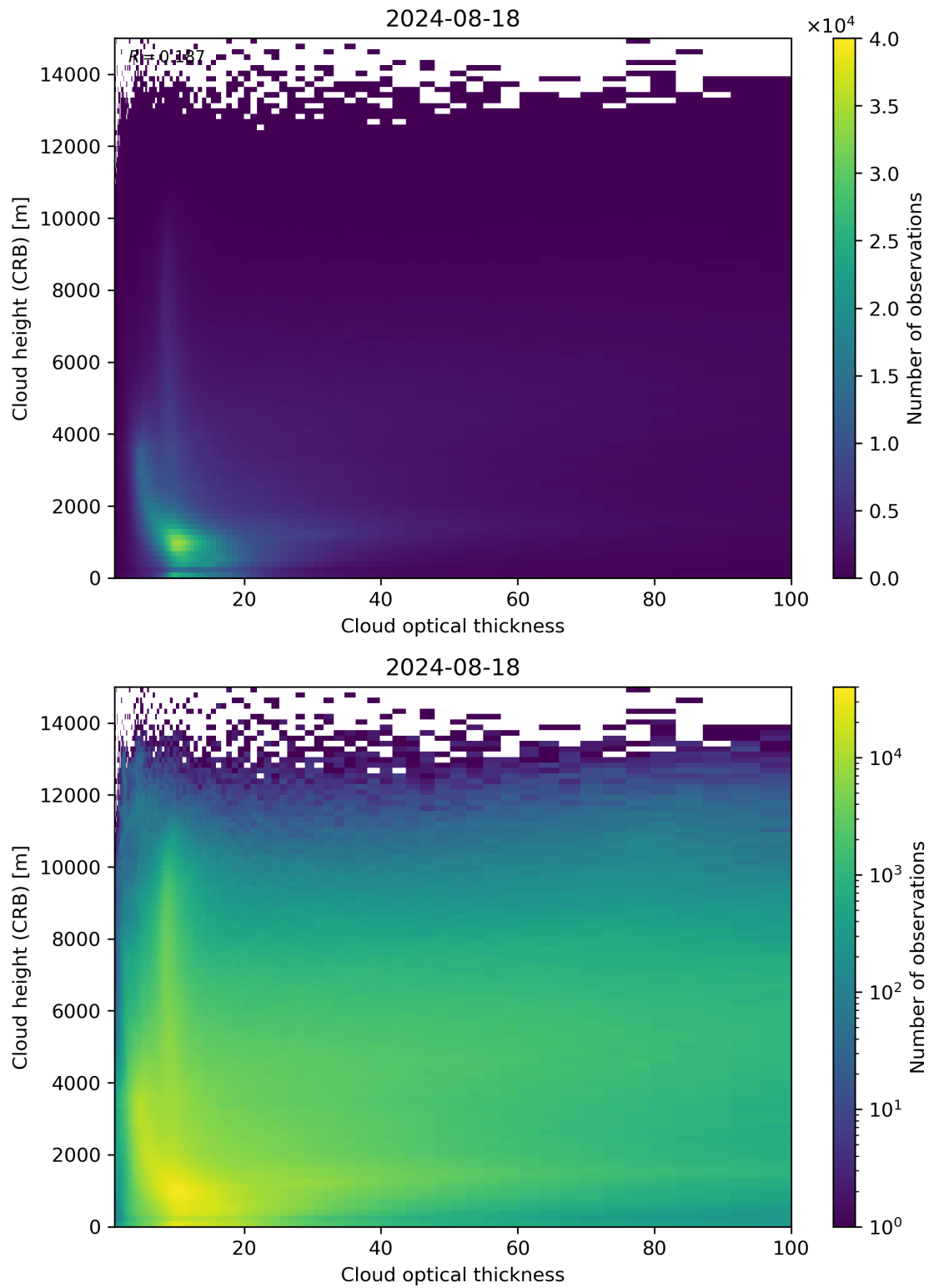
Figure 85: Scatter density plot of “Cloud optical thickness” against “Cloud height (CRB)” for 2024-08-17 to 2024-08-19.
