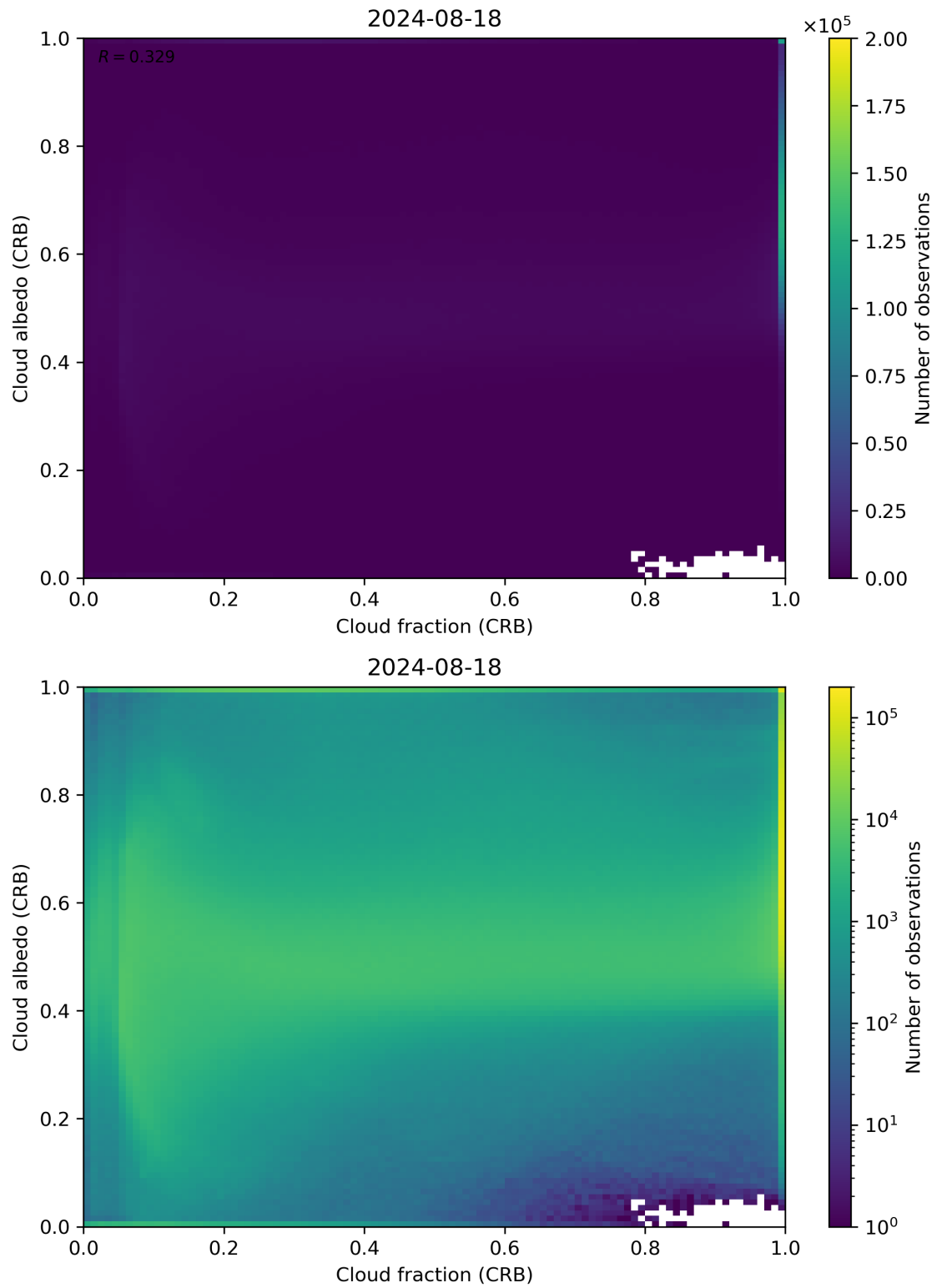
Figure 77: Scatter density plot of “Cloud fraction (CRB)” against “Cloud albedo (CRB)” for 2024-08-17 to 2024-08-19.
