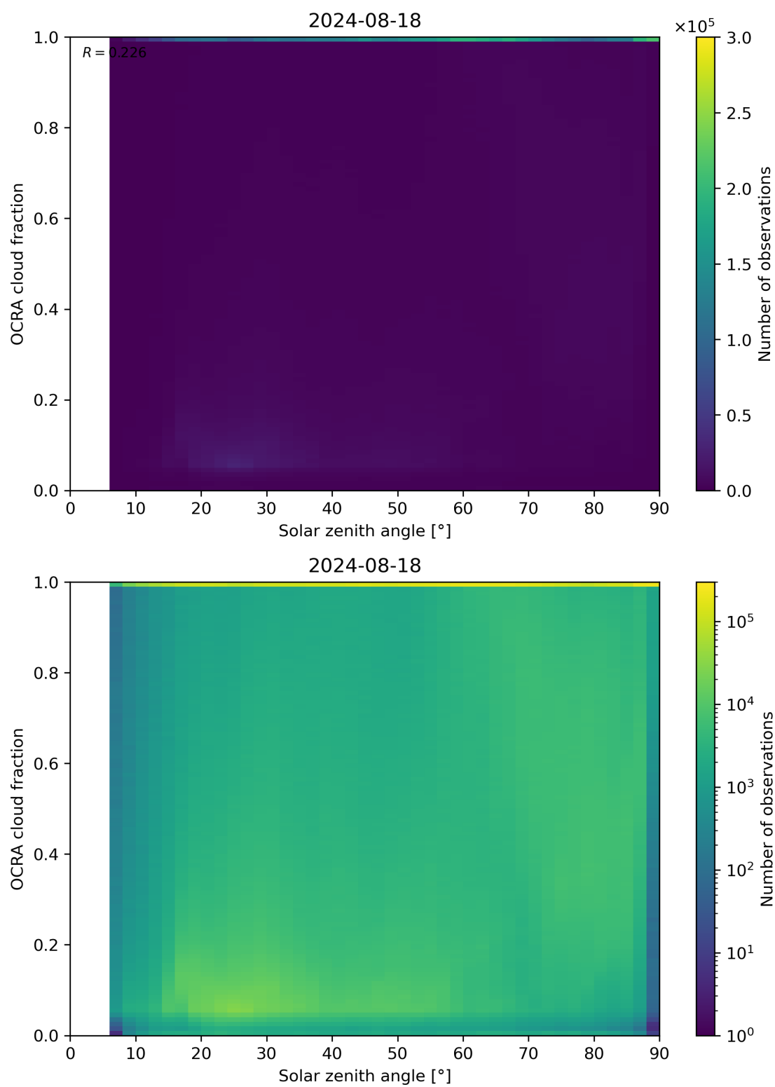
Figure 100: Scatter density plot of “Solar zenith angle” against “OCRA cloud fraction” for 2024-08-17 to 2024-08-19.
