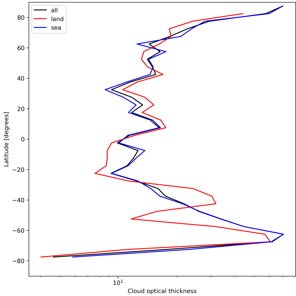
Figure 25: Zonal average of “Cloud optical thickness” for 2024-08-17 to 2024-08-19.
