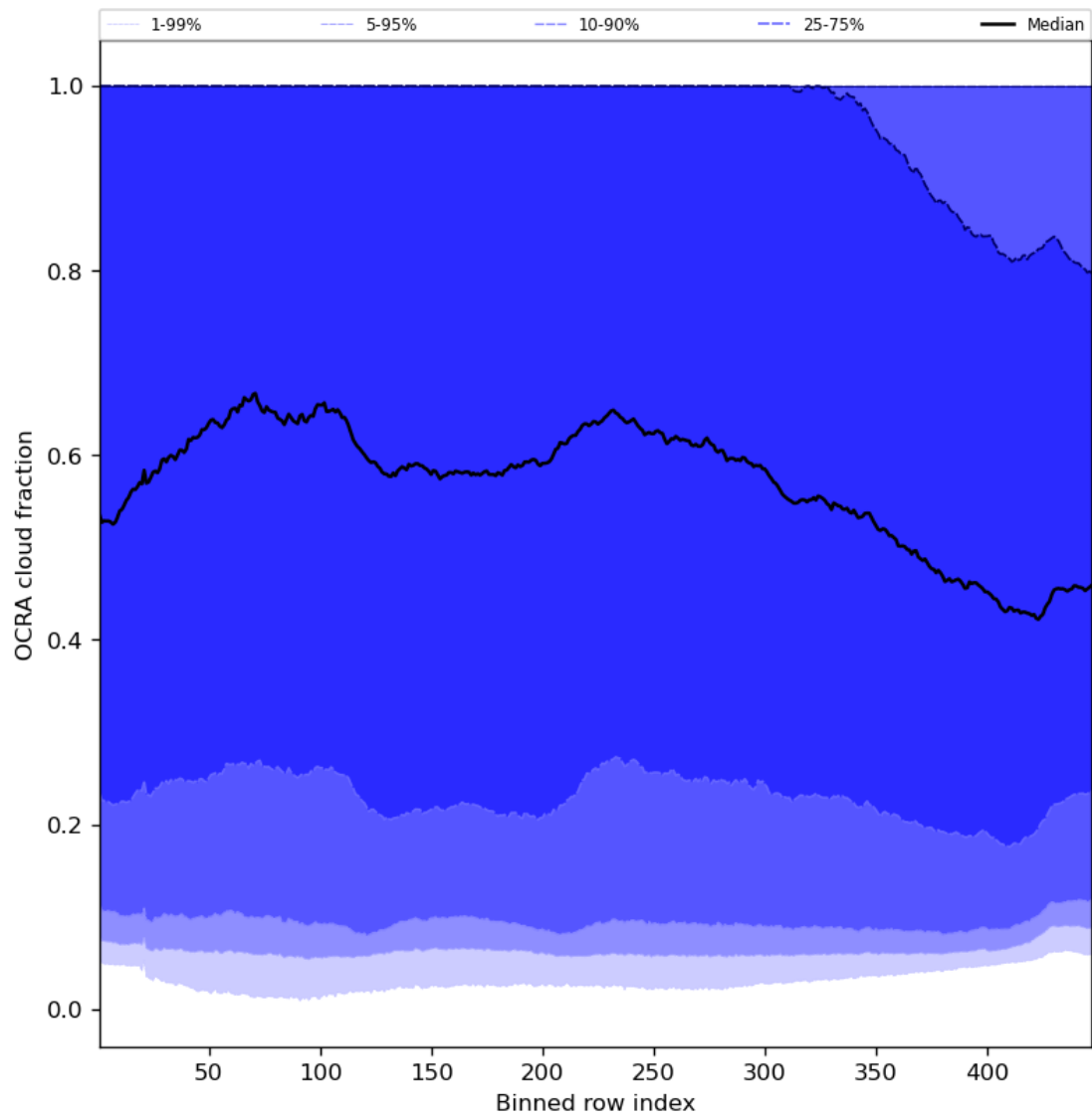
Figure 66: Along track statistics of “OCRA cloud fraction” for 2024-08-17 to 2024-08-19
