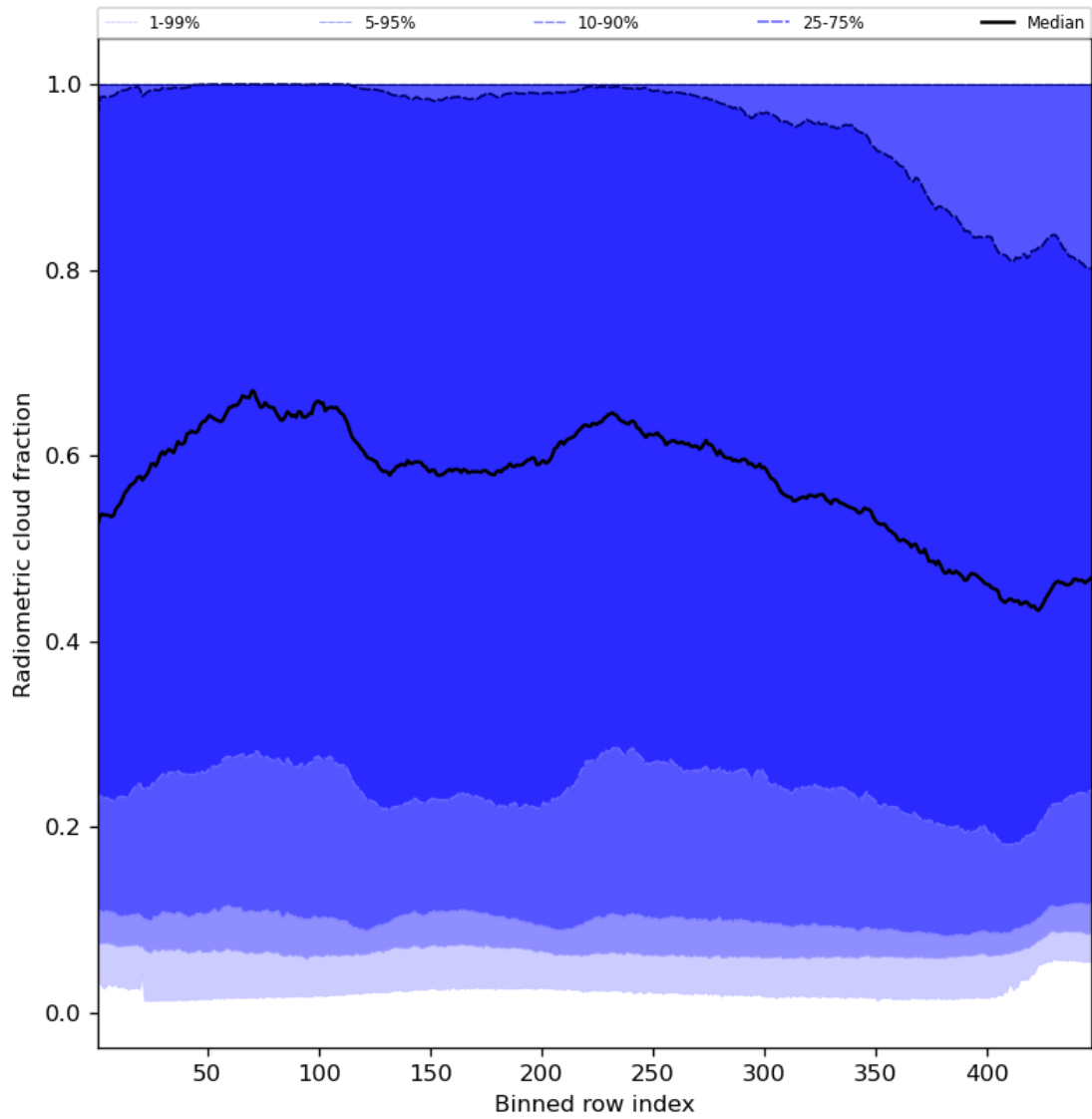
Figure 55: Along track statistics of “Radiometric cloud fraction” for 2024-08-17 to 2024-08-19
