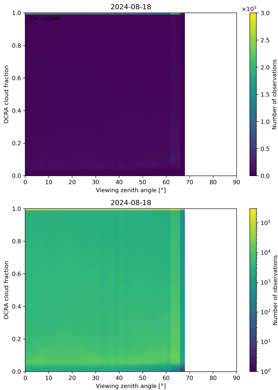
Figure 108: Scatter density plot of “Viewing zenith angle” against “OCRA cloud fraction” for 2024-08-17 to 2024-08-19.
