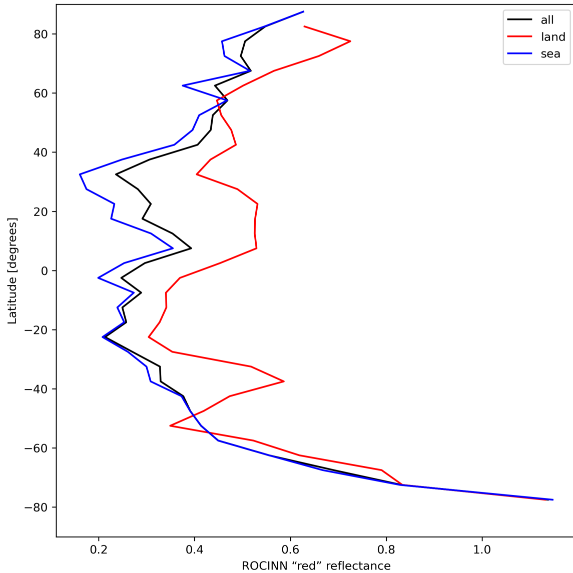
Figure 37: Zonal average of “ROCINN “red” reflectance” for 2024-08-17 to 2024-08-19.
