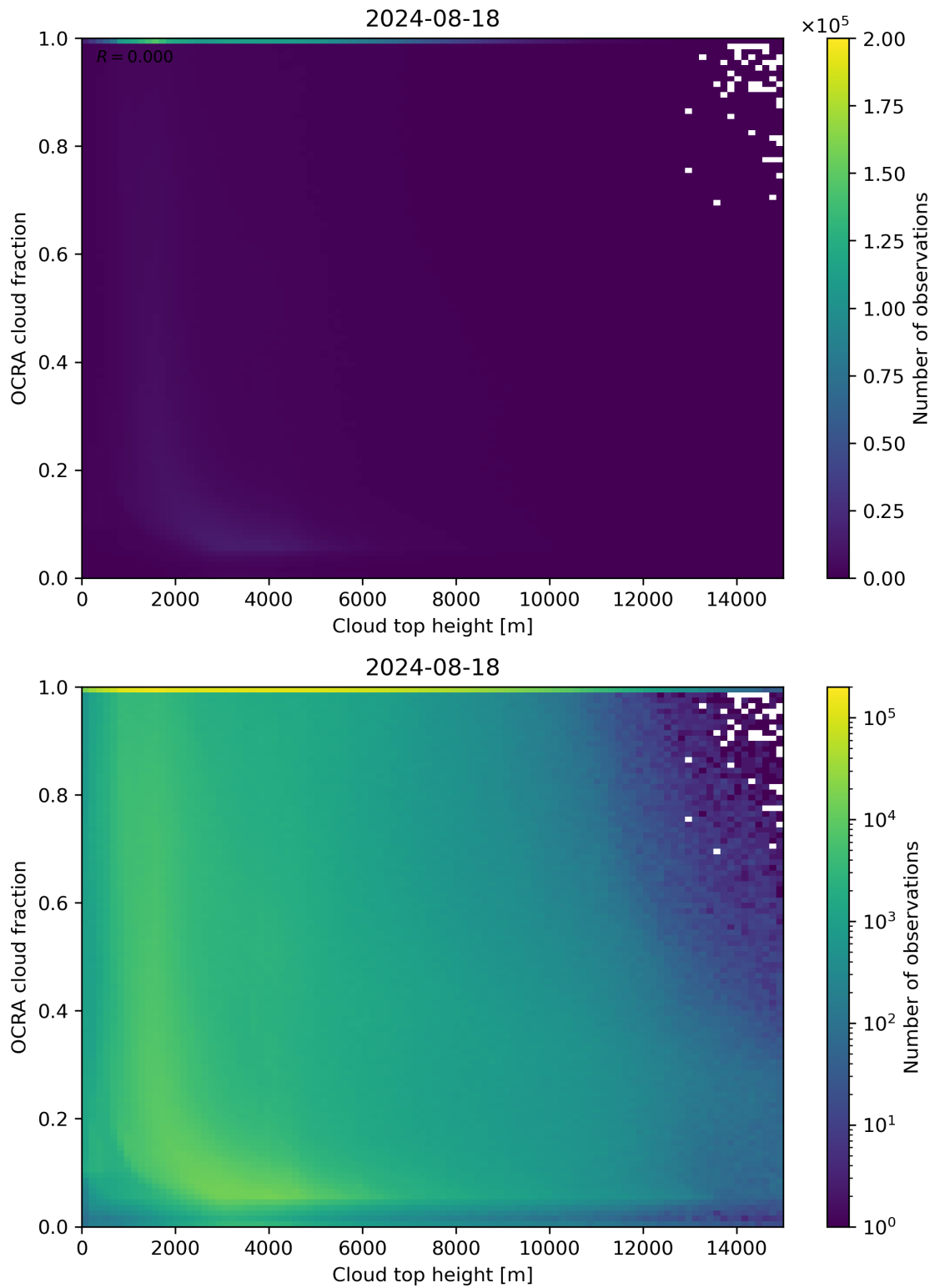
Figure 87: Scatter density plot of “Cloud top height” against “OCRA cloud fraction” for 2024-08-17 to 2024-08-19.
