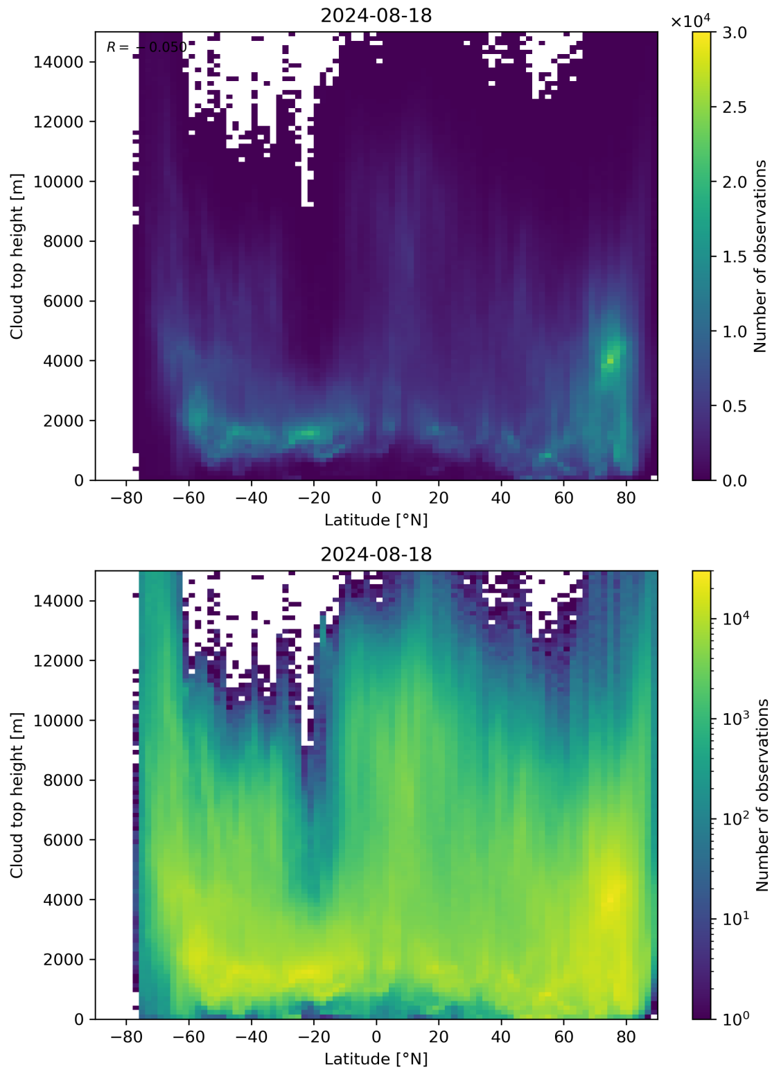
Figure 97: Scatter density plot of “Latitude” against “Cloud top height” for 2024-08-17 to 2024-08-19.
