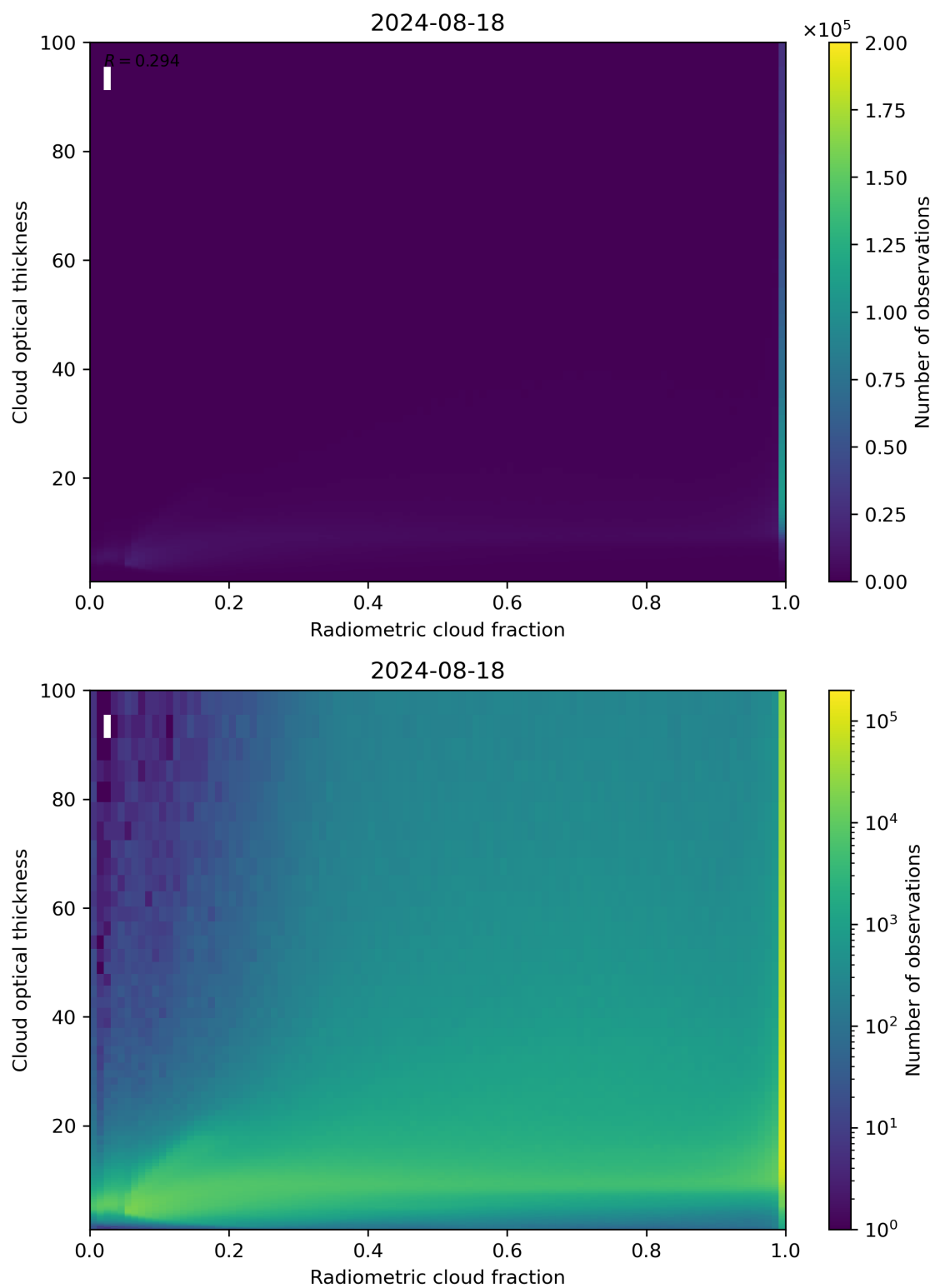
Figure 75: Scatter density plot of “Radiometric cloud fraction” against “Cloud optical thickness” for 2024-08-17 to 2024-08-19.
