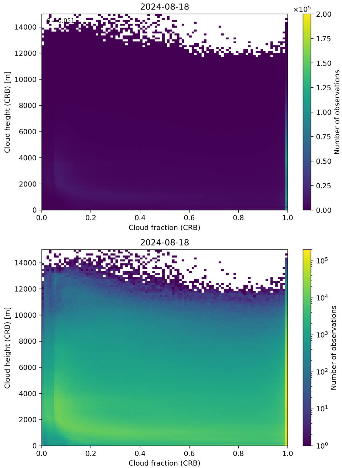
Figure 79: Scatter density plot of “Cloud fraction (CRB)” against “Cloud height (CRB)” for 2024-08-17 to 2024-08-19.
