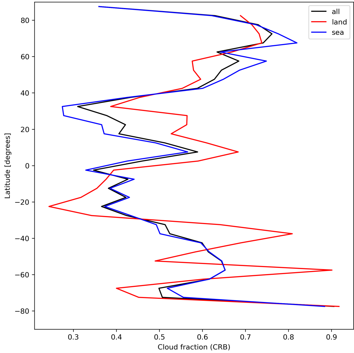
Figure 26: Zonal average of “Cloud fraction (CRB)” for 2024-08-17 to 2024-08-19.
