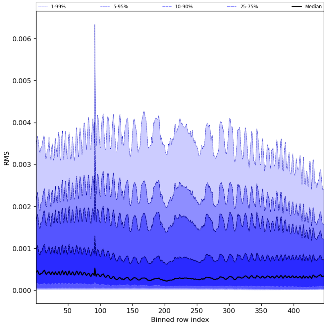
Figure 63: Along track statistics of “RMS” for 2024-08-17 to 2024-08-19
