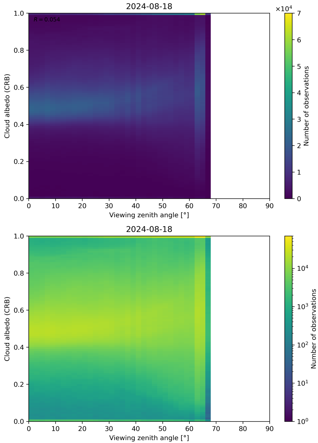
Figure 106: Scatter density plot of “Viewing zenith angle” against “Cloud albedo (CRB)” for 2024-08-17 to 2024-08-19.
