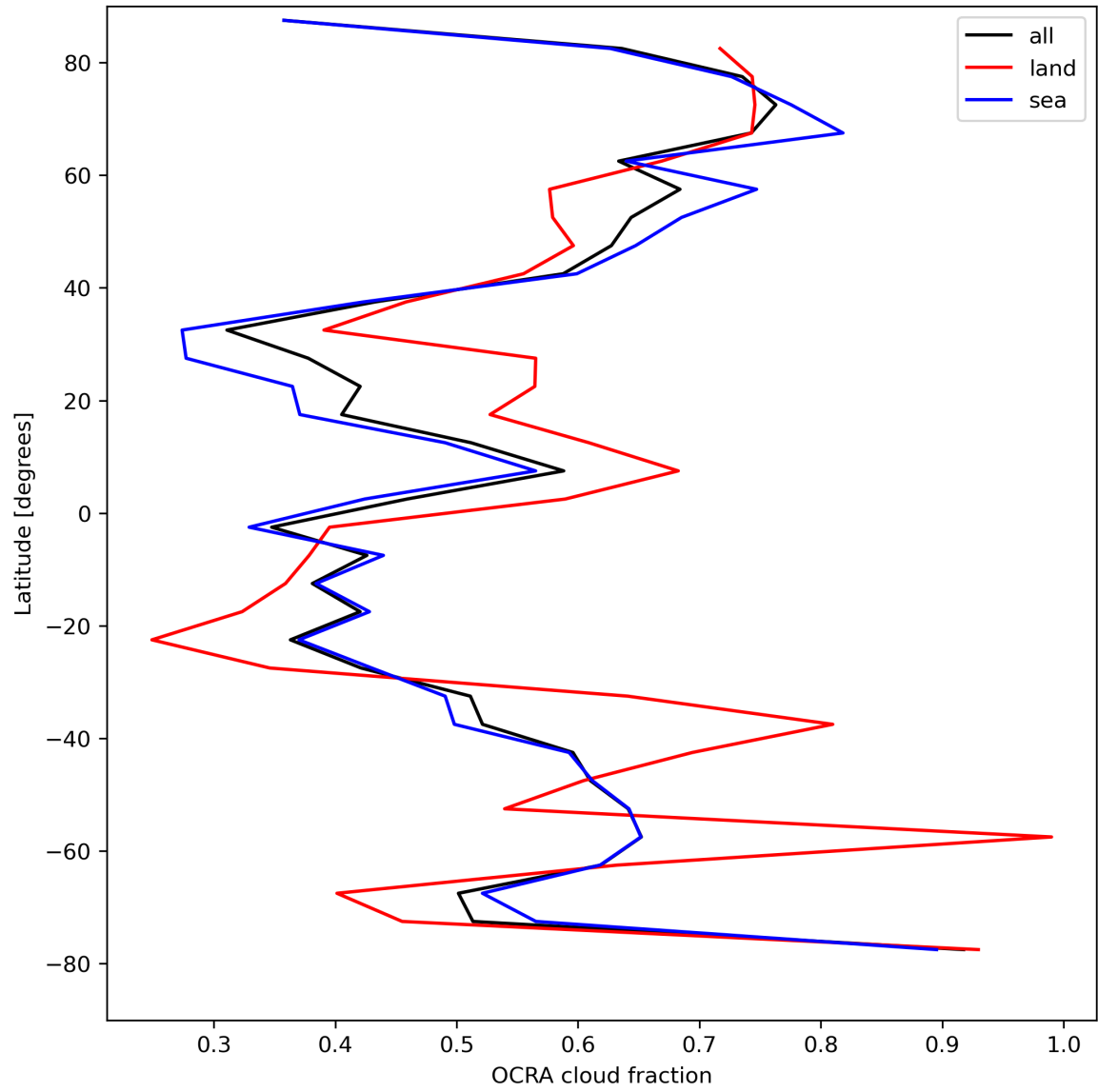
Figure 34: Zonal average of “OCRA cloud fraction” for 2024-08-17 to 2024-08-19.
