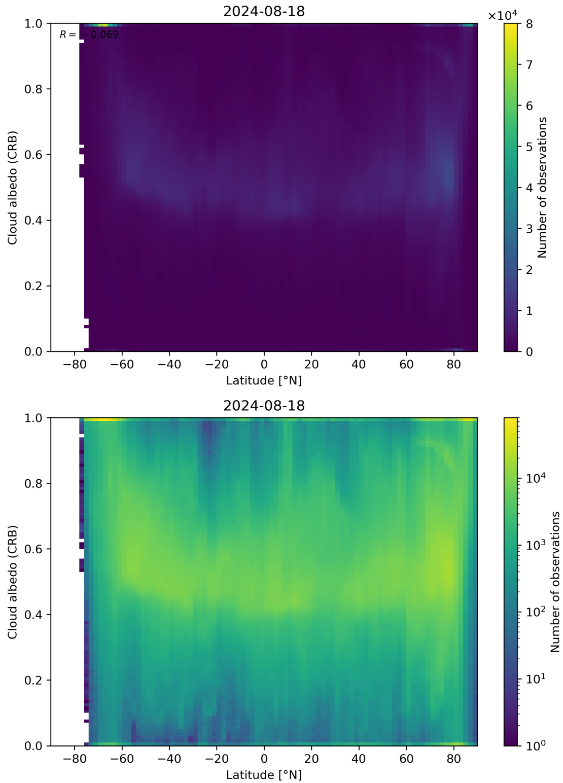
Figure 91: Scatter density plot of “Latitude” against “Cloud albedo (CRB)” for 2024-08-17 to 2024-08-19.
