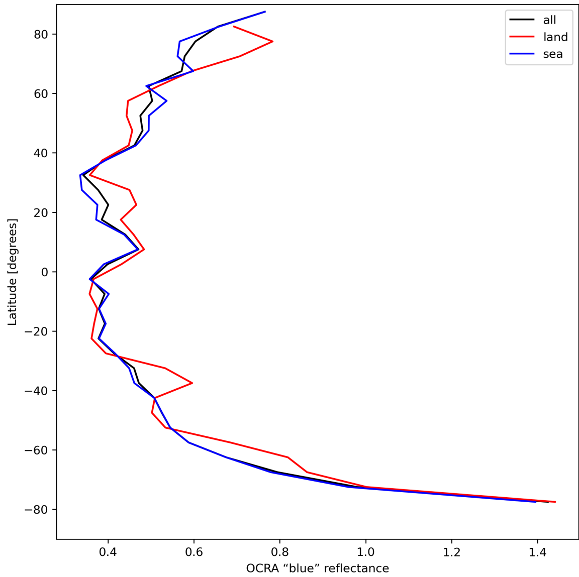
Figure 35: Zonal average of “OCRA “blue” reflectance” for 2024-08-17 to 2024-08-19.
