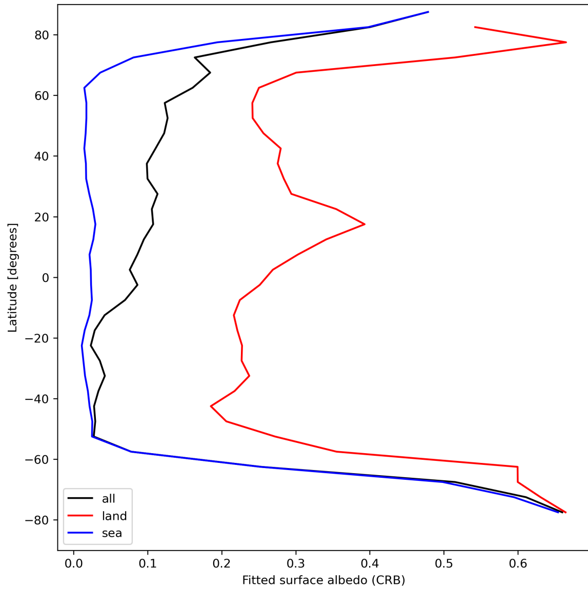
Figure 30: Zonal average of “Fitted surface albedo (CRB)” for 2024-08-17 to 2024-08-19.
