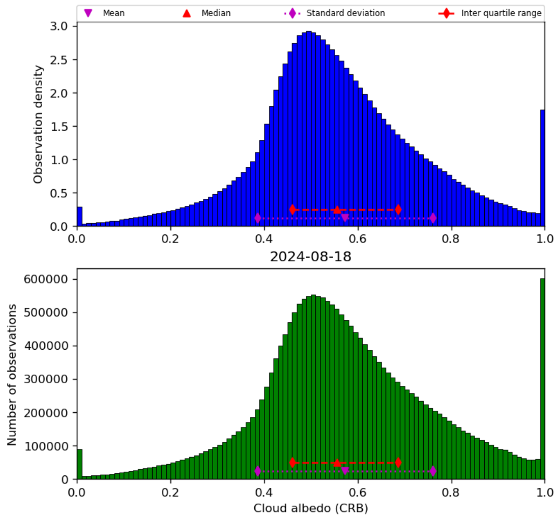
Figure 44: Histogram of “Cloud albedo (CRB)” for 2024-08-17 to 2024-08-19
