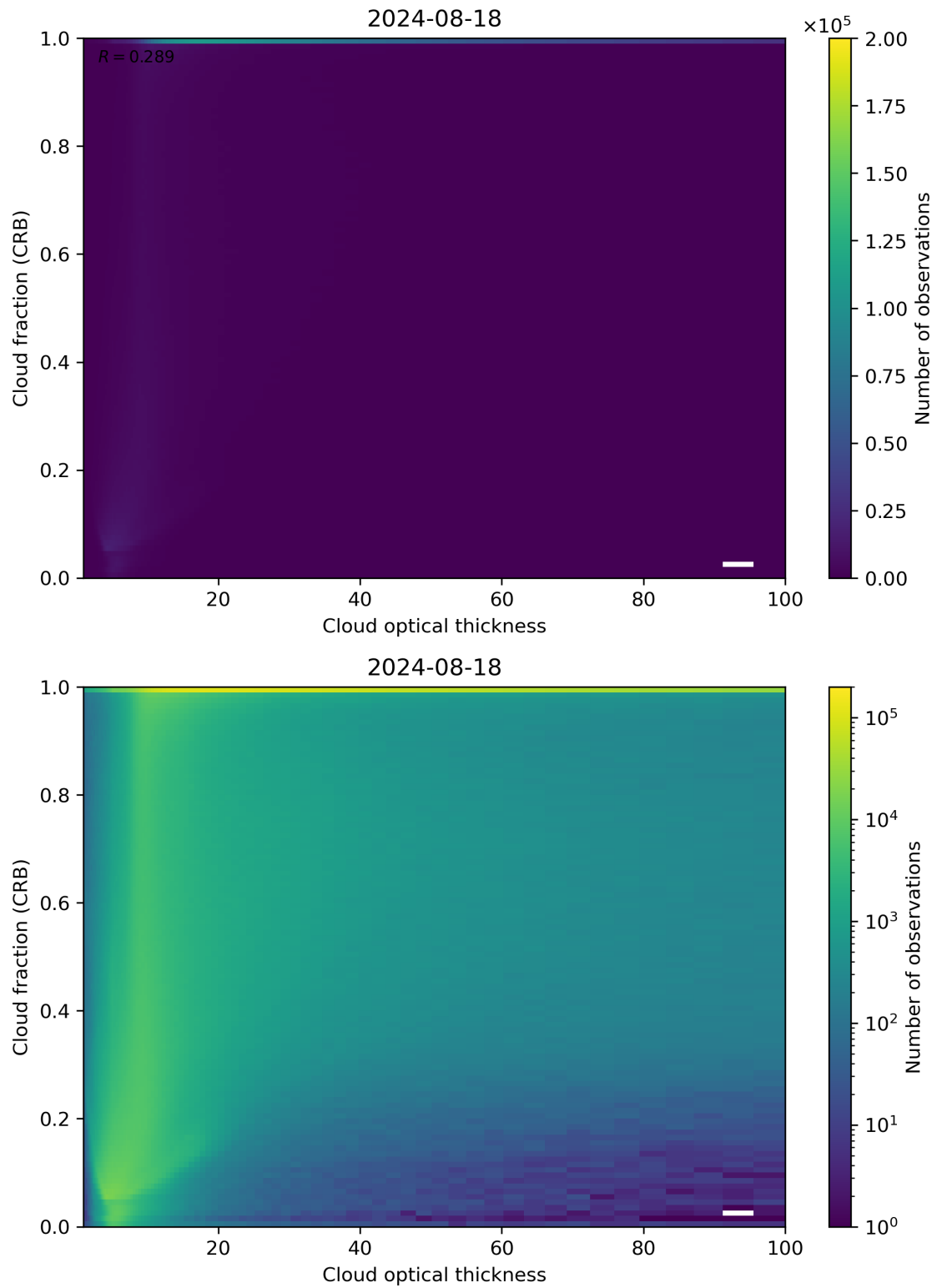
Figure 84: Scatter density plot of “Cloud optical thickness” against “Cloud fraction (CRB)” for 2024-08-17 to 2024-08-19.
