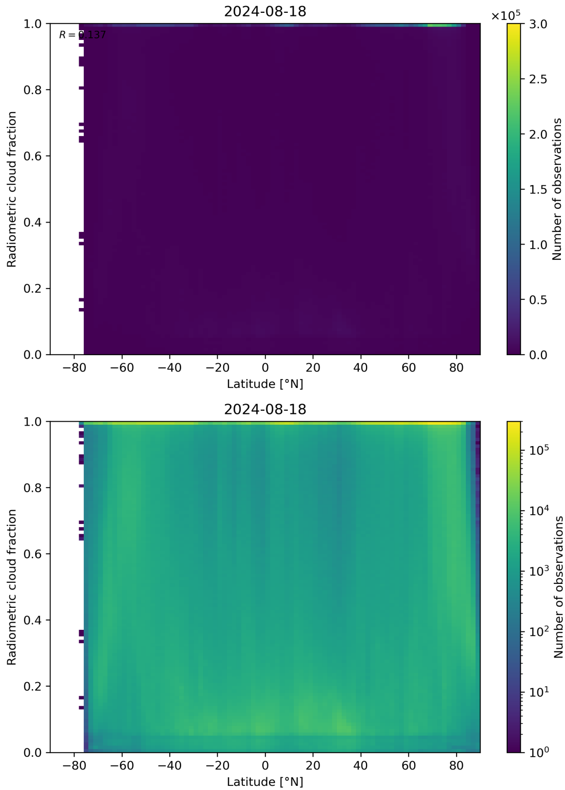
Figure 92: Scatter density plot of “Latitude” against “Radiometric cloud fraction” for 2024-08-17 to 2024-08-19.
