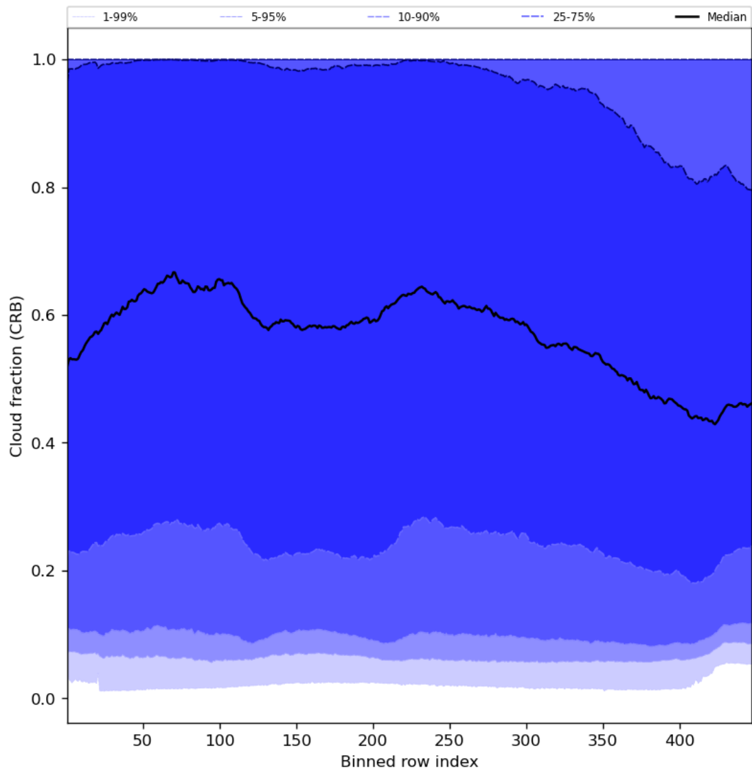
Figure 58: Along track statistics of “Cloud fraction (CRB)” for 2024-08-17 to 2024-08-19
