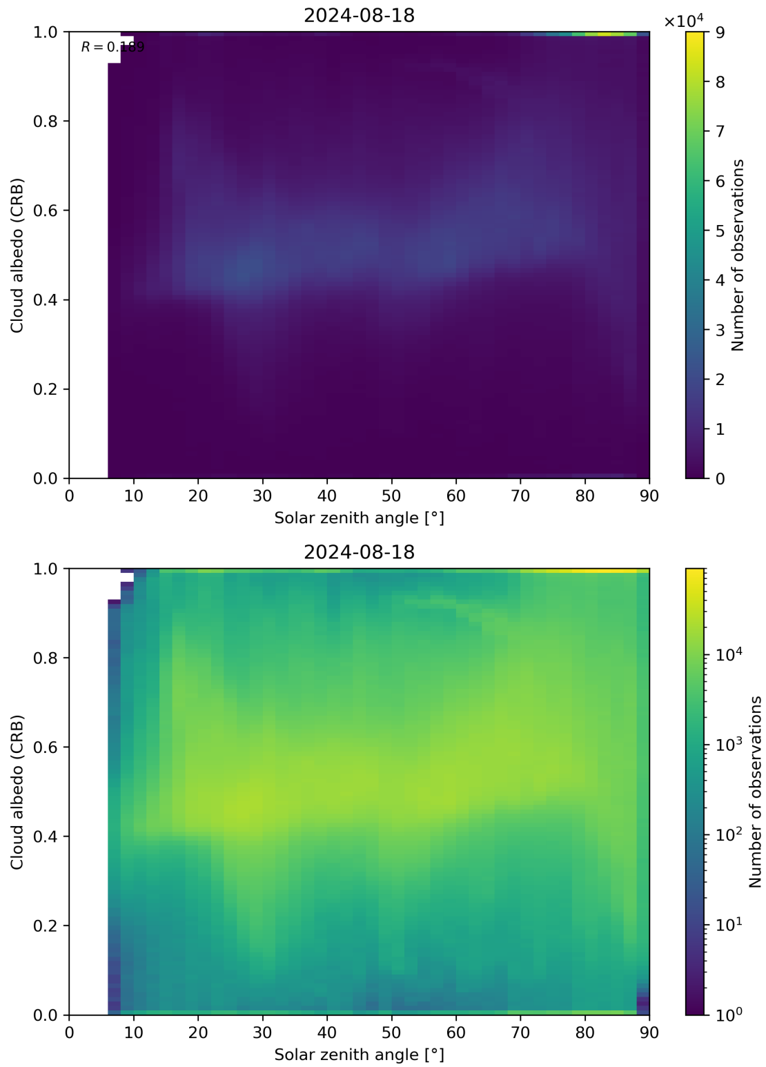
Figure 98: Scatter density plot of “Solar zenith angle” against “Cloud albedo (CRB)” for 2024-08-17 to 2024-08-19.
