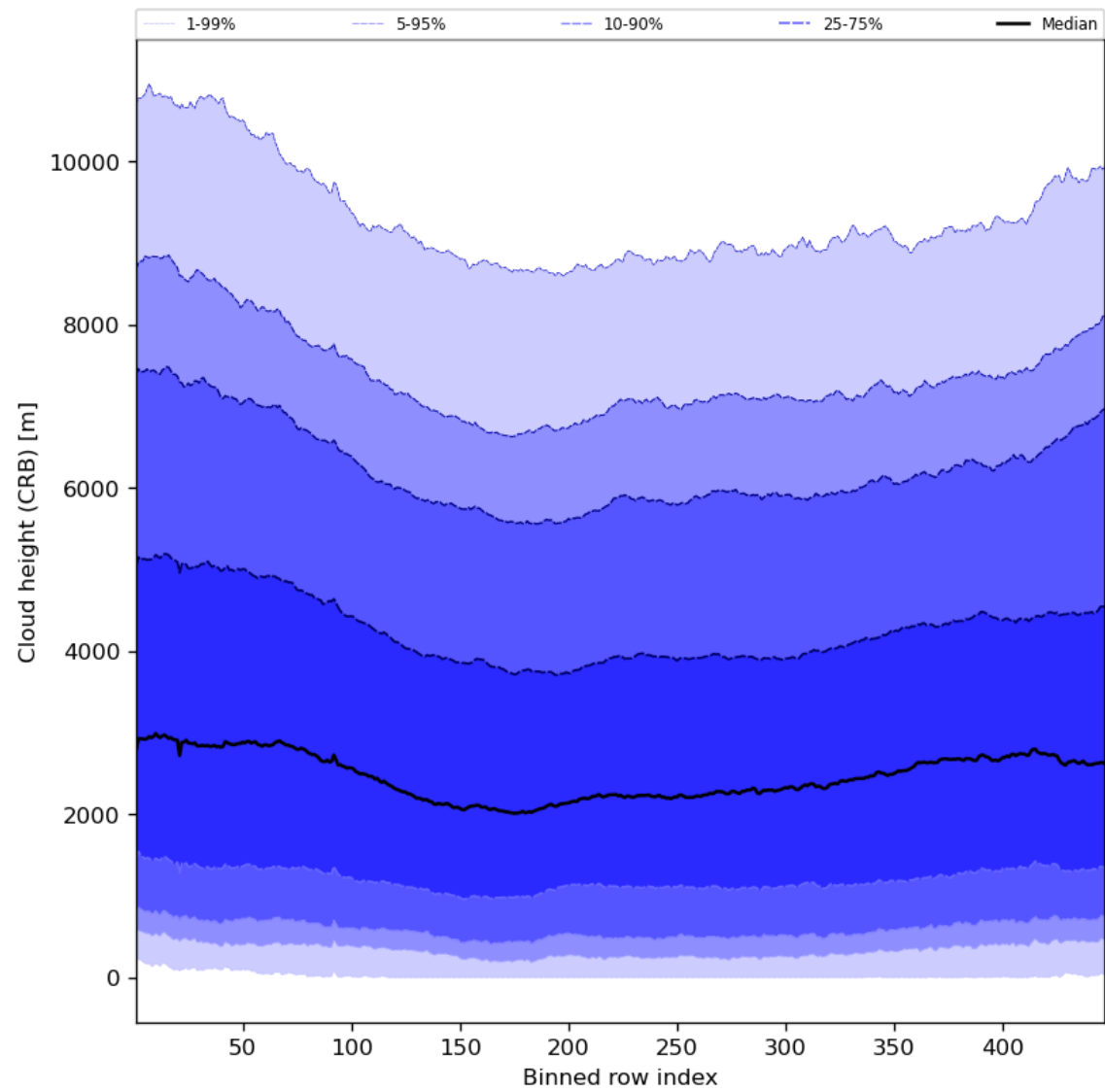
Figure 59: Along track statistics of “Cloud height (CRB)” for 2024-08-17 to 2024-08-19
