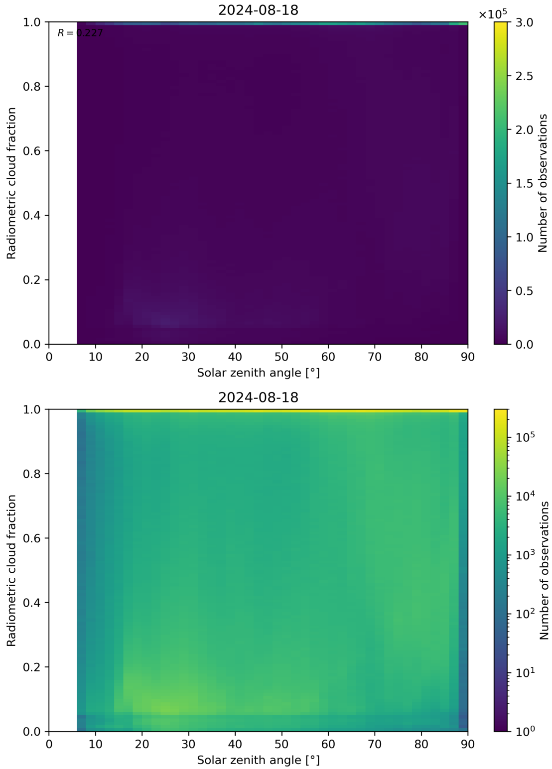
Figure 99: Scatter density plot of “Solar zenith angle” against “Radiometric cloud fraction” for 2024-08-17 to 2024-08-19.
