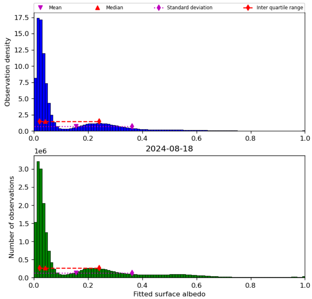
Figure 45: Histogram of “Fitted surface albedo” for 2024-08-17 to 2024-08-19
