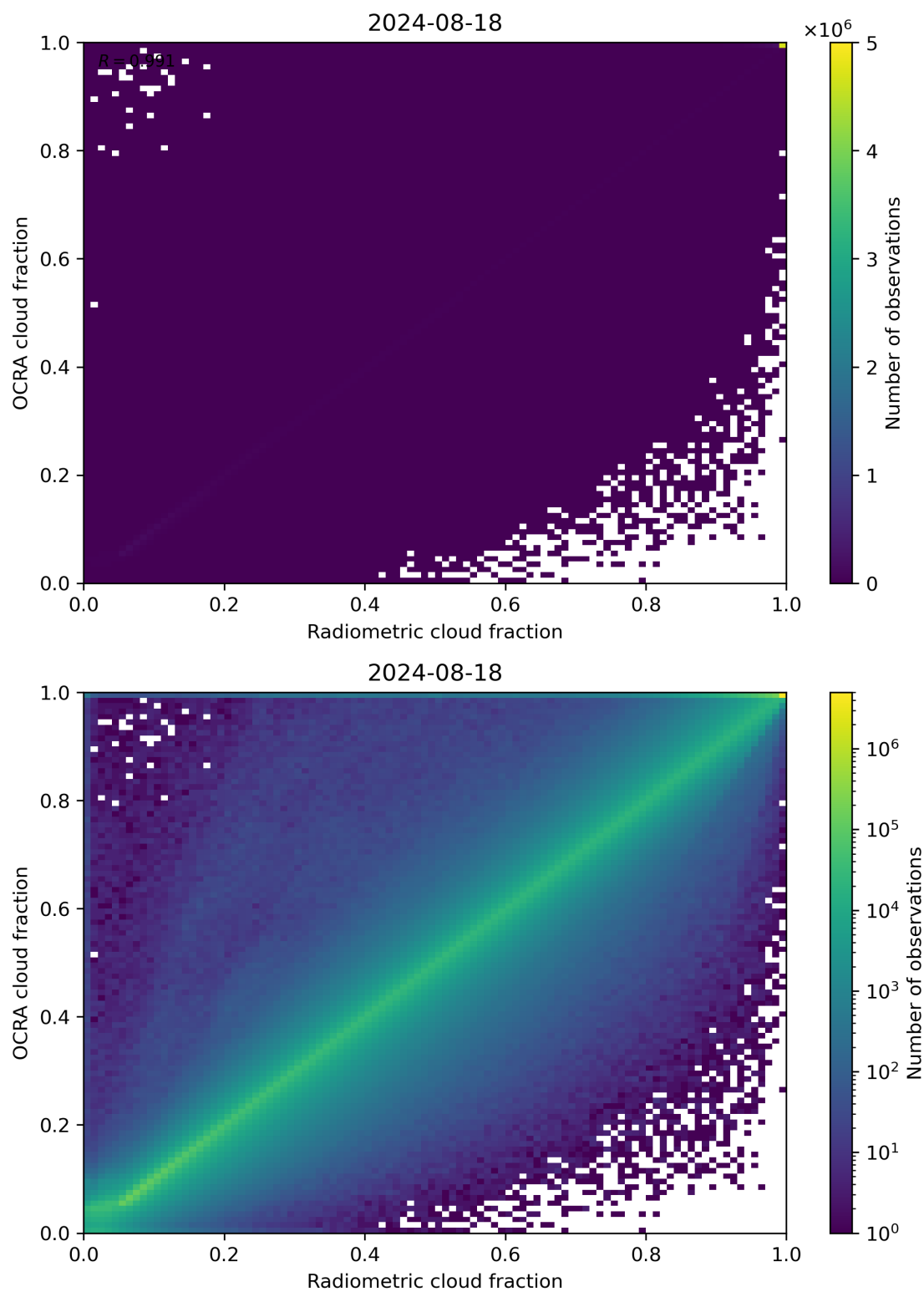
Figure 72: Scatter density plot of “Radiometric cloud fraction” against “OCRA cloud fraction” for 2024-08-17 to 2024-08-19.
