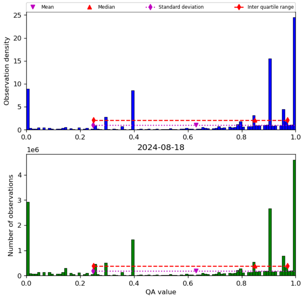
Figure 38: Histogram of “QA value” for 2024-08-17 to 2024-08-19
