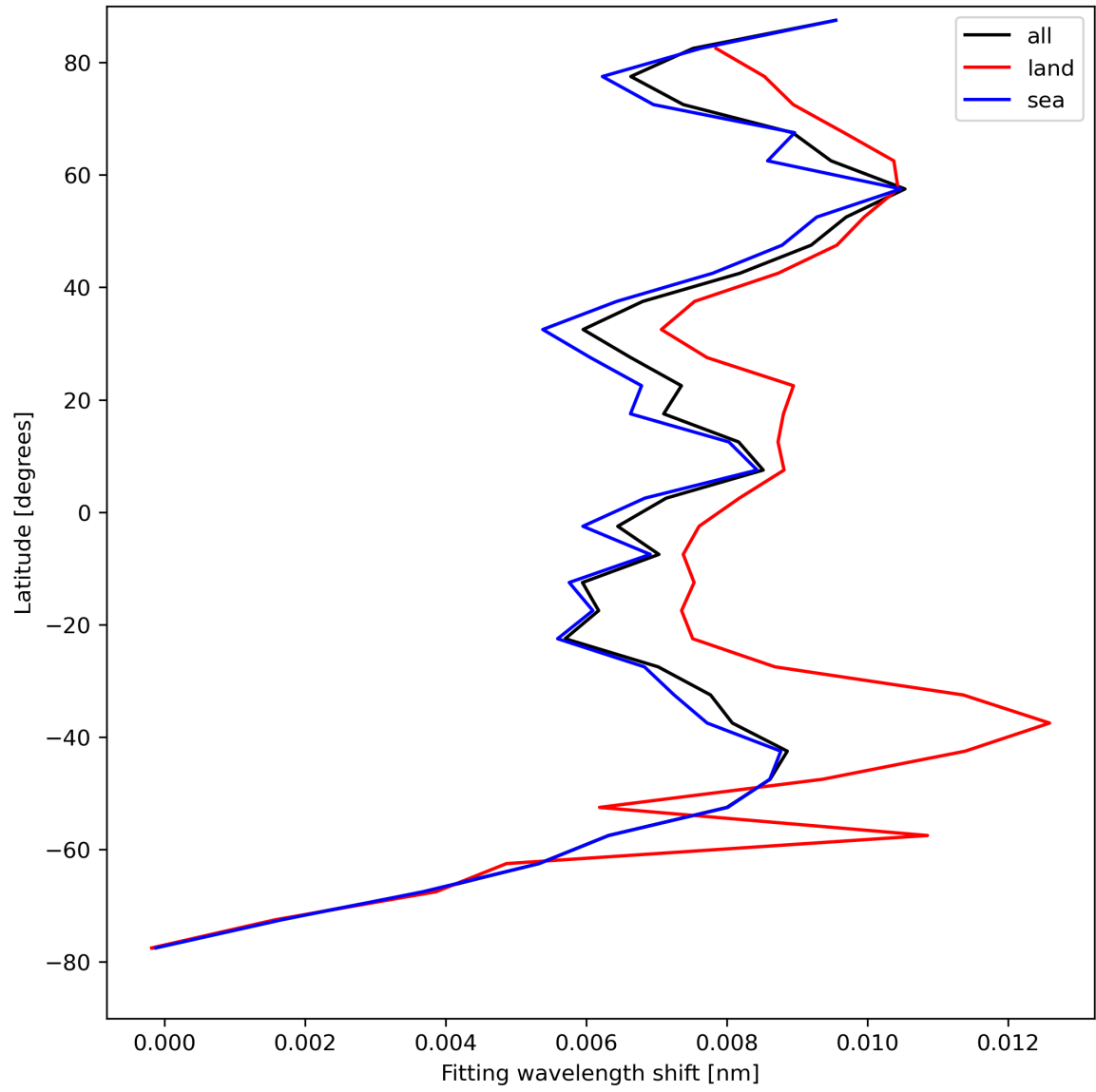
Figure 33: Zonal average of “Fitting wavelength shift” for 2024-08-17 to 2024-08-19.
