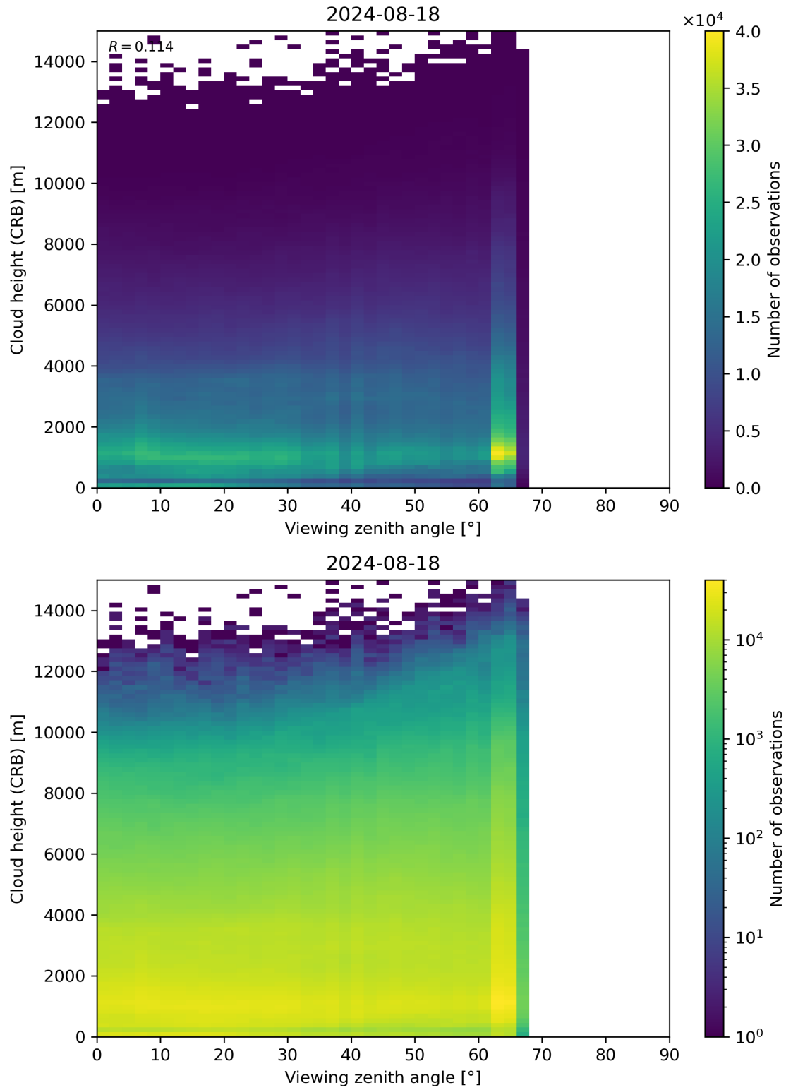
Figure 110: Scatter density plot of “Viewing zenith angle” against “Cloud height (CRB)” for 2024-08-17 to 2024-08-19.
