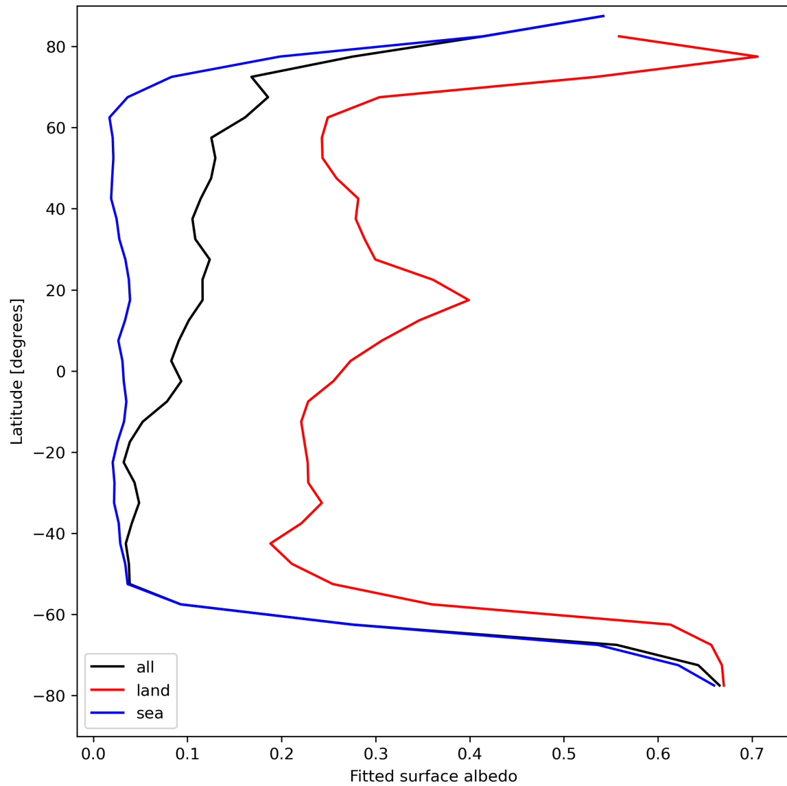
Figure 29: Zonal average of “Fitted surface albedo” for 2024-08-17 to 2024-08-19.
