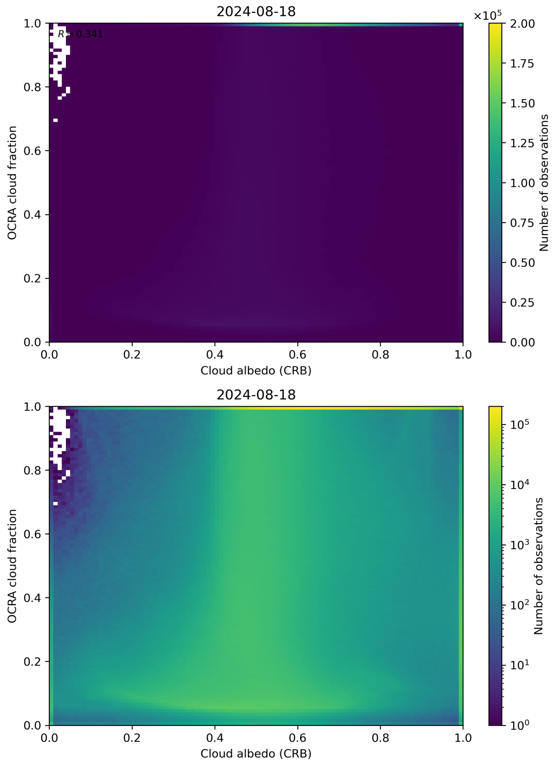
Figure 70: Scatter density plot of “Cloud albedo (CRB)” against “OCRA cloud fraction” for 2024-08-17 to 2024-08-19.
