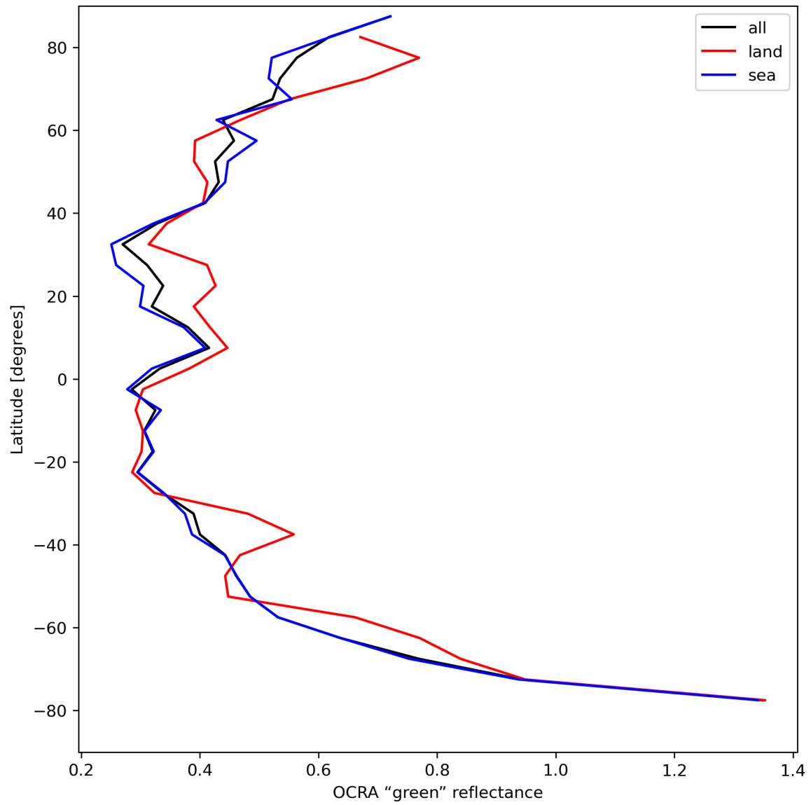
Figure 36: Zonal average of “OCRA “green” reflectance” for 2024-08-17 to 2024-08-19.
