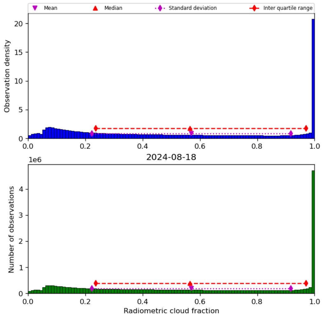
Figure 39: Histogram of “Radiometric cloud fraction” for 2024-08-17 to 2024-08-19
