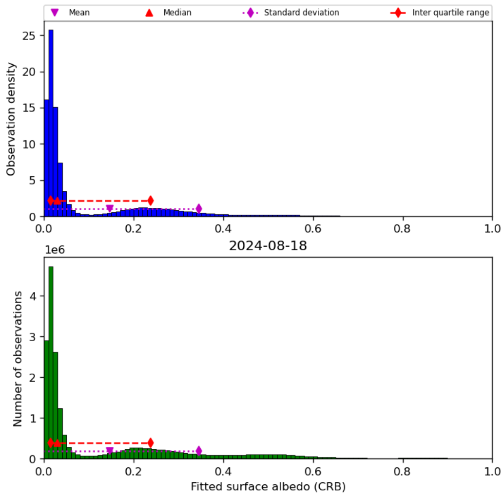
Figure 46: Histogram of “Fitted surface albedo (CRB)” for 2024-08-17 to 2024-08-19
