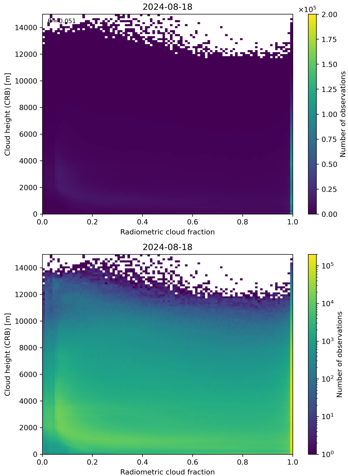
Figure 74: Scatter density plot of “Radiometric cloud fraction” against “Cloud height (CRB)” for 2024-08-17 to 2024-08-19.
