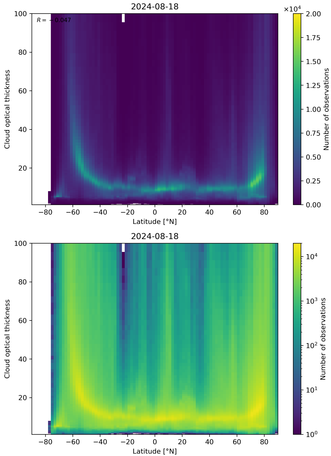
Figure 96: Scatter density plot of “Latitude” against “Cloud optical thickness” for 2024-08-17 to 2024-08-19.
