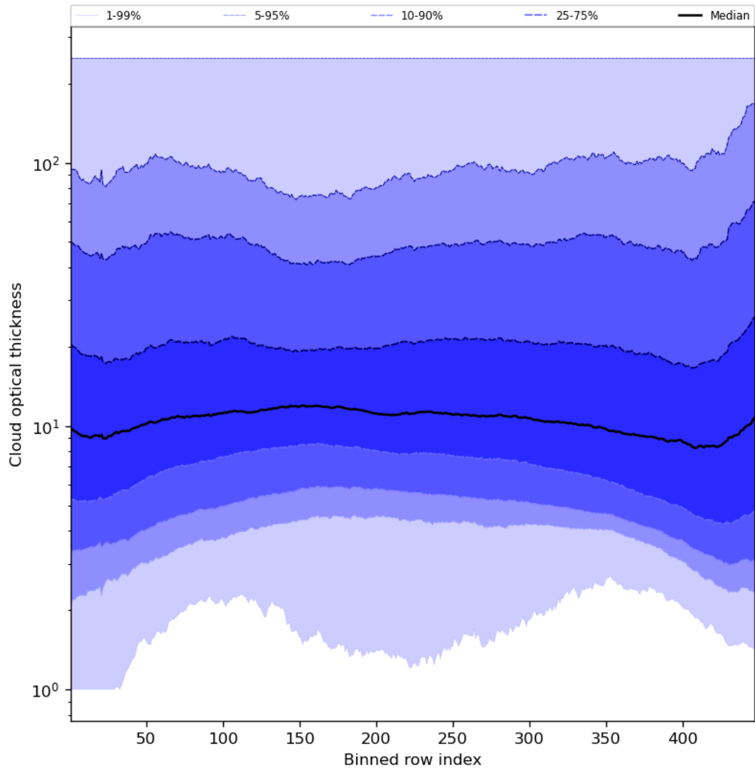
Figure 57: Along track statistics of “Cloud optical thickness” for 2024-08-17 to 2024-08-19
