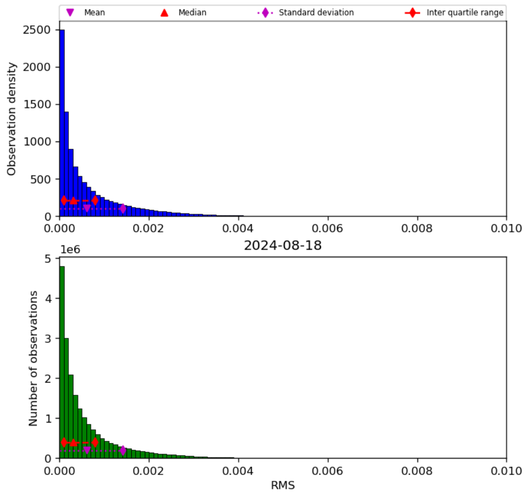
Figure 47: Histogram of “RMS” for 2024-08-17 to 2024-08-19
