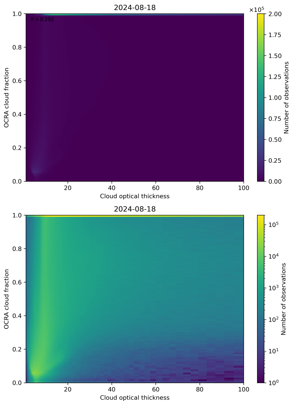
Figure 83: Scatter density plot of “Cloud optical thickness” against “OCRA cloud fraction” for 2024-08-17 to 2024-08-19.
