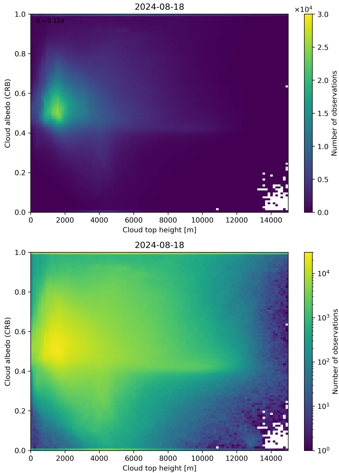
Figure 86: Scatter density plot of “Cloud top height” against “Cloud albedo (CRB)” for 2024-08-17 to 2024-08-19.
