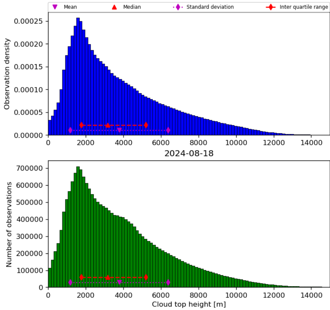
Figure 40: Histogram of “Cloud top height” for 2024-08-17 to 2024-08-19
