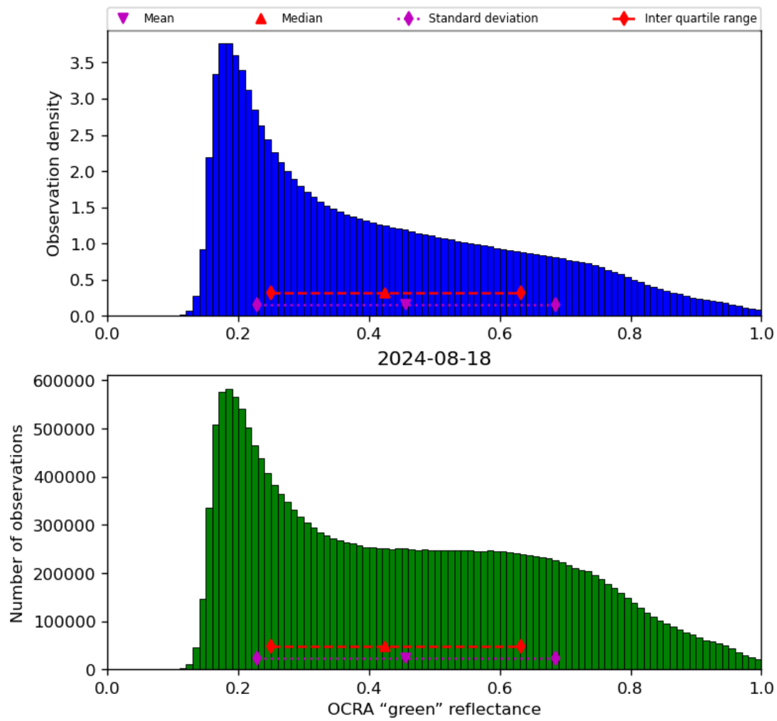
Figure 52: Histogram of “OCRA “green” reflectance” for 2024-08-17 to 2024-08-19
