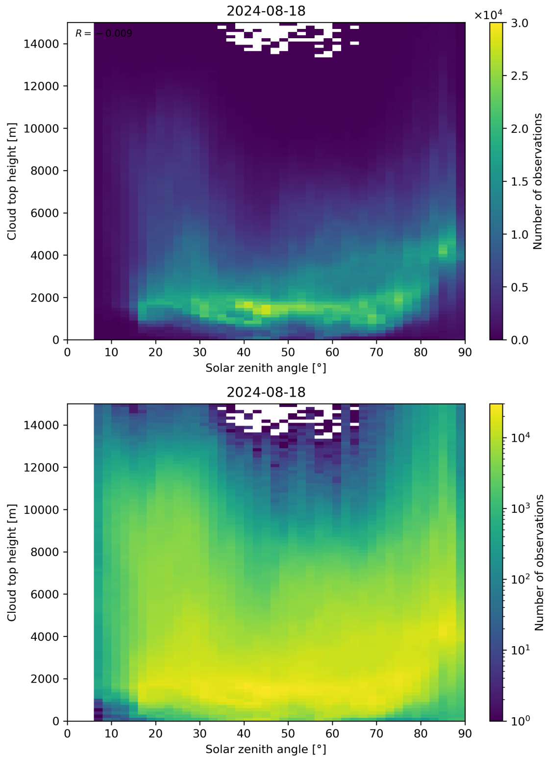
Figure 104: Scatter density plot of “Solar zenith angle” against “Cloud top height” for 2024-08-17 to 2024-08-19.
