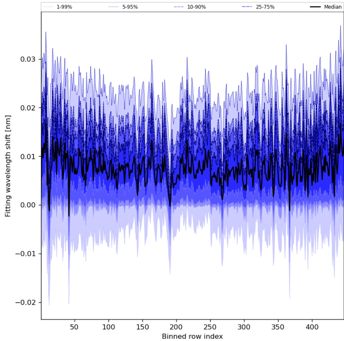
Figure 65: Along track statistics of “Fitting wavelength shift” for 2024-08-17 to 2024-08-19
