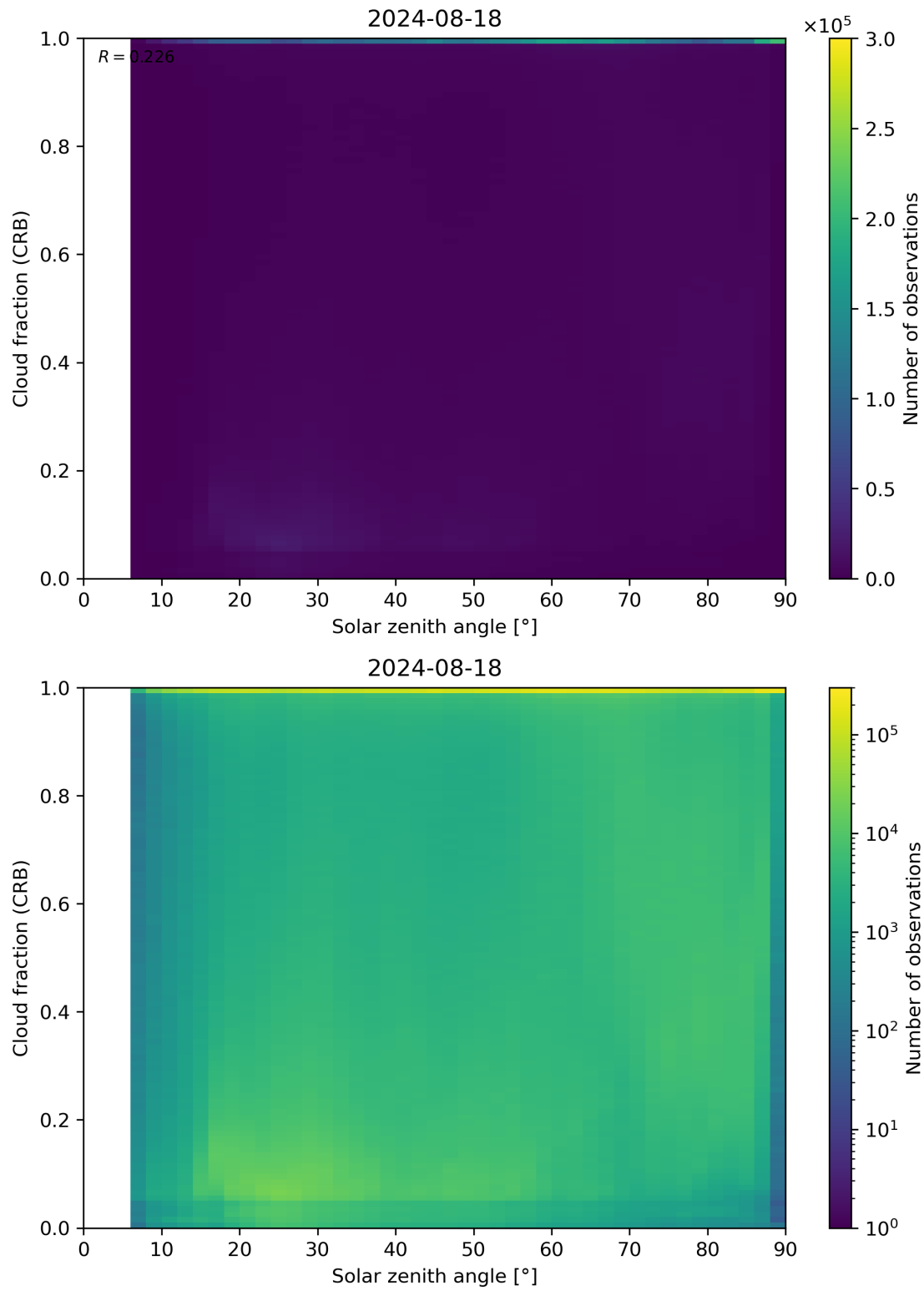
Figure 101: Scatter density plot of “Solar zenith angle” against “Cloud fraction (CRB)” for 2024-08-17 to 2024-08-19.
