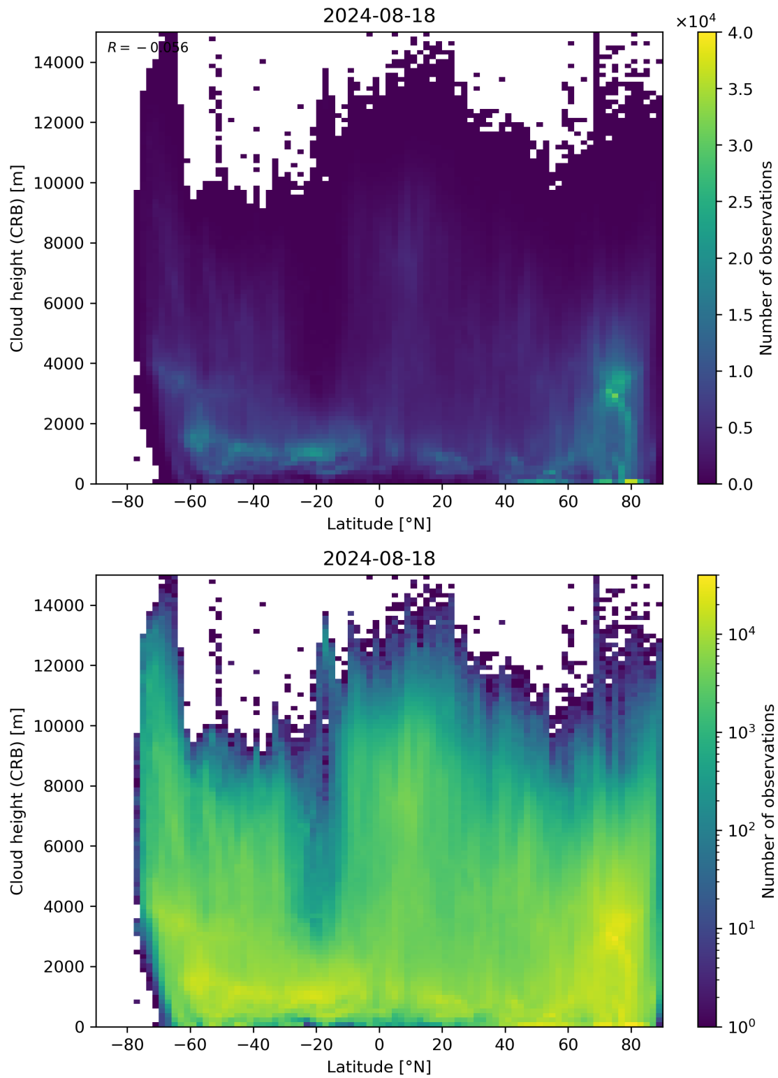
Figure 95: Scatter density plot of “Latitude” against “Cloud height (CRB)” for 2024-08-17 to 2024-08-19.
