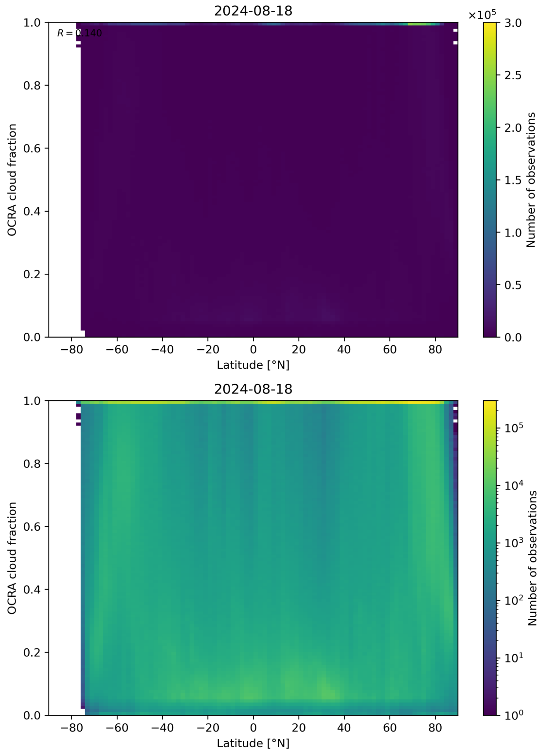
Figure 93: Scatter density plot of “Latitude” against “OCRA cloud fraction” for 2024-08-17 to 2024-08-19.
