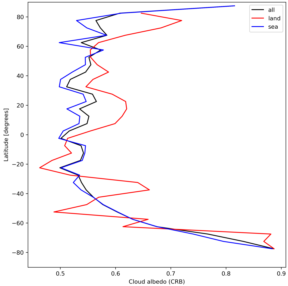
Figure 28: Zonal average of “Cloud albedo (CRB)” for 2024-08-17 to 2024-08-19.
