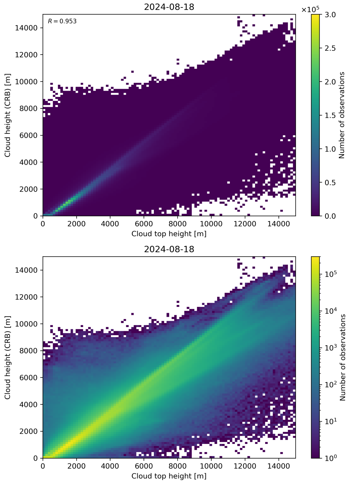
Figure 89: Scatter density plot of “Cloud top height” against “Cloud height (CRB)” for 2024-08-17 to 2024-08-19.
