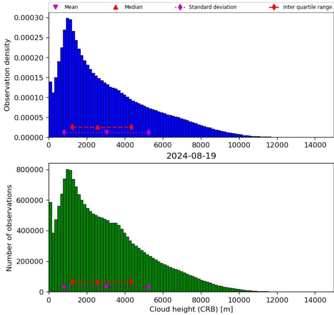
Figure 43: Histogram of “Cloud height (CRB)” for 2024-08-18 to 2024-08-20
