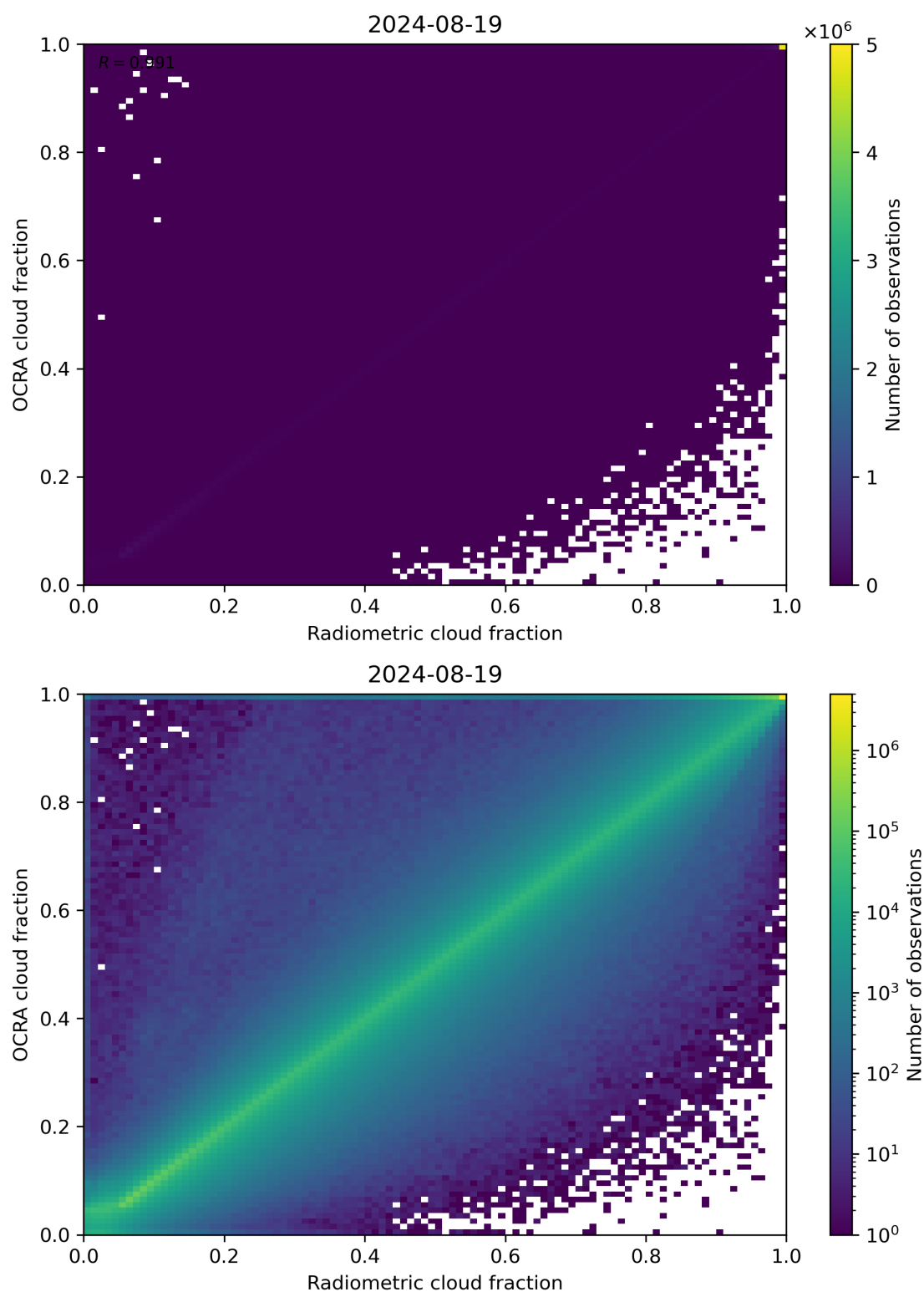
Figure 72: Scatter density plot of “Radiometric cloud fraction” against “OCRA cloud fraction” for 2024-08-18 to 2024-08-20.
