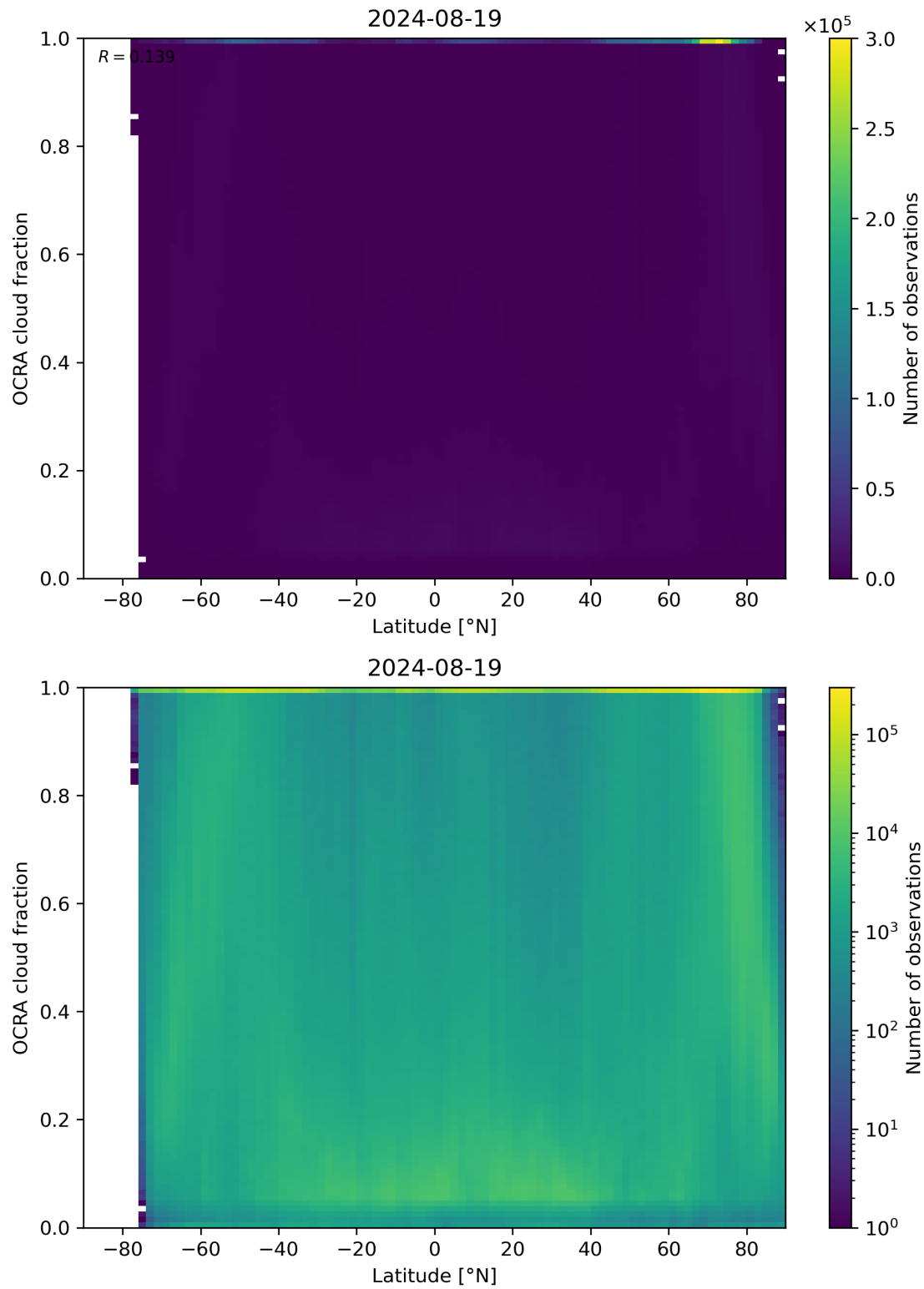
Figure 93: Scatter density plot of “Latitude” against “OCRA cloud fraction” for 2024-08-18 to 2024-08-20.
