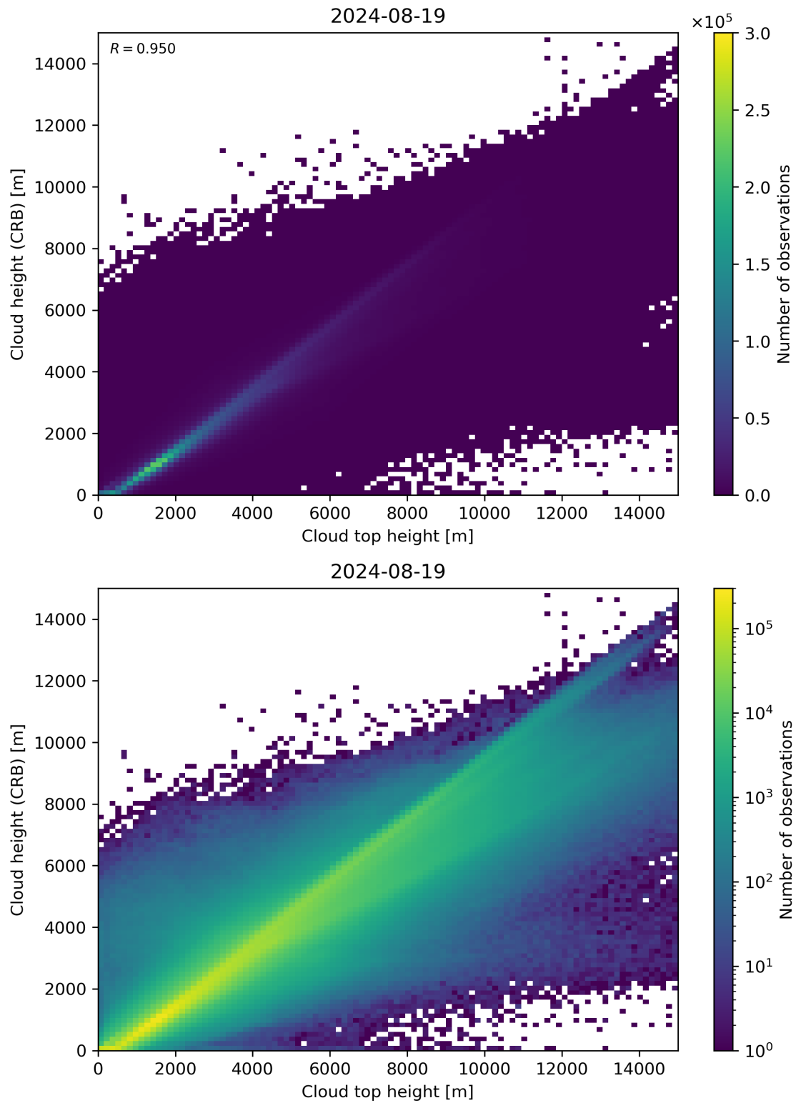
Figure 89: Scatter density plot of “Cloud top height” against “Cloud height (CRB)” for 2024-08-18 to 2024-08-20.
