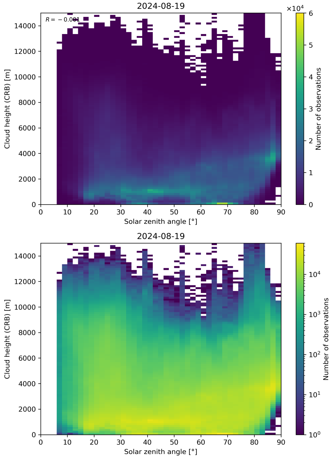
Figure 102: Scatter density plot of “Solar zenith angle” against “Cloud height (CRB)” for 2024-08-18 to 2024-08-20.
