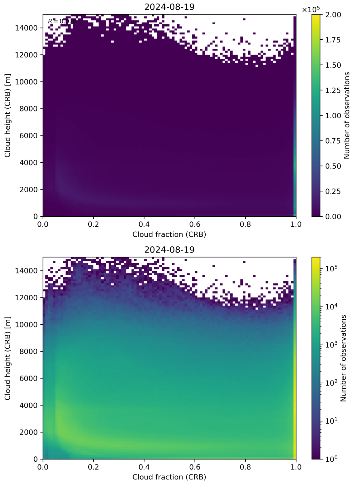
Figure 79: Scatter density plot of “Cloud fraction (CRB)” against “Cloud height (CRB)” for 2024-08-18 to 2024-08-20.
