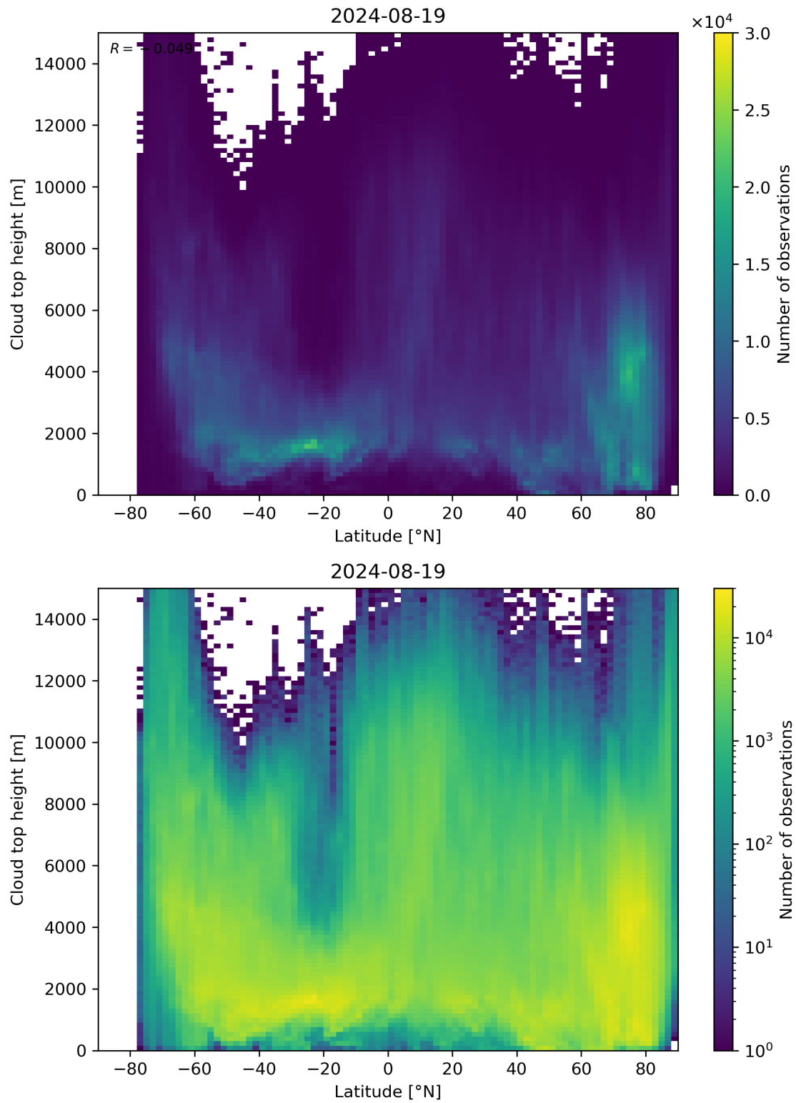
Figure 97: Scatter density plot of “Latitude” against “Cloud top height” for 2024-08-18 to 2024-08-20.
