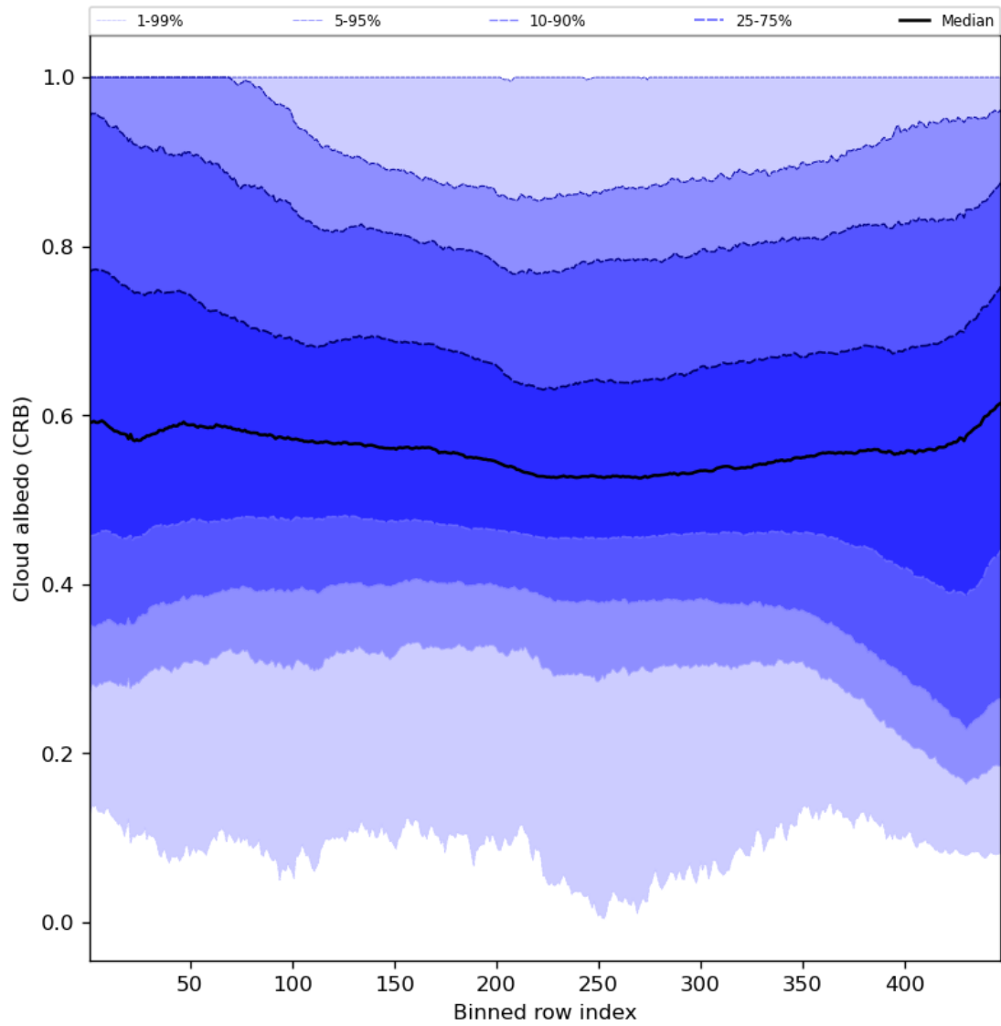
Figure 60: Along track statistics of “Cloud albedo (CRB)” for 2024-08-18 to 2024-08-20
