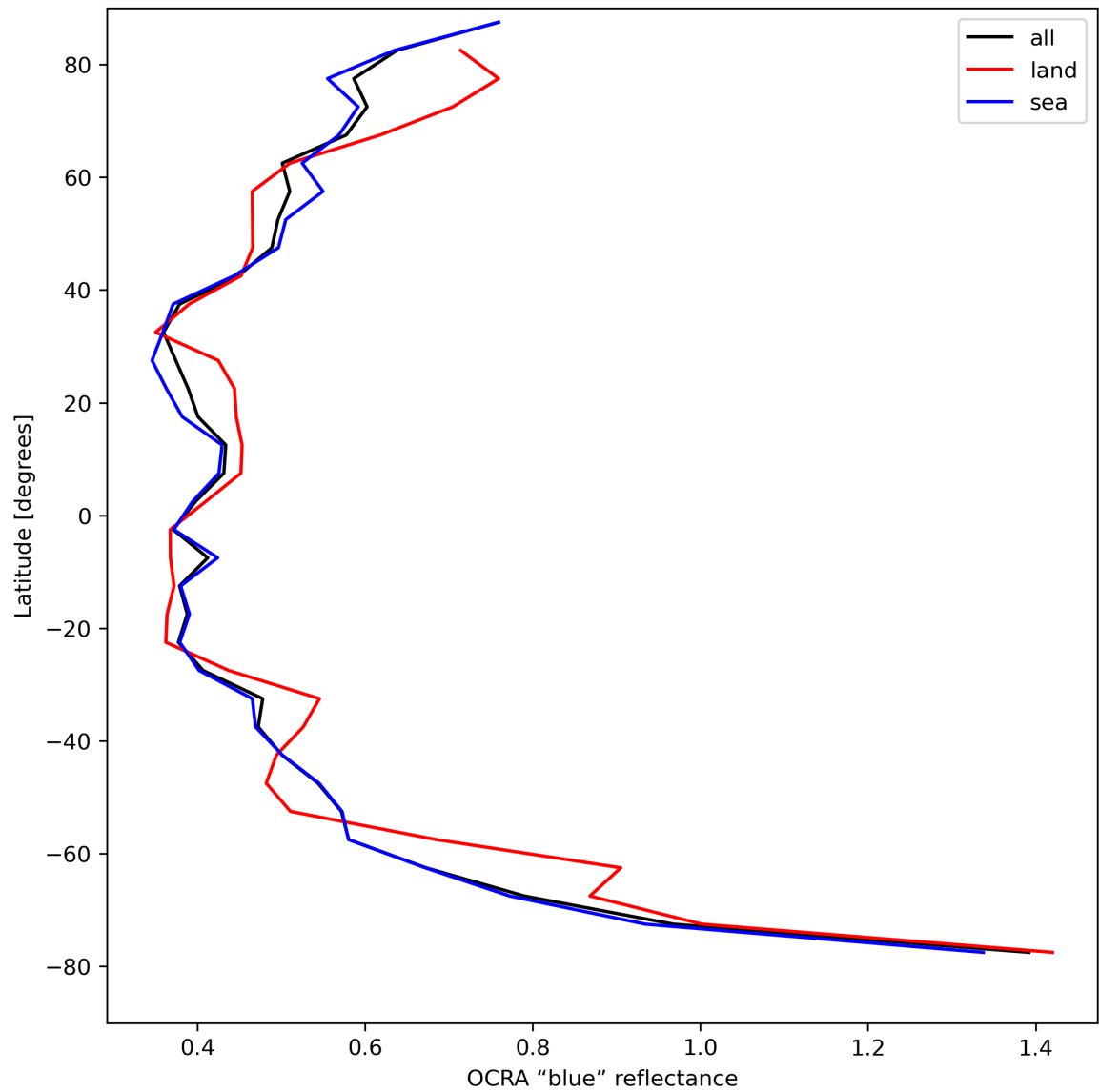
Figure 35: Zonal average of "OCRA "blue" reflectance" for 2024-08-18 to 2024-08-20.
