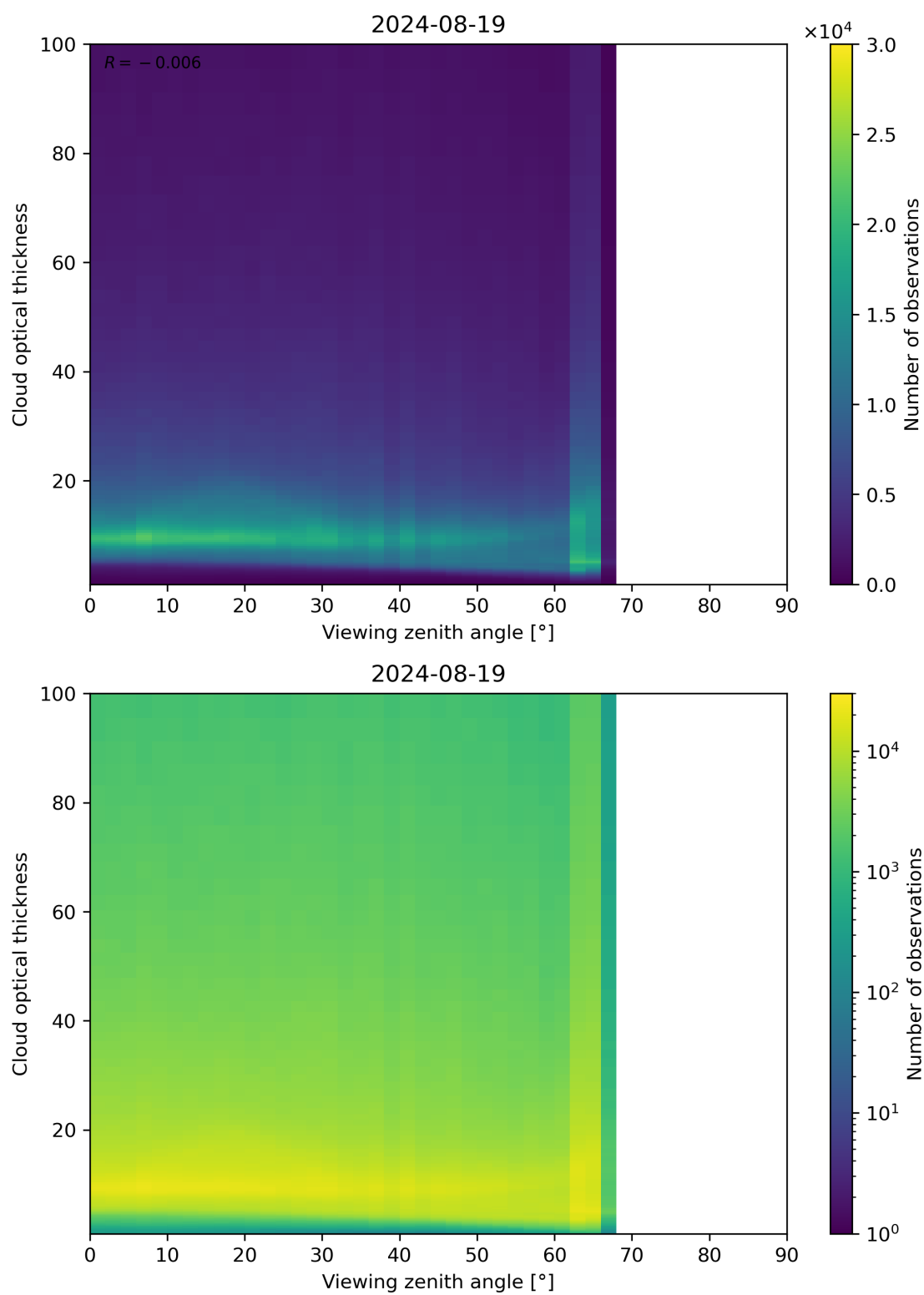
Figure 111: Scatter density plot of “Viewing zenith angle” against “Cloud optical thickness” for 2024-08-18 to 2024-08-20.
