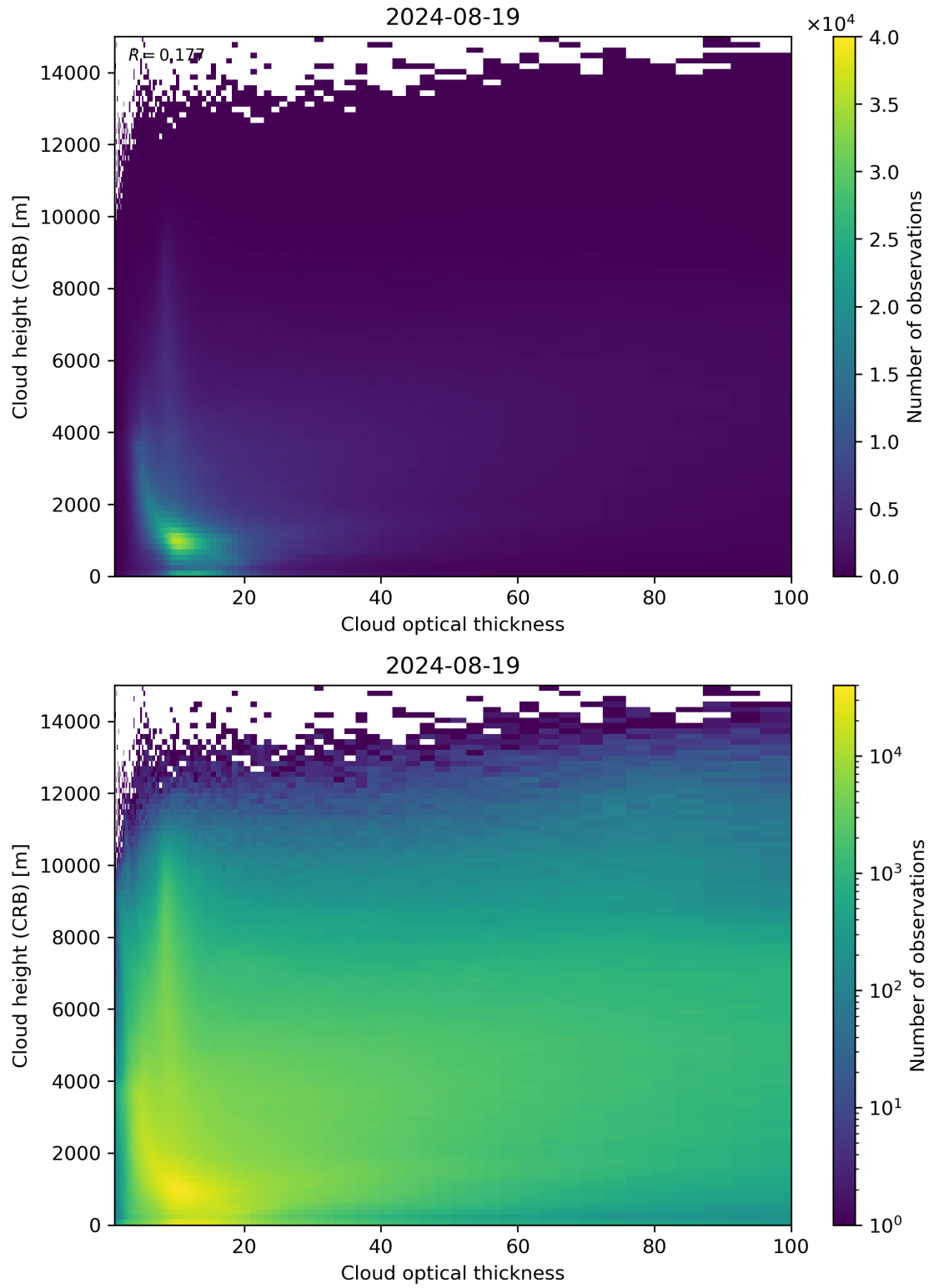
Figure 85: Scatter density plot of “Cloud optical thickness” against “Cloud height (CRB)” for 2024-08-18 to 2024-08-20.
