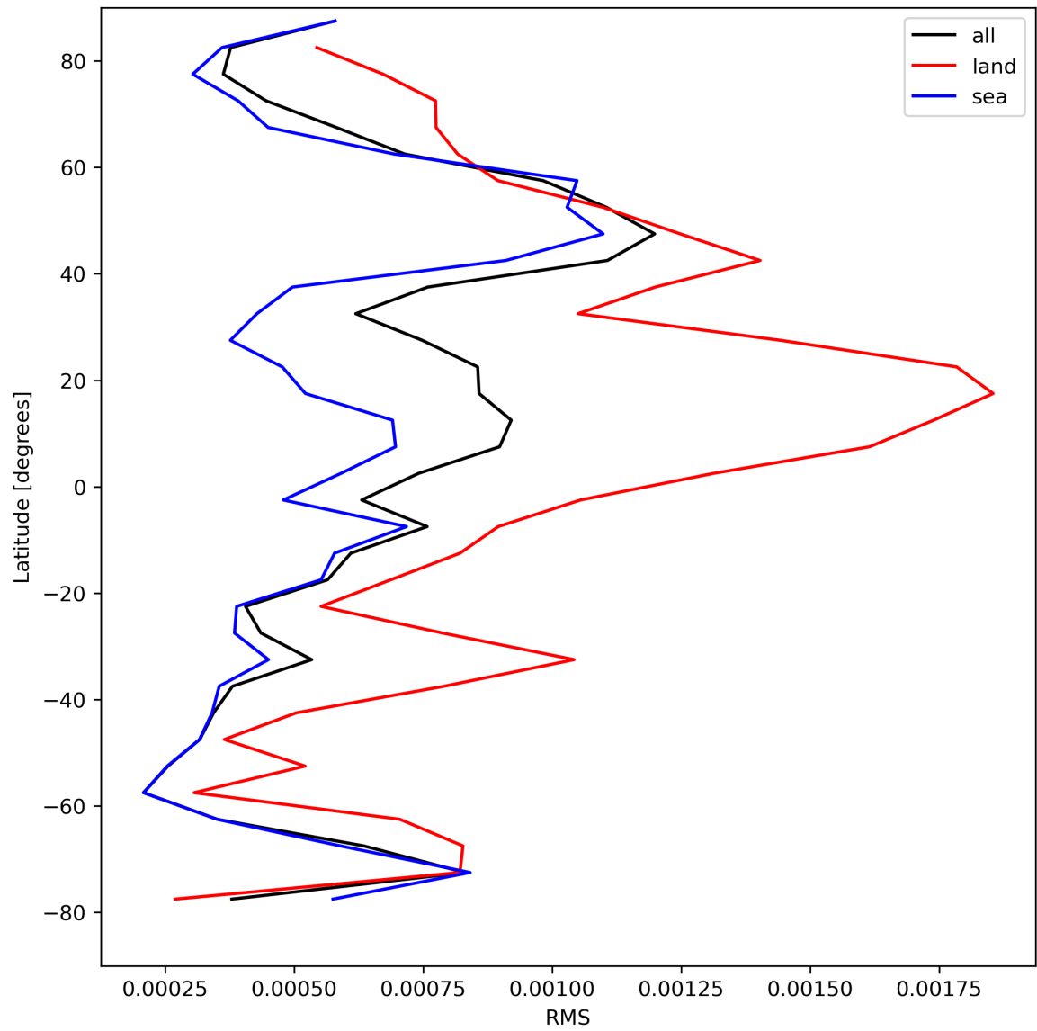
Figure 31: Zonal average of “RMS” for 2024-08-18 to 2024-08-20.
