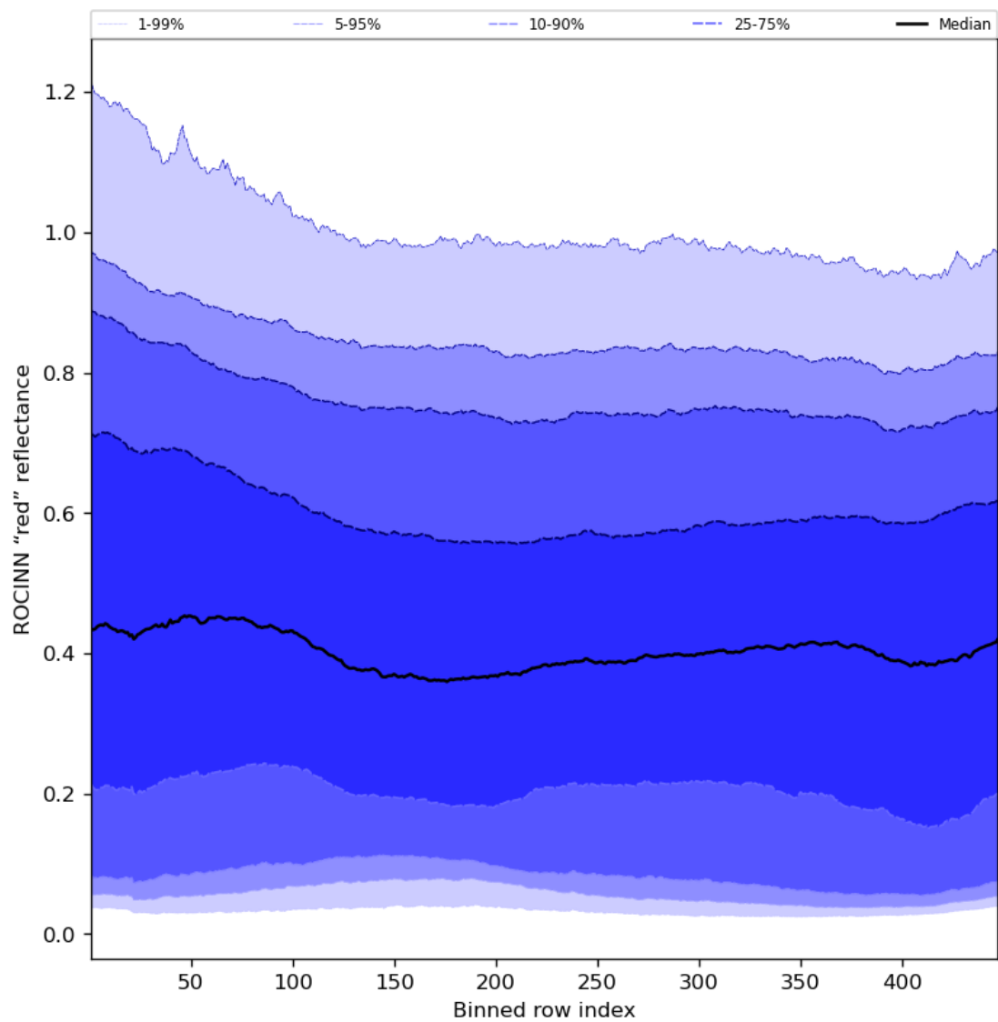
Figure 69: Along track statistics of “ROCINN “red” reflectance” for 2024-08-18 to 2024-08-20
