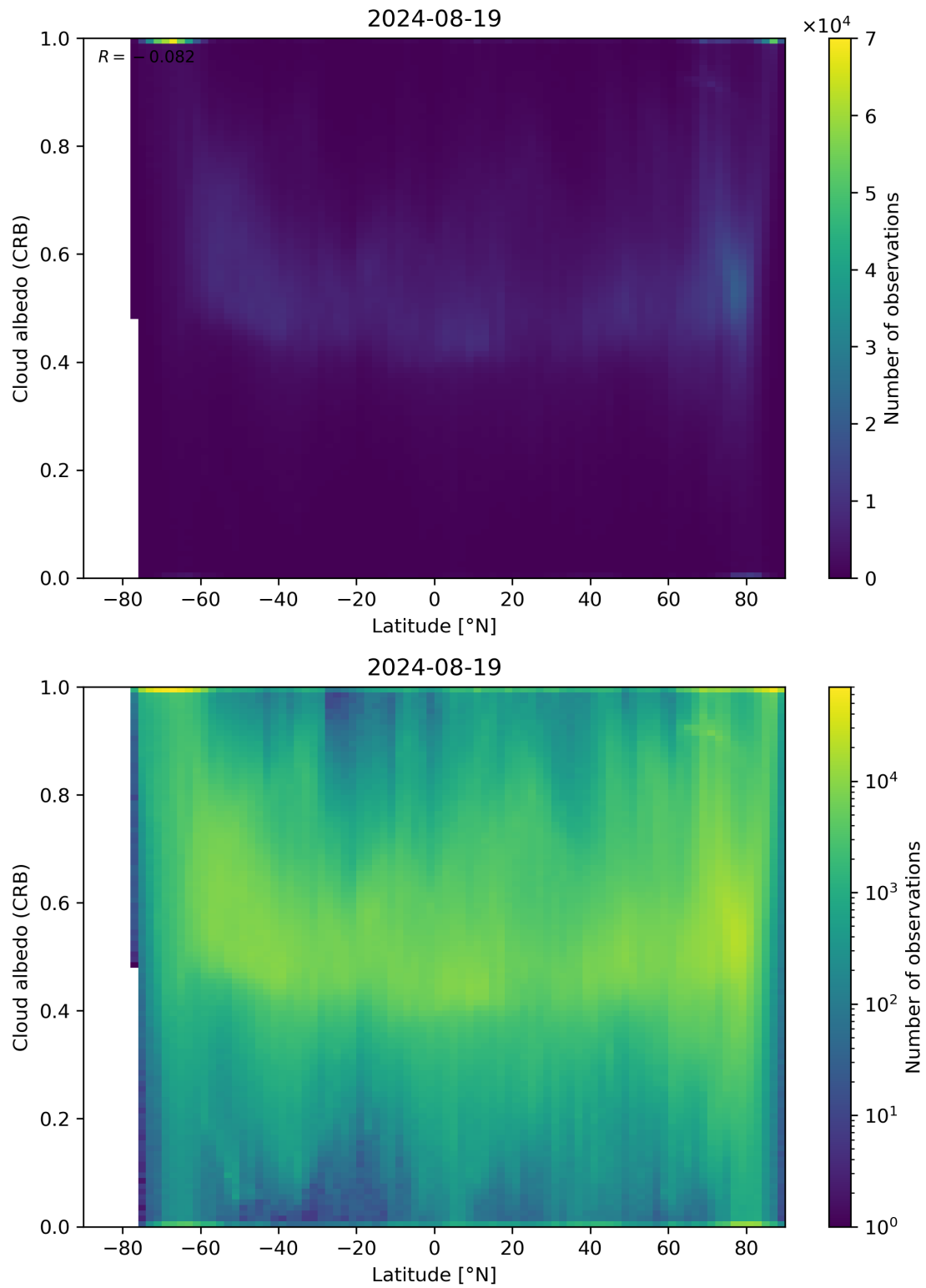
Figure 91: Scatter density plot of “Latitude” against “Cloud albedo (CRB)” for 2024-08-18 to 2024-08-20.
