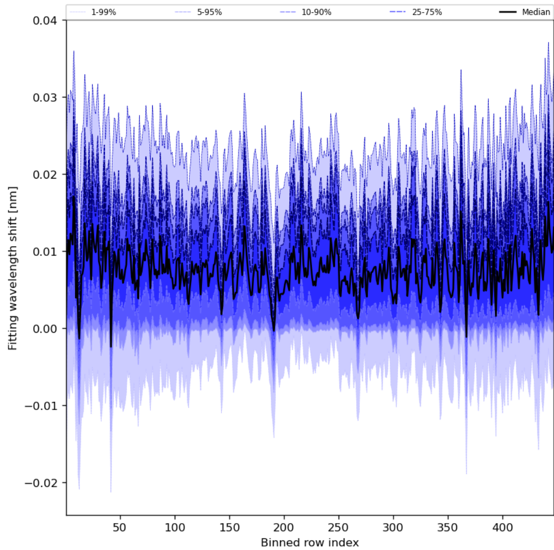
Figure 65: Along track statistics of “Fitting wavelength shift” for 2024-08-18 to 2024-08-20
