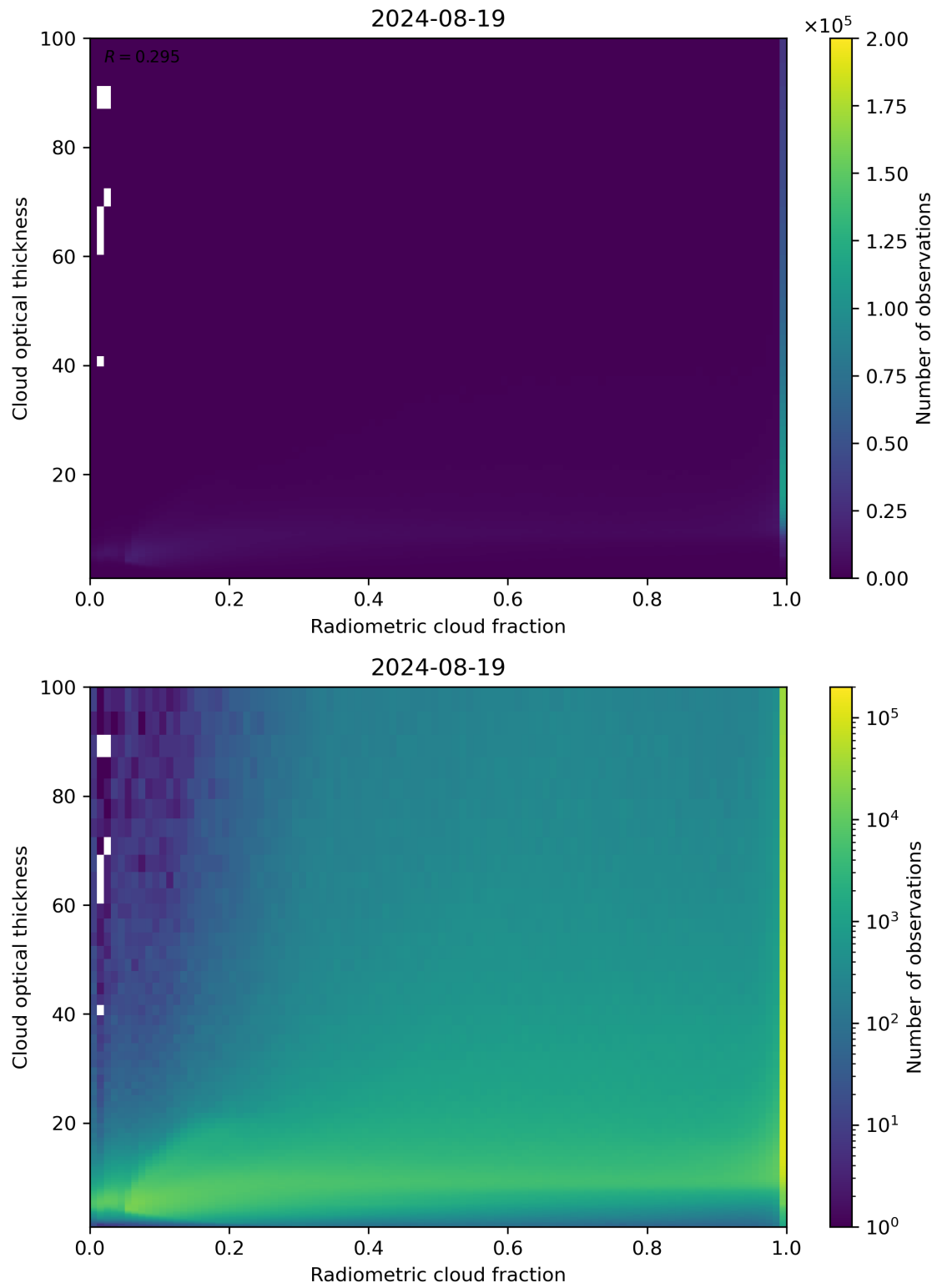
Figure 75: Scatter density plot of “Radiometric cloud fraction” against “Cloud optical thickness” for 2024-08-18 to 2024-08-20.
