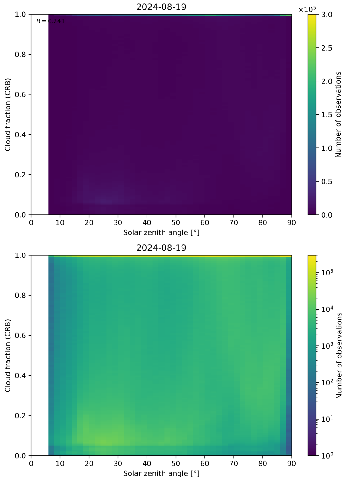
Figure 101: Scatter density plot of “Solar zenith angle” against “Cloud fraction (CRB)” for 2024-08-18 to 2024-08-20.
