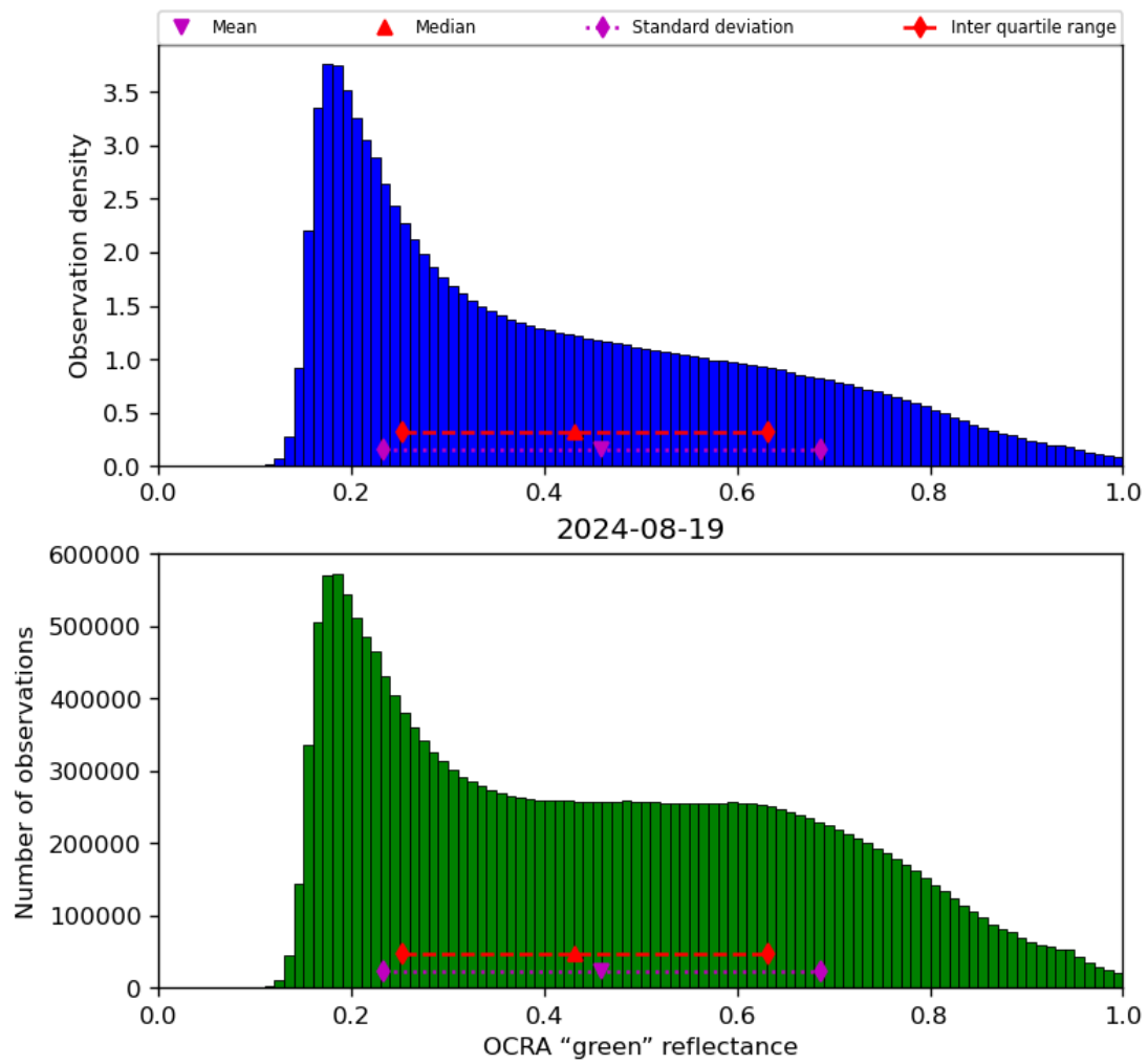
Figure 52: Histogram of “OCRA “green” reflectance” for 2024-08-18 to 2024-08-20
