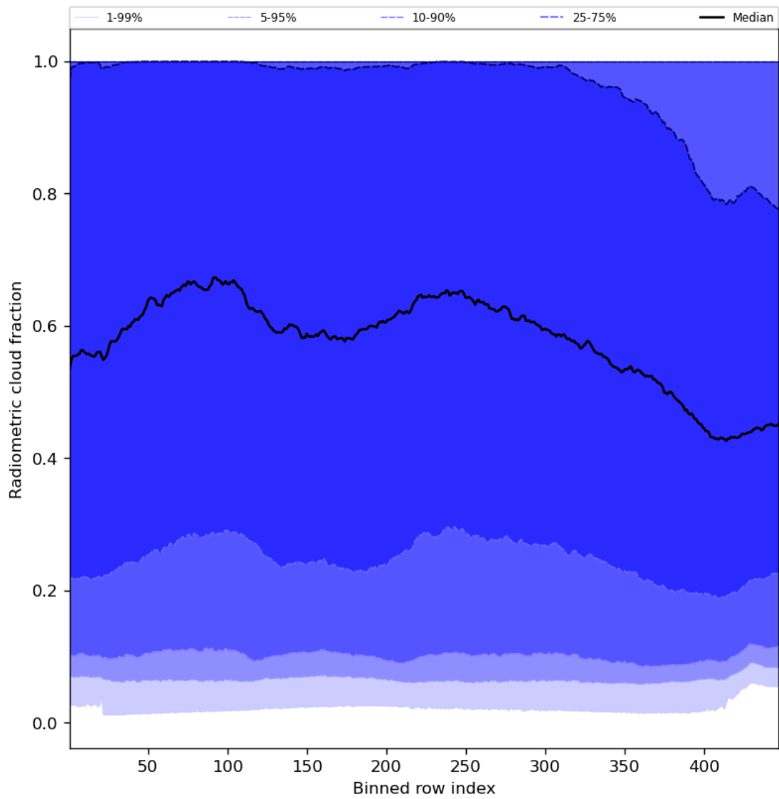
Figure 55: Along track statistics of “Radiometric cloud fraction” for 2024-08-18 to 2024-08-20
