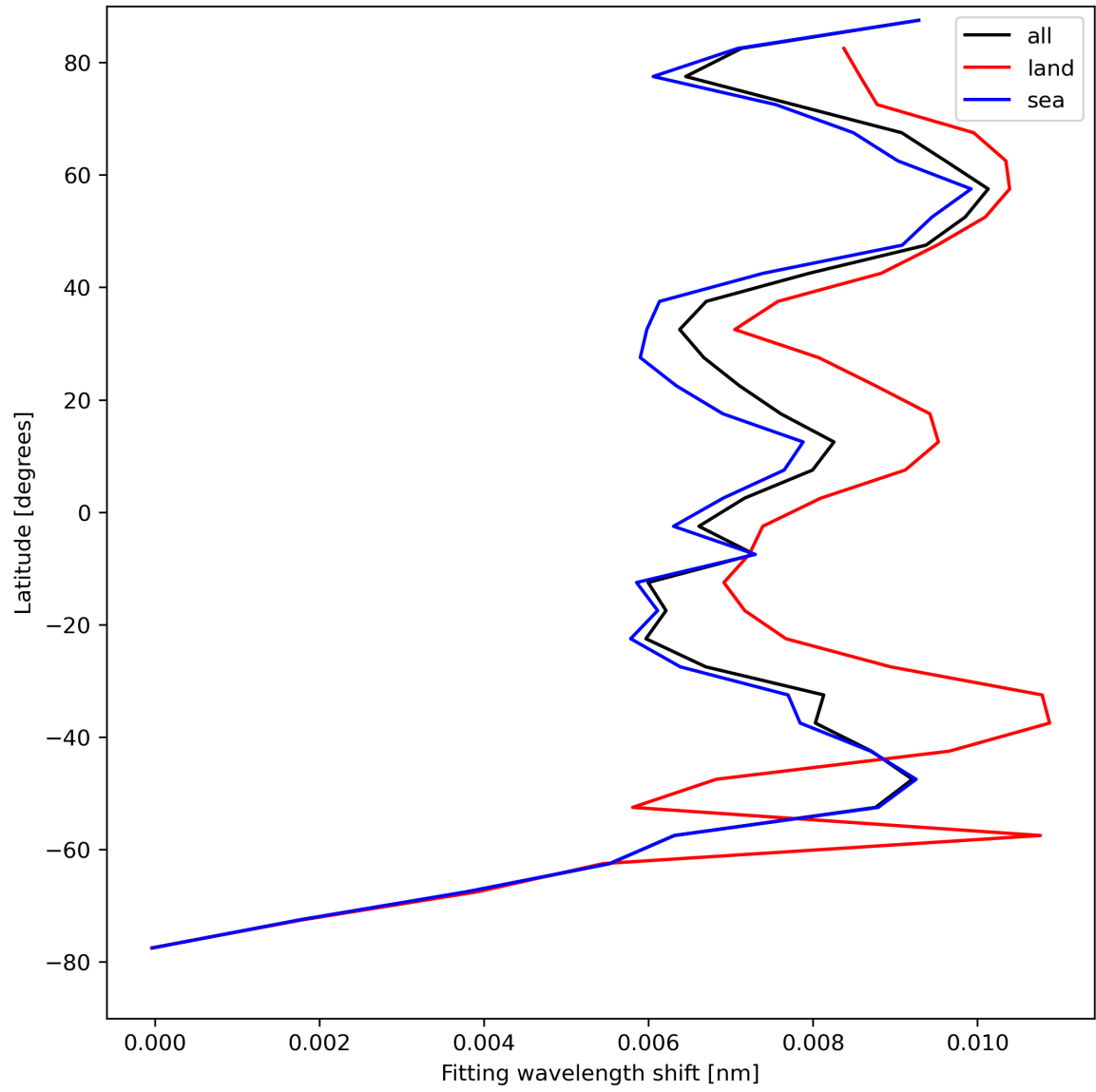
Figure 33: Zonal average of “Fitting wavelength shift” for 2024-08-18 to 2024-08-20.
