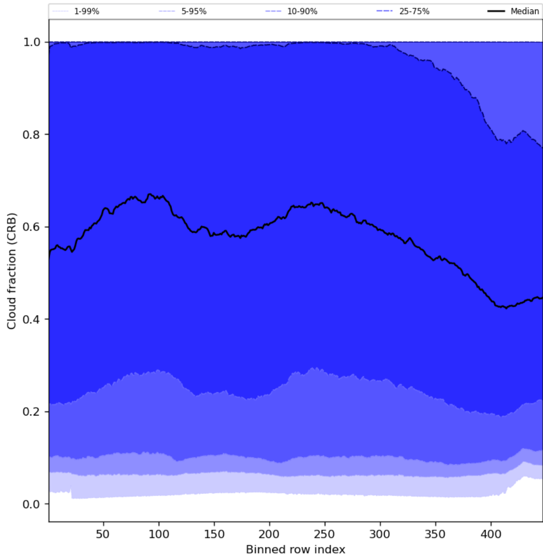
Figure 58: Along track statistics of “Cloud fraction (CRB)” for 2024-08-18 to 2024-08-20
