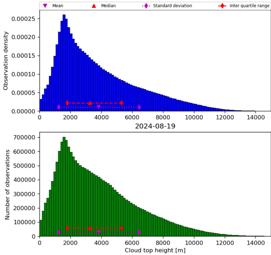
Figure 40: Histogram of “Cloud top height” for 2024-08-18 to 2024-08-20
