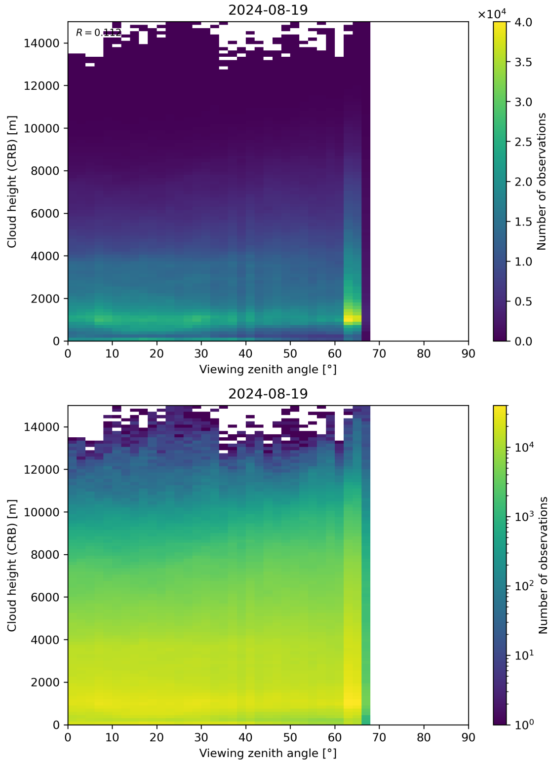
Figure 110: Scatter density plot of “Viewing zenith angle” against “Cloud height (CRB)” for 2024-08-18 to 2024-08-20.
