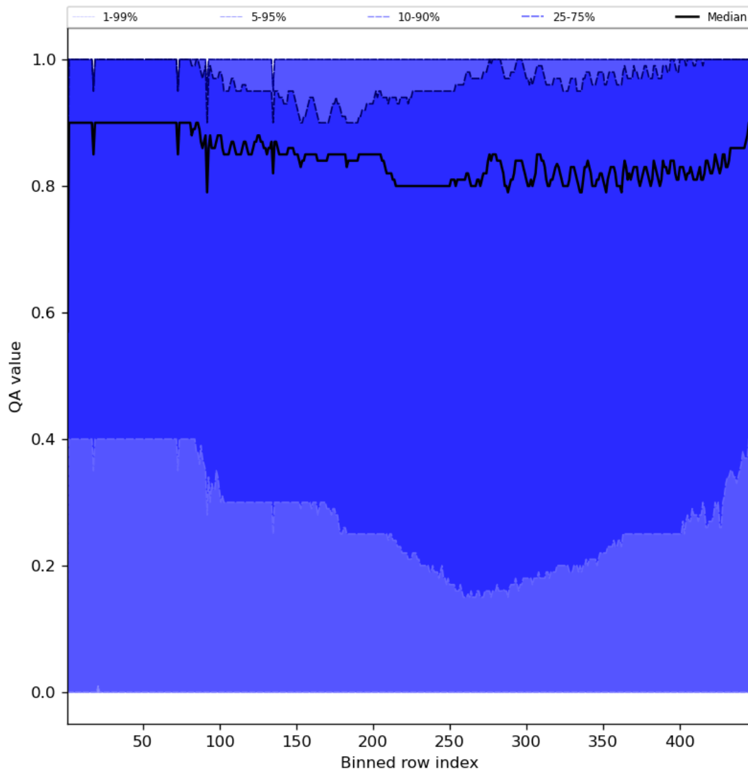
Figure 54: Along track statistics of “QA value” for 2024-08-18 to 2024-08-20
