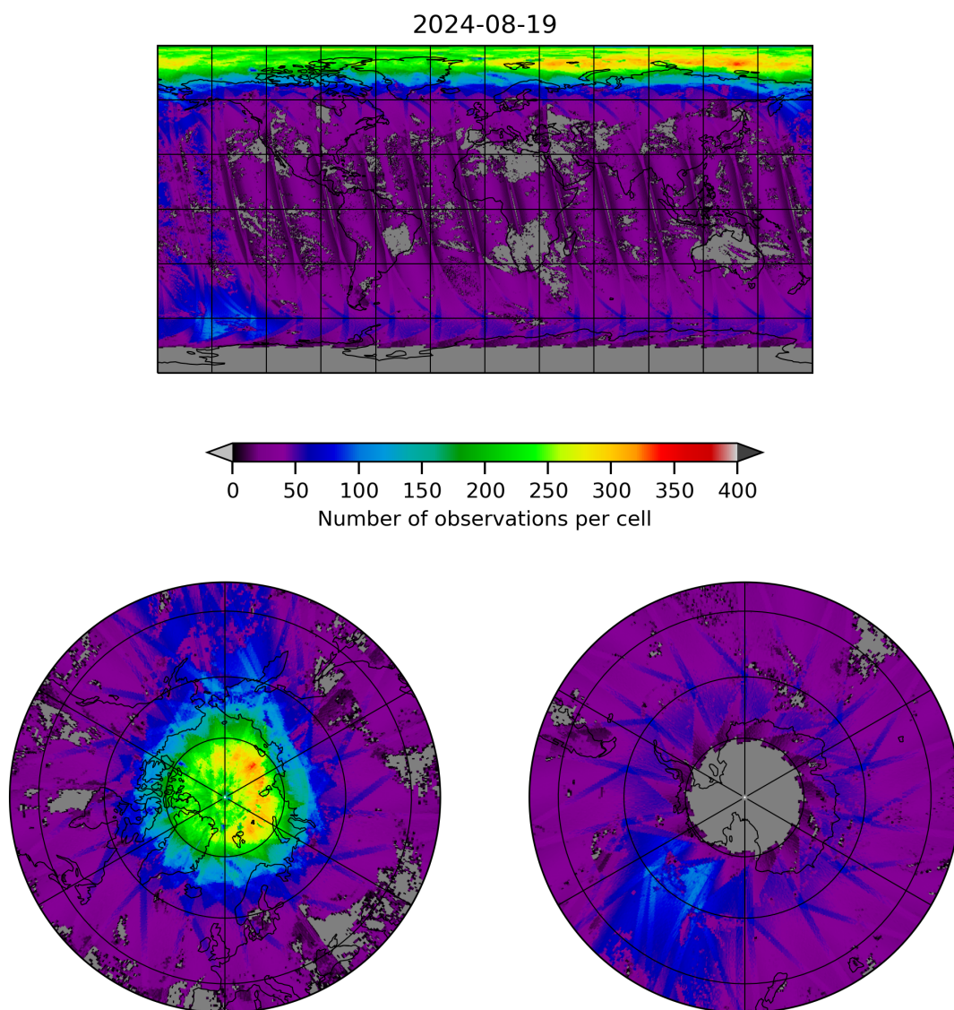
Figure 21: Map of the number of observations for 2024-08-18 to 2024-08-20
