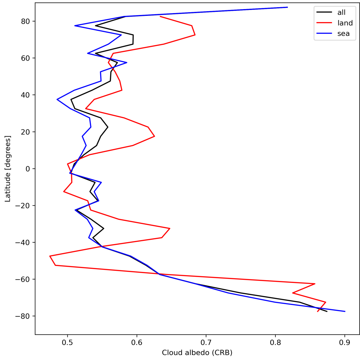
Figure 28: Zonal average of “Cloud albedo (CRB)” for 2024-08-18 to 2024-08-20.
