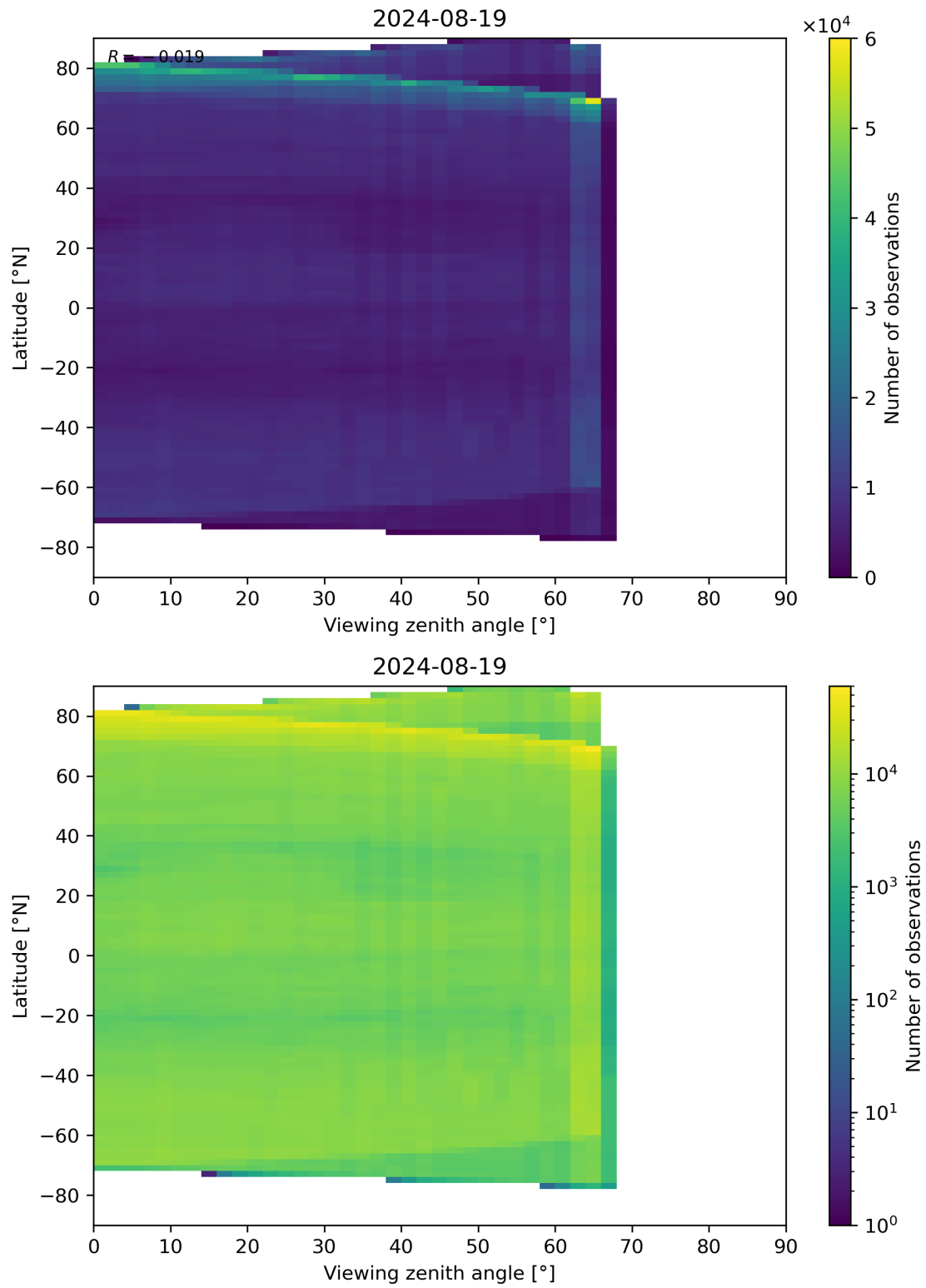
Figure 113: Scatter density plot of “Viewing zenith angle” against “Latitude” for 2024-08-18 to 2024-08-20.
