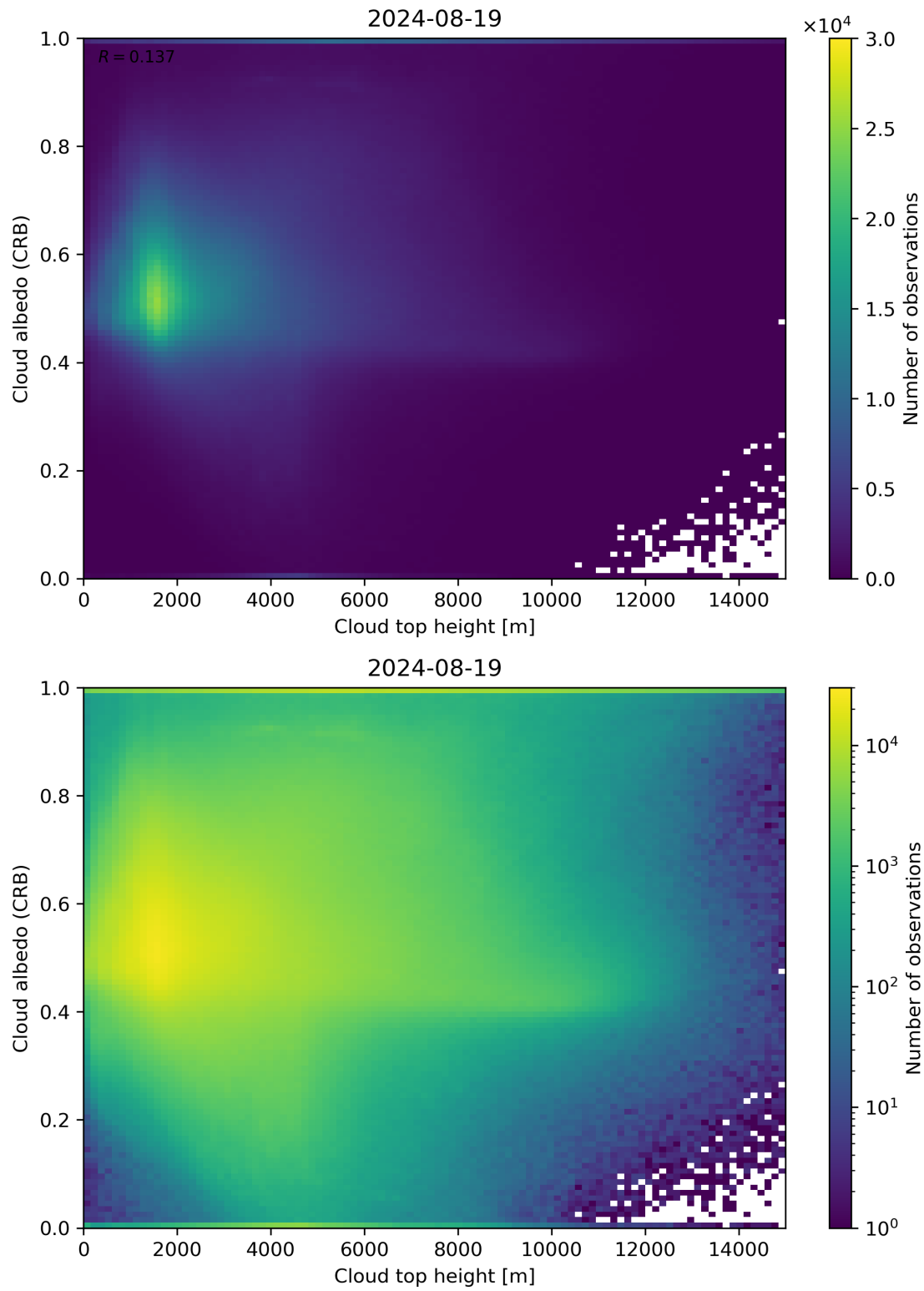
Figure 86: Scatter density plot of “Cloud top height” against “Cloud albedo (CRB)” for 2024-08-18 to 2024-08-20.
