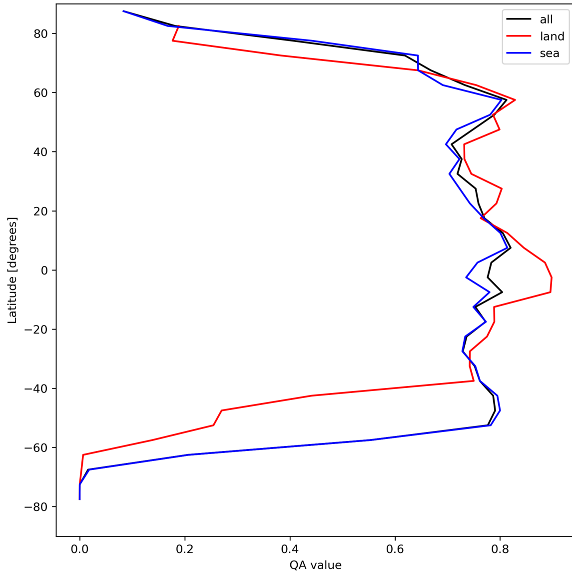
Figure 22: Zonal average of “QA value” for 2024-08-18 to 2024-08-20.
