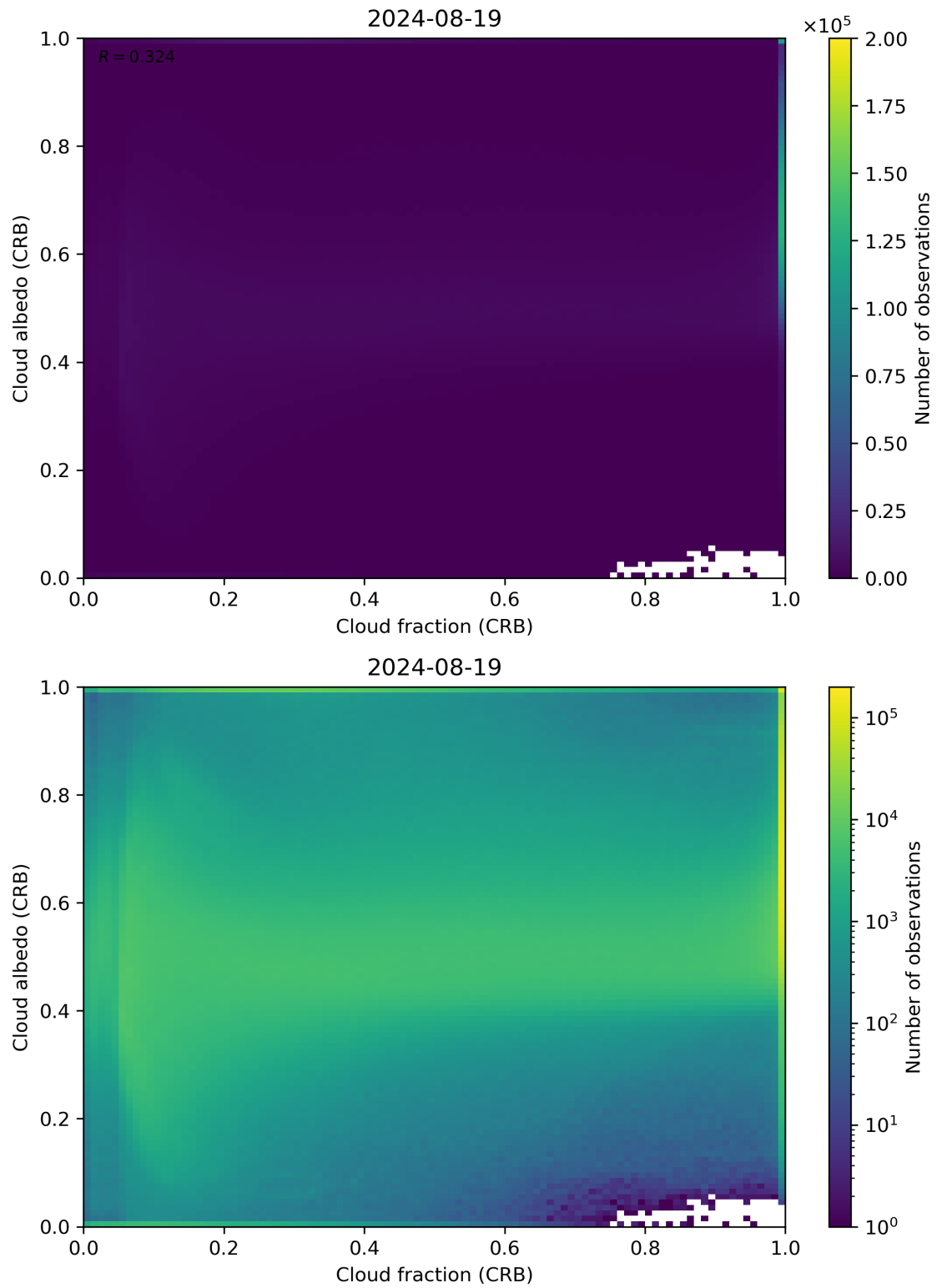
Figure 77: Scatter density plot of “Cloud fraction (CRB)” against “Cloud albedo (CRB)” for 2024-08-18 to 2024-08-20.
