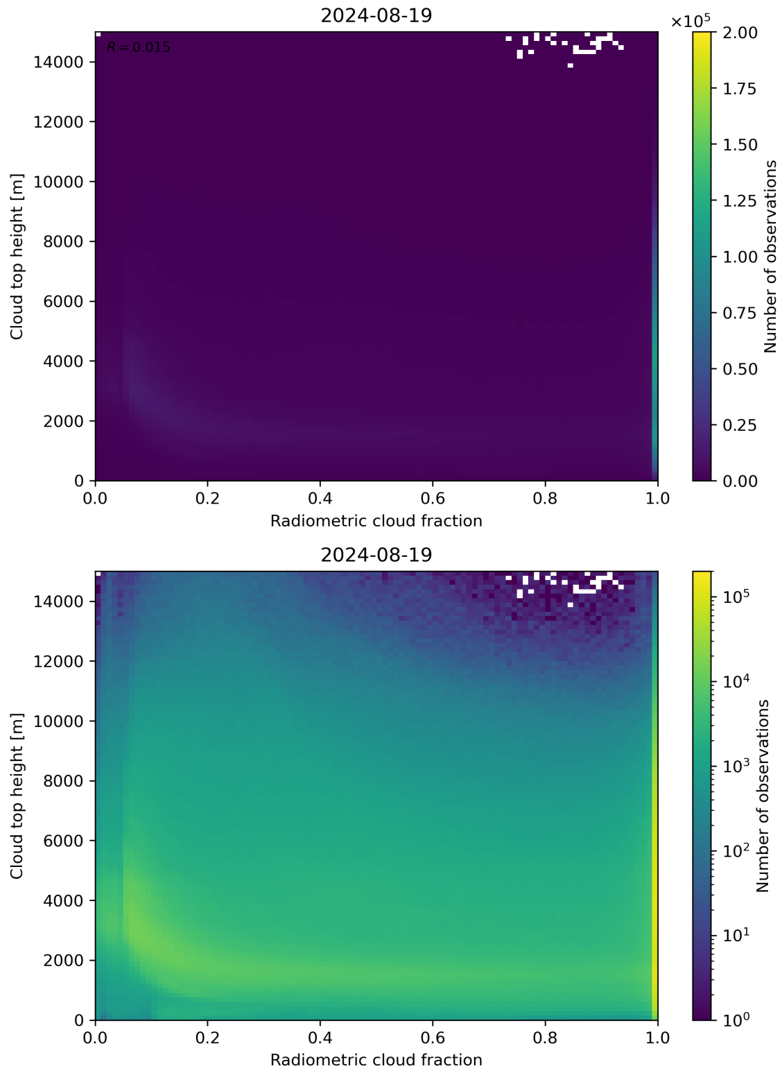
Figure 76: Scatter density plot of “Radiometric cloud fraction” against “Cloud top height” for 2024-08-18 to 2024-08-20.
