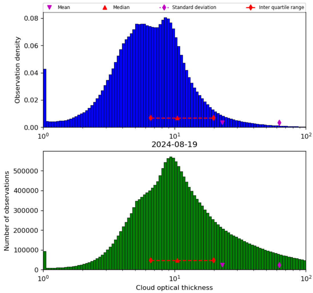
Figure 41: Histogram of “Cloud optical thickness” for 2024-08-18 to 2024-08-20
