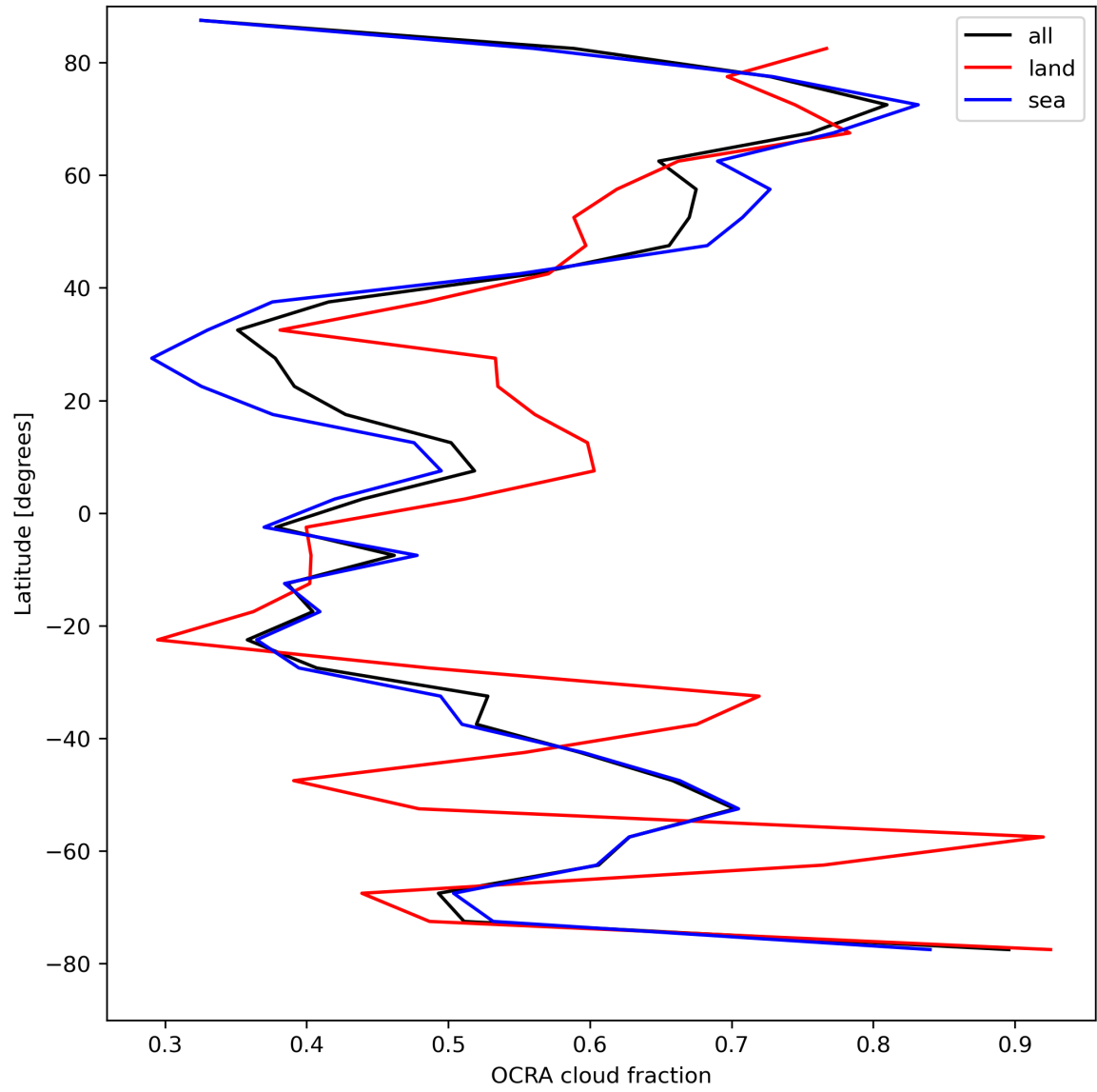
Figure 34: Zonal average of “OCRA cloud fraction” for 2024-08-18 to 2024-08-20.
