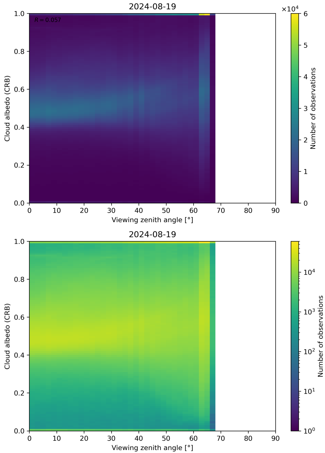
Figure 106: Scatter density plot of “Viewing zenith angle” against “Cloud albedo (CRB)” for 2024-08-18 to 2024-08-20.
