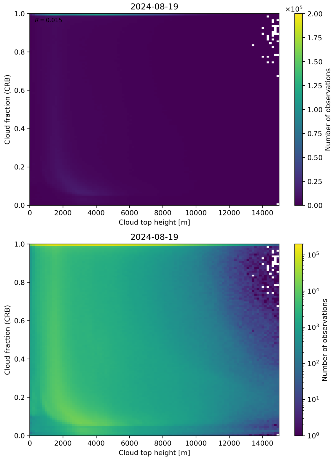
Figure 88: Scatter density plot of “Cloud top height” against “Cloud fraction (CRB)” for 2024-08-18 to 2024-08-20.
