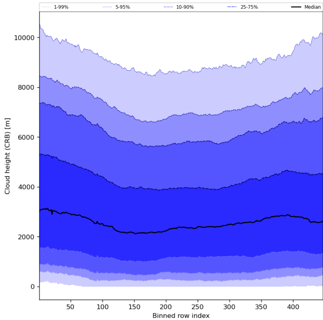
Figure 59: Along track statistics of “Cloud height (CRB)” for 2024-08-18 to 2024-08-20
