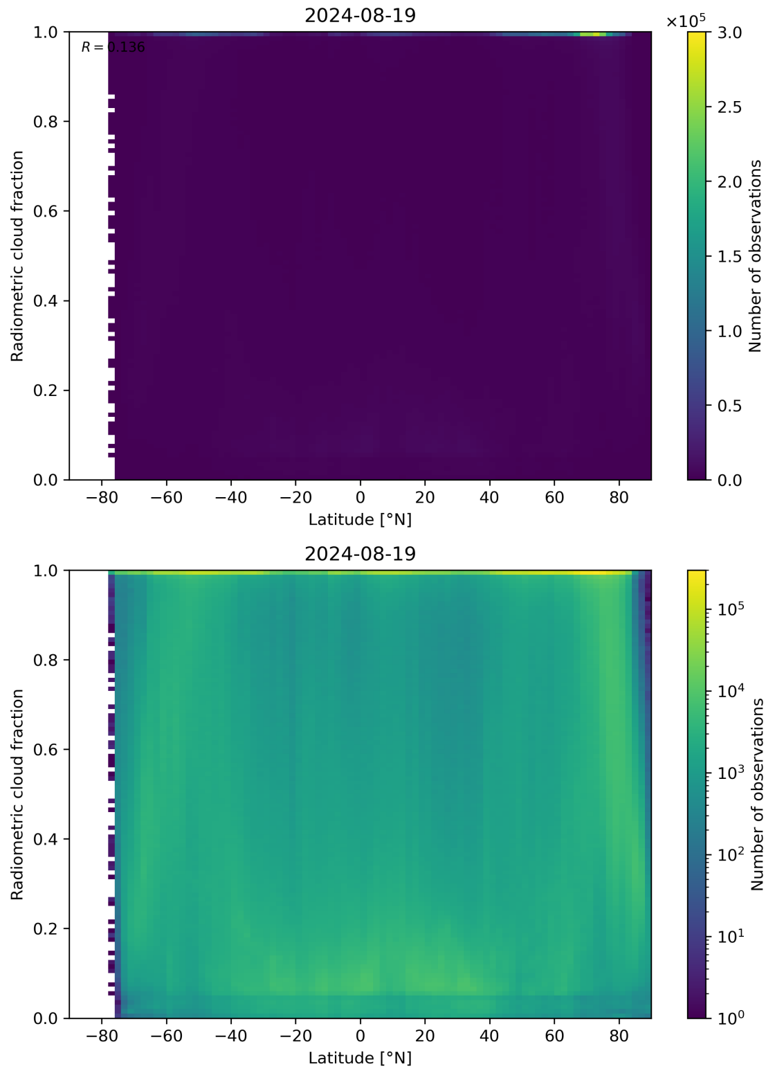
Figure 92: Scatter density plot of “Latitude” against “Radiometric cloud fraction” for 2024-08-18 to 2024-08-20.
