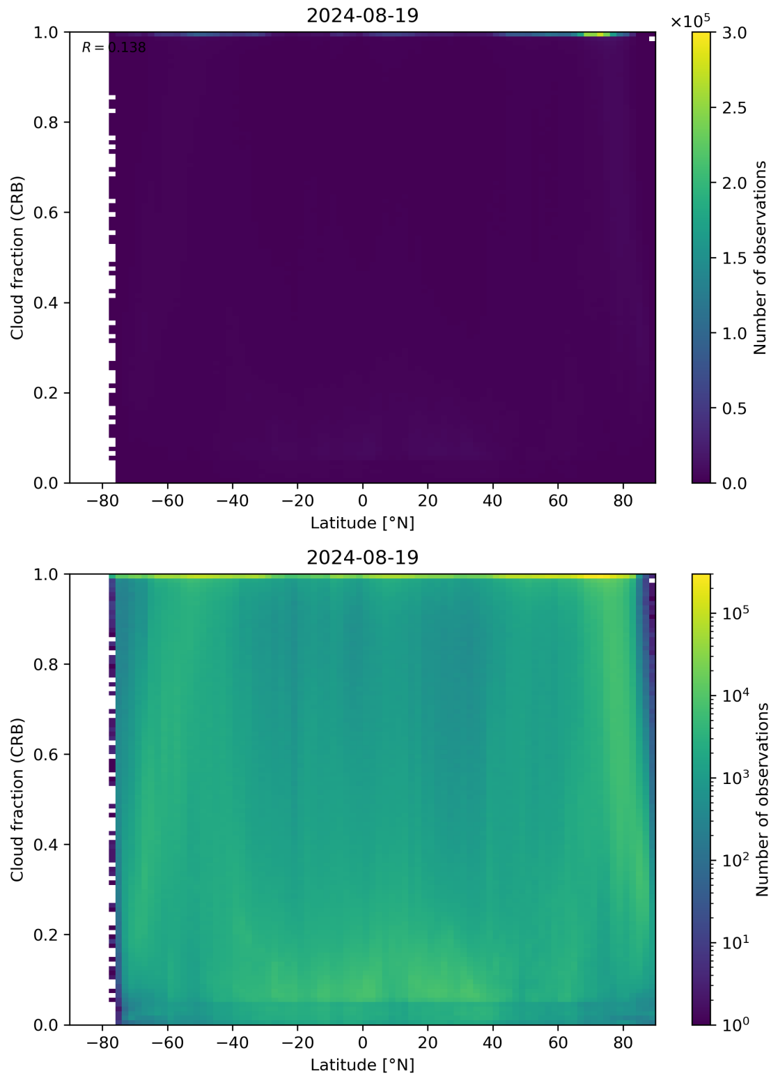
Figure 94: Scatter density plot of “Latitude” against “Cloud fraction (CRB)” for 2024-08-18 to 2024-08-20.
