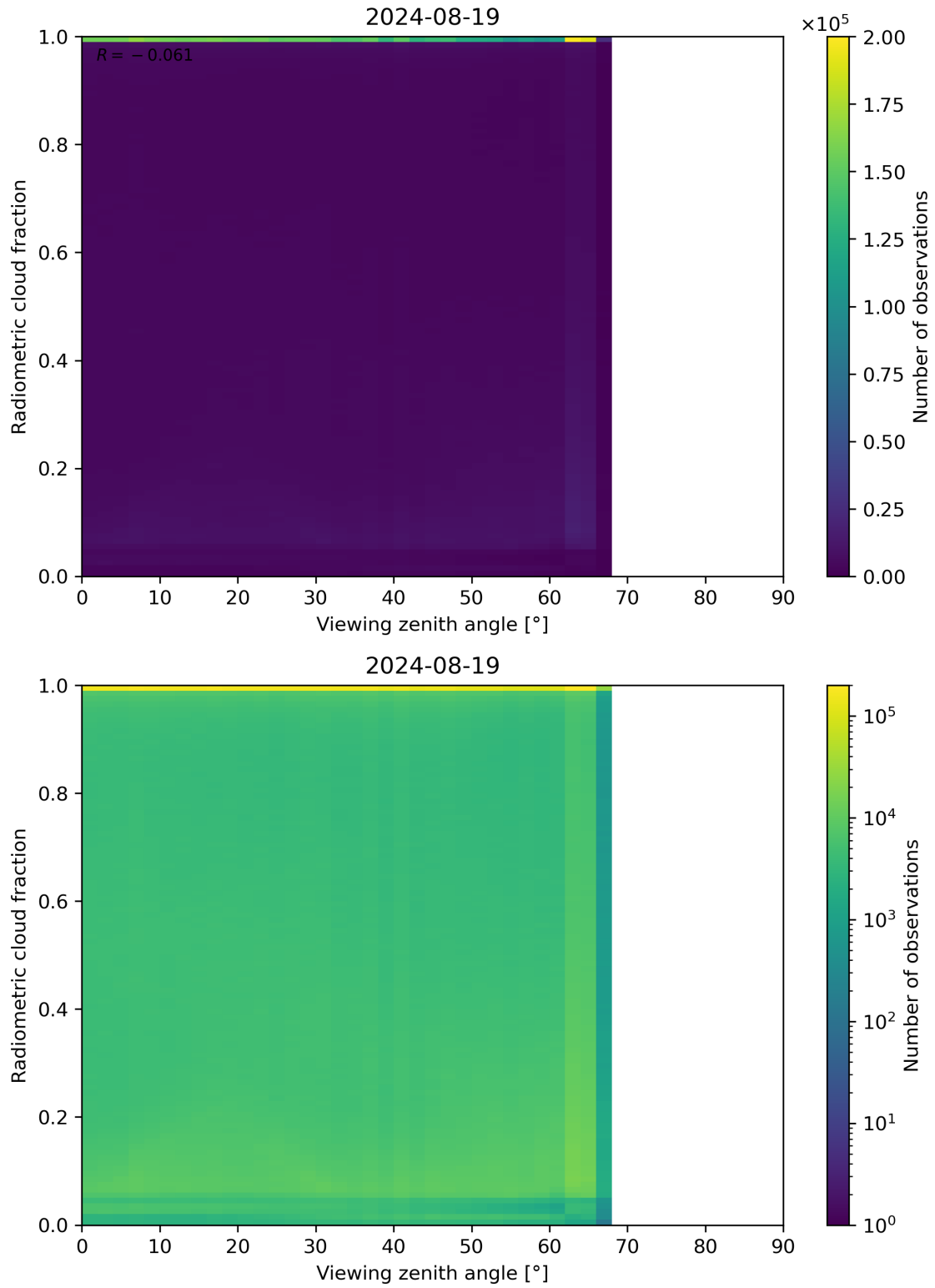
Figure 107: Scatter density plot of “Viewing zenith angle” against “Radiometric cloud fraction” for 2024-08-18 to 2024-08-20.
