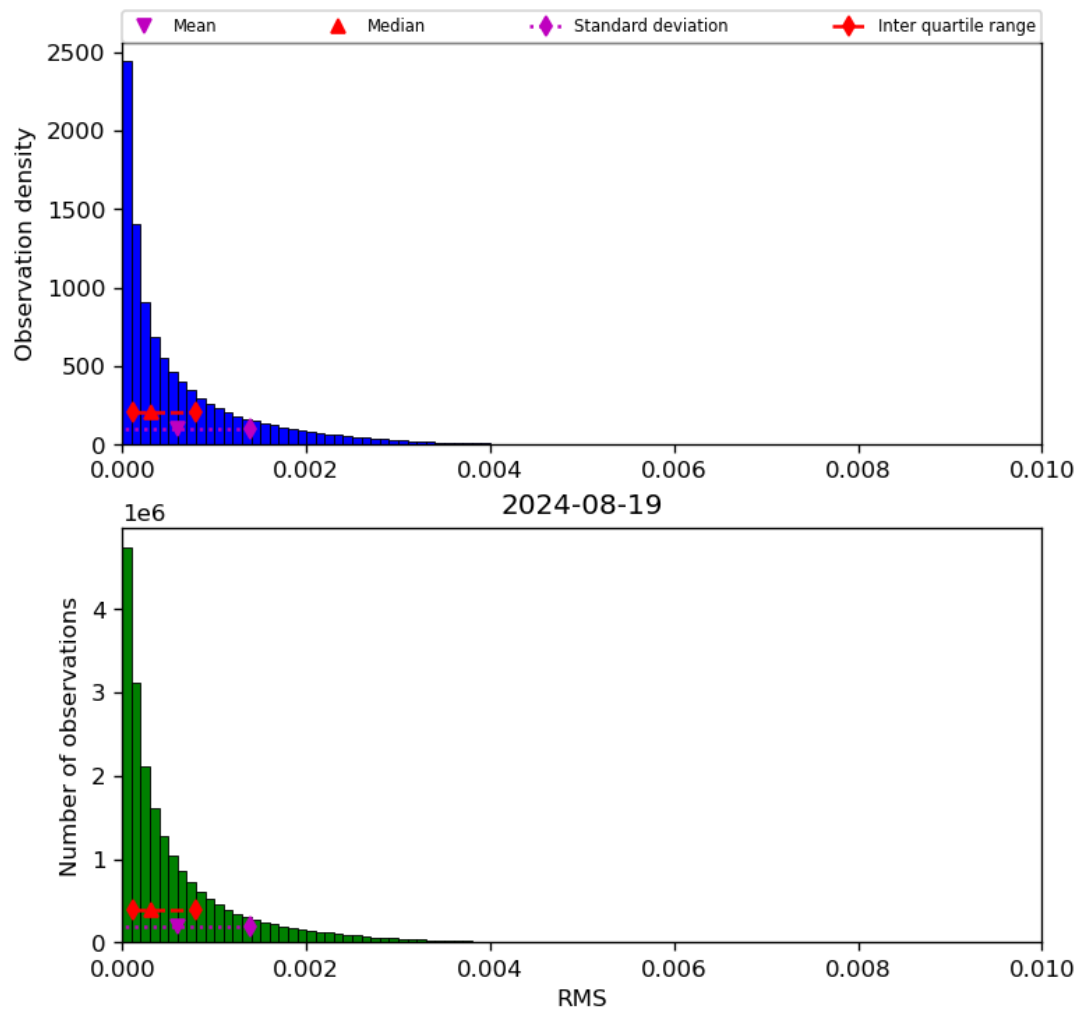
Figure 47: Histogram of “RMS” for 2024-08-18 to 2024-08-20
