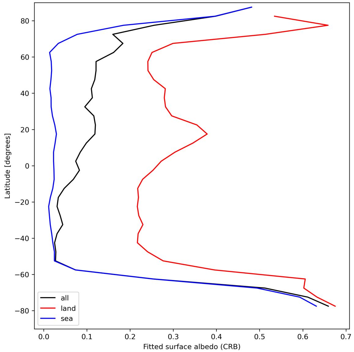
Figure 30: Zonal average of “Fitted surface albedo (CRB)” for 2024-08-18 to 2024-08-20.
