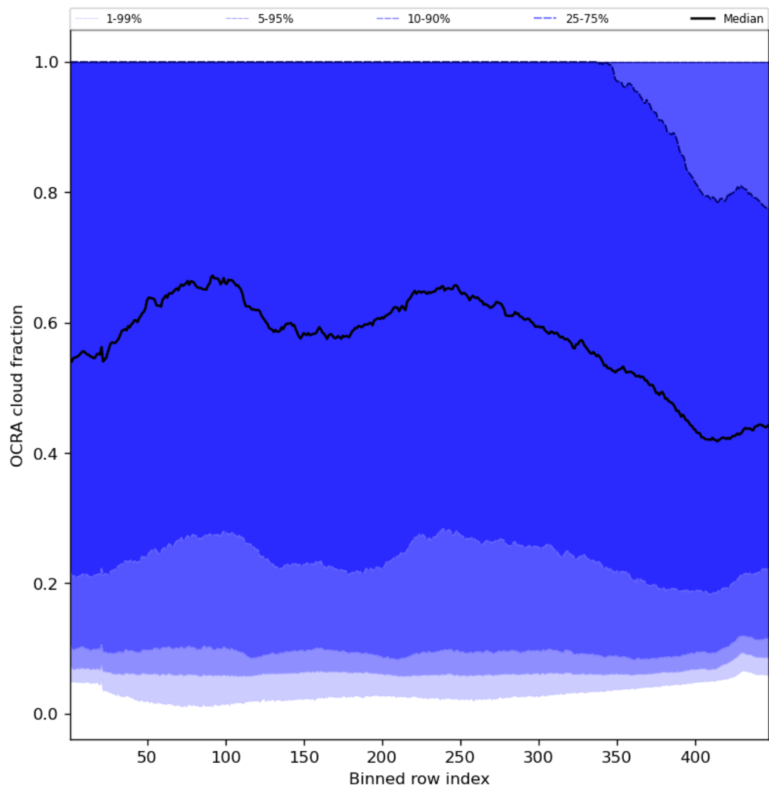
Figure 66: Along track statistics of “OCRA cloud fraction” for 2024-08-18 to 2024-08-20
