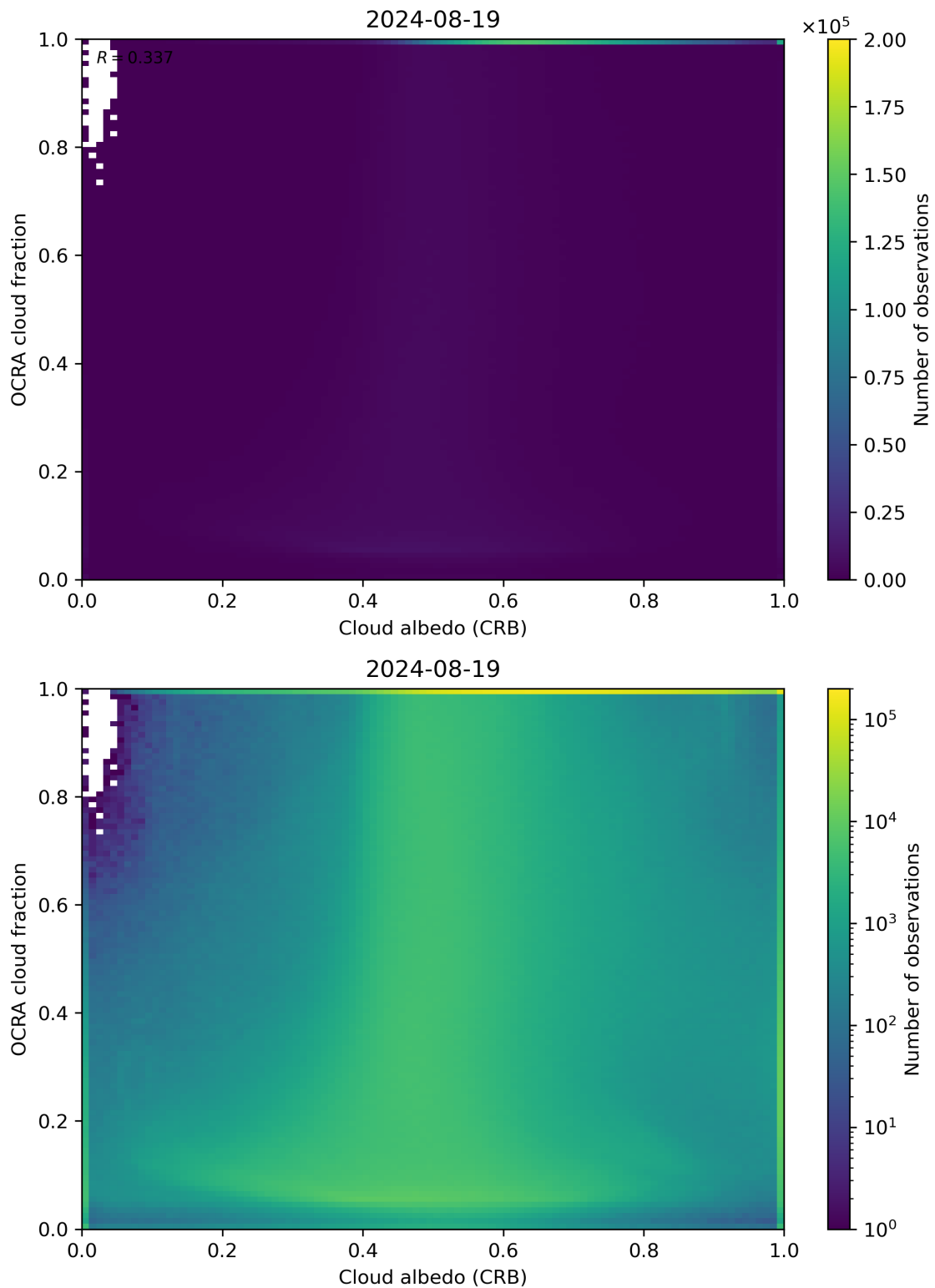
Figure 70: Scatter density plot of “Cloud albedo (CRB)” against “OCRA cloud fraction” for 2024-08-18 to 2024-08-20.
