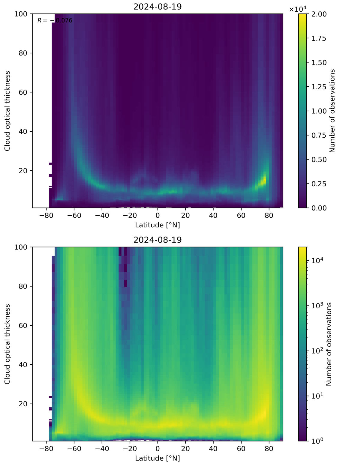
Figure 96: Scatter density plot of “Latitude” against “Cloud optical thickness” for 2024-08-18 to 2024-08-20.
