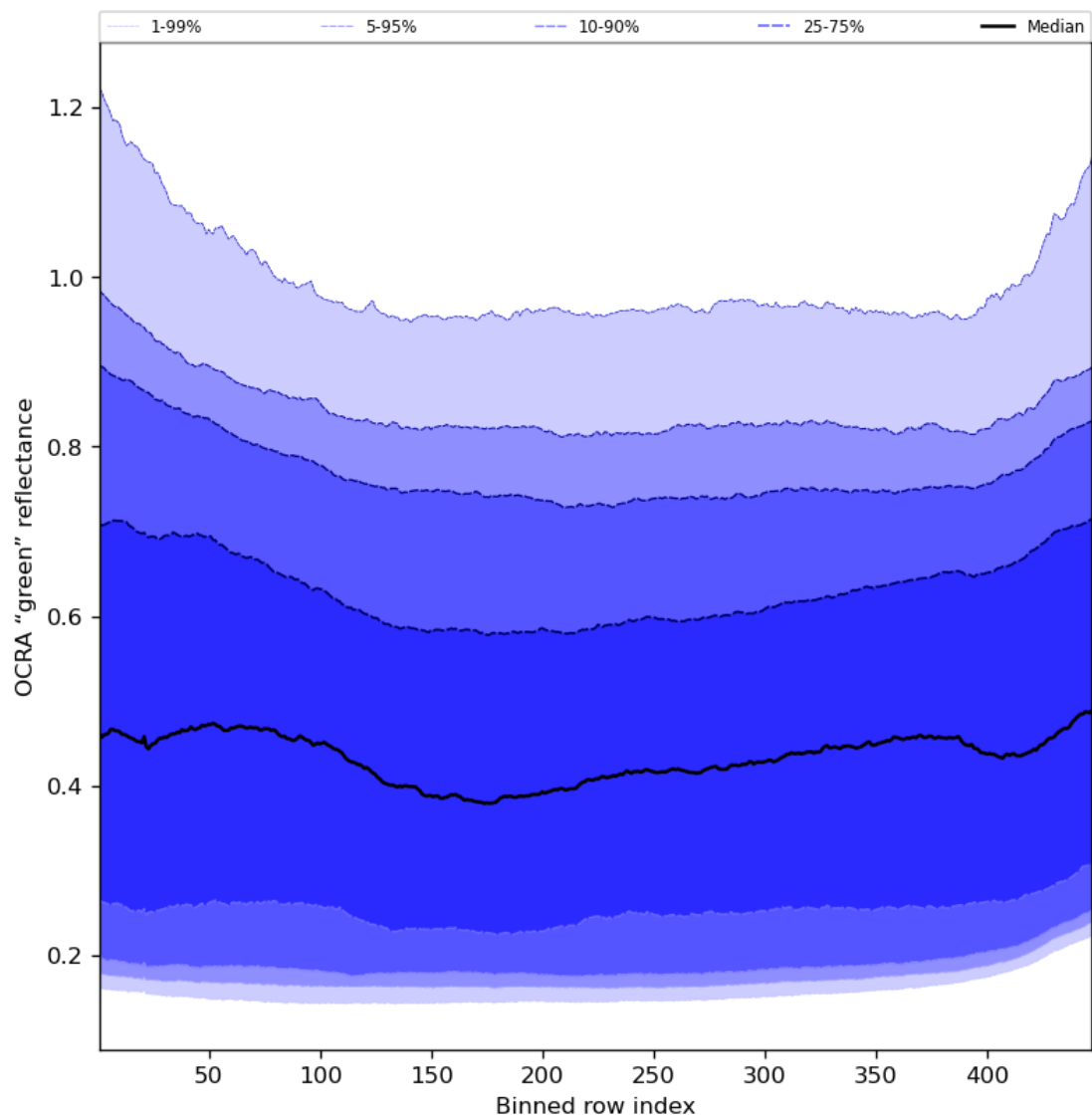
Figure 68: Along track statistics of “OCRA “green” reflectance” for 2024-08-18 to 2024-08-20
