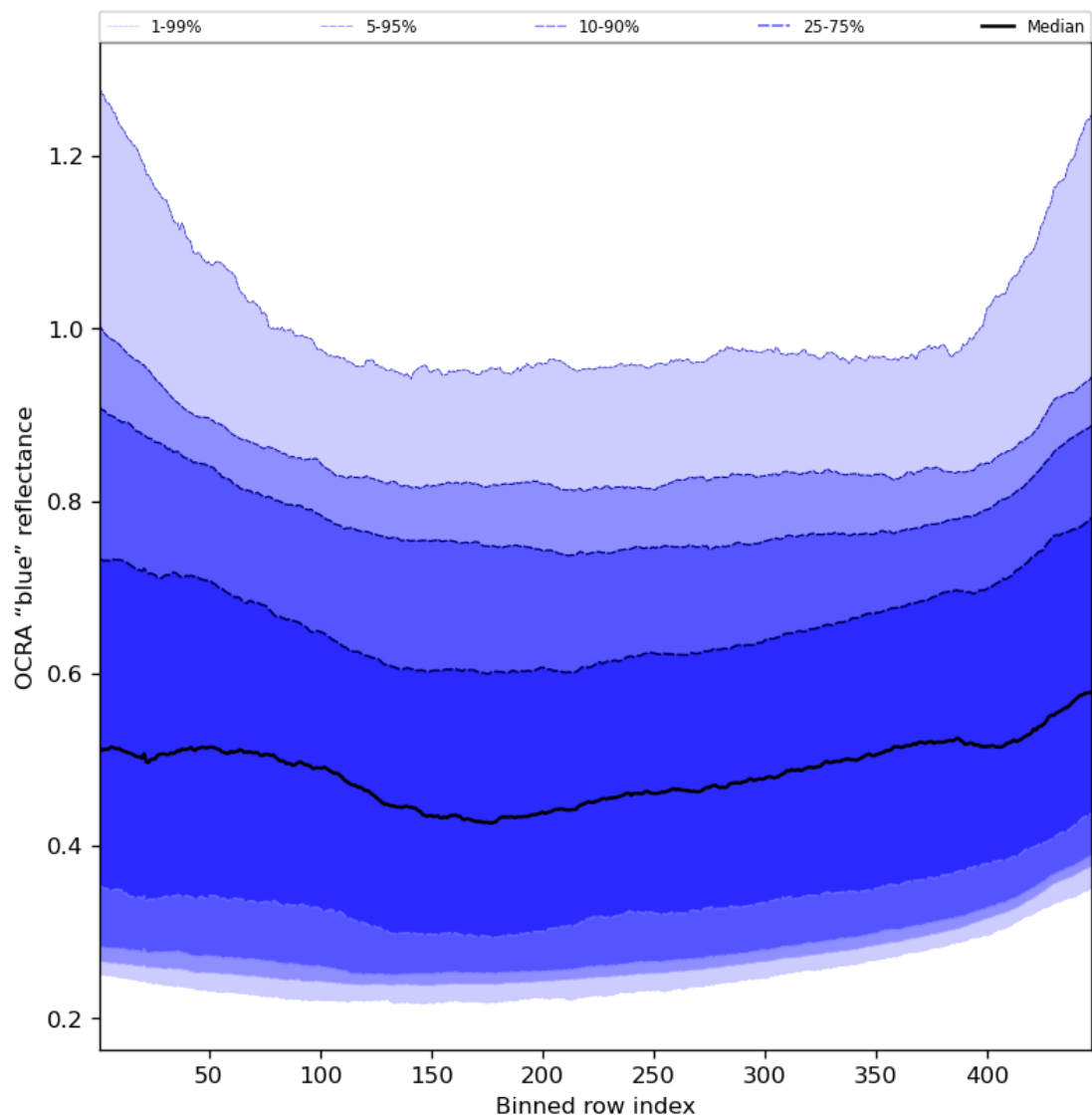
Figure 67: Along track statistics of “OCRA “blue” reflectance” for 2024-08-18 to 2024-08-20
