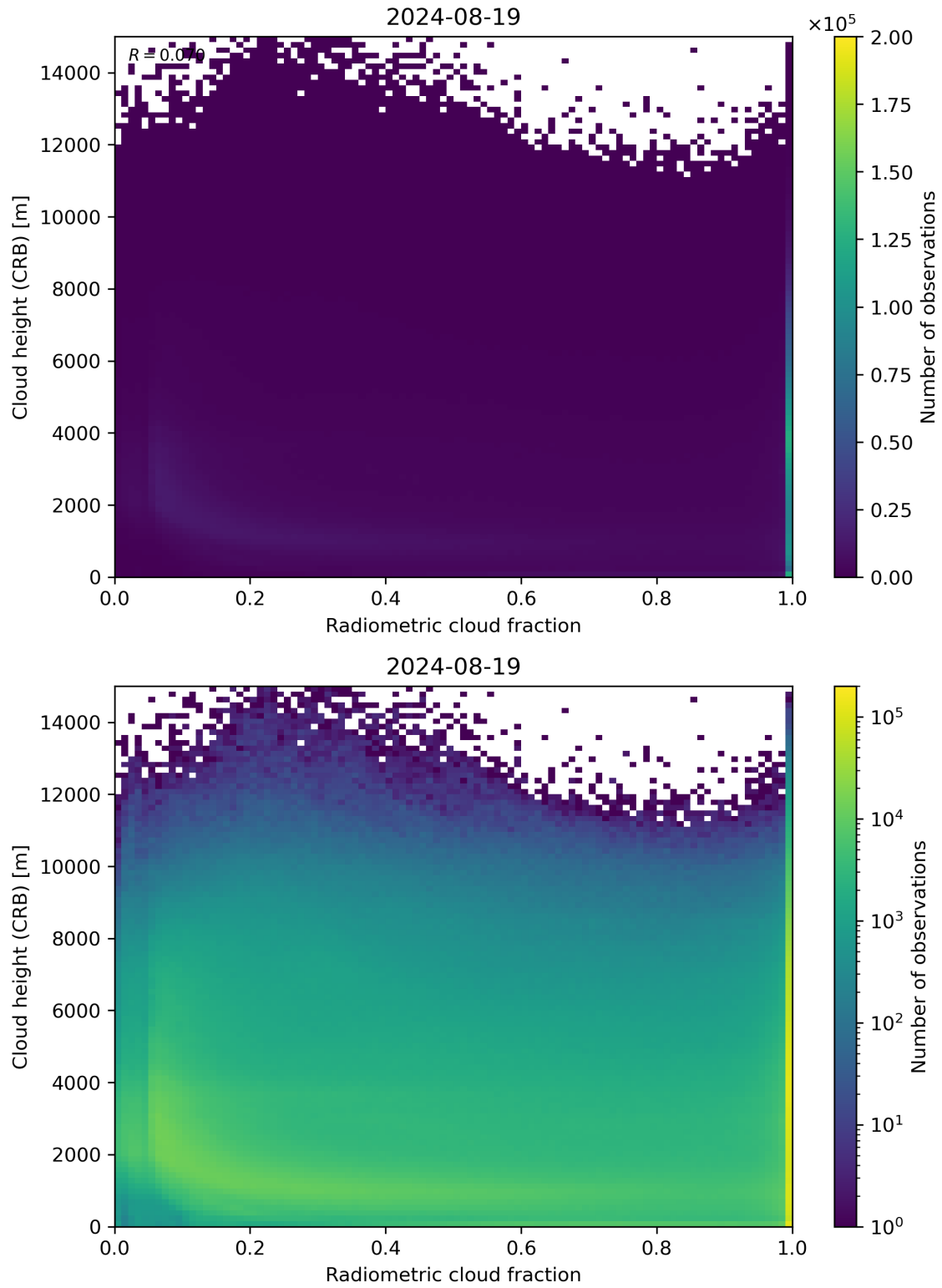
Figure 74: Scatter density plot of “Radiometric cloud fraction” against “Cloud height (CRB)” for 2024-08-18 to 2024-08-20.
