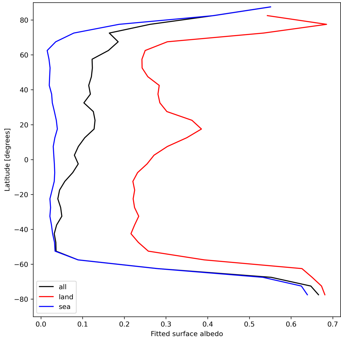
Figure 29: Zonal average of “Fitted surface albedo” for 2024-08-18 to 2024-08-20.
