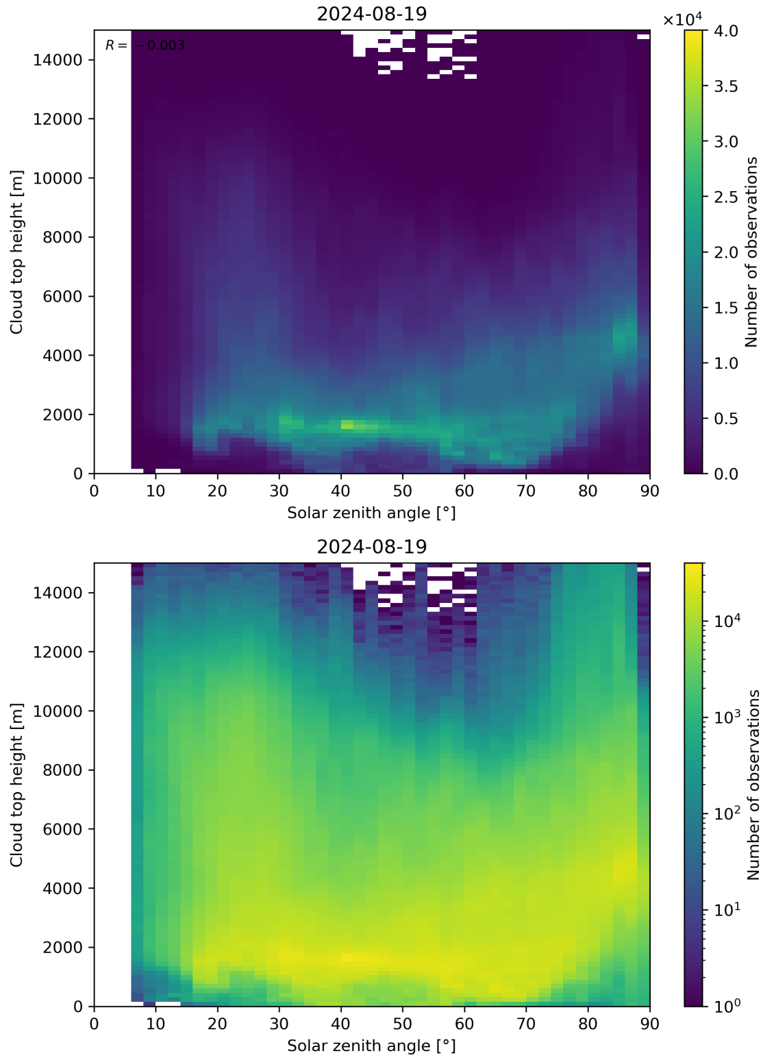
Figure 104: Scatter density plot of “Solar zenith angle” against “Cloud top height” for 2024-08-18 to 2024-08-20.
