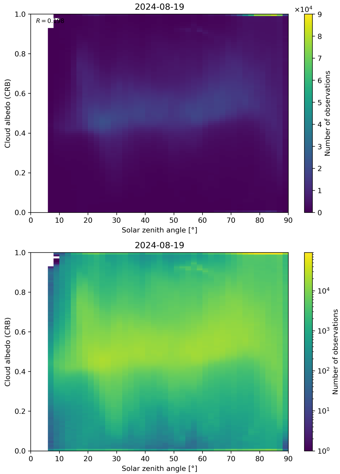
Figure 98: Scatter density plot of “Solar zenith angle” against “Cloud albedo (CRB)” for 2024-08-18 to 2024-08-20.
