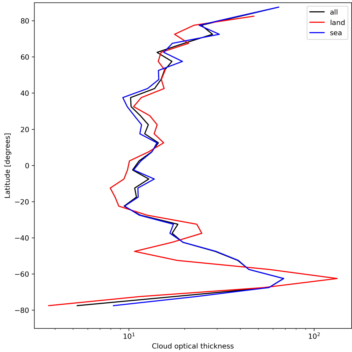
Figure 25: Zonal average of “Cloud optical thickness” for 2024-08-18 to 2024-08-20.
