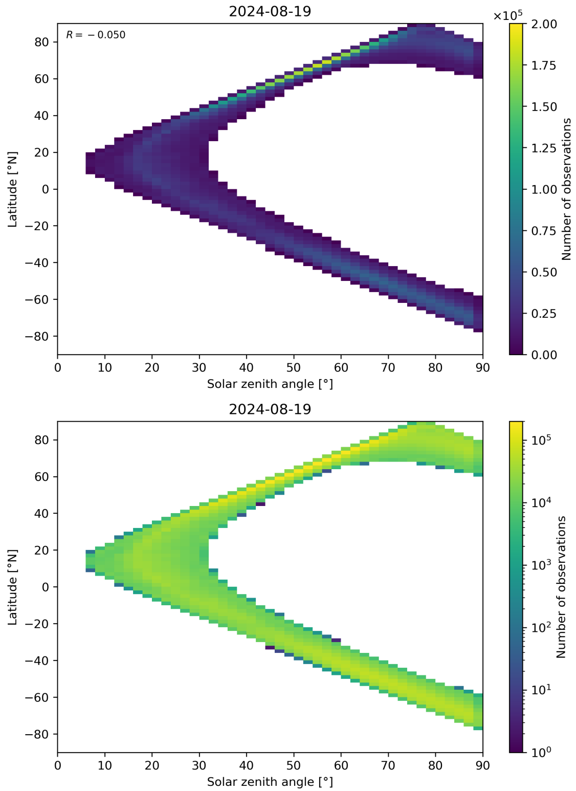
Figure 105: Scatter density plot of “Solar zenith angle” against “Latitude” for 2024-08-18 to 2024-08-20.
