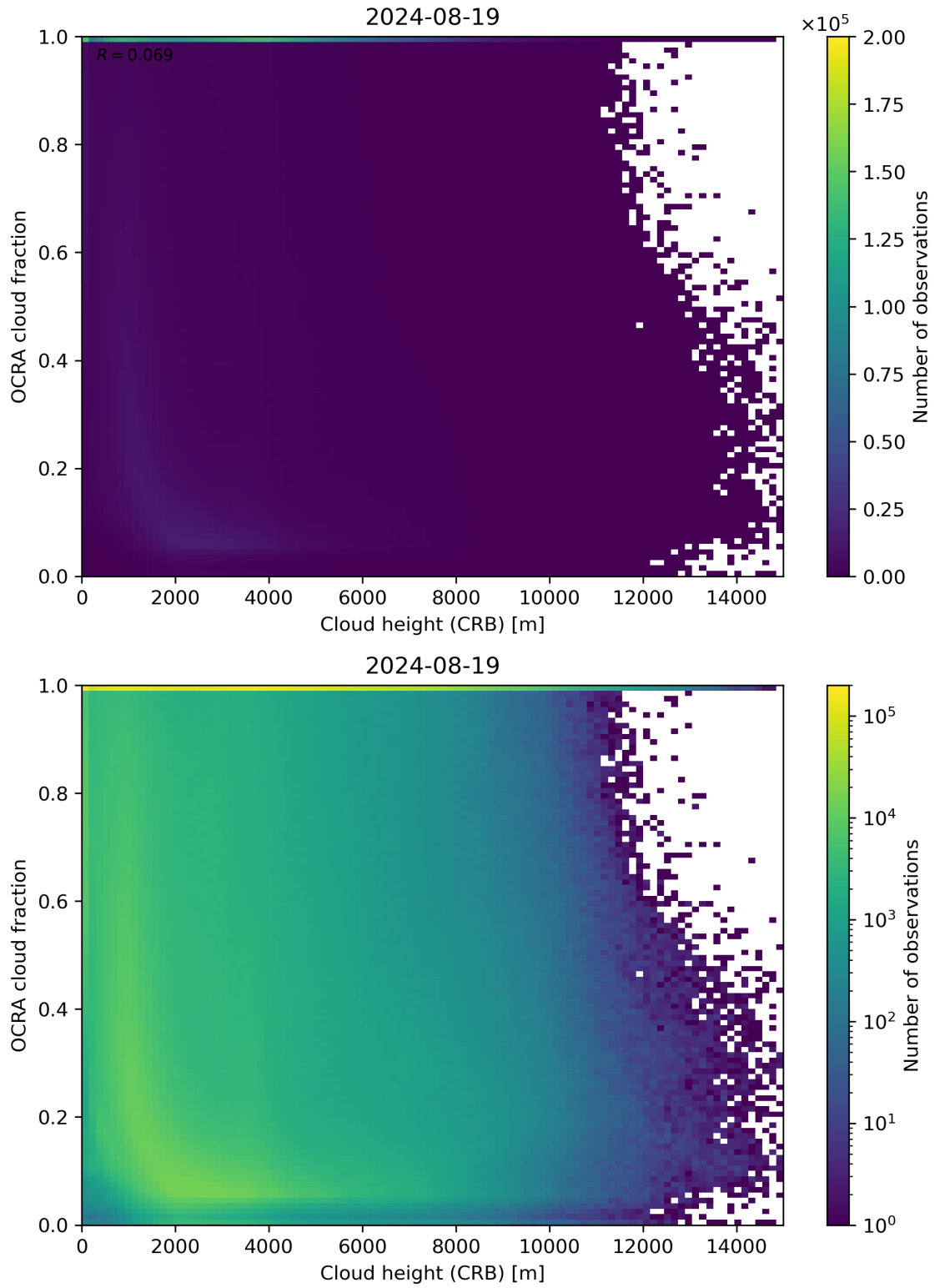
Figure 81: Scatter density plot of “Cloud height (CRB)” against “OCRA cloud fraction” for 2024-08-18 to 2024-08-20.
