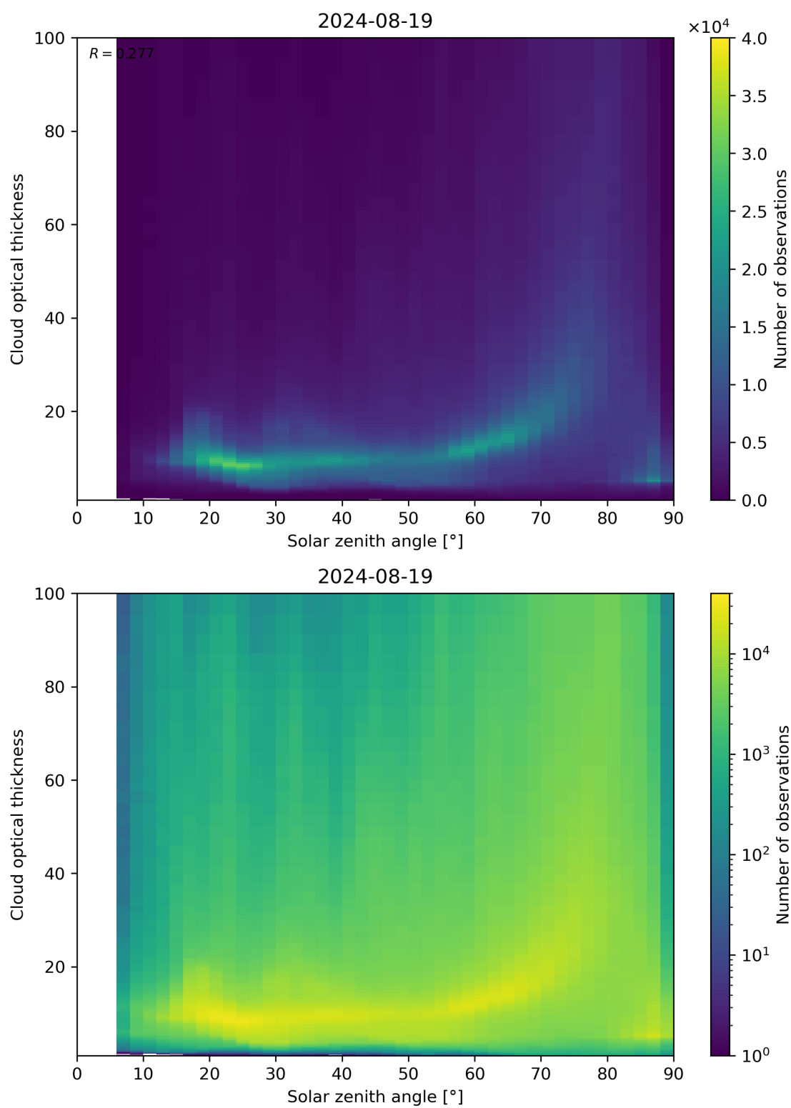
Figure 103: Scatter density plot of “Solar zenith angle” against “Cloud optical thickness” for 2024-08-18 to 2024-08-20.
