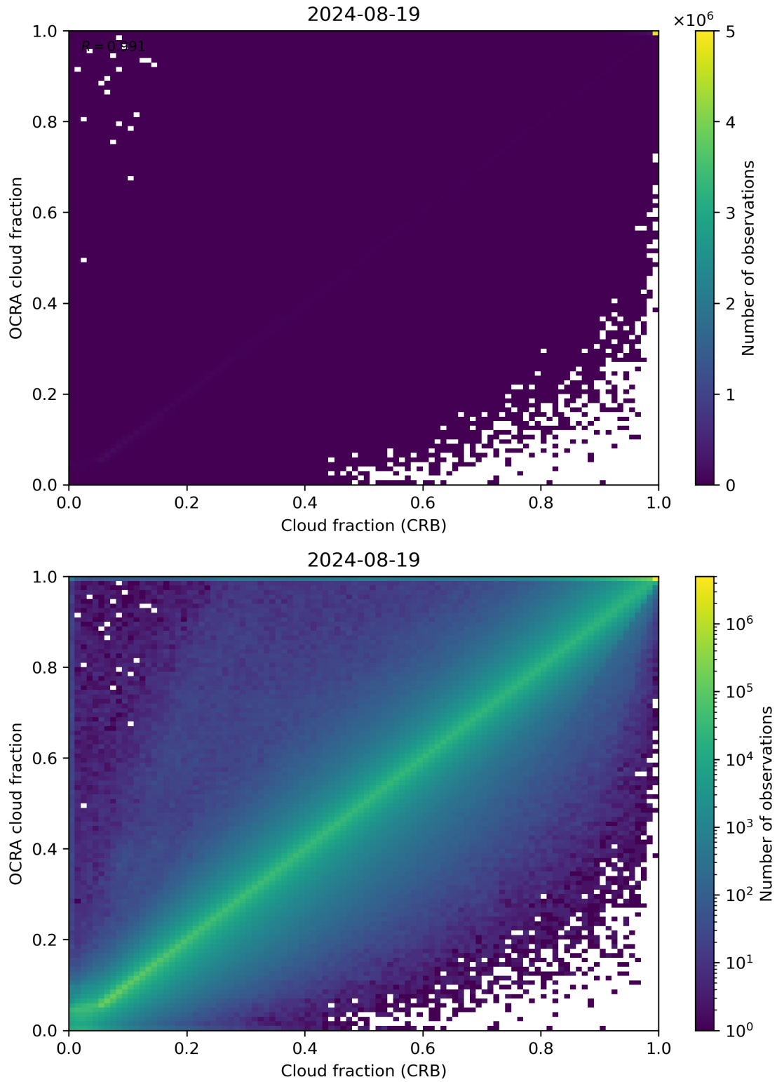
Figure 78: Scatter density plot of “Cloud fraction (CRB)” against “OCRA cloud fraction” for 2024-08-18 to 2024-08-20.
