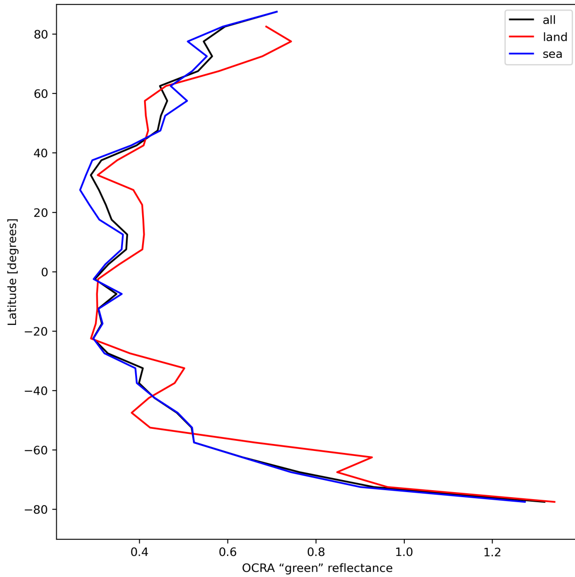
Figure 36: Zonal average of “OCRA “green” reflectance” for 2024-08-18 to 2024-08-20.
