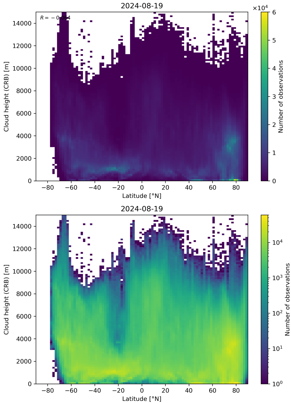
Figure 95: Scatter density plot of “Latitude” against “Cloud height (CRB)” for 2024-08-18 to 2024-08-20.
