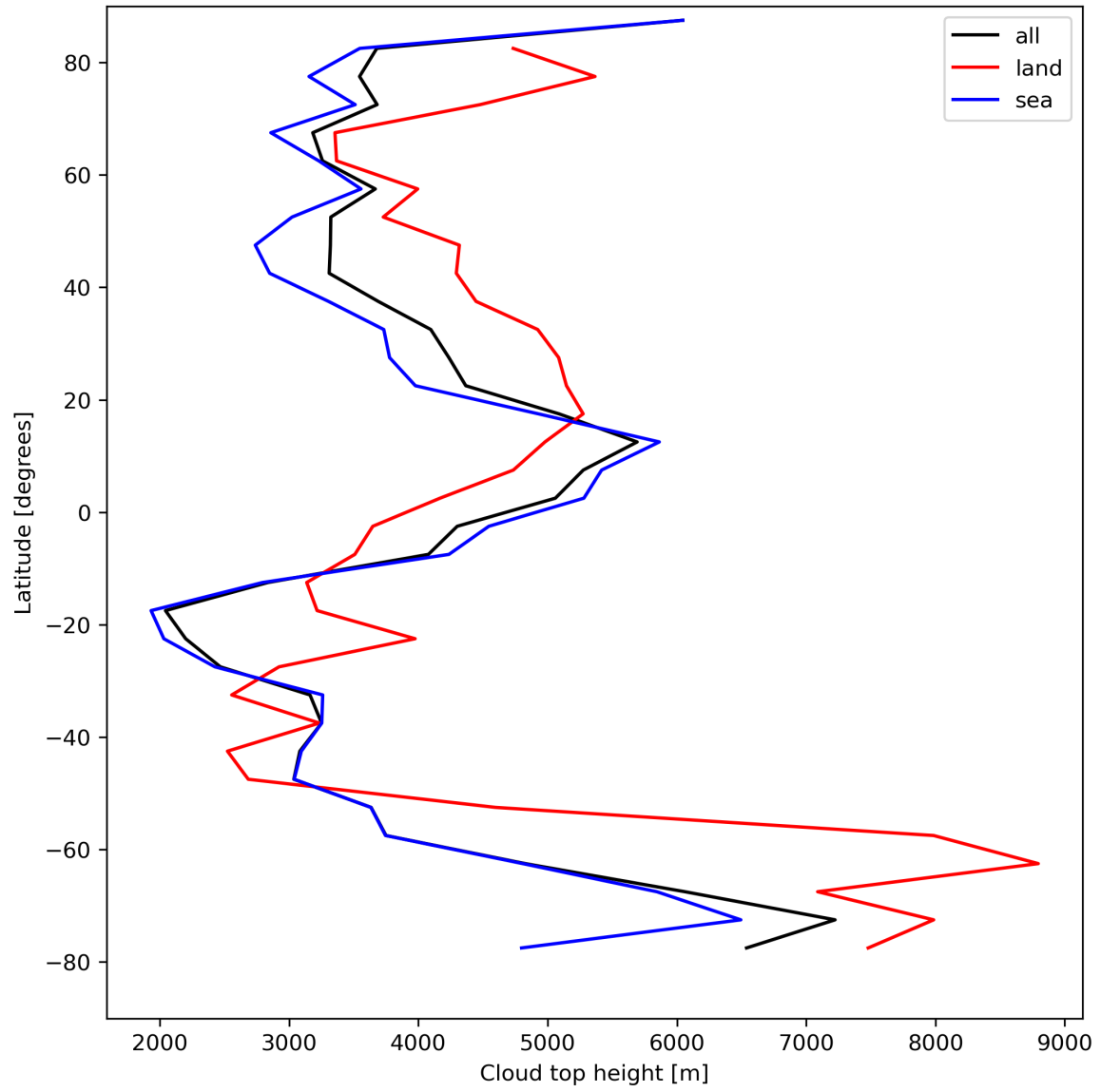
Figure 24: Zonal average of “Cloud top height” for 2024-08-18 to 2024-08-20.
