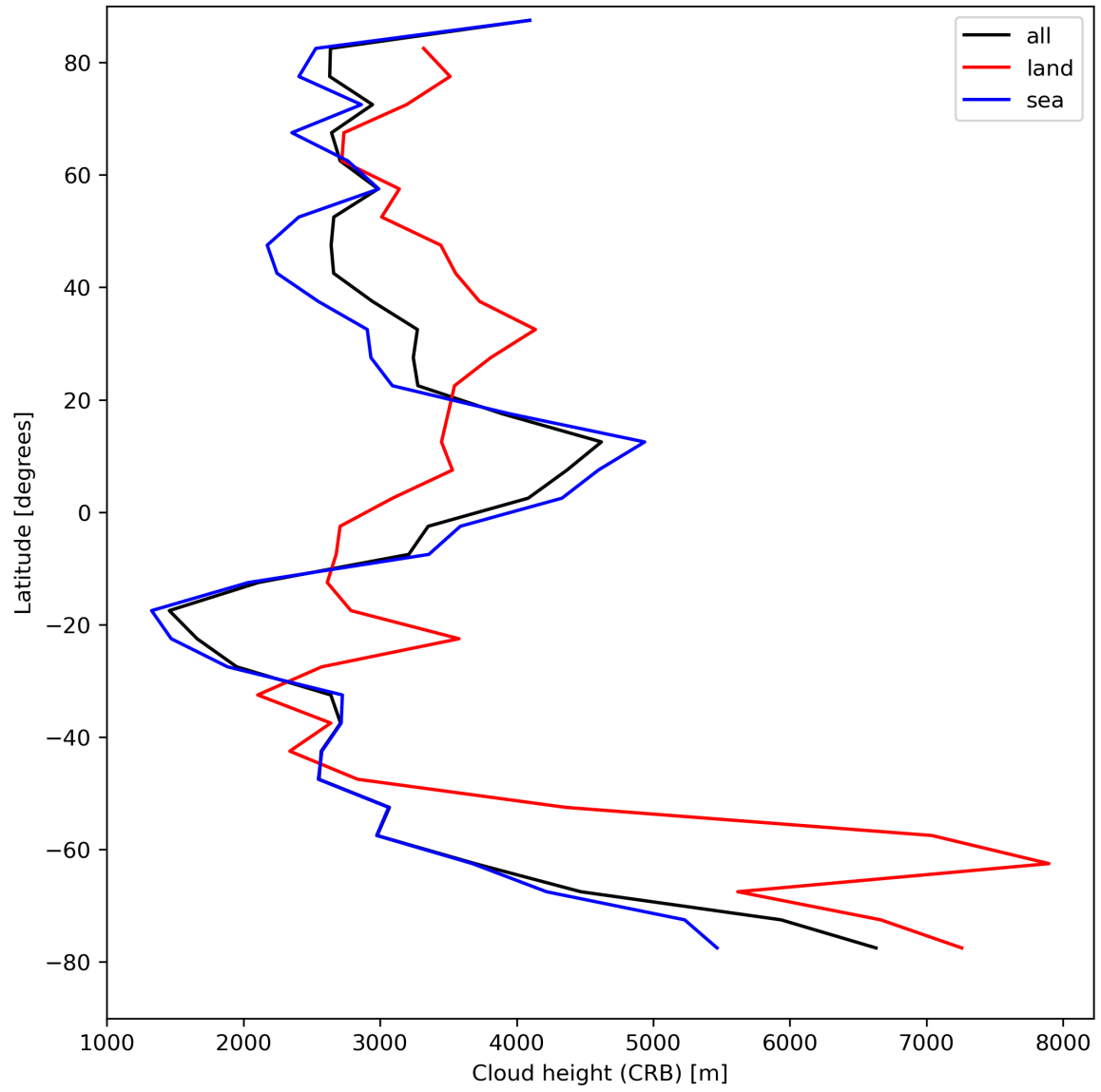
Figure 27: Zonal average of “Cloud height (CRB)” for 2024-08-18 to 2024-08-20.
