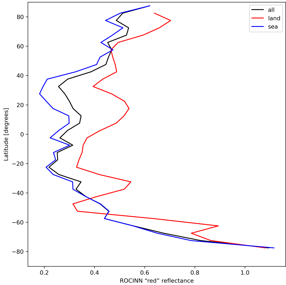
Figure 37: Zonal average of “ROCINN “red” reflectance” for 2024-08-18 to 2024-08-20.
