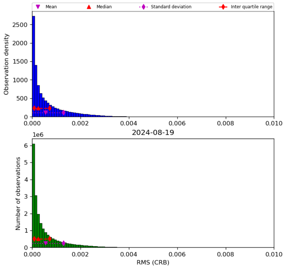
Figure 48: Histogram of “RMS (CRB)” for 2024-08-18 to 2024-08-20
