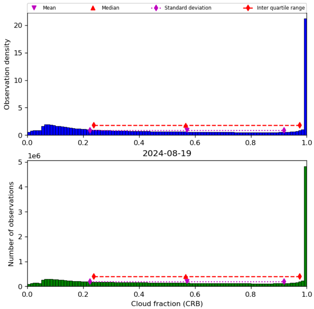
Figure 42: Histogram of “Cloud fraction (CRB)” for 2024-08-18 to 2024-08-20
