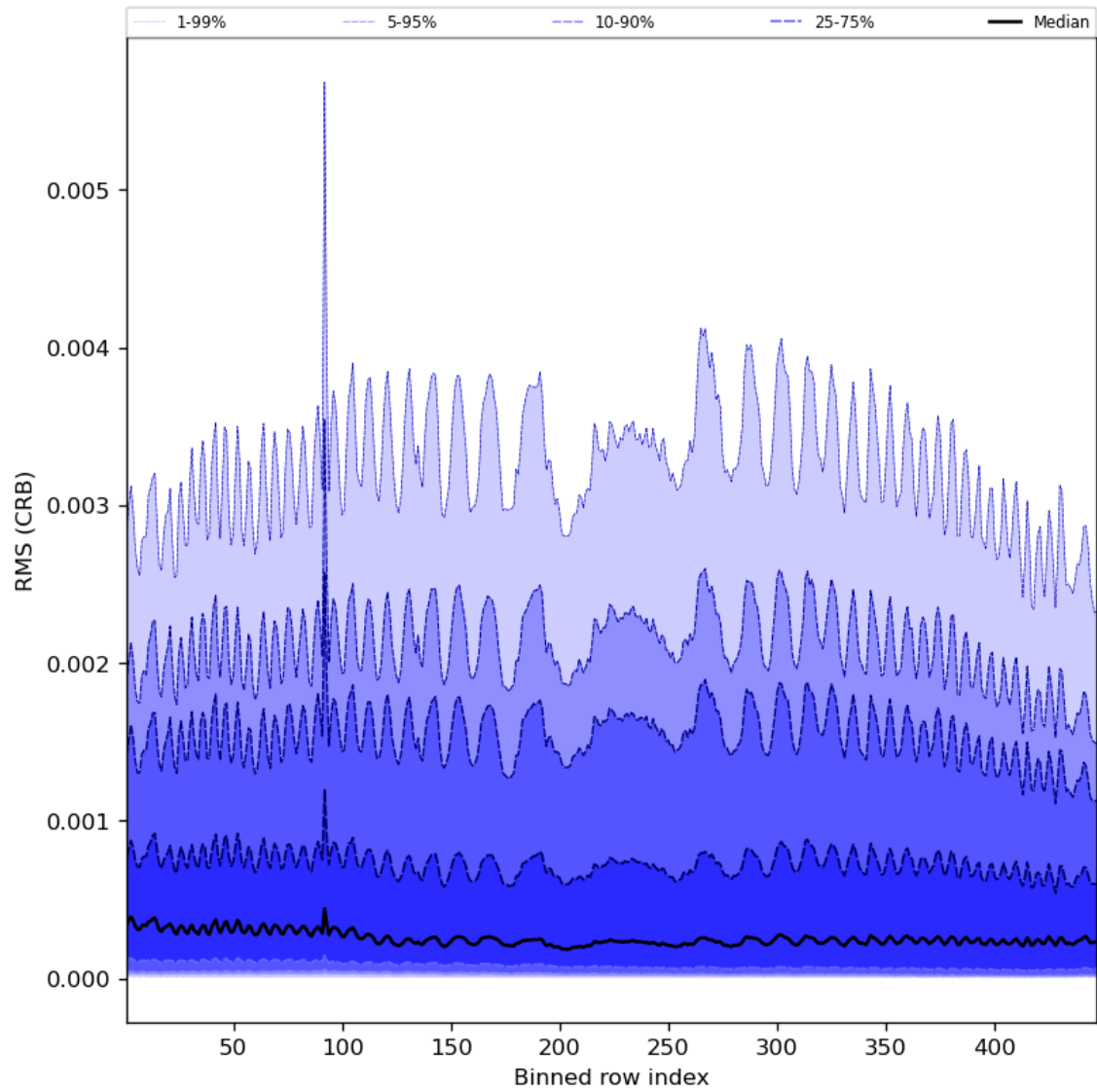
Figure 64: Along track statistics of “RMS (CRB)” for 2024-08-18 to 2024-08-20
