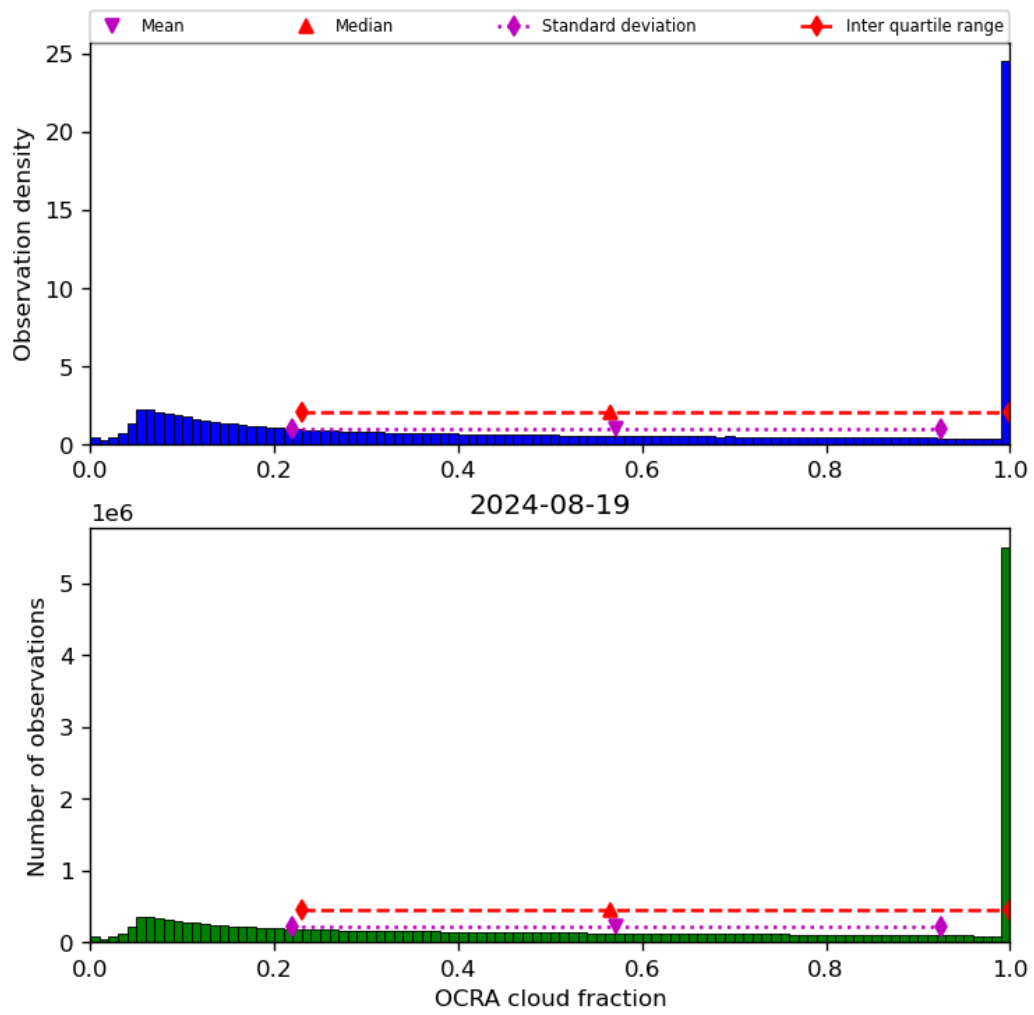
Figure 50: Histogram of “OCRA cloud fraction” for 2024-08-18 to 2024-08-20
