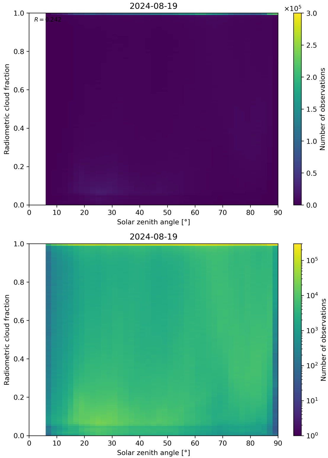
Figure 99: Scatter density plot of “Solar zenith angle” against “Radiometric cloud fraction” for 2024-08-18 to 2024-08-20.
