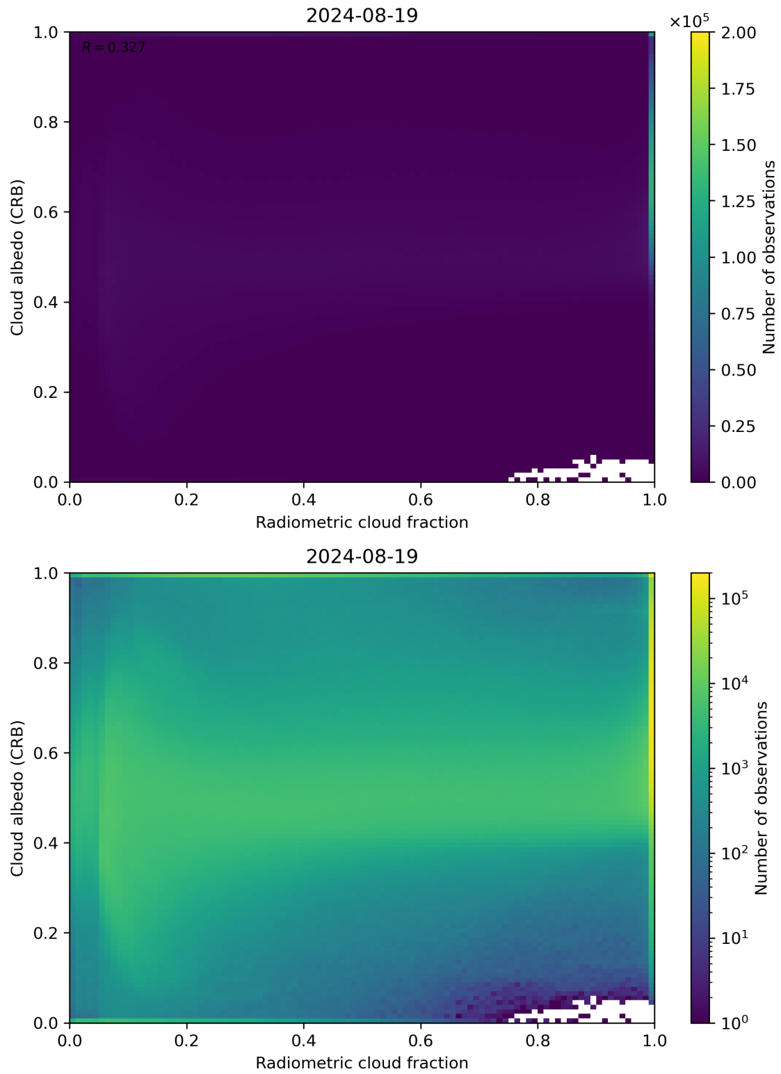
Figure 71: Scatter density plot of “Radiometric cloud fraction” against “Cloud albedo (CRB)” for 2024-08-18 to 2024-08-20.
