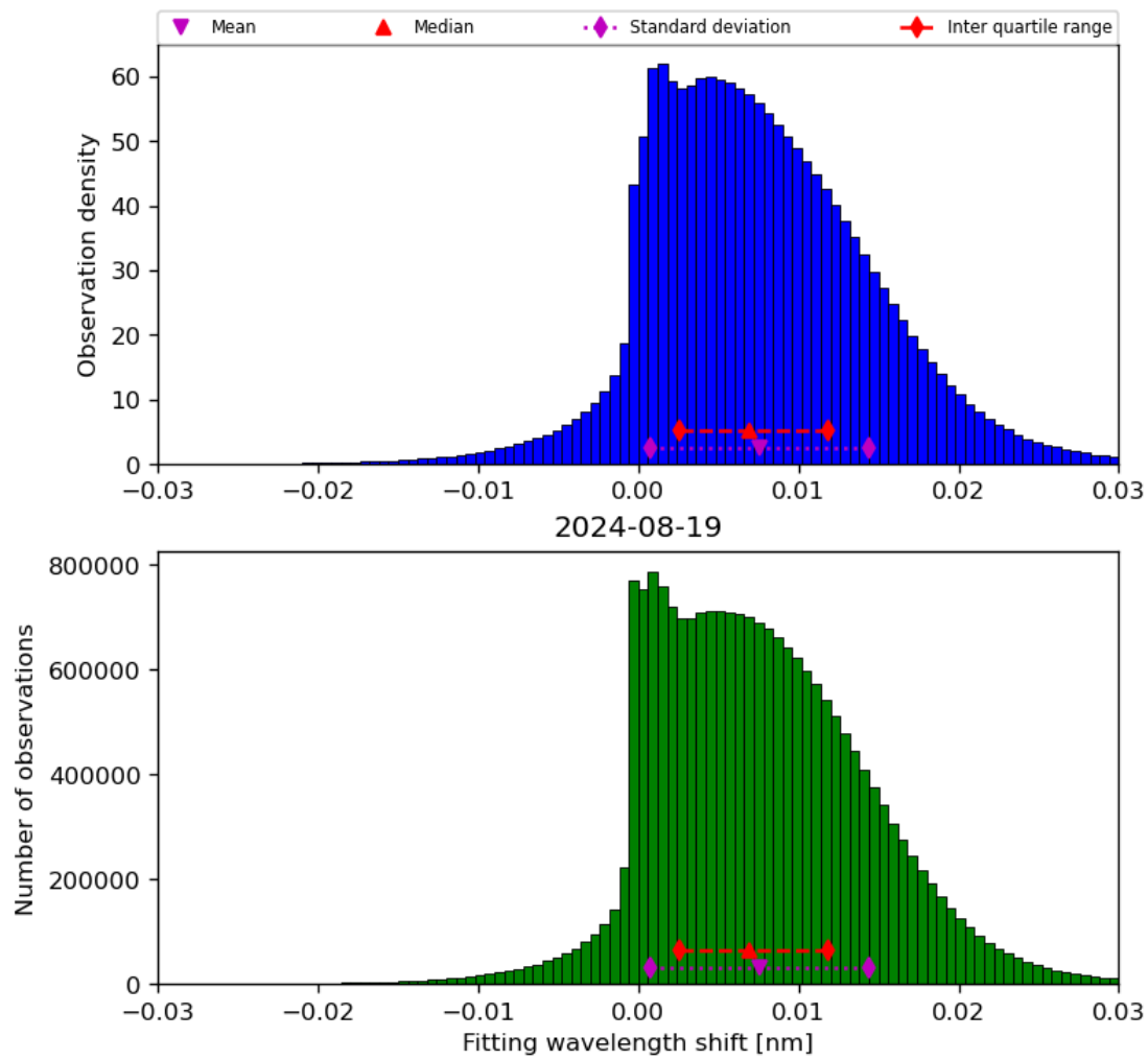
Figure 49: Histogram of “Fitting wavelength shift” for 2024-08-18 to 2024-08-20
