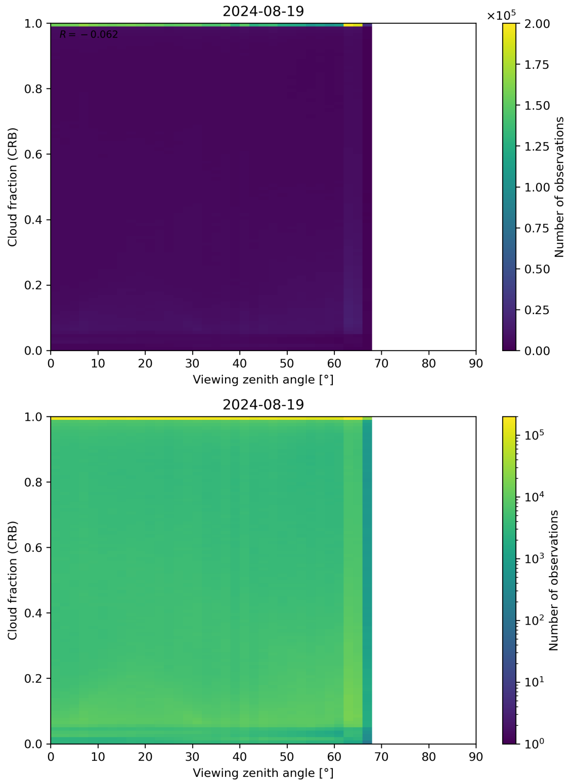
Figure 109: Scatter density plot of “Viewing zenith angle” against “Cloud fraction (CRB)” for 2024-08-18 to 2024-08-20.
