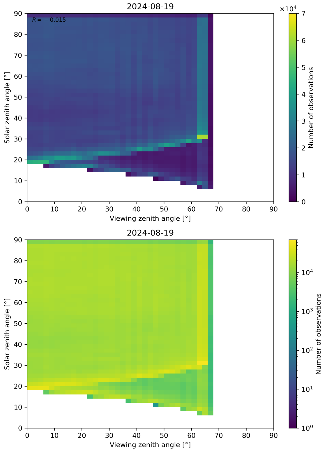
Figure 114: Scatter density plot of “Viewing zenith angle” against “Solar zenith angle” for 2024-08-18 to 2024-08-20.
