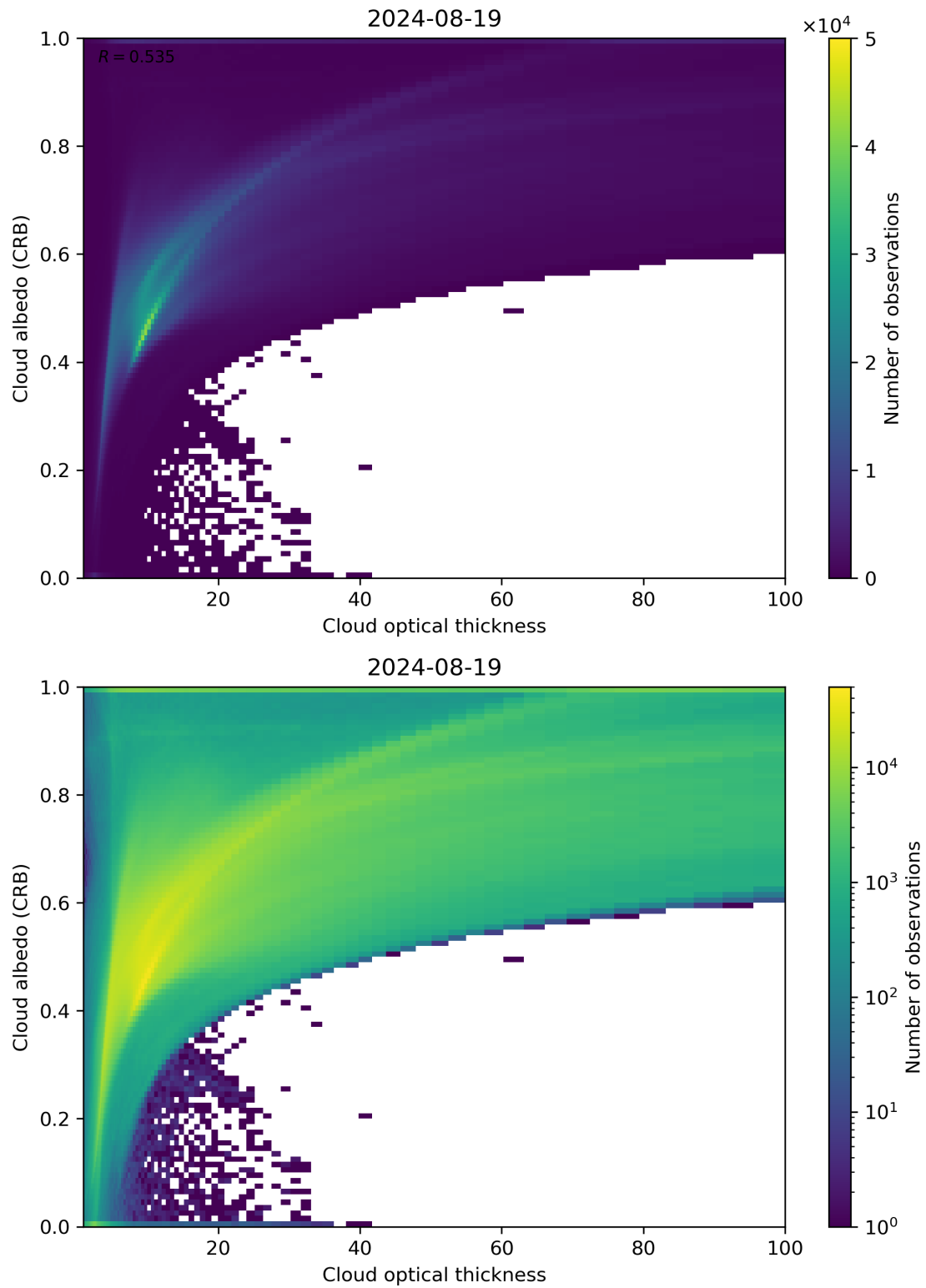
Figure 82: Scatter density plot of “Cloud optical thickness” against “Cloud albedo (CRB)” for 2024-08-18 to 2024-08-20.
