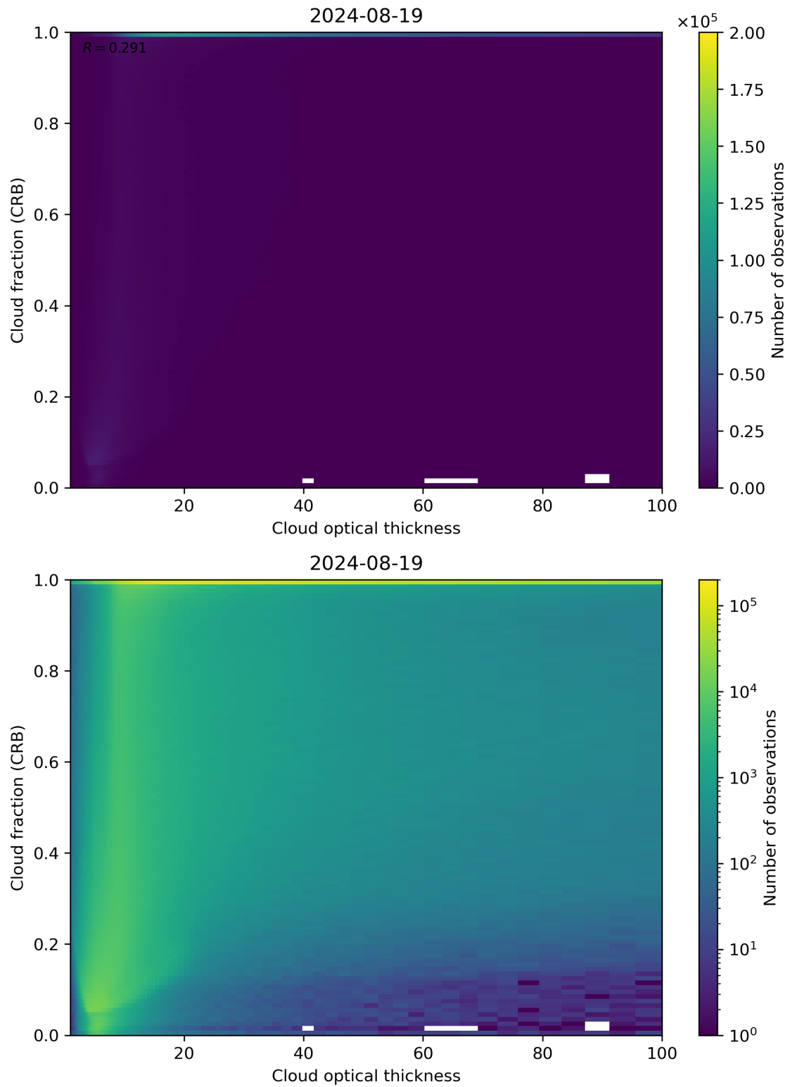
Figure 84: Scatter density plot of “Cloud optical thickness” against “Cloud fraction (CRB)” for 2024-08-18 to 2024-08-20.
