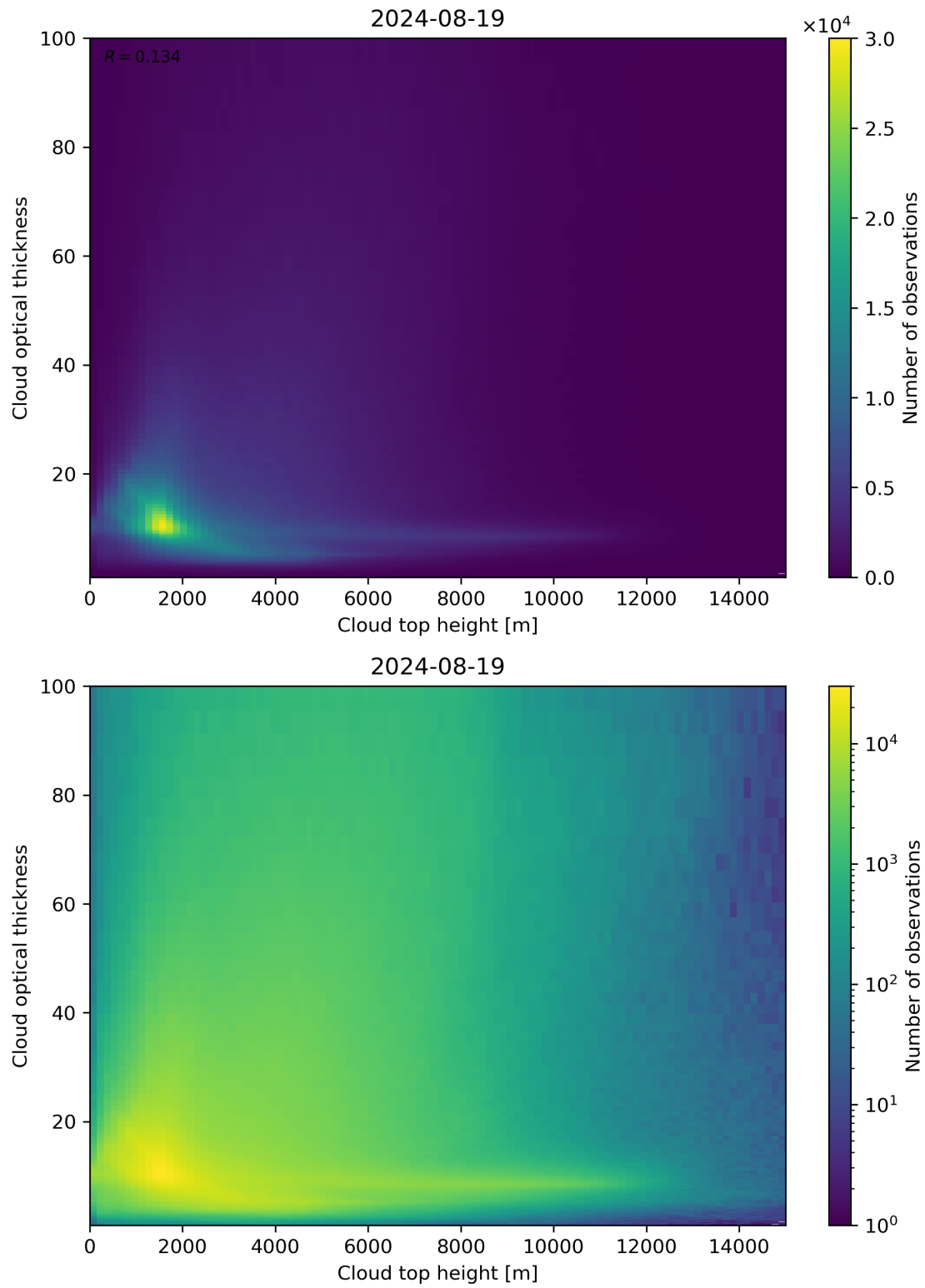
Figure 90: Scatter density plot of “Cloud top height” against “Cloud optical thickness” for 2024-08-18 to 2024-08-20.
