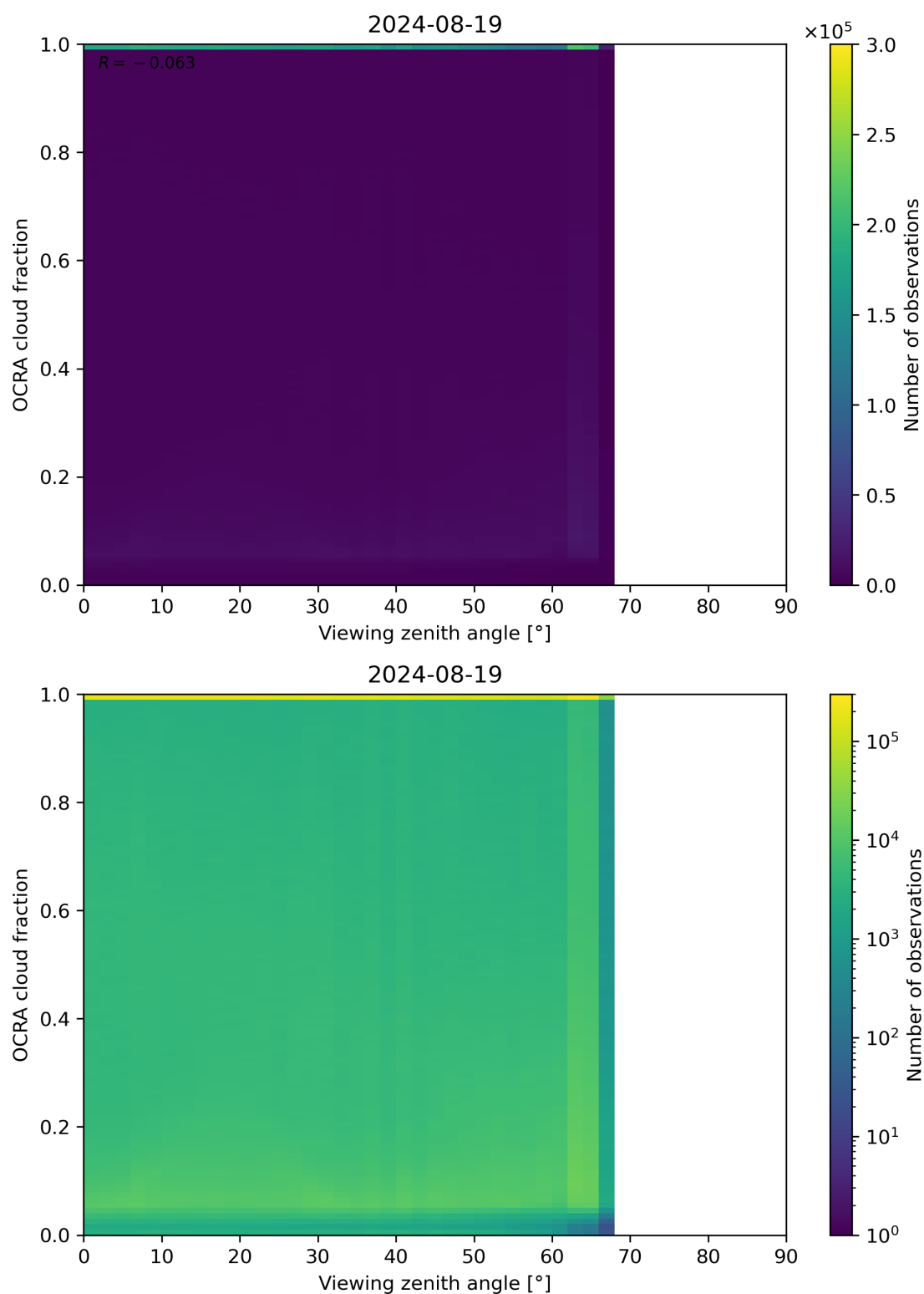
Figure 108: Scatter density plot of “Viewing zenith angle” against “OCRA cloud fraction” for 2024-08-18 to 2024-08-20.
