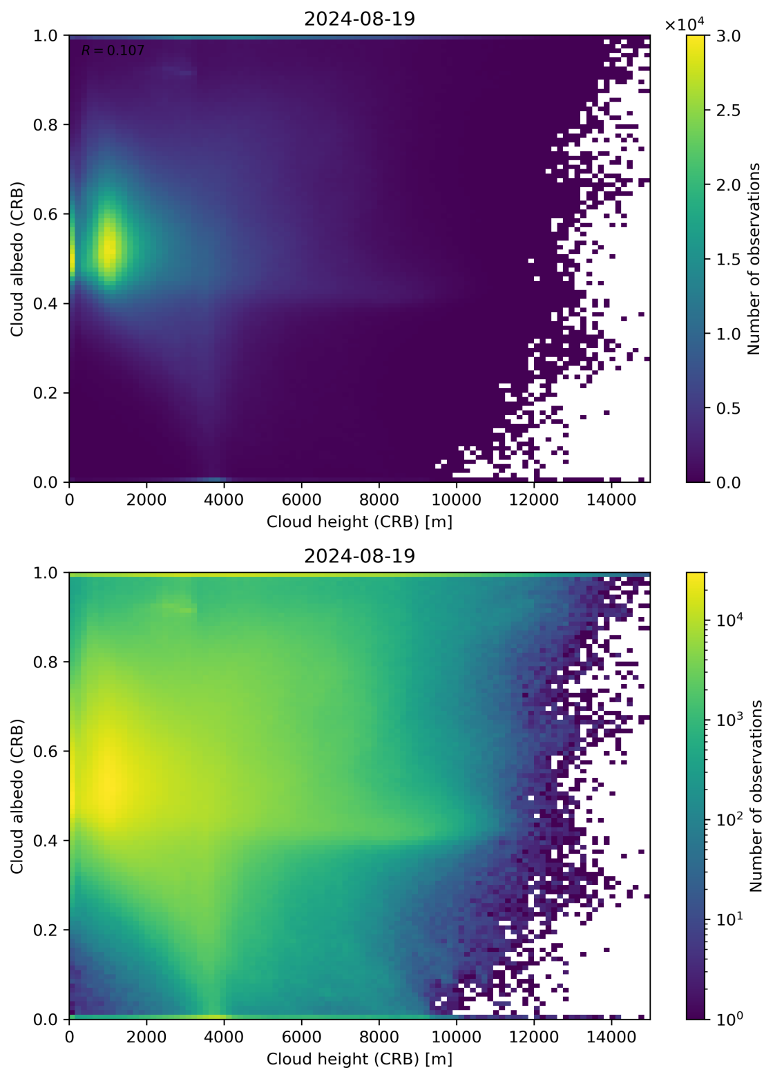
Figure 80: Scatter density plot of “Cloud height (CRB)” against “Cloud albedo (CRB)” for 2024-08-18 to 2024-08-20.
