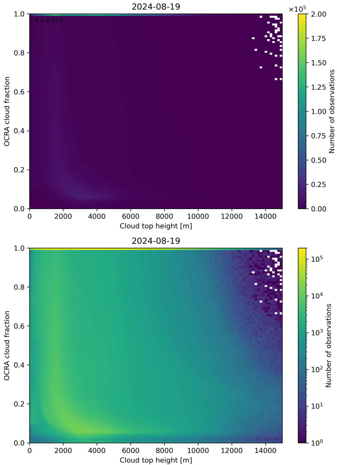
Figure 87: Scatter density plot of “Cloud top height” against “OCRA cloud fraction” for 2024-08-18 to 2024-08-20.
