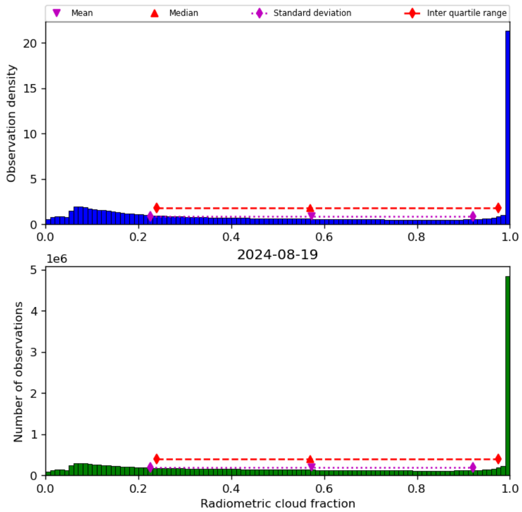
Figure 39: Histogram of “Radiometric cloud fraction” for 2024-08-18 to 2024-08-20
