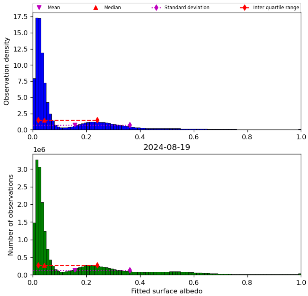
Figure 45: Histogram of “Fitted surface albedo” for 2024-08-18 to 2024-08-20
