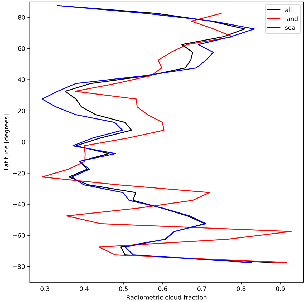
Figure 23: Zonal average of “Radiometric cloud fraction” for 2024-08-18 to 2024-08-20.
