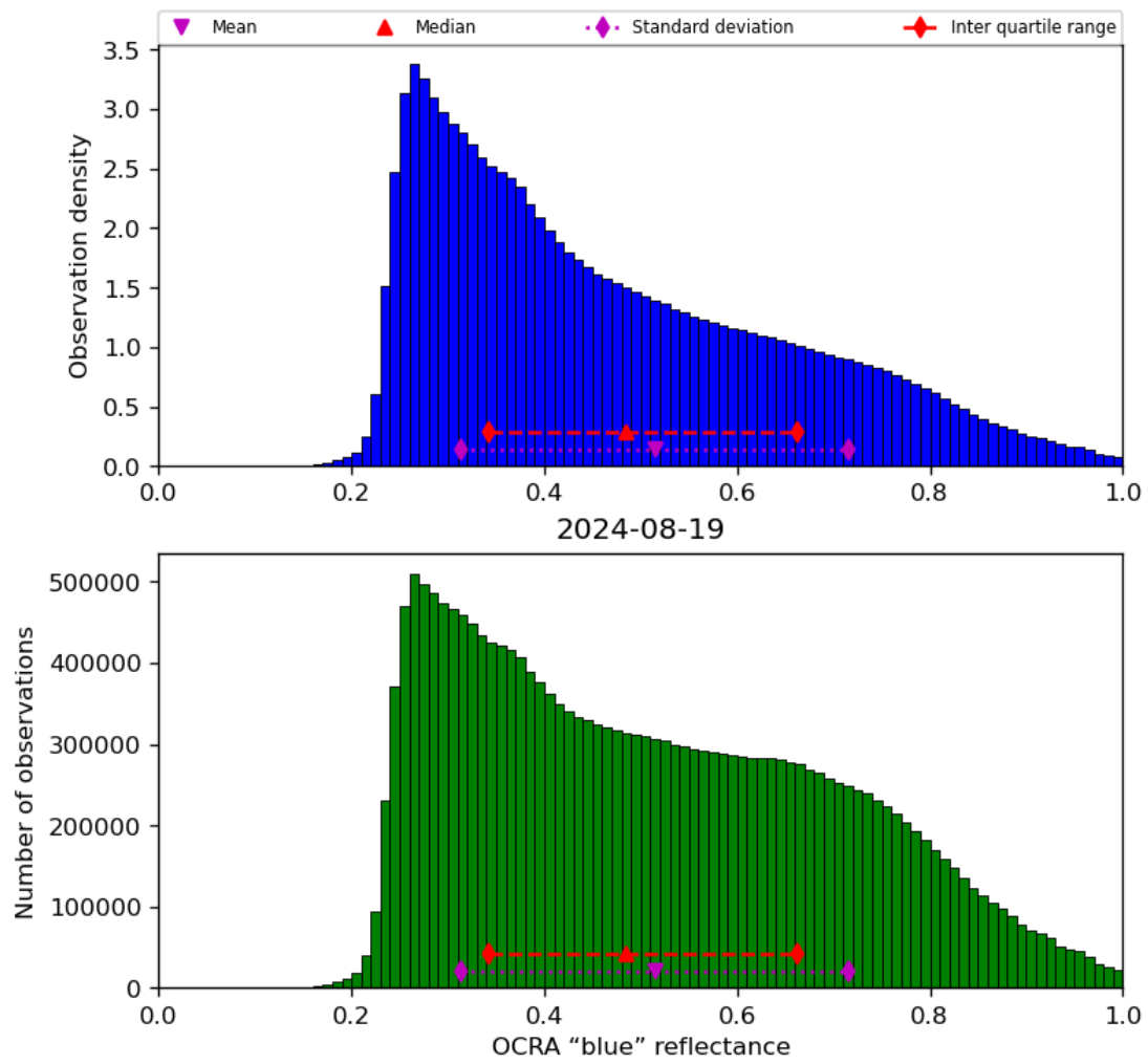
Figure 51: Histogram of “OCRA “blue” reflectance” for 2024-08-18 to 2024-08-20
