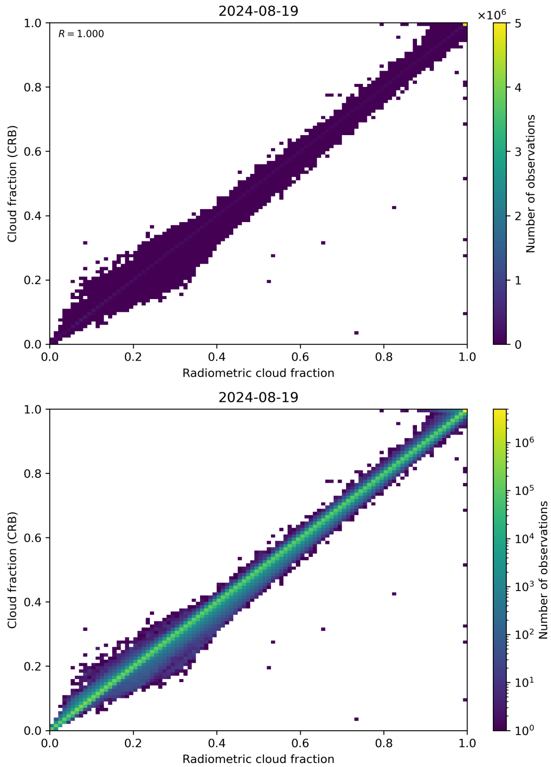
Figure 73: Scatter density plot of “Radiometric cloud fraction” against “Cloud fraction (CRB)” for 2024-08-18 to 2024-08-20.
