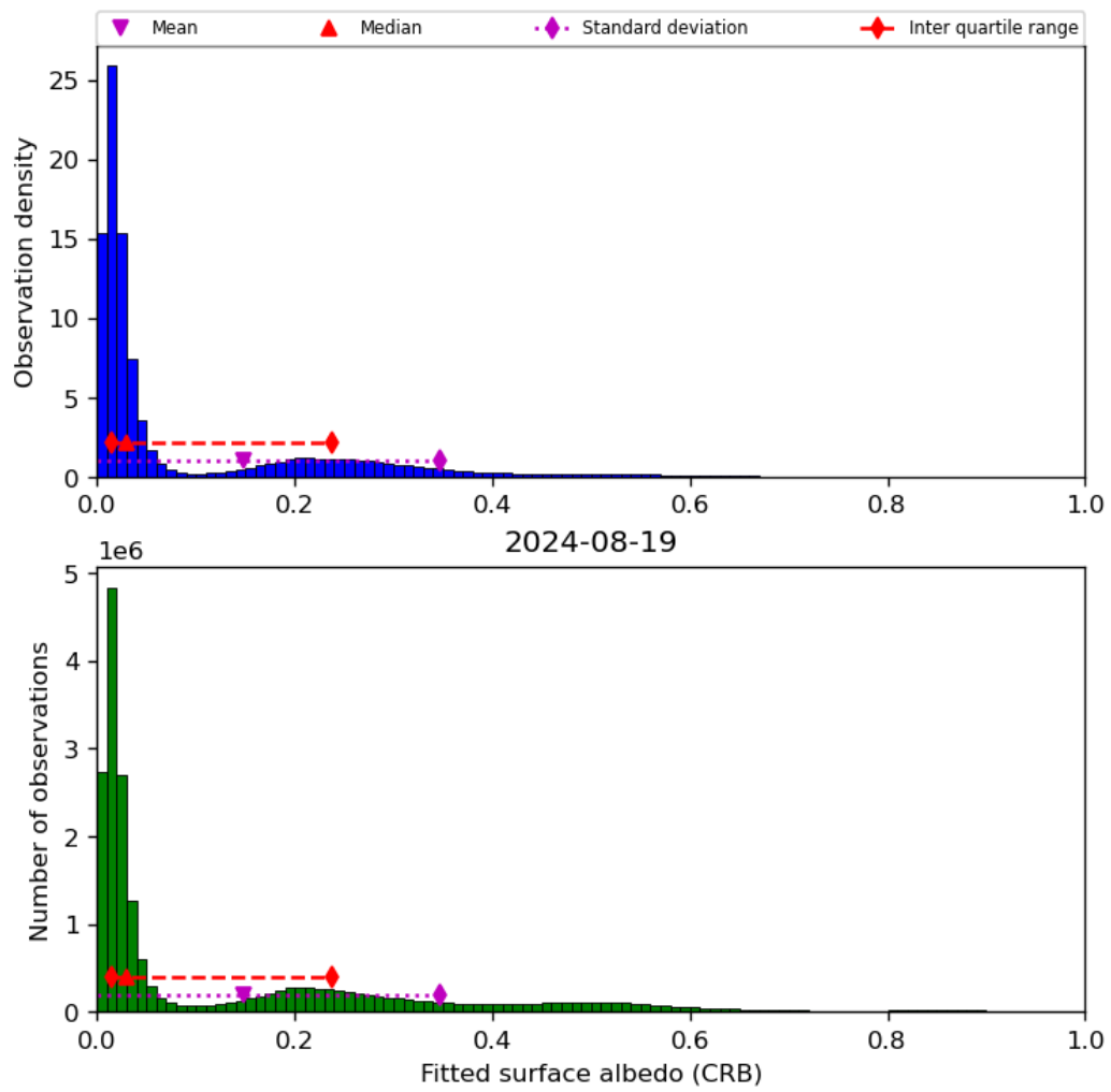
Figure 46: Histogram of “Fitted surface albedo (CRB)” for 2024-08-18 to 2024-08-20
