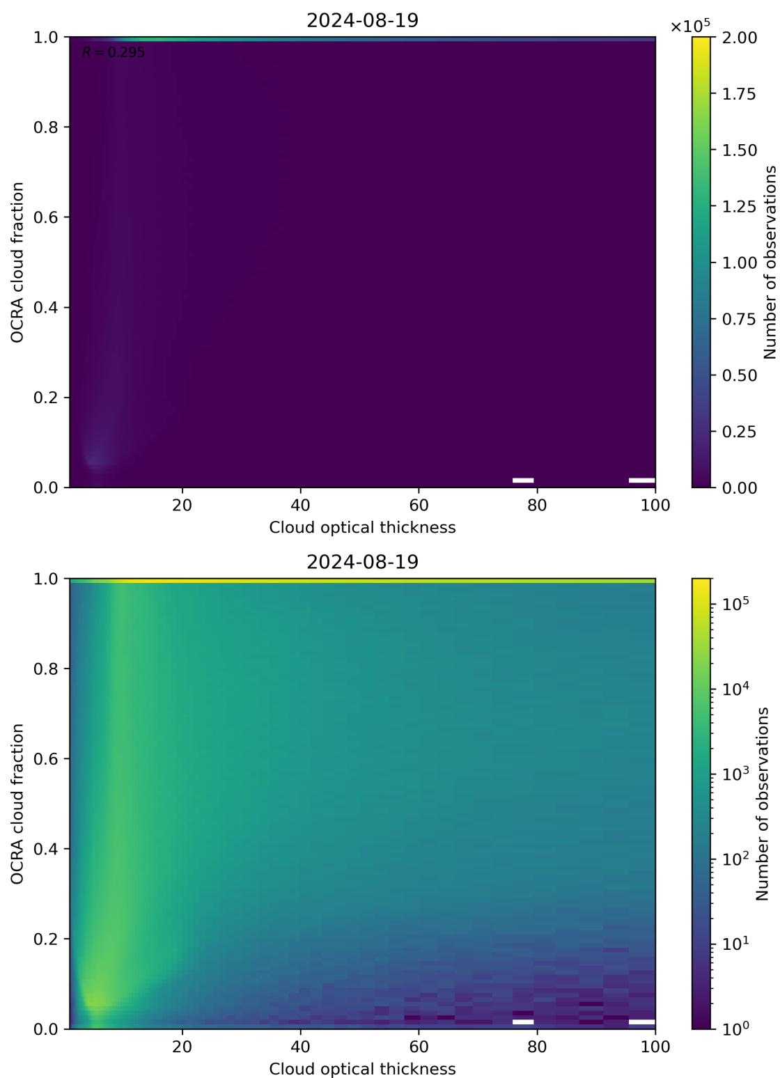
Figure 83: Scatter density plot of “Cloud optical thickness” against “OCRA cloud fraction” for 2024-08-18 to 2024-08-20.
