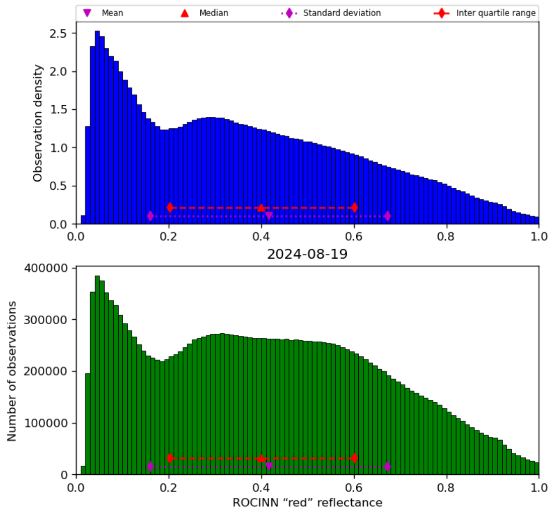
Figure 53: Histogram of “ROCINN “red” reflectance” for 2024-08-18 to 2024-08-20
