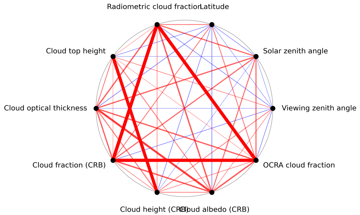
Figure 1: Map of correlation graph for 2024-08-18 to 2024-08-20.
