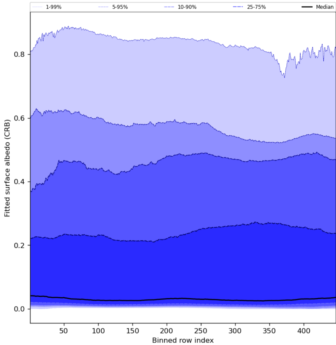
Figure 62: Along track statistics of “Fitted surface albedo (CRB)” for 2024-08-18 to 2024-08-20
