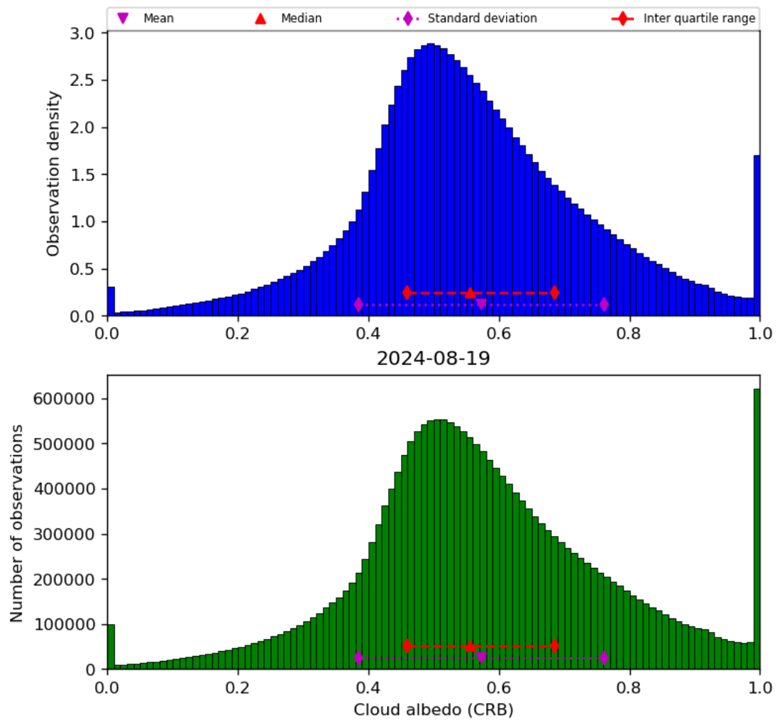
Figure 44: Histogram of “Cloud albedo (CRB)” for 2024-08-18 to 2024-08-20
