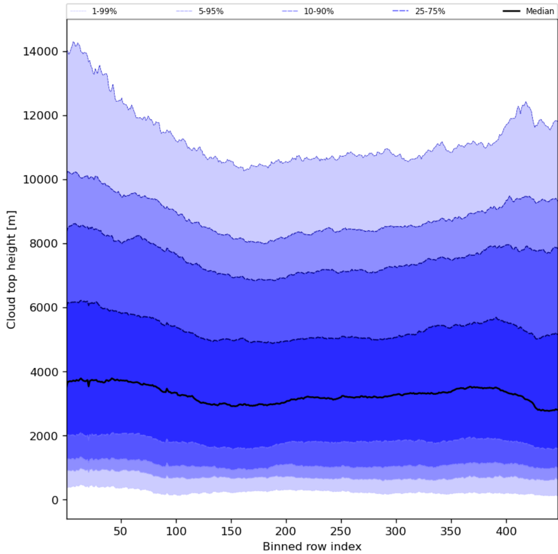
Figure 56: Along track statistics of “Cloud top height” for 2024-08-18 to 2024-08-20
