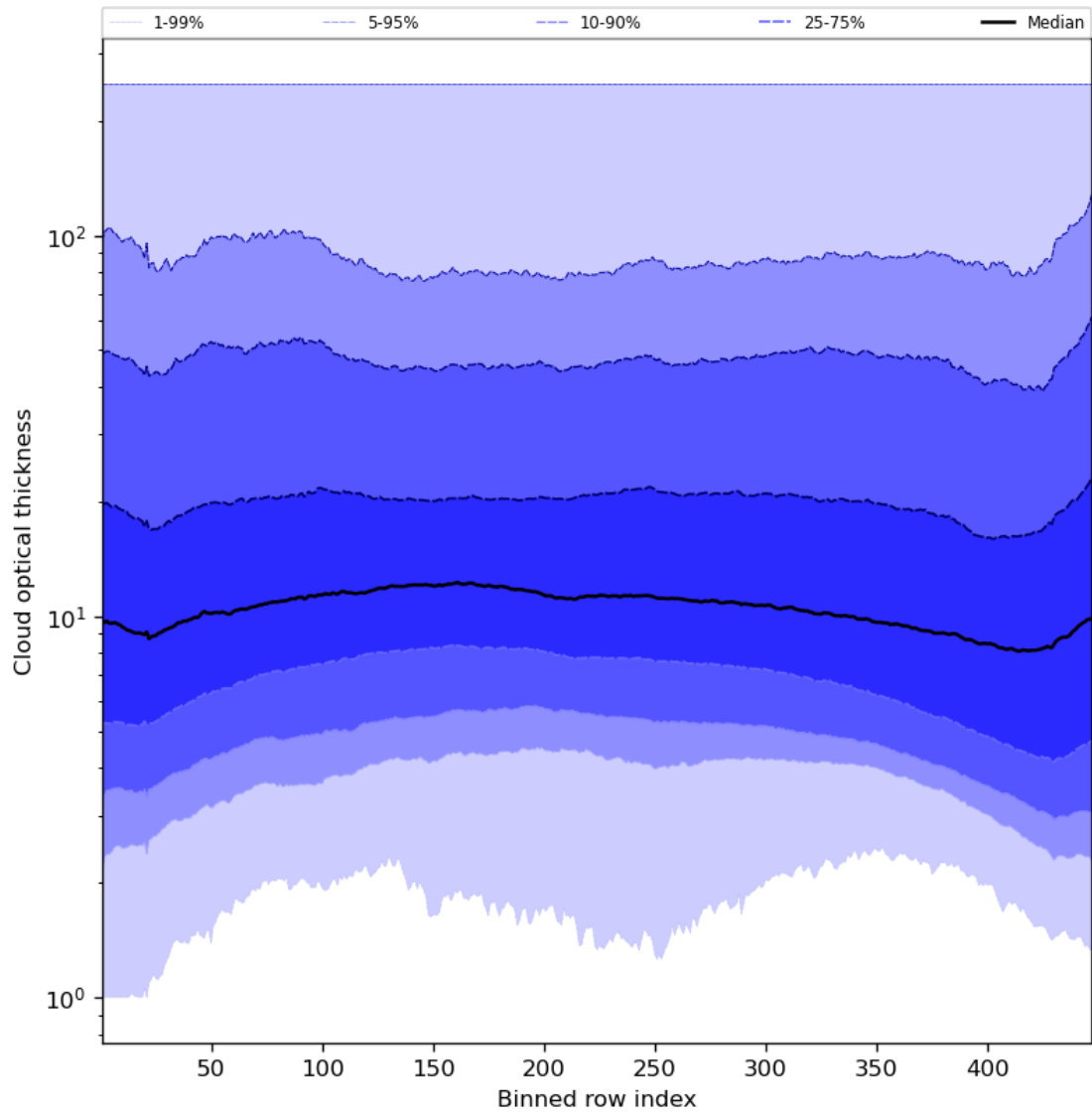
Figure 57: Along track statistics of “Cloud optical thickness” for 2024-08-18 to 2024-08-20
