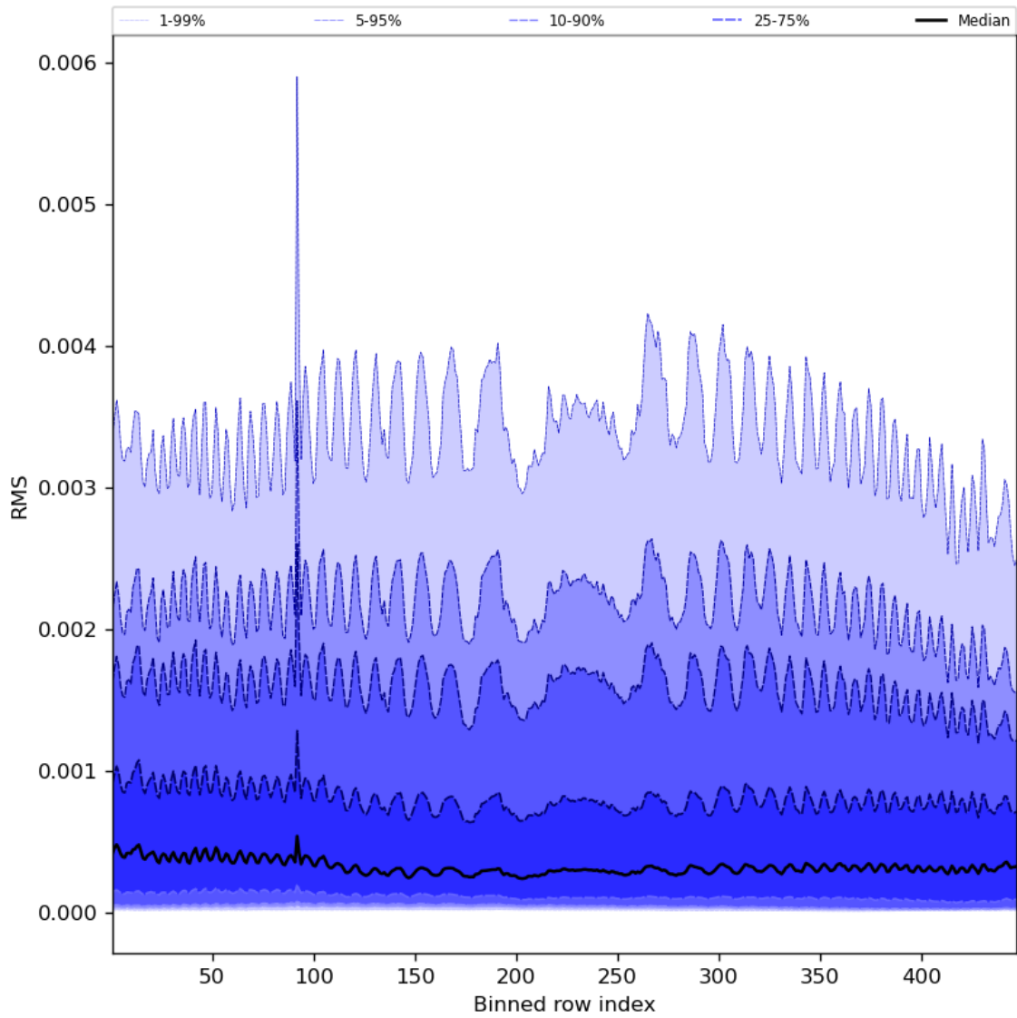
Figure 63: Along track statistics of “RMS” for 2024-08-18 to 2024-08-20
