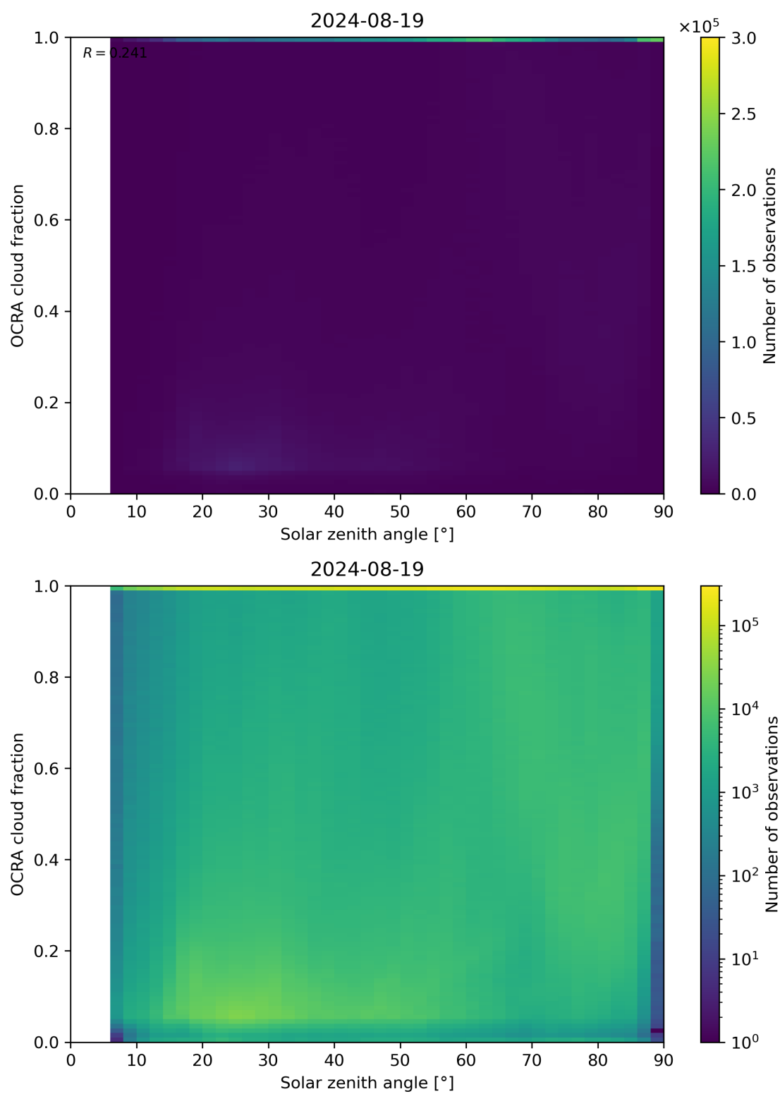
Figure 100: Scatter density plot of “Solar zenith angle” against “OCRA cloud fraction” for 2024-08-18 to 2024-08-20.
