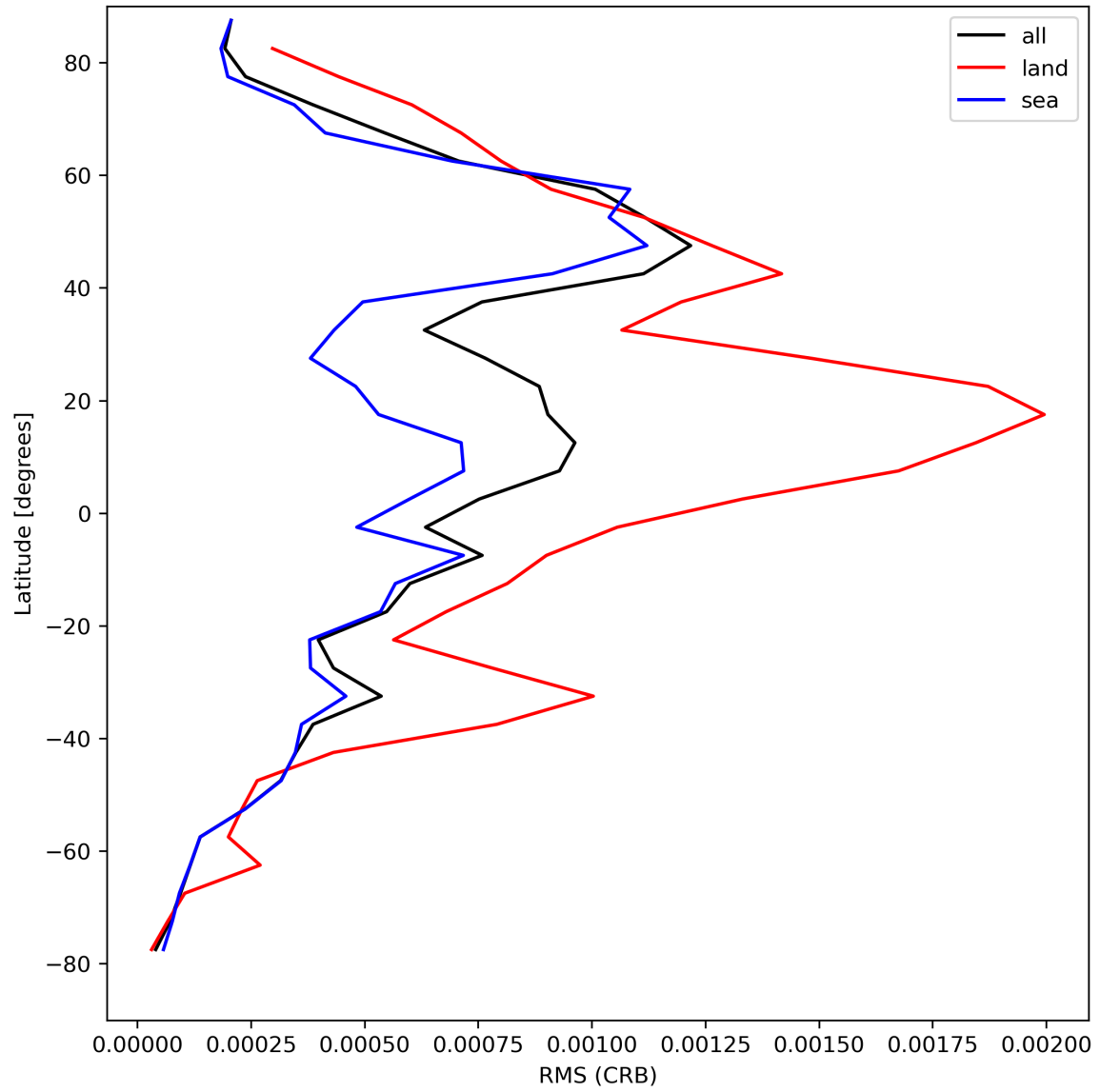
Figure 32: Zonal average of “RMS (CRB)” for 2024-08-18 to 2024-08-20.
