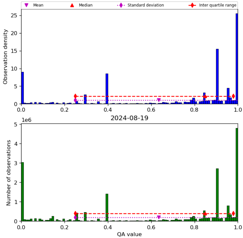
Figure 38: Histogram of “QA value” for 2024-08-18 to 2024-08-20
