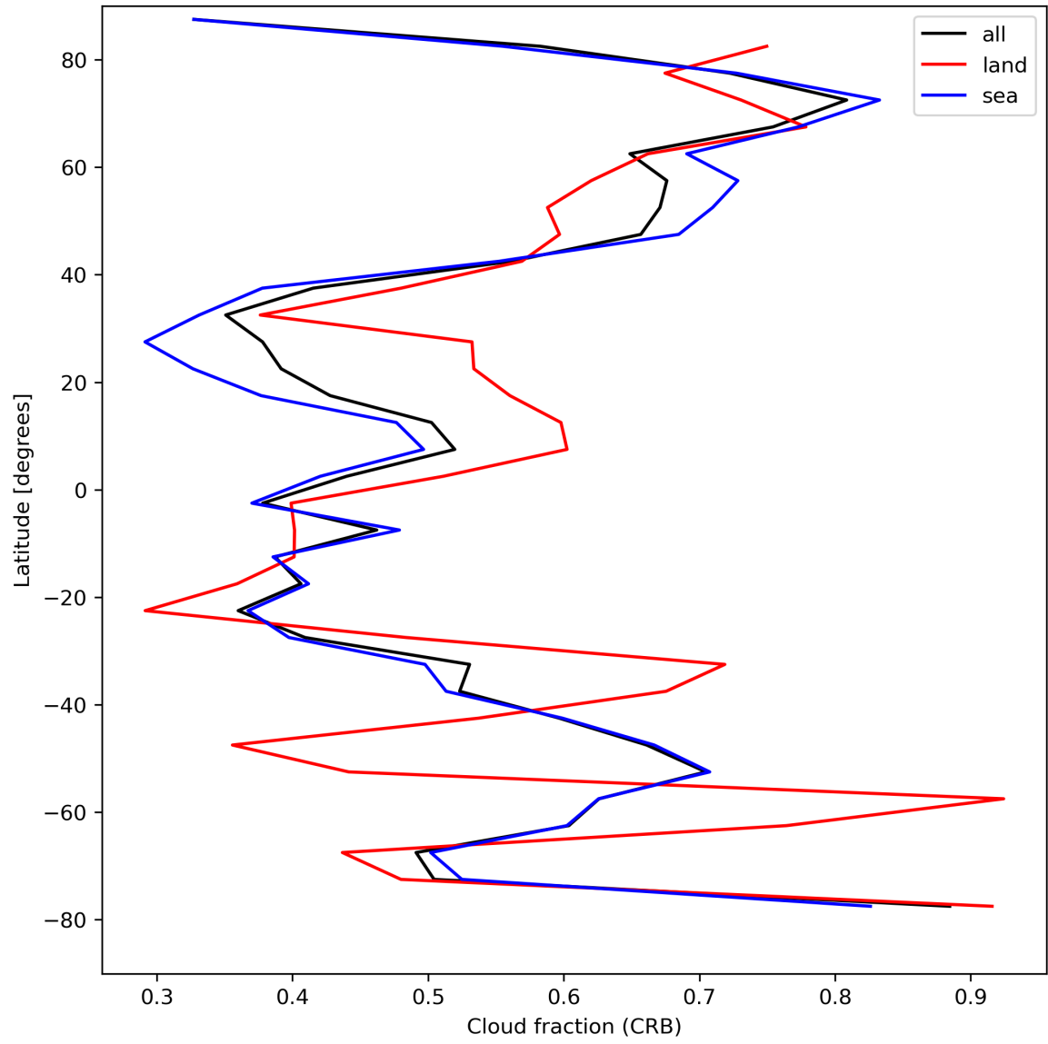
Figure 26: Zonal average of “Cloud fraction (CRB)” for 2024-08-18 to 2024-08-20.
