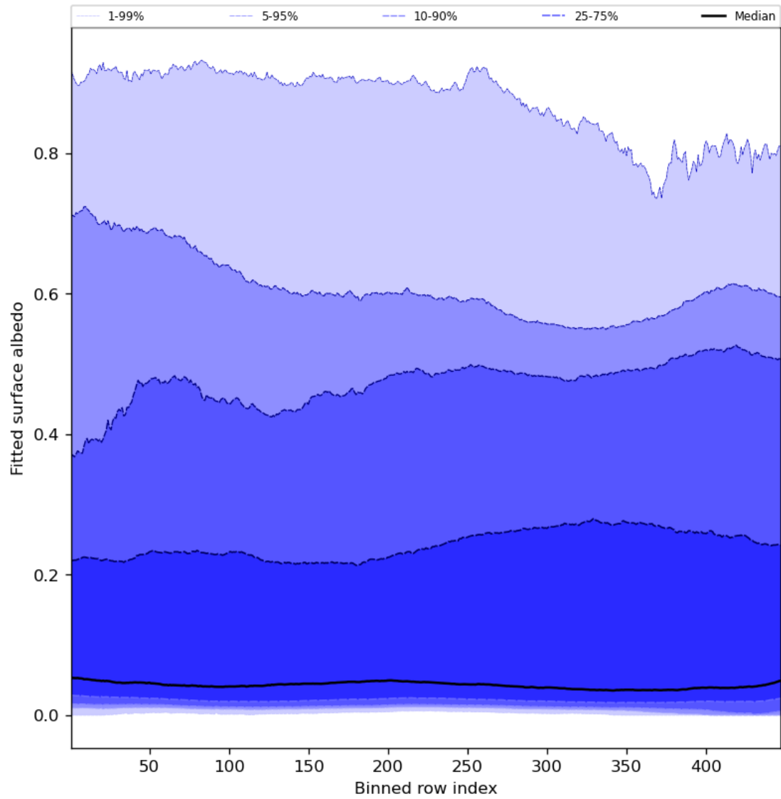
Figure 61: Along track statistics of “Fitted surface albedo” for 2024-08-18 to 2024-08-20
