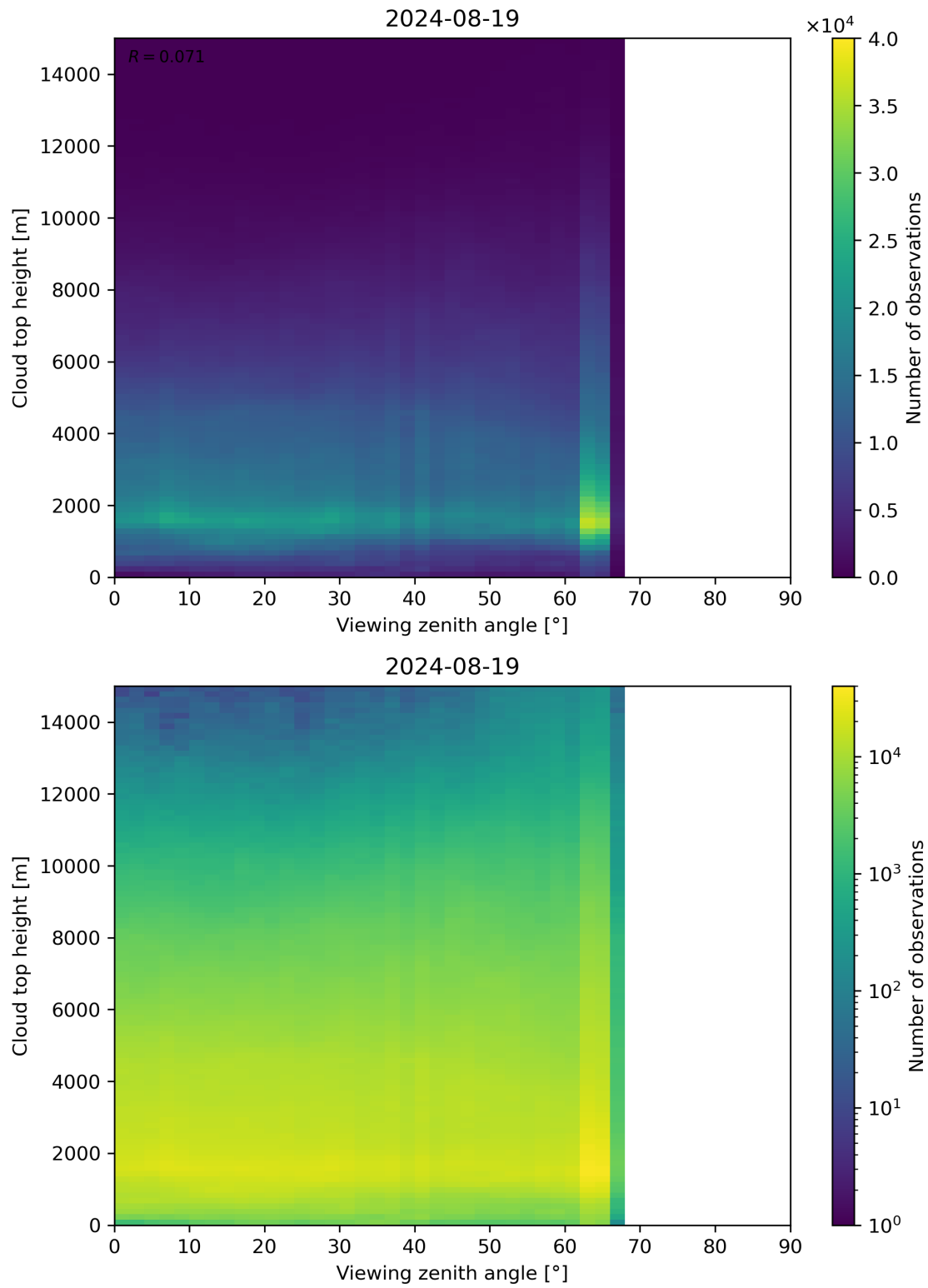
Figure 112: Scatter density plot of “Viewing zenith angle” against “Cloud top height” for 2024-08-18 to 2024-08-20.
