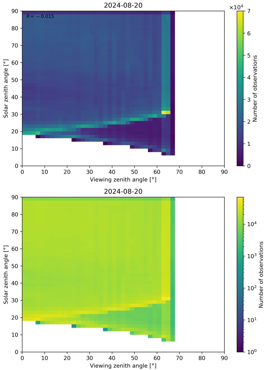
Figure 114: Scatter density plot of “Viewing zenith angle” against “Solar zenith angle” for 2024-08-19 to 2024-08-21.
