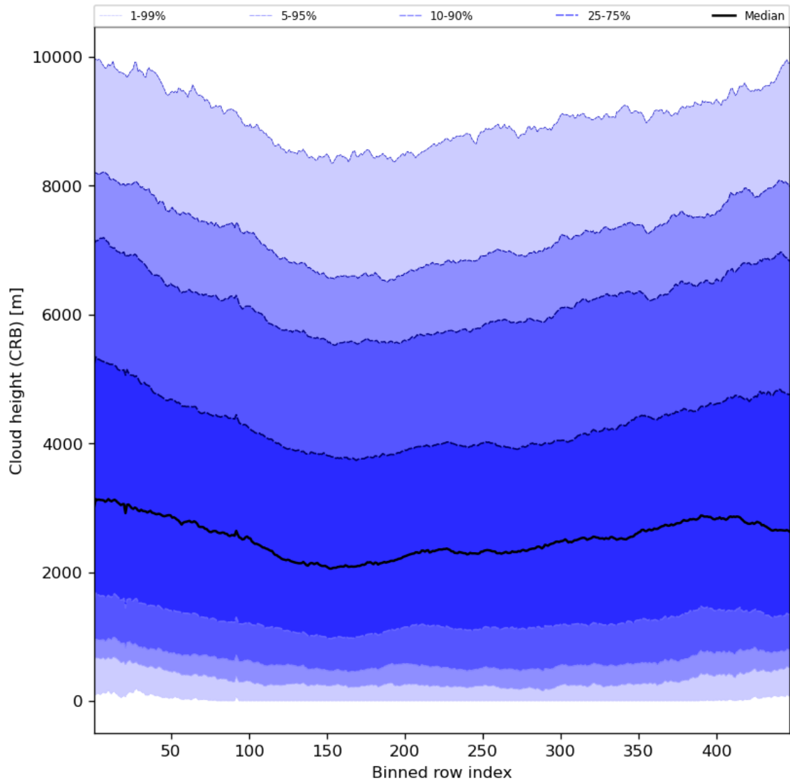
Figure 59: Along track statistics of “Cloud height (CRB)” for 2024-08-19 to 2024-08-21
