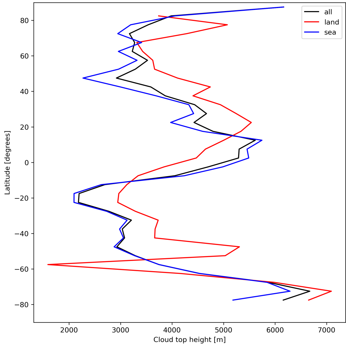
Figure 24: Zonal average of “Cloud top height” for 2024-08-19 to 2024-08-21.
