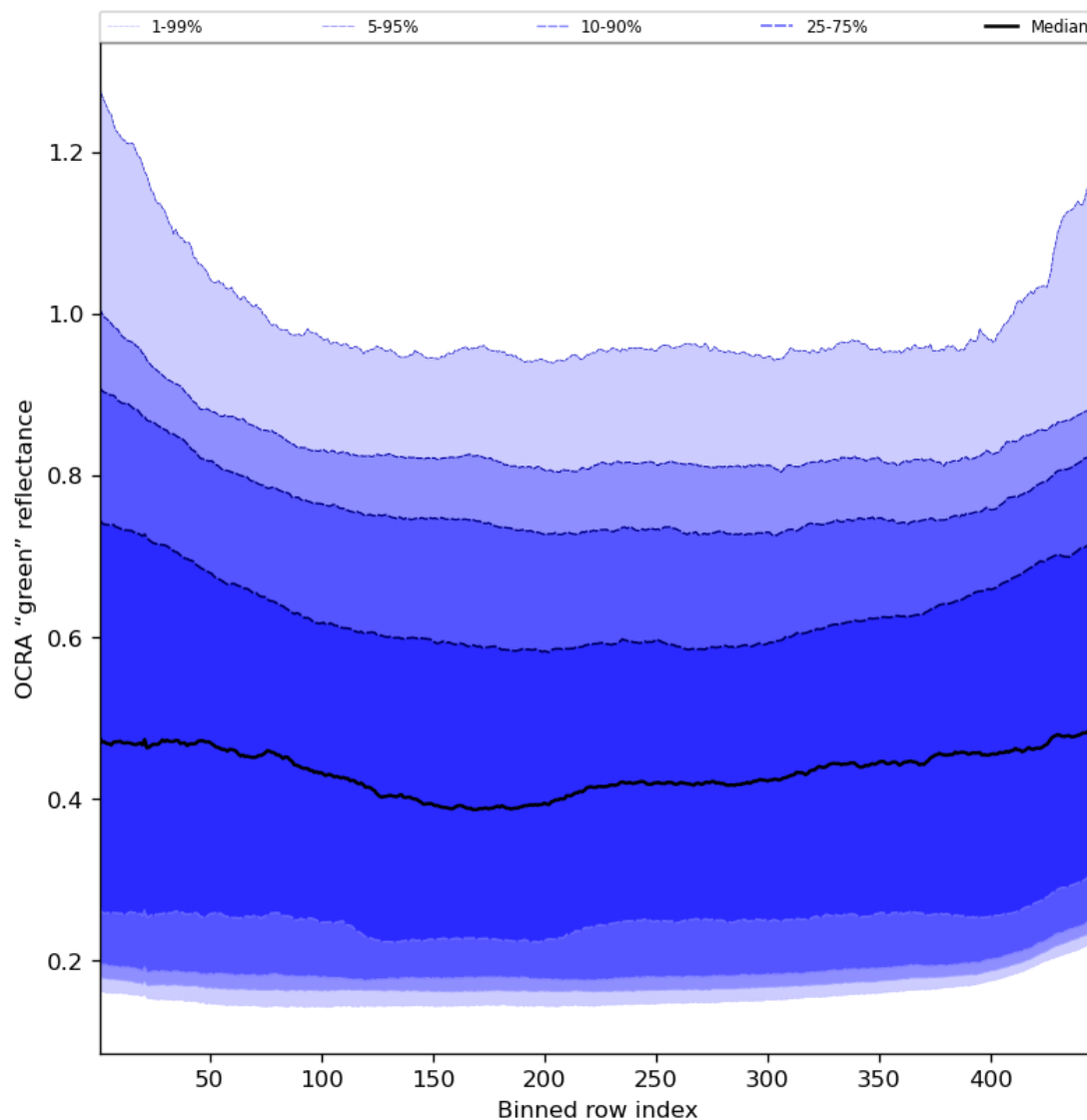
Figure 68: Along track statistics of “OCRA “green” reflectance” for 2024-08-19 to 2024-08-21
