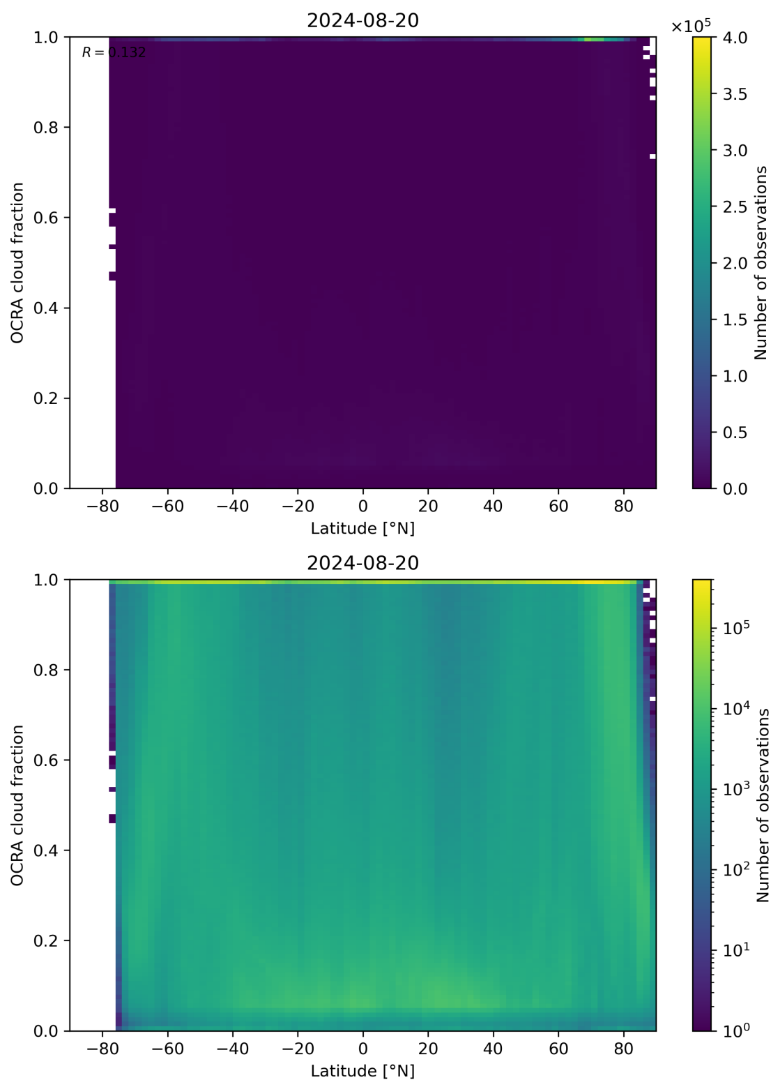
Figure 93: Scatter density plot of “Latitude” against “OCRA cloud fraction” for 2024-08-19 to 2024-08-21.
