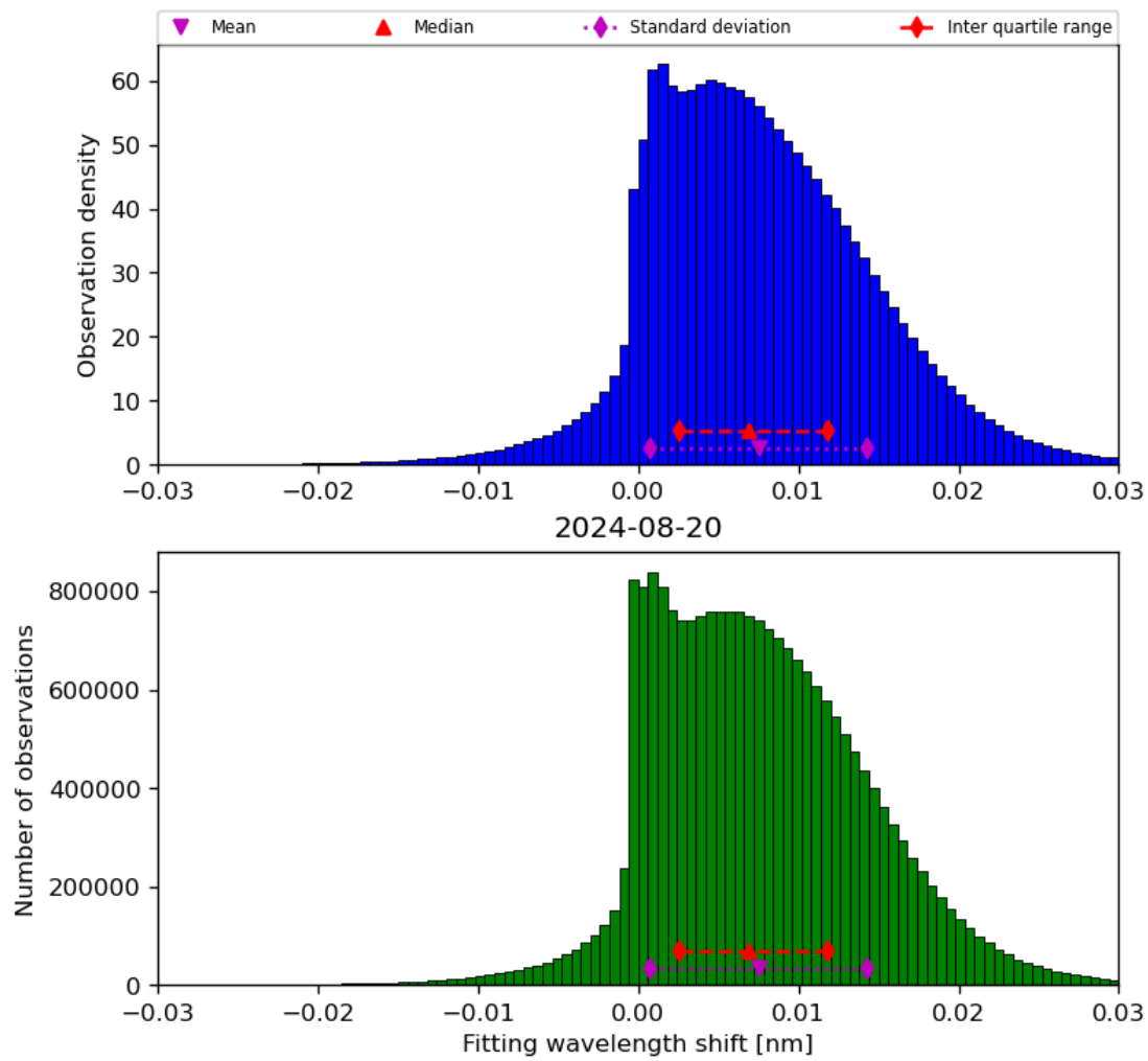
Figure 49: Histogram of “Fitting wavelength shift” for 2024-08-19 to 2024-08-21
