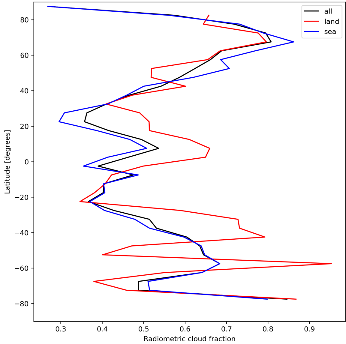
Figure 23: Zonal average of “Radiometric cloud fraction” for 2024-08-19 to 2024-08-21.
