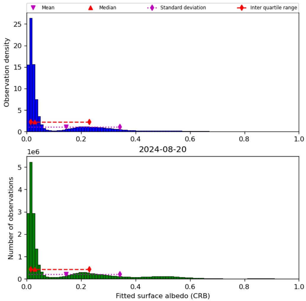
Figure 46: Histogram of “Fitted surface albedo (CRB)” for 2024-08-19 to 2024-08-21
