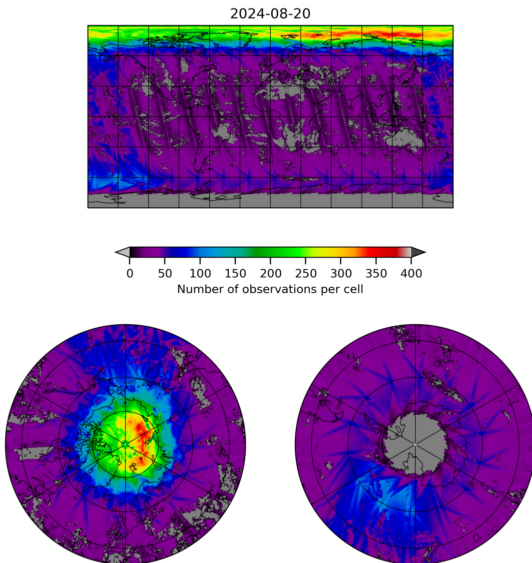
Figure 21: Map of the number of observations for 2024-08-19 to 2024-08-21
