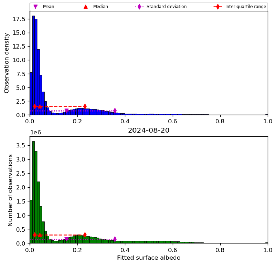
Figure 45: Histogram of “Fitted surface albedo” for 2024-08-19 to 2024-08-21
