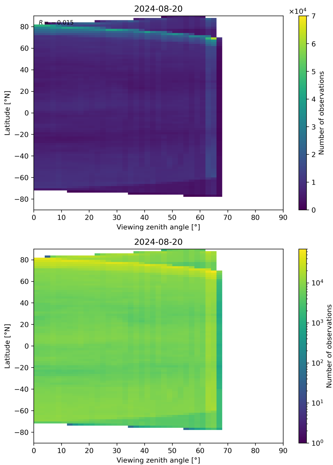
Figure 113: Scatter density plot of “Viewing zenith angle” against “Latitude” for 2024-08-19 to 2024-08-21.
