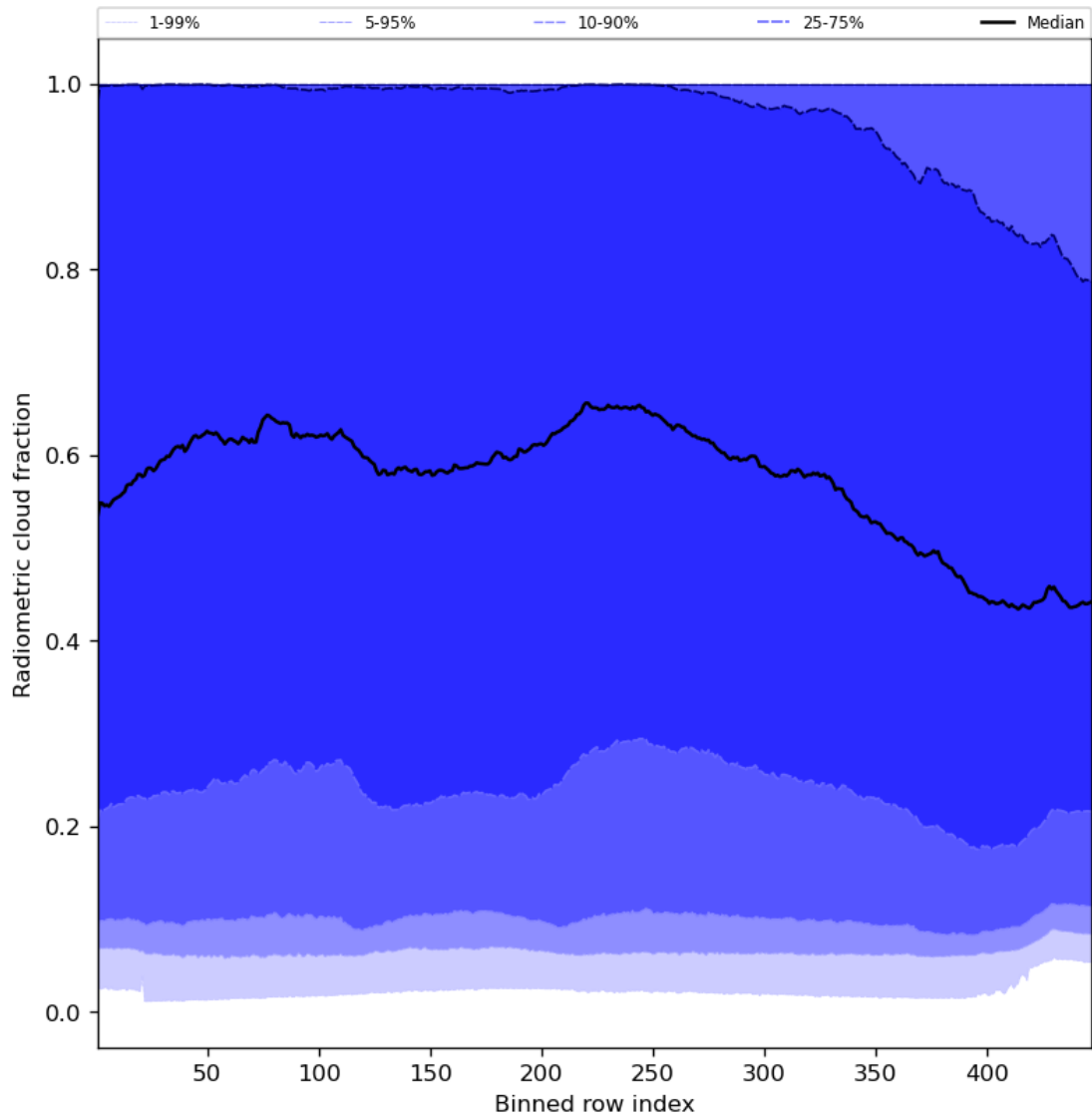
Figure 55: Along track statistics of “Radiometric cloud fraction” for 2024-08-19 to 2024-08-21
