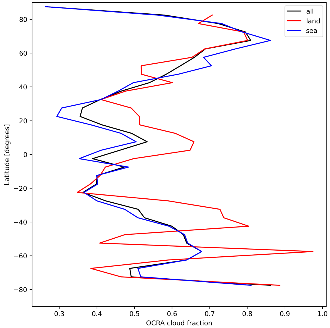
Figure 34: Zonal average of “OCRA cloud fraction” for 2024-08-19 to 2024-08-21.
