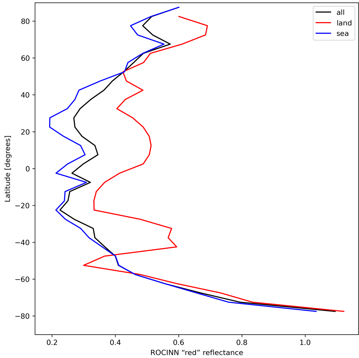
Figure 37: Zonal average of “ROCINN “red” reflectance” for 2024-08-19 to 2024-08-21.
