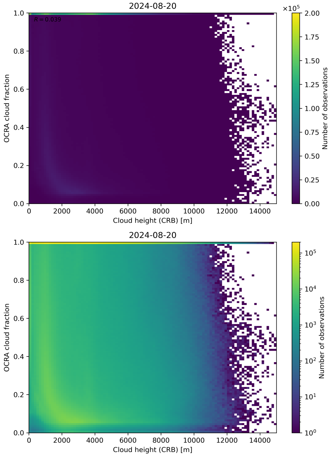
Figure 81: Scatter density plot of “Cloud height (CRB)” against “OCRA cloud fraction” for 2024-08-19 to 2024-08-21.
