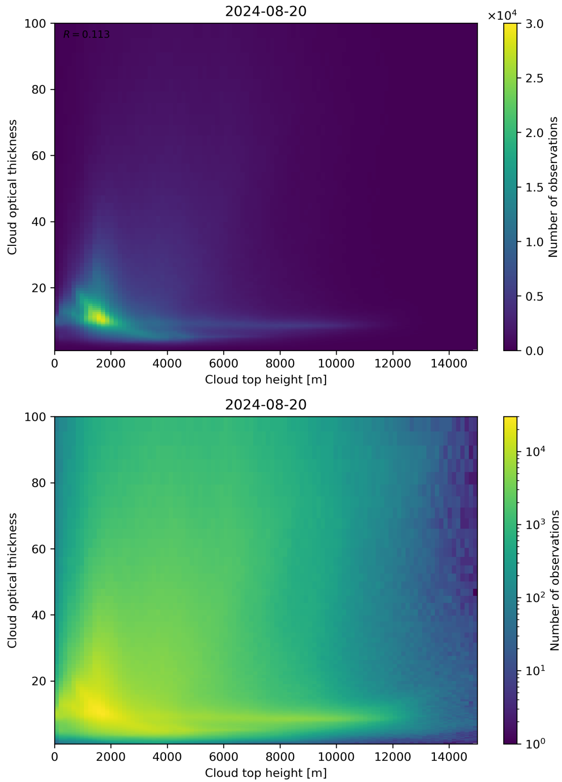
Figure 90: Scatter density plot of “Cloud top height” against “Cloud optical thickness” for 2024-08-19 to 2024-08-21.
