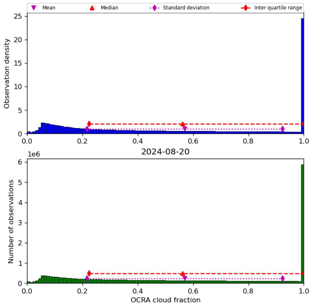
Figure 50: Histogram of “OCRA cloud fraction” for 2024-08-19 to 2024-08-21
