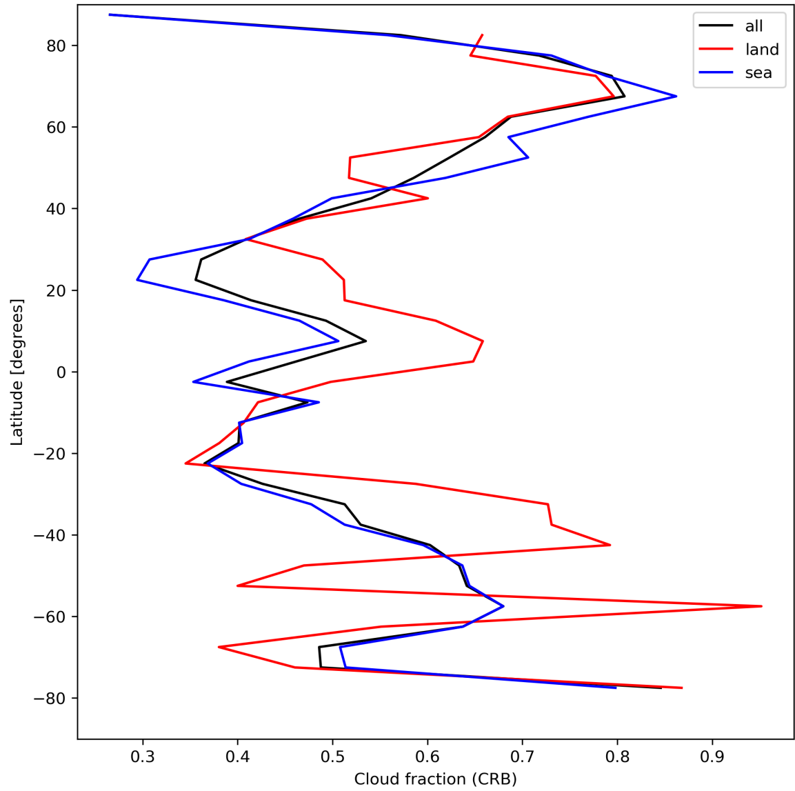
Figure 26: Zonal average of “Cloud fraction (CRB)” for 2024-08-19 to 2024-08-21.
