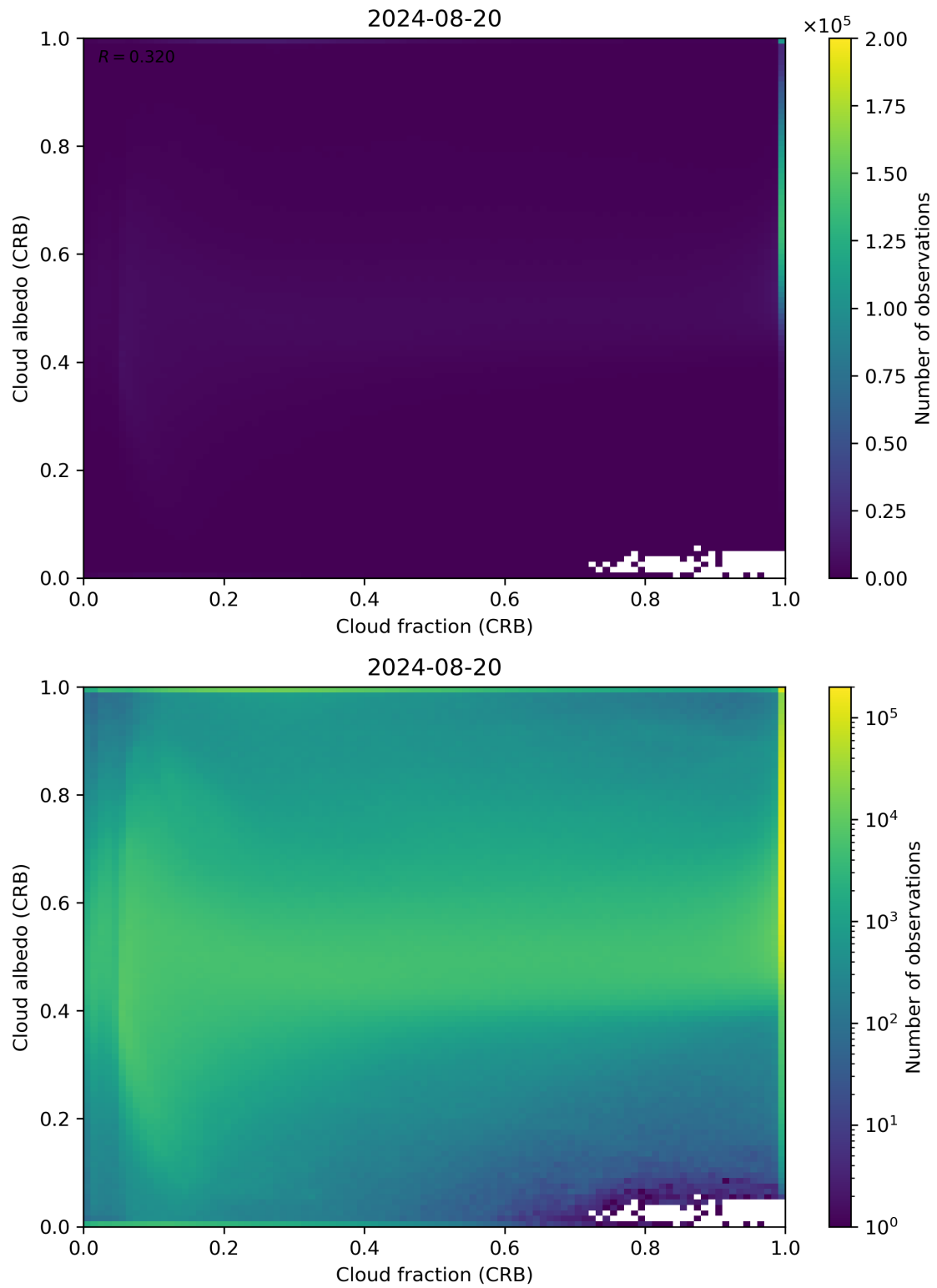
Figure 77: Scatter density plot of “Cloud fraction (CRB)” against “Cloud albedo (CRB)” for 2024-08-19 to 2024-08-21.
