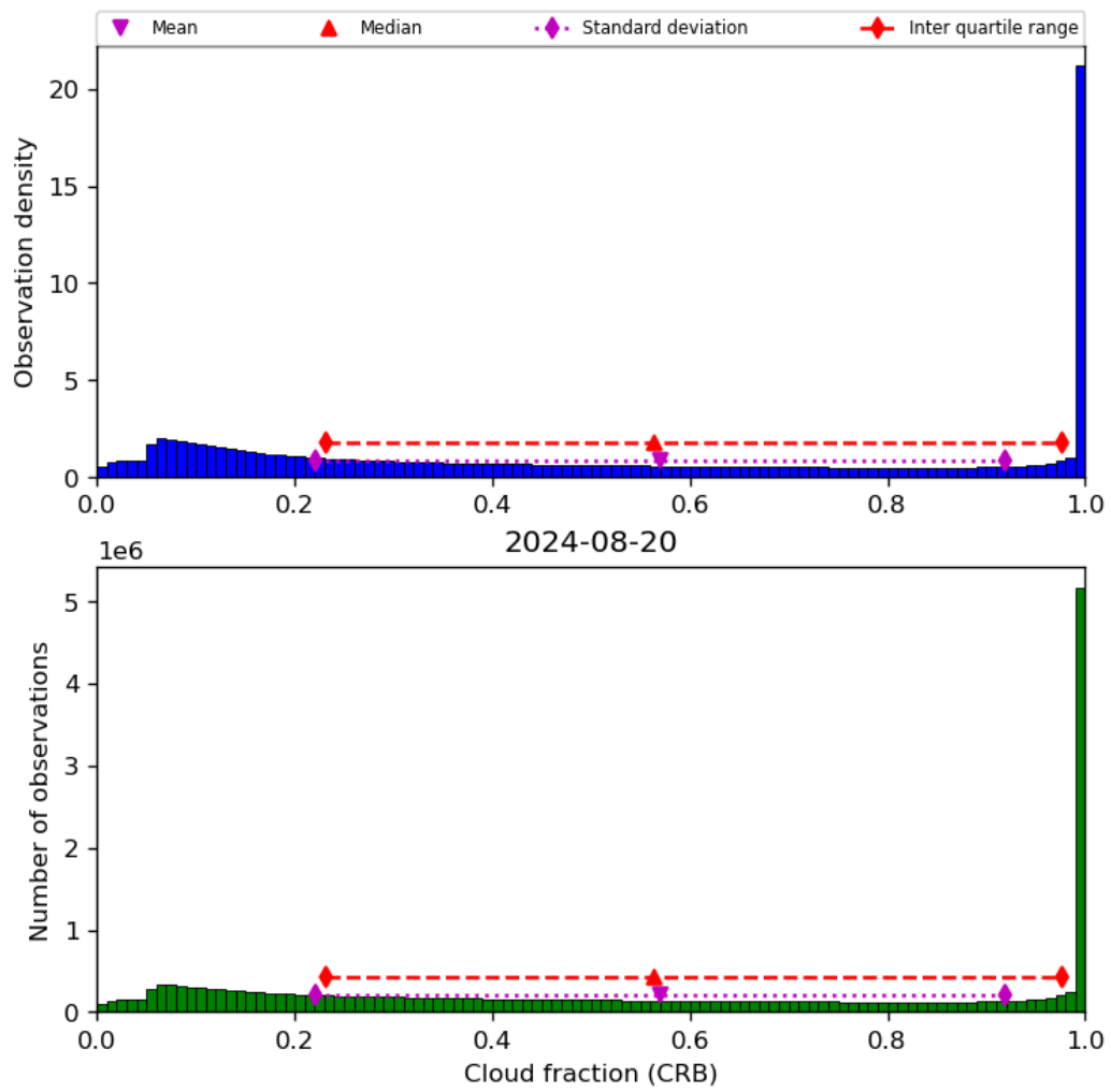
Figure 42: Histogram of “Cloud fraction (CRB)” for 2024-08-19 to 2024-08-21
