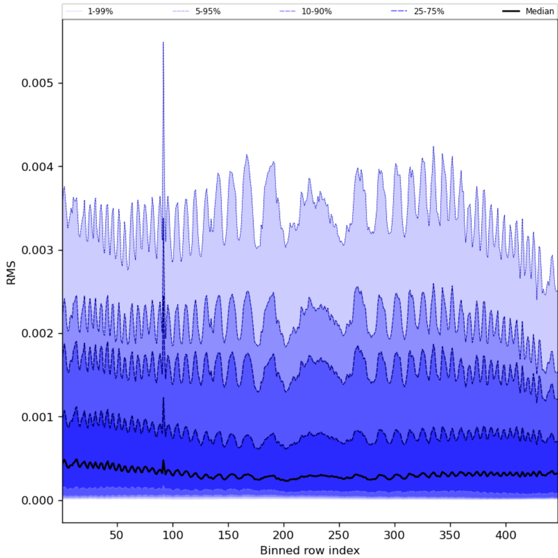
Figure 63: Along track statistics of “RMS” for 2024-08-19 to 2024-08-21
