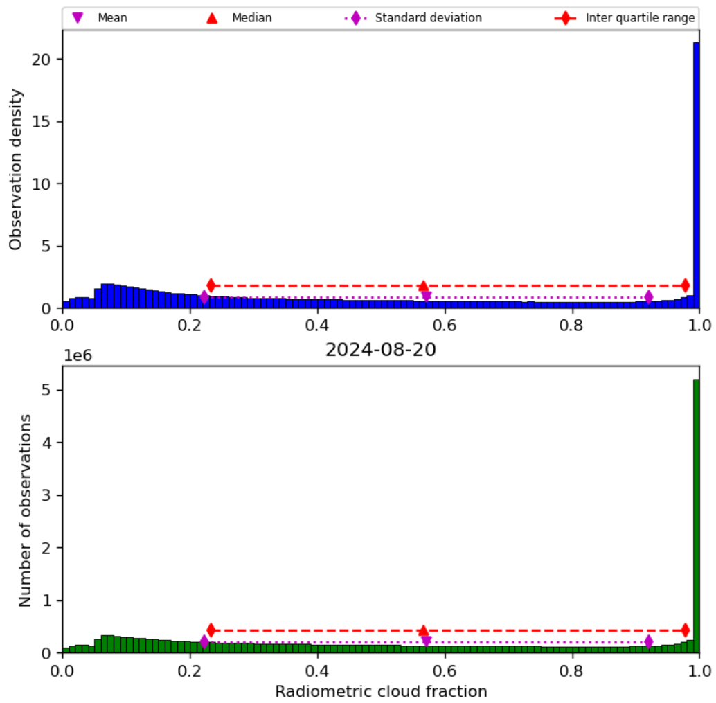
Figure 39: Histogram of “Radiometric cloud fraction” for 2024-08-19 to 2024-08-21
