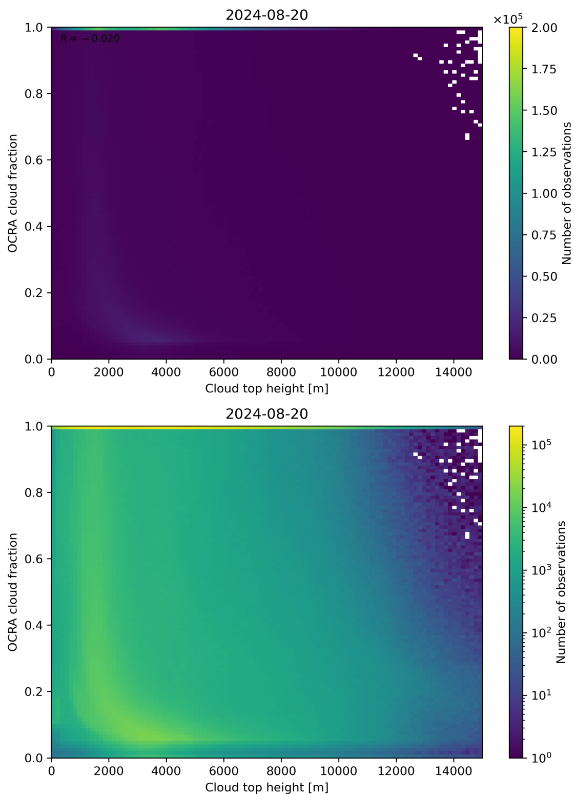
Figure 87: Scatter density plot of “Cloud top height” against “OCRA cloud fraction” for 2024-08-19 to 2024-08-21.
