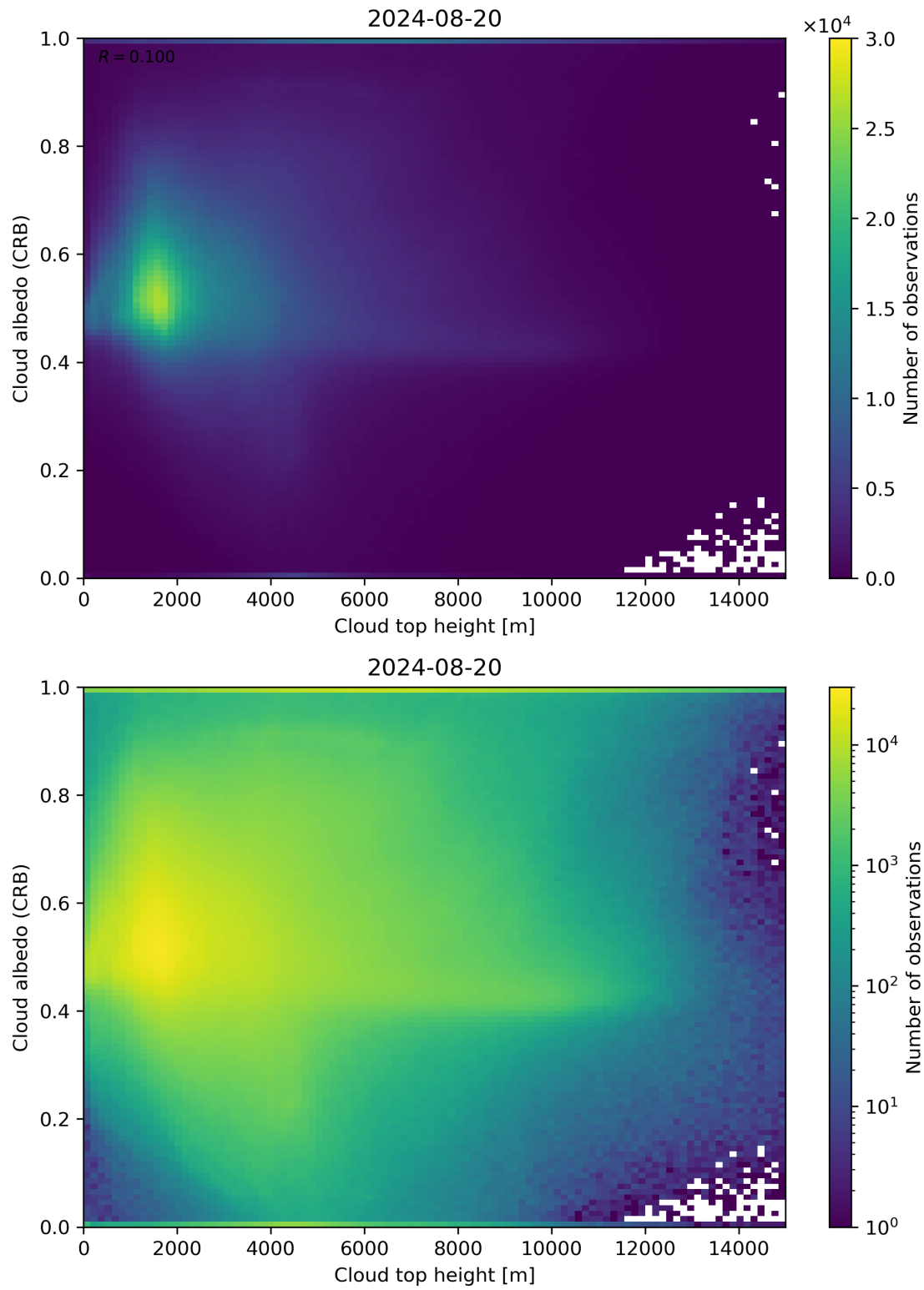
Figure 86: Scatter density plot of “Cloud top height” against “Cloud albedo (CRB)” for 2024-08-19 to 2024-08-21.
