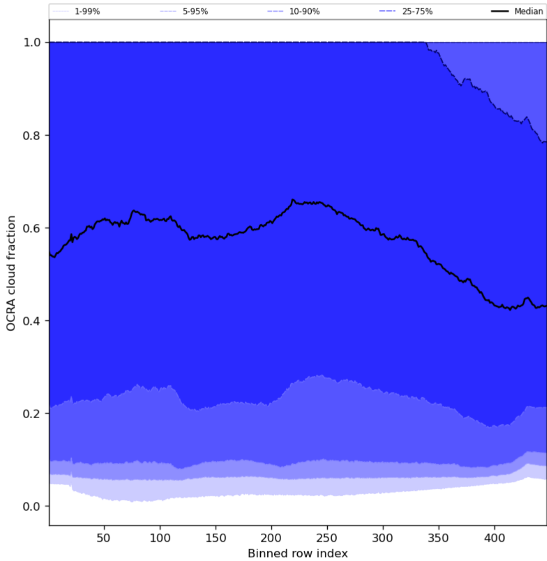
Figure 66: Along track statistics of “OCRA cloud fraction” for 2024-08-19 to 2024-08-21
