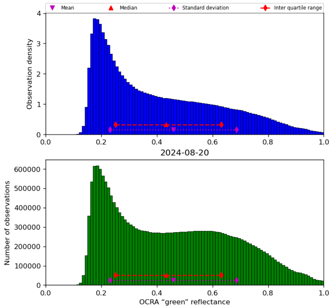
Figure 52: Histogram of “OCRA “green” reflectance” for 2024-08-19 to 2024-08-21
