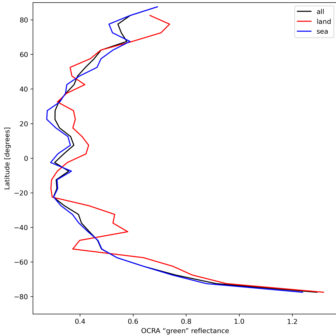
Figure 36: Zonal average of “OCRA “green” reflectance” for 2024-08-19 to 2024-08-21.
