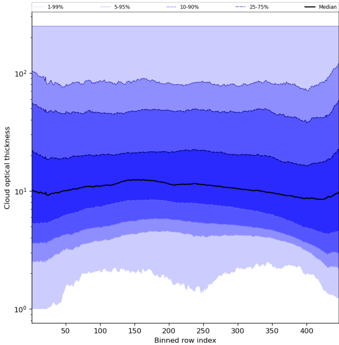
Figure 57: Along track statistics of “Cloud optical thickness” for 2024-08-19 to 2024-08-21
