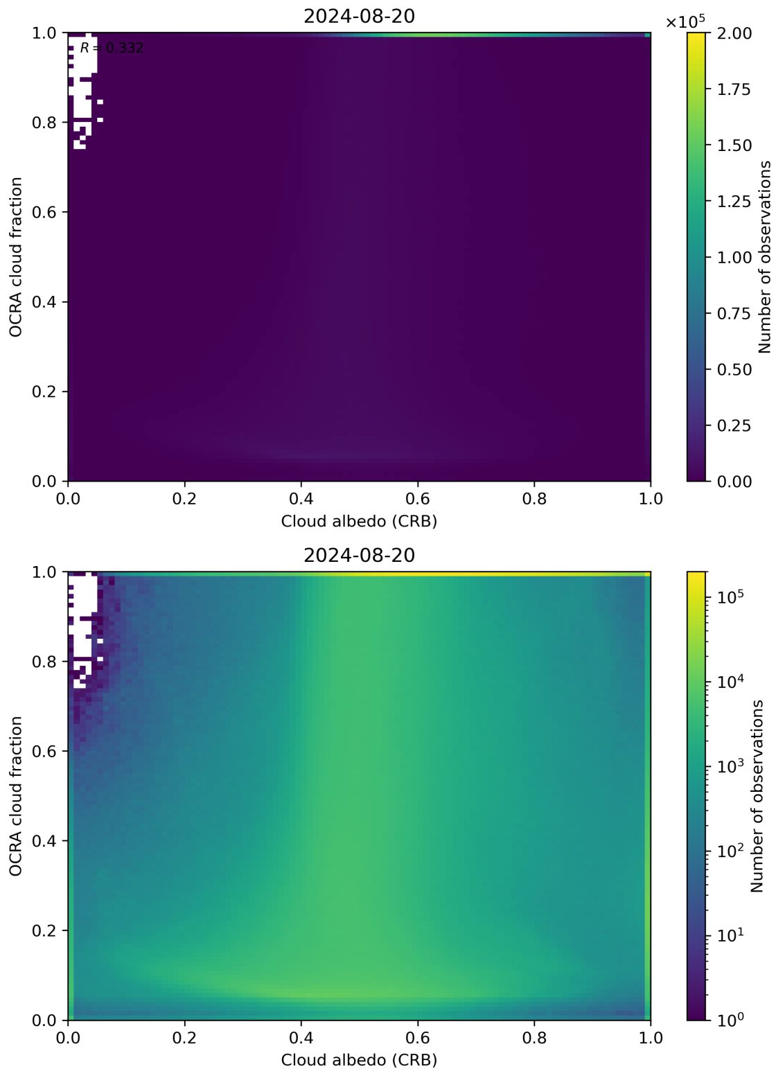
Figure 70: Scatter density plot of “Cloud albedo (CRB)” against “OCRA cloud fraction” for 2024-08-19 to 2024-08-21.
