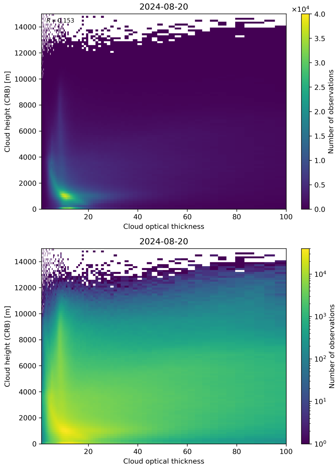
Figure 85: Scatter density plot of “Cloud optical thickness” against “Cloud height (CRB)” for 2024-08-19 to 2024-08-21.
