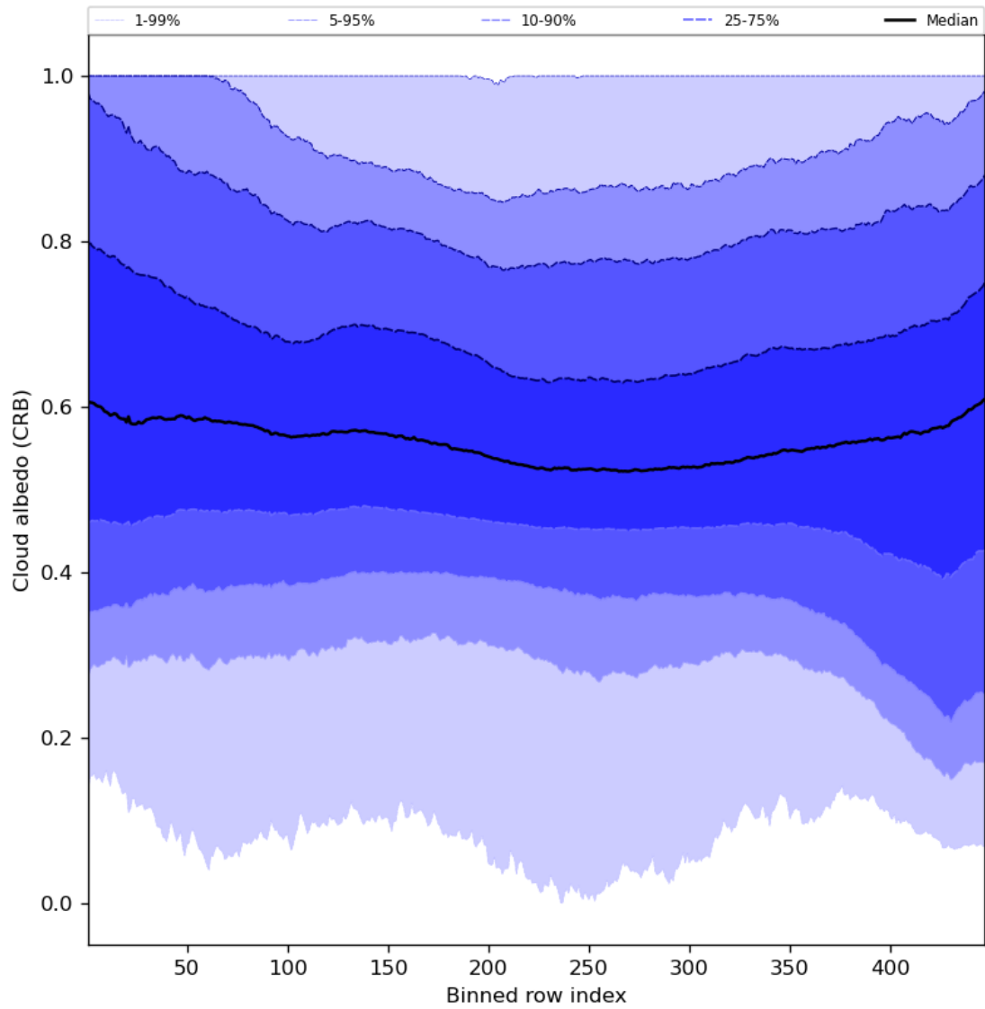
Figure 60: Along track statistics of “Cloud albedo (CRB)” for 2024-08-19 to 2024-08-21
