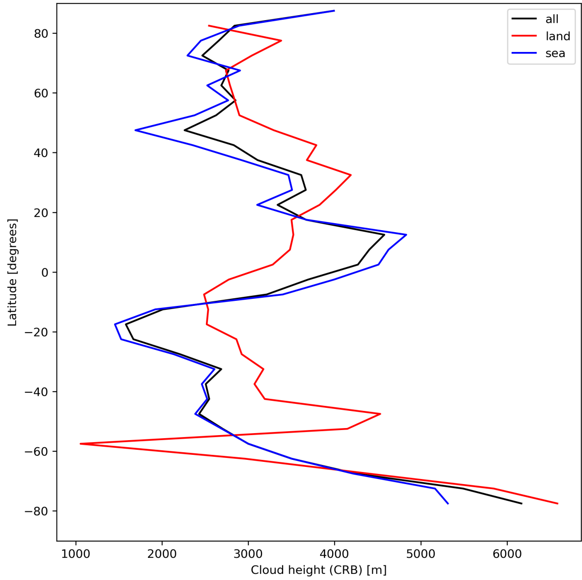
Figure 27: Zonal average of “Cloud height (CRB)” for 2024-08-19 to 2024-08-21.
