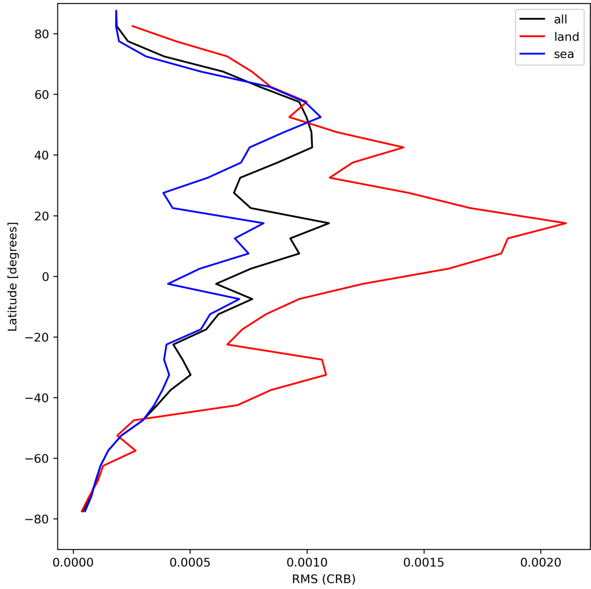
Figure 32: Zonal average of “RMS (CRB)” for 2024-08-19 to 2024-08-21.
