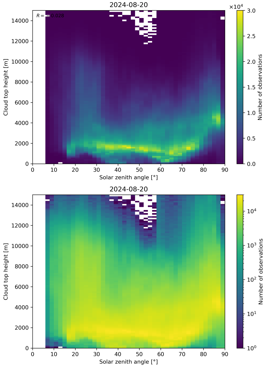
Figure 104: Scatter density plot of “Solar zenith angle” against “Cloud top height” for 2024-08-19 to 2024-08-21.
