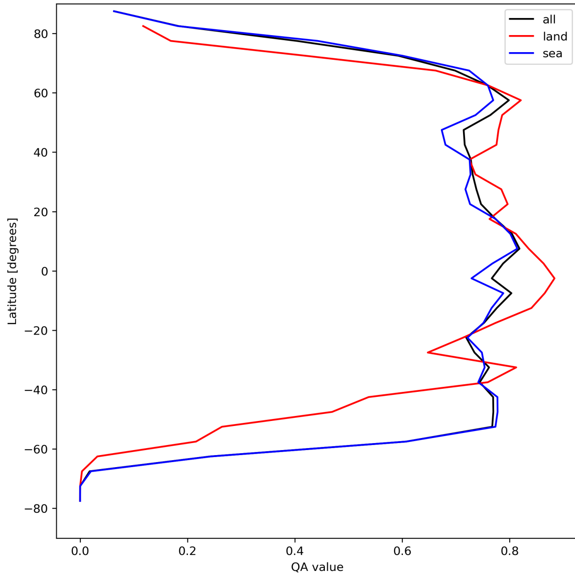
Figure 22: Zonal average of “QA value” for 2024-08-19 to 2024-08-21.
