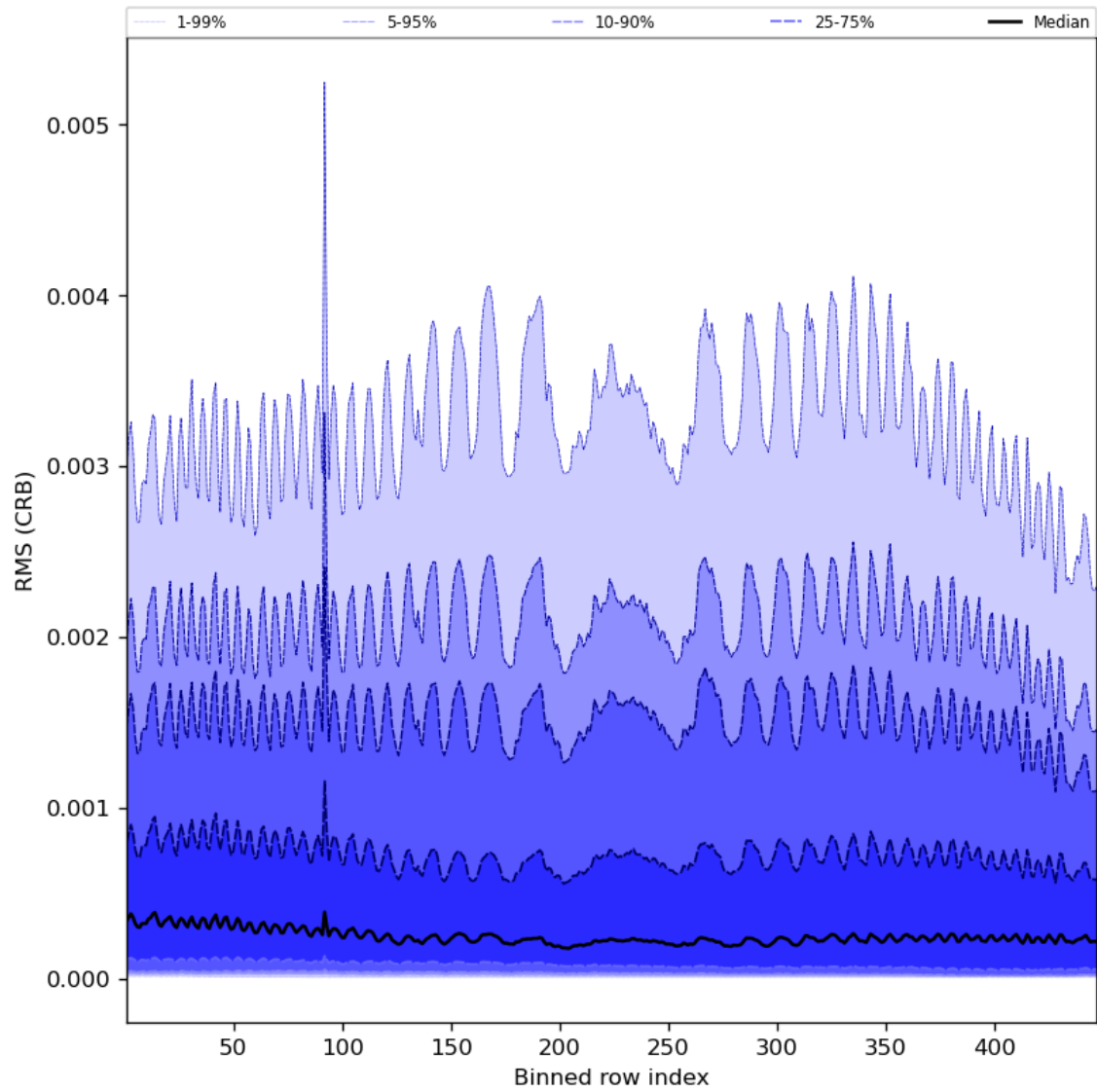
Figure 64: Along track statistics of “RMS (CRB)” for 2024-08-19 to 2024-08-21
