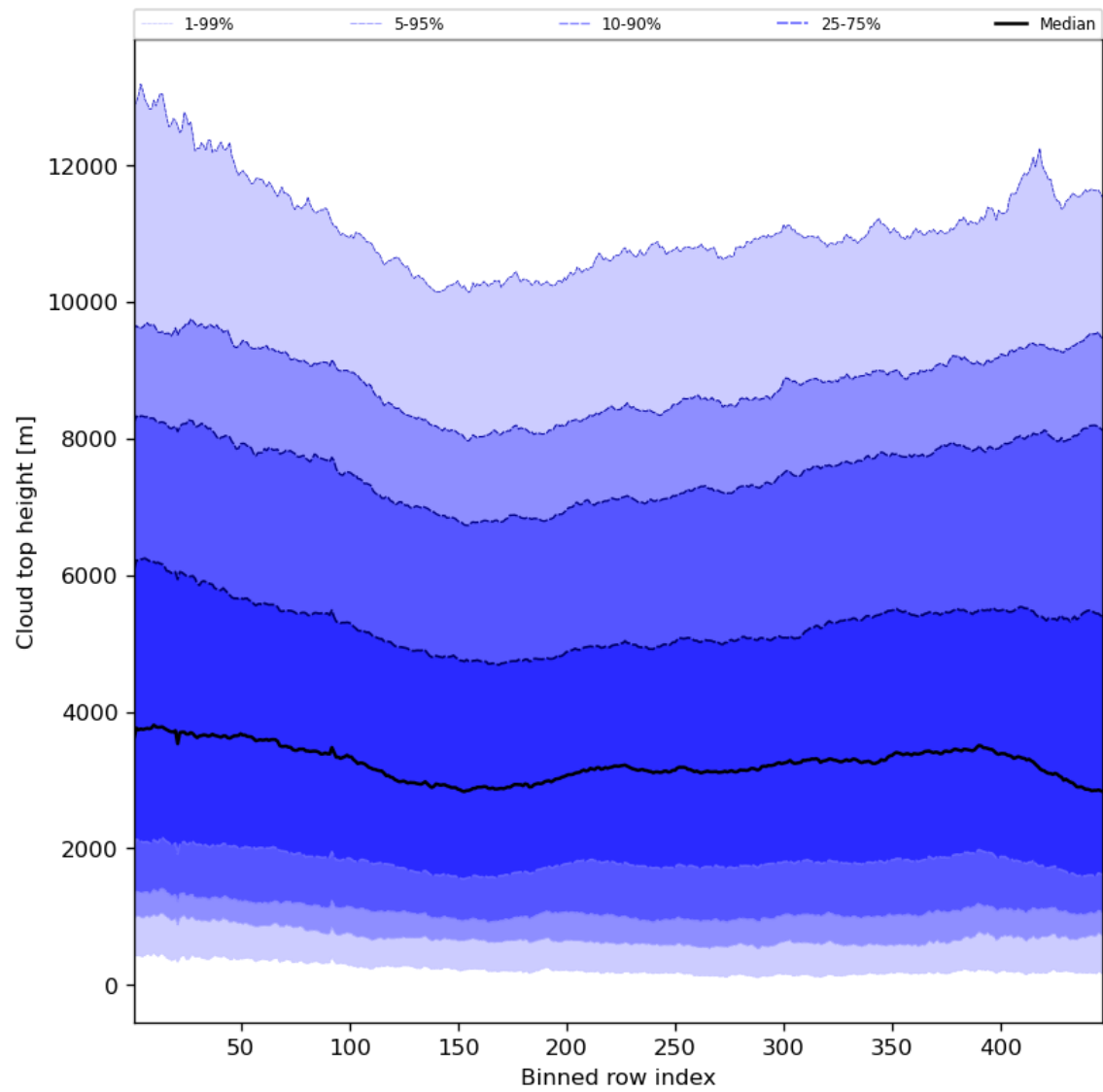
Figure 56: Along track statistics of “Cloud top height” for 2024-08-19 to 2024-08-21
