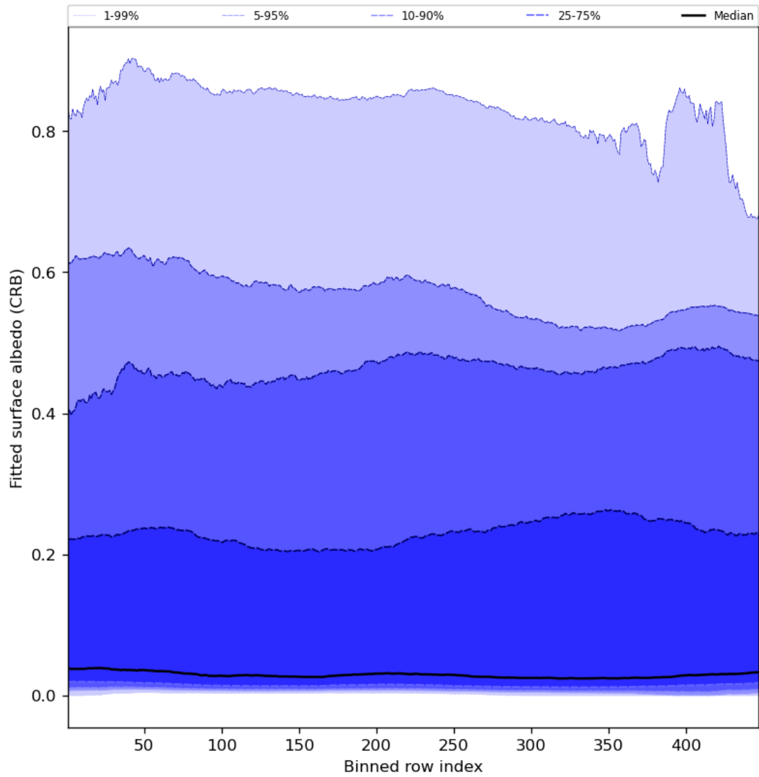
Figure 62: Along track statistics of “Fitted surface albedo (CRB)” for 2024-08-19 to 2024-08-21
