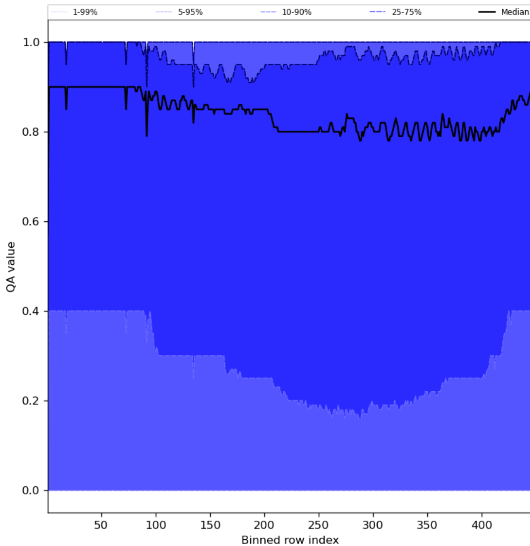
Figure 54: Along track statistics of "QA value" for 2024-08-19 to 2024-08-21
