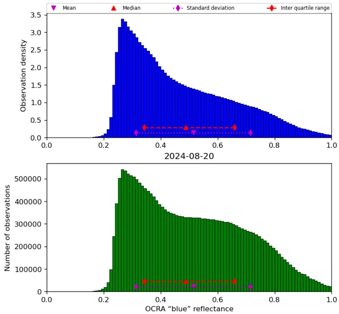
Figure 51: Histogram of “OCRA “blue” reflectance” for 2024-08-19 to 2024-08-21
