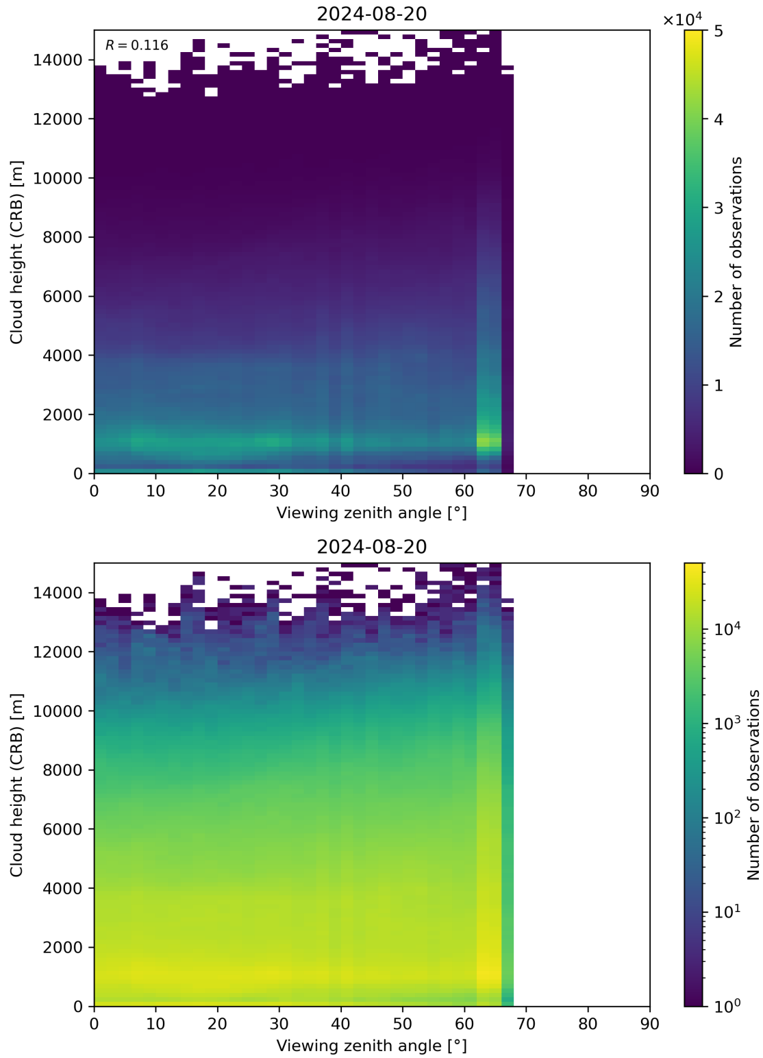
Figure 110: Scatter density plot of “Viewing zenith angle” against “Cloud height (CRB)” for 2024-08-19 to 2024-08-21.
