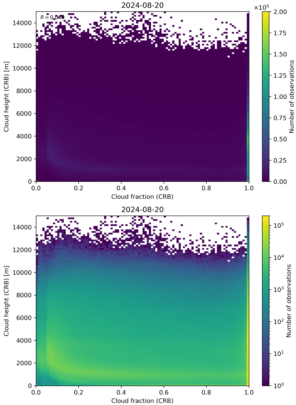
Figure 79: Scatter density plot of “Cloud fraction (CRB)” against “Cloud height (CRB)” for 2024-08-19 to 2024-08-21.
