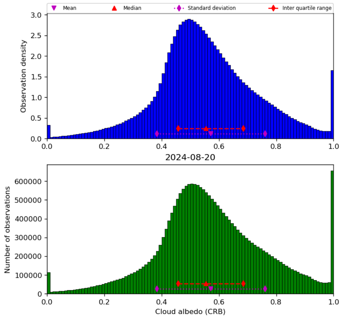
Figure 44: Histogram of “Cloud albedo (CRB)” for 2024-08-19 to 2024-08-21
