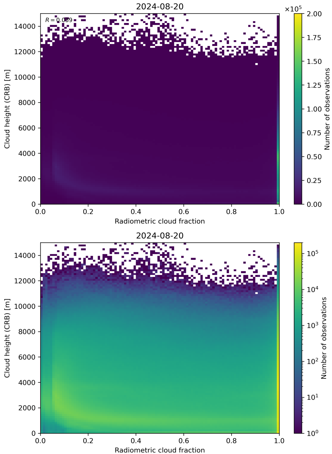
Figure 74: Scatter density plot of “Radiometric cloud fraction” against “Cloud height (CRB)” for 2024-08-19 to 2024-08-21.
