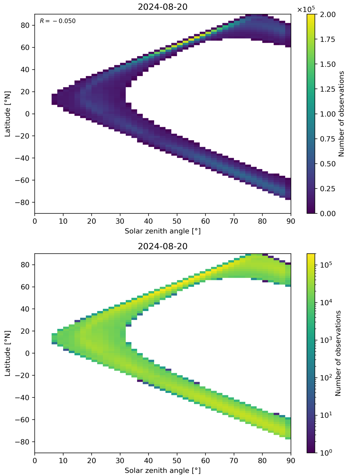
Figure 105: Scatter density plot of “Solar zenith angle” against “Latitude” for 2024-08-19 to 2024-08-21.
