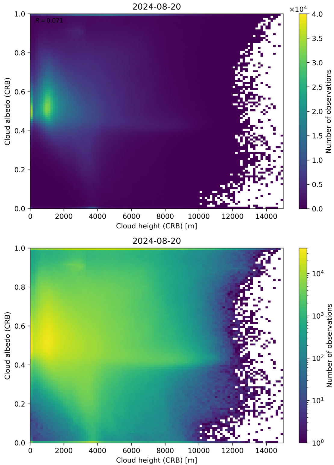
Figure 80: Scatter density plot of “Cloud height (CRB)” against “Cloud albedo (CRB)” for 2024-08-19 to 2024-08-21.
