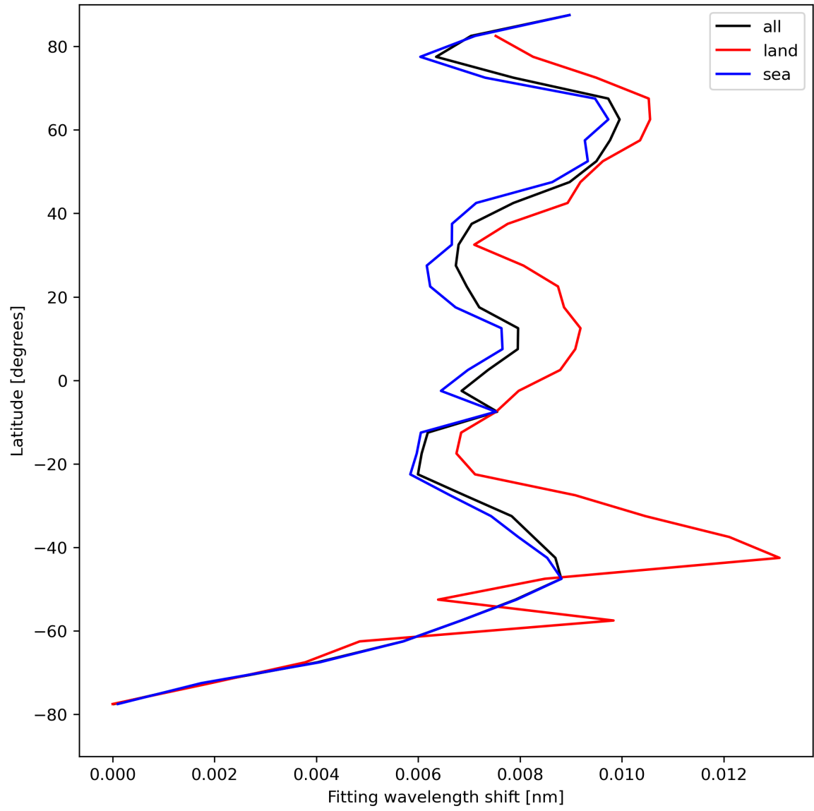
Figure 33: Zonal average of “Fitting wavelength shift” for 2024-08-19 to 2024-08-21.
