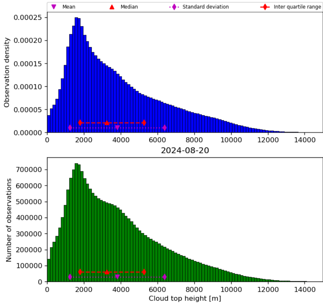
Figure 40: Histogram of “Cloud top height” for 2024-08-19 to 2024-08-21
