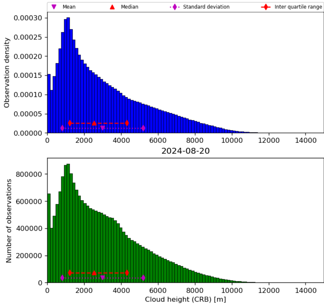
Figure 43: Histogram of “Cloud height (CRB)” for 2024-08-19 to 2024-08-21
