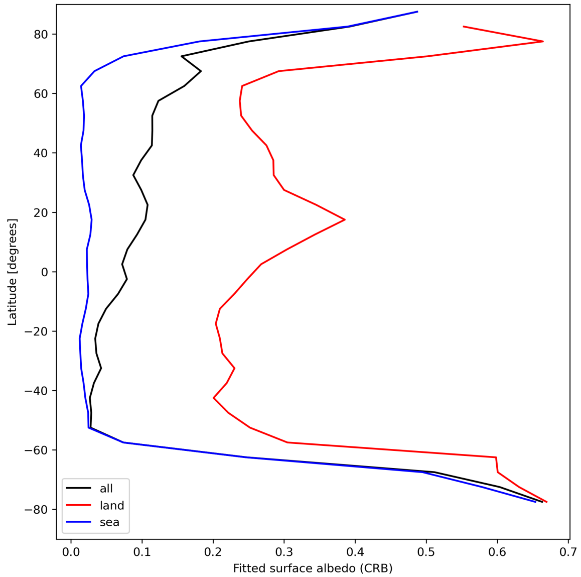
Figure 30: Zonal average of “Fitted surface albedo (CRB)” for 2024-08-19 to 2024-08-21.
