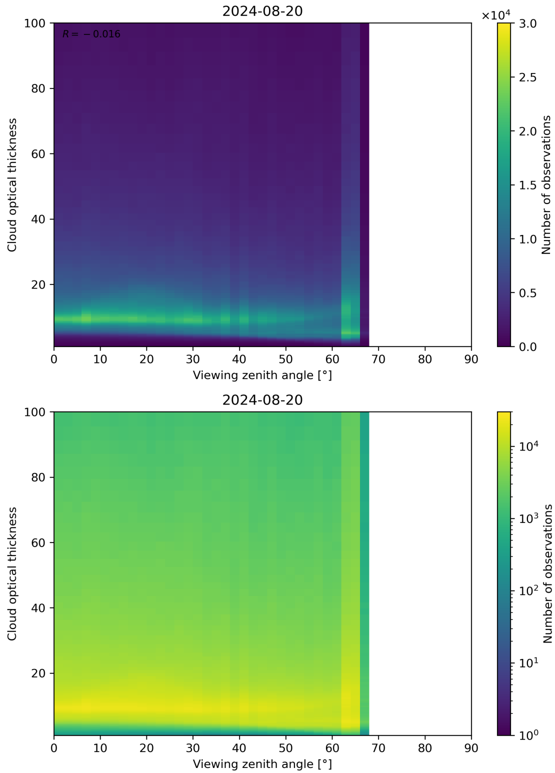
Figure 111: Scatter density plot of “Viewing zenith angle” against “Cloud optical thickness” for 2024-08-19 to 2024-08-21.
