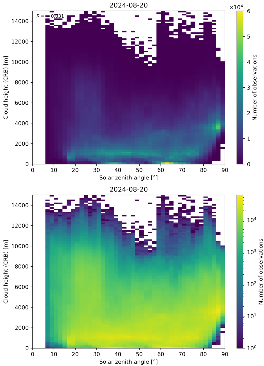
Figure 102: Scatter density plot of “Solar zenith angle” against “Cloud height (CRB)” for 2024-08-19 to 2024-08-21.
