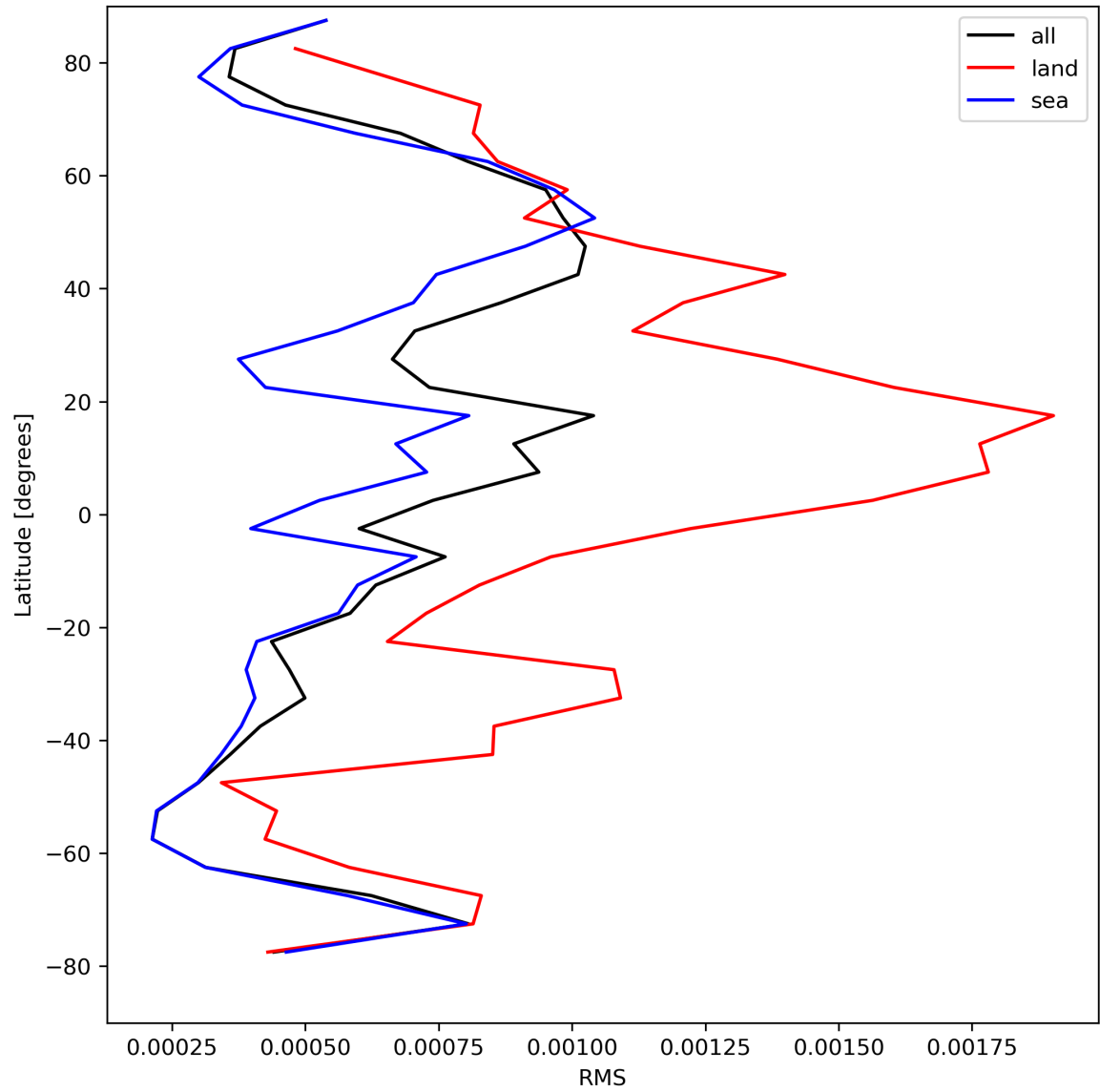
Figure 31: Zonal average of “RMS” for 2024-08-19 to 2024-08-21.
