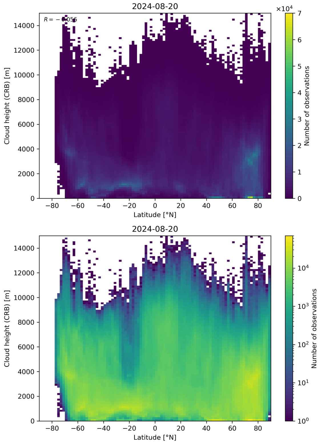
Figure 95: Scatter density plot of “Latitude” against “Cloud height (CRB)” for 2024-08-19 to 2024-08-21.
