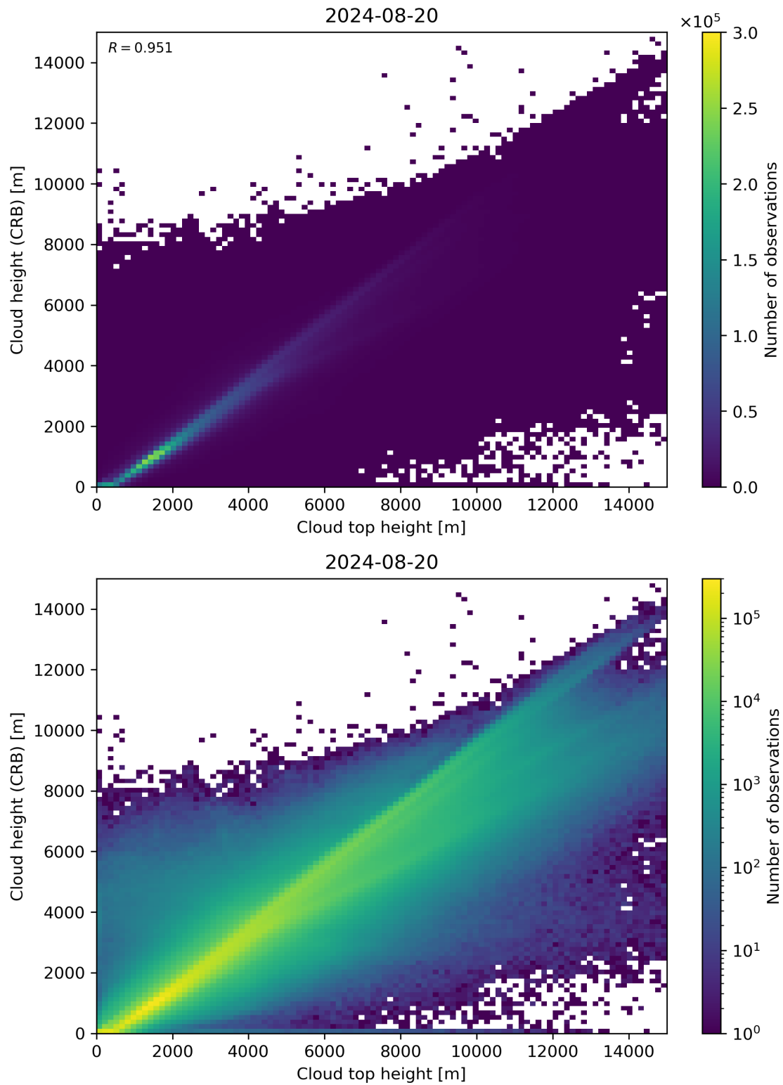
Figure 89: Scatter density plot of “Cloud top height” against “Cloud height (CRB)” for 2024-08-19 to 2024-08-21.
