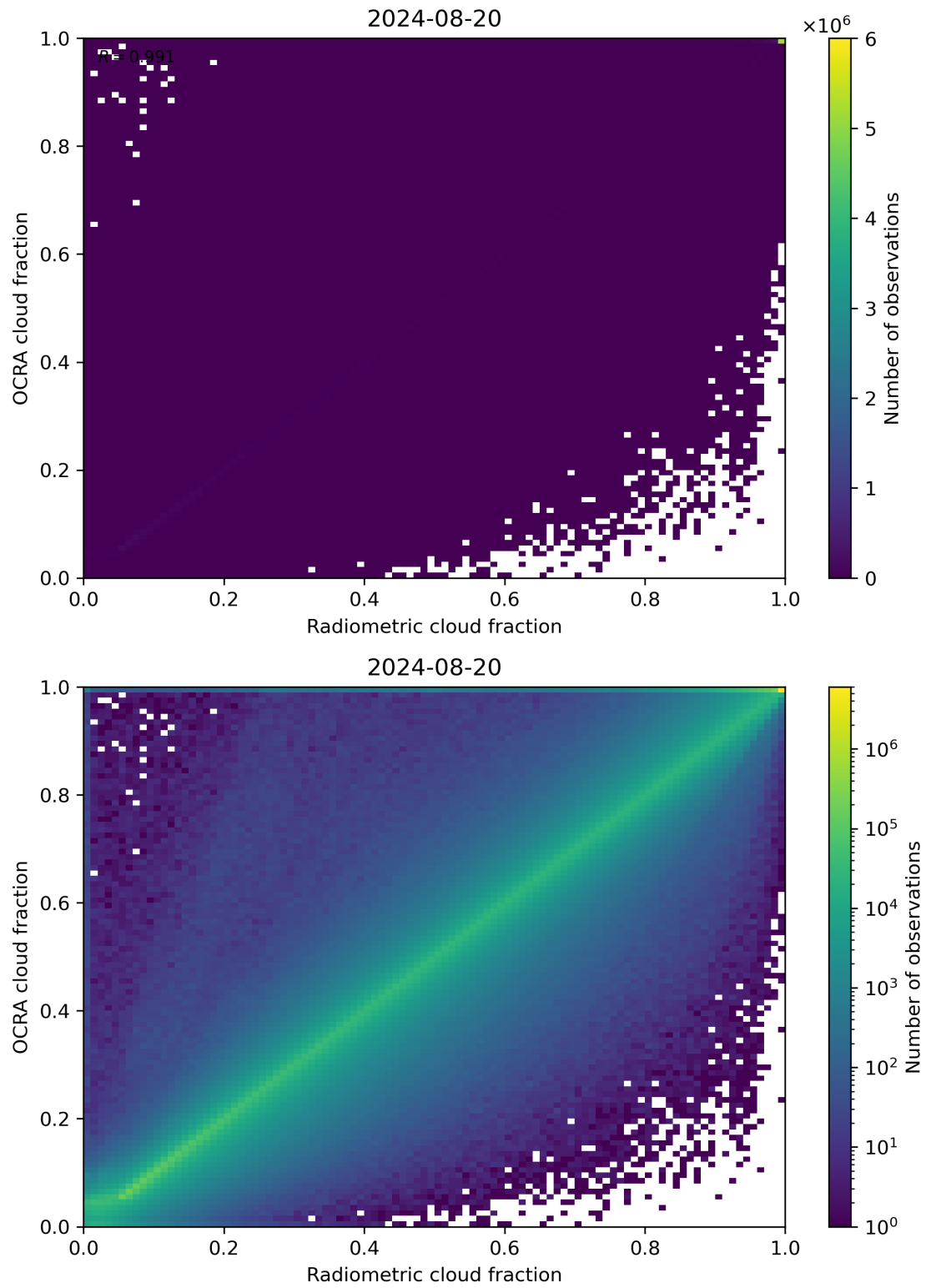
Figure 72: Scatter density plot of “Radiometric cloud fraction” against “OCRA cloud fraction” for 2024-08-19 to 2024-08-21.
