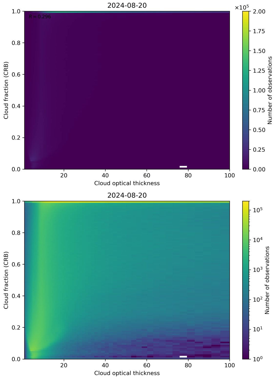
Figure 84: Scatter density plot of “Cloud optical thickness” against “Cloud fraction (CRB)” for 2024-08-19 to 2024-08-21.
