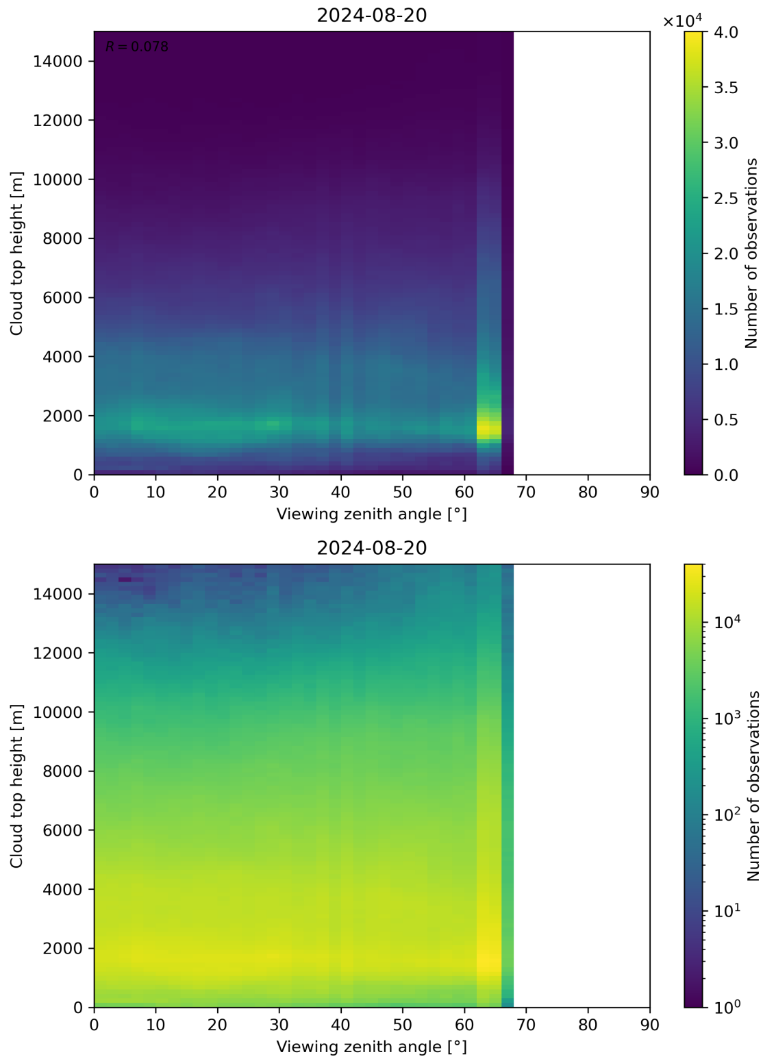
Figure 112: Scatter density plot of “Viewing zenith angle” against “Cloud top height” for 2024-08-19 to 2024-08-21.
