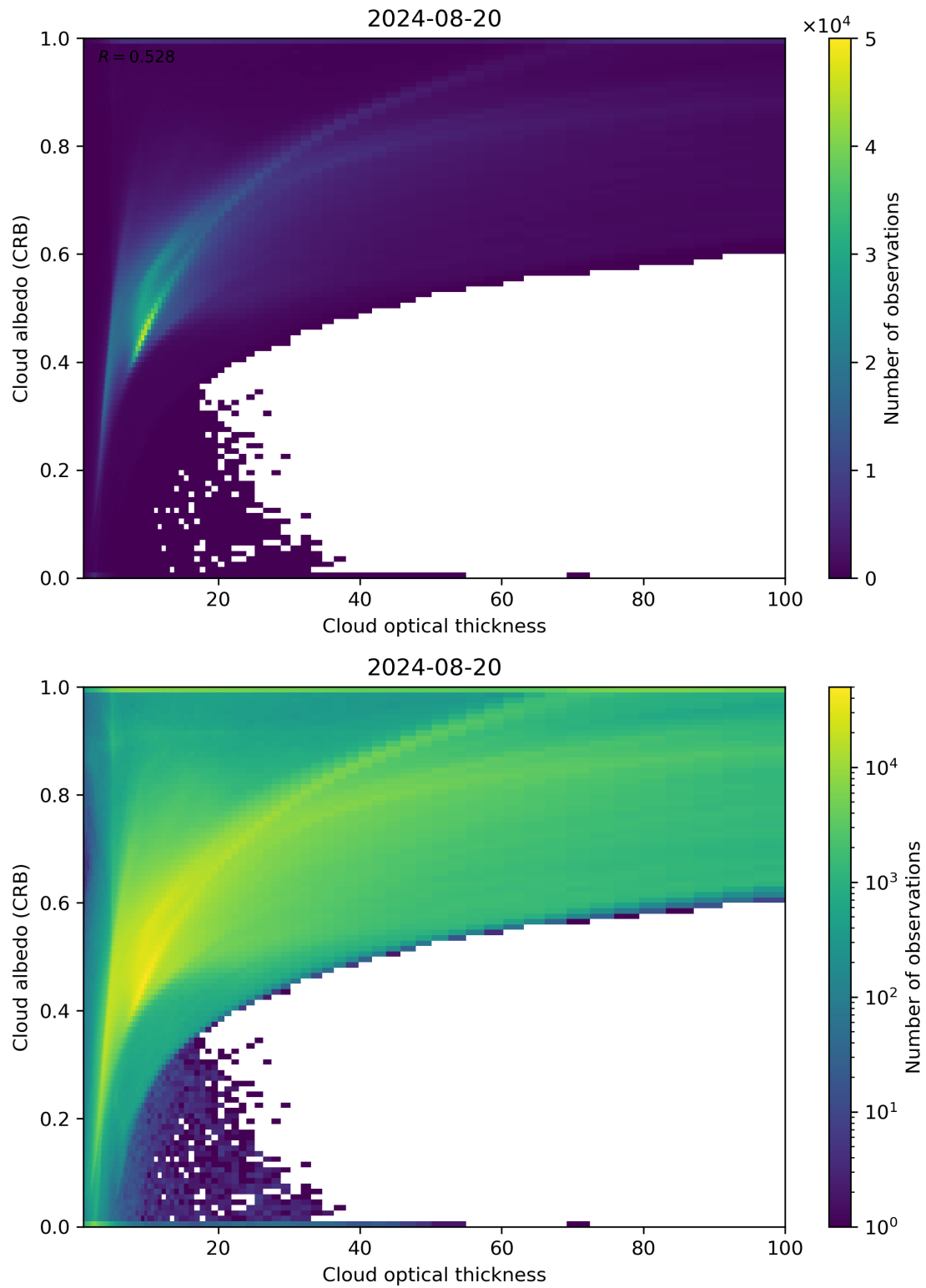
Figure 82: Scatter density plot of “Cloud optical thickness” against “Cloud albedo (CRB)” for 2024-08-19 to 2024-08-21.
