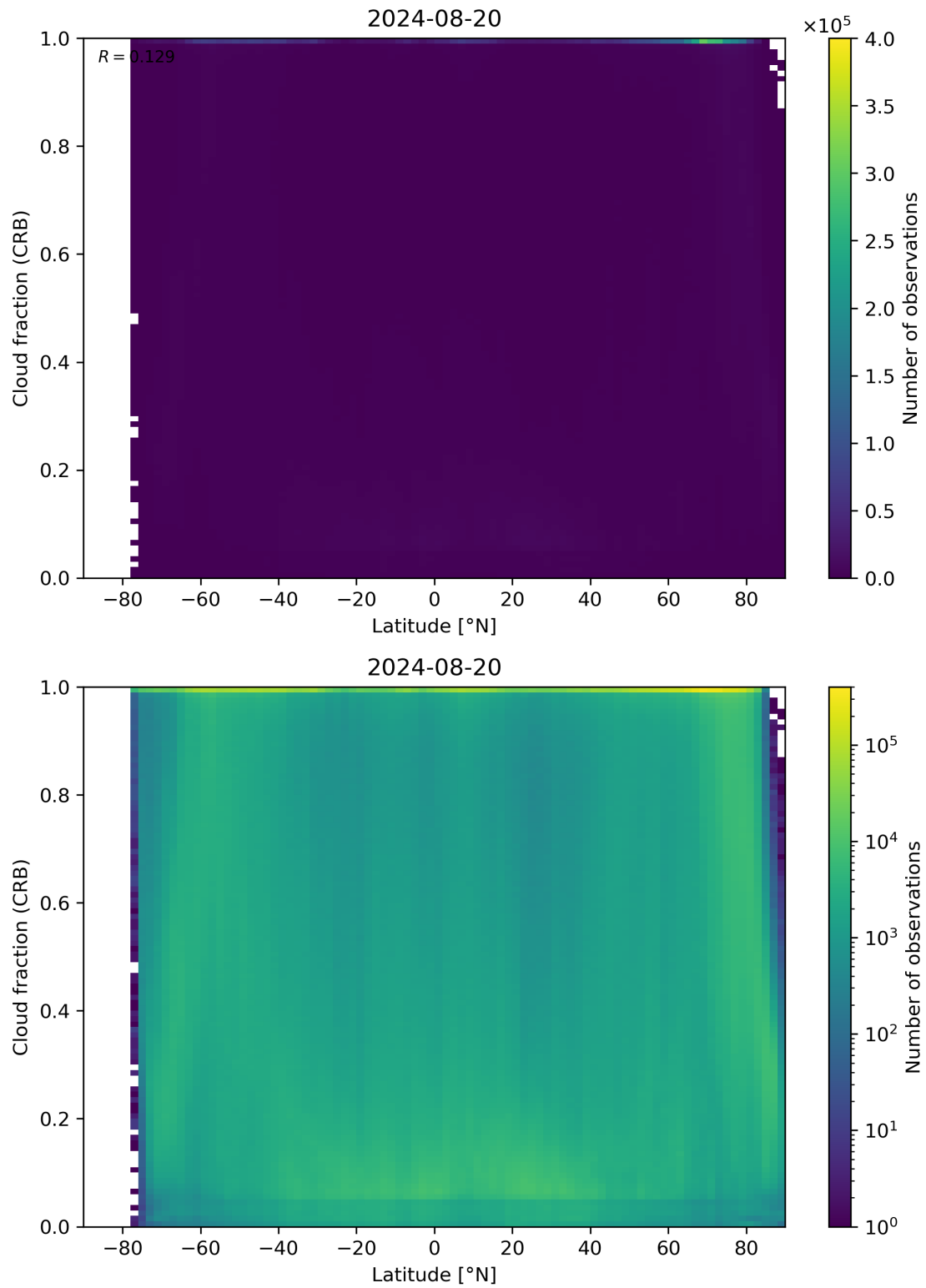
Figure 94: Scatter density plot of “Latitude” against “Cloud fraction (CRB)” for 2024-08-19 to 2024-08-21.
