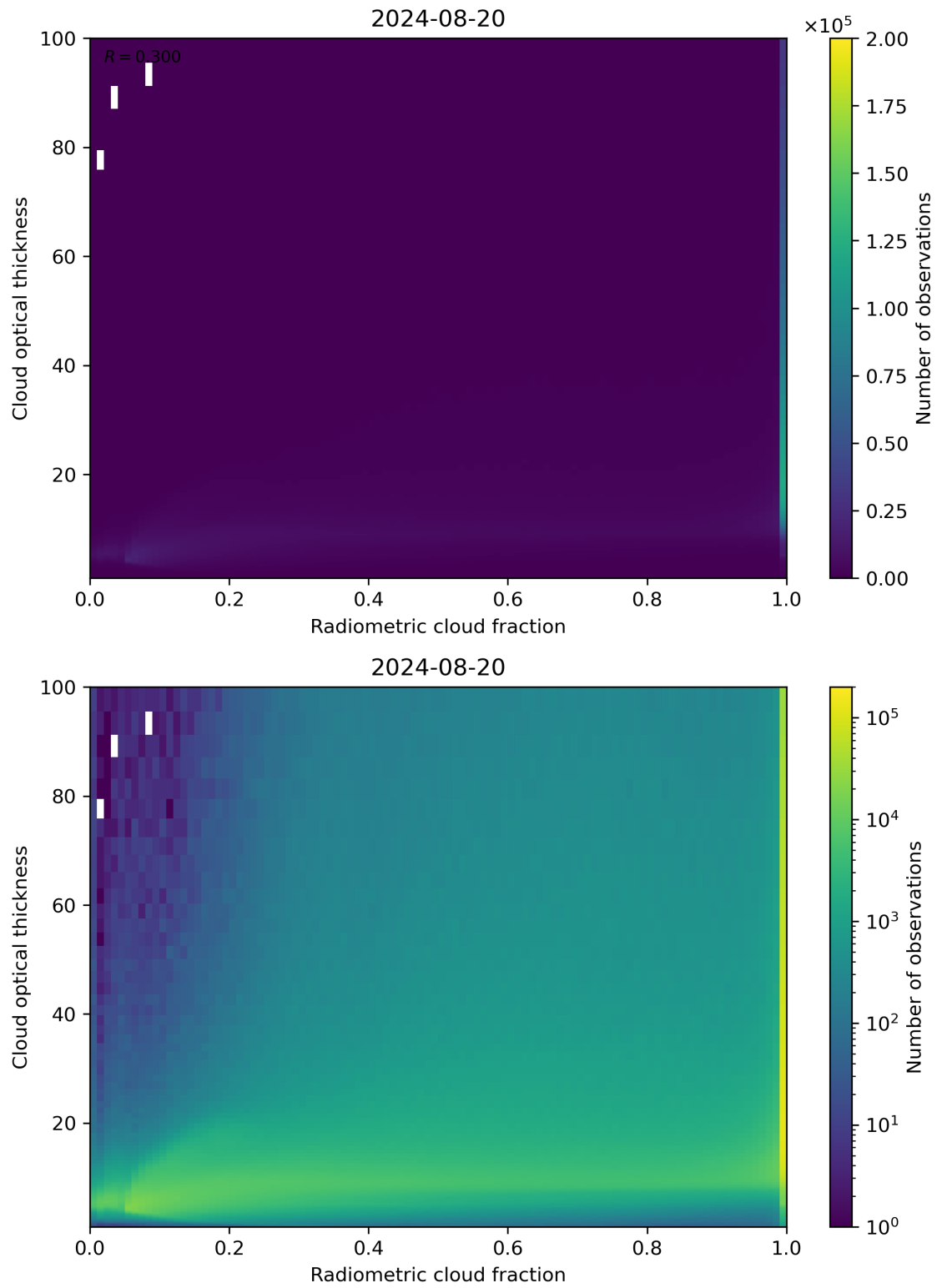
Figure 75: Scatter density plot of “Radiometric cloud fraction” against “Cloud optical thickness” for 2024-08-19 to 2024-08-21.
