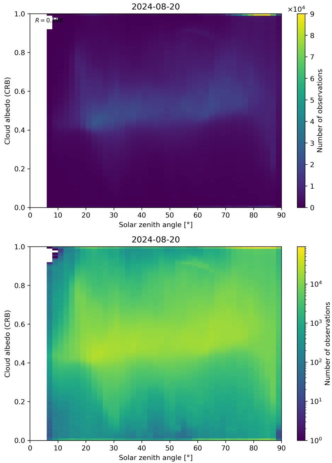
Figure 98: Scatter density plot of “Solar zenith angle” against “Cloud albedo (CRB)” for 2024-08-19 to 2024-08-21.
