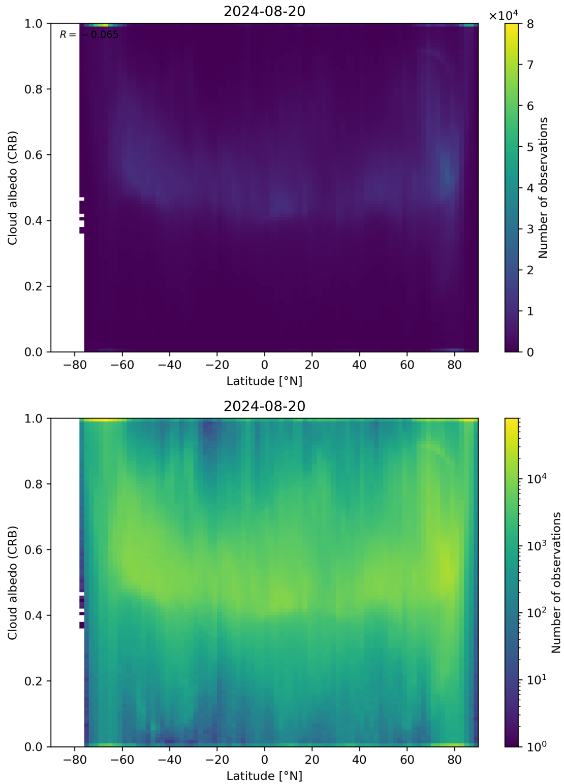
Figure 91: Scatter density plot of “Latitude” against “Cloud albedo (CRB)” for 2024-08-19 to 2024-08-21.
