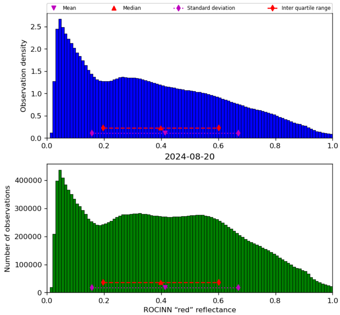
Figure 53: Histogram of “ROCINN “red” reflectance” for 2024-08-19 to 2024-08-21
