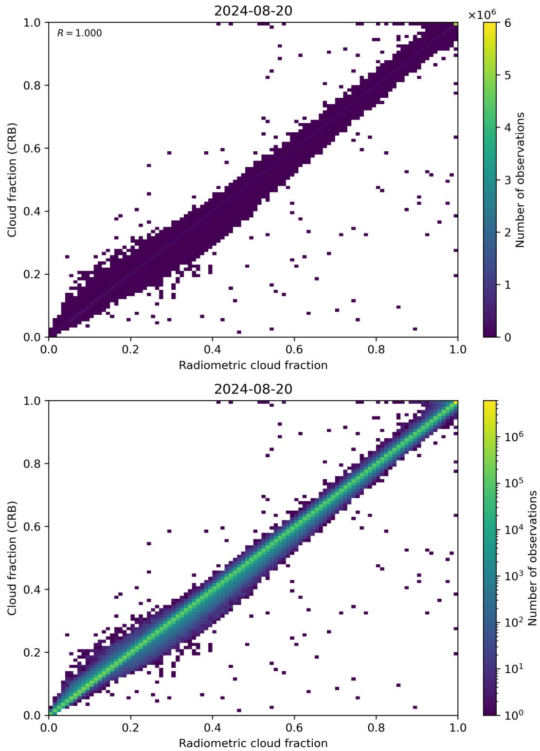
Figure 73: Scatter density plot of “Radiometric cloud fraction” against “Cloud fraction (CRB)” for 2024-08-19 to 2024-08-21.
