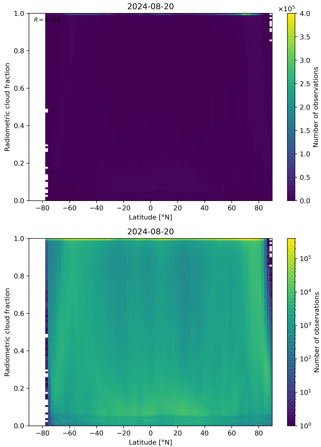
Figure 92: Scatter density plot of “Latitude” against “Radiometric cloud fraction” for 2024-08-19 to 2024-08-21.
