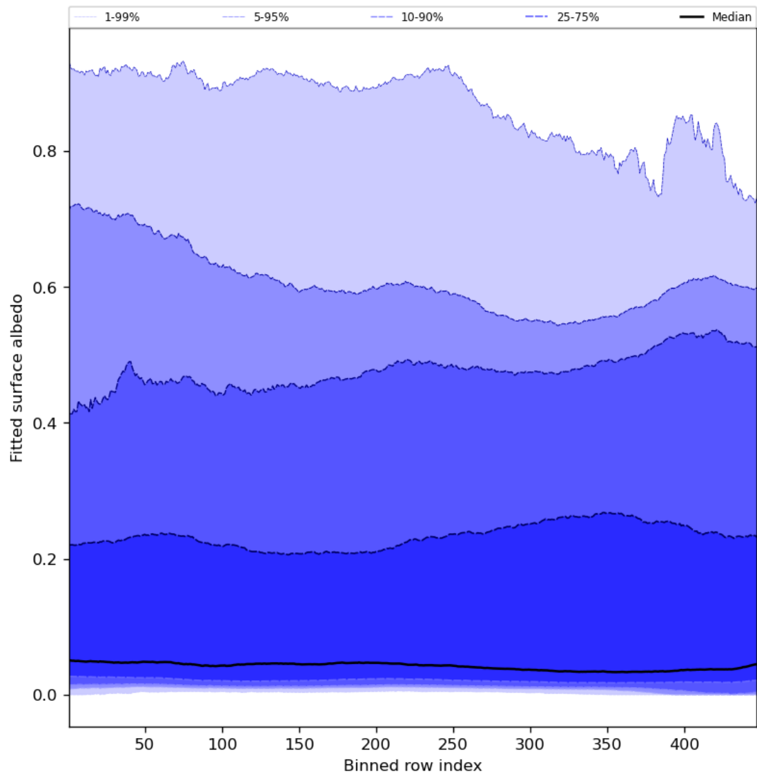
Figure 61: Along track statistics of “Fitted surface albedo” for 2024-08-19 to 2024-08-21
