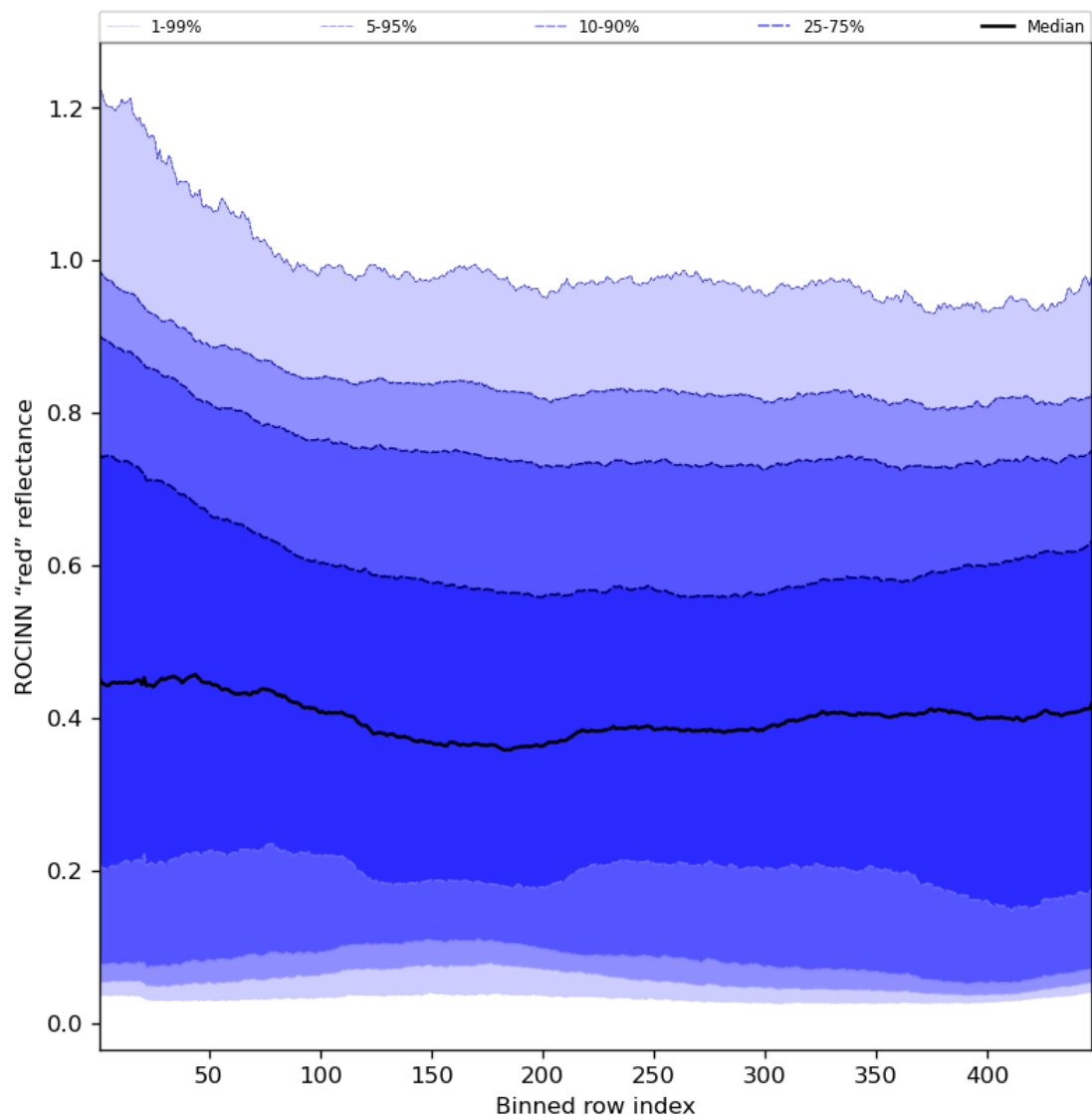
Figure 69: Along track statistics of "ROCINN "red" reflectance" for 2024-08-19 to 2024-08-21
