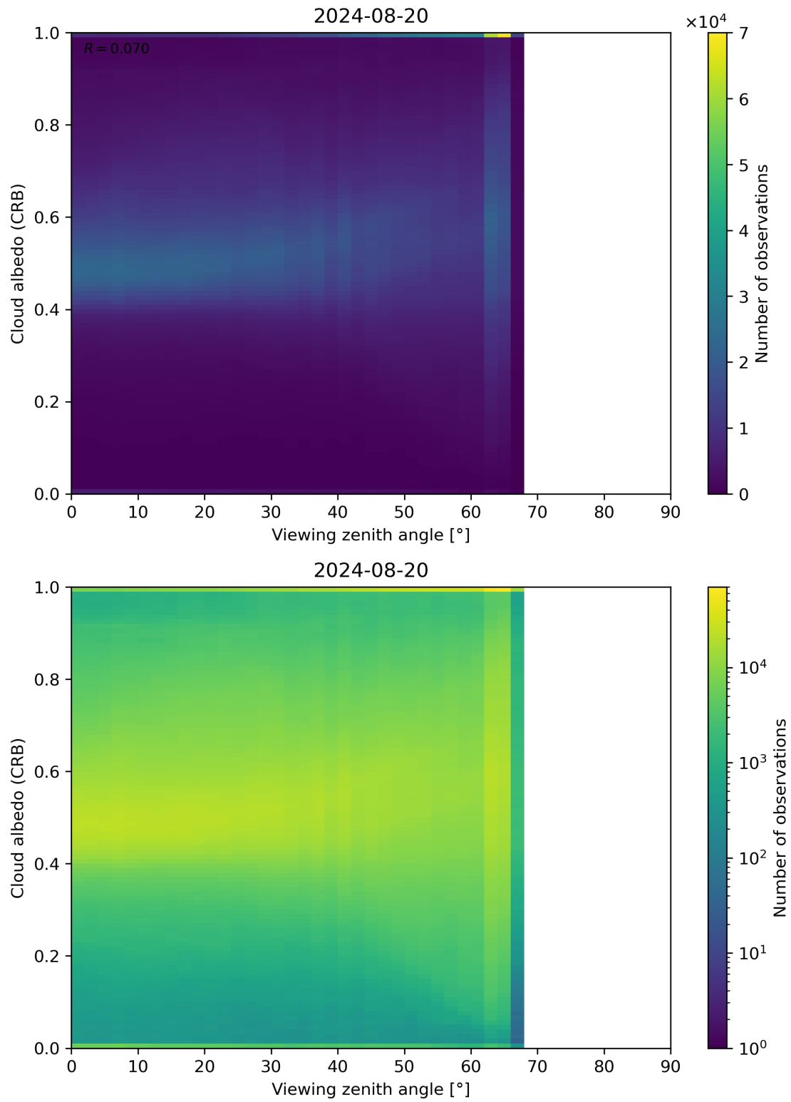
Figure 106: Scatter density plot of “Viewing zenith angle” against “Cloud albedo (CRB)” for 2024-08-19 to 2024-08-21.
