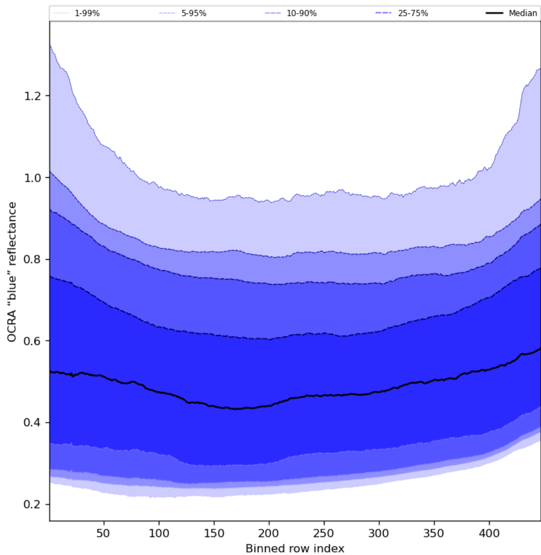
Figure 67: Along track statistics of “OCRA “blue” reflectance” for 2024-08-19 to 2024-08-21
