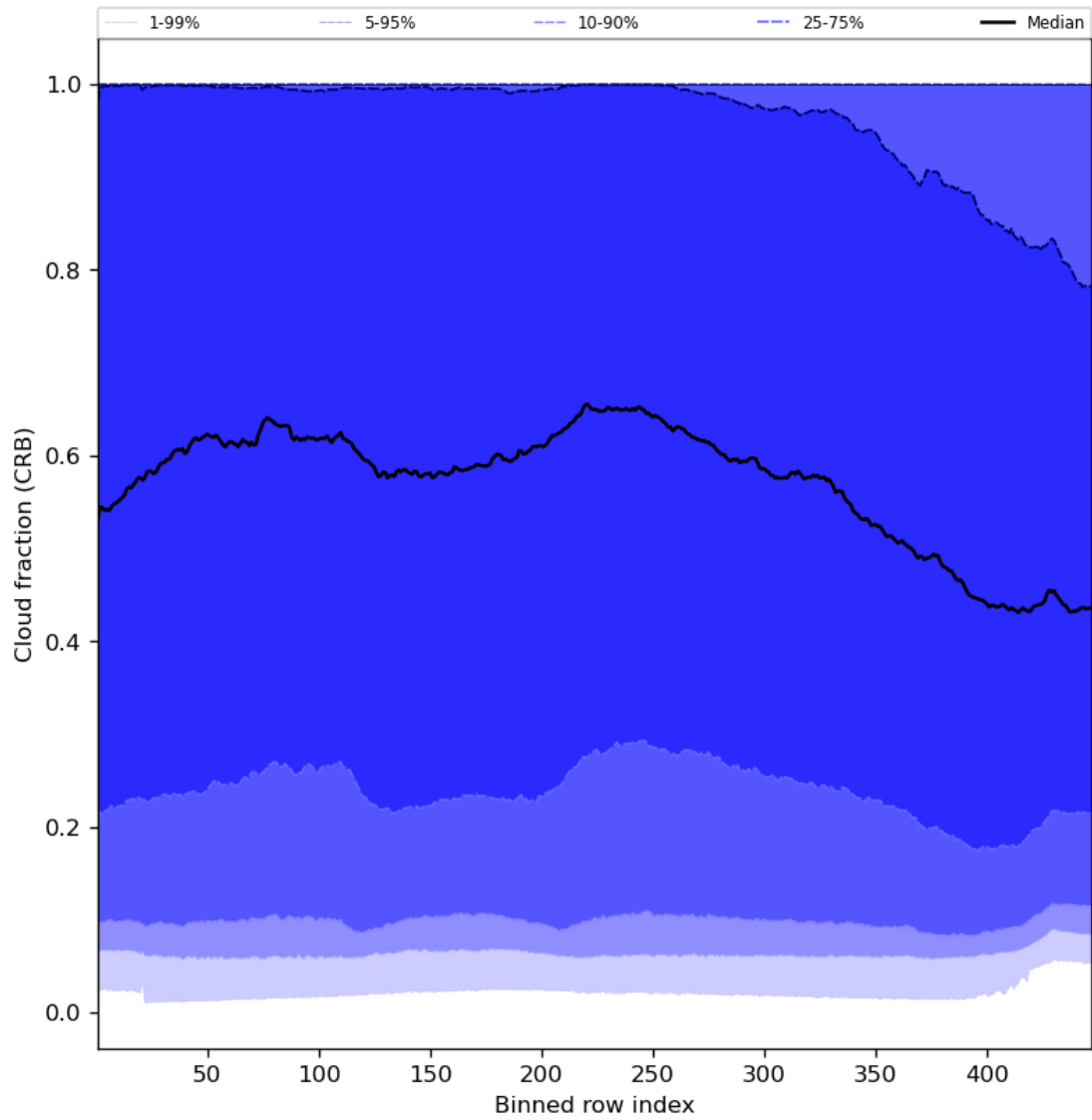
Figure 58: Along track statistics of “Cloud fraction (CRB)” for 2024-08-19 to 2024-08-21
