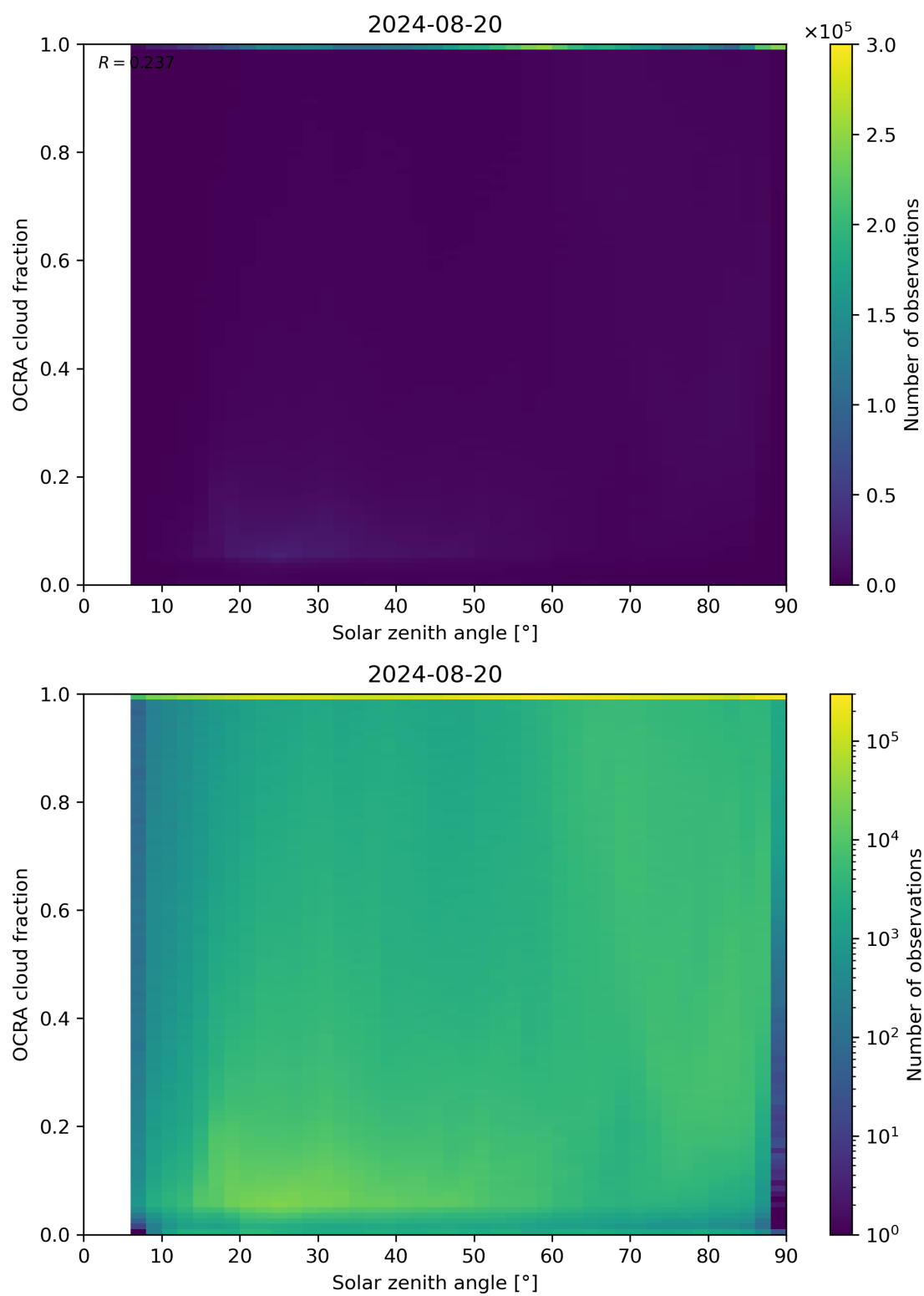
Figure 100: Scatter density plot of “Solar zenith angle” against “OCRA cloud fraction” for 2024-08-19 to 2024-08-21.
