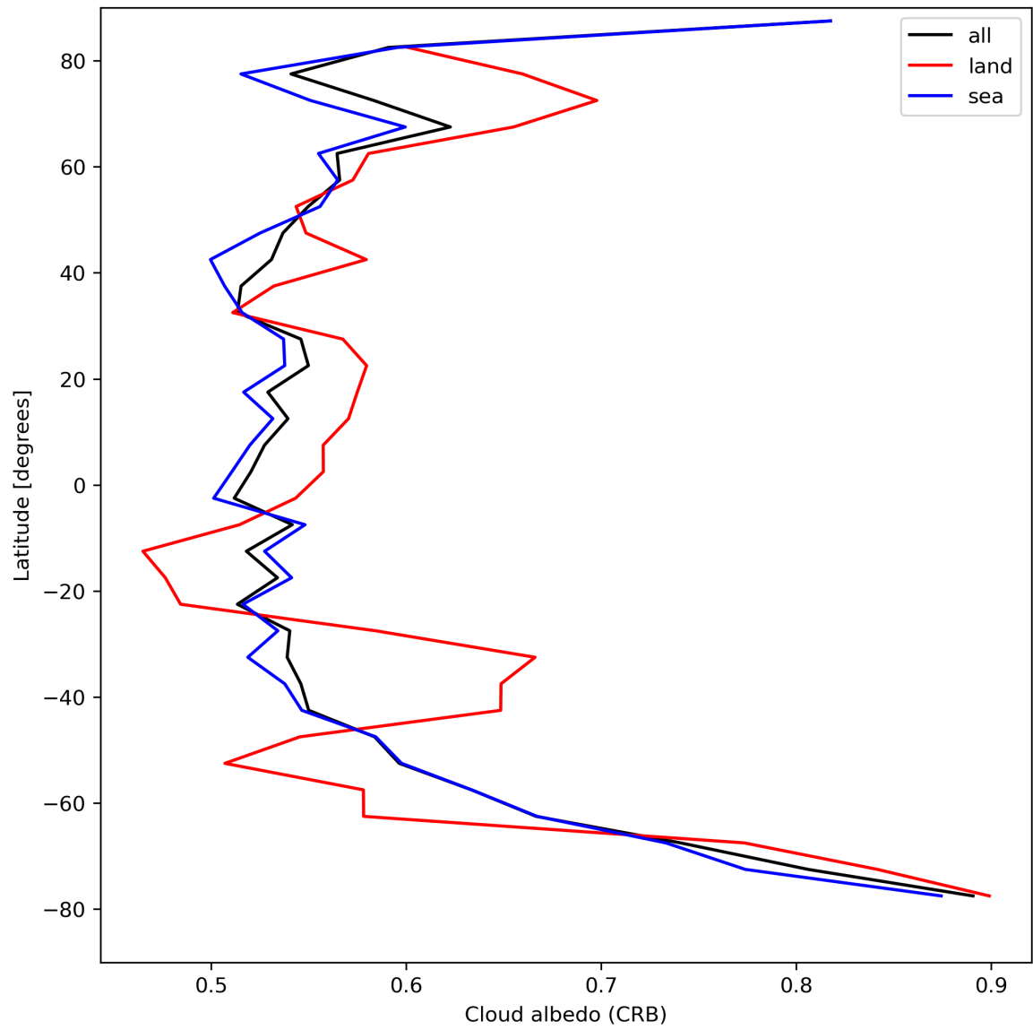
Figure 28: Zonal average of “Cloud albedo (CRB)” for 2024-08-19 to 2024-08-21.
