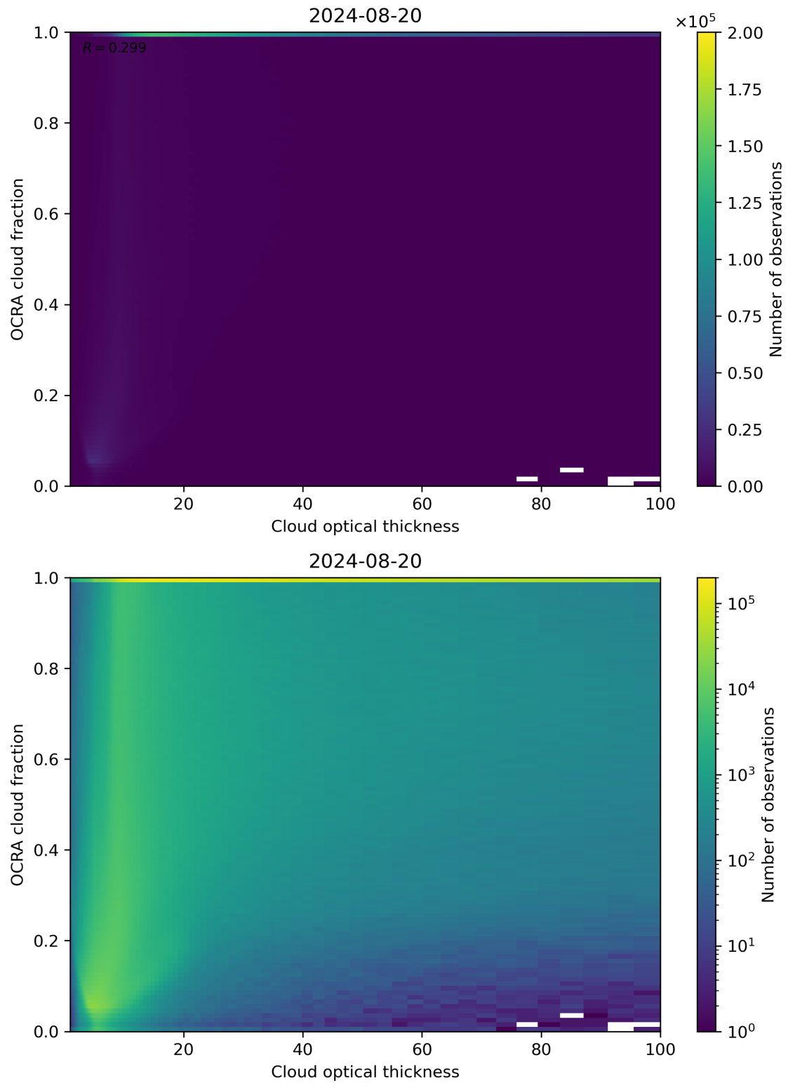
Figure 83: Scatter density plot of “Cloud optical thickness” against “OCRA cloud fraction” for 2024-08-19 to 2024-08-21.
