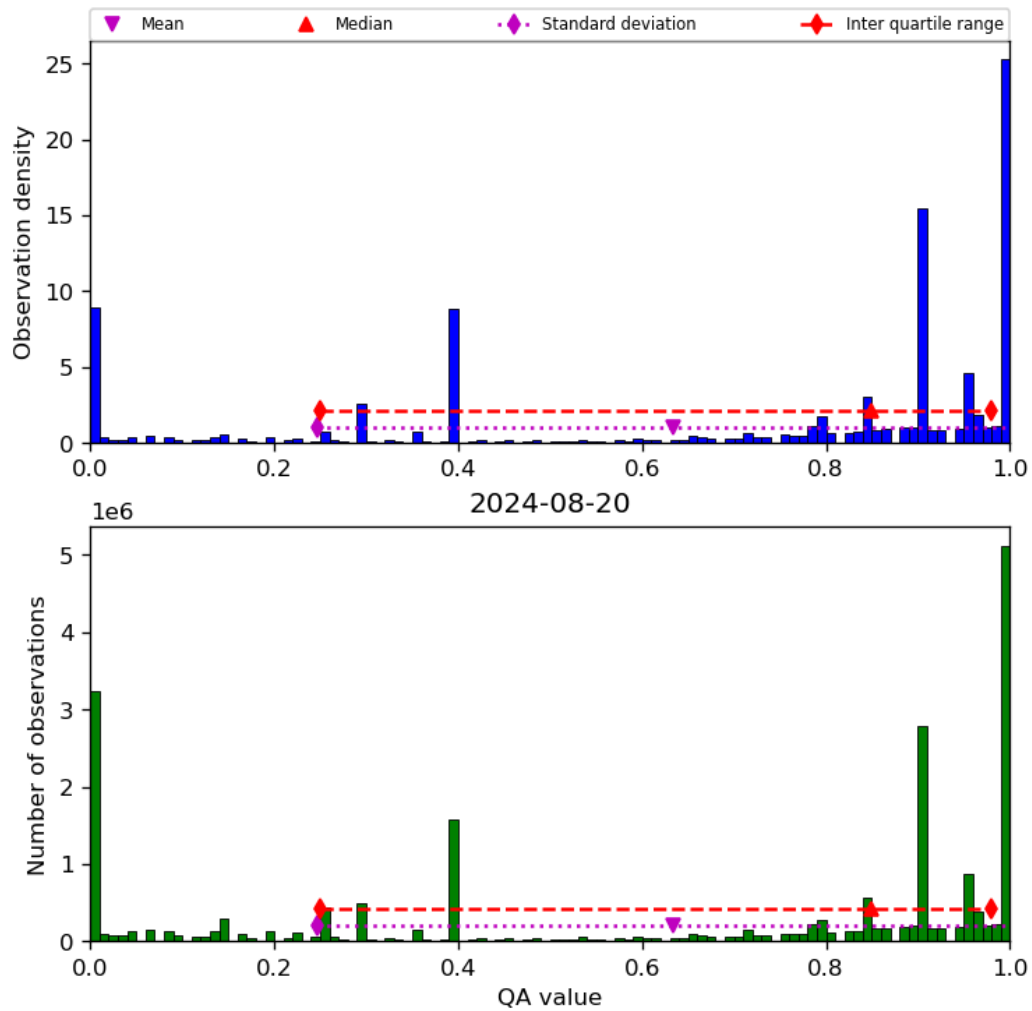
Figure 38: Histogram of “QA value” for 2024-08-19 to 2024-08-21
