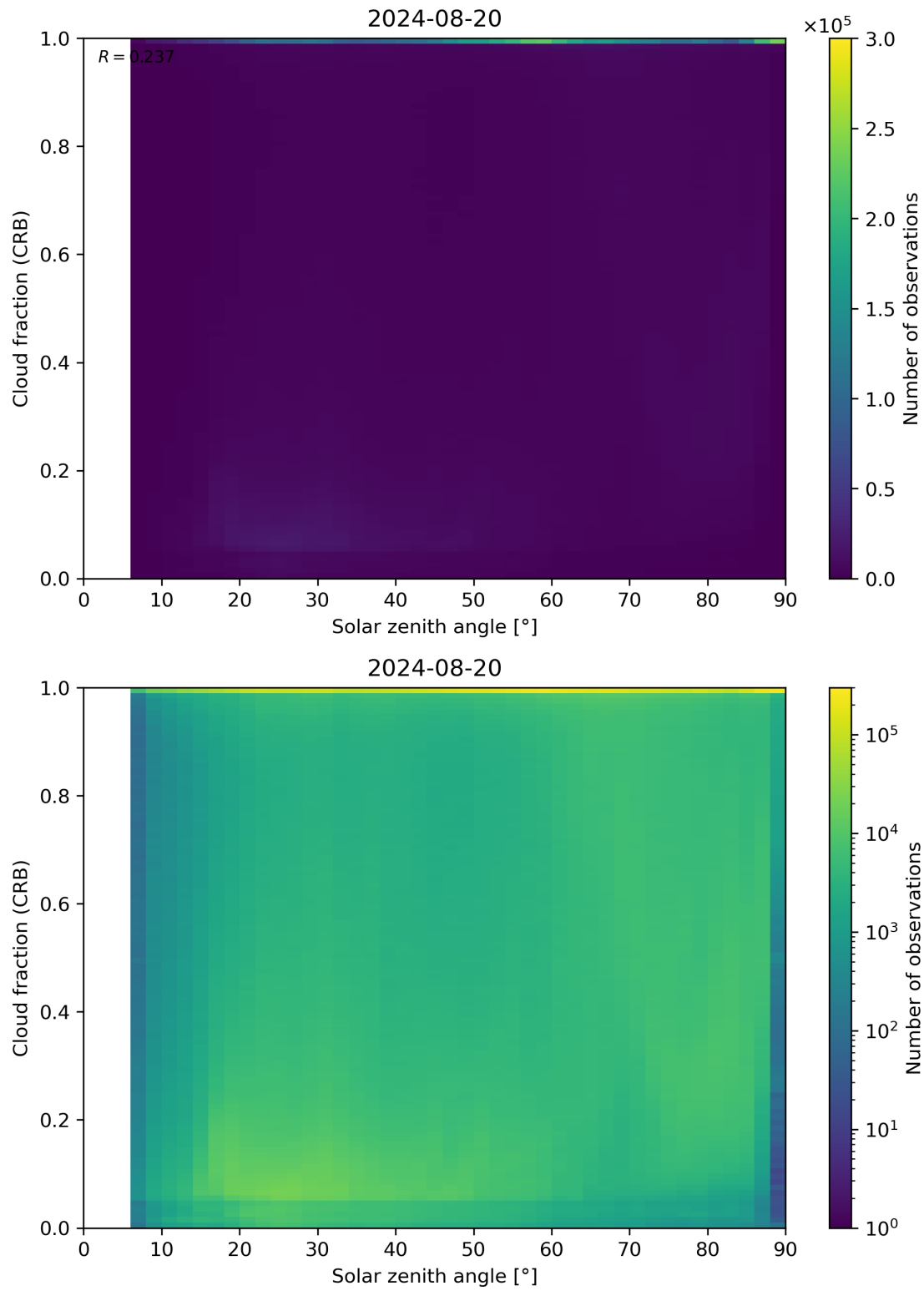
Figure 101: Scatter density plot of “Solar zenith angle” against “Cloud fraction (CRB)” for 2024-08-19 to 2024-08-21.
