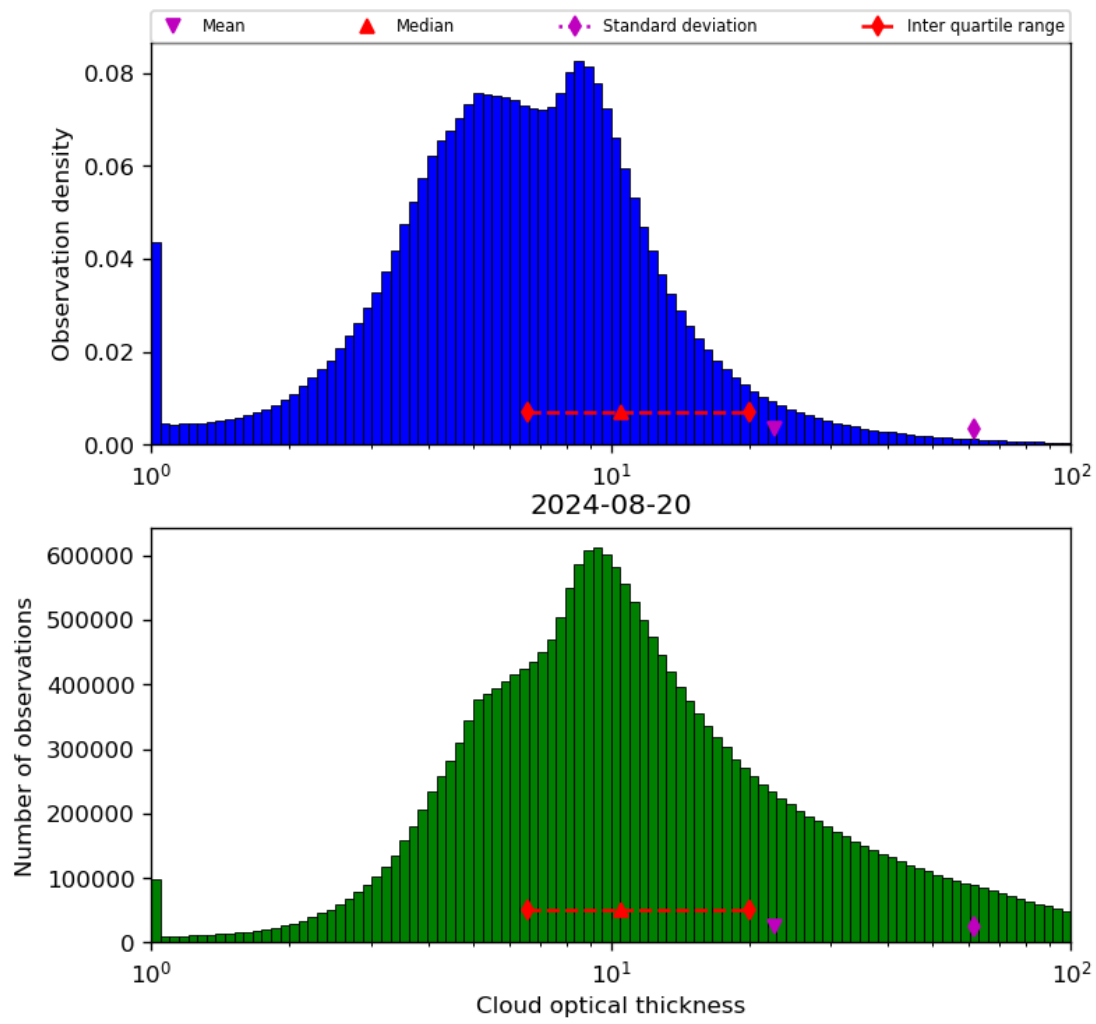
Figure 41: Histogram of “Cloud optical thickness” for 2024-08-19 to 2024-08-21
