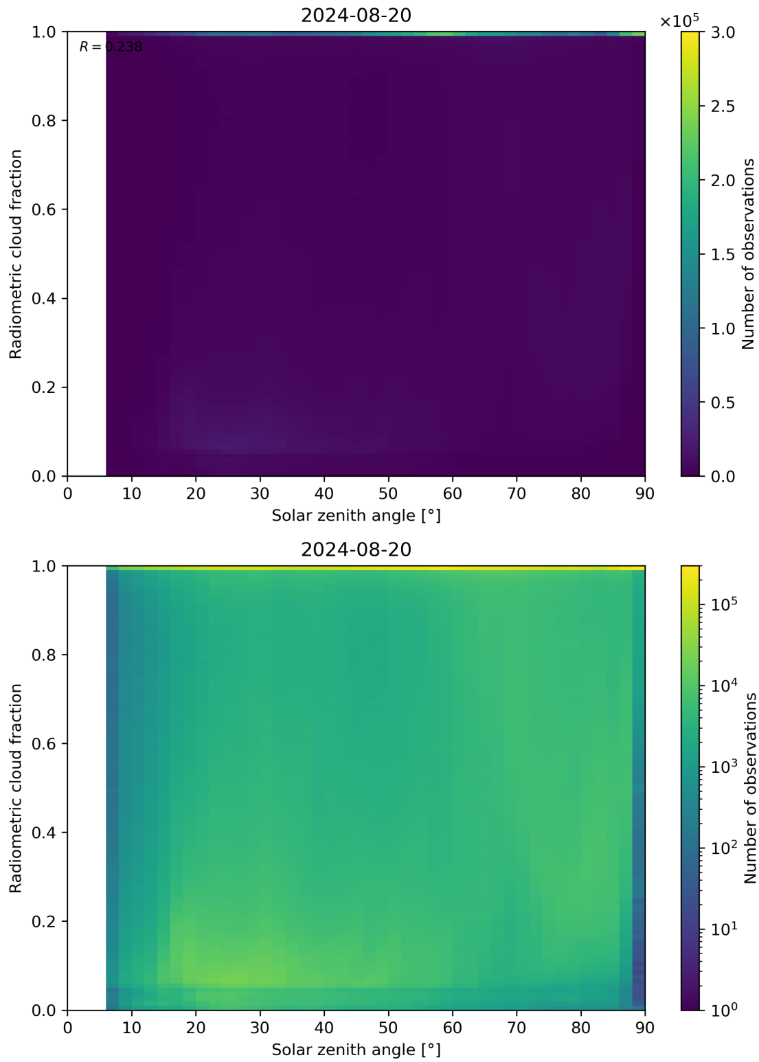
Figure 99: Scatter density plot of “Solar zenith angle” against “Radiometric cloud fraction” for 2024-08-19 to 2024-08-21.
