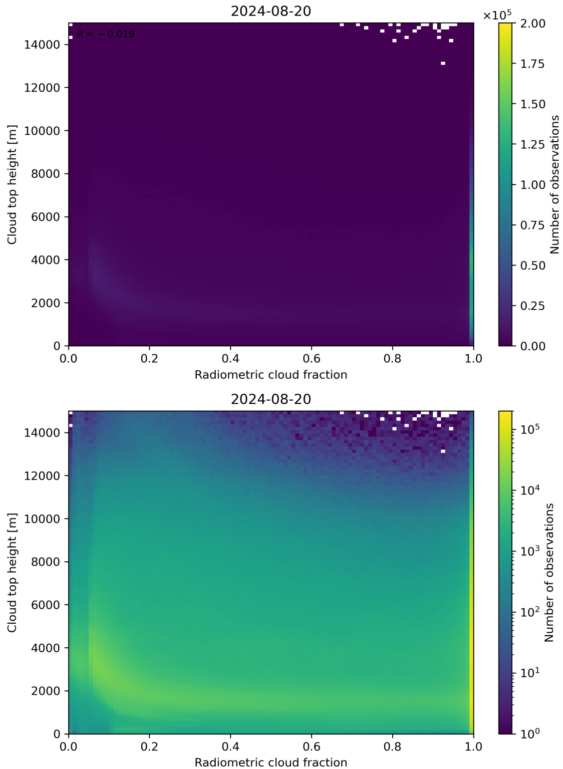
Figure 76: Scatter density plot of “Radiometric cloud fraction” against “Cloud top height” for 2024-08-19 to 2024-08-21.
