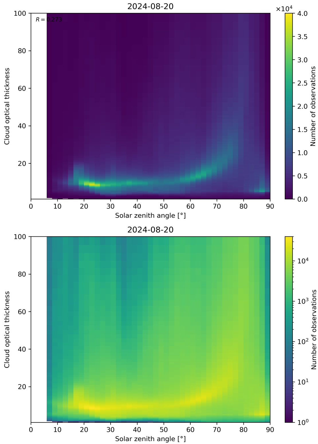
Figure 103: Scatter density plot of “Solar zenith angle” against “Cloud optical thickness” for 2024-08-19 to 2024-08-21.
