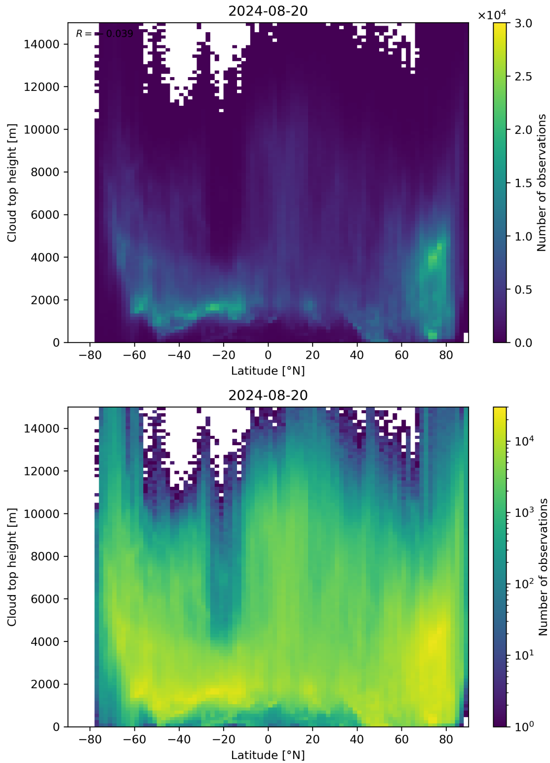
Figure 97: Scatter density plot of “Latitude” against “Cloud top height” for 2024-08-19 to 2024-08-21.
