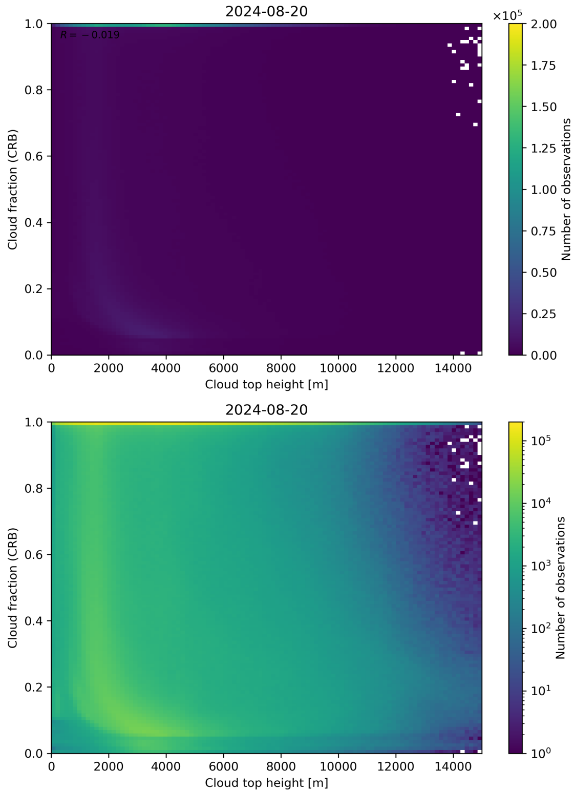
Figure 88: Scatter density plot of “Cloud top height” against “Cloud fraction (CRB)” for 2024-08-19 to 2024-08-21.
