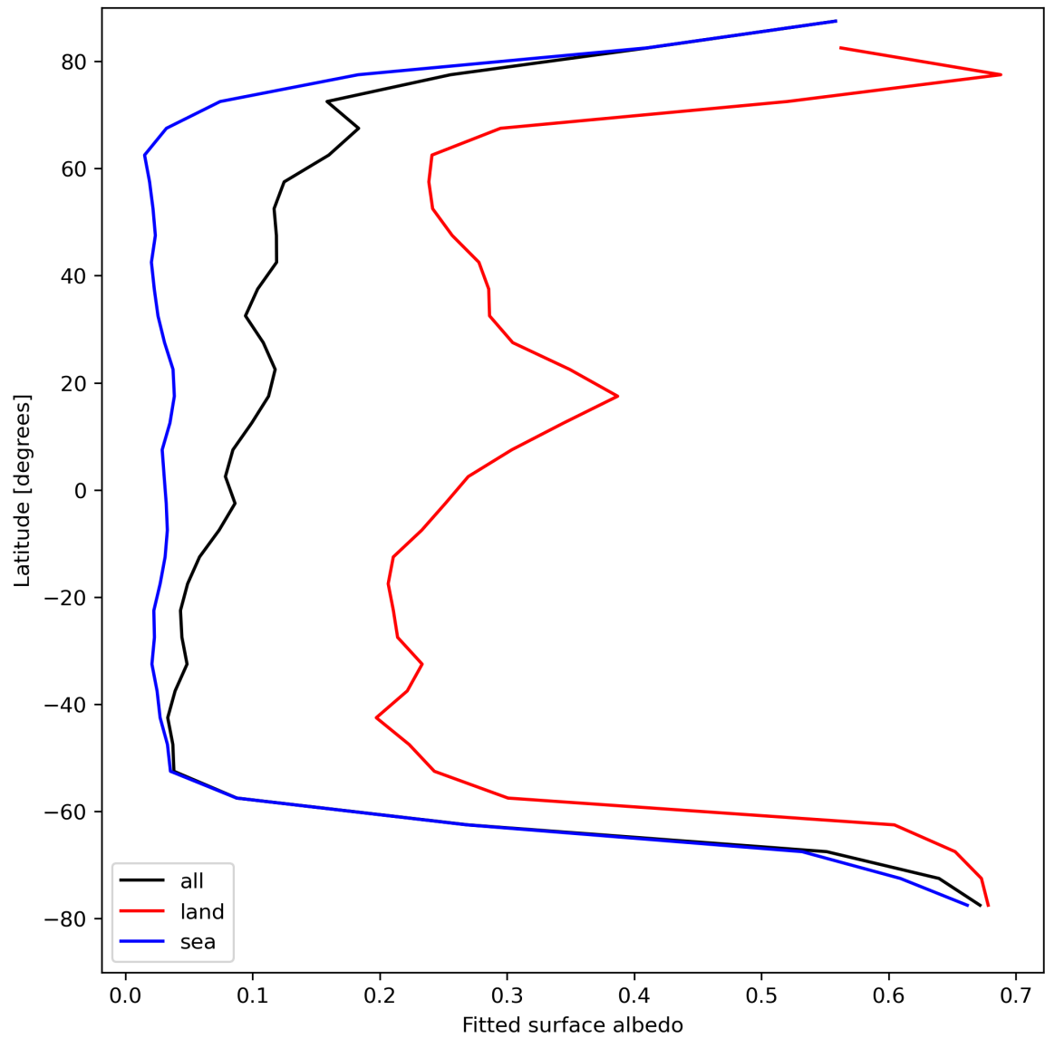
Figure 29: Zonal average of “Fitted surface albedo” for 2024-08-19 to 2024-08-21.
