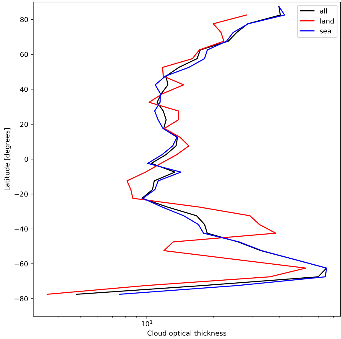
Figure 25: Zonal average of “Cloud optical thickness” for 2024-08-19 to 2024-08-21.
