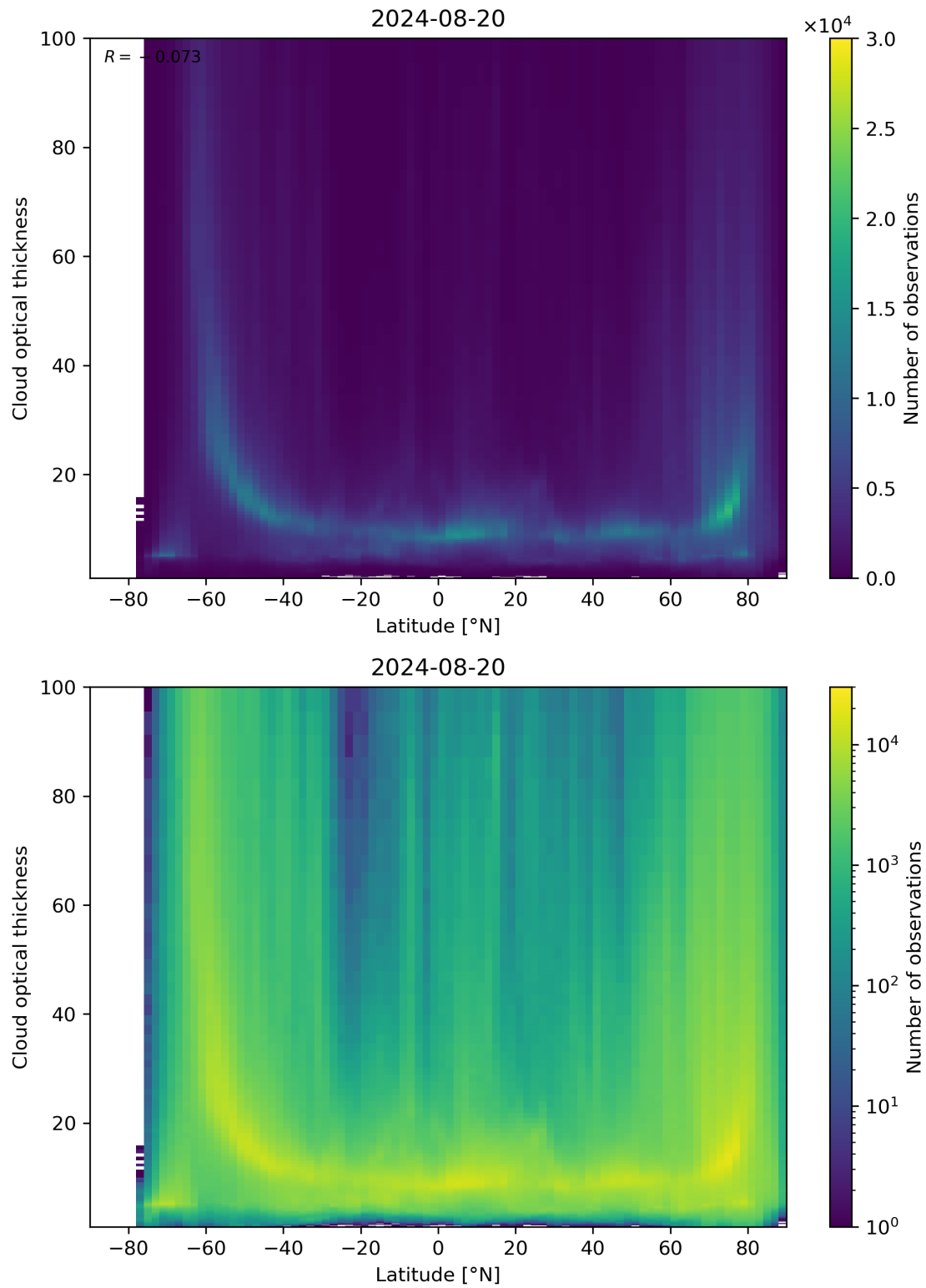
Figure 96: Scatter density plot of “Latitude” against “Cloud optical thickness” for 2024-08-19 to 2024-08-21.
