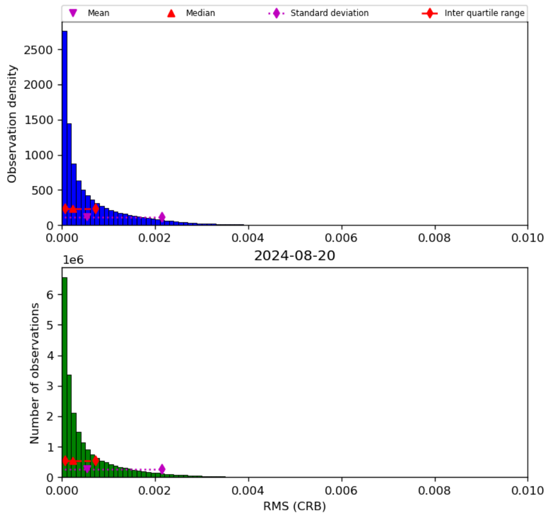
Figure 48: Histogram of “RMS (CRB)” for 2024-08-19 to 2024-08-21
