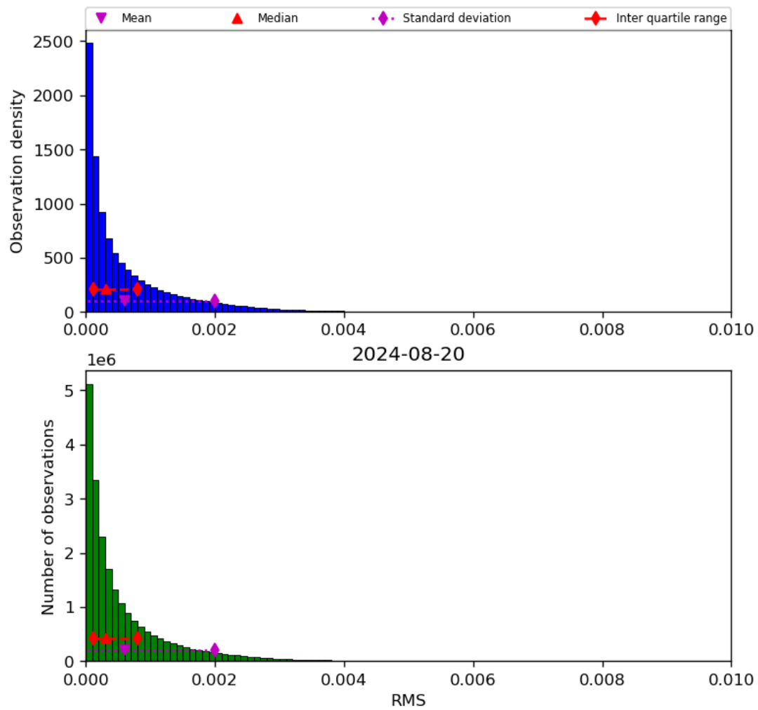
Figure 47: Histogram of “RMS” for 2024-08-19 to 2024-08-21
