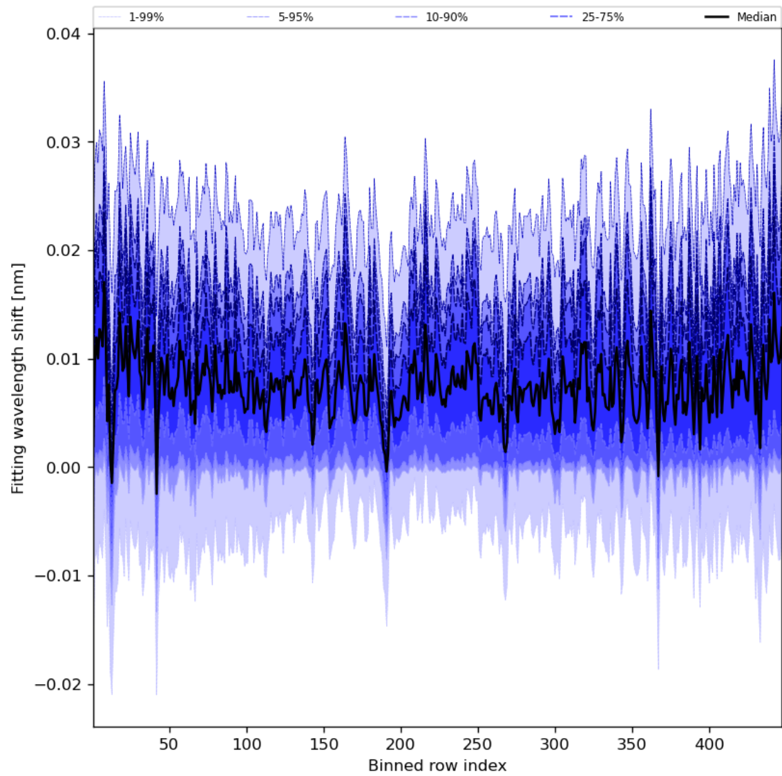
Figure 65: Along track statistics of “Fitting wavelength shift” for 2024-08-19 to 2024-08-21
