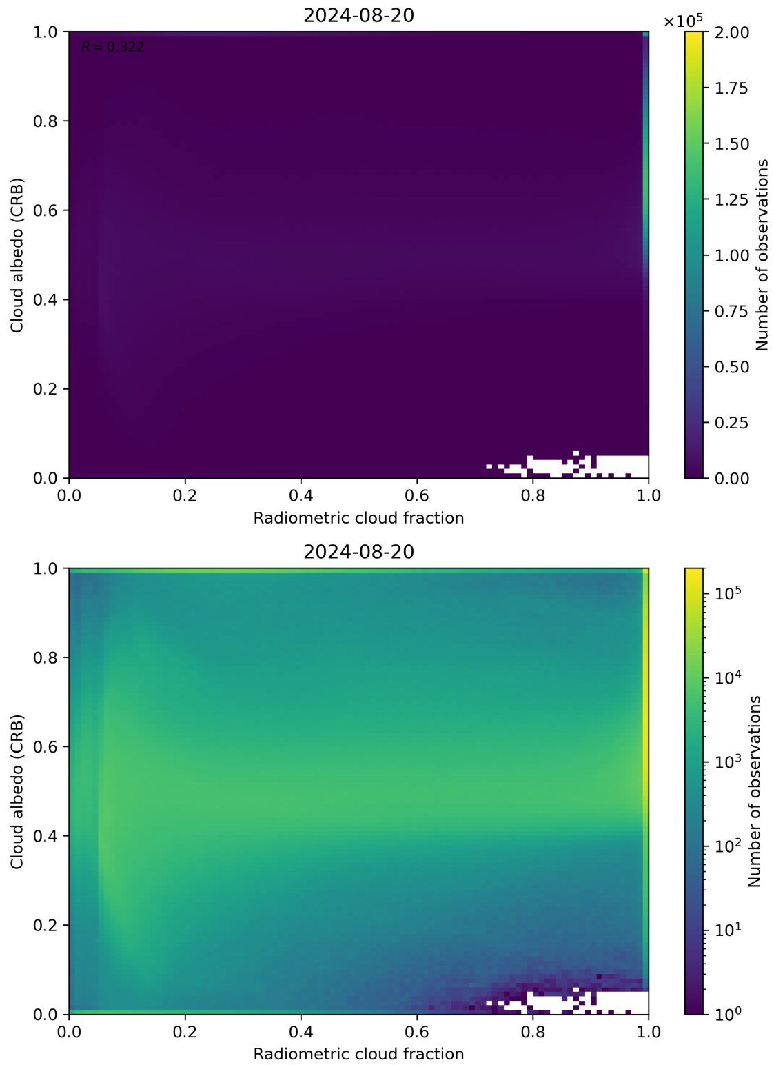
Figure 71: Scatter density plot of “Radiometric cloud fraction” against “Cloud albedo (CRB)” for 2024-08-19 to 2024-08-21.
