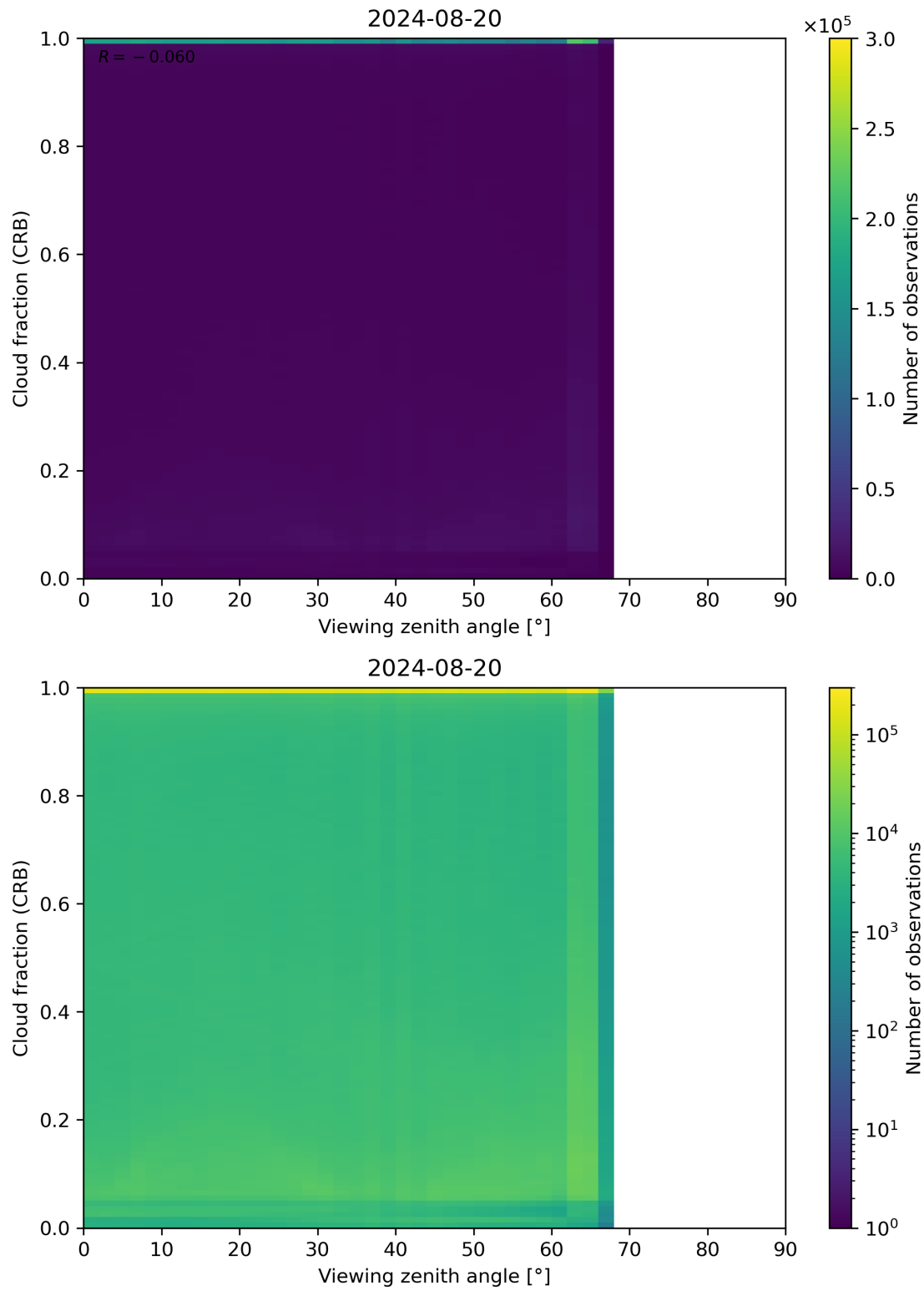
Figure 109: Scatter density plot of “Viewing zenith angle” against “Cloud fraction (CRB)” for 2024-08-19 to 2024-08-21.
