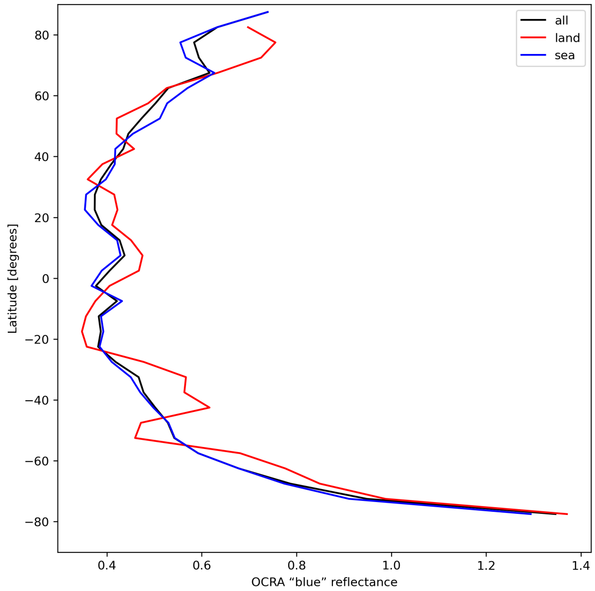
Figure 35: Zonal average of “OCRA “blue” reflectance” for 2024-08-19 to 2024-08-21.
