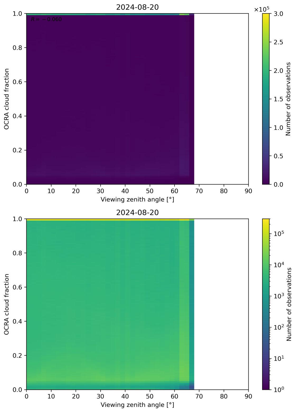
Figure 108: Scatter density plot of “Viewing zenith angle” against “OCRA cloud fraction” for 2024-08-19 to 2024-08-21.
