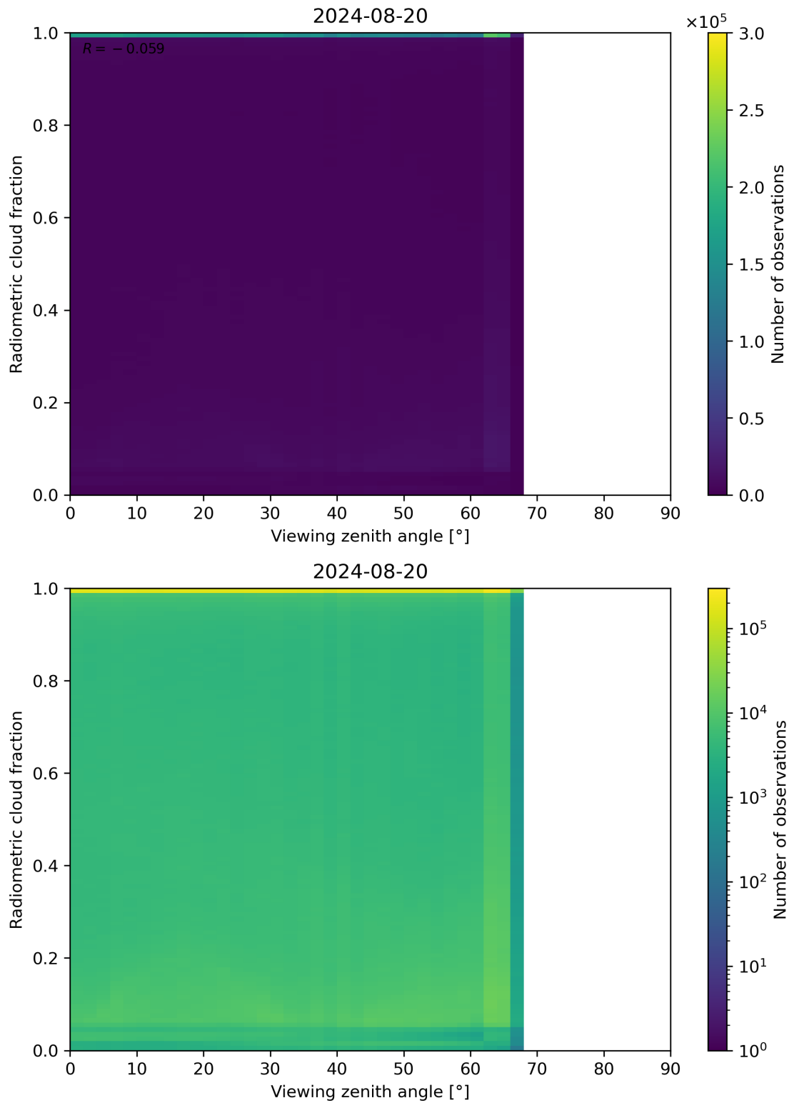
Figure 107: Scatter density plot of “Viewing zenith angle” against “Radiometric cloud fraction” for 2024-08-19 to 2024-08-21.
