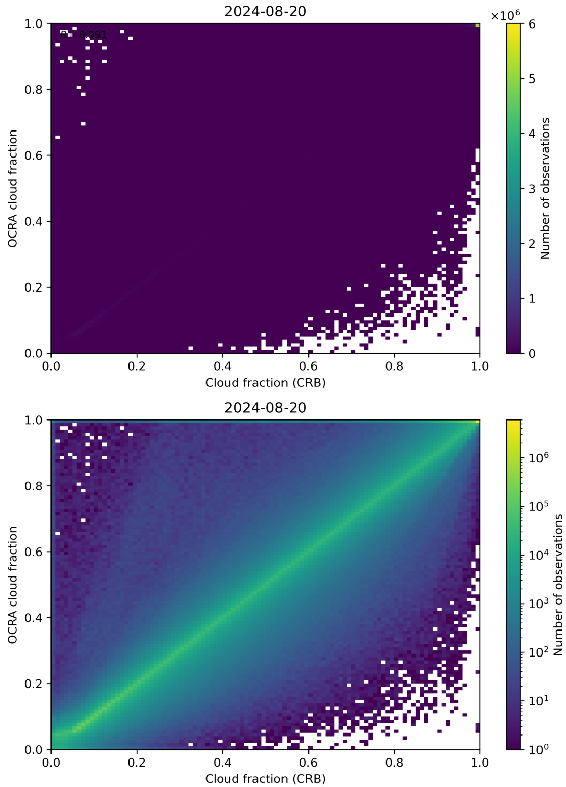
Figure 78: Scatter density plot of “Cloud fraction (CRB)” against “OCRA cloud fraction” for 2024-08-19 to 2024-08-21.
