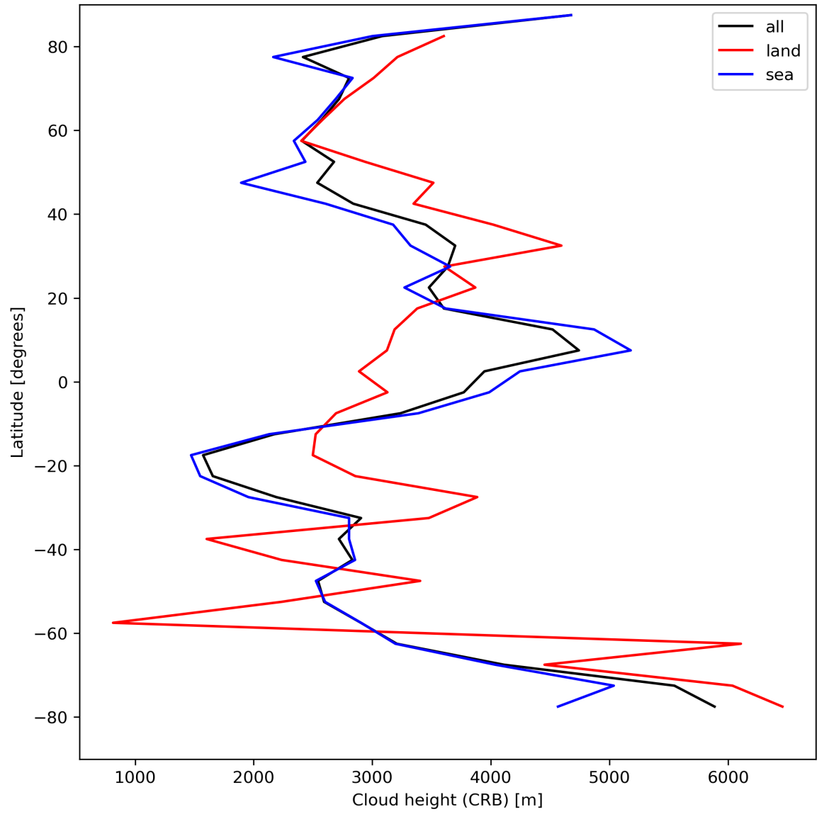
Figure 27: Zonal average of “Cloud height (CRB)” for 2024-08-21 to 2024-08-22.
