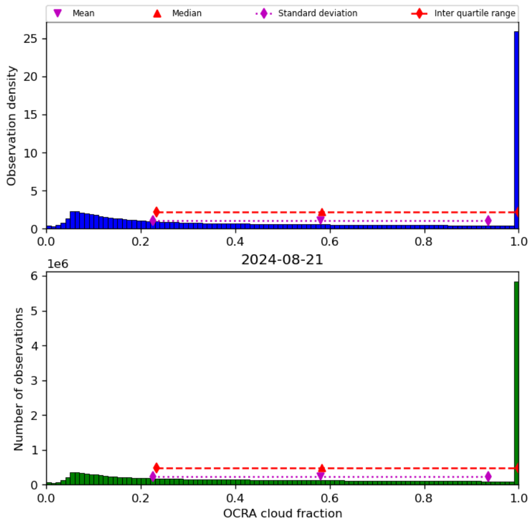
Figure 50: Histogram of “OCRA cloud fraction” for 2024-08-21 to 2024-08-22
