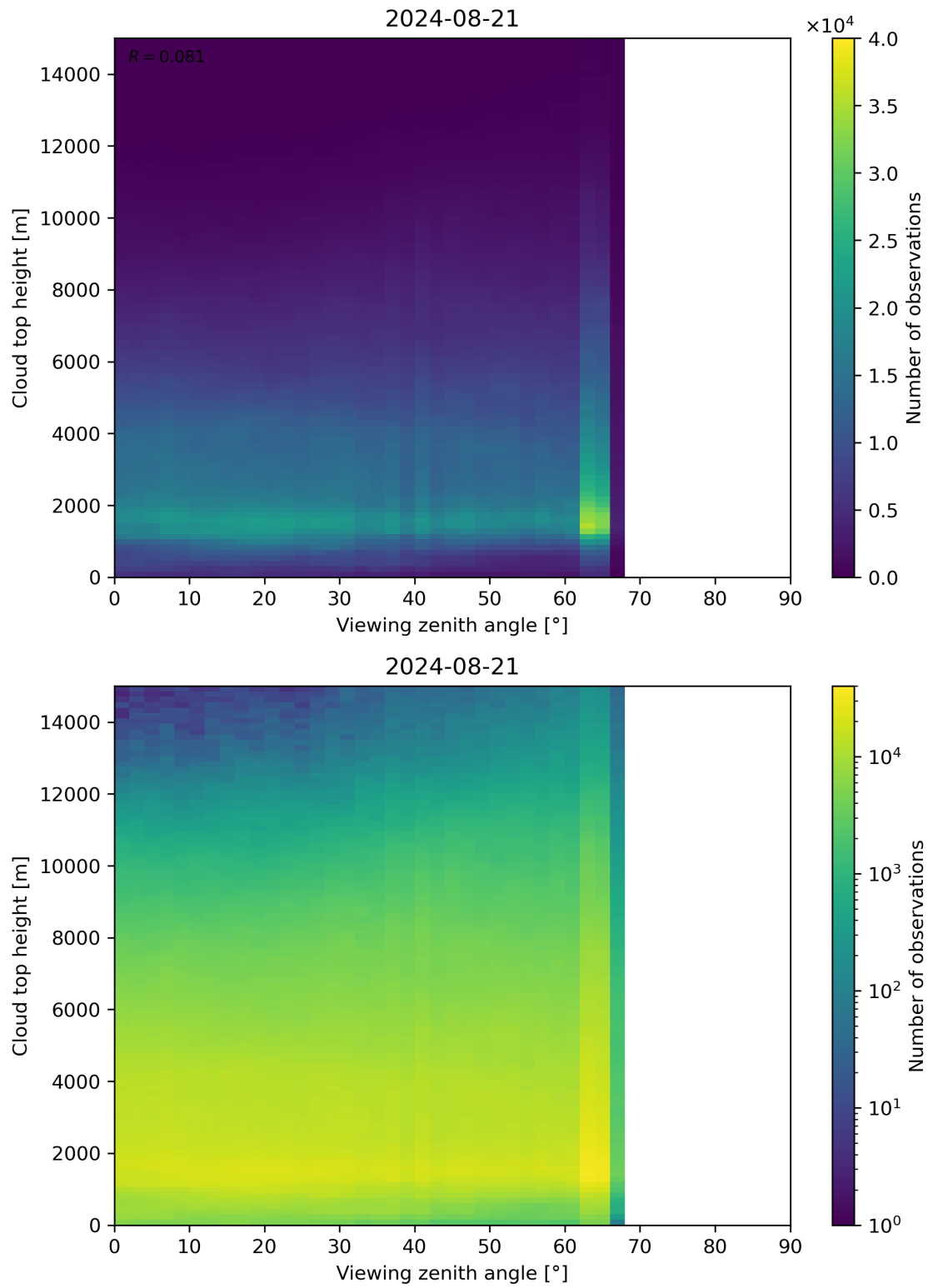
Figure 112: Scatter density plot of “Viewing zenith angle” against “Cloud top height” for 2024-08-21 to 2024-08-22.
