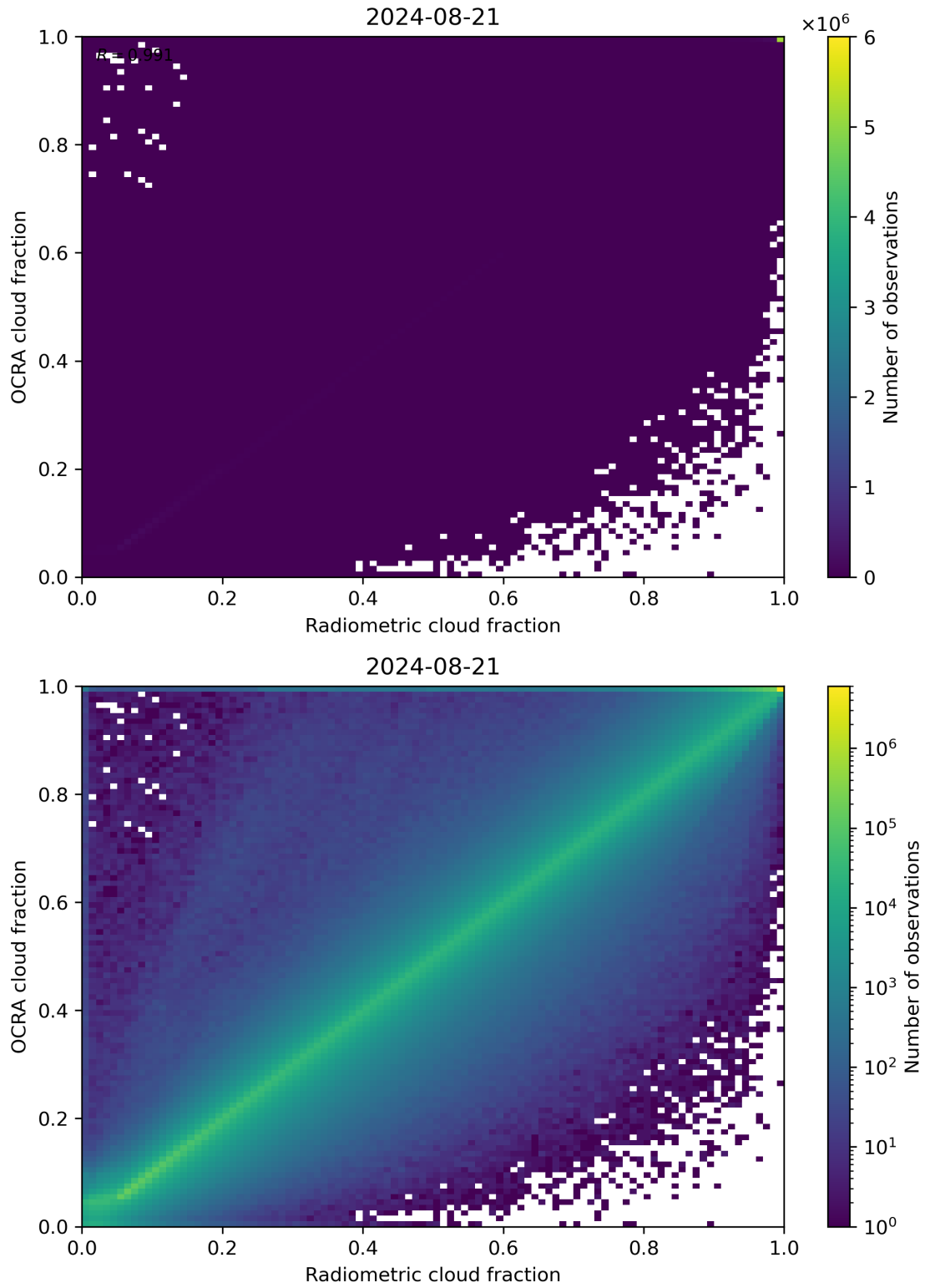
Figure 72: Scatter density plot of “Radiometric cloud fraction” against “OCRA cloud fraction” for 2024-08-21 to 2024-08-22.
