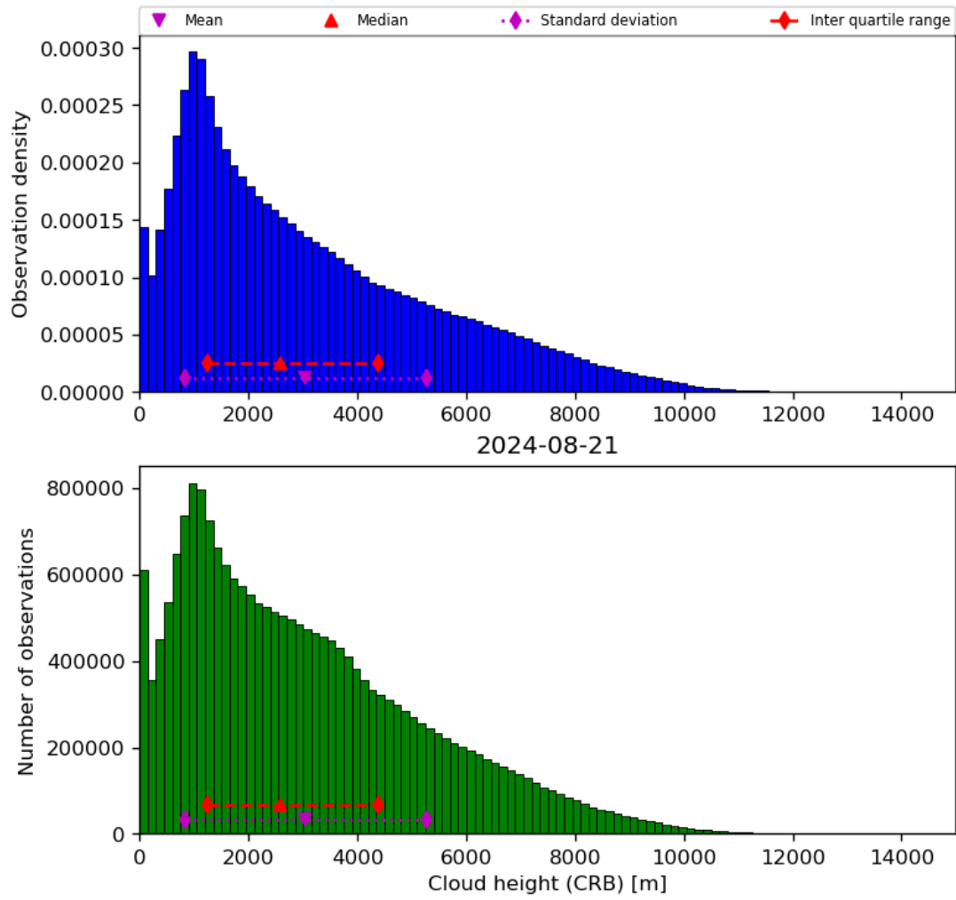
Figure 43: Histogram of “Cloud height (CRB)” for 2024-08-21 to 2024-08-22
