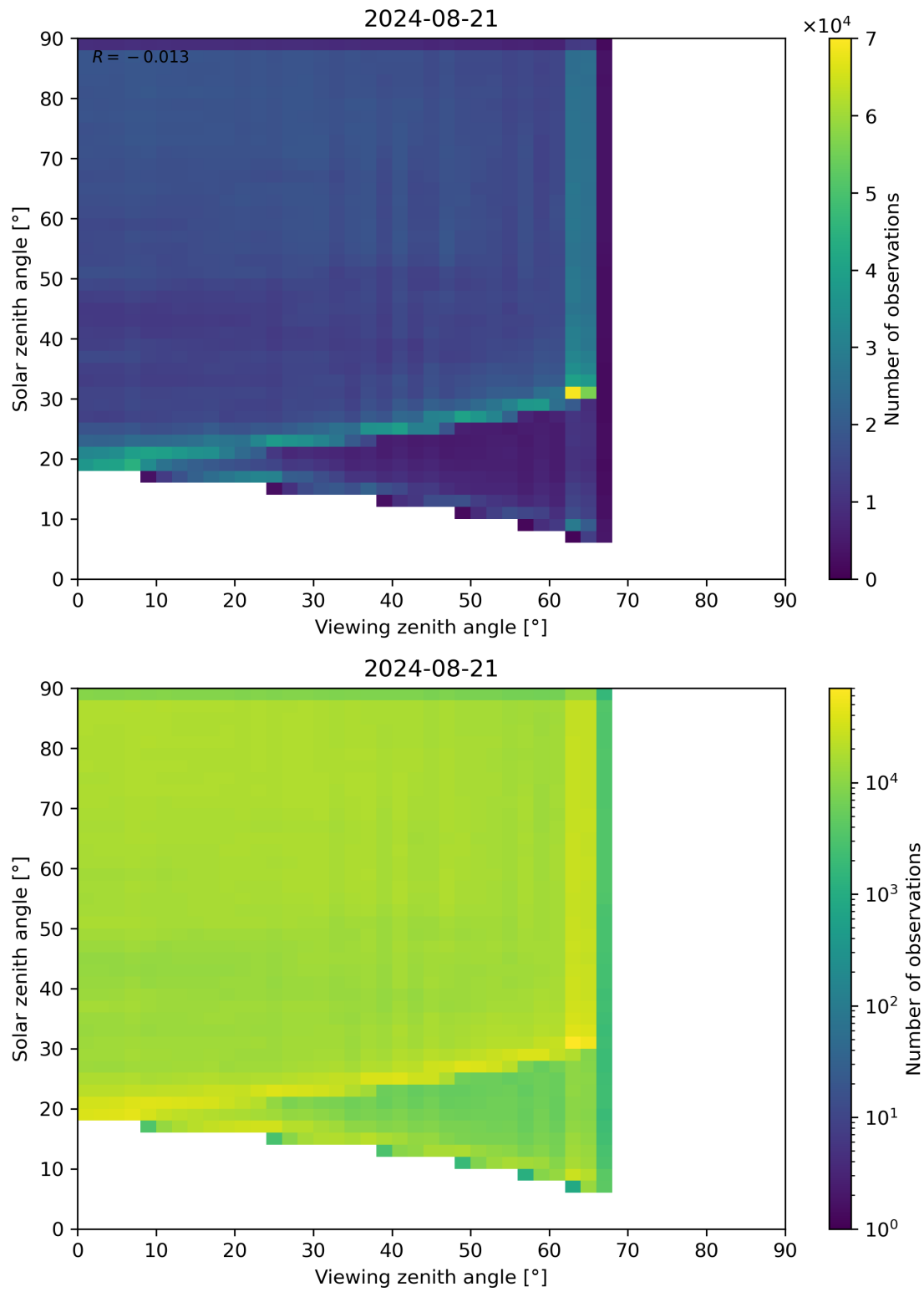
Figure 114: Scatter density plot of “Viewing zenith angle” against “Solar zenith angle” for 2024-08-21 to 2024-08-22.
