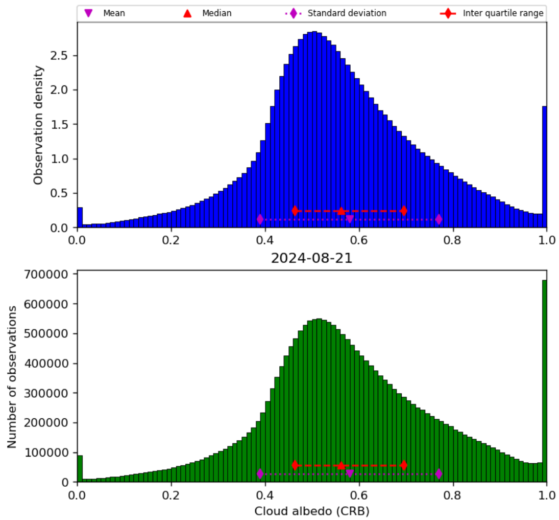
Figure 44: Histogram of “Cloud albedo (CRB)” for 2024-08-21 to 2024-08-22
