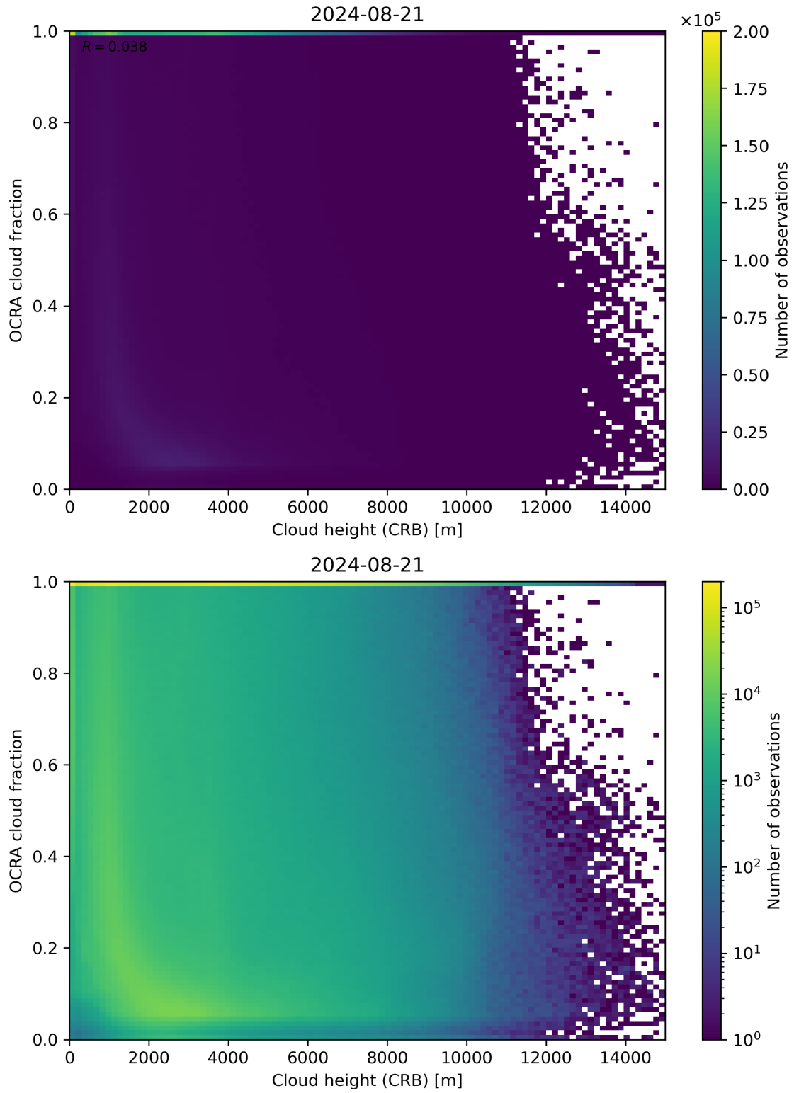
Figure 81: Scatter density plot of “Cloud height (CRB)” against “OCRA cloud fraction” for 2024-08-21 to 2024-08-22.
