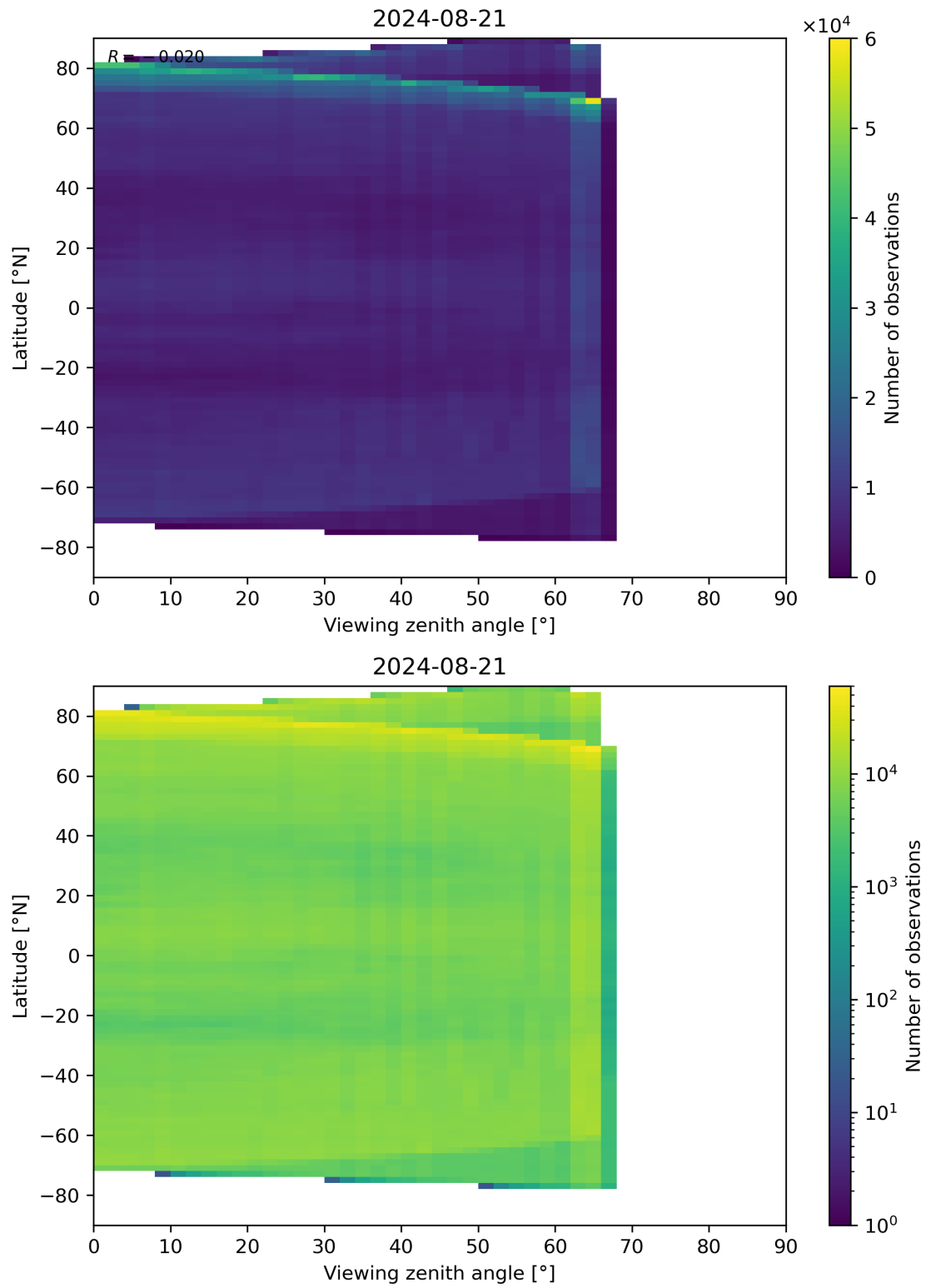
Figure 113: Scatter density plot of “Viewing zenith angle” against “Latitude” for 2024-08-21 to 2024-08-22.
