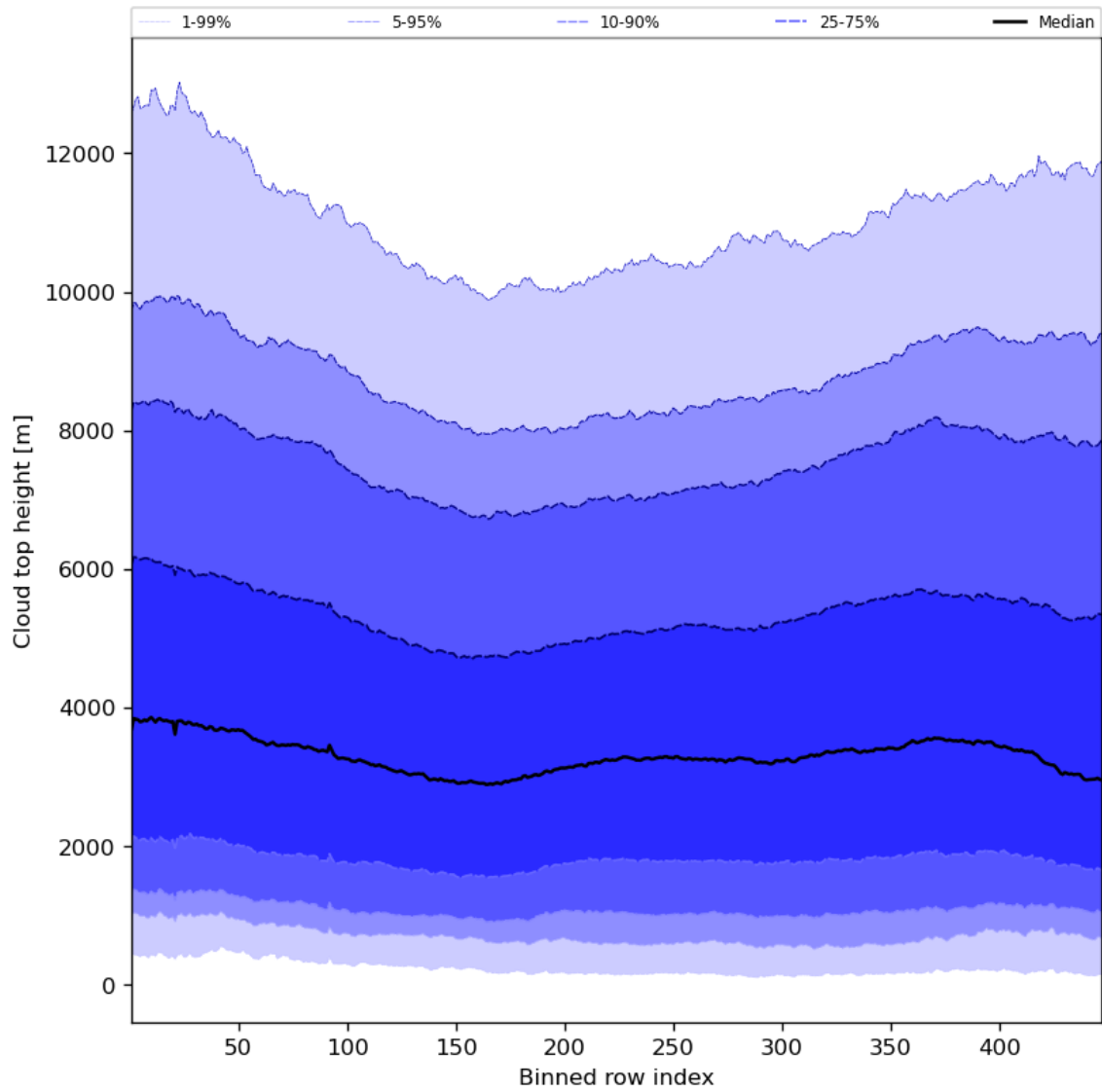
Figure 56: Along track statistics of “Cloud top height” for 2024-08-21 to 2024-08-22
