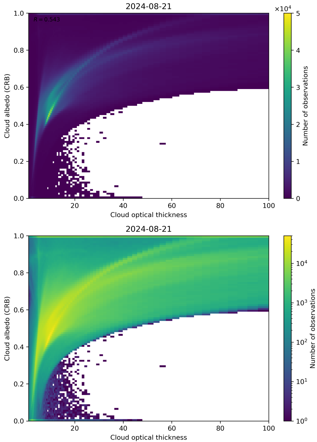
Figure 82: Scatter density plot of “Cloud optical thickness” against “Cloud albedo (CRB)” for 2024-08-21 to 2024-08-22.
