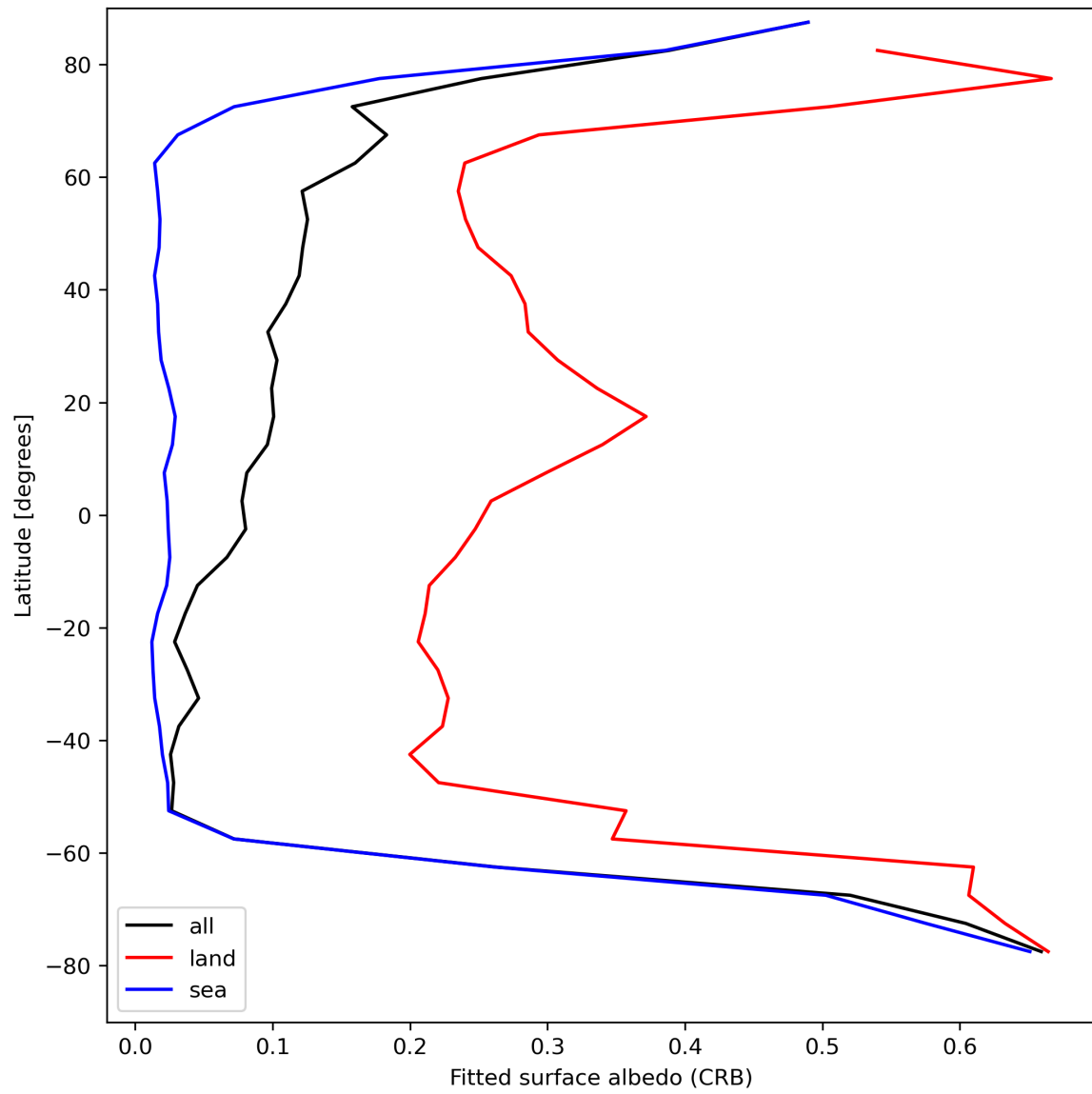
Figure 30: Zonal average of “Fitted surface albedo (CRB)” for 2024-08-21 to 2024-08-22.
