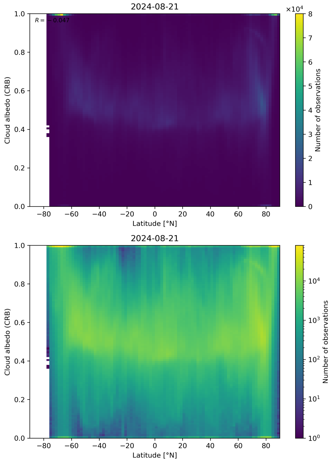
Figure 91: Scatter density plot of “Latitude” against “Cloud albedo (CRB)” for 2024-08-21 to 2024-08-22.
