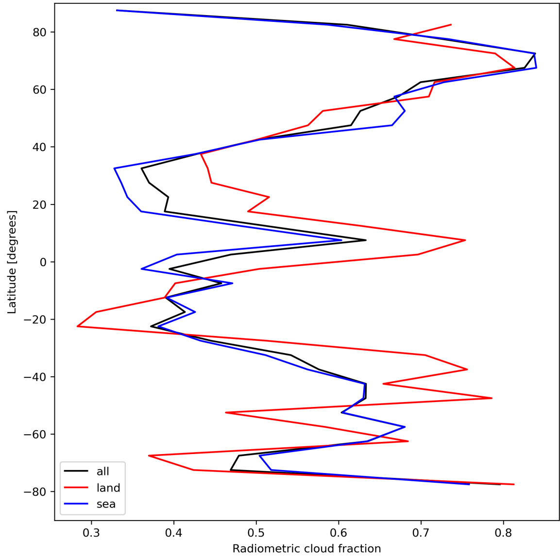
Figure 23: Zonal average of “Radiometric cloud fraction” for 2024-08-21 to 2024-08-22.
