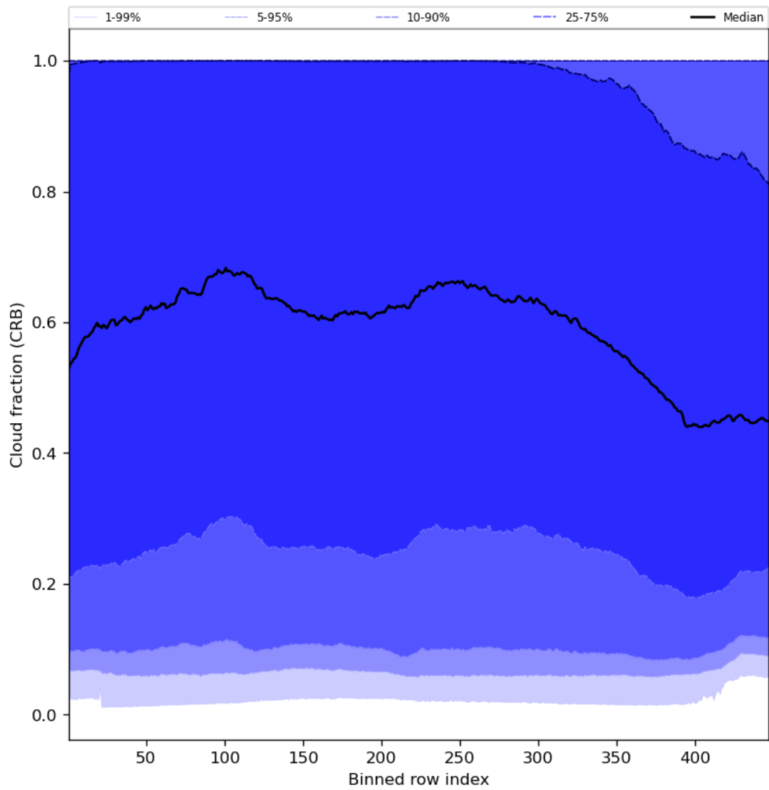
Figure 58: Along track statistics of “Cloud fraction (CRB)” for 2024-08-21 to 2024-08-22
