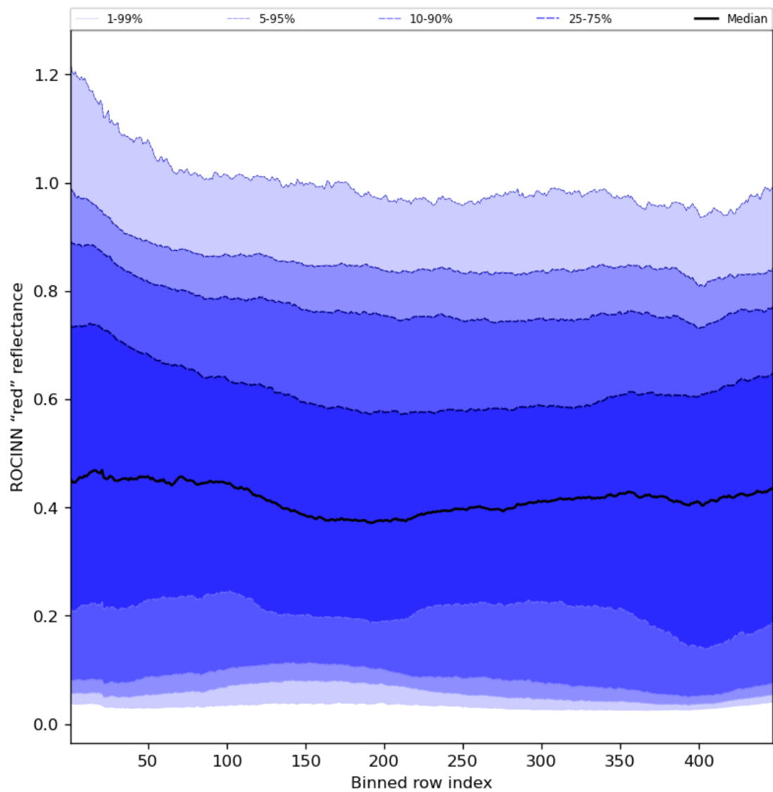
Figure 69: Along track statistics of “ROCINN “red” reflectance” for 2024-08-21 to 2024-08-22
