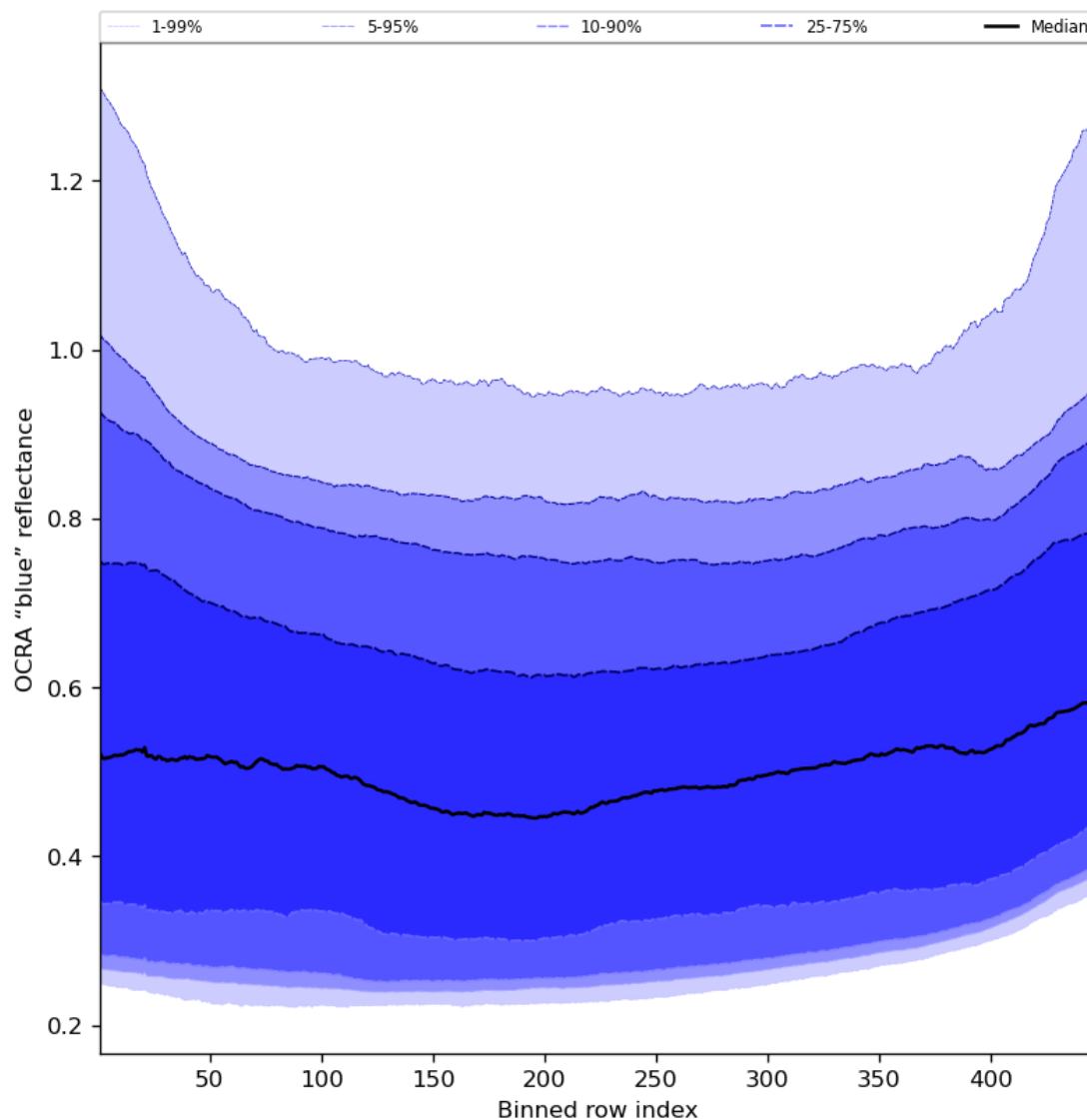
Figure 67: Along track statistics of “OCRA “blue” reflectance” for 2024-08-21 to 2024-08-22
