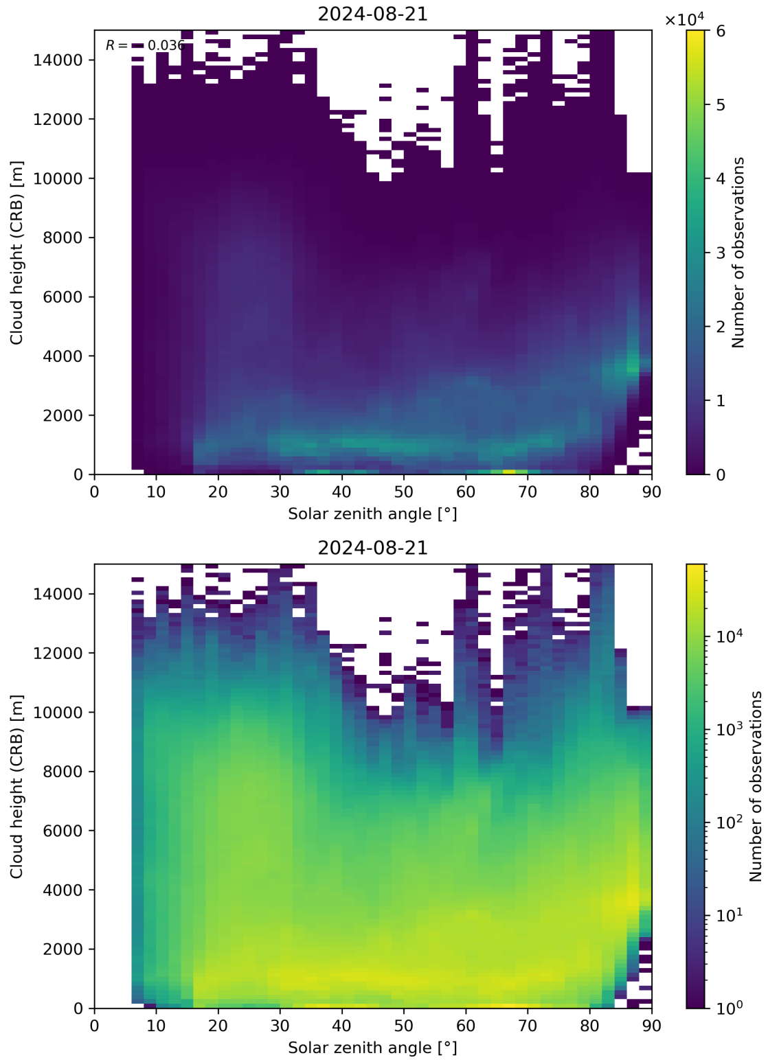
Figure 102: Scatter density plot of “Solar zenith angle” against “Cloud height (CRB)” for 2024-08-21 to 2024-08-22.
