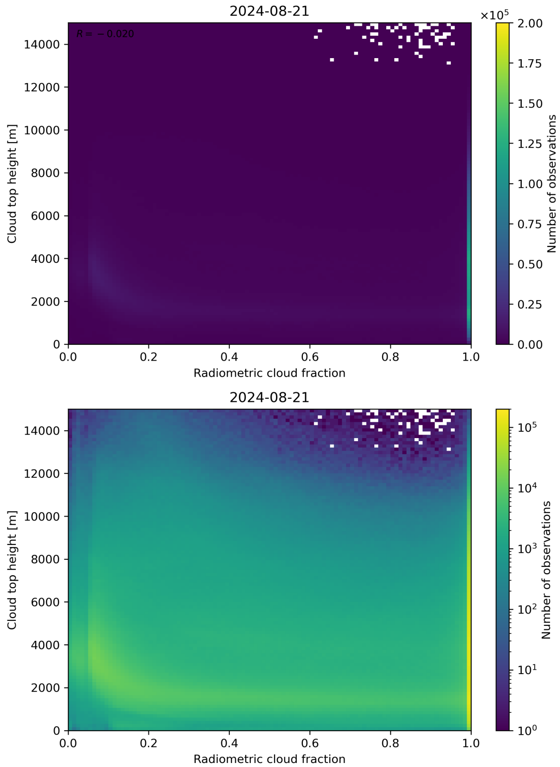
Figure 76: Scatter density plot of “Radiometric cloud fraction” against “Cloud top height” for 2024-08-21 to 2024-08-22.
