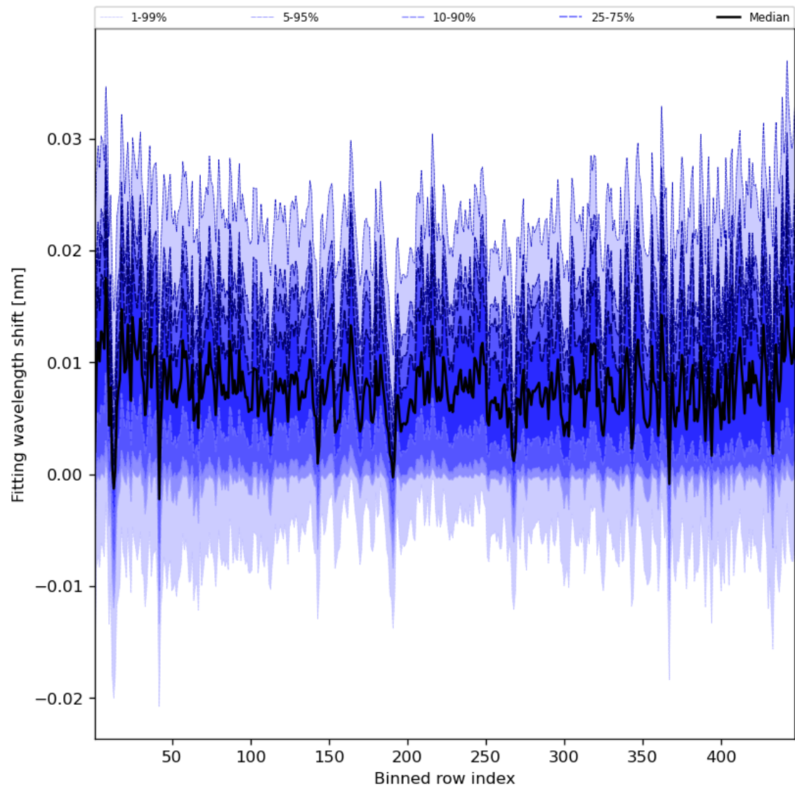
Figure 65: Along track statistics of “Fitting wavelength shift” for 2024-08-21 to 2024-08-22
