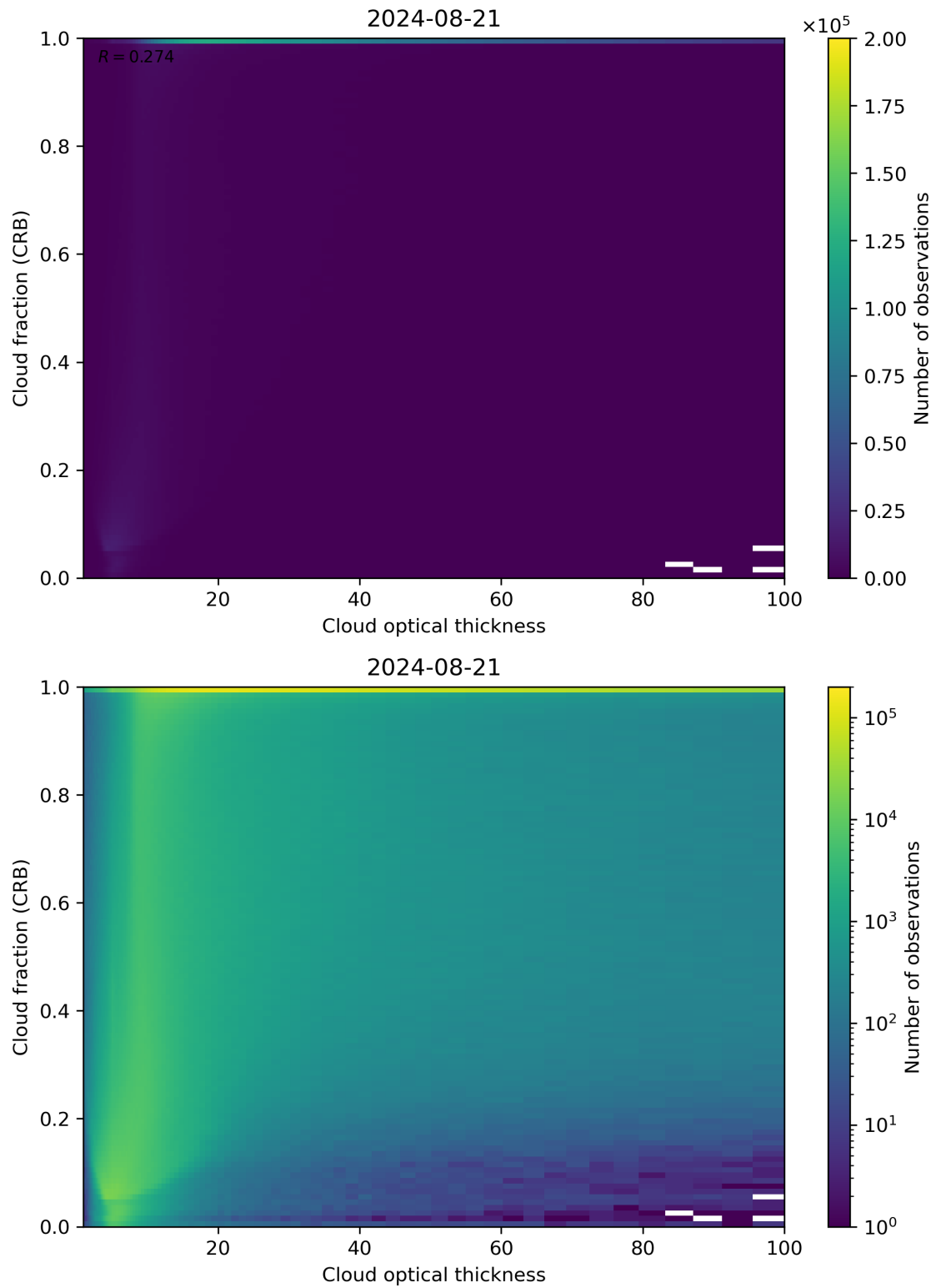
Figure 84: Scatter density plot of “Cloud optical thickness” against “Cloud fraction (CRB)” for 2024-08-21 to 2024-08-22.
