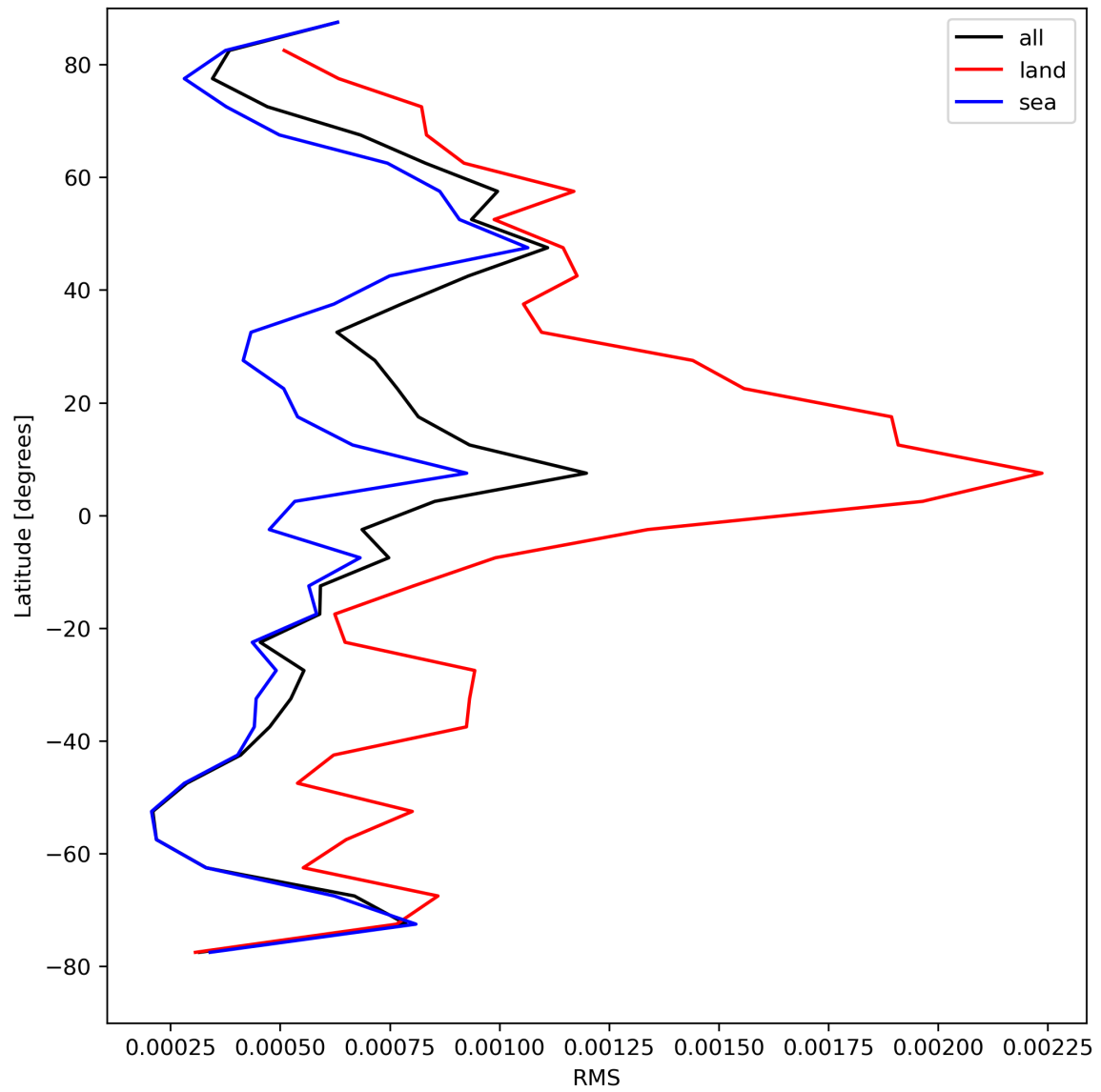
Figure 31: Zonal average of “RMS” for 2024-08-21 to 2024-08-22.
