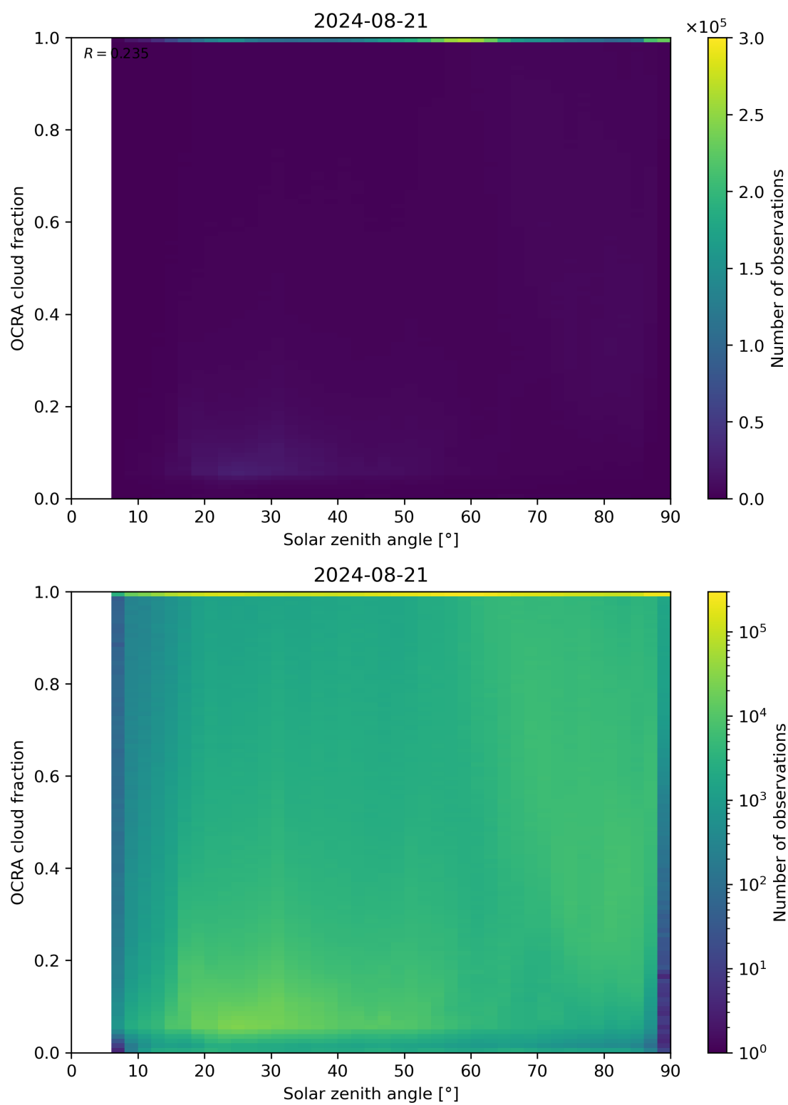
Figure 100: Scatter density plot of “Solar zenith angle” against “OCRA cloud fraction” for 2024-08-21 to 2024-08-22.
