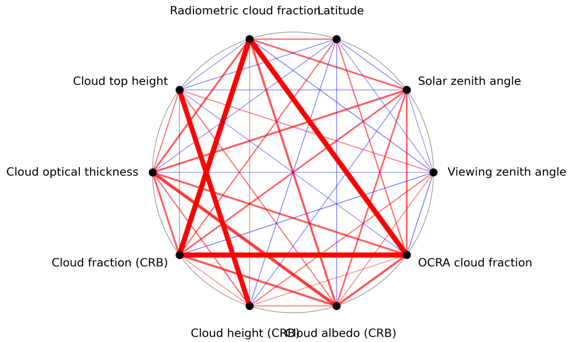
Figure 1: Map of correlation graph for 2024-08-21 to 2024-08-22.
