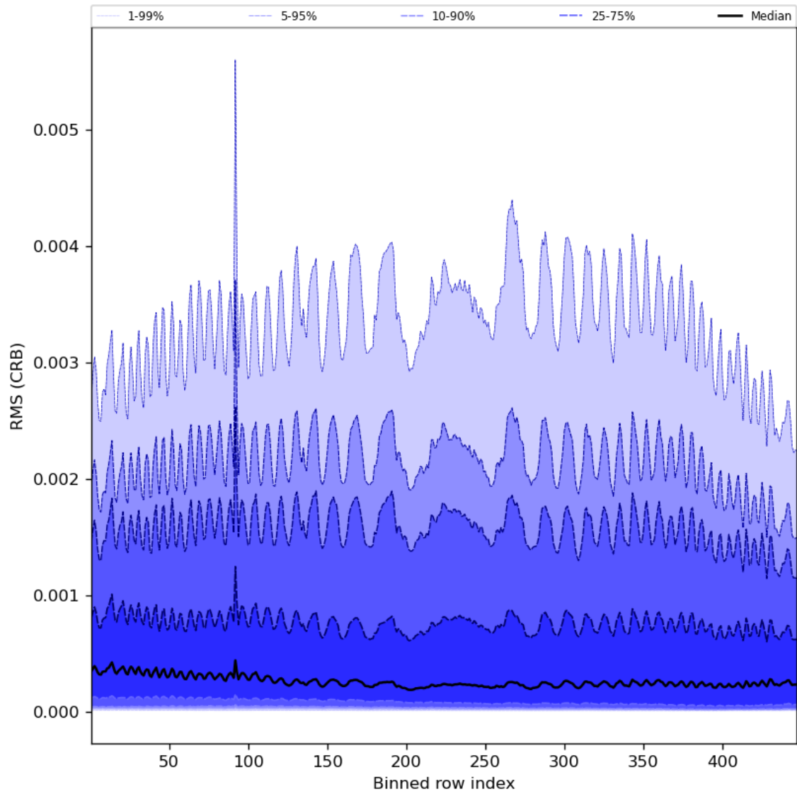
Figure 64: Along track statistics of “RMS (CRB)” for 2024-08-21 to 2024-08-22
