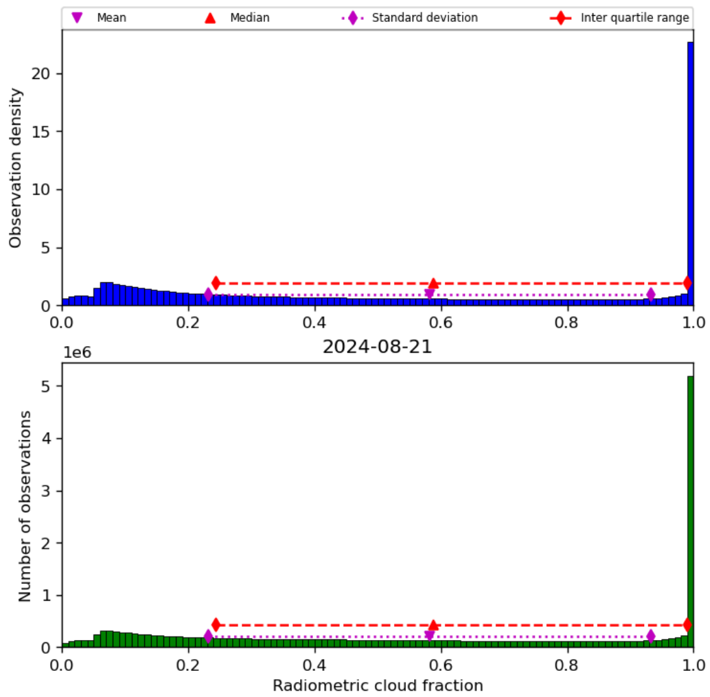
Figure 39: Histogram of “Radiometric cloud fraction” for 2024-08-21 to 2024-08-22
