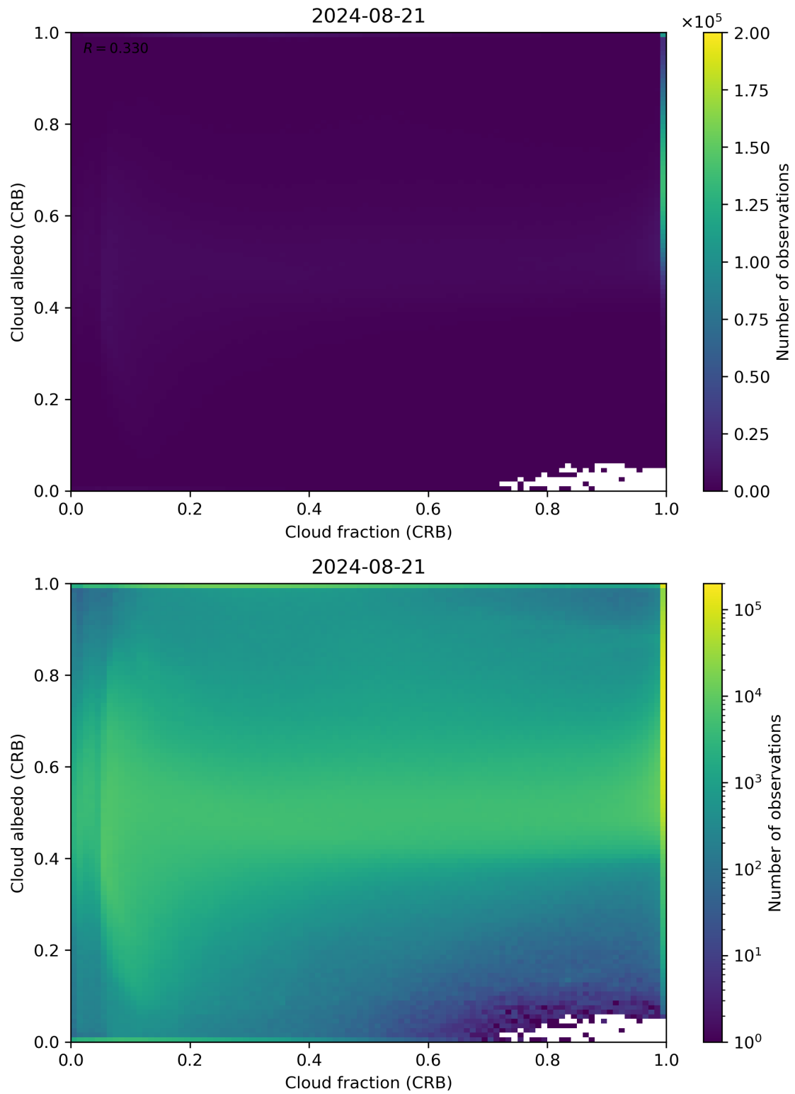
Figure 77: Scatter density plot of “Cloud fraction (CRB)” against “Cloud albedo (CRB)” for 2024-08-21 to 2024-08-22.
