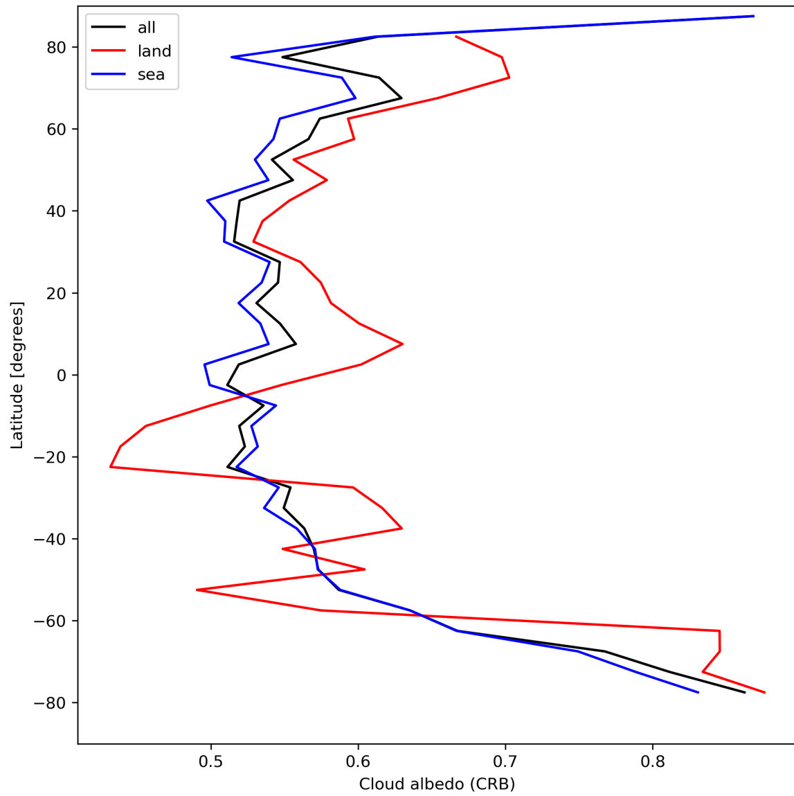
Figure 28: Zonal average of “Cloud albedo (CRB)” for 2024-08-21 to 2024-08-22.
