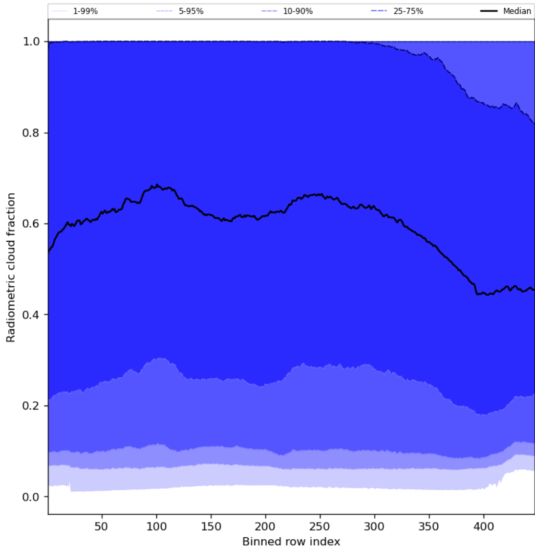
Figure 55: Along track statistics of “Radiometric cloud fraction” for 2024-08-21 to 2024-08-22
