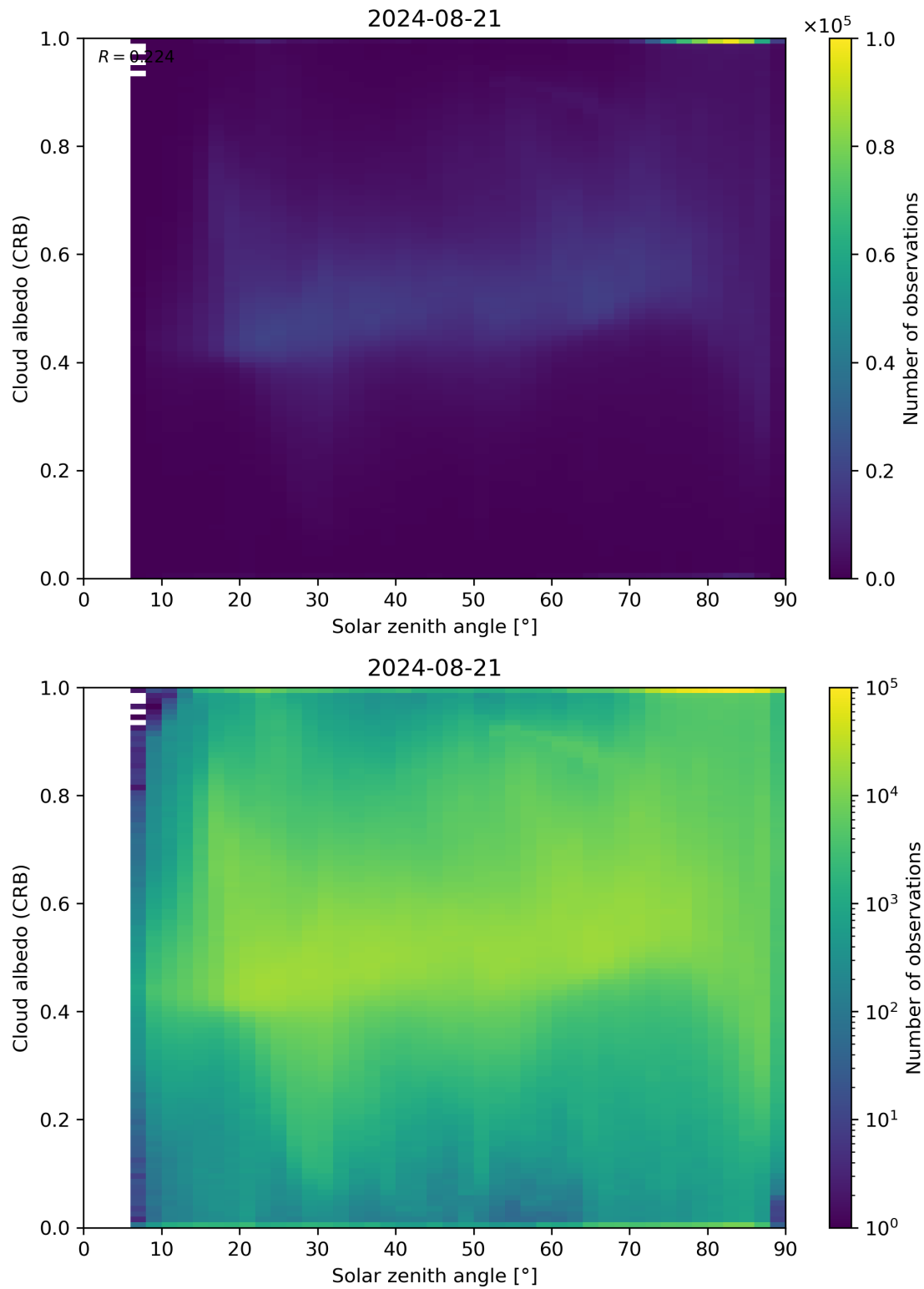
Figure 98: Scatter density plot of “Solar zenith angle” against “Cloud albedo (CRB)” for 2024-08-21 to 2024-08-22.
