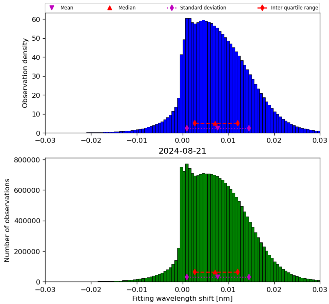
Figure 49: Histogram of “Fitting wavelength shift” for 2024-08-21 to 2024-08-22
