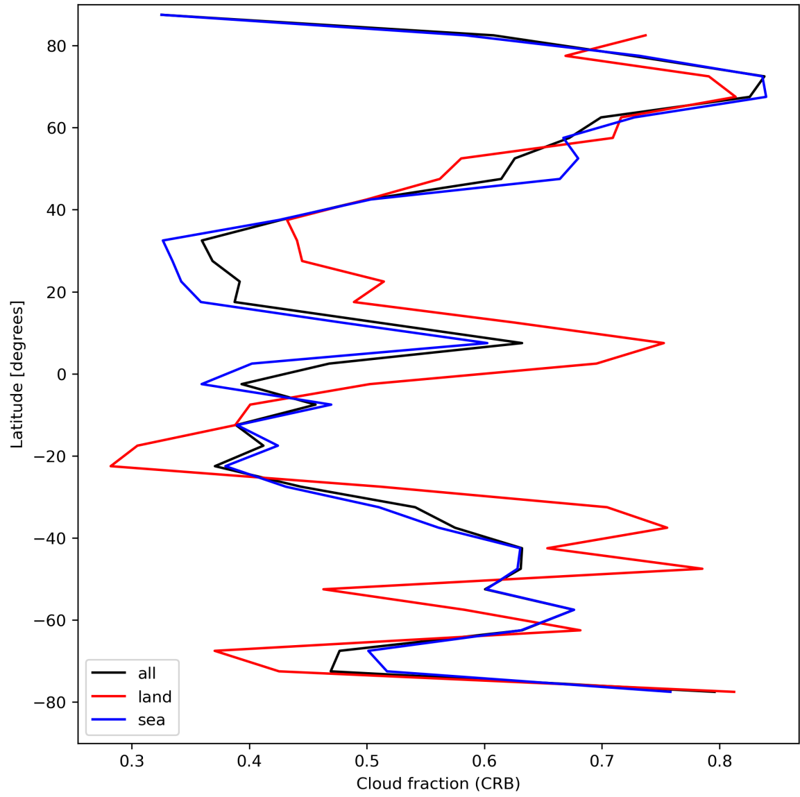
Figure 26: Zonal average of “Cloud fraction (CRB)” for 2024-08-21 to 2024-08-22.
