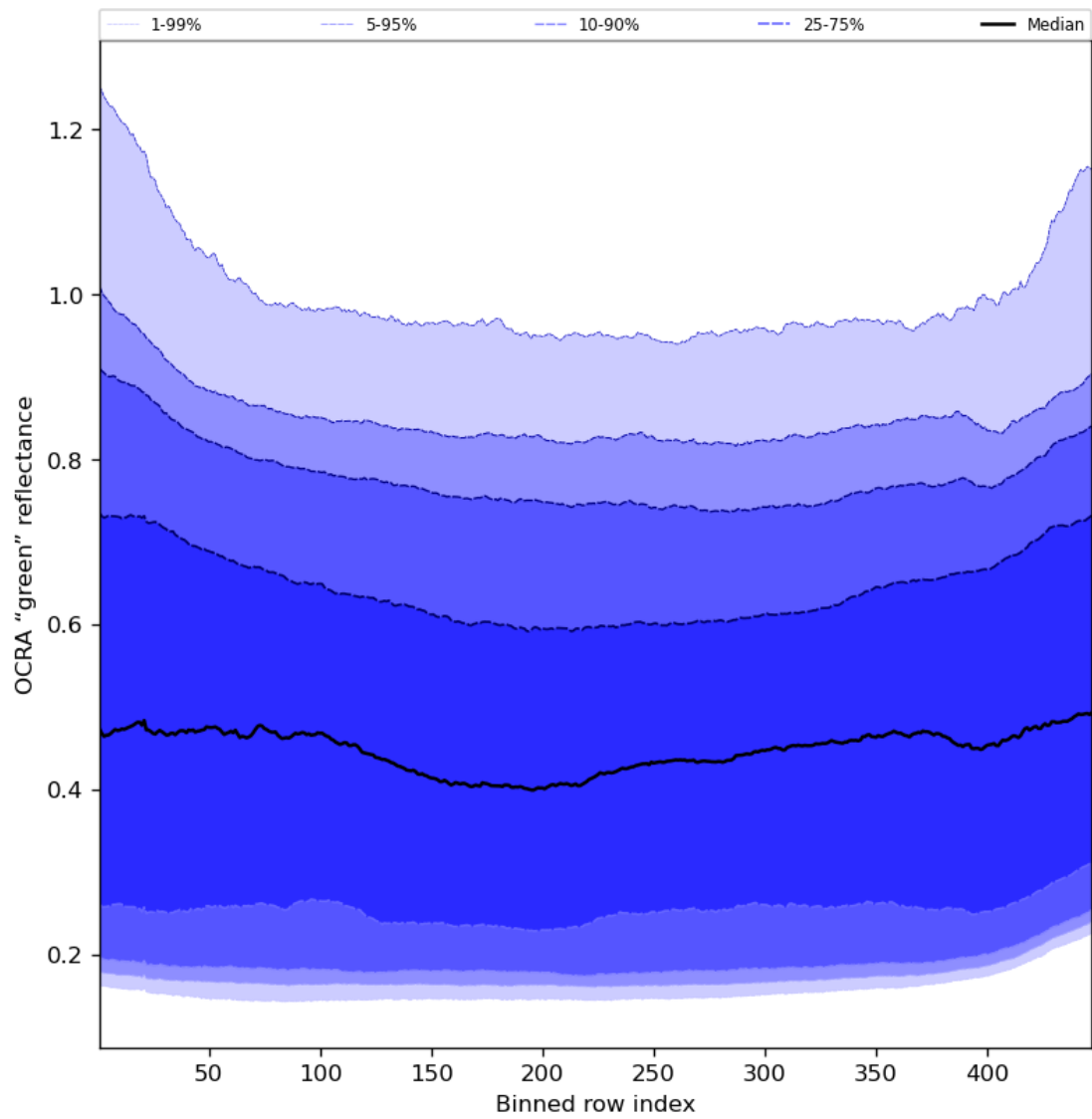
Figure 68: Along track statistics of “OCRA “green” reflectance” for 2024-08-21 to 2024-08-22
