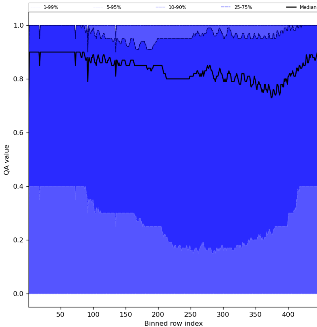
Figure 54: Along track statistics of “QA value” for 2024-08-21 to 2024-08-22
