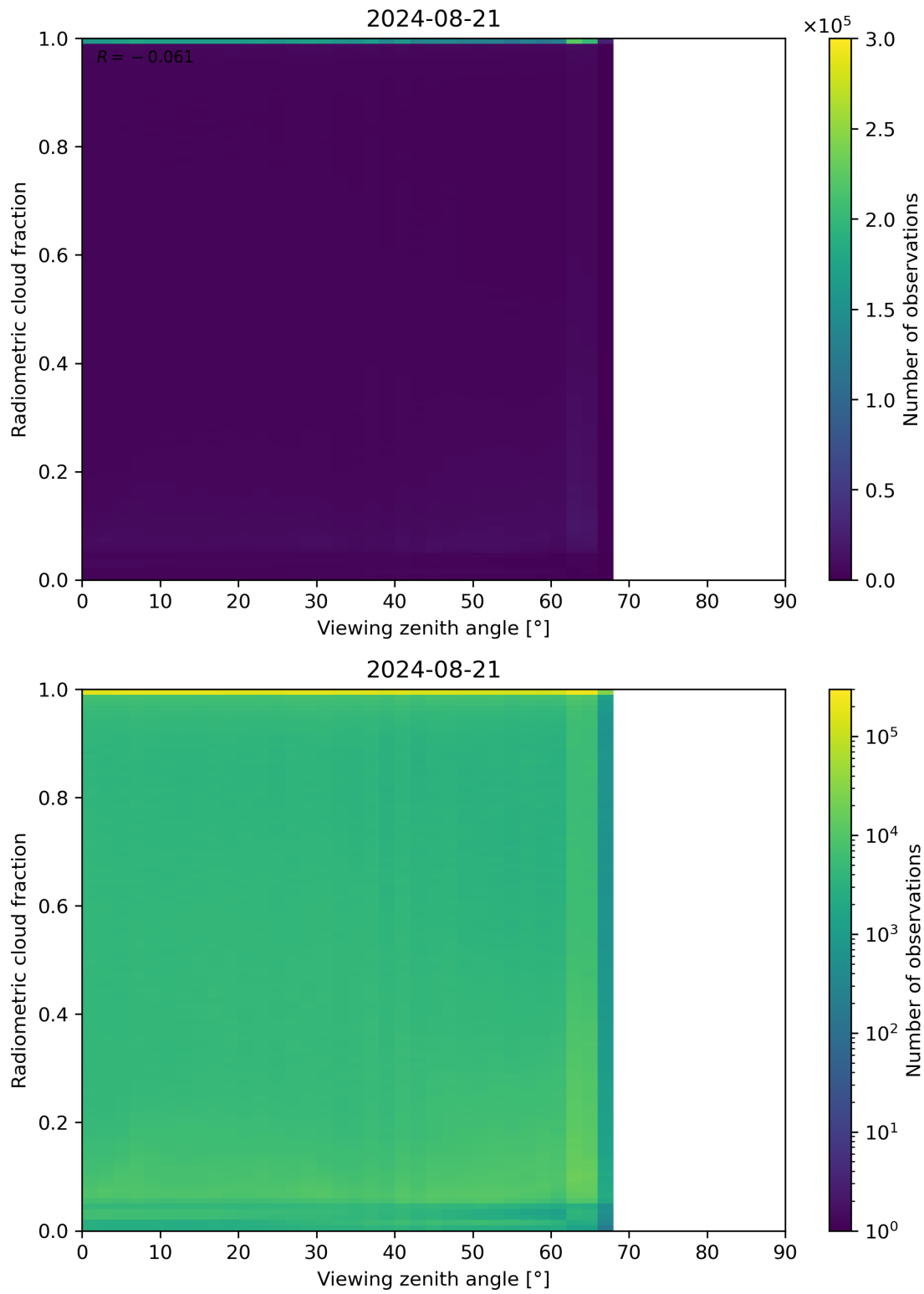
Figure 107: Scatter density plot of “Viewing zenith angle” against “Radiometric cloud fraction” for 2024-08-21 to 2024-08-22.
