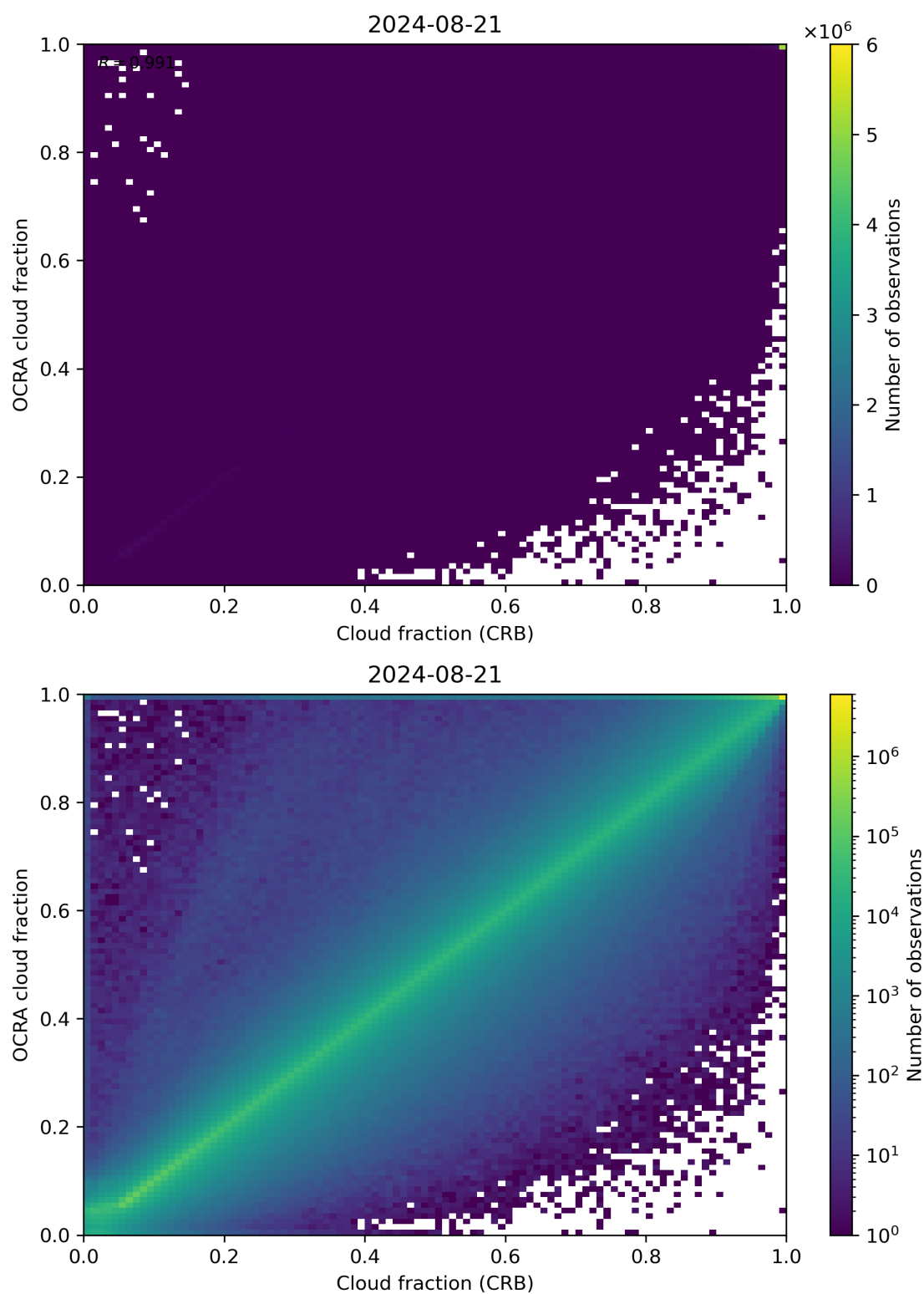
Figure 78: Scatter density plot of “Cloud fraction (CRB)” against “OCRA cloud fraction” for 2024-08-21 to 2024-08-22.
