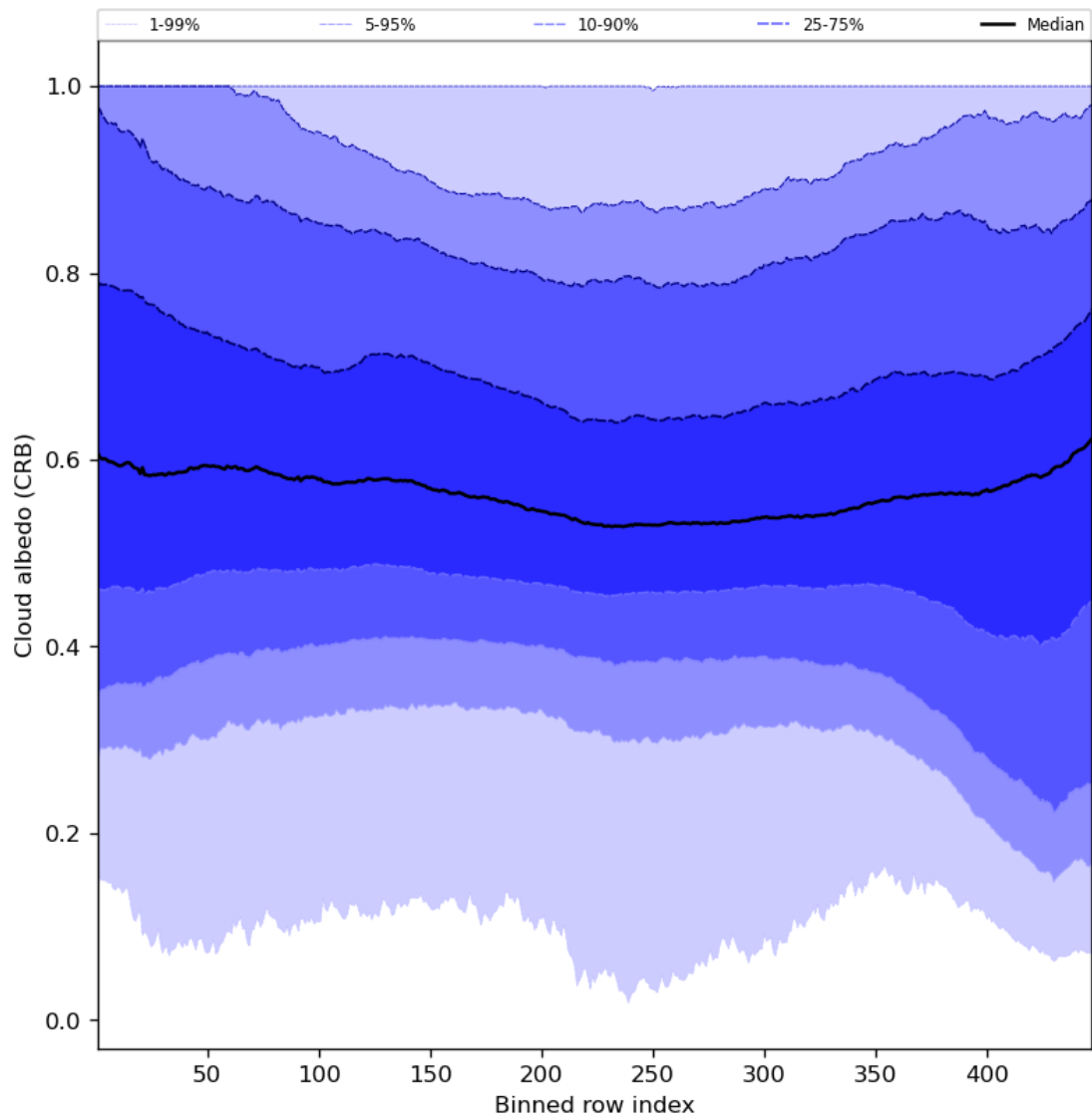
Figure 60: Along track statistics of “Cloud albedo (CRB)” for 2024-08-21 to 2024-08-22
