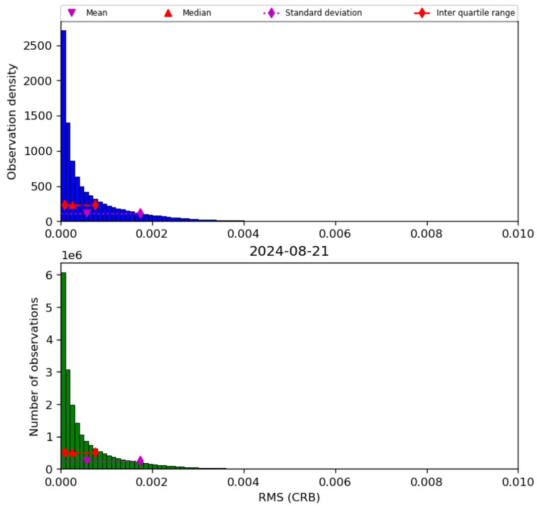
Figure 48: Histogram of “RMS (CRB)” for 2024-08-21 to 2024-08-22
