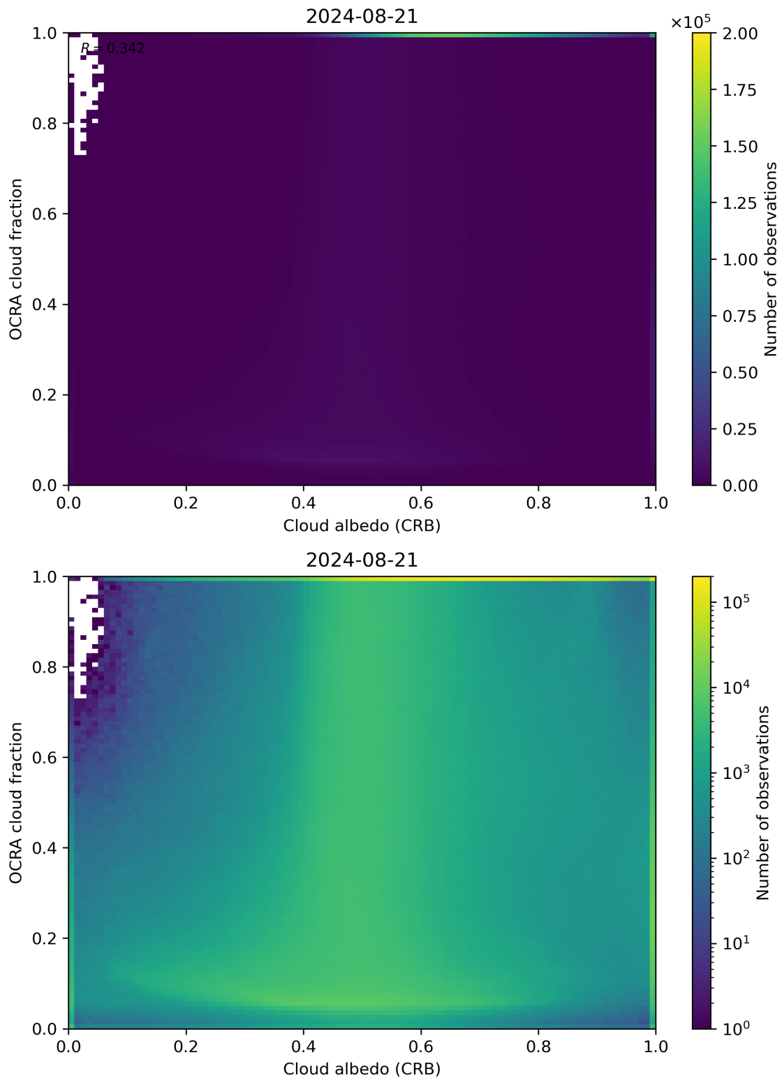
Figure 70: Scatter density plot of “Cloud albedo (CRB)” against “OCRA cloud fraction” for 2024-08-21 to 2024-08-22.
