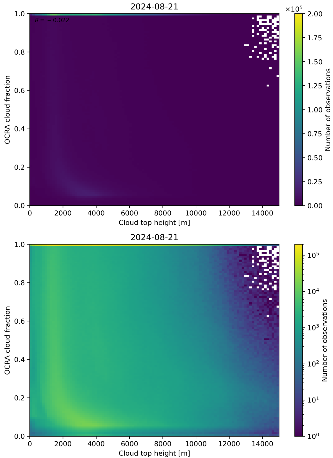
Figure 87: Scatter density plot of “Cloud top height” against “OCRA cloud fraction” for 2024-08-21 to 2024-08-22.
