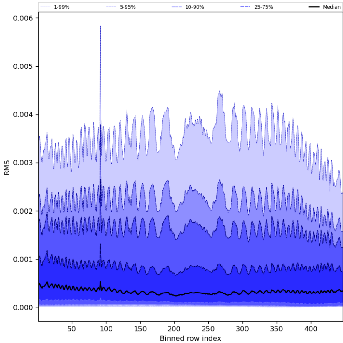
Figure 63: Along track statistics of “RMS” for 2024-08-21 to 2024-08-22
