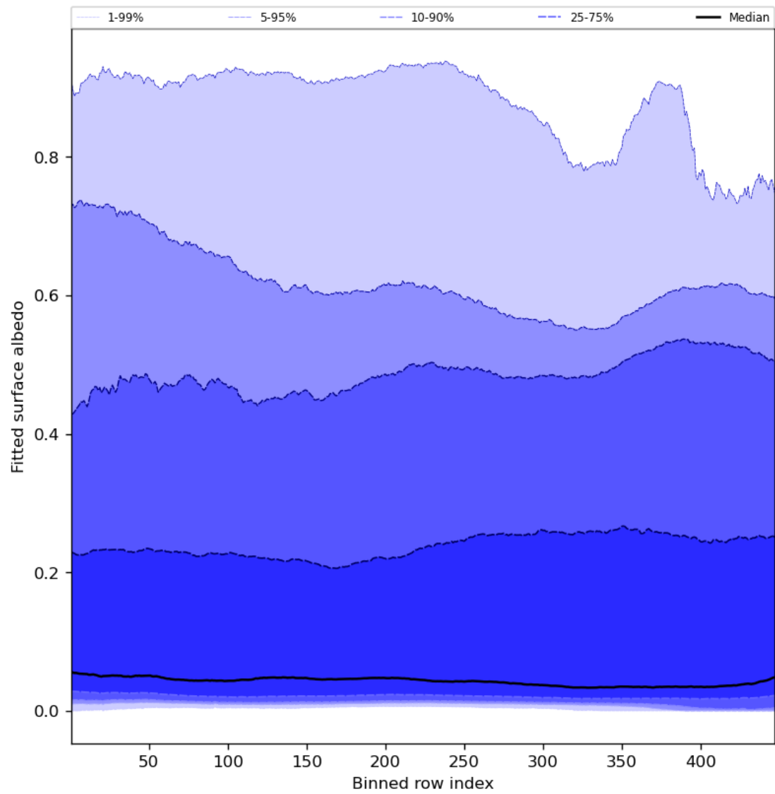
Figure 61: Along track statistics of “Fitted surface albedo” for 2024-08-21 to 2024-08-22
