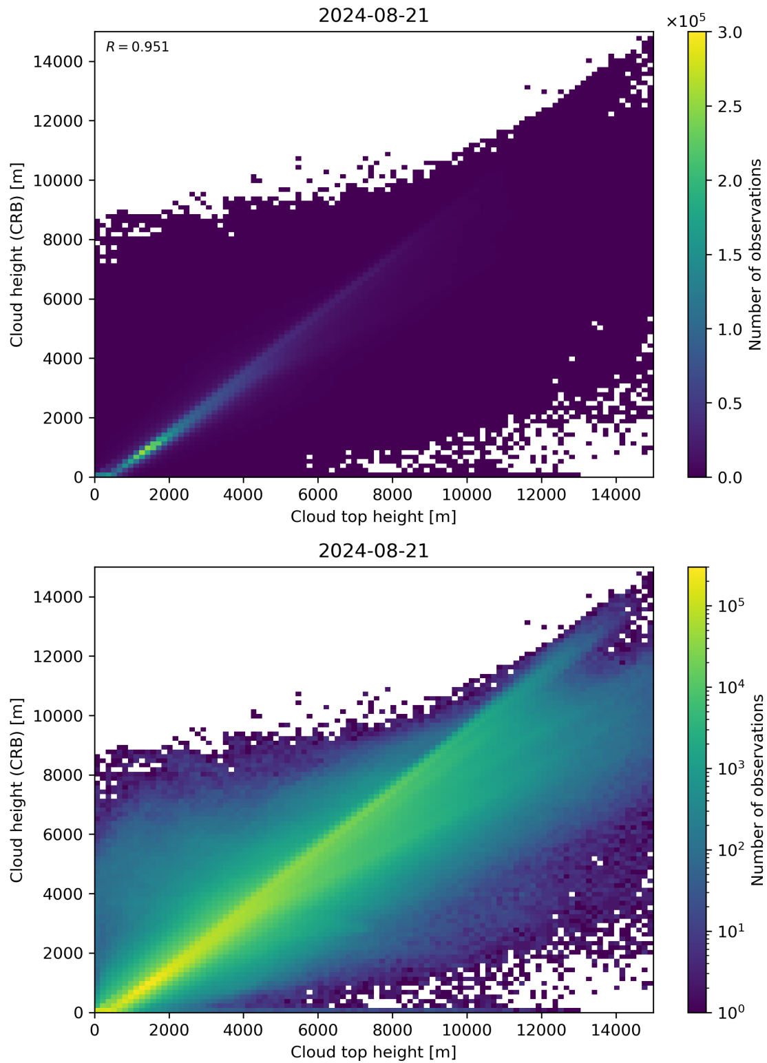
Figure 89: Scatter density plot of “Cloud top height” against “Cloud height (CRB)” for 2024-08-21 to 2024-08-22.
