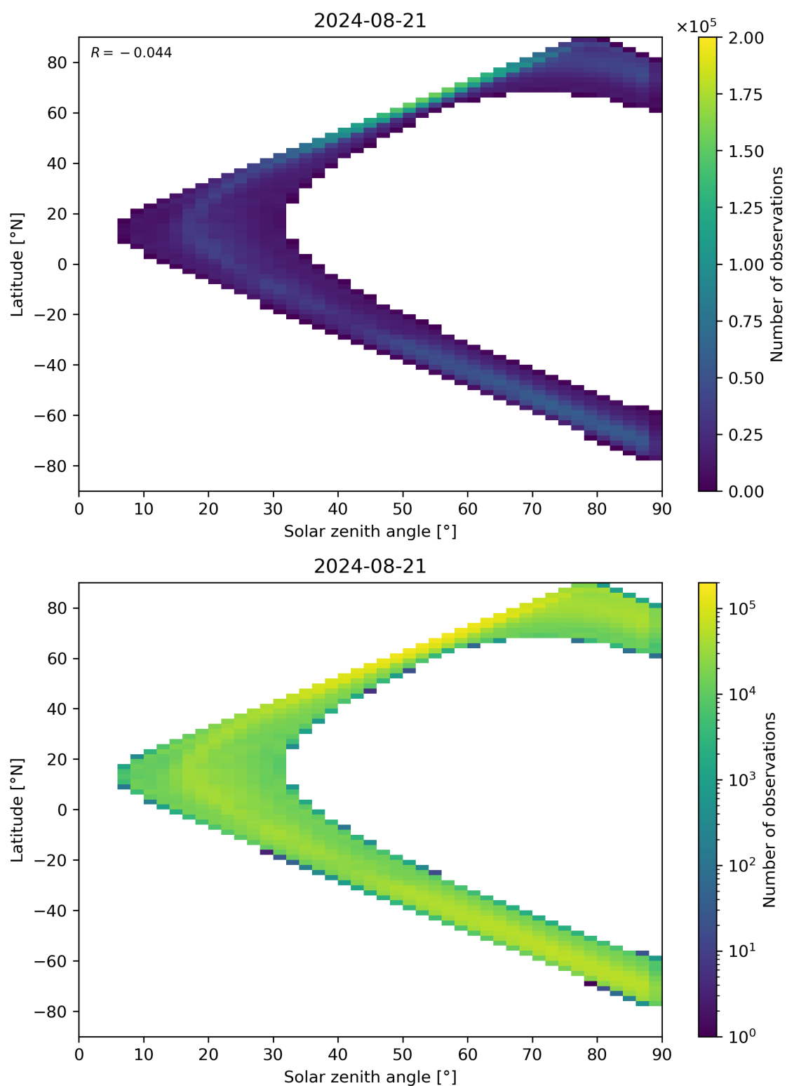
Figure 105: Scatter density plot of “Solar zenith angle” against “Latitude” for 2024-08-21 to 2024-08-22.
