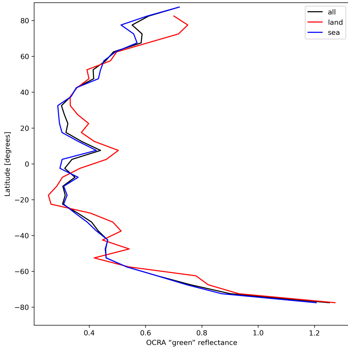
Figure 36: Zonal average of “OCRA “green” reflectance” for 2024-08-21 to 2024-08-22.
