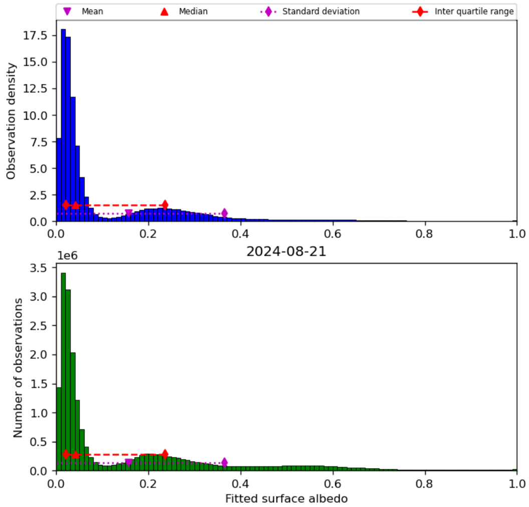
Figure 45: Histogram of “Fitted surface albedo” for 2024-08-21 to 2024-08-22
