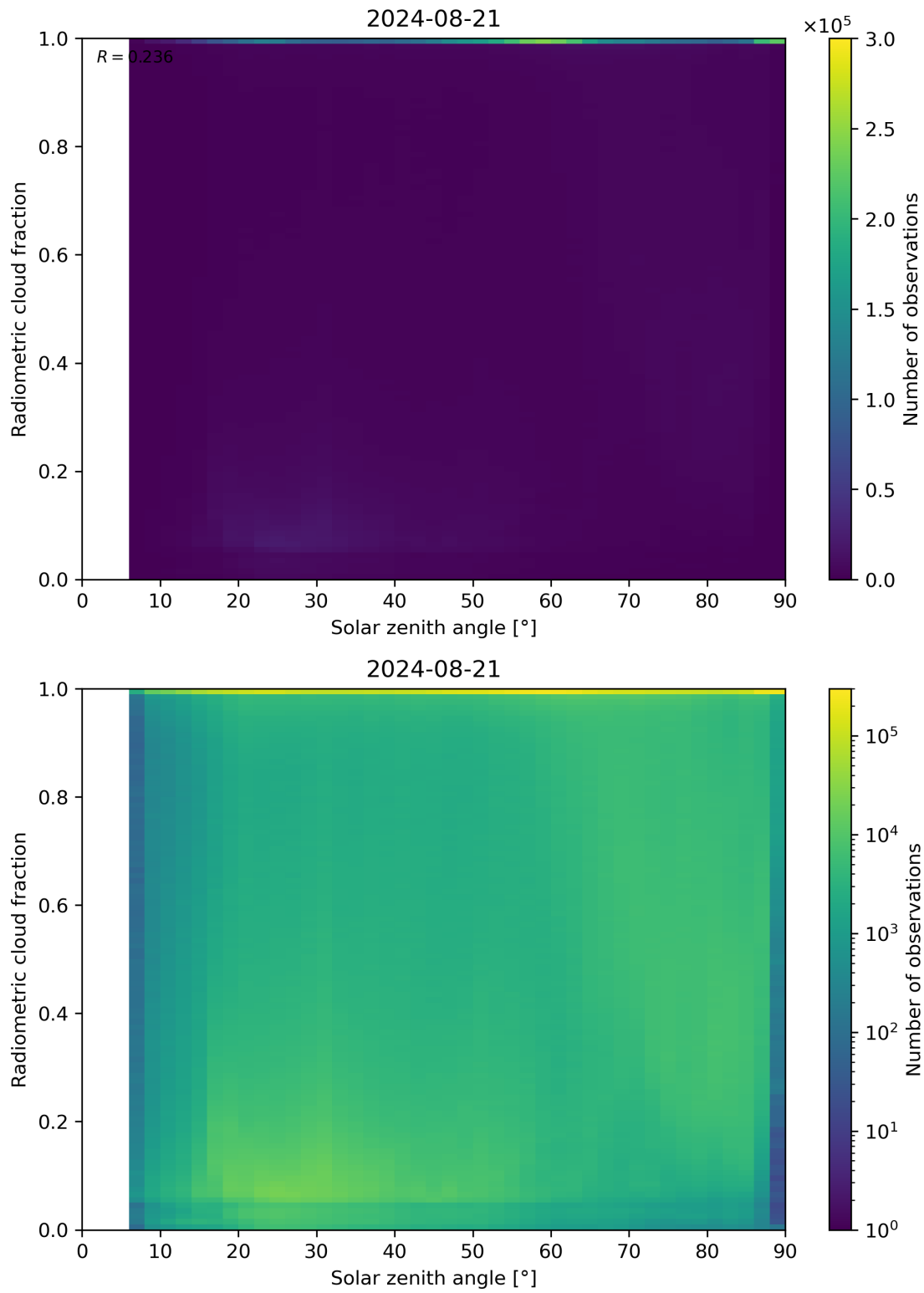
Figure 99: Scatter density plot of “Solar zenith angle” against “Radiometric cloud fraction” for 2024-08-21 to 2024-08-22.
