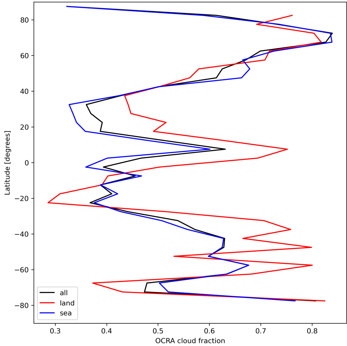
Figure 34: Zonal average of “OCRA cloud fraction” for 2024-08-21 to 2024-08-22.
