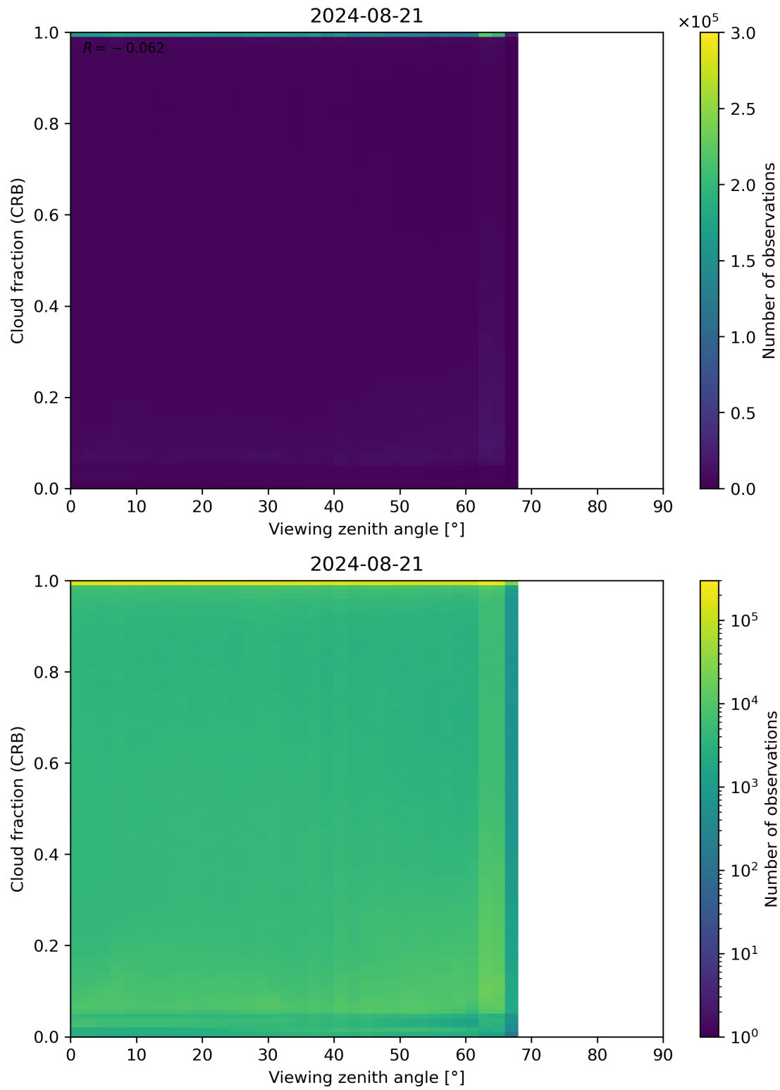
Figure 109: Scatter density plot of “Viewing zenith angle” against “Cloud fraction (CRB)” for 2024-08-21 to 2024-08-22.
