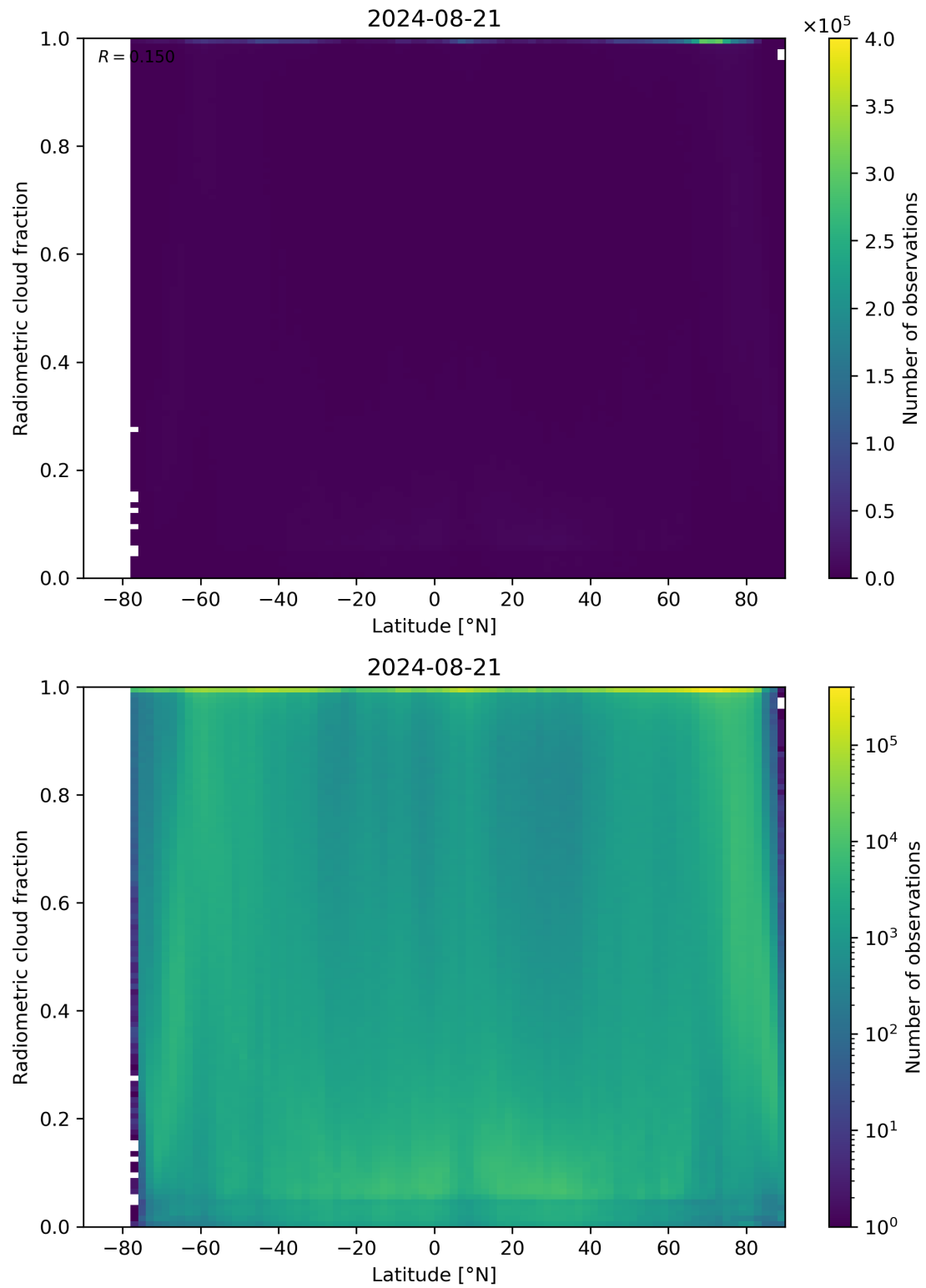
Figure 92: Scatter density plot of “Latitude” against “Radiometric cloud fraction” for 2024-08-21 to 2024-08-22.
