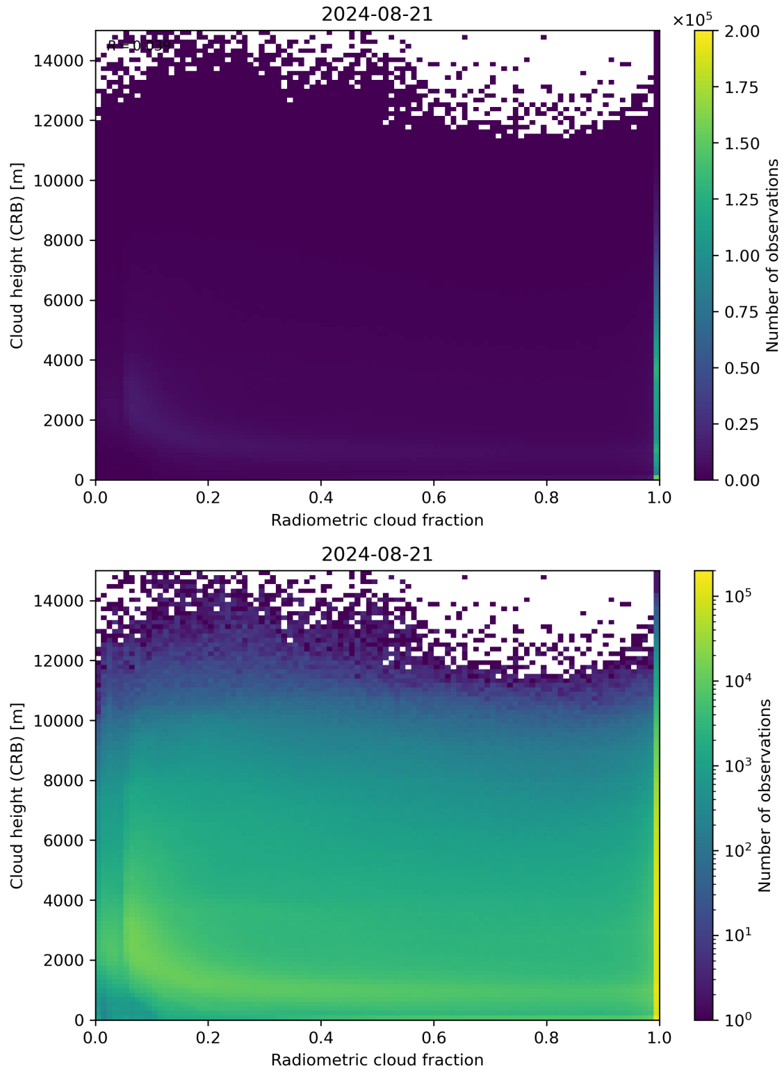
Figure 74: Scatter density plot of “Radiometric cloud fraction” against “Cloud height (CRB)” for 2024-08-21 to 2024-08-22.
