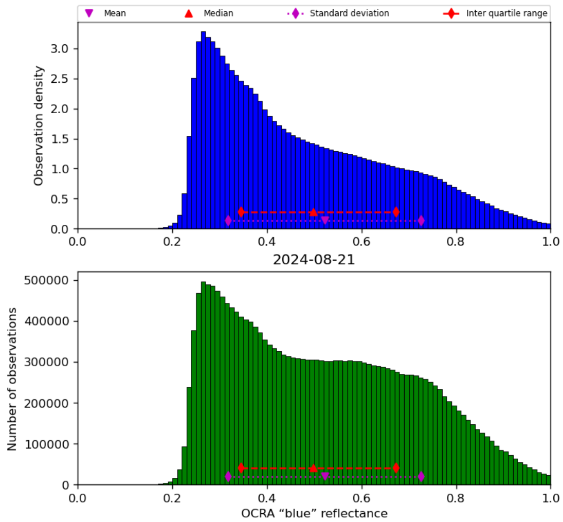
Figure 51: Histogram of “OCRA “blue” reflectance” for 2024-08-21 to 2024-08-22
