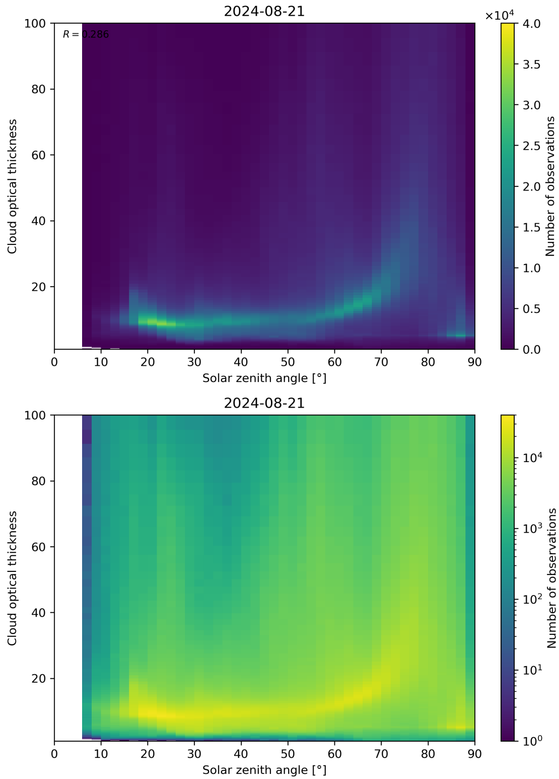
Figure 103: Scatter density plot of “Solar zenith angle” against “Cloud optical thickness” for 2024-08-21 to 2024-08-22.
