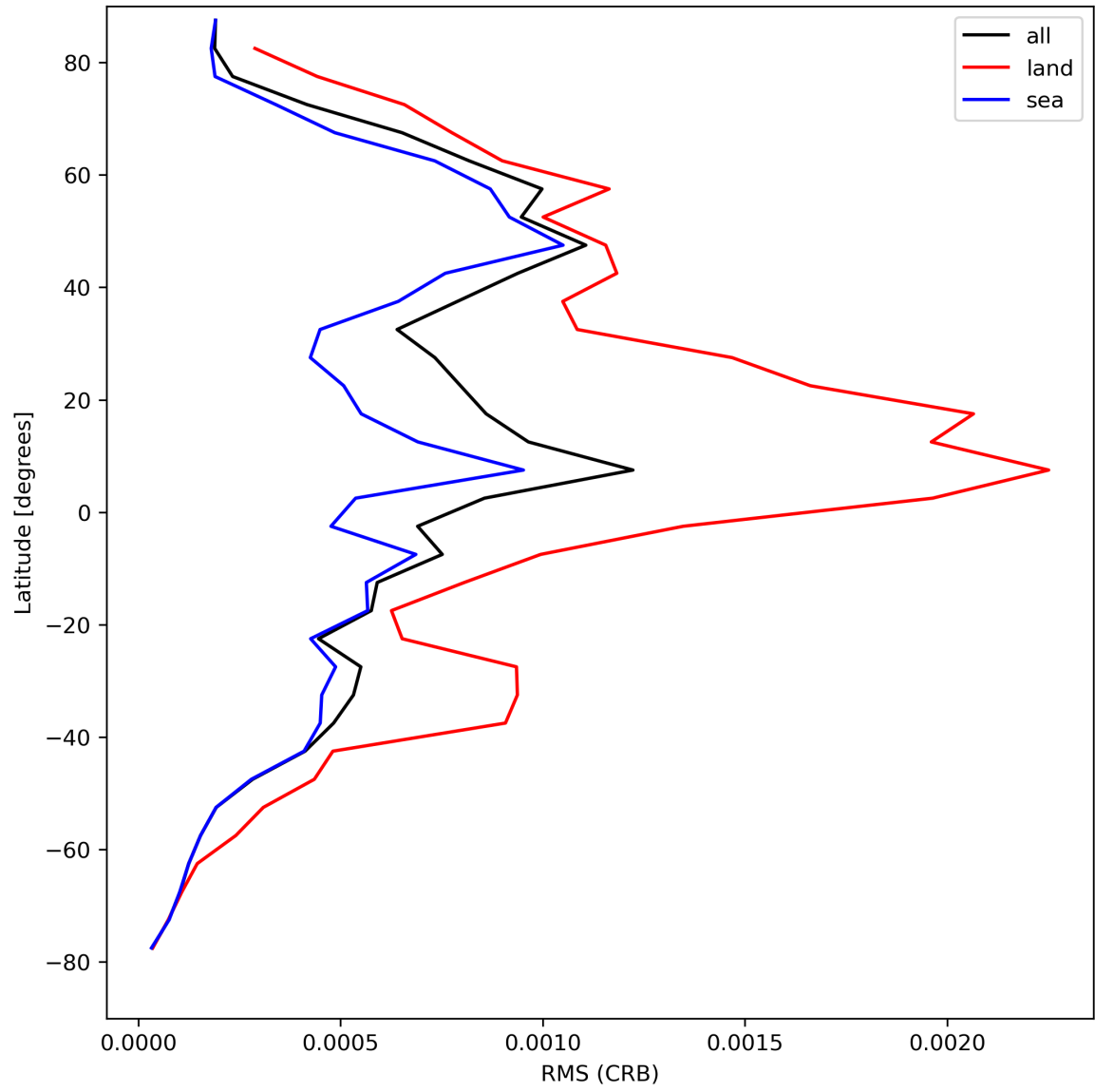
Figure 32: Zonal average of “RMS (CRB)” for 2024-08-21 to 2024-08-22.
