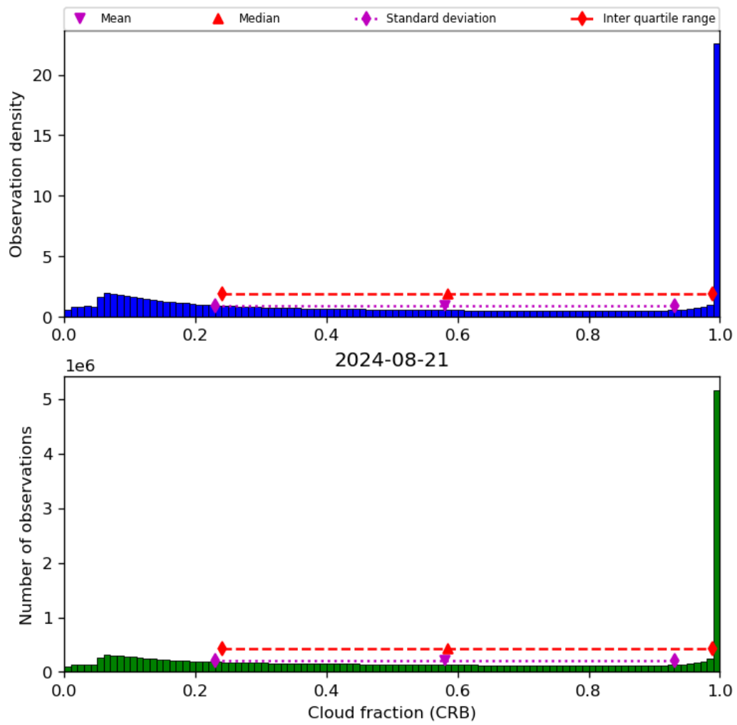
Figure 42: Histogram of “Cloud fraction (CRB)” for 2024-08-21 to 2024-08-22
