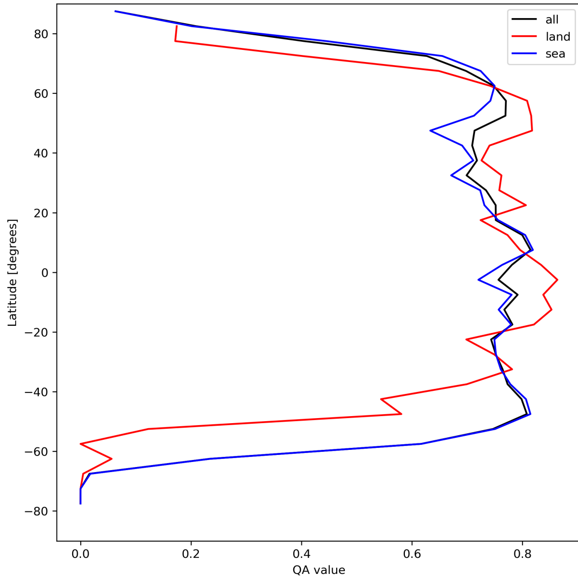
Figure 22: Zonal average of “QA value” for 2024-08-21 to 2024-08-22.
