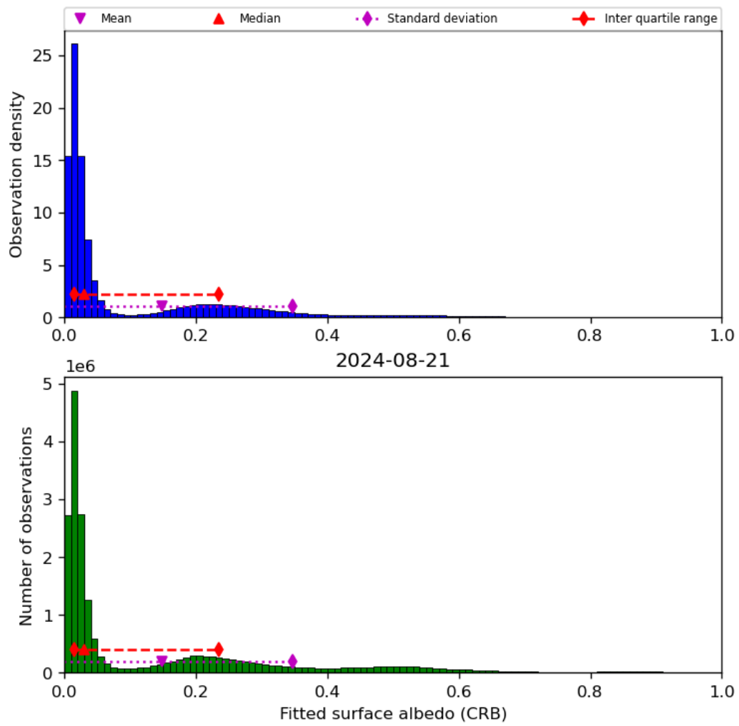
Figure 46: Histogram of “Fitted surface albedo (CRB)” for 2024-08-21 to 2024-08-22
