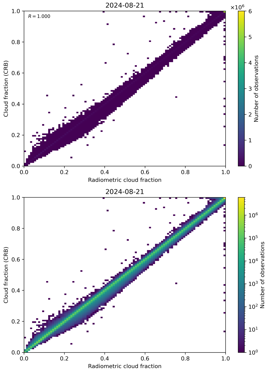
Figure 73: Scatter density plot of “Radiometric cloud fraction” against “Cloud fraction (CRB)” for 2024-08-21 to 2024-08-22.
