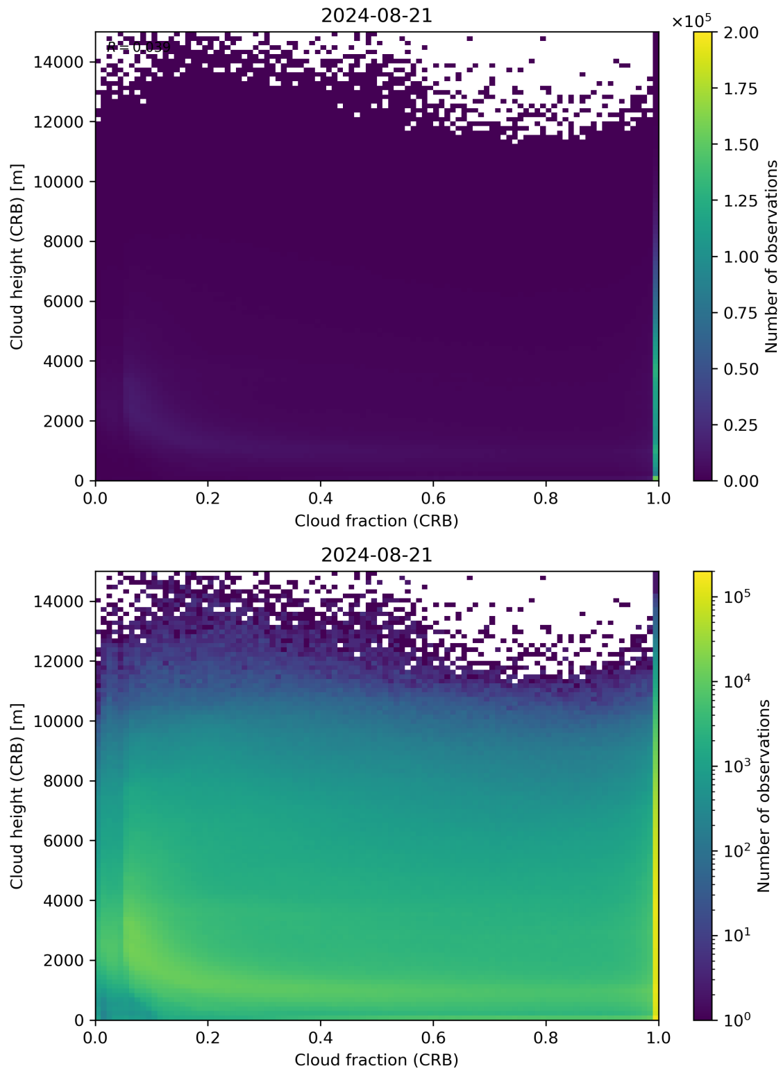
Figure 79: Scatter density plot of “Cloud fraction (CRB)” against “Cloud height (CRB)” for 2024-08-21 to 2024-08-22.
