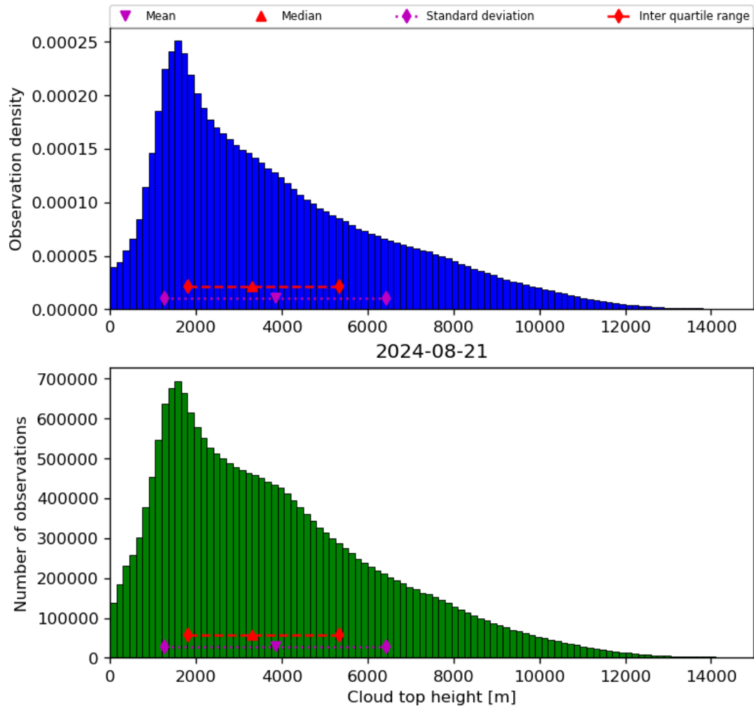
Figure 40: Histogram of “Cloud top height” for 2024-08-21 to 2024-08-22
