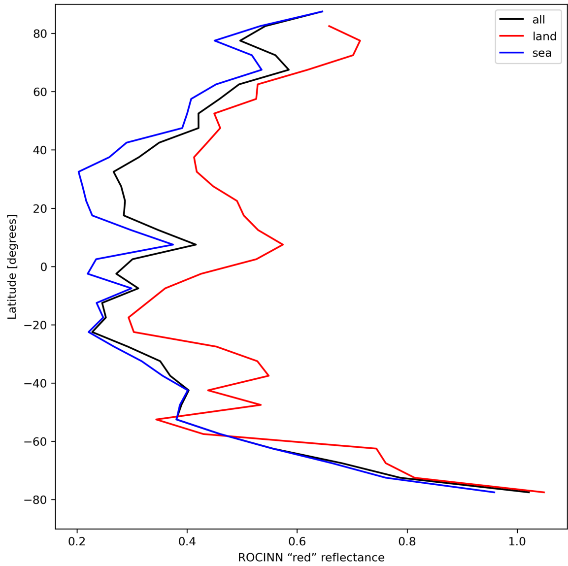
Figure 37: Zonal average of “ROCINN “red” reflectance” for 2024-08-21 to 2024-08-22.
