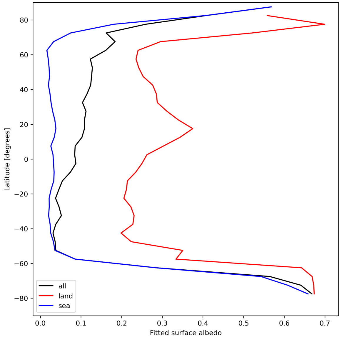
Figure 29: Zonal average of “Fitted surface albedo” for 2024-08-21 to 2024-08-22.
