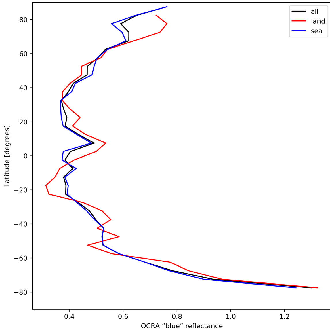
Figure 35: Zonal average of “OCRA “blue” reflectance” for 2024-08-21 to 2024-08-22.
