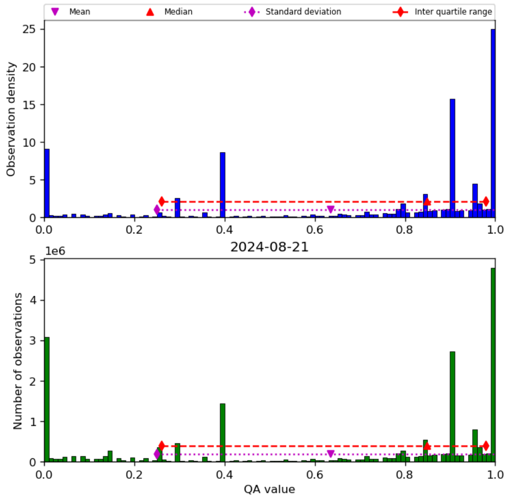
Figure 38: Histogram of “QA value” for 2024-08-21 to 2024-08-22
