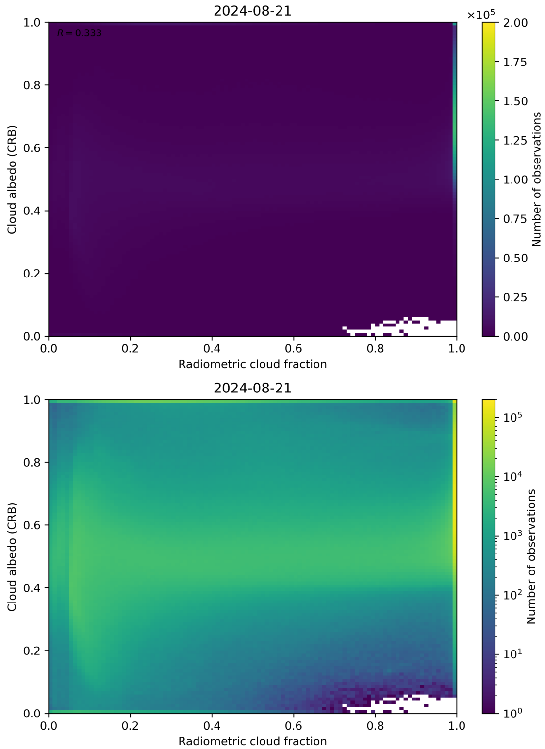
Figure 71: Scatter density plot of “Radiometric cloud fraction” against “Cloud albedo (CRB)” for 2024-08-21 to 2024-08-22.
