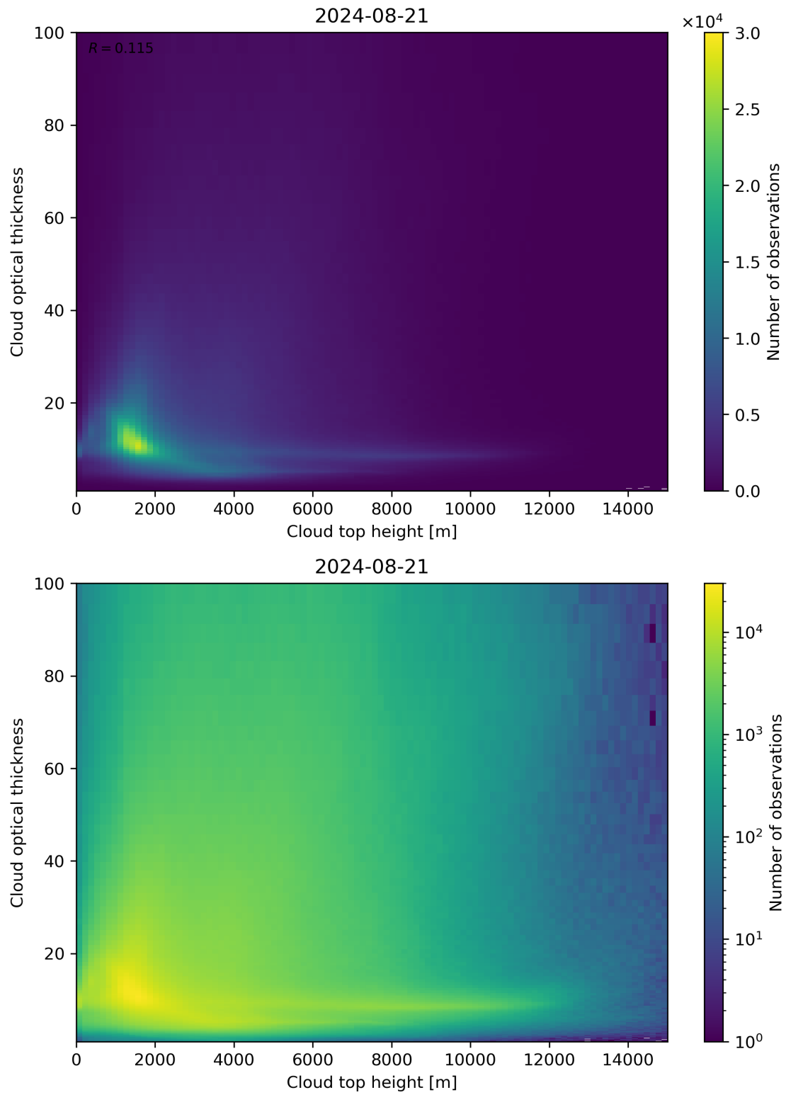
Figure 90: Scatter density plot of “Cloud top height” against “Cloud optical thickness” for 2024-08-21 to 2024-08-22.
