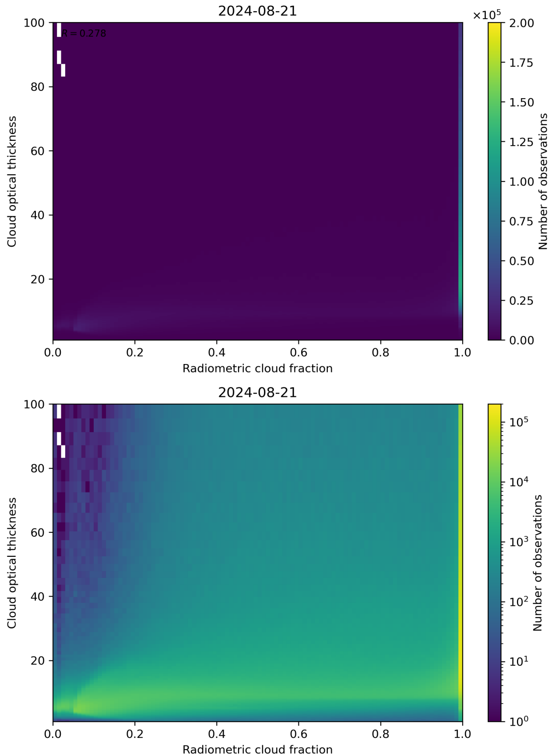
Figure 75: Scatter density plot of “Radiometric cloud fraction” against “Cloud optical thickness” for 2024-08-21 to 2024-08-22.
