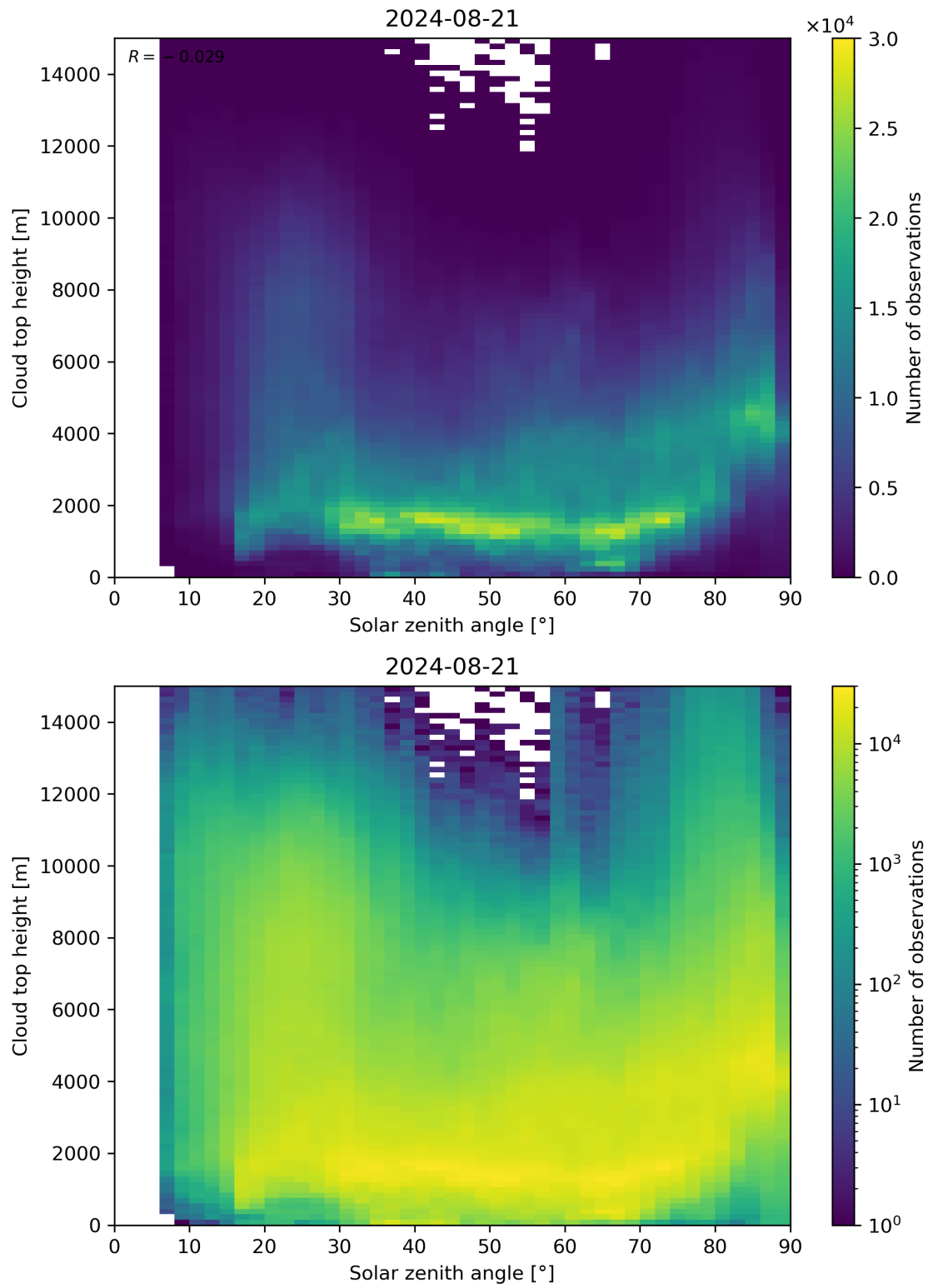
Figure 104: Scatter density plot of “Solar zenith angle” against “Cloud top height” for 2024-08-21 to 2024-08-22.
