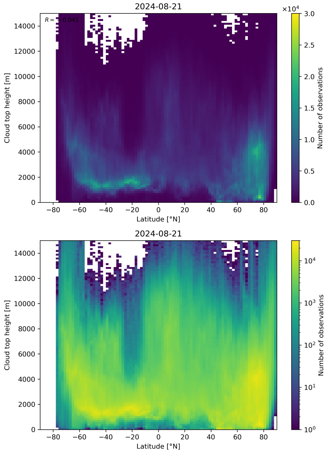
Figure 97: Scatter density plot of “Latitude” against “Cloud top height” for 2024-08-21 to 2024-08-22.
