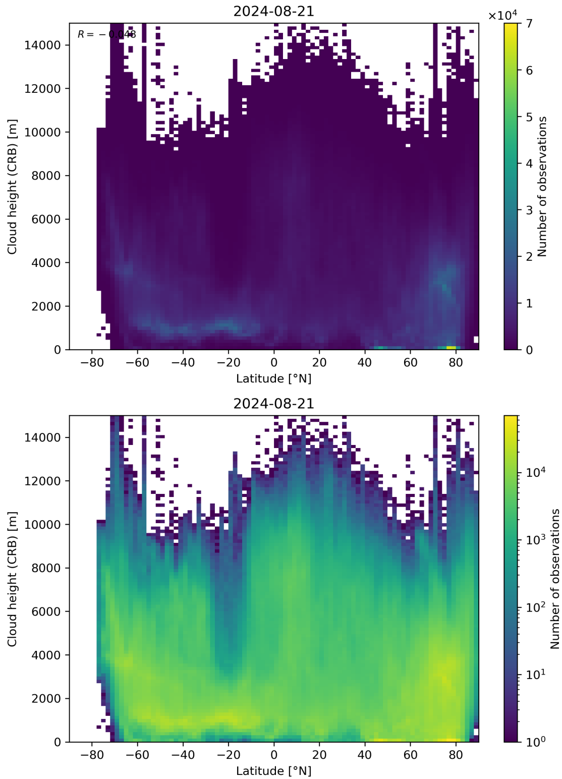
Figure 95: Scatter density plot of “Latitude” against “Cloud height (CRB)” for 2024-08-21 to 2024-08-22.
