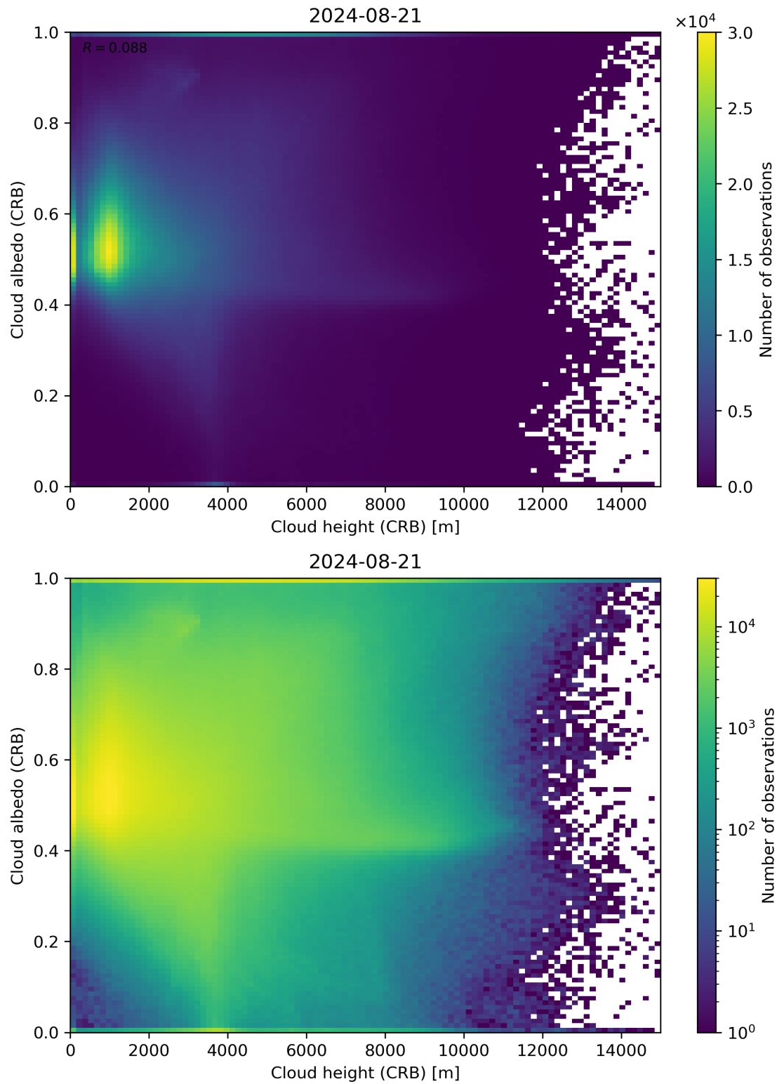
Figure 80: Scatter density plot of “Cloud height (CRB)” against “Cloud albedo (CRB)” for 2024-08-21 to 2024-08-22.
