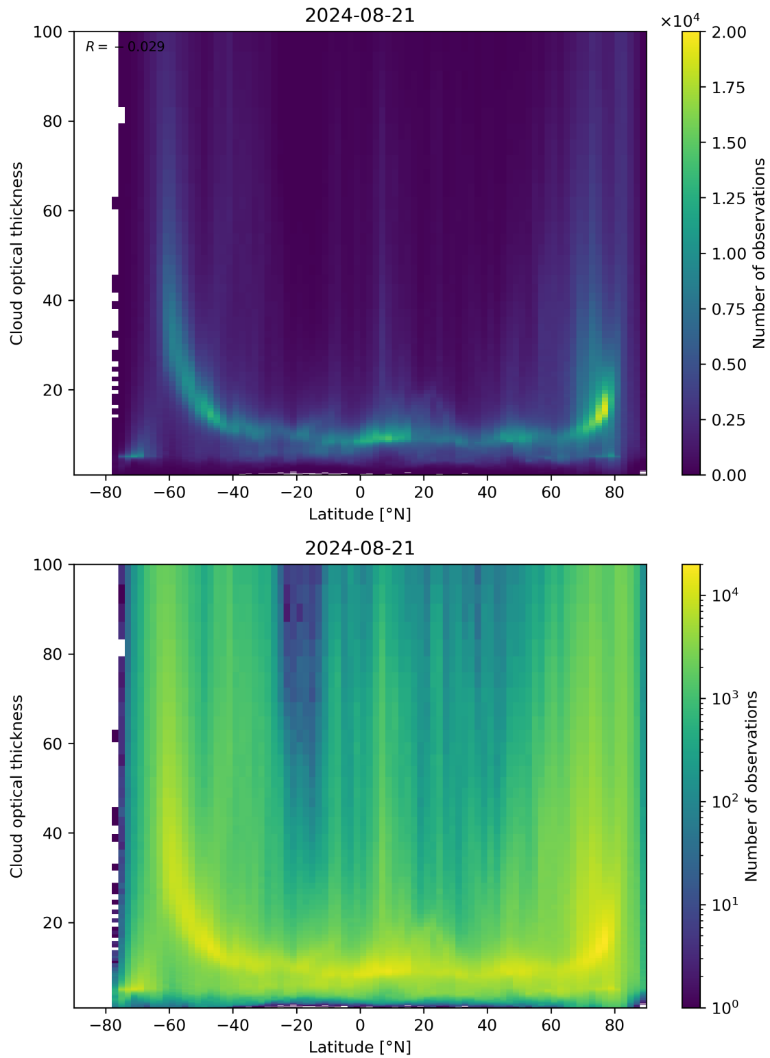
Figure 96: Scatter density plot of “Latitude” against “Cloud optical thickness” for 2024-08-21 to 2024-08-22.
