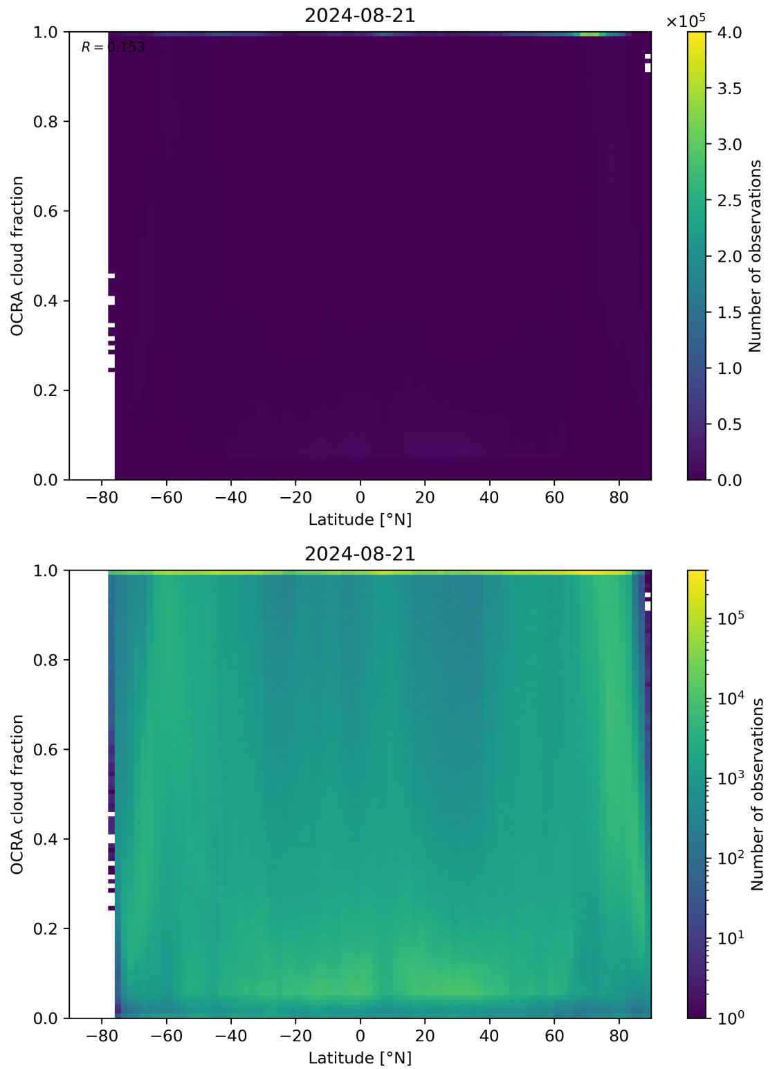
Figure 93: Scatter density plot of “Latitude” against “OCRA cloud fraction” for 2024-08-21 to 2024-08-22.
