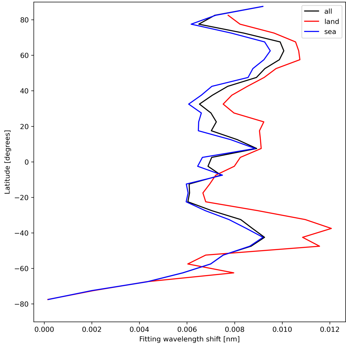
Figure 33: Zonal average of “Fitting wavelength shift” for 2024-08-21 to 2024-08-22.
