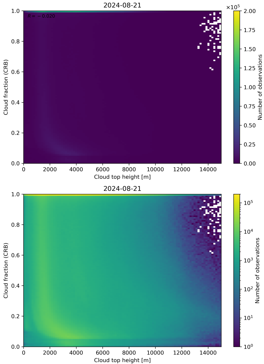
Figure 88: Scatter density plot of “Cloud top height” against “Cloud fraction (CRB)” for 2024-08-21 to 2024-08-22.
