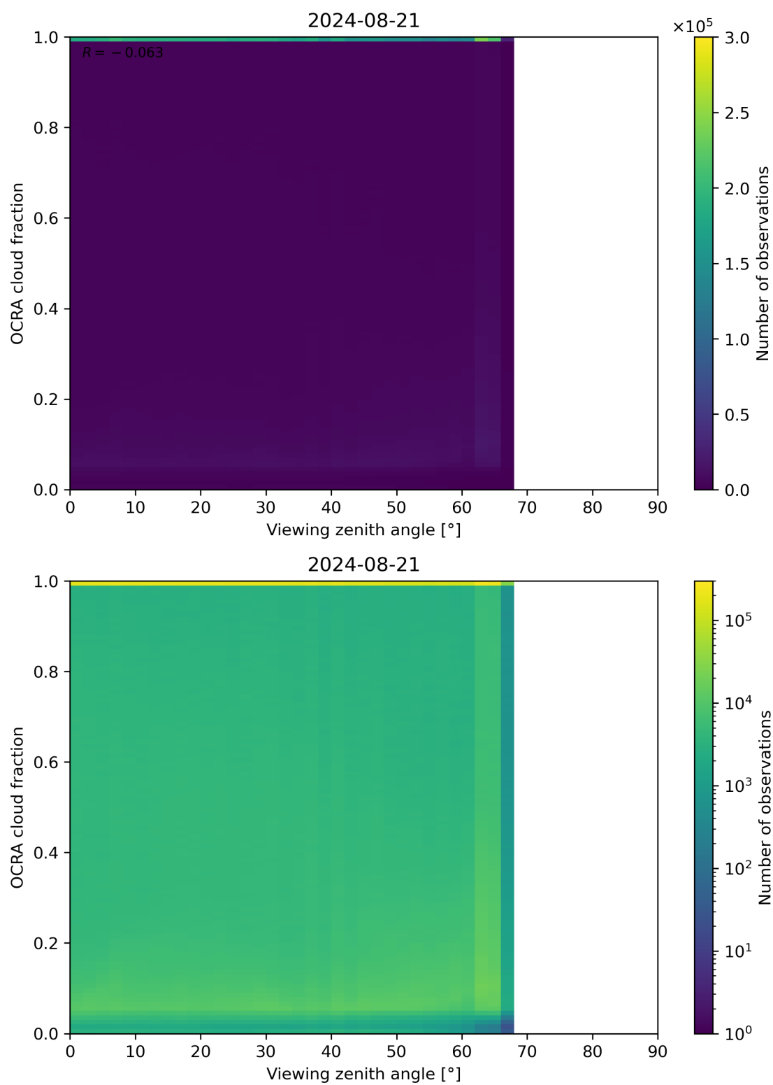
Figure 108: Scatter density plot of “Viewing zenith angle” against “OCRA cloud fraction” for 2024-08-21 to 2024-08-22.
