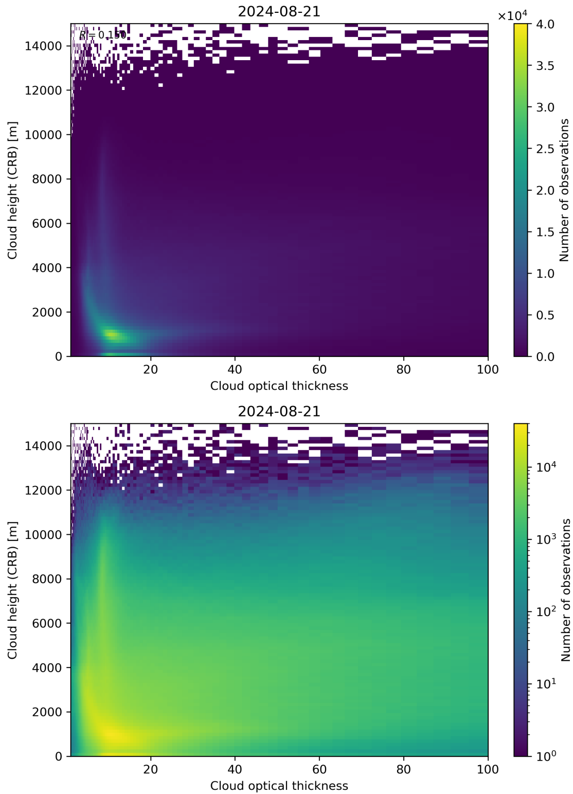
Figure 85: Scatter density plot of “Cloud optical thickness” against “Cloud height (CRB)” for 2024-08-21 to 2024-08-22.
