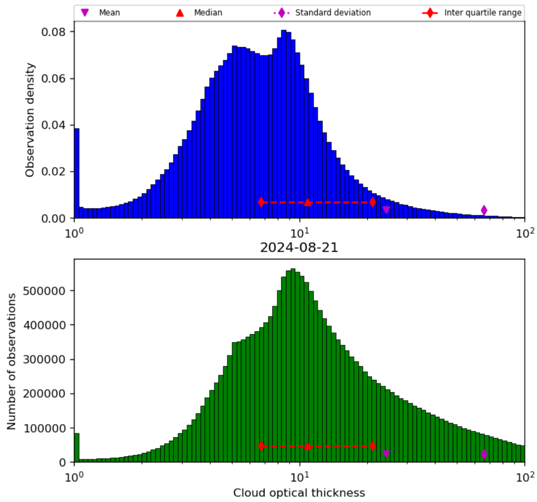
Figure 41: Histogram of “Cloud optical thickness” for 2024-08-21 to 2024-08-22
