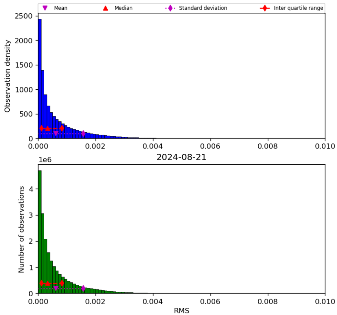
Figure 47: Histogram of “RMS” for 2024-08-21 to 2024-08-22
