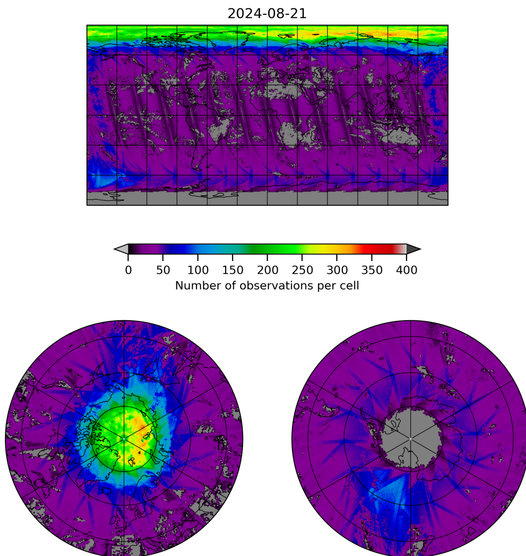
Figure 21: Map of the number of observations for 2024-08-21 to 2024-08-22
