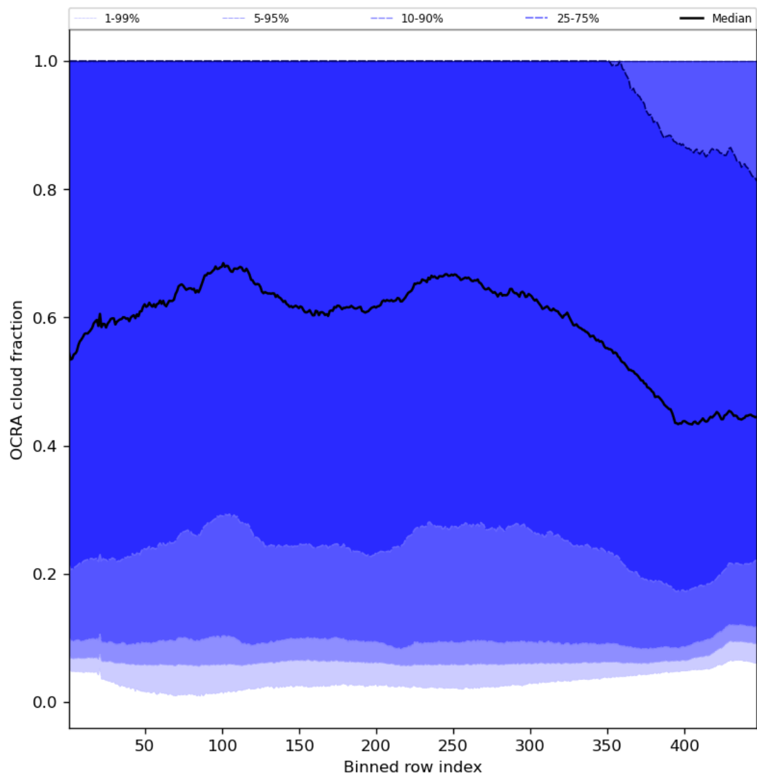
Figure 66: Along track statistics of “OCRA cloud fraction” for 2024-08-21 to 2024-08-22
