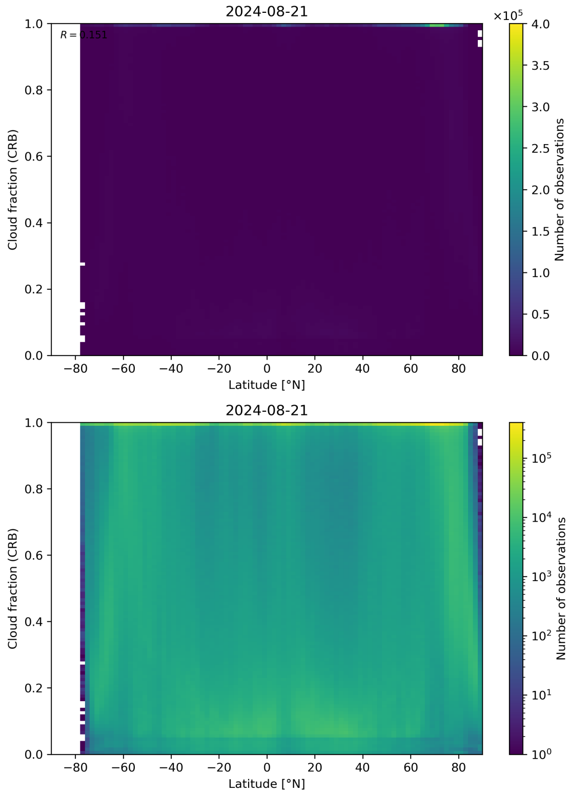
Figure 94: Scatter density plot of “Latitude” against “Cloud fraction (CRB)” for 2024-08-21 to 2024-08-22.
