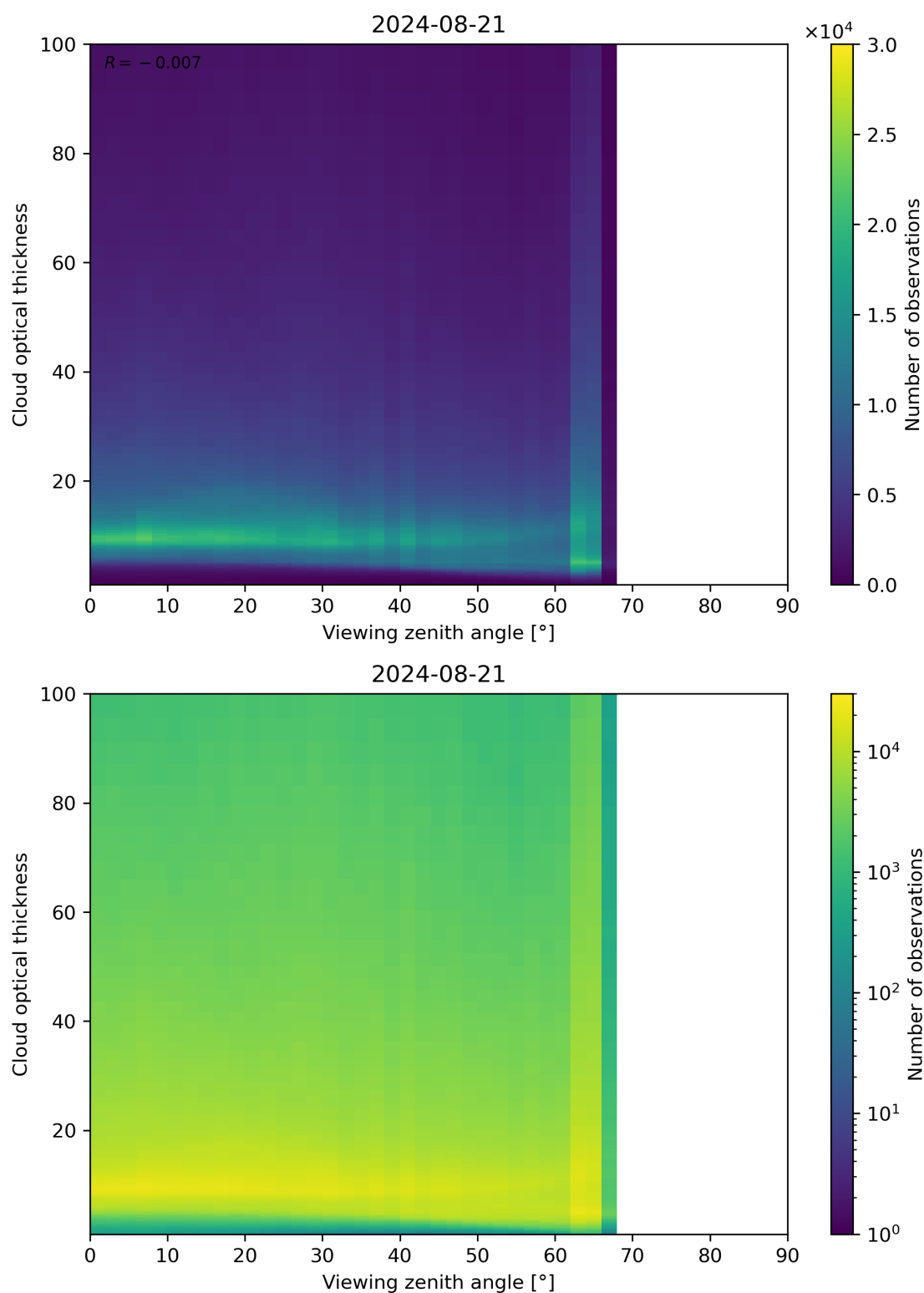
Figure 111: Scatter density plot of “Viewing zenith angle” against “Cloud optical thickness” for 2024-08-21 to 2024-08-22.
