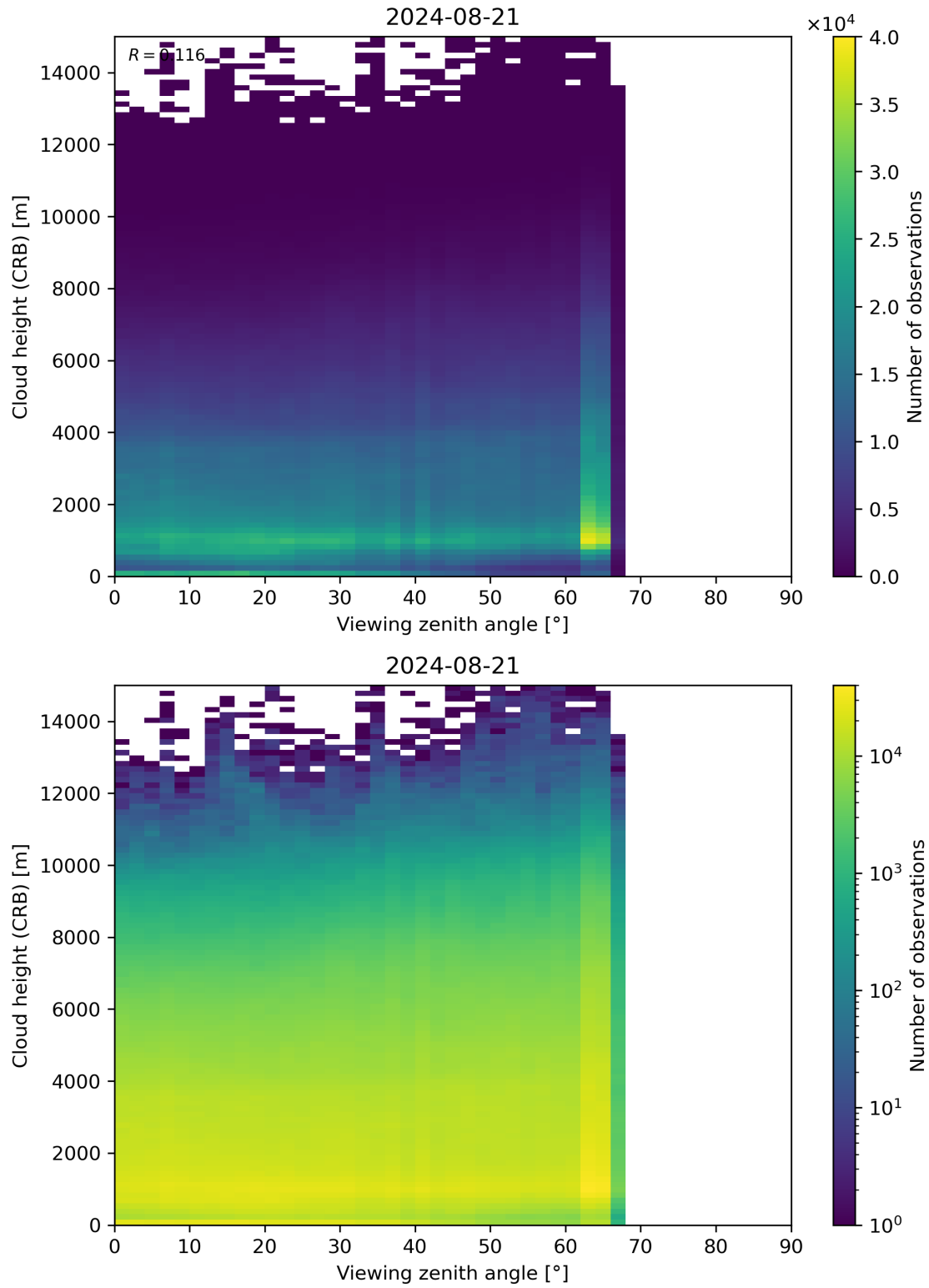
Figure 110: Scatter density plot of “Viewing zenith angle” against “Cloud height (CRB)” for 2024-08-21 to 2024-08-22.
