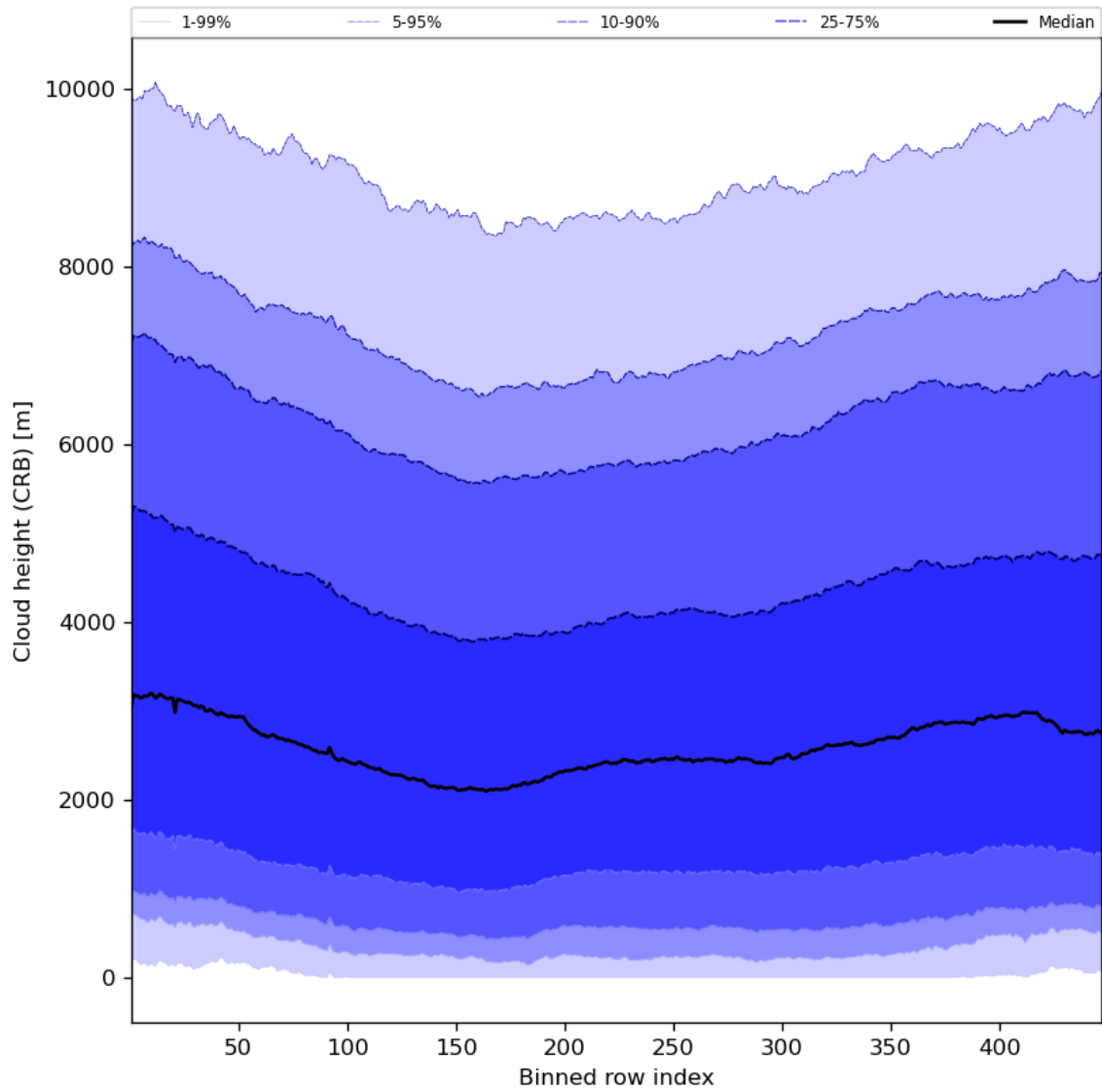
Figure 59: Along track statistics of “Cloud height (CRB)” for 2024-08-21 to 2024-08-22
