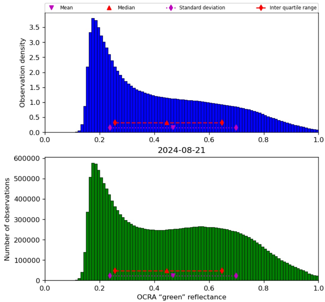
Figure 52: Histogram of “OCRA “green” reflectance” for 2024-08-21 to 2024-08-22
