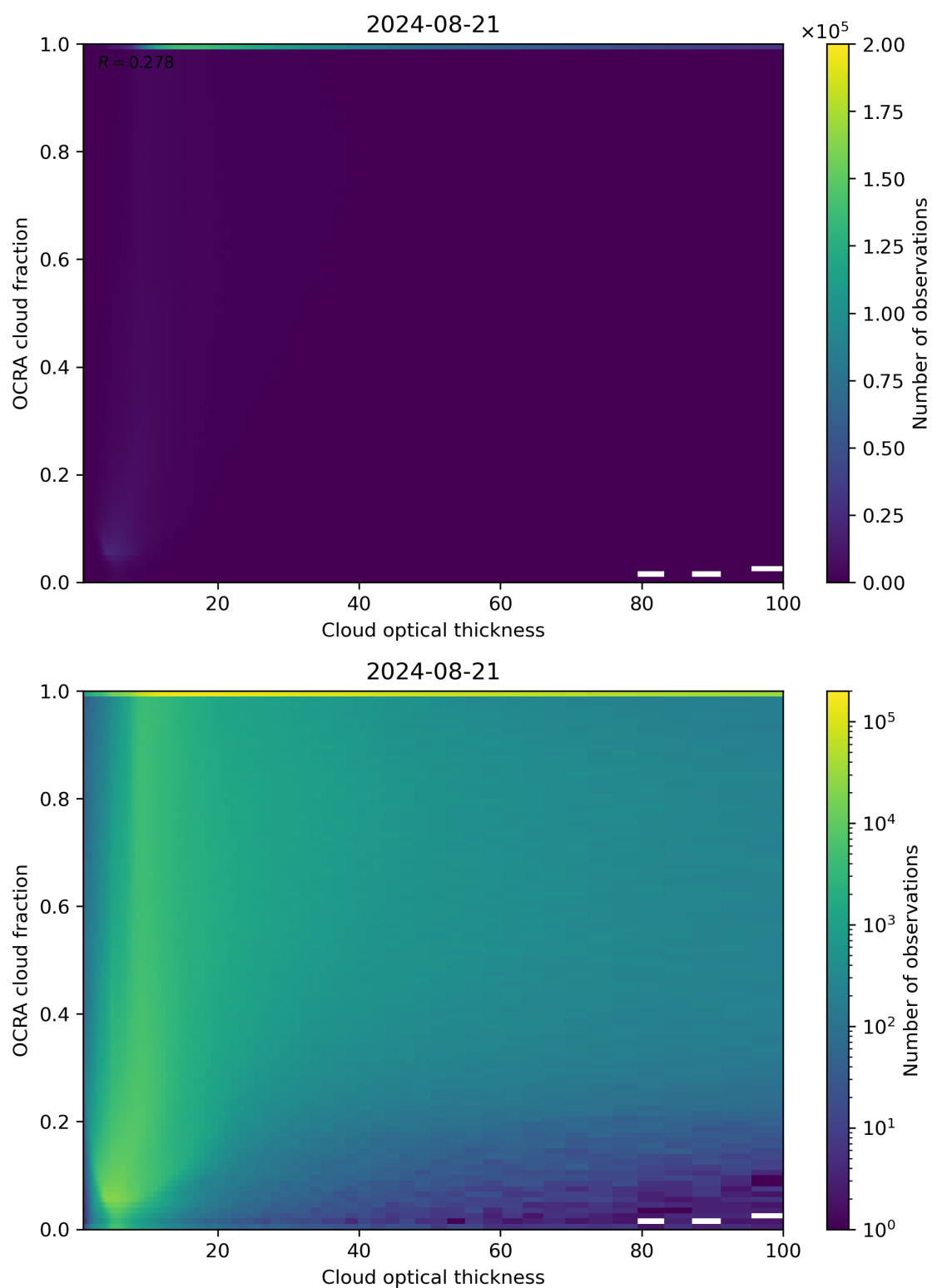
Figure 83: Scatter density plot of “Cloud optical thickness” against “OCRA cloud fraction” for 2024-08-21 to 2024-08-22.
