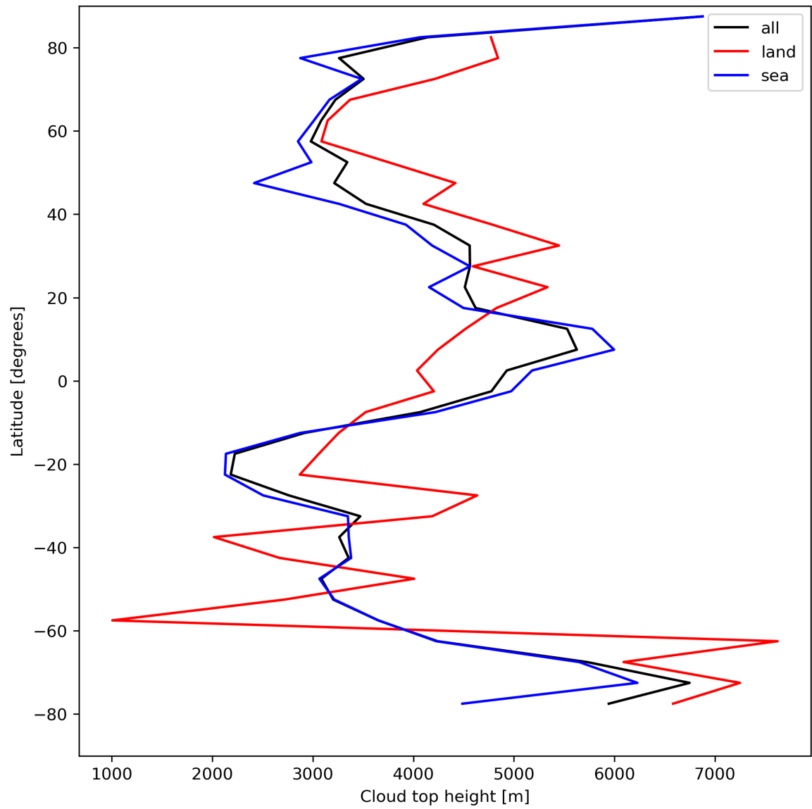
Figure 24: Zonal average of “Cloud top height” for 2024-08-21 to 2024-08-22.
