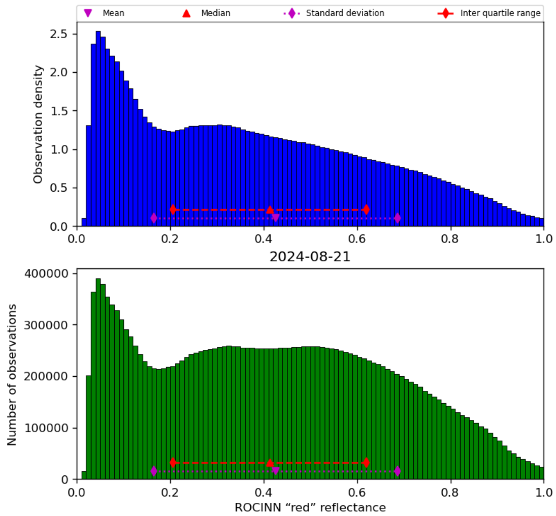
Figure 53: Histogram of “ROCINN “red” reflectance” for 2024-08-21 to 2024-08-22
