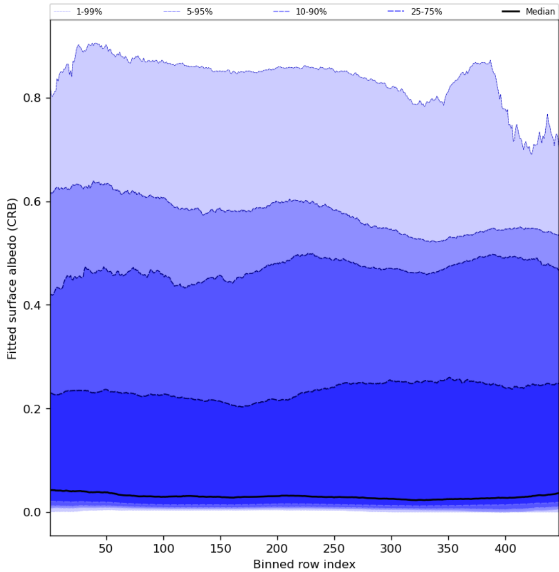
Figure 62: Along track statistics of “Fitted surface albedo (CRB)” for 2024-08-21 to 2024-08-22
