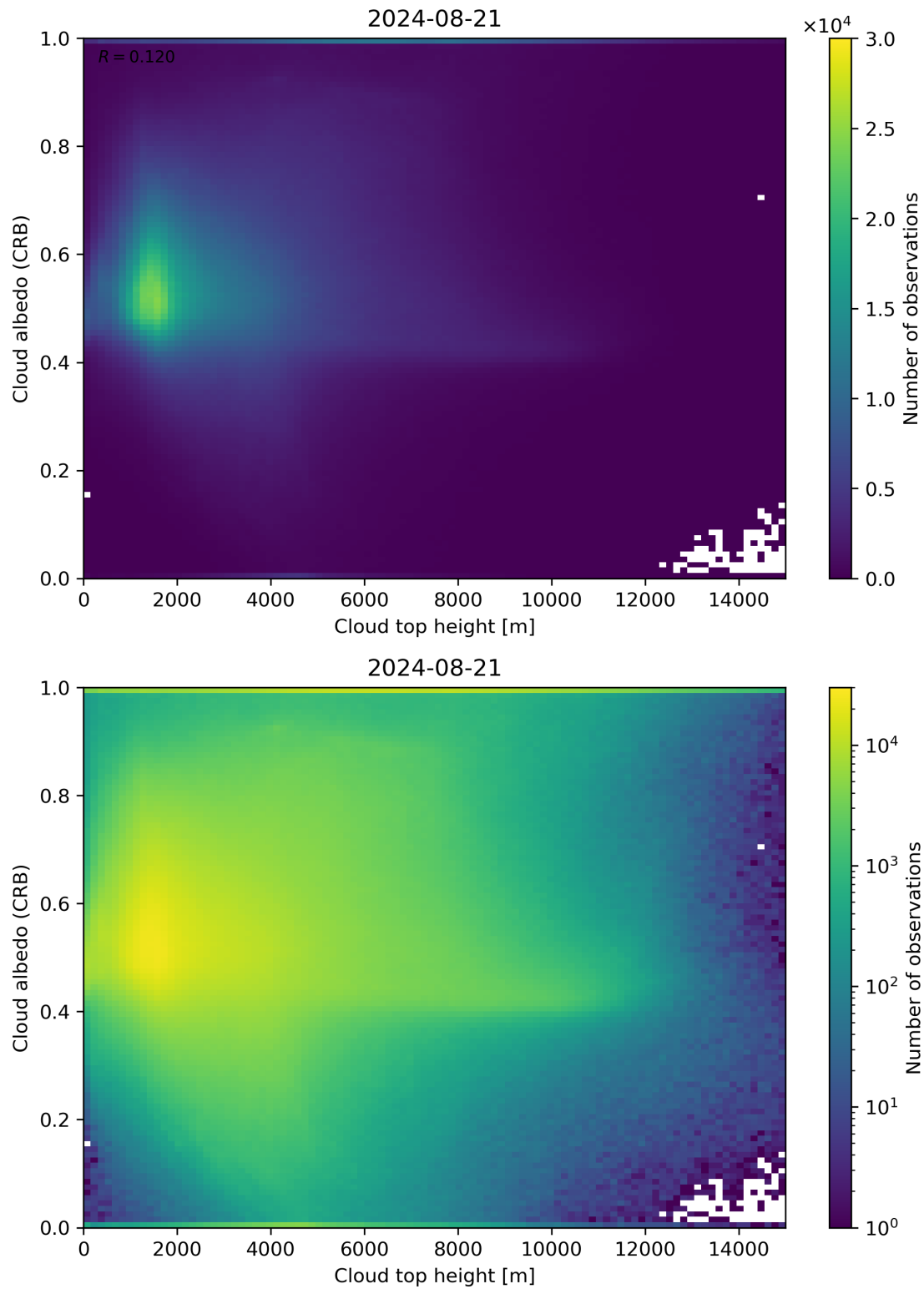
Figure 86: Scatter density plot of “Cloud top height” against “Cloud albedo (CRB)” for 2024-08-21 to 2024-08-22.
