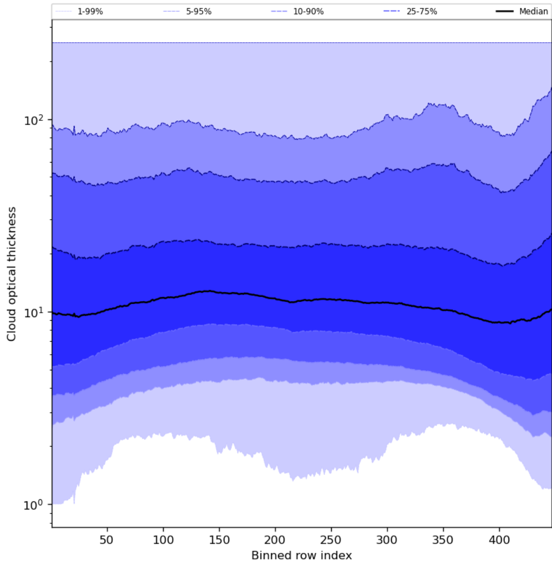
Figure 57: Along track statistics of “Cloud optical thickness” for 2024-08-21 to 2024-08-22
