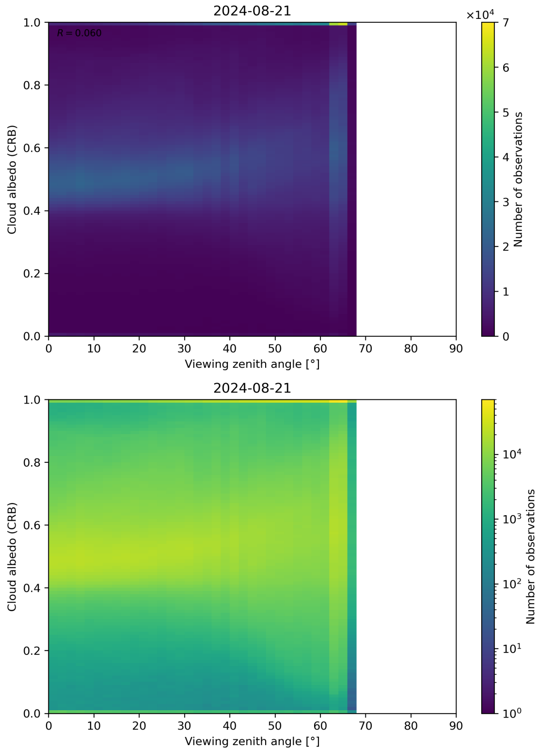
Figure 106: Scatter density plot of “Viewing zenith angle” against “Cloud albedo (CRB)” for 2024-08-21 to 2024-08-22.
