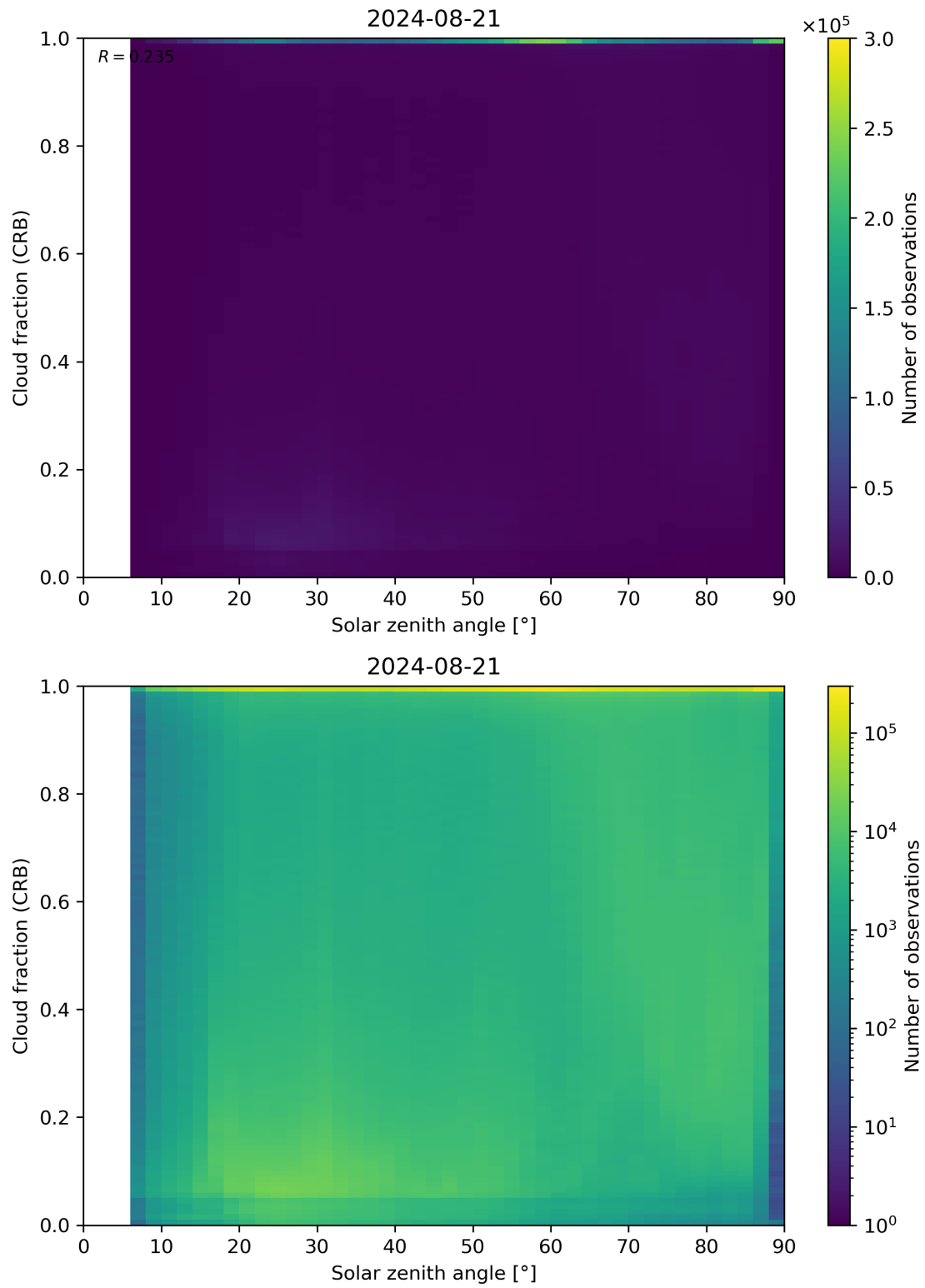
Figure 101: Scatter density plot of “Solar zenith angle” against “Cloud fraction (CRB)” for 2024-08-21 to 2024-08-22.
