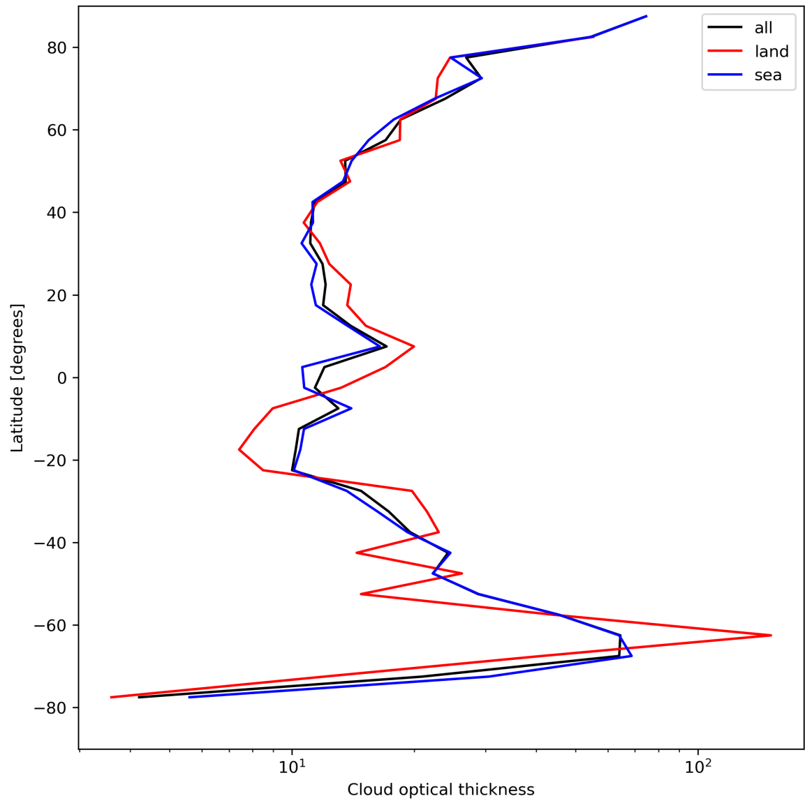
Figure 25: Zonal average of “Cloud optical thickness” for 2024-08-21 to 2024-08-22.
