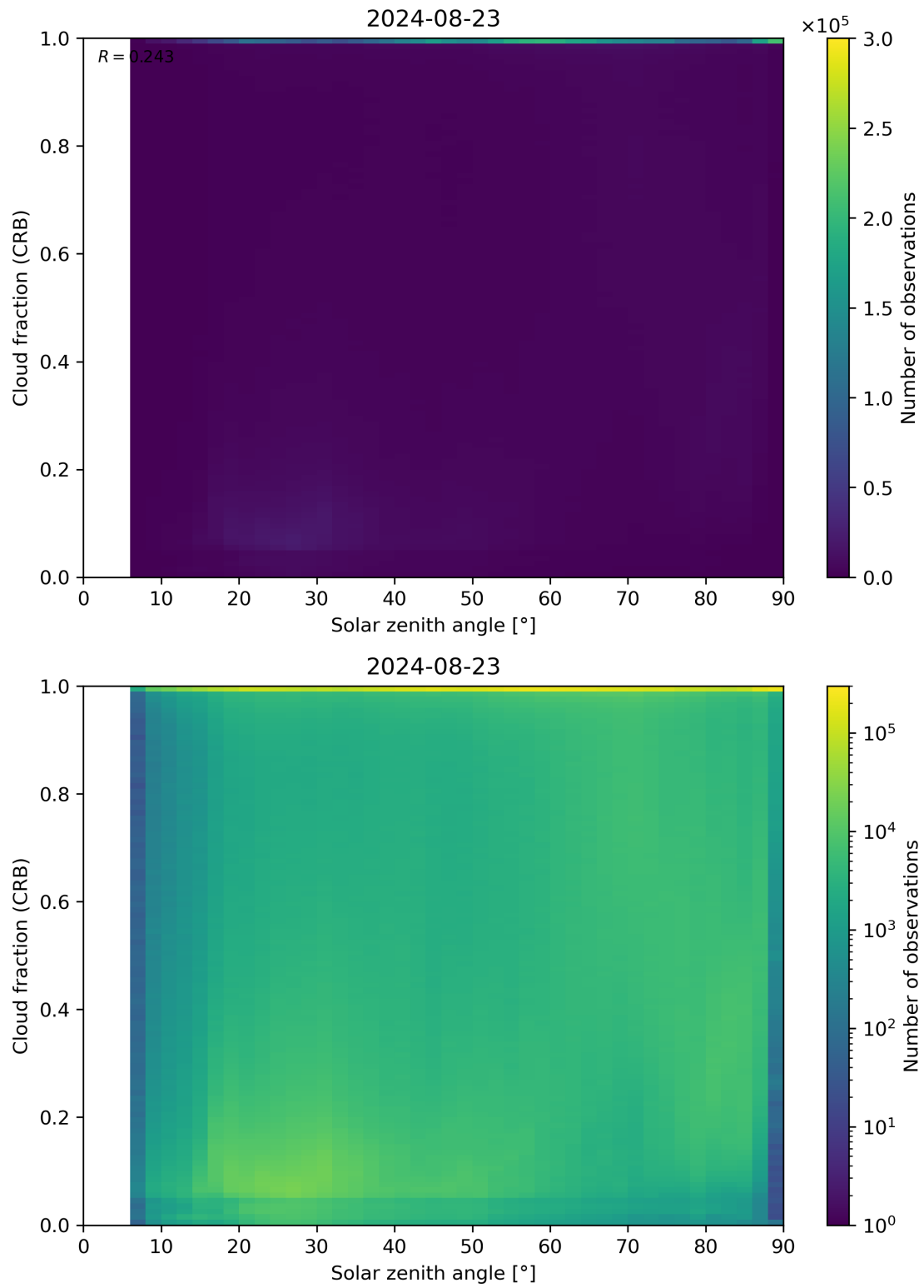
Figure 101: Scatter density plot of “Solar zenith angle” against “Cloud fraction (CRB)” for 2024-08-22 to 2024-08-24.
