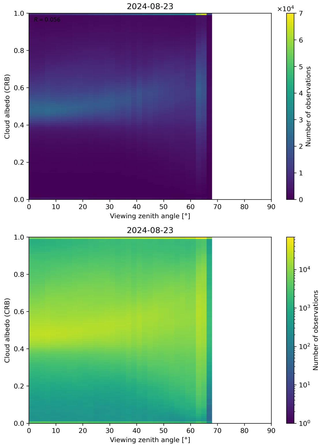
Figure 106: Scatter density plot of “Viewing zenith angle” against “Cloud albedo (CRB)” for 2024-08-22 to 2024-08-24.
