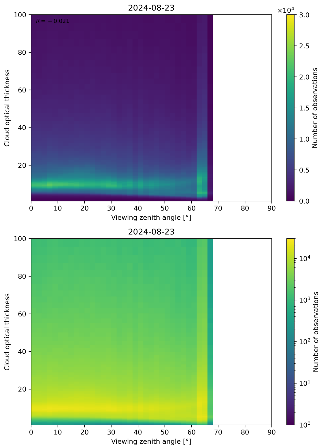
Figure 111: Scatter density plot of “Viewing zenith angle” against “Cloud optical thickness” for 2024-08-22 to 2024-08-24.
