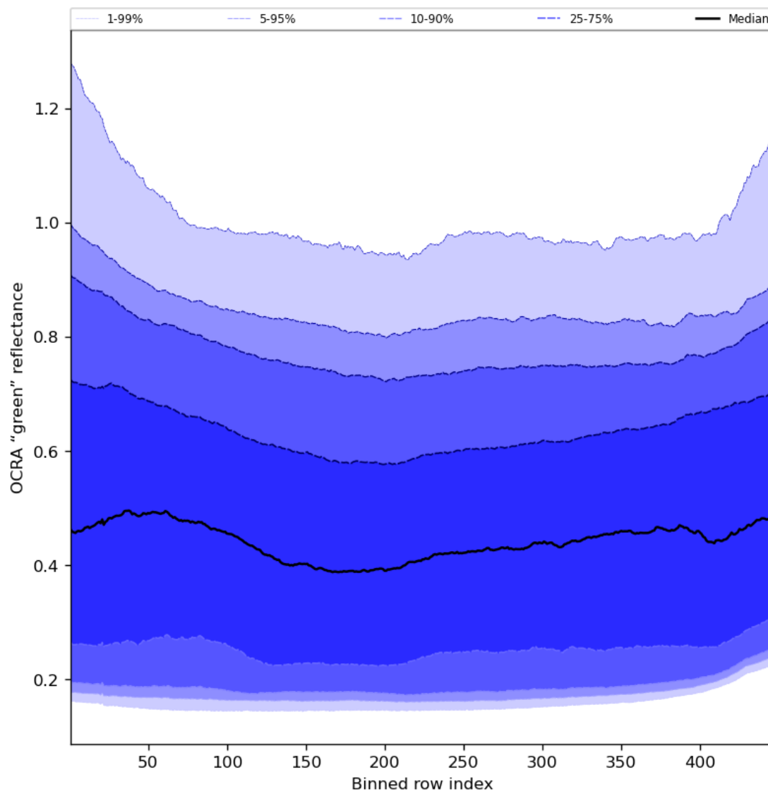
Figure 68: Along track statistics of “OCRA “green” reflectance” for 2024-08-22 to 2024-08-24
