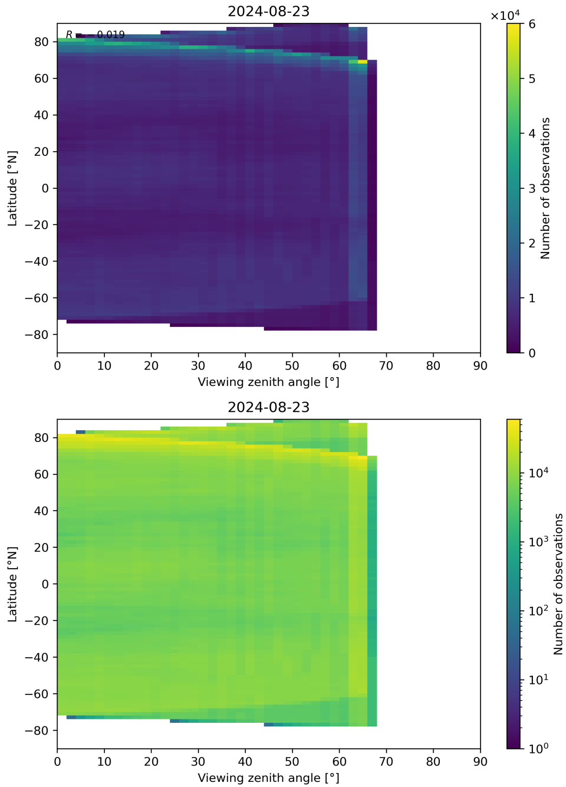
Figure 113: Scatter density plot of “Viewing zenith angle” against “Latitude” for 2024-08-22 to 2024-08-24.
