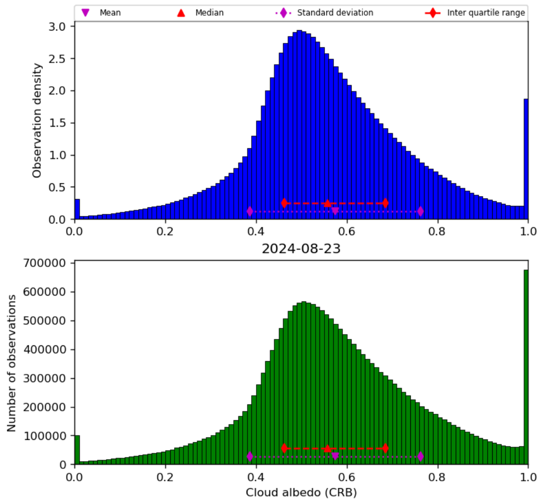
Figure 44: Histogram of “Cloud albedo (CRB)” for 2024-08-22 to 2024-08-24
