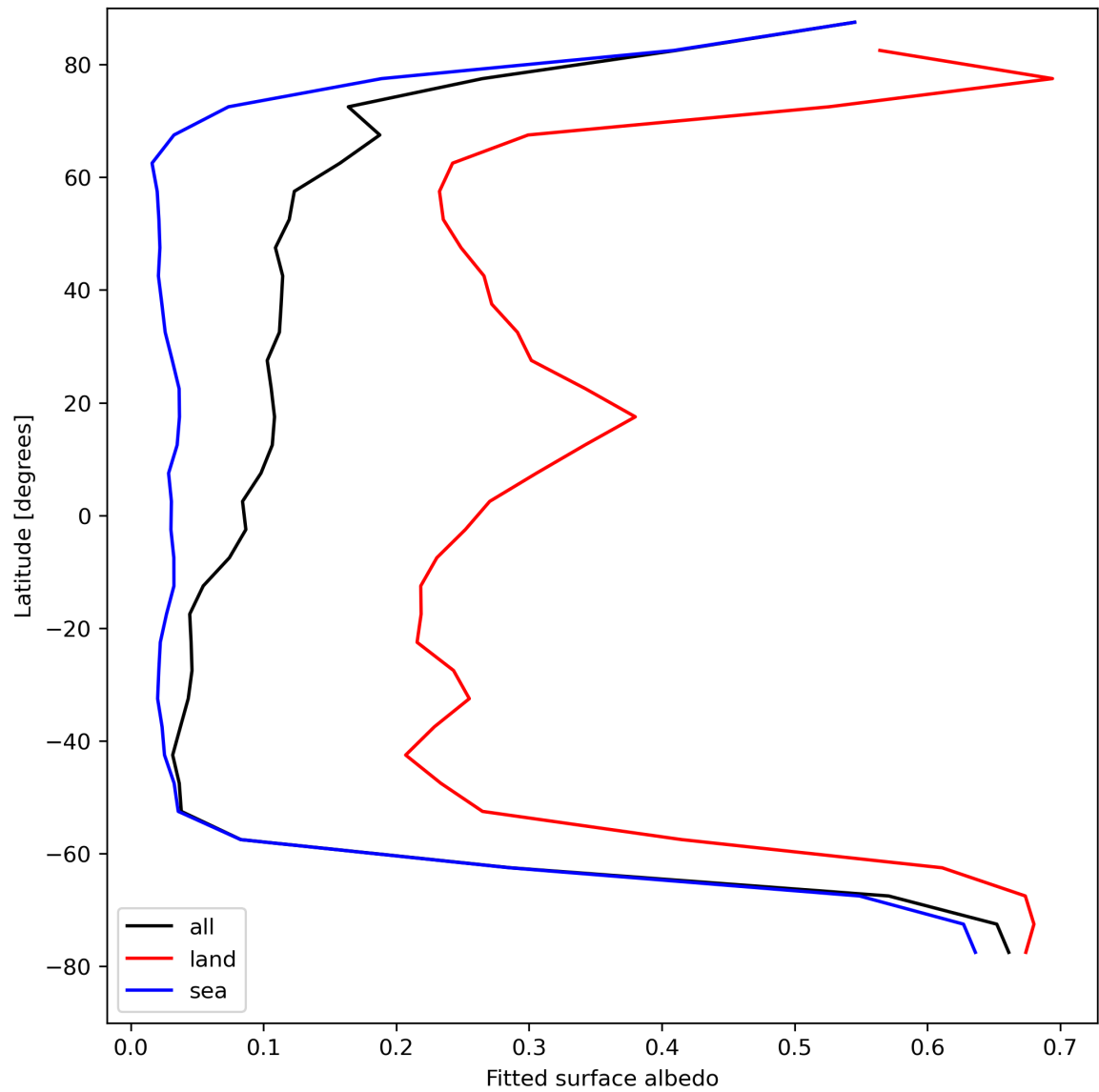
Figure 29: Zonal average of “Fitted surface albedo” for 2024-08-22 to 2024-08-24.
