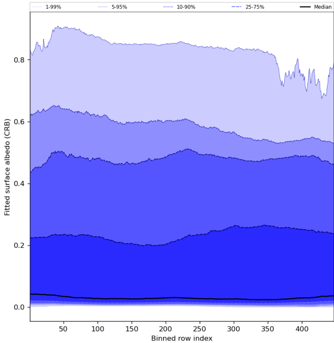
Figure 62: Along track statistics of “Fitted surface albedo (CRB)” for 2024-08-22 to 2024-08-24
