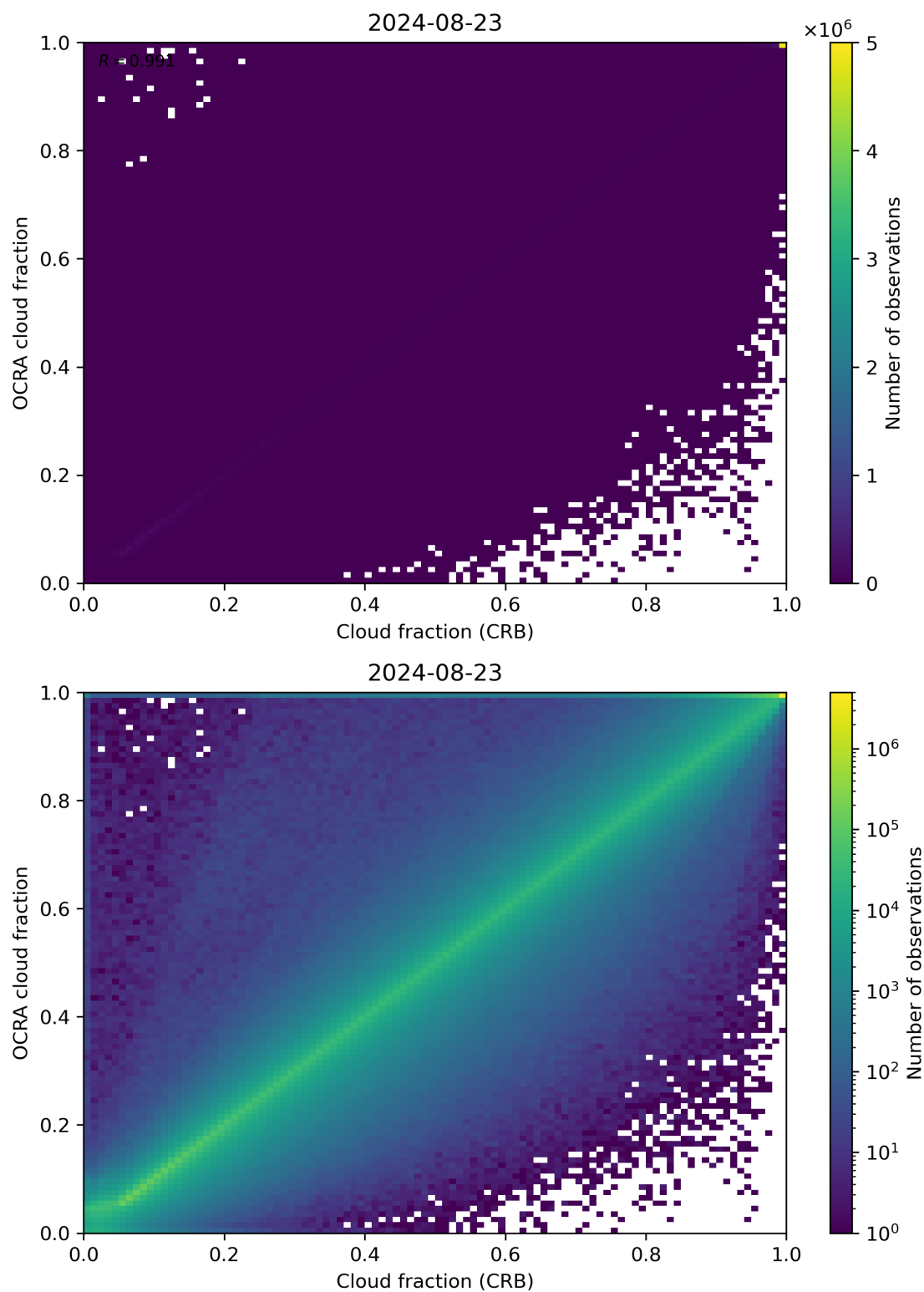
Figure 78: Scatter density plot of “Cloud fraction (CRB)” against “OCRA cloud fraction” for 2024-08-22 to 2024-08-24.
