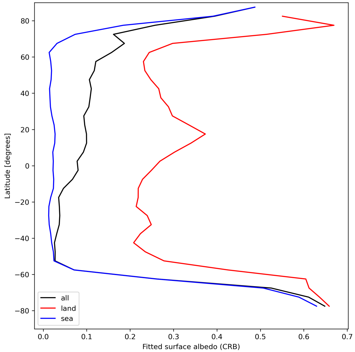
Figure 30: Zonal average of “Fitted surface albedo (CRB)” for 2024-08-22 to 2024-08-24.
