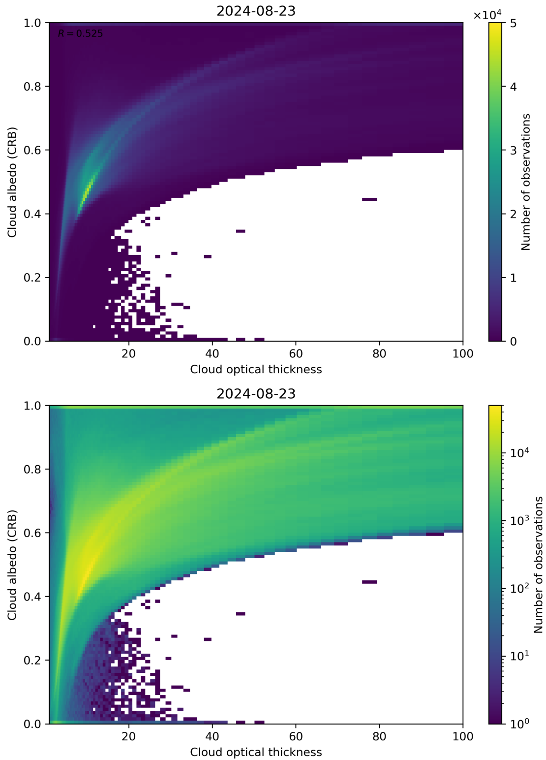
Figure 82: Scatter density plot of “Cloud optical thickness” against “Cloud albedo (CRB)” for 2024-08-22 to 2024-08-24.
