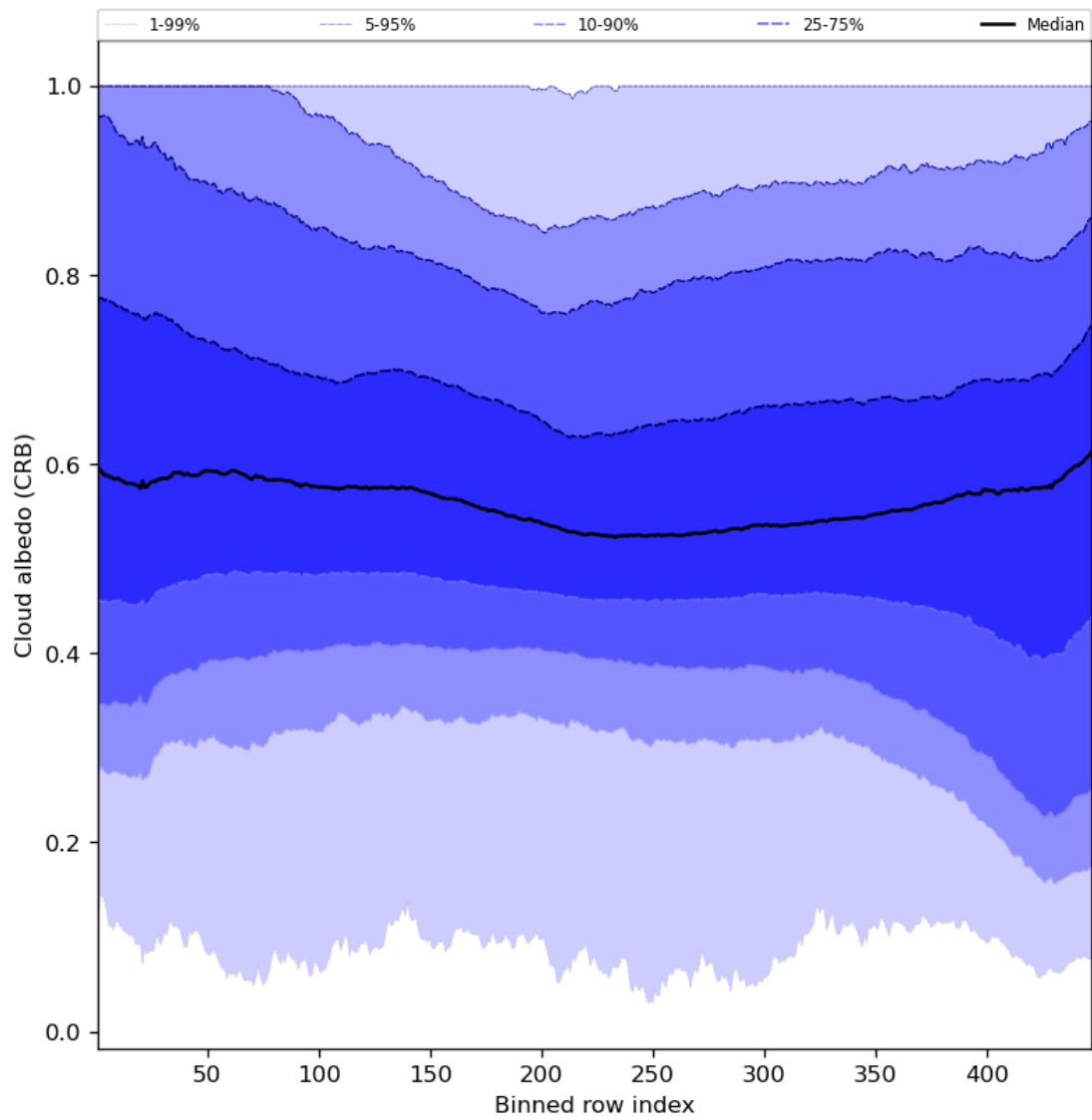
Figure 60: Along track statistics of “Cloud albedo (CRB)” for 2024-08-22 to 2024-08-24
