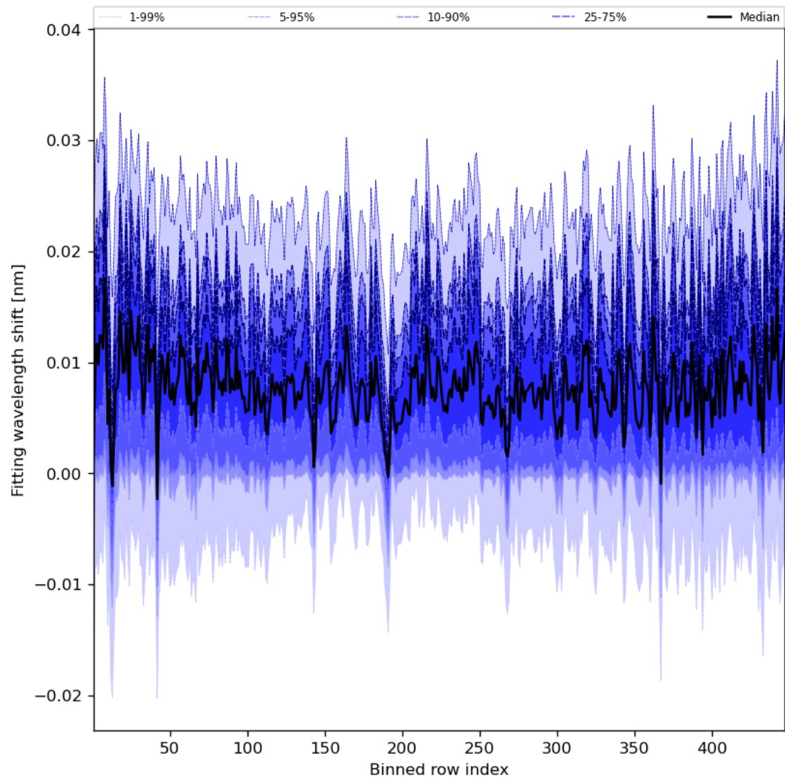
Figure 65: Along track statistics of “Fitting wavelength shift” for 2024-08-22 to 2024-08-24
