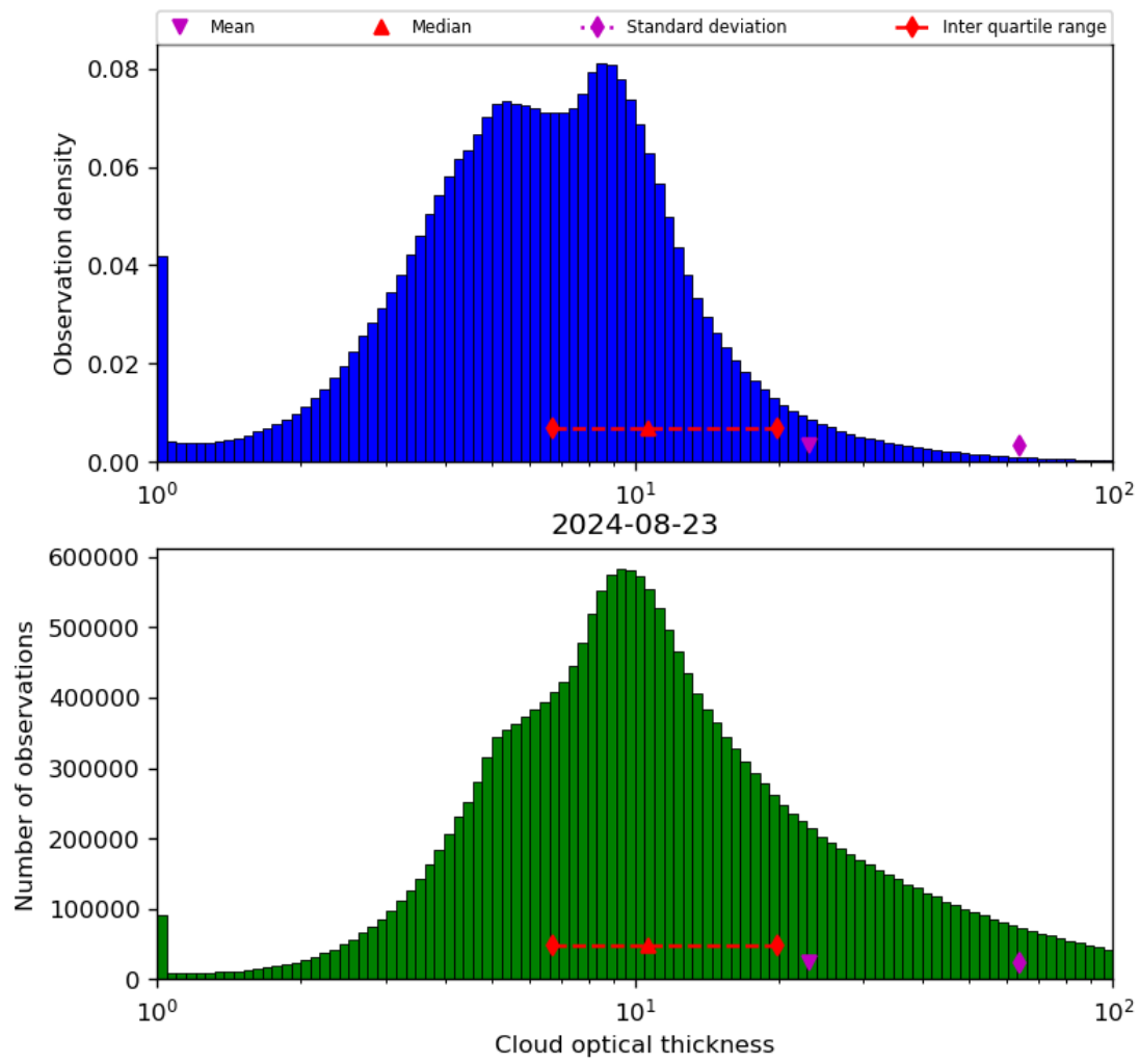
Figure 41: Histogram of “Cloud optical thickness” for 2024-08-22 to 2024-08-24
