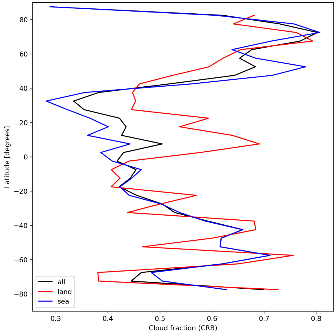
Figure 26: Zonal average of “Cloud fraction (CRB)” for 2024-08-22 to 2024-08-24.
