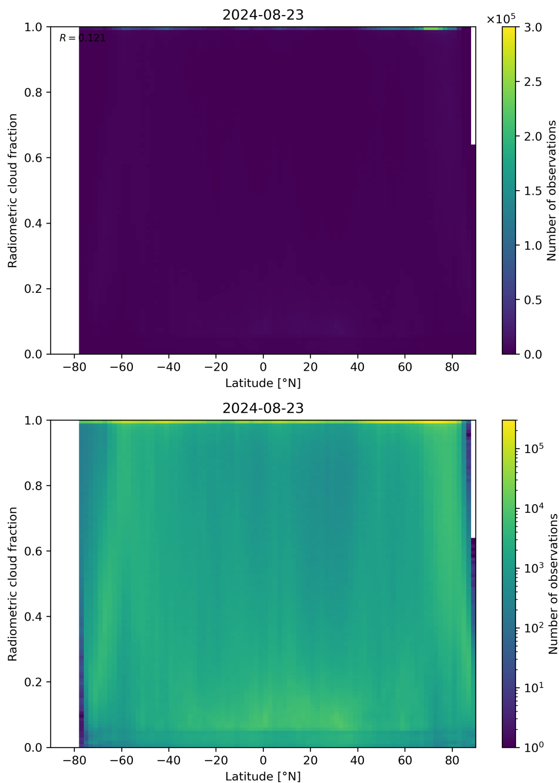
Figure 92: Scatter density plot of “Latitude” against “Radiometric cloud fraction” for 2024-08-22 to 2024-08-24.
