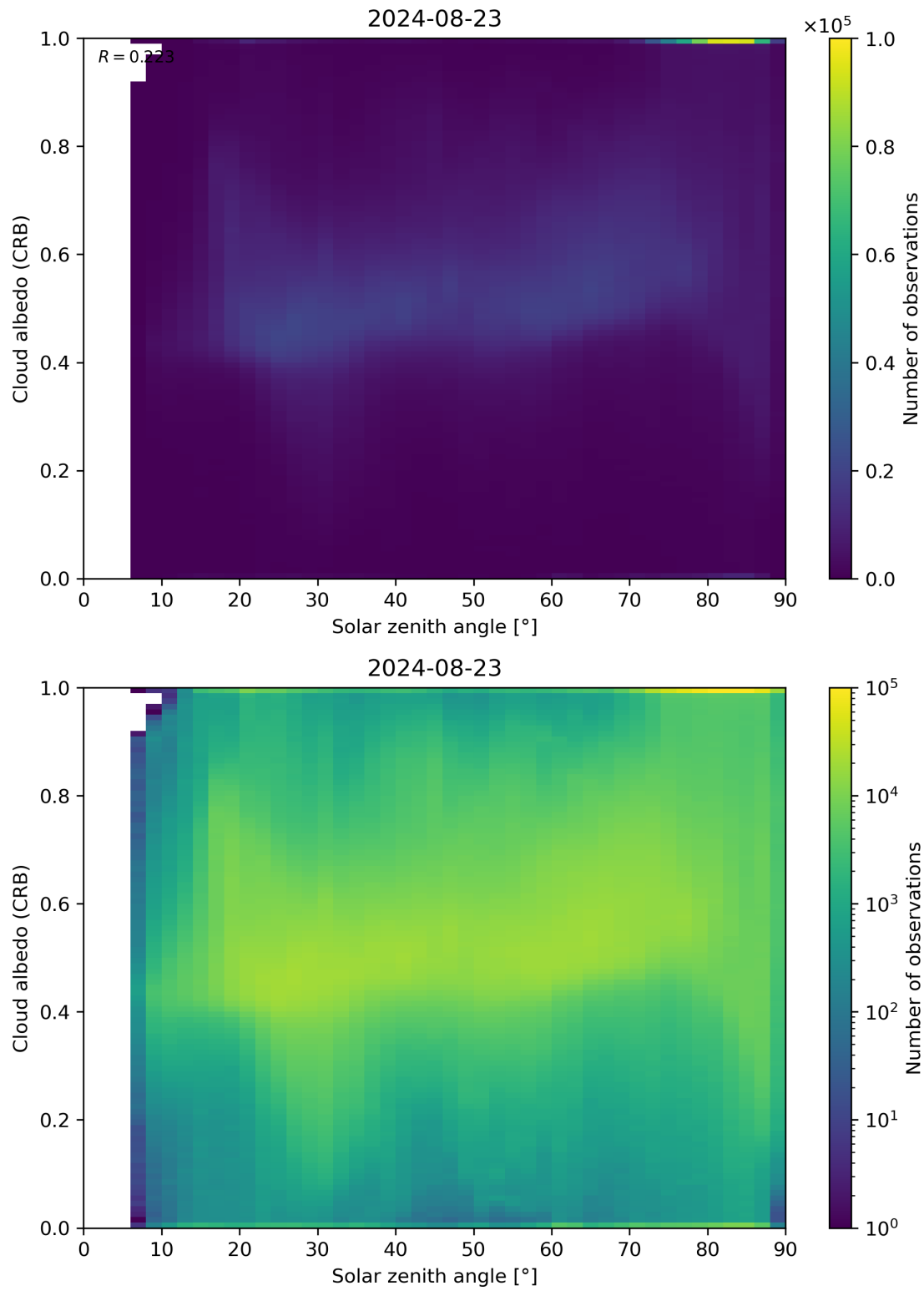
Figure 98: Scatter density plot of “Solar zenith angle” against “Cloud albedo (CRB)” for 2024-08-22 to 2024-08-24.
