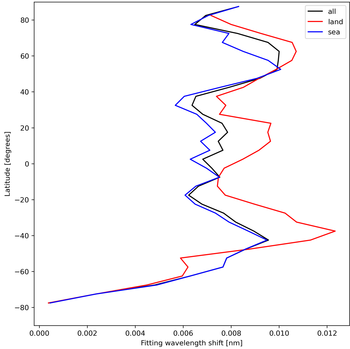
Figure 33: Zonal average of “Fitting wavelength shift” for 2024-08-22 to 2024-08-24.
