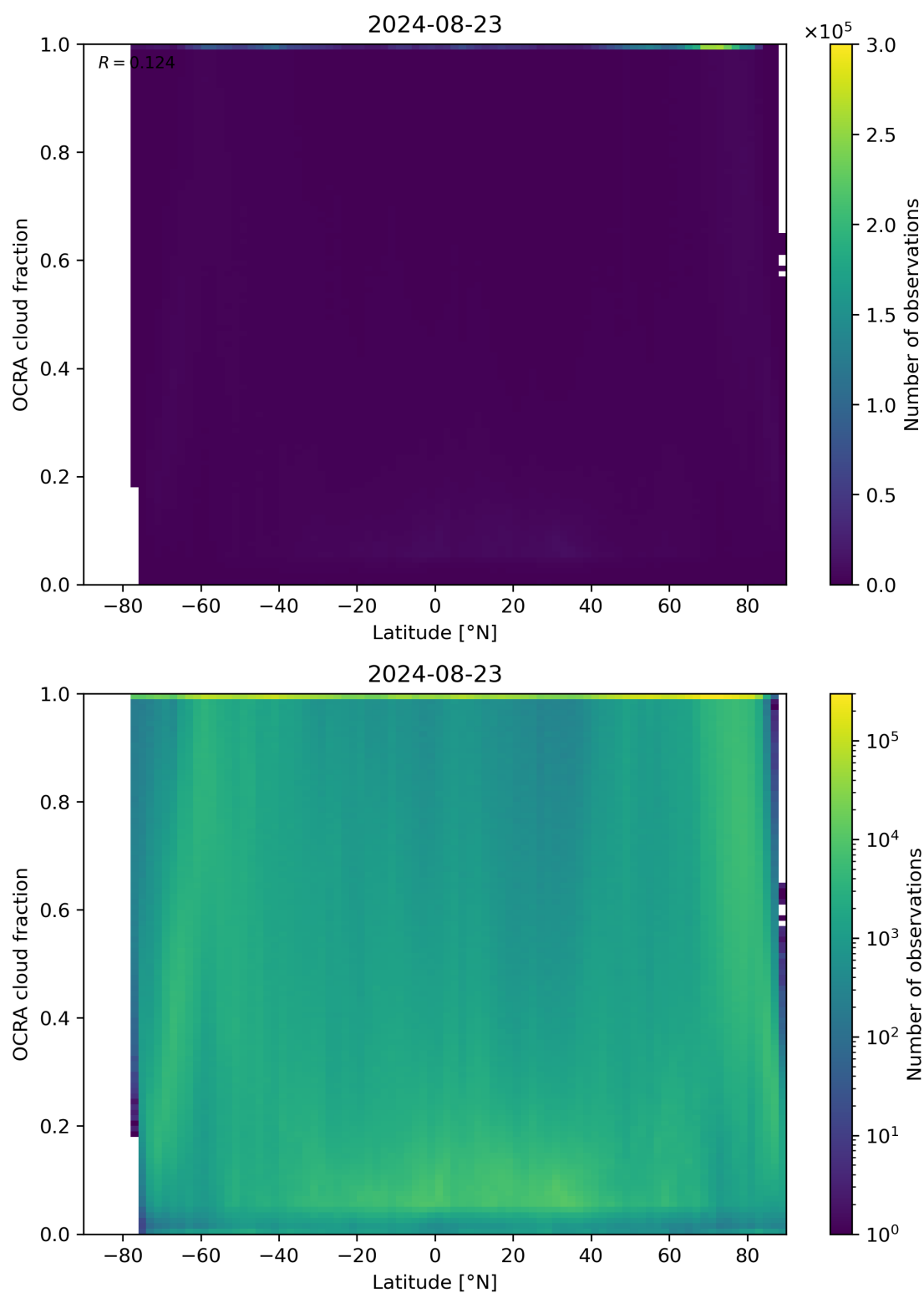
Figure 93: Scatter density plot of “Latitude” against “OCRA cloud fraction” for 2024-08-22 to 2024-08-24.
