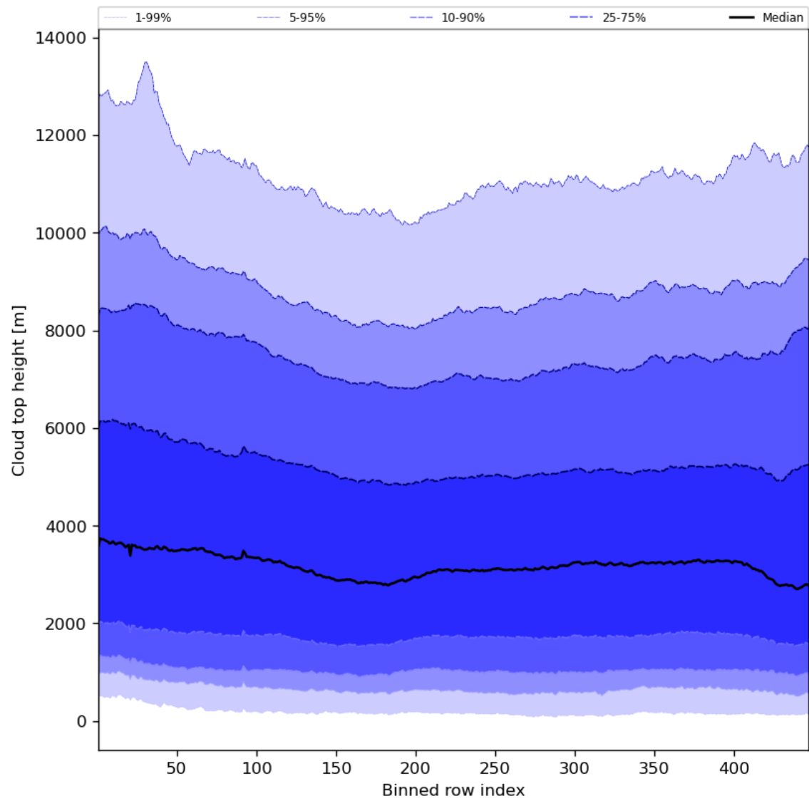
Figure 56: Along track statistics of “Cloud top height” for 2024-08-22 to 2024-08-24
