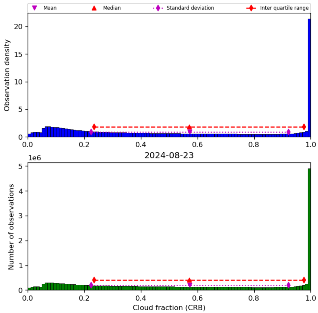
Figure 42: Histogram of “Cloud fraction (CRB)” for 2024-08-22 to 2024-08-24
