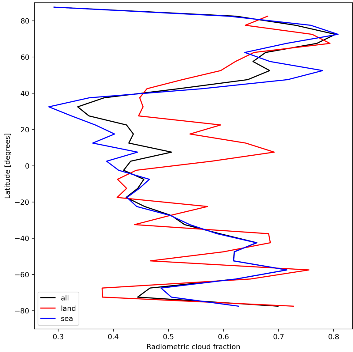
Figure 23: Zonal average of “Radiometric cloud fraction” for 2024-08-22 to 2024-08-24.
