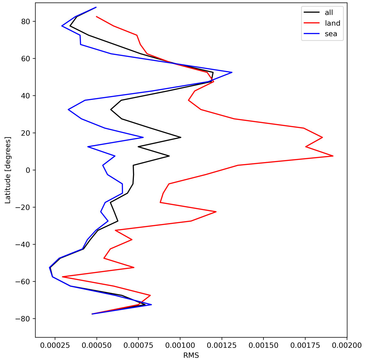
Figure 31: Zonal average of “RMS” for 2024-08-22 to 2024-08-24.
