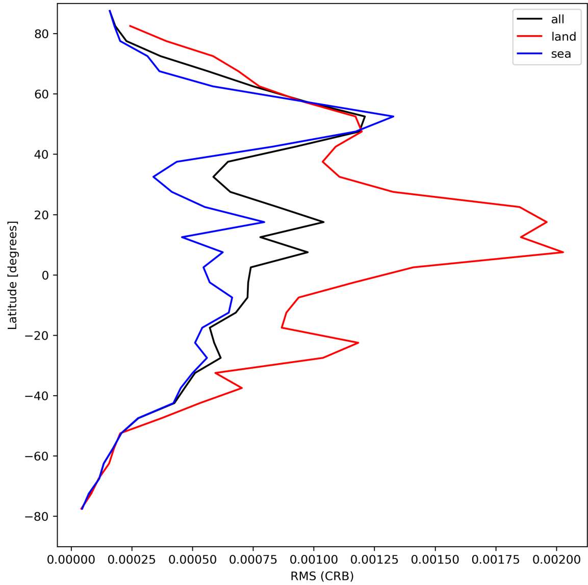
Figure 32: Zonal average of “RMS (CRB)” for 2024-08-22 to 2024-08-24.
