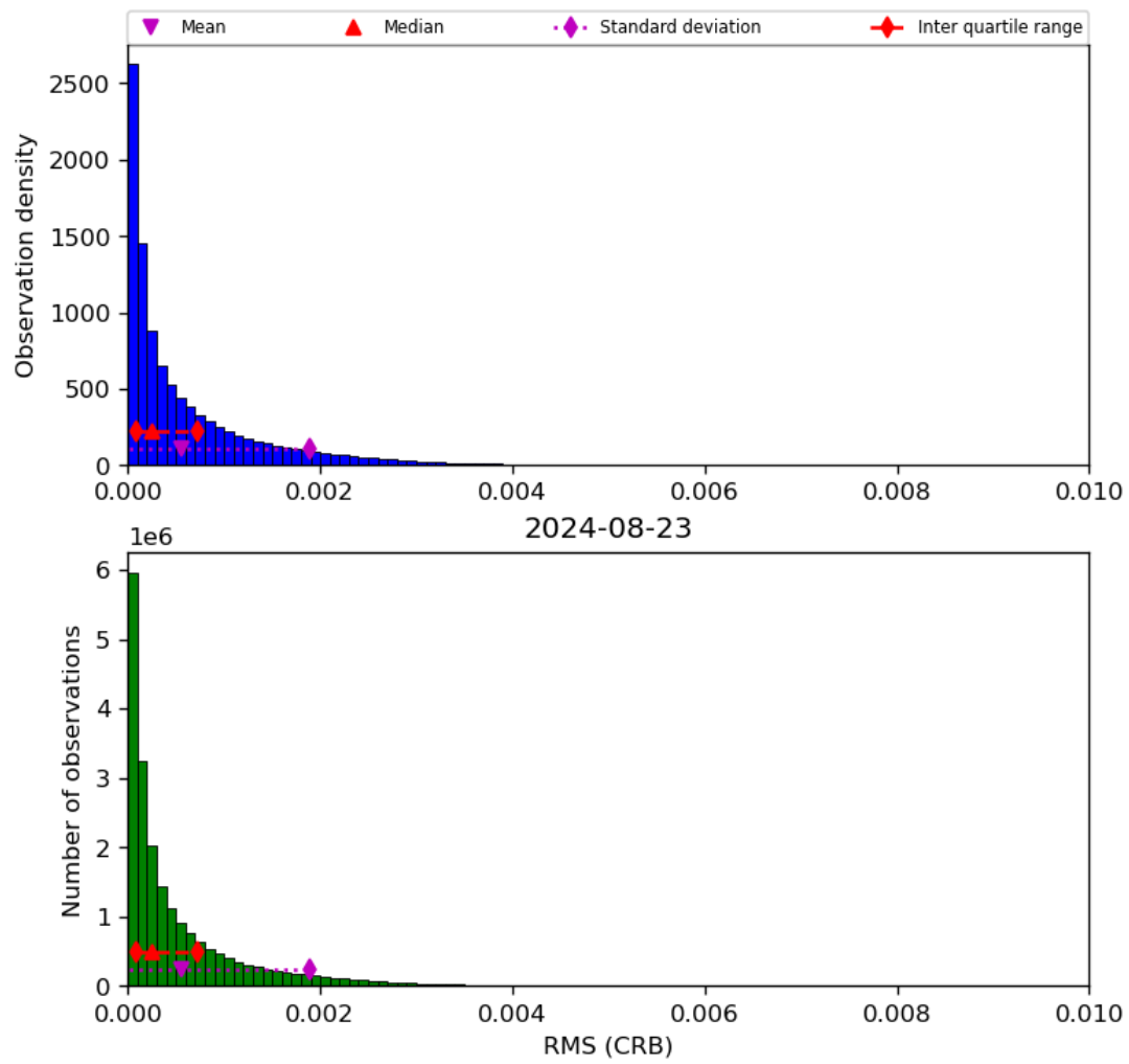
Figure 48: Histogram of “RMS (CRB)” for 2024-08-22 to 2024-08-24
