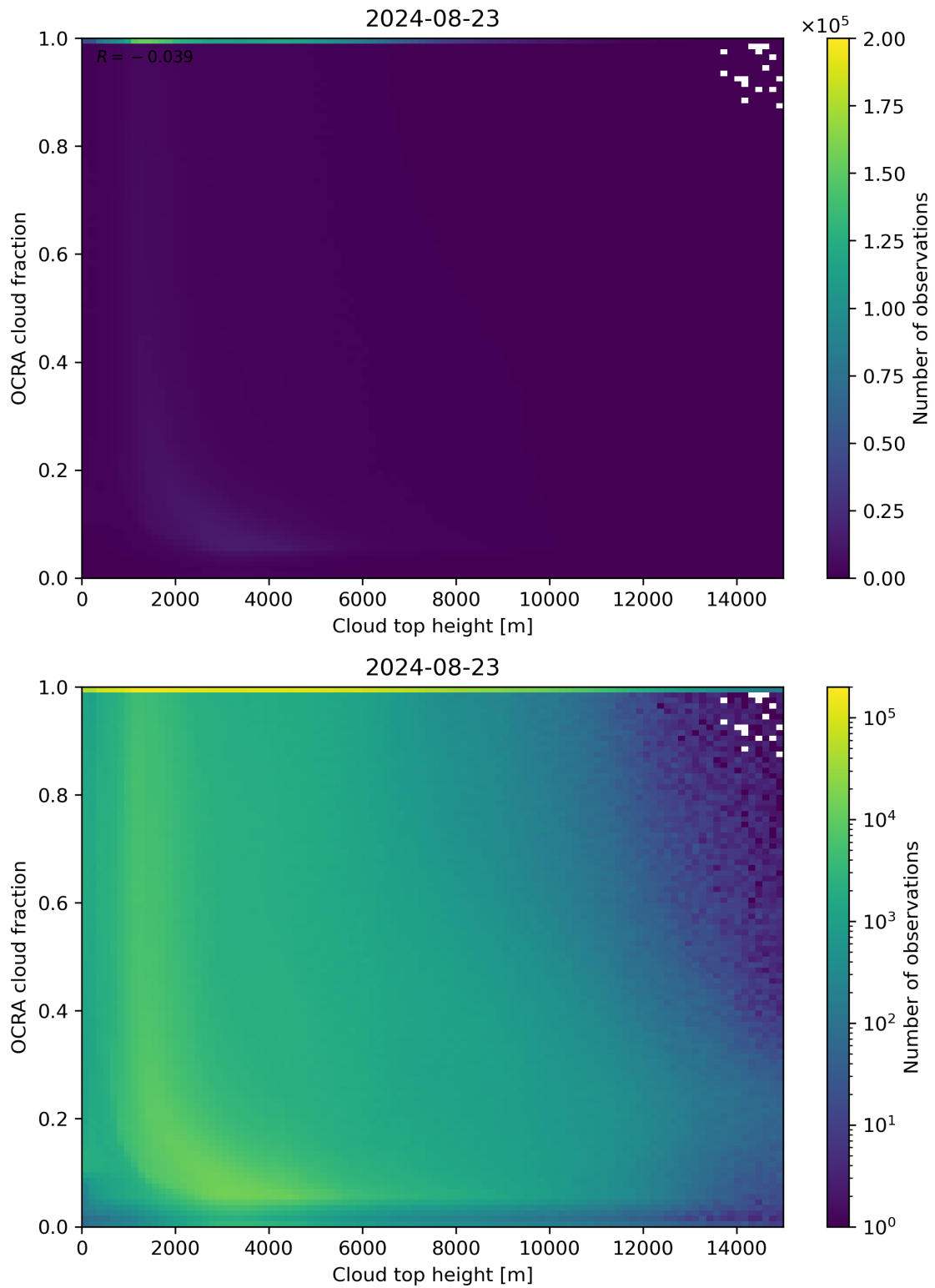
Figure 87: Scatter density plot of “Cloud top height” against “OCRA cloud fraction” for 2024-08-22 to 2024-08-24.
