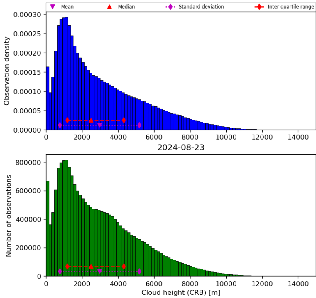
Figure 43: Histogram of “Cloud height (CRB)” for 2024-08-22 to 2024-08-24
