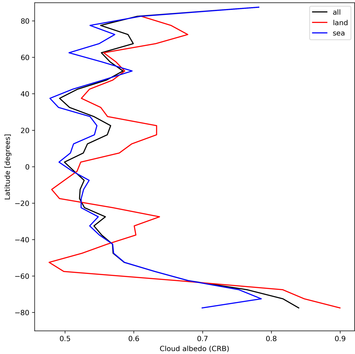
Figure 28: Zonal average of “Cloud albedo (CRB)” for 2024-08-22 to 2024-08-24.
