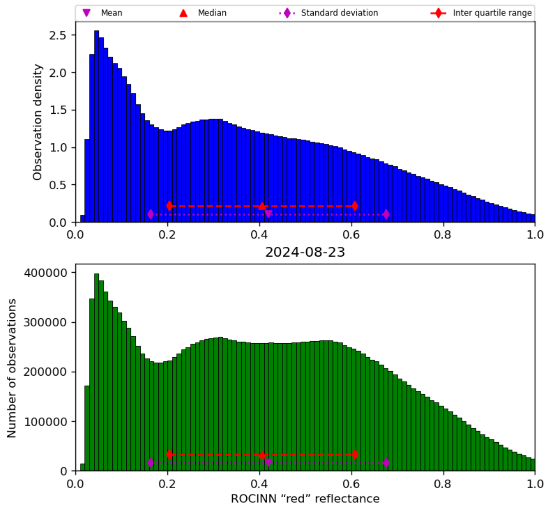
Figure 53: Histogram of “ROCINN “red” reflectance” for 2024-08-22 to 2024-08-24
