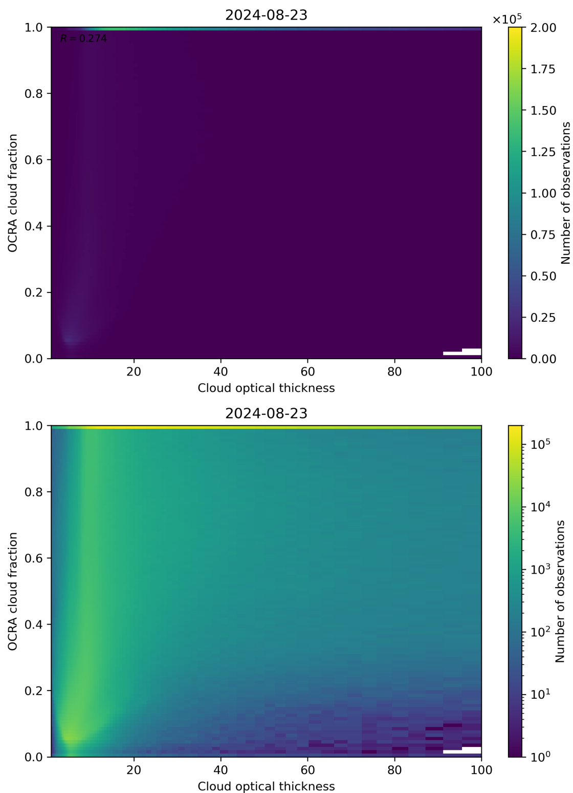
Figure 83: Scatter density plot of “Cloud optical thickness” against “OCRA cloud fraction” for 2024-08-22 to 2024-08-24.
