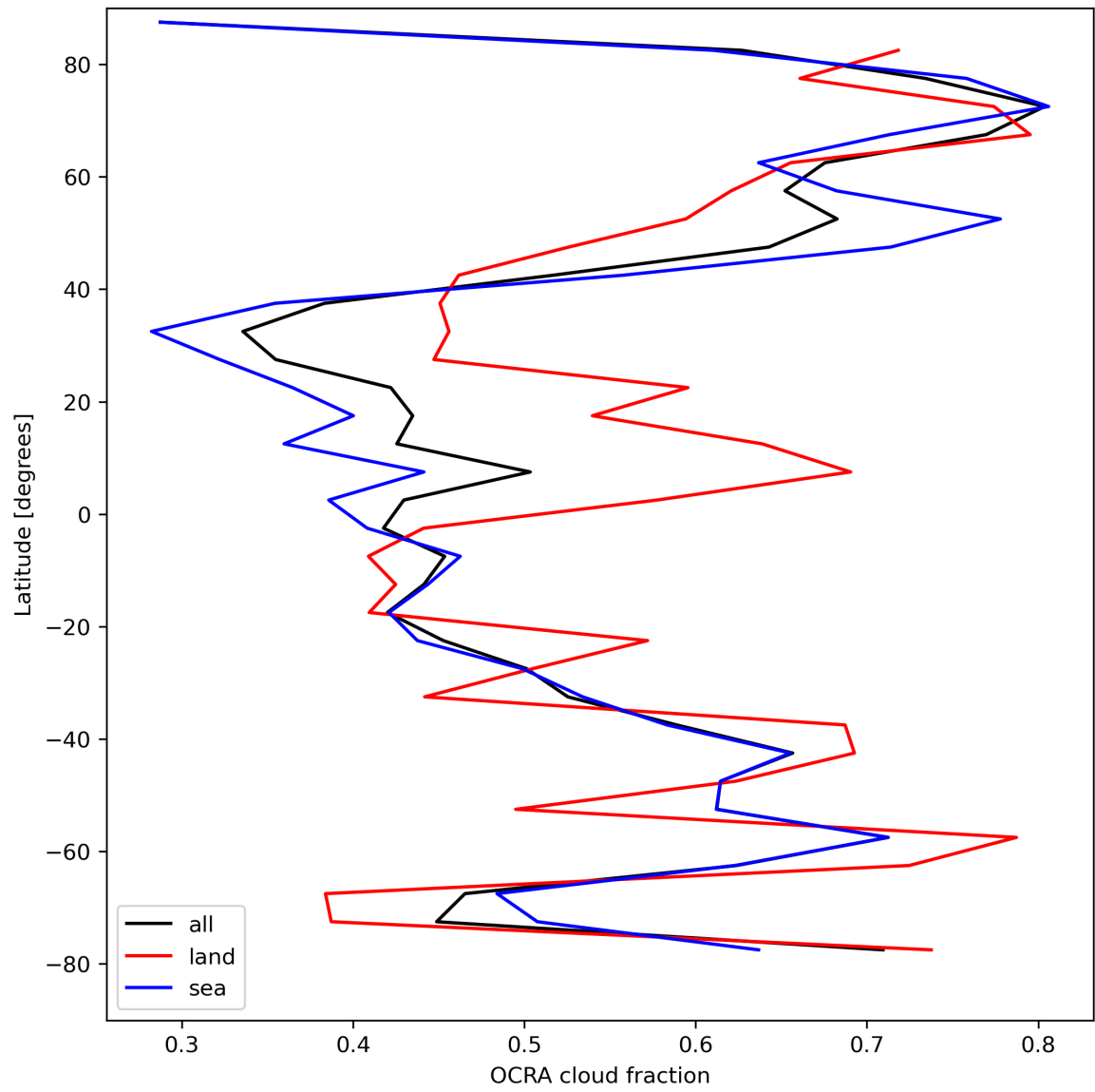
Figure 34: Zonal average of “OCRA cloud fraction” for 2024-08-22 to 2024-08-24.
