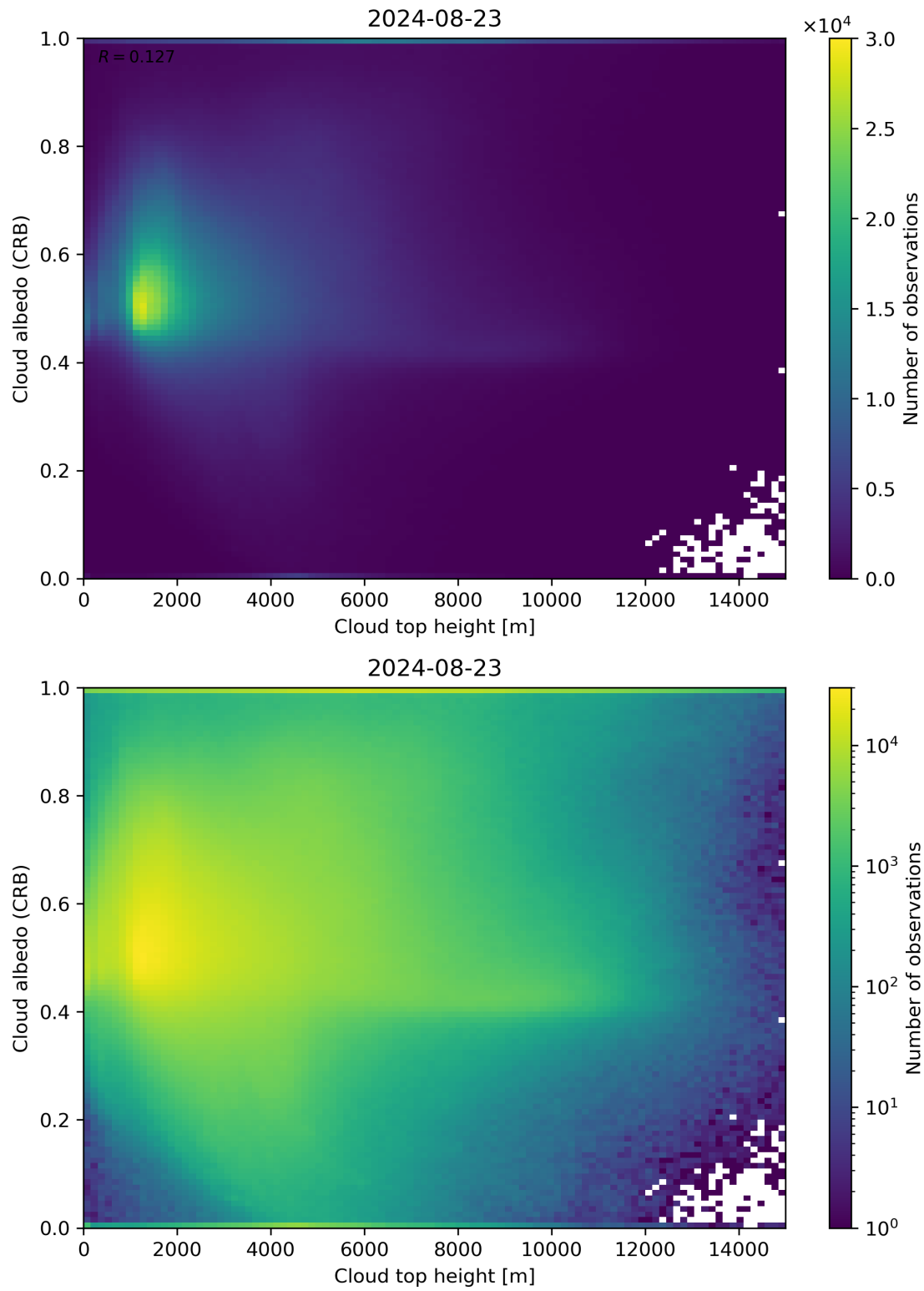
Figure 86: Scatter density plot of “Cloud top height” against “Cloud albedo (CRB)” for 2024-08-22 to 2024-08-24.
