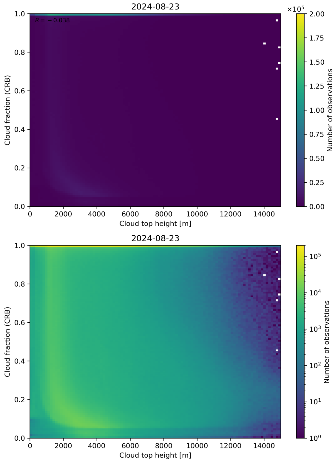
Figure 88: Scatter density plot of “Cloud top height” against “Cloud fraction (CRB)” for 2024-08-22 to 2024-08-24.
