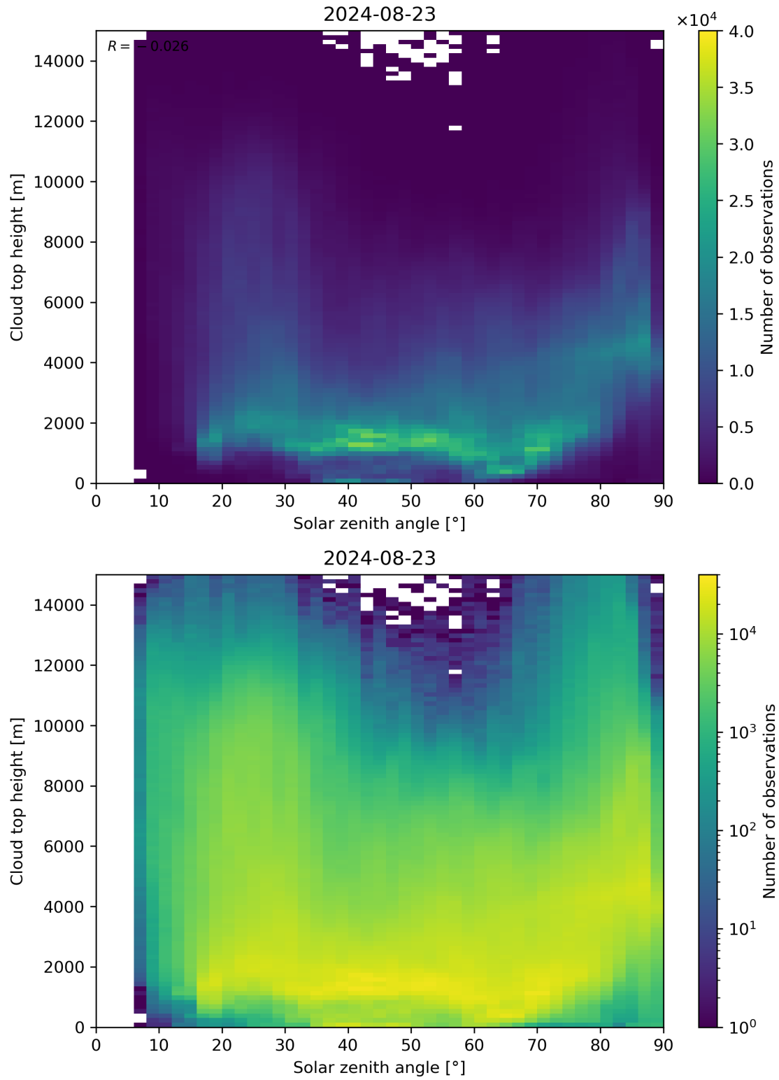
Figure 104: Scatter density plot of “Solar zenith angle” against “Cloud top height” for 2024-08-22 to 2024-08-24.
