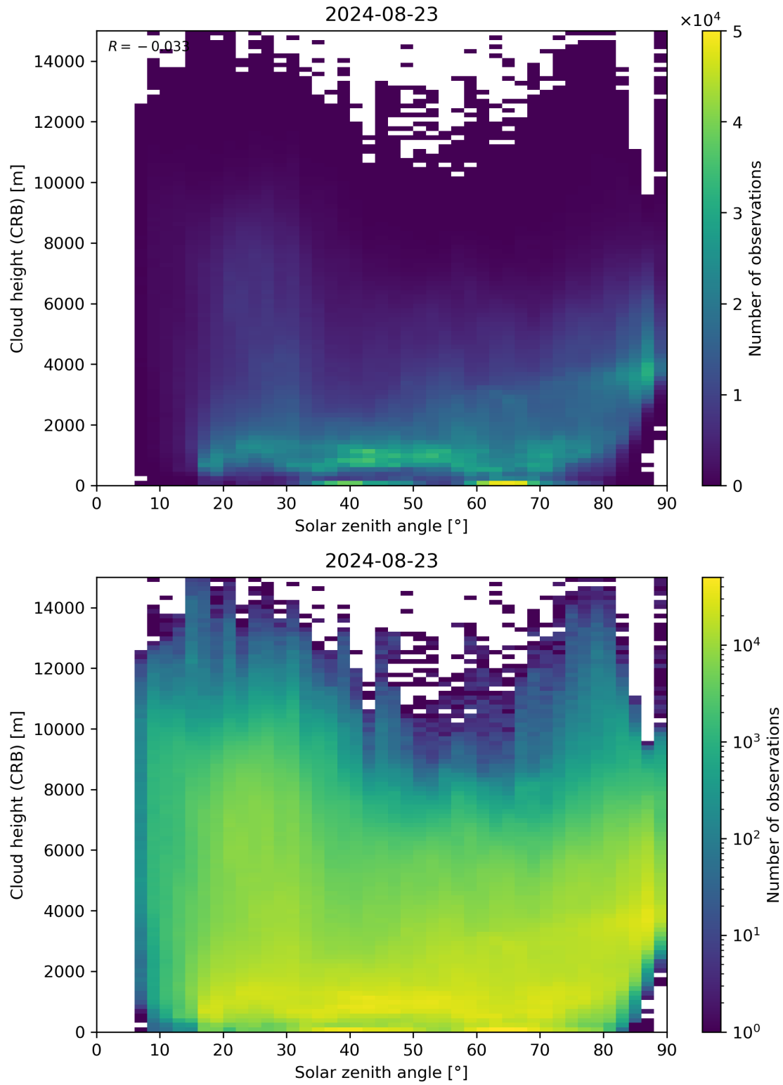
Figure 102: Scatter density plot of “Solar zenith angle” against “Cloud height (CRB)” for 2024-08-22 to 2024-08-24.
