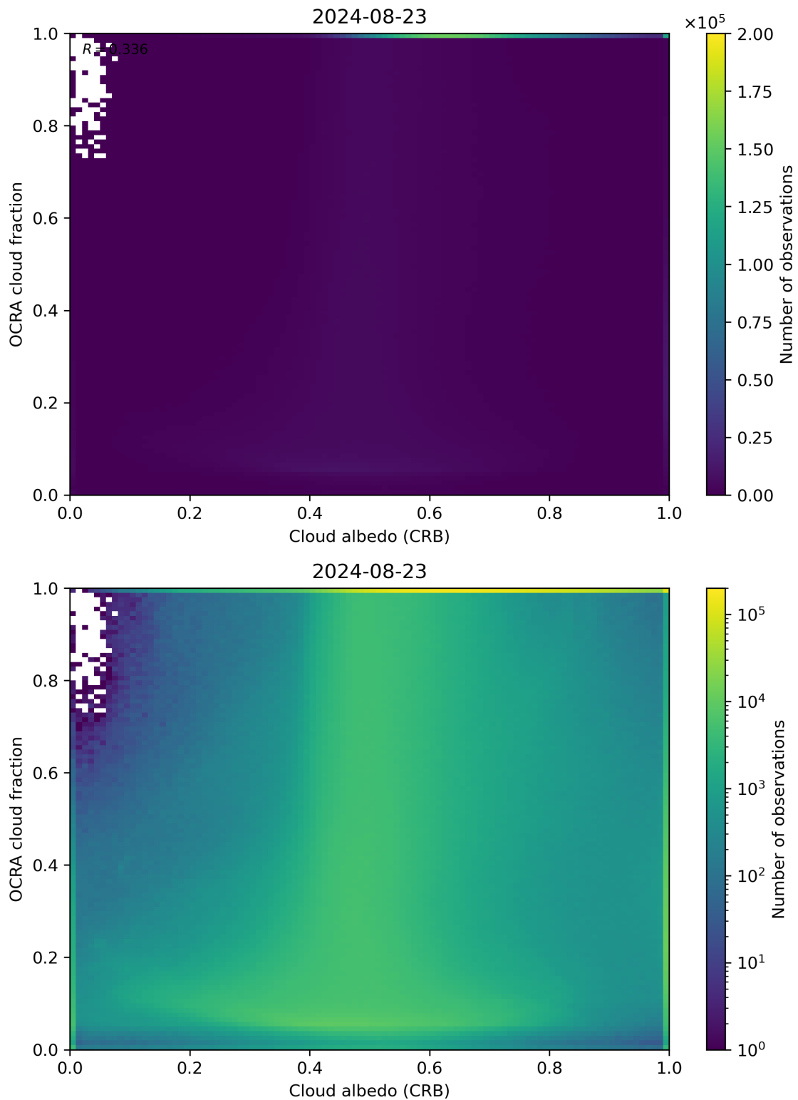
Figure 70: Scatter density plot of “Cloud albedo (CRB)” against “OCRA cloud fraction” for 2024-08-22 to 2024-08-24.
