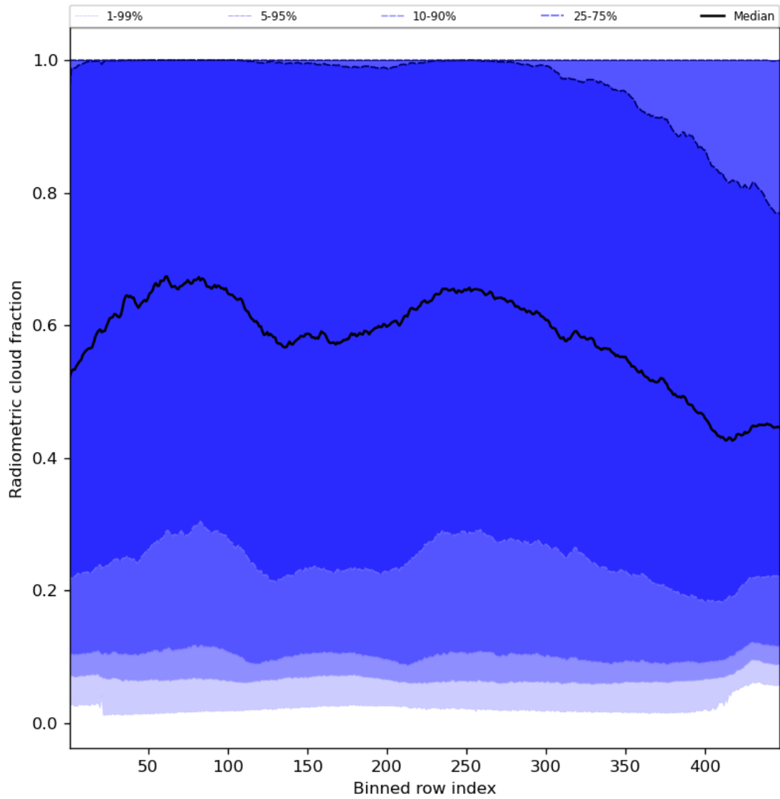
Figure 55: Along track statistics of “Radiometric cloud fraction” for 2024-08-22 to 2024-08-24
