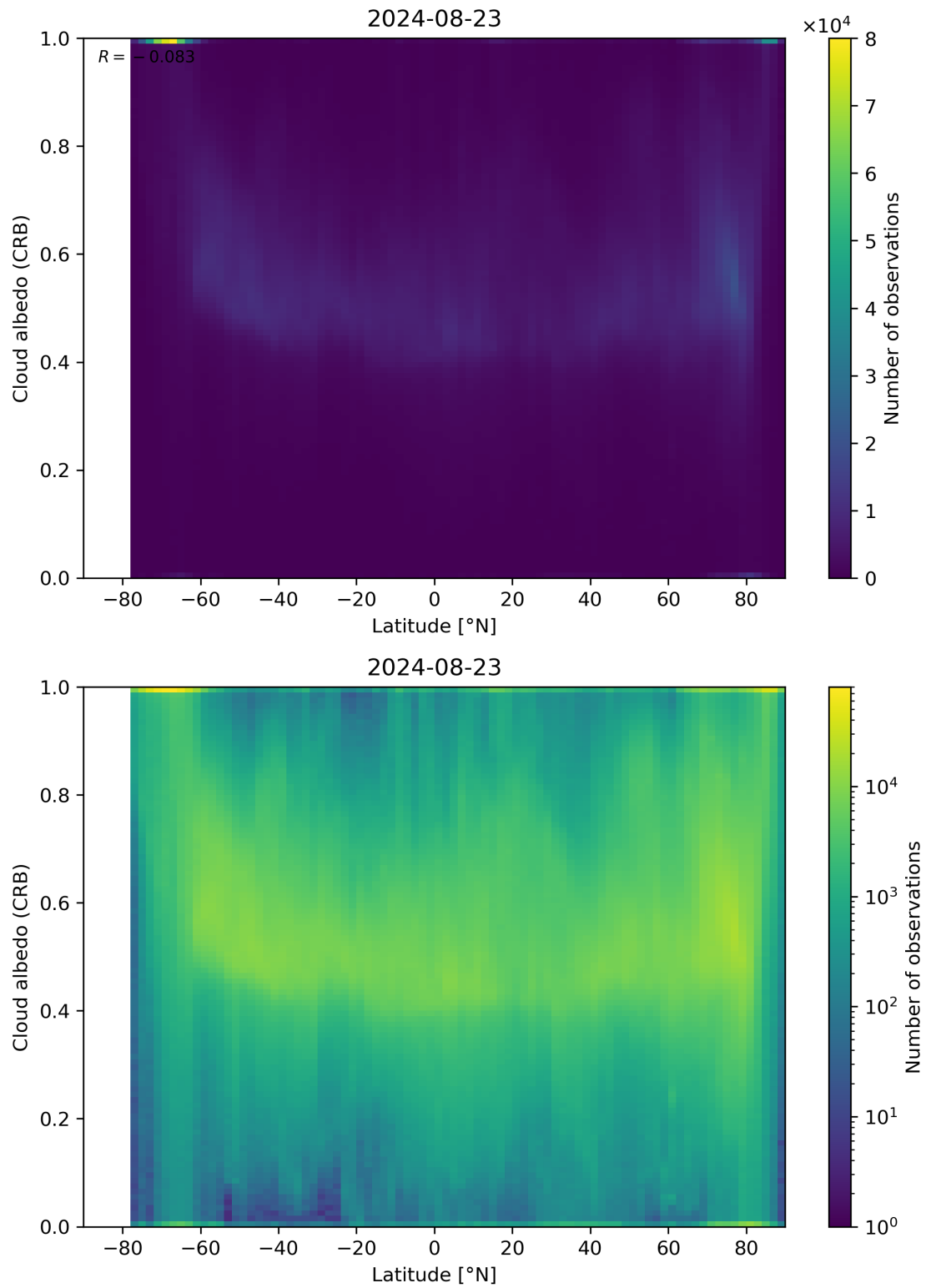
Figure 91: Scatter density plot of “Latitude” against “Cloud albedo (CRB)” for 2024-08-22 to 2024-08-24.
