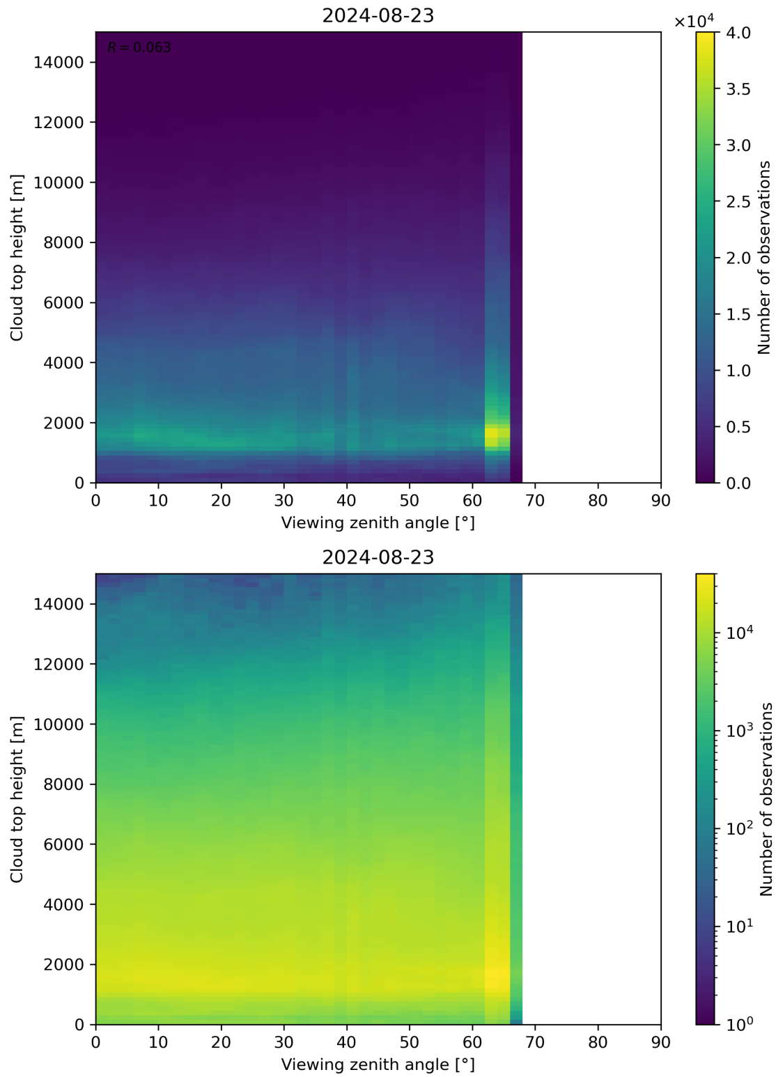
Figure 112: Scatter density plot of “Viewing zenith angle” against “Cloud top height” for 2024-08-22 to 2024-08-24.
