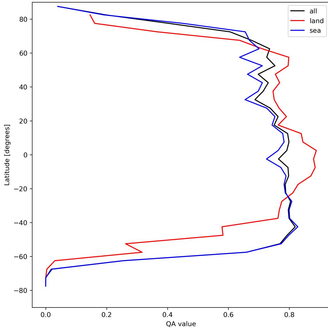
Figure 22: Zonal average of “QA value” for 2024-08-22 to 2024-08-24.
