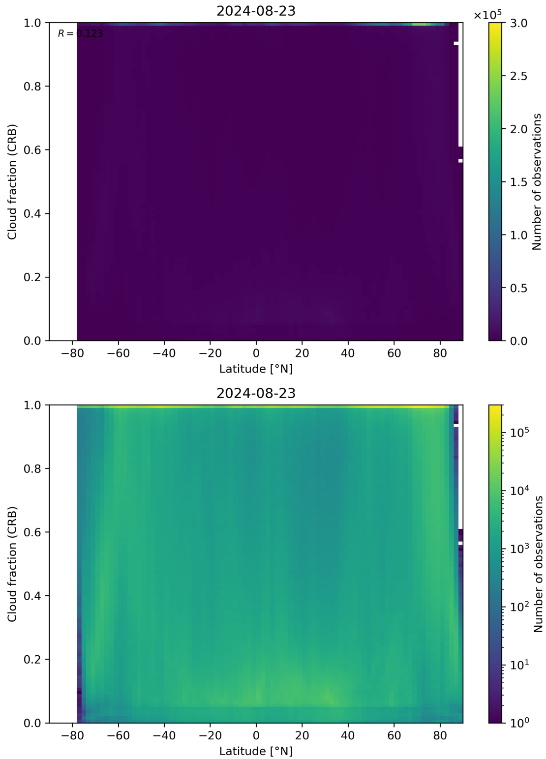
Figure 94: Scatter density plot of “Latitude” against “Cloud fraction (CRB)” for 2024-08-22 to 2024-08-24.
