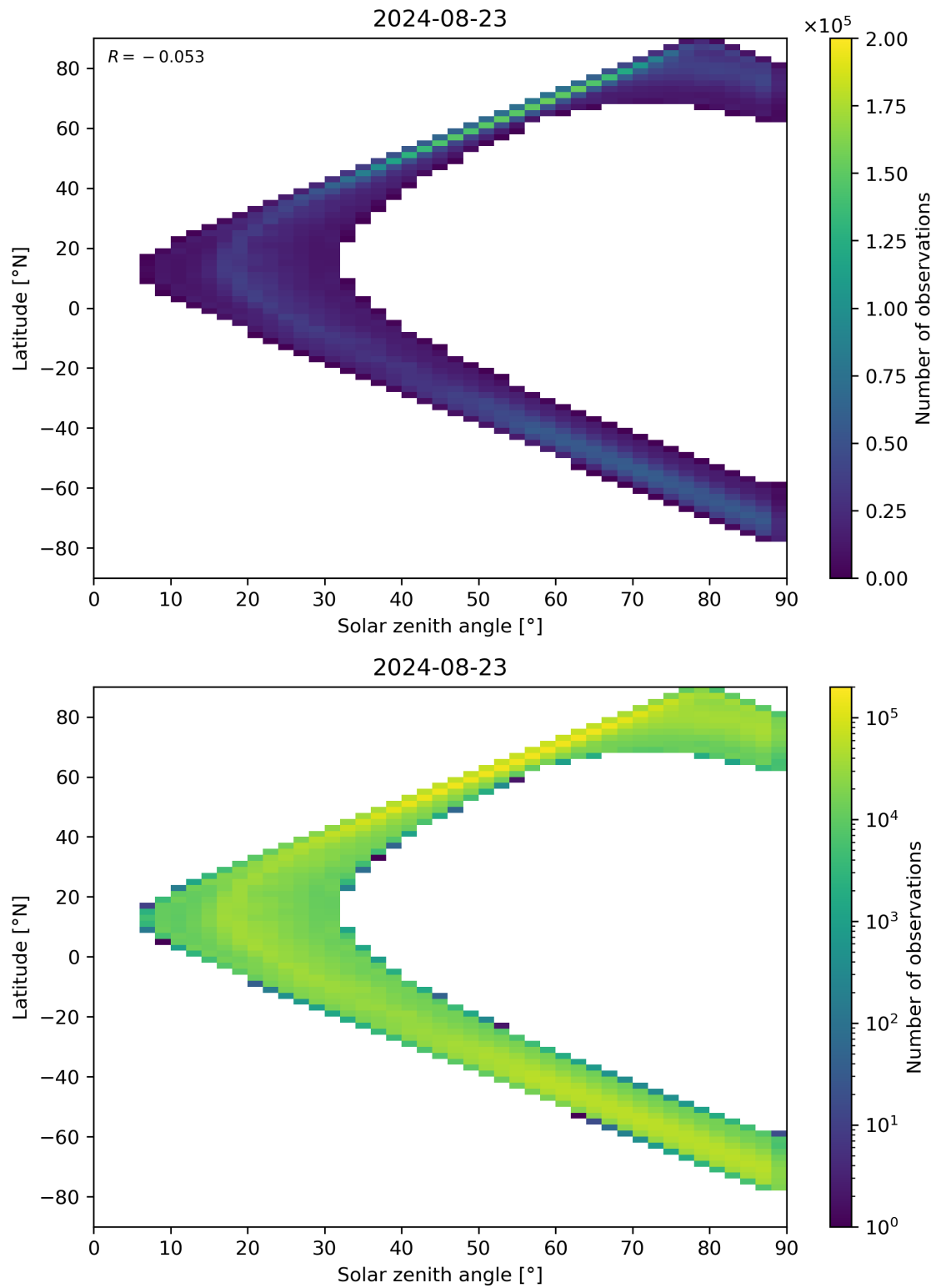
Figure 105: Scatter density plot of “Solar zenith angle” against “Latitude” for 2024-08-22 to 2024-08-24.
