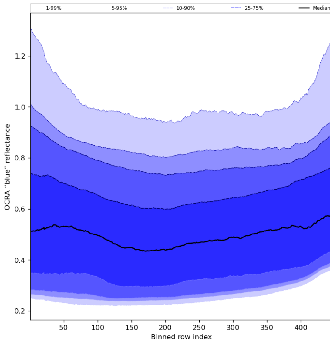
Figure 67: Along track statistics of “OCRA “blue” reflectance” for 2024-08-22 to 2024-08-24
