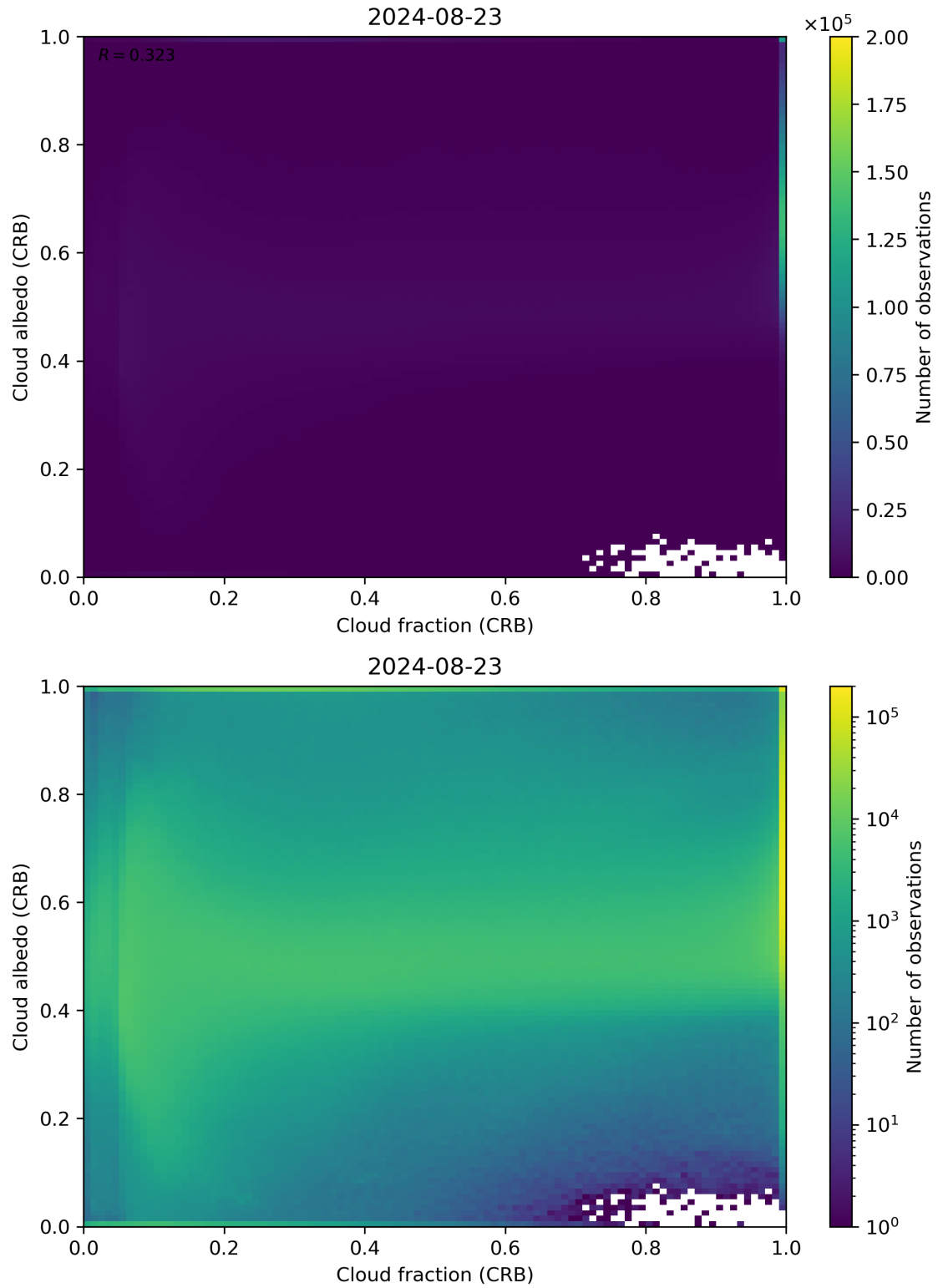
Figure 77: Scatter density plot of “Cloud fraction (CRB)” against “Cloud albedo (CRB)” for 2024-08-22 to 2024-08-24.
