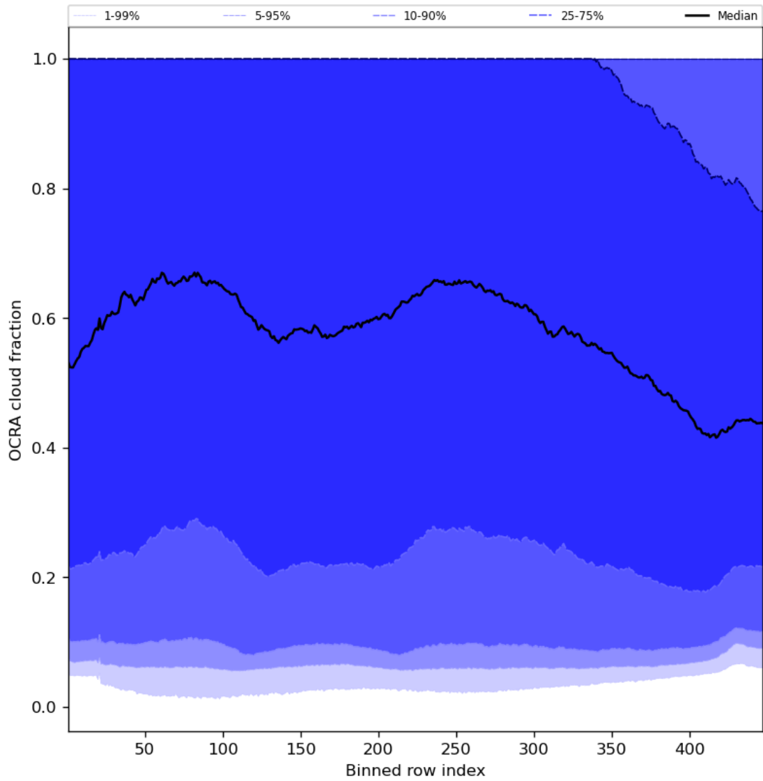
Figure 66: Along track statistics of “OCRA cloud fraction” for 2024-08-22 to 2024-08-24
