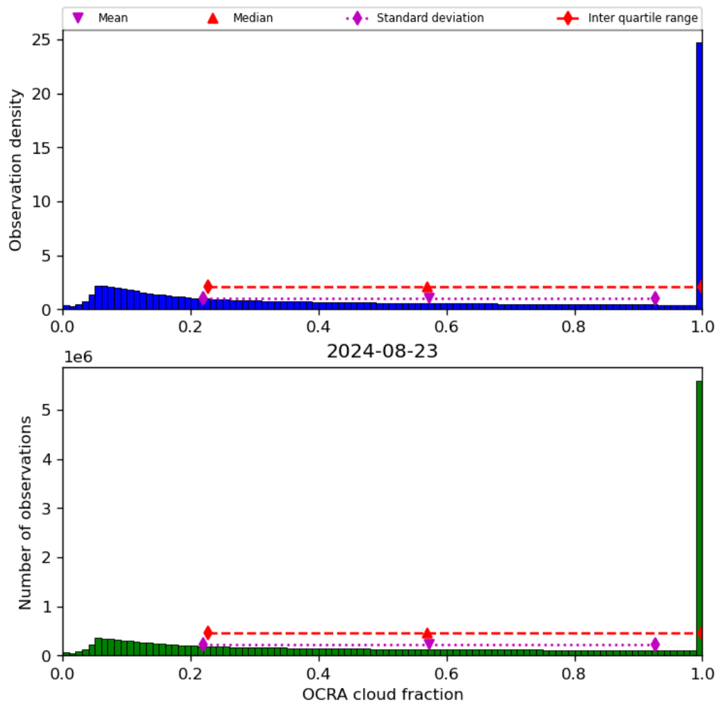
Figure 50: Histogram of “OCRA cloud fraction” for 2024-08-22 to 2024-08-24
