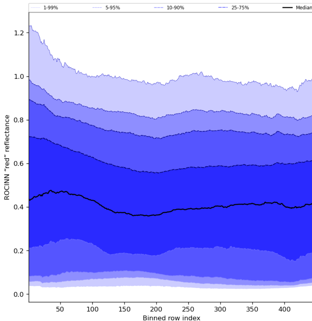
Figure 69: Along track statistics of “ROCINN “red” reflectance” for 2024-08-22 to 2024-08-24
