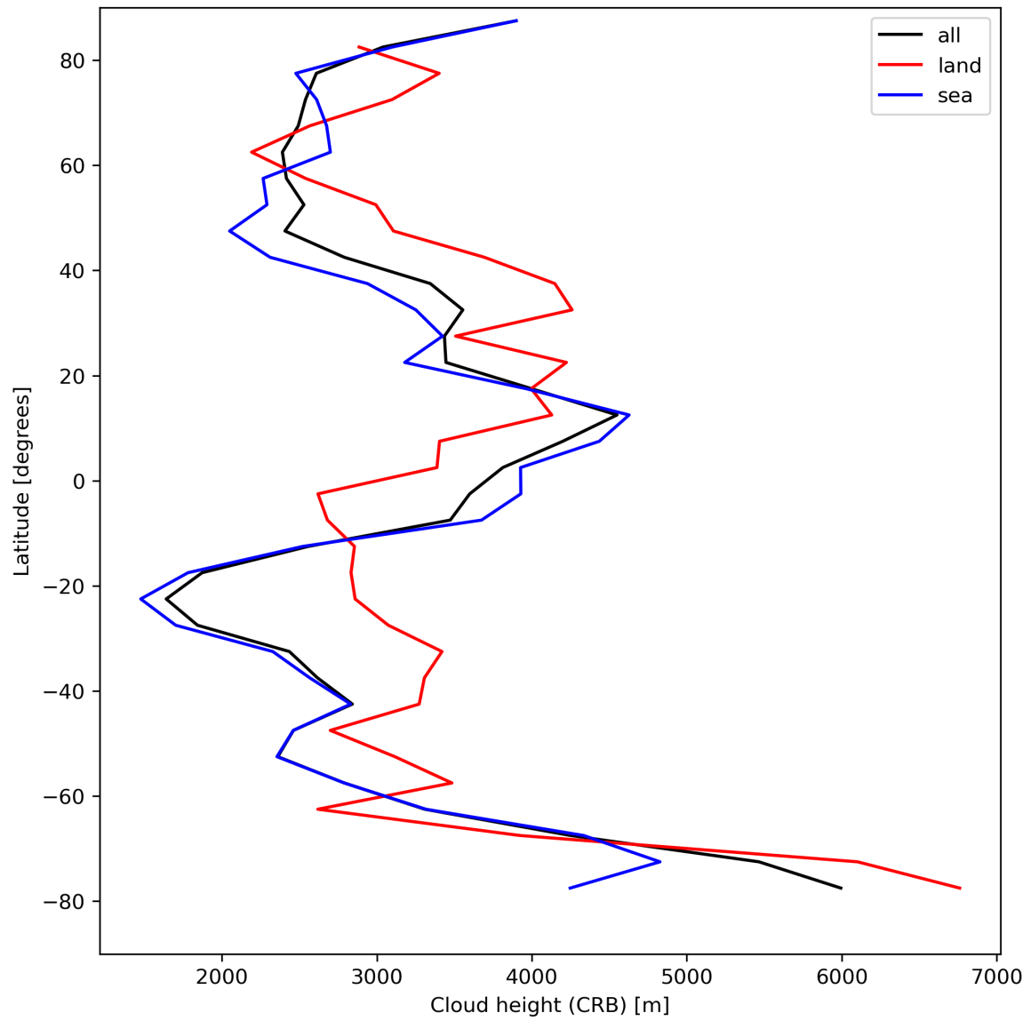
Figure 27: Zonal average of “Cloud height (CRB)” for 2024-08-22 to 2024-08-24.
