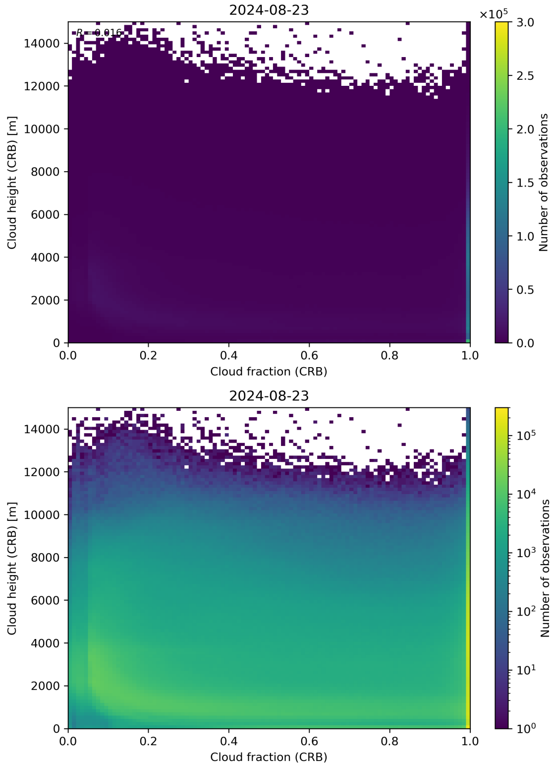
Figure 79: Scatter density plot of “Cloud fraction (CRB)” against “Cloud height (CRB)” for 2024-08-22 to 2024-08-24.
