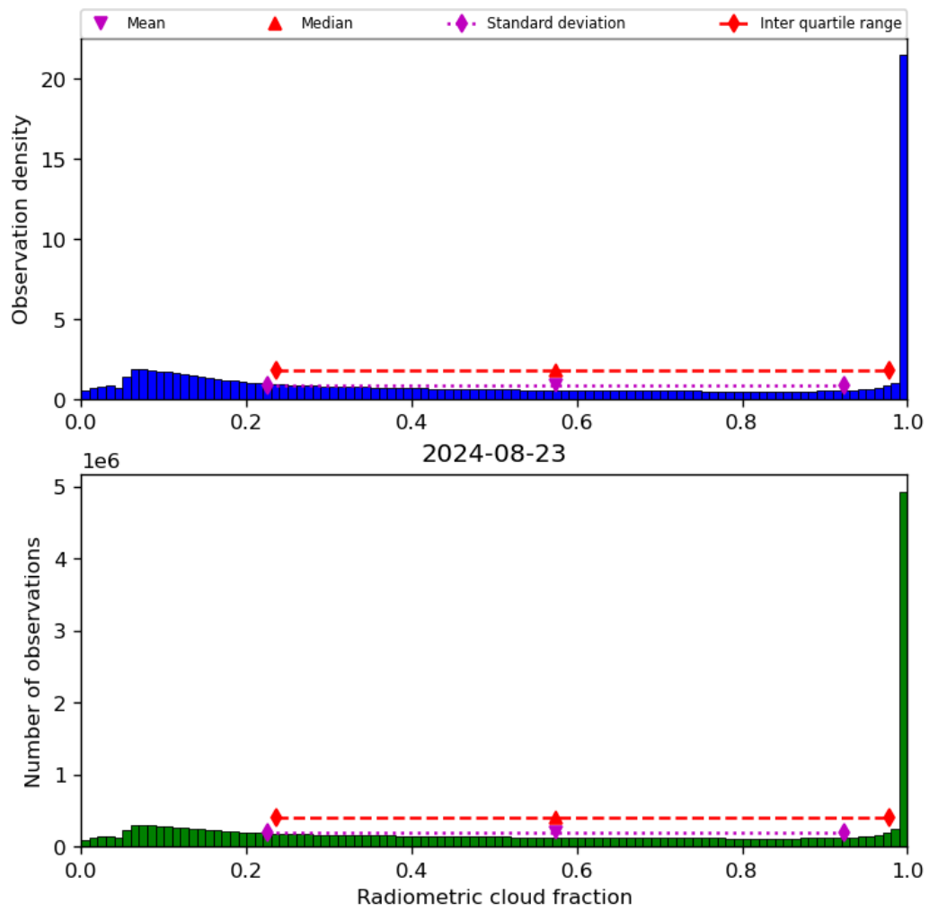
Figure 39: Histogram of “Radiometric cloud fraction” for 2024-08-22 to 2024-08-24
