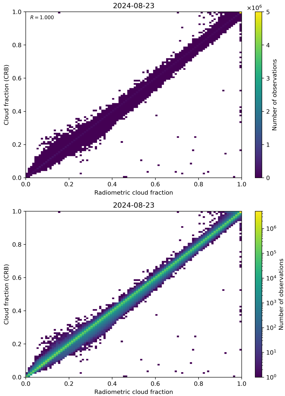
Figure 73: Scatter density plot of “Radiometric cloud fraction” against “Cloud fraction (CRB)” for 2024-08-22 to 2024-08-24.
