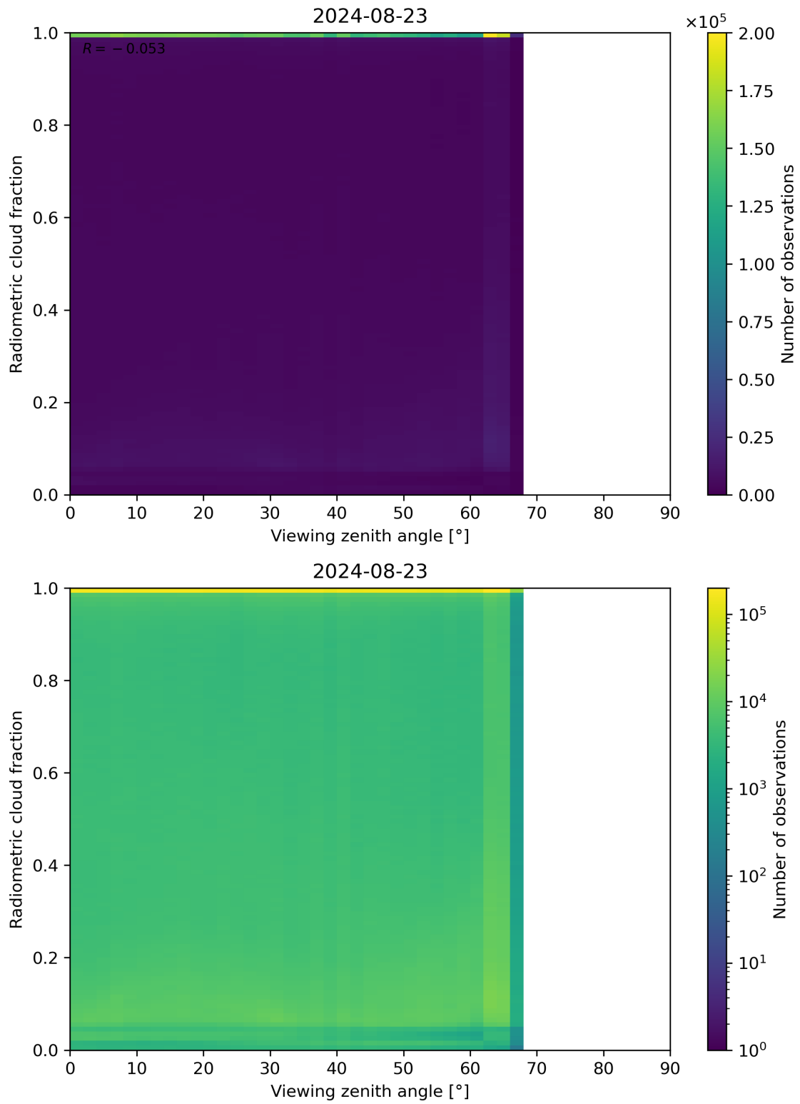
Figure 107: Scatter density plot of “Viewing zenith angle” against “Radiometric cloud fraction” for 2024-08-22 to 2024-08-24.
