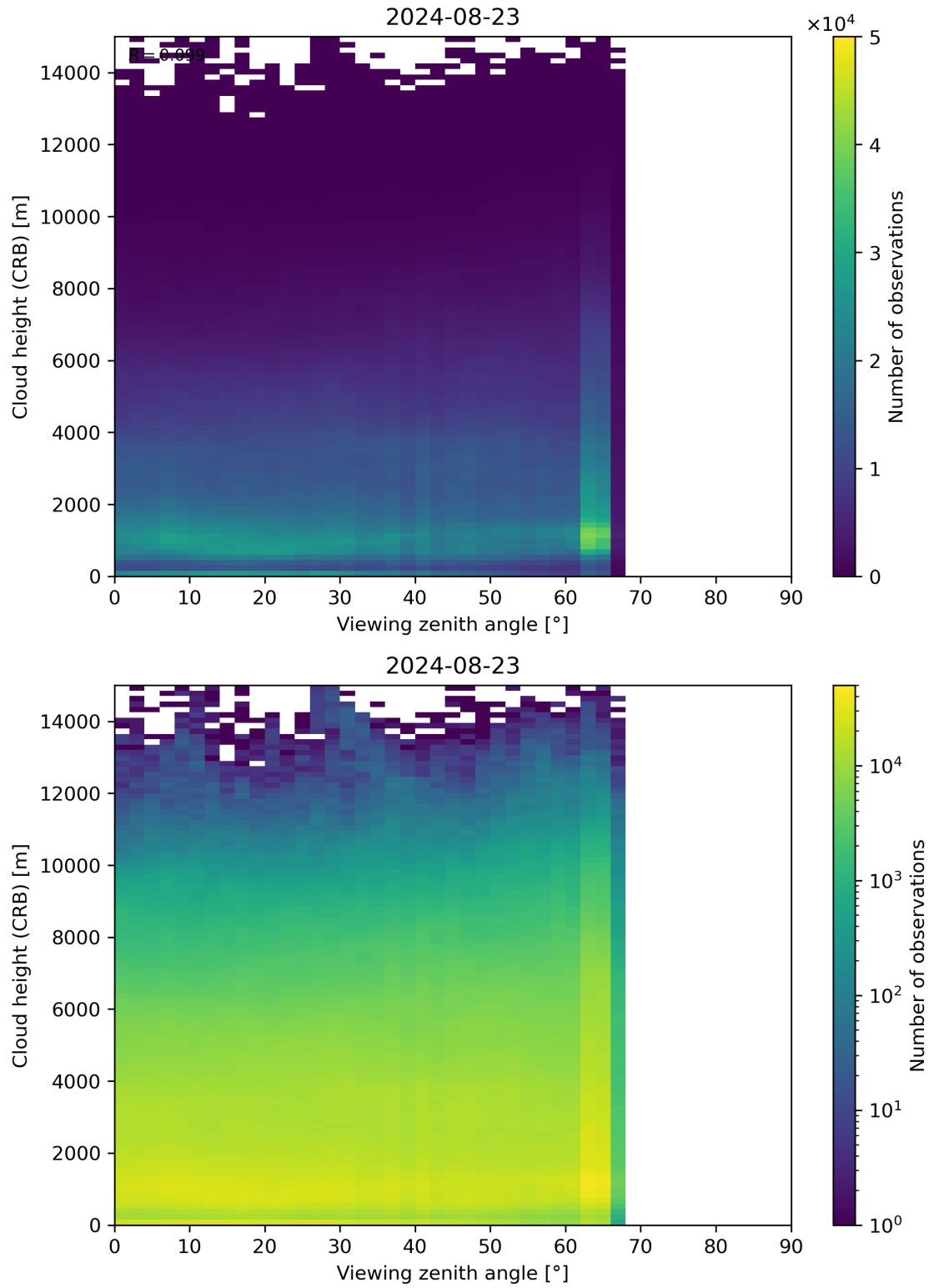
Figure 110: Scatter density plot of “Viewing zenith angle” against “Cloud height (CRB)” for 2024-08-22 to 2024-08-24.
