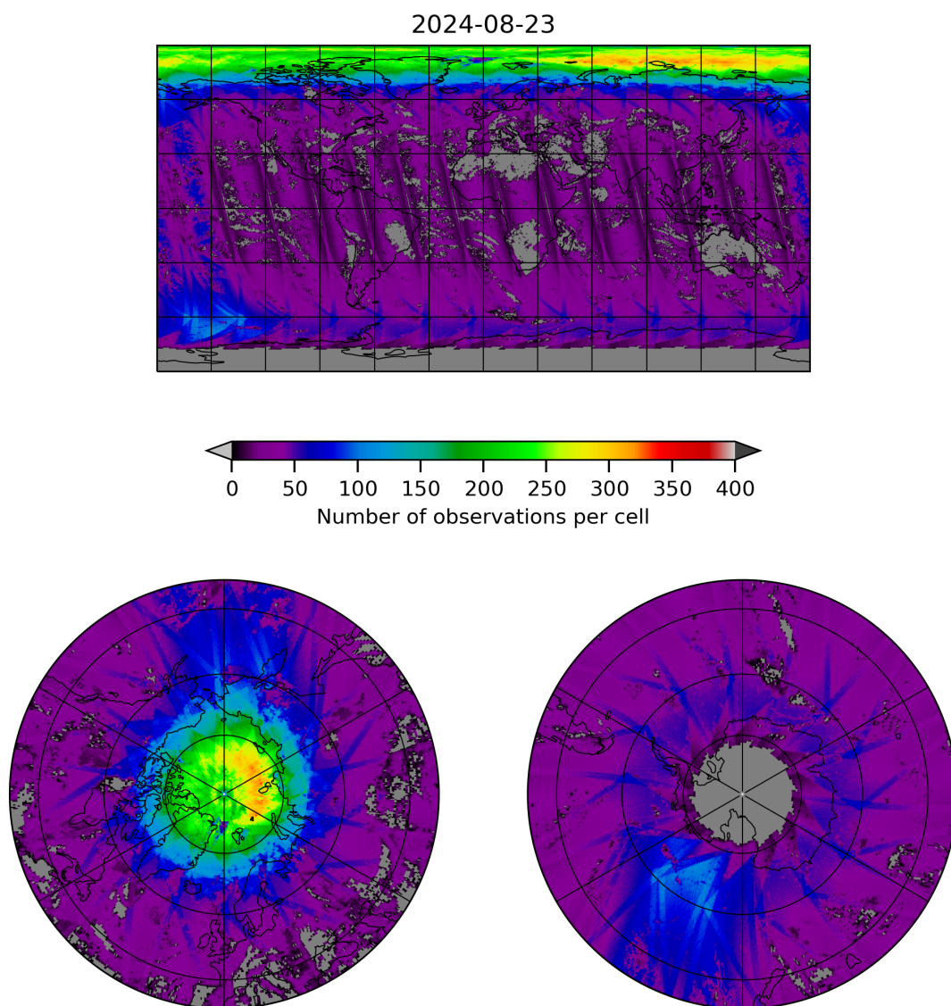
Figure 21: Map of the number of observations for 2024-08-22 to 2024-08-24
