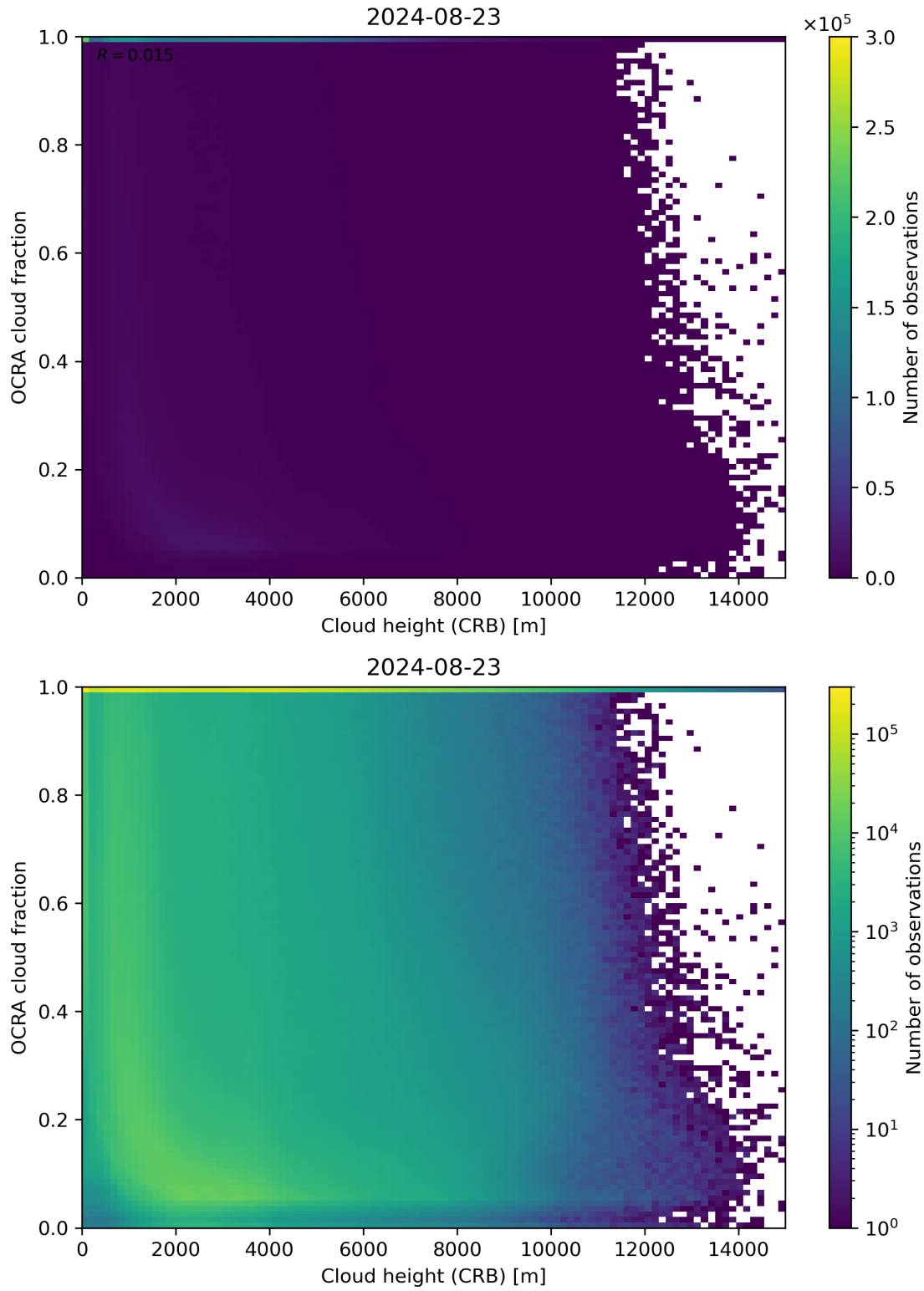
Figure 81: Scatter density plot of “Cloud height (CRB)” against “OCRA cloud fraction” for 2024-08-22 to 2024-08-24.
