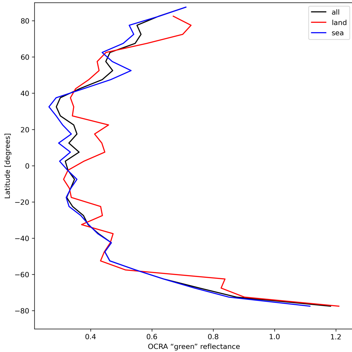
Figure 36: Zonal average of “OCRA “green” reflectance” for 2024-08-22 to 2024-08-24.
