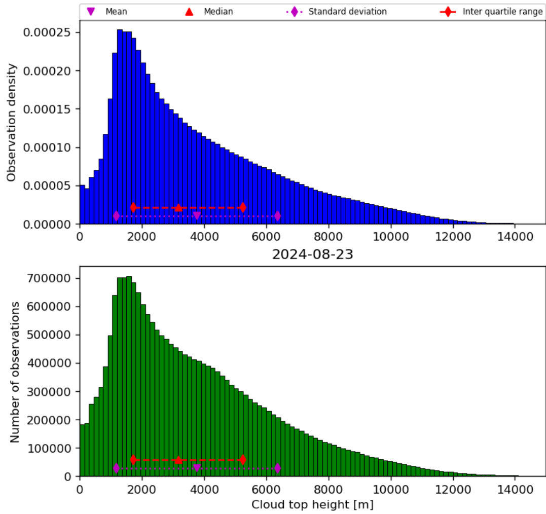
Figure 40: Histogram of “Cloud top height” for 2024-08-22 to 2024-08-24
