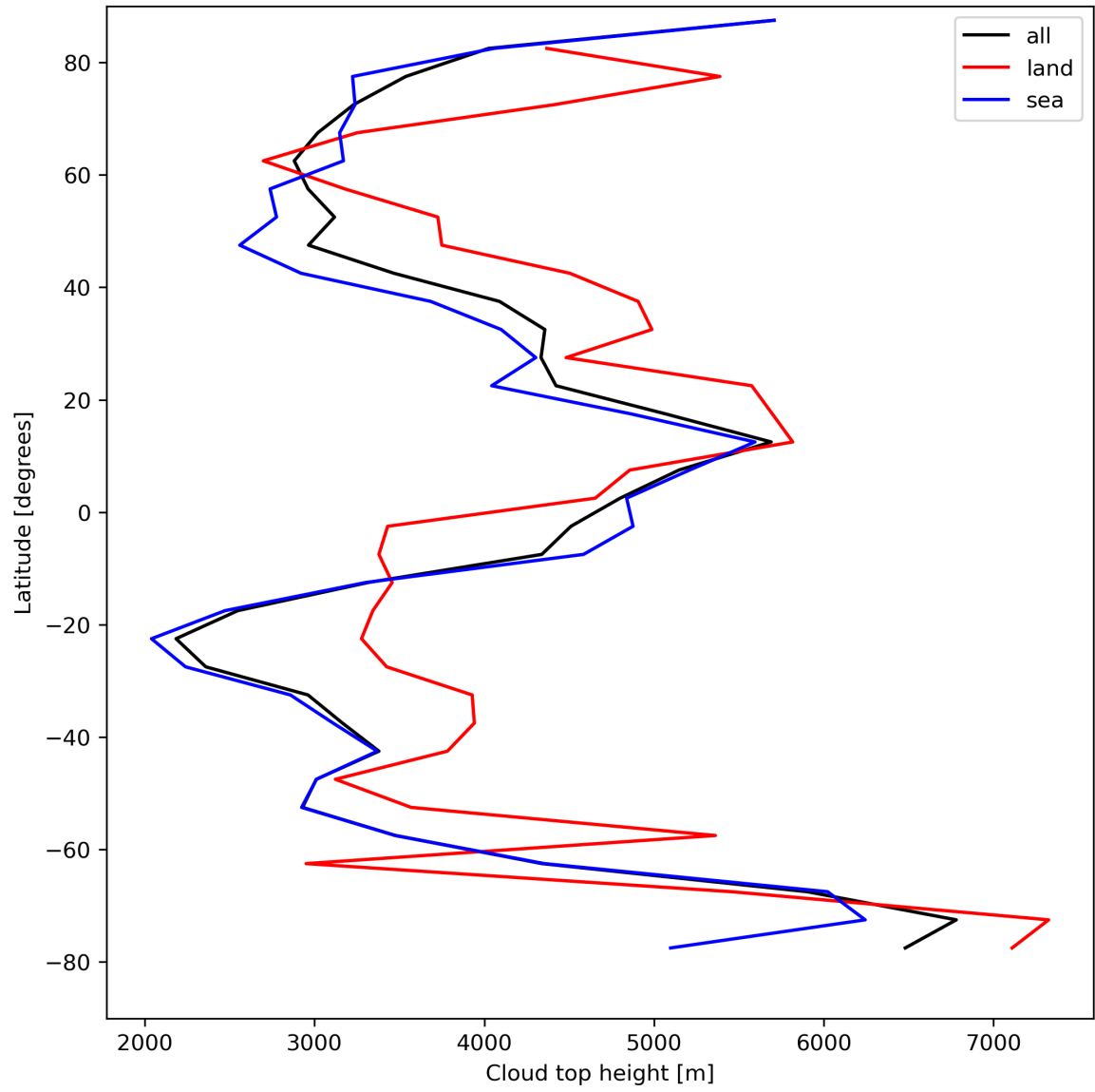
Figure 24: Zonal average of “Cloud top height” for 2024-08-22 to 2024-08-24.
