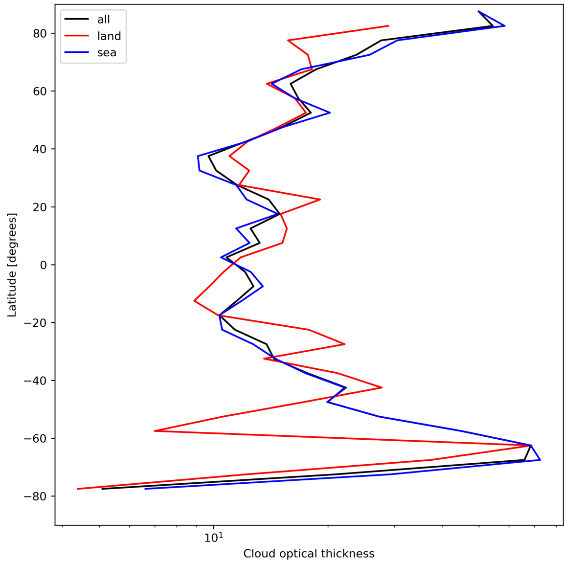
Figure 25: Zonal average of “Cloud optical thickness” for 2024-08-22 to 2024-08-24.
