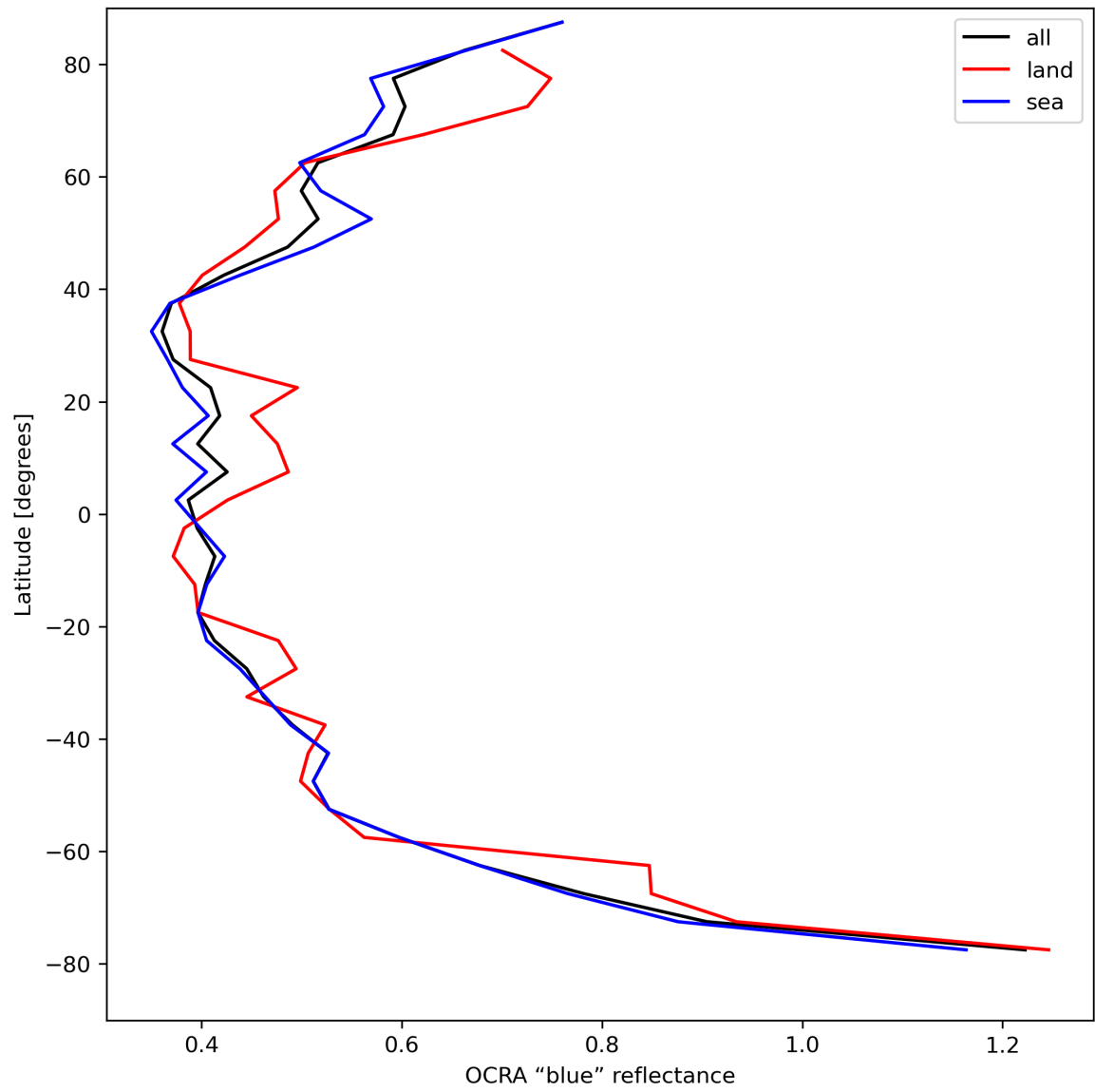
Figure 35: Zonal average of “OCRA “blue” reflectance” for 2024-08-22 to 2024-08-24.
