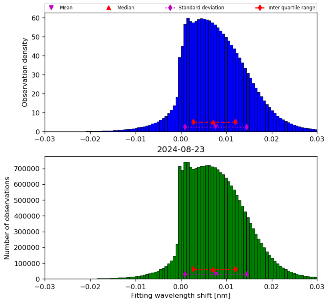
Figure 49: Histogram of “Fitting wavelength shift” for 2024-08-22 to 2024-08-24
