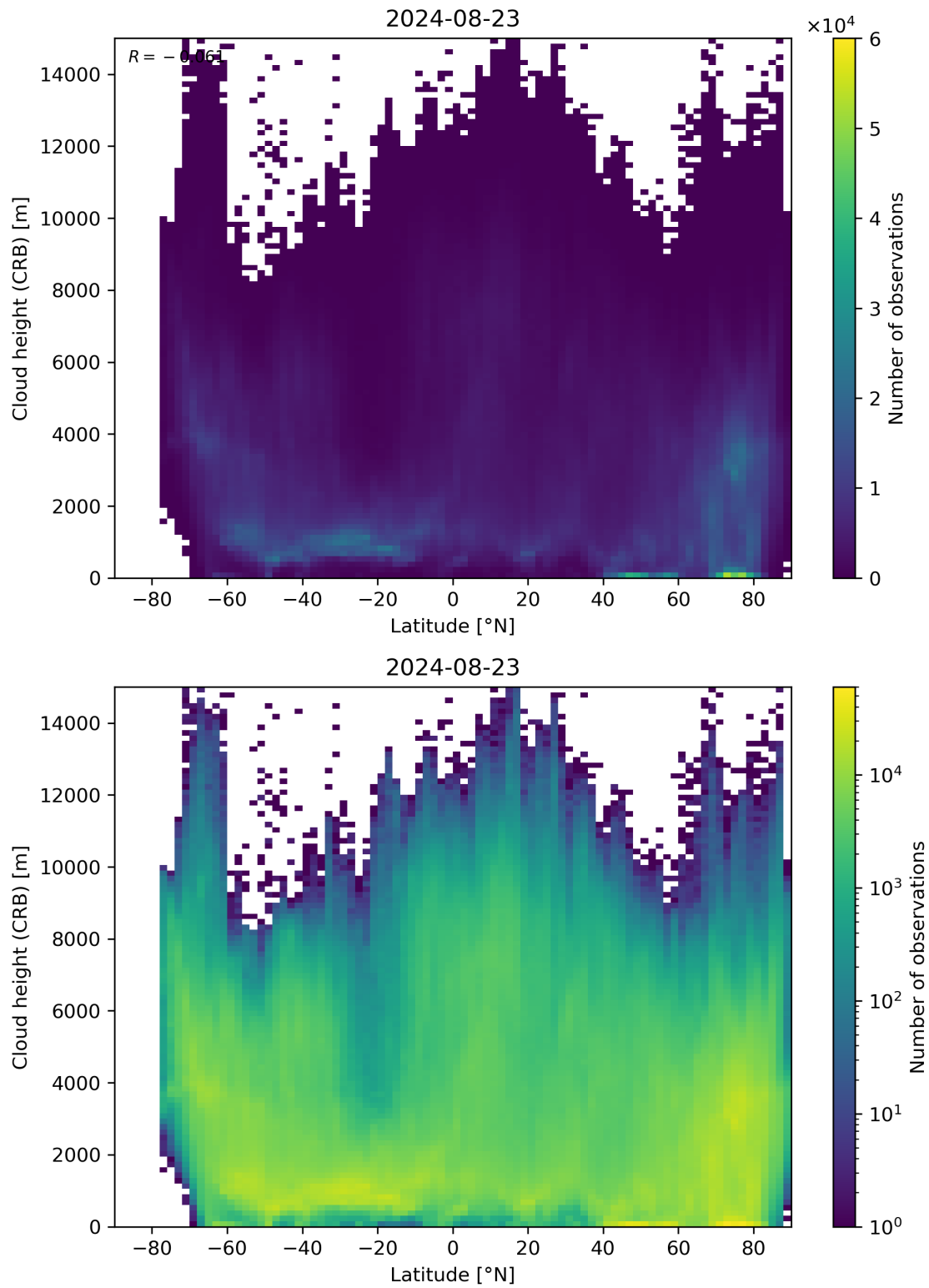
Figure 95: Scatter density plot of “Latitude” against “Cloud height (CRB)” for 2024-08-22 to 2024-08-24.
