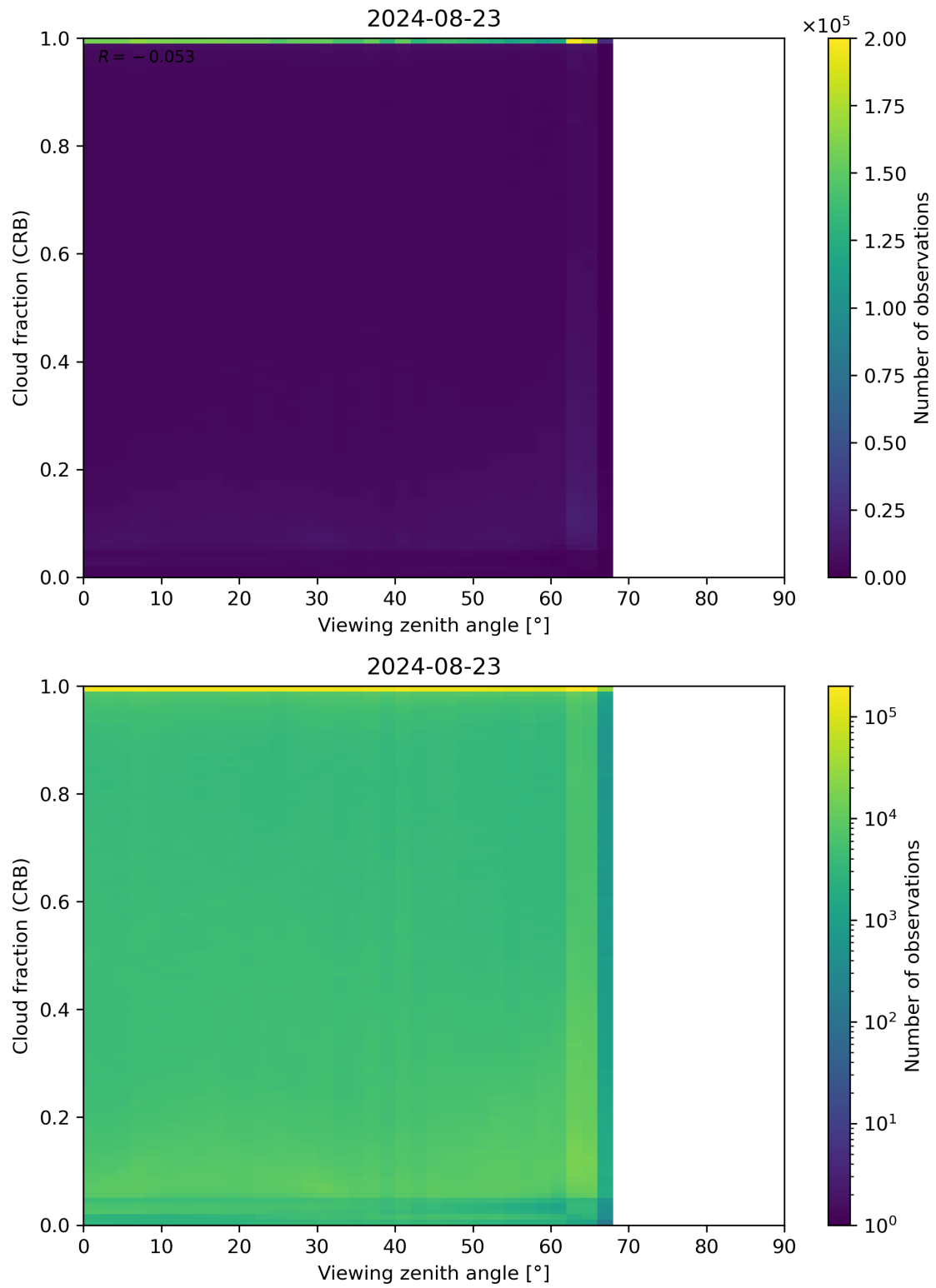
Figure 109: Scatter density plot of “Viewing zenith angle” against “Cloud fraction (CRB)” for 2024-08-22 to 2024-08-24.
