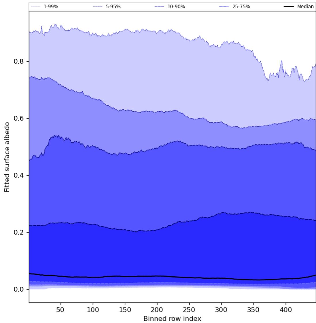
Figure 61: Along track statistics of “Fitted surface albedo” for 2024-08-22 to 2024-08-24
