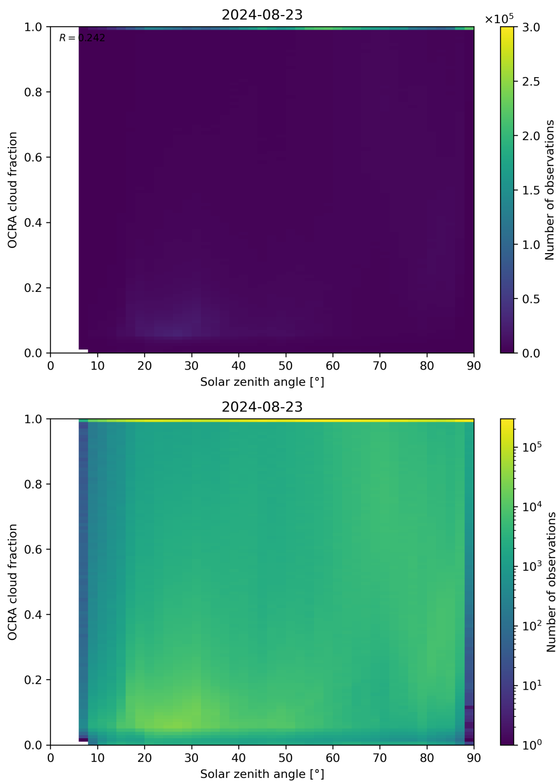
Figure 100: Scatter density plot of “Solar zenith angle” against “OCRA cloud fraction” for 2024-08-22 to 2024-08-24.
