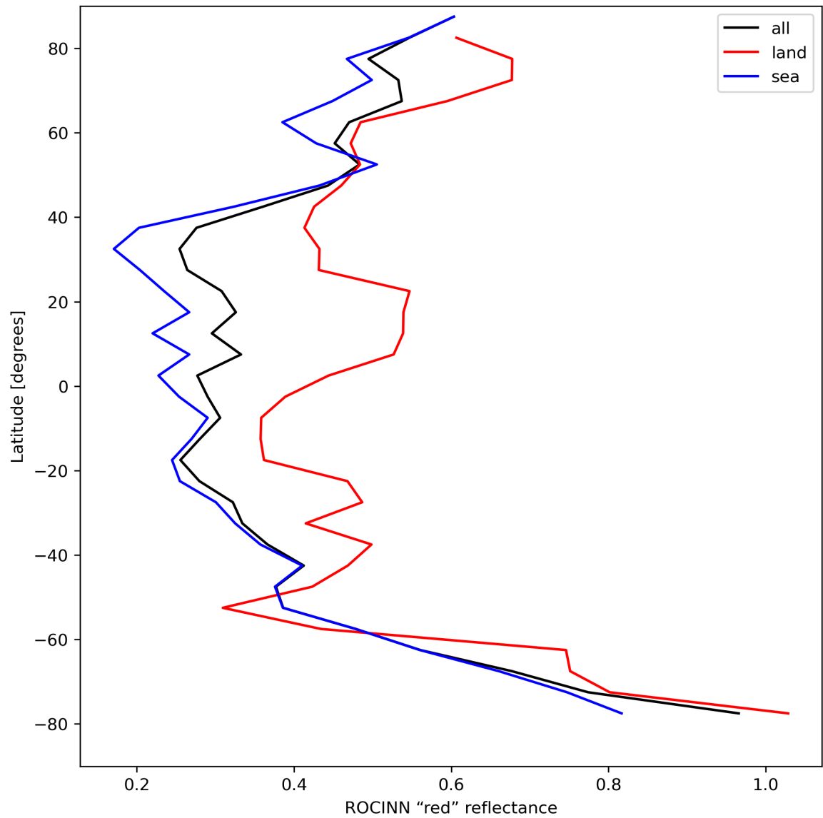
Figure 37: Zonal average of “ROCINN “red” reflectance” for 2024-08-22 to 2024-08-24.
