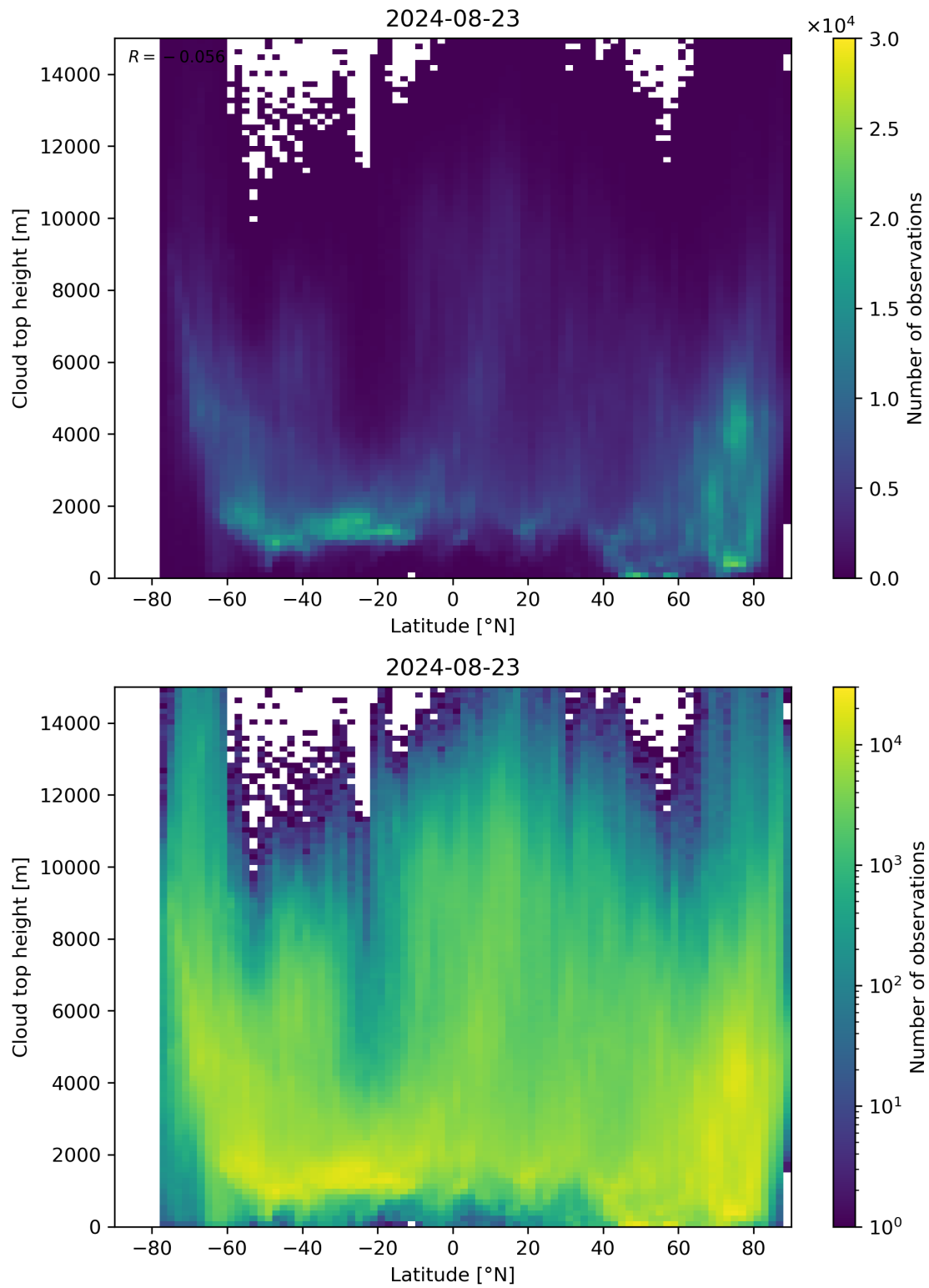
Figure 97: Scatter density plot of “Latitude” against “Cloud top height” for 2024-08-22 to 2024-08-24.
