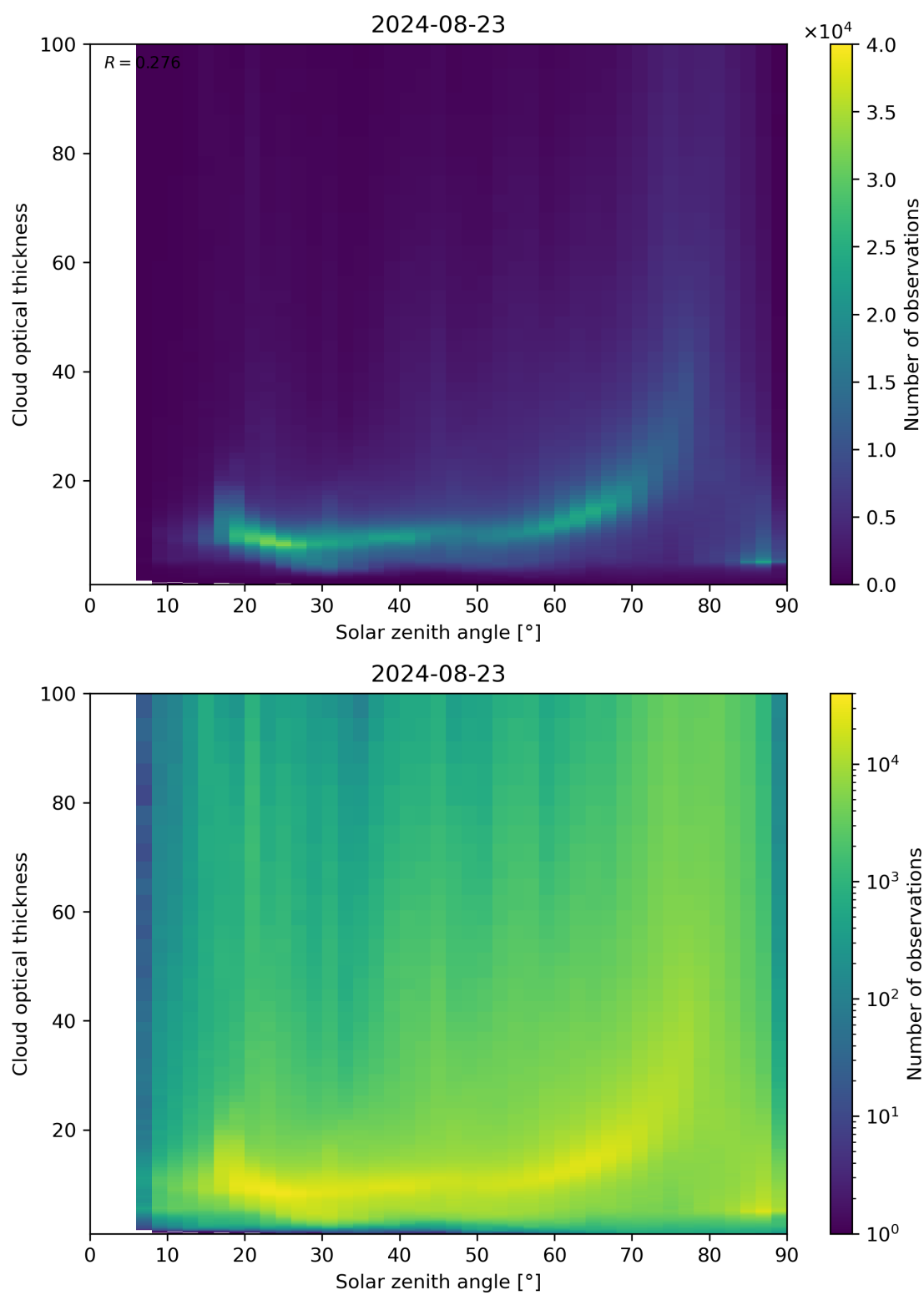
Figure 103: Scatter density plot of “Solar zenith angle” against “Cloud optical thickness” for 2024-08-22 to 2024-08-24.
