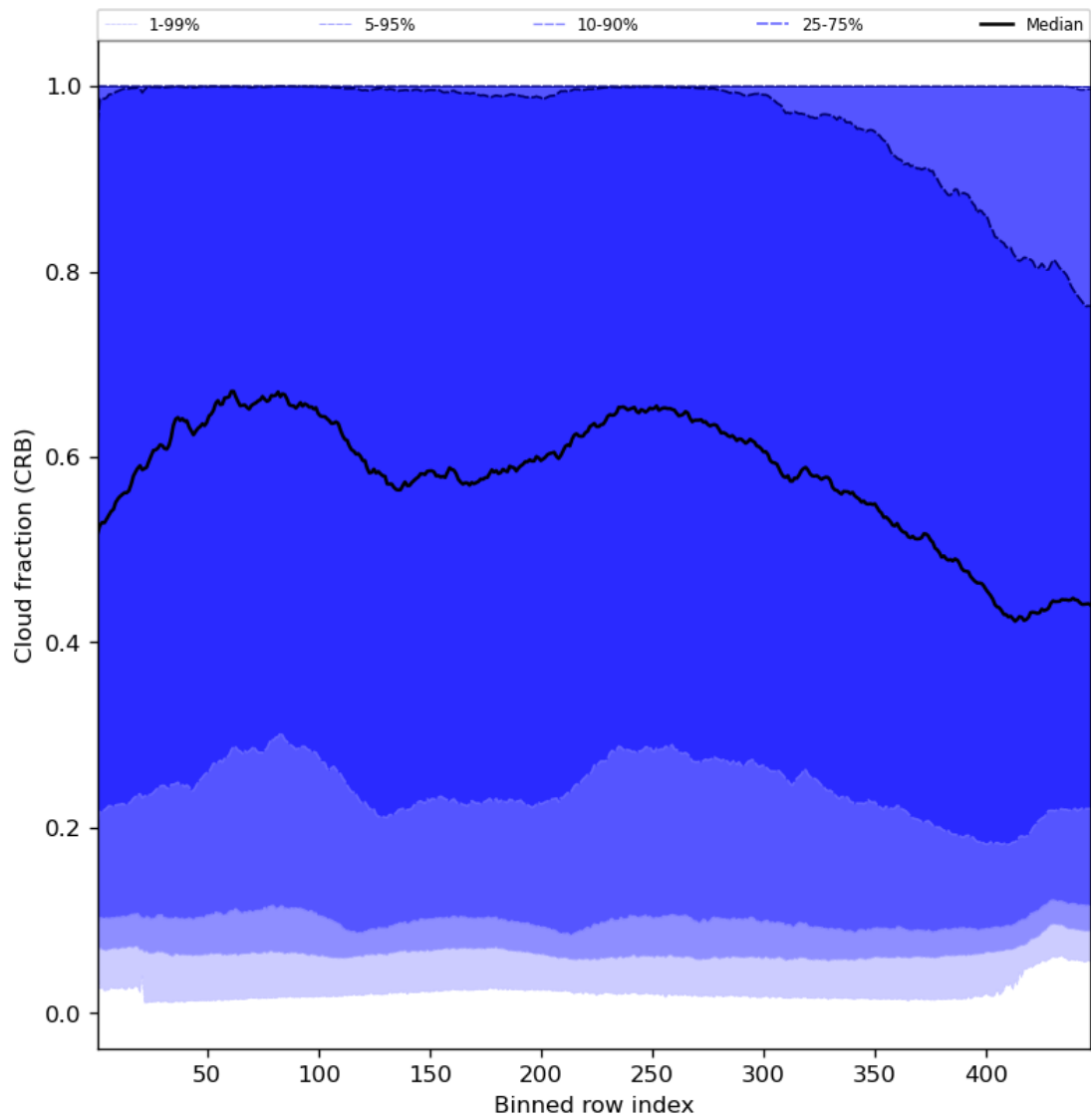
Figure 58: Along track statistics of “Cloud fraction (CRB)” for 2024-08-22 to 2024-08-24
