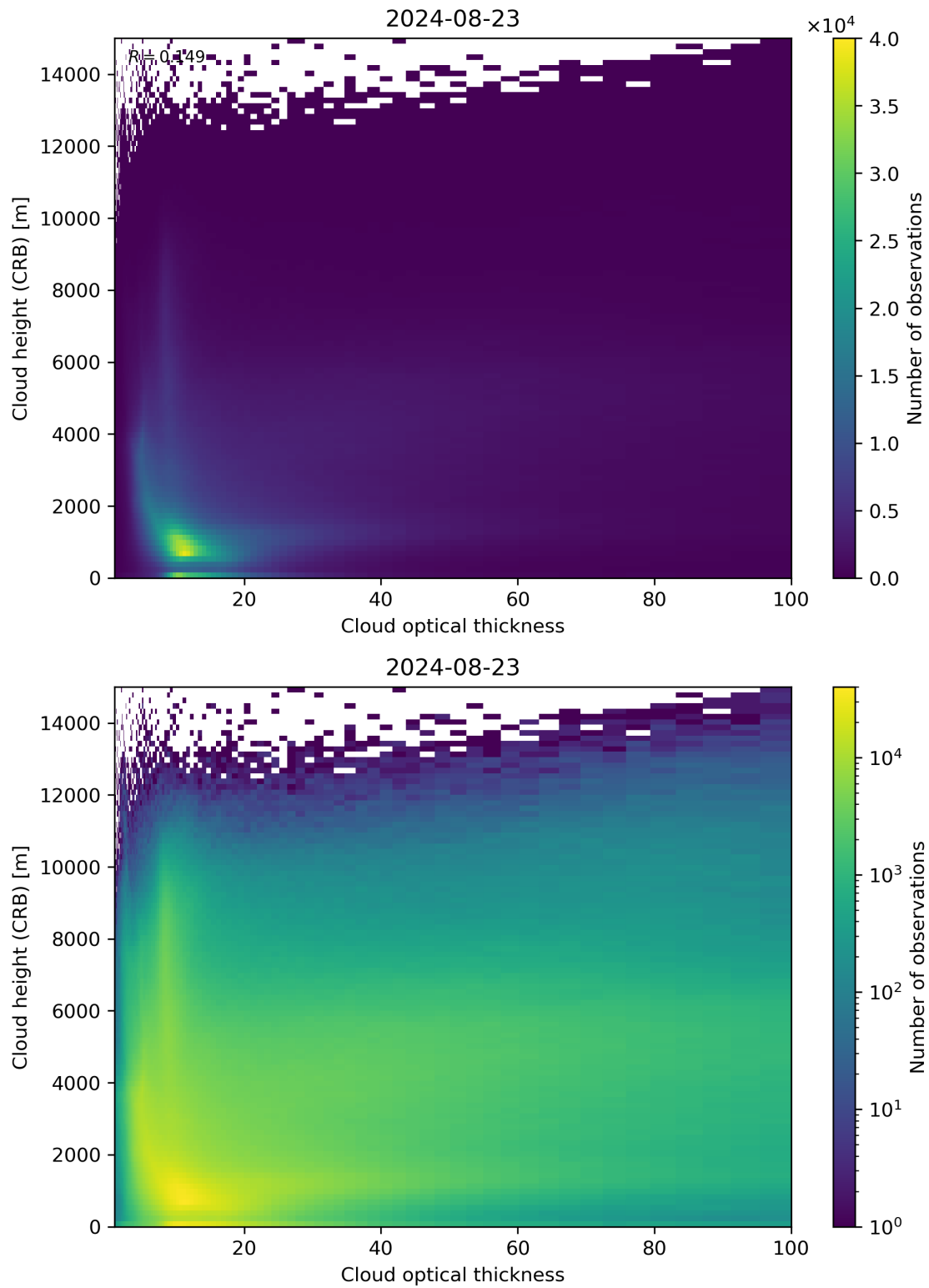
Figure 85: Scatter density plot of “Cloud optical thickness” against “Cloud height (CRB)” for 2024-08-22 to 2024-08-24.
