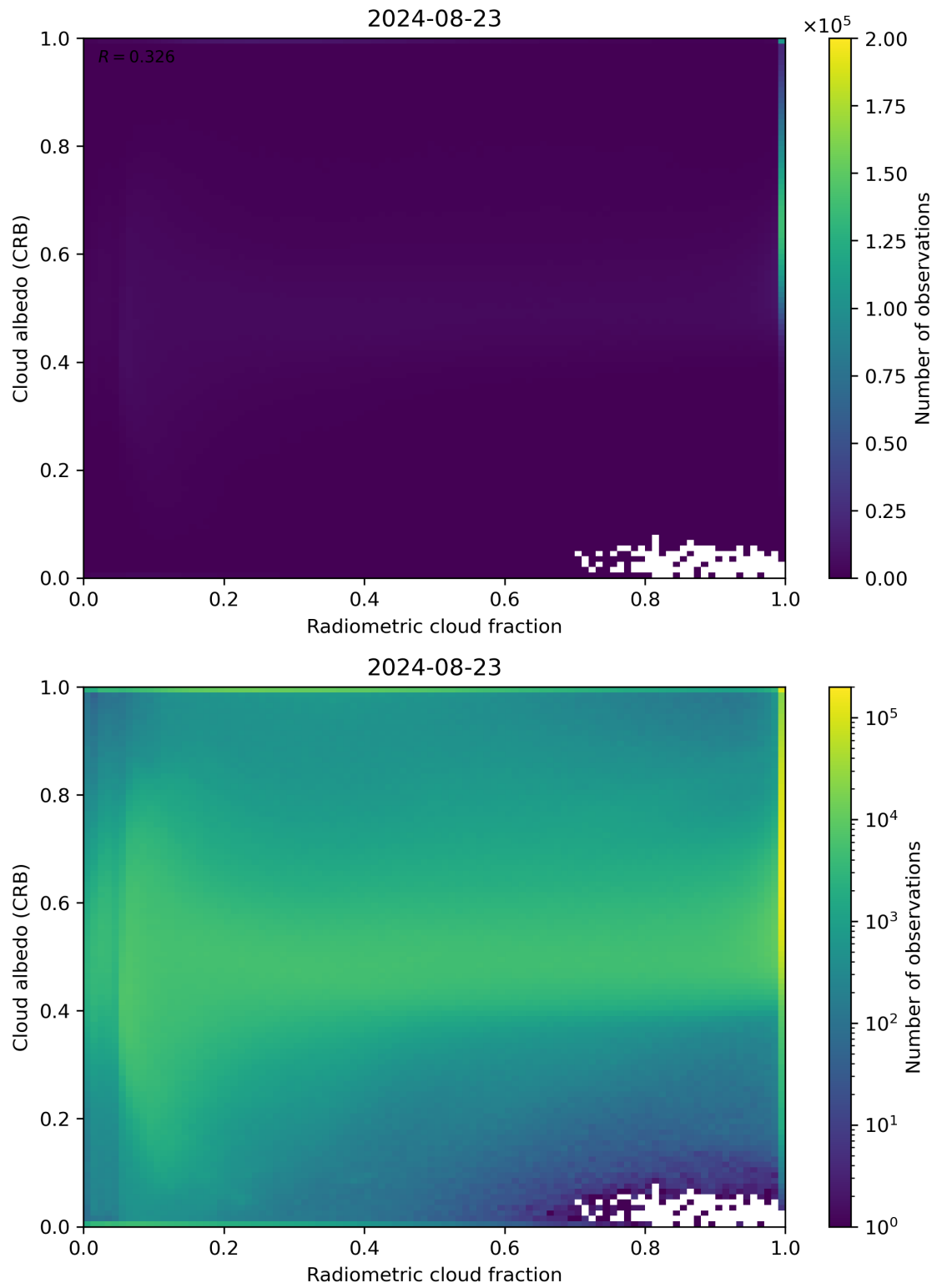
Figure 71: Scatter density plot of “Radiometric cloud fraction” against “Cloud albedo (CRB)” for 2024-08-22 to 2024-08-24.
