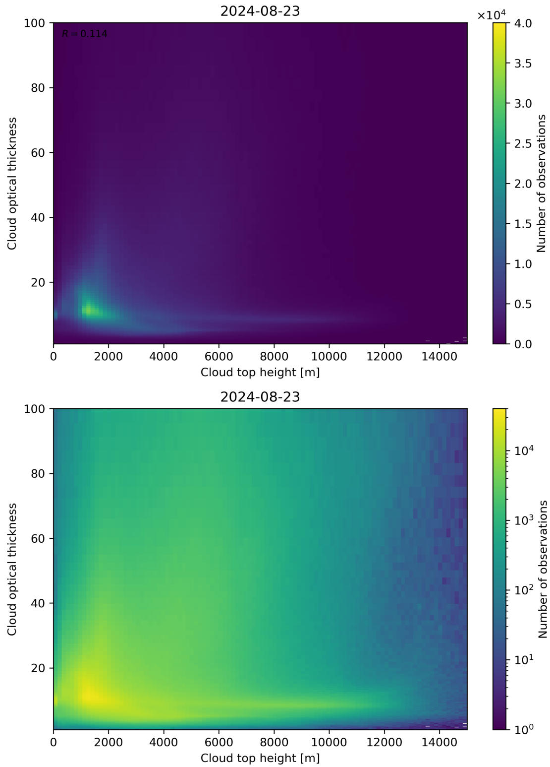
Figure 90: Scatter density plot of “Cloud top height” against “Cloud optical thickness” for 2024-08-22 to 2024-08-24.
