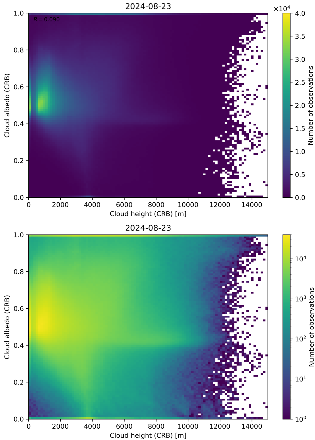
Figure 80: Scatter density plot of “Cloud height (CRB)” against “Cloud albedo (CRB)” for 2024-08-22 to 2024-08-24.
