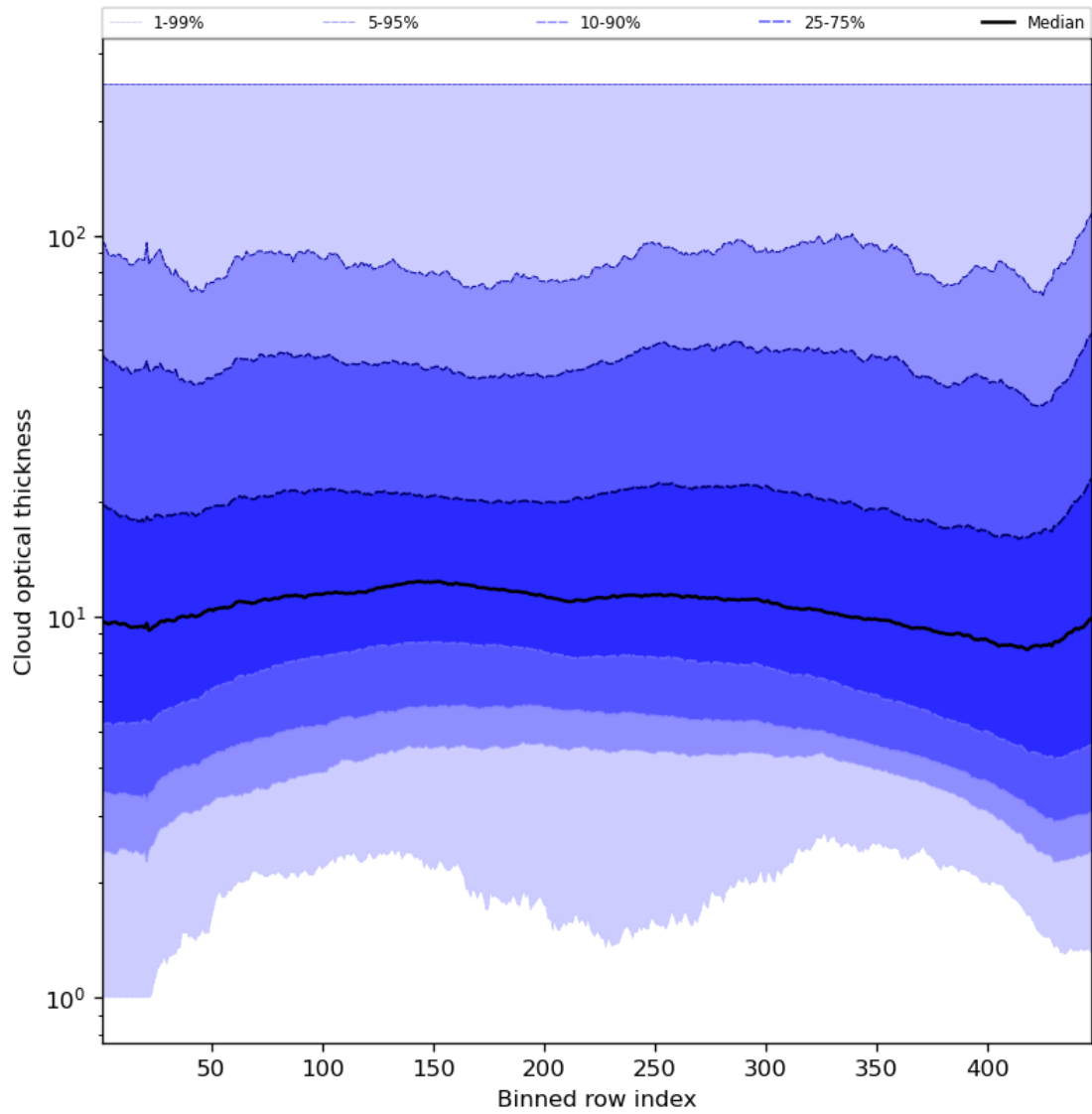
Figure 57: Along track statistics of “Cloud optical thickness” for 2024-08-22 to 2024-08-24
