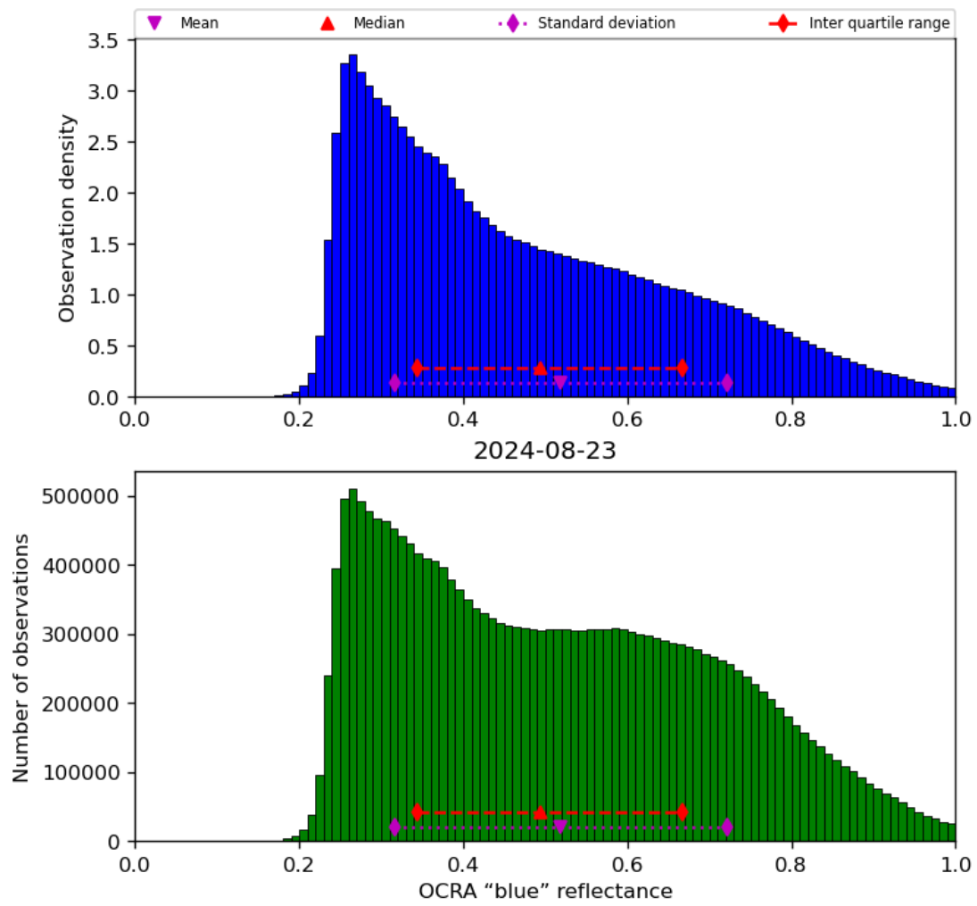
Figure 51: Histogram of “OCRA “blue” reflectance” for 2024-08-22 to 2024-08-24
