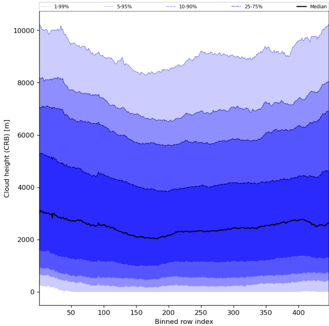
Figure 59: Along track statistics of “Cloud height (CRB)” for 2024-08-22 to 2024-08-24
