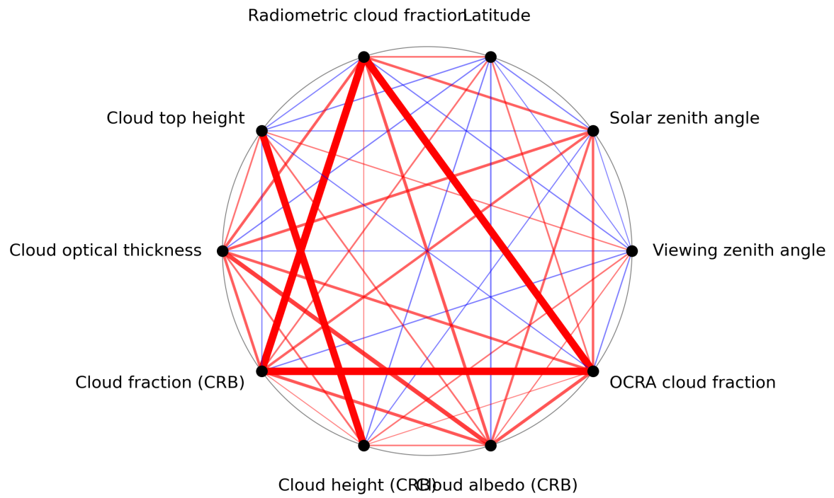
Figure 1: Map of correlation graph for 2024-08-22 to 2024-08-24.
