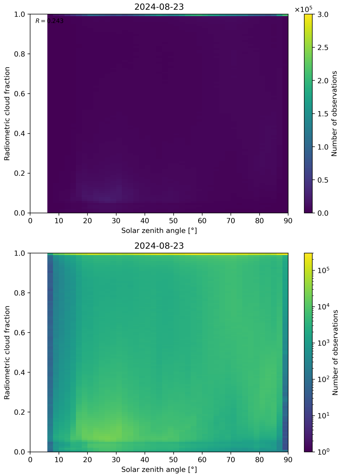
Figure 99: Scatter density plot of “Solar zenith angle” against “Radiometric cloud fraction” for 2024-08-22 to 2024-08-24.
