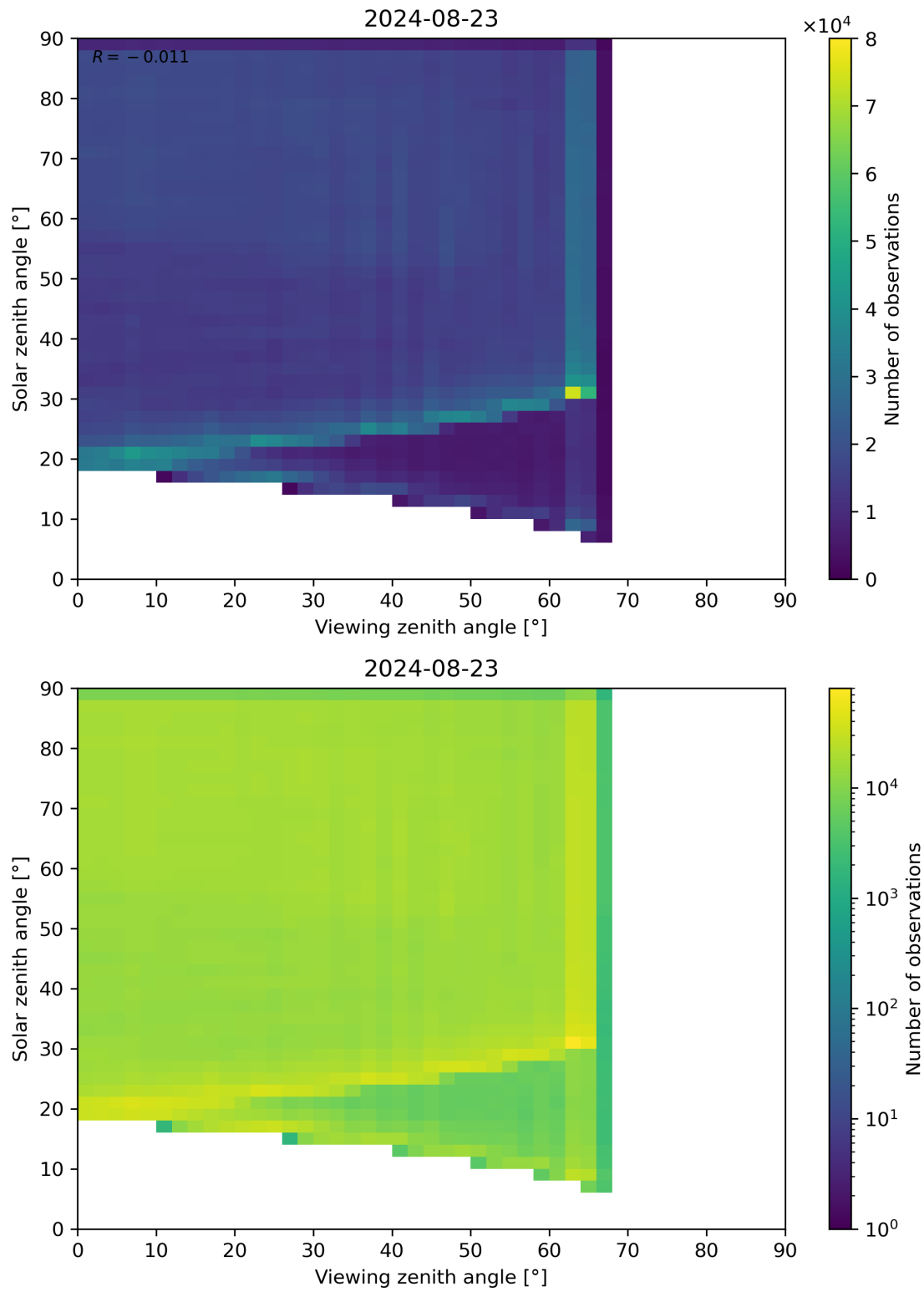
Figure 114: Scatter density plot of “Viewing zenith angle” against “Solar zenith angle” for 2024-08-22 to 2024-08-24.
