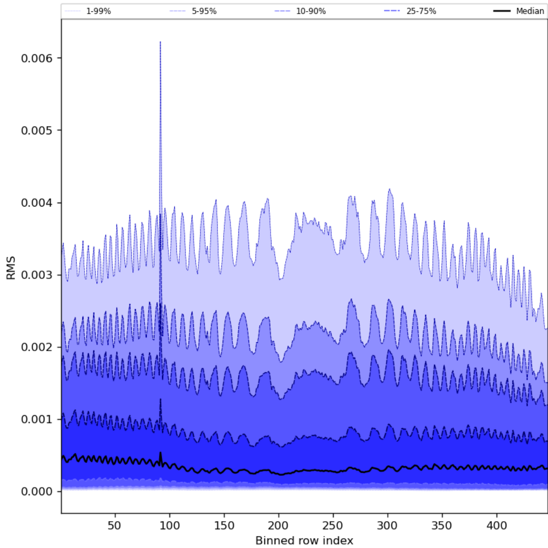
Figure 63: Along track statistics of “RMS” for 2024-08-22 to 2024-08-24
