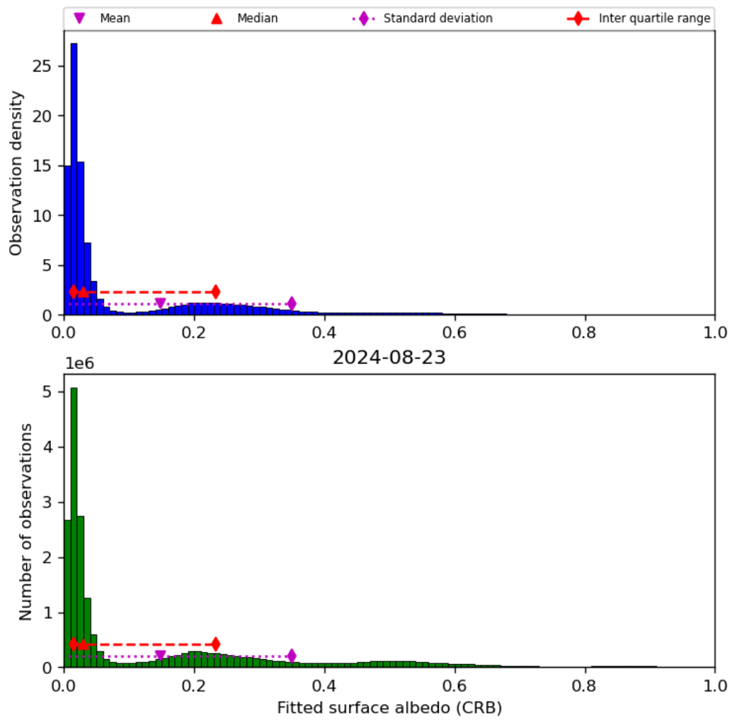
Figure 46: Histogram of “Fitted surface albedo (CRB)” for 2024-08-22 to 2024-08-24
