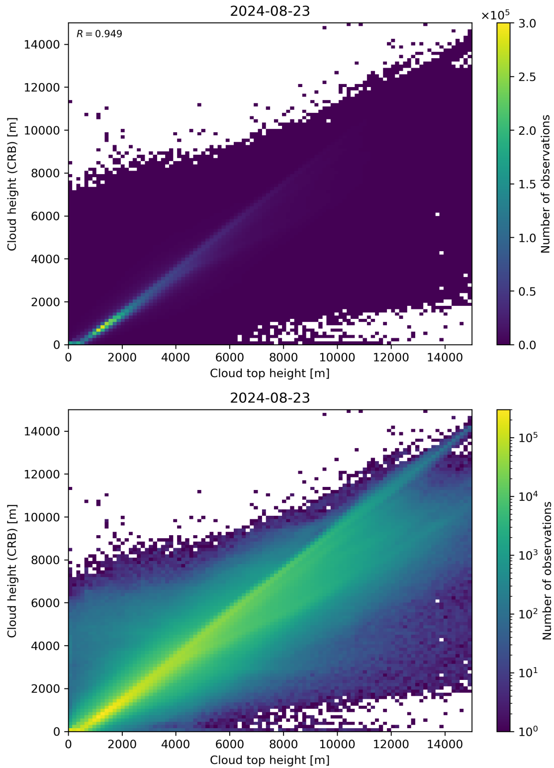
Figure 89: Scatter density plot of “Cloud top height” against “Cloud height (CRB)” for 2024-08-22 to 2024-08-24.
