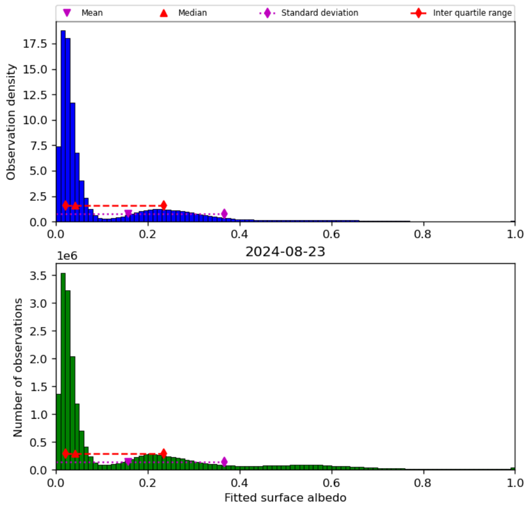
Figure 45: Histogram of “Fitted surface albedo” for 2024-08-22 to 2024-08-24
