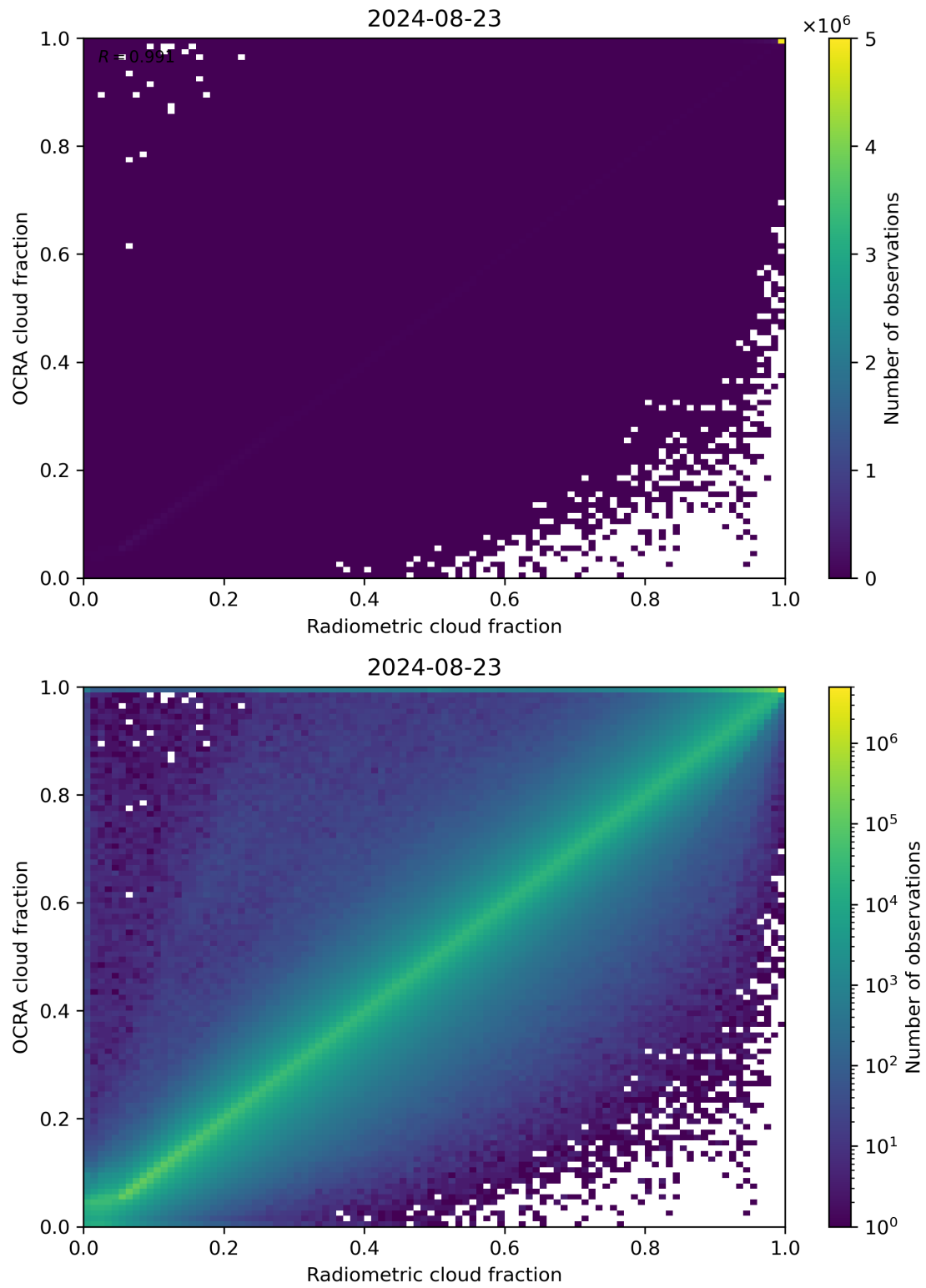
Figure 72: Scatter density plot of “Radiometric cloud fraction” against “OCRA cloud fraction” for 2024-08-22 to 2024-08-24.
