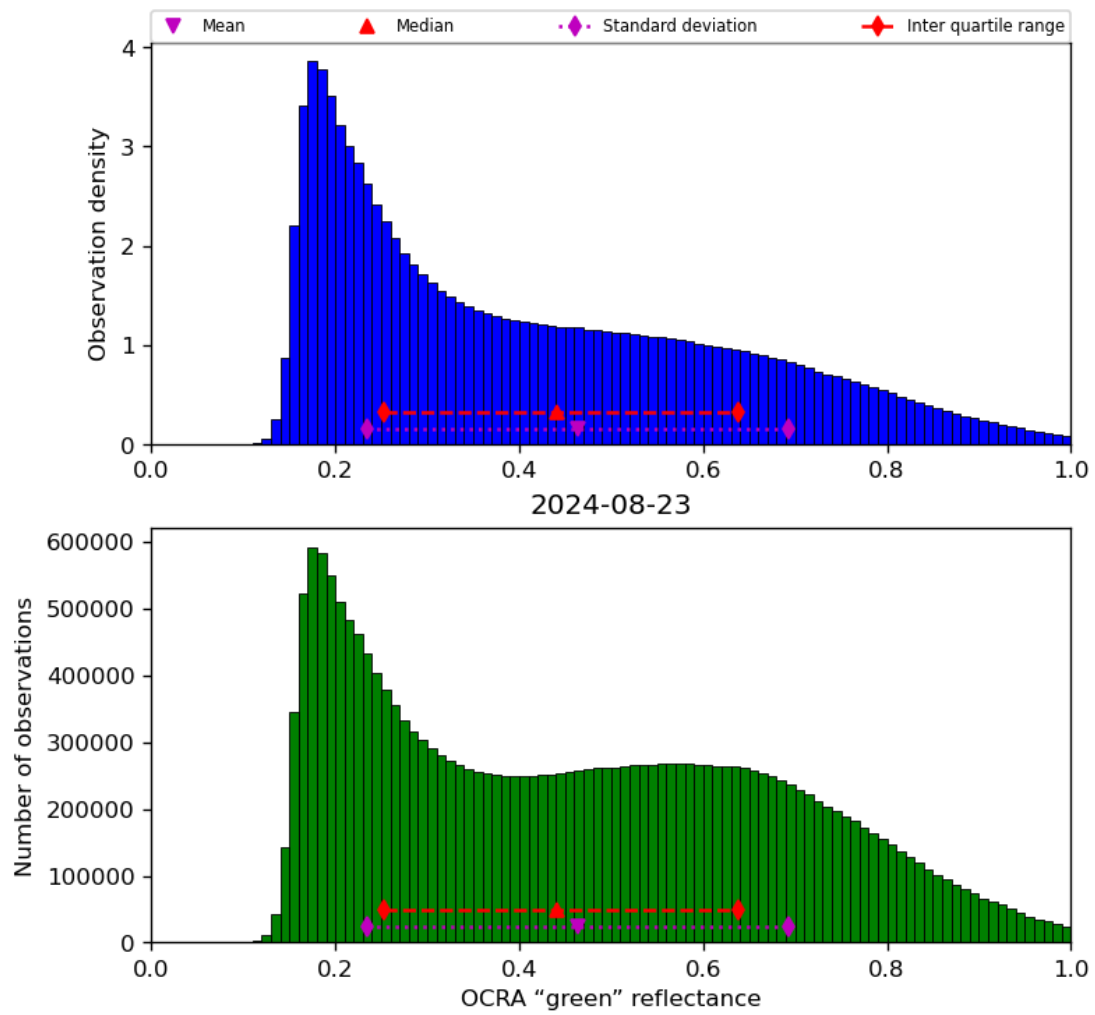
Figure 52: Histogram of “OCRA “green” reflectance” for 2024-08-22 to 2024-08-24
