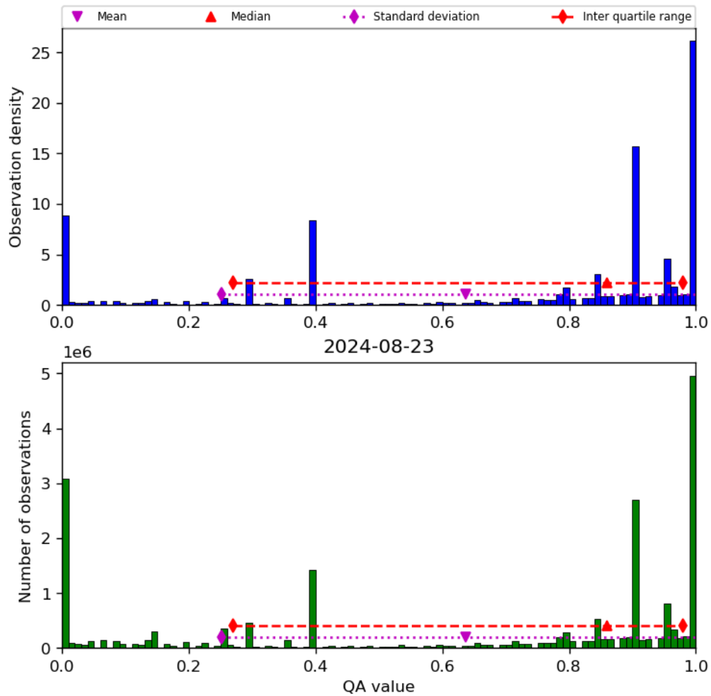
Figure 38: Histogram of “QA value” for 2024-08-22 to 2024-08-24
