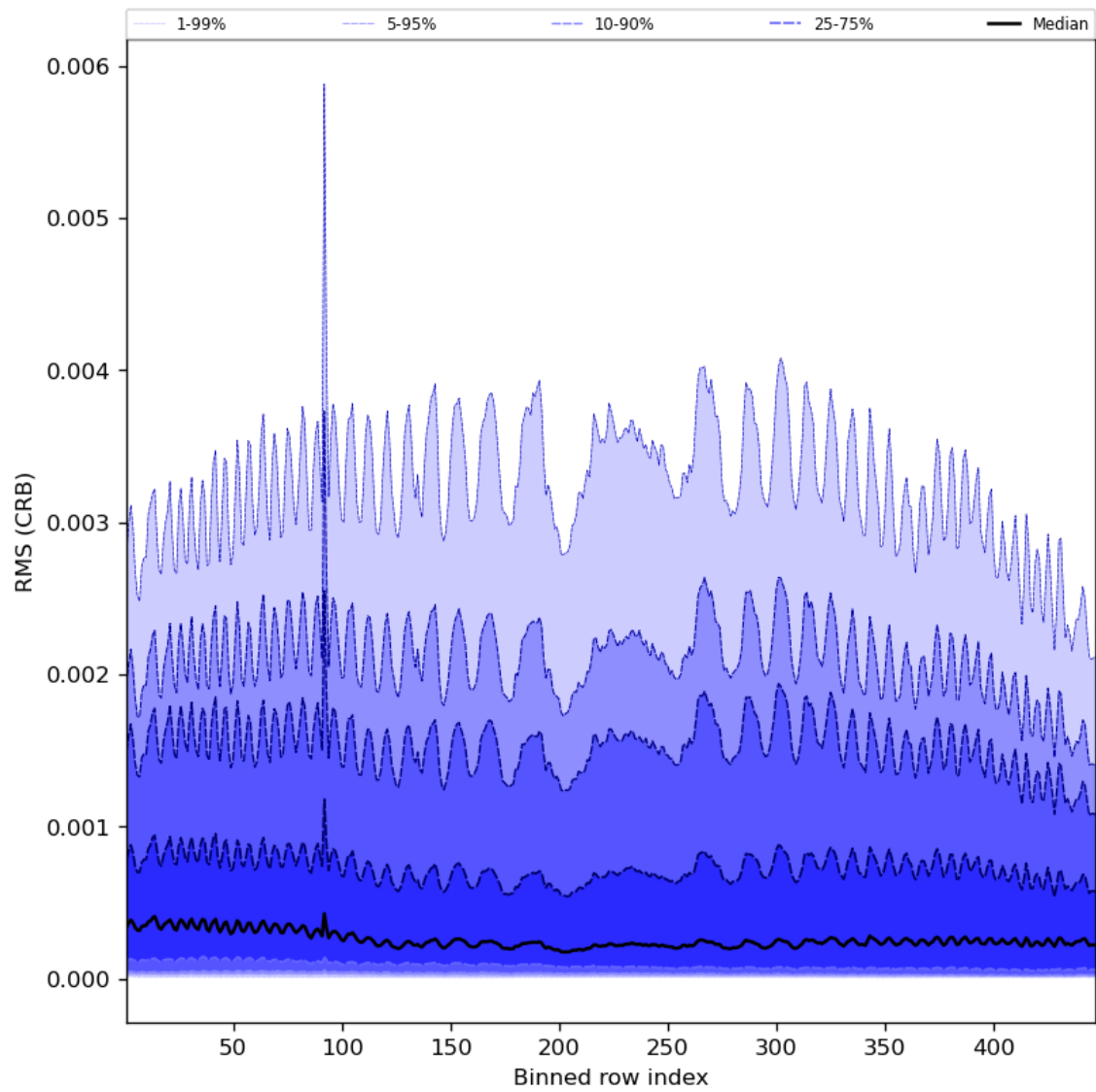
Figure 64: Along track statistics of “RMS (CRB)” for 2024-08-22 to 2024-08-24
