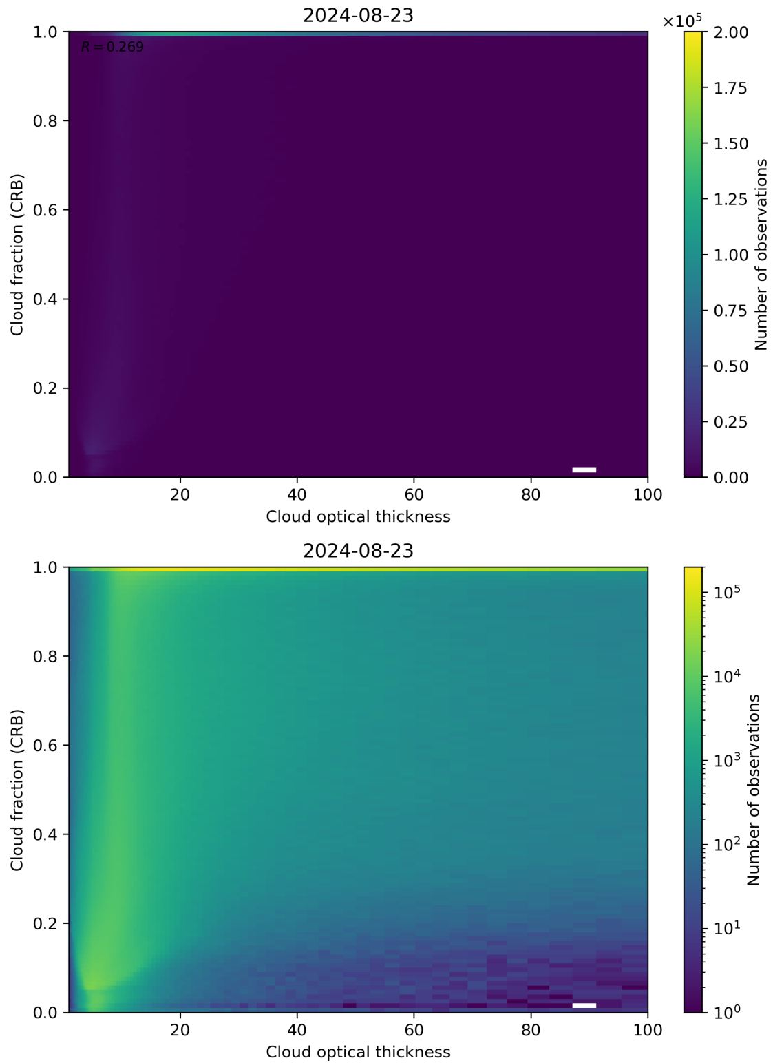
Figure 84: Scatter density plot of “Cloud optical thickness” against “Cloud fraction (CRB)” for 2024-08-22 to 2024-08-24.
