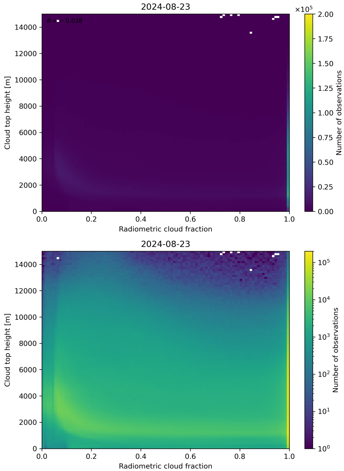
Figure 76: Scatter density plot of “Radiometric cloud fraction” against “Cloud top height” for 2024-08-22 to 2024-08-24.
