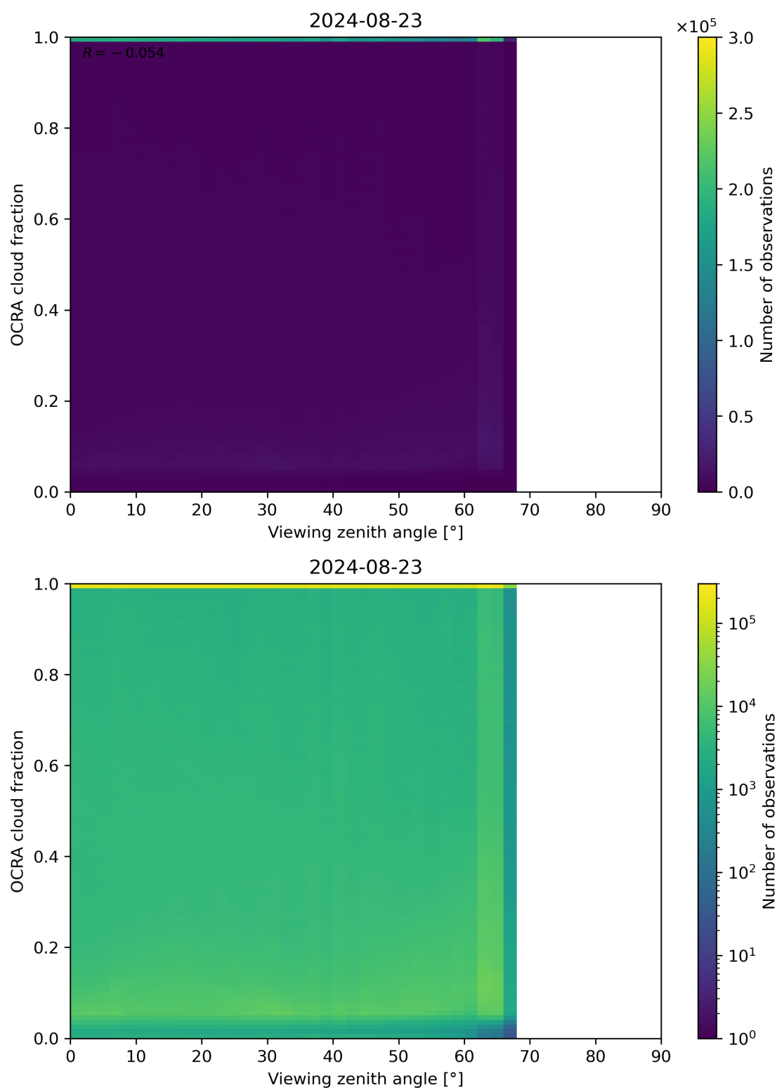
Figure 108: Scatter density plot of “Viewing zenith angle” against “OCRA cloud fraction” for 2024-08-22 to 2024-08-24.
