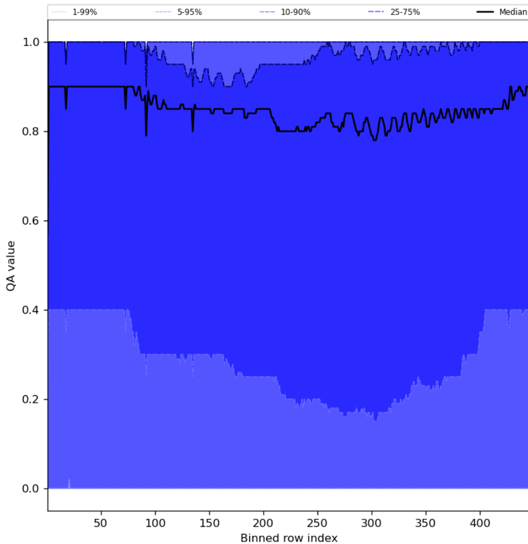
Figure 54: Along track statistics of “QA value” for 2024-08-22 to 2024-08-24
