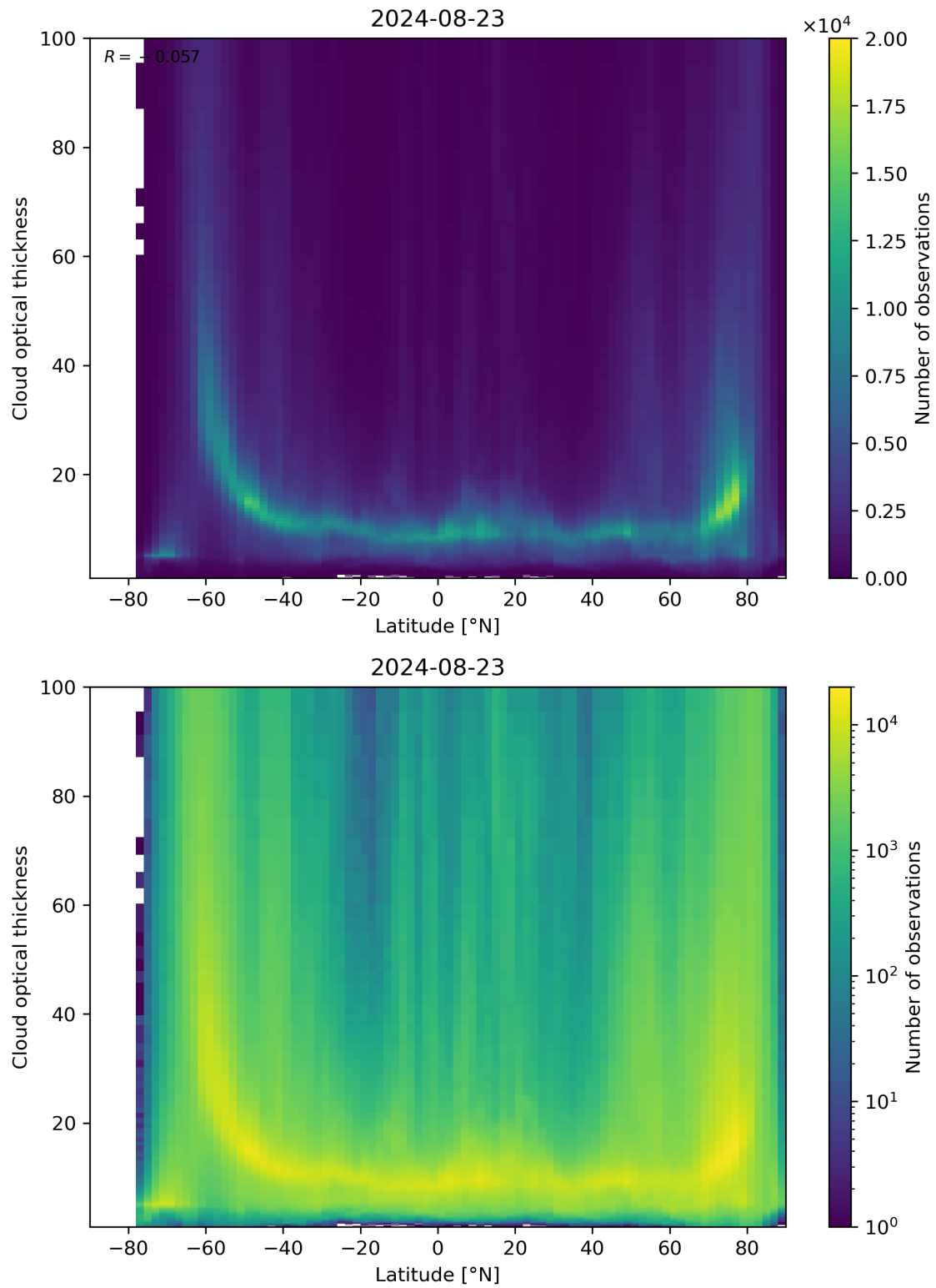
Figure 96: Scatter density plot of “Latitude” against “Cloud optical thickness” for 2024-08-22 to 2024-08-24.
