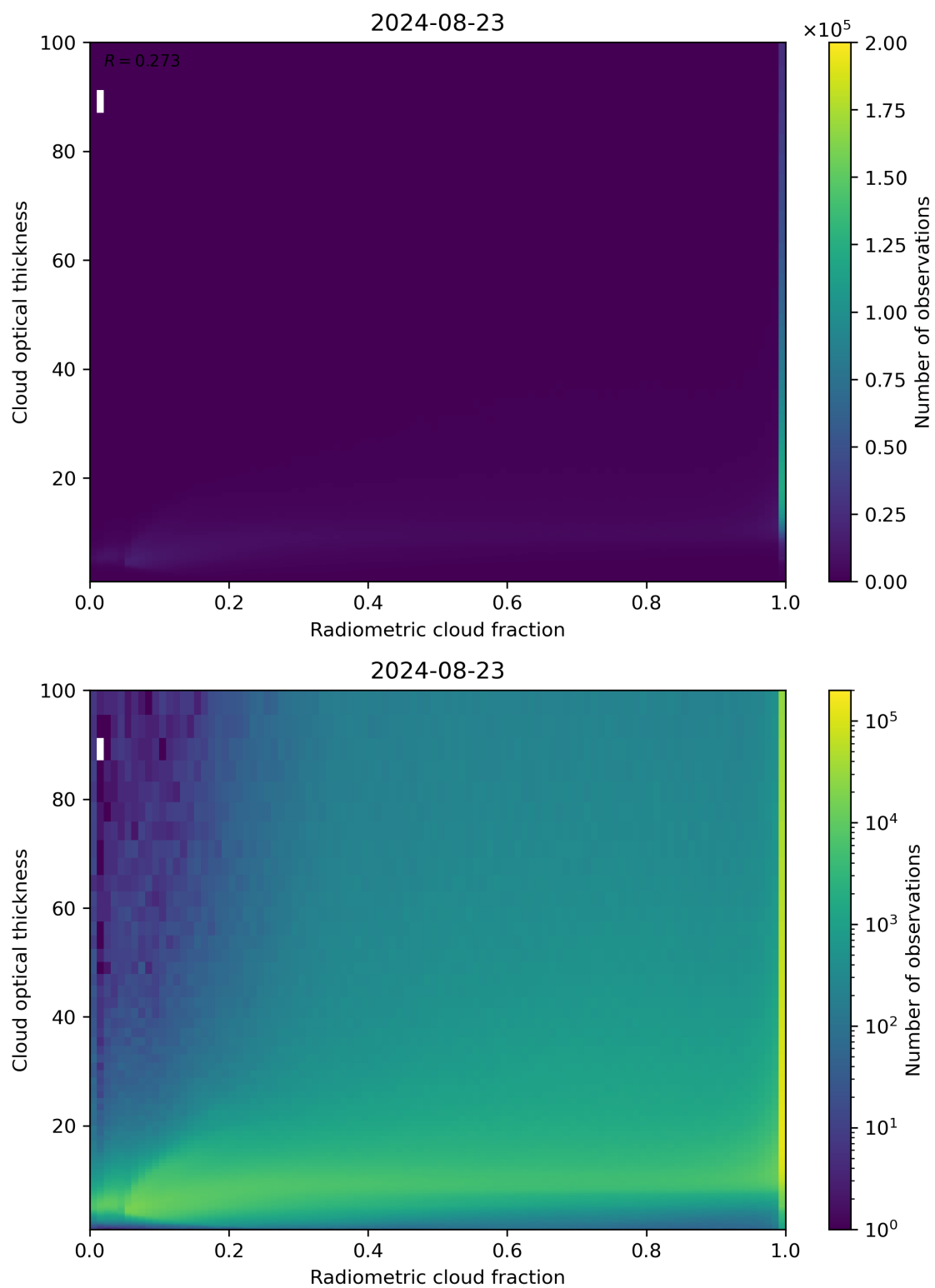
Figure 75: Scatter density plot of “Radiometric cloud fraction” against “Cloud optical thickness” for 2024-08-22 to 2024-08-24.
