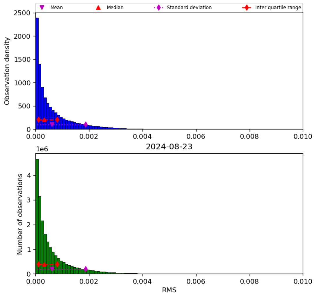
Figure 47: Histogram of “RMS” for 2024-08-22 to 2024-08-24
