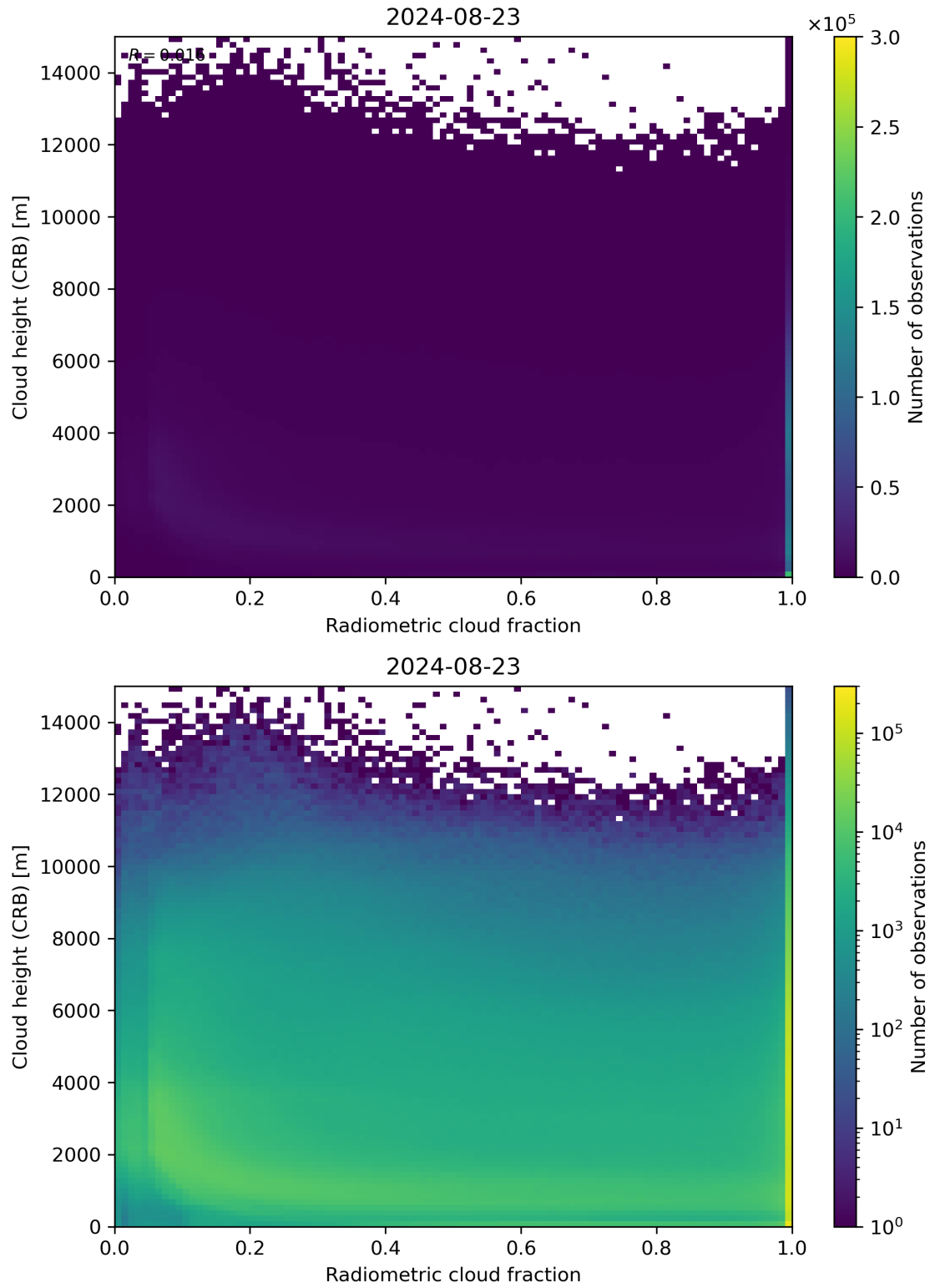
Figure 74: Scatter density plot of “Radiometric cloud fraction” against “Cloud height (CRB)” for 2024-08-22 to 2024-08-24.
