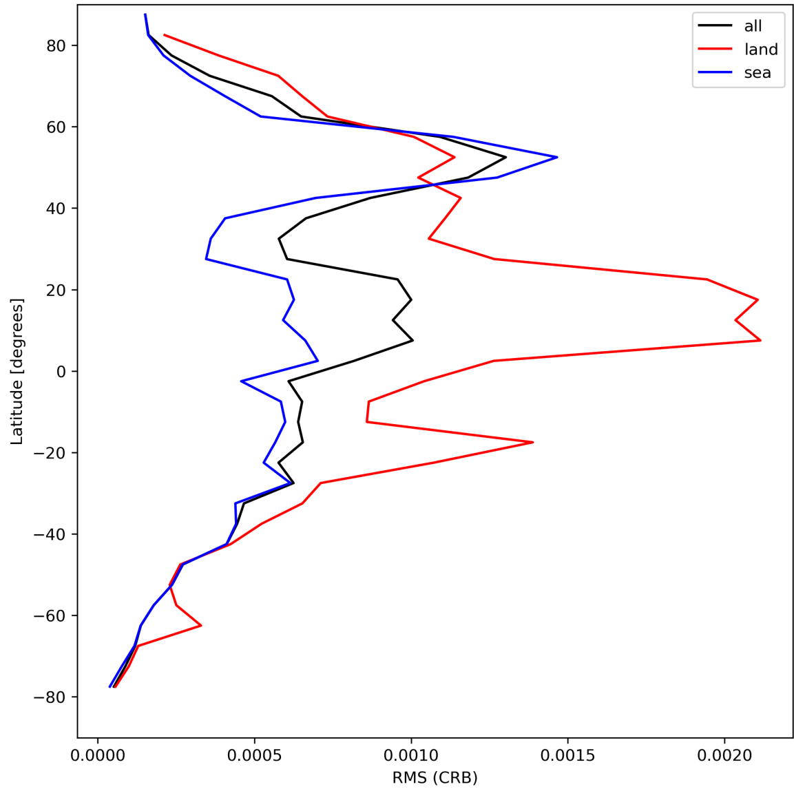
Figure 32: Zonal average of “RMS (CRB)” for 2024-08-23 to 2024-08-25.
