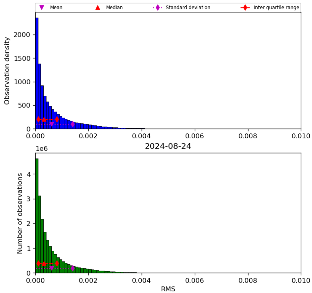
Figure 47: Histogram of “RMS” for 2024-08-23 to 2024-08-25
