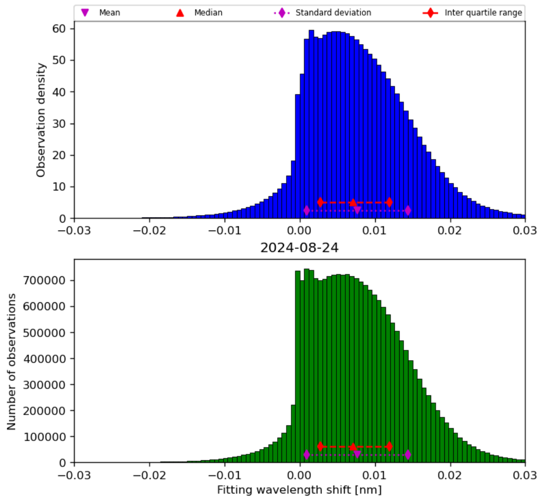
Figure 49: Histogram of “Fitting wavelength shift” for 2024-08-23 to 2024-08-25
