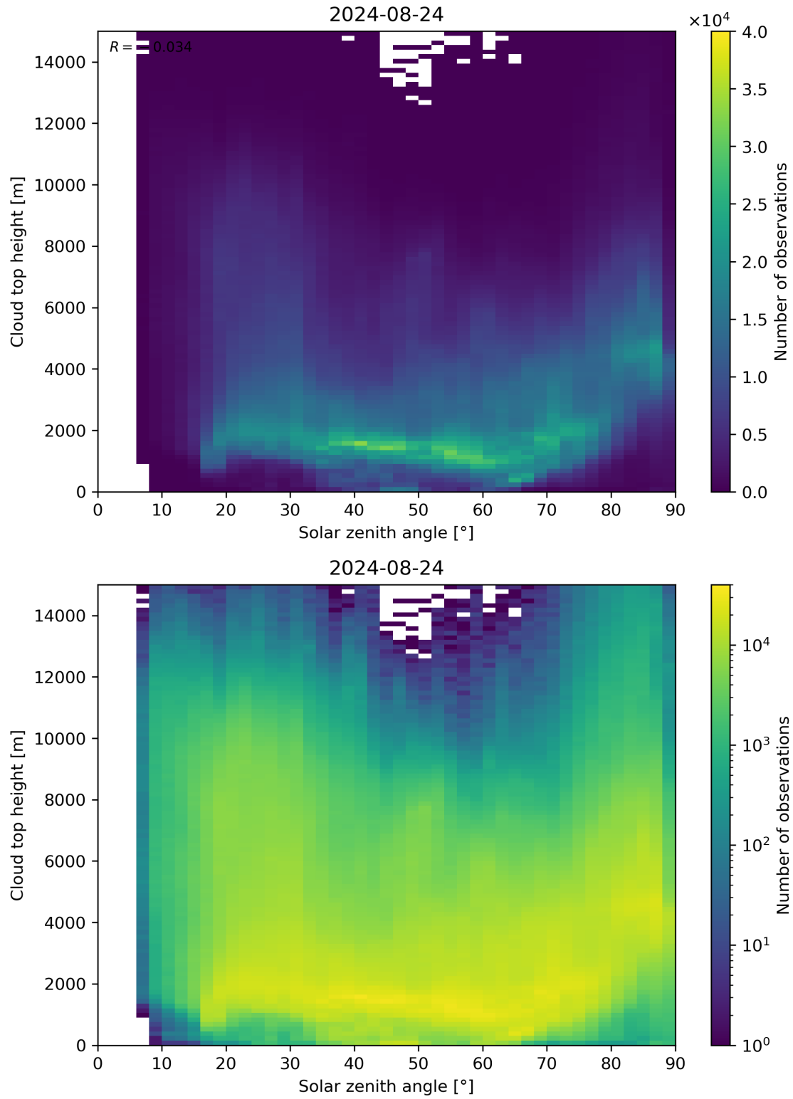
Figure 104: Scatter density plot of “Solar zenith angle” against “Cloud top height” for 2024-08-23 to 2024-08-25.
