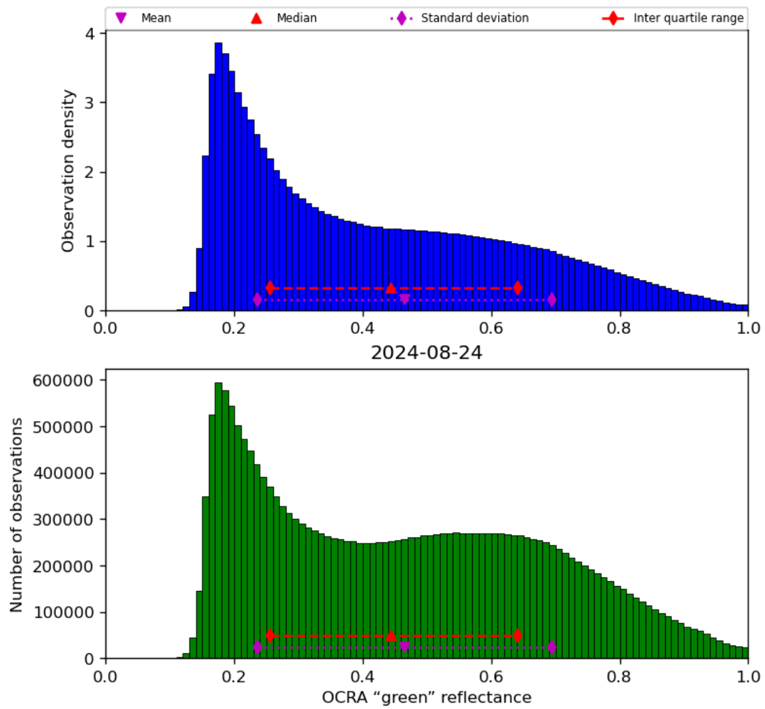
Figure 52: Histogram of “OCRA “green” reflectance” for 2024-08-23 to 2024-08-25
