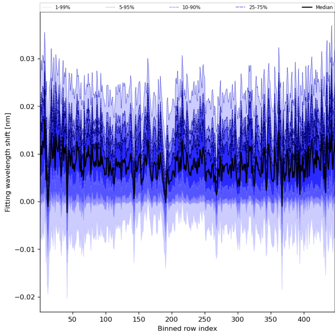
Figure 65: Along track statistics of “Fitting wavelength shift” for 2024-08-23 to 2024-08-25
