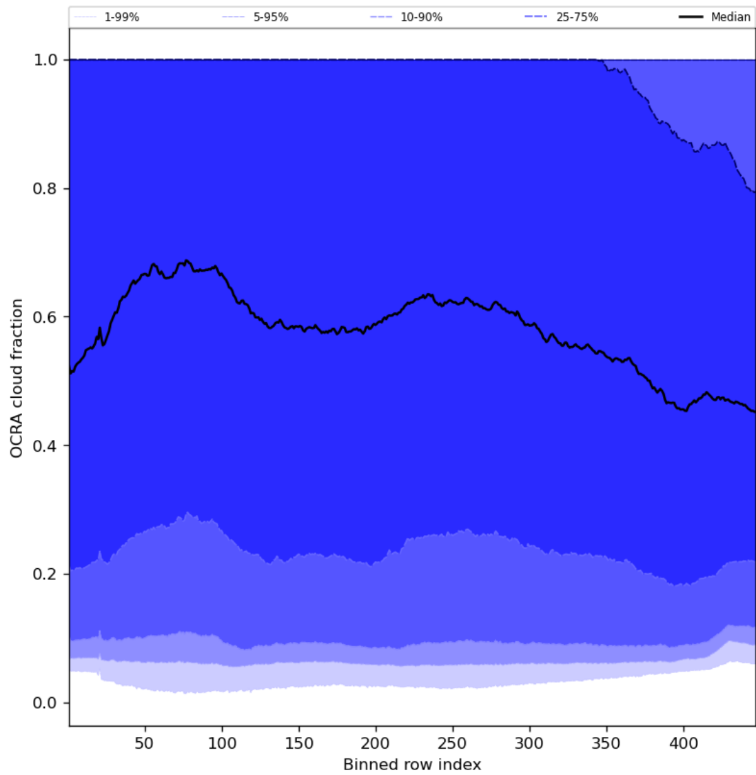
Figure 66: Along track statistics of “OCRA cloud fraction” for 2024-08-23 to 2024-08-25
