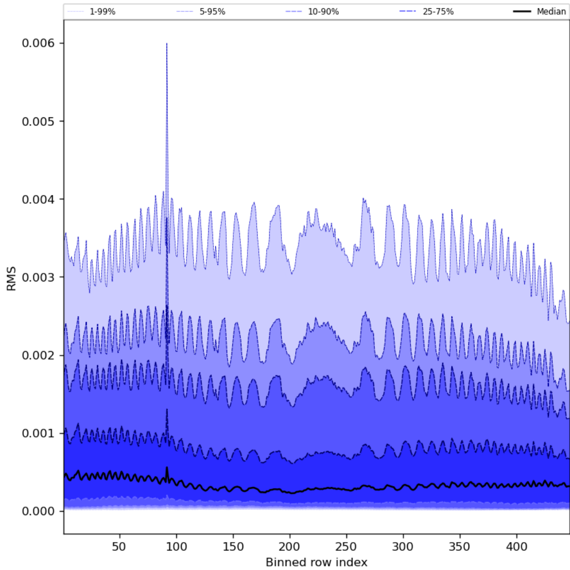
Figure 63: Along track statistics of “RMS” for 2024-08-23 to 2024-08-25
