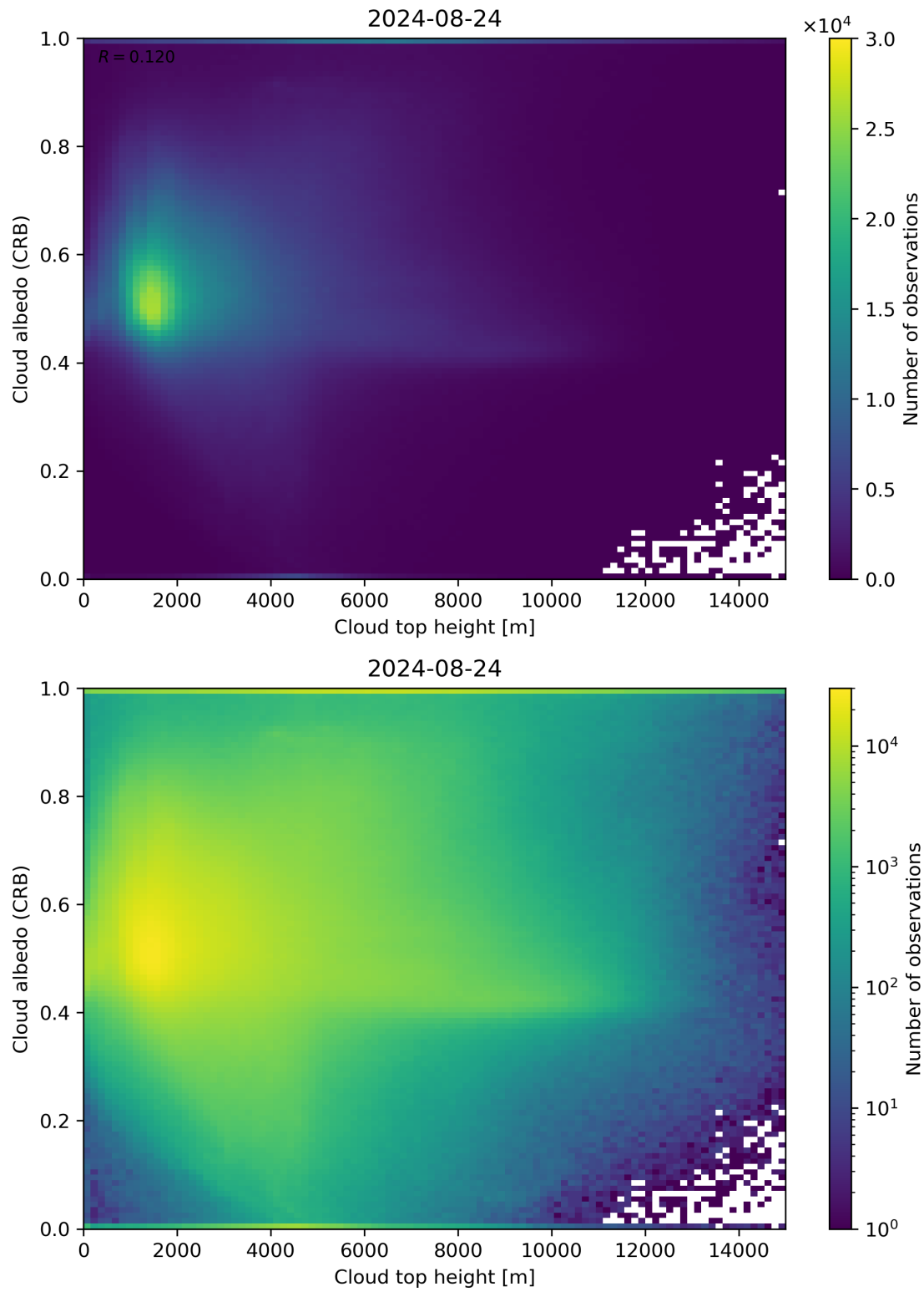
Figure 86: Scatter density plot of “Cloud top height” against “Cloud albedo (CRB)” for 2024-08-23 to 2024-08-25.
