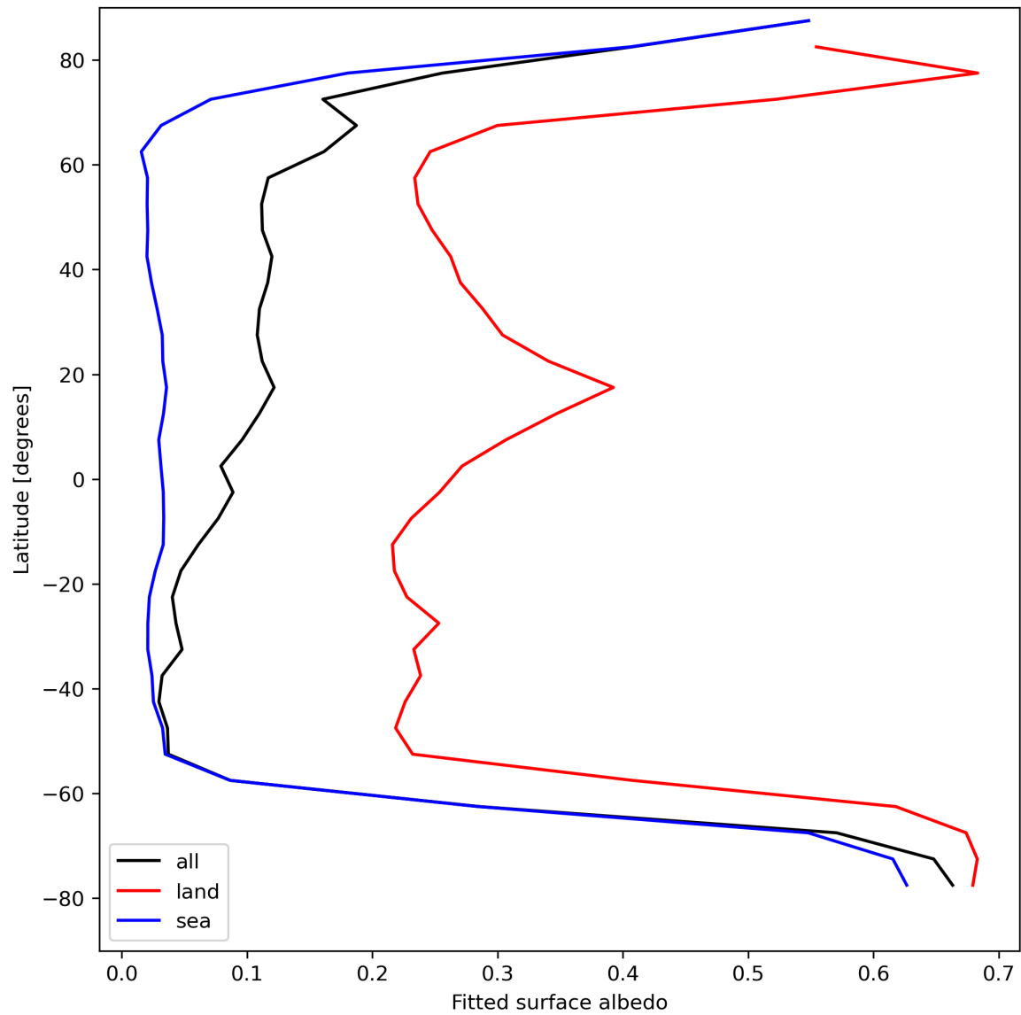
Figure 29: Zonal average of “Fitted surface albedo” for 2024-08-23 to 2024-08-25.
