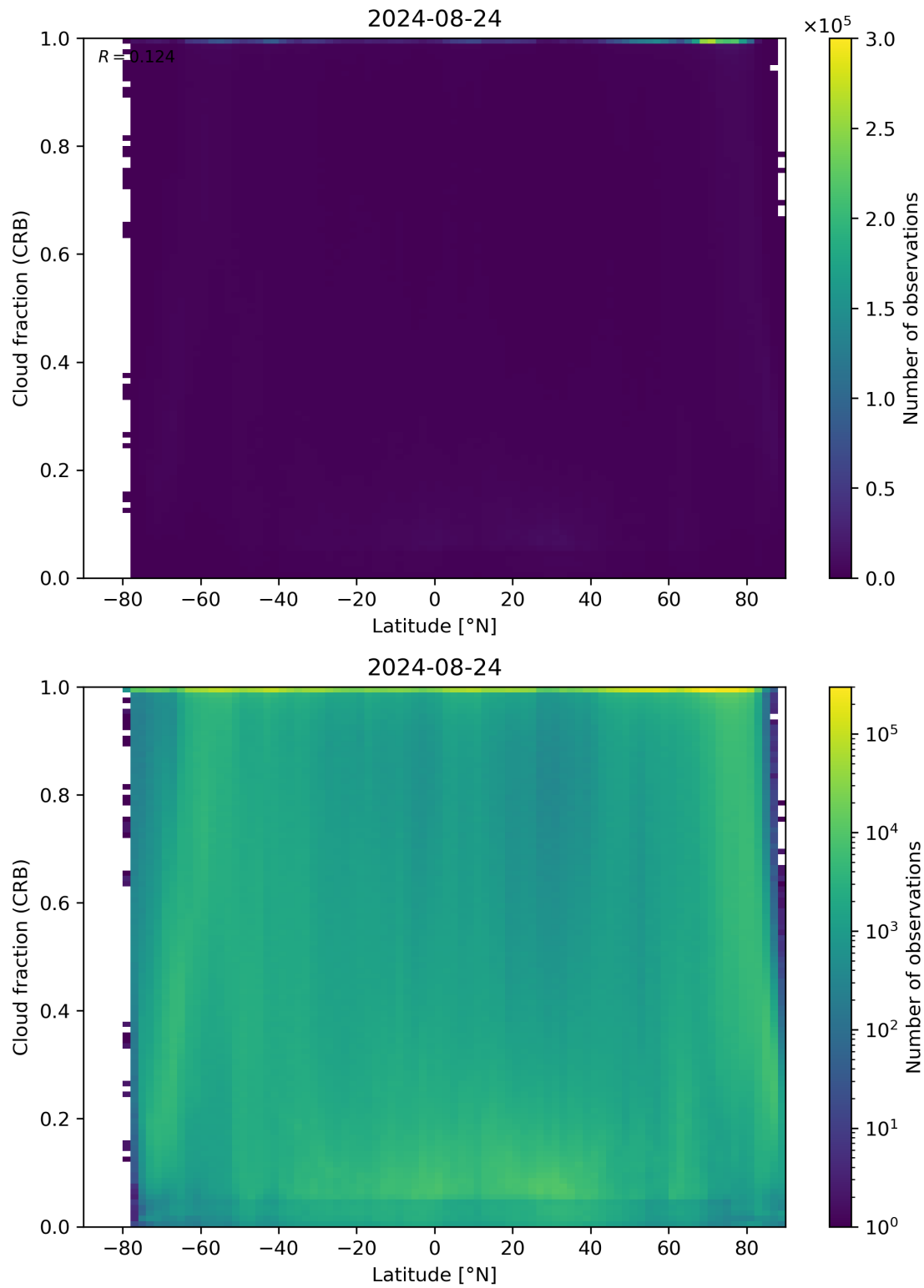
Figure 94: Scatter density plot of “Latitude” against “Cloud fraction (CRB)” for 2024-08-23 to 2024-08-25.
