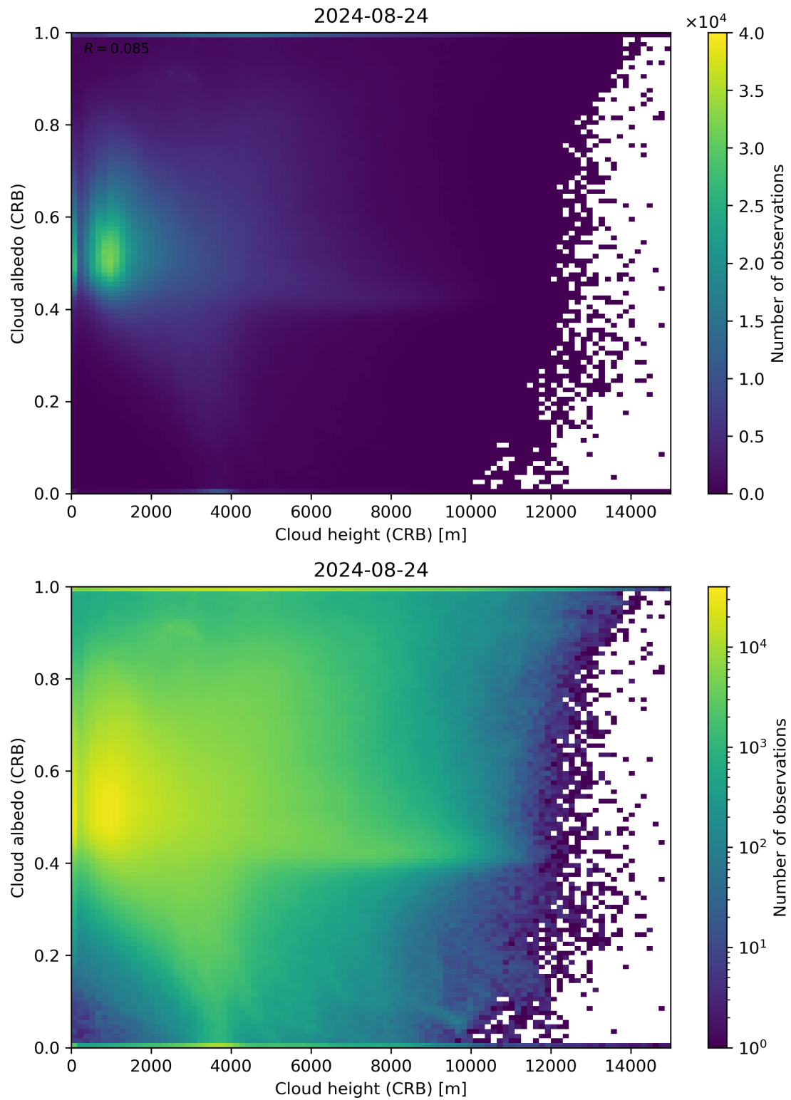
Figure 80: Scatter density plot of “Cloud height (CRB)” against “Cloud albedo (CRB)” for 2024-08-23 to 2024-08-25.
