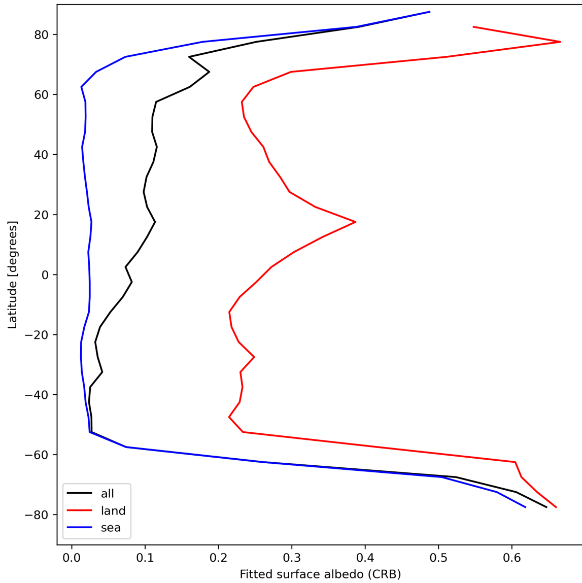
Figure 30: Zonal average of “Fitted surface albedo (CRB)” for 2024-08-23 to 2024-08-25.
