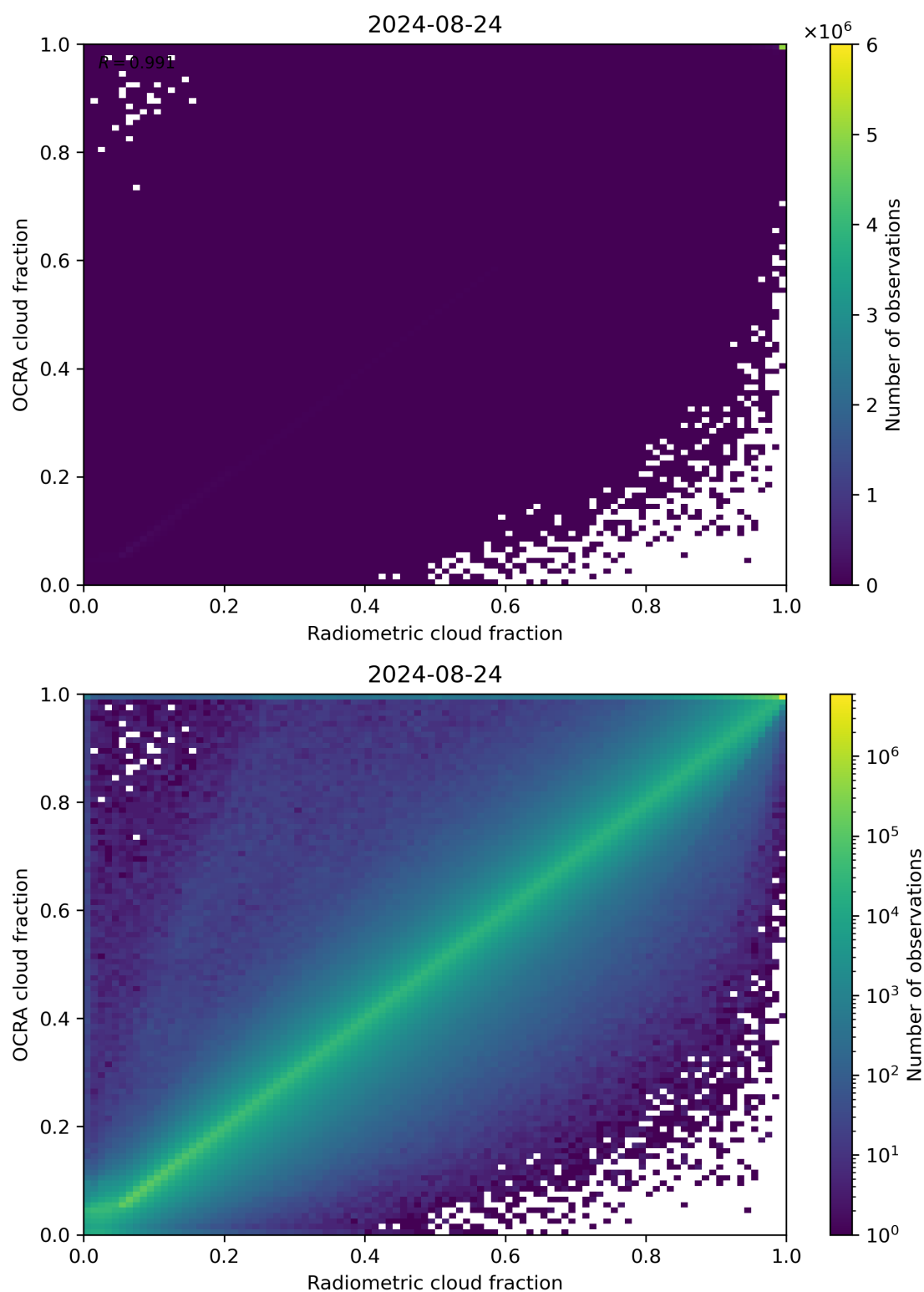
Figure 72: Scatter density plot of “Radiometric cloud fraction” against “OCRA cloud fraction” for 2024-08-23 to 2024-08-25.
