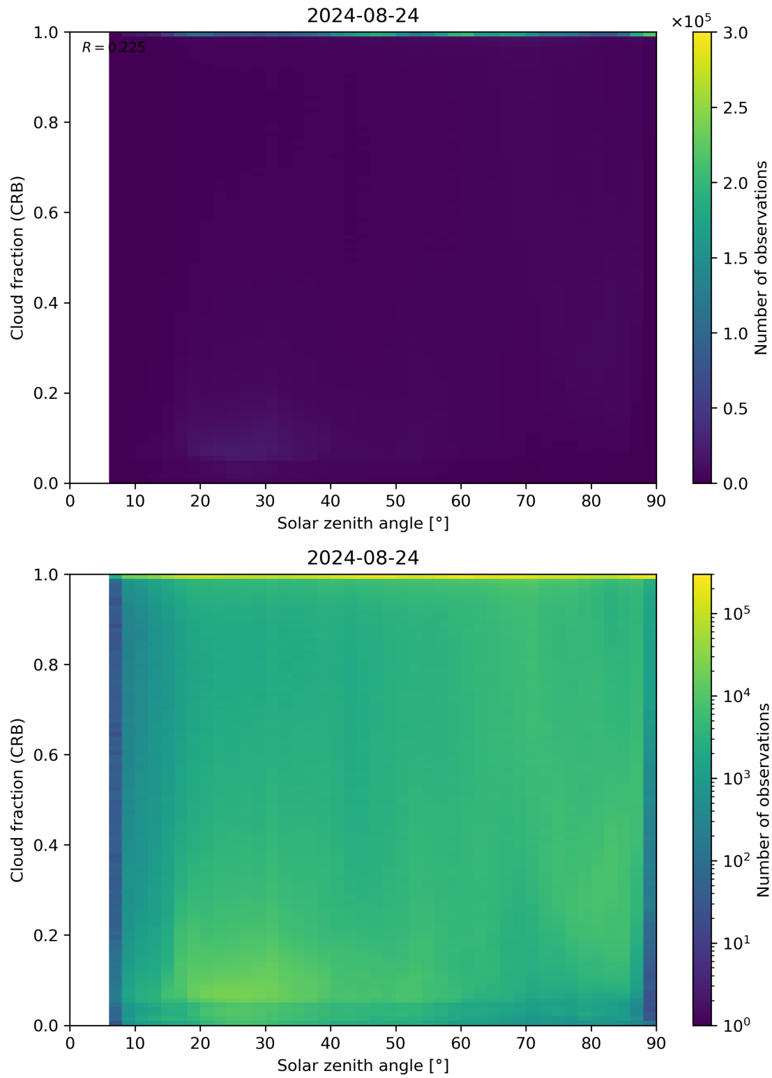
Figure 101: Scatter density plot of “Solar zenith angle” against “Cloud fraction (CRB)” for 2024-08-23 to 2024-08-25.
