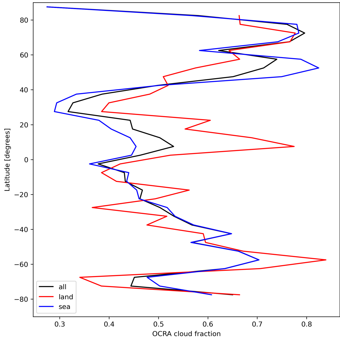
Figure 34: Zonal average of “OCRA cloud fraction” for 2024-08-23 to 2024-08-25.
