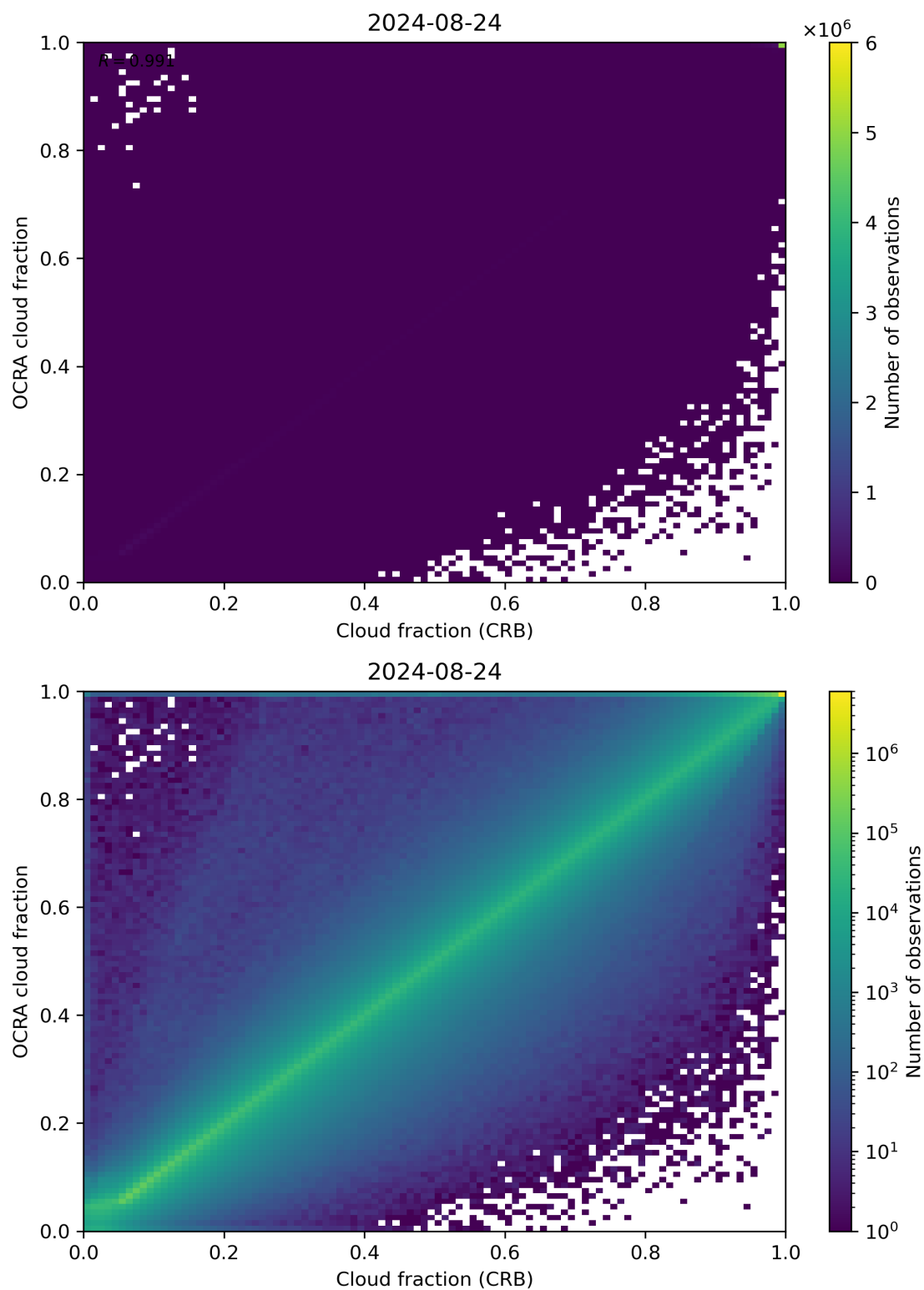
Figure 78: Scatter density plot of “Cloud fraction (CRB)” against “OCRA cloud fraction” for 2024-08-23 to 2024-08-25.
