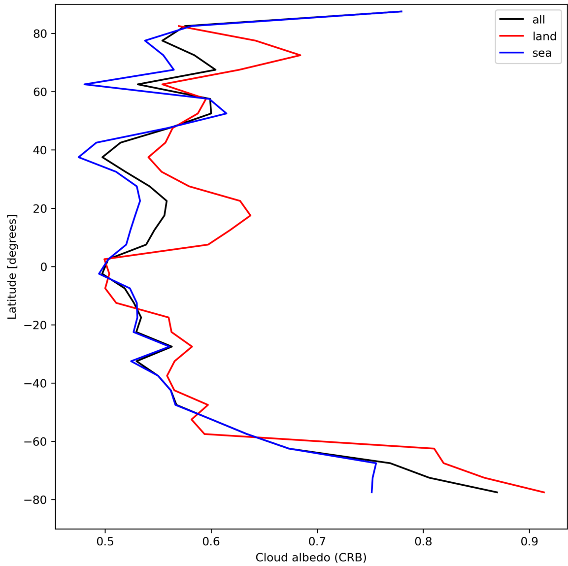
Figure 28: Zonal average of “Cloud albedo (CRB)” for 2024-08-23 to 2024-08-25.
