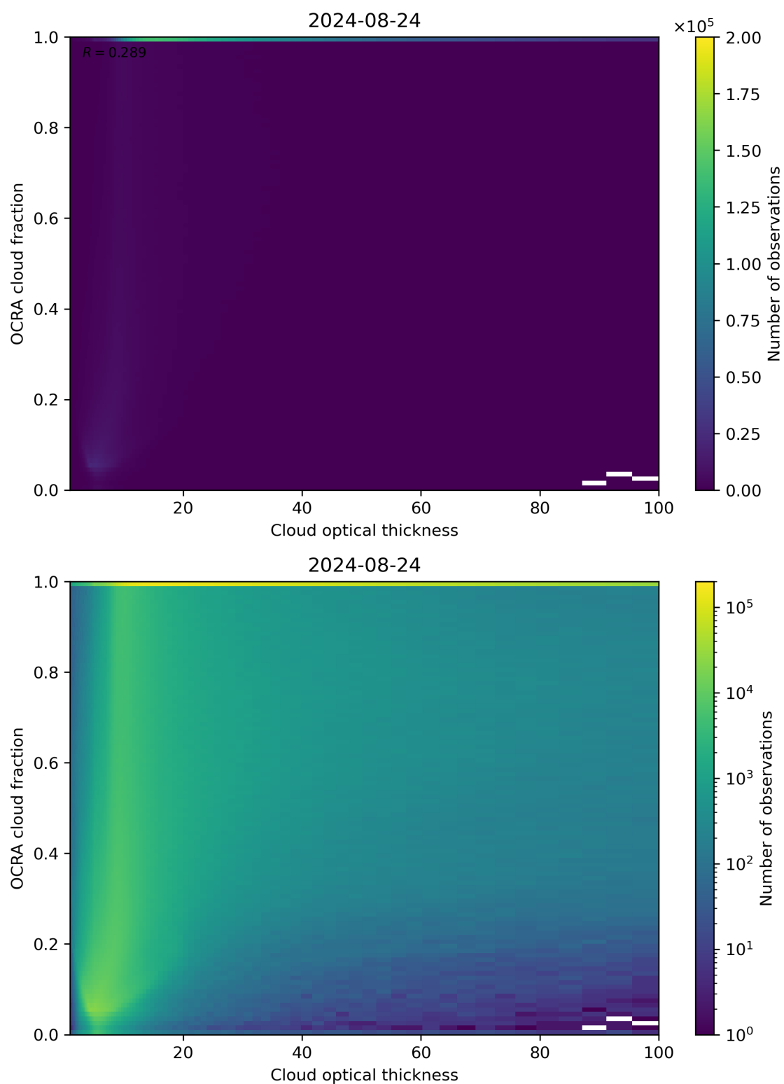
Figure 83: Scatter density plot of “Cloud optical thickness” against “OCRA cloud fraction” for 2024-08-23 to 2024-08-25.
