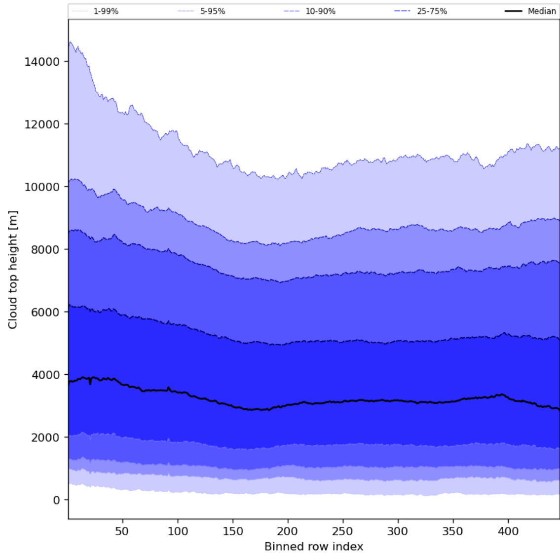
Figure 56: Along track statistics of “Cloud top height” for 2024-08-23 to 2024-08-25
