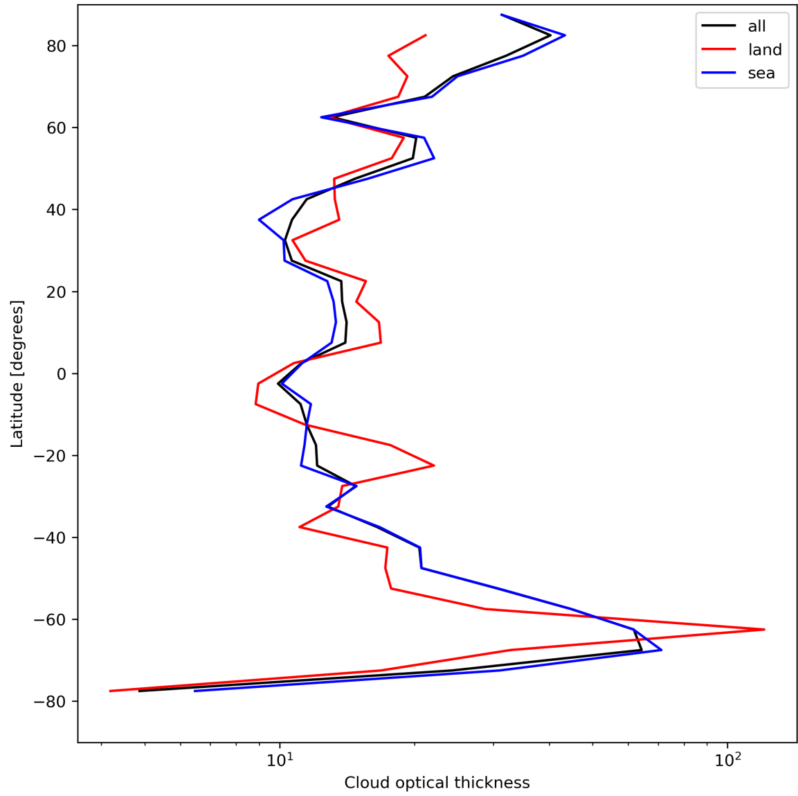
Figure 25: Zonal average of “Cloud optical thickness” for 2024-08-23 to 2024-08-25.
