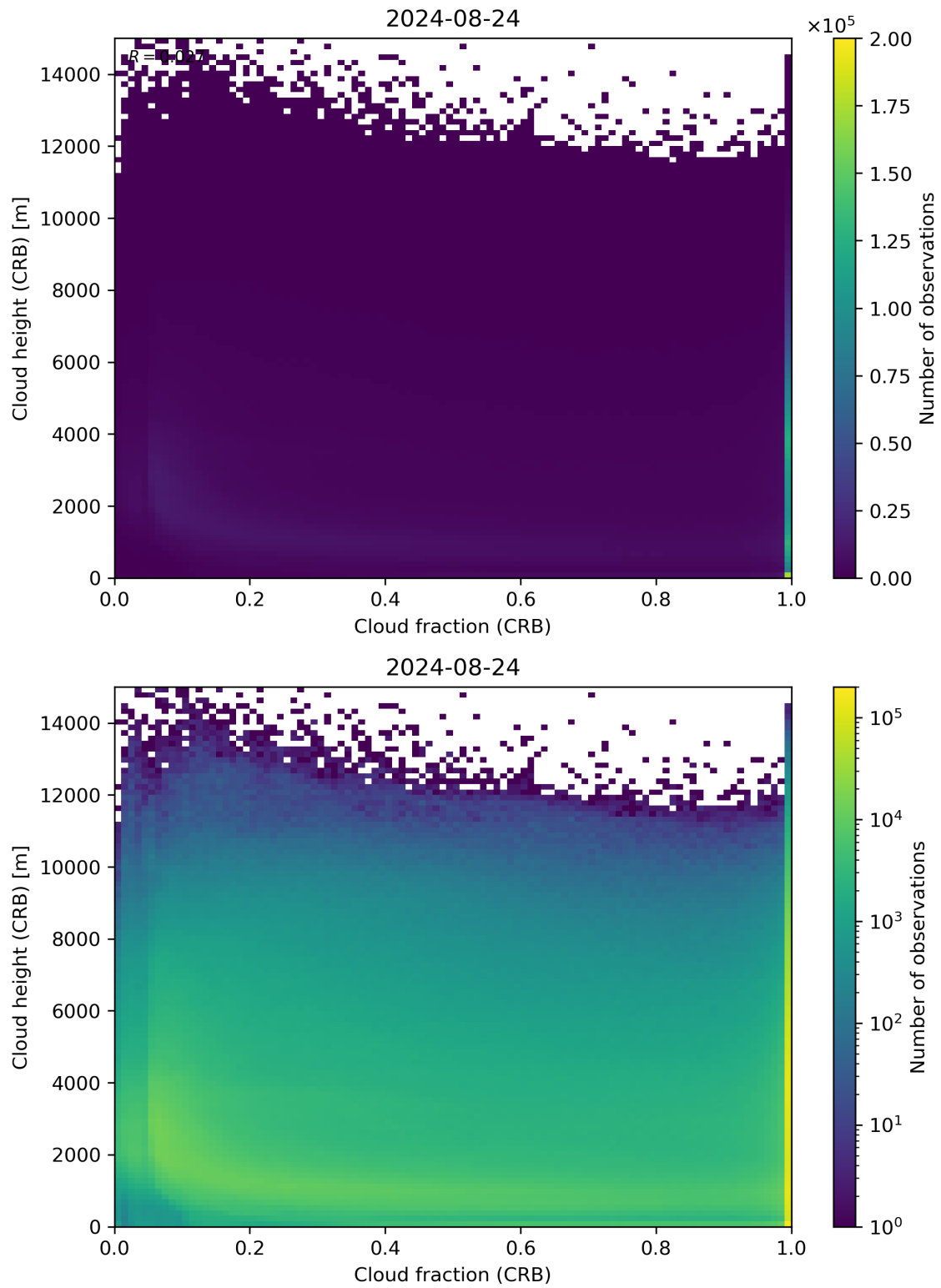
Figure 79: Scatter density plot of “Cloud fraction (CRB)” against “Cloud height (CRB)” for 2024-08-23 to 2024-08-25.
