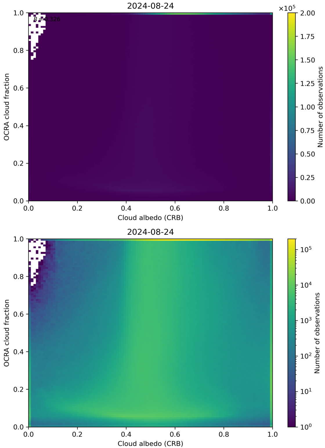
Figure 70: Scatter density plot of “Cloud albedo (CRB)” against “OCRA cloud fraction” for 2024-08-23 to 2024-08-25.
