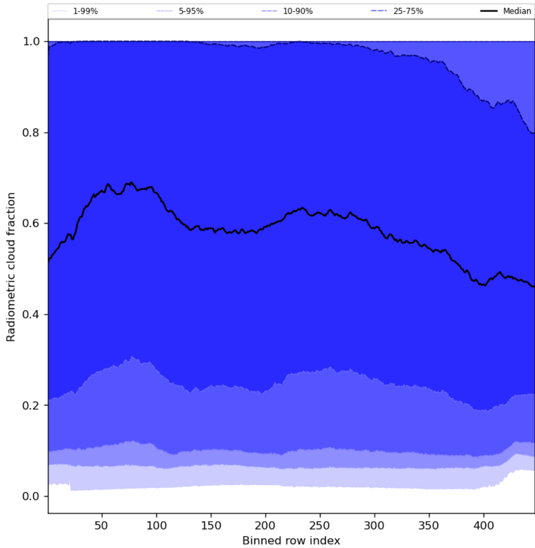
Figure 55: Along track statistics of “Radiometric cloud fraction” for 2024-08-23 to 2024-08-25
