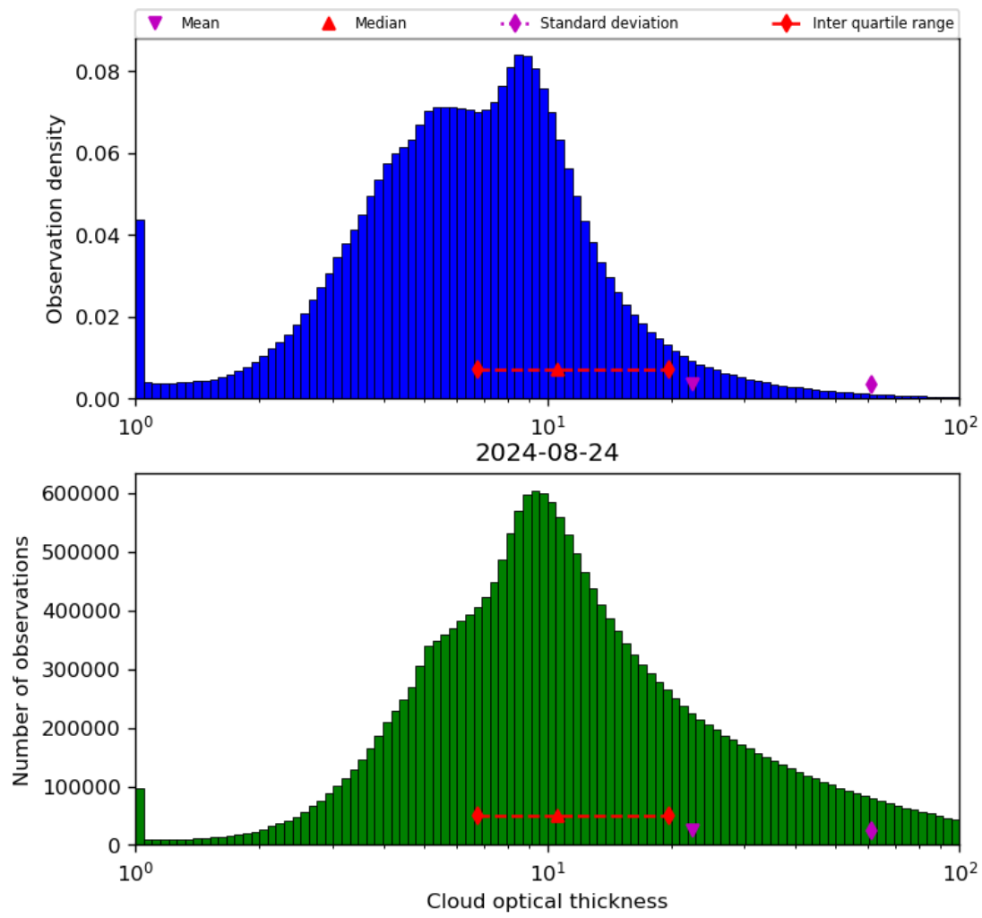
Figure 41: Histogram of “Cloud optical thickness” for 2024-08-23 to 2024-08-25
