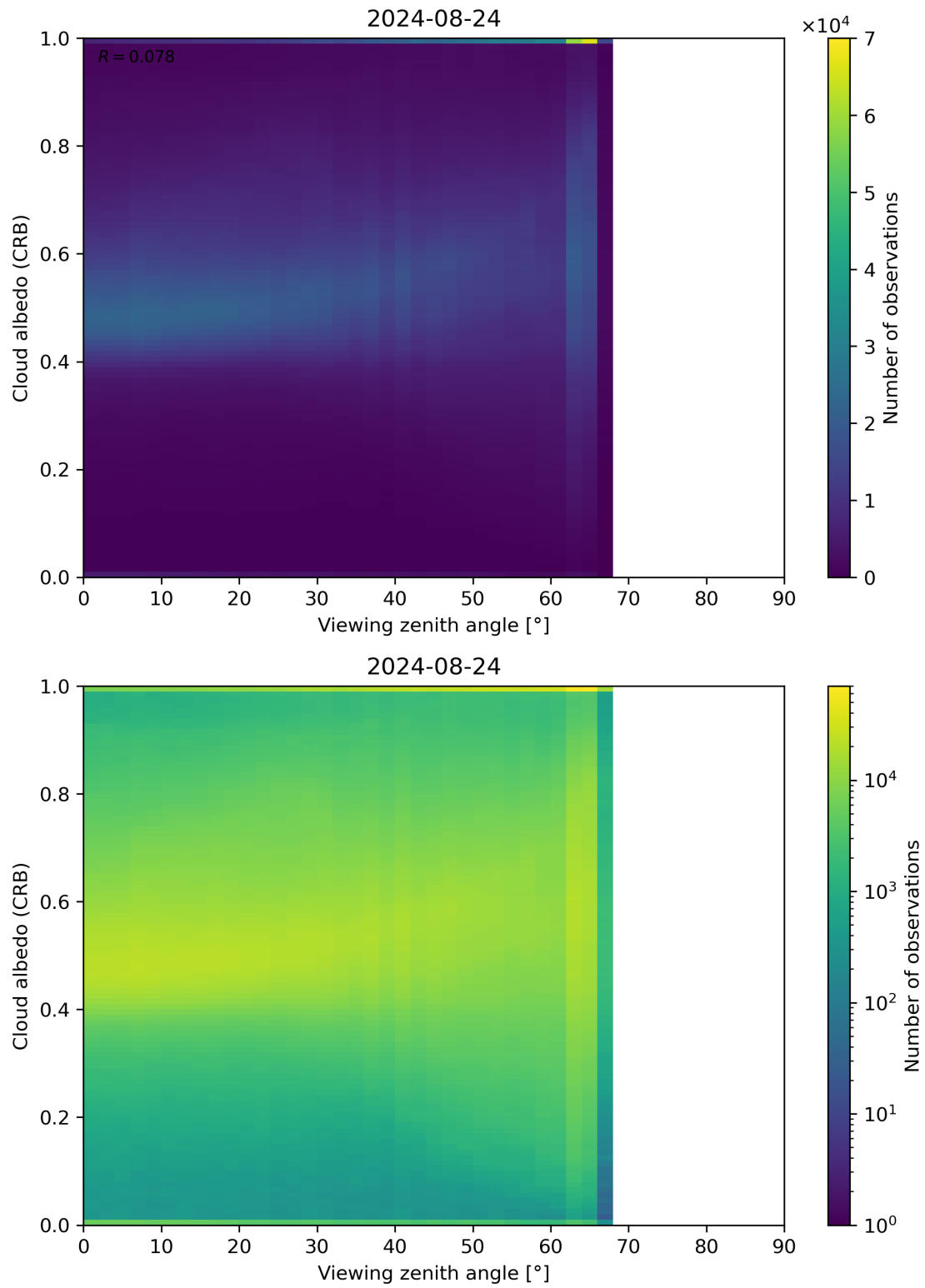
Figure 106: Scatter density plot of “Viewing zenith angle” against “Cloud albedo (CRB)” for 2024-08-23 to 2024-08-25.
