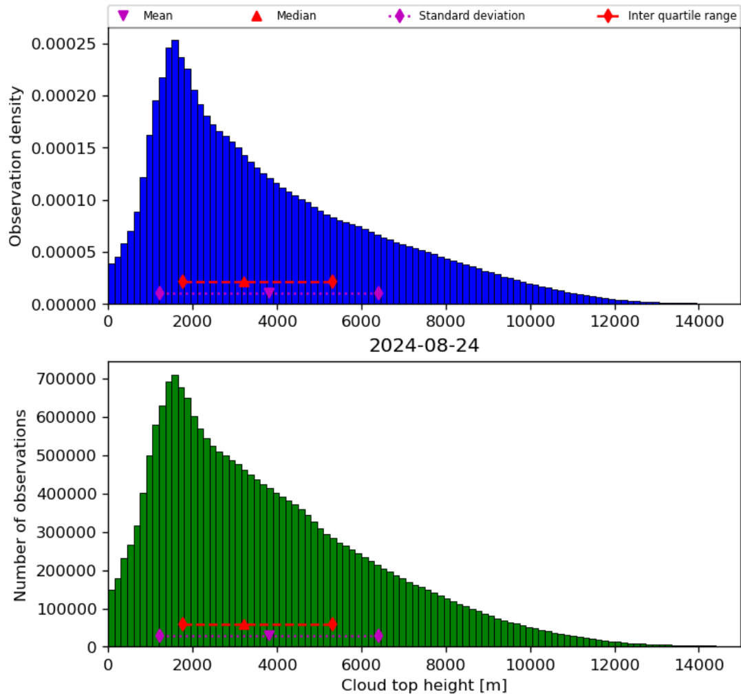
Figure 40: Histogram of “Cloud top height” for 2024-08-23 to 2024-08-25
