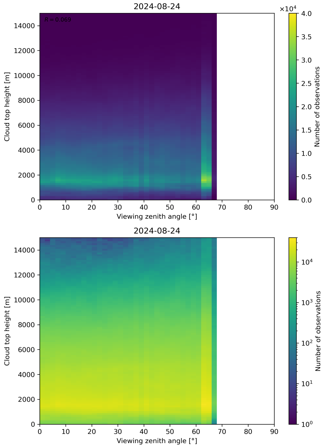
Figure 112: Scatter density plot of “Viewing zenith angle” against “Cloud top height” for 2024-08-23 to 2024-08-25.
