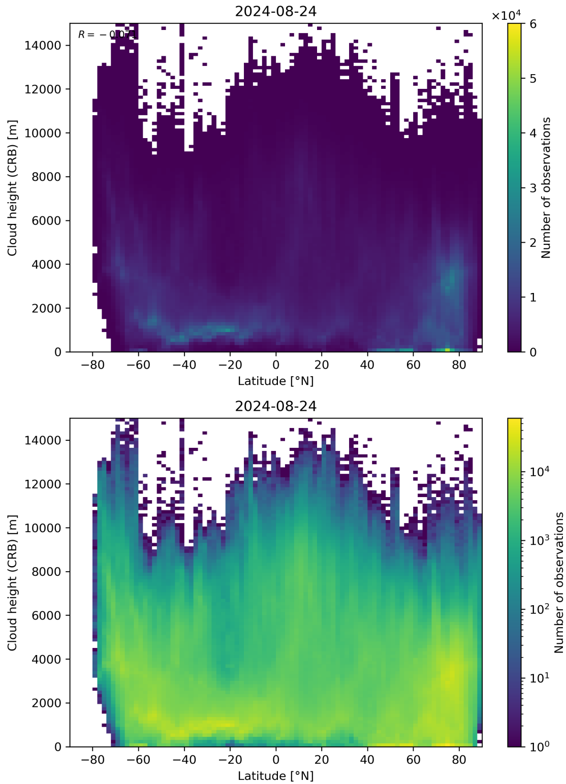
Figure 95: Scatter density plot of “Latitude” against “Cloud height (CRB)” for 2024-08-23 to 2024-08-25.
