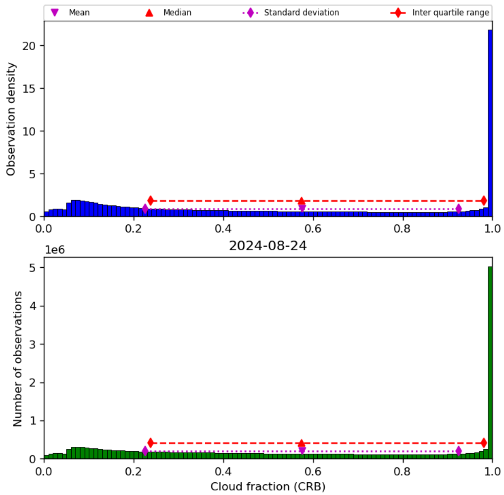
Figure 42: Histogram of “Cloud fraction (CRB)” for 2024-08-23 to 2024-08-25
