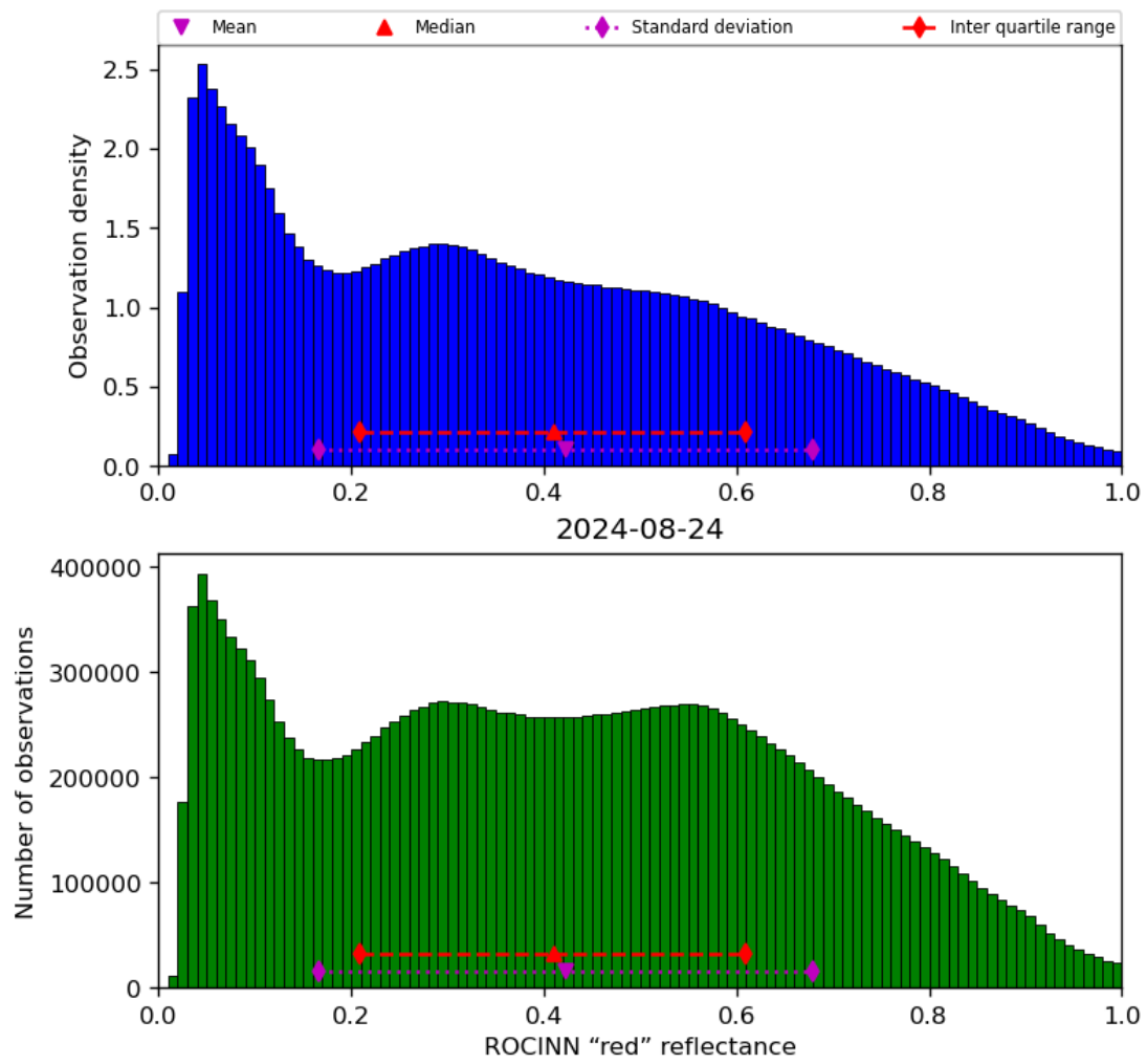
Figure 53: Histogram of “ROCINN “red” reflectance” for 2024-08-23 to 2024-08-25
