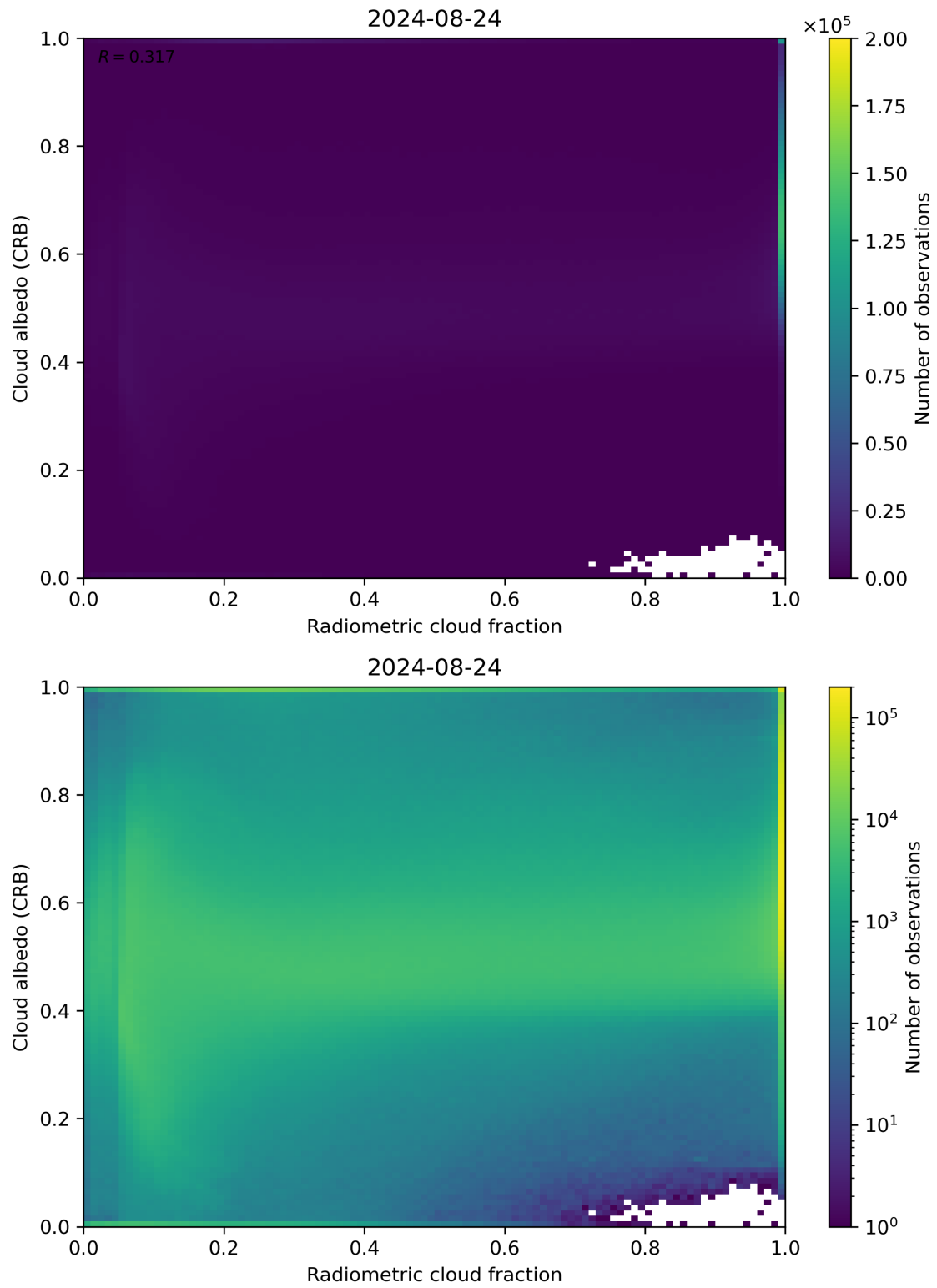
Figure 71: Scatter density plot of “Radiometric cloud fraction” against “Cloud albedo (CRB)” for 2024-08-23 to 2024-08-25.
