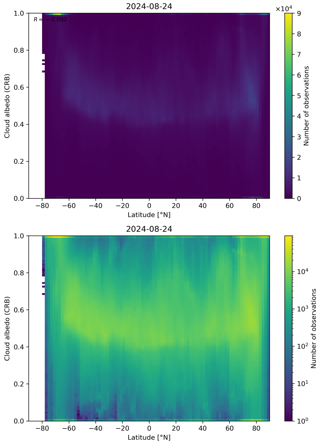
Figure 91: Scatter density plot of “Latitude” against “Cloud albedo (CRB)” for 2024-08-23 to 2024-08-25.
