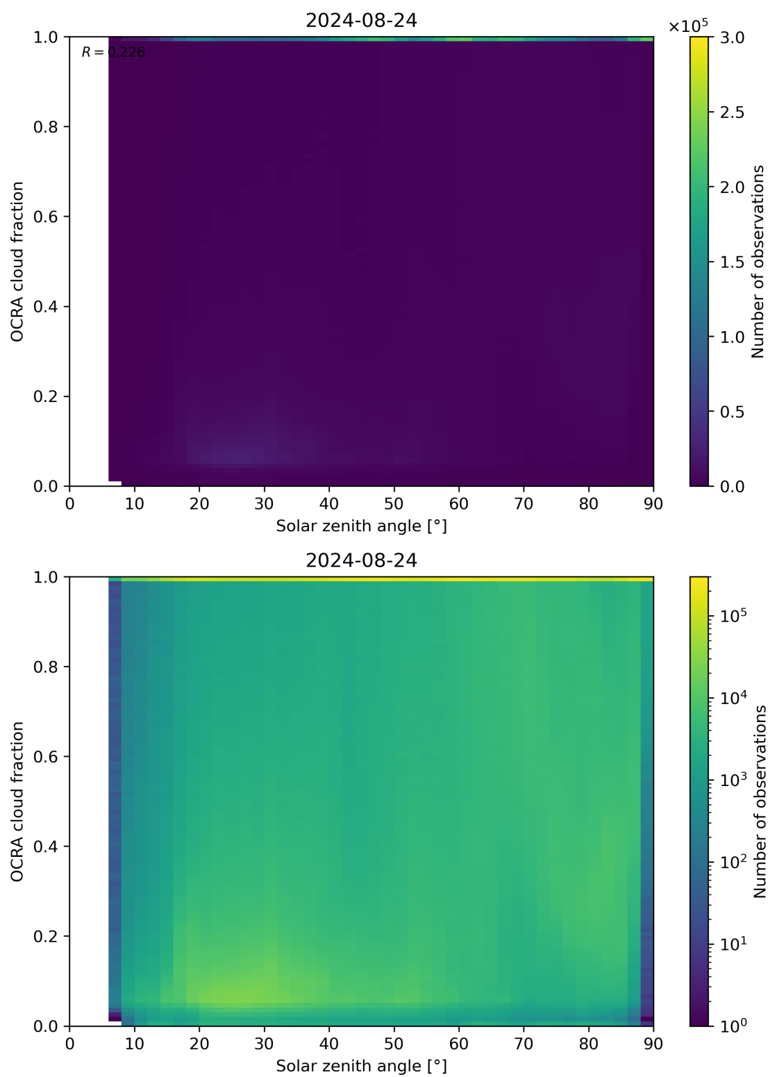
Figure 100: Scatter density plot of “Solar zenith angle” against “OCRA cloud fraction” for 2024-08-23 to 2024-08-25.
