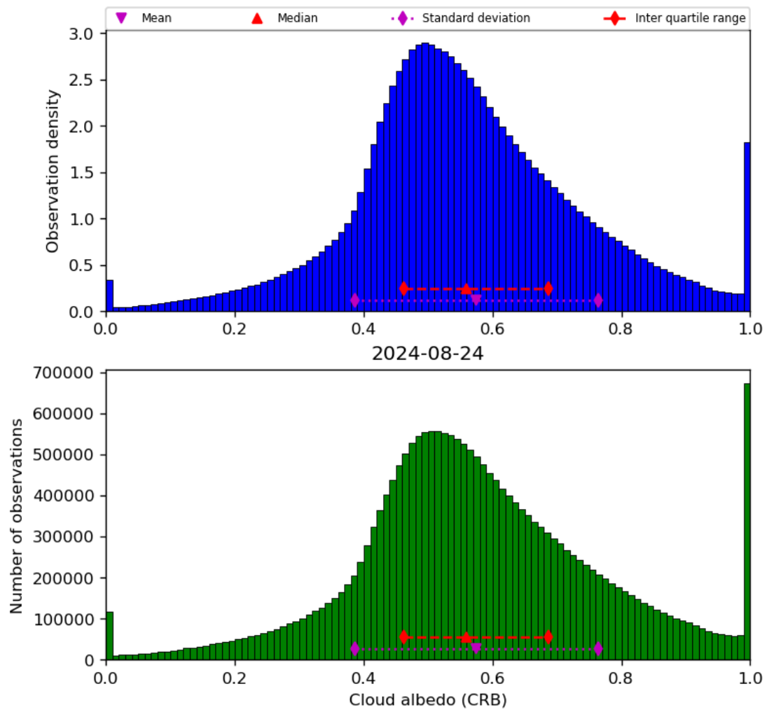
Figure 44: Histogram of “Cloud albedo (CRB)” for 2024-08-23 to 2024-08-25
