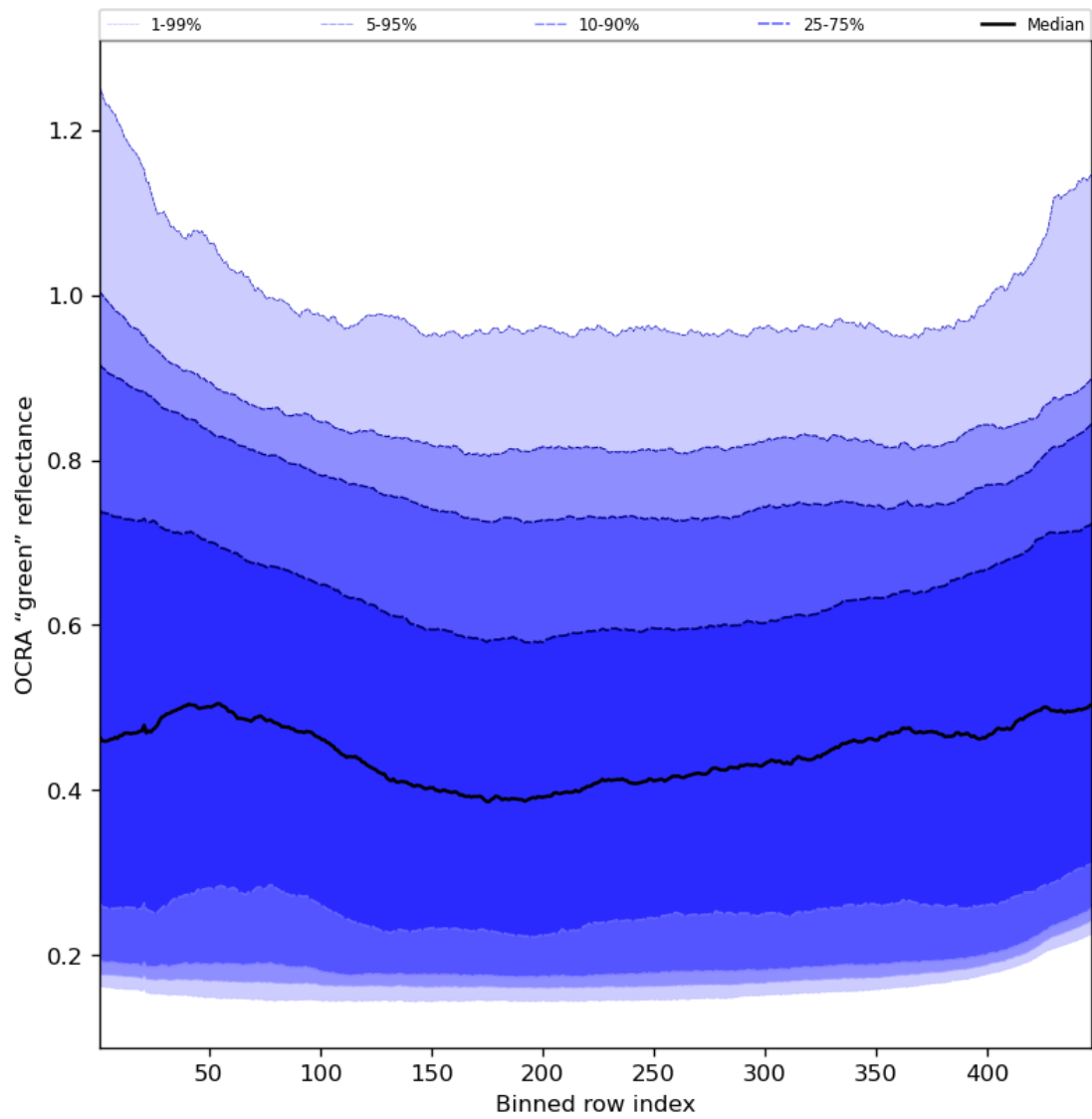
Figure 68: Along track statistics of "OCRA "green" reflectance" for 2024-08-23 to 2024-08-25
