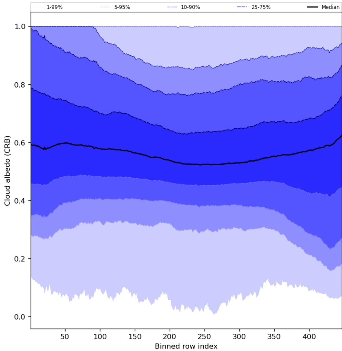
Figure 60: Along track statistics of “Cloud albedo (CRB)” for 2024-08-23 to 2024-08-25
