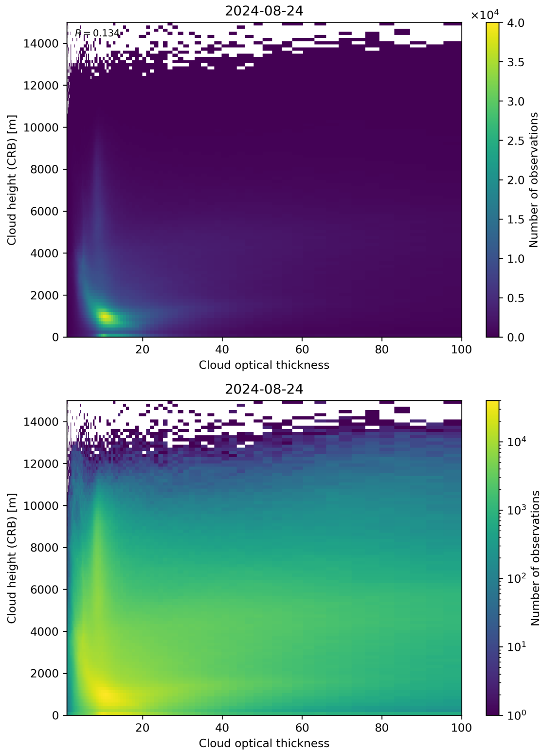
Figure 85: Scatter density plot of “Cloud optical thickness” against “Cloud height (CRB)” for 2024-08-23 to 2024-08-25.
