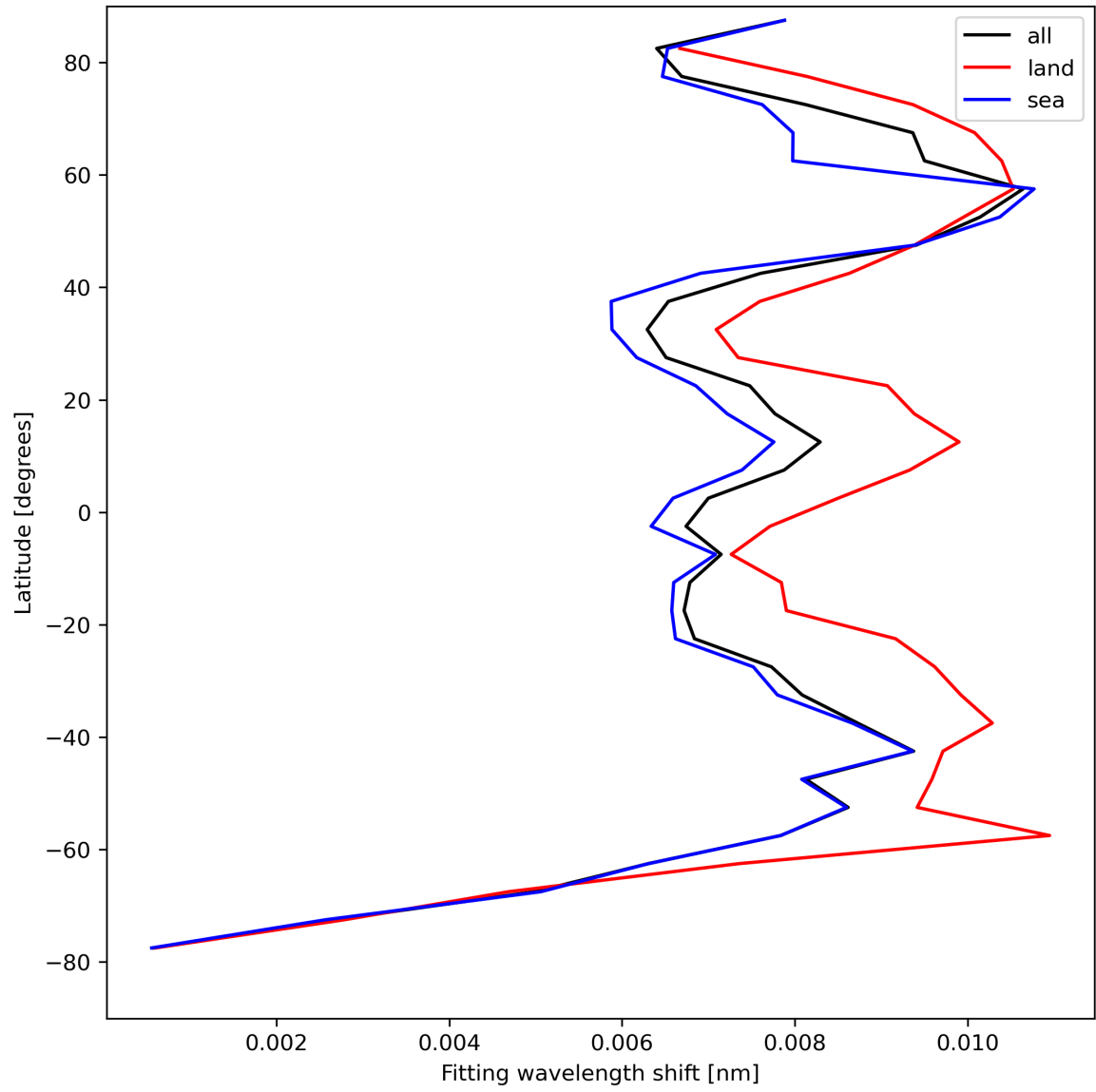
Figure 33: Zonal average of “Fitting wavelength shift” for 2024-08-23 to 2024-08-25.
