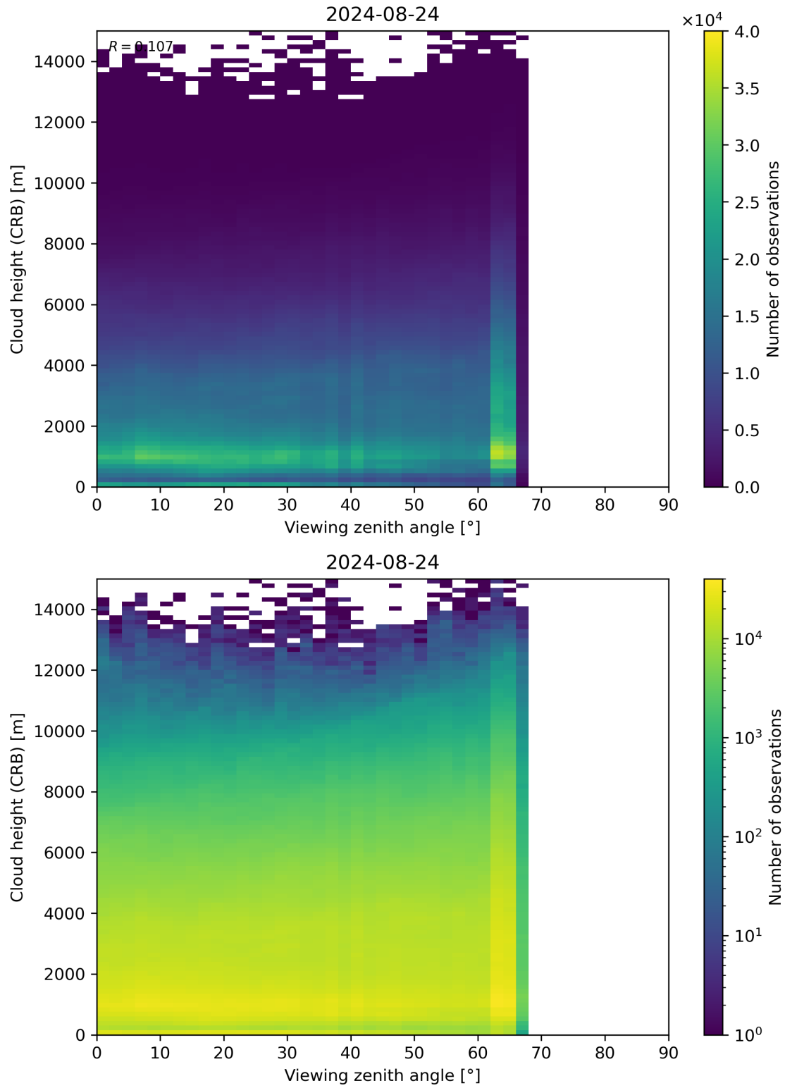
Figure 110: Scatter density plot of “Viewing zenith angle” against “Cloud height (CRB)” for 2024-08-23 to 2024-08-25.
