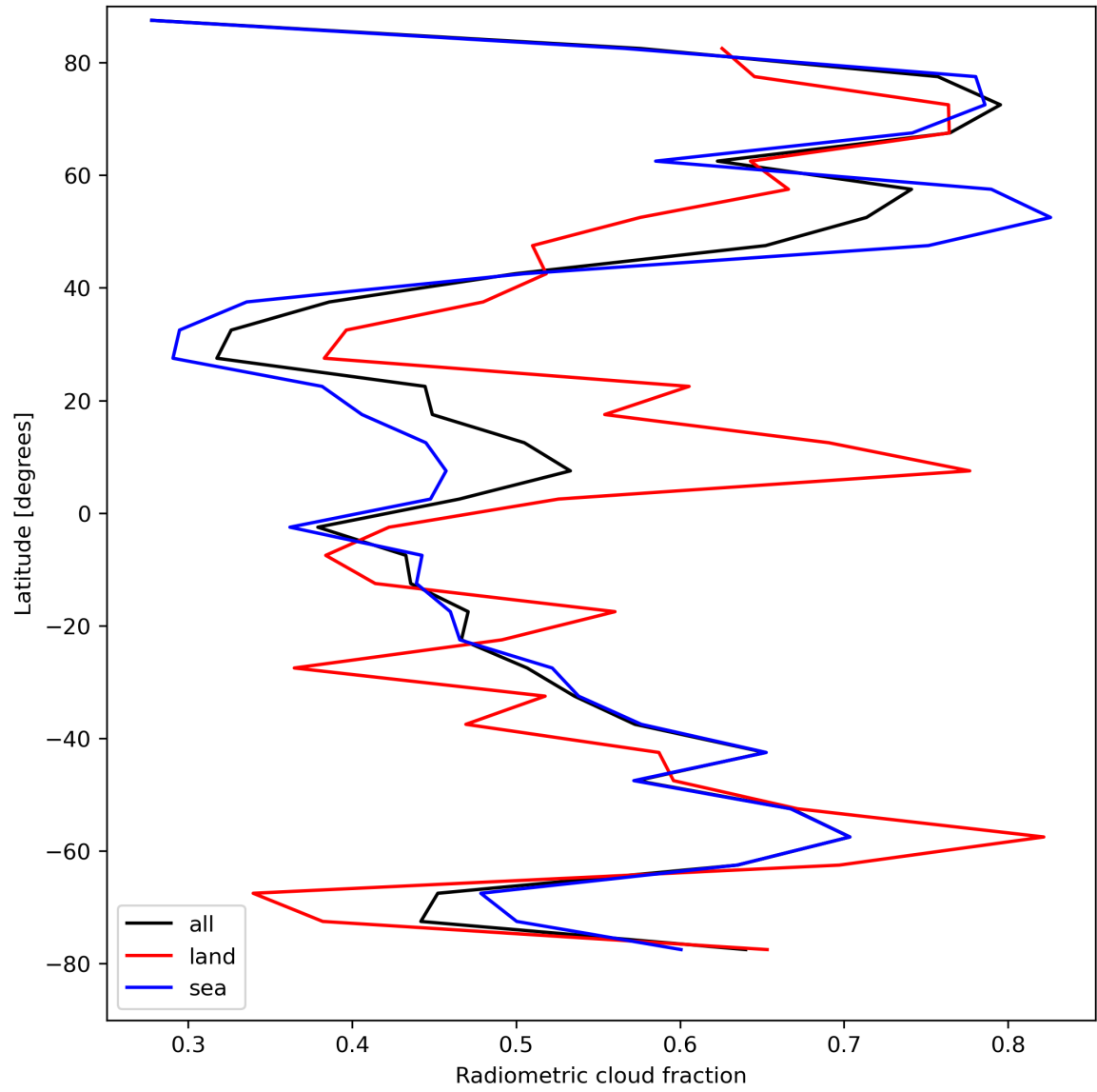
Figure 23: Zonal average of “Radiometric cloud fraction” for 2024-08-23 to 2024-08-25.
