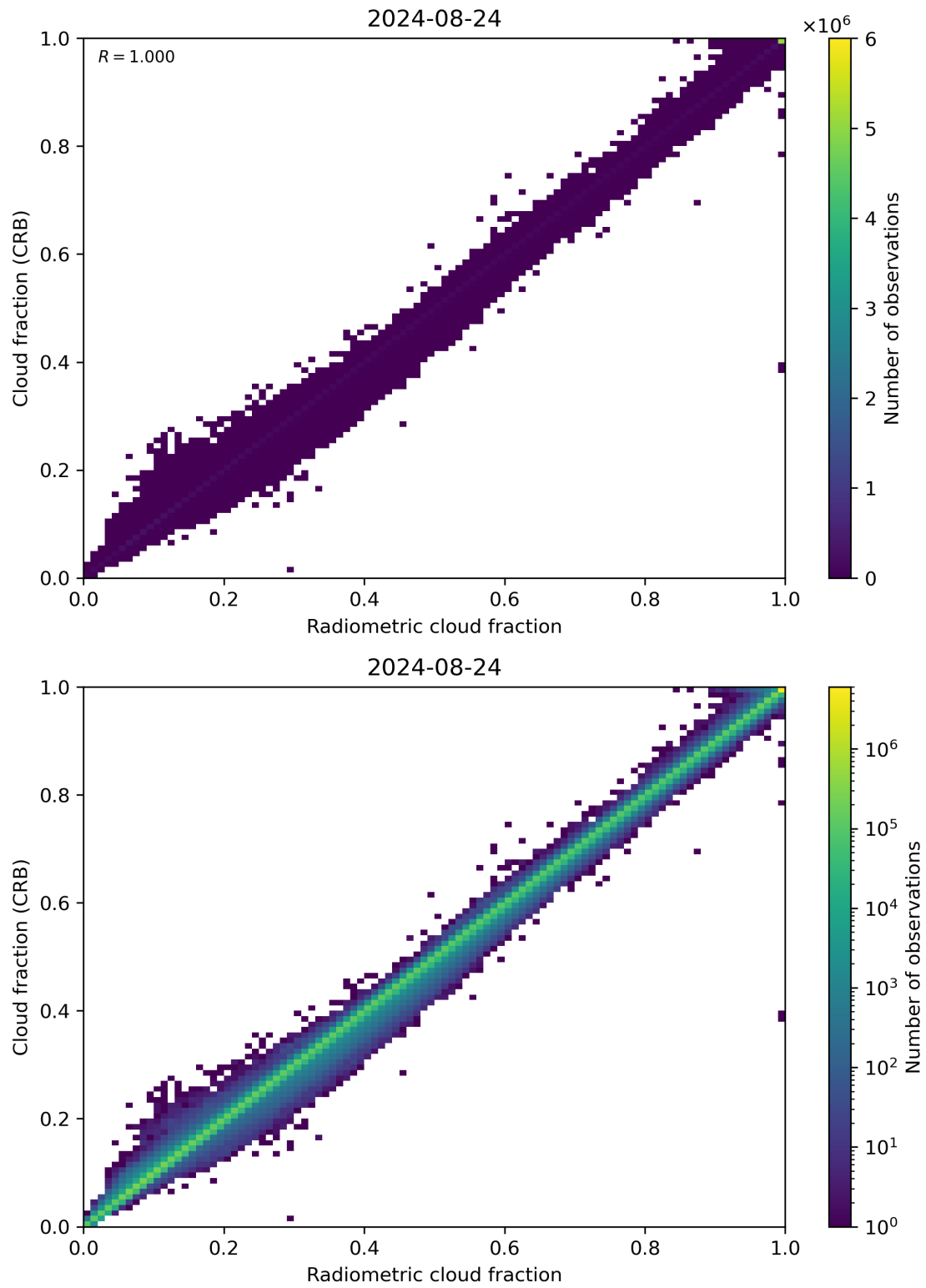
Figure 73: Scatter density plot of “Radiometric cloud fraction” against “Cloud fraction (CRB)” for 2024-08-23 to 2024-08-25.
