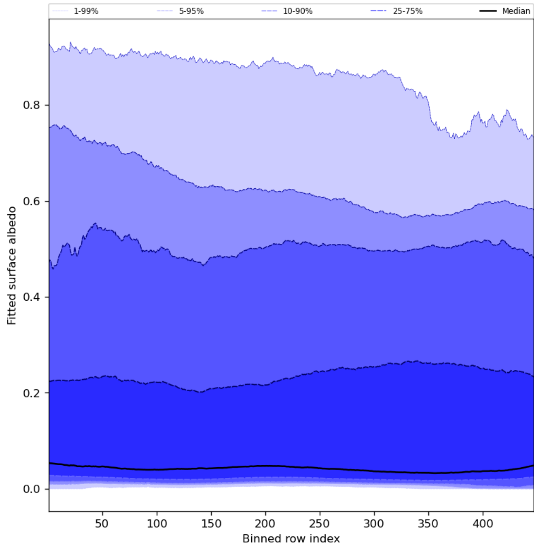
Figure 61: Along track statistics of “Fitted surface albedo” for 2024-08-23 to 2024-08-25
