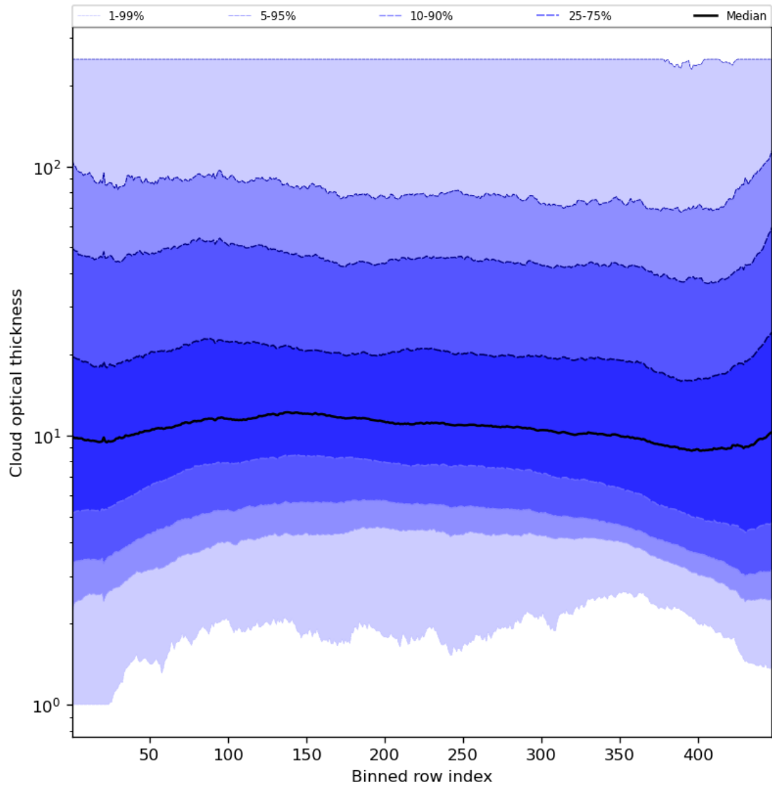
Figure 57: Along track statistics of “Cloud optical thickness” for 2024-08-23 to 2024-08-25
