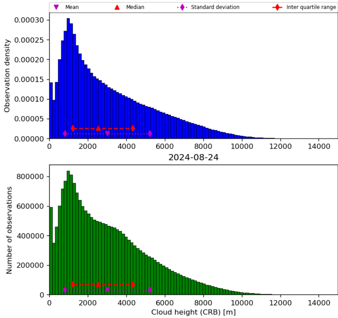
Figure 43: Histogram of “Cloud height (CRB)” for 2024-08-23 to 2024-08-25
