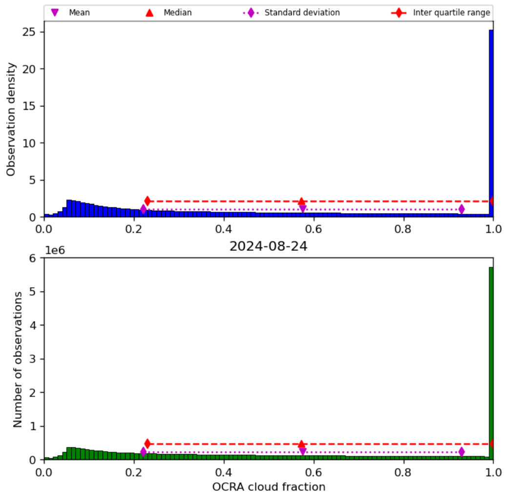
Figure 50: Histogram of “OCRA cloud fraction” for 2024-08-23 to 2024-08-25
