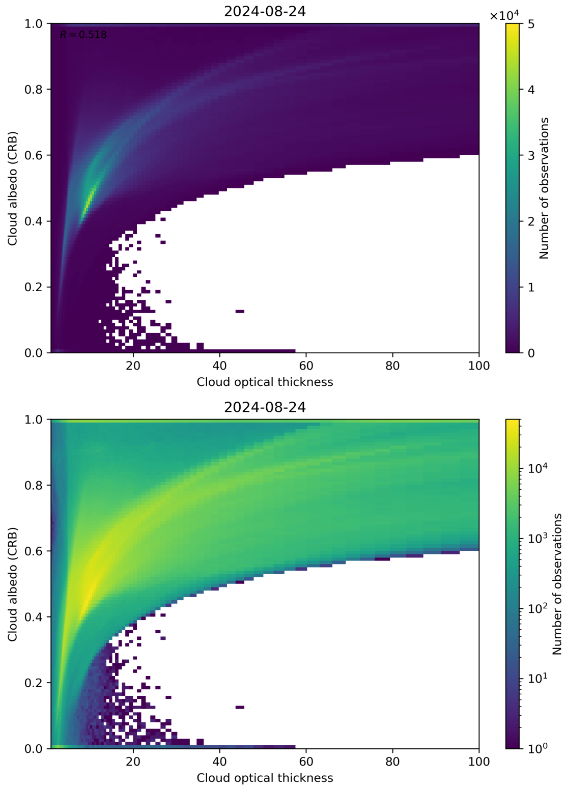
Figure 82: Scatter density plot of “Cloud optical thickness” against “Cloud albedo (CRB)” for 2024-08-23 to 2024-08-25.
