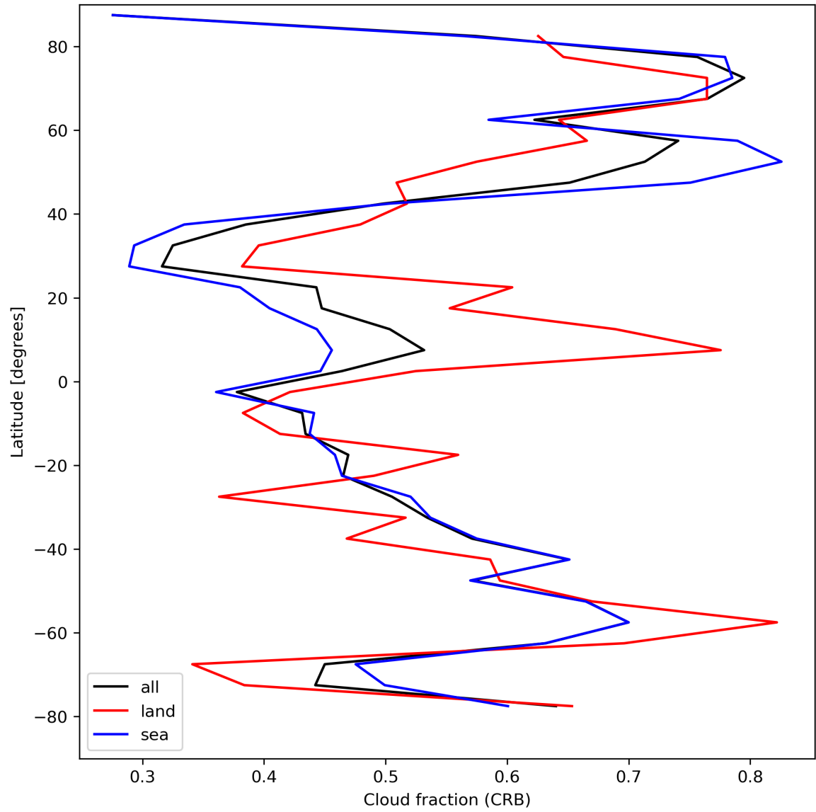
Figure 26: Zonal average of “Cloud fraction (CRB)” for 2024-08-23 to 2024-08-25.
