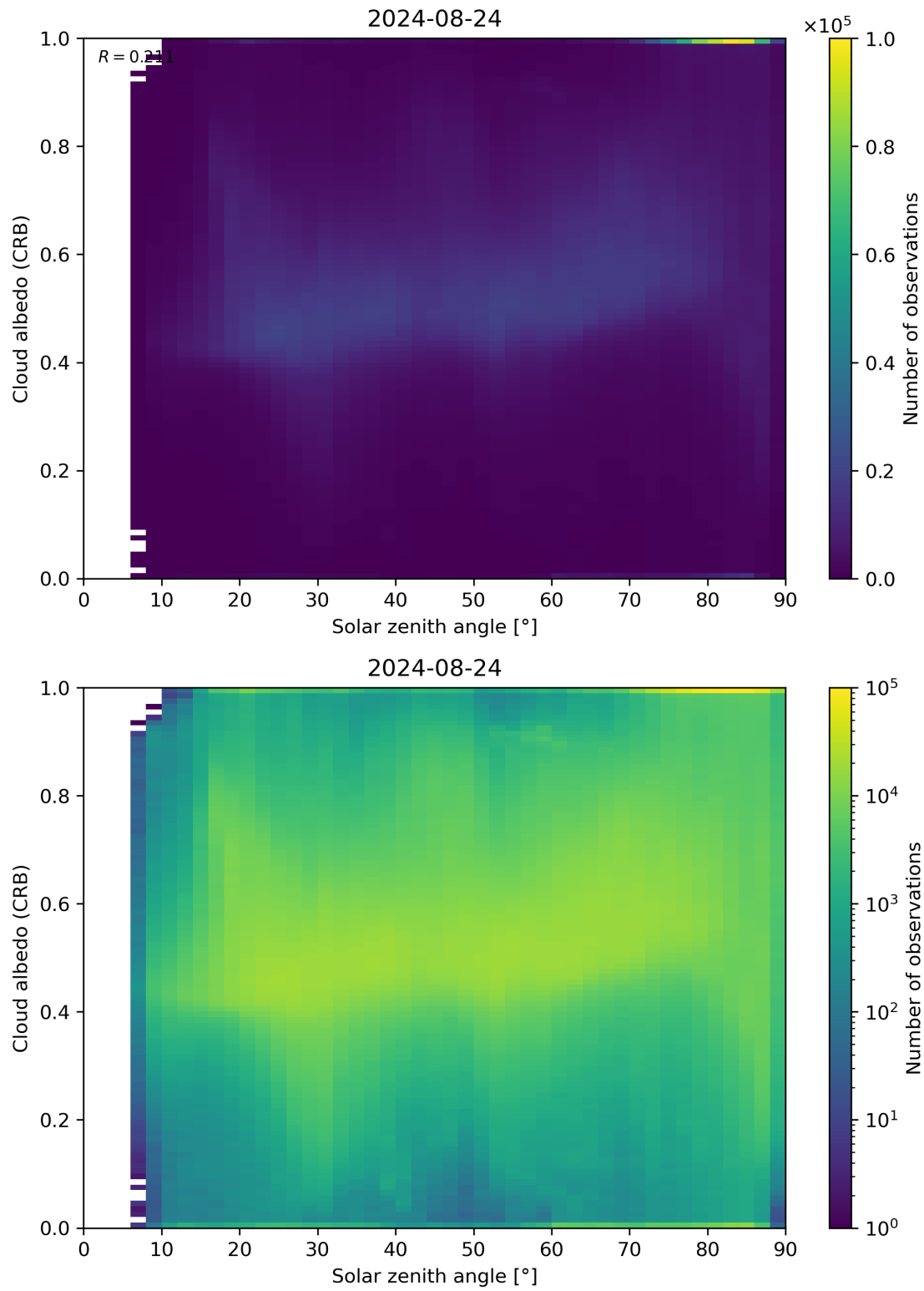
Figure 98: Scatter density plot of “Solar zenith angle” against “Cloud albedo (CRB)” for 2024-08-23 to 2024-08-25.
