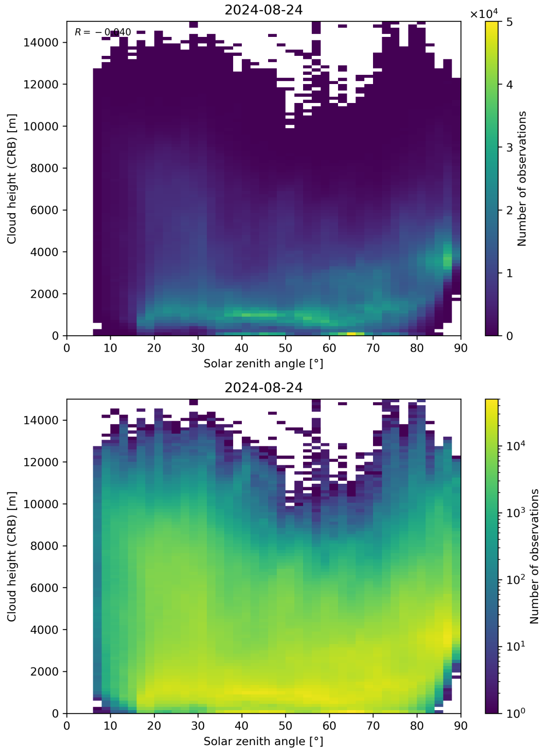
Figure 102: Scatter density plot of “Solar zenith angle” against “Cloud height (CRB)” for 2024-08-23 to 2024-08-25.
