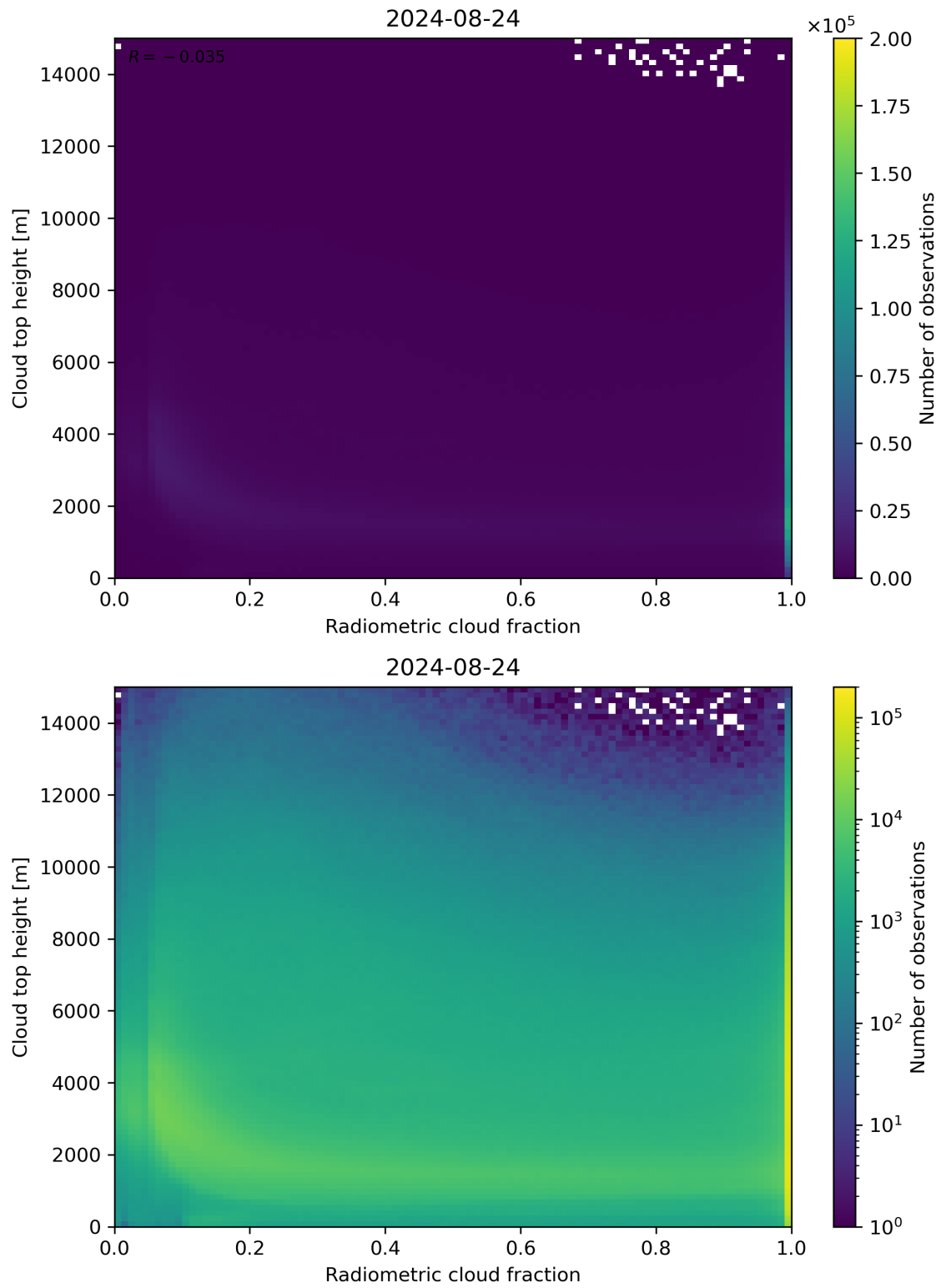
Figure 76: Scatter density plot of “Radiometric cloud fraction” against “Cloud top height” for 2024-08-23 to 2024-08-25.
