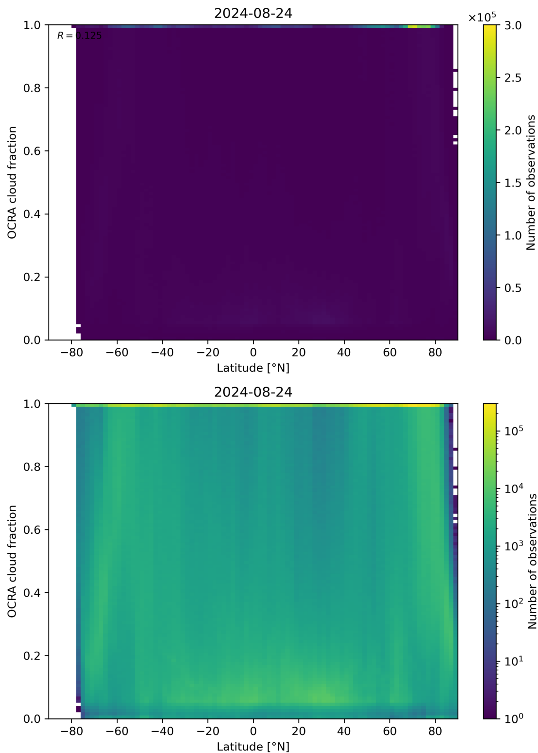
Figure 93: Scatter density plot of “Latitude” against “OCRA cloud fraction” for 2024-08-23 to 2024-08-25.
