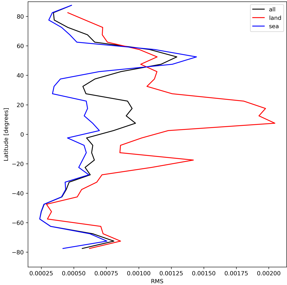
Figure 31: Zonal average of “RMS” for 2024-08-23 to 2024-08-25.
