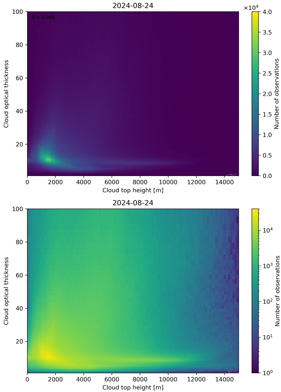
Figure 90: Scatter density plot of “Cloud top height” against “Cloud optical thickness” for 2024-08-23 to 2024-08-25.
