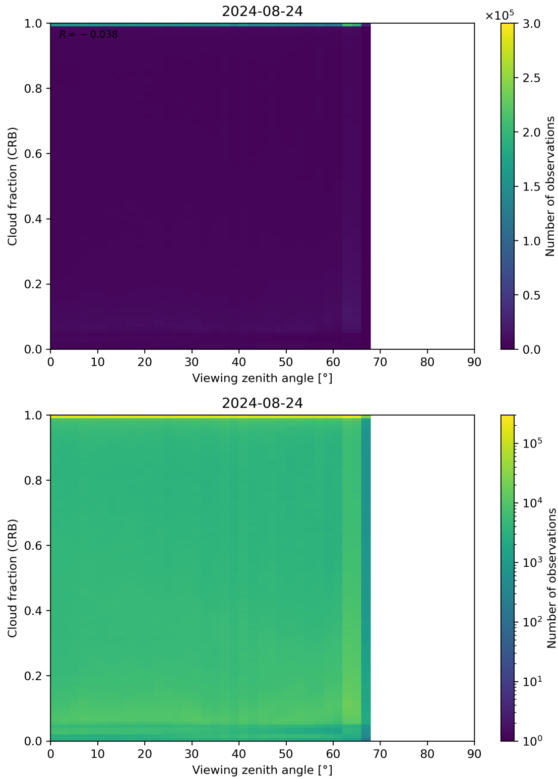
Figure 109: Scatter density plot of “Viewing zenith angle” against “Cloud fraction (CRB)” for 2024-08-23 to 2024-08-25.
