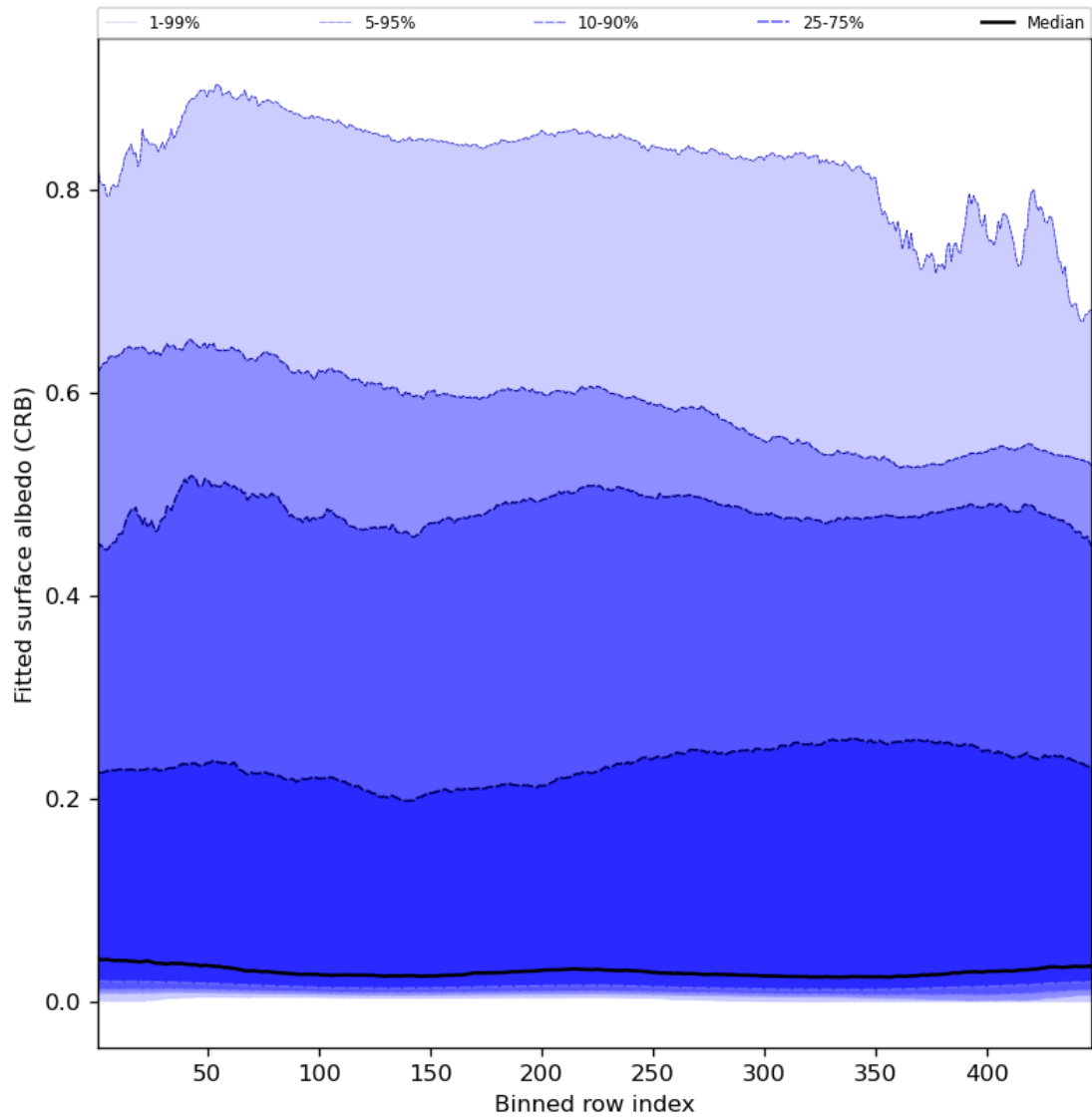
Figure 62: Along track statistics of “Fitted surface albedo (CRB)” for 2024-08-23 to 2024-08-25
