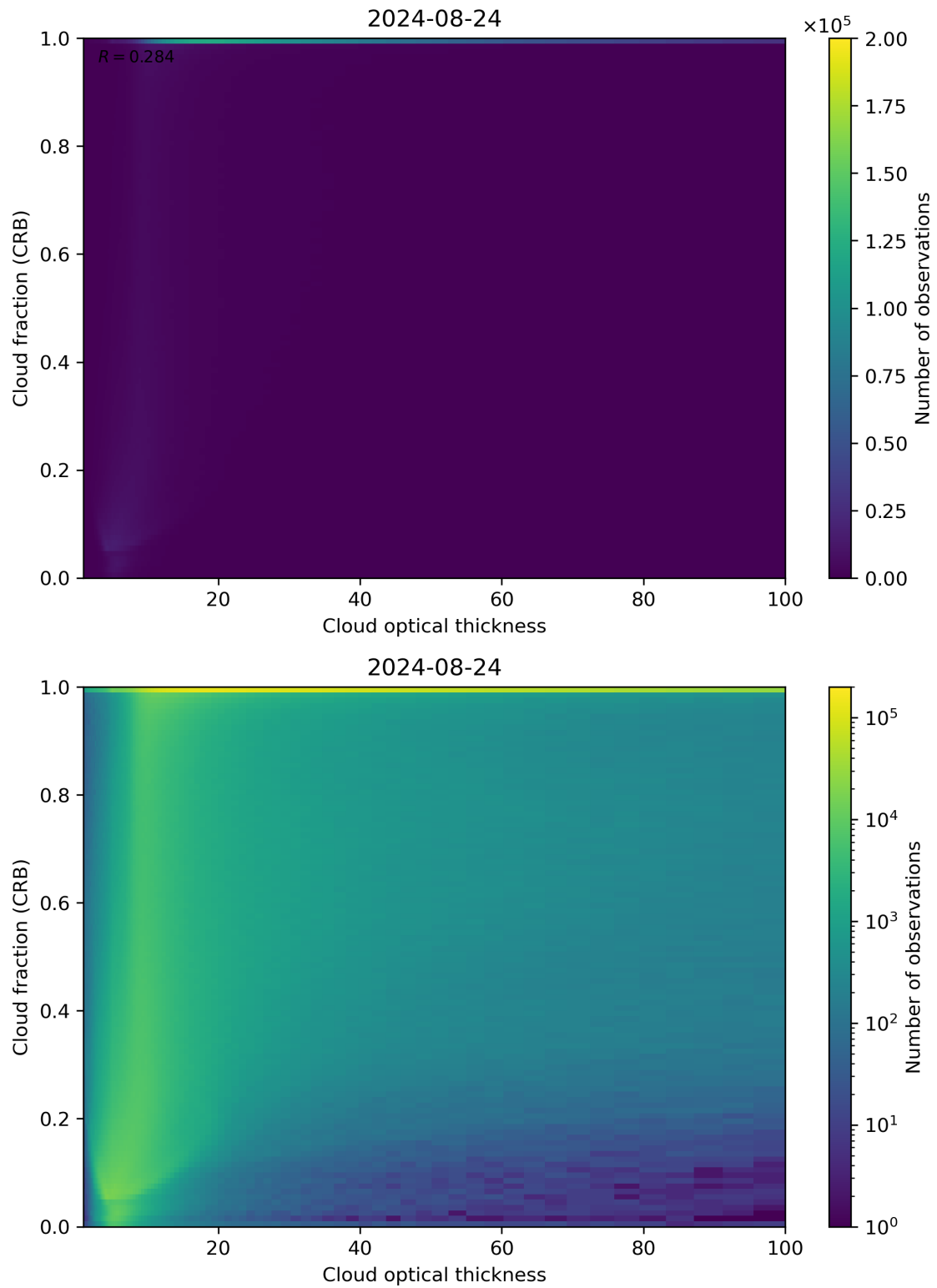
Figure 84: Scatter density plot of “Cloud optical thickness” against “Cloud fraction (CRB)” for 2024-08-23 to 2024-08-25.
