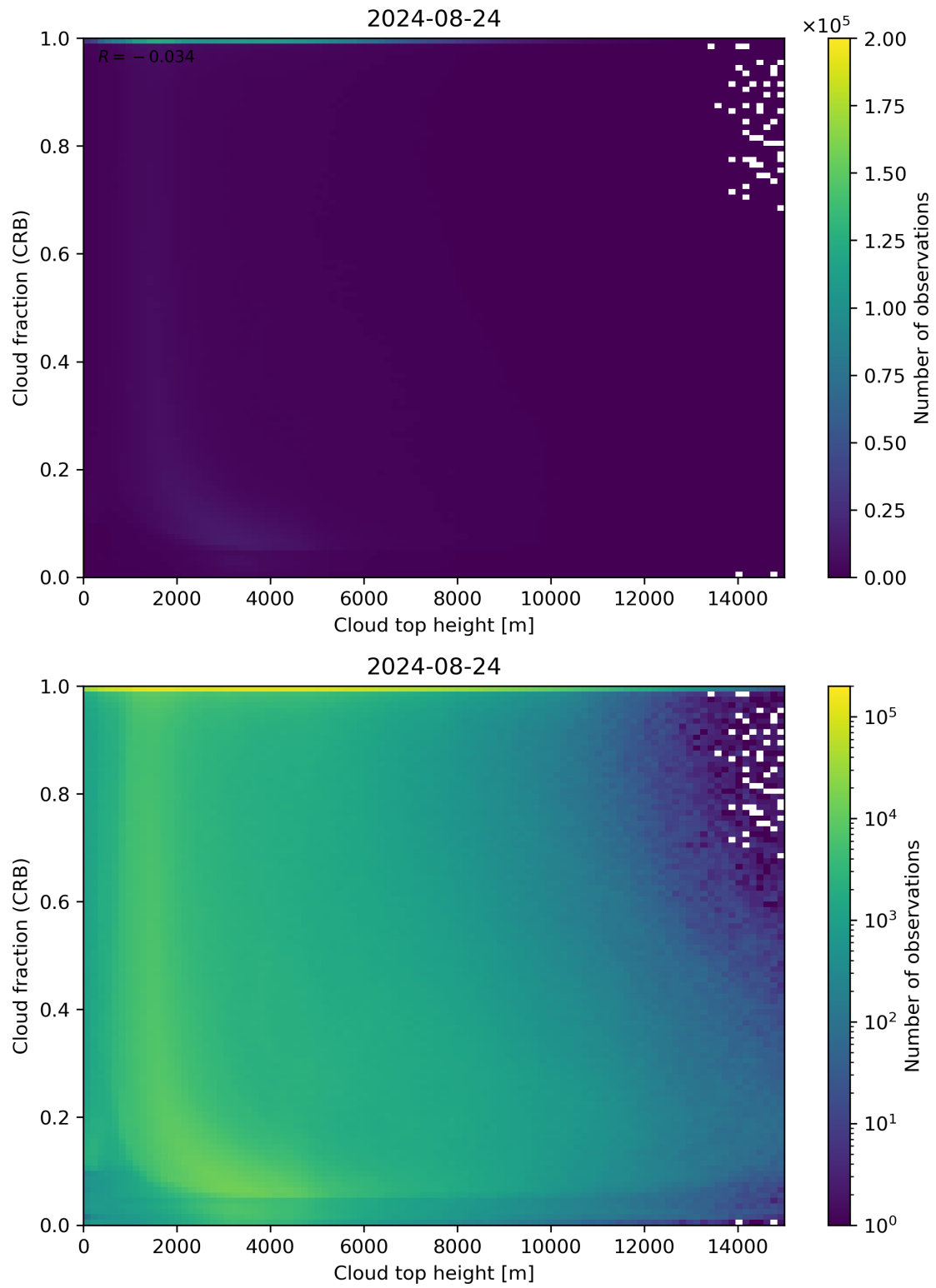
Figure 88: Scatter density plot of “Cloud top height” against “Cloud fraction (CRB)” for 2024-08-23 to 2024-08-25.
