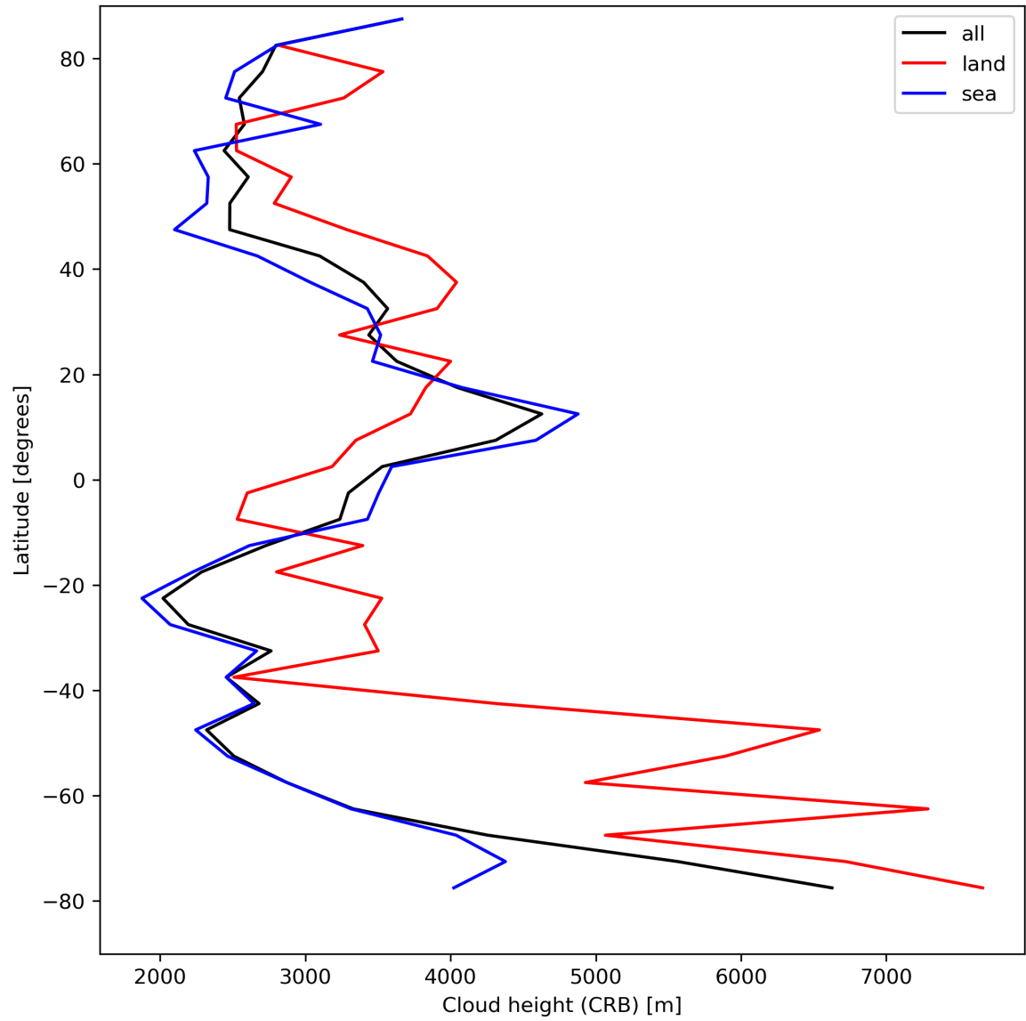
Figure 27: Zonal average of “Cloud height (CRB)” for 2024-08-23 to 2024-08-25.
