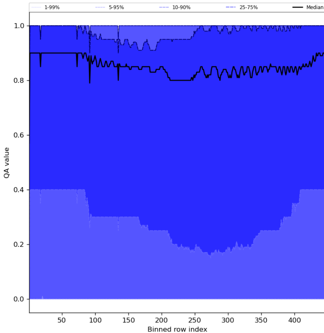
Figure 54: Along track statistics of “QA value” for 2024-08-23 to 2024-08-25
