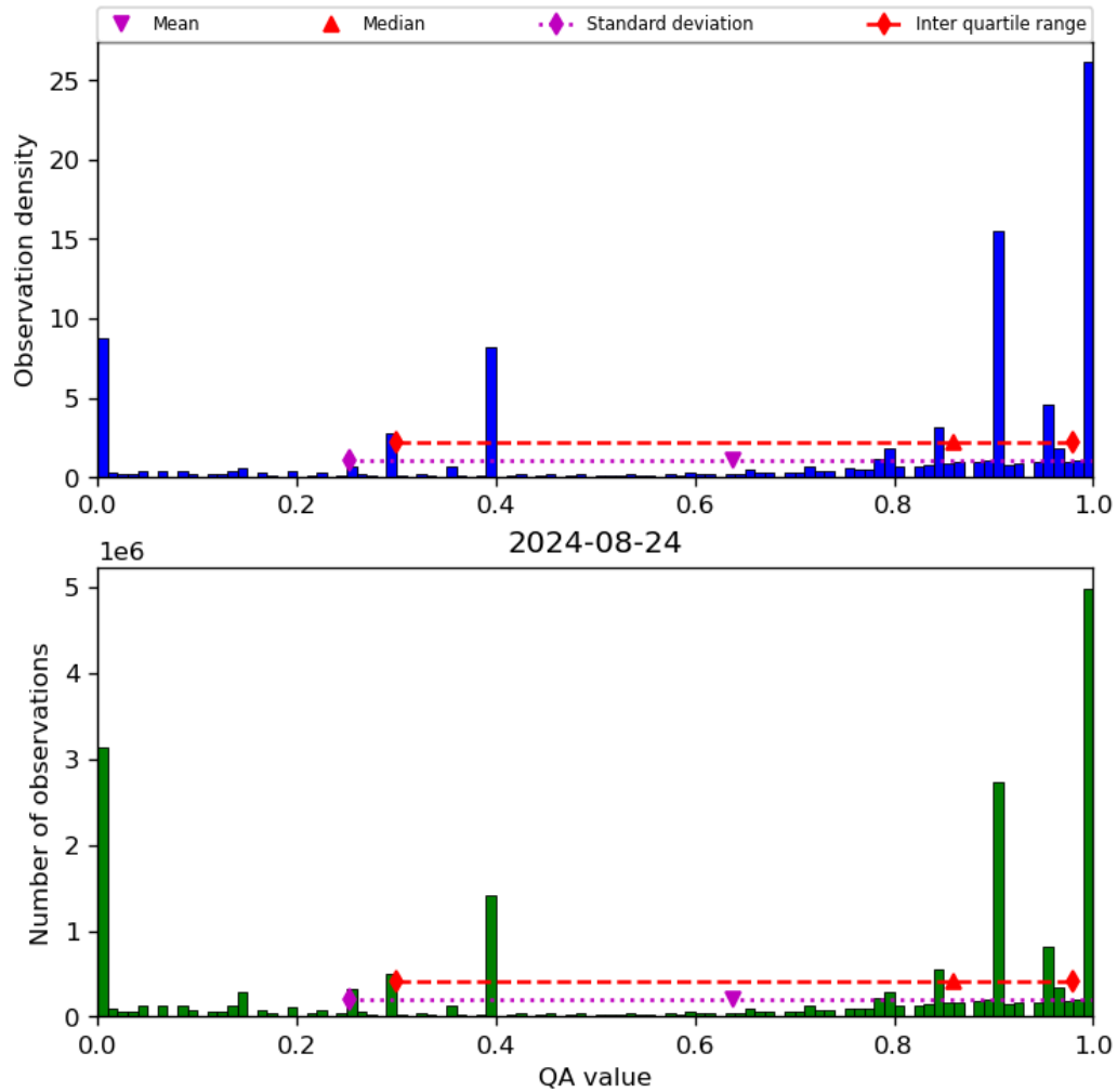
Figure 38: Histogram of “QA value” for 2024-08-23 to 2024-08-25
