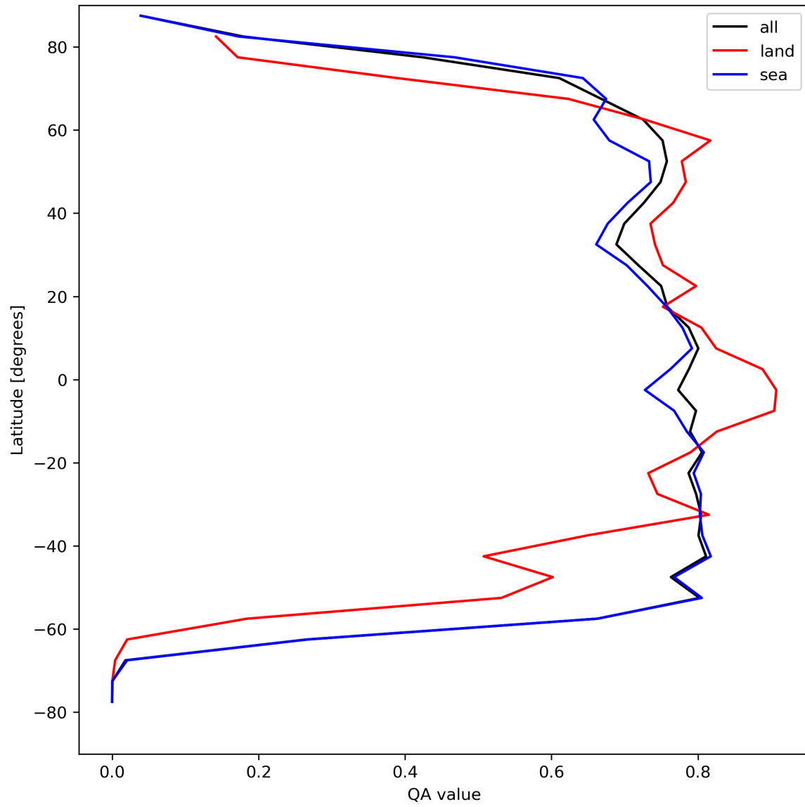
Figure 22: Zonal average of “QA value” for 2024-08-23 to 2024-08-25.
