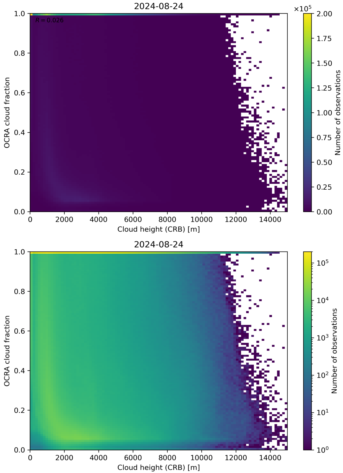
Figure 81: Scatter density plot of “Cloud height (CRB)” against “OCRA cloud fraction” for 2024-08-23 to 2024-08-25.
