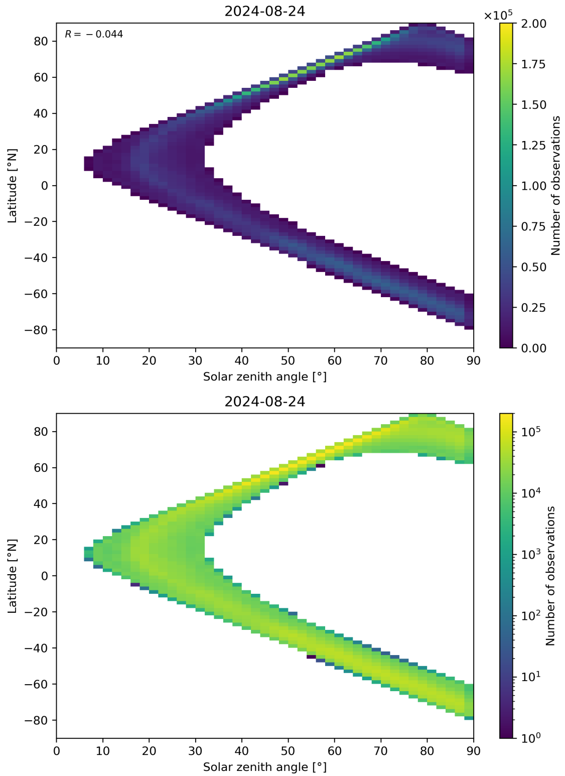
Figure 105: Scatter density plot of “Solar zenith angle” against “Latitude” for 2024-08-23 to 2024-08-25.
