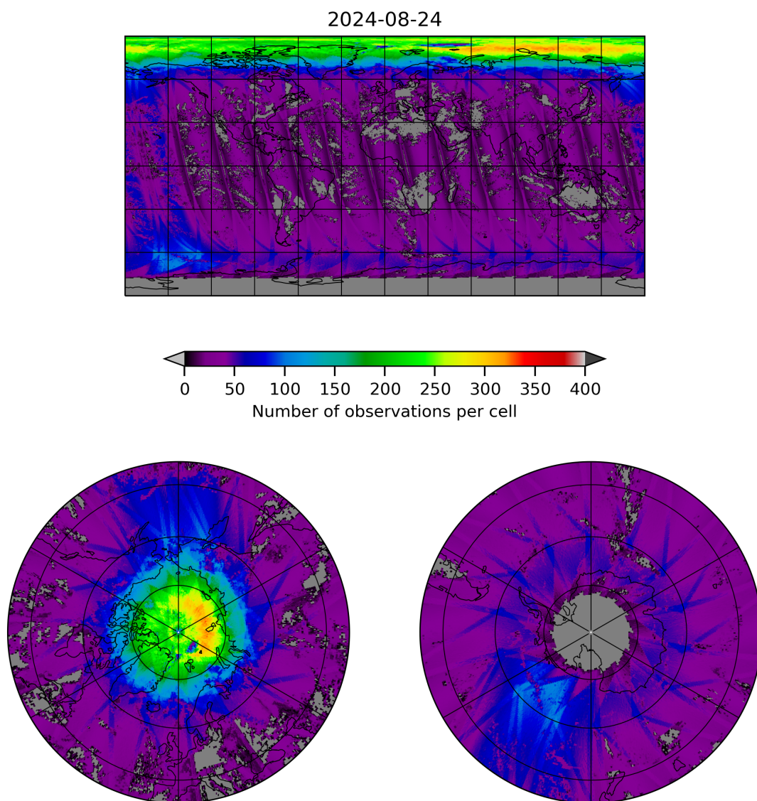
Figure 21: Map of the number of observations for 2024-08-23 to 2024-08-25
