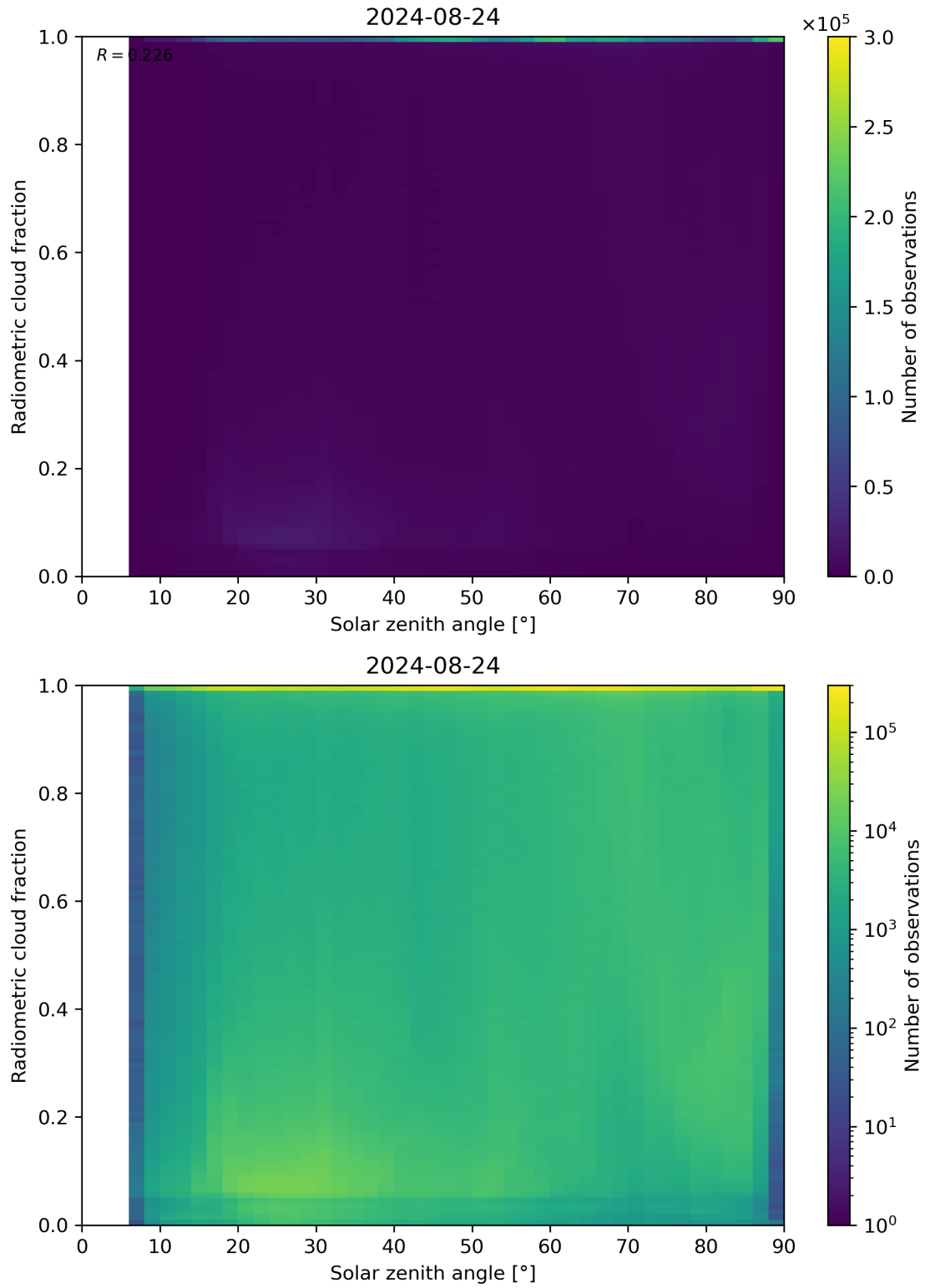
Figure 99: Scatter density plot of “Solar zenith angle” against “Radiometric cloud fraction” for 2024-08-23 to 2024-08-25.
