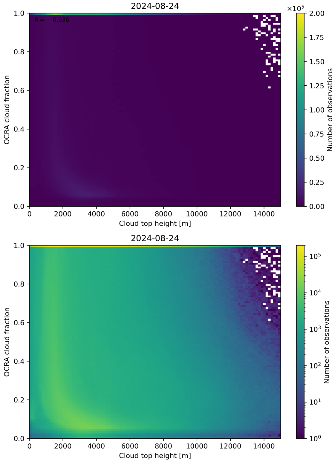
Figure 87: Scatter density plot of “Cloud top height” against “OCRA cloud fraction” for 2024-08-23 to 2024-08-25.
