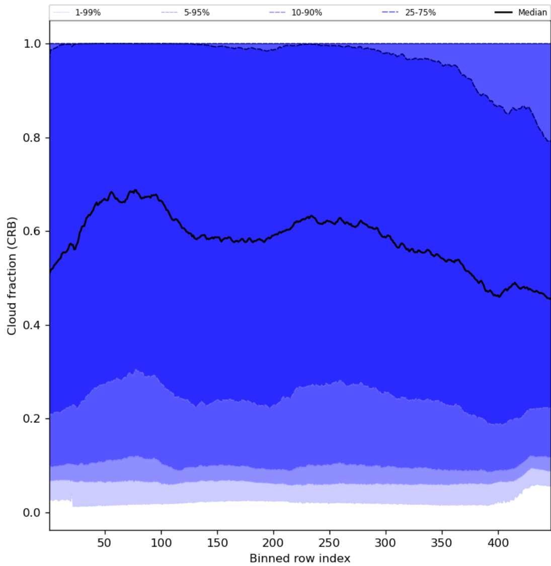
Figure 58: Along track statistics of “Cloud fraction (CRB)” for 2024-08-23 to 2024-08-25
