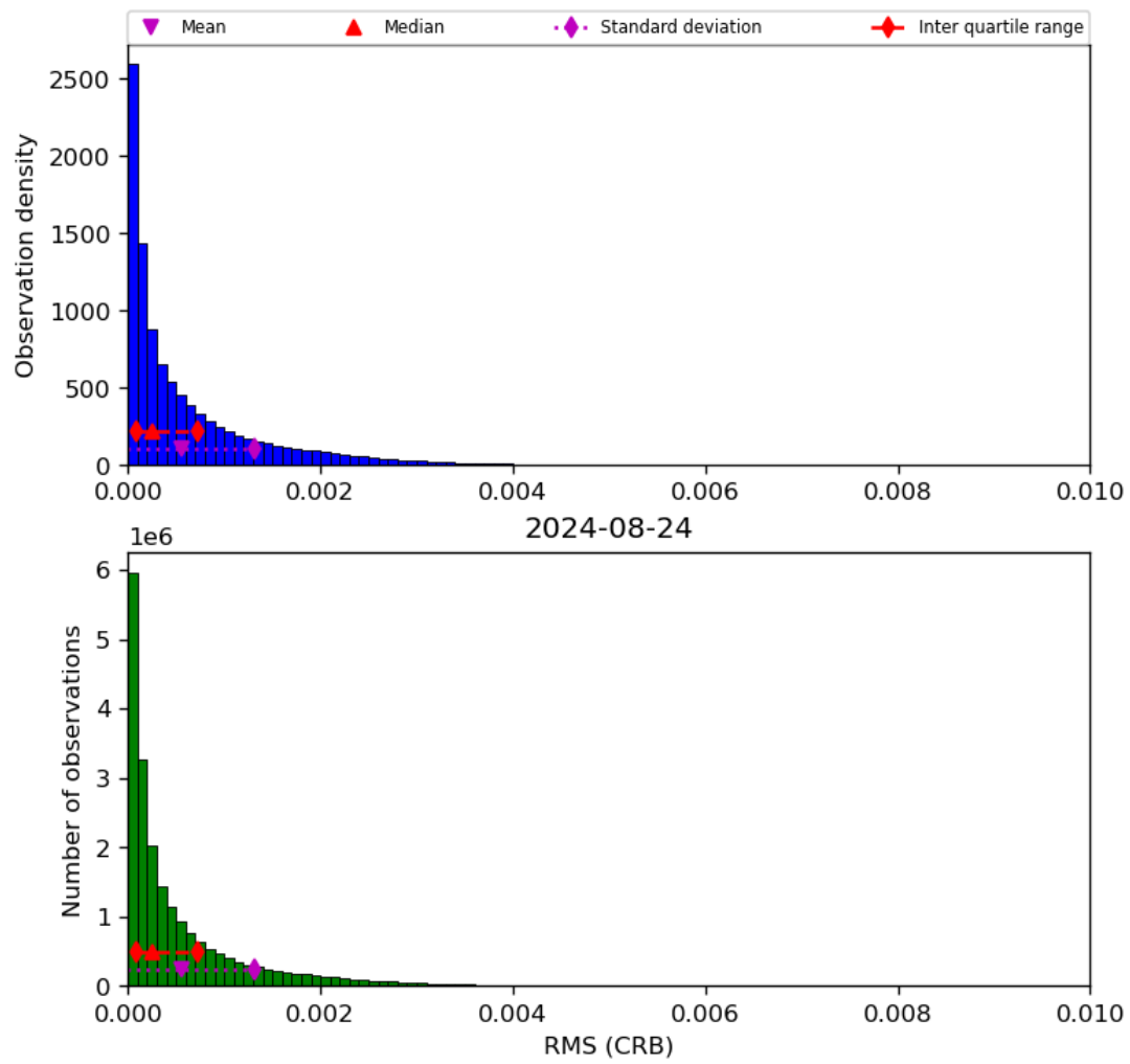
Figure 48: Histogram of “RMS (CRB)” for 2024-08-23 to 2024-08-25
