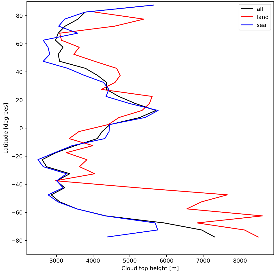
Figure 24: Zonal average of “Cloud top height” for 2024-08-23 to 2024-08-25.
