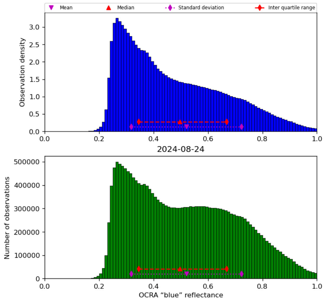
Figure 51: Histogram of “OCRA “blue” reflectance” for 2024-08-23 to 2024-08-25
