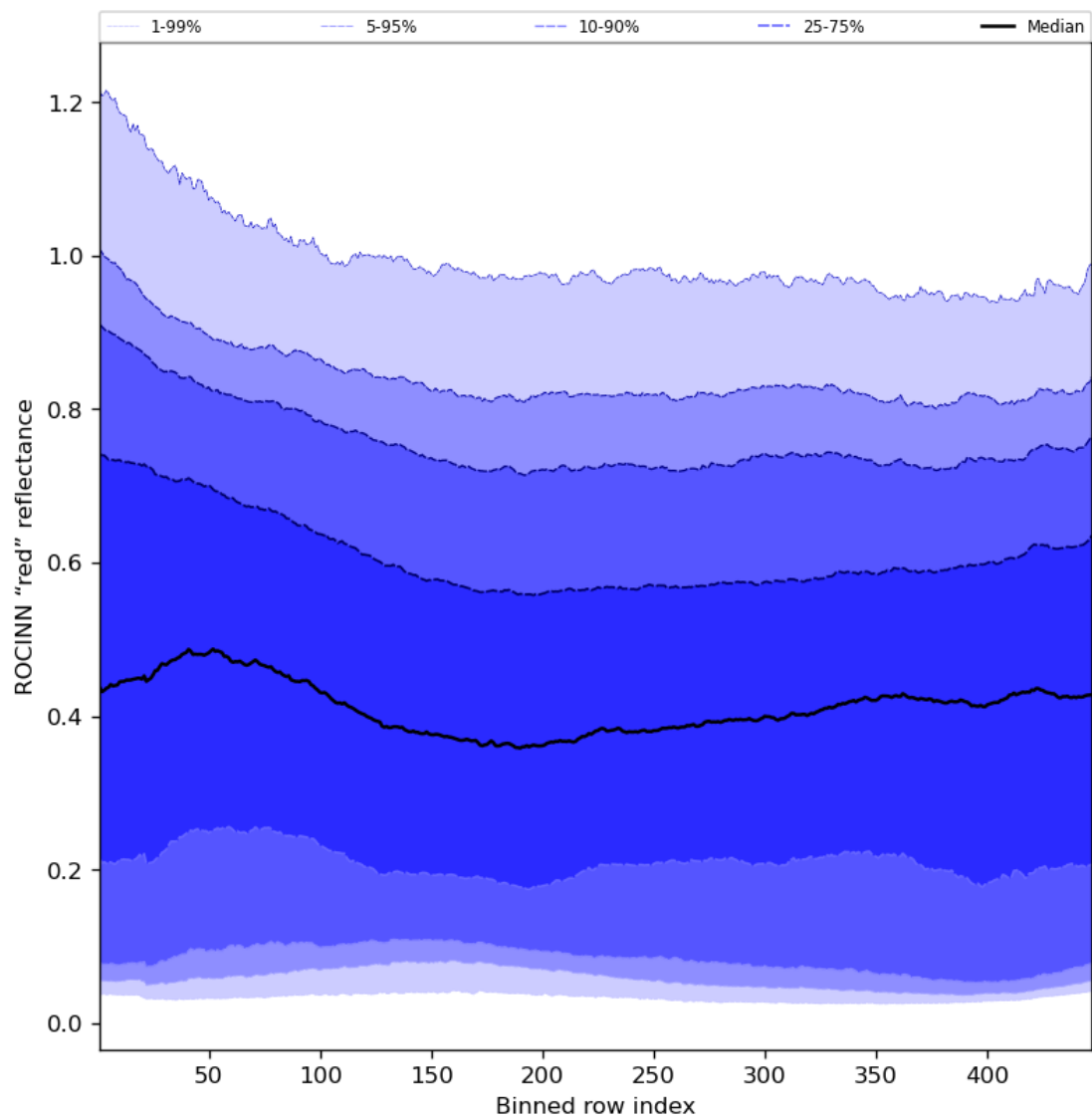
Figure 69: Along track statistics of “ROCINN “red” reflectance” for 2024-08-23 to 2024-08-25
