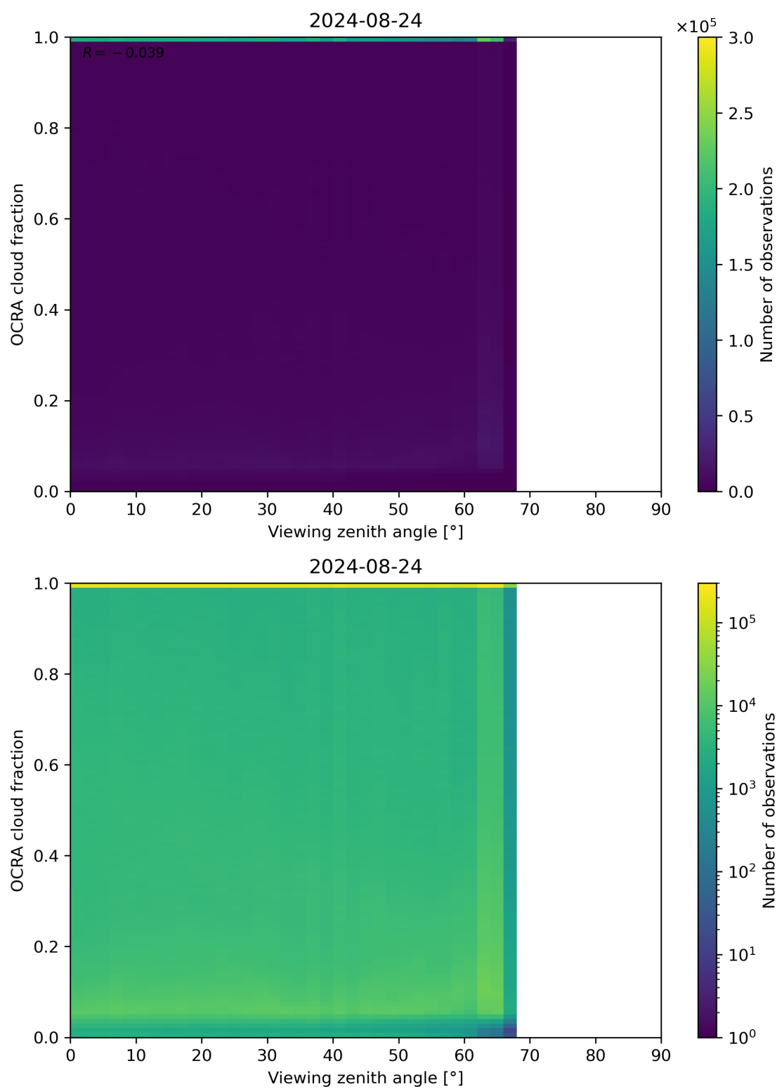
Figure 108: Scatter density plot of “Viewing zenith angle” against “OCRA cloud fraction” for 2024-08-23 to 2024-08-25.
