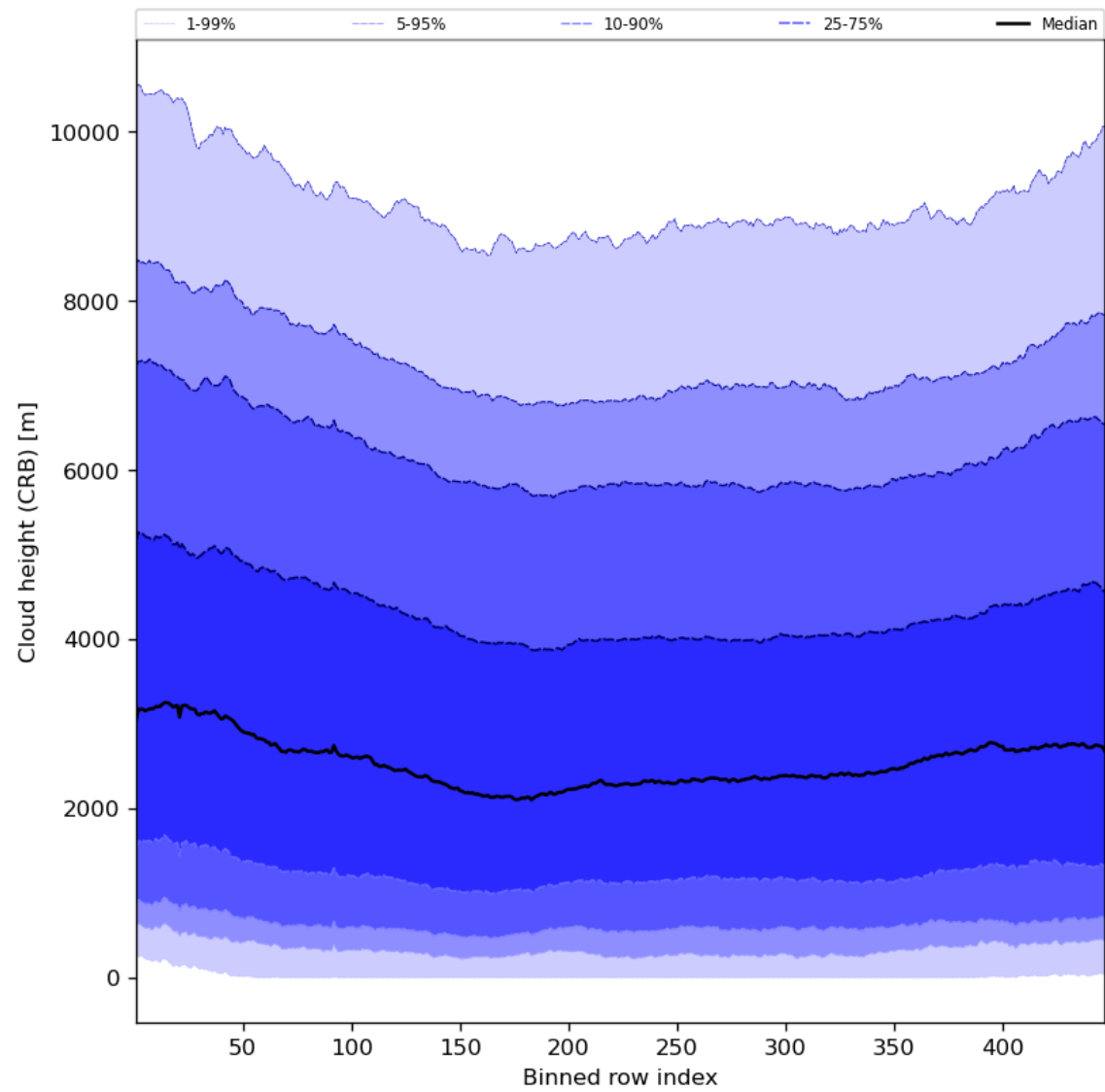
Figure 59: Along track statistics of “Cloud height (CRB)” for 2024-08-23 to 2024-08-25
