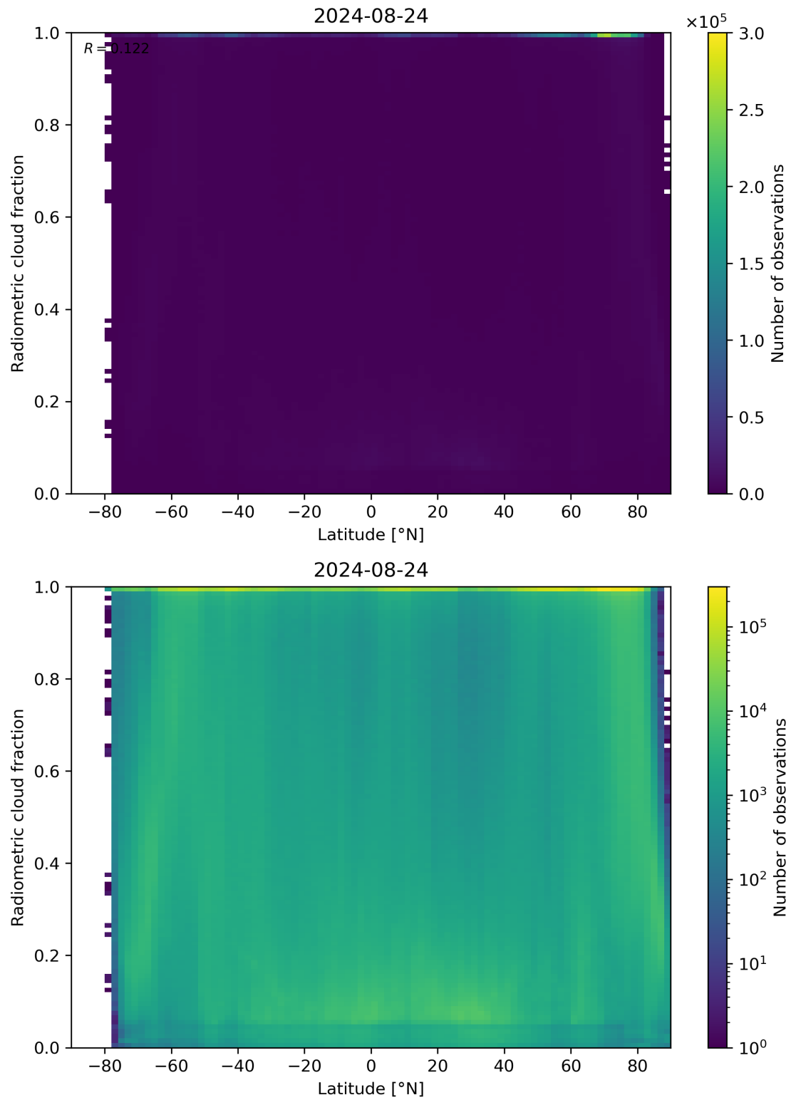
Figure 92: Scatter density plot of “Latitude” against “Radiometric cloud fraction” for 2024-08-23 to 2024-08-25.
