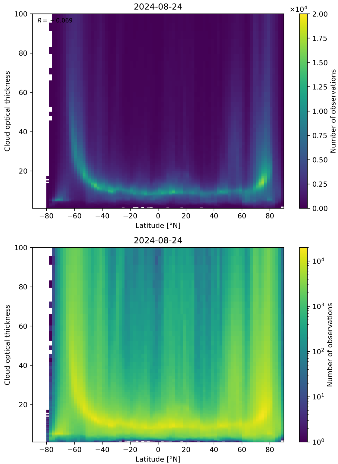
Figure 96: Scatter density plot of “Latitude” against “Cloud optical thickness” for 2024-08-23 to 2024-08-25.
