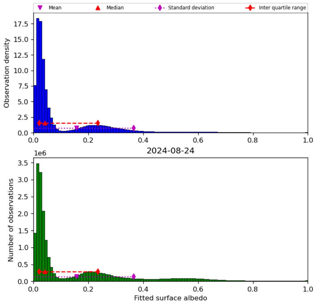
Figure 45: Histogram of “Fitted surface albedo” for 2024-08-23 to 2024-08-25
