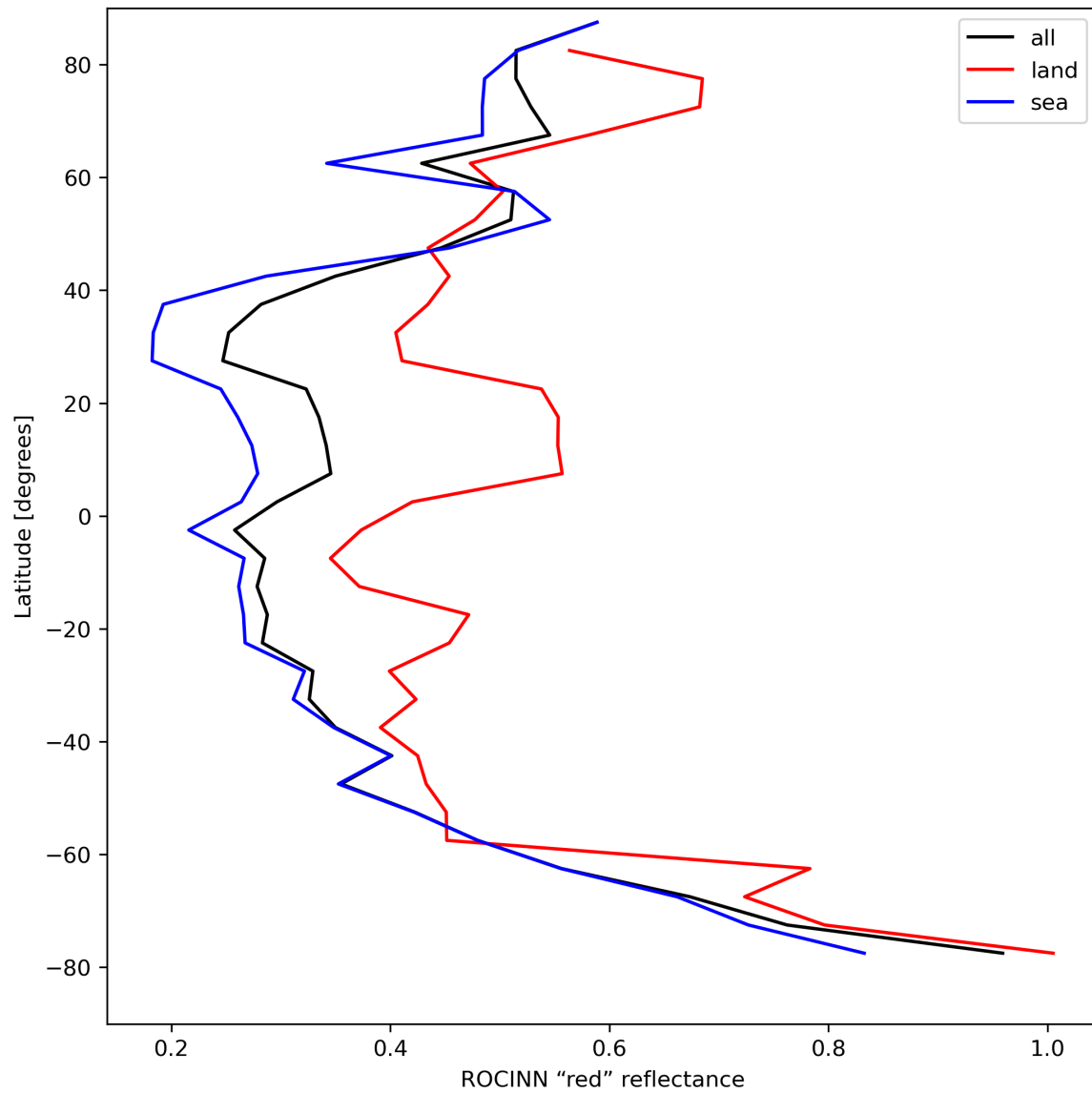
Figure 37: Zonal average of “ROCINN “red” reflectance” for 2024-08-23 to 2024-08-25.
