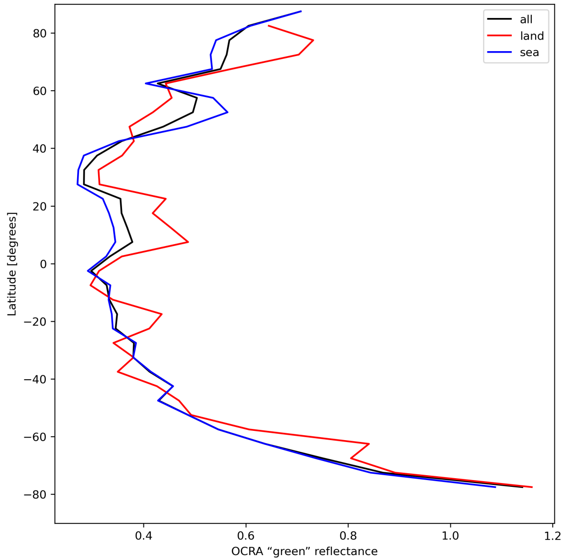
Figure 36: Zonal average of “OCRA “green” reflectance” for 2024-08-23 to 2024-08-25.
