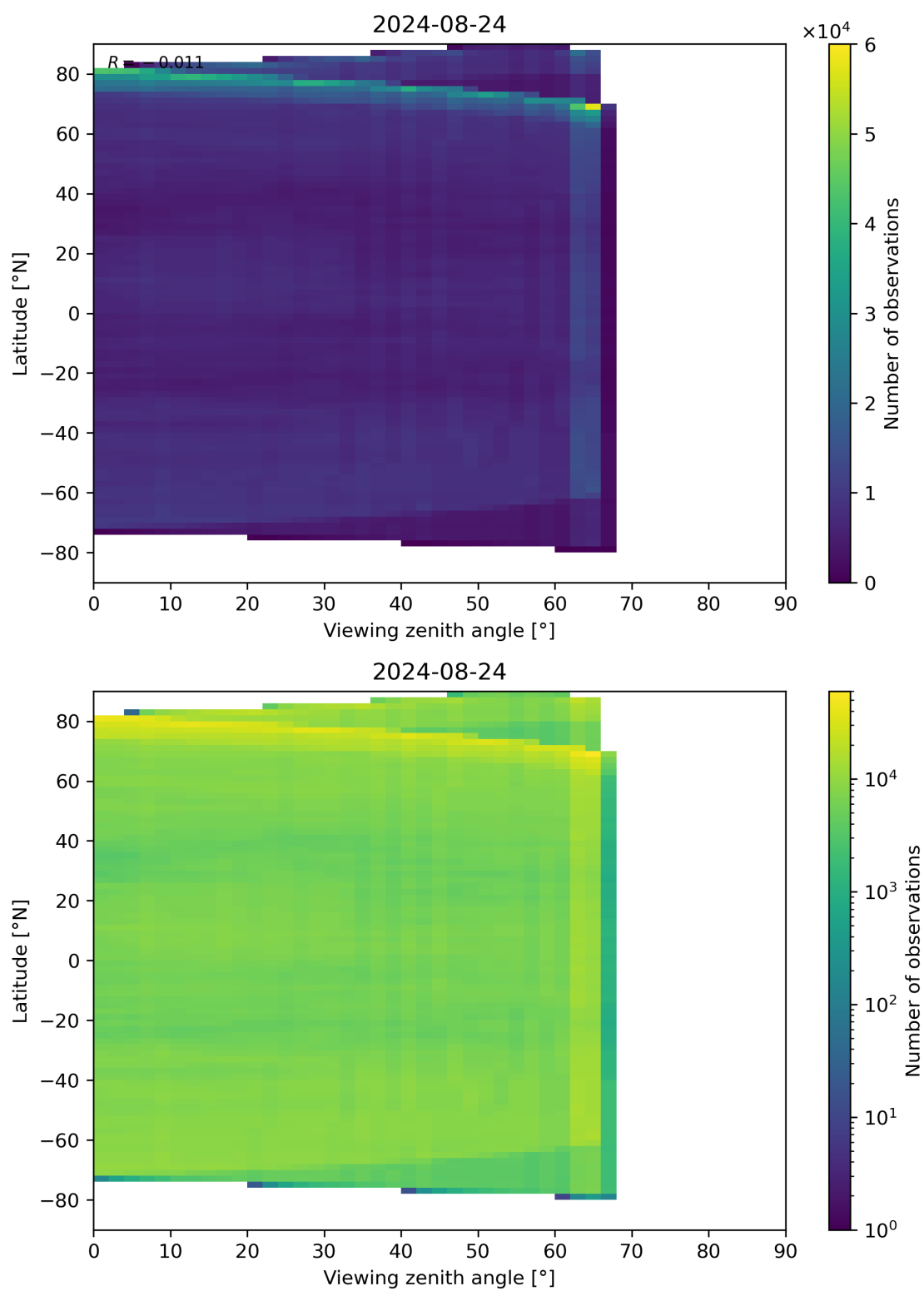
Figure 113: Scatter density plot of “Viewing zenith angle” against “Latitude” for 2024-08-23 to 2024-08-25.
