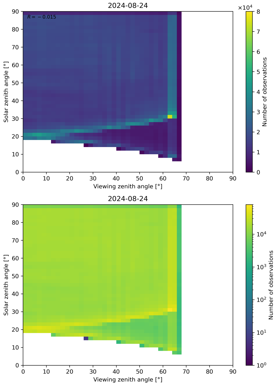
Figure 114: Scatter density plot of “Viewing zenith angle” against “Solar zenith angle” for 2024-08-23 to 2024-08-25.
