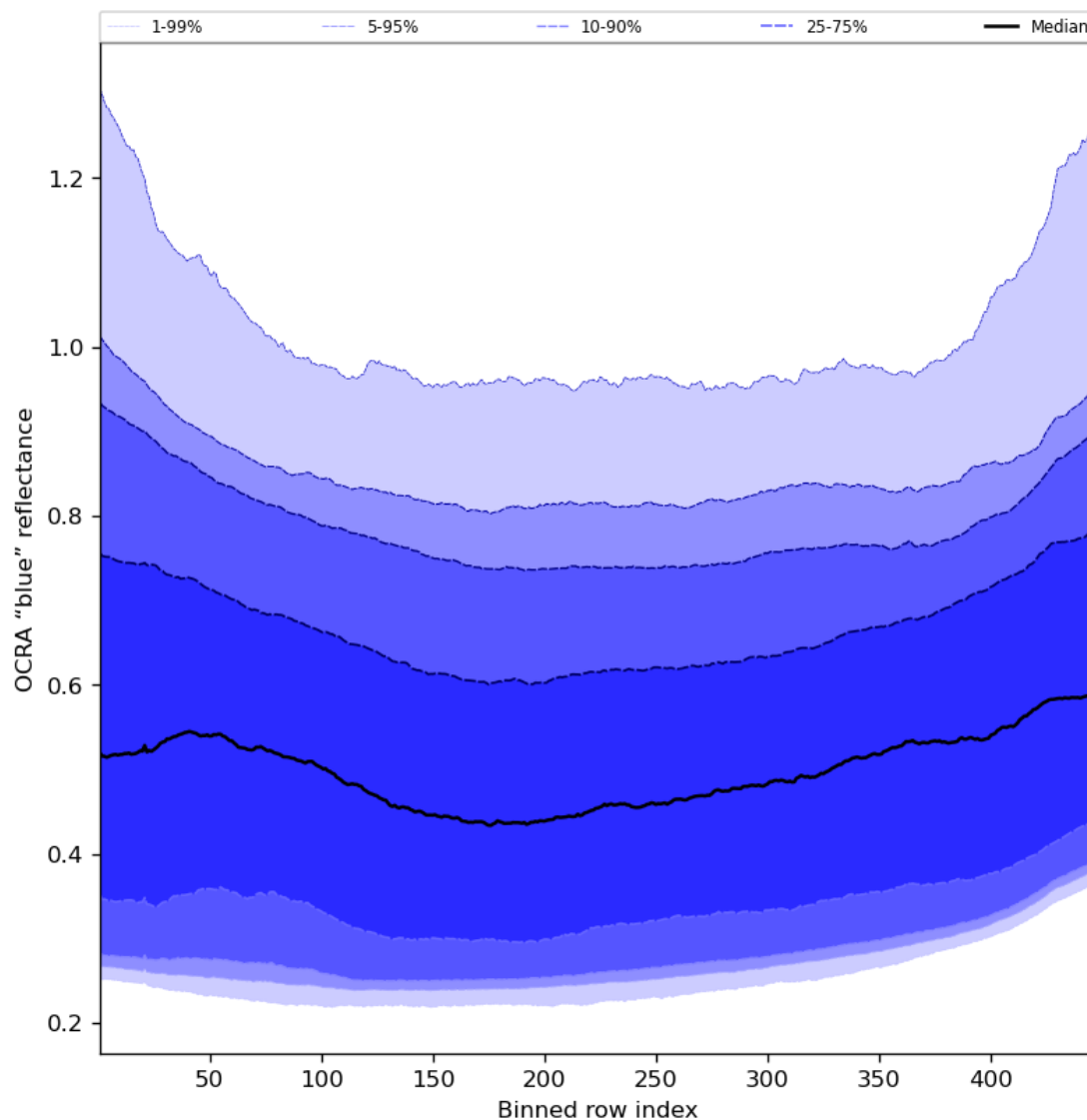
Figure 67: Along track statistics of “OCRA “blue” reflectance” for 2024-08-23 to 2024-08-25
