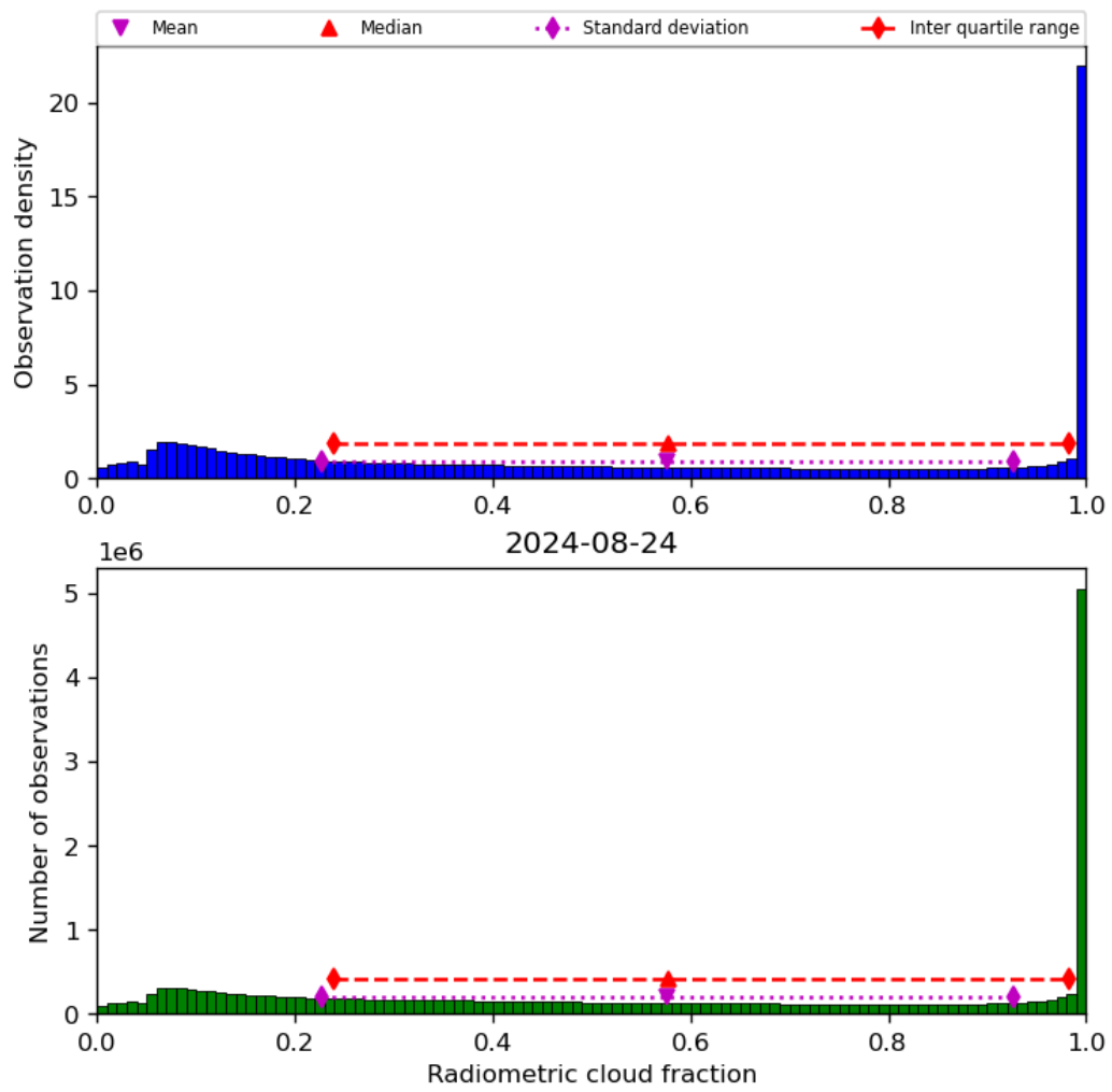
Figure 39: Histogram of “Radiometric cloud fraction” for 2024-08-23 to 2024-08-25
