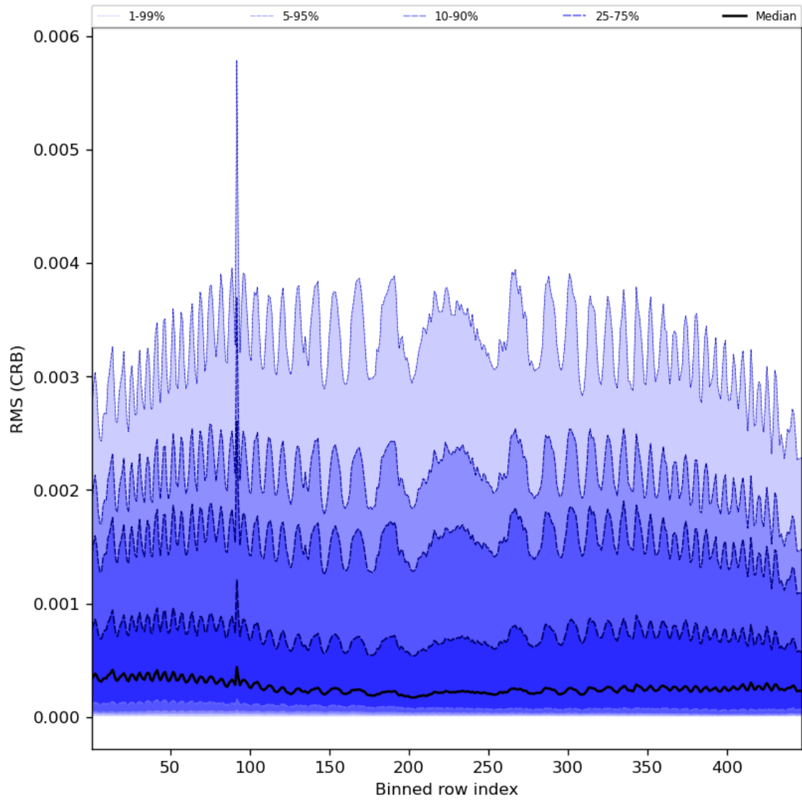
Figure 64: Along track statistics of “RMS (CRB)” for 2024-08-23 to 2024-08-25
