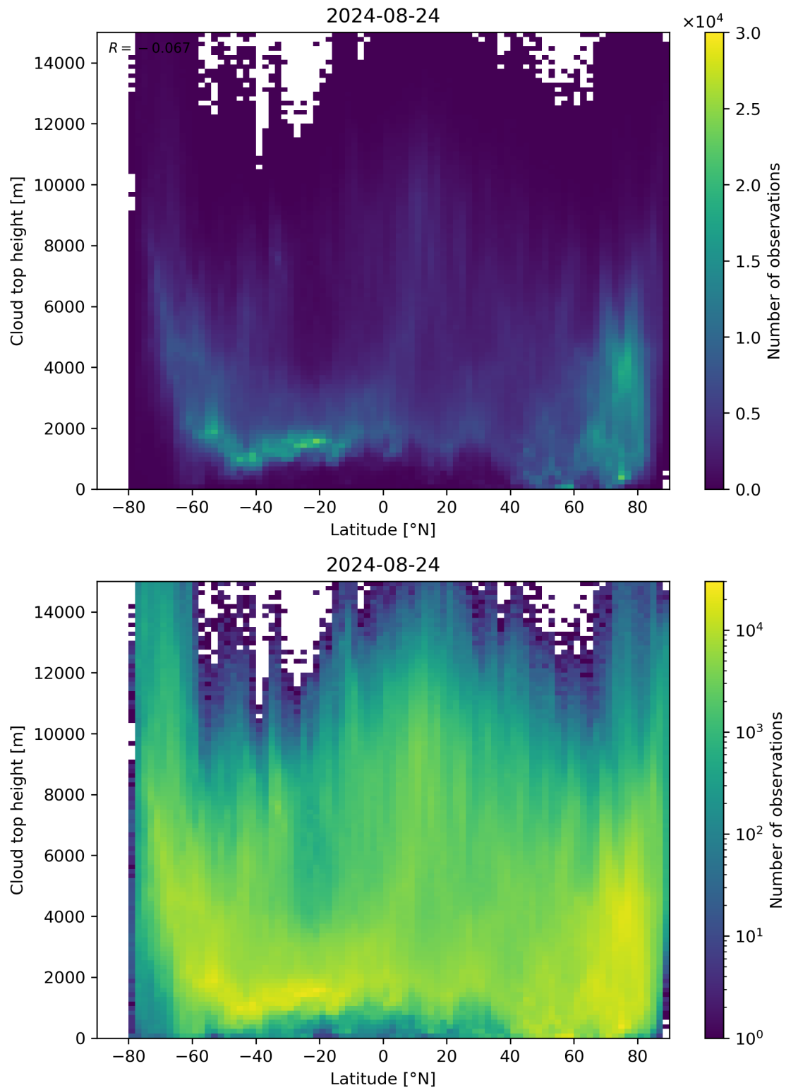
Figure 97: Scatter density plot of “Latitude” against “Cloud top height” for 2024-08-23 to 2024-08-25.
