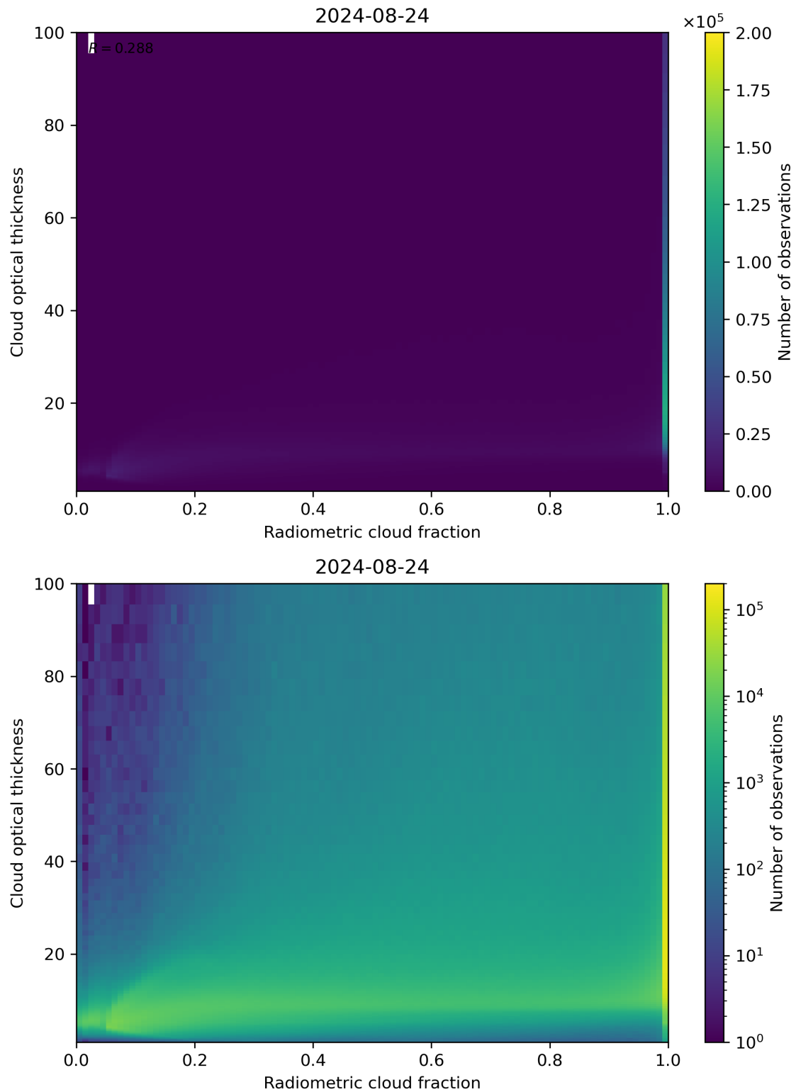
Figure 75: Scatter density plot of “Radiometric cloud fraction” against “Cloud optical thickness” for 2024-08-23 to 2024-08-25.
