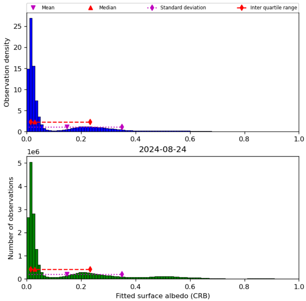
Figure 46: Histogram of “Fitted surface albedo (CRB)” for 2024-08-23 to 2024-08-25
