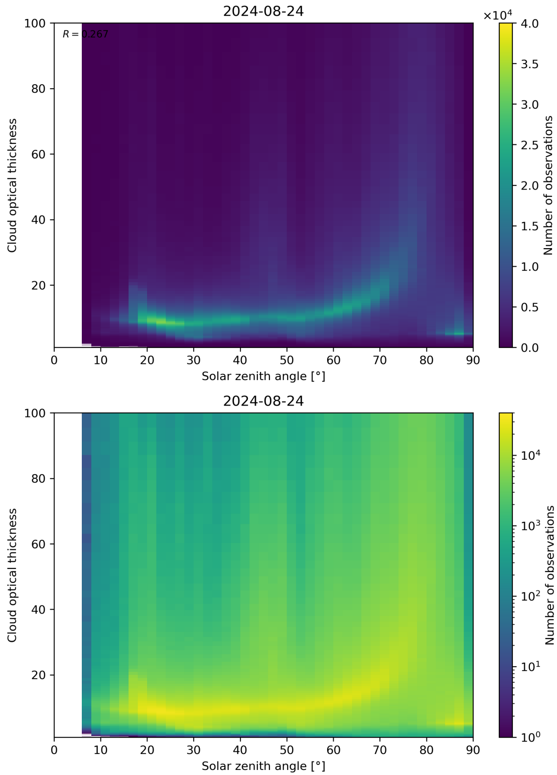
Figure 103: Scatter density plot of “Solar zenith angle” against “Cloud optical thickness” for 2024-08-23 to 2024-08-25.
