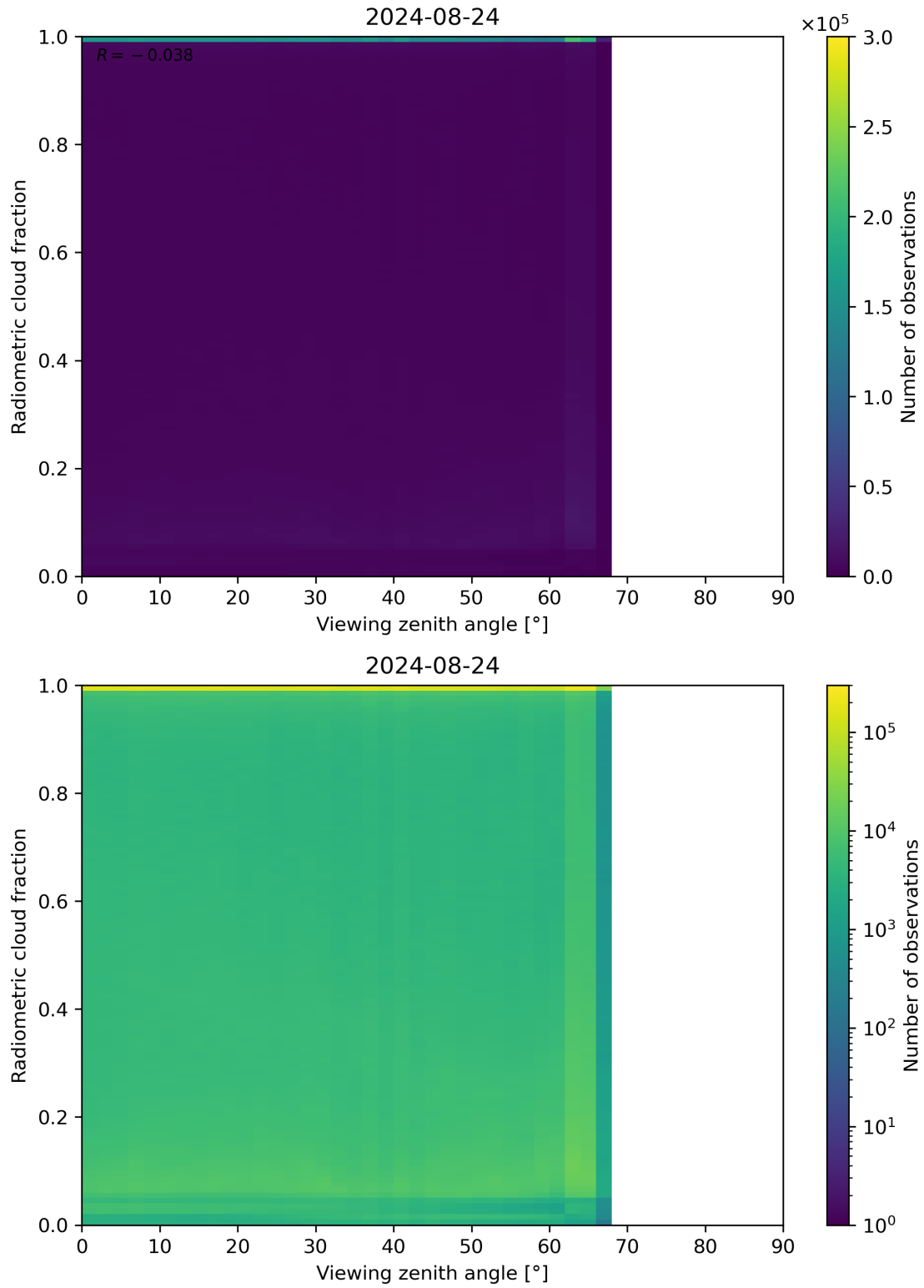
Figure 107: Scatter density plot of “Viewing zenith angle” against “Radiometric cloud fraction” for 2024-08-23 to 2024-08-25.
