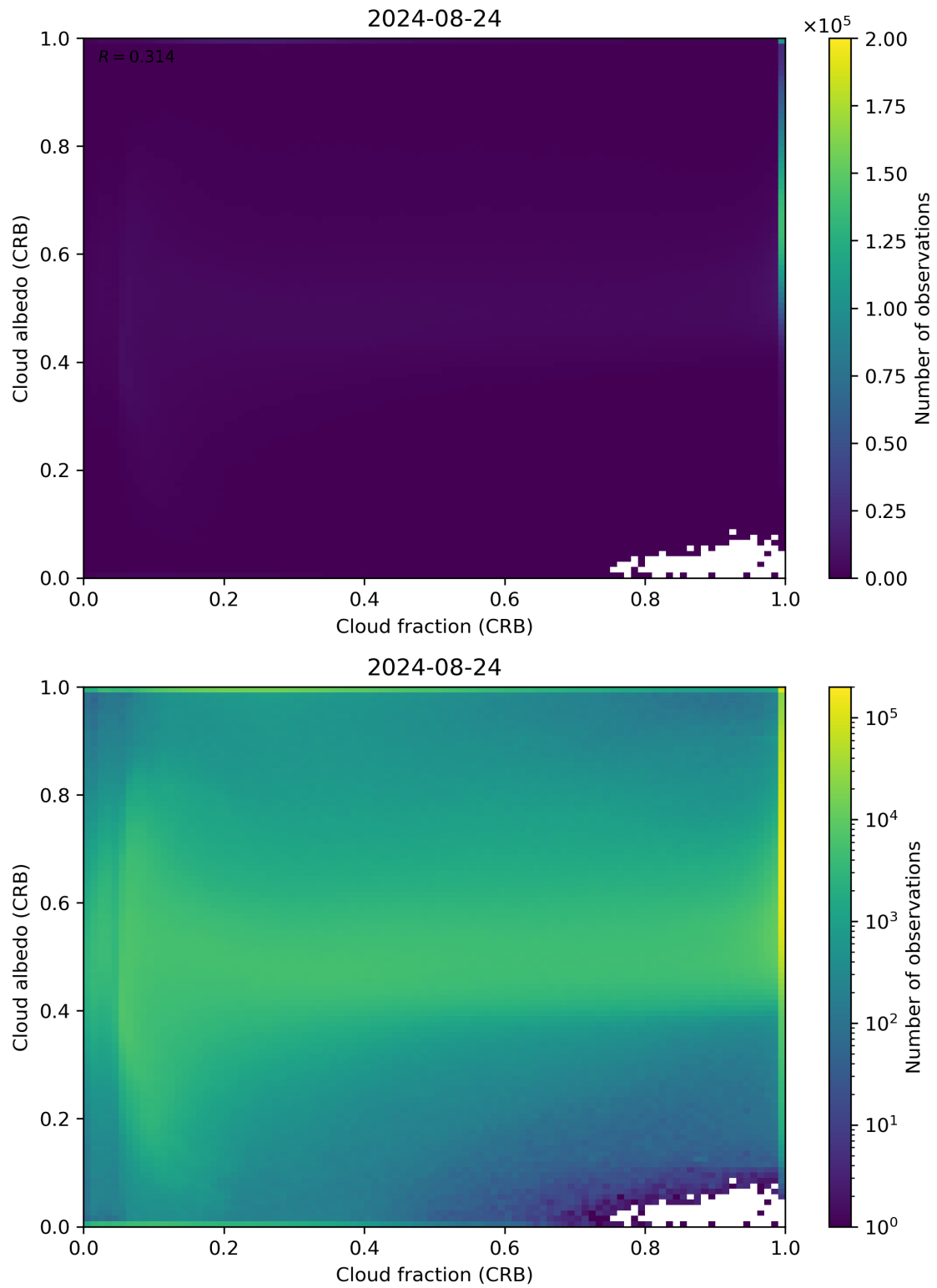
Figure 77: Scatter density plot of “Cloud fraction (CRB)” against “Cloud albedo (CRB)” for 2024-08-23 to 2024-08-25.
