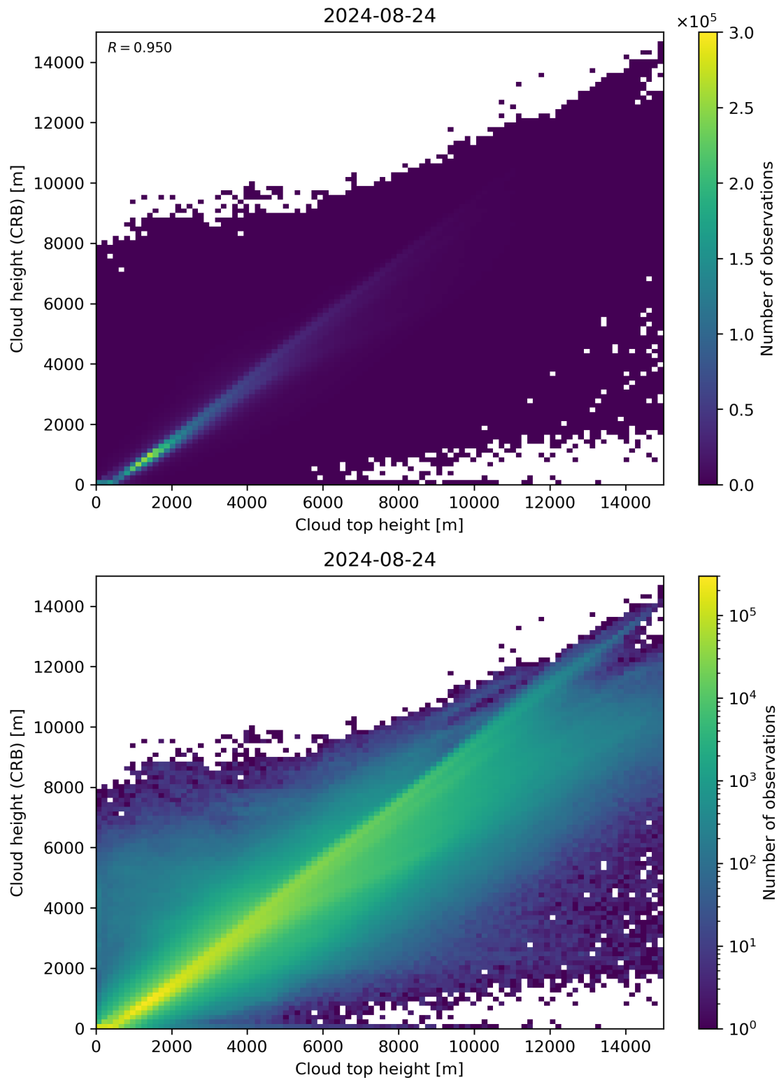
Figure 89: Scatter density plot of “Cloud top height” against “Cloud height (CRB)” for 2024-08-23 to 2024-08-25.
