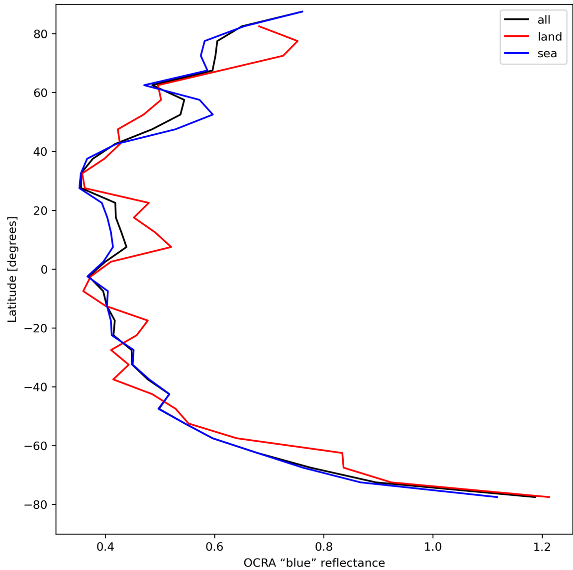
Figure 35: Zonal average of “OCRA “blue” reflectance” for 2024-08-23 to 2024-08-25.
