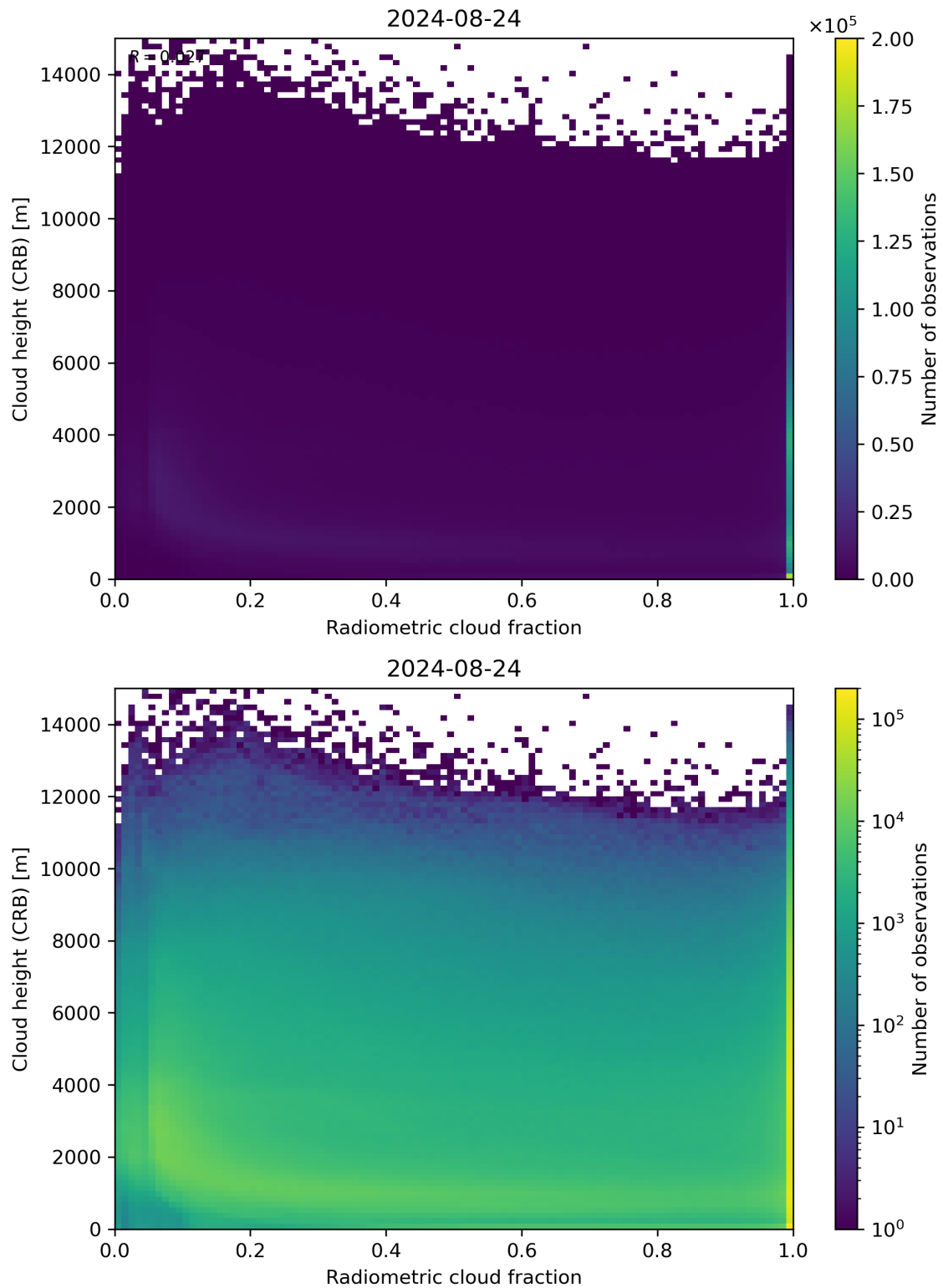
Figure 74: Scatter density plot of “Radiometric cloud fraction” against “Cloud height (CRB)” for 2024-08-23 to 2024-08-25.
