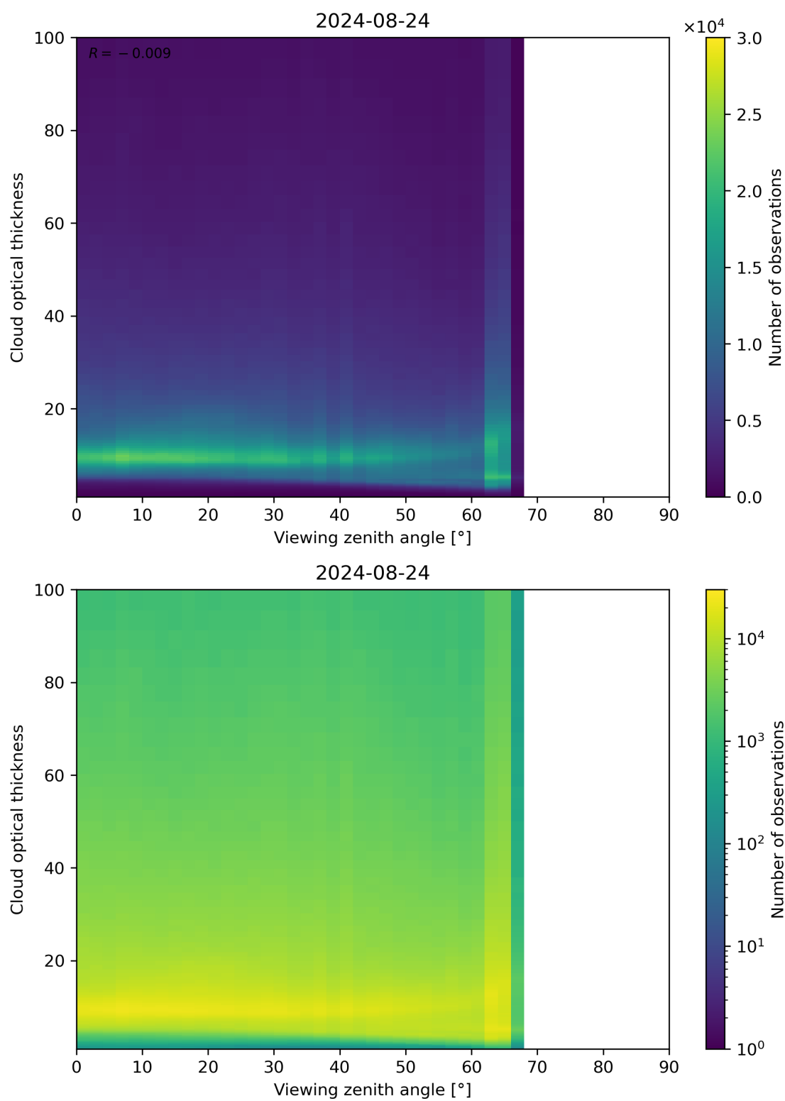
Figure 111: Scatter density plot of “Viewing zenith angle” against “Cloud optical thickness” for 2024-08-23 to 2024-08-25.
