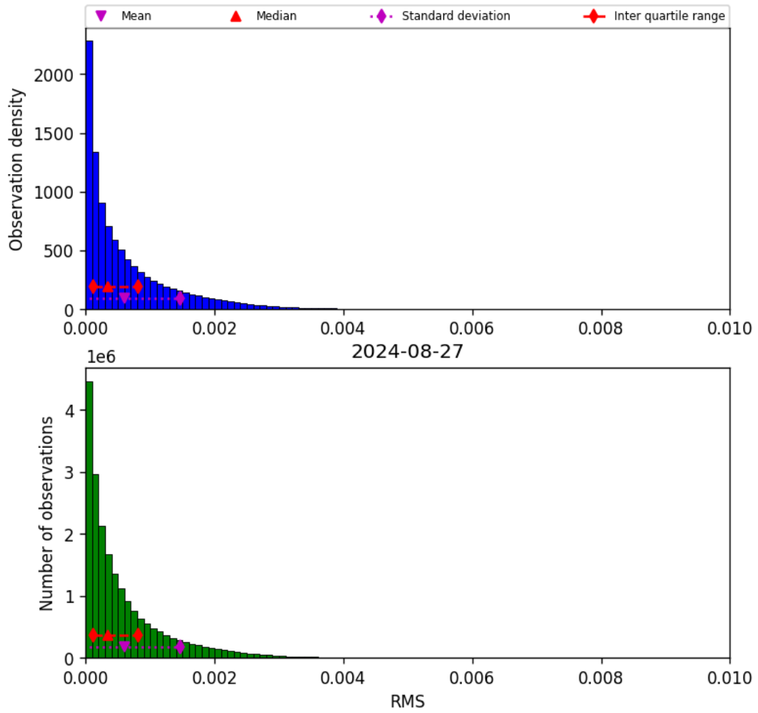
Figure 47: Histogram of “RMS” for 2024-08-27 to 2024-08-28
