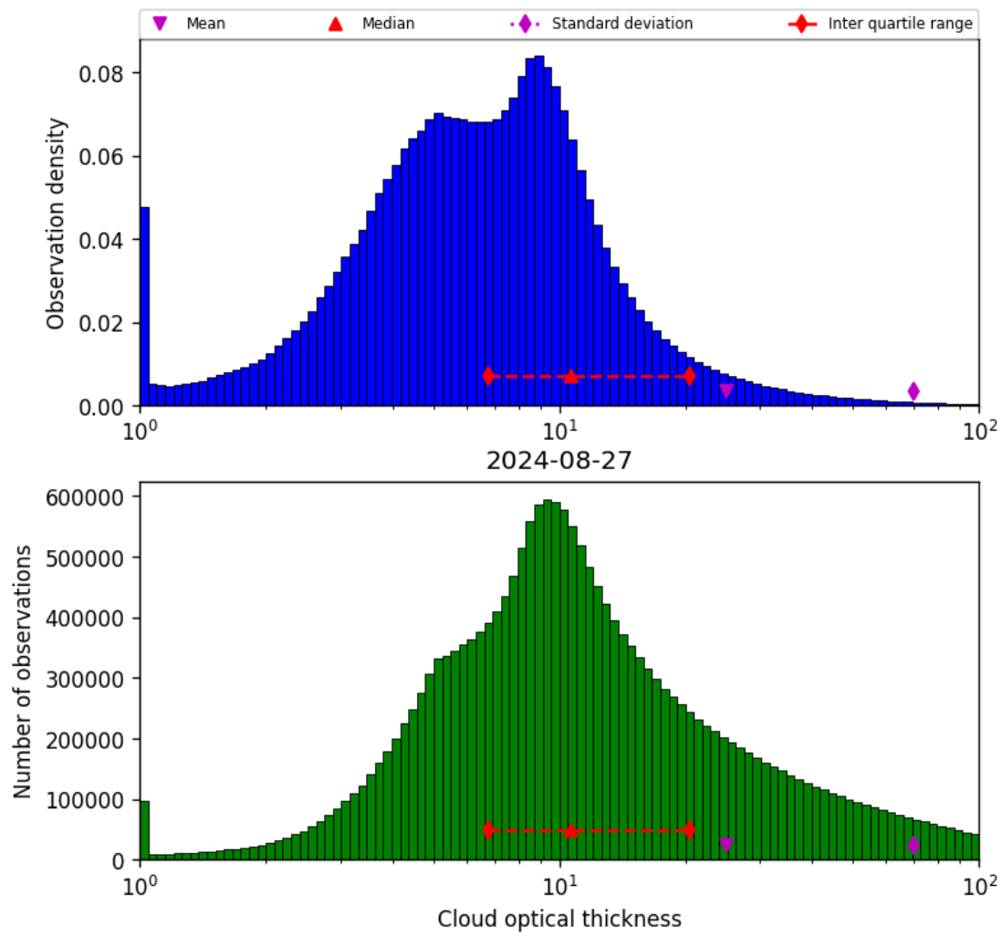
Figure 41: Histogram of “Cloud optical thickness” for 2024-08-27 to 2024-08-28
