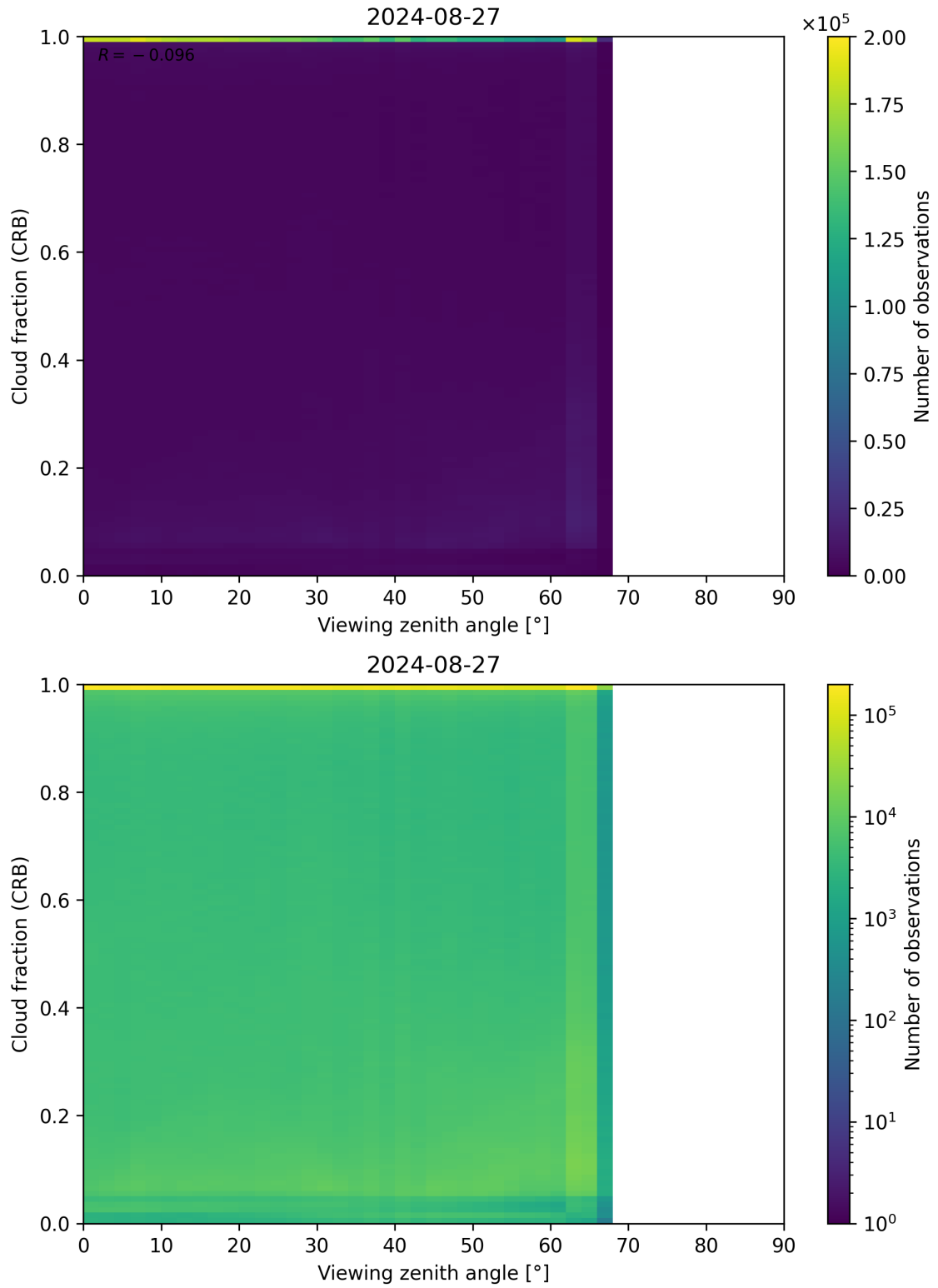
Figure 109: Scatter density plot of “Viewing zenith angle” against “Cloud fraction (CRB)” for 2024-08-27 to 2024-08-28.
