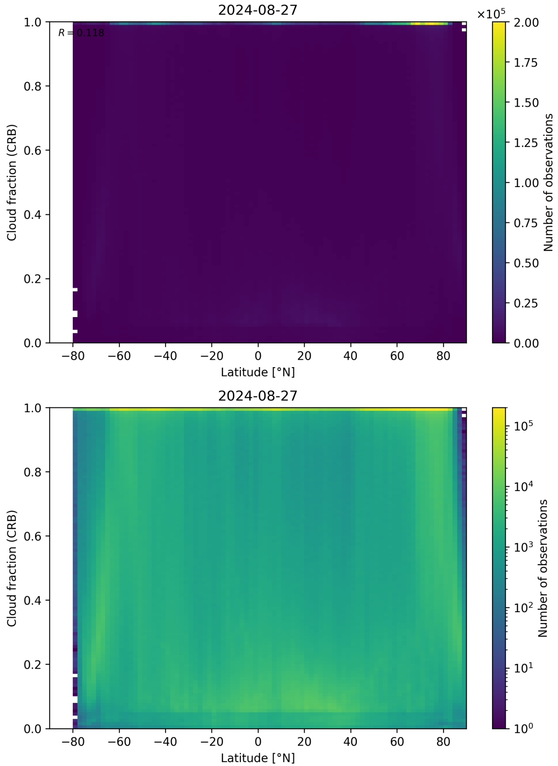
Figure 94: Scatter density plot of “Latitude” against “Cloud fraction (CRB)” for 2024-08-27 to 2024-08-28.
