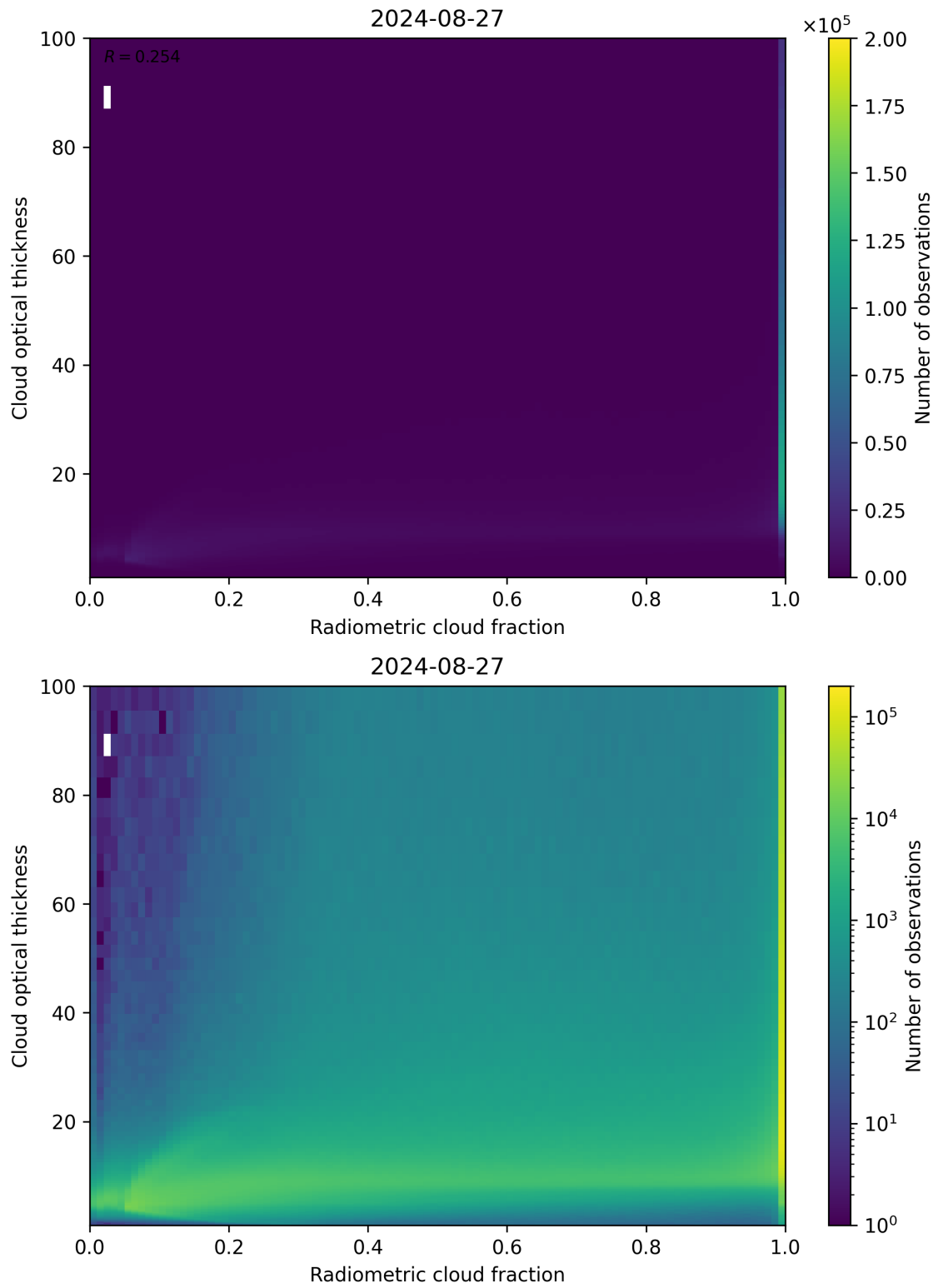
Figure 75: Scatter density plot of “Radiometric cloud fraction” against “Cloud optical thickness” for 2024-08-27 to 2024-08-28.
