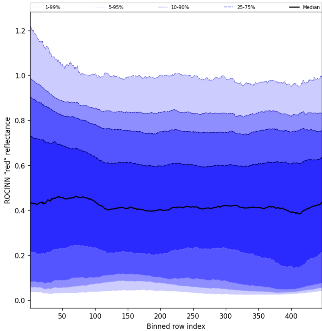
Figure 69: Along track statistics of “ROCINN “red” reflectance” for 2024-08-27 to 2024-08-28
