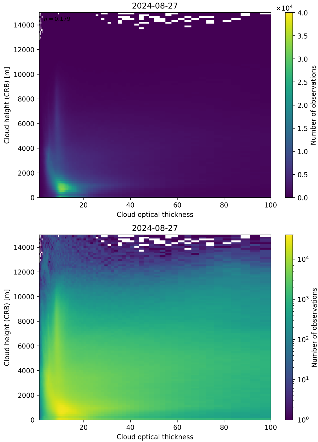
Figure 85: Scatter density plot of “Cloud optical thickness” against “Cloud height (CRB)” for 2024-08-27 to 2024-08-28.
