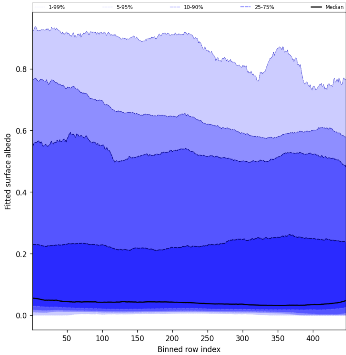
Figure 61: Along track statistics of “Fitted surface albedo” for 2024-08-27 to 2024-08-28
