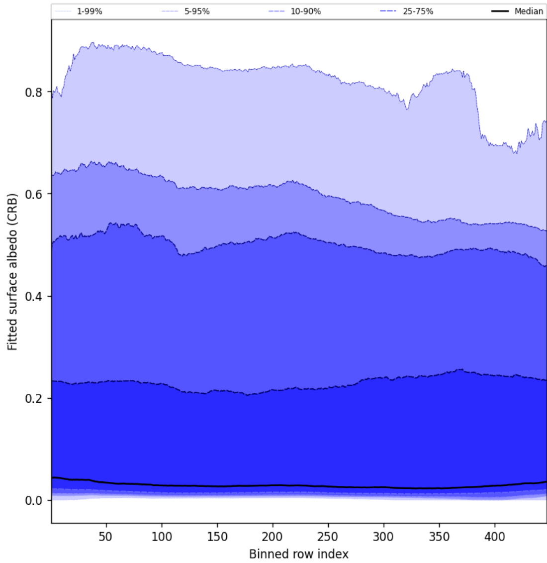
Figure 62: Along track statistics of “Fitted surface albedo (CRB)” for 2024-08-27 to 2024-08-28
