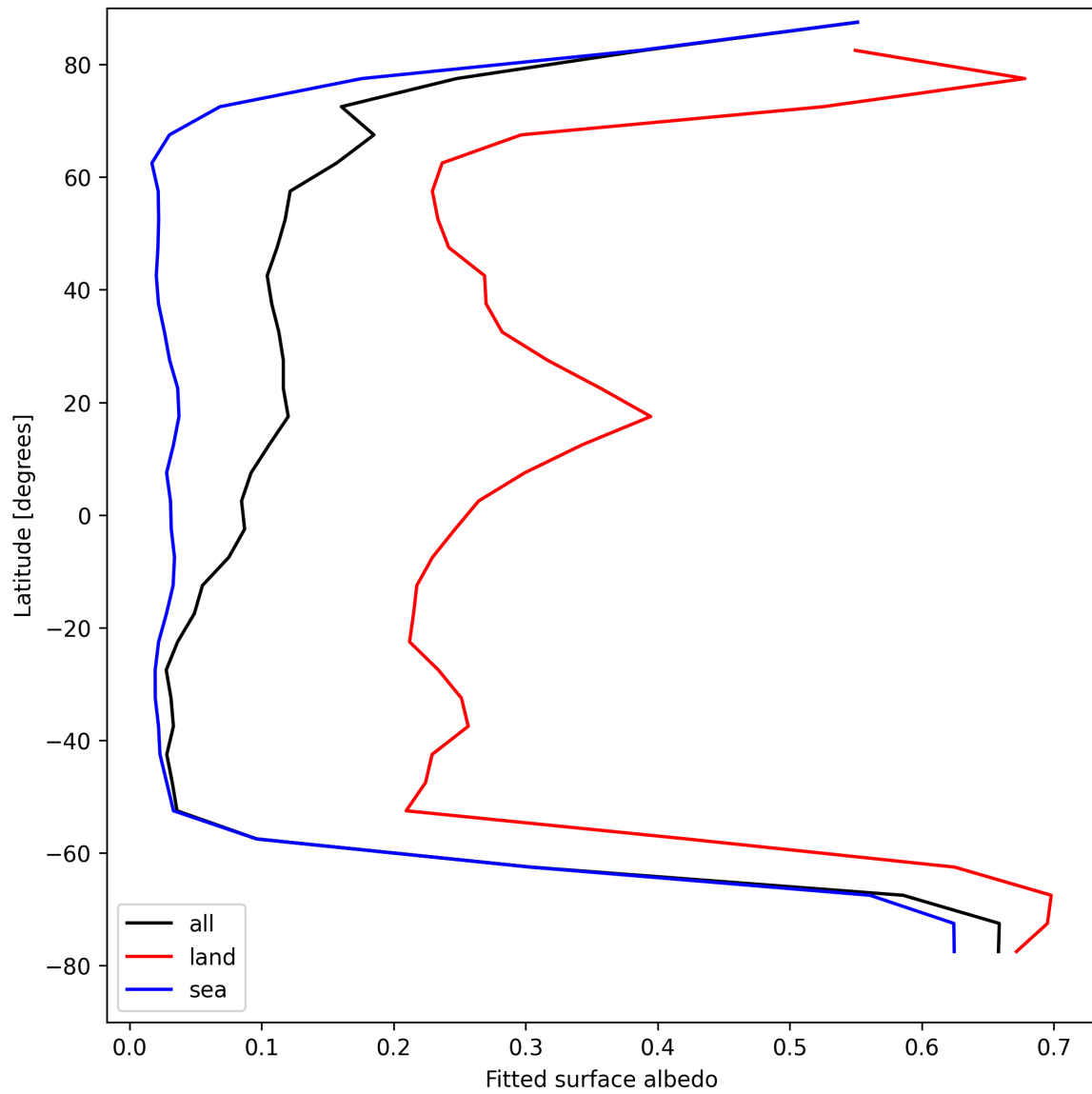
Figure 29: Zonal average of “Fitted surface albedo” for 2024-08-27 to 2024-08-28.
