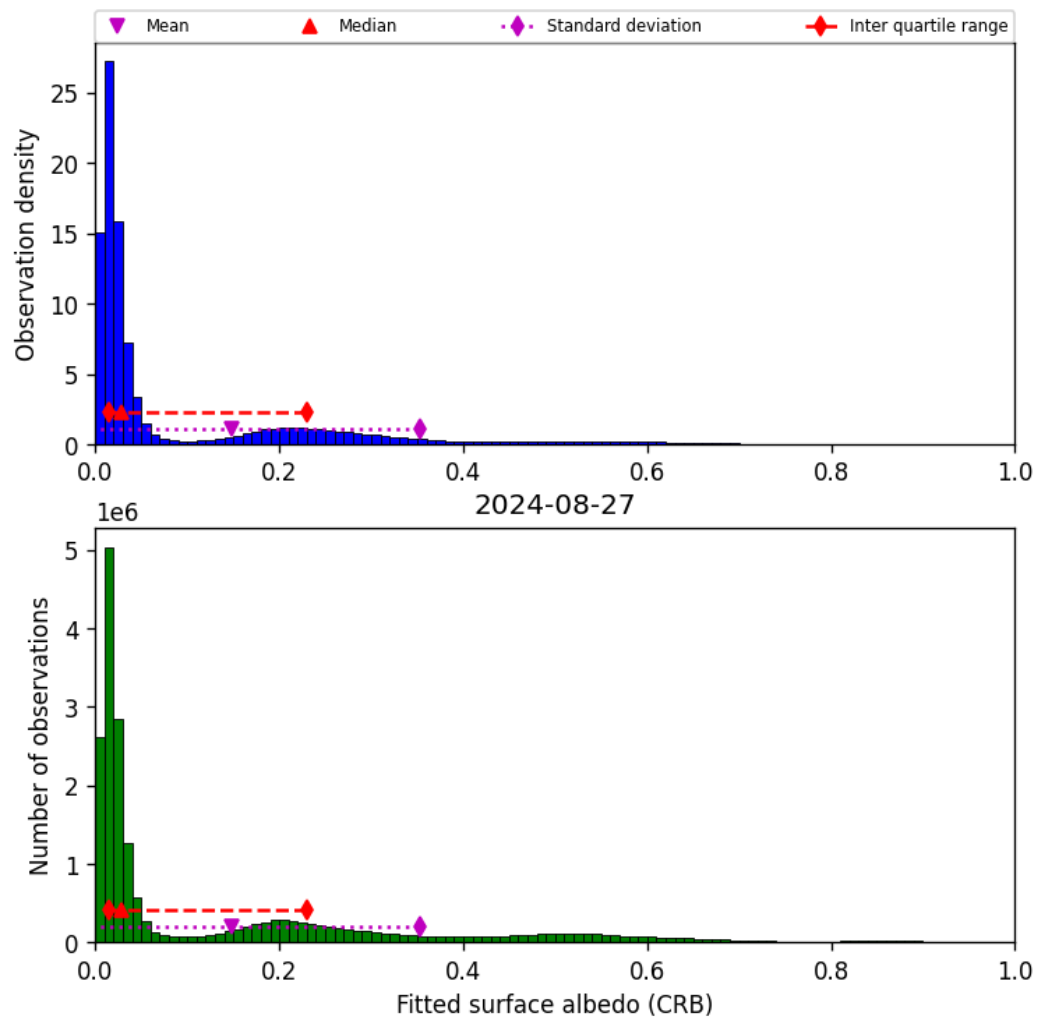
Figure 46: Histogram of “Fitted surface albedo (CRB)” for 2024-08-27 to 2024-08-28
