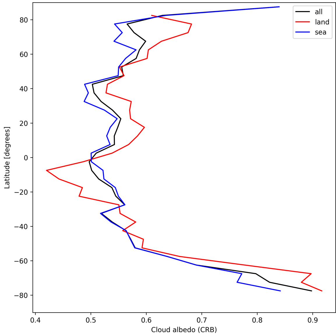
Figure 28: Zonal average of “Cloud albedo (CRB)” for 2024-08-27 to 2024-08-28.
