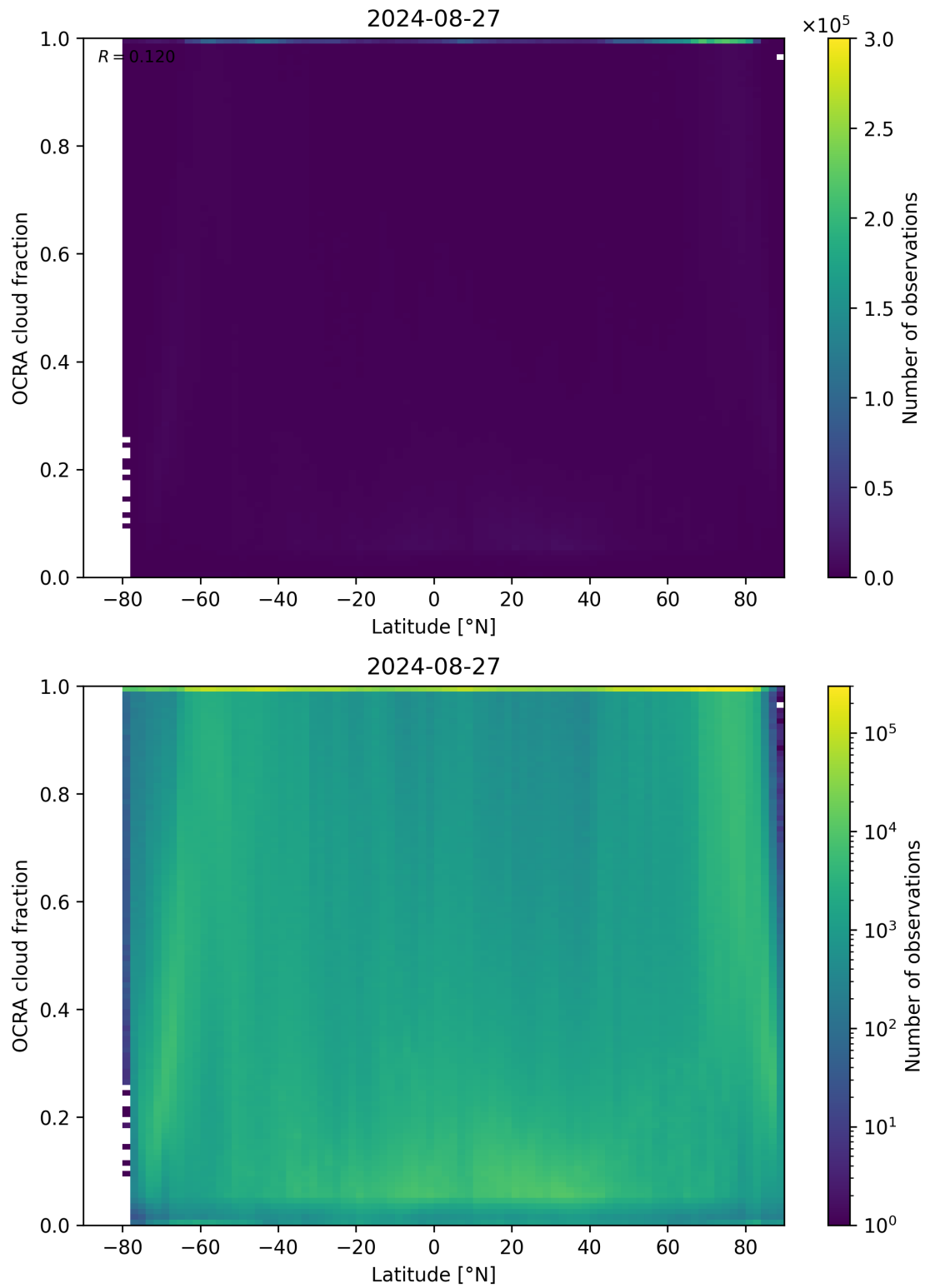
Figure 93: Scatter density plot of “Latitude” against “OCRA cloud fraction” for 2024-08-27 to 2024-08-28.
