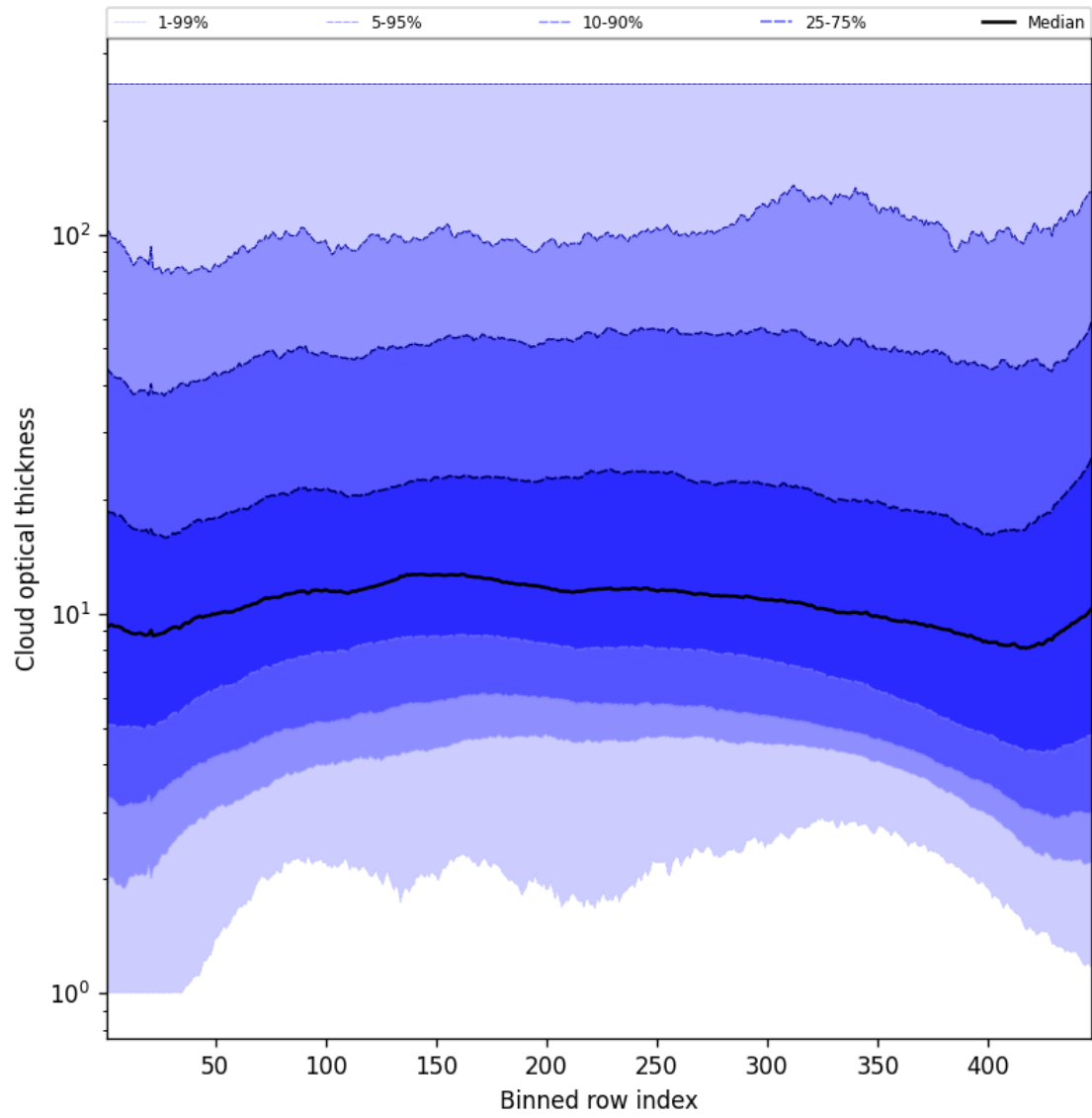
Figure 57: Along track statistics of “Cloud optical thickness” for 2024-08-27 to 2024-08-28
