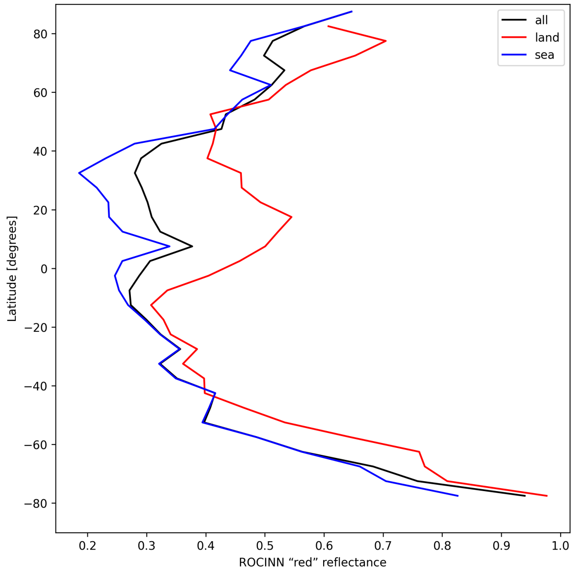
Figure 37: Zonal average of “ROCINN “red” reflectance” for 2024-08-27 to 2024-08-28.
