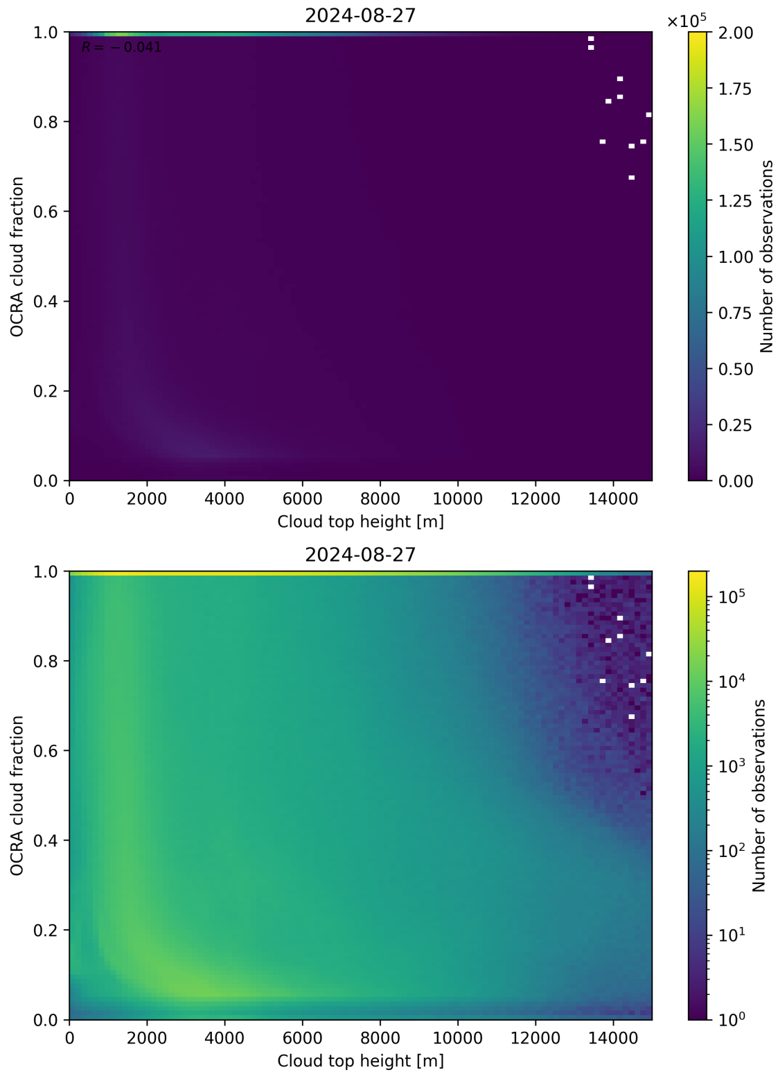
Figure 87: Scatter density plot of “Cloud top height” against “OCRA cloud fraction” for 2024-08-27 to 2024-08-28.
