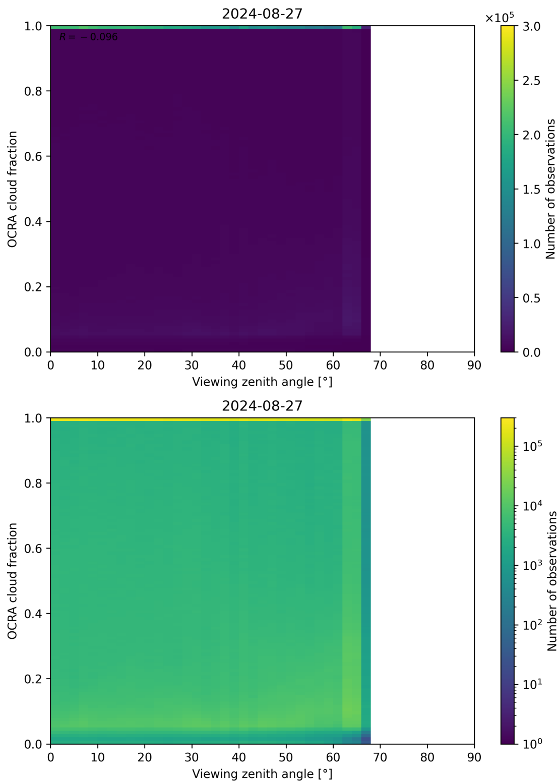
Figure 108: Scatter density plot of “Viewing zenith angle” against “OCRA cloud fraction” for 2024-08-27 to 2024-08-28.
