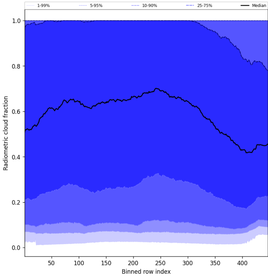
Figure 55: Along track statistics of “Radiometric cloud fraction” for 2024-08-27 to 2024-08-28
