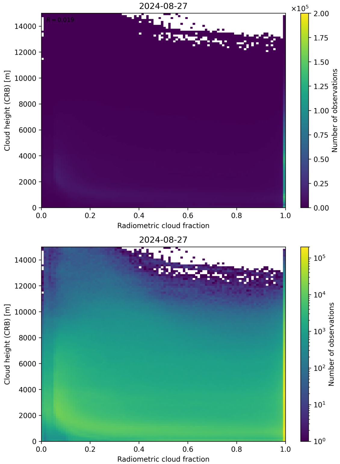
Figure 74: Scatter density plot of “Radiometric cloud fraction” against “Cloud height (CRB)” for 2024-08-27 to 2024-08-28.
