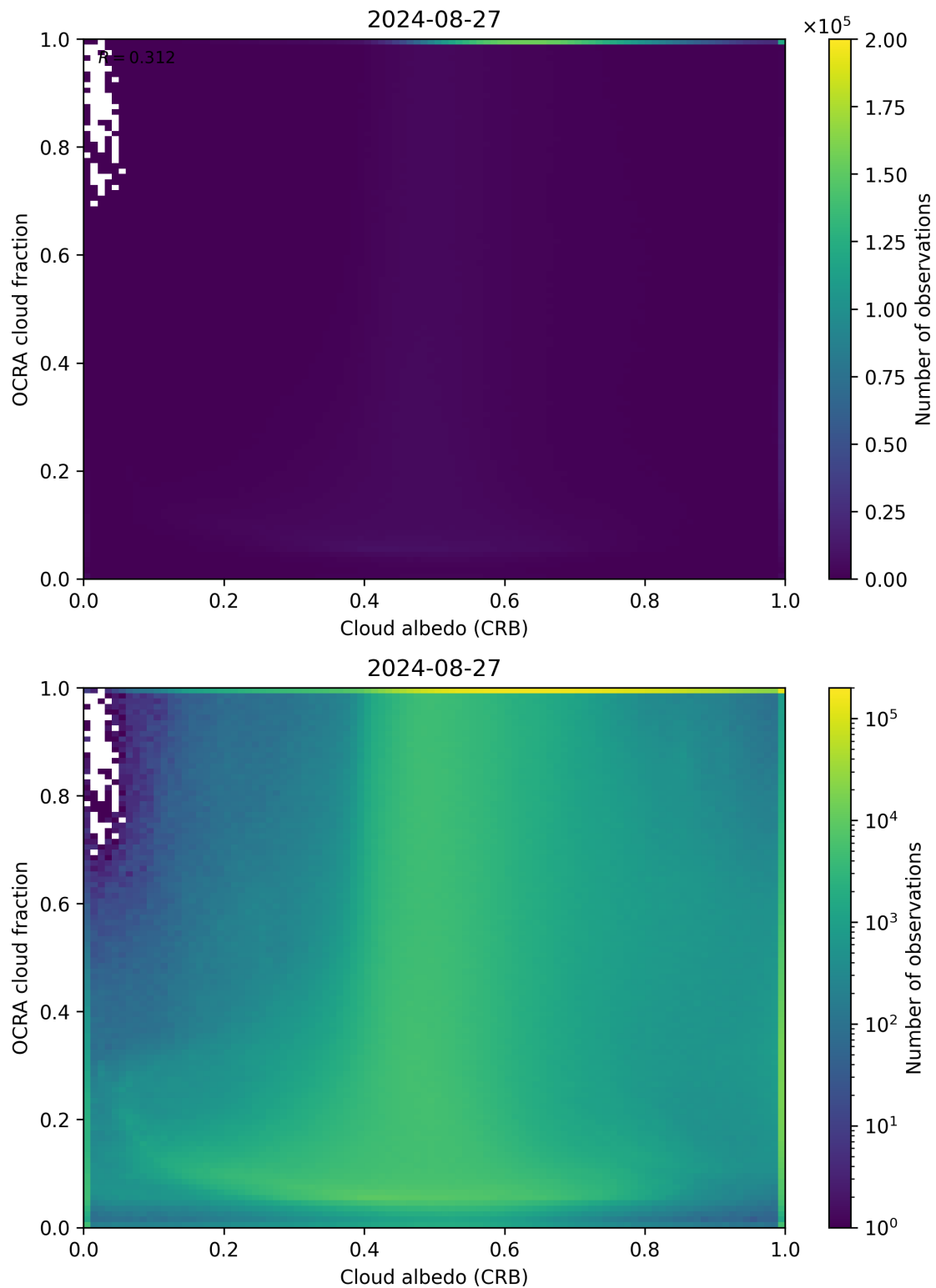
Figure 70: Scatter density plot of “Cloud albedo (CRB)” against “OCRA cloud fraction” for 2024-08-27 to 2024-08-28.
