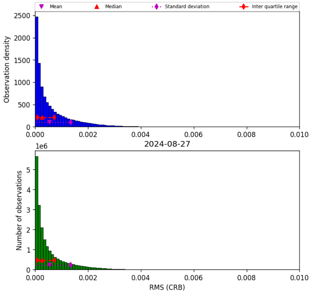
Figure 48: Histogram of “RMS (CRB)” for 2024-08-27 to 2024-08-28
