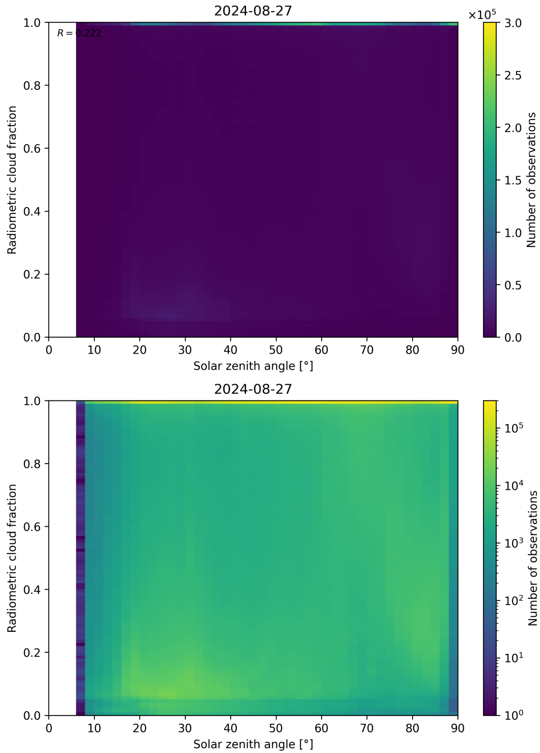
Figure 99: Scatter density plot of “Solar zenith angle” against “Radiometric cloud fraction” for 2024-08-27 to 2024-08-28.
