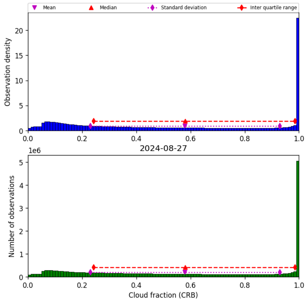
Figure 42: Histogram of “Cloud fraction (CRB)” for 2024-08-27 to 2024-08-28
