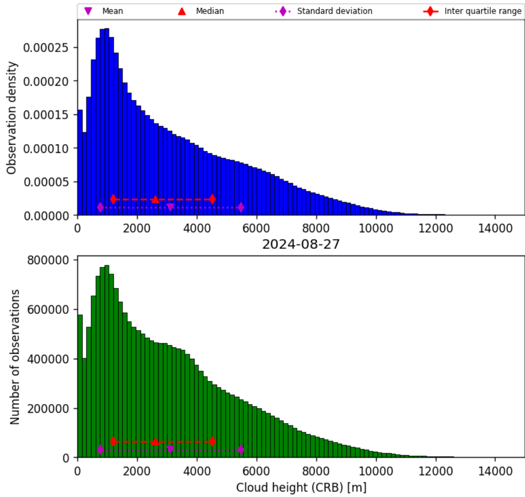
Figure 43: Histogram of “Cloud height (CRB)” for 2024-08-27 to 2024-08-28
