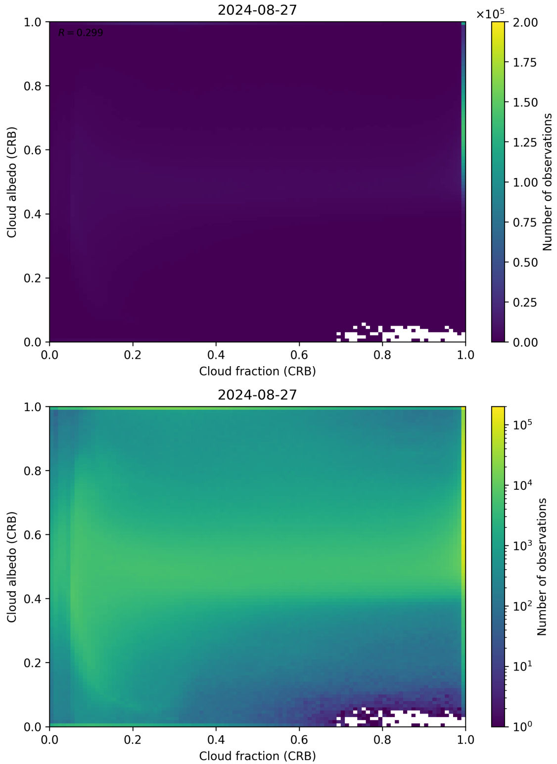
Figure 77: Scatter density plot of “Cloud fraction (CRB)” against “Cloud albedo (CRB)” for 2024-08-27 to 2024-08-28.
