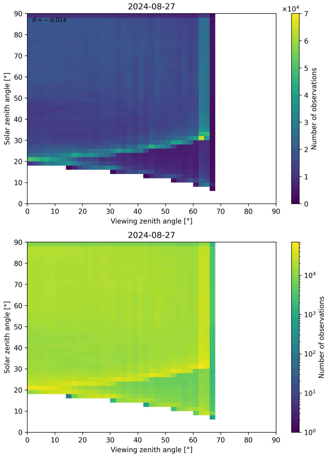
Figure 114: Scatter density plot of “Viewing zenith angle” against “Solar zenith angle” for 2024-08-27 to 2024-08-28.
