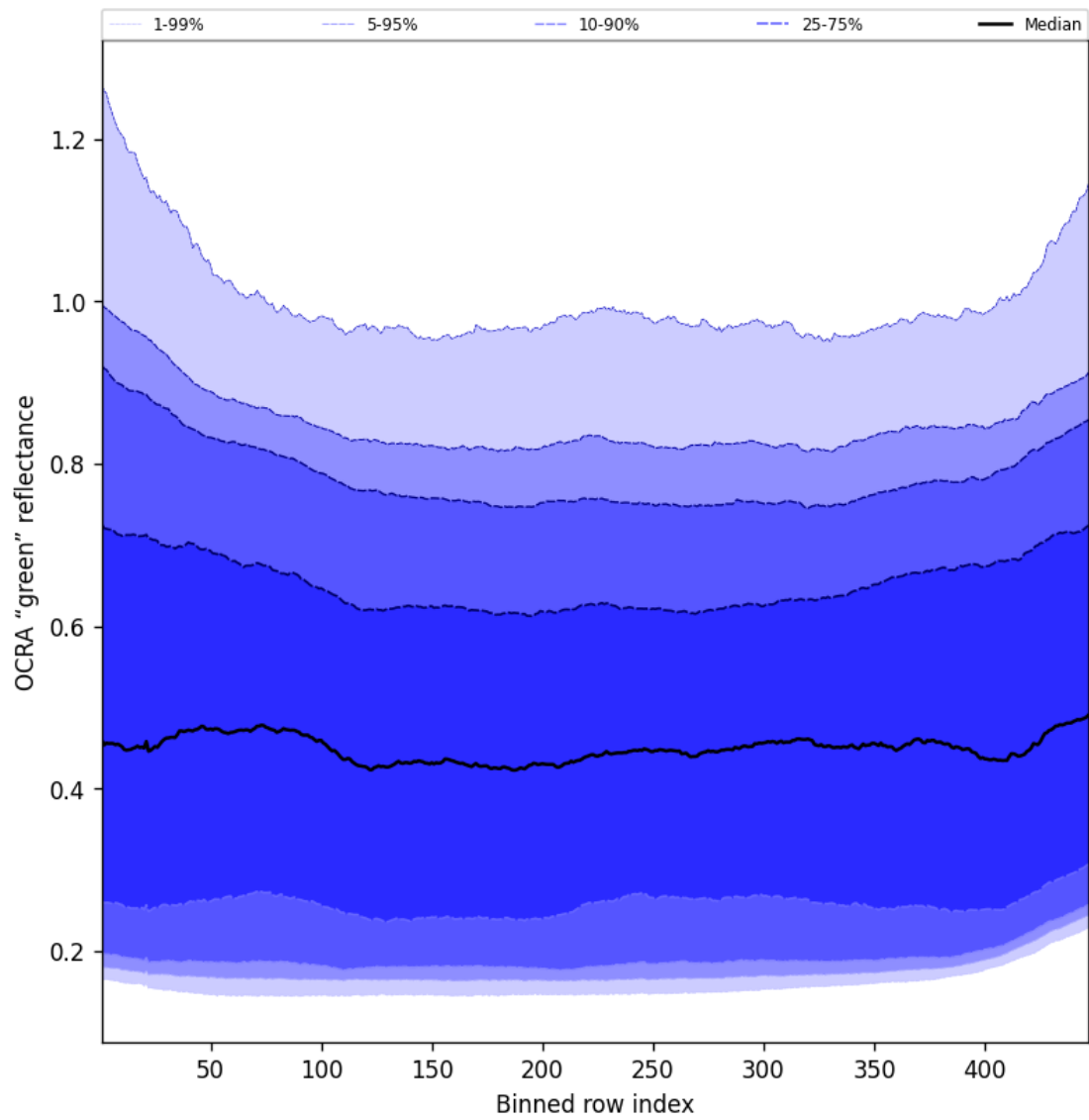
Figure 68: Along track statistics of “OCRA “green” reflectance” for 2024-08-27 to 2024-08-28
