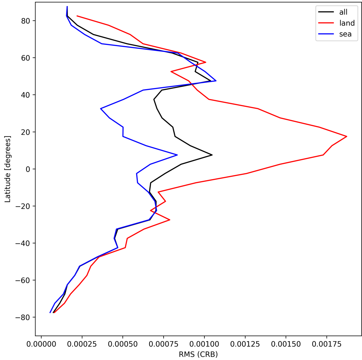
Figure 32: Zonal average of “RMS (CRB)” for 2024-08-27 to 2024-08-28.
