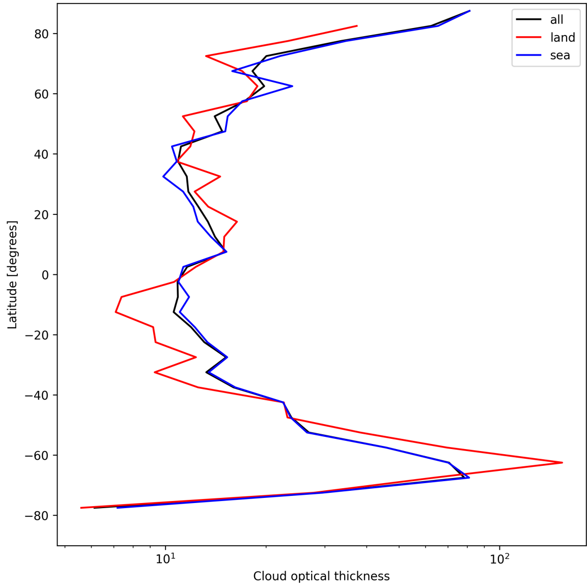
Figure 25: Zonal average of “Cloud optical thickness” for 2024-08-27 to 2024-08-28.
