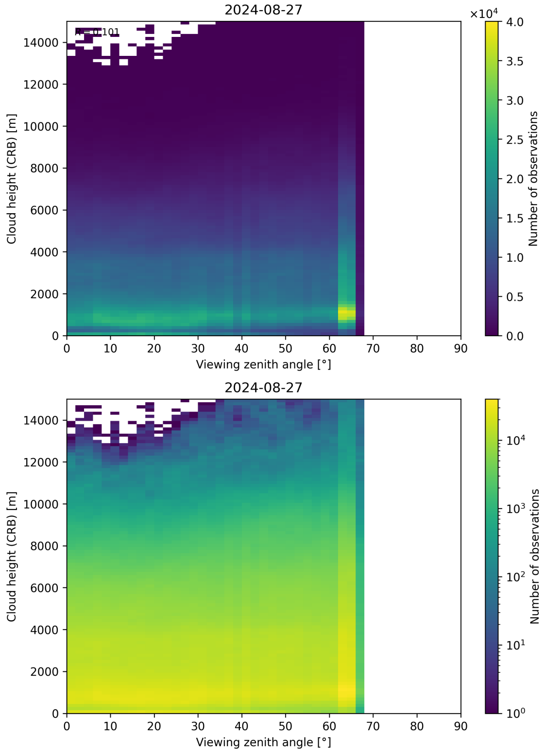
Figure 110: Scatter density plot of “Viewing zenith angle” against “Cloud height (CRB)” for 2024-08-27 to 2024-08-28.
