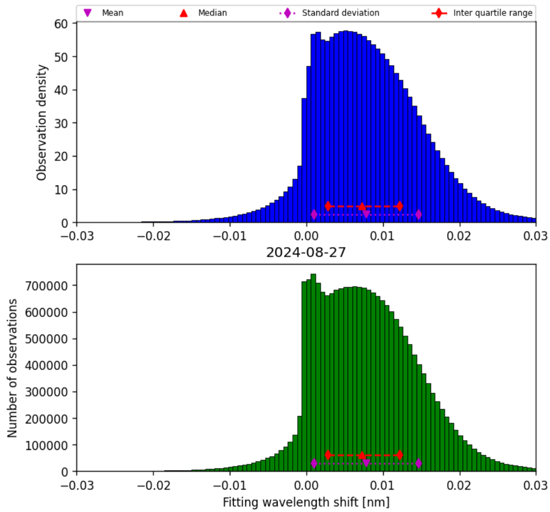
Figure 49: Histogram of “Fitting wavelength shift” for 2024-08-27 to 2024-08-28
