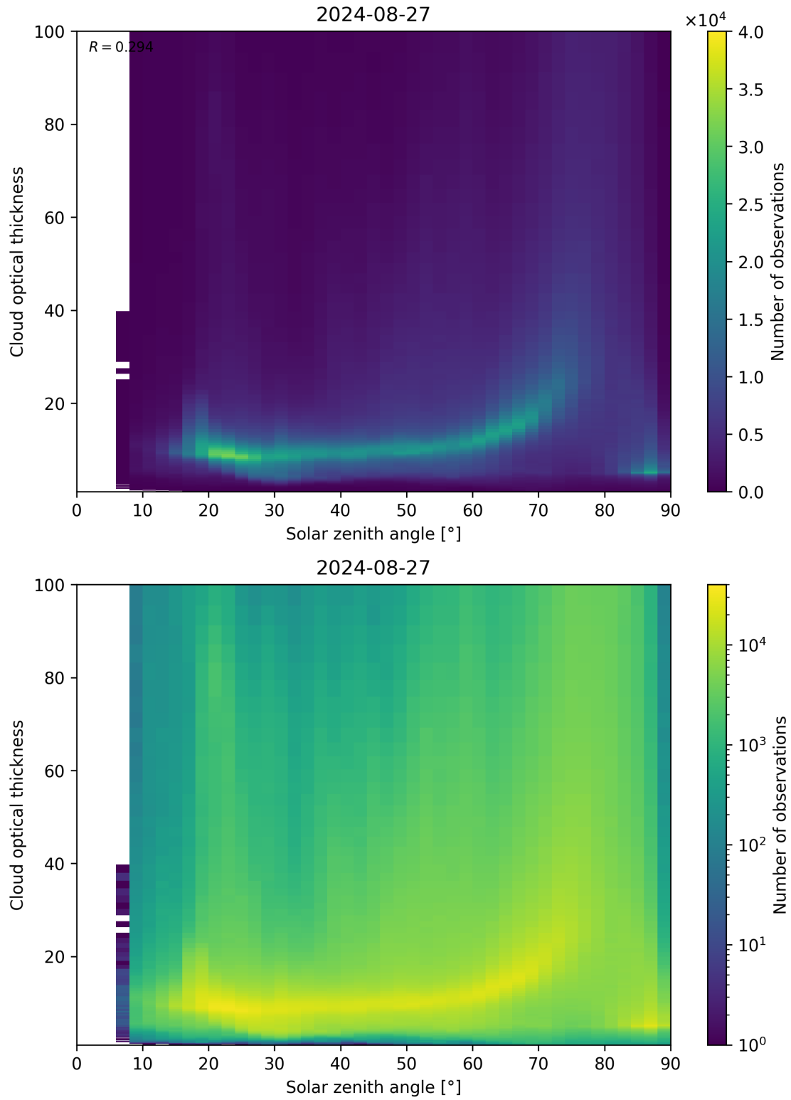
Figure 103: Scatter density plot of “Solar zenith angle” against “Cloud optical thickness” for 2024-08-27 to 2024-08-28.
