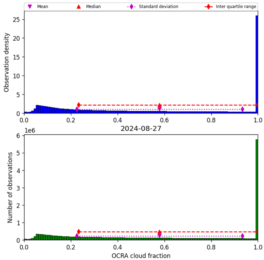
Figure 50: Histogram of “OCRA cloud fraction” for 2024-08-27 to 2024-08-28
