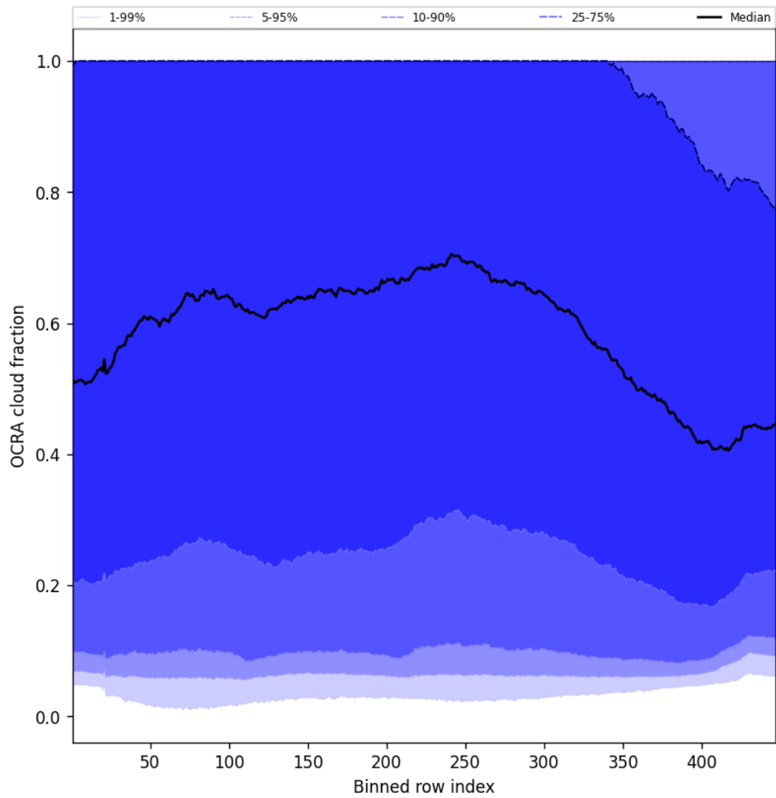
Figure 66: Along track statistics of “OCRA cloud fraction” for 2024-08-27 to 2024-08-28
