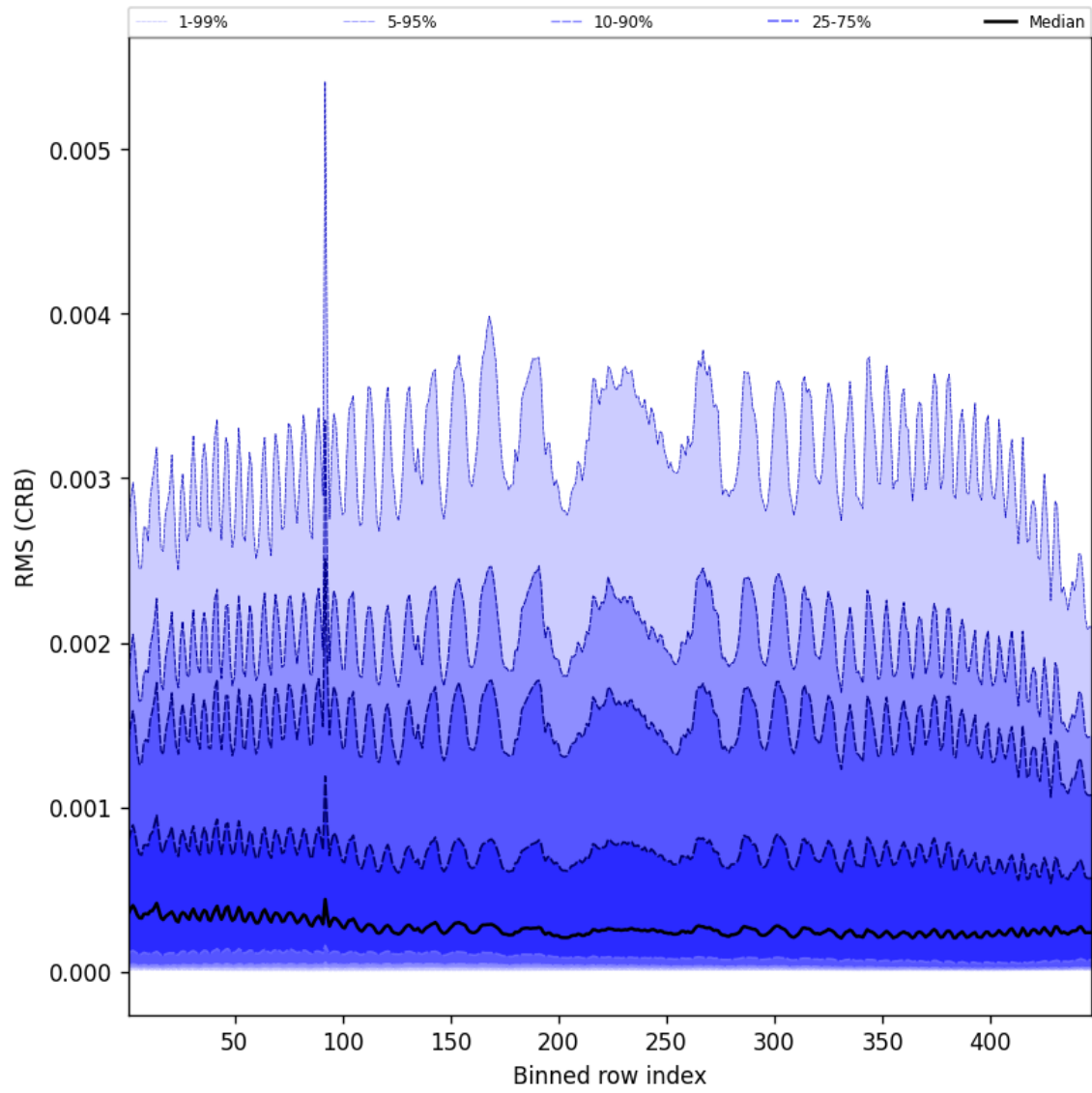
Figure 64: Along track statistics of “RMS (CRB)” for 2024-08-27 to 2024-08-28
