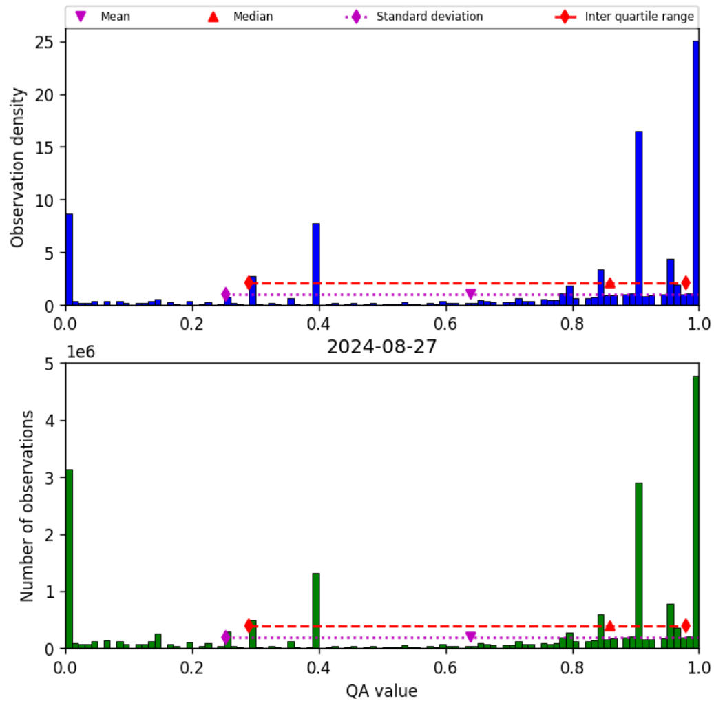
Figure 38: Histogram of “QA value” for 2024-08-27 to 2024-08-28
