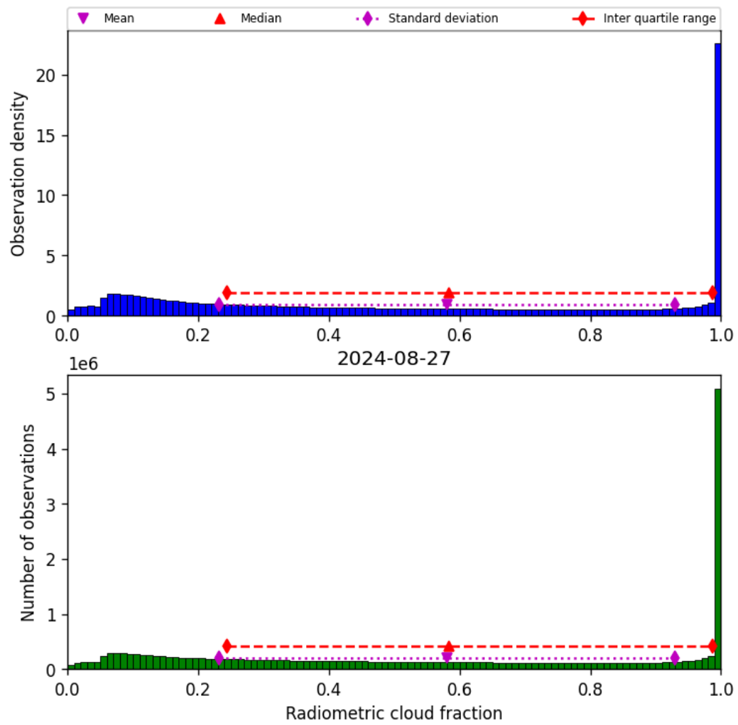
Figure 39: Histogram of “Radiometric cloud fraction” for 2024-08-27 to 2024-08-28
