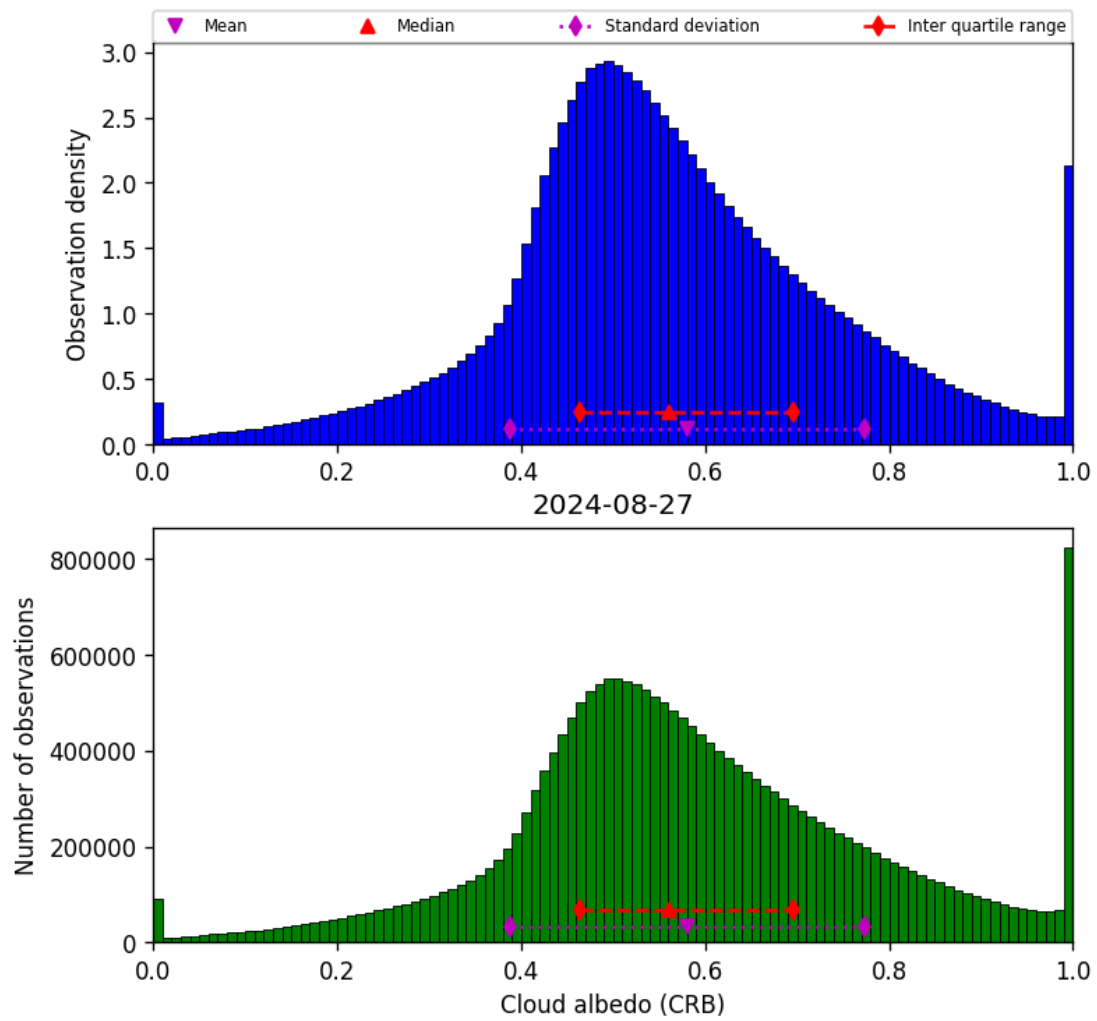
Figure 44: Histogram of “Cloud albedo (CRB)” for 2024-08-27 to 2024-08-28
