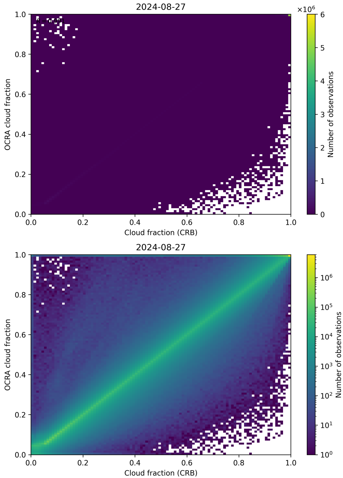
Figure 78: Scatter density plot of “Cloud fraction (CRB)” against “OCRA cloud fraction” for 2024-08-27 to 2024-08-28.
