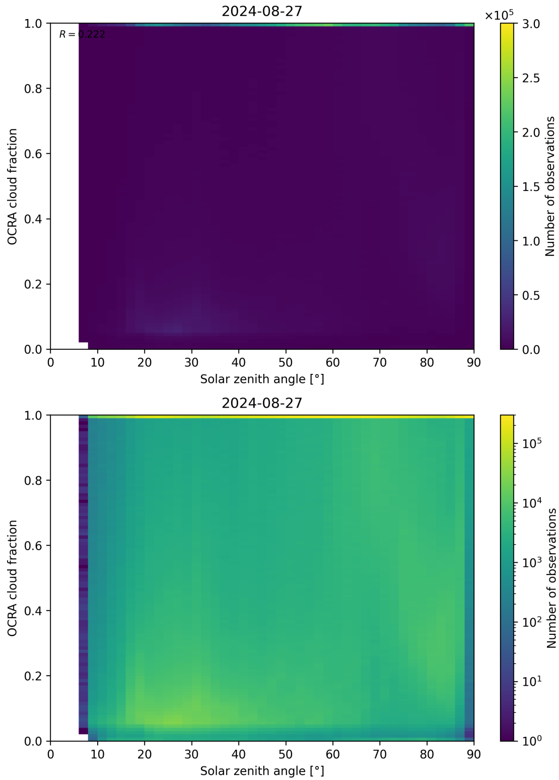
Figure 100: Scatter density plot of “Solar zenith angle” against “OCRA cloud fraction” for 2024-08-27 to 2024-08-28.
