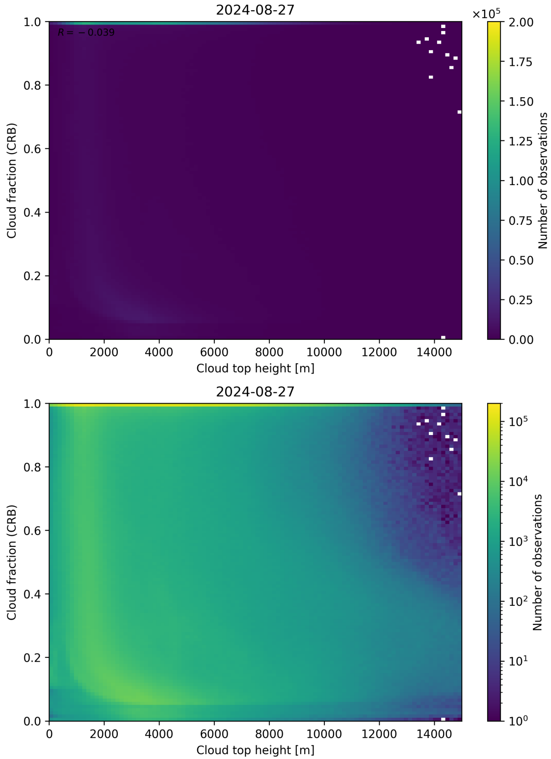
Figure 88: Scatter density plot of “Cloud top height” against “Cloud fraction (CRB)” for 2024-08-27 to 2024-08-28.
