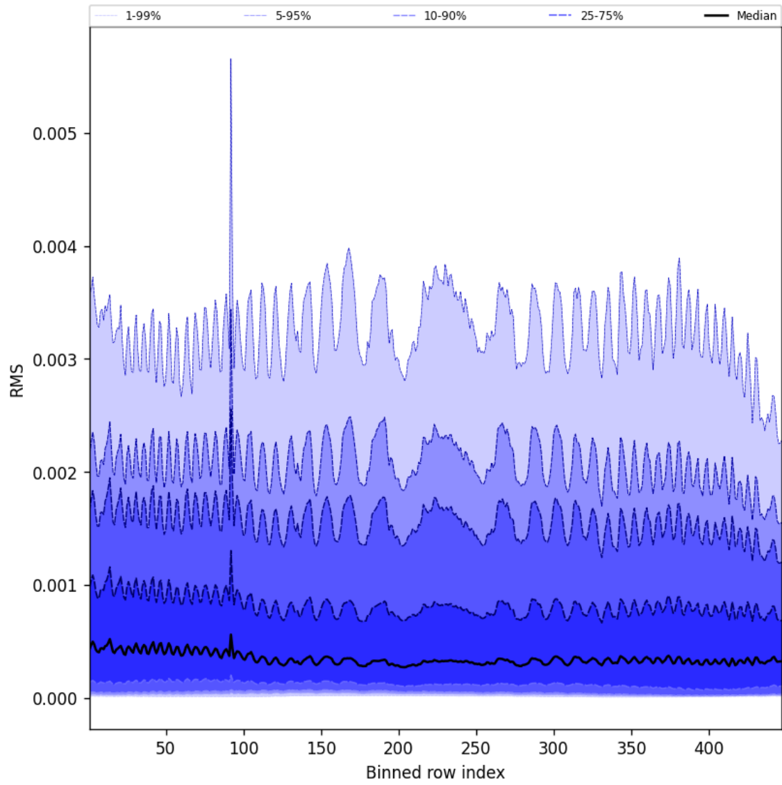
Figure 63: Along track statistics of “RMS” for 2024-08-27 to 2024-08-28
