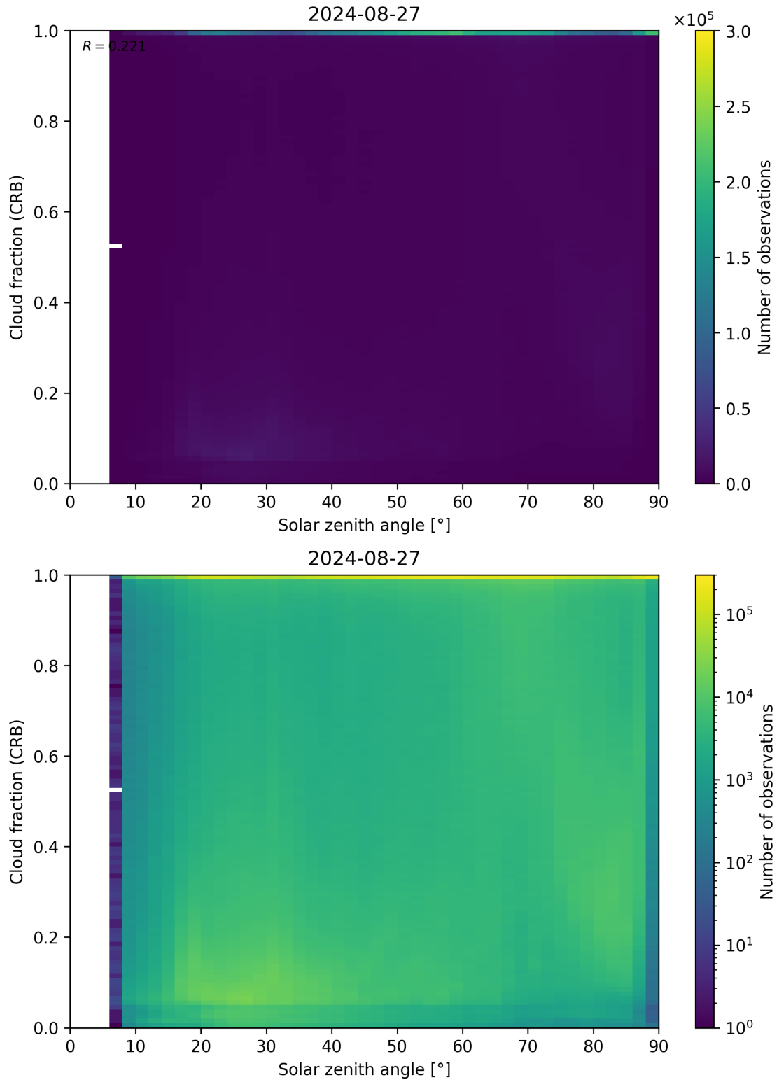
Figure 101: Scatter density plot of “Solar zenith angle” against “Cloud fraction (CRB)” for 2024-08-27 to 2024-08-28.
