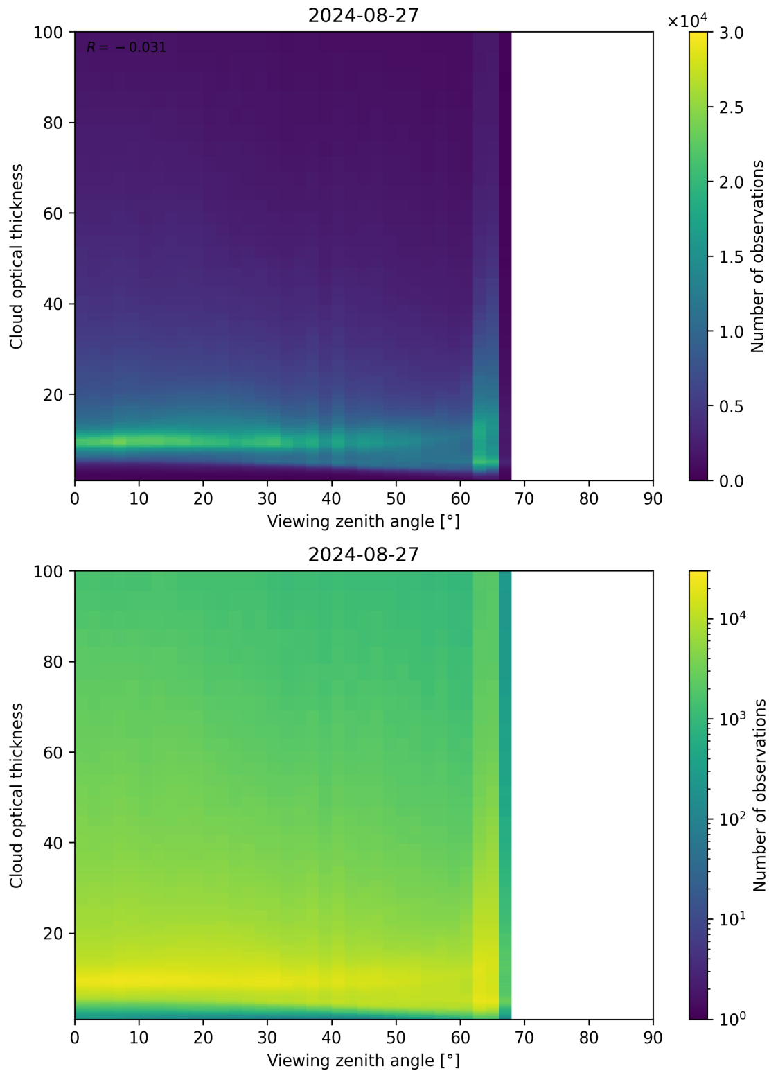
Figure 111: Scatter density plot of “Viewing zenith angle” against “Cloud optical thickness” for 2024-08-27 to 2024-08-28.
