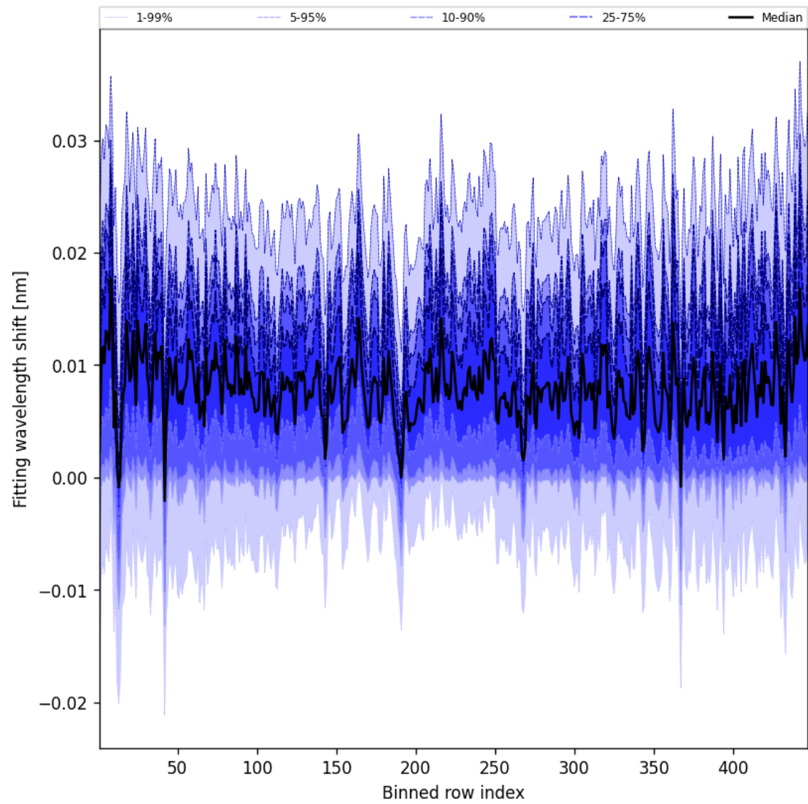
Figure 65: Along track statistics of “Fitting wavelength shift” for 2024-08-27 to 2024-08-28
