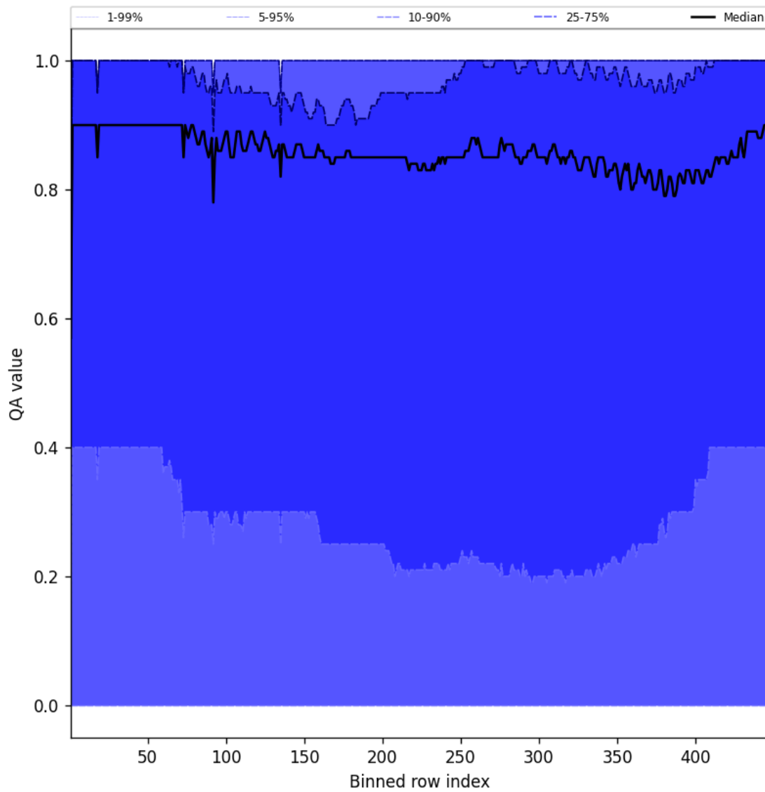
Figure 54: Along track statistics of “QA value” for 2024-08-27 to 2024-08-28
