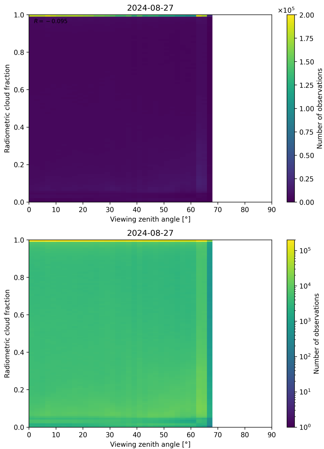
Figure 107: Scatter density plot of “Viewing zenith angle” against “Radiometric cloud fraction” for 2024-08-27 to 2024-08-28.
