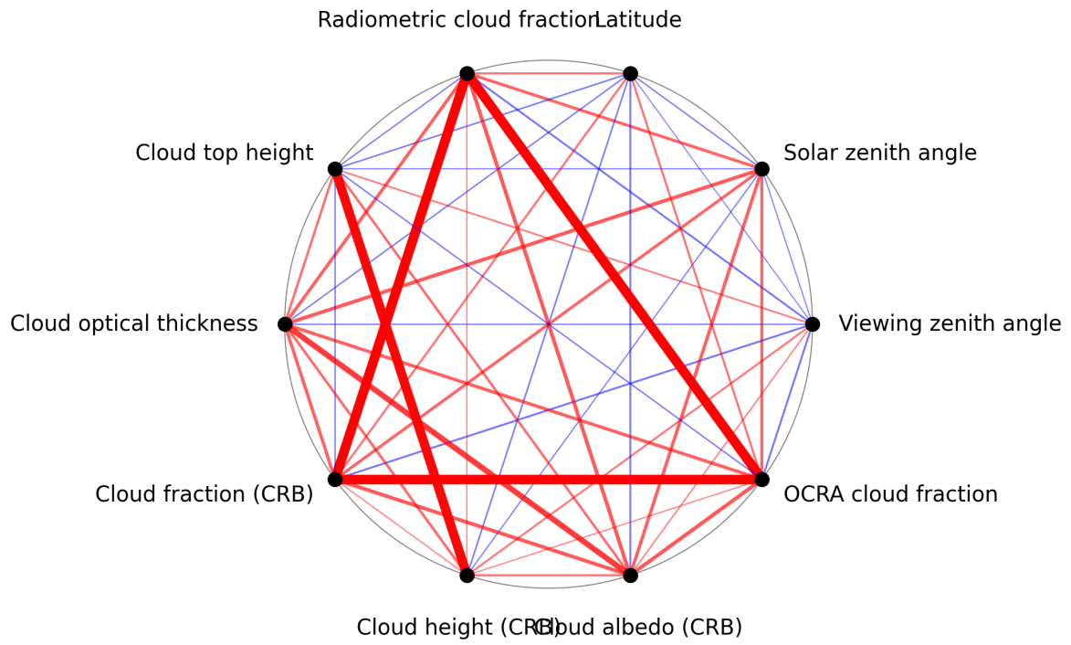
Figure 1: Map of correlation graph for 2024-08-27 to 2024-08-28.
