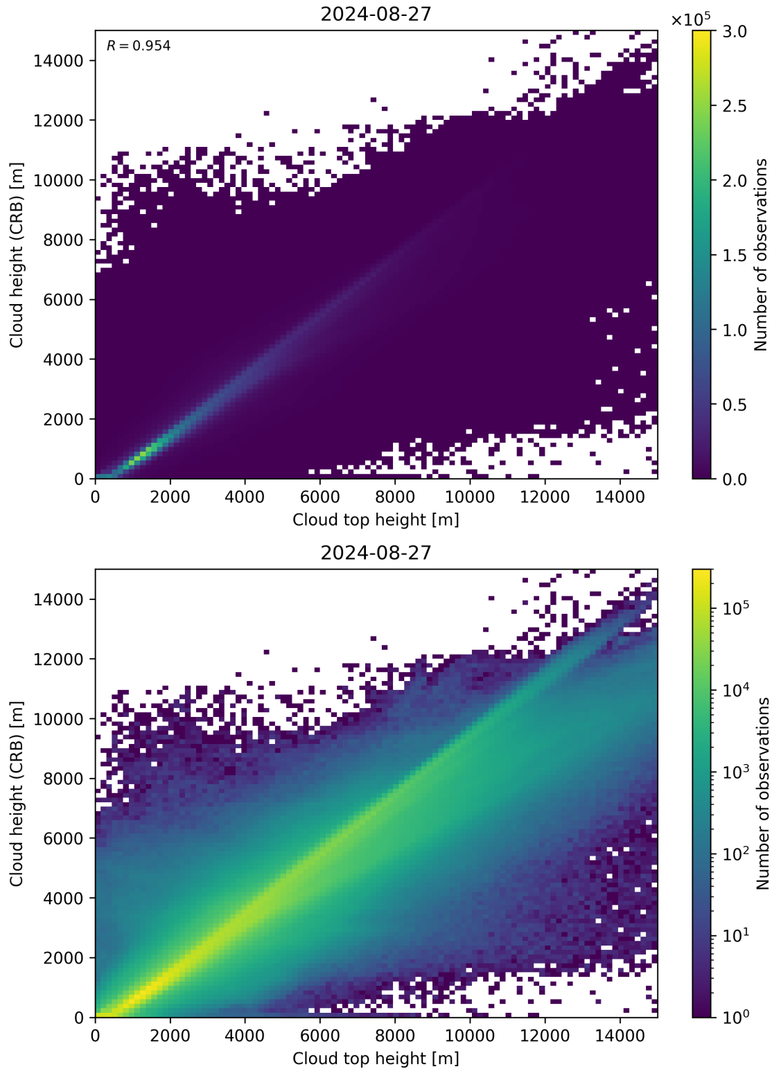
Figure 89: Scatter density plot of “Cloud top height” against “Cloud height (CRB)” for 2024-08-27 to 2024-08-28.
