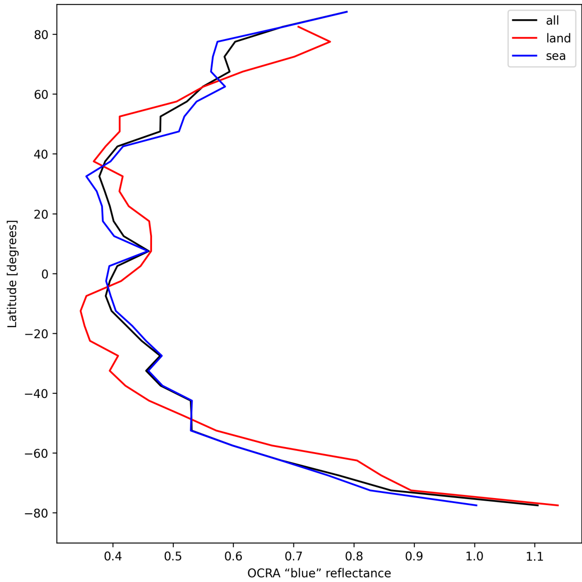
Figure 35: Zonal average of “OCRA “blue” reflectance” for 2024-08-27 to 2024-08-28.
