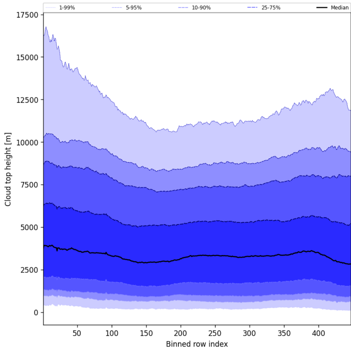
Figure 56: Along track statistics of “Cloud top height” for 2024-08-27 to 2024-08-28
