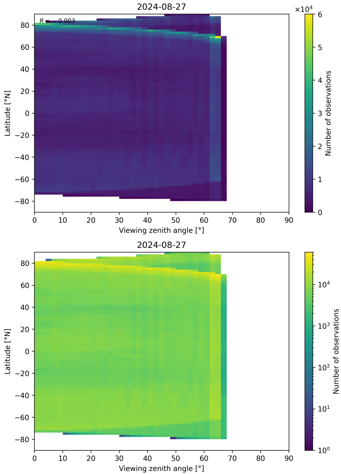
Figure 113: Scatter density plot of “Viewing zenith angle” against “Latitude” for 2024-08-27 to 2024-08-28.
