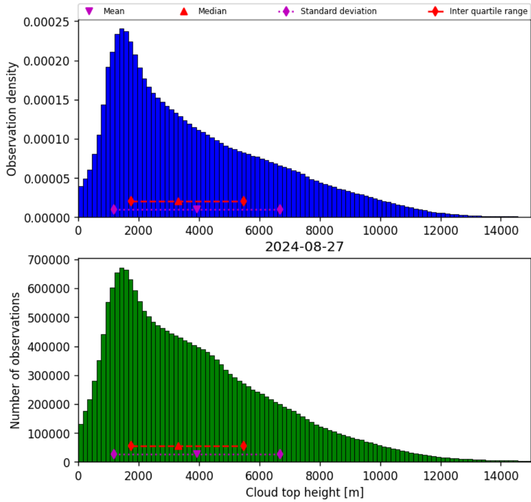
Figure 40: Histogram of “Cloud top height” for 2024-08-27 to 2024-08-28
