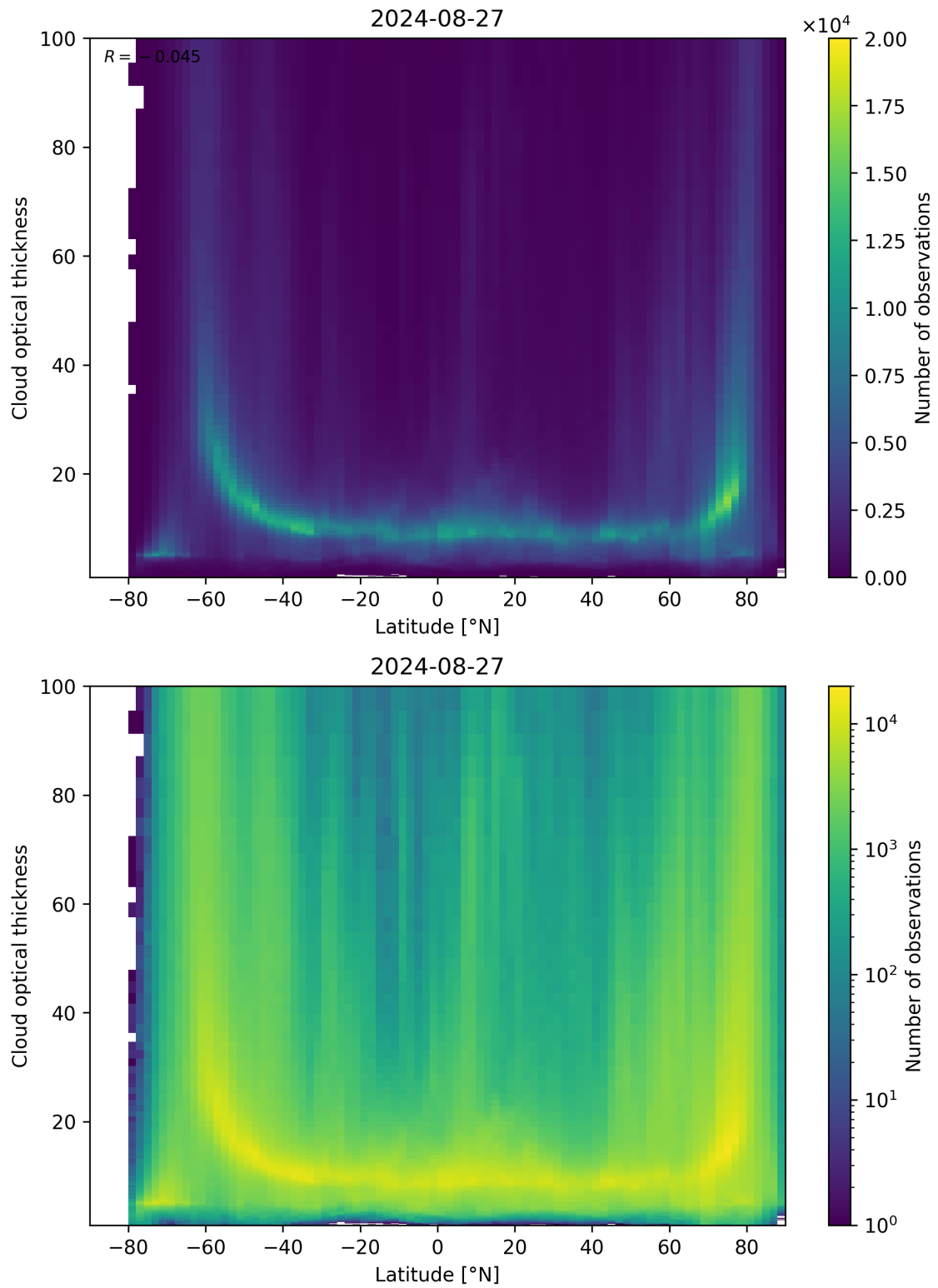
Figure 96: Scatter density plot of “Latitude” against “Cloud optical thickness” for 2024-08-27 to 2024-08-28.
