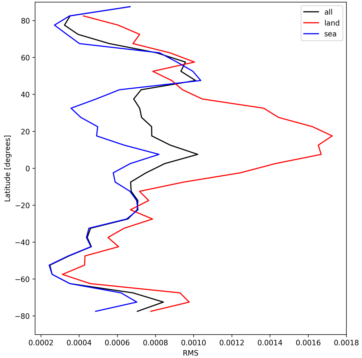
Figure 31: Zonal average of “RMS” for 2024-08-27 to 2024-08-28.
