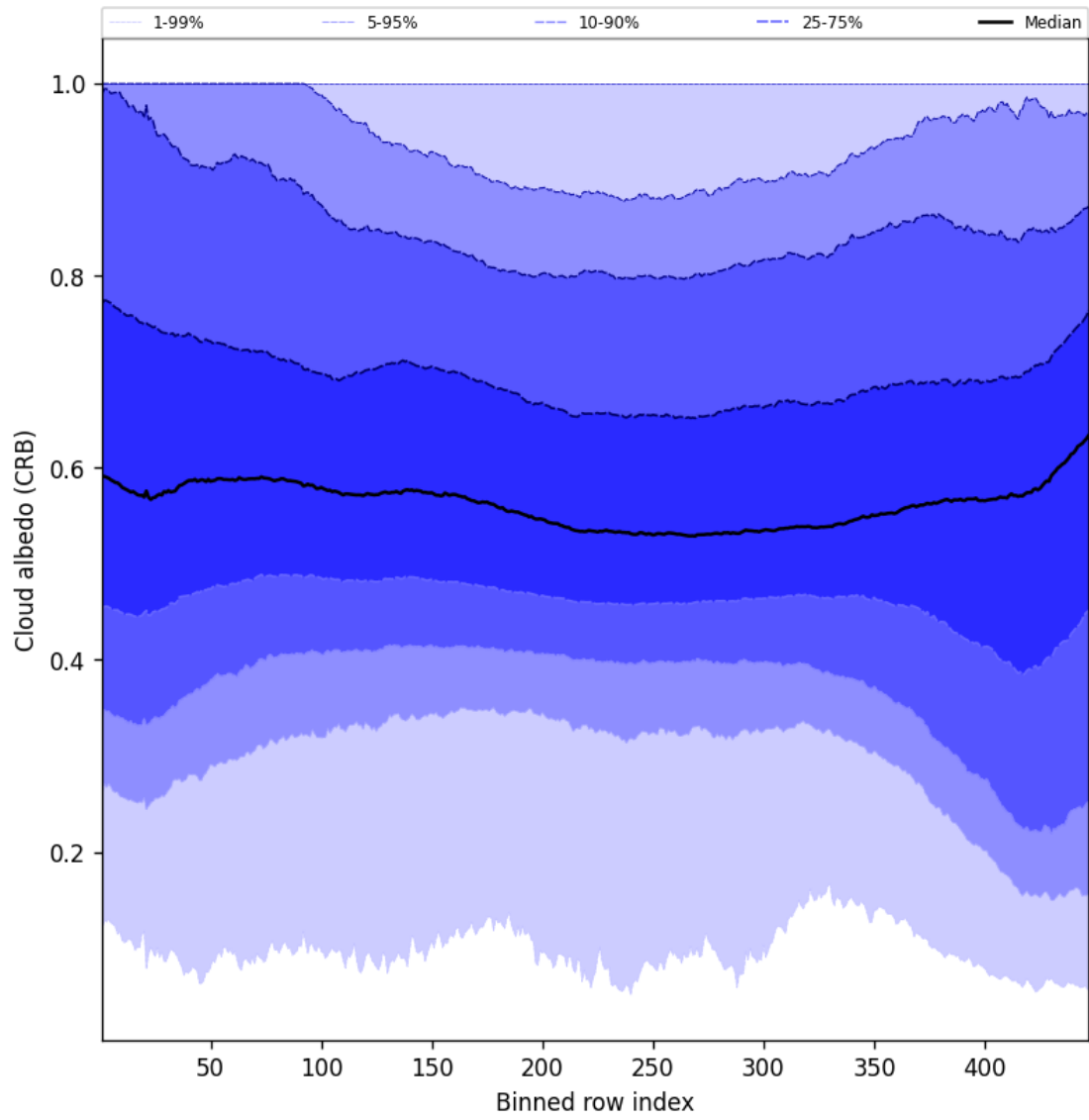
Figure 60: Along track statistics of “Cloud albedo (CRB)” for 2024-08-27 to 2024-08-28
