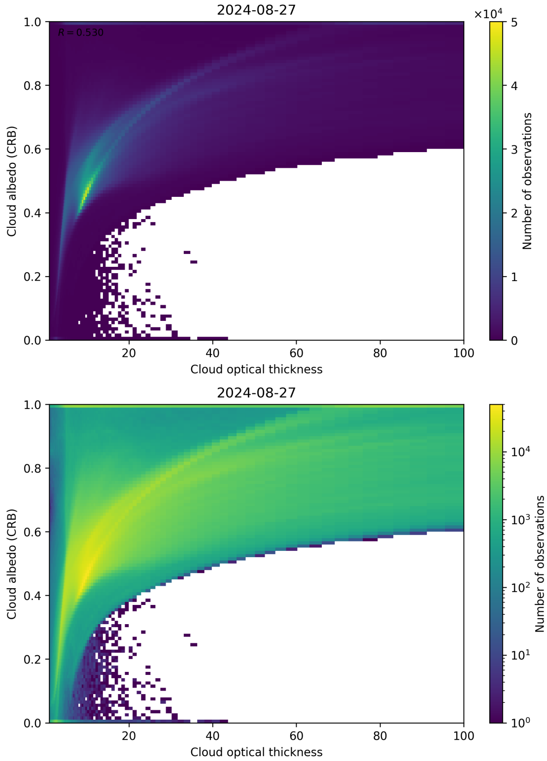
Figure 82: Scatter density plot of “Cloud optical thickness” against “Cloud albedo (CRB)” for 2024-08-27 to 2024-08-28.
