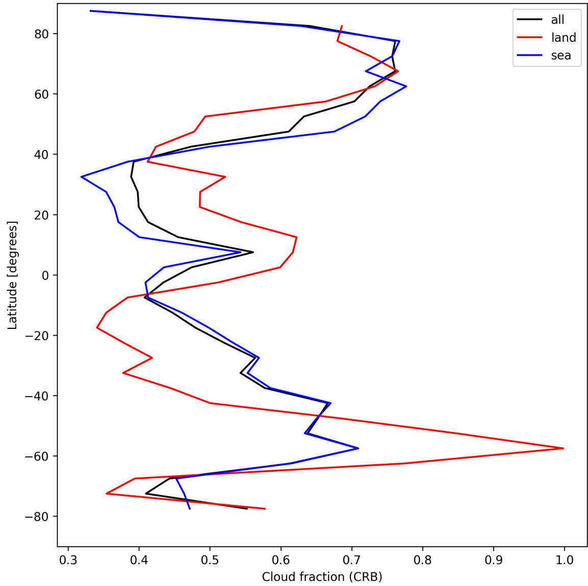
Figure 26: Zonal average of “Cloud fraction (CRB)” for 2024-08-27 to 2024-08-28.
