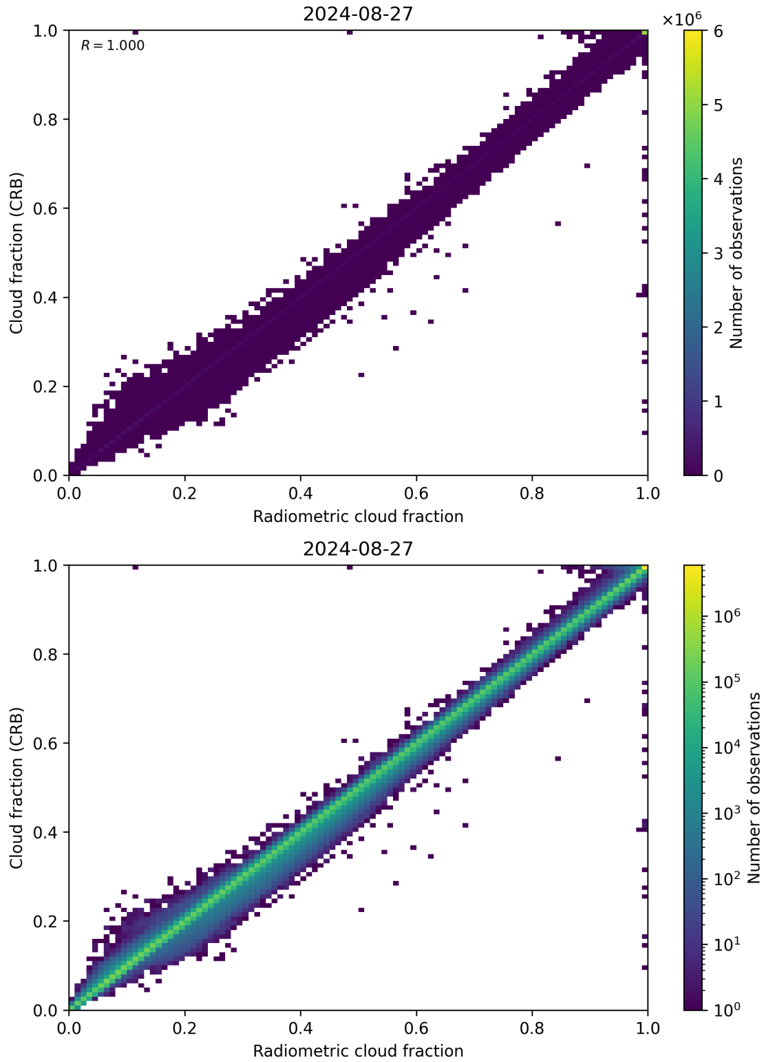
Figure 73: Scatter density plot of “Radiometric cloud fraction” against “Cloud fraction (CRB)” for 2024-08-27 to 2024-08-28.
