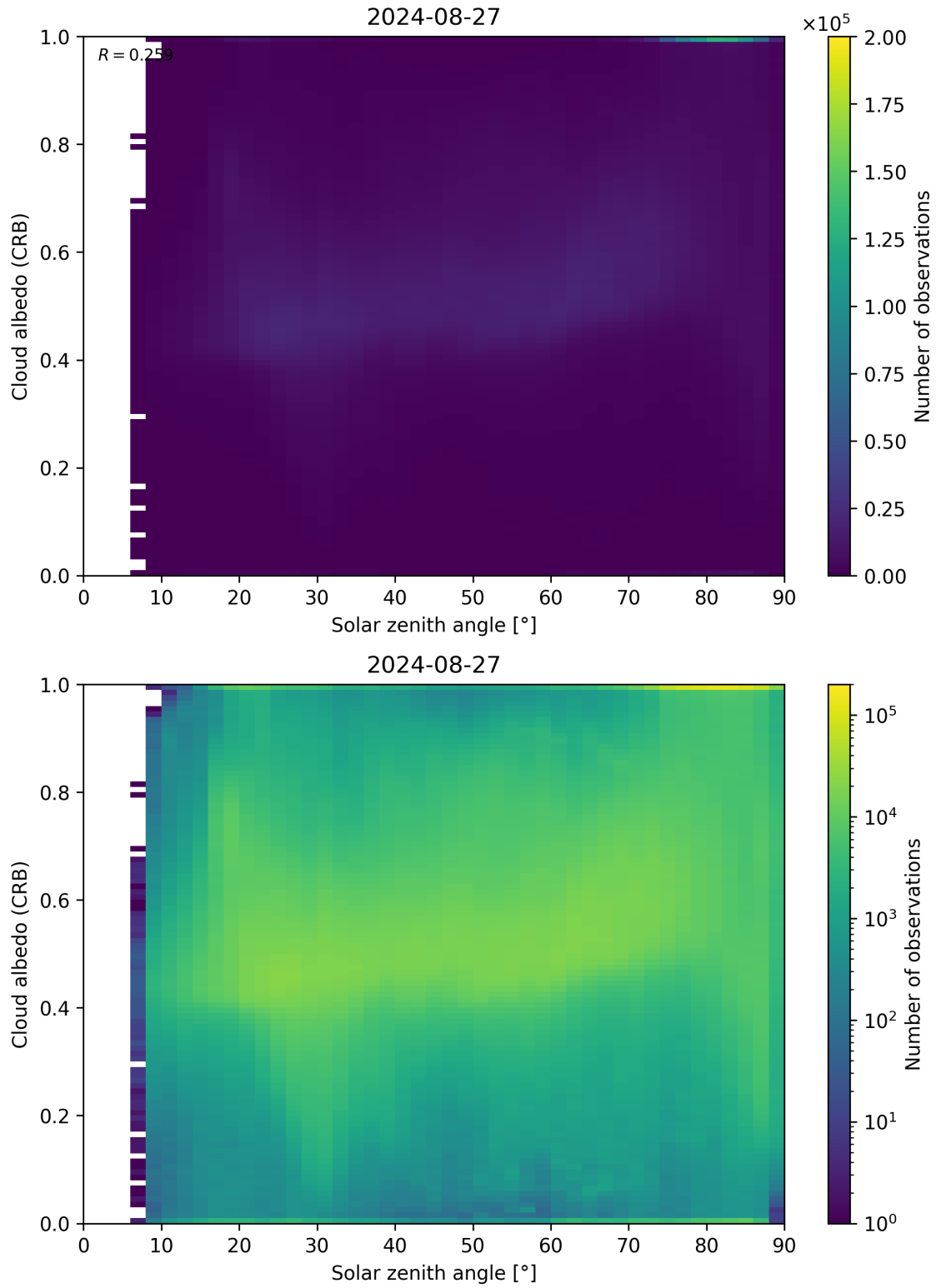
Figure 98: Scatter density plot of “Solar zenith angle” against “Cloud albedo (CRB)” for 2024-08-27 to 2024-08-28.
