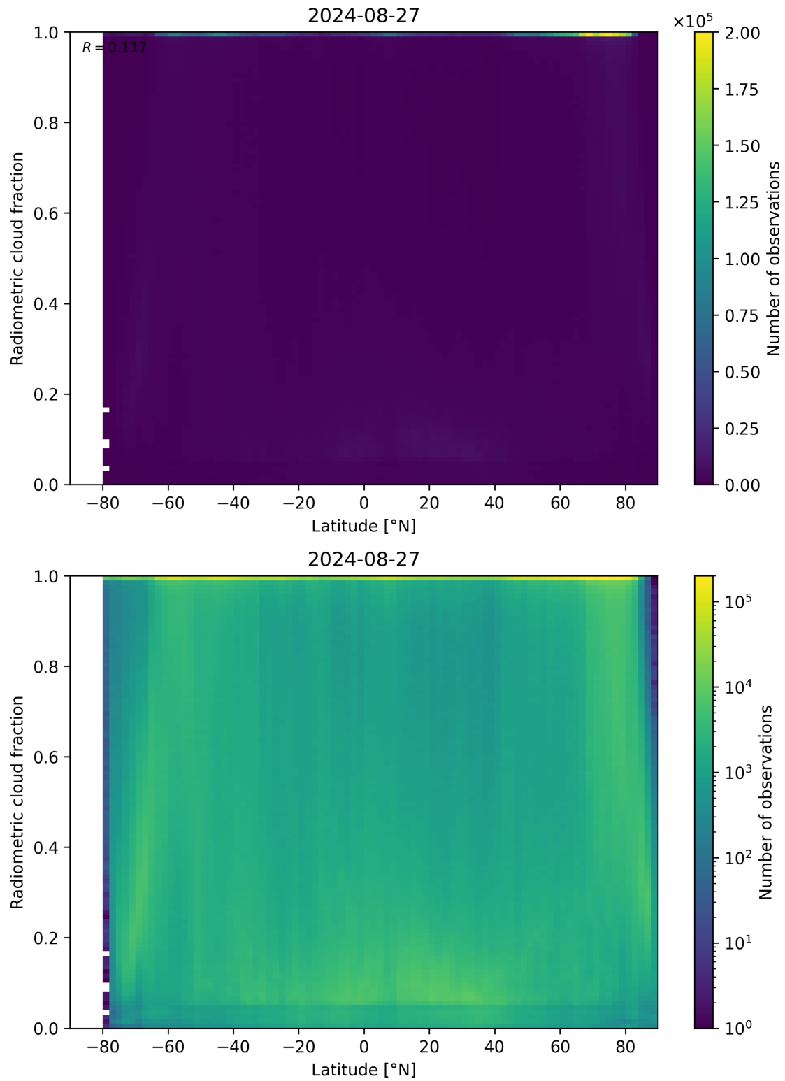
Figure 92: Scatter density plot of “Latitude” against “Radiometric cloud fraction” for 2024-08-27 to 2024-08-28.
