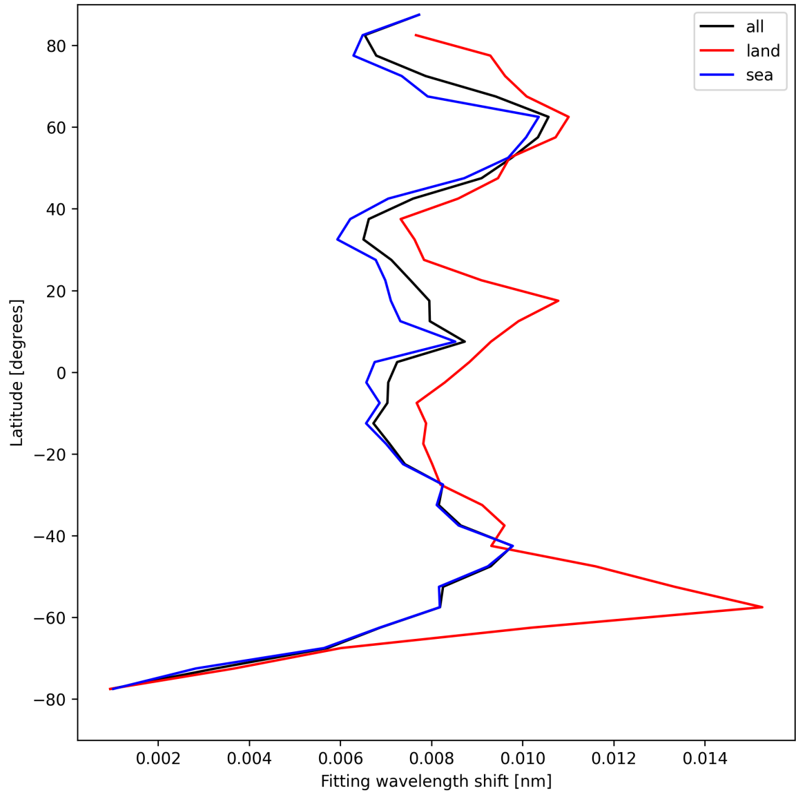
Figure 33: Zonal average of “Fitting wavelength shift” for 2024-08-27 to 2024-08-28.
