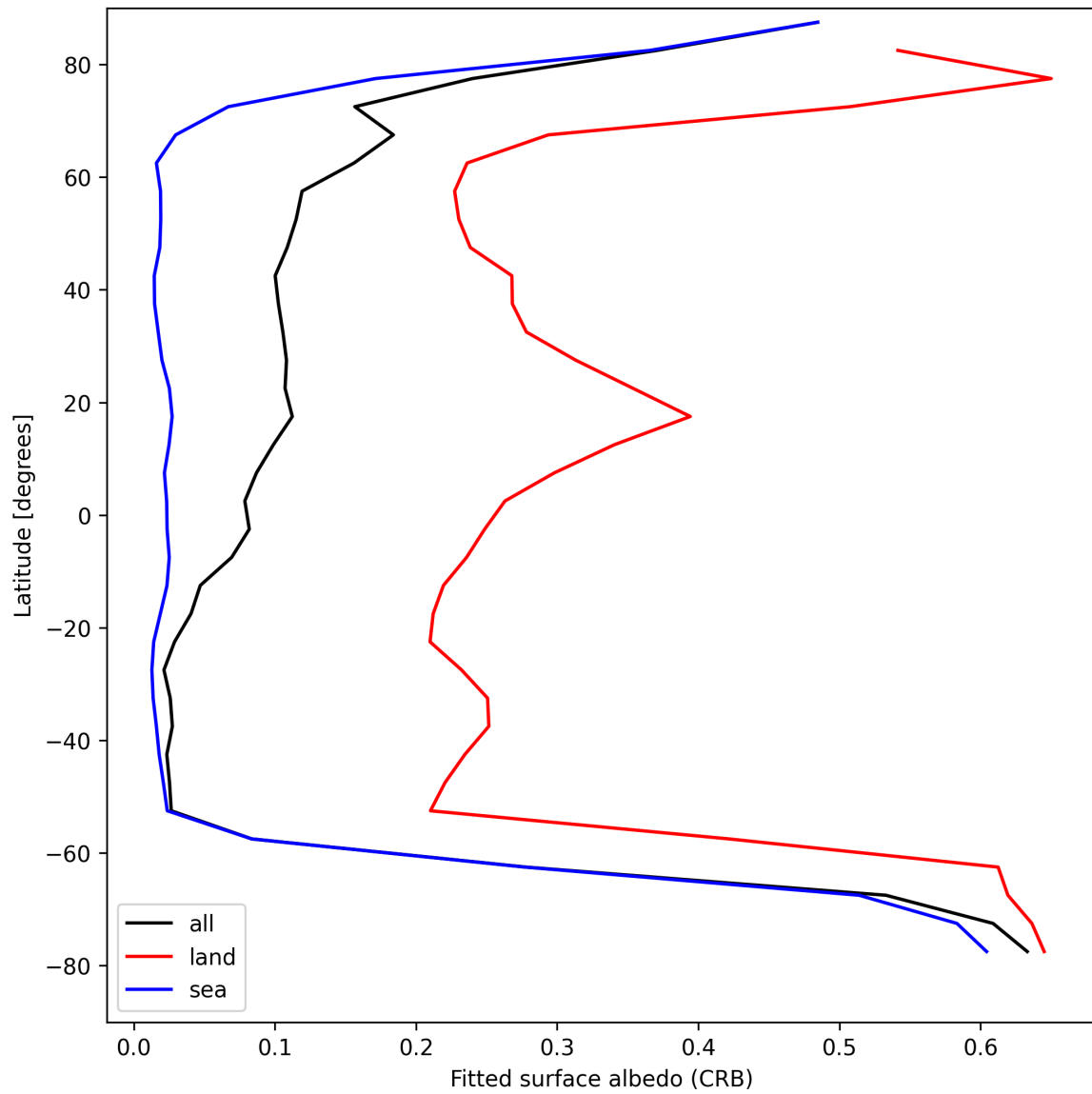
Figure 30: Zonal average of “Fitted surface albedo (CRB)” for 2024-08-27 to 2024-08-28.
