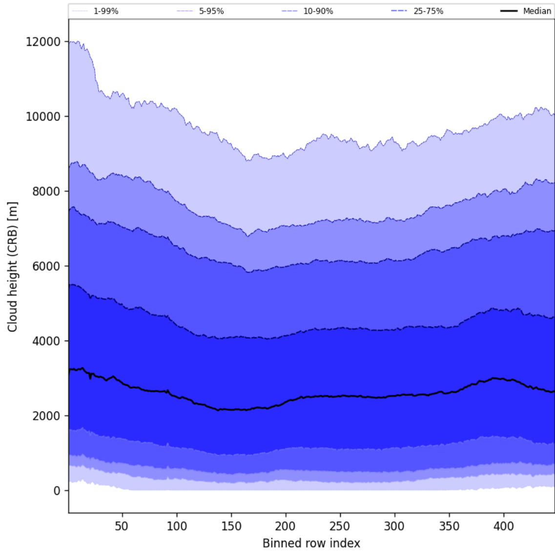
Figure 59: Along track statistics of “Cloud height (CRB)” for 2024-08-27 to 2024-08-28
