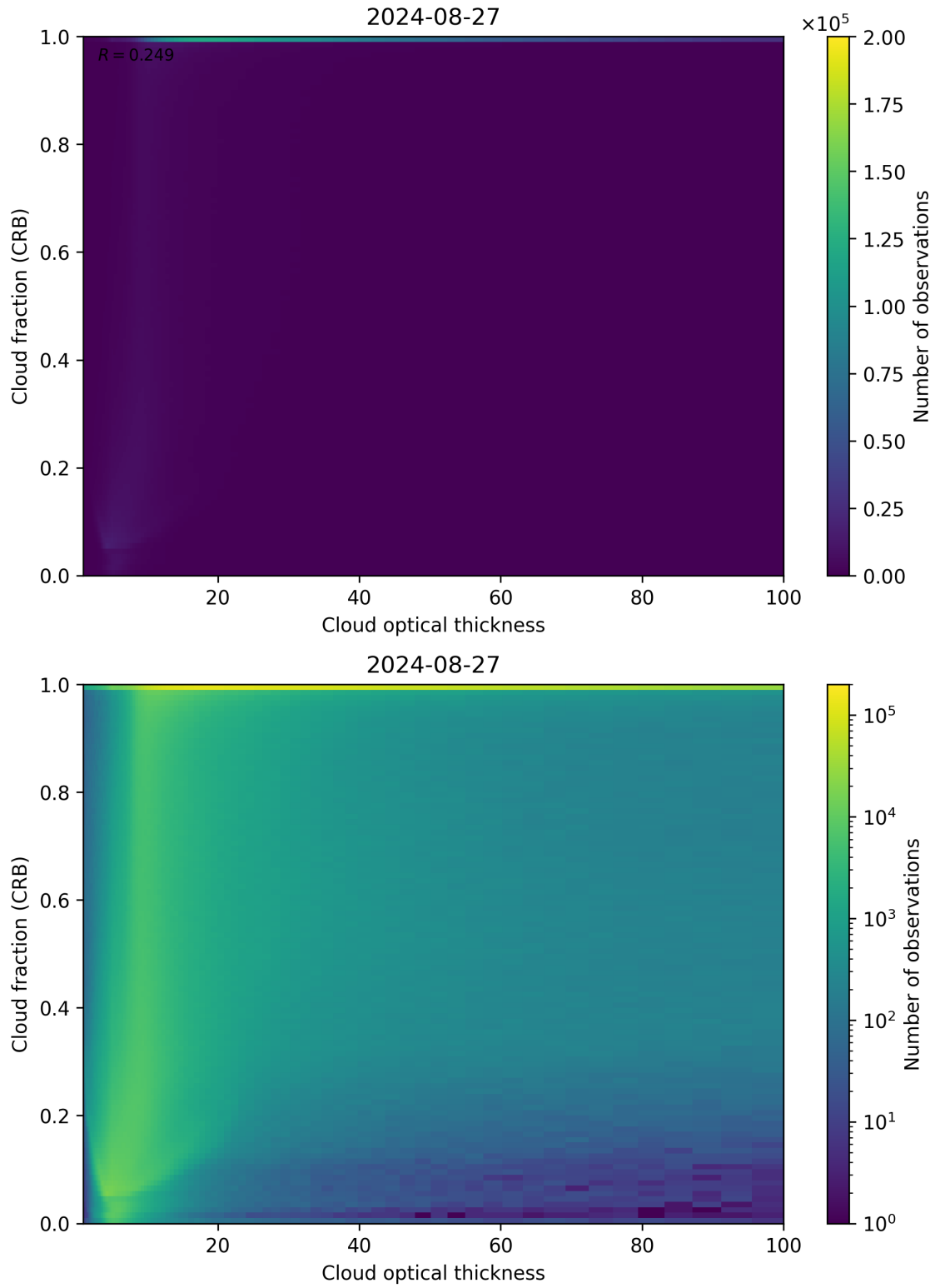
Figure 84: Scatter density plot of “Cloud optical thickness” against “Cloud fraction (CRB)” for 2024-08-27 to 2024-08-28.
