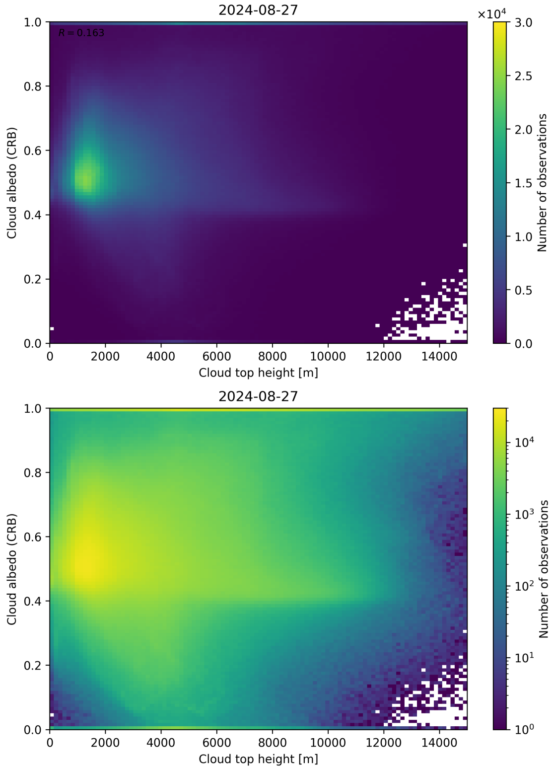
Figure 86: Scatter density plot of “Cloud top height” against “Cloud albedo (CRB)” for 2024-08-27 to 2024-08-28.
