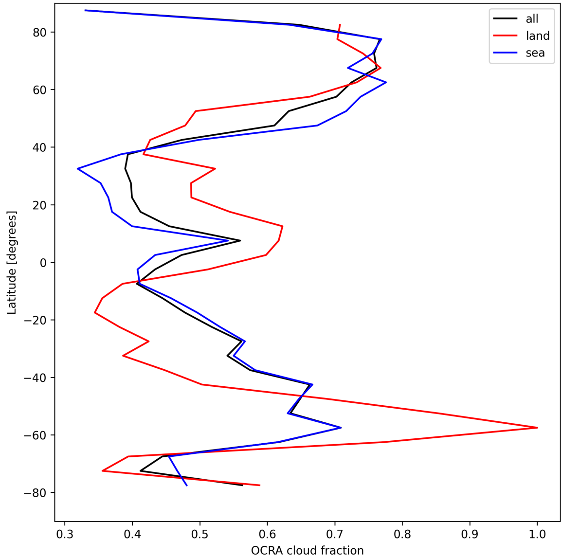
Figure 34: Zonal average of “OCRA cloud fraction” for 2024-08-27 to 2024-08-28.
