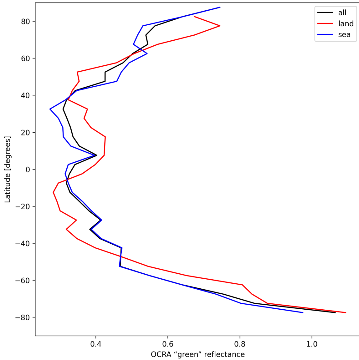
Figure 36: Zonal average of “OCRA “green” reflectance” for 2024-08-27 to 2024-08-28.
