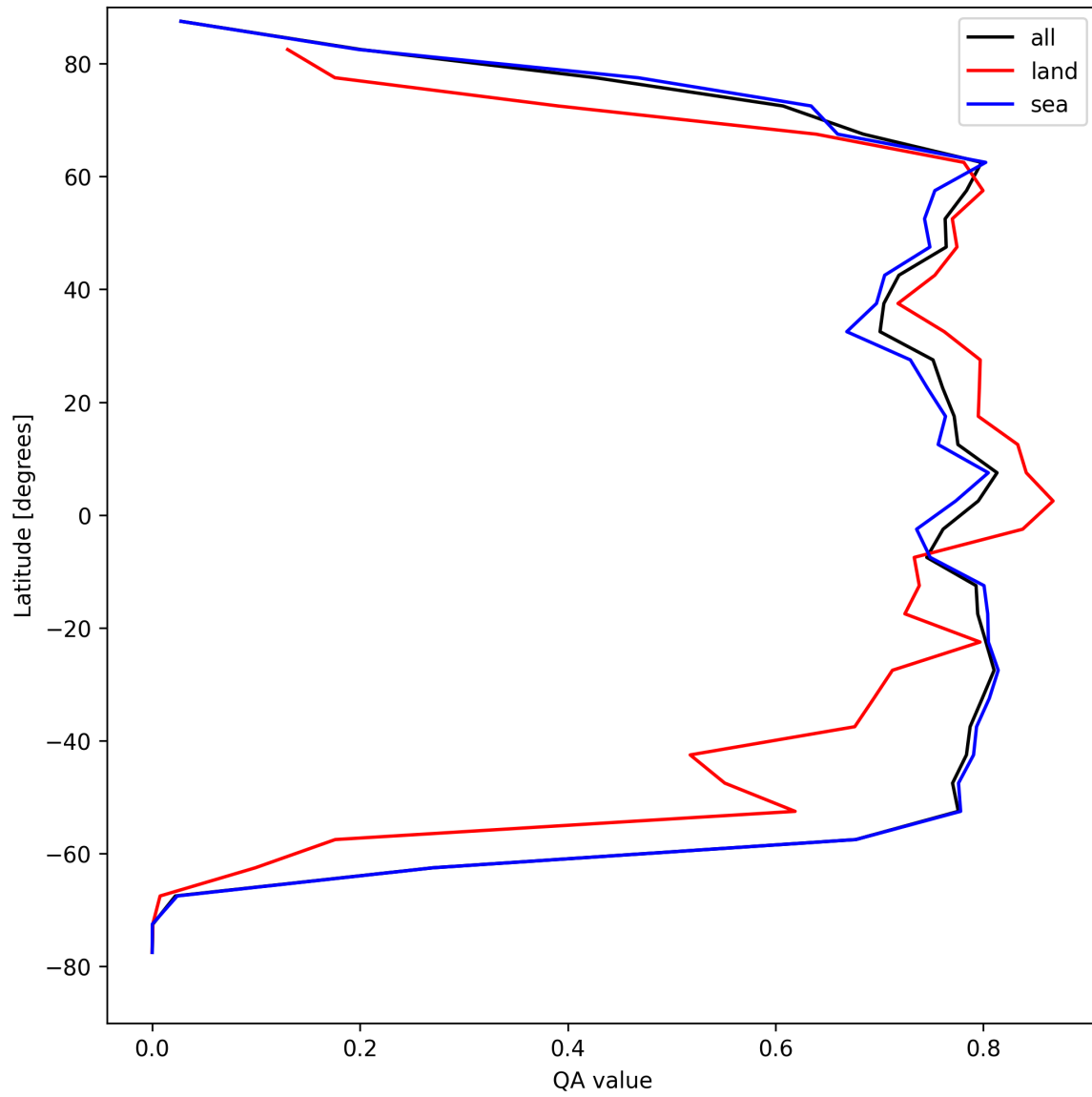
Figure 22: Zonal average of “QA value” for 2024-08-27 to 2024-08-28.
