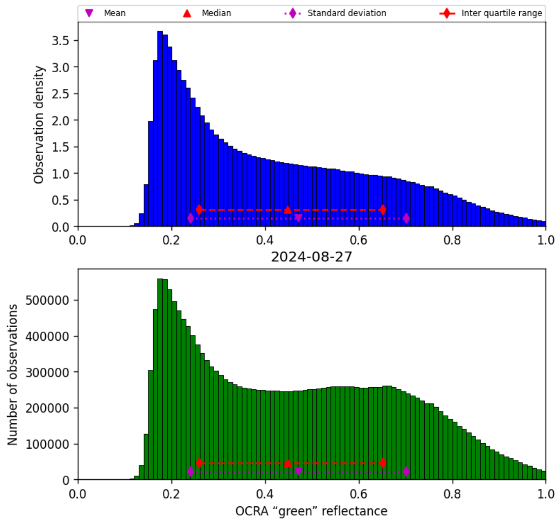
Figure 52: Histogram of “OCRA “green” reflectance” for 2024-08-27 to 2024-08-28
