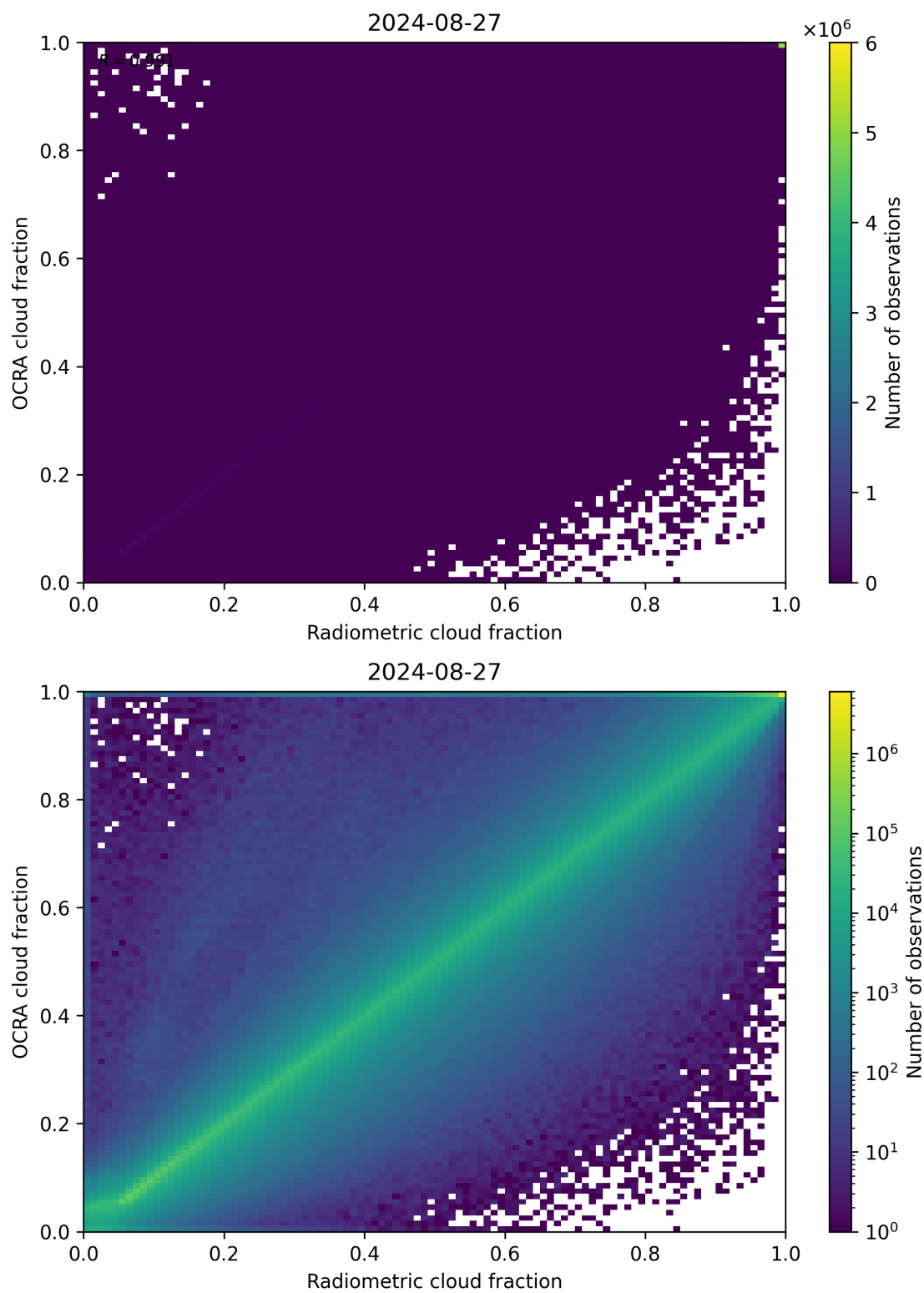
Figure 72: Scatter density plot of “Radiometric cloud fraction” against “OCRA cloud fraction” for 2024-08-27 to 2024-08-28.
