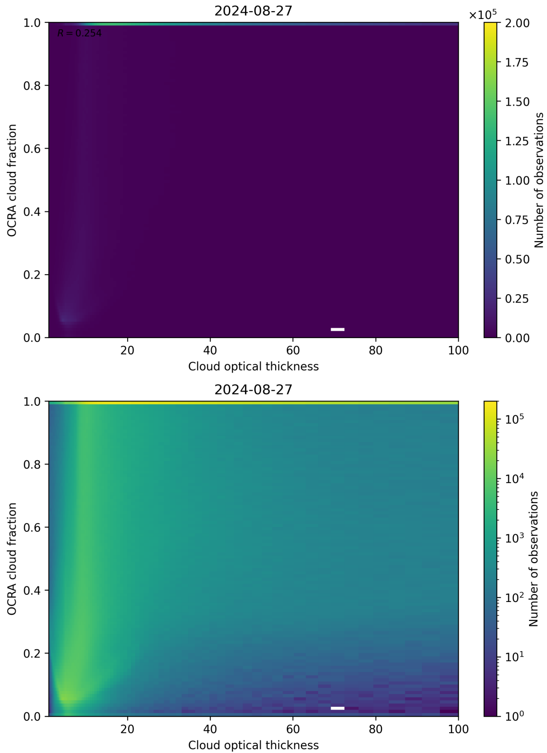
Figure 83: Scatter density plot of “Cloud optical thickness” against “OCRA cloud fraction” for 2024-08-27 to 2024-08-28.
