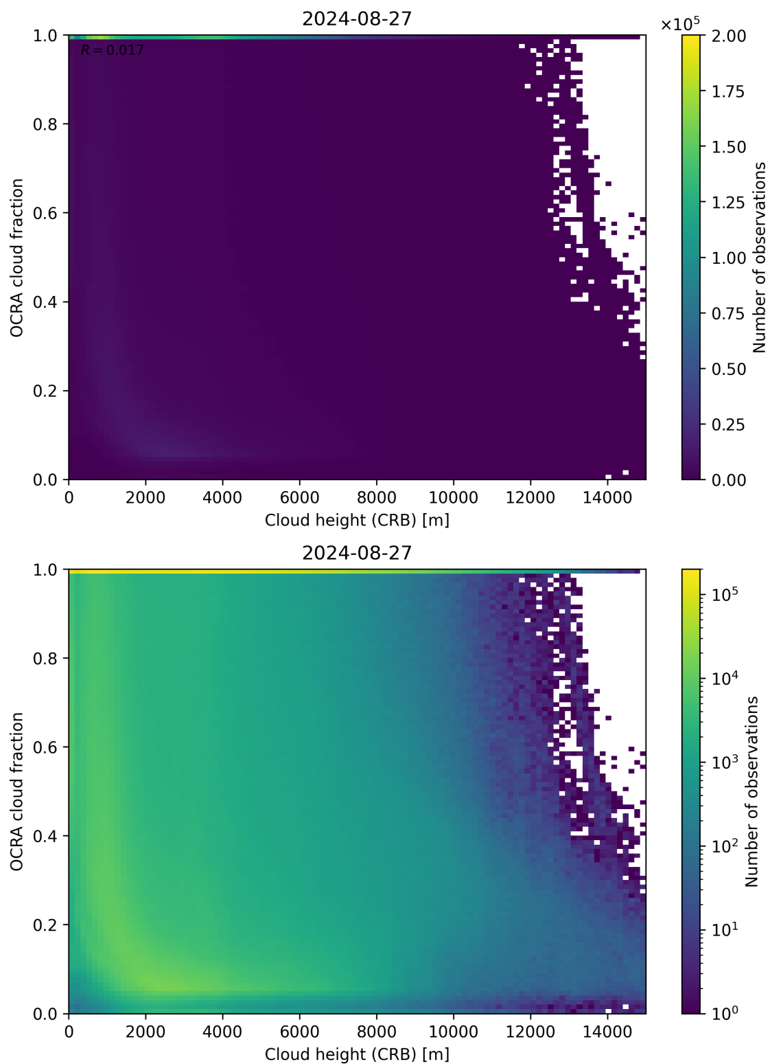
Figure 81: Scatter density plot of “Cloud height (CRB)” against “OCRA cloud fraction” for 2024-08-27 to 2024-08-28.
