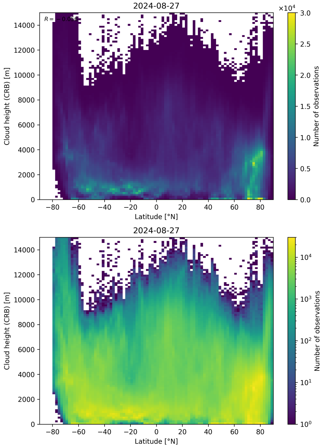
Figure 95: Scatter density plot of “Latitude” against “Cloud height (CRB)” for 2024-08-27 to 2024-08-28.
