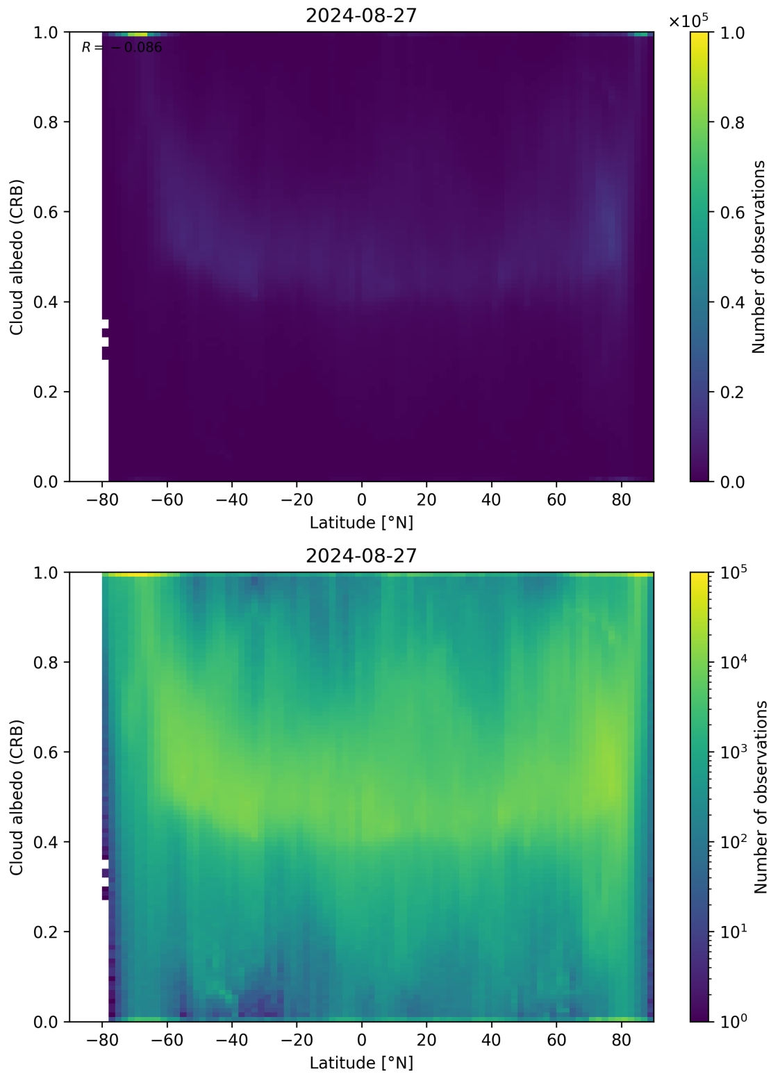
Figure 91: Scatter density plot of “Latitude” against “Cloud albedo (CRB)” for 2024-08-27 to 2024-08-28.
