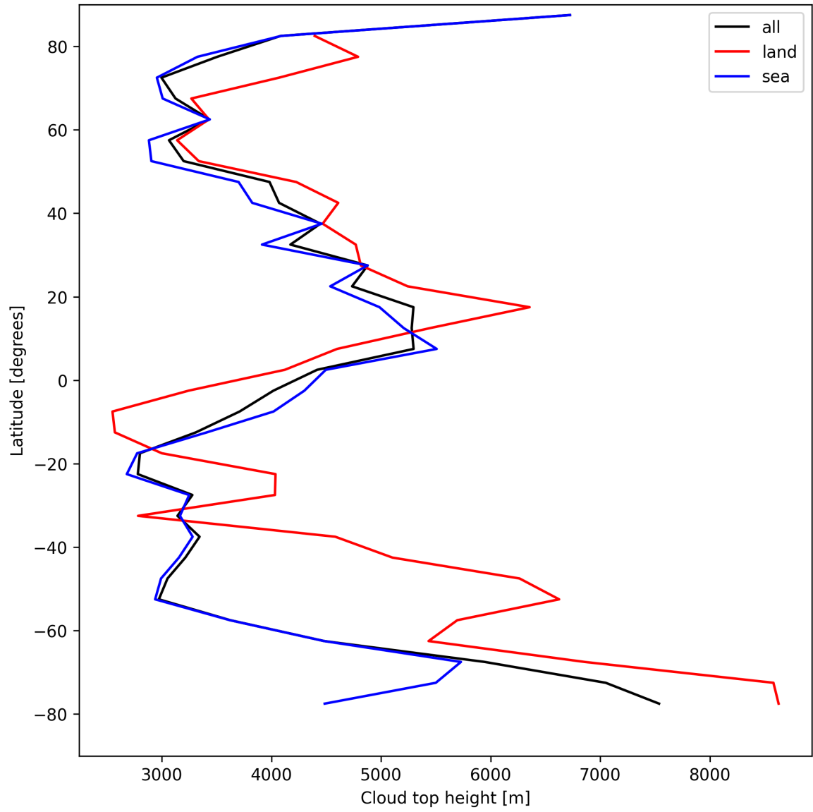
Figure 24: Zonal average of “Cloud top height” for 2024-08-27 to 2024-08-28.
