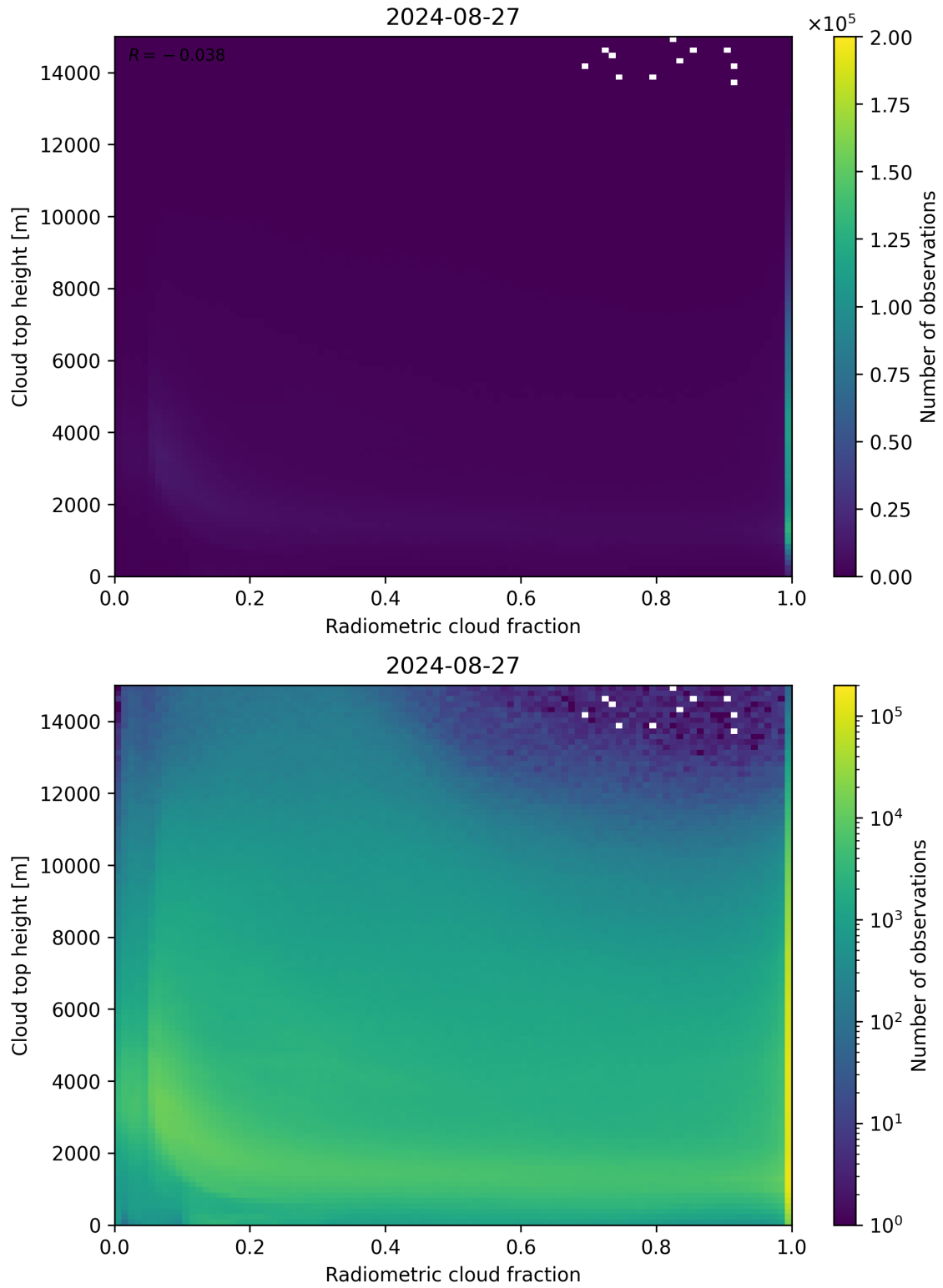
Figure 76: Scatter density plot of “Radiometric cloud fraction” against “Cloud top height” for 2024-08-27 to 2024-08-28.
