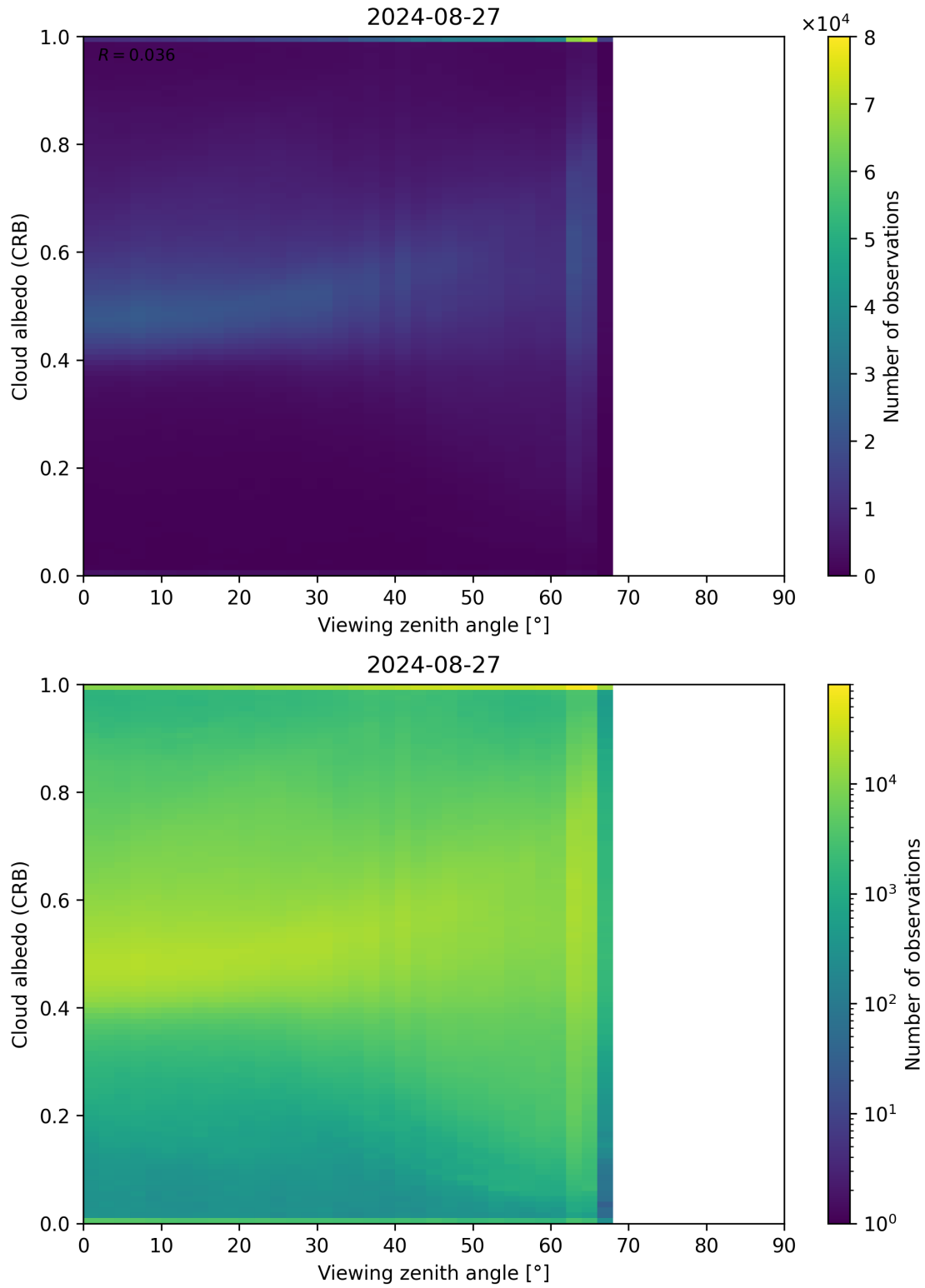
Figure 106: Scatter density plot of “Viewing zenith angle” against “Cloud albedo (CRB)” for 2024-08-27 to 2024-08-28.
