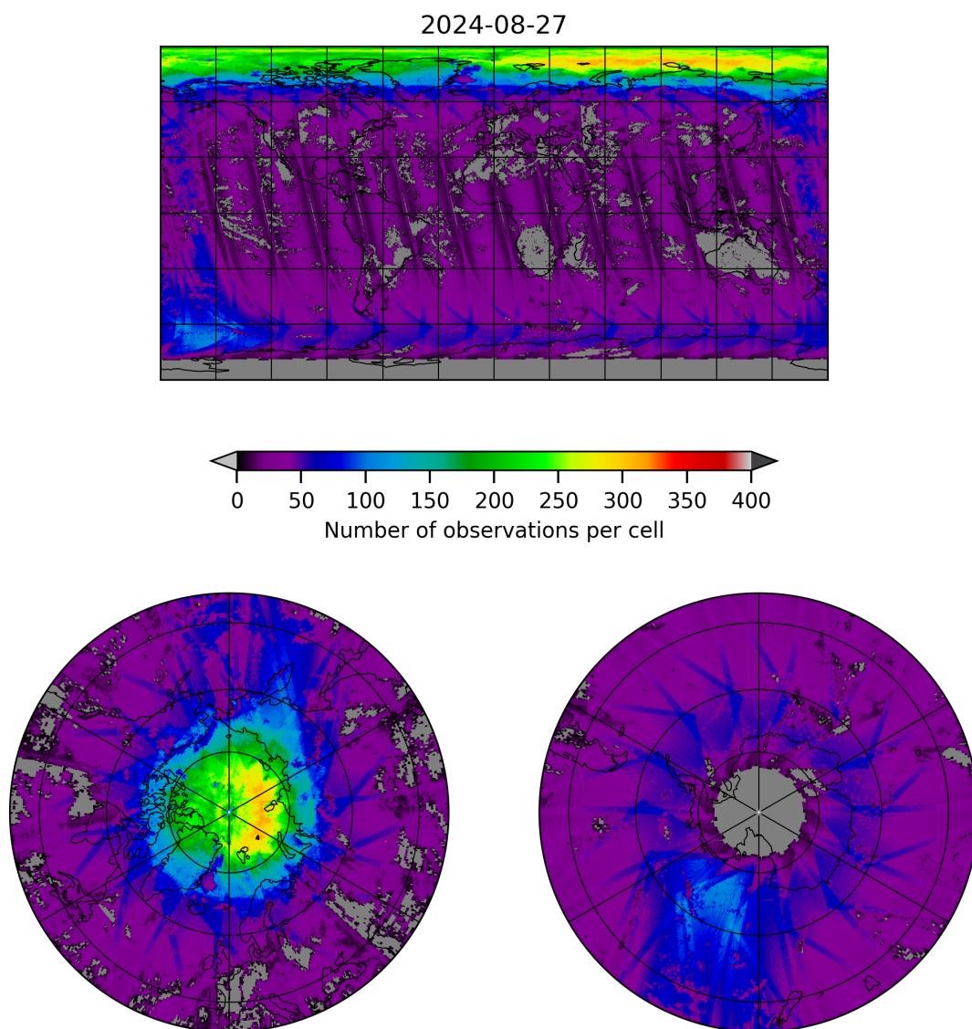
Figure 21: Map of the number of observations for 2024-08-27 to 2024-08-28
