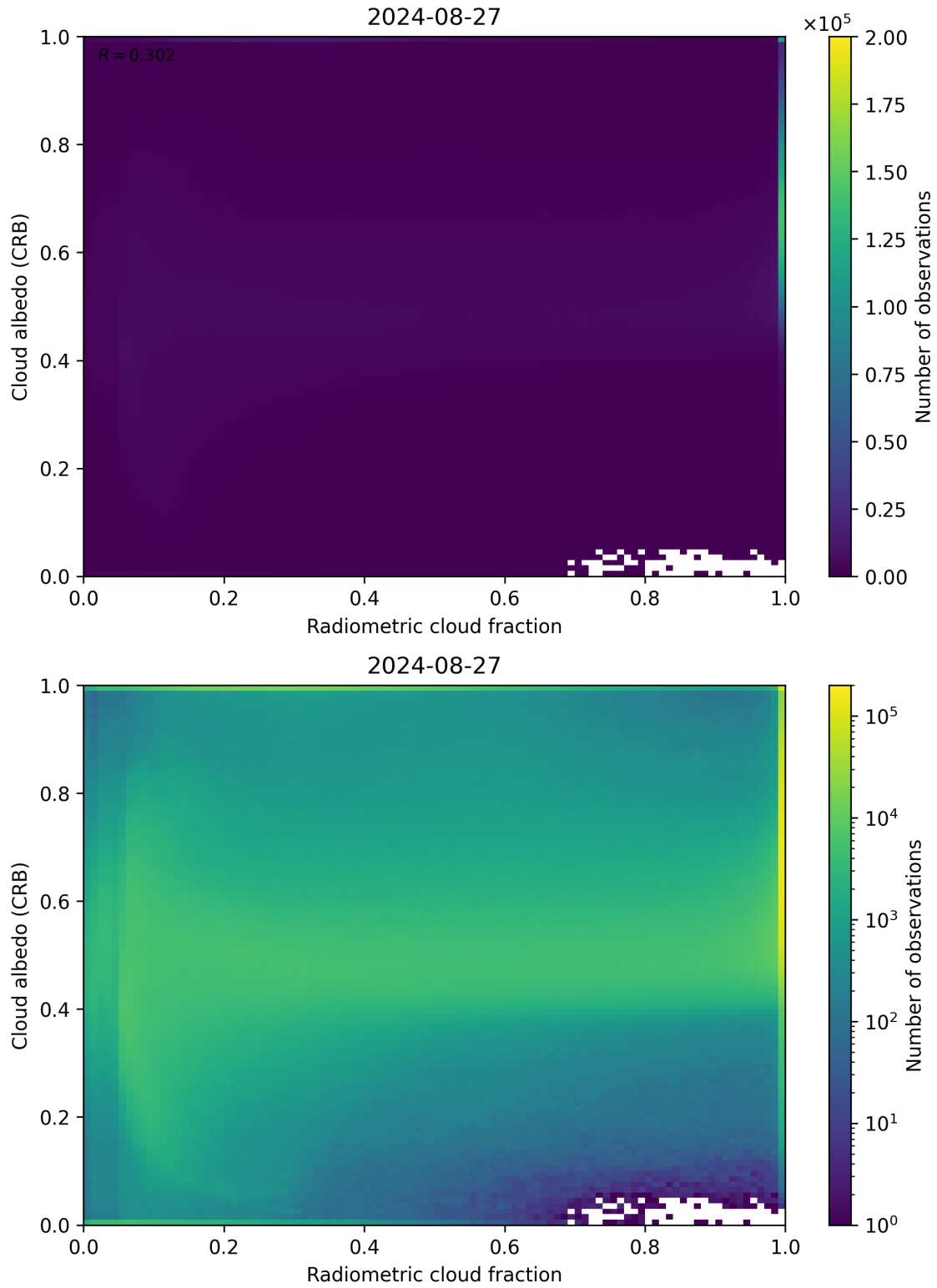
Figure 71: Scatter density plot of “Radiometric cloud fraction” against “Cloud albedo (CRB)” for 2024-08-27 to 2024-08-28.
