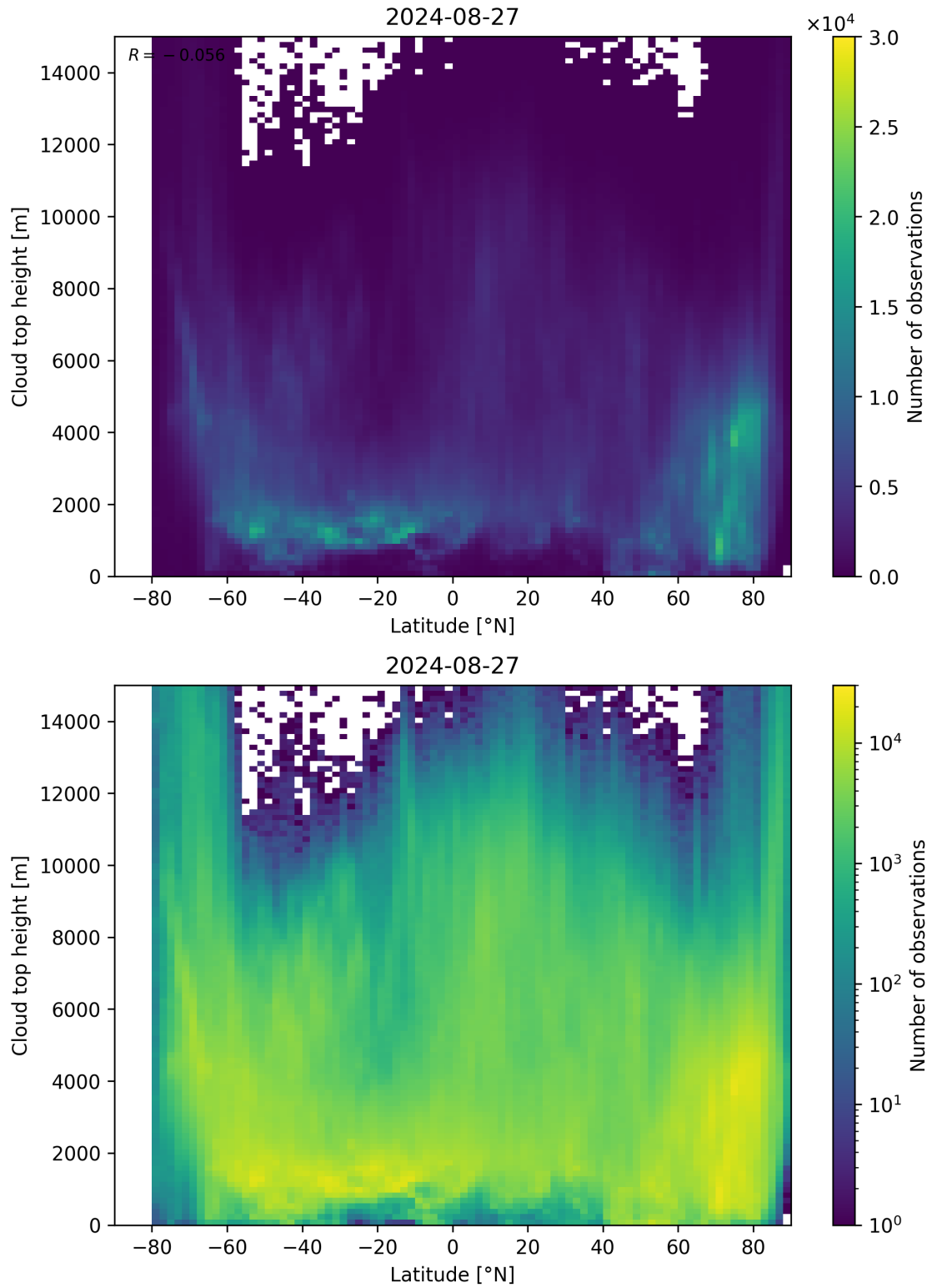
Figure 97: Scatter density plot of “Latitude” against “Cloud top height” for 2024-08-27 to 2024-08-28.
