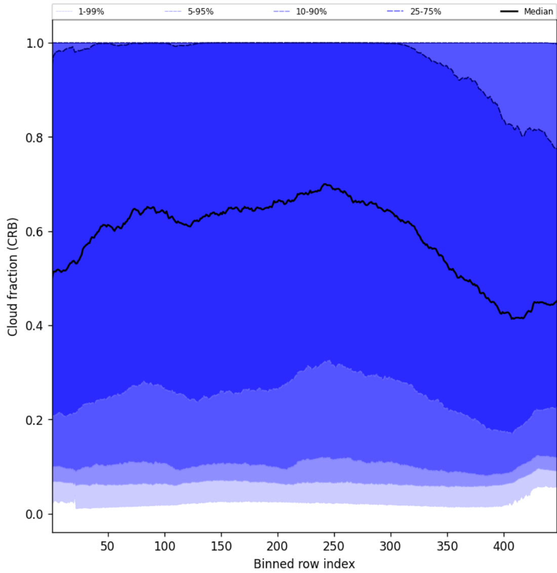
Figure 58: Along track statistics of “Cloud fraction (CRB)” for 2024-08-27 to 2024-08-28
