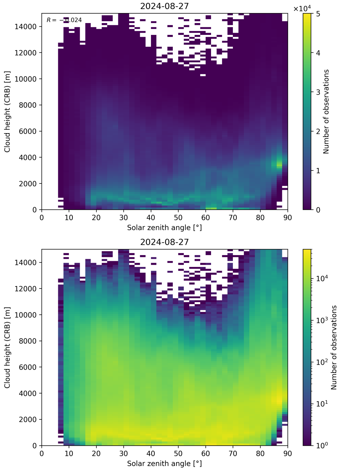
Figure 102: Scatter density plot of “Solar zenith angle” against “Cloud height (CRB)” for 2024-08-27 to 2024-08-28.
