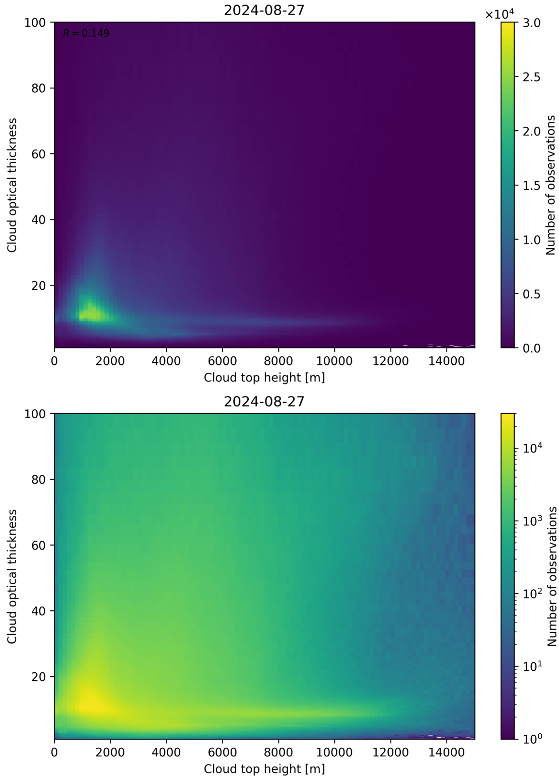
Figure 90: Scatter density plot of “Cloud top height” against “Cloud optical thickness” for 2024-08-27 to 2024-08-28.
