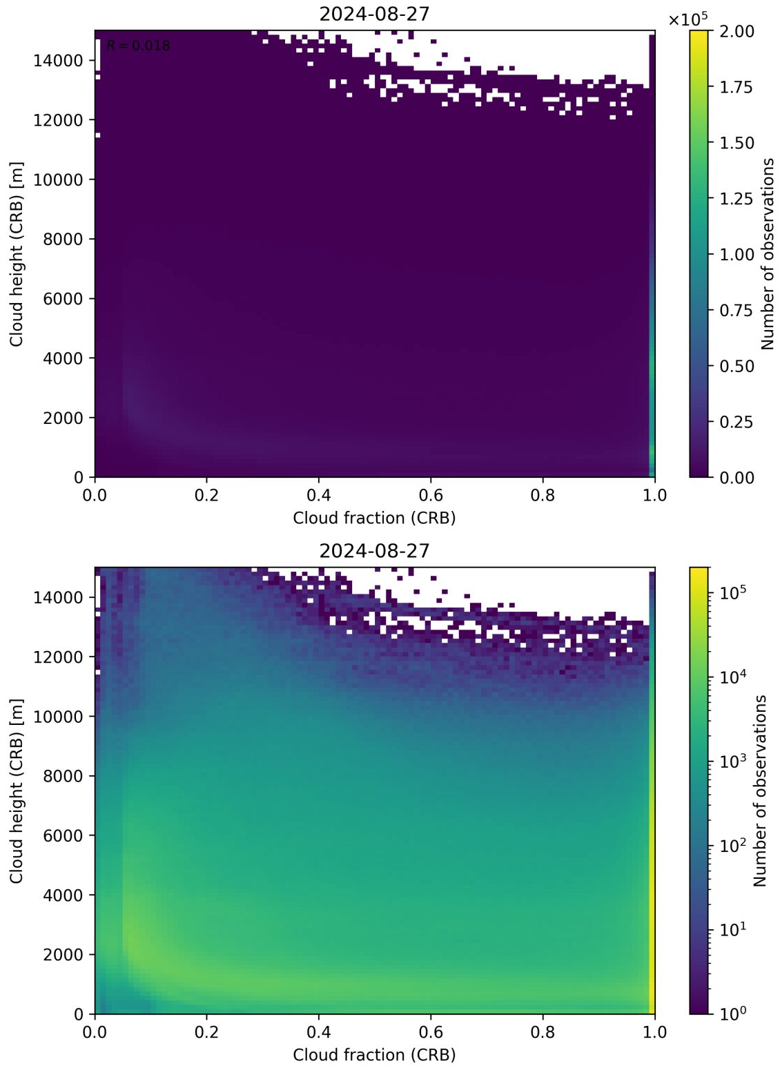
Figure 79: Scatter density plot of “Cloud fraction (CRB)” against “Cloud height (CRB)” for 2024-08-27 to 2024-08-28.
