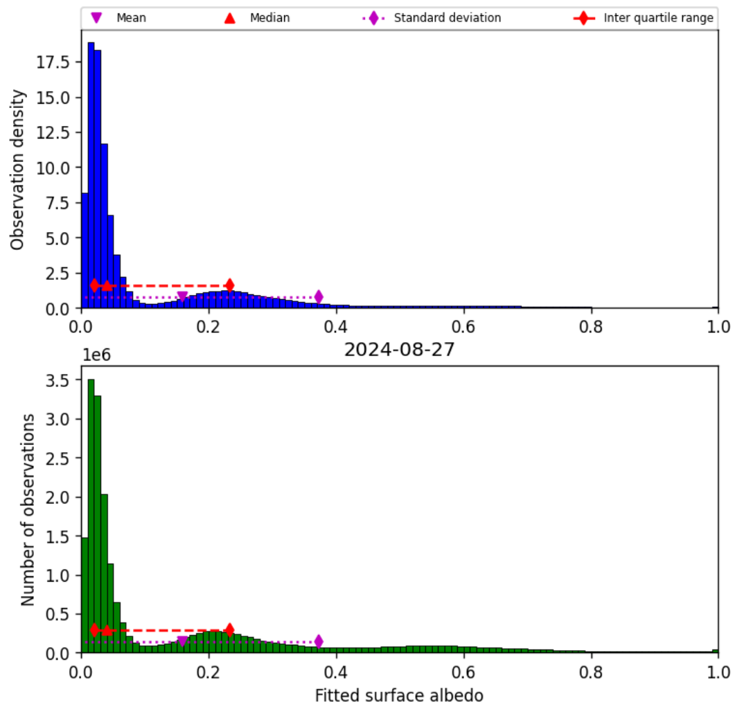
Figure 45: Histogram of “Fitted surface albedo” for 2024-08-27 to 2024-08-28
