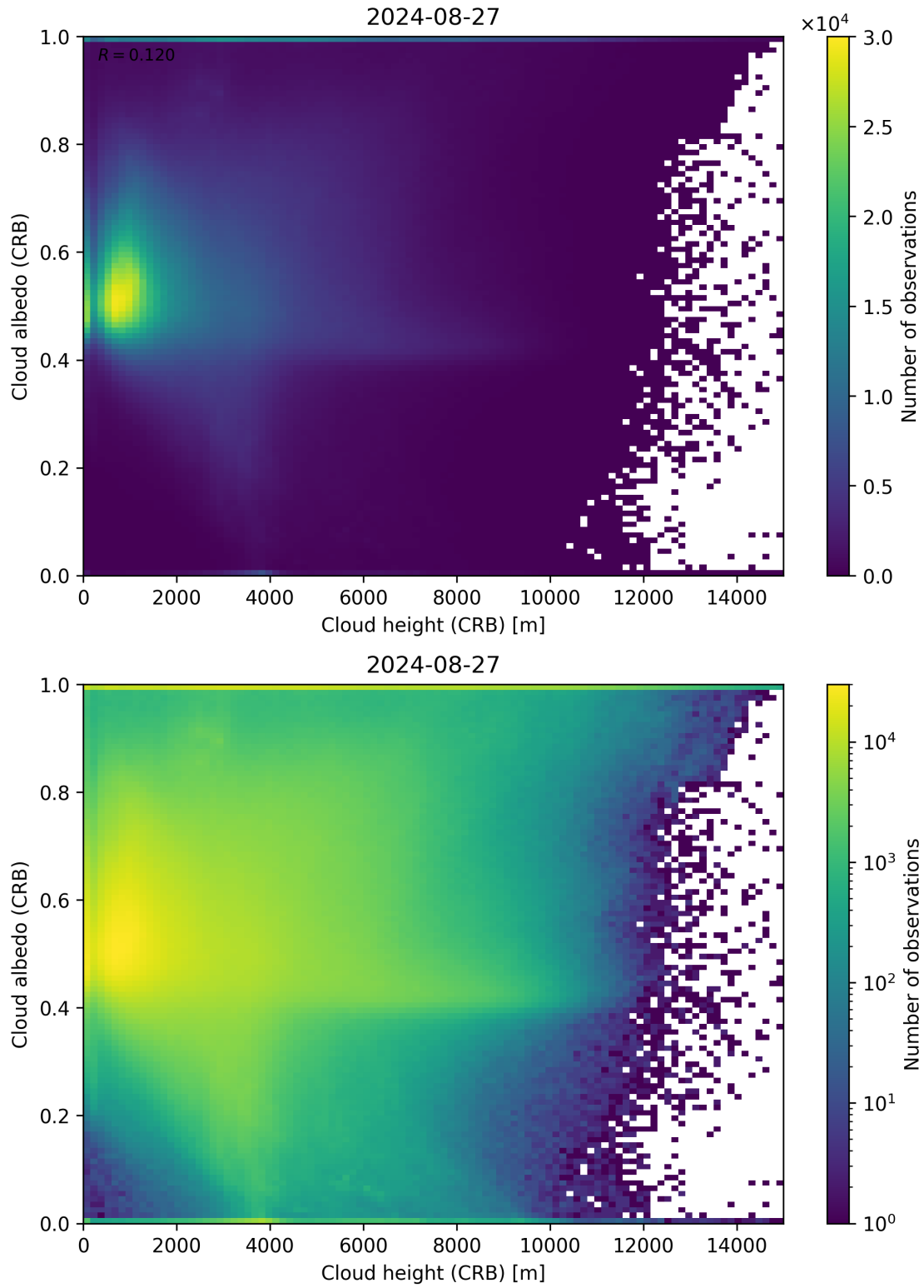
Figure 80: Scatter density plot of “Cloud height (CRB)” against “Cloud albedo (CRB)” for 2024-08-27 to 2024-08-28.
