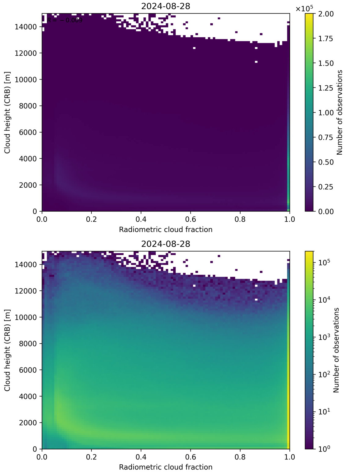
Figure 74: Scatter density plot of “Radiometric cloud fraction” against “Cloud height (CRB)” for 2024-08-27 to 2024-08-29.
