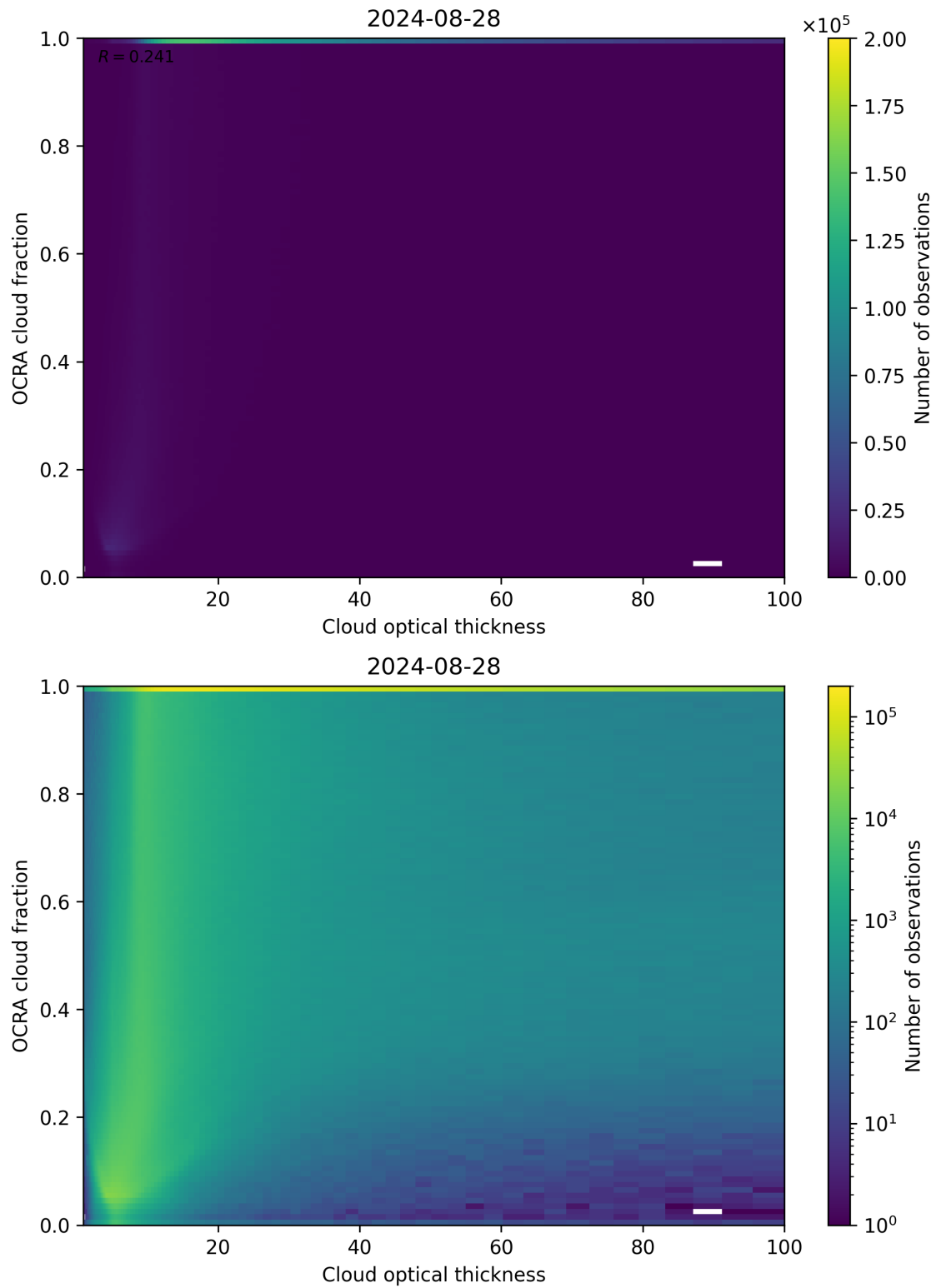
Figure 83: Scatter density plot of “Cloud optical thickness” against “OCRA cloud fraction” for 2024-08-27 to 2024-08-29.
