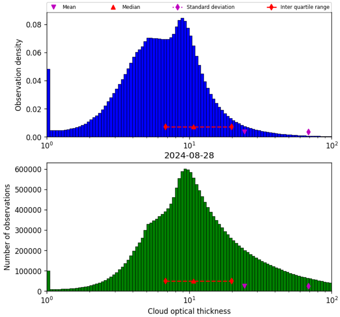
Figure 41: Histogram of “Cloud optical thickness” for 2024-08-27 to 2024-08-29
