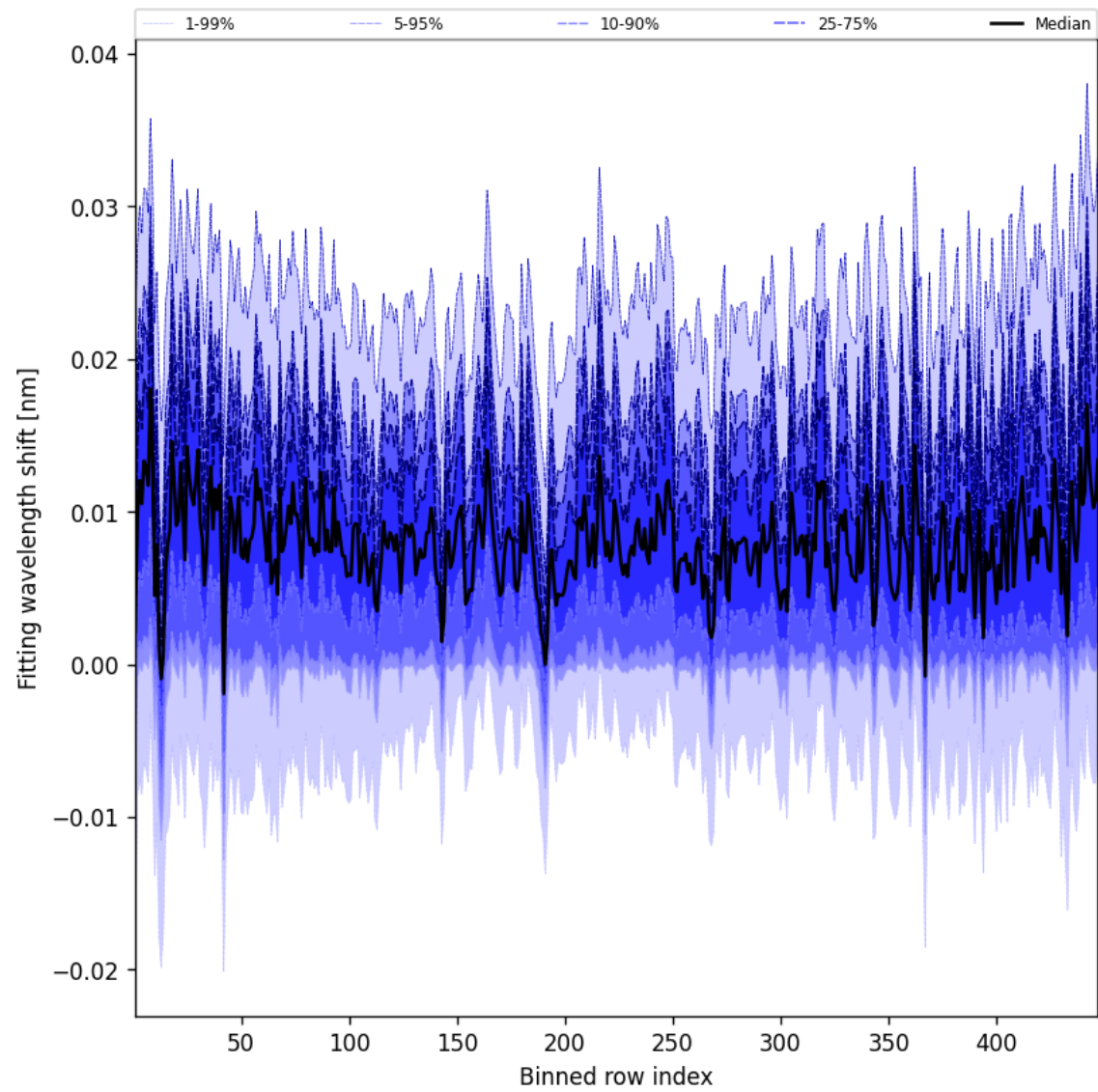
Figure 65: Along track statistics of “Fitting wavelength shift” for 2024-08-27 to 2024-08-29
