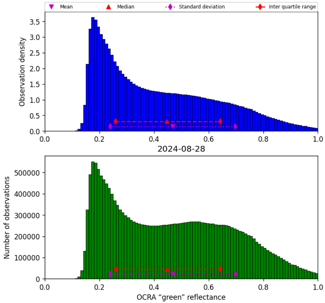
Figure 52: Histogram of “OCRA “green” reflectance” for 2024-08-27 to 2024-08-29
