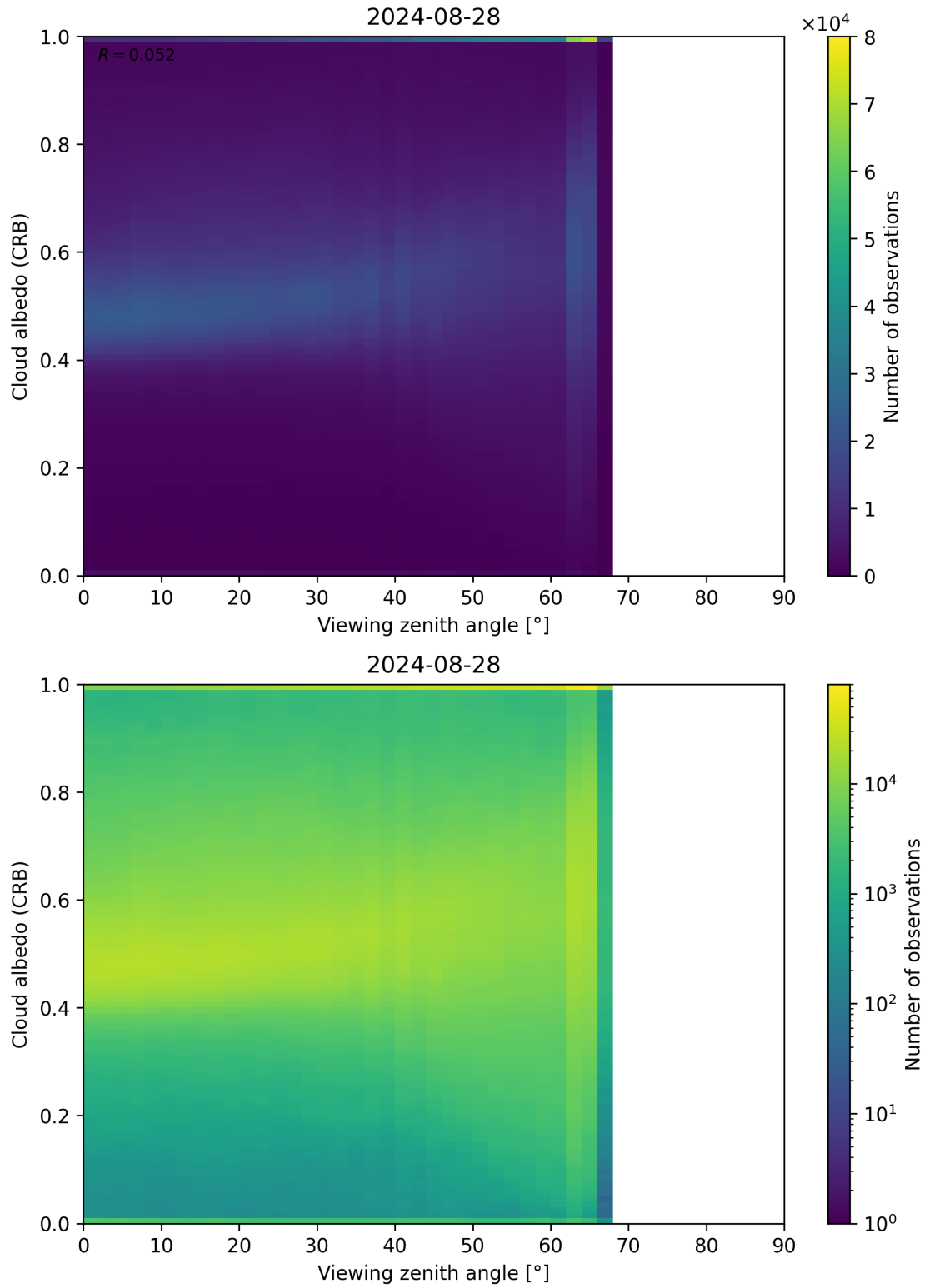
Figure 106: Scatter density plot of “Viewing zenith angle” against “Cloud albedo (CRB)” for 2024-08-27 to 2024-08-29.
