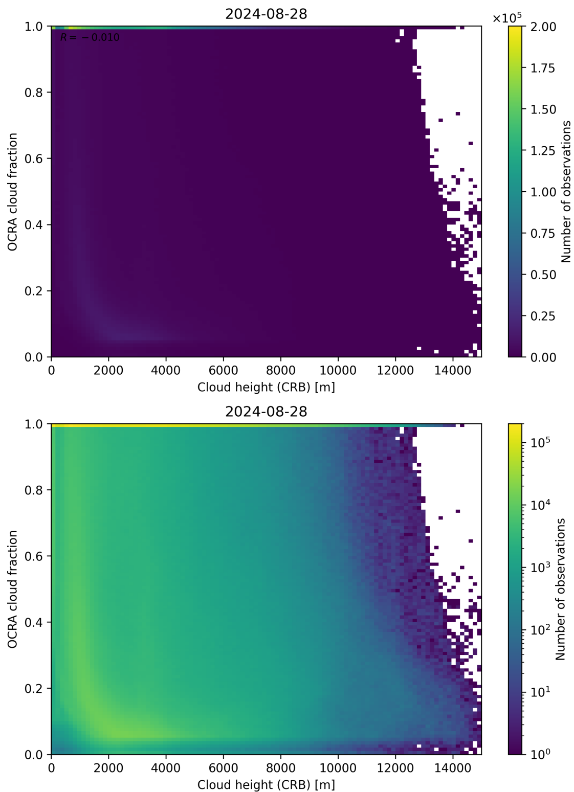
Figure 81: Scatter density plot of “Cloud height (CRB)” against “OCRA cloud fraction” for 2024-08-27 to 2024-08-29.
