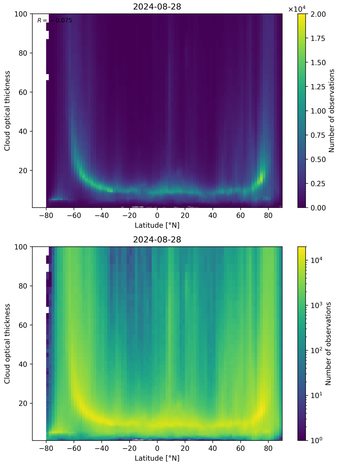
Figure 96: Scatter density plot of “Latitude” against “Cloud optical thickness” for 2024-08-27 to 2024-08-29.
