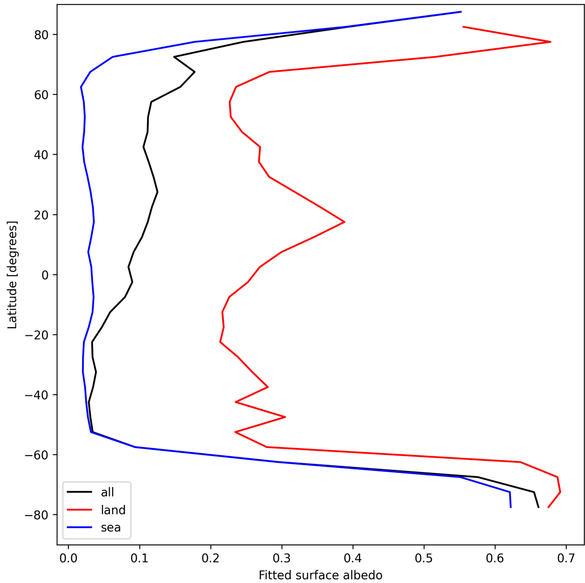
Figure 29: Zonal average of “Fitted surface albedo” for 2024-08-27 to 2024-08-29.
