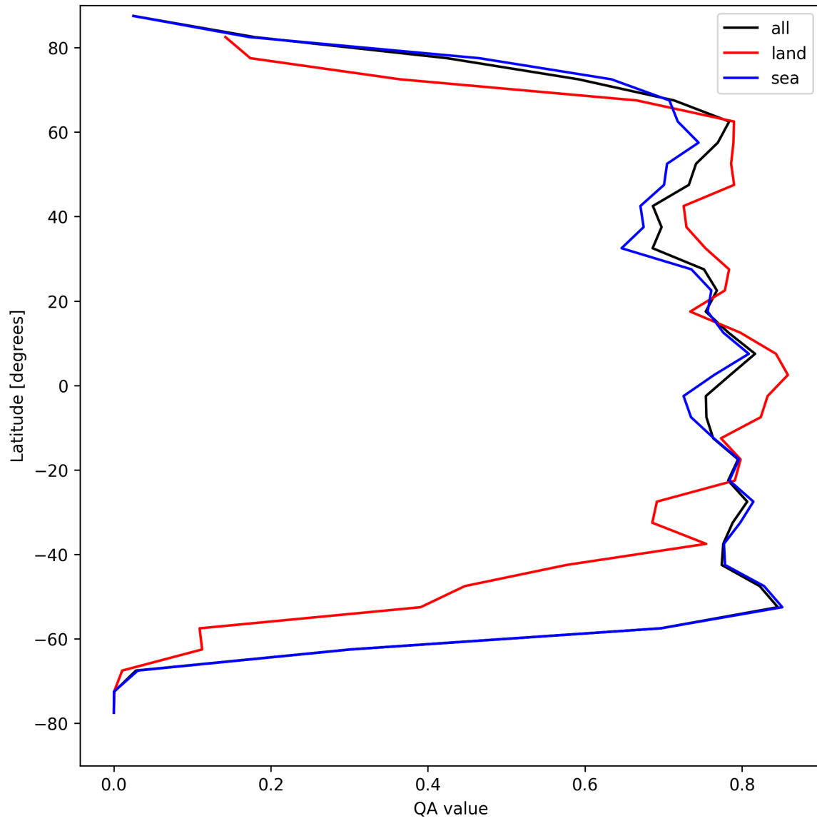
Figure 22: Zonal average of “QA value” for 2024-08-27 to 2024-08-29.
