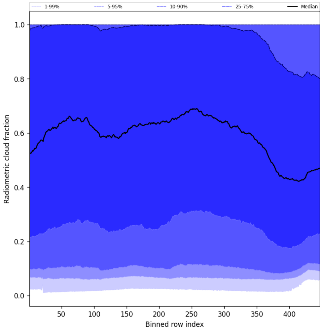
Figure 55: Along track statistics of “Radiometric cloud fraction” for 2024-08-27 to 2024-08-29
