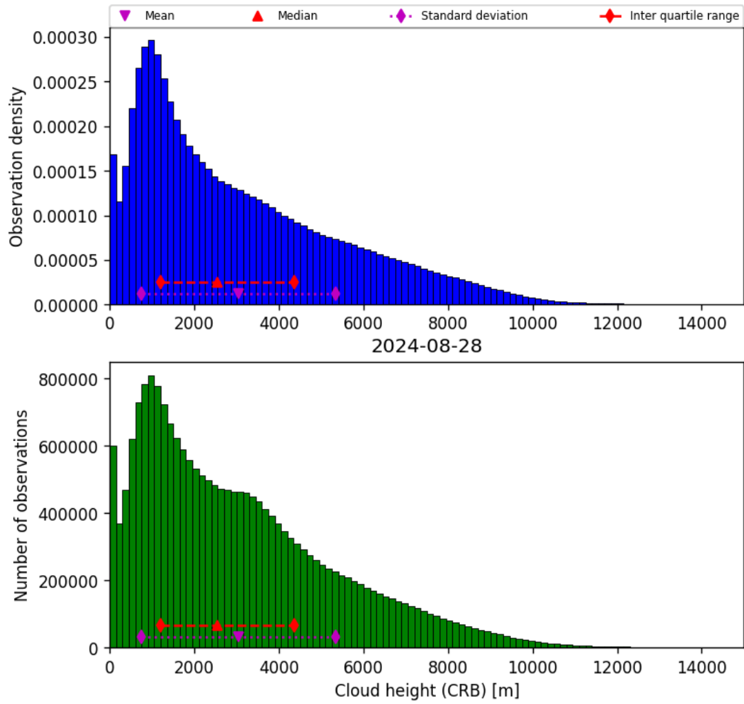
Figure 43: Histogram of “Cloud height (CRB)” for 2024-08-27 to 2024-08-29
