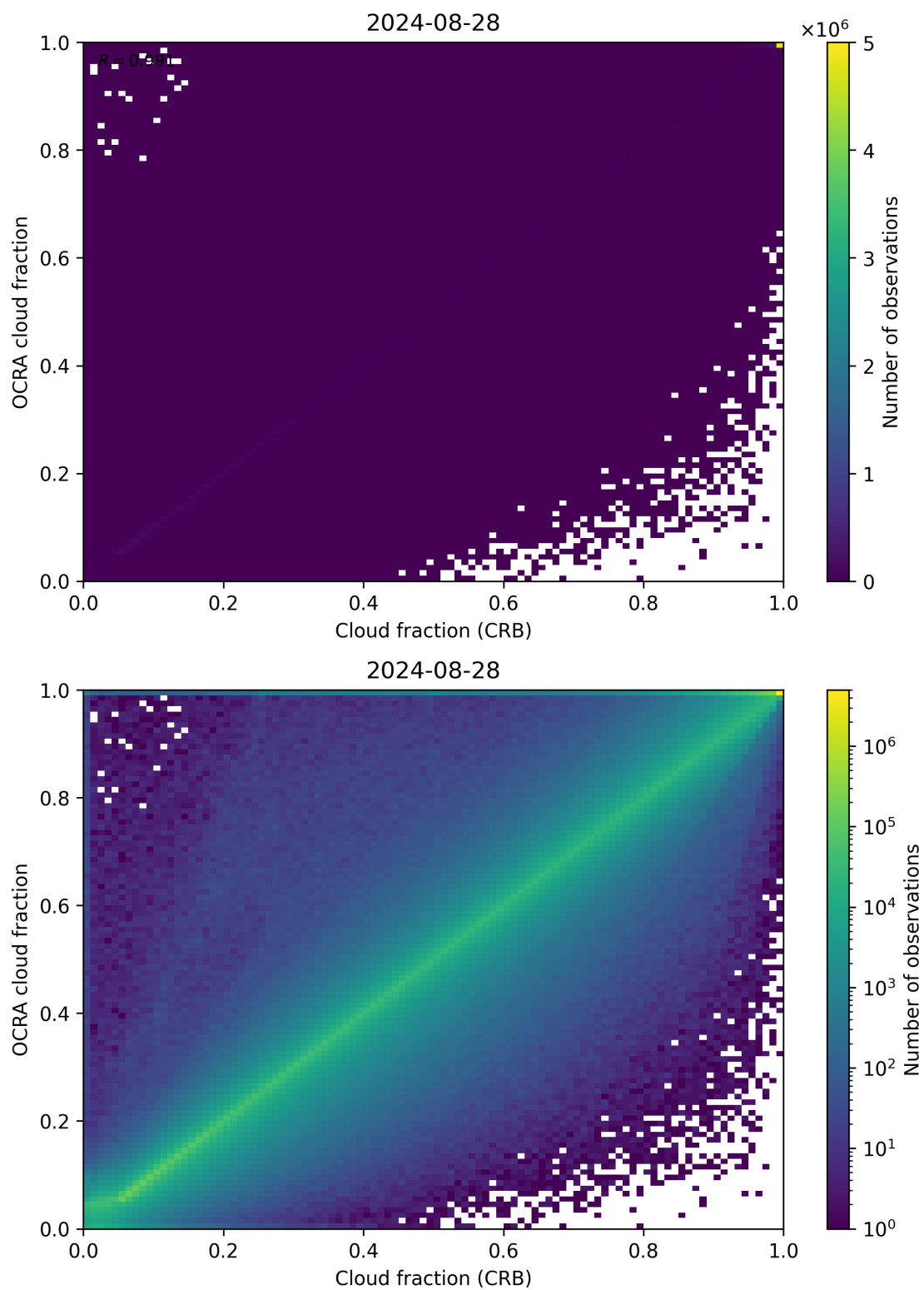
Figure 78: Scatter density plot of “Cloud fraction (CRB)” against “OCRA cloud fraction” for 2024-08-27 to 2024-08-29.
