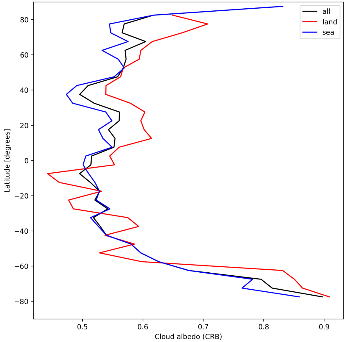
Figure 28: Zonal average of “Cloud albedo (CRB)” for 2024-08-27 to 2024-08-29.
