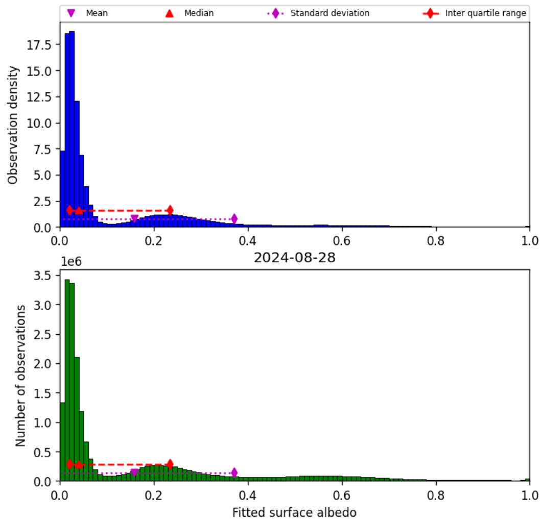
Figure 45: Histogram of “Fitted surface albedo” for 2024-08-27 to 2024-08-29
