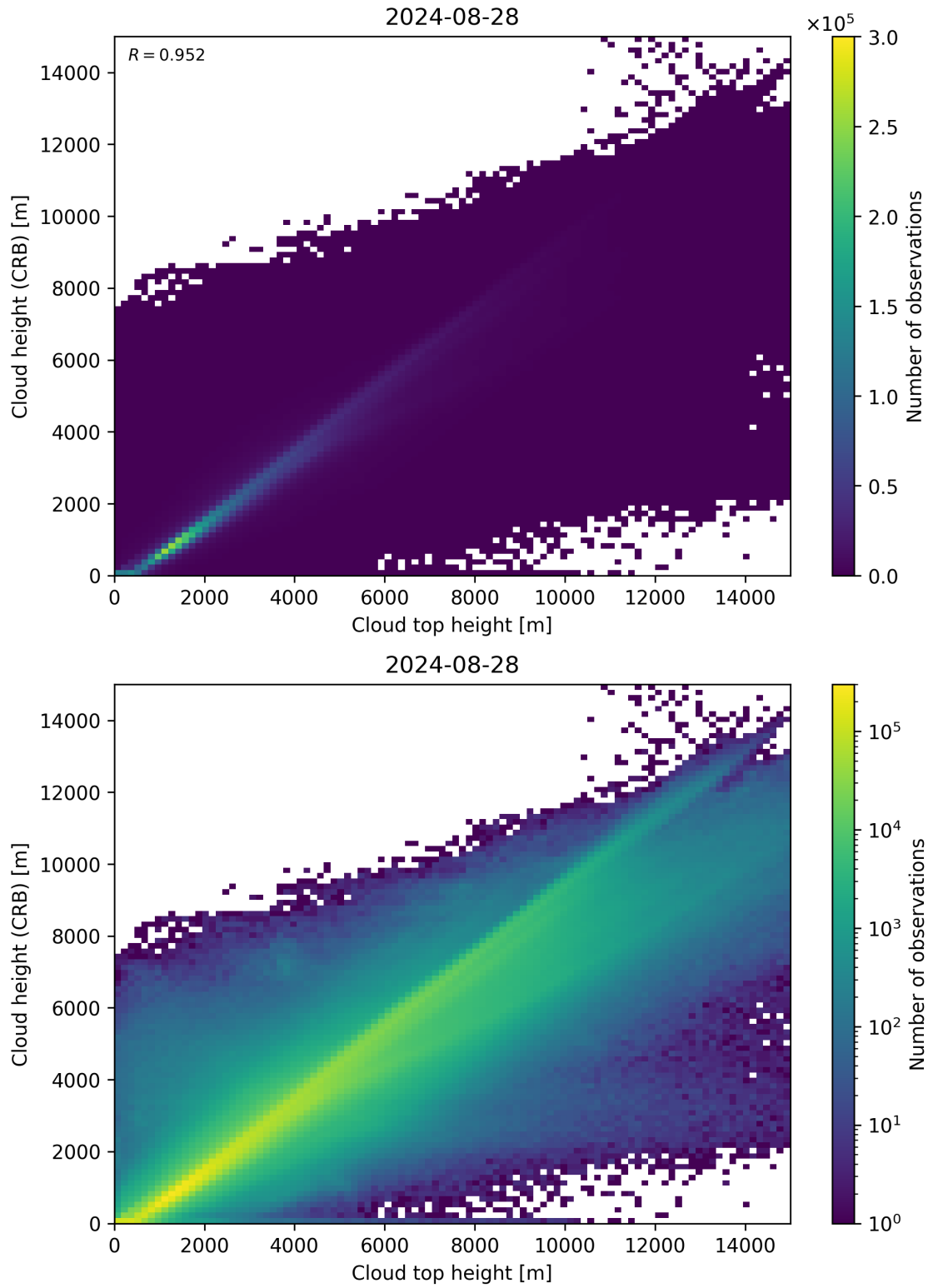
Figure 89: Scatter density plot of “Cloud top height” against “Cloud height (CRB)” for 2024-08-27 to 2024-08-29.
