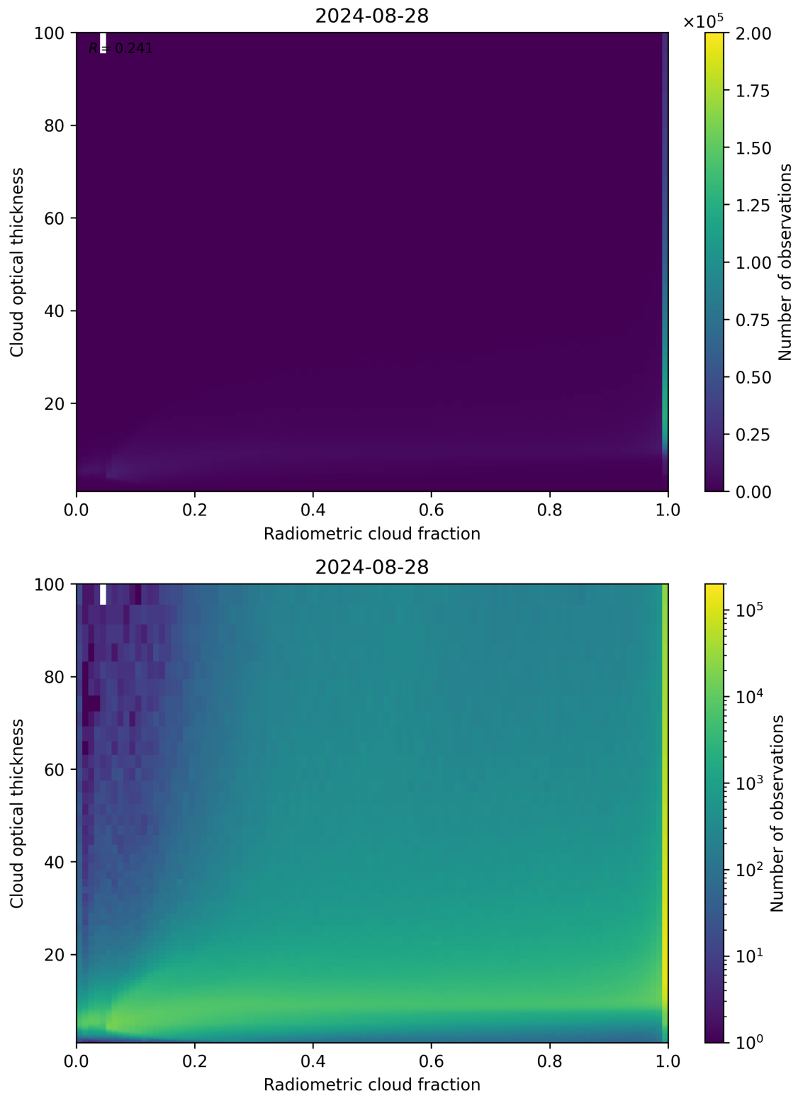
Figure 75: Scatter density plot of “Radiometric cloud fraction” against “Cloud optical thickness” for 2024-08-27 to 2024-08-29.
