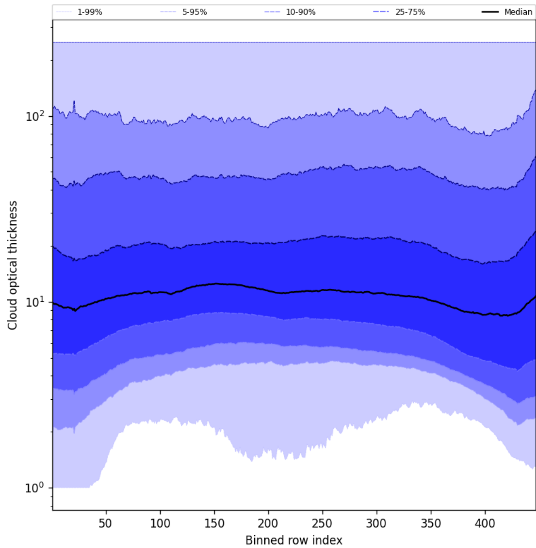
Figure 57: Along track statistics of “Cloud optical thickness” for 2024-08-27 to 2024-08-29
