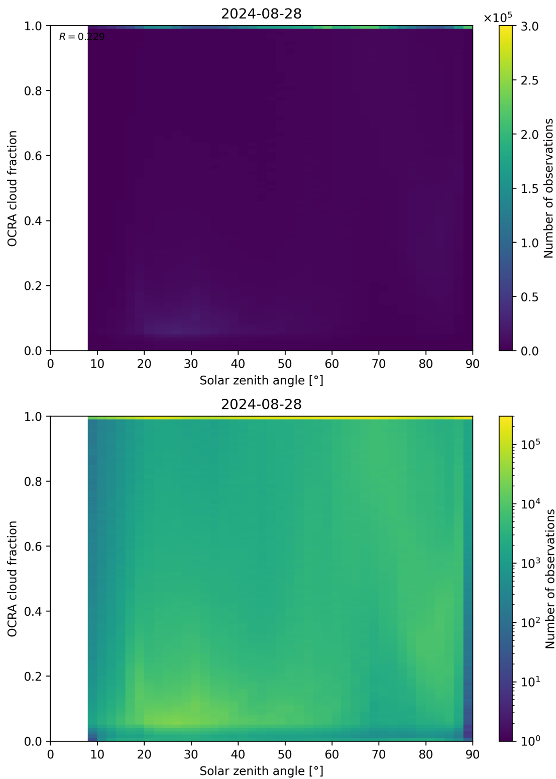
Figure 100: Scatter density plot of “Solar zenith angle” against “OCRA cloud fraction” for 2024-08-27 to 2024-08-29.
