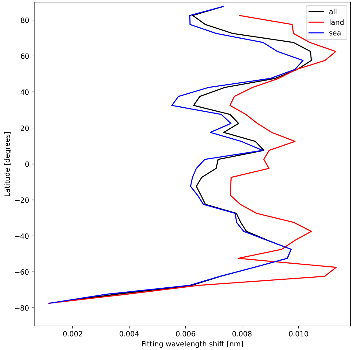
Figure 33: Zonal average of “Fitting wavelength shift” for 2024-08-27 to 2024-08-29.
