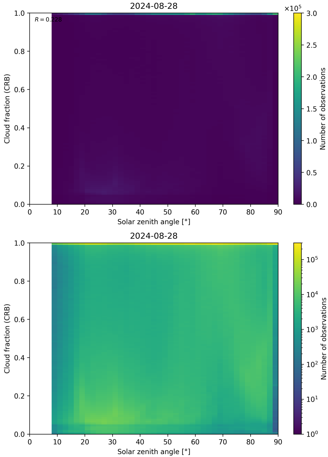
Figure 101: Scatter density plot of “Solar zenith angle” against “Cloud fraction (CRB)” for 2024-08-27 to 2024-08-29.
