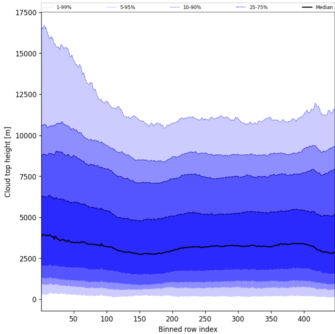
Figure 56: Along track statistics of “Cloud top height” for 2024-08-27 to 2024-08-29
