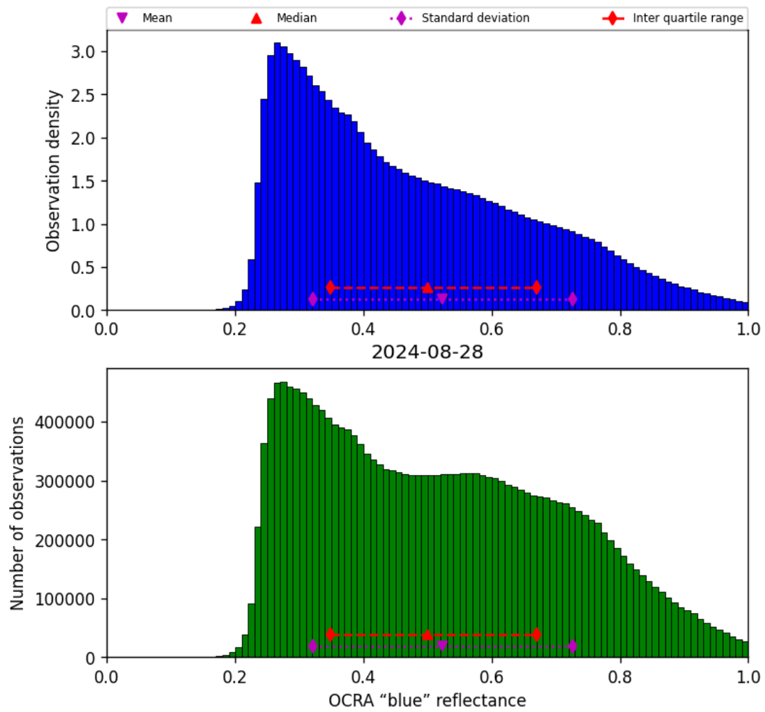
Figure 51: Histogram of “OCRA “blue” reflectance” for 2024-08-27 to 2024-08-29
