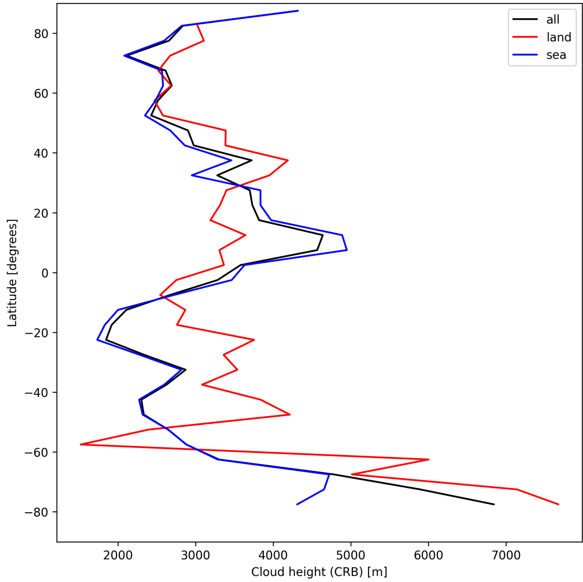
Figure 27: Zonal average of “Cloud height (CRB)” for 2024-08-27 to 2024-08-29.
