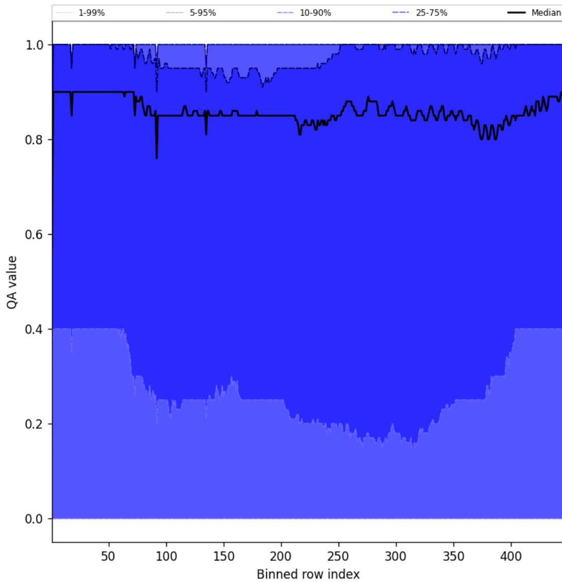
Figure 54: Along track statistics of “QA value” for 2024-08-27 to 2024-08-29
