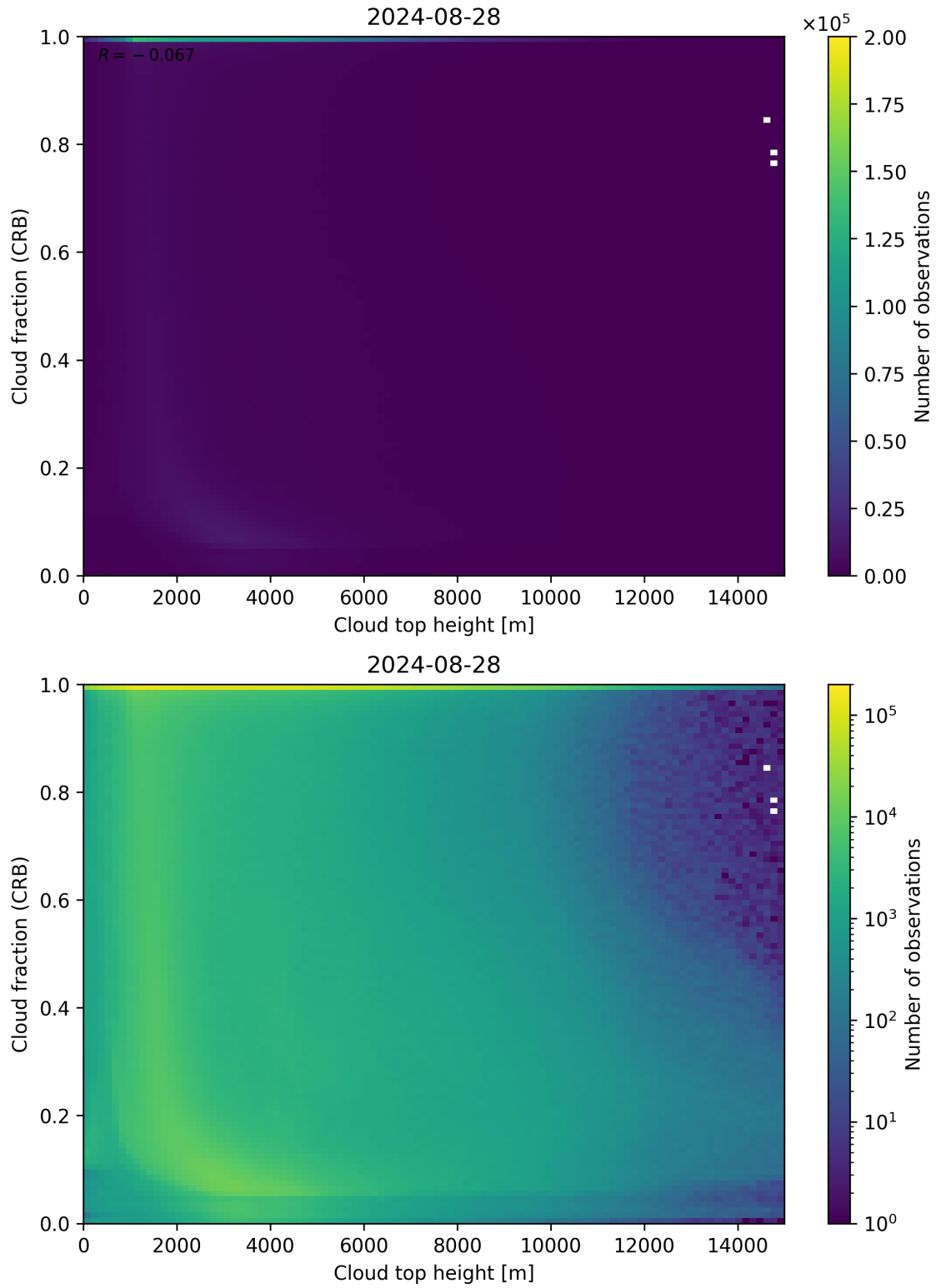
Figure 88: Scatter density plot of “Cloud top height” against “Cloud fraction (CRB)” for 2024-08-27 to 2024-08-29.
