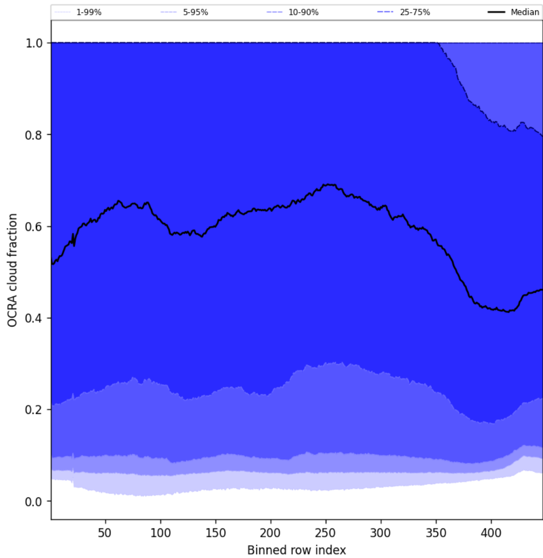
Figure 66: Along track statistics of “OCRA cloud fraction” for 2024-08-27 to 2024-08-29
