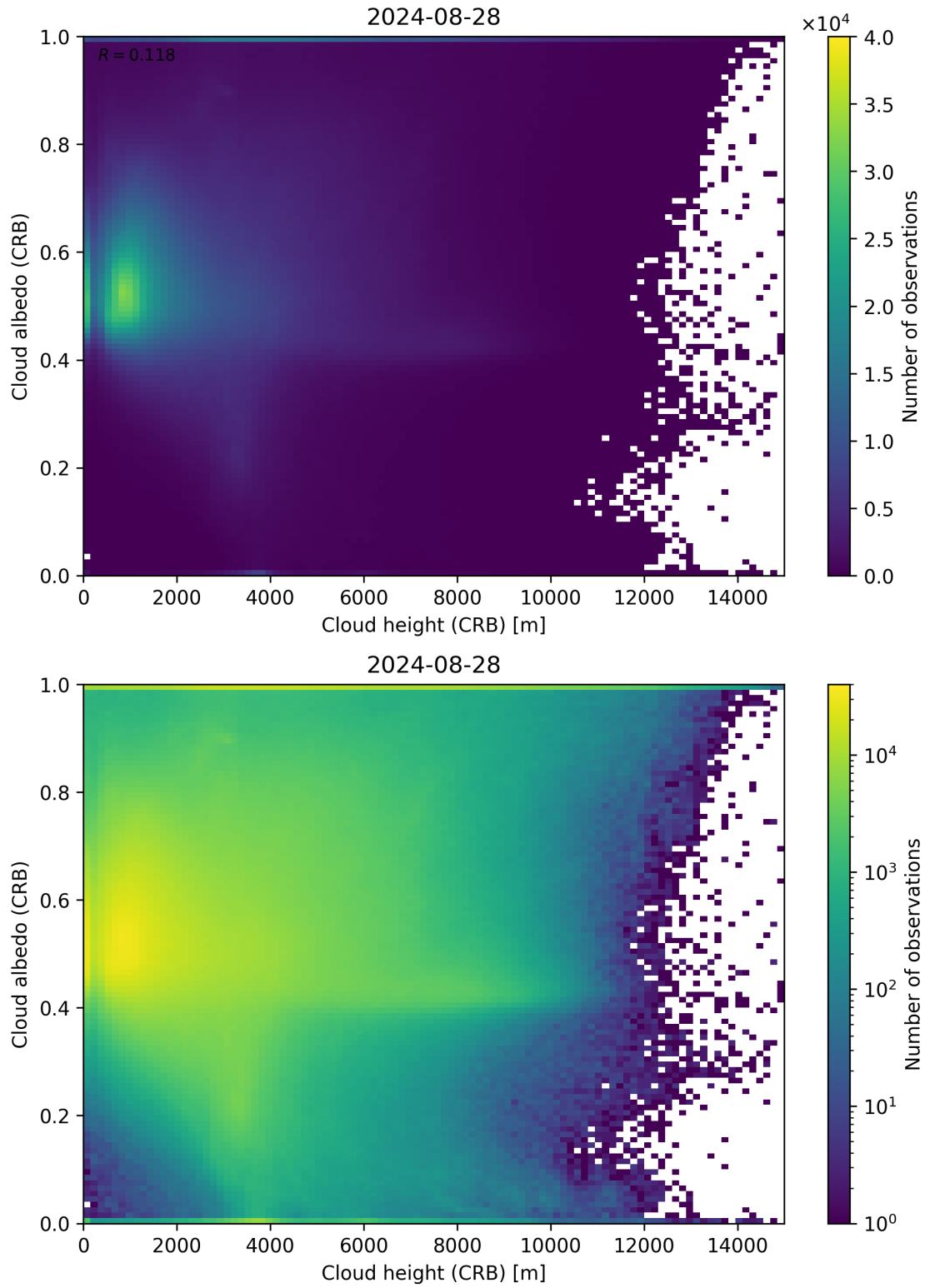
Figure 80: Scatter density plot of “Cloud height (CRB)” against “Cloud albedo (CRB)” for 2024-08-27 to 2024-08-29.
