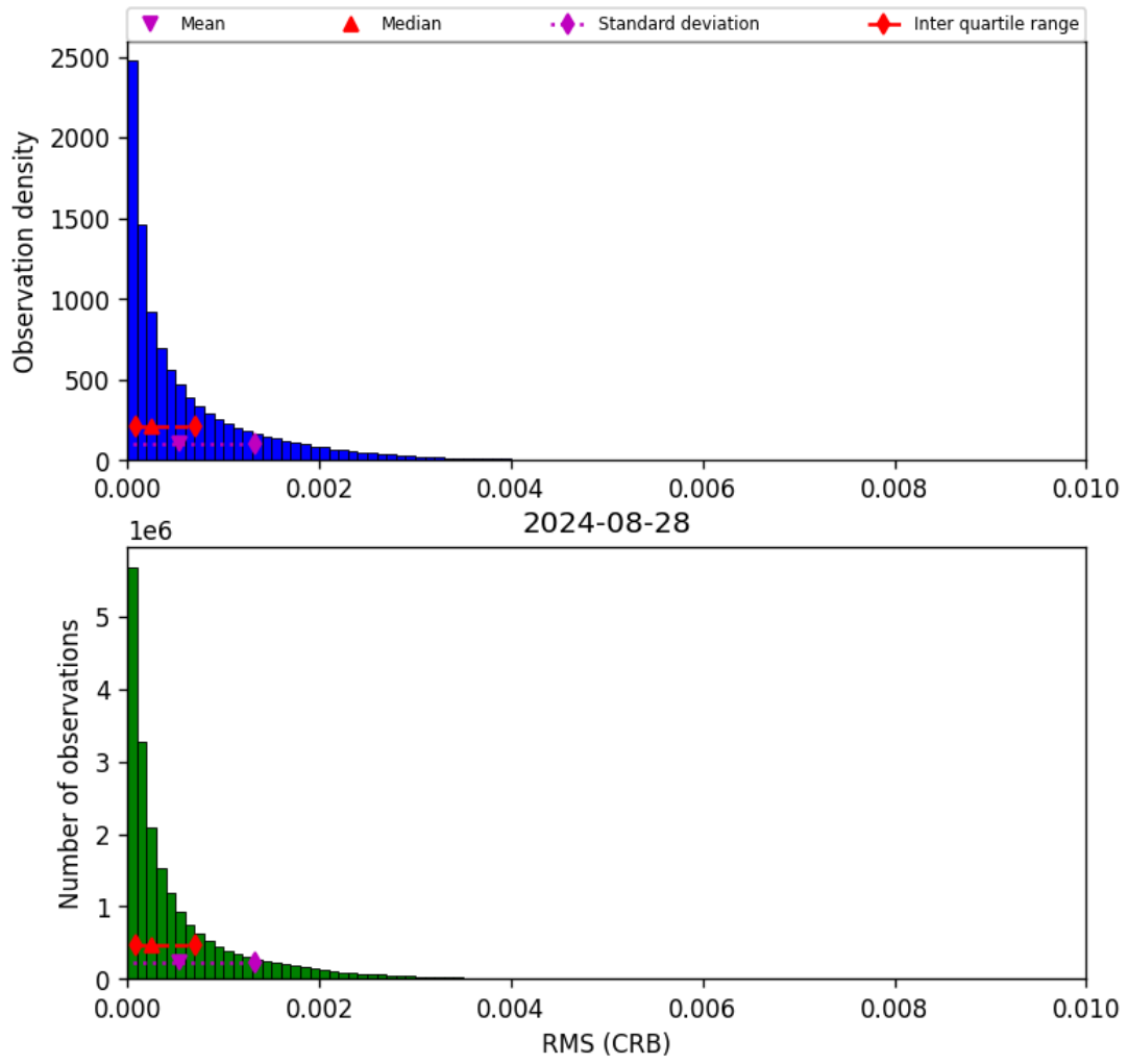
Figure 48: Histogram of “RMS (CRB)” for 2024-08-27 to 2024-08-29
