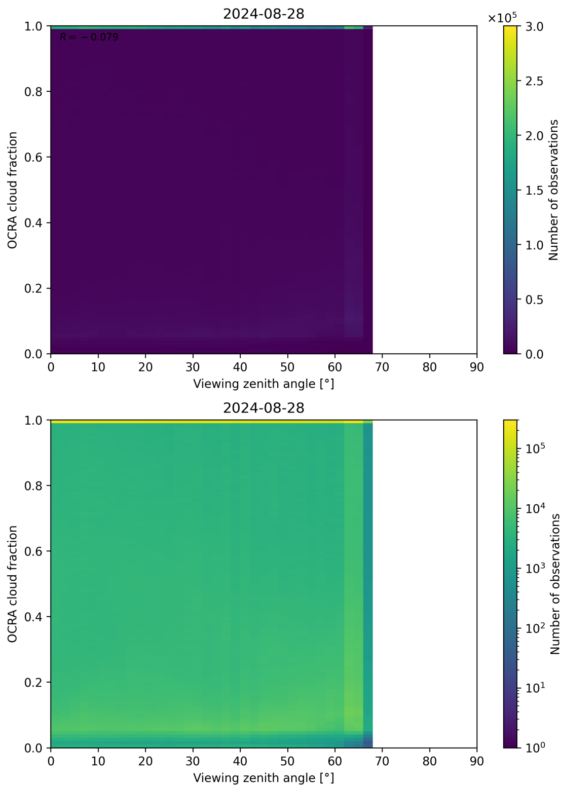
Figure 108: Scatter density plot of “Viewing zenith angle” against “OCRA cloud fraction” for 2024-08-27 to 2024-08-29.
