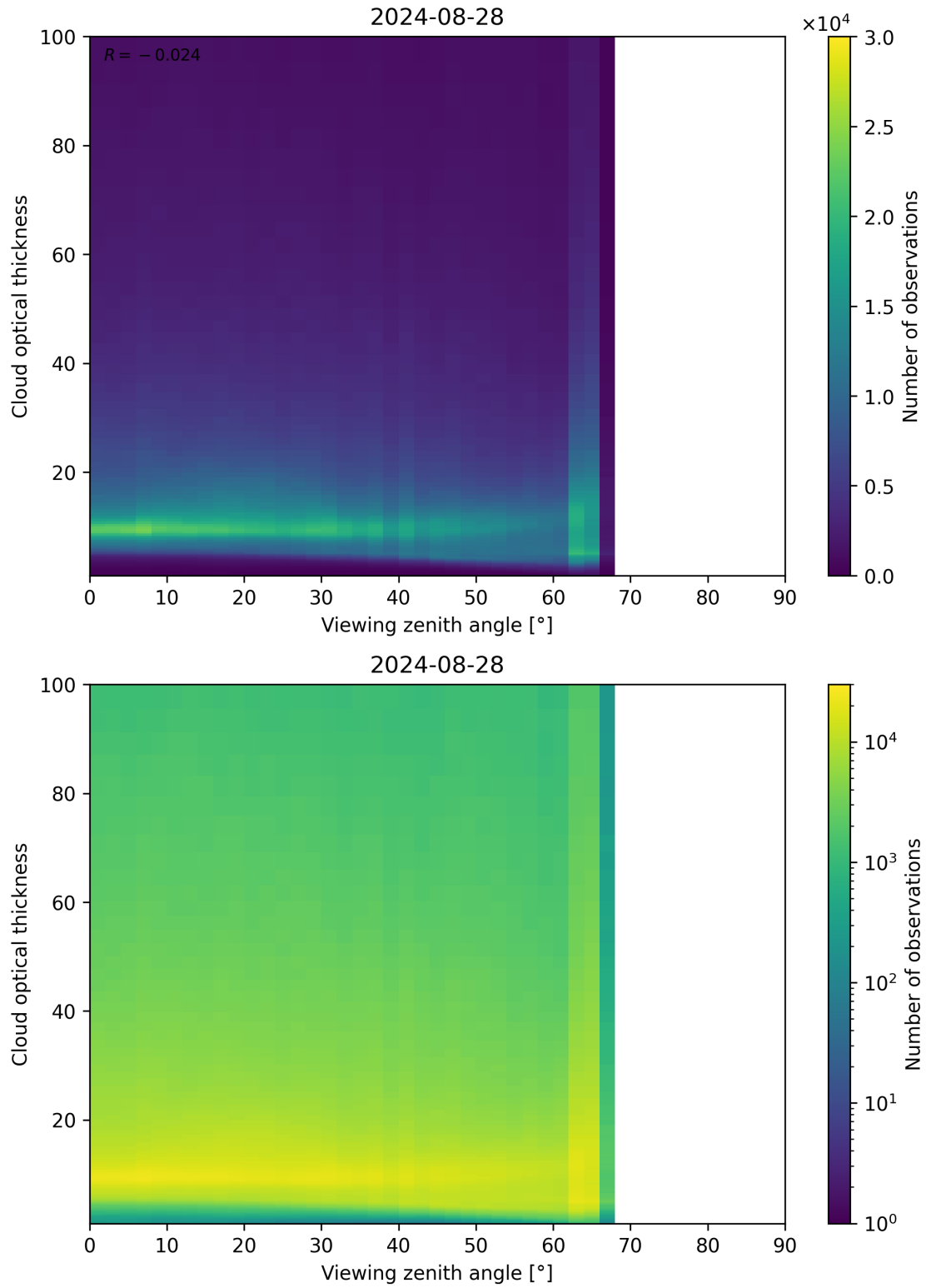
Figure 111: Scatter density plot of “Viewing zenith angle” against “Cloud optical thickness” for 2024-08-27 to 2024-08-29.
