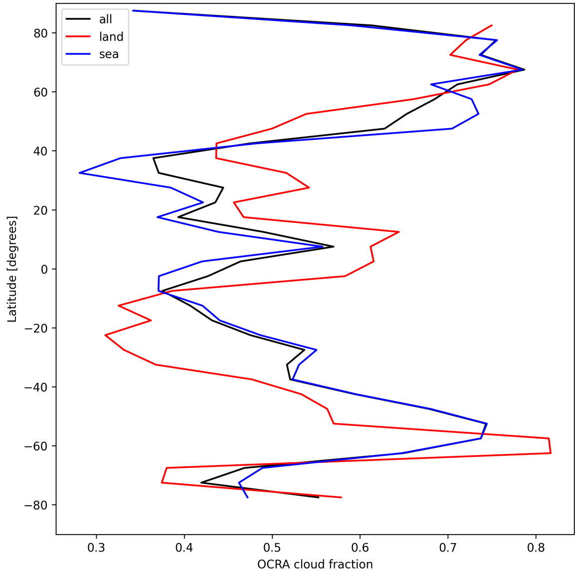
Figure 34: Zonal average of “OCRA cloud fraction” for 2024-08-27 to 2024-08-29.
