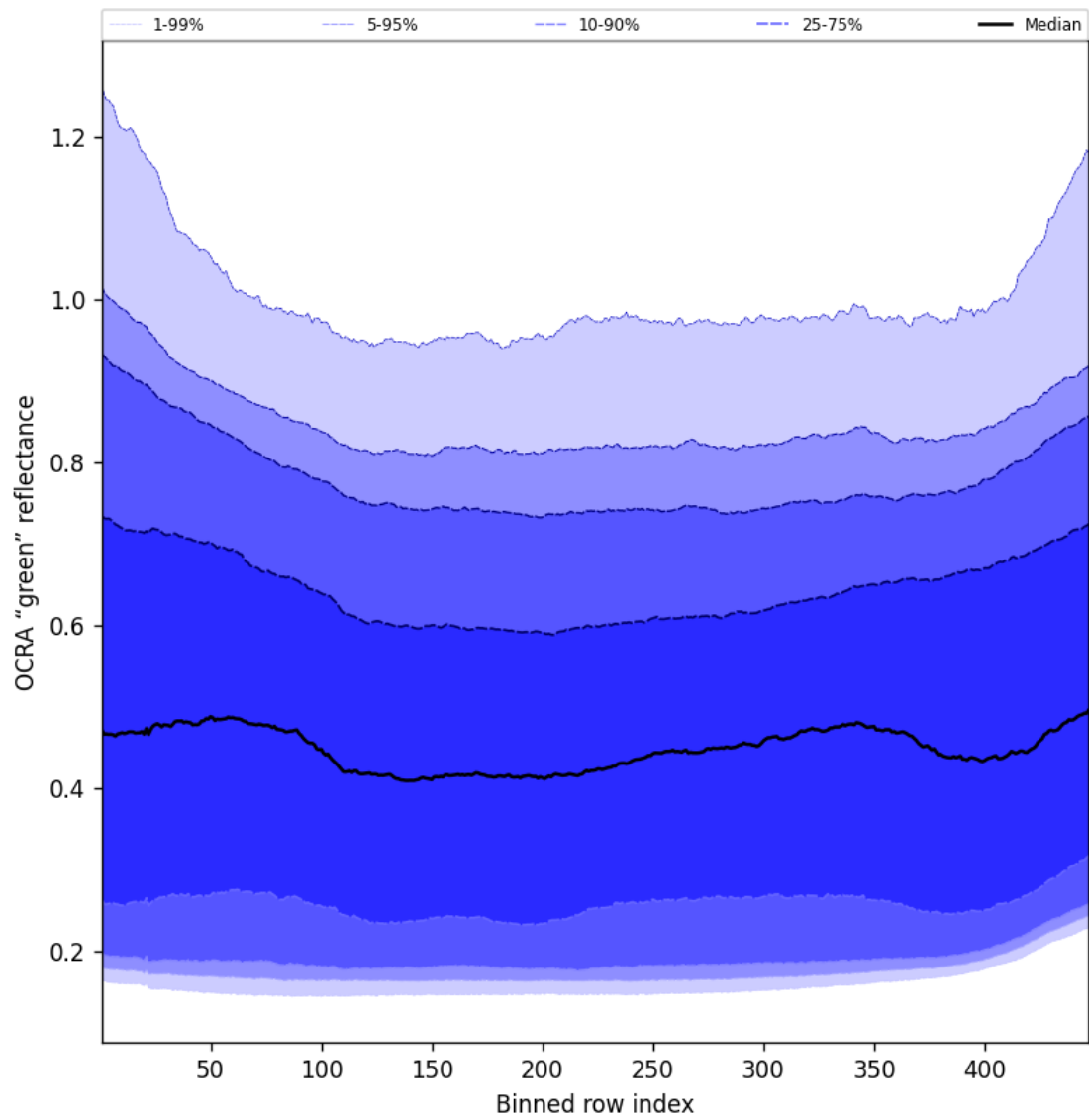
Figure 68: Along track statistics of “OCRA “green” reflectance” for 2024-08-27 to 2024-08-29
