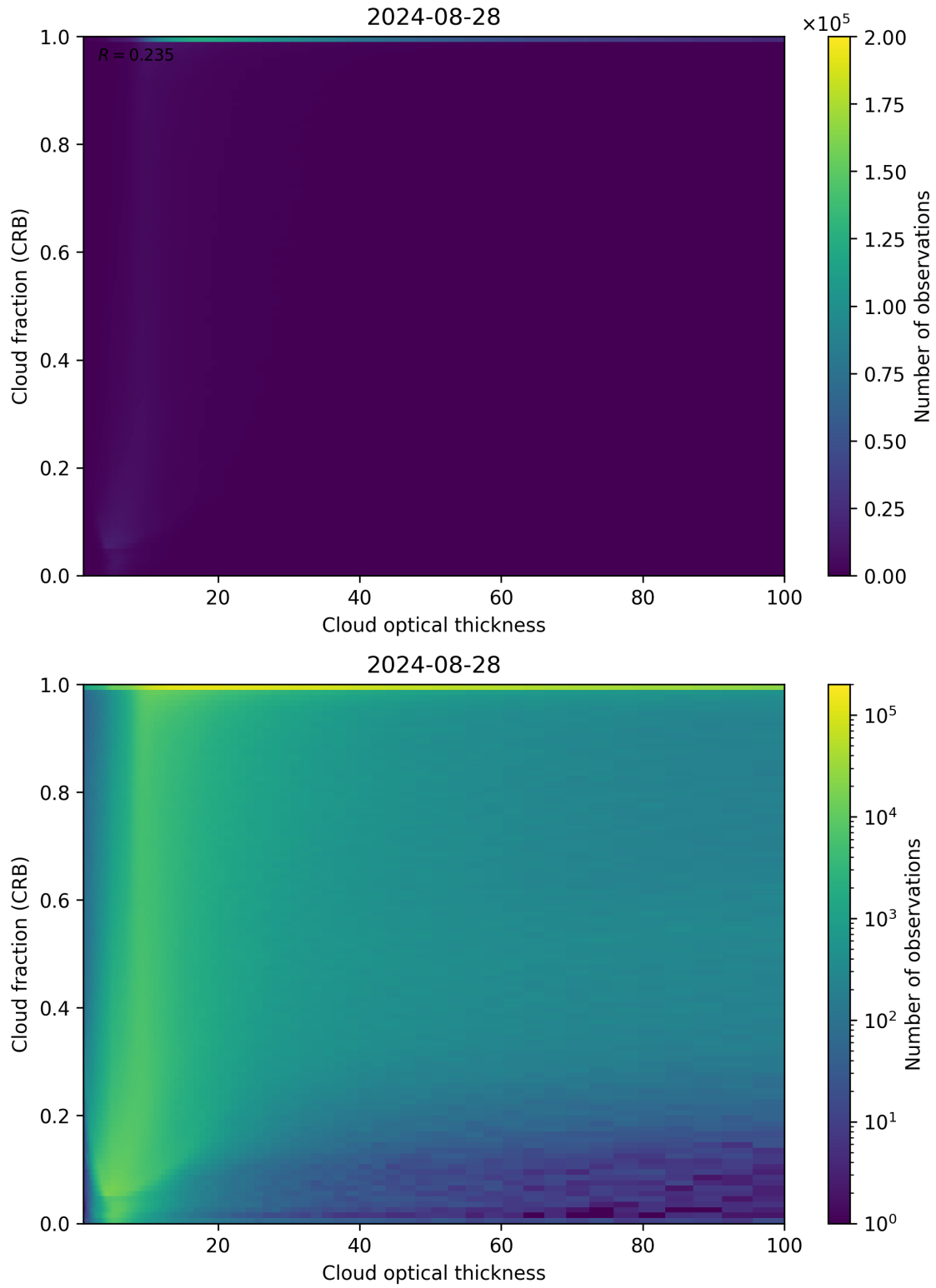
Figure 84: Scatter density plot of “Cloud optical thickness” against “Cloud fraction (CRB)” for 2024-08-27 to 2024-08-29.
