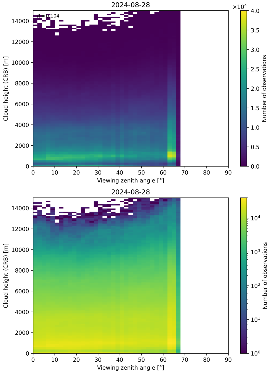
Figure 110: Scatter density plot of “Viewing zenith angle” against “Cloud height (CRB)” for 2024-08-27 to 2024-08-29.
