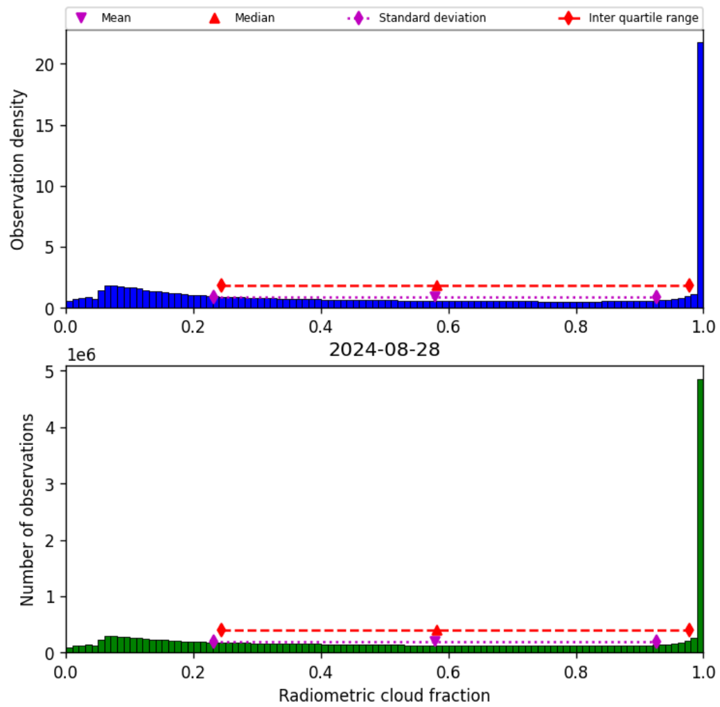
Figure 39: Histogram of “Radiometric cloud fraction” for 2024-08-27 to 2024-08-29
