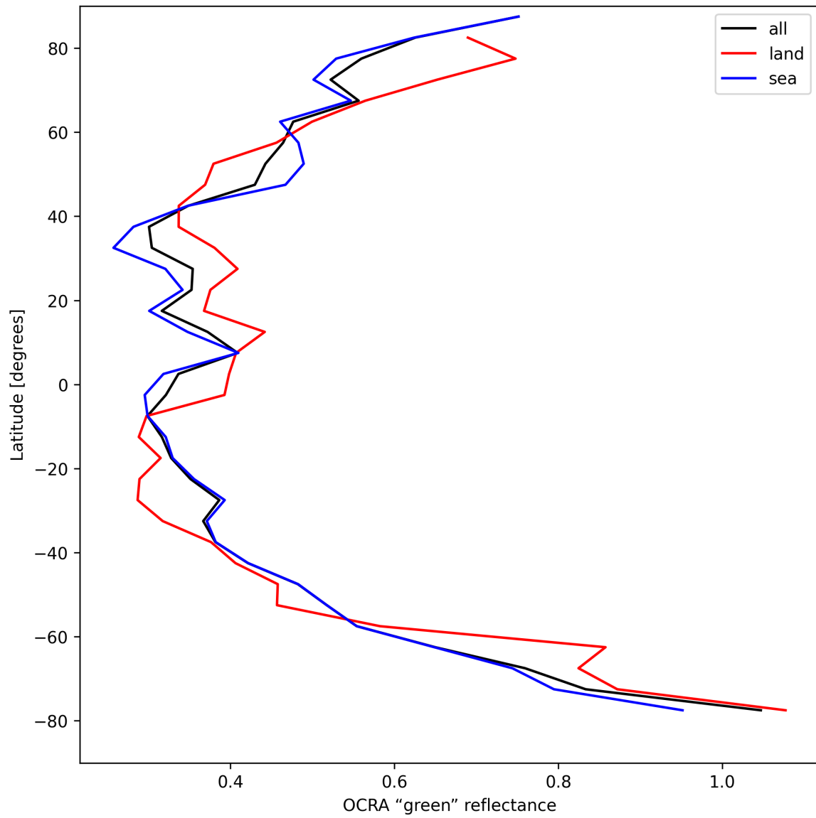
Figure 36: Zonal average of “OCRA “green” reflectance” for 2024-08-27 to 2024-08-29.
