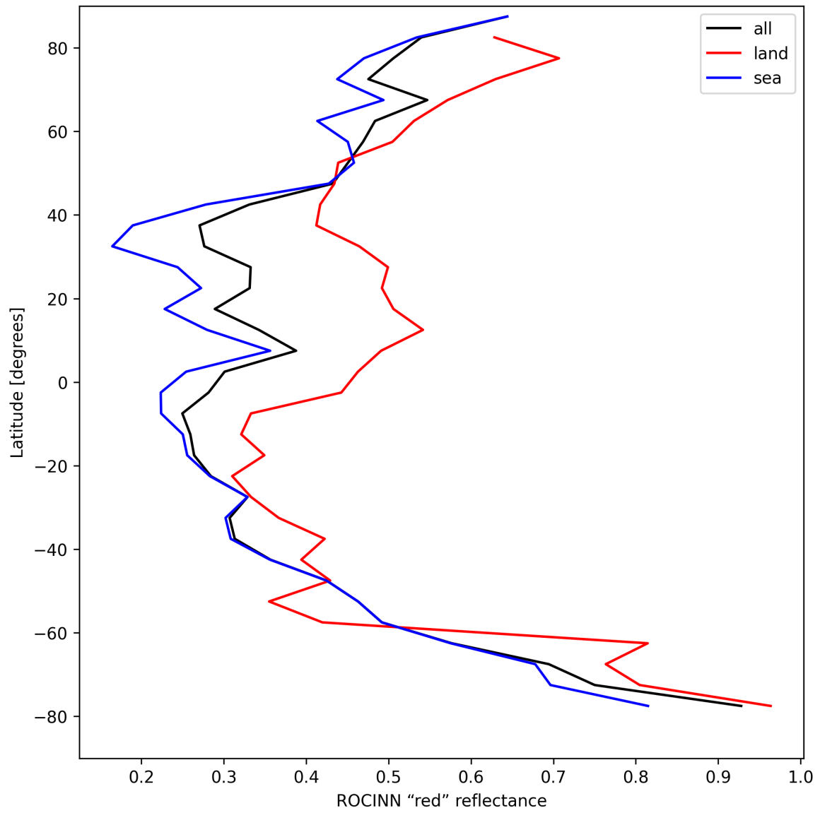
Figure 37: Zonal average of “ROCINN “red” reflectance” for 2024-08-27 to 2024-08-29.
