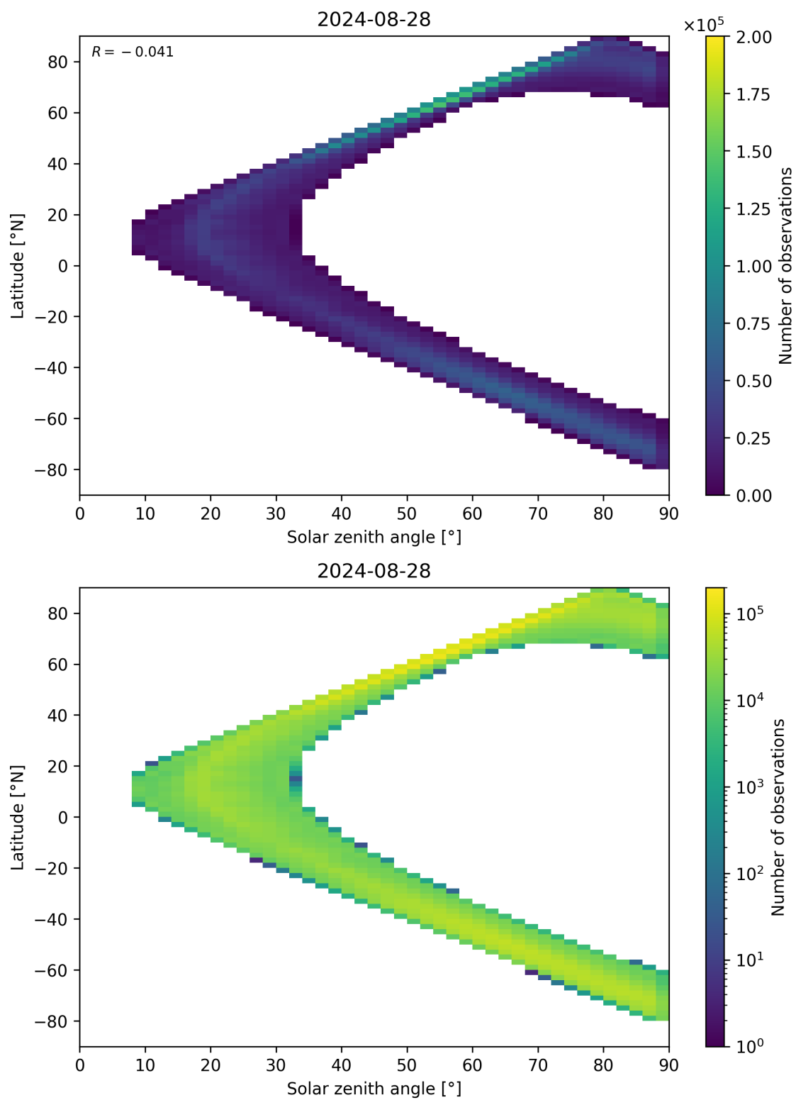
Figure 105: Scatter density plot of “Solar zenith angle” against “Latitude” for 2024-08-27 to 2024-08-29.
