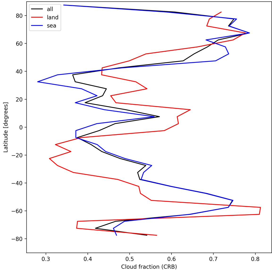
Figure 26: Zonal average of “Cloud fraction (CRB)” for 2024-08-27 to 2024-08-29.
