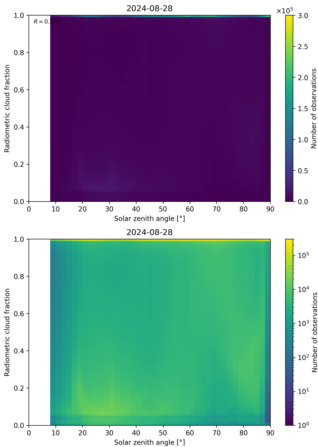
Figure 99: Scatter density plot of “Solar zenith angle” against “Radiometric cloud fraction” for 2024-08-27 to 2024-08-29.
