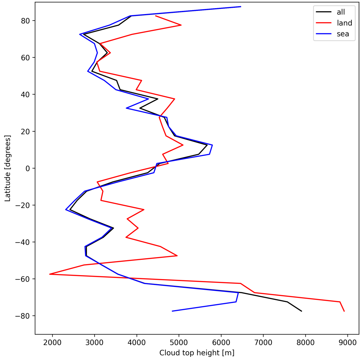
Figure 24: Zonal average of “Cloud top height” for 2024-08-27 to 2024-08-29.
