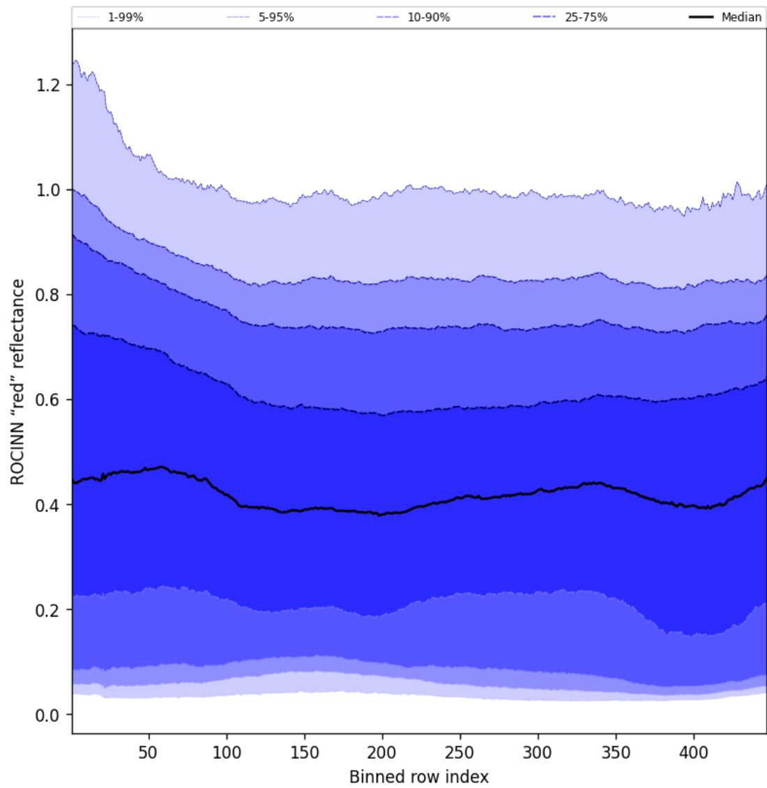
Figure 69: Along track statistics of "ROCINN red" reflectance" for 2024-08-27 to 2024-08-29
