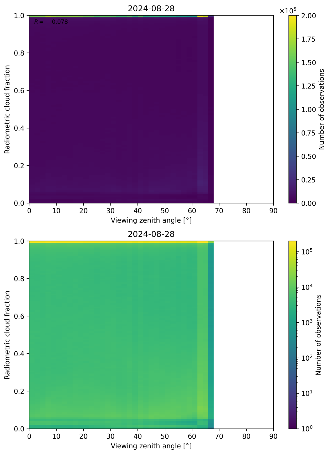
Figure 107: Scatter density plot of “Viewing zenith angle” against “Radiometric cloud fraction” for 2024-08-27 to 2024-08-29.
