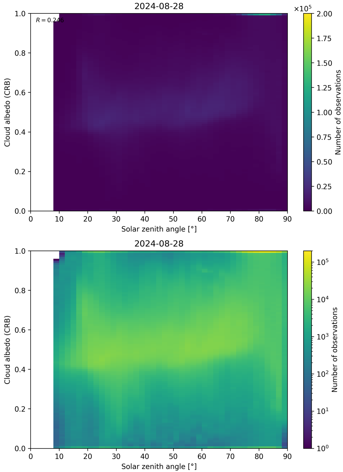
Figure 98: Scatter density plot of “Solar zenith angle” against “Cloud albedo (CRB)” for 2024-08-27 to 2024-08-29.
