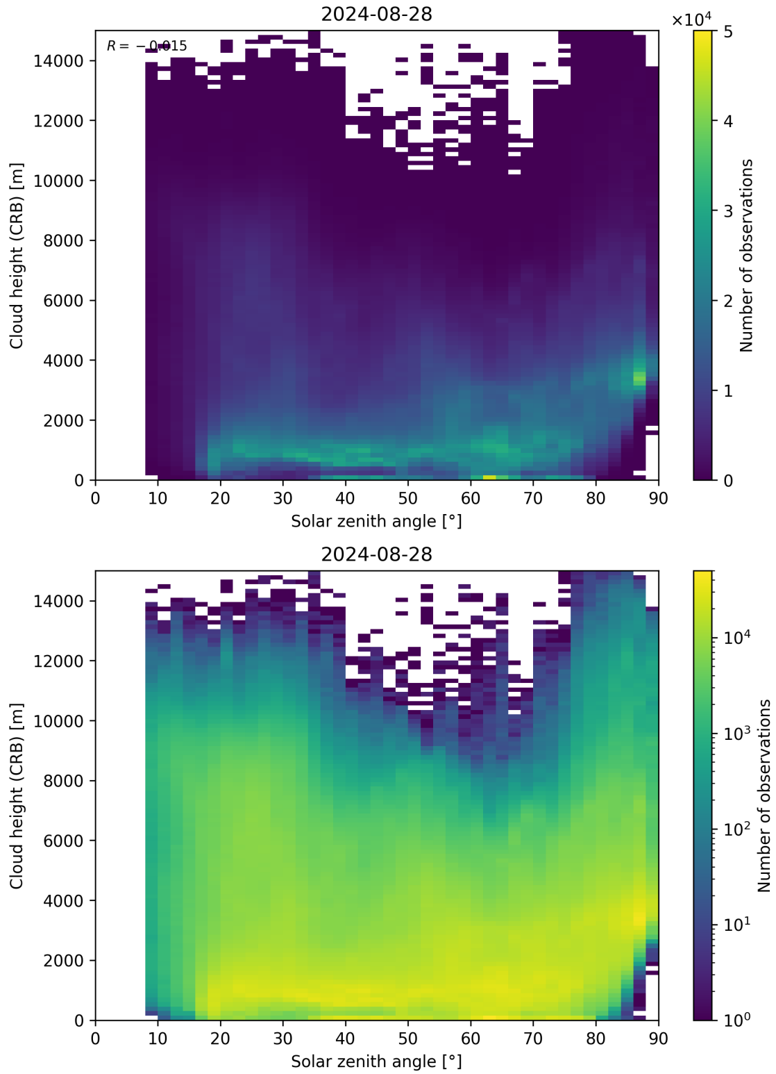
Figure 102: Scatter density plot of “Solar zenith angle” against “Cloud height (CRB)” for 2024-08-27 to 2024-08-29.
