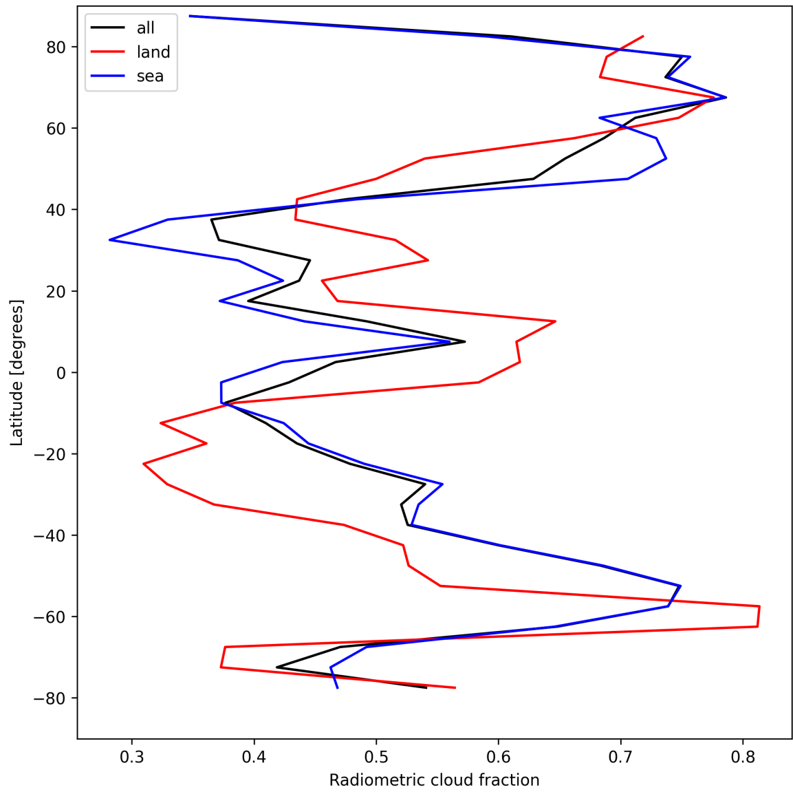
Figure 23: Zonal average of “Radiometric cloud fraction” for 2024-08-27 to 2024-08-29.
