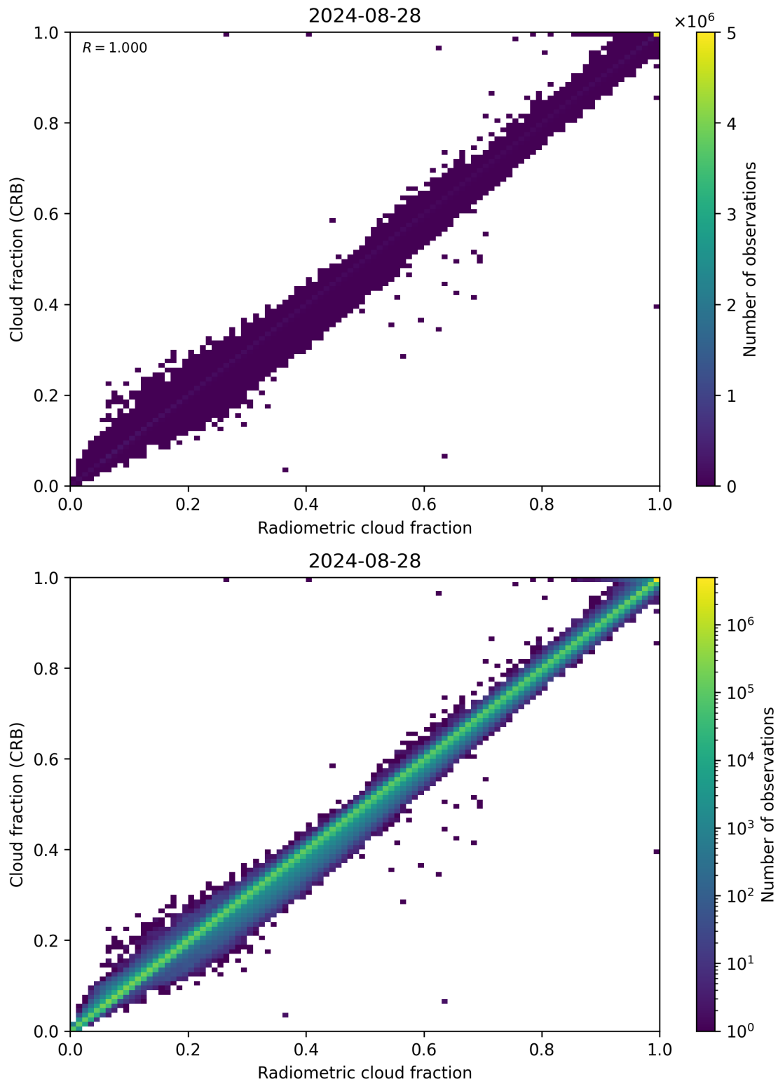
Figure 73: Scatter density plot of “Radiometric cloud fraction” against “Cloud fraction (CRB)” for 2024-08-27 to 2024-08-29.
