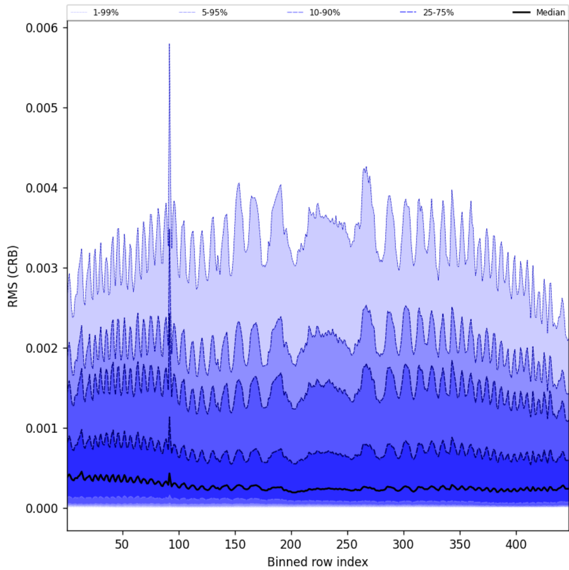
Figure 64: Along track statistics of “RMS (CRB)” for 2024-08-27 to 2024-08-29
