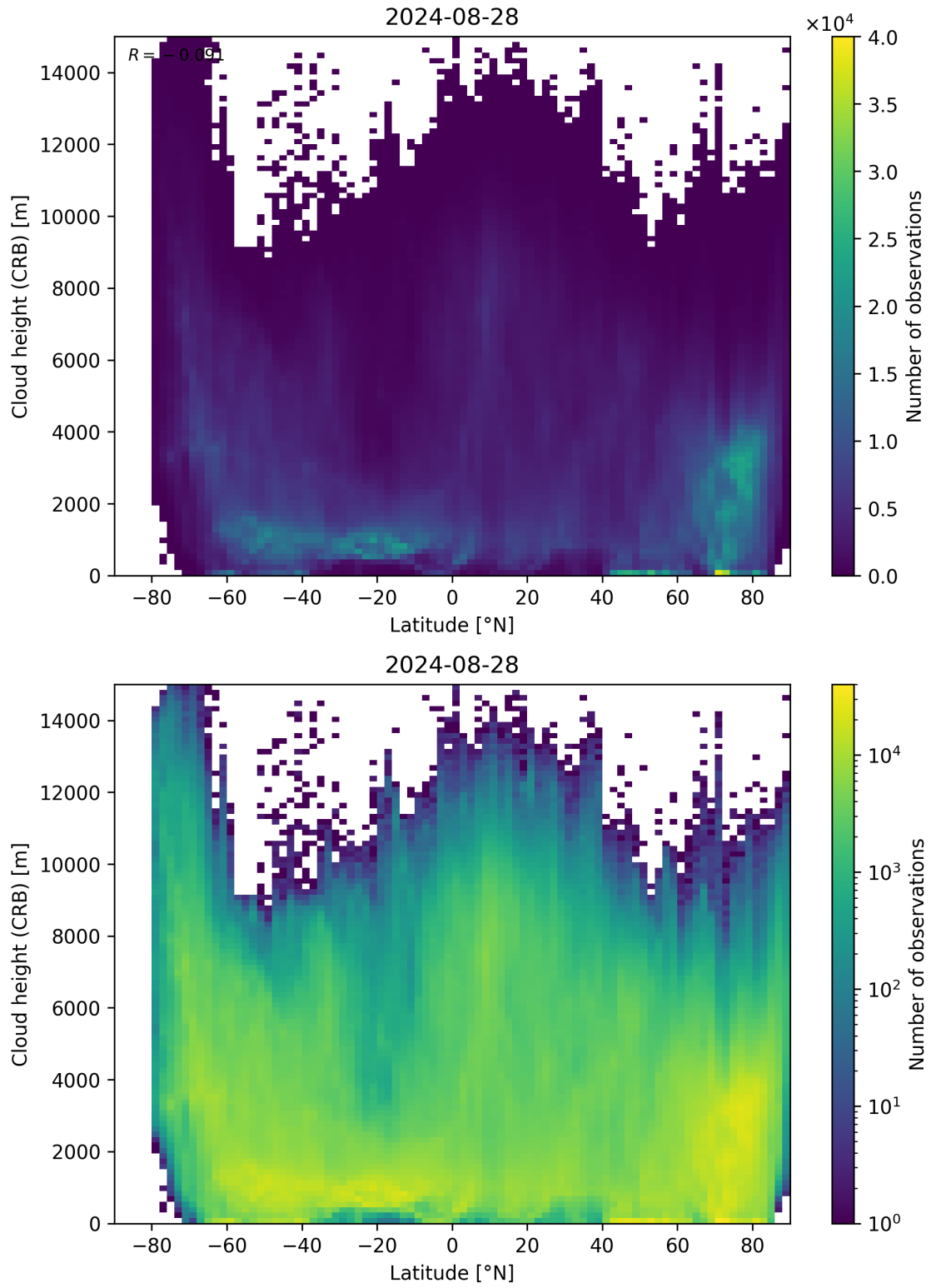
Figure 95: Scatter density plot of “Latitude” against “Cloud height (CRB)” for 2024-08-27 to 2024-08-29.
