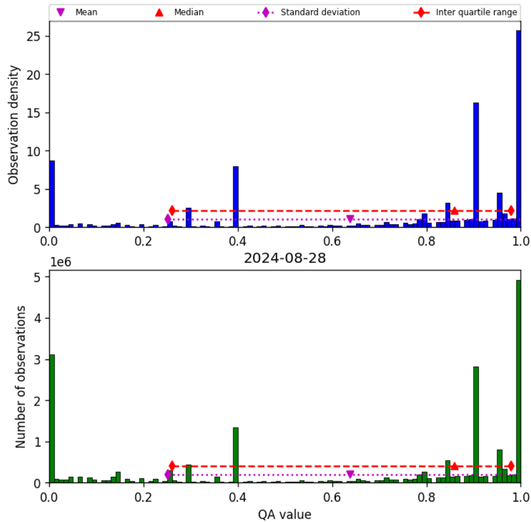
Figure 38: Histogram of “QA value” for 2024-08-27 to 2024-08-29
