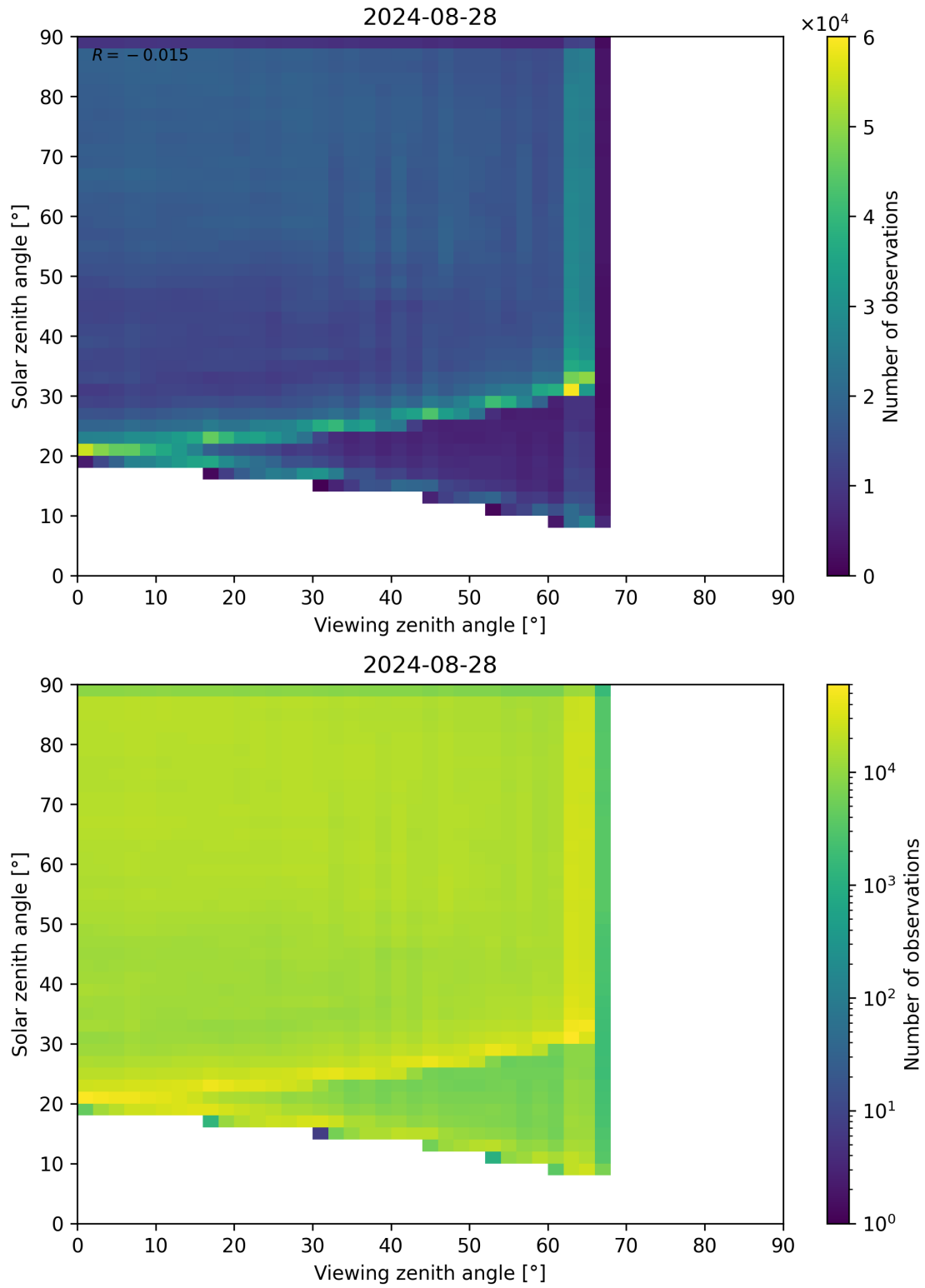
Figure 114: Scatter density plot of “Viewing zenith angle” against “Solar zenith angle” for 2024-08-27 to 2024-08-29.
