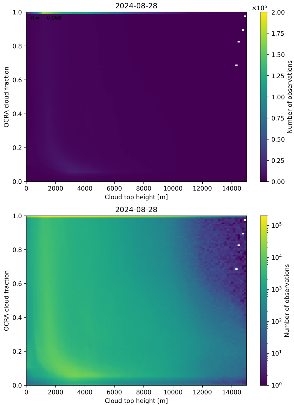
Figure 87: Scatter density plot of “Cloud top height” against “OCRA cloud fraction” for 2024-08-27 to 2024-08-29.
