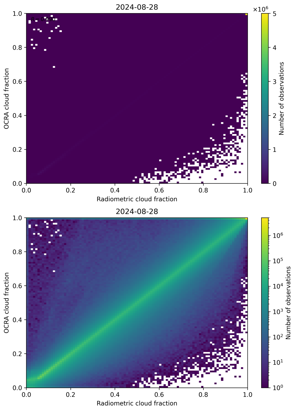
Figure 72: Scatter density plot of “Radiometric cloud fraction” against “OCRA cloud fraction” for 2024-08-27 to 2024-08-29.
