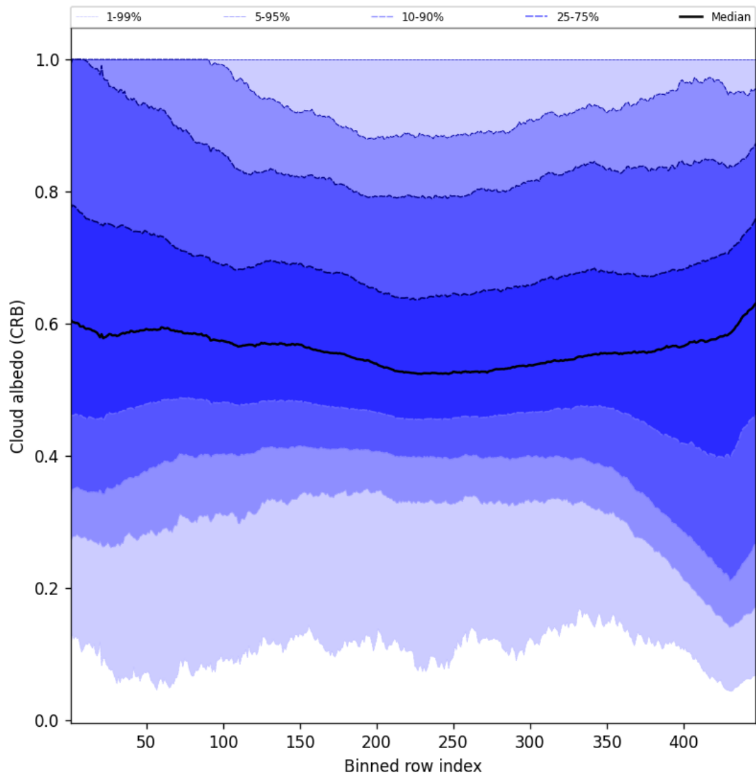
Figure 60: Along track statistics of “Cloud albedo (CRB)” for 2024-08-27 to 2024-08-29
