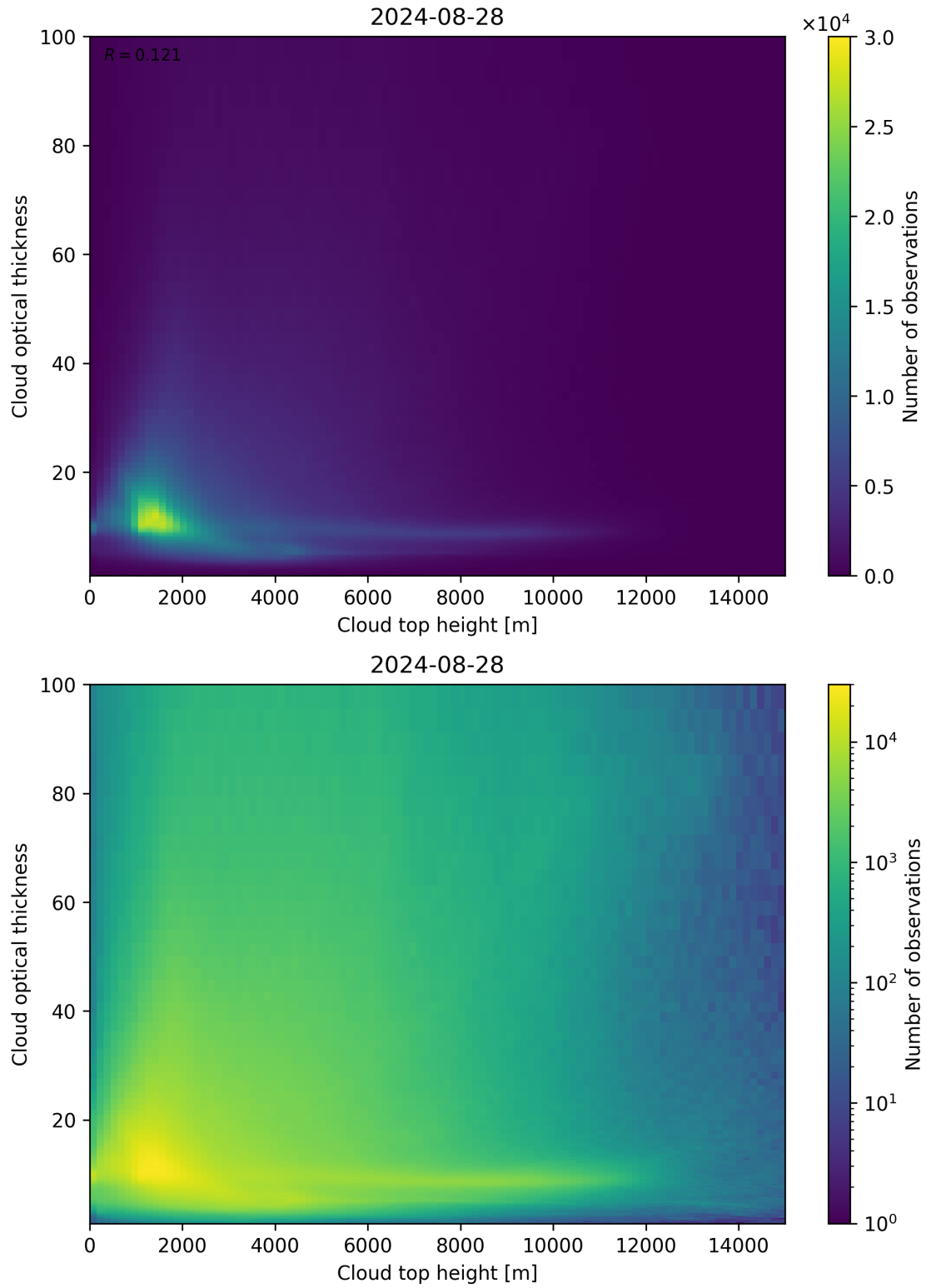
Figure 90: Scatter density plot of “Cloud top height” against “Cloud optical thickness” for 2024-08-27 to 2024-08-29.
