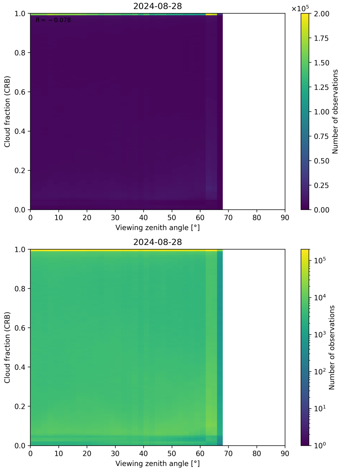
Figure 109: Scatter density plot of “Viewing zenith angle” against “Cloud fraction (CRB)” for 2024-08-27 to 2024-08-29.
