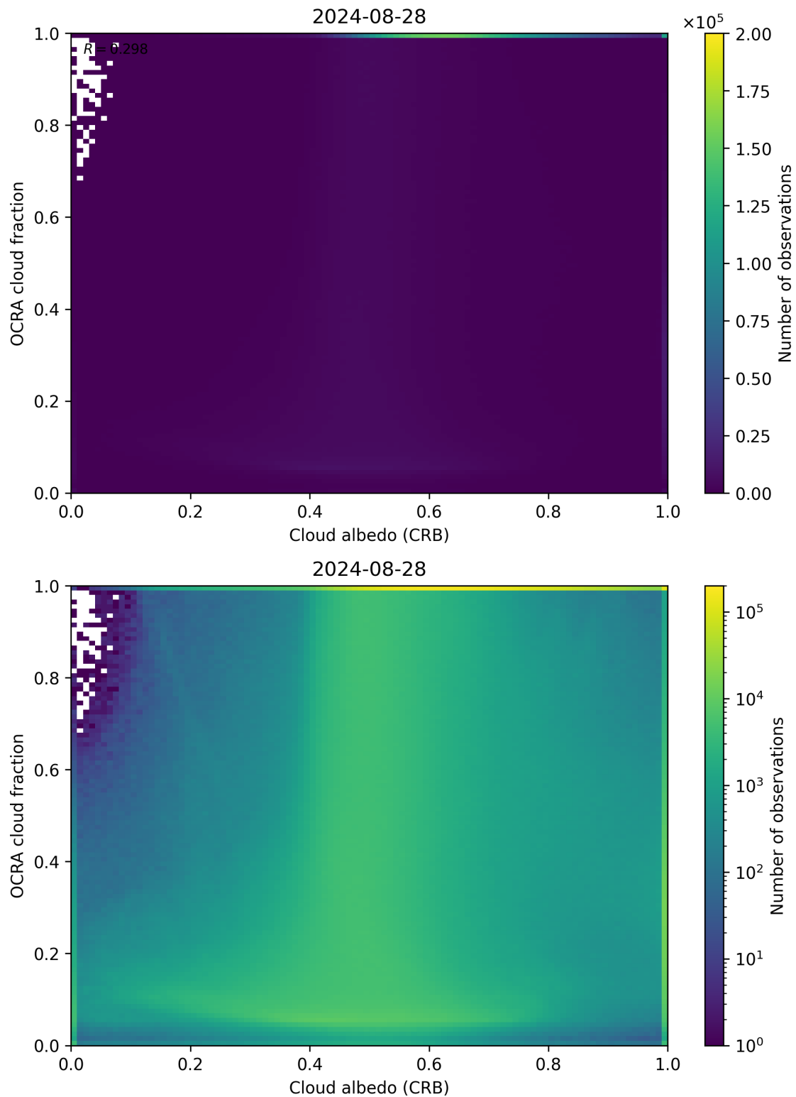
Figure 70: Scatter density plot of “Cloud albedo (CRB)” against “OCRA cloud fraction” for 2024-08-27 to 2024-08-29.
