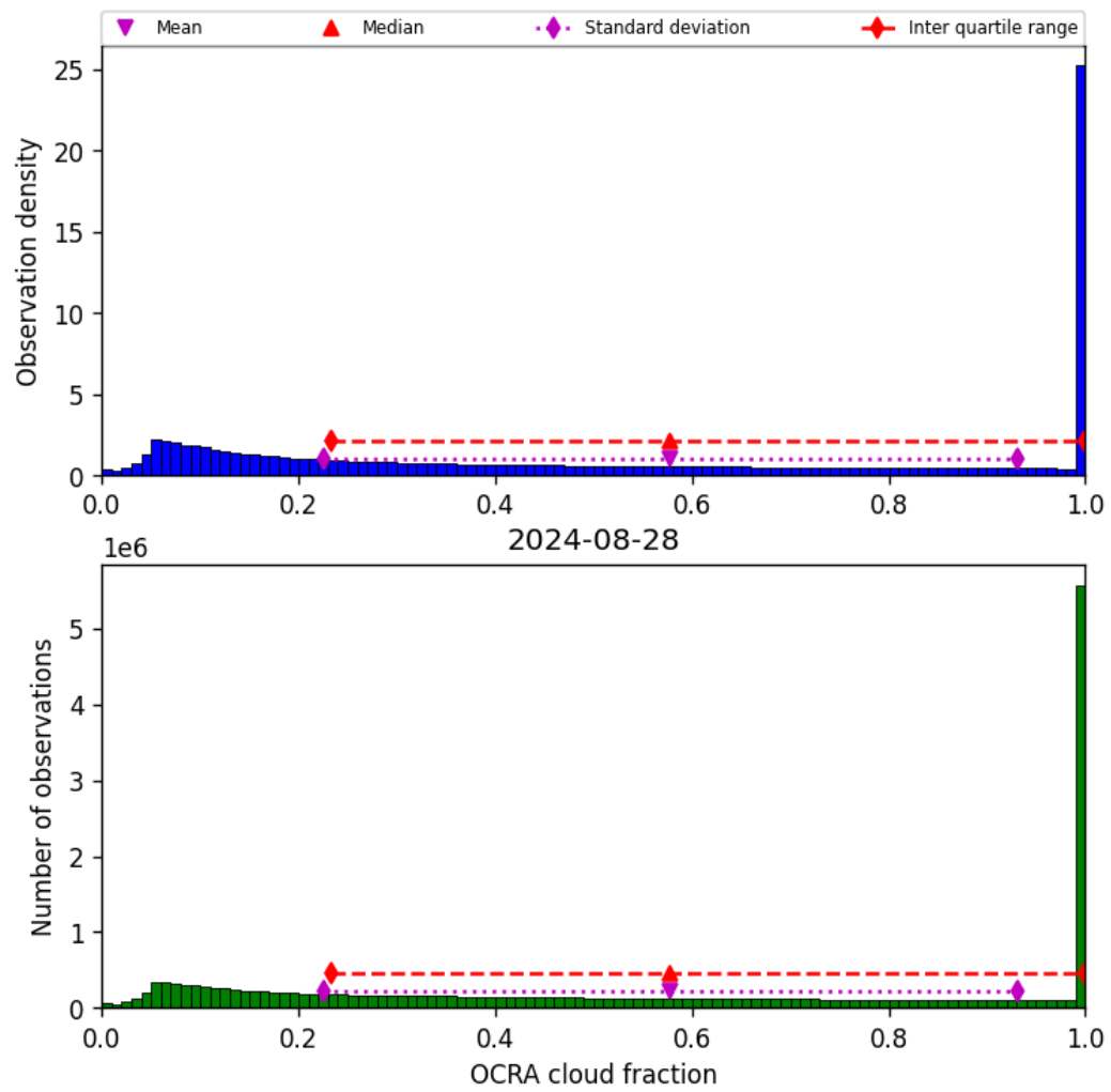
Figure 50: Histogram of “OCRA cloud fraction” for 2024-08-27 to 2024-08-29
