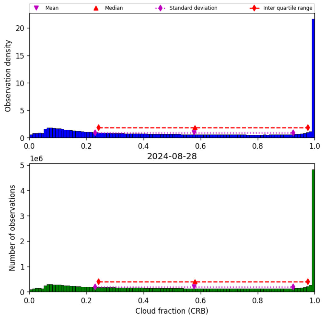
Figure 42: Histogram of “Cloud fraction (CRB)” for 2024-08-27 to 2024-08-29
