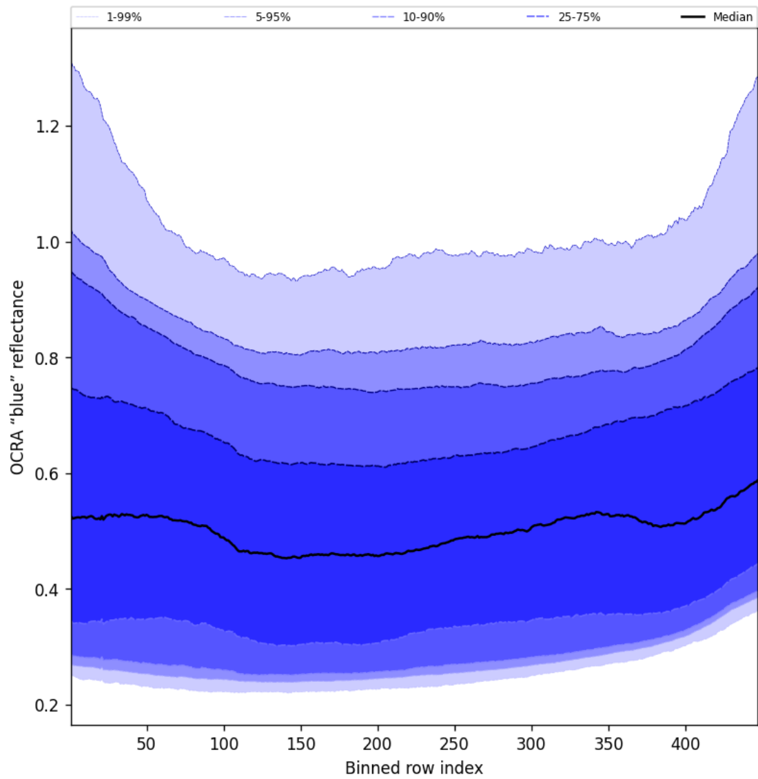
Figure 67: Along track statistics of “OCRA “blue” reflectance” for 2024-08-27 to 2024-08-29
