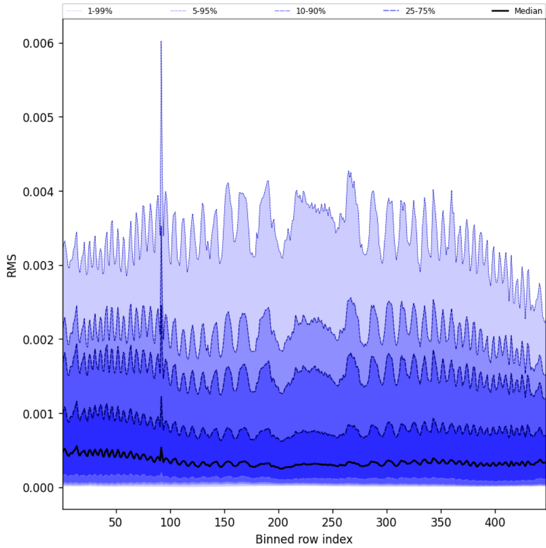
Figure 63: Along track statistics of “RMS” for 2024-08-27 to 2024-08-29
