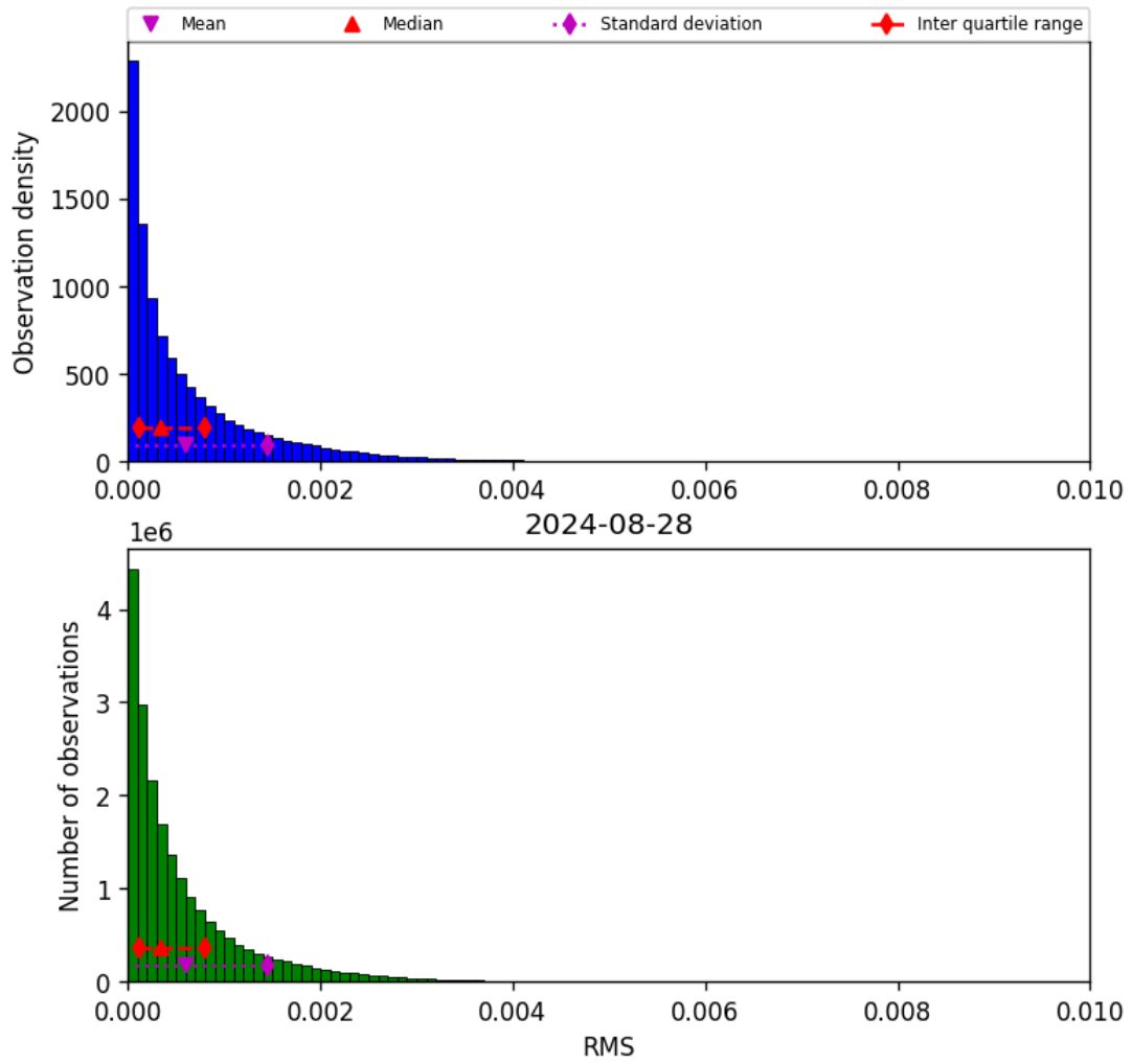
Figure 47: Histogram of “RMS” for 2024-08-27 to 2024-08-29
