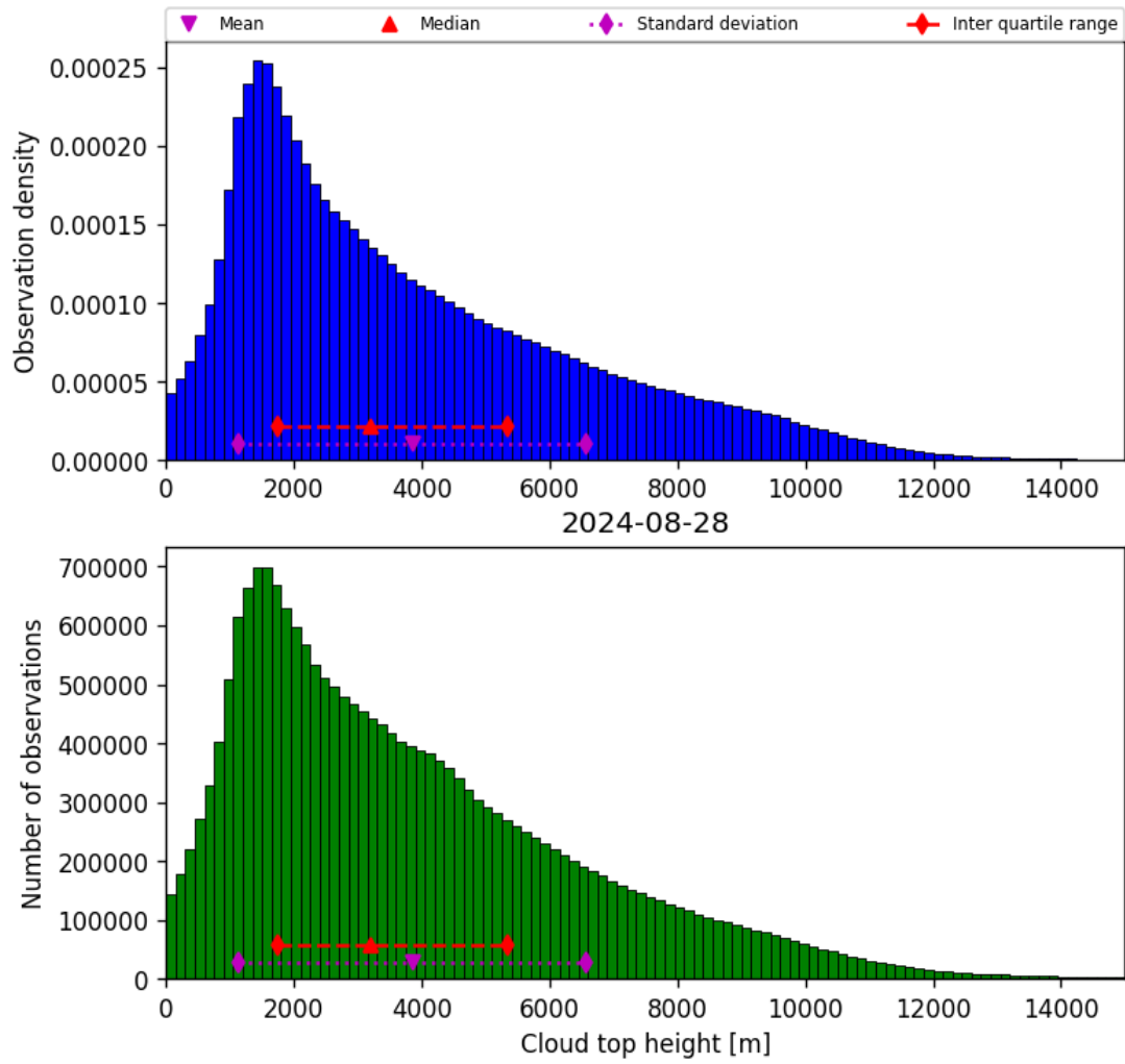
Figure 40: Histogram of “Cloud top height” for 2024-08-27 to 2024-08-29
