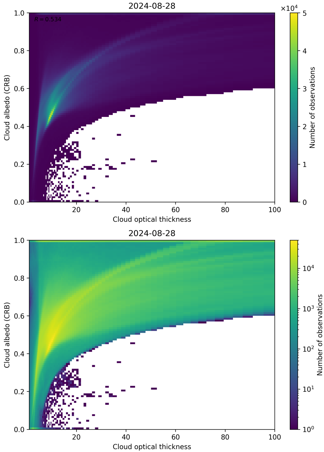
Figure 82: Scatter density plot of “Cloud optical thickness” against “Cloud albedo (CRB)” for 2024-08-27 to 2024-08-29.
