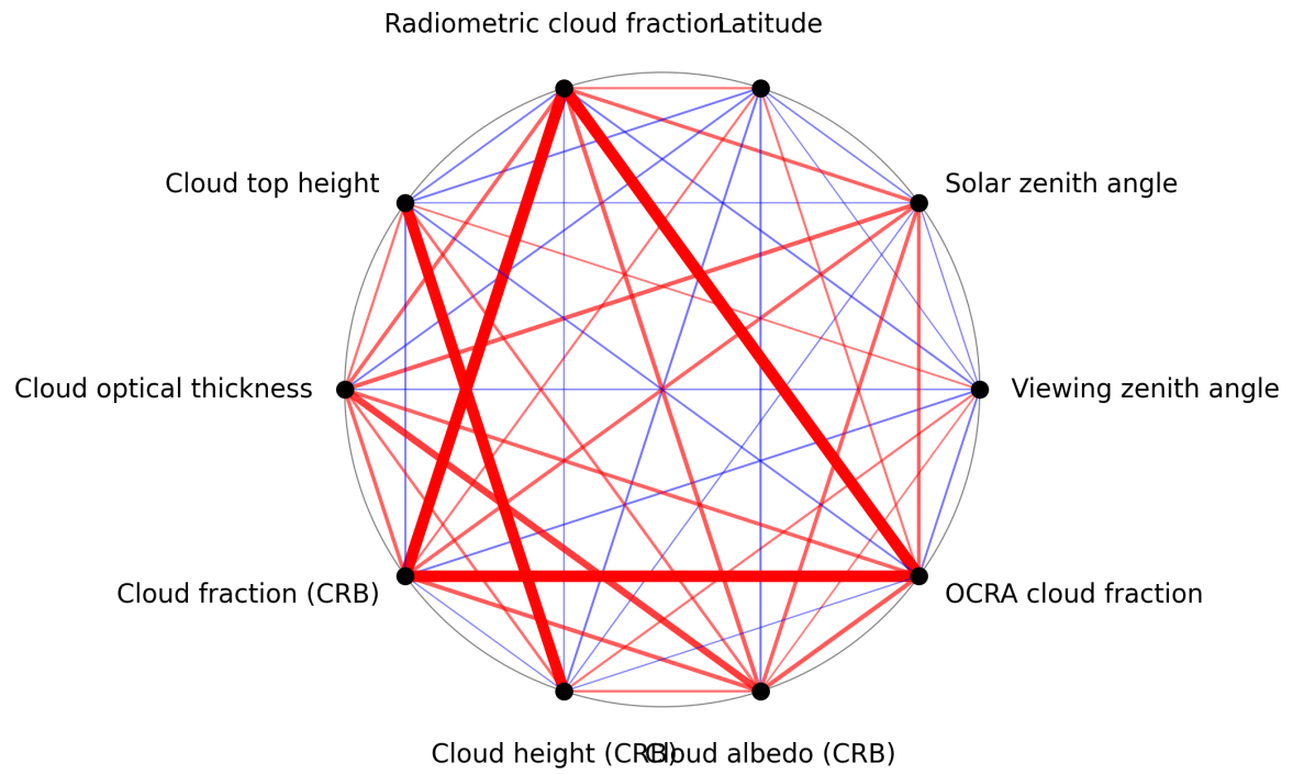
Figure 1: Map of correlation graph for 2024-08-27 to 2024-08-29.
