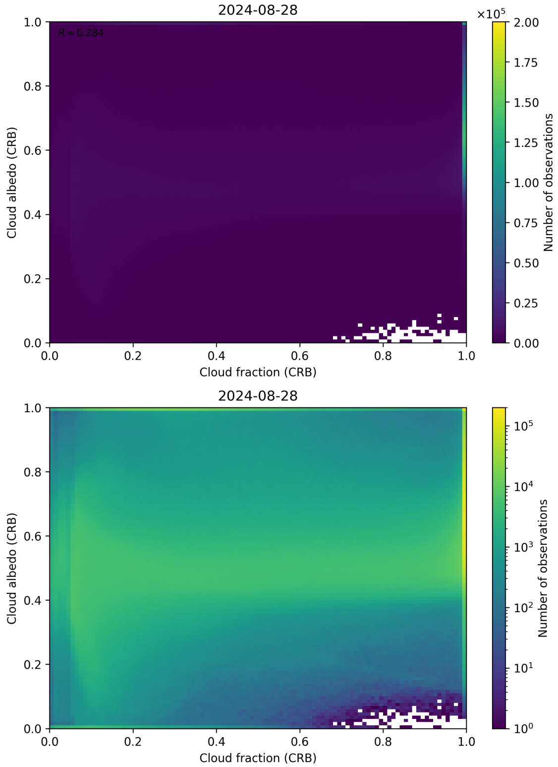
Figure 77: Scatter density plot of “Cloud fraction (CRB)” against “Cloud albedo (CRB)” for 2024-08-27 to 2024-08-29.
