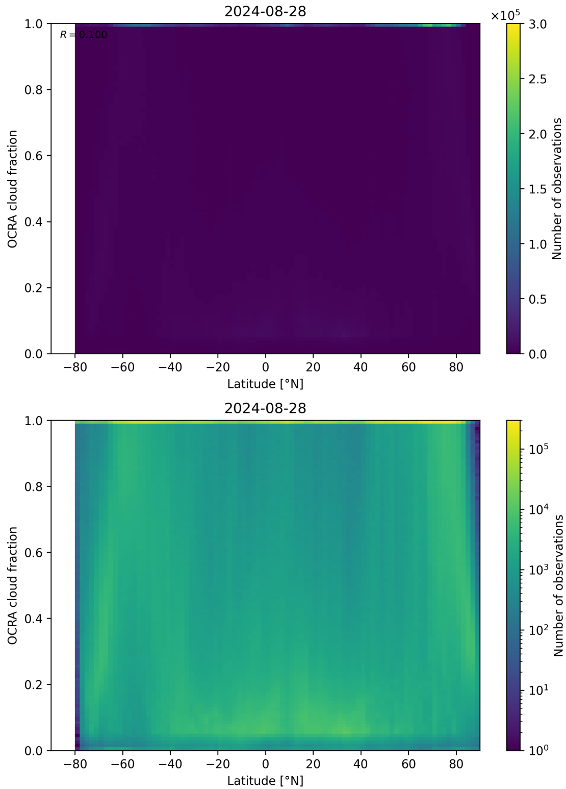
Figure 93: Scatter density plot of “Latitude” against “OCRA cloud fraction” for 2024-08-27 to 2024-08-29.
