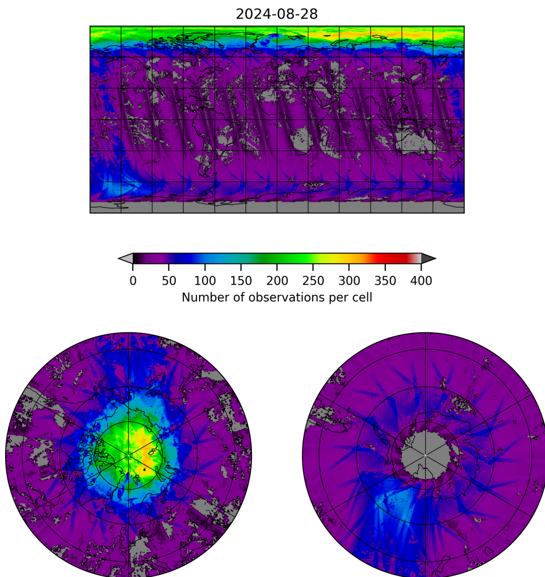
Figure 21: Map of the number of observations for 2024-08-27 to 2024-08-29
