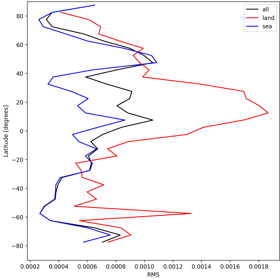
Figure 31: Zonal average of “RMS” for 2024-08-27 to 2024-08-29.
