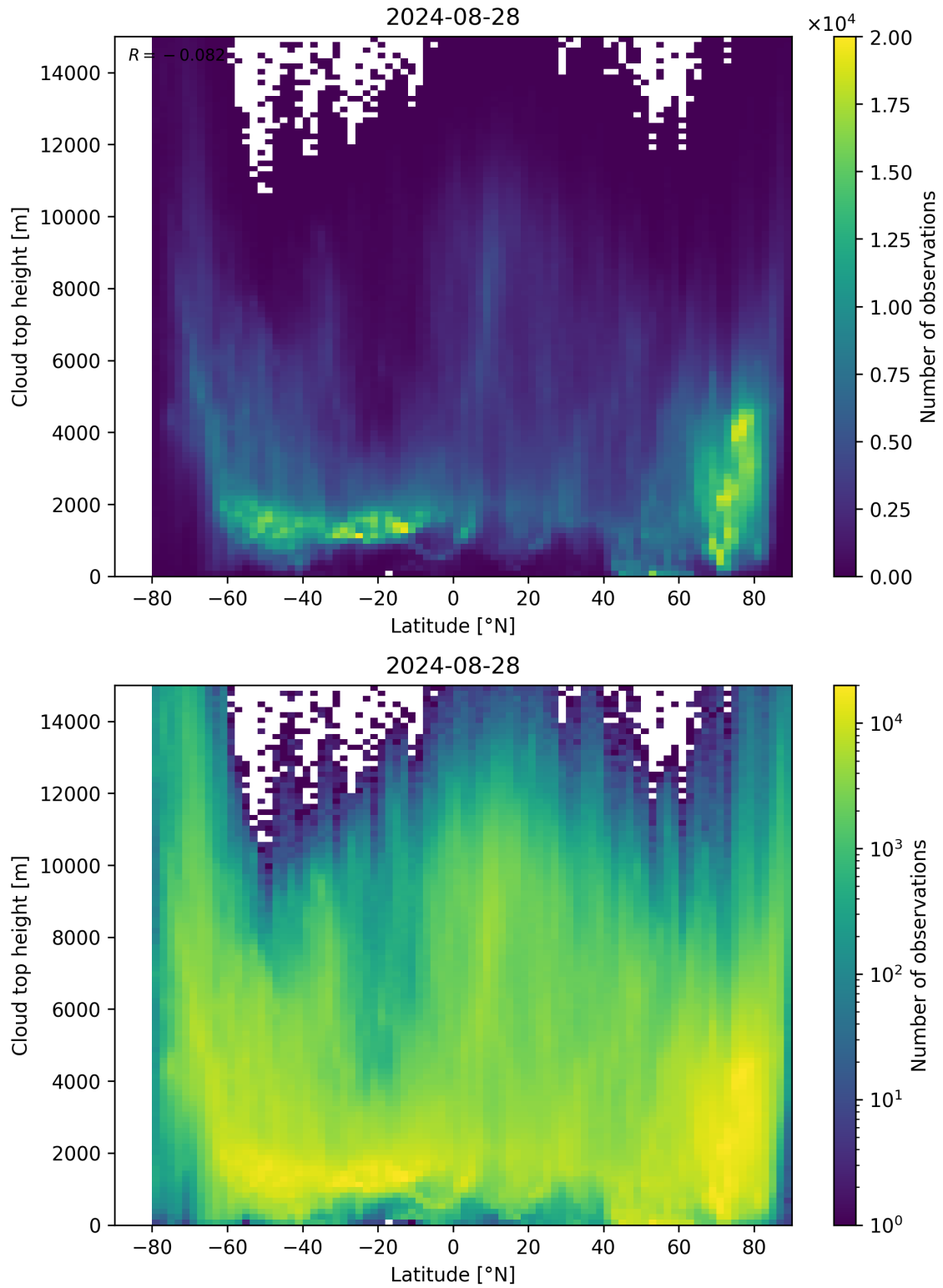
Figure 97: Scatter density plot of “Latitude” against “Cloud top height” for 2024-08-27 to 2024-08-29.
