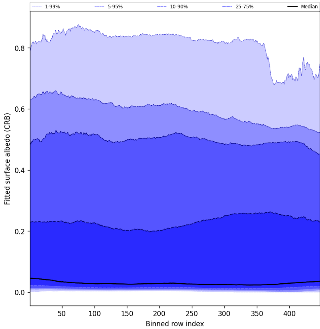
Figure 62: Along track statistics of “Fitted surface albedo (CRB)” for 2024-08-27 to 2024-08-29
