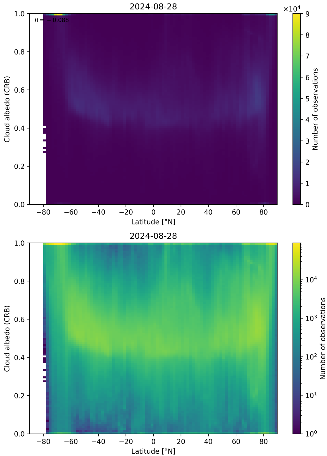
Figure 91: Scatter density plot of “Latitude” against “Cloud albedo (CRB)” for 2024-08-27 to 2024-08-29.
