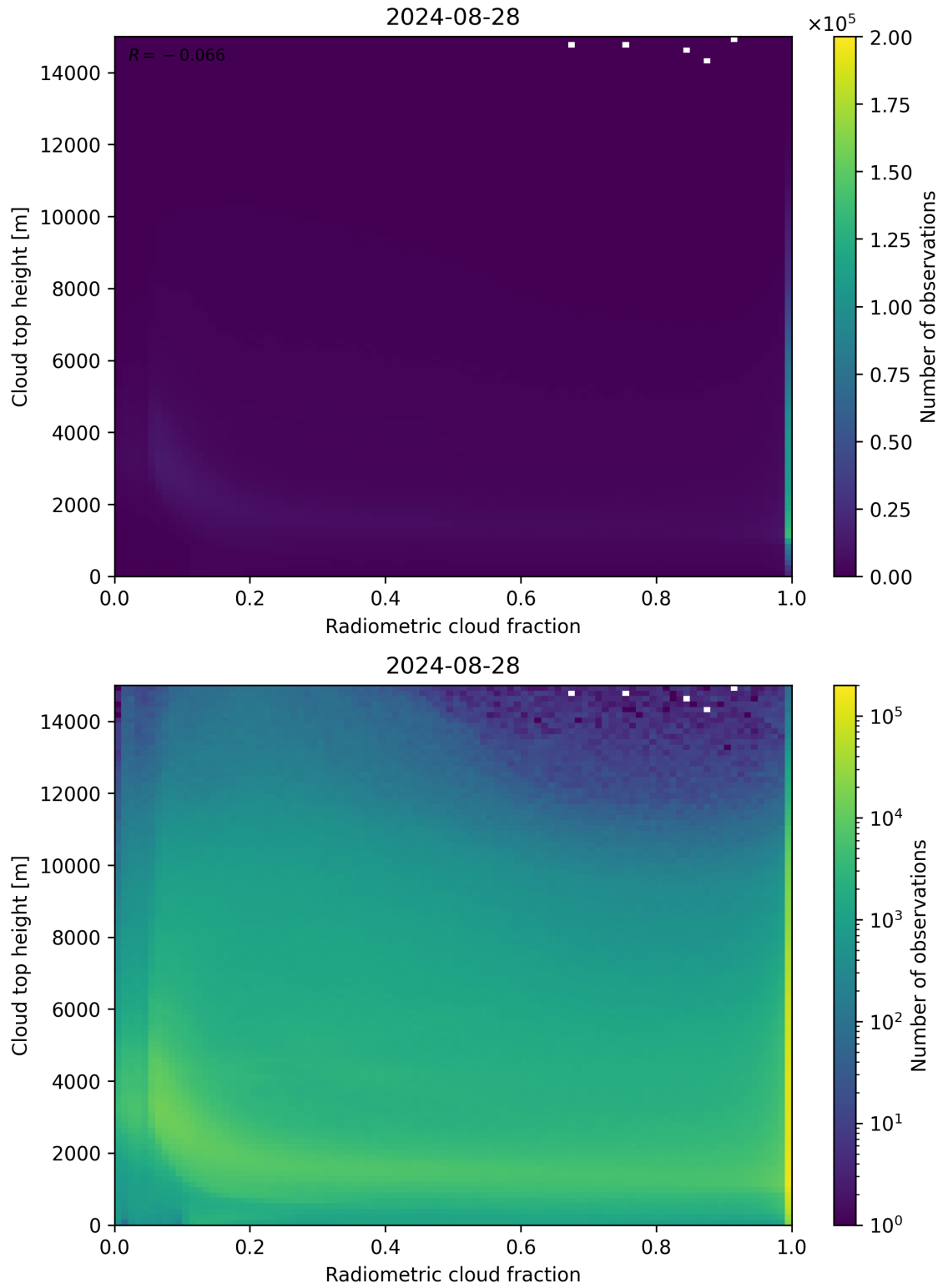
Figure 76: Scatter density plot of “Radiometric cloud fraction” against “Cloud top height” for 2024-08-27 to 2024-08-29.
