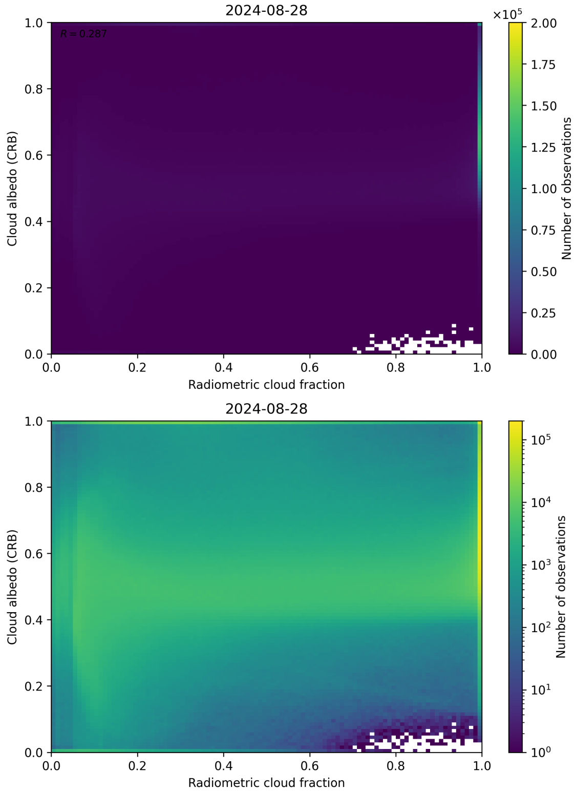
Figure 71: Scatter density plot of “Radiometric cloud fraction” against “Cloud albedo (CRB)” for 2024-08-27 to 2024-08-29.
