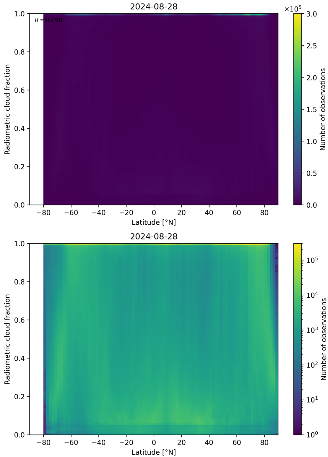
Figure 92: Scatter density plot of “Latitude” against “Radiometric cloud fraction” for 2024-08-27 to 2024-08-29.
