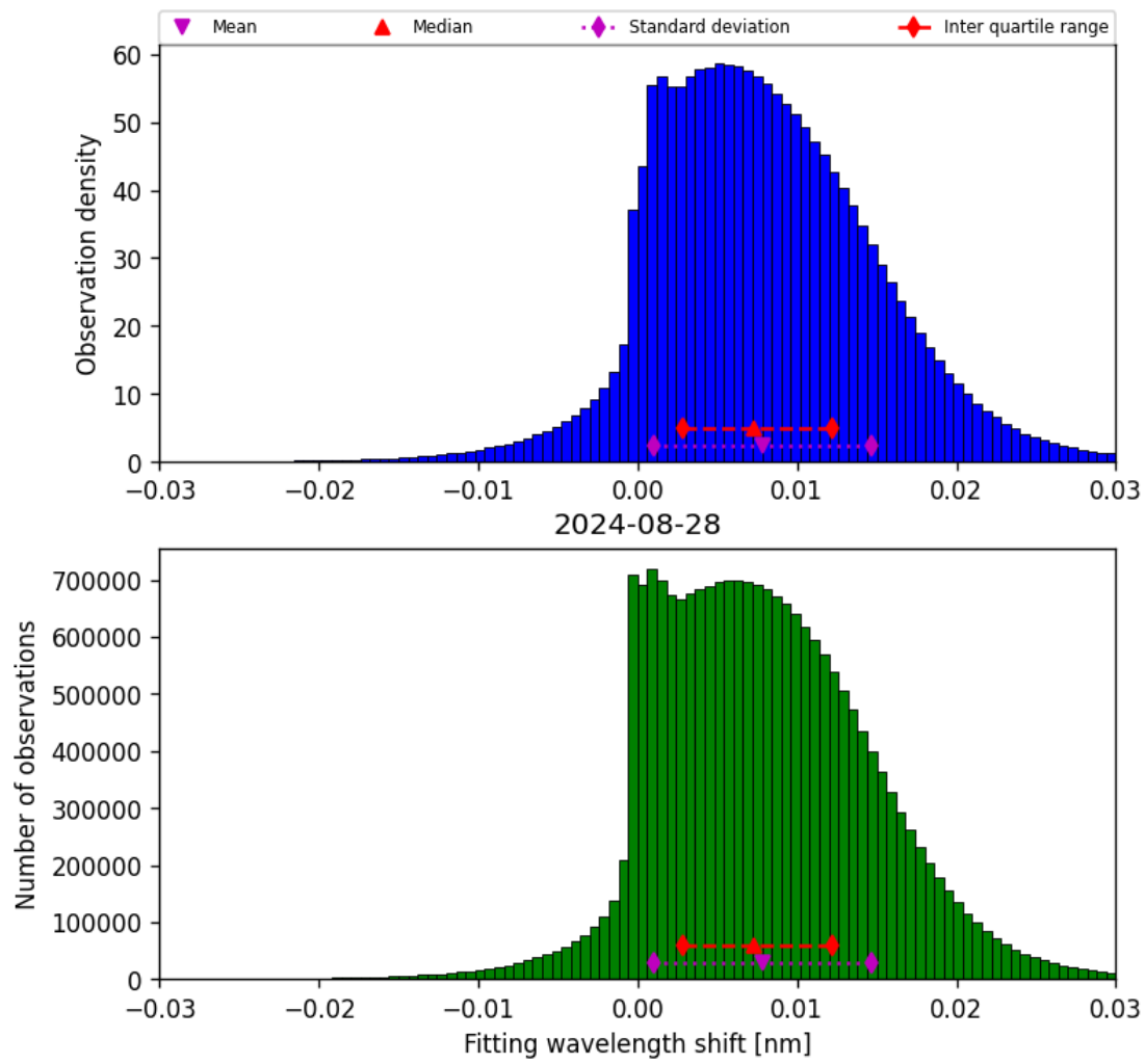
Figure 49: Histogram of “Fitting wavelength shift” for 2024-08-27 to 2024-08-29
