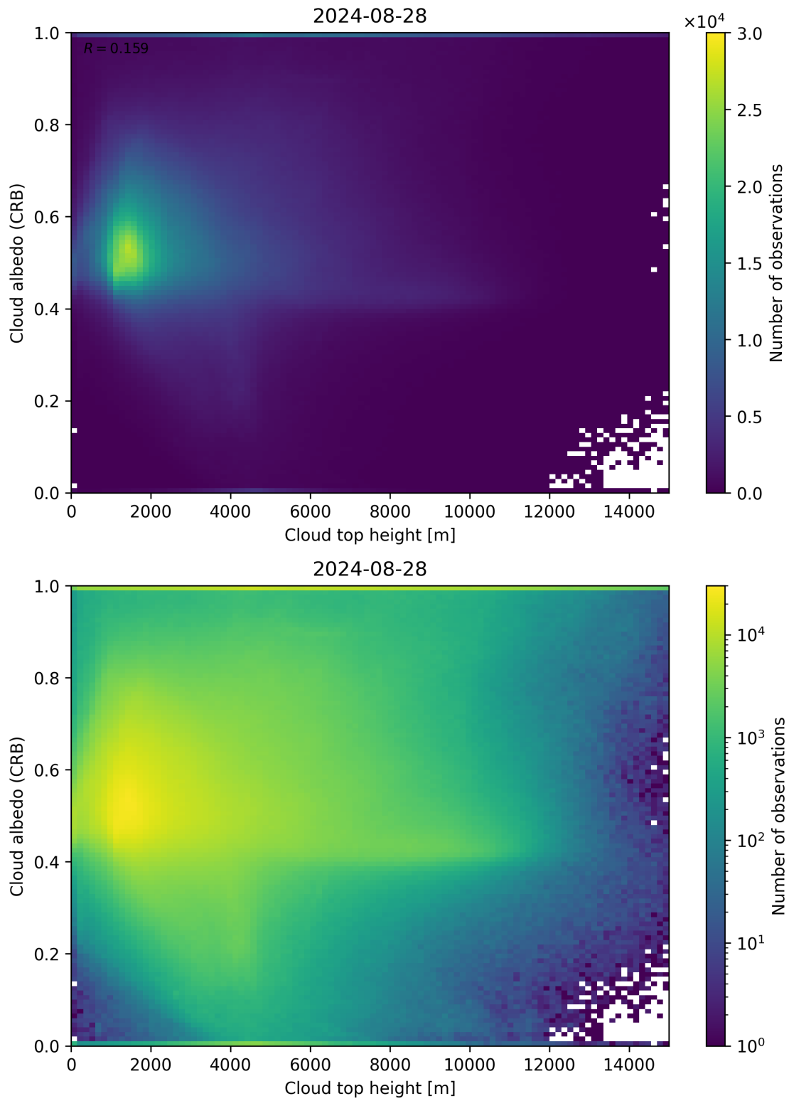
Figure 86: Scatter density plot of “Cloud top height” against “Cloud albedo (CRB)” for 2024-08-27 to 2024-08-29.
