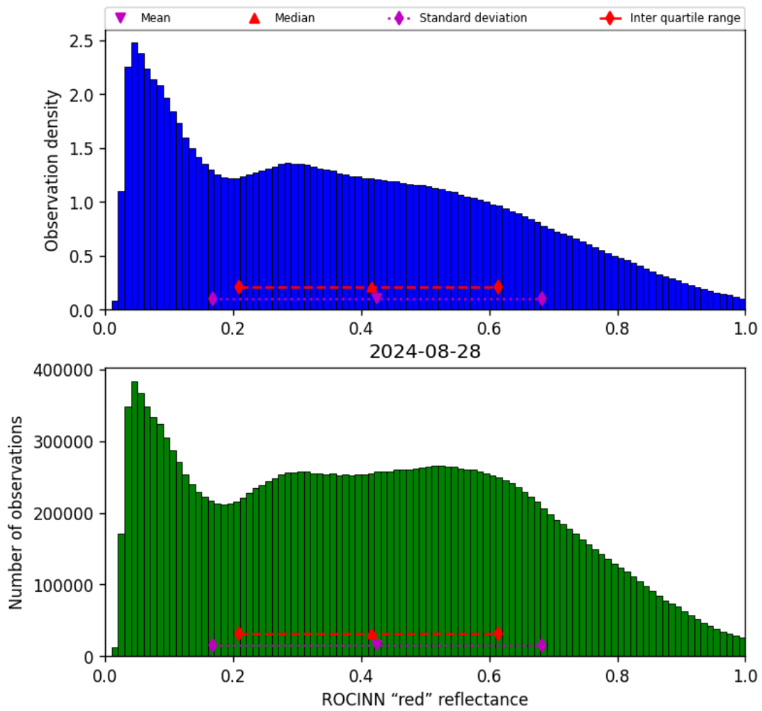
Figure 53: Histogram of “ROCINN “red” reflectance” for 2024-08-27 to 2024-08-29
