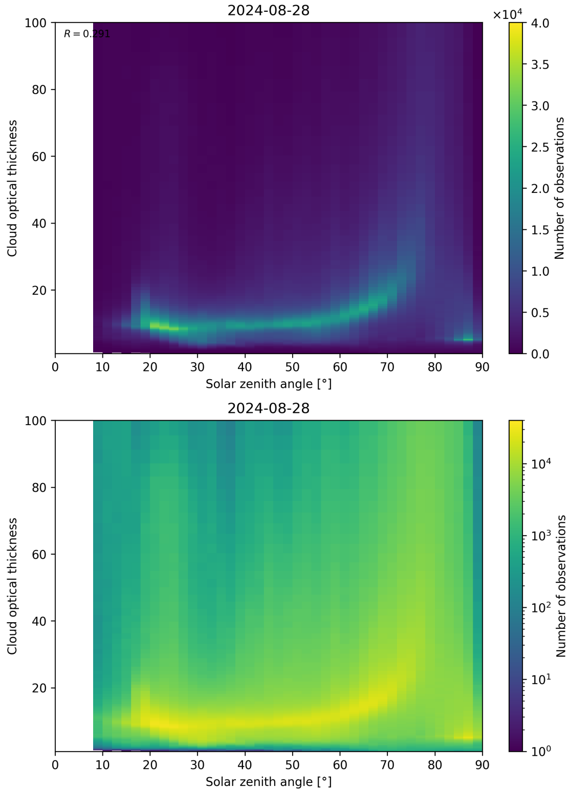
Figure 103: Scatter density plot of “Solar zenith angle” against “Cloud optical thickness” for 2024-08-27 to 2024-08-29.
