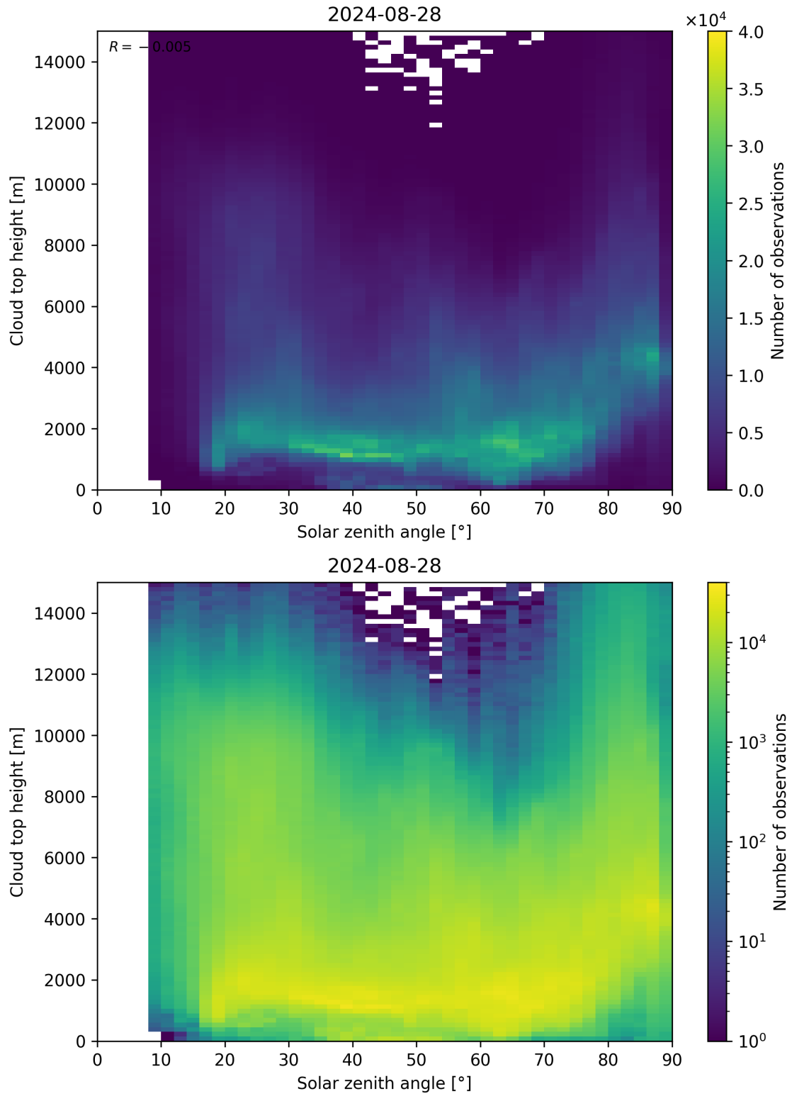
Figure 104: Scatter density plot of “Solar zenith angle” against “Cloud top height” for 2024-08-27 to 2024-08-29.
