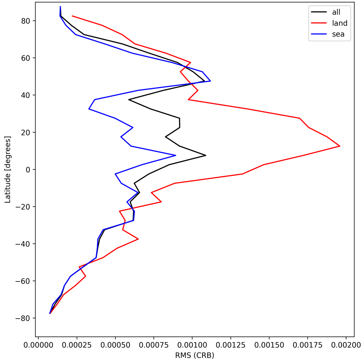
Figure 32: Zonal average of “RMS (CRB)” for 2024-08-27 to 2024-08-29.
