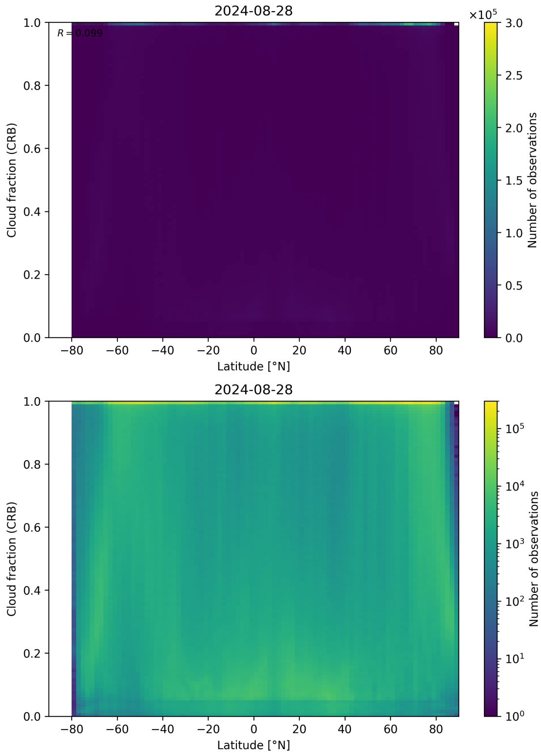
Figure 94: Scatter density plot of “Latitude” against “Cloud fraction (CRB)” for 2024-08-27 to 2024-08-29.
