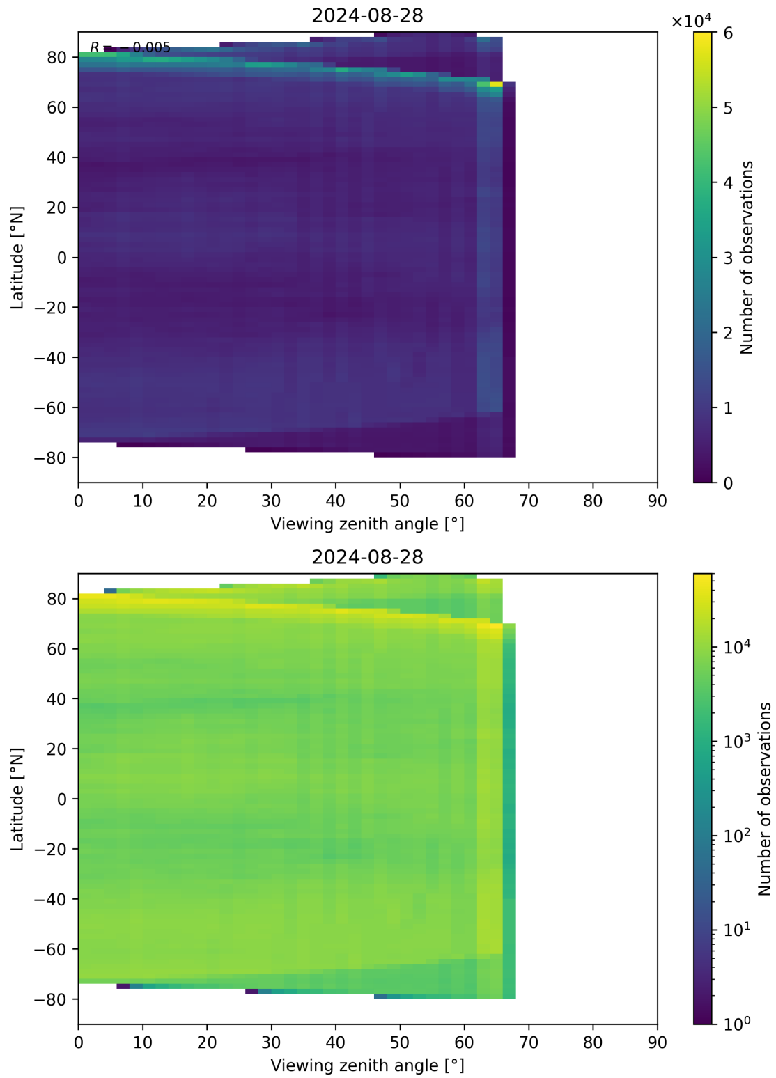
Figure 113: Scatter density plot of “Viewing zenith angle” against “Latitude” for 2024-08-27 to 2024-08-29.
