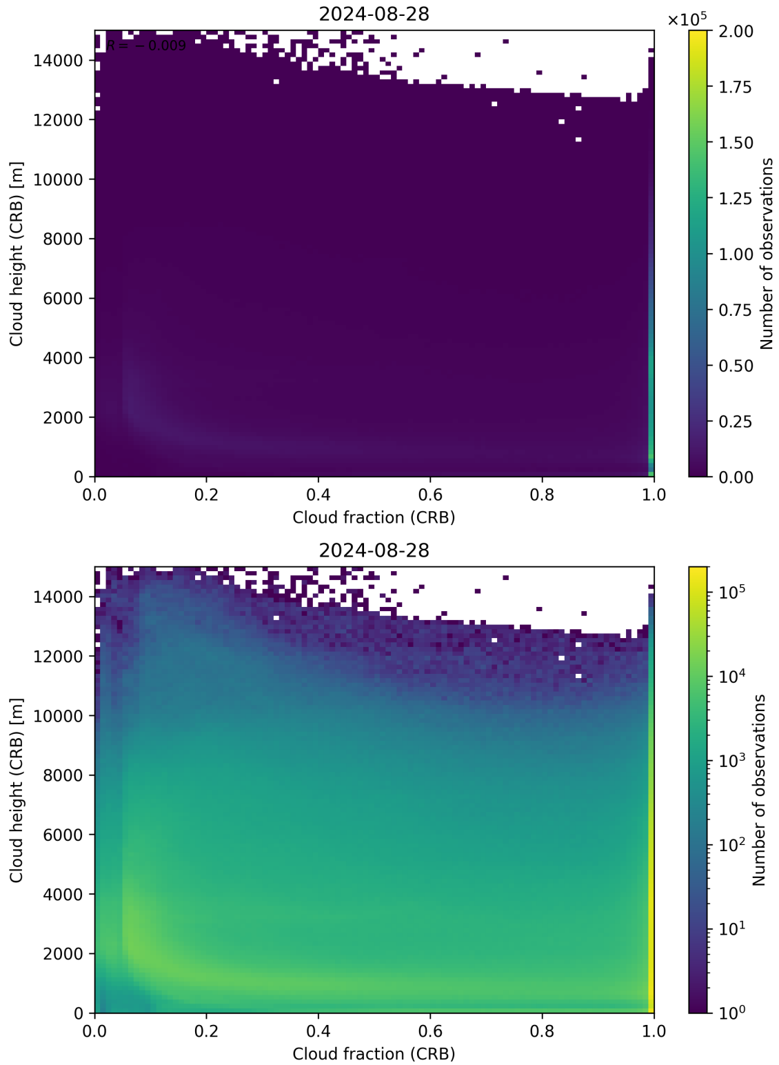
Figure 79: Scatter density plot of “Cloud fraction (CRB)” against “Cloud height (CRB)” for 2024-08-27 to 2024-08-29.
