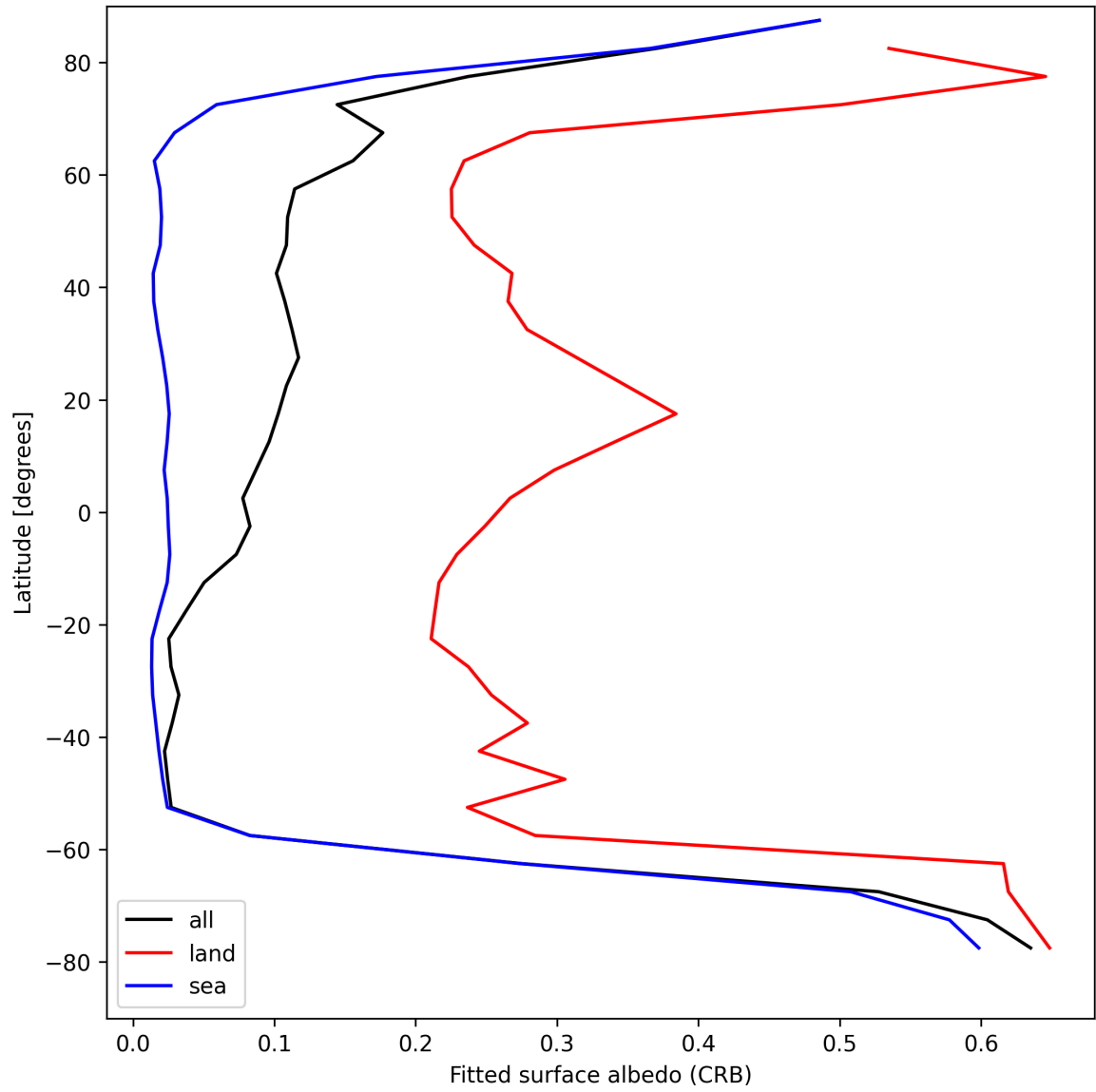
Figure 30: Zonal average of “Fitted surface albedo (CRB)” for 2024-08-27 to 2024-08-29.
