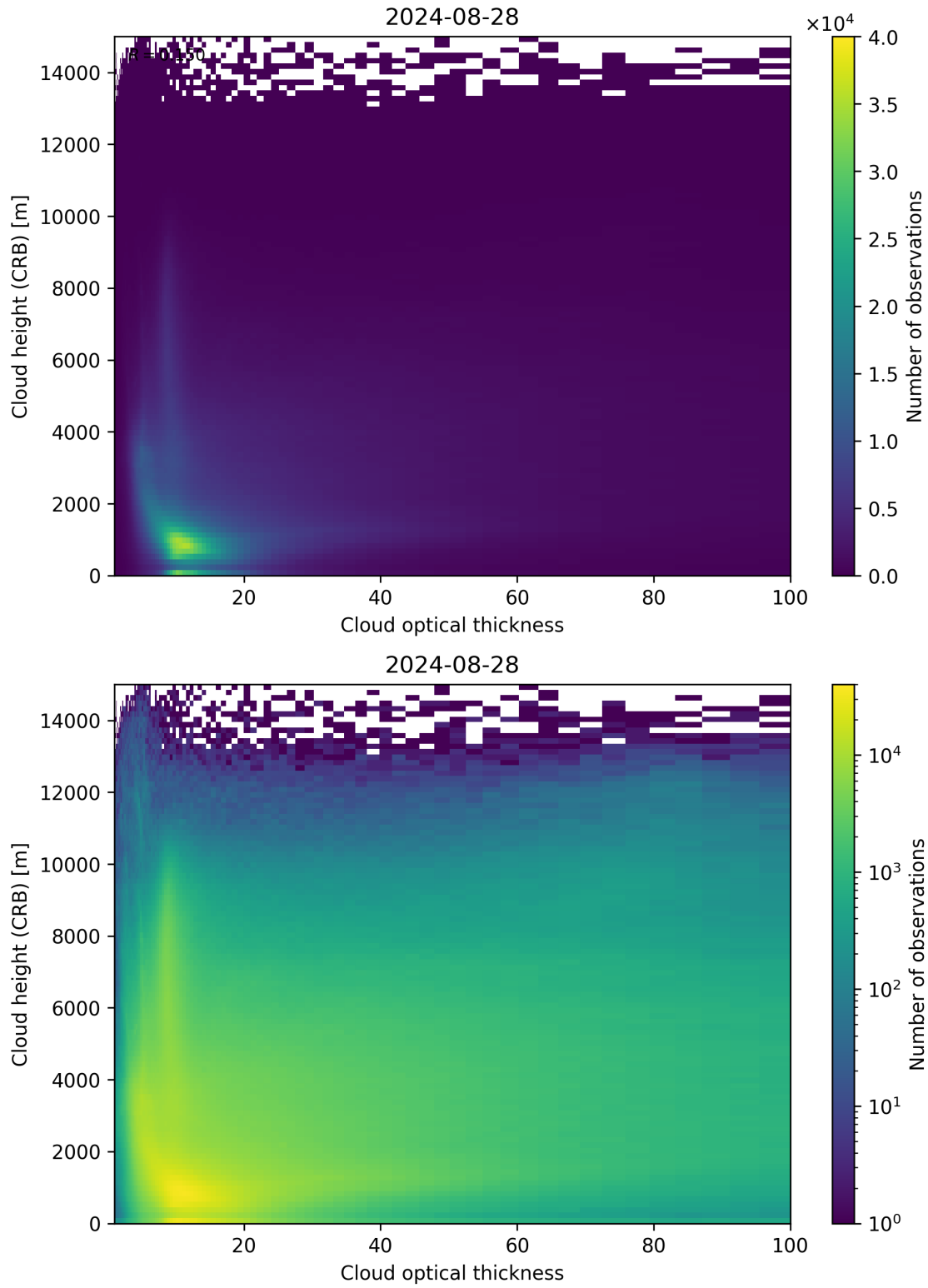
Figure 85: Scatter density plot of “Cloud optical thickness” against “Cloud height (CRB)” for 2024-08-27 to 2024-08-29.
