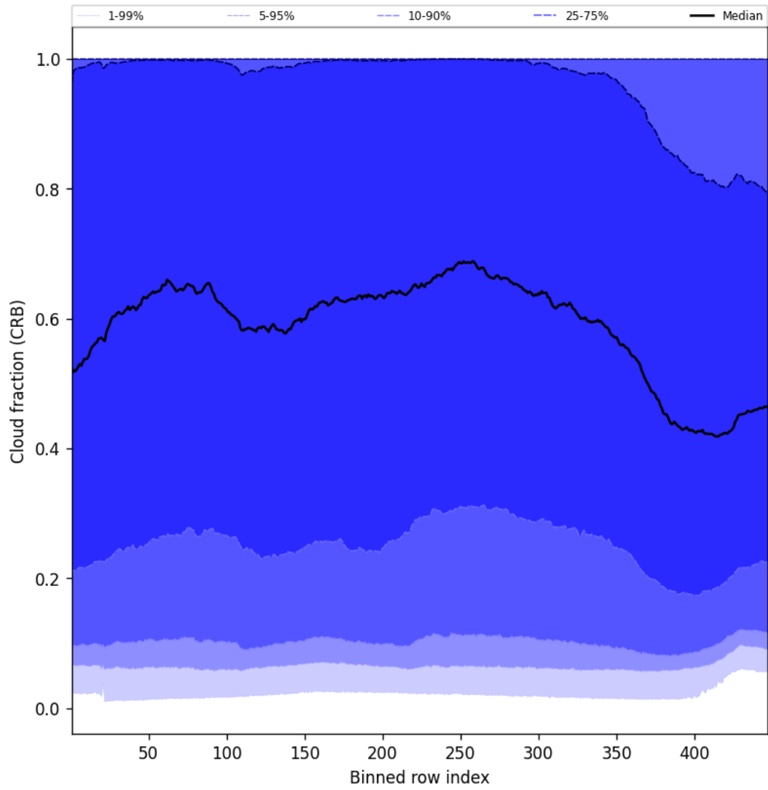
Figure 58: Along track statistics of “Cloud fraction (CRB)” for 2024-08-27 to 2024-08-29
