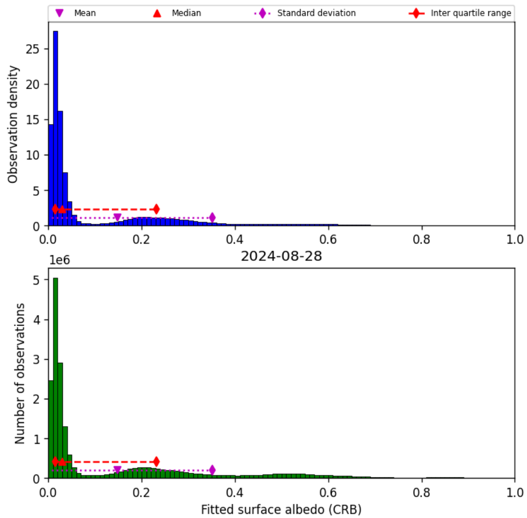
Figure 46: Histogram of “Fitted surface albedo (CRB)” for 2024-08-27 to 2024-08-29
