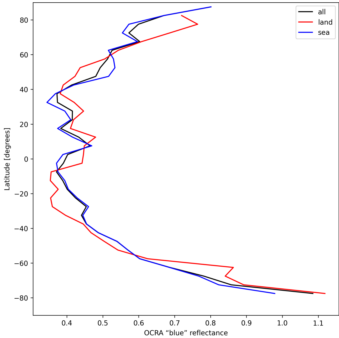
Figure 35: Zonal average of “OCRA “blue” reflectance” for 2024-08-27 to 2024-08-29.
