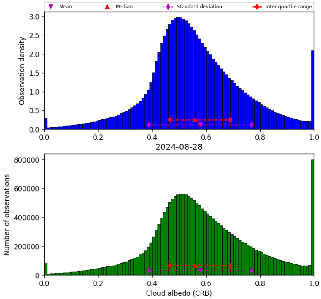
Figure 44: Histogram of “Cloud albedo (CRB)” for 2024-08-27 to 2024-08-29
