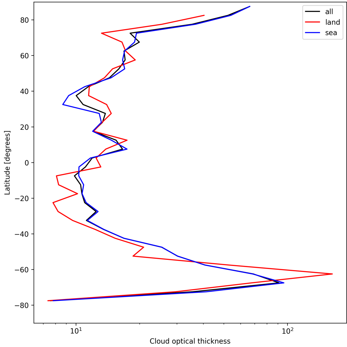
Figure 25: Zonal average of “Cloud optical thickness” for 2024-08-27 to 2024-08-29.
