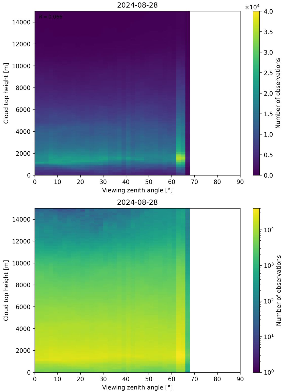
Figure 112: Scatter density plot of “Viewing zenith angle” against “Cloud top height” for 2024-08-27 to 2024-08-29.
