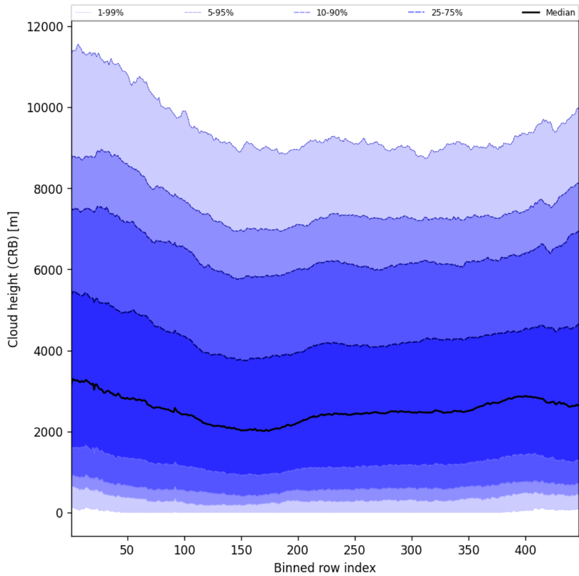
Figure 59: Along track statistics of “Cloud height (CRB)” for 2024-08-27 to 2024-08-29
