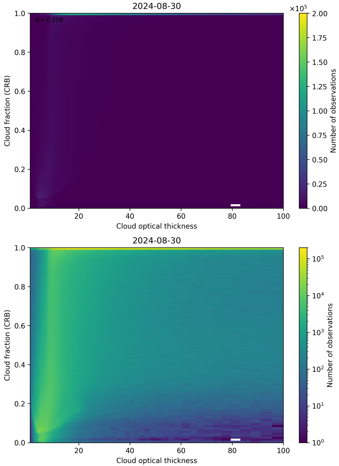
Figure 84: Scatter density plot of “Cloud optical thickness” against “Cloud fraction (CRB)” for 2024-08-29 to 2024-08-31.
