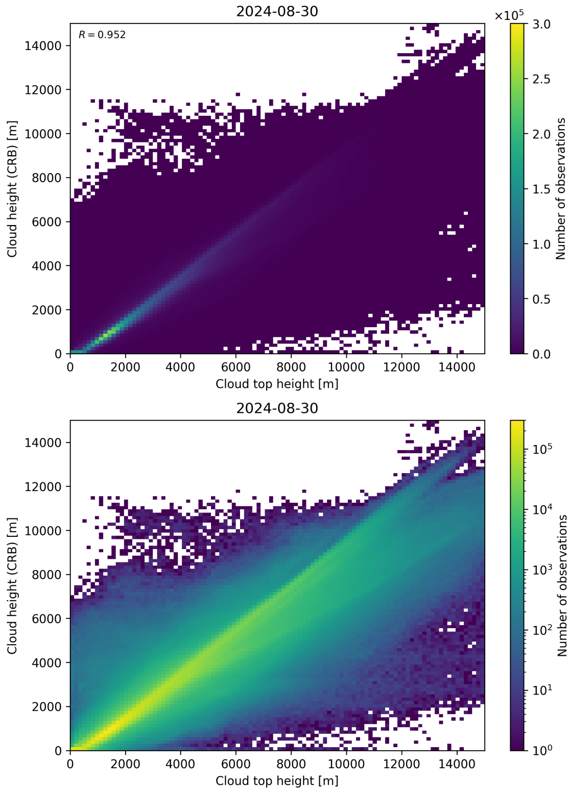
Figure 89: Scatter density plot of “Cloud top height” against “Cloud height (CRB)” for 2024-08-29 to 2024-08-31.
