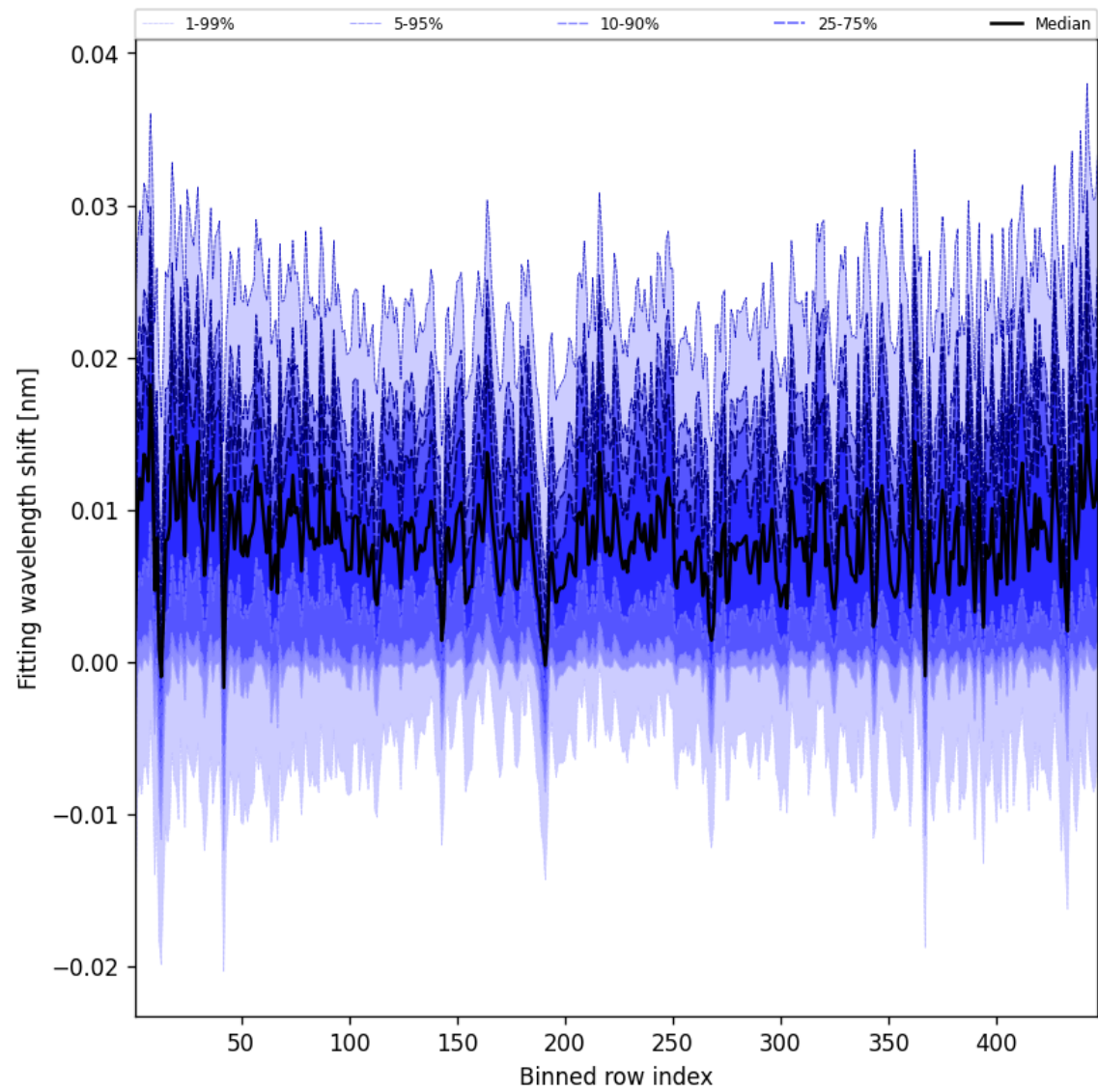
Figure 65: Along track statistics of “Fitting wavelength shift” for 2024-08-29 to 2024-08-31
