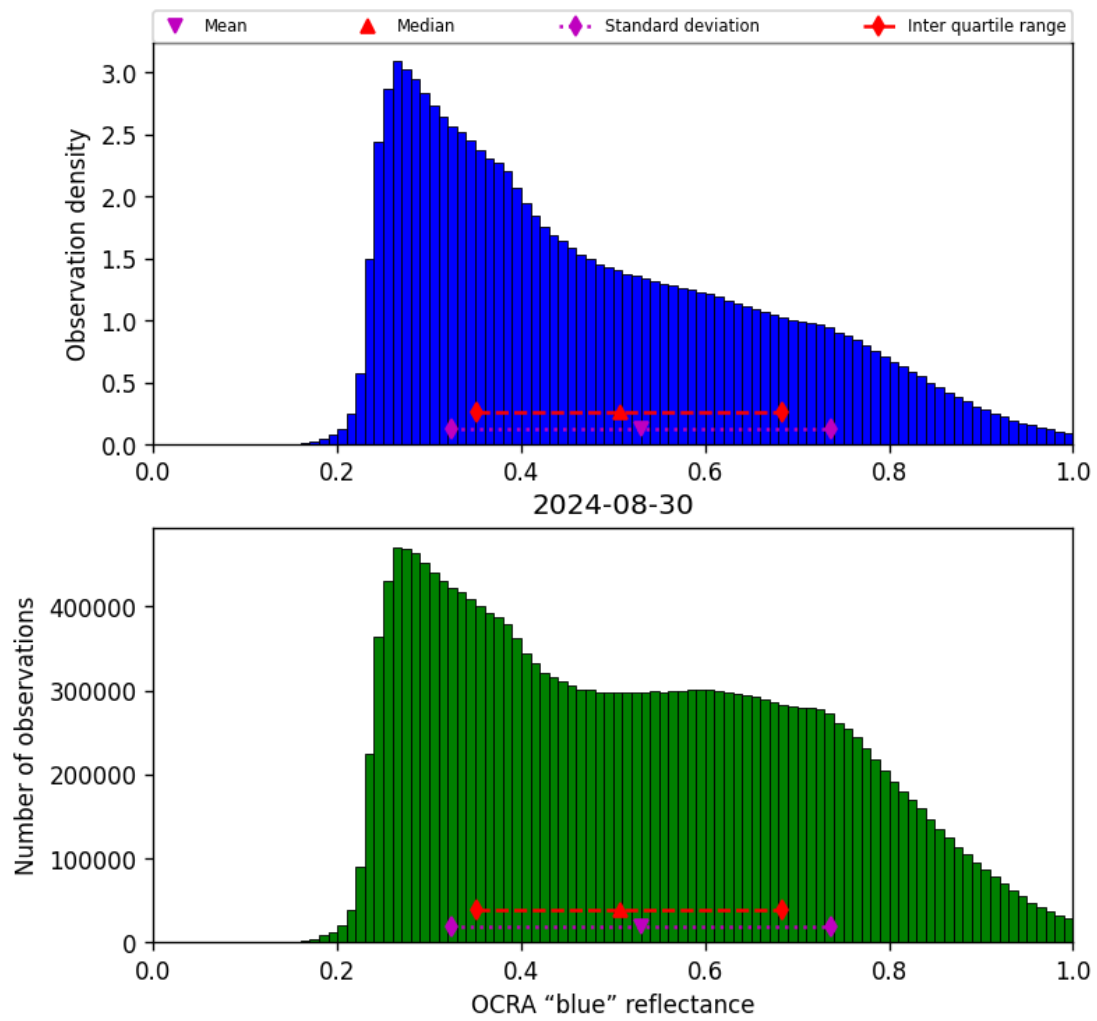
Figure 51: Histogram of “OCRA “blue” reflectance” for 2024-08-29 to 2024-08-31
