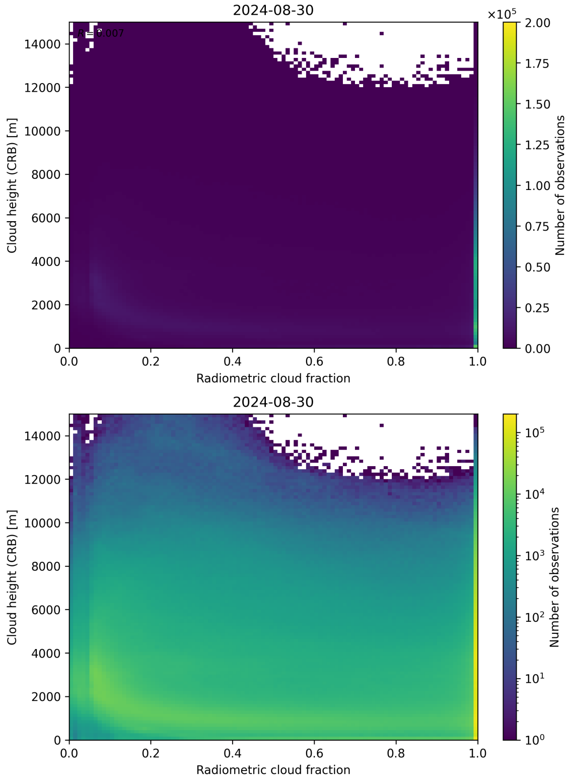
Figure 74: Scatter density plot of “Radiometric cloud fraction” against “Cloud height (CRB)” for 2024-08-29 to 2024-08-31.
