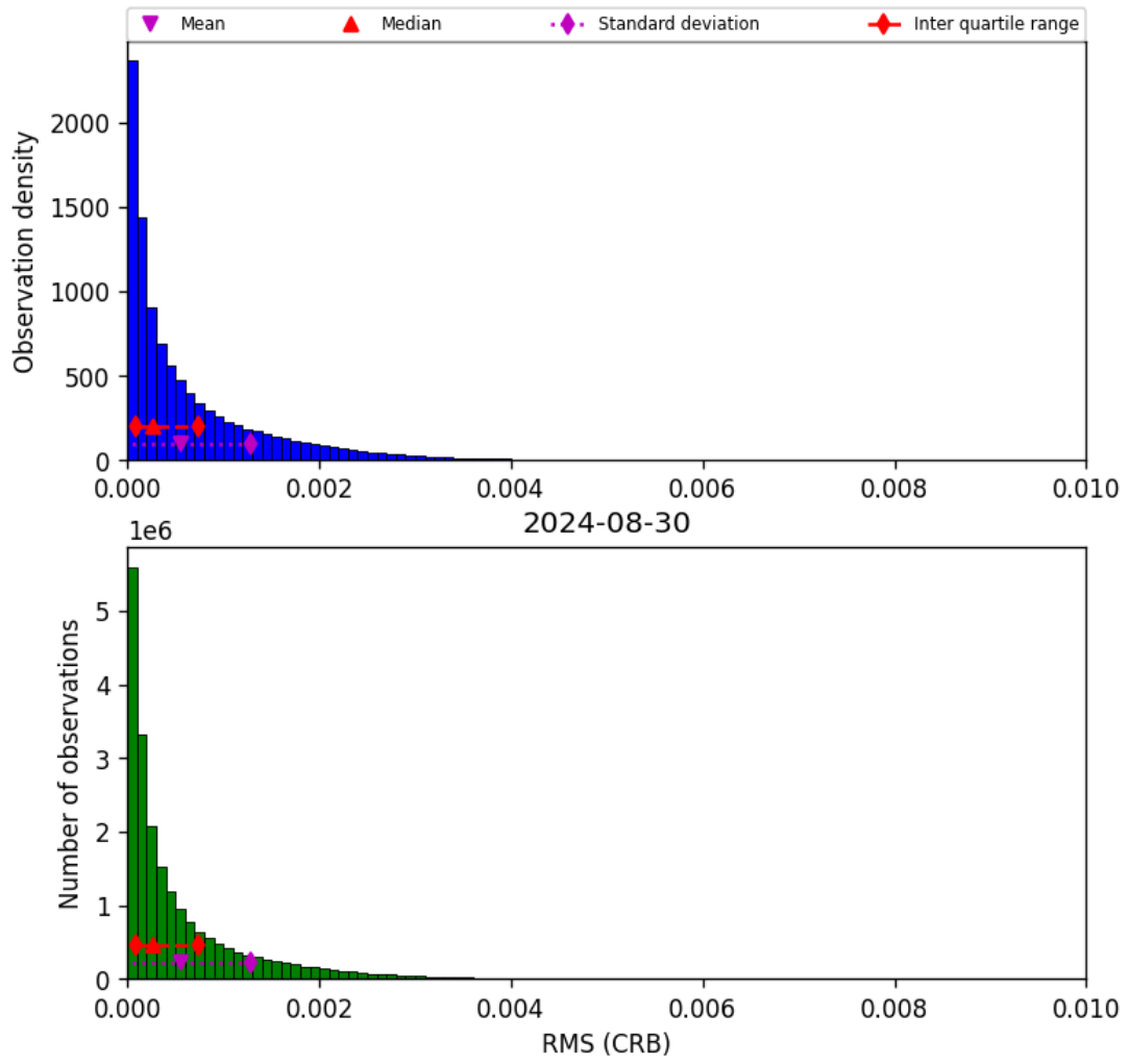
Figure 48: Histogram of “RMS (CRB)” for 2024-08-29 to 2024-08-31
