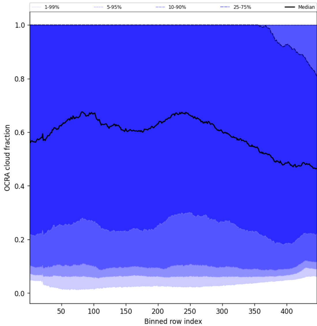
Figure 66: Along track statistics of “OCRA cloud fraction” for 2024-08-29 to 2024-08-31
