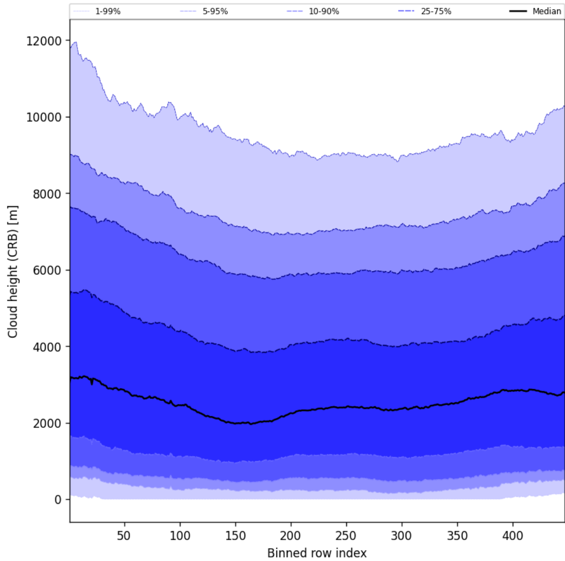
Figure 59: Along track statistics of “Cloud height (CRB)” for 2024-08-29 to 2024-08-31
