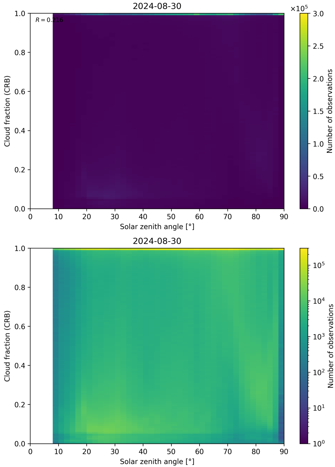
Figure 101: Scatter density plot of “Solar zenith angle” against “Cloud fraction (CRB)” for 2024-08-29 to 2024-08-31.
