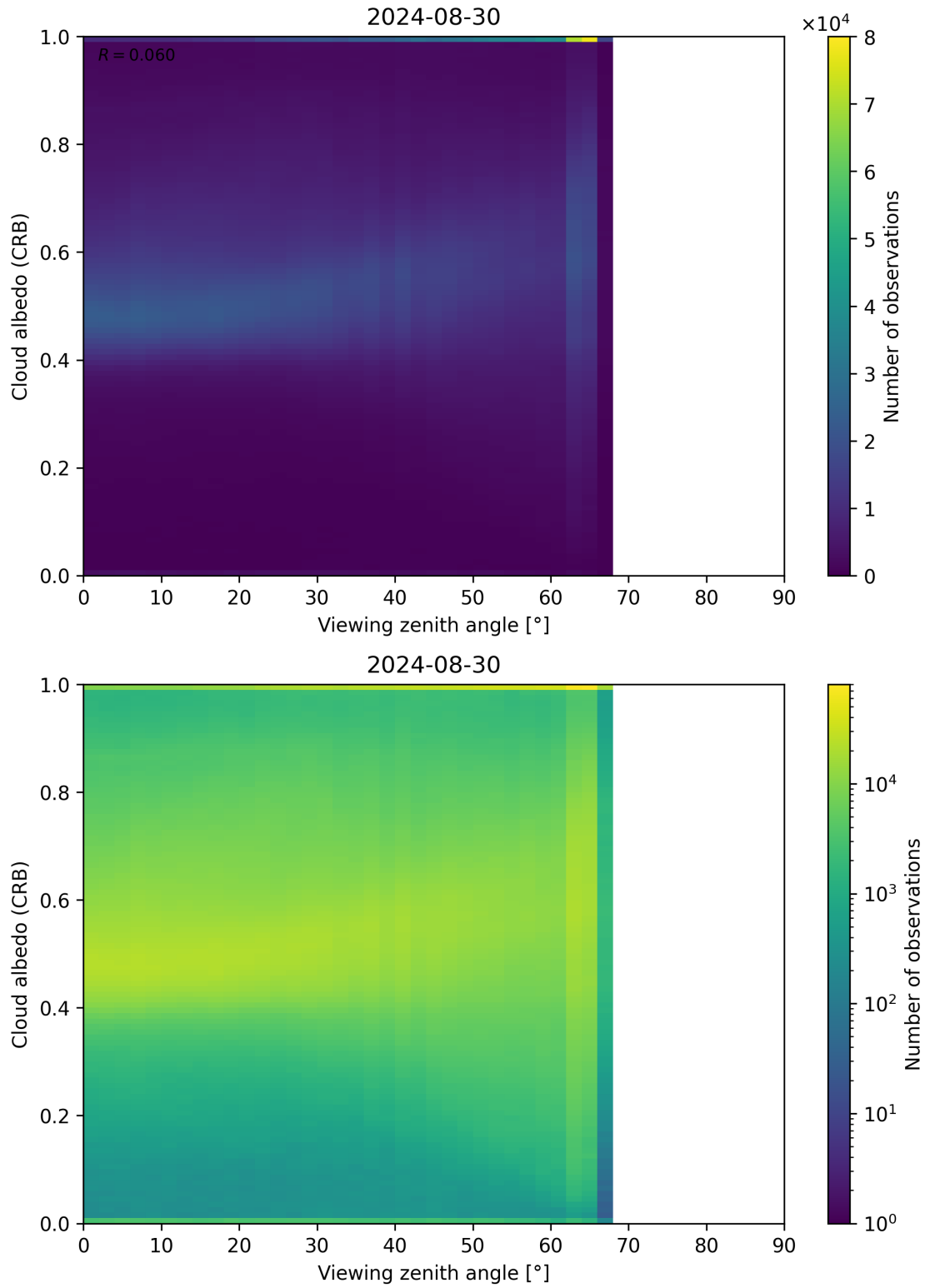
Figure 106: Scatter density plot of “Viewing zenith angle” against “Cloud albedo (CRB)” for 2024-08-29 to 2024-08-31.
