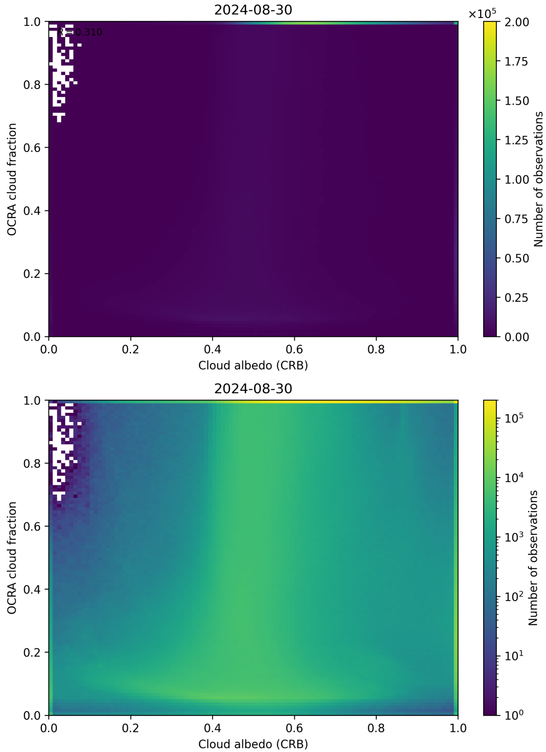
Figure 70: Scatter density plot of “Cloud albedo (CRB)” against “OCRA cloud fraction” for 2024-08-29 to 2024-08-31.
