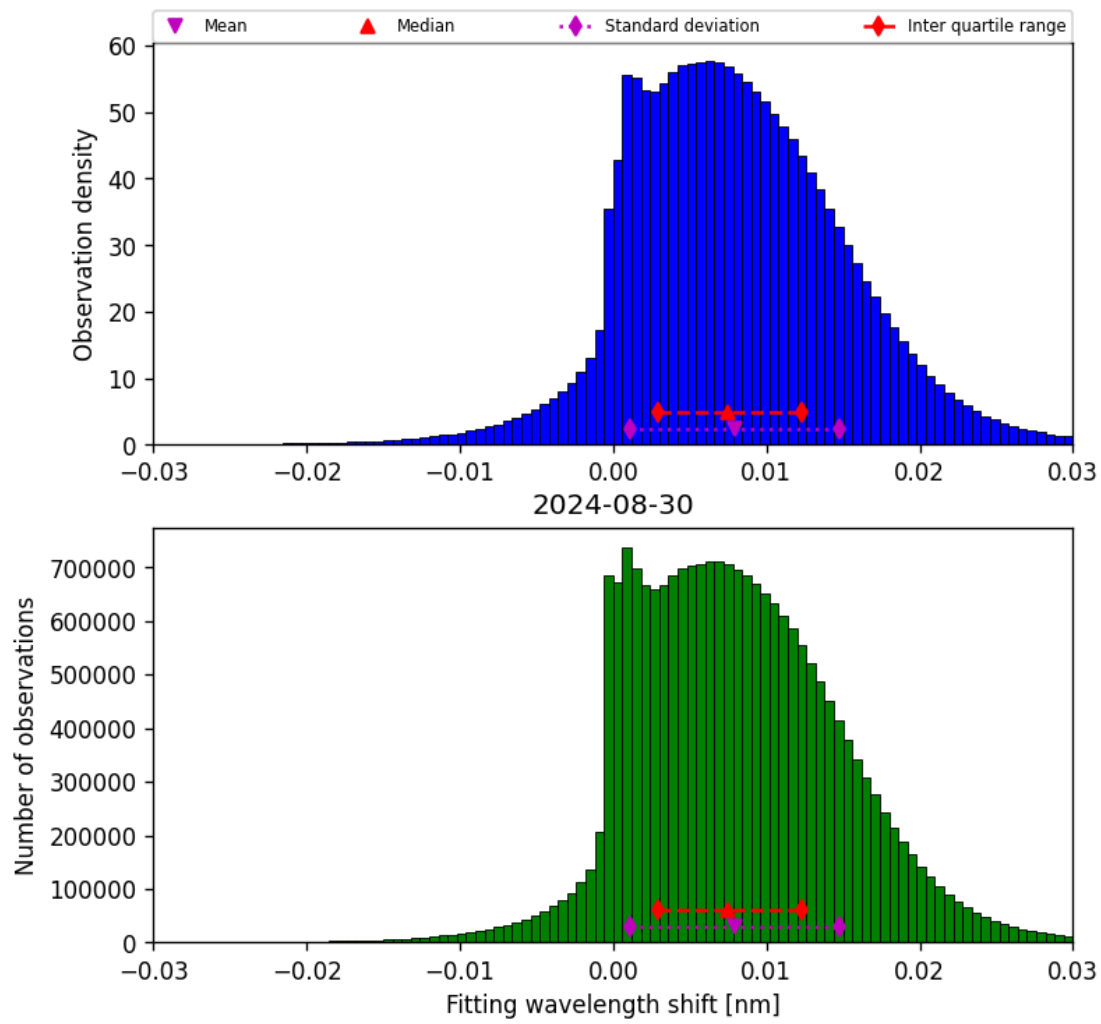
Figure 49: Histogram of “Fitting wavelength shift” for 2024-08-29 to 2024-08-31
