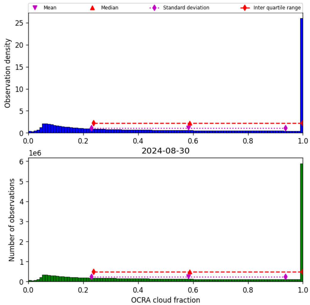
Figure 50: Histogram of “OCRA cloud fraction” for 2024-08-29 to 2024-08-31
