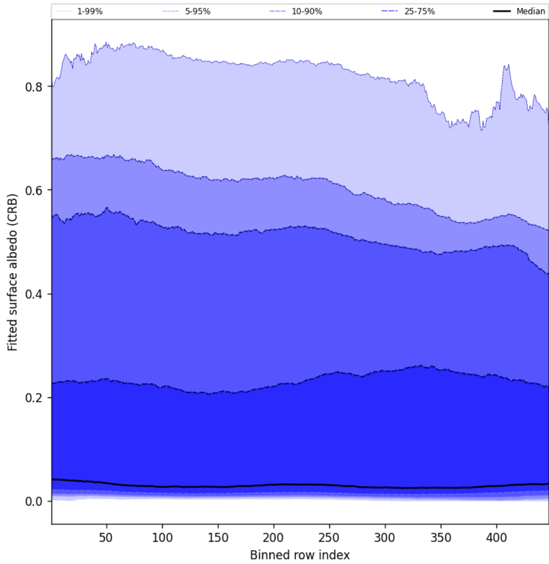
Figure 62: Along track statistics of “Fitted surface albedo (CRB)” for 2024-08-29 to 2024-08-31
