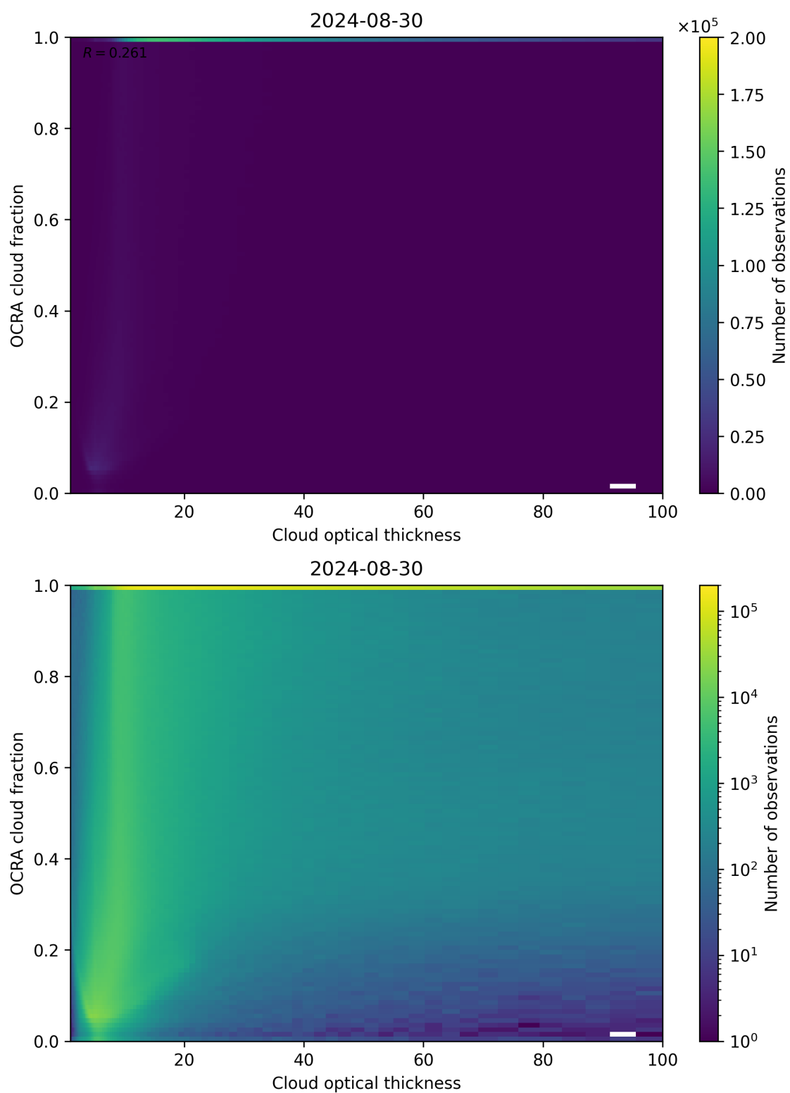
Figure 83: Scatter density plot of “Cloud optical thickness” against “OCRA cloud fraction” for 2024-08-29 to 2024-08-31.
