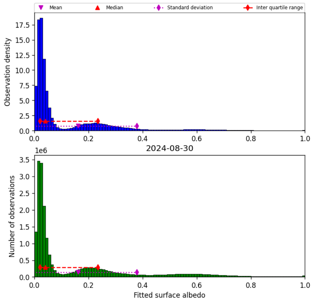
Figure 45: Histogram of “Fitted surface albedo” for 2024-08-29 to 2024-08-31
