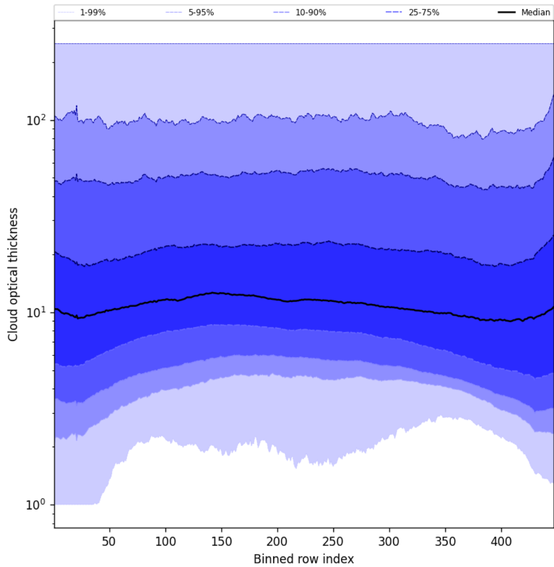
Figure 57: Along track statistics of “Cloud optical thickness” for 2024-08-29 to 2024-08-31
