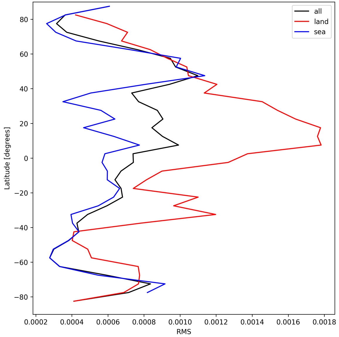
Figure 31: Zonal average of “RMS” for 2024-08-29 to 2024-08-31.
