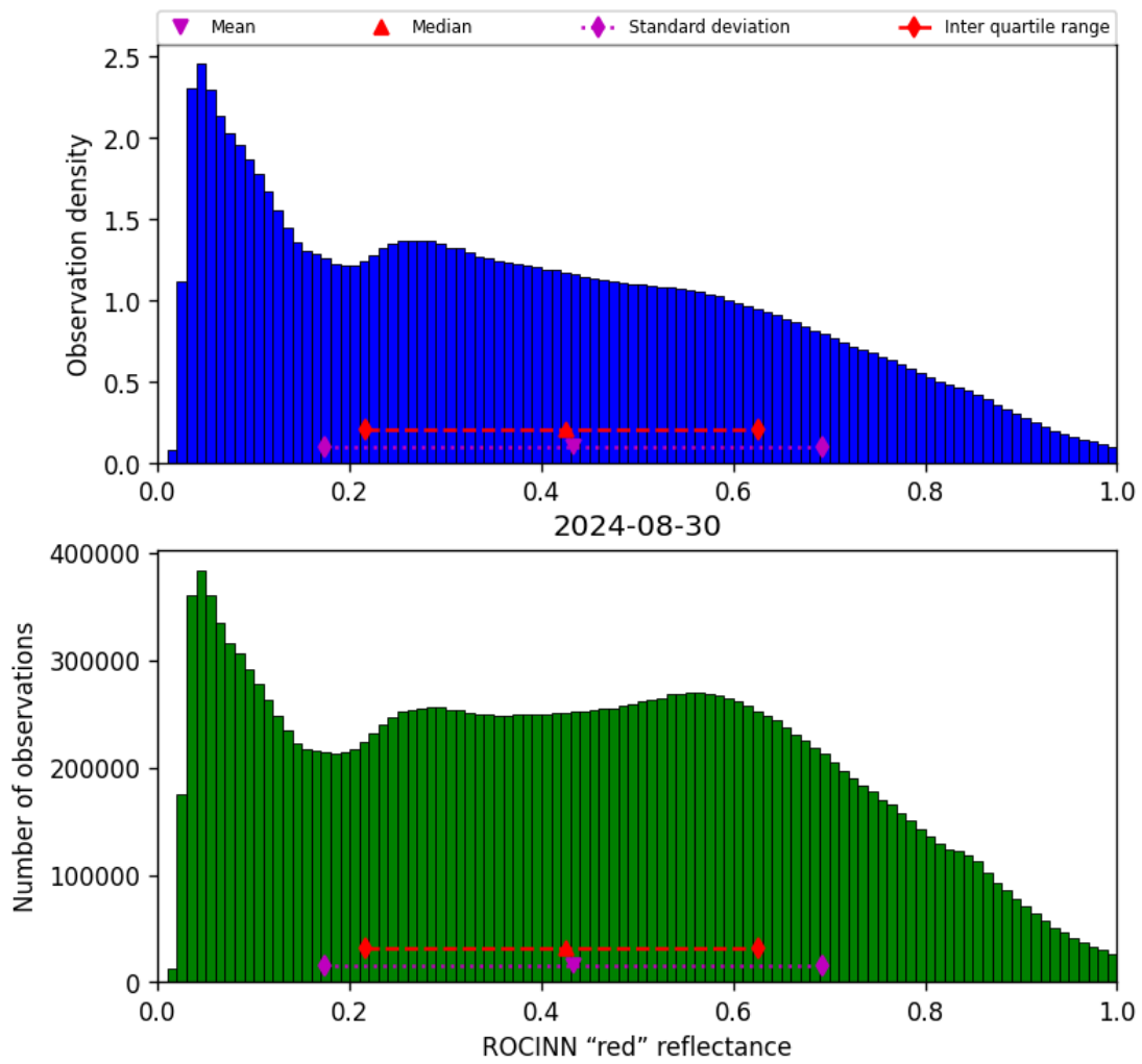
Figure 53: Histogram of “ROCINN “red” reflectance” for 2024-08-29 to 2024-08-31
