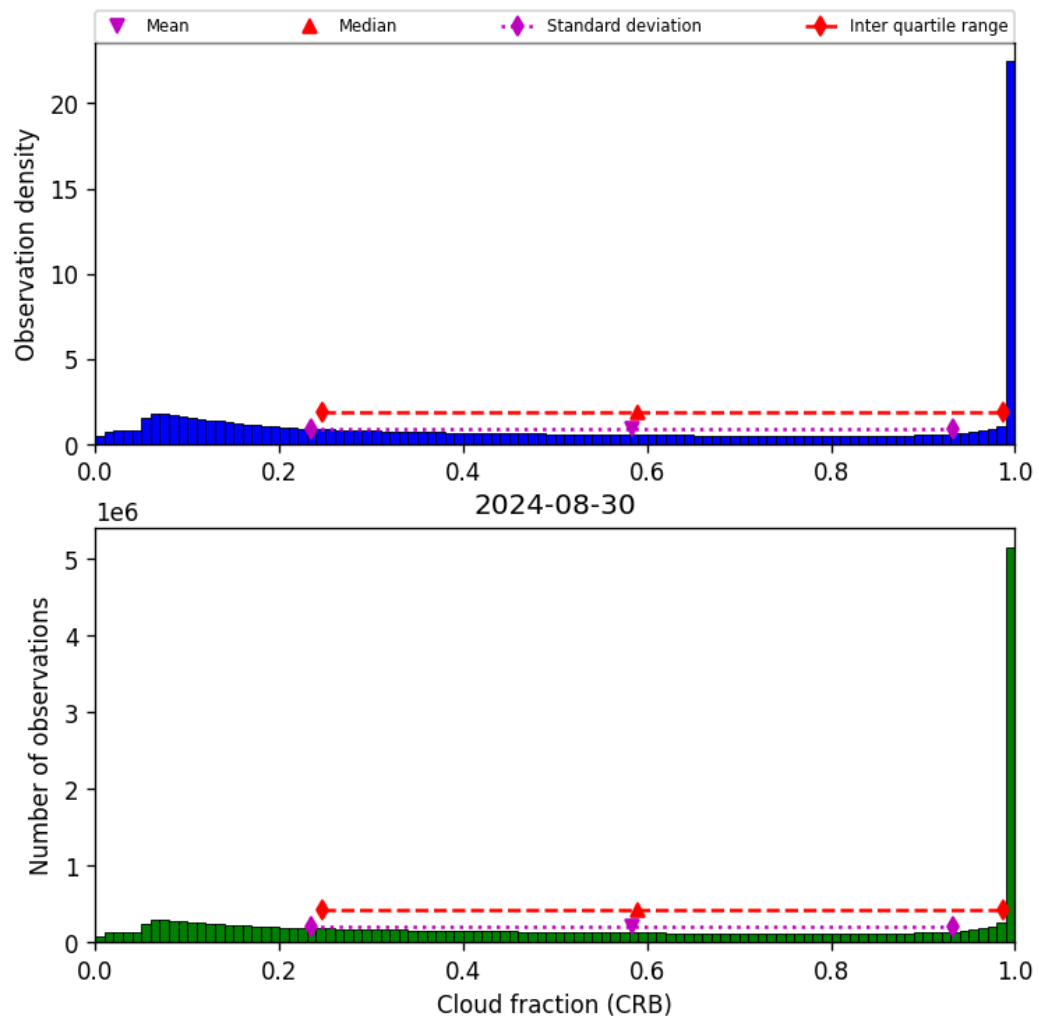
Figure 42: Histogram of “Cloud fraction (CRB)” for 2024-08-29 to 2024-08-31
