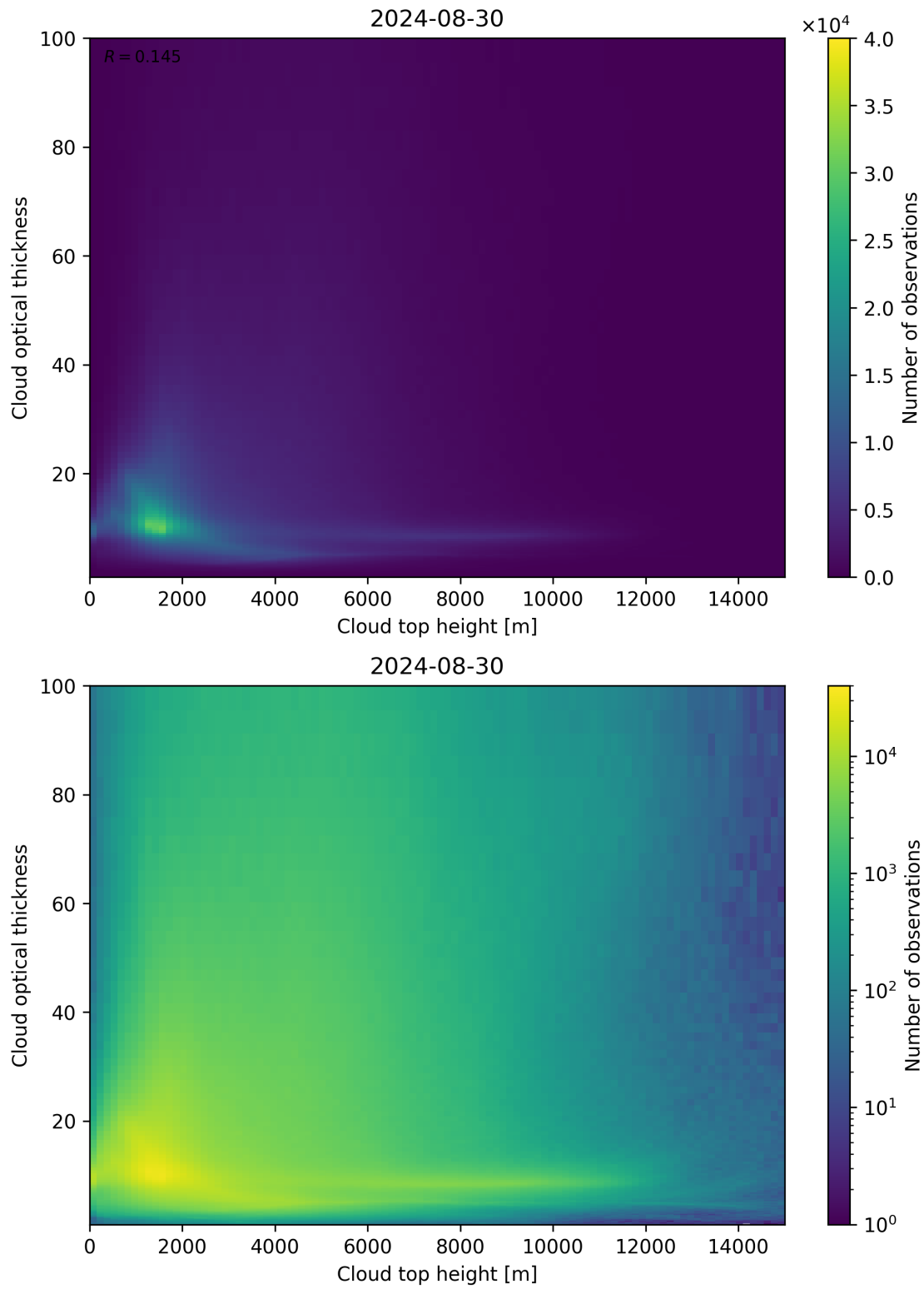
Figure 90: Scatter density plot of “Cloud top height” against “Cloud optical thickness” for 2024-08-29 to 2024-08-31.
