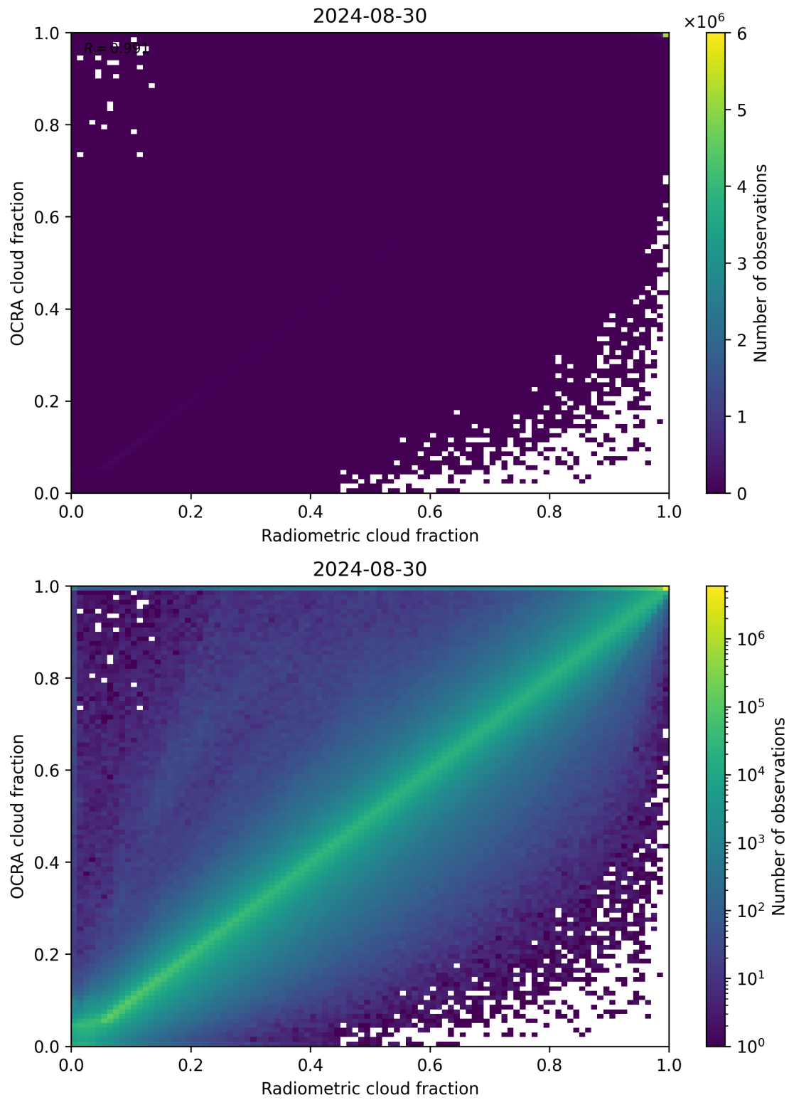
Figure 72: Scatter density plot of “Radiometric cloud fraction” against “OCRA cloud fraction” for 2024-08-29 to 2024-08-31.
