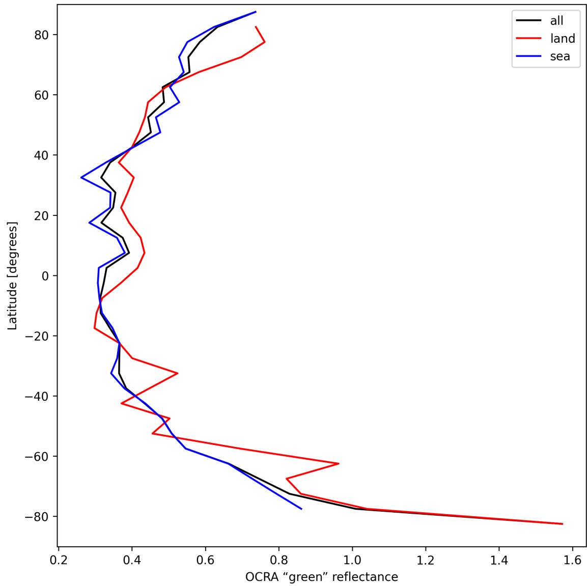
Figure 36: Zonal average of “OCRA “green” reflectance” for 2024-08-29 to 2024-08-31.
