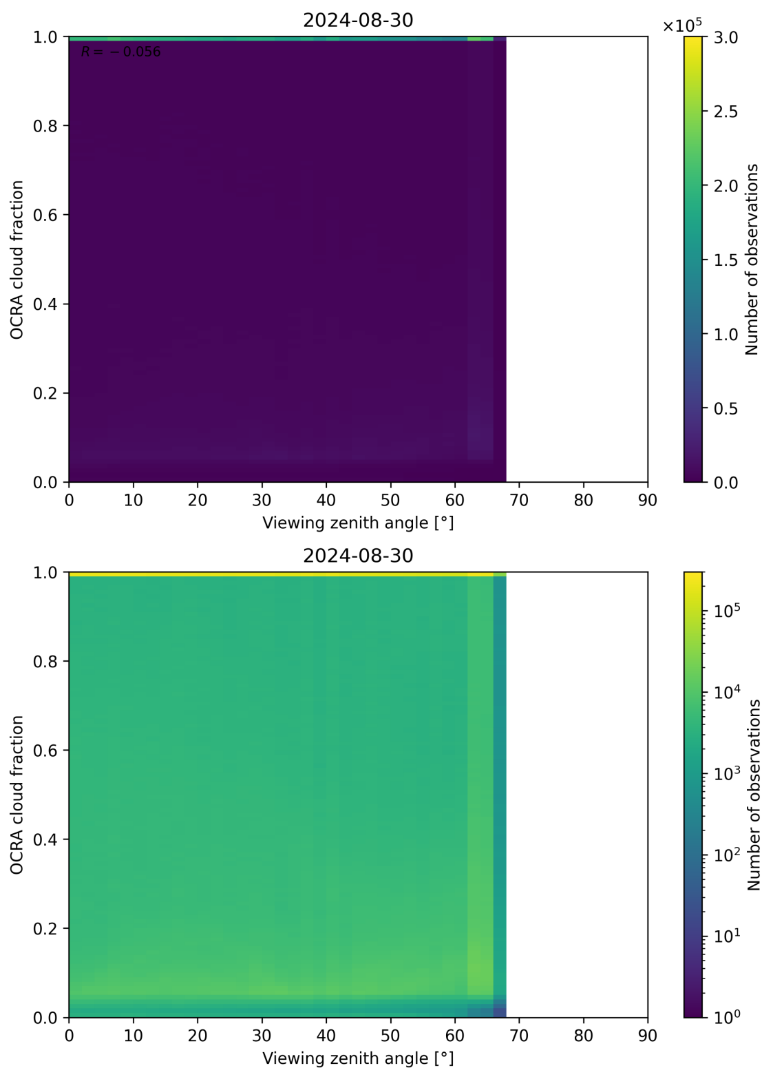
Figure 108: Scatter density plot of “Viewing zenith angle” against “OCRA cloud fraction” for 2024-08-29 to 2024-08-31.
