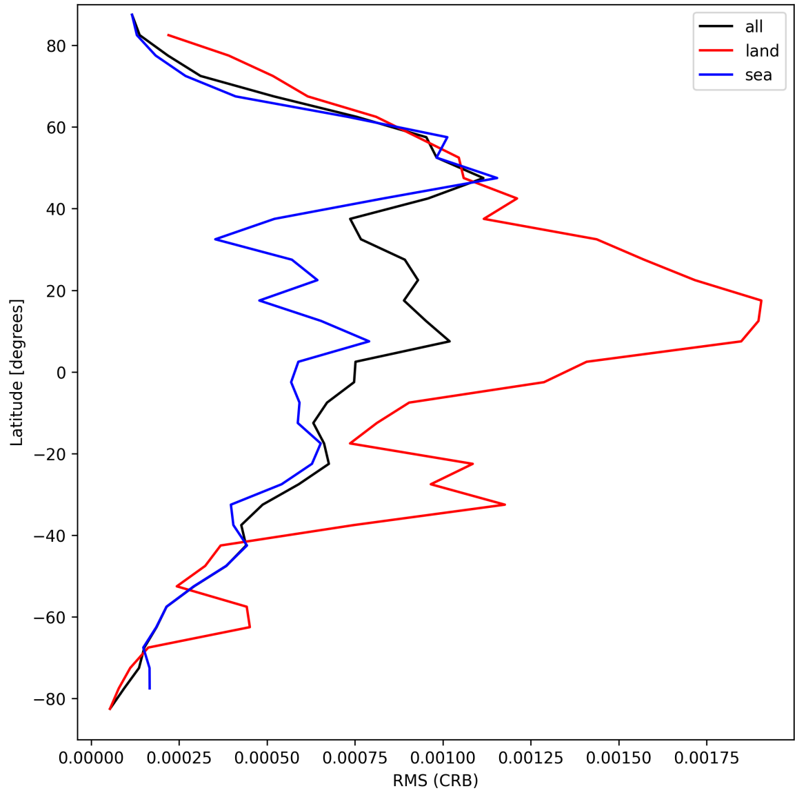
Figure 32: Zonal average of “RMS (CRB)” for 2024-08-29 to 2024-08-31.
