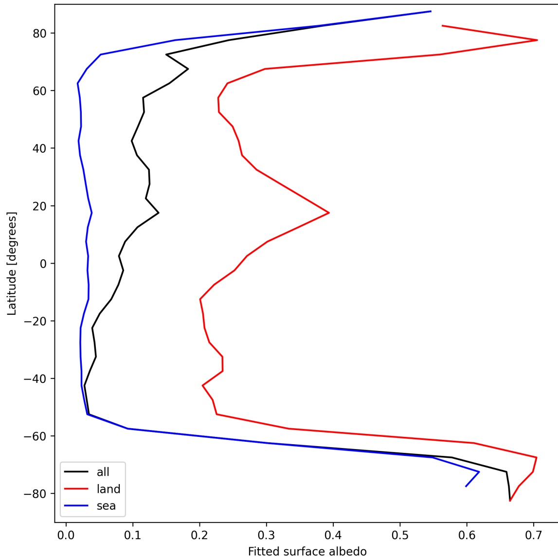
Figure 29: Zonal average of “Fitted surface albedo” for 2024-08-29 to 2024-08-31.
