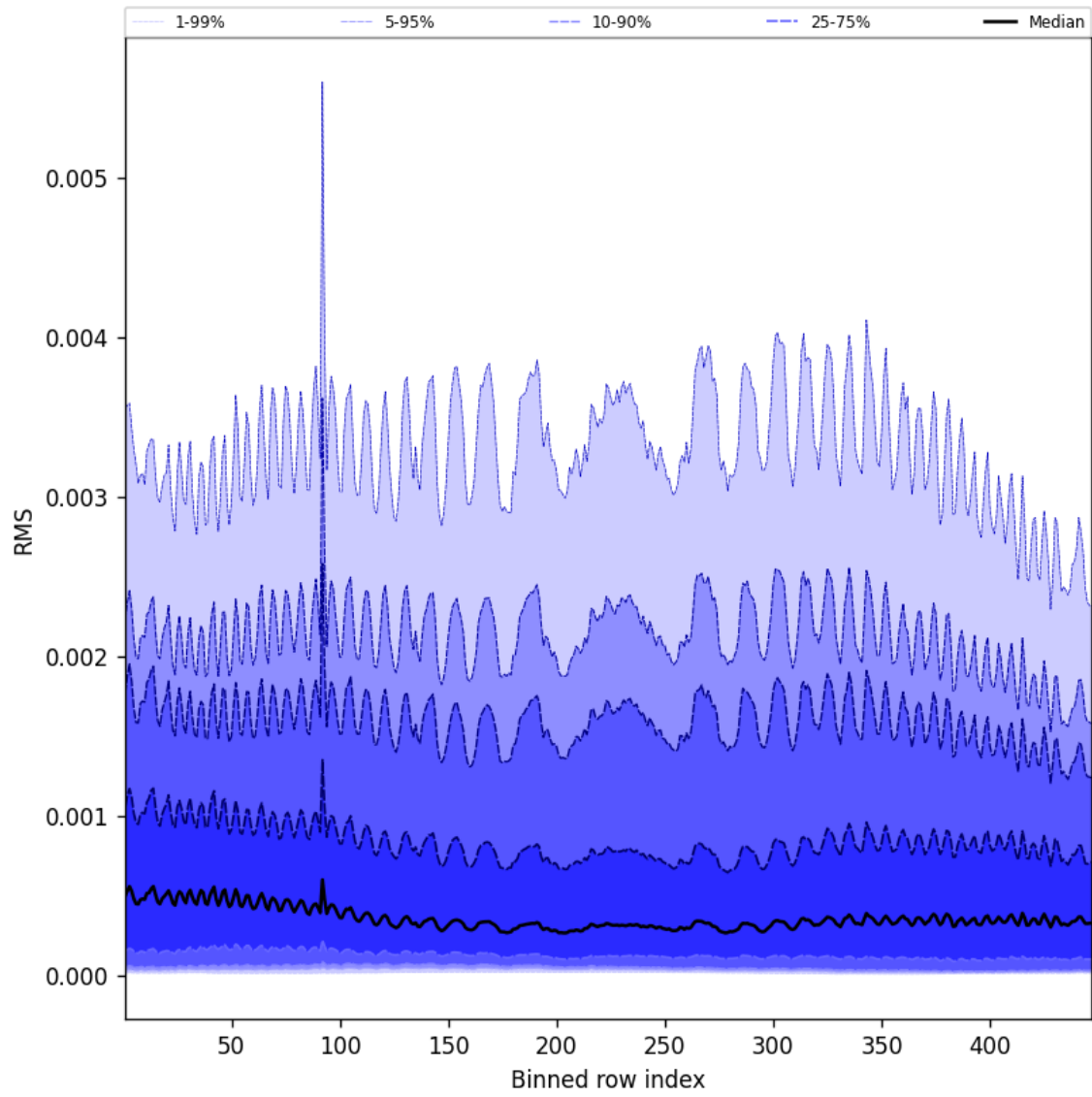
Figure 63: Along track statistics of “RMS” for 2024-08-29 to 2024-08-31
