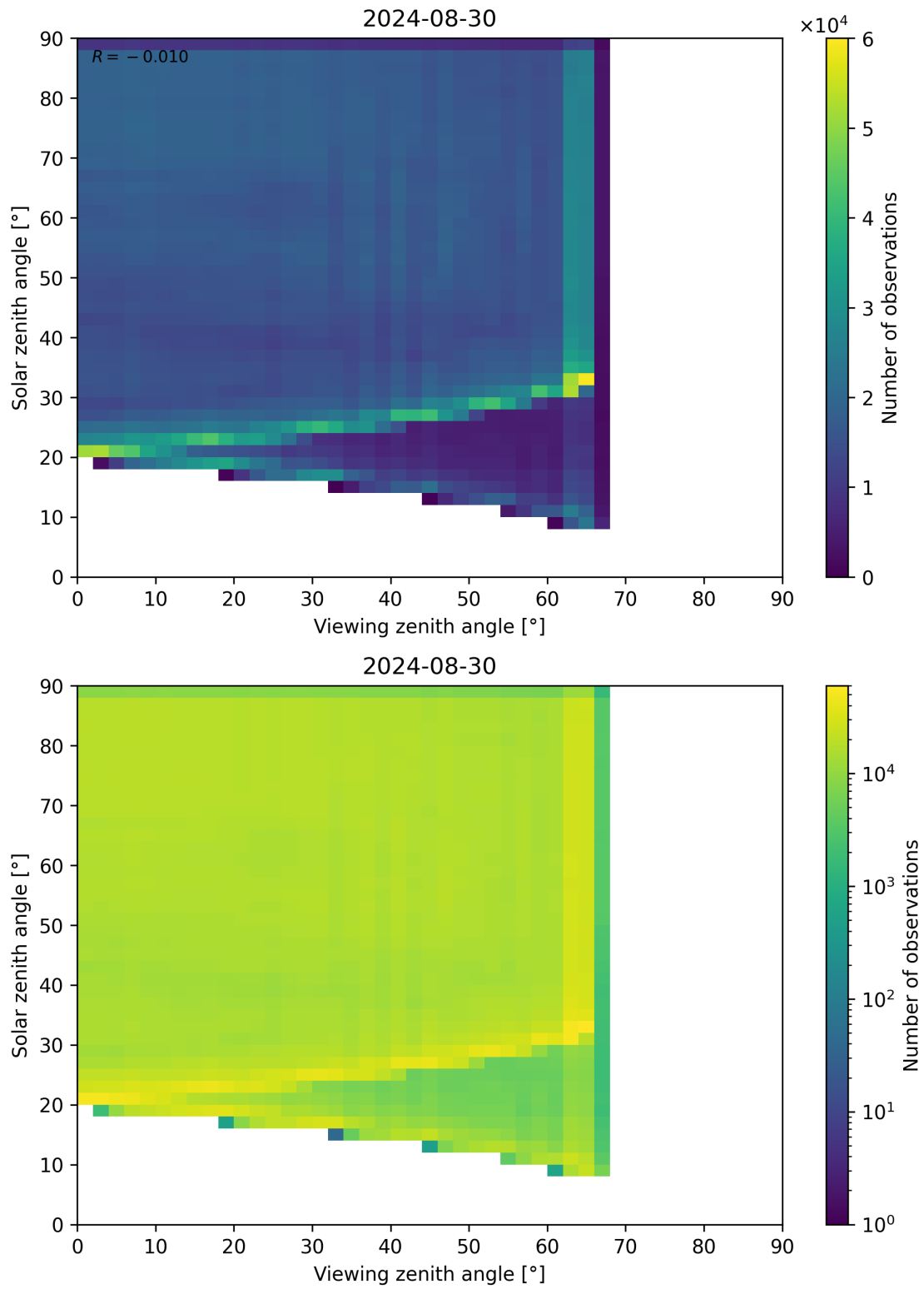
Figure 114: Scatter density plot of “Viewing zenith angle” against “Solar zenith angle” for 2024-08-29 to 2024-08-31.
