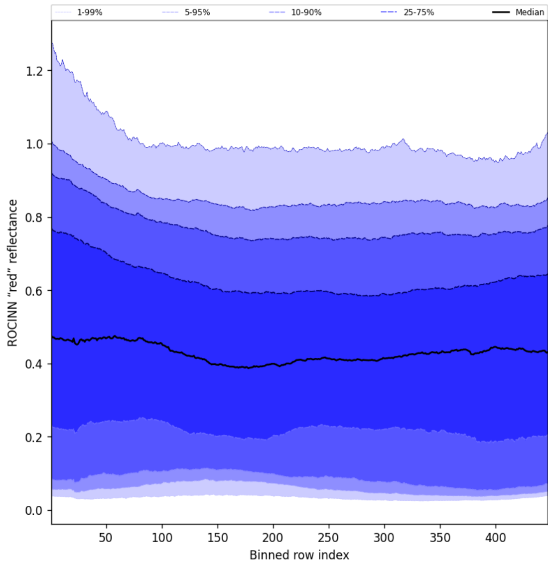
Figure 69: Along track statistics of “ROCINN “red” reflectance” for 2024-08-29 to 2024-08-31
