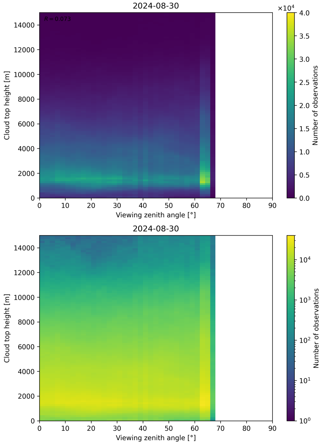
Figure 112: Scatter density plot of “Viewing zenith angle” against “Cloud top height” for 2024-08-29 to 2024-08-31.
