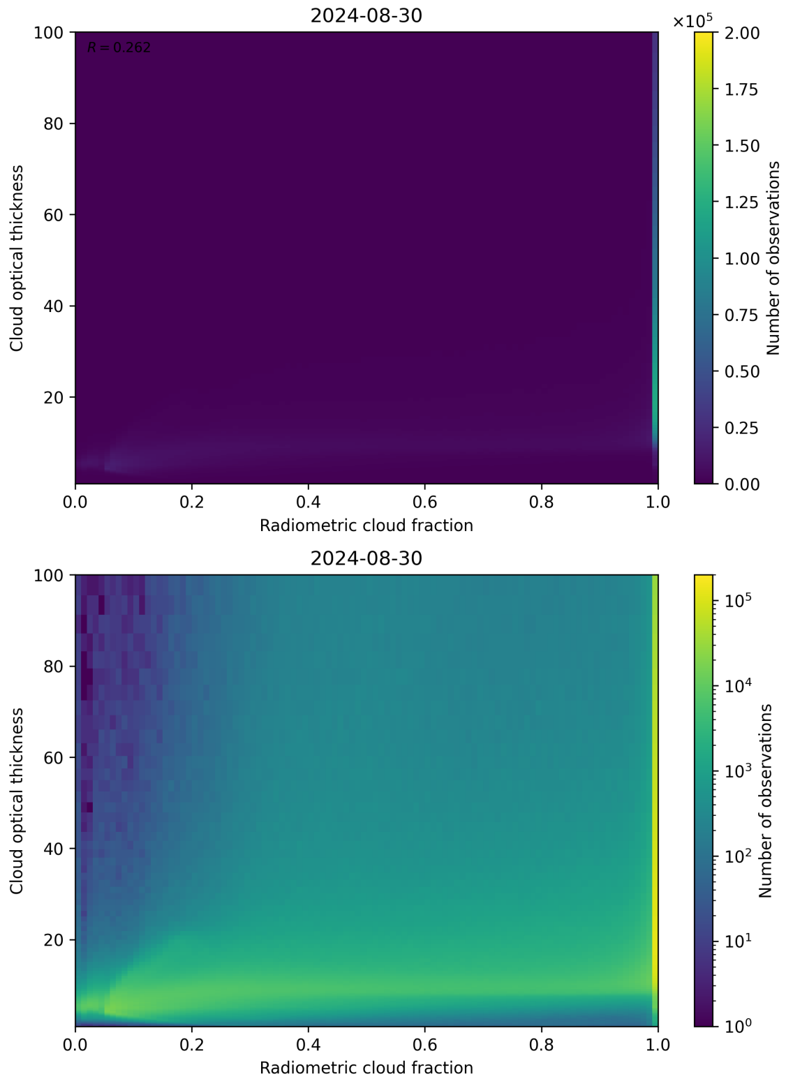
Figure 75: Scatter density plot of “Radiometric cloud fraction” against “Cloud optical thickness” for 2024-08-29 to 2024-08-31.
