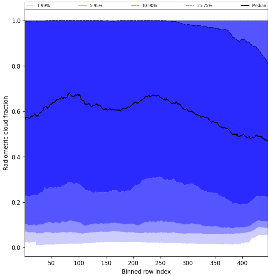
Figure 55: Along track statistics of “Radiometric cloud fraction” for 2024-08-29 to 2024-08-31
