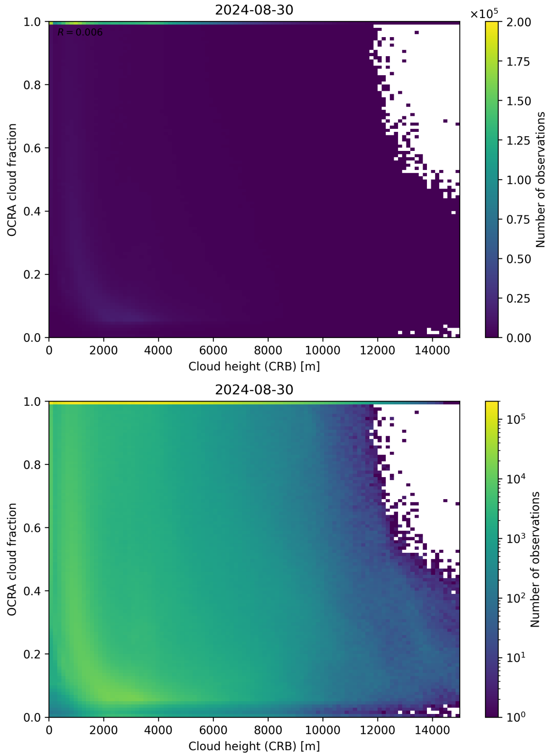
Figure 81: Scatter density plot of “Cloud height (CRB)” against “OCRA cloud fraction” for 2024-08-29 to 2024-08-31.
