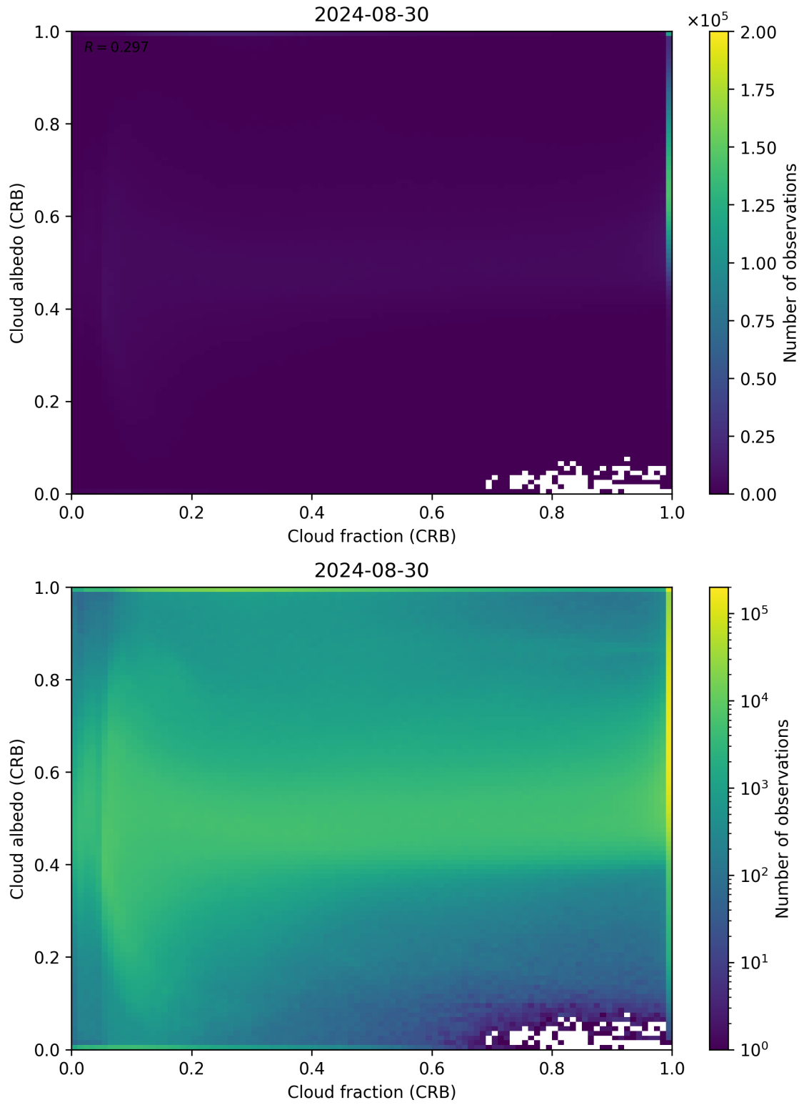
Figure 77: Scatter density plot of “Cloud fraction (CRB)” against “Cloud albedo (CRB)” for 2024-08-29 to 2024-08-31.
