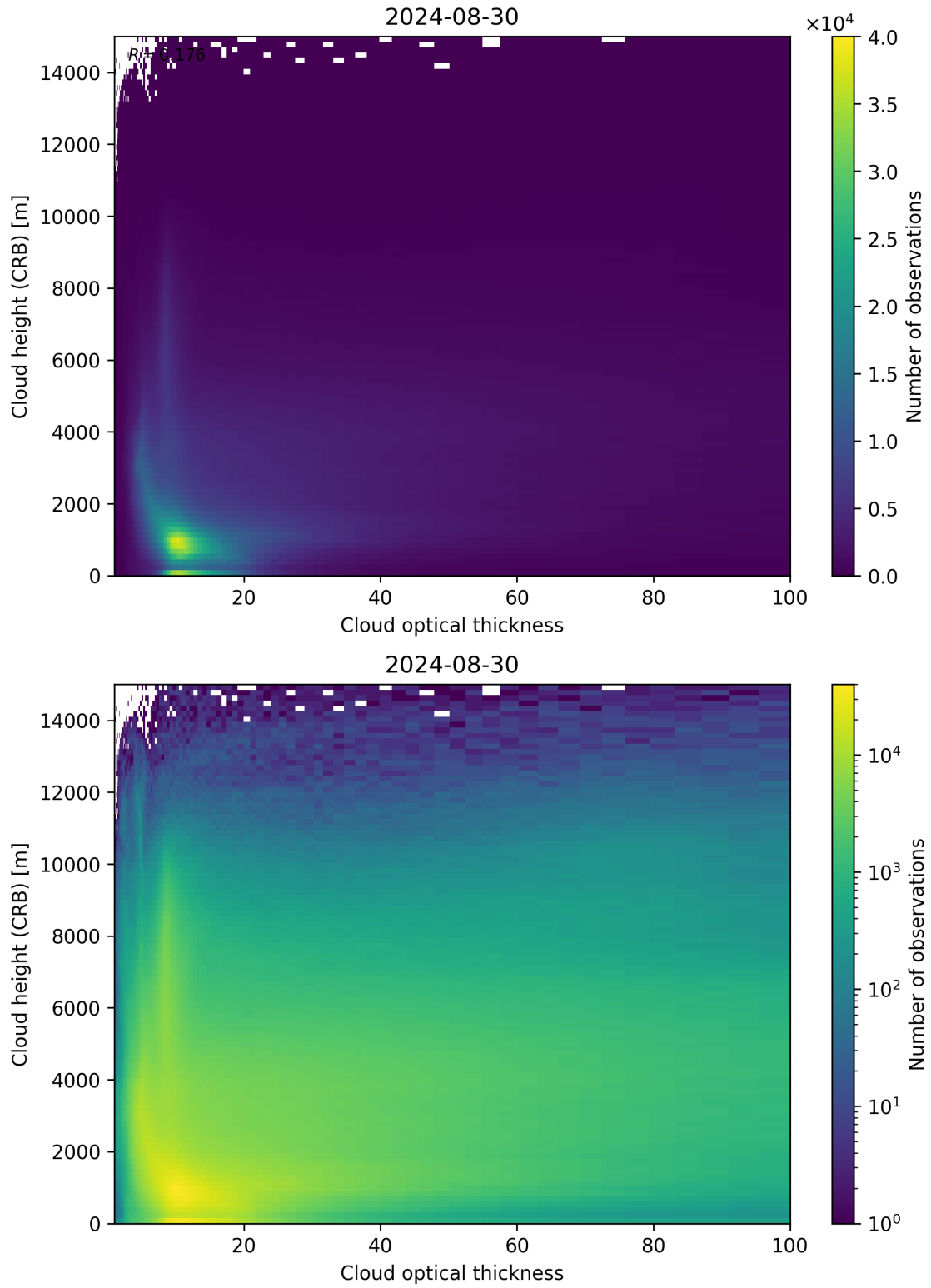
Figure 85: Scatter density plot of “Cloud optical thickness” against “Cloud height (CRB)” for 2024-08-29 to 2024-08-31.
