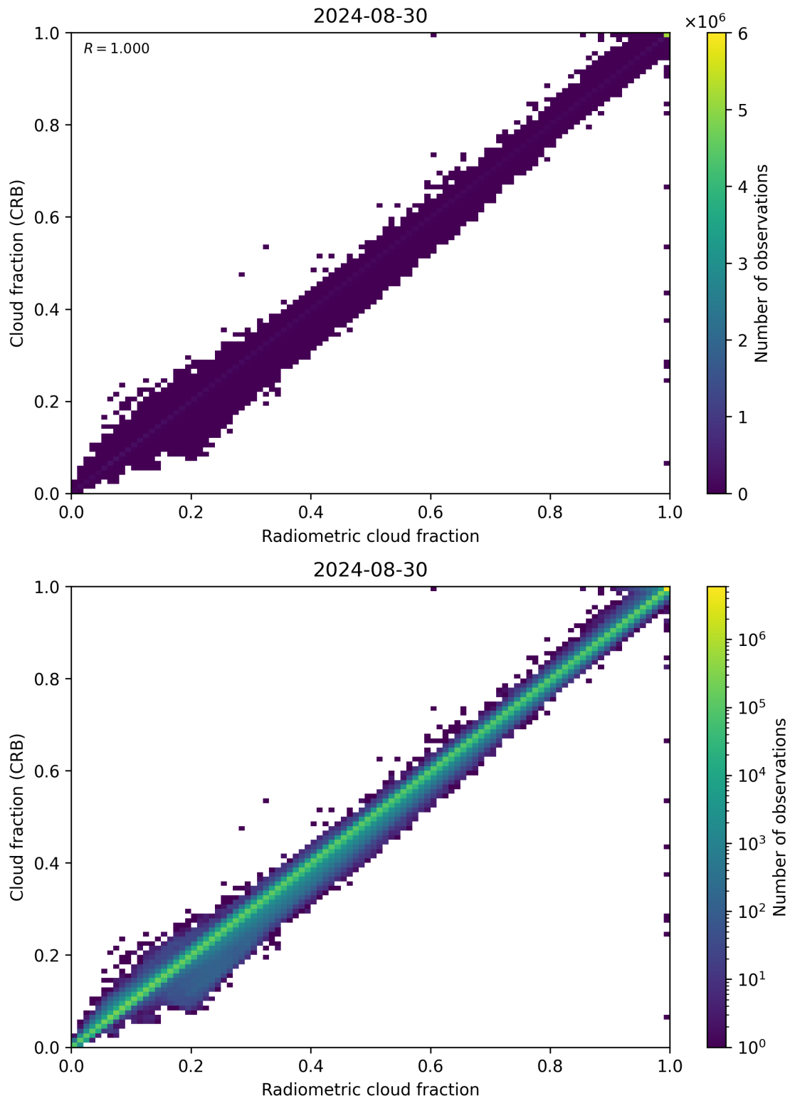
Figure 73: Scatter density plot of “Radiometric cloud fraction” against “Cloud fraction (CRB)” for 2024-08-29 to 2024-08-31.
