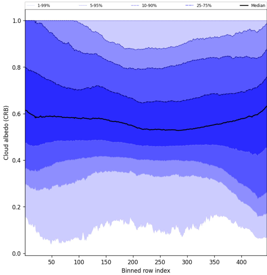
Figure 60: Along track statistics of “Cloud albedo (CRB)” for 2024-08-29 to 2024-08-31
