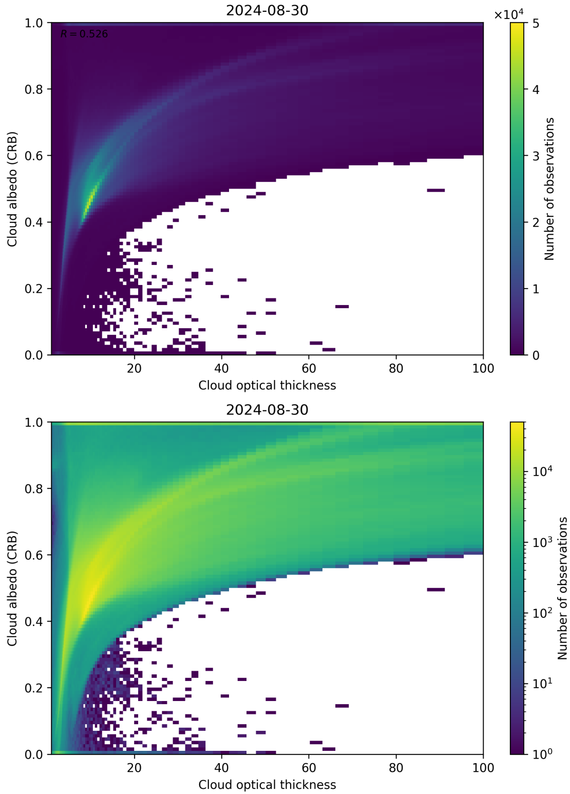
Figure 82: Scatter density plot of “Cloud optical thickness” against “Cloud albedo (CRB)” for 2024-08-29 to 2024-08-31.
