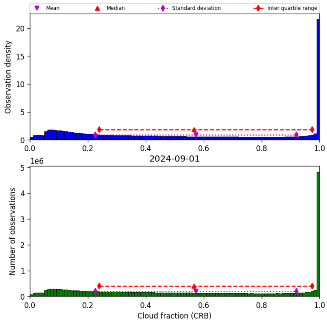
Figure 42: Histogram of “Cloud fraction (CRB)” for 2024-09-01 to 2024-09-02
