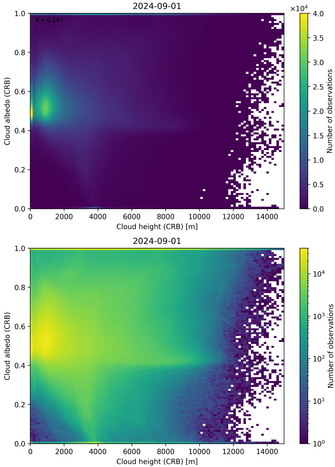
Figure 80: Scatter density plot of “Cloud height (CRB)” against “Cloud albedo (CRB)” for 2024-09-01 to 2024-09-02.
