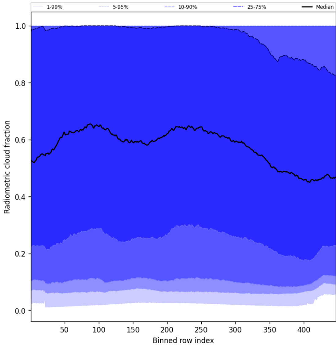
Figure 55: Along track statistics of “Radiometric cloud fraction” for 2024-09-01 to 2024-09-02
