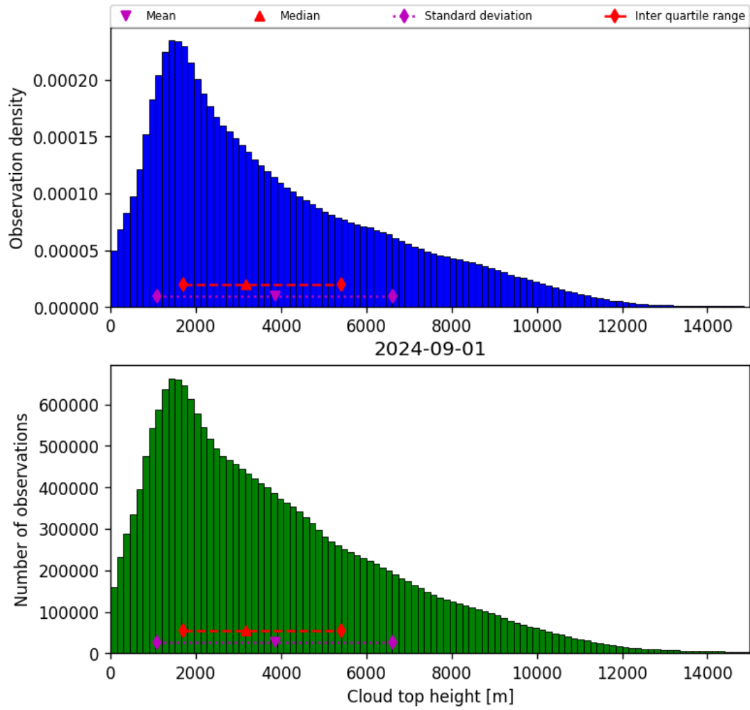
Figure 40: Histogram of “Cloud top height” for 2024-09-01 to 2024-09-02
