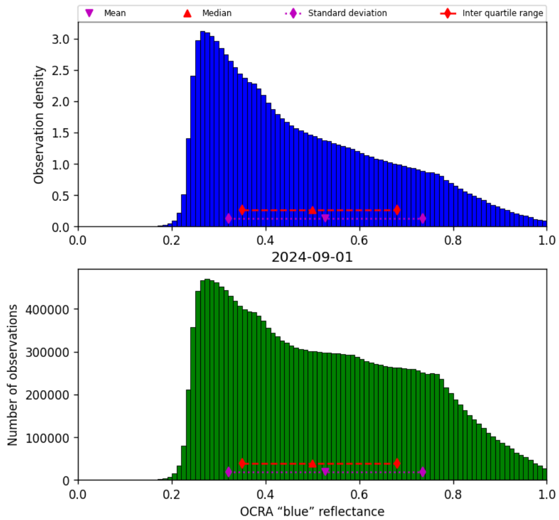
Figure 51: Histogram of “OCRA “blue” reflectance” for 2024-09-01 to 2024-09-02
