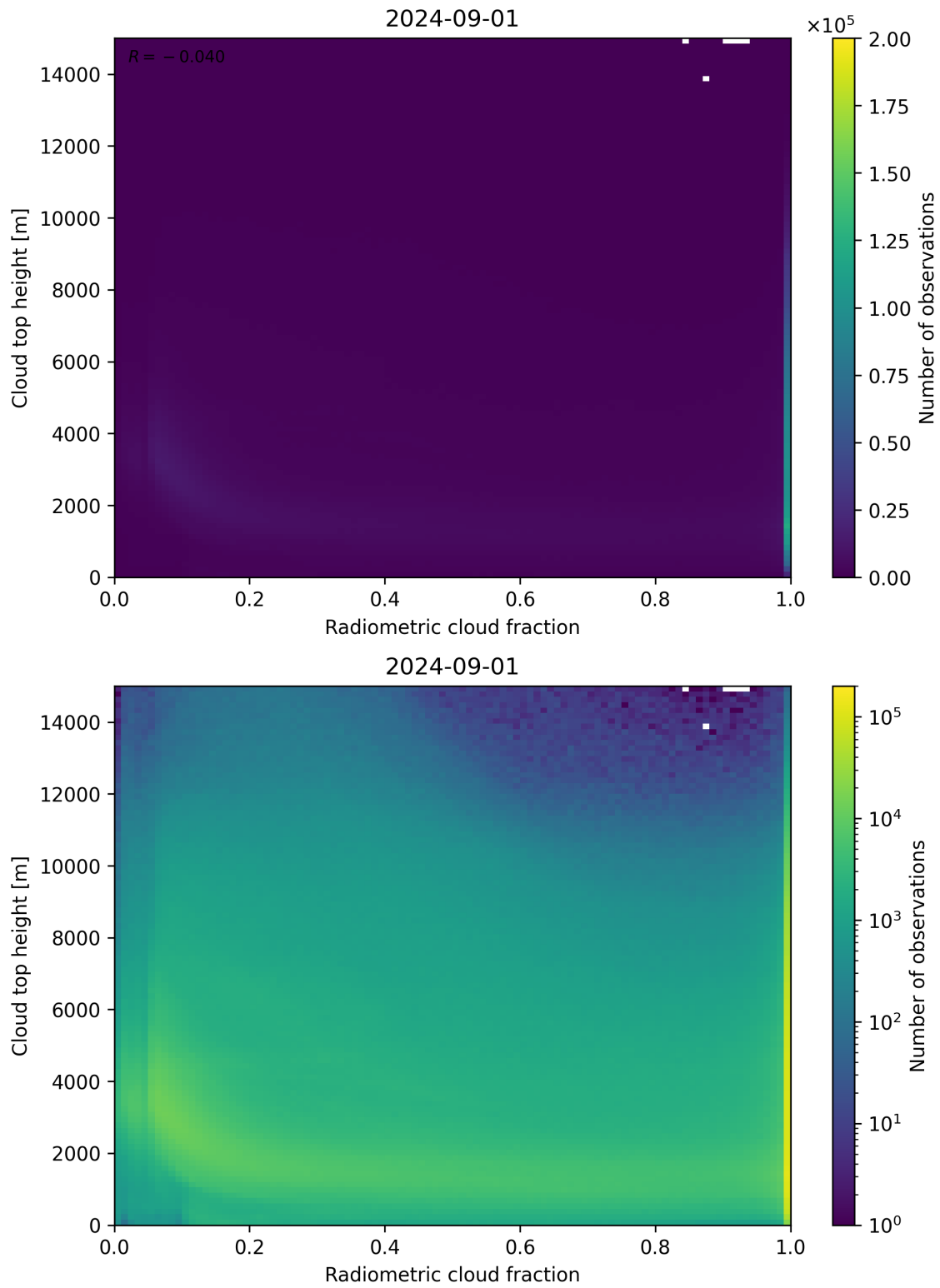
Figure 76: Scatter density plot of “Radiometric cloud fraction” against “Cloud top height” for 2024-09-01 to 2024-09-02.
