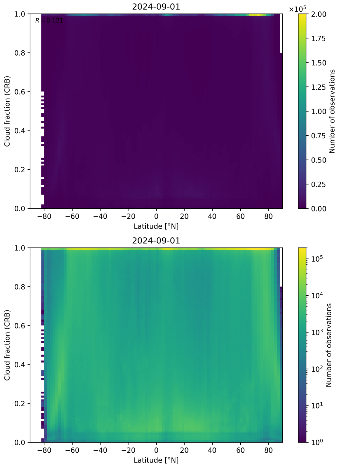
Figure 94: Scatter density plot of “Latitude” against “Cloud fraction (CRB)” for 2024-09-01 to 2024-09-02.
