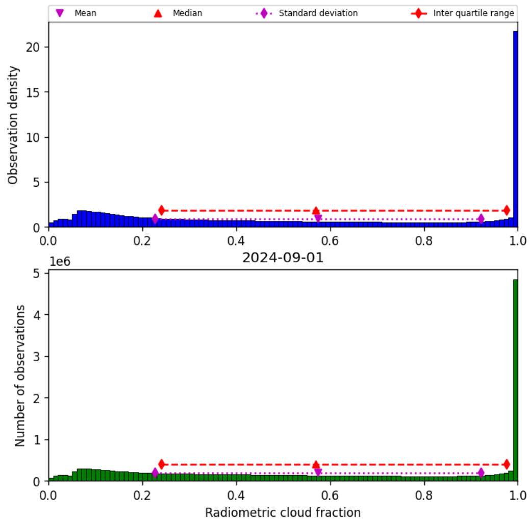
Figure 39: Histogram of “Radiometric cloud fraction” for 2024-09-01 to 2024-09-02
