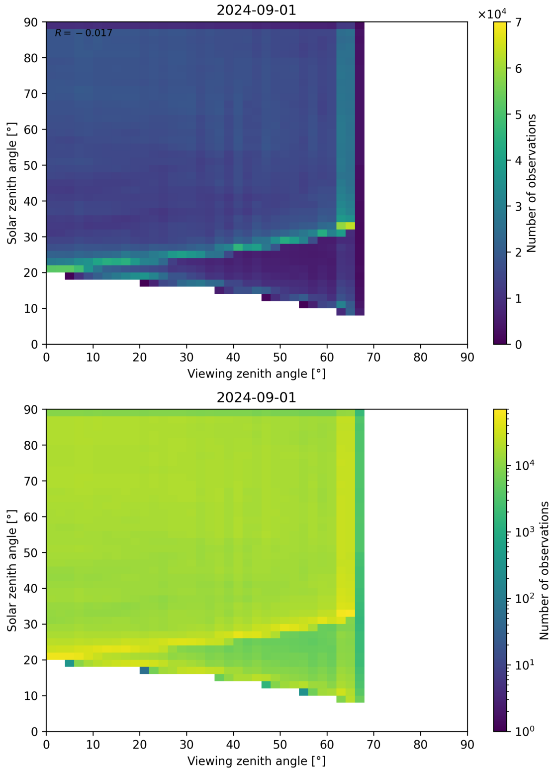
Figure 114: Scatter density plot of “Viewing zenith angle” against “Solar zenith angle” for 2024-09-01 to 2024-09-02.
