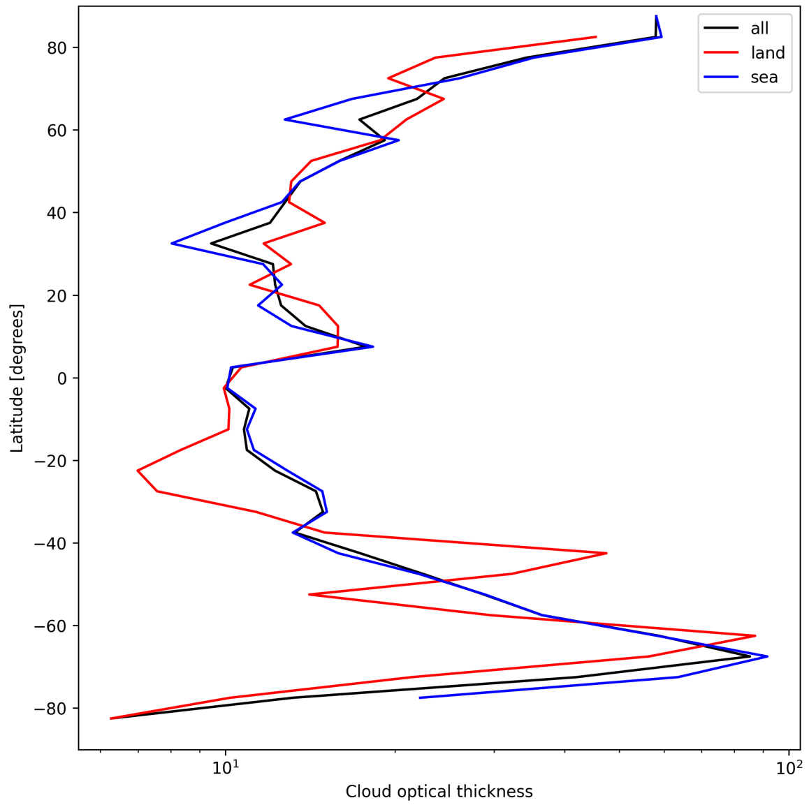
Figure 25: Zonal average of “Cloud optical thickness” for 2024-09-01 to 2024-09-02.
