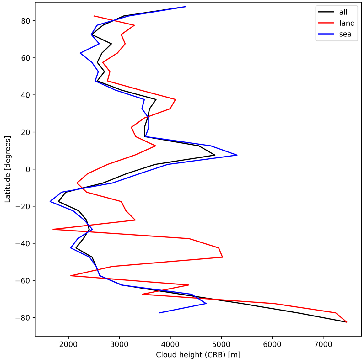
Figure 27: Zonal average of “Cloud height (CRB)” for 2024-09-01 to 2024-09-02.
