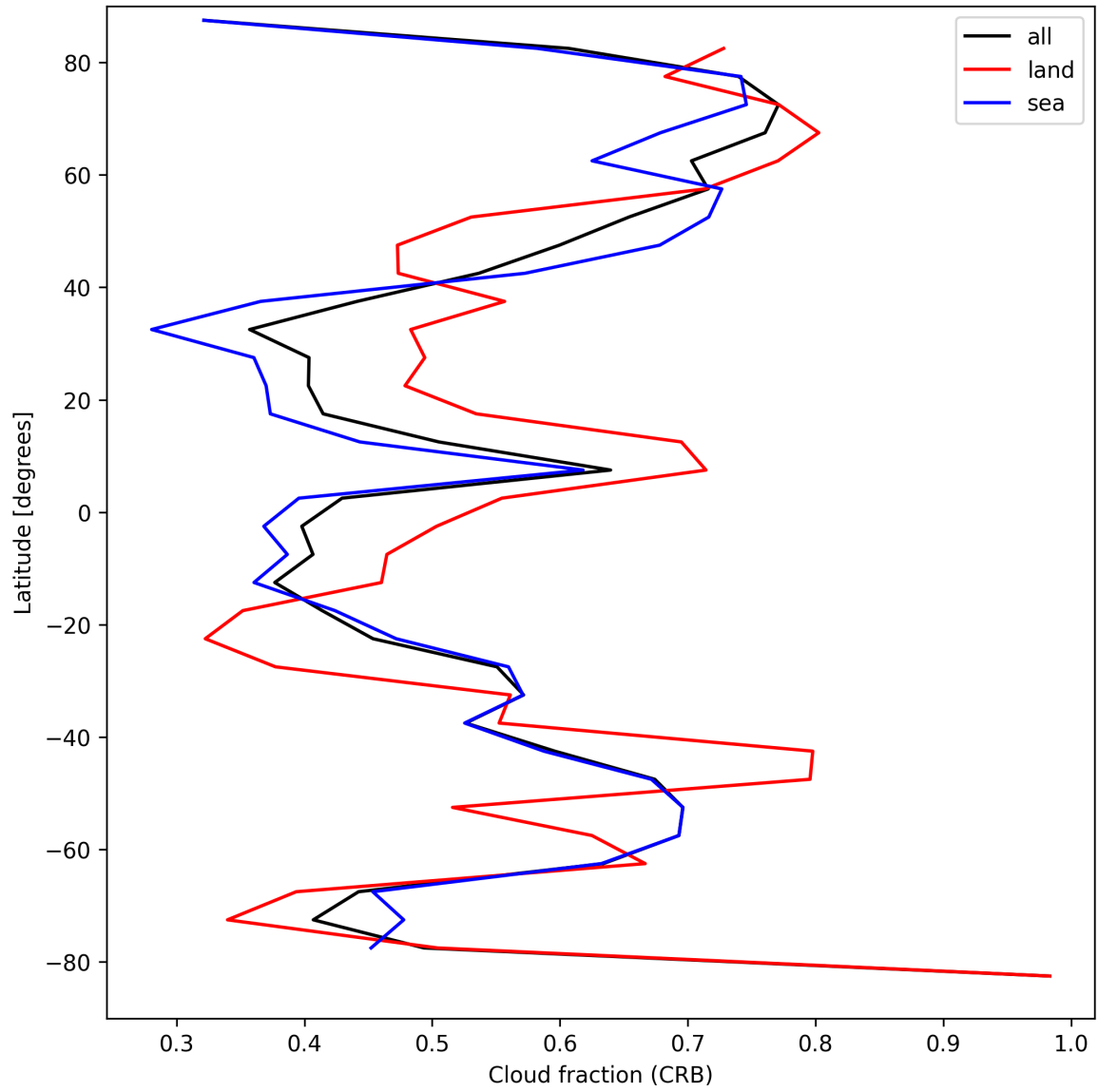
Figure 26: Zonal average of “Cloud fraction (CRB)” for 2024-09-01 to 2024-09-02.
