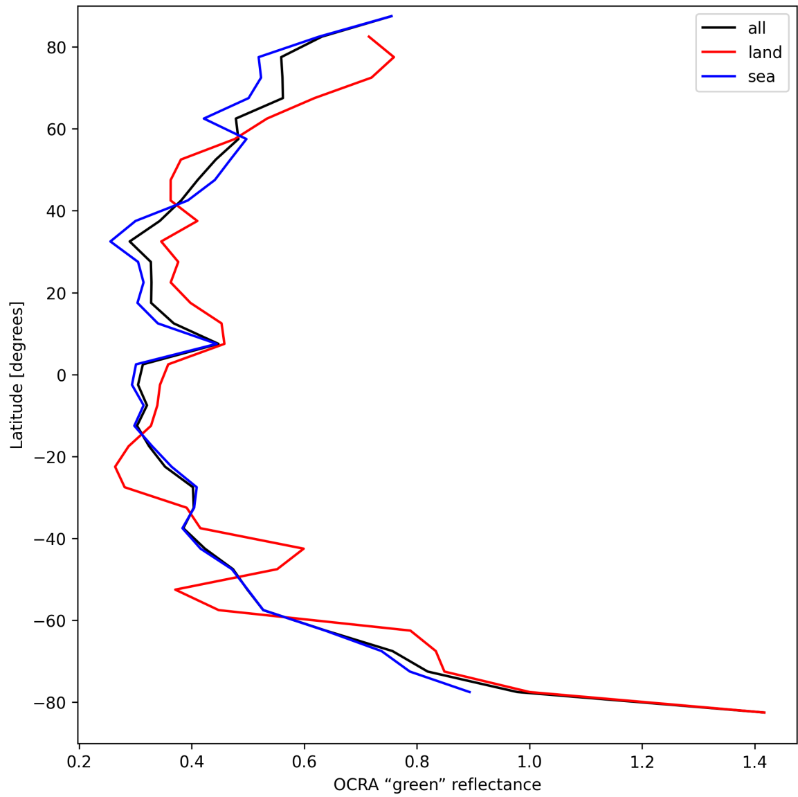
Figure 36: Zonal average of “OCRA “green” reflectance” for 2024-09-01 to 2024-09-02.
