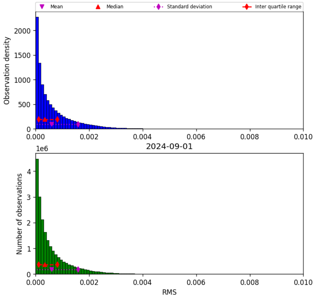
Figure 47: Histogram of “RMS” for 2024-09-01 to 2024-09-02
