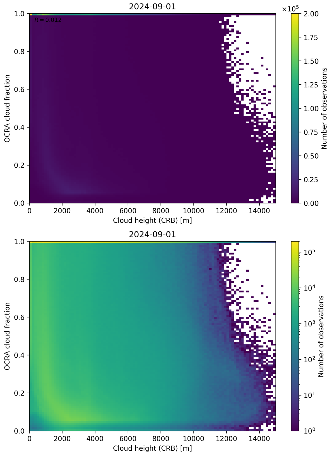
Figure 81: Scatter density plot of “Cloud height (CRB)” against “OCRA cloud fraction” for 2024-09-01 to 2024-09-02.
