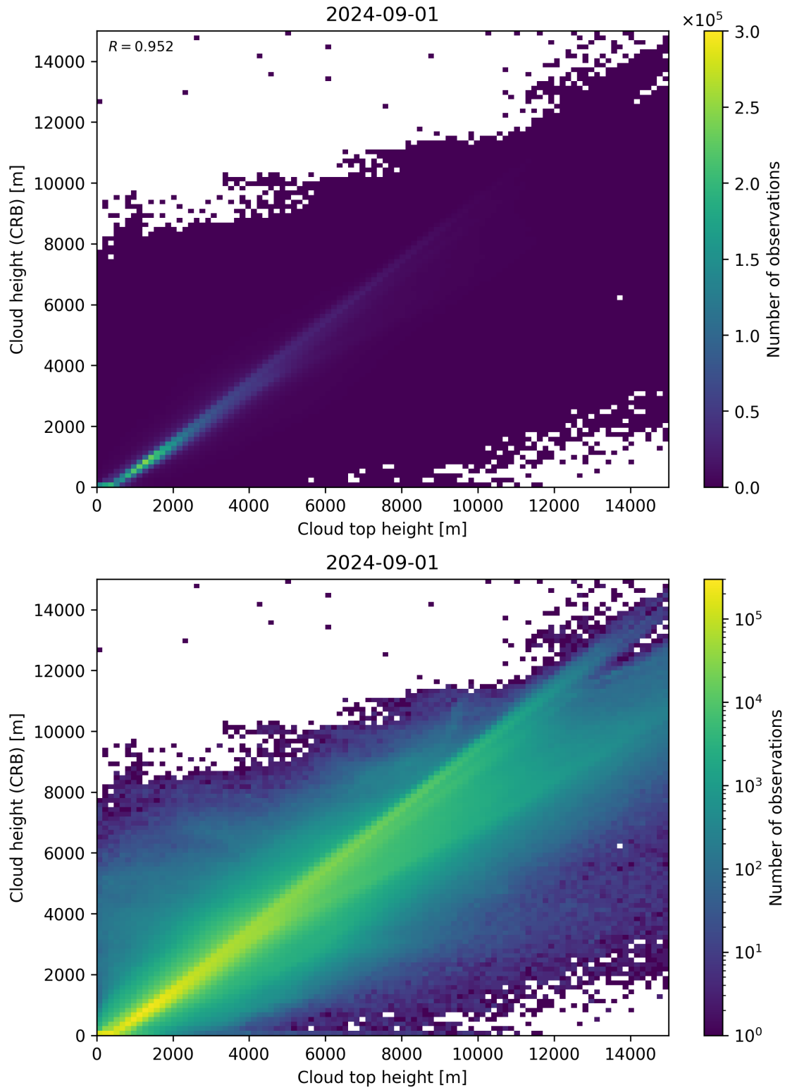
Figure 89: Scatter density plot of “Cloud top height” against “Cloud height (CRB)” for 2024-09-01 to 2024-09-02.
