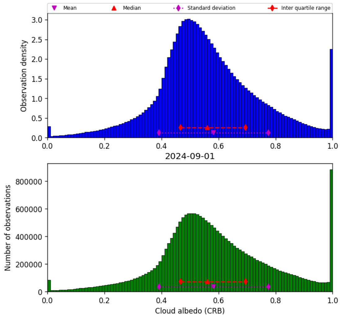
Figure 44: Histogram of “Cloud albedo (CRB)” for 2024-09-01 to 2024-09-02
