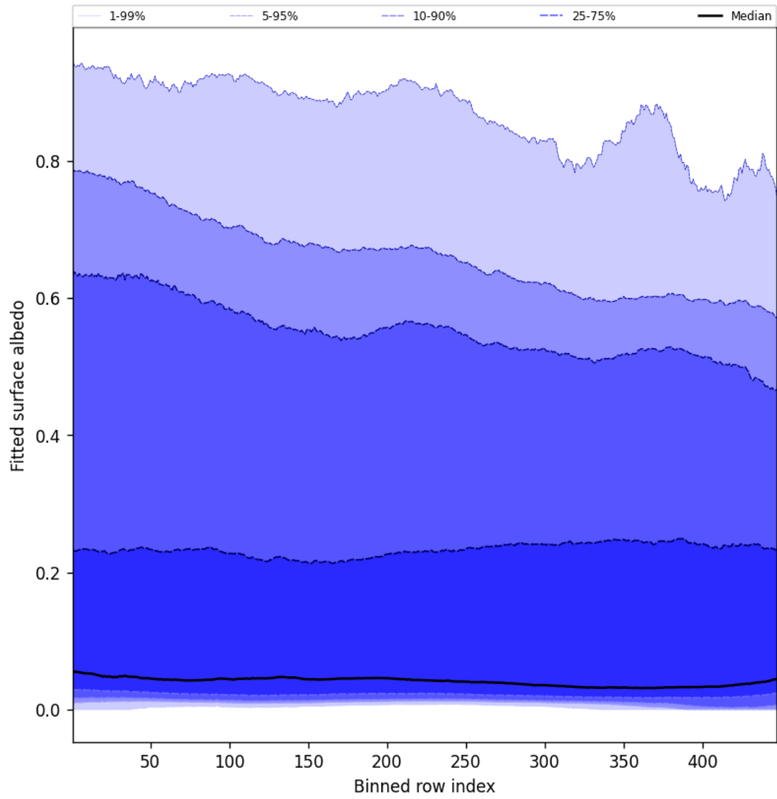
Figure 61: Along track statistics of “Fitted surface albedo” for 2024-09-01 to 2024-09-02
