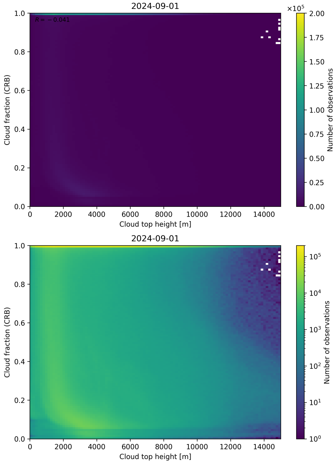
Figure 88: Scatter density plot of “Cloud top height” against “Cloud fraction (CRB)” for 2024-09-01 to 2024-09-02.
