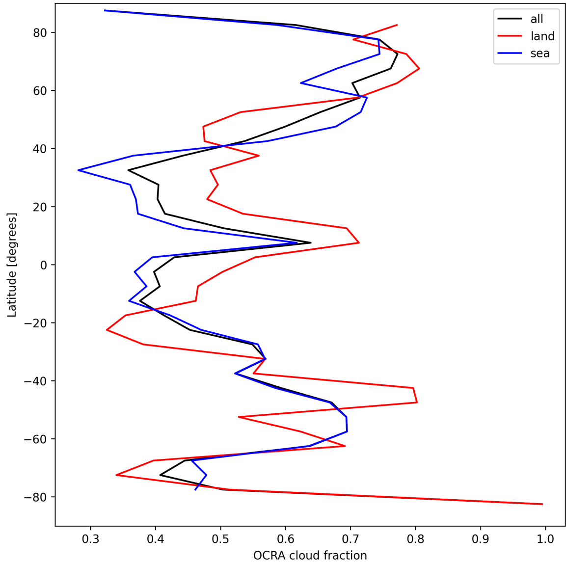
Figure 34: Zonal average of “OCRA cloud fraction” for 2024-09-01 to 2024-09-02.
