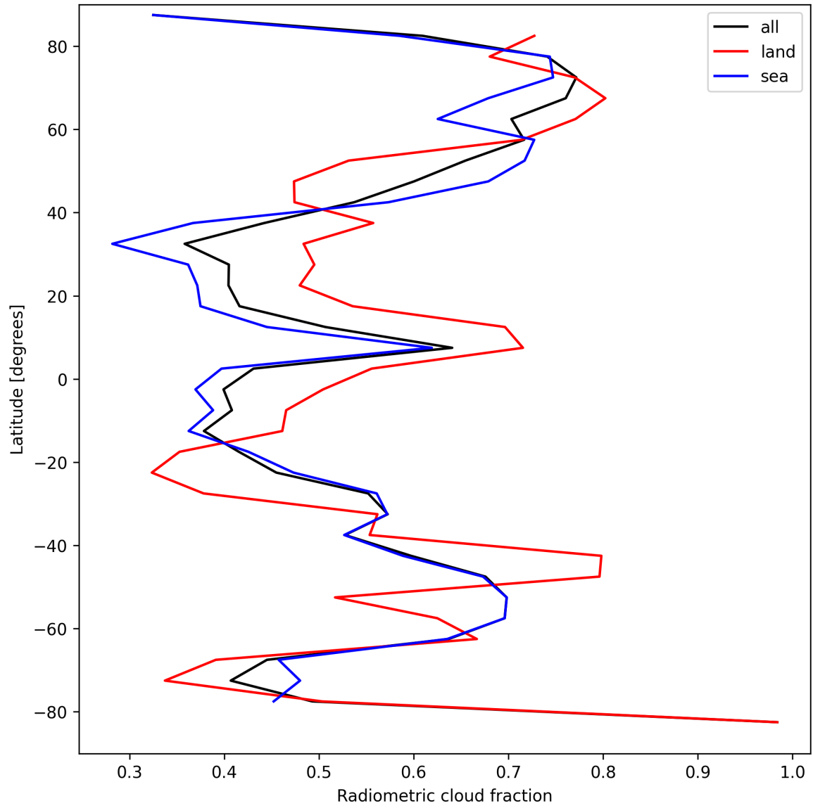
Figure 23: Zonal average of “Radiometric cloud fraction” for 2024-09-01 to 2024-09-02.
