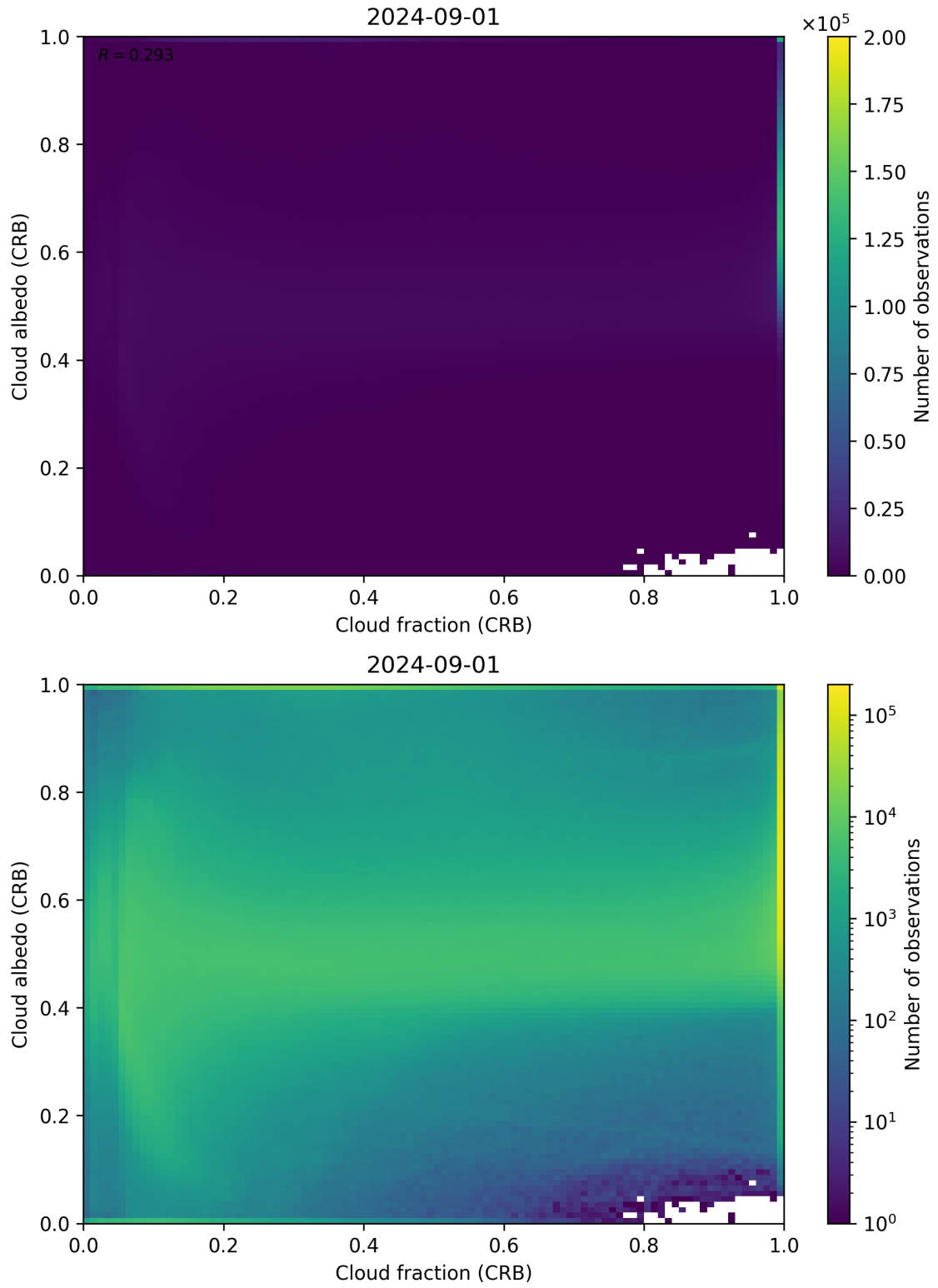
Figure 77: Scatter density plot of “Cloud fraction (CRB)” against “Cloud albedo (CRB)” for 2024-09-01 to 2024-09-02.
