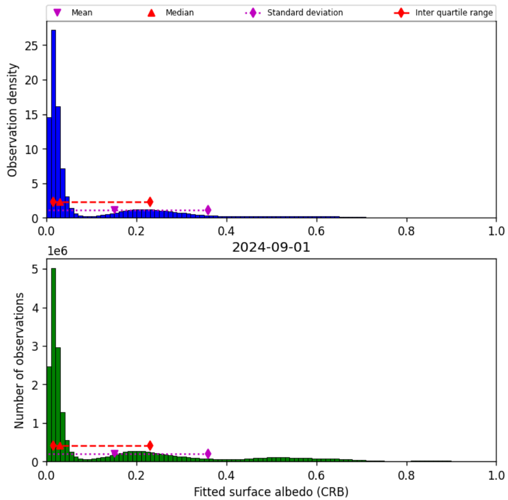
Figure 46: Histogram of “Fitted surface albedo (CRB)” for 2024-09-01 to 2024-09-02
