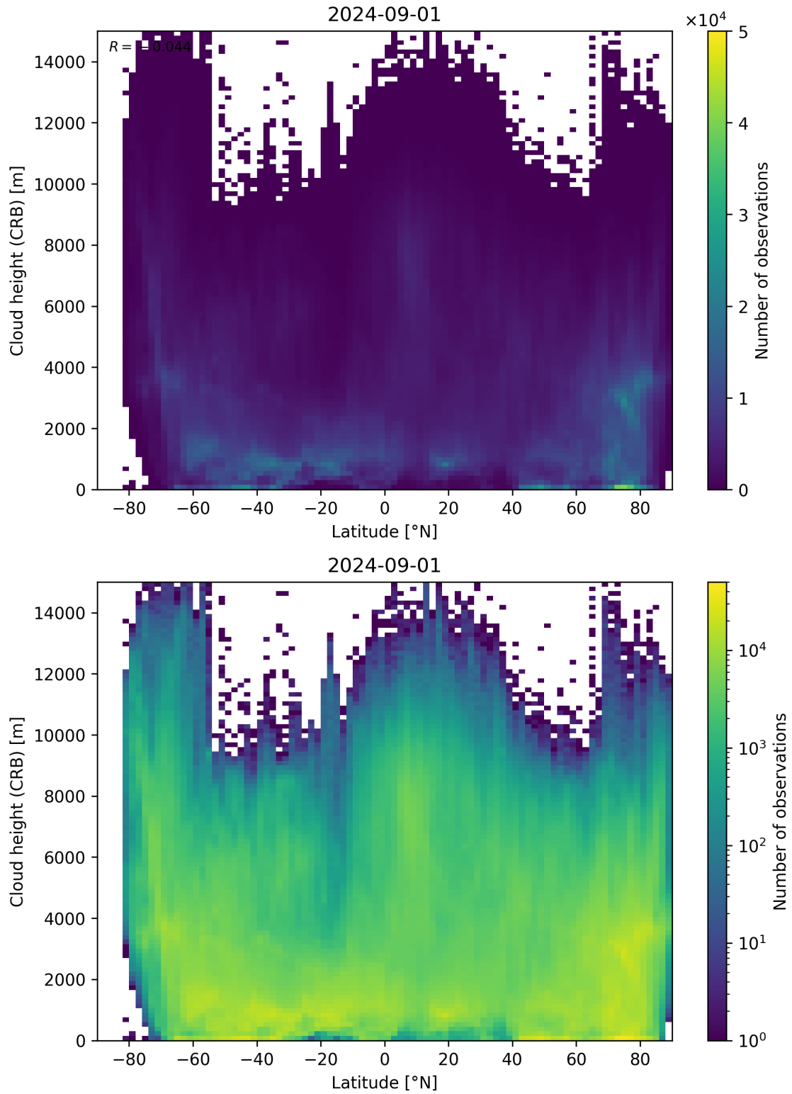
Figure 95: Scatter density plot of “Latitude” against “Cloud height (CRB)” for 2024-09-01 to 2024-09-02.
