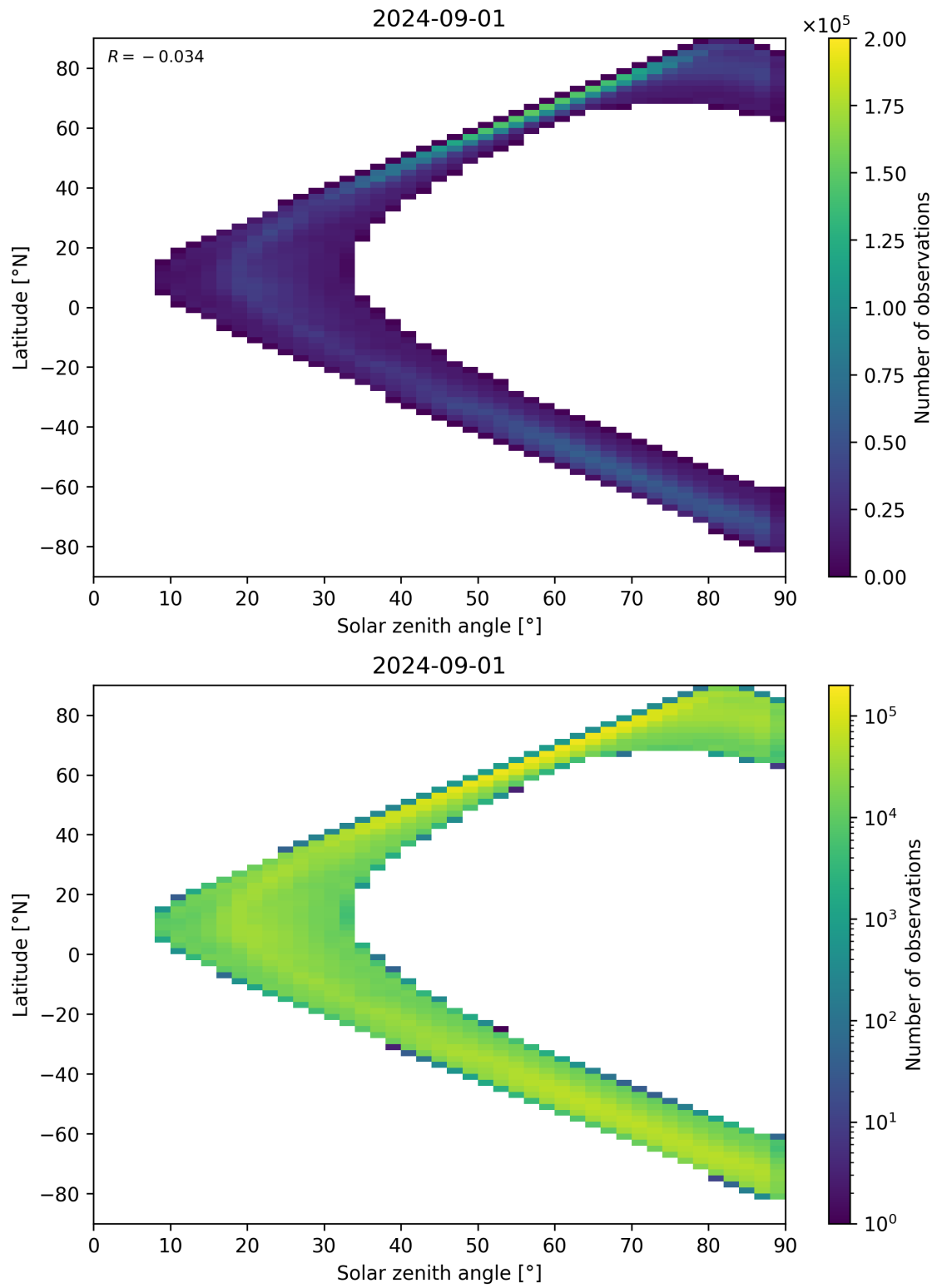
Figure 105: Scatter density plot of “Solar zenith angle” against “Latitude” for 2024-09-01 to 2024-09-02.
