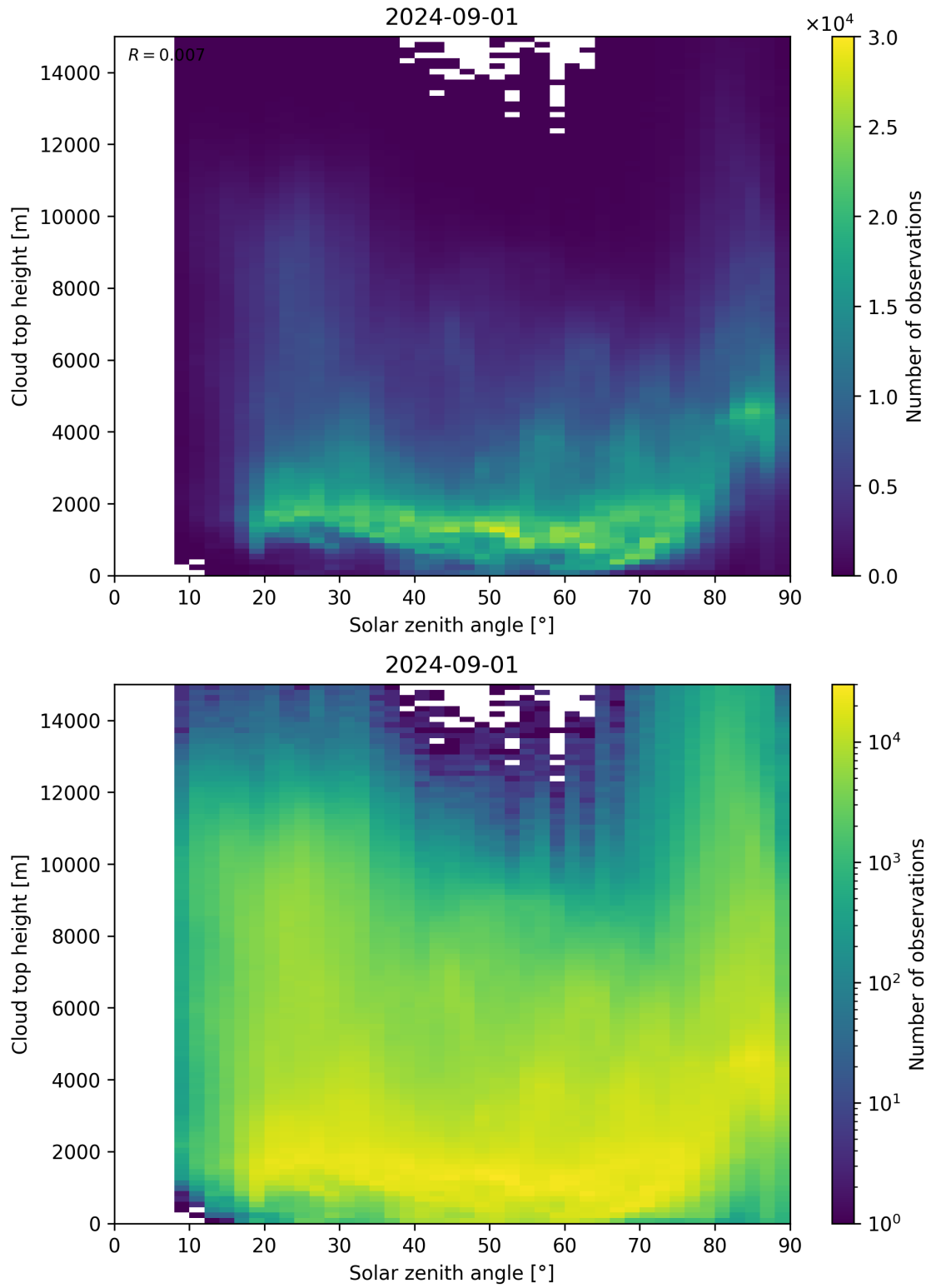
Figure 104: Scatter density plot of “Solar zenith angle” against “Cloud top height” for 2024-09-01 to 2024-09-02.
