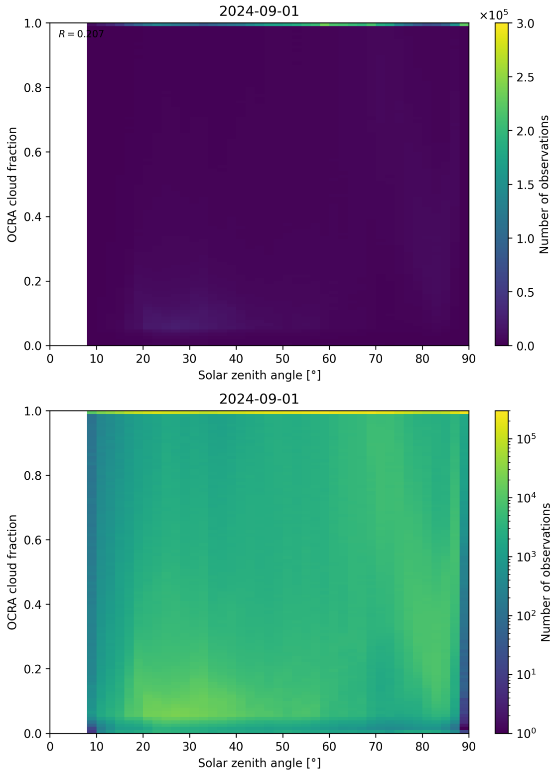
Figure 100: Scatter density plot of “Solar zenith angle” against “OCRA cloud fraction” for 2024-09-01 to 2024-09-02.
