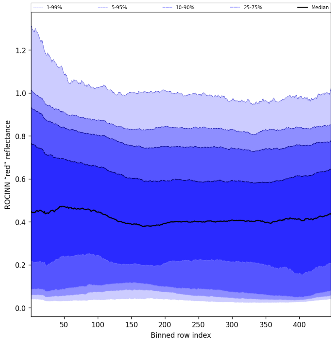
Figure 69: Along track statistics of “ROCINN “red” reflectance” for 2024-09-01 to 2024-09-02
