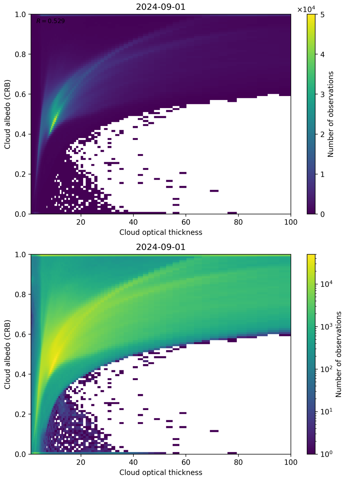
Figure 82: Scatter density plot of “Cloud optical thickness” against “Cloud albedo (CRB)” for 2024-09-01 to 2024-09-02.
