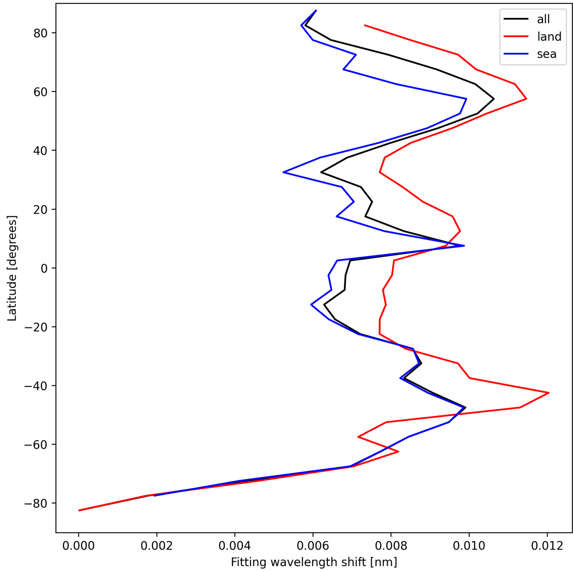
Figure 33: Zonal average of “Fitting wavelength shift” for 2024-09-01 to 2024-09-02.
