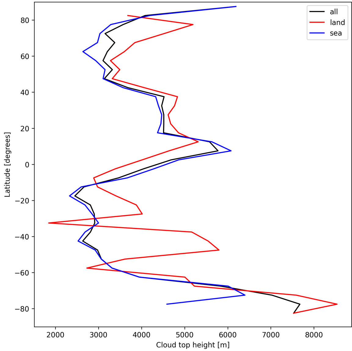
Figure 24: Zonal average of “Cloud top height” for 2024-09-01 to 2024-09-02.
