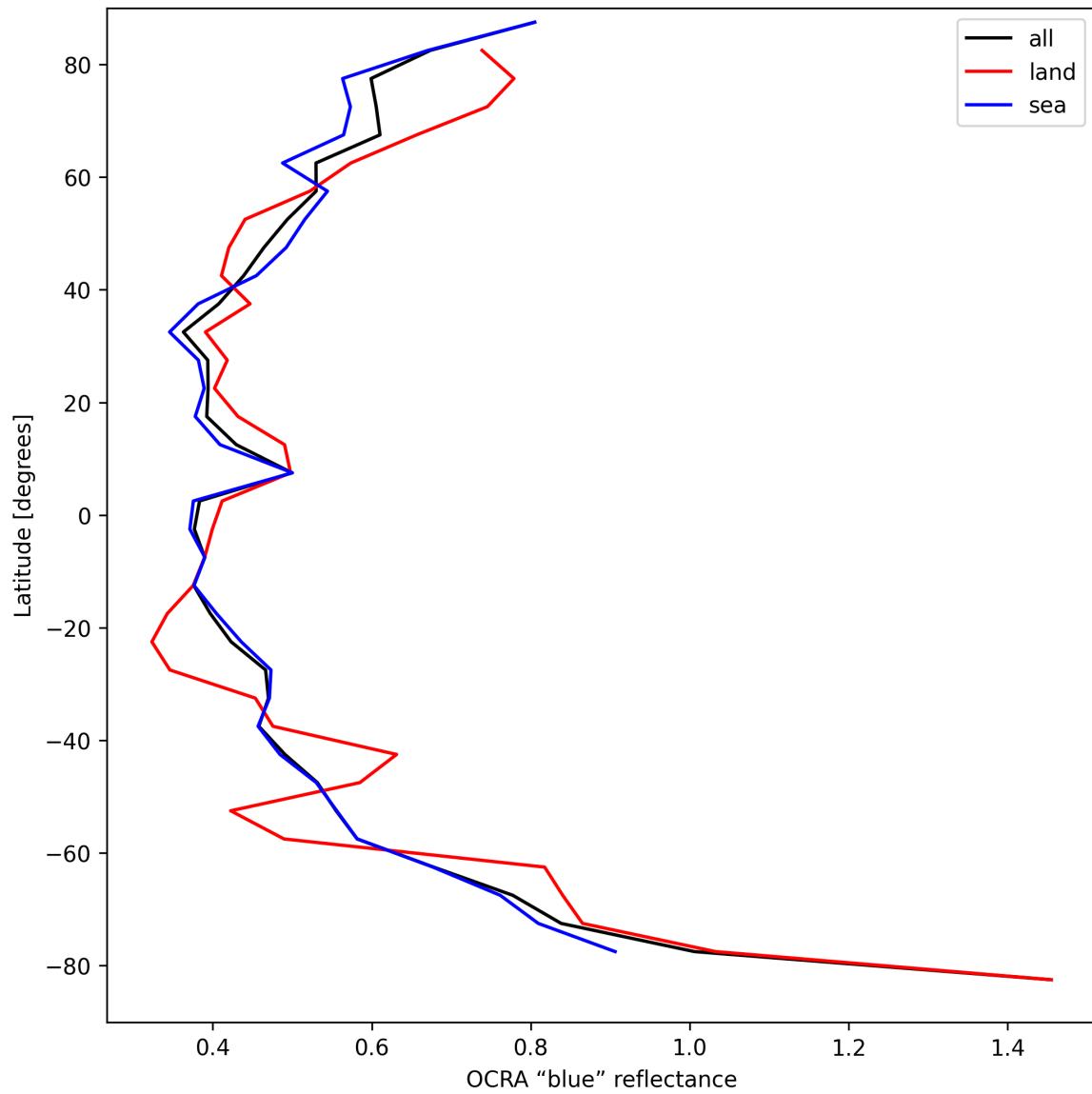
Figure 35: Zonal average of "OCRA "blue" reflectance" for 2024-09-01 to 2024-09-02.
