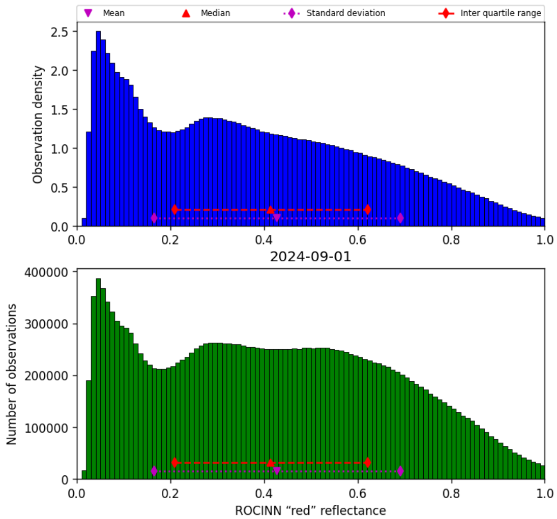
Figure 53: Histogram of “ROCINN “red” reflectance” for 2024-09-01 to 2024-09-02
