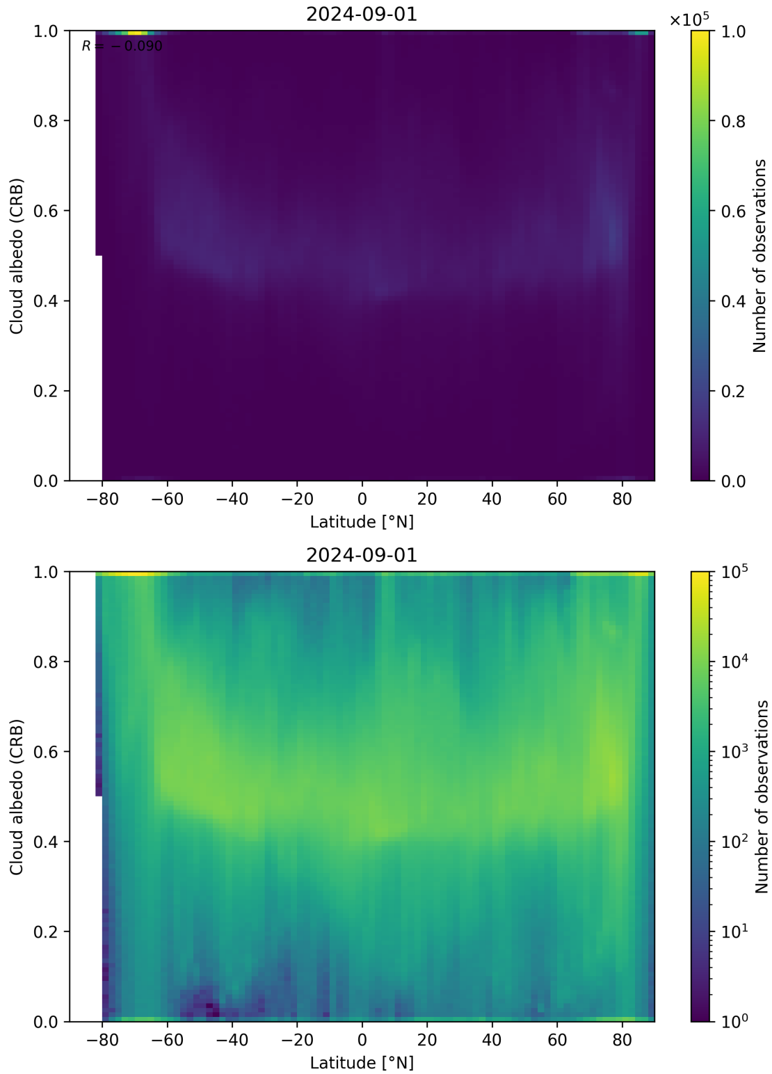
Figure 91: Scatter density plot of “Latitude” against “Cloud albedo (CRB)” for 2024-09-01 to 2024-09-02.
