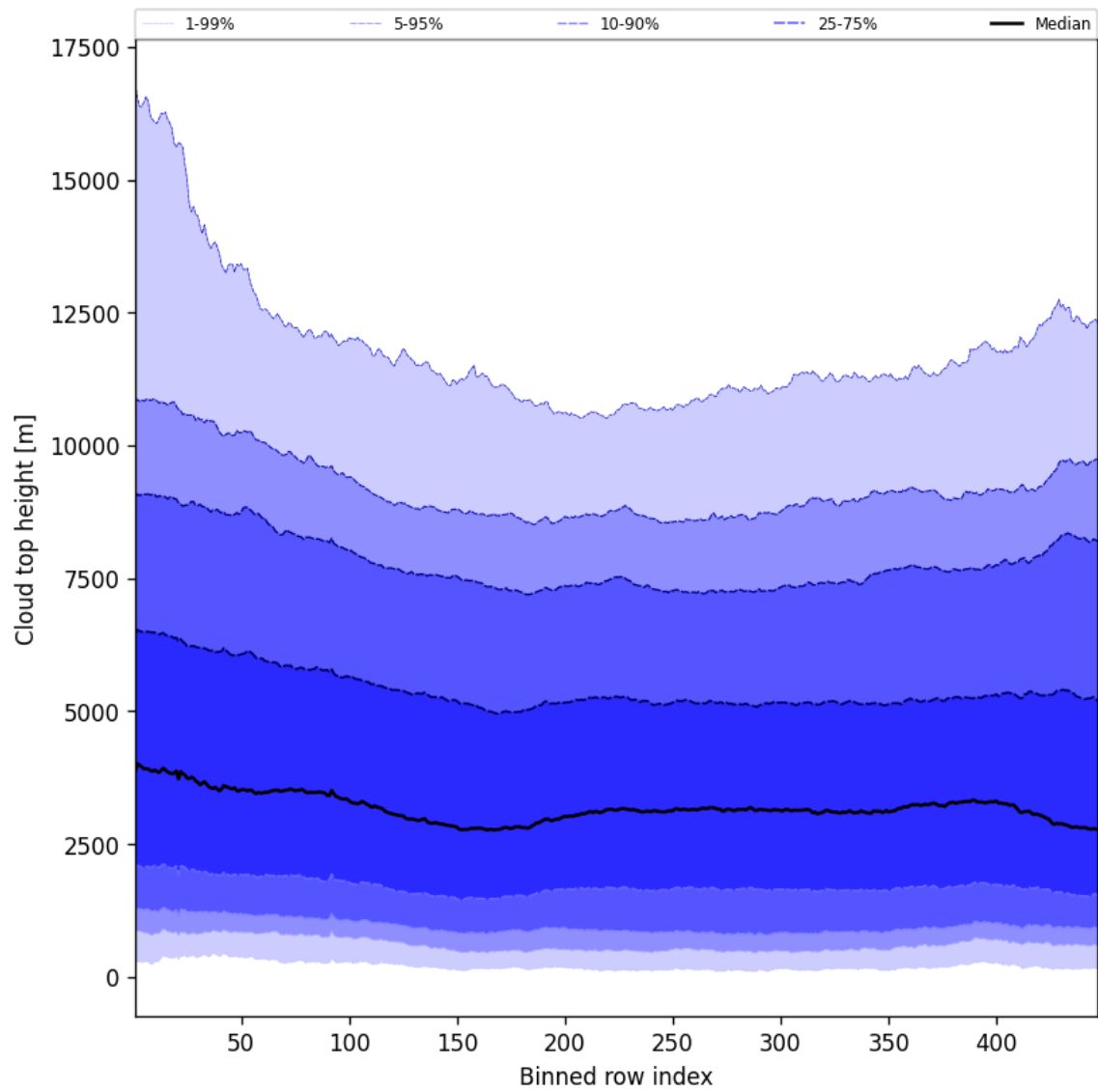
Figure 56: Along track statistics of “Cloud top height” for 2024-09-01 to 2024-09-02
