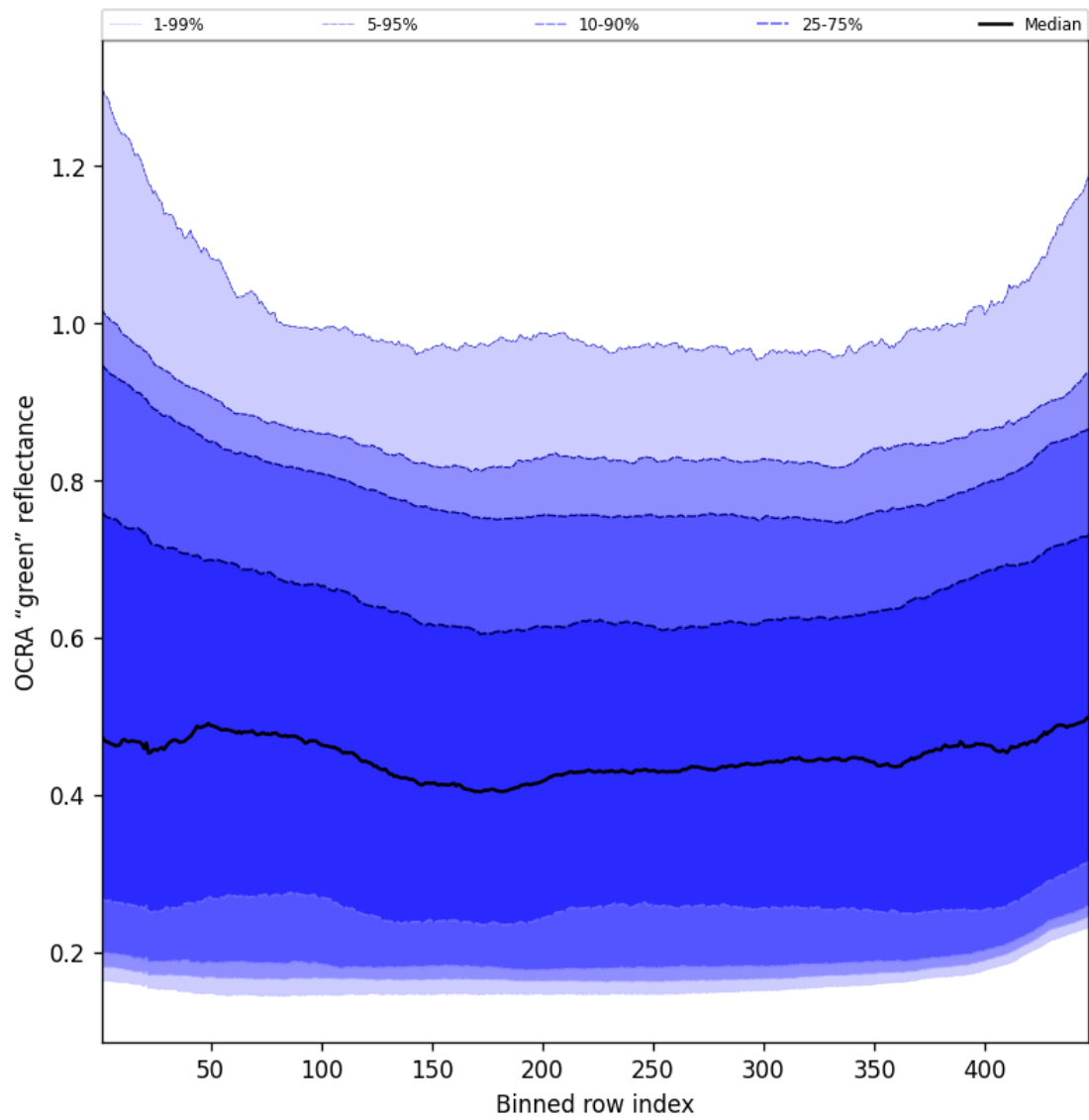
Figure 68: Along track statistics of "OCRA "green" reflectance" for 2024-09-01 to 2024-09-02
