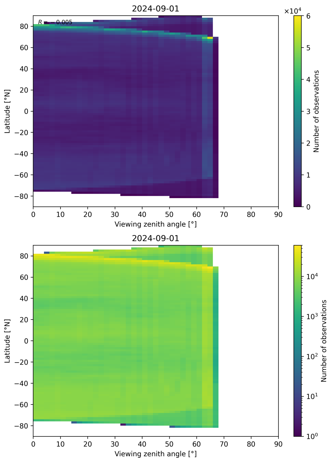
Figure 113: Scatter density plot of “Viewing zenith angle” against “Latitude” for 2024-09-01 to 2024-09-02.
