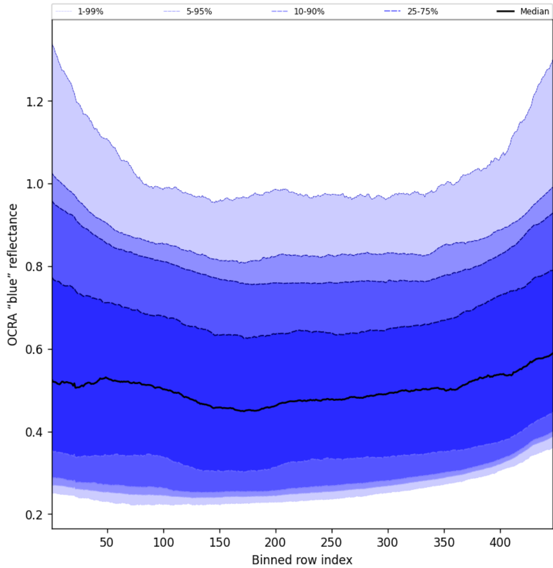
Figure 67: Along track statistics of "OCRA "blue" reflectance" for 2024-09-01 to 2024-09-02
