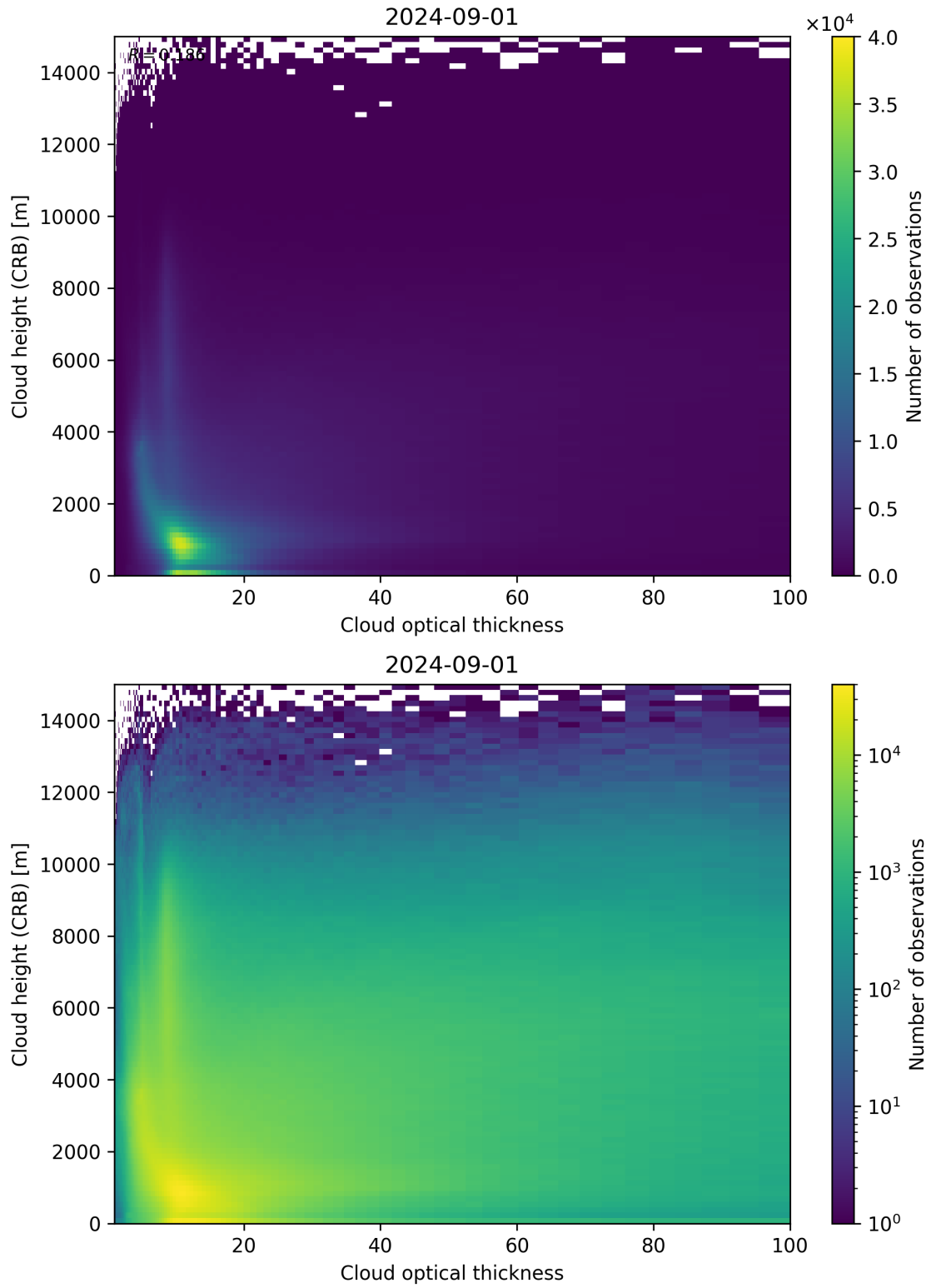
Figure 85: Scatter density plot of “Cloud optical thickness” against “Cloud height (CRB)” for 2024-09-01 to 2024-09-02.
