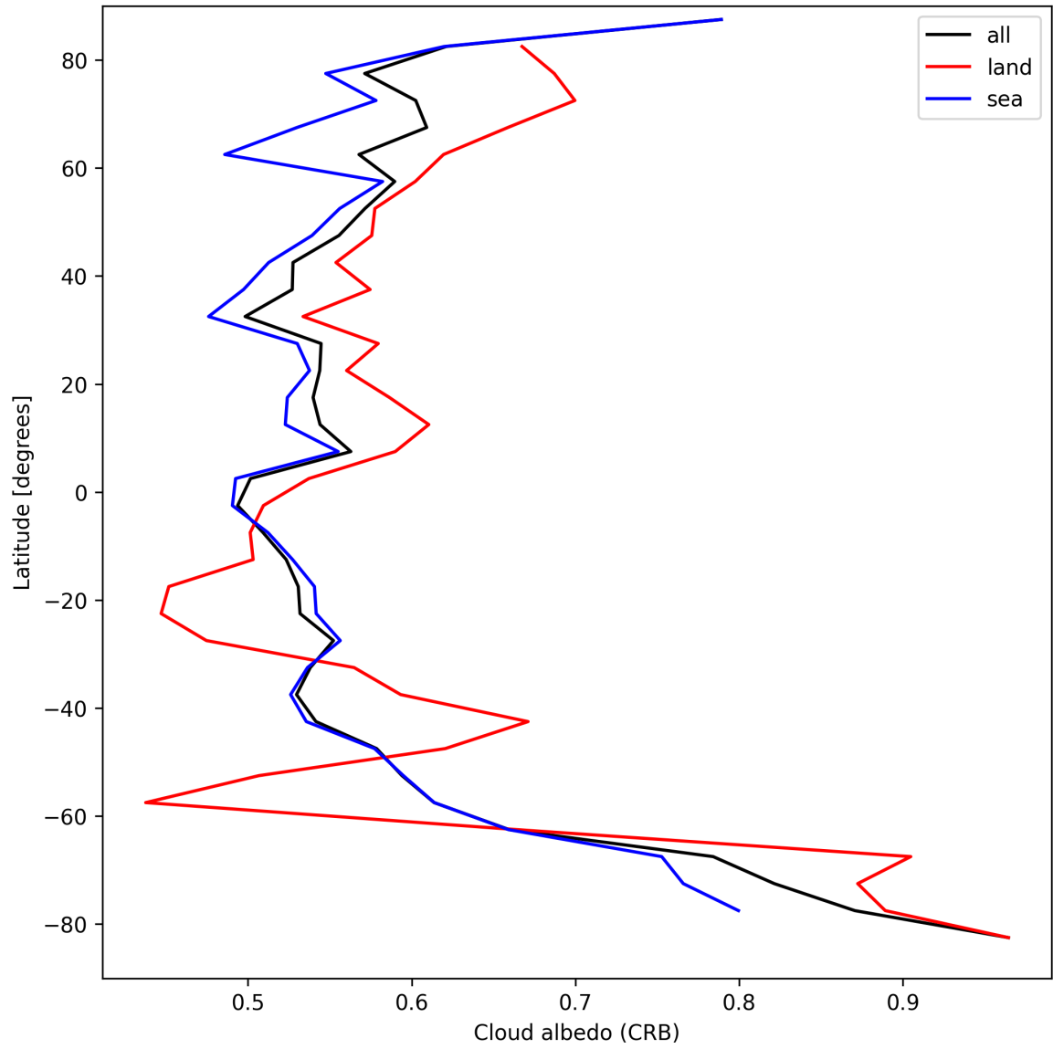
Figure 28: Zonal average of “Cloud albedo (CRB)” for 2024-09-01 to 2024-09-02.
