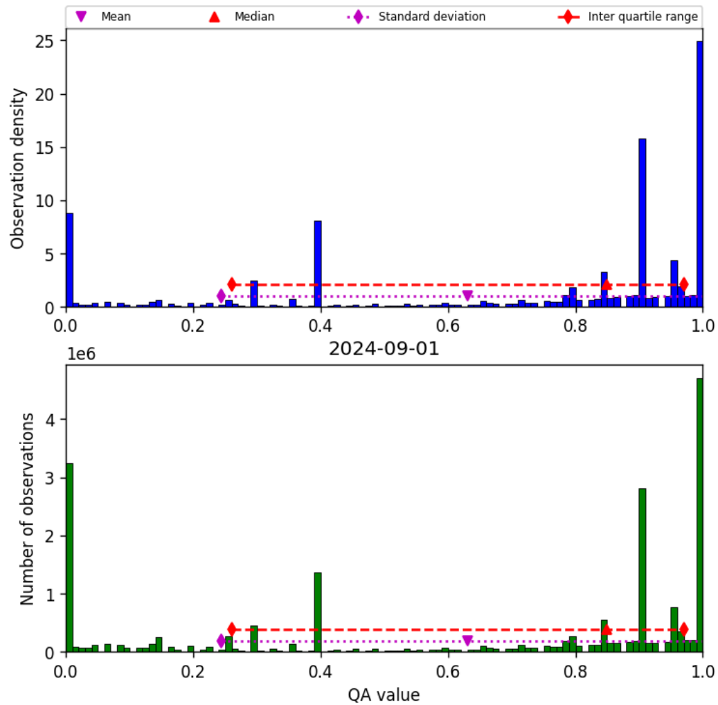
Figure 38: Histogram of “QA value” for 2024-09-01 to 2024-09-02
