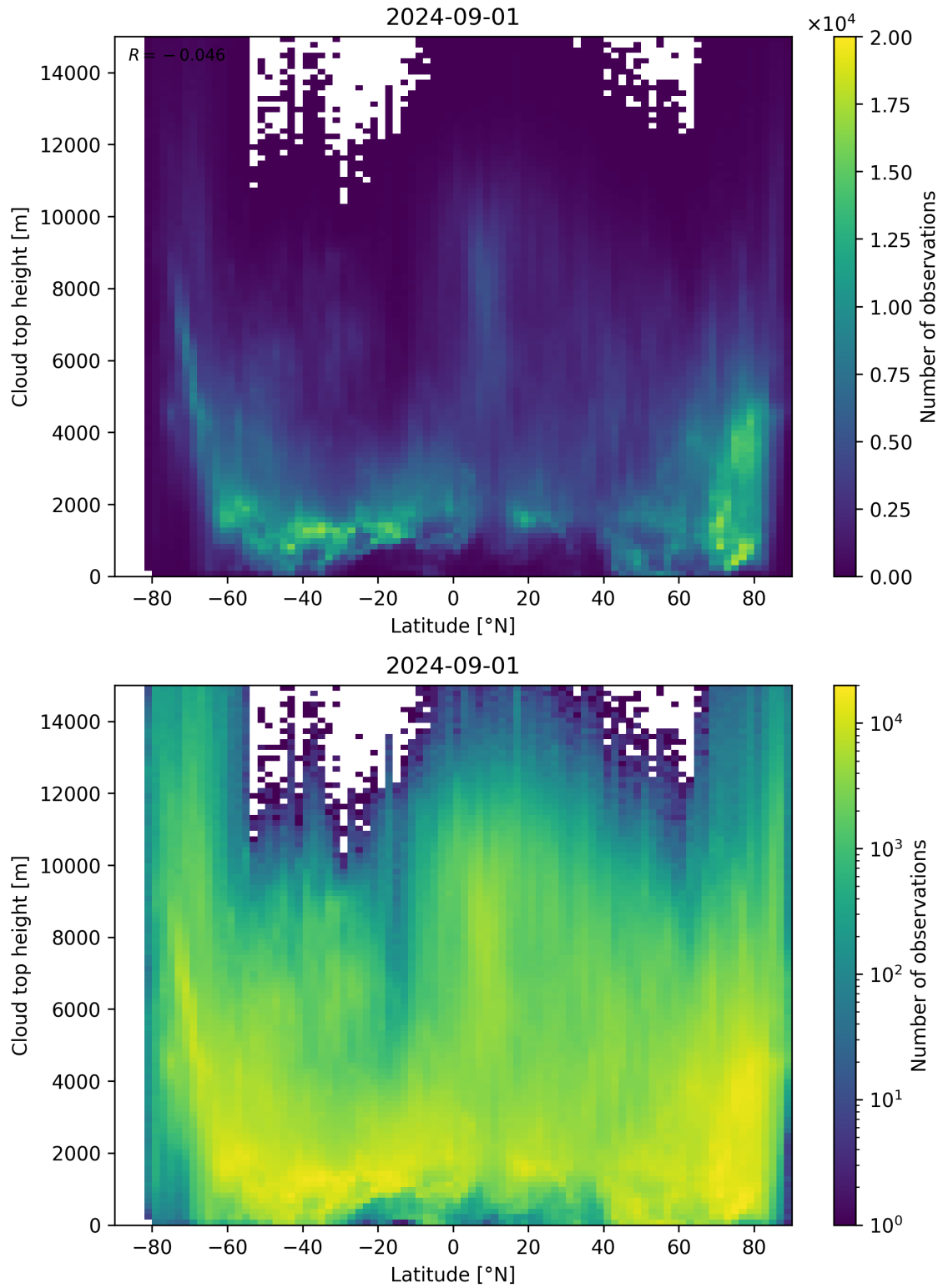
Figure 97: Scatter density plot of “Latitude” against “Cloud top height” for 2024-09-01 to 2024-09-02.
