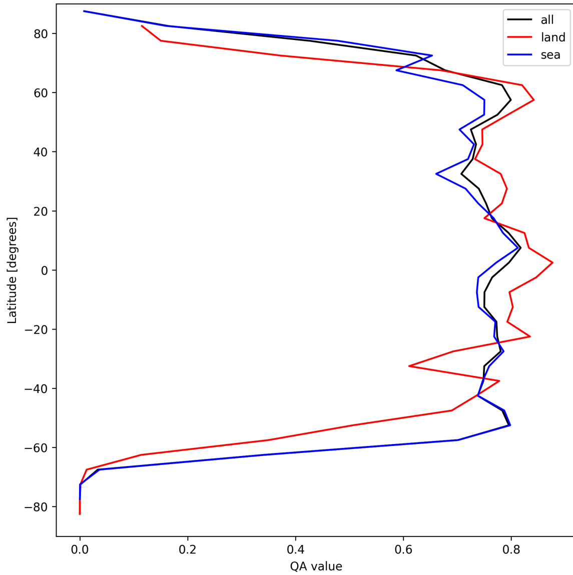
Figure 22: Zonal average of “QA value” for 2024-09-01 to 2024-09-02.
