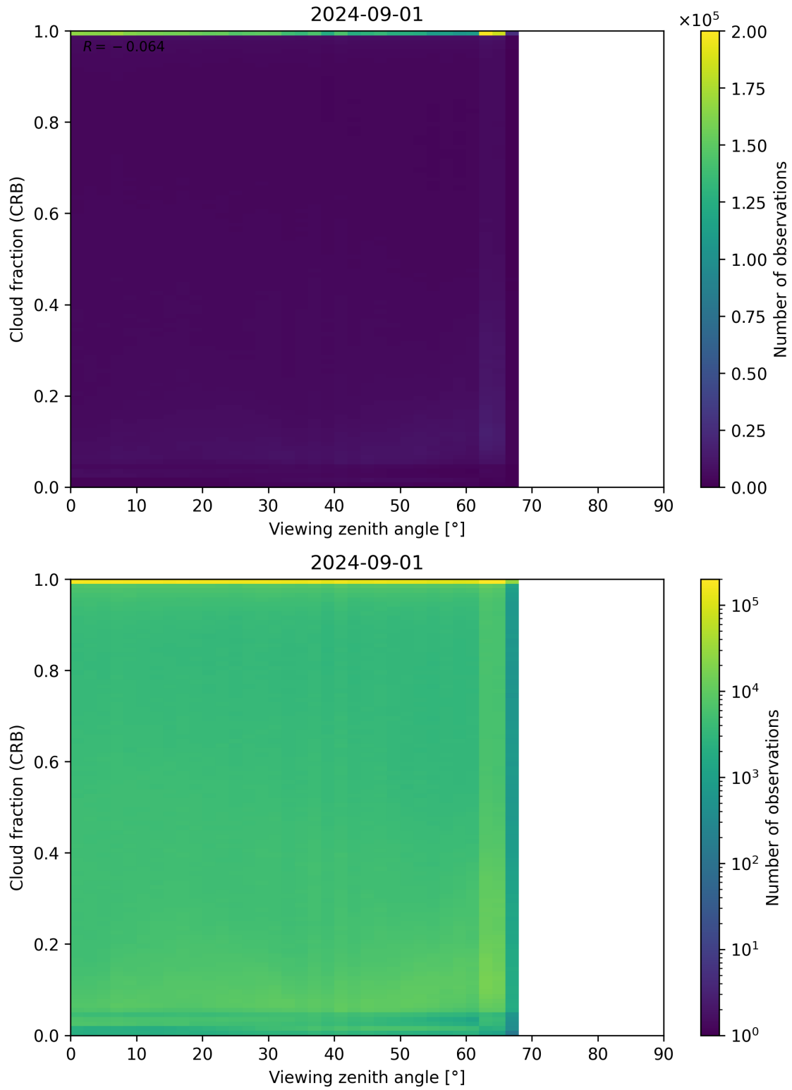
Figure 109: Scatter density plot of “Viewing zenith angle” against “Cloud fraction (CRB)” for 2024-09-01 to 2024-09-02.
