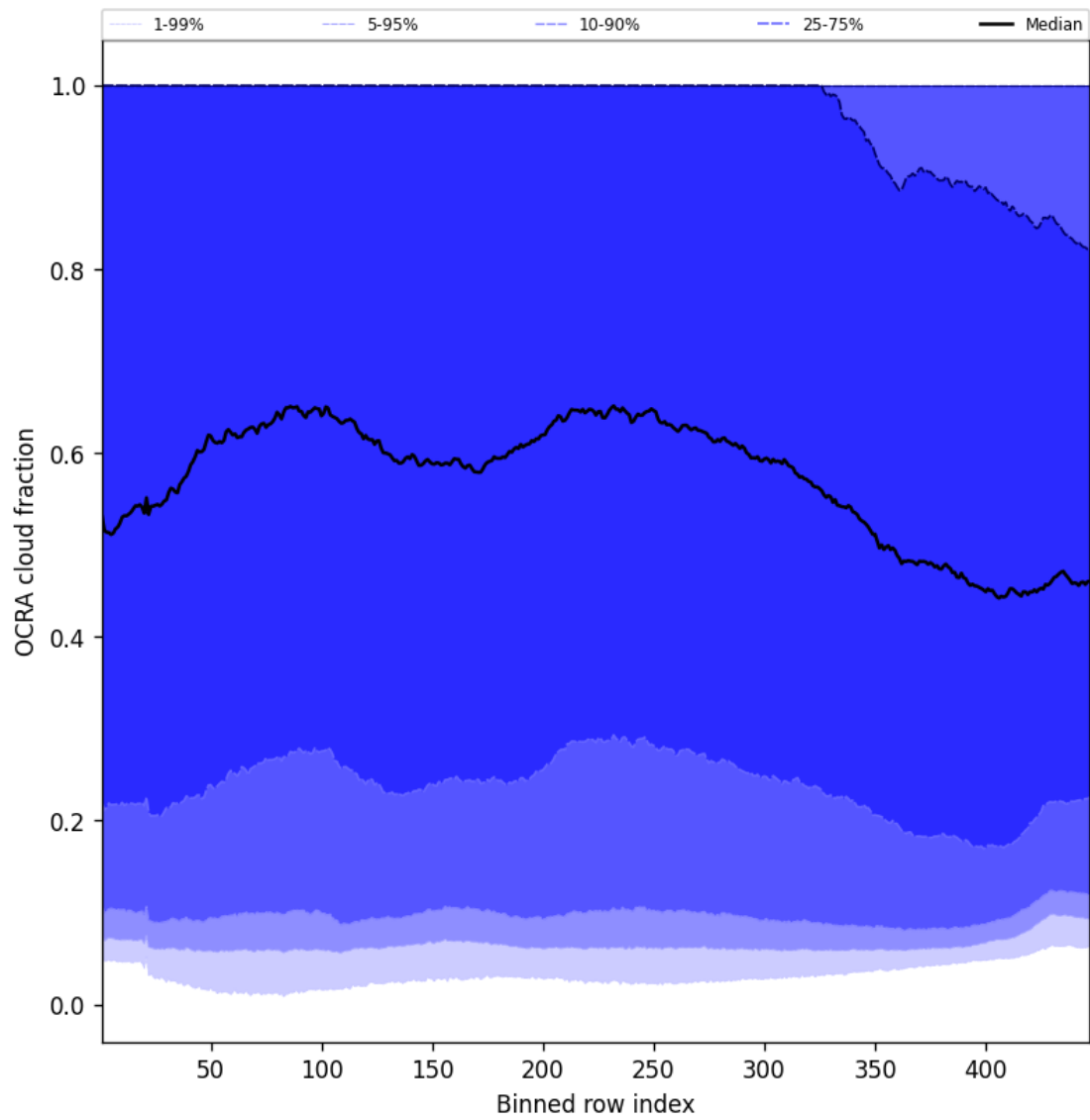
Figure 66: Along track statistics of “OCRA cloud fraction” for 2024-09-01 to 2024-09-02
