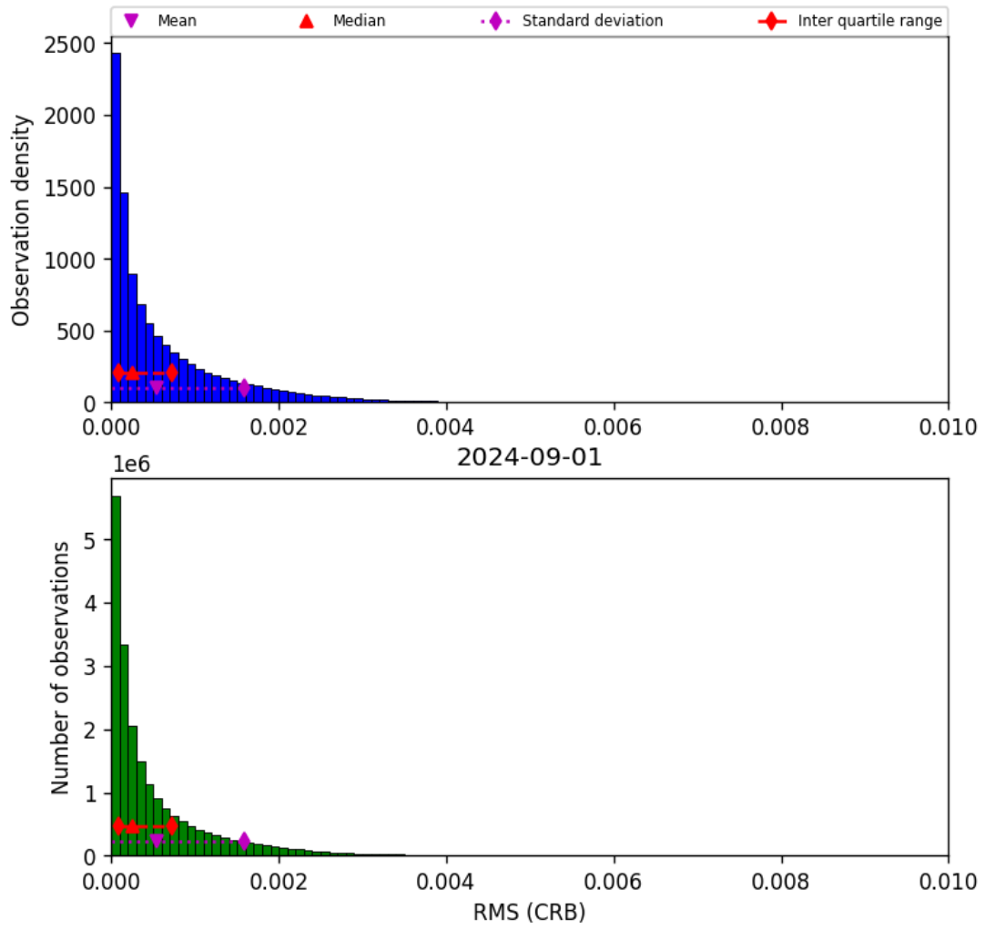
Figure 48: Histogram of “RMS (CRB)” for 2024-09-01 to 2024-09-02
