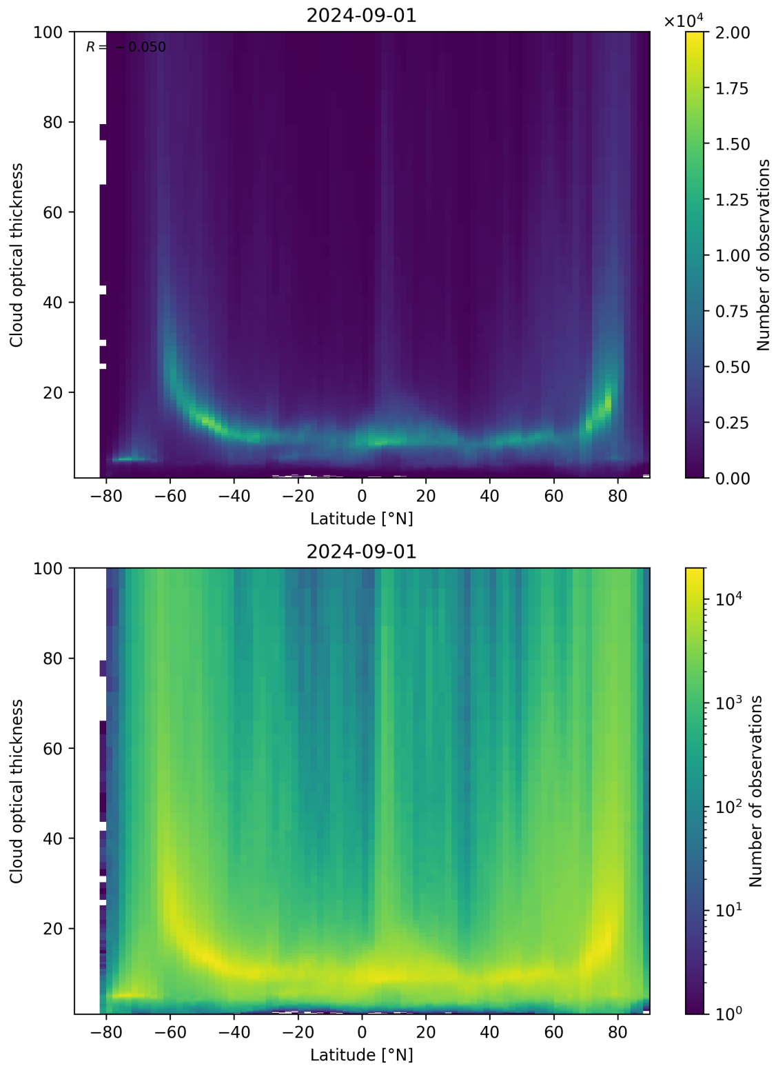
Figure 96: Scatter density plot of “Latitude” against “Cloud optical thickness” for 2024-09-01 to 2024-09-02.
