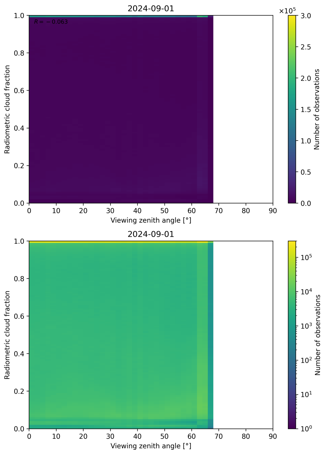
Figure 107: Scatter density plot of “Viewing zenith angle” against “Radiometric cloud fraction” for 2024-09-01 to 2024-09-02.
