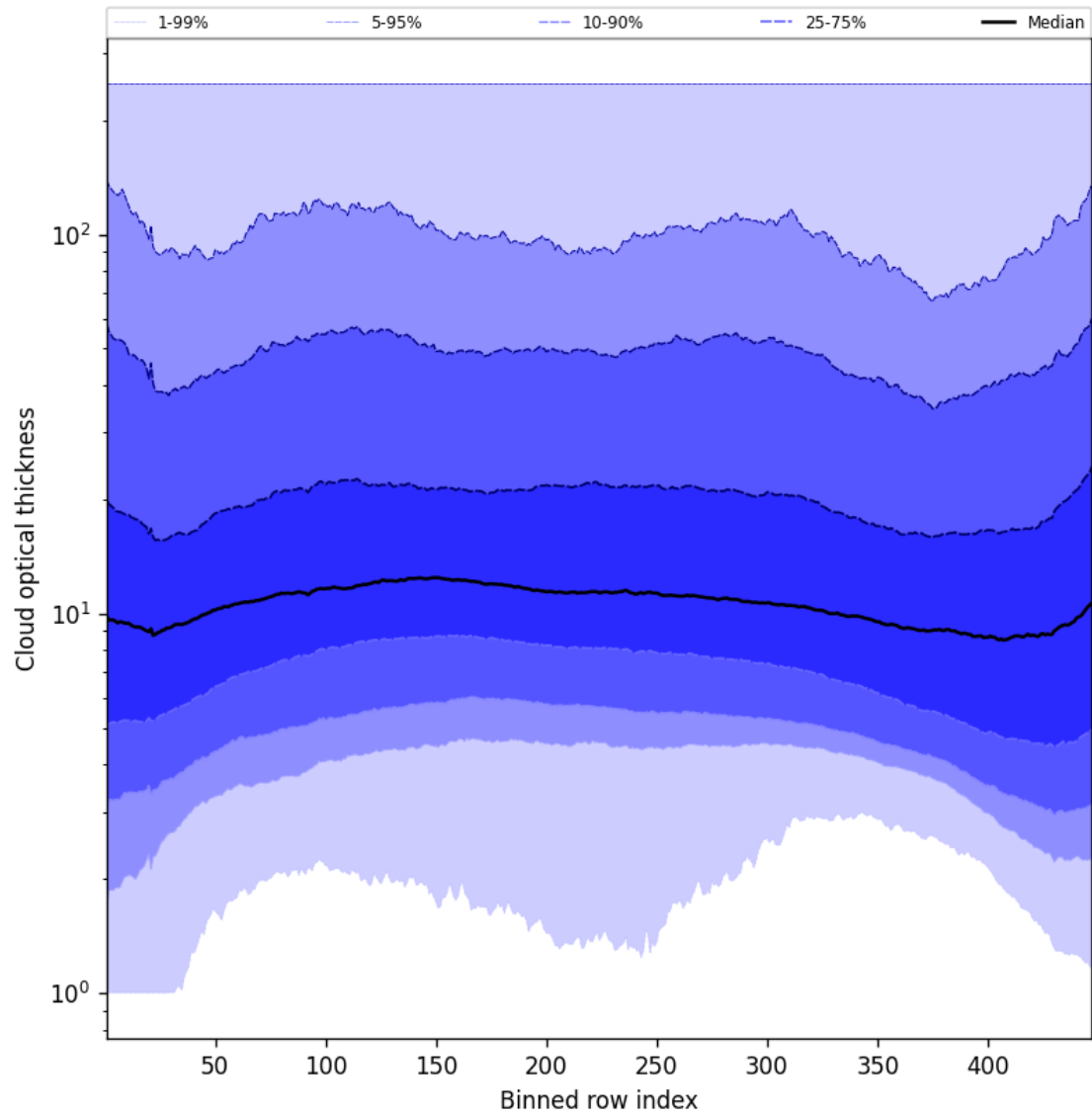
Figure 57: Along track statistics of “Cloud optical thickness” for 2024-09-01 to 2024-09-02
