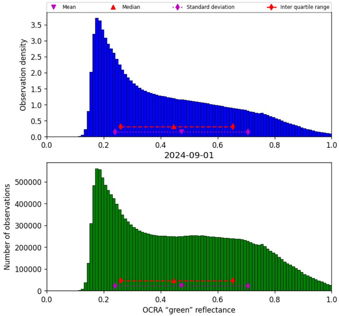
Figure 52: Histogram of “OCRA “green” reflectance” for 2024-09-01 to 2024-09-02
