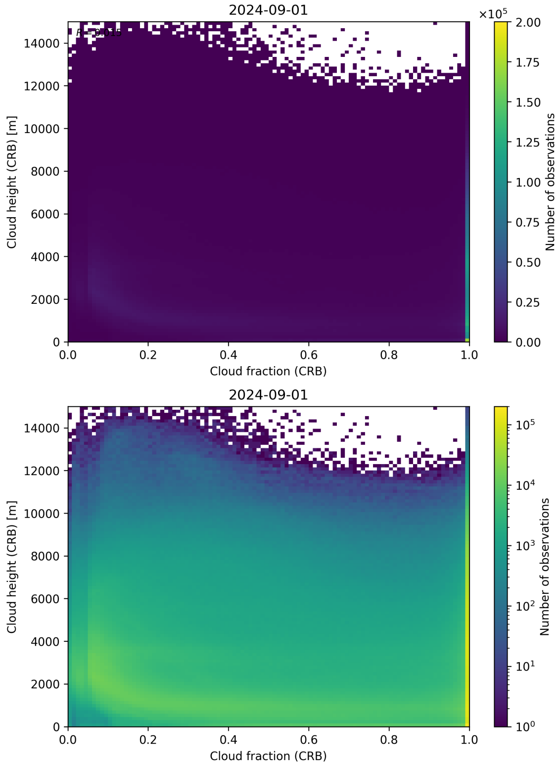
Figure 79: Scatter density plot of “Cloud fraction (CRB)” against “Cloud height (CRB)” for 2024-09-01 to 2024-09-02.
