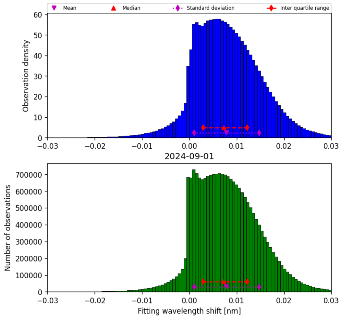
Figure 49: Histogram of “Fitting wavelength shift” for 2024-09-01 to 2024-09-02
