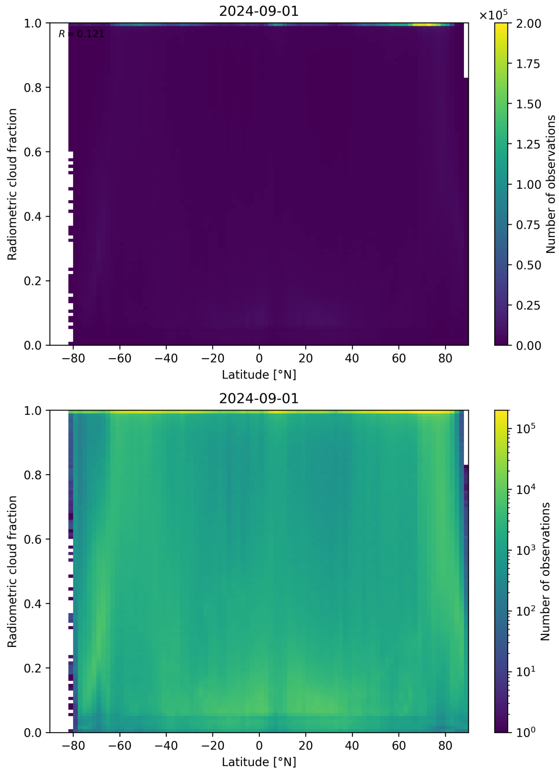
Figure 92: Scatter density plot of “Latitude” against “Radiometric cloud fraction” for 2024-09-01 to 2024-09-02.
