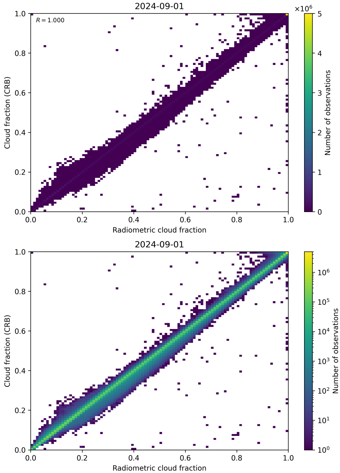
Figure 73: Scatter density plot of “Radiometric cloud fraction” against “Cloud fraction (CRB)” for 2024-09-01 to 2024-09-02.
