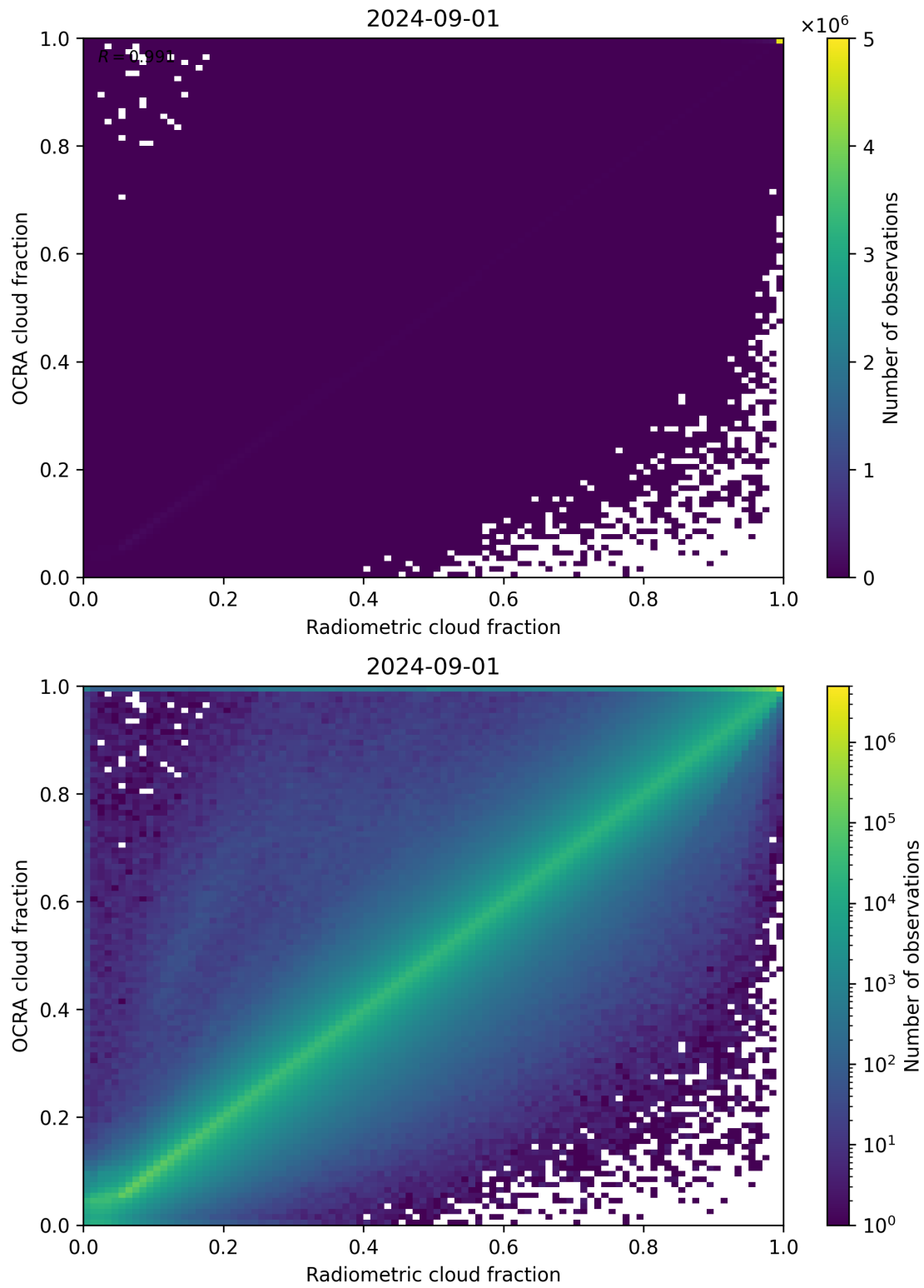
Figure 72: Scatter density plot of “Radiometric cloud fraction” against “OCRA cloud fraction” for 2024-09-01 to 2024-09-02.
