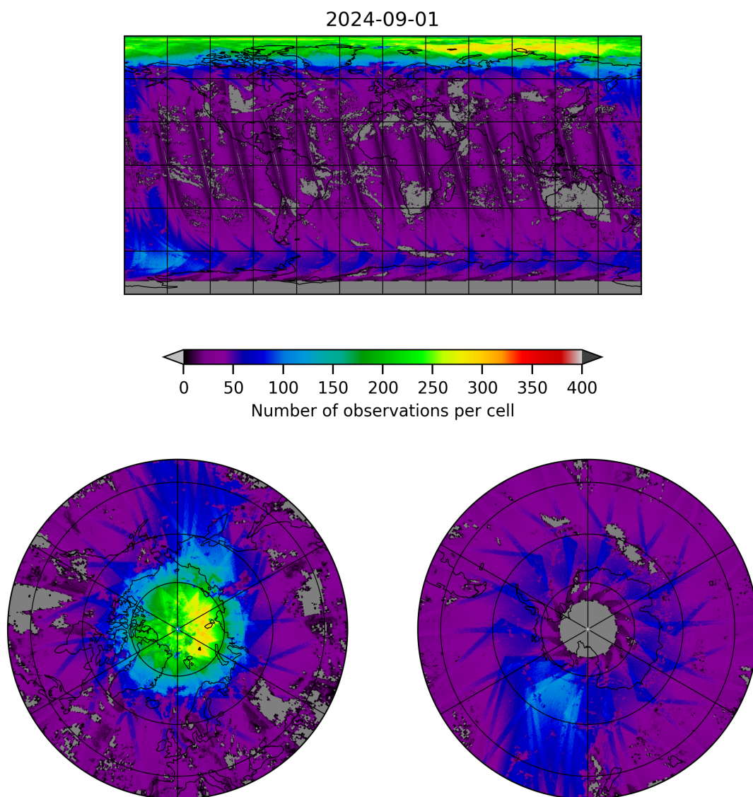
Figure 21: Map of the number of observations for 2024-09-01 to 2024-09-02
