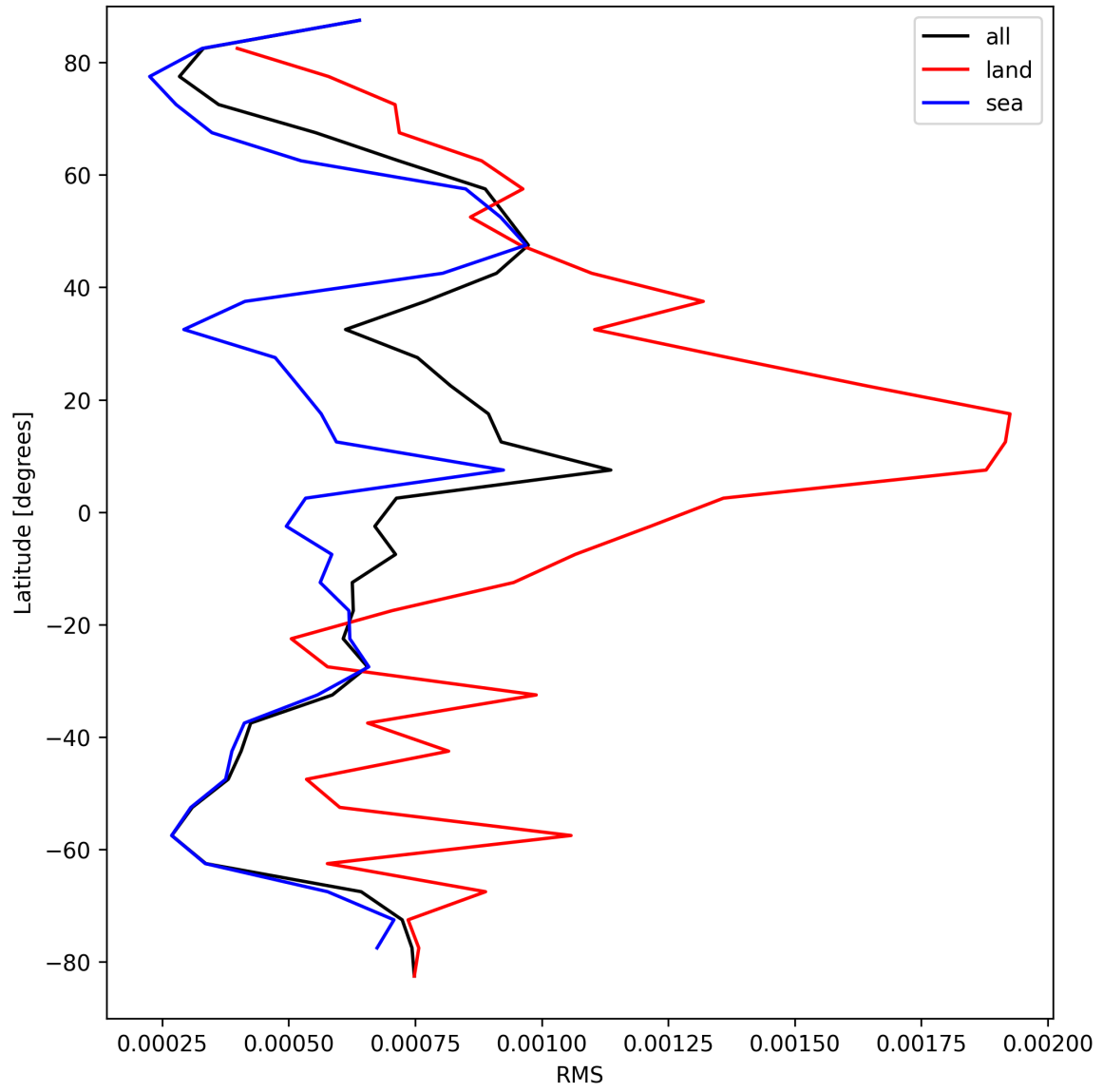
Figure 31: Zonal average of “RMS” for 2024-09-01 to 2024-09-02.
