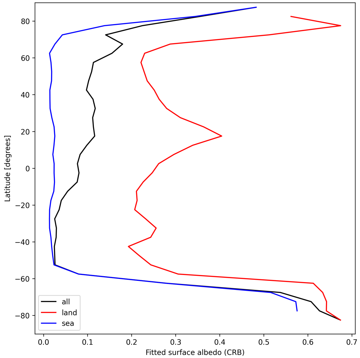
Figure 30: Zonal average of “Fitted surface albedo (CRB)” for 2024-09-01 to 2024-09-02.
