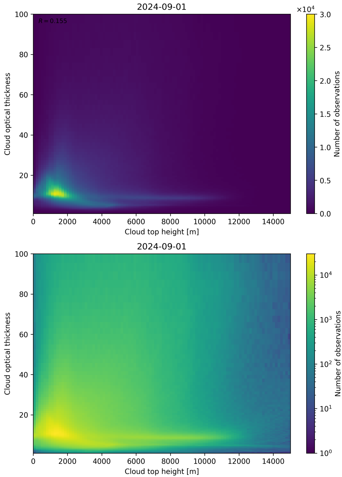
Figure 90: Scatter density plot of “Cloud top height” against “Cloud optical thickness” for 2024-09-01 to 2024-09-02.
