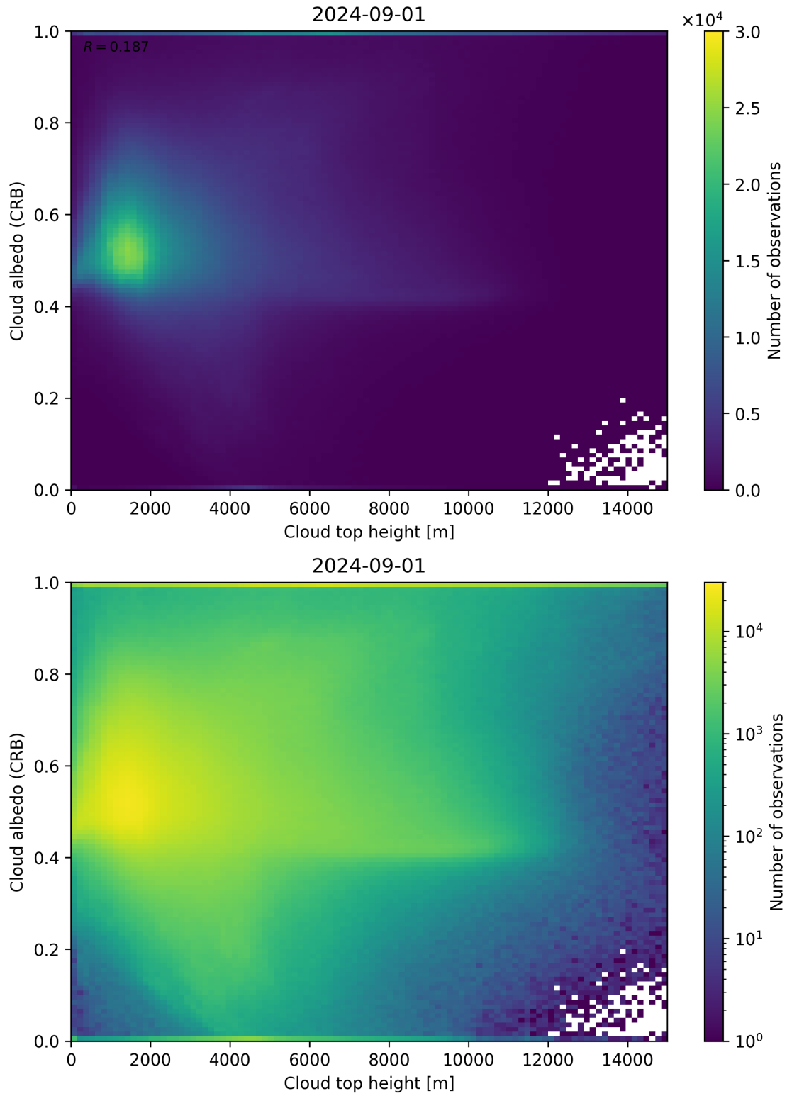
Figure 86: Scatter density plot of “Cloud top height” against “Cloud albedo (CRB)” for 2024-09-01 to 2024-09-02.
