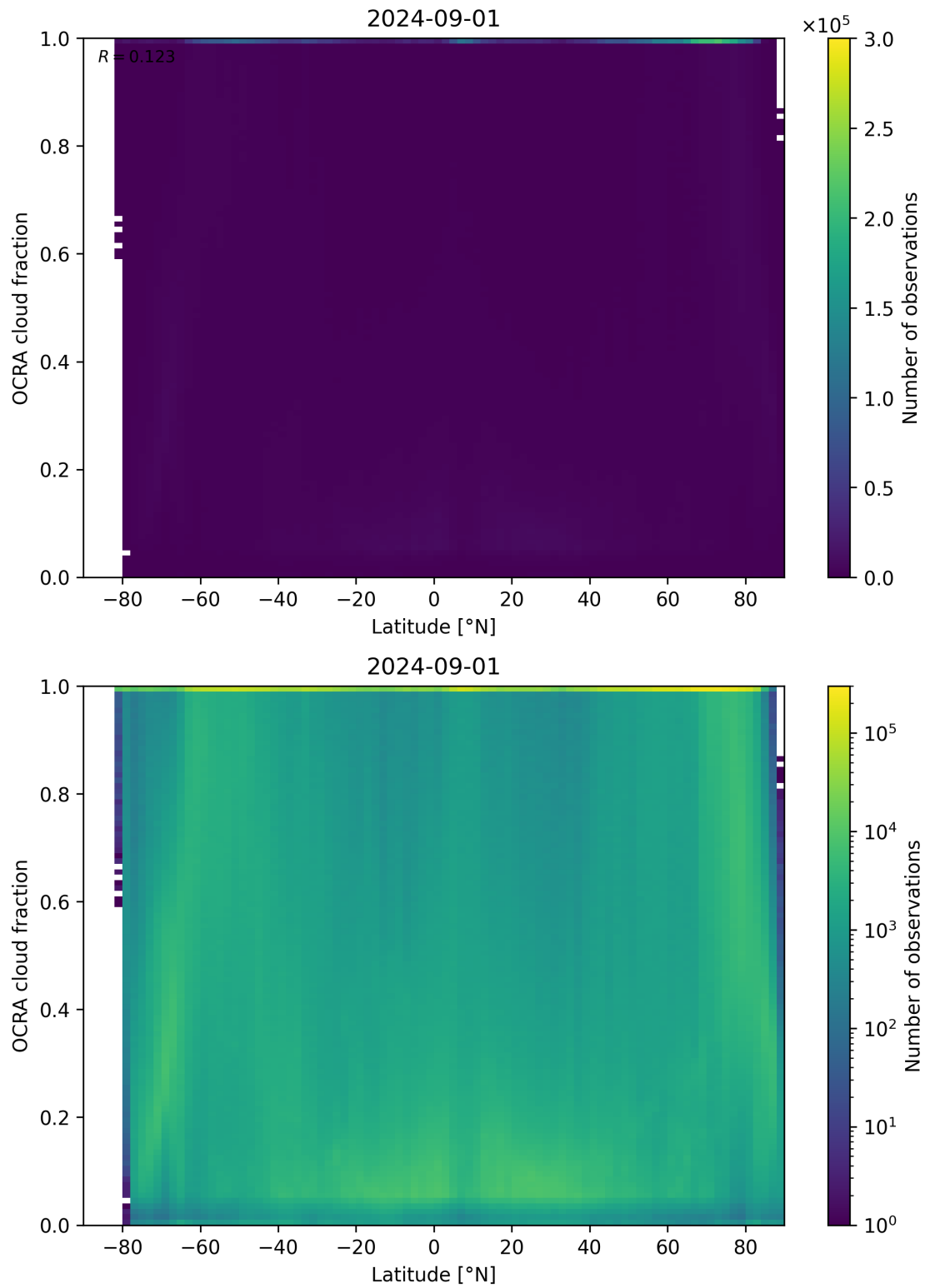
Figure 93: Scatter density plot of “Latitude” against “OCRA cloud fraction” for 2024-09-01 to 2024-09-02.
