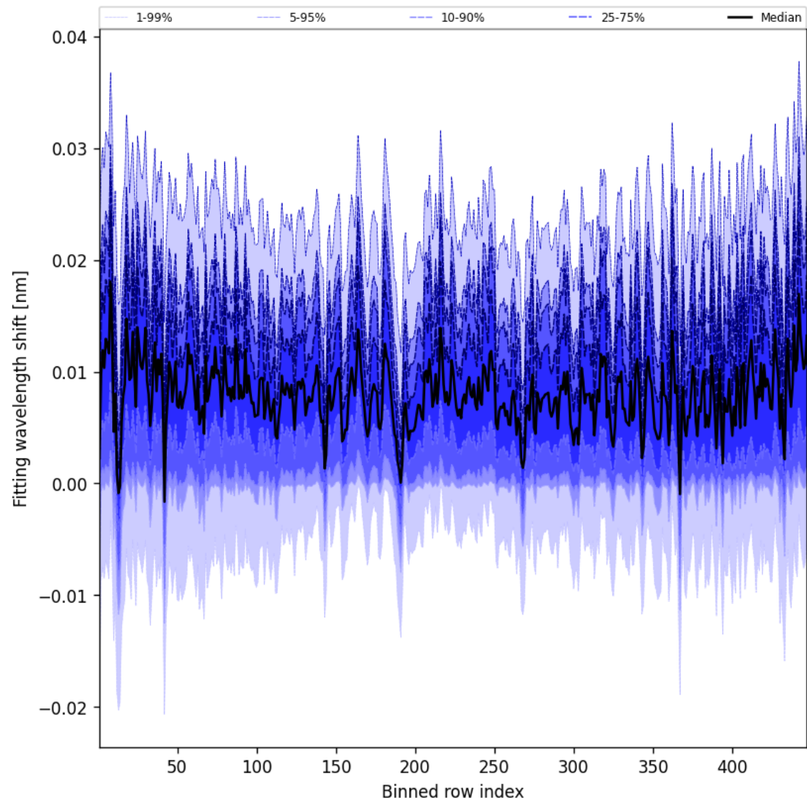
Figure 65: Along track statistics of “Fitting wavelength shift” for 2024-09-01 to 2024-09-02
