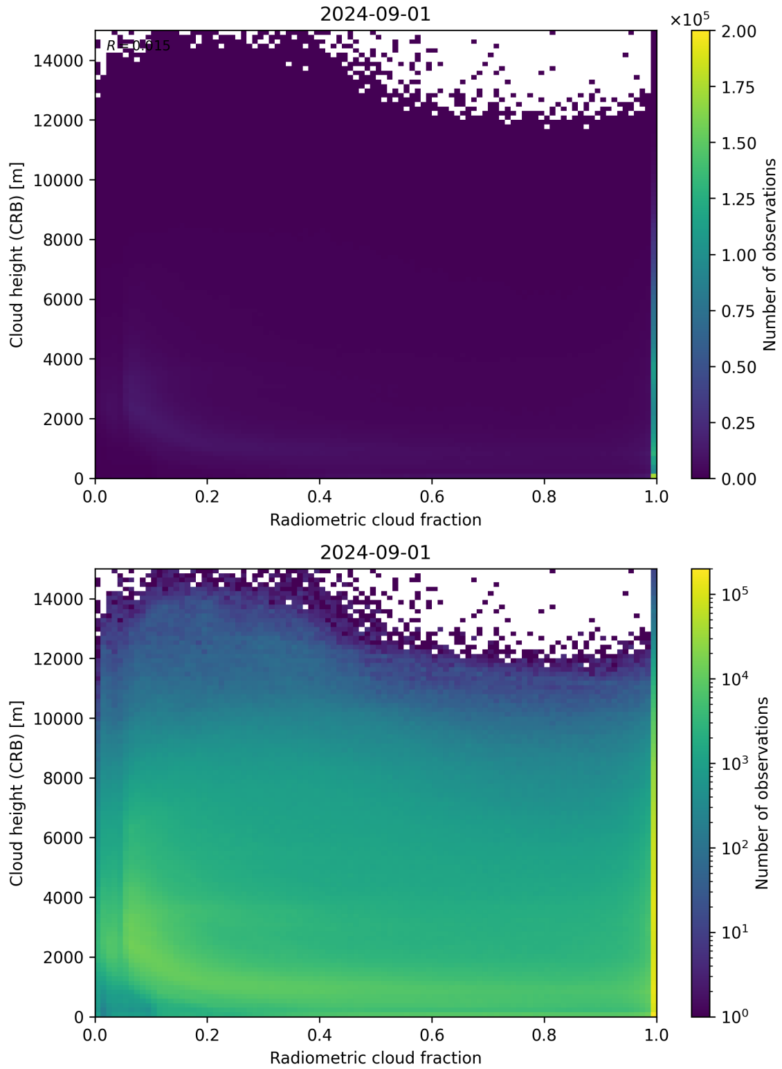
Figure 74: Scatter density plot of “Radiometric cloud fraction” against “Cloud height (CRB)” for 2024-09-01 to 2024-09-02.
