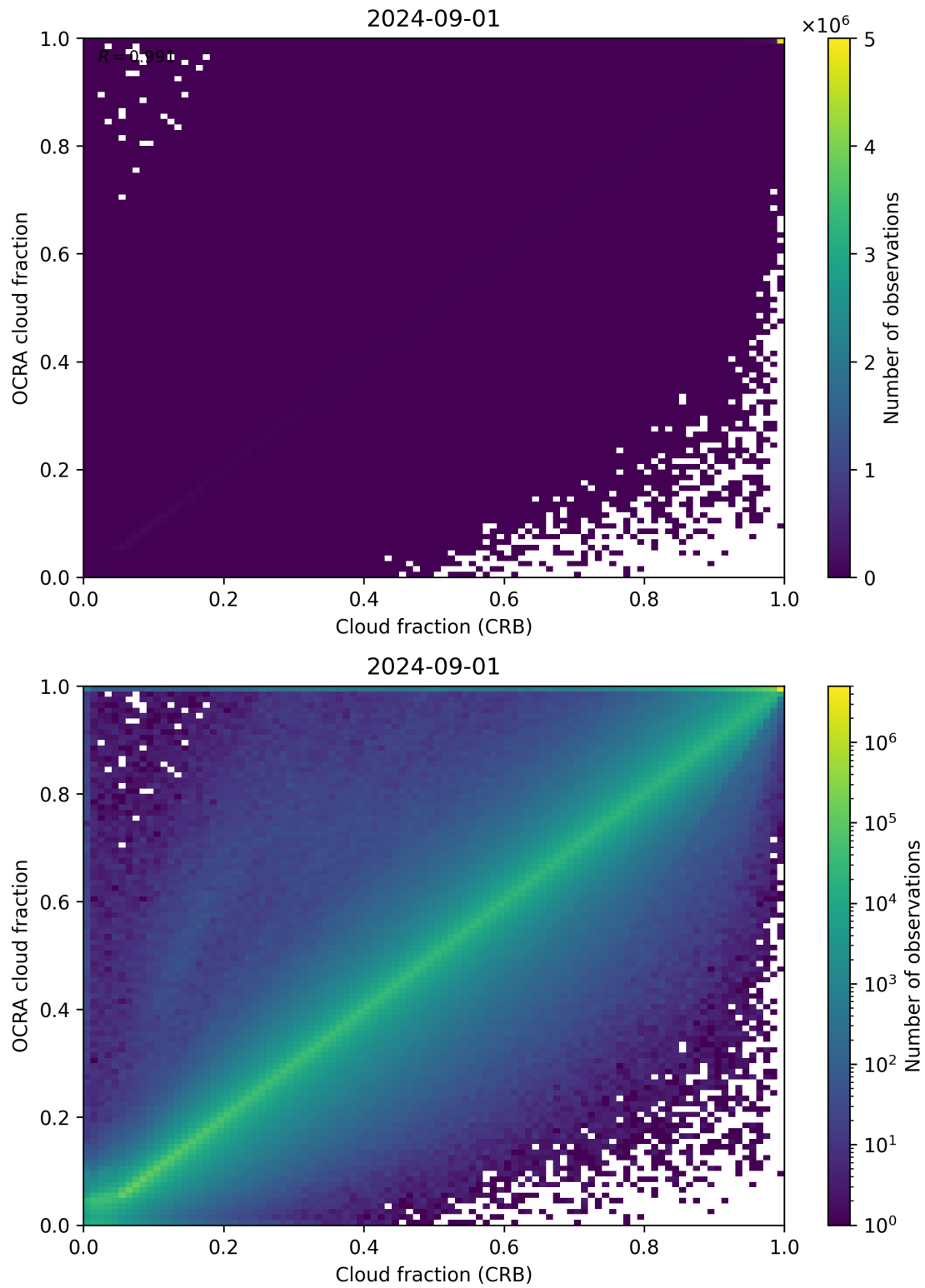
Figure 78: Scatter density plot of “Cloud fraction (CRB)” against “OCRA cloud fraction” for 2024-09-01 to 2024-09-02.
