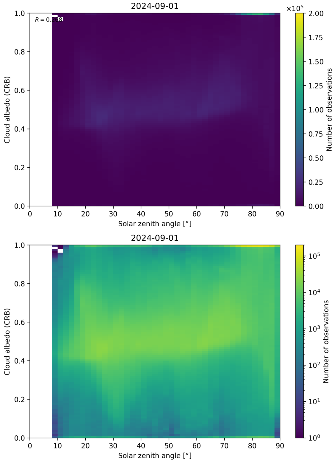
Figure 98: Scatter density plot of “Solar zenith angle” against “Cloud albedo (CRB)” for 2024-09-01 to 2024-09-02.
