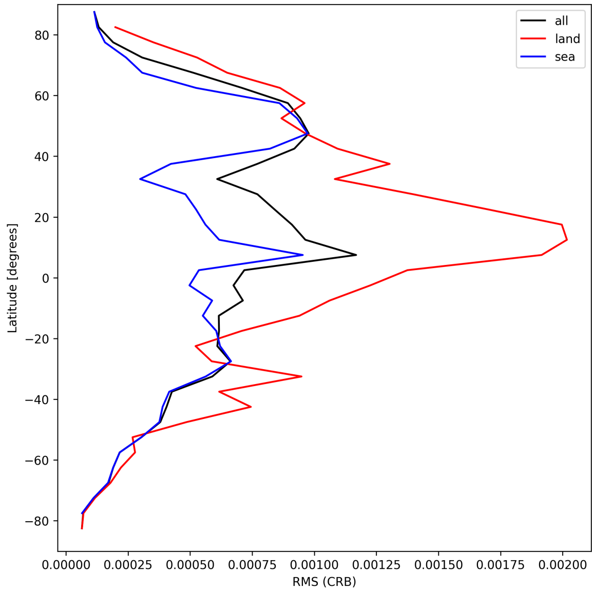
Figure 32: Zonal average of “RMS (CRB)” for 2024-09-01 to 2024-09-02.
