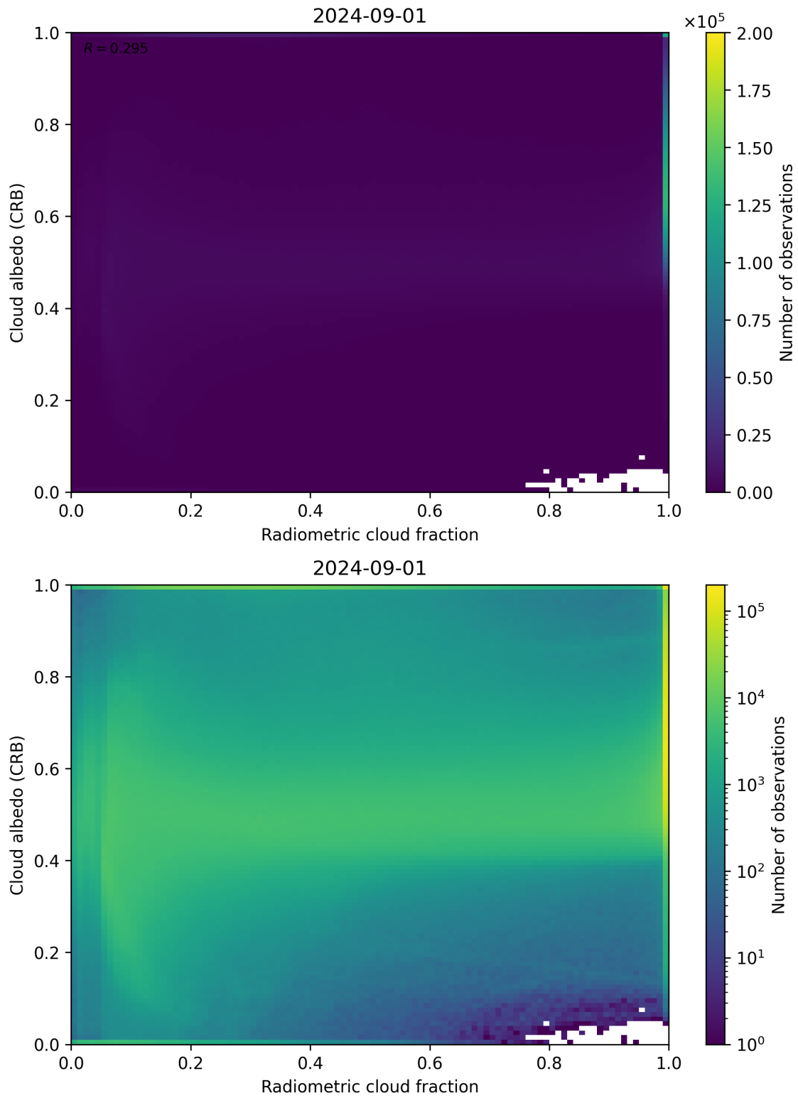
Figure 71: Scatter density plot of “Radiometric cloud fraction” against “Cloud albedo (CRB)” for 2024-09-01 to 2024-09-02.
