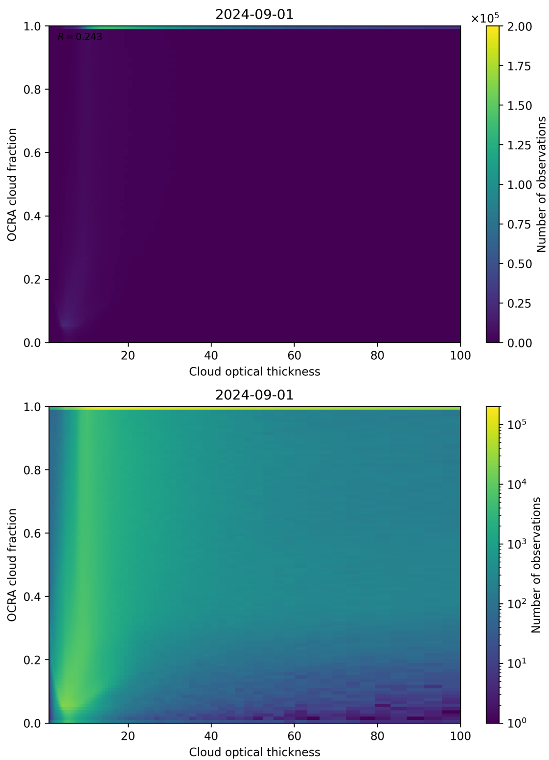
Figure 83: Scatter density plot of “Cloud optical thickness” against “OCRA cloud fraction” for 2024-09-01 to 2024-09-02.
