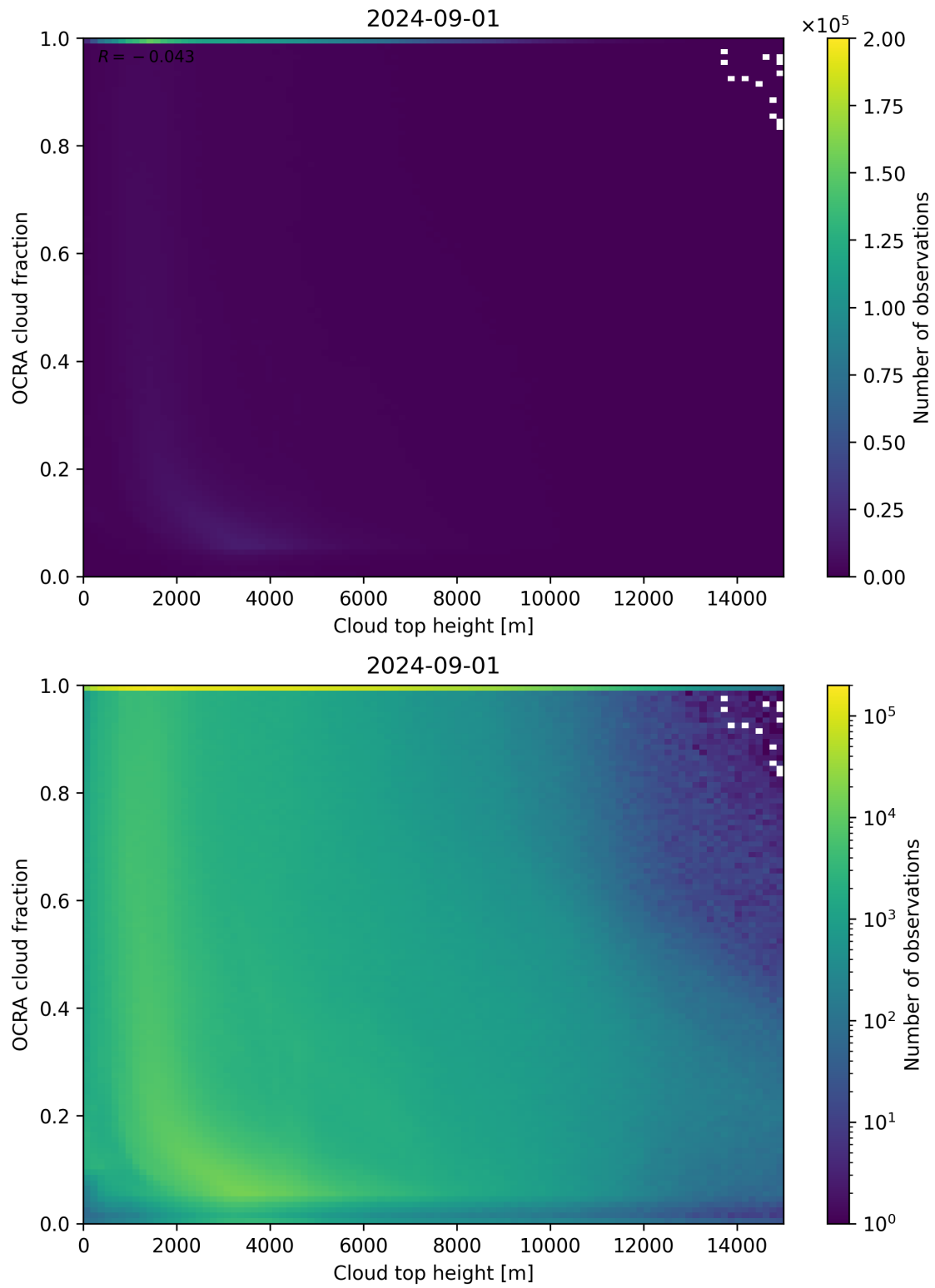
Figure 87: Scatter density plot of “Cloud top height” against “OCRA cloud fraction” for 2024-09-01 to 2024-09-02.
