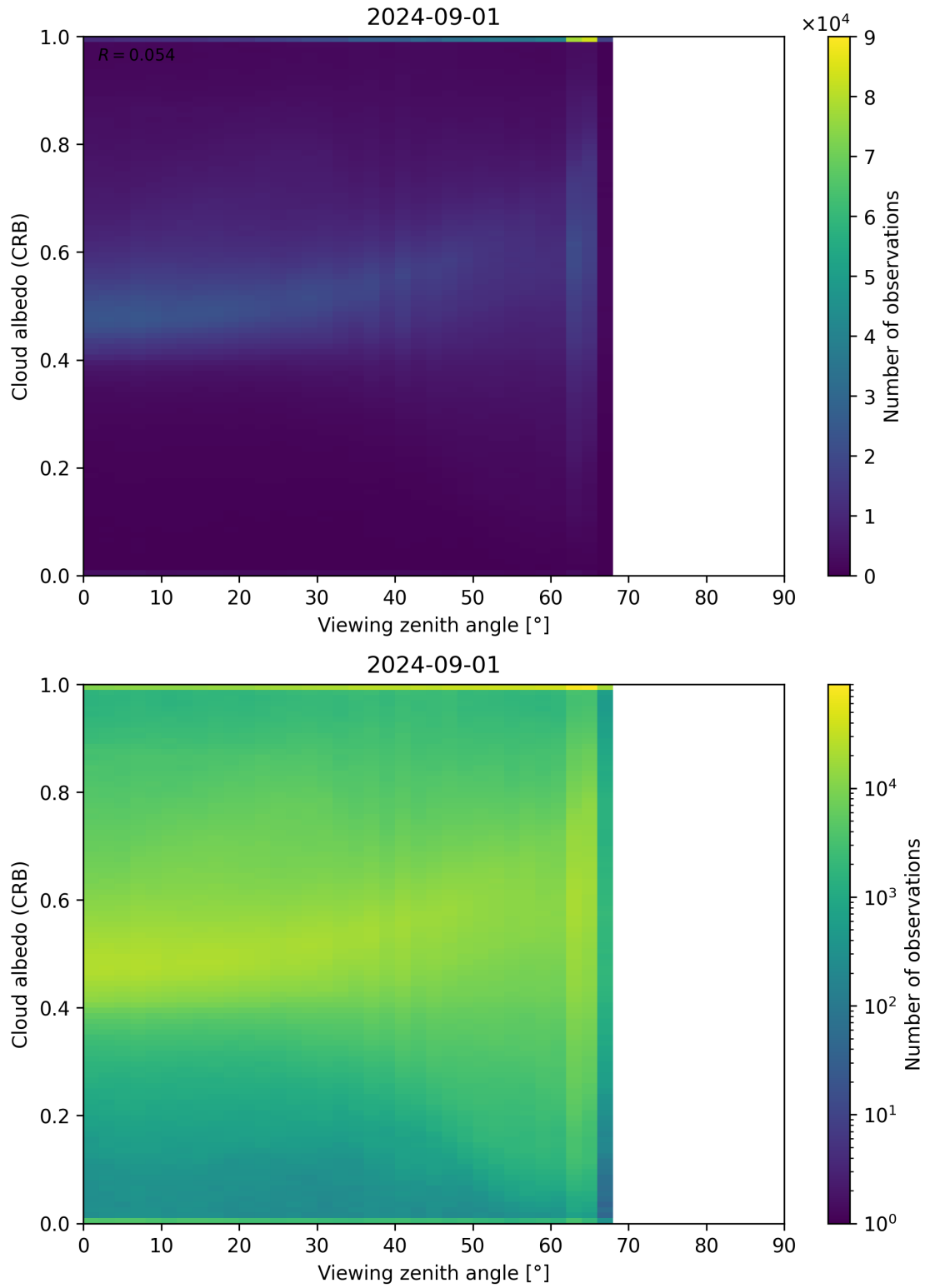
Figure 106: Scatter density plot of “Viewing zenith angle” against “Cloud albedo (CRB)” for 2024-09-01 to 2024-09-02.
