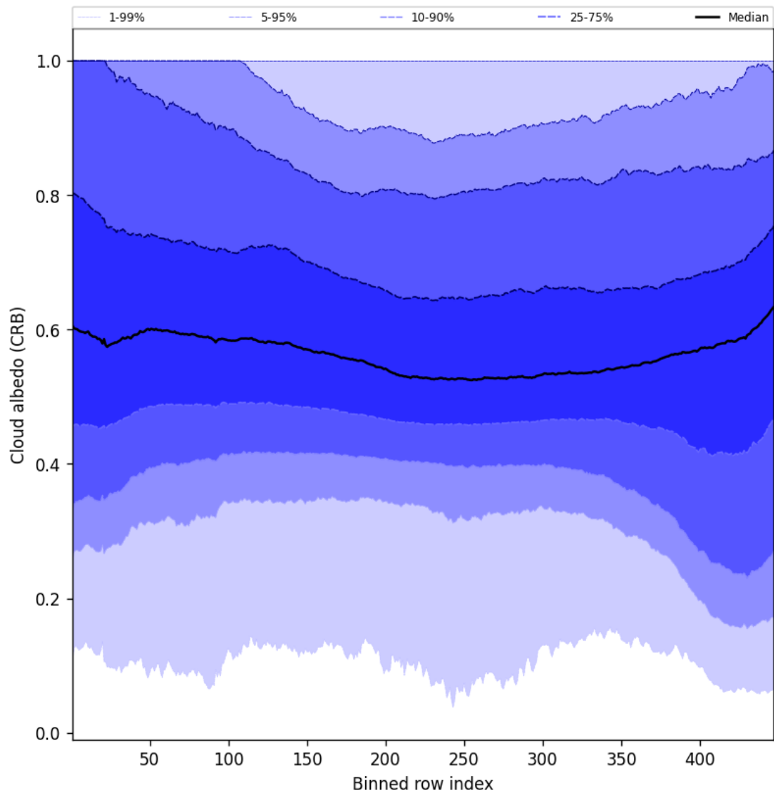
Figure 60: Along track statistics of “Cloud albedo (CRB)” for 2024-09-01 to 2024-09-02
