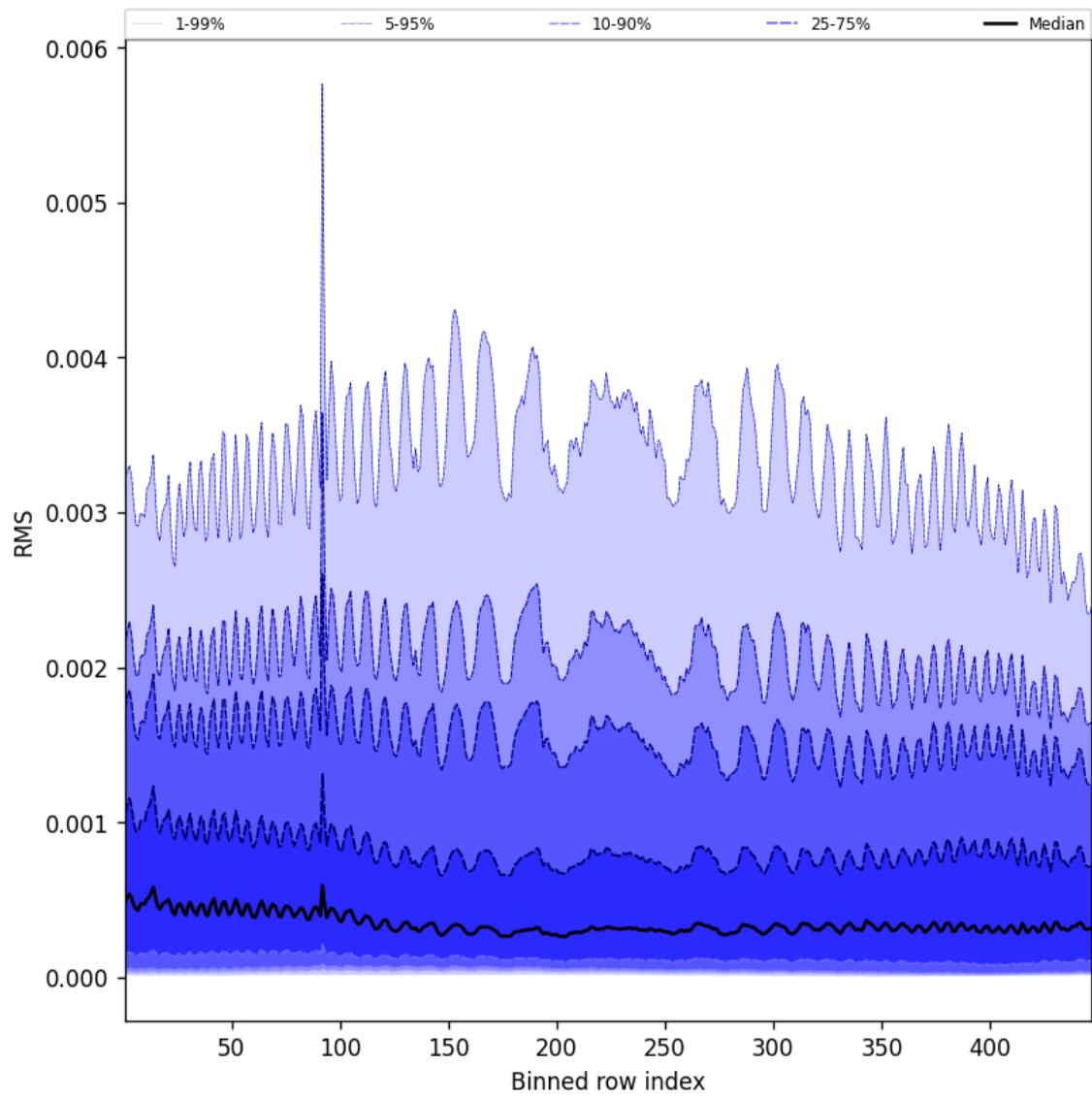
Figure 63: Along track statistics of “RMS” for 2024-09-01 to 2024-09-02
