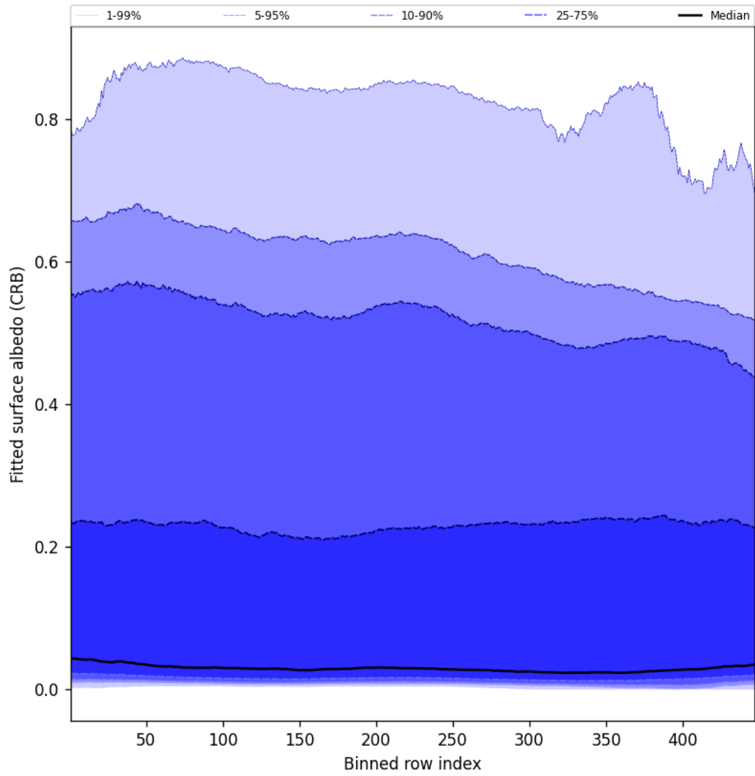
Figure 62: Along track statistics of “Fitted surface albedo (CRB)” for 2024-09-01 to 2024-09-02
