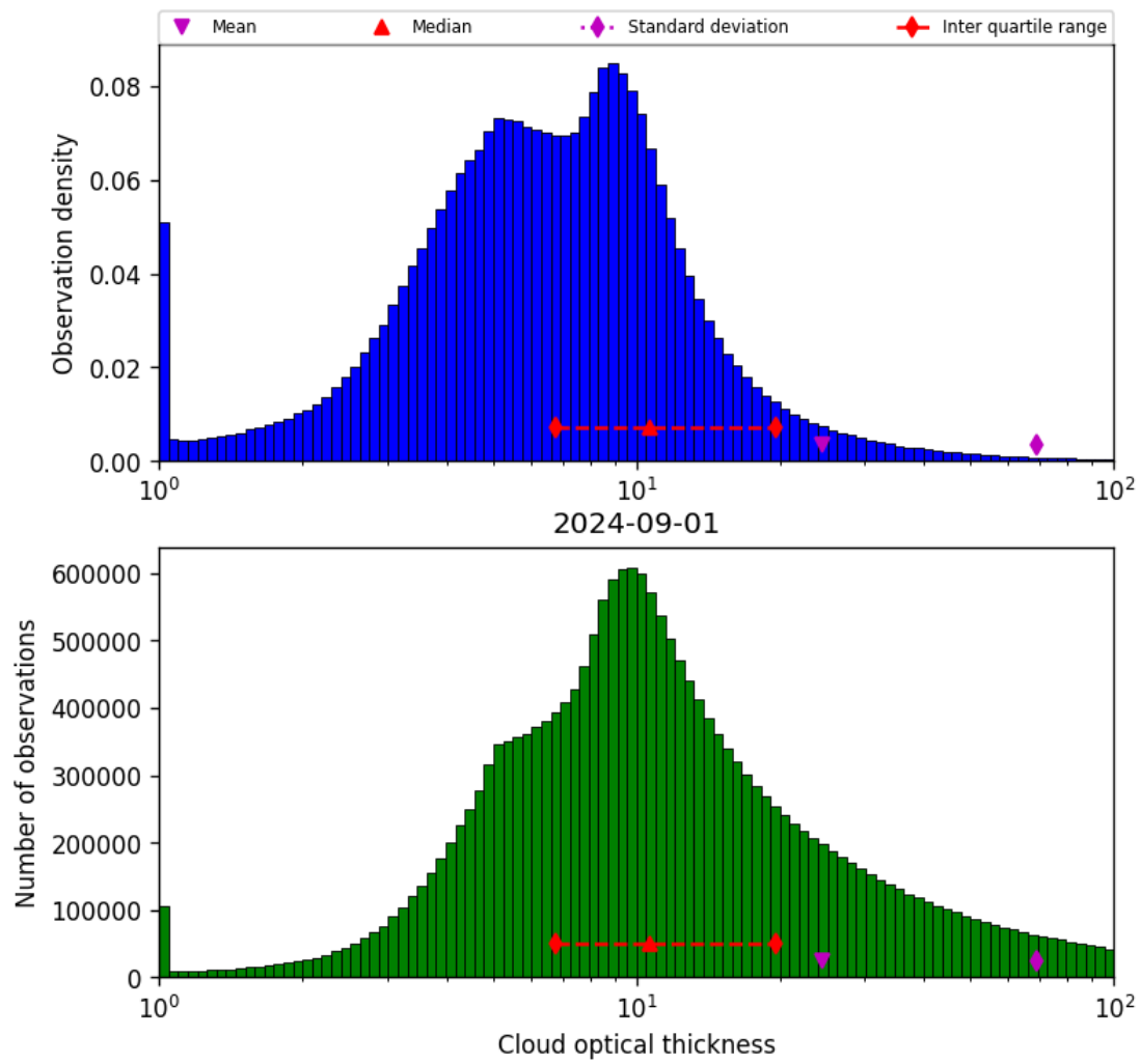
Figure 41: Histogram of “Cloud optical thickness” for 2024-09-01 to 2024-09-02
