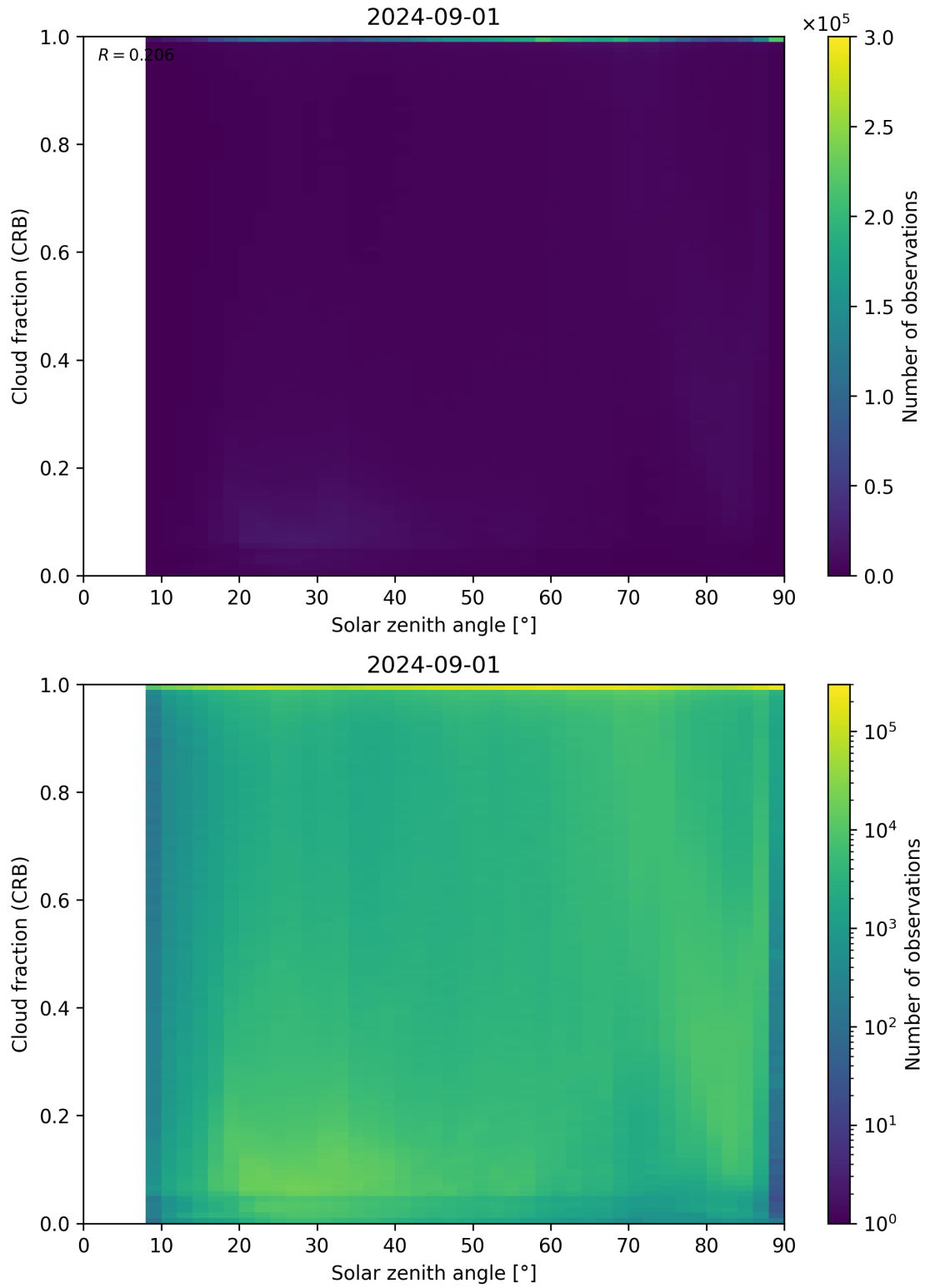
Figure 101: Scatter density plot of “Solar zenith angle” against “Cloud fraction (CRB)” for 2024-09-01 to 2024-09-02.
