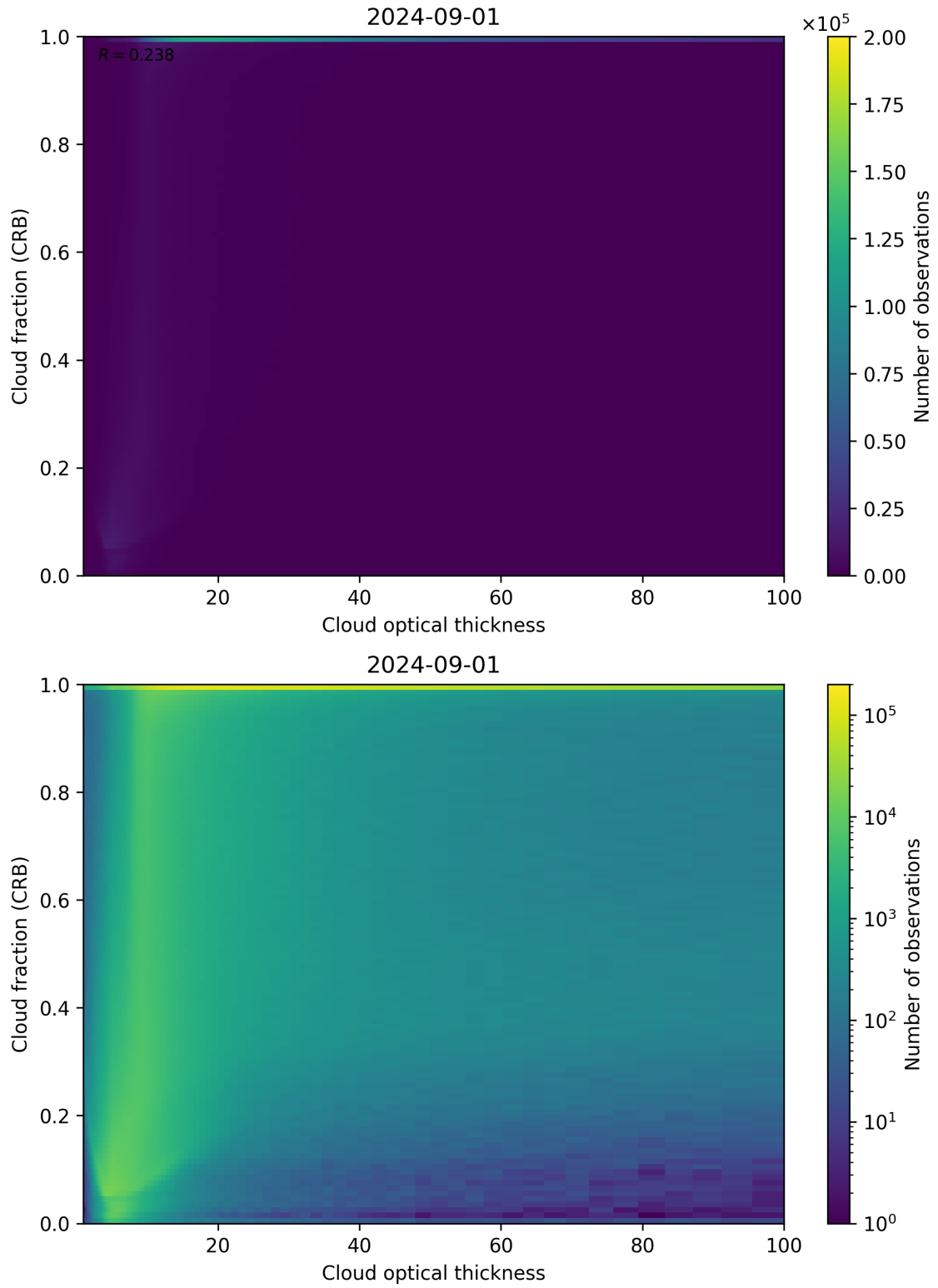
Figure 84: Scatter density plot of “Cloud optical thickness” against “Cloud fraction (CRB)” for 2024-09-01 to 2024-09-02.
