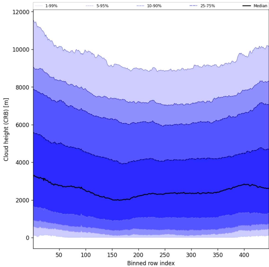
Figure 59: Along track statistics of “Cloud height (CRB)” for 2024-09-01 to 2024-09-02
