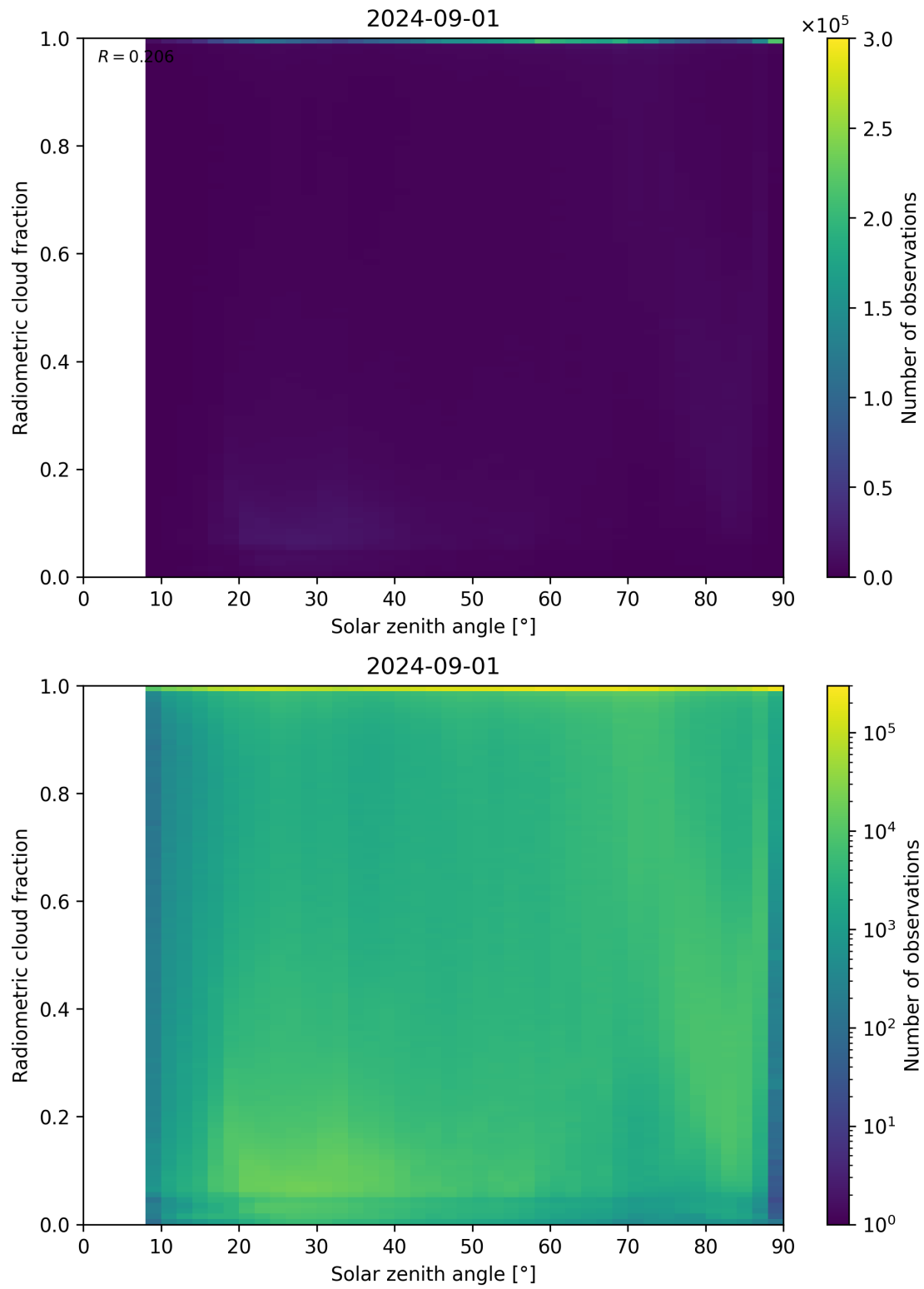
Figure 99: Scatter density plot of “Solar zenith angle” against “Radiometric cloud fraction” for 2024-09-01 to 2024-09-02.
