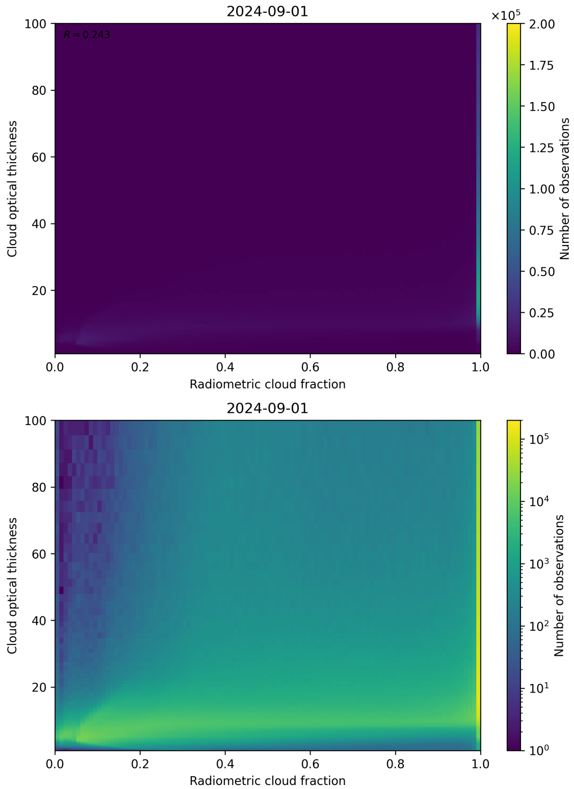
Figure 75: Scatter density plot of “Radiometric cloud fraction” against “Cloud optical thickness” for 2024-09-01 to 2024-09-02.
