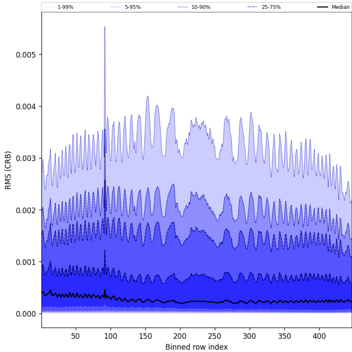
Figure 64: Along track statistics of “RMS (CRB)” for 2024-09-01 to 2024-09-02
