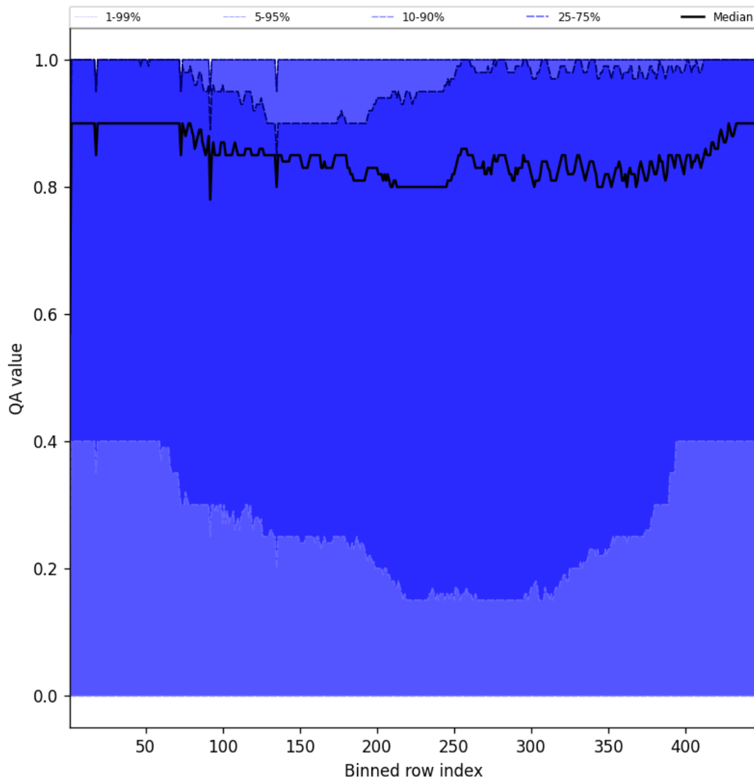
Figure 54: Along track statistics of “QA value” for 2024-09-01 to 2024-09-02
