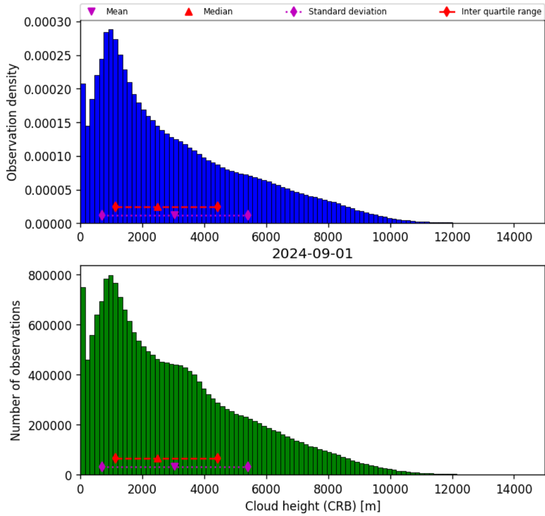
Figure 43: Histogram of “Cloud height (CRB)” for 2024-09-01 to 2024-09-02
