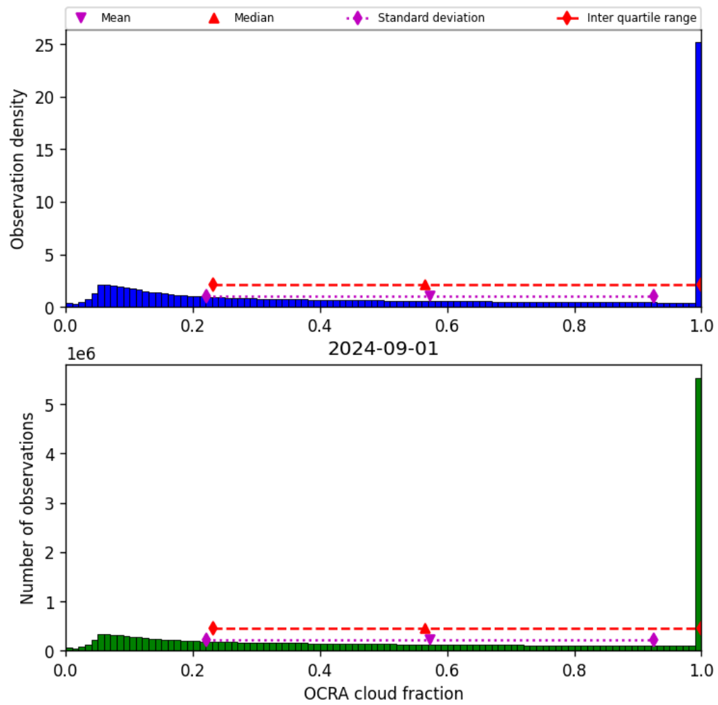
Figure 50: Histogram of “OCRA cloud fraction” for 2024-09-01 to 2024-09-02
