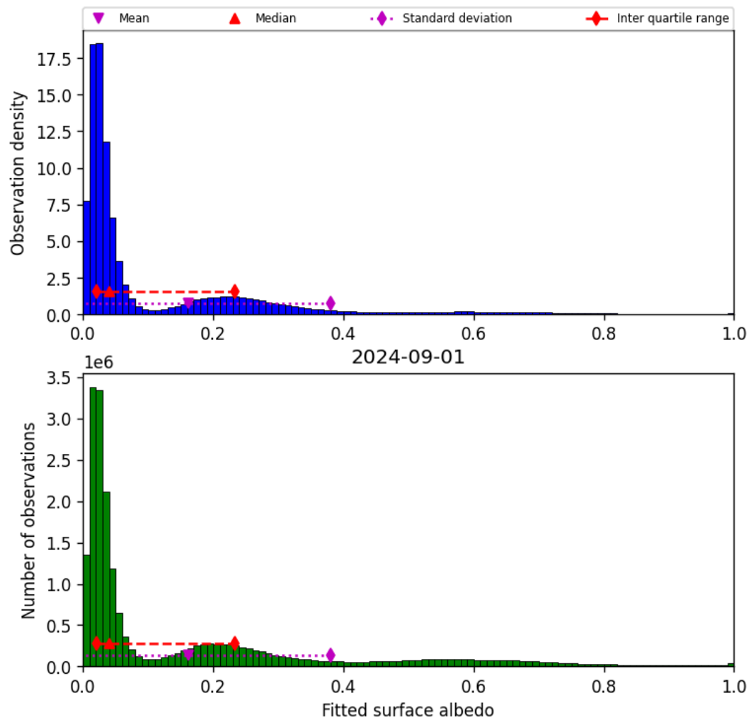
Figure 45: Histogram of “Fitted surface albedo” for 2024-09-01 to 2024-09-02
