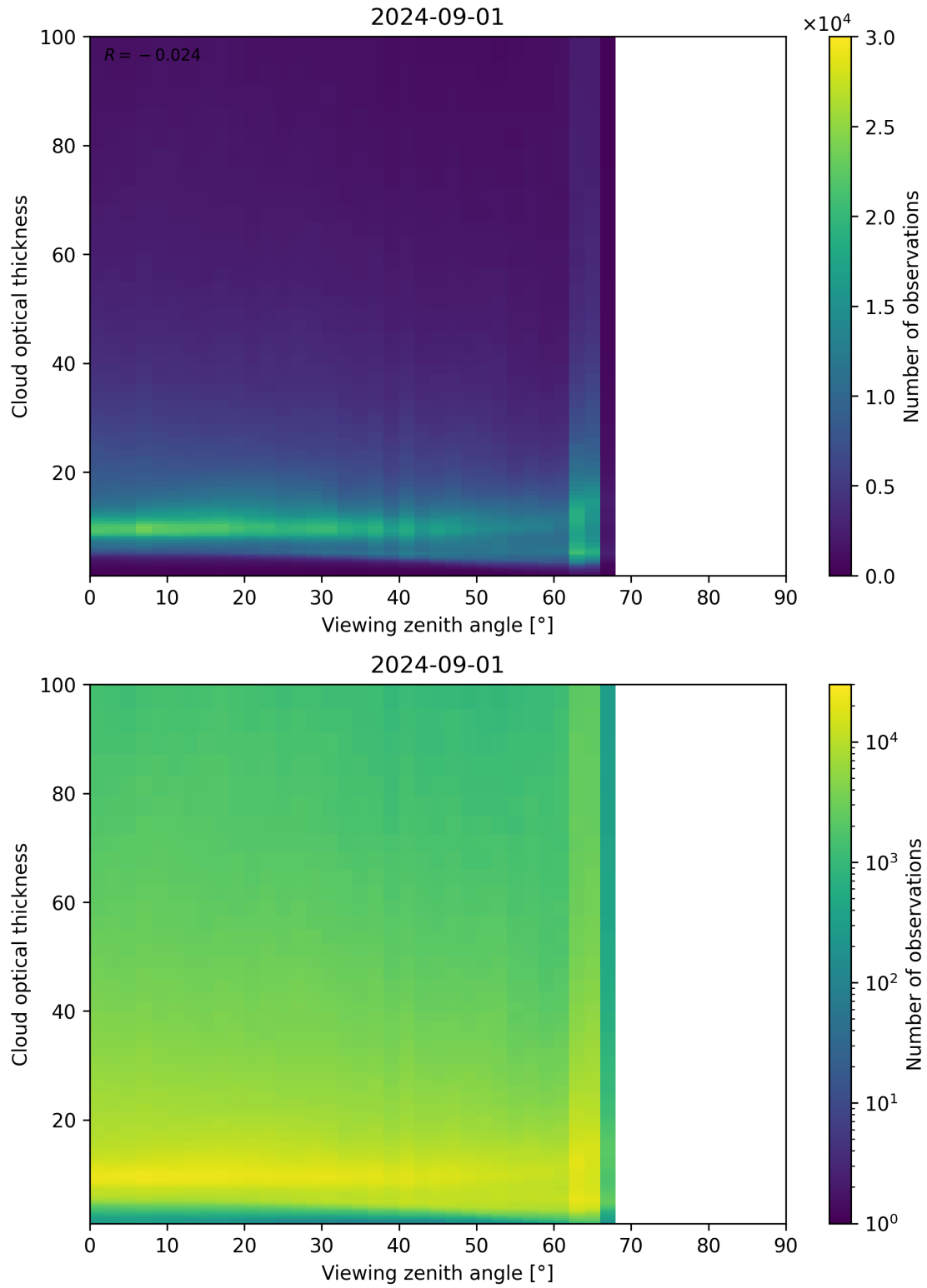
Figure 111: Scatter density plot of “Viewing zenith angle” against “Cloud optical thickness” for 2024-09-01 to 2024-09-02.
