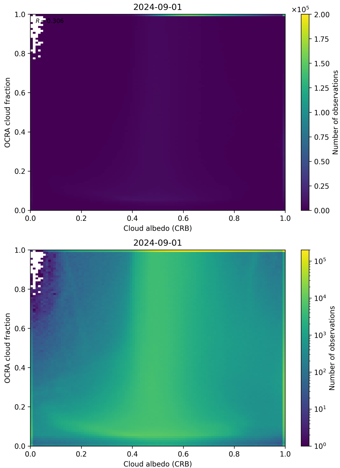
Figure 70: Scatter density plot of “Cloud albedo (CRB)” against “OCRA cloud fraction” for 2024-09-01 to 2024-09-02.
