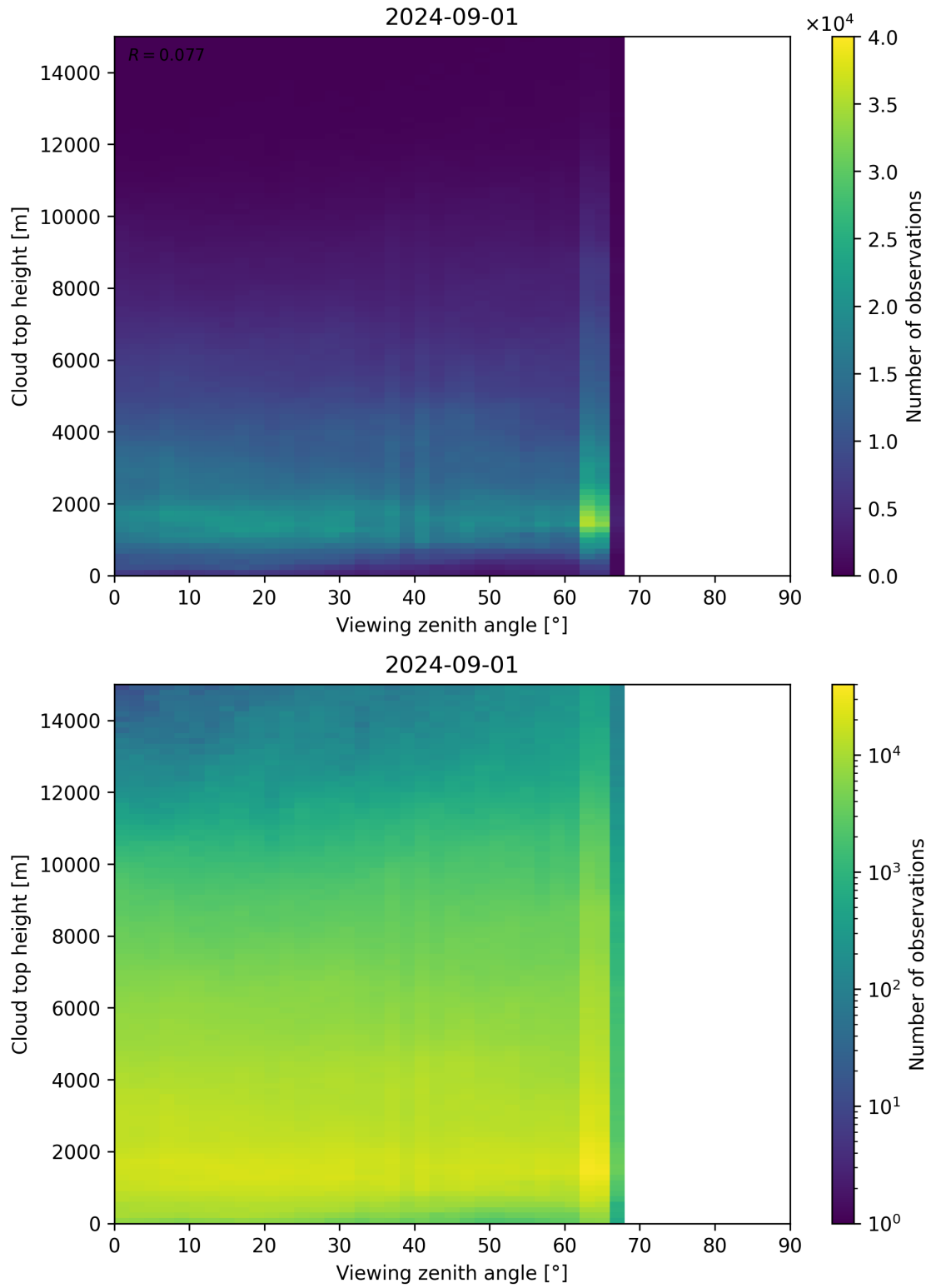
Figure 112: Scatter density plot of “Viewing zenith angle” against “Cloud top height” for 2024-09-01 to 2024-09-02.
