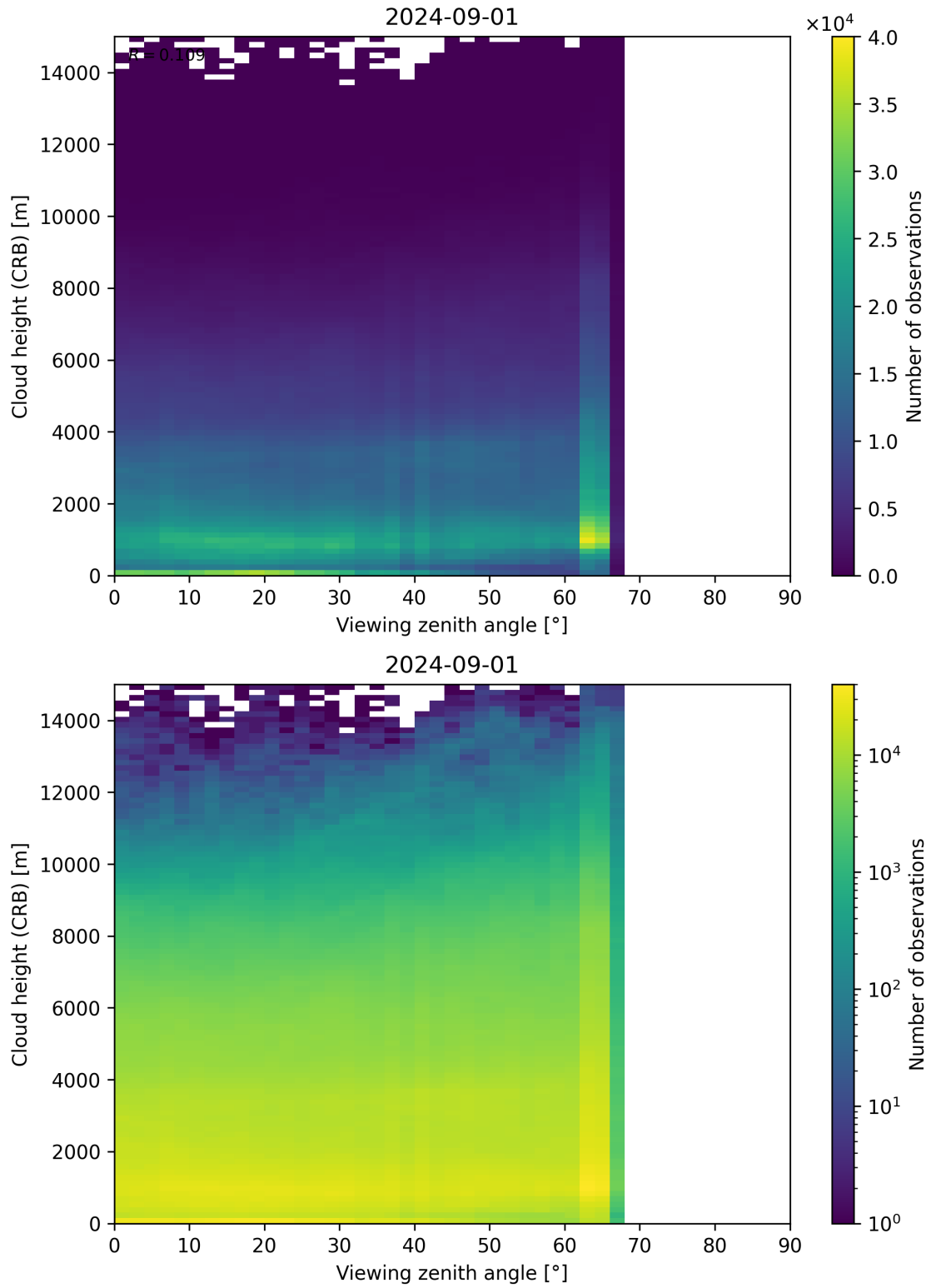
Figure 110: Scatter density plot of “Viewing zenith angle” against “Cloud height (CRB)” for 2024-09-01 to 2024-09-02.
