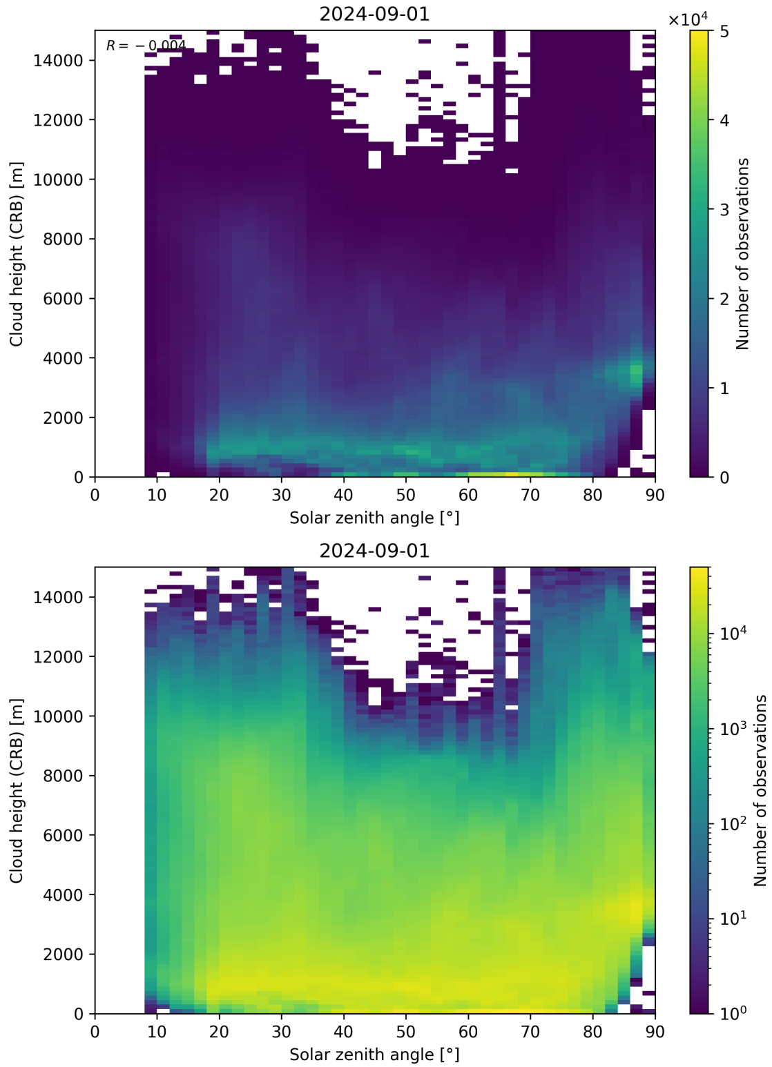
Figure 102: Scatter density plot of “Solar zenith angle” against “Cloud height (CRB)” for 2024-09-01 to 2024-09-02.
