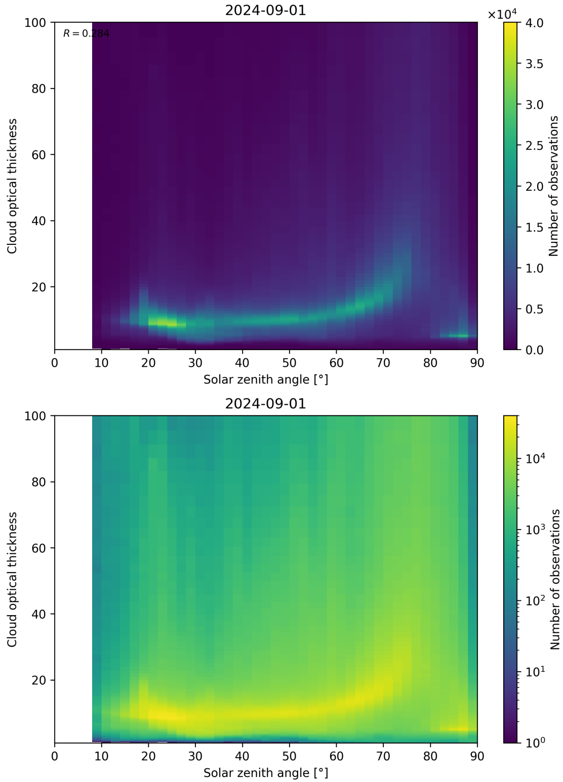
Figure 103: Scatter density plot of “Solar zenith angle” against “Cloud optical thickness” for 2024-09-01 to 2024-09-02.
