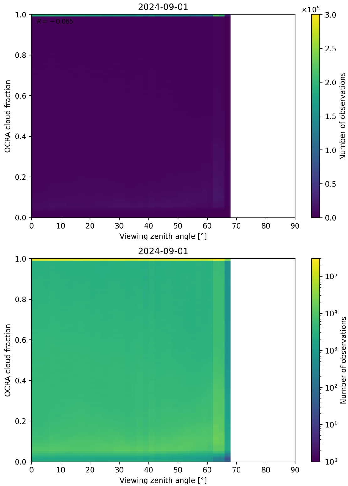
Figure 108: Scatter density plot of “Viewing zenith angle” against “OCRA cloud fraction” for 2024-09-01 to 2024-09-02.
