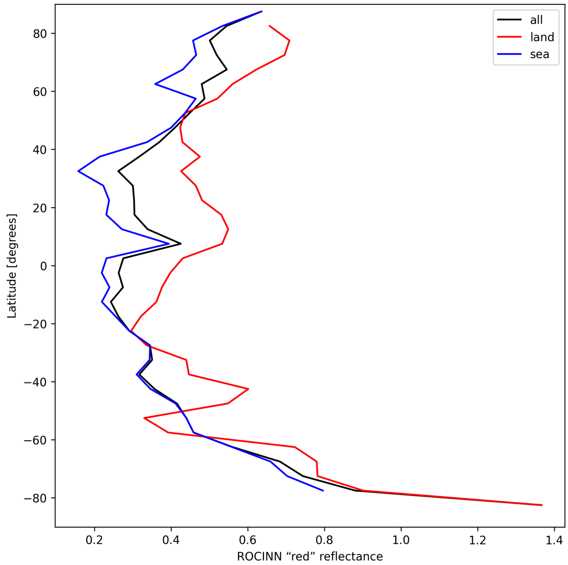
Figure 37: Zonal average of “ROCINN “red” reflectance” for 2024-09-01 to 2024-09-02.
