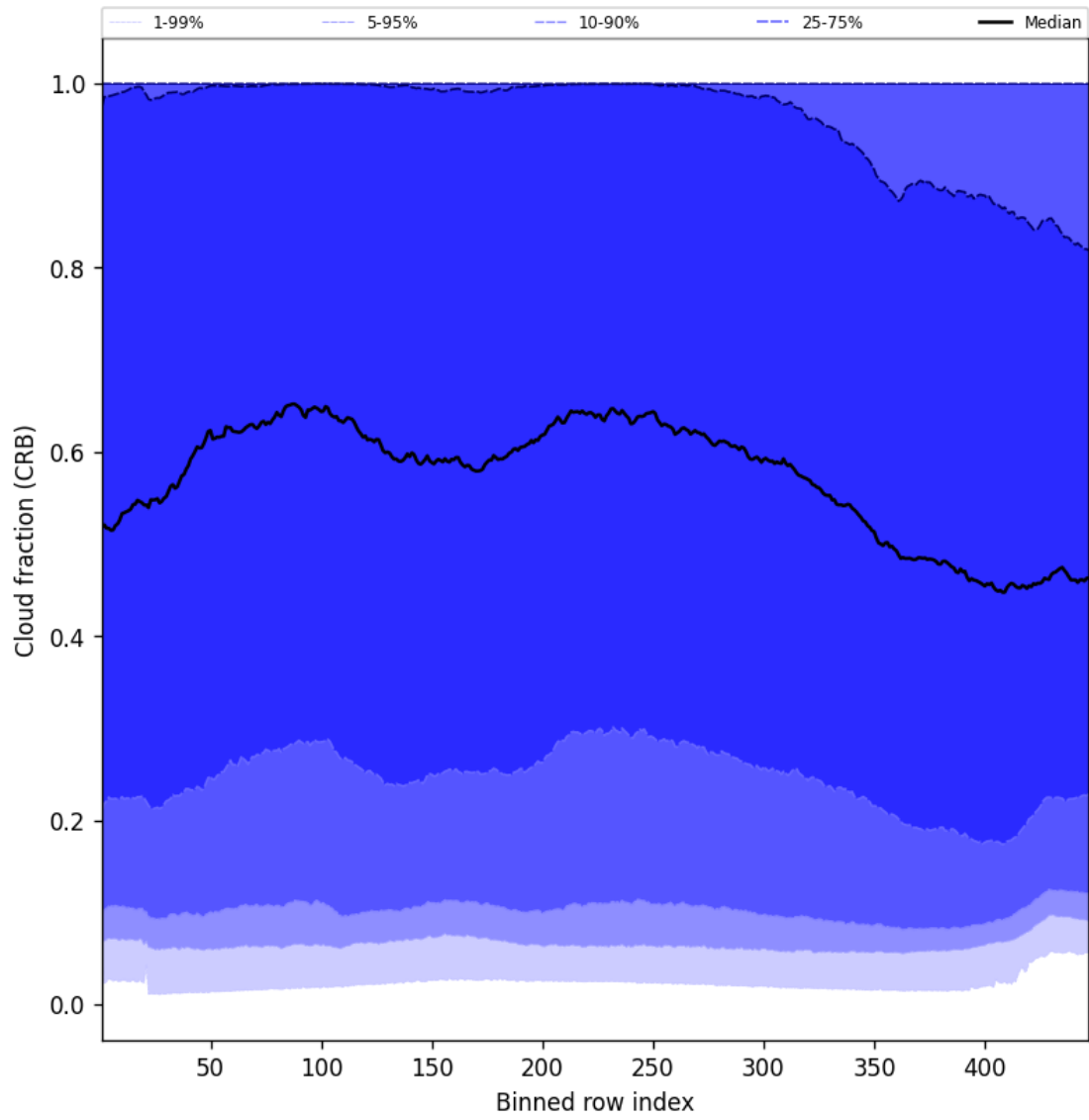
Figure 58: Along track statistics of “Cloud fraction (CRB)” for 2024-09-01 to 2024-09-02
