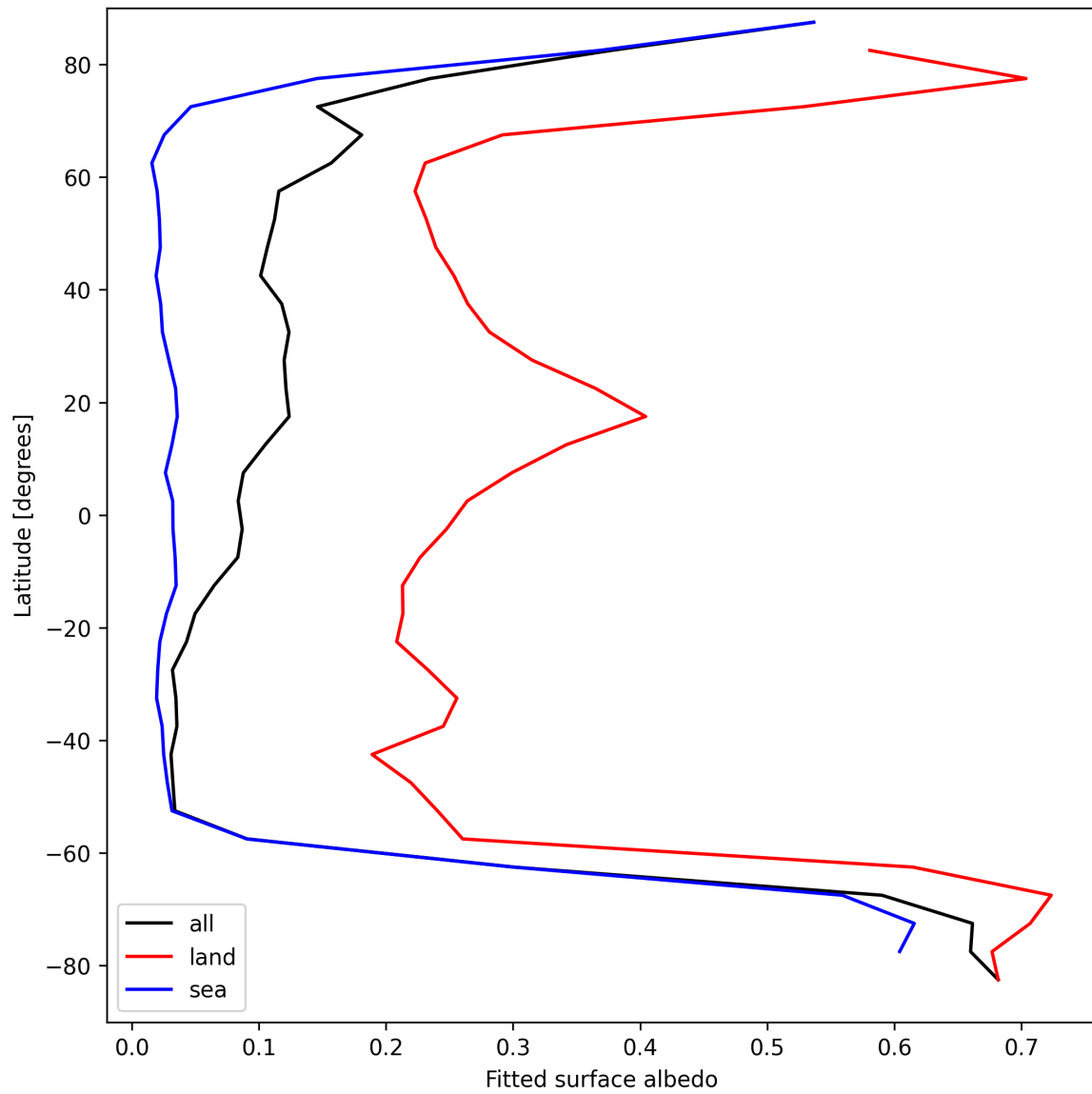
Figure 29: Zonal average of “Fitted surface albedo” for 2024-09-01 to 2024-09-02.
