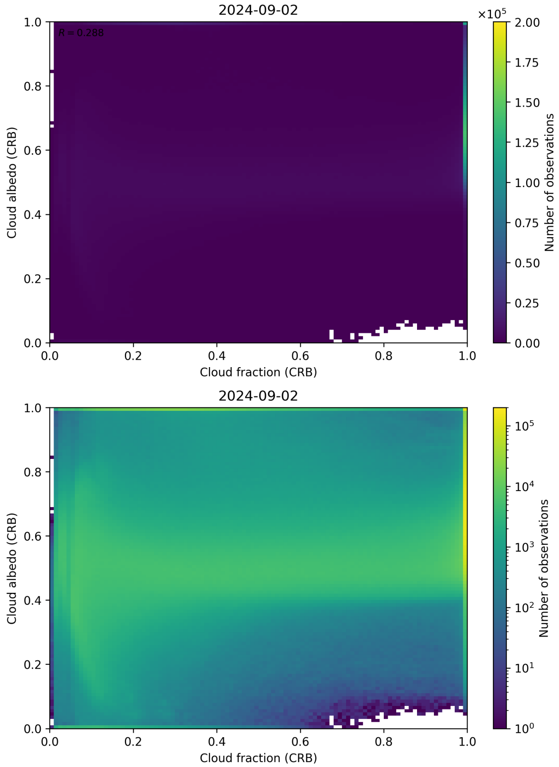
Figure 77: Scatter density plot of “Cloud fraction (CRB)” against “Cloud albedo (CRB)” for 2024-09-01 to 2024-09-03.
