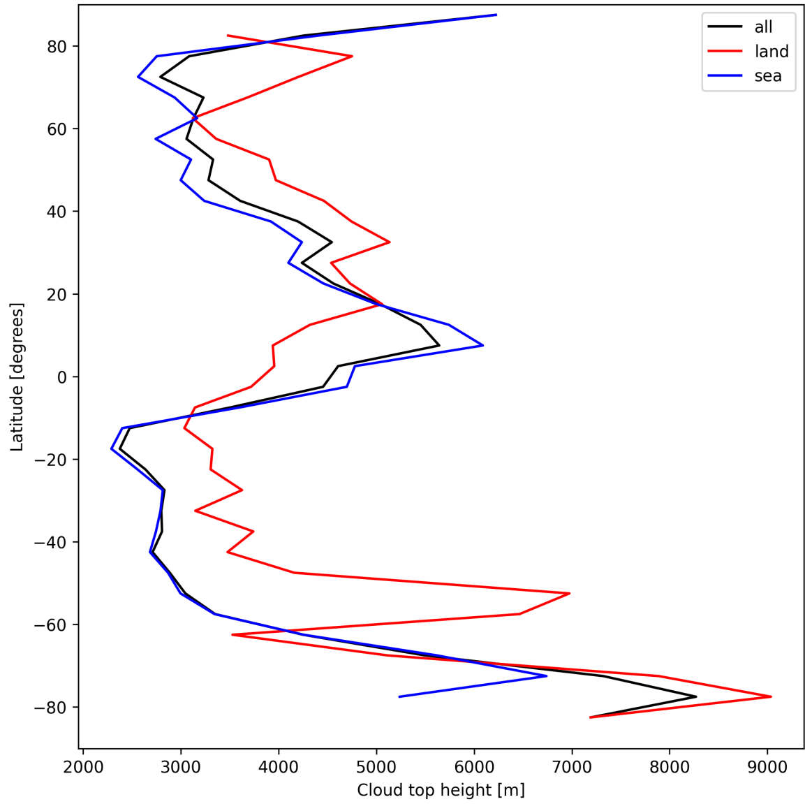
Figure 24: Zonal average of “Cloud top height” for 2024-09-01 to 2024-09-03.
