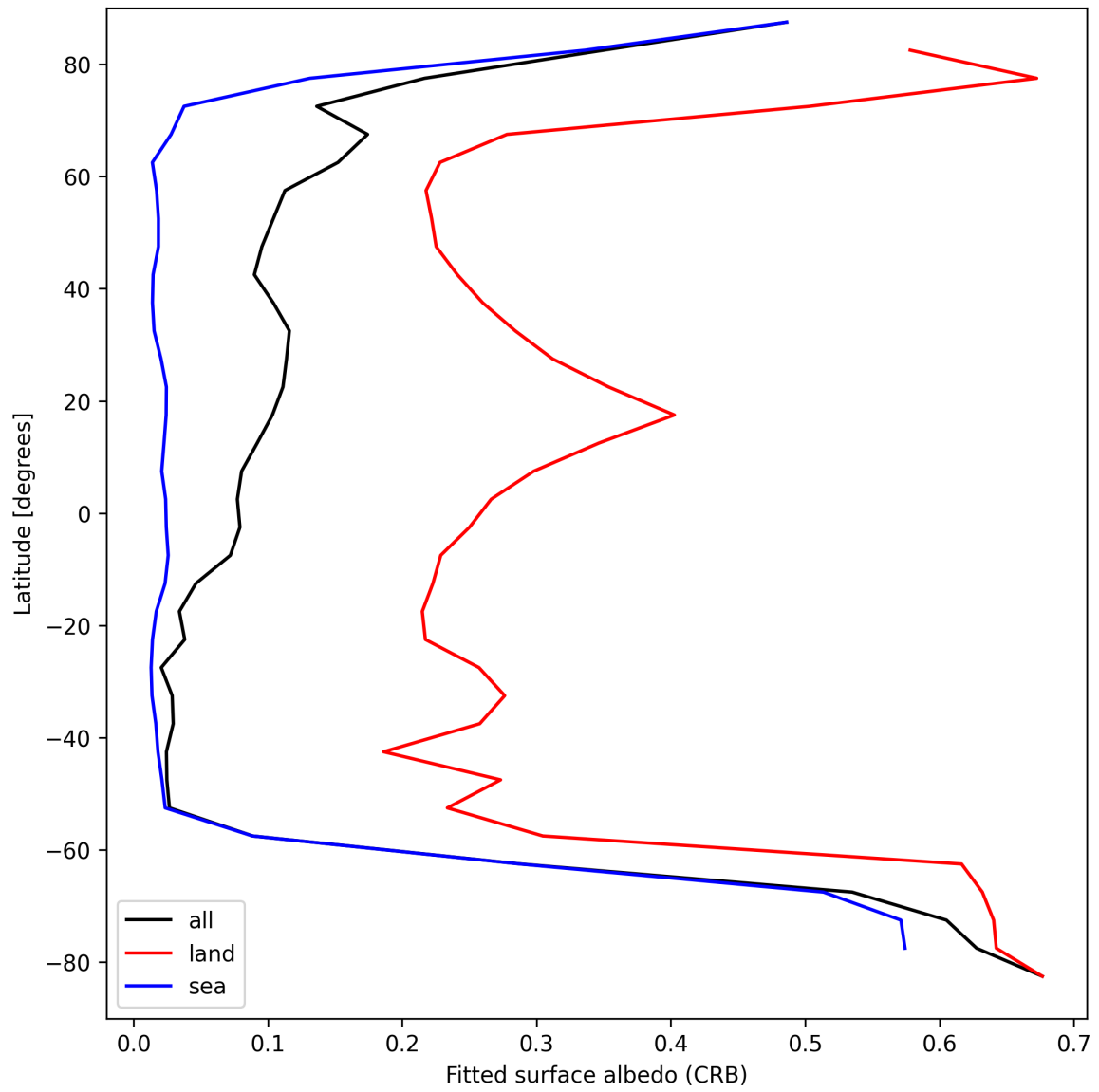
Figure 30: Zonal average of “Fitted surface albedo (CRB)” for 2024-09-01 to 2024-09-03.
