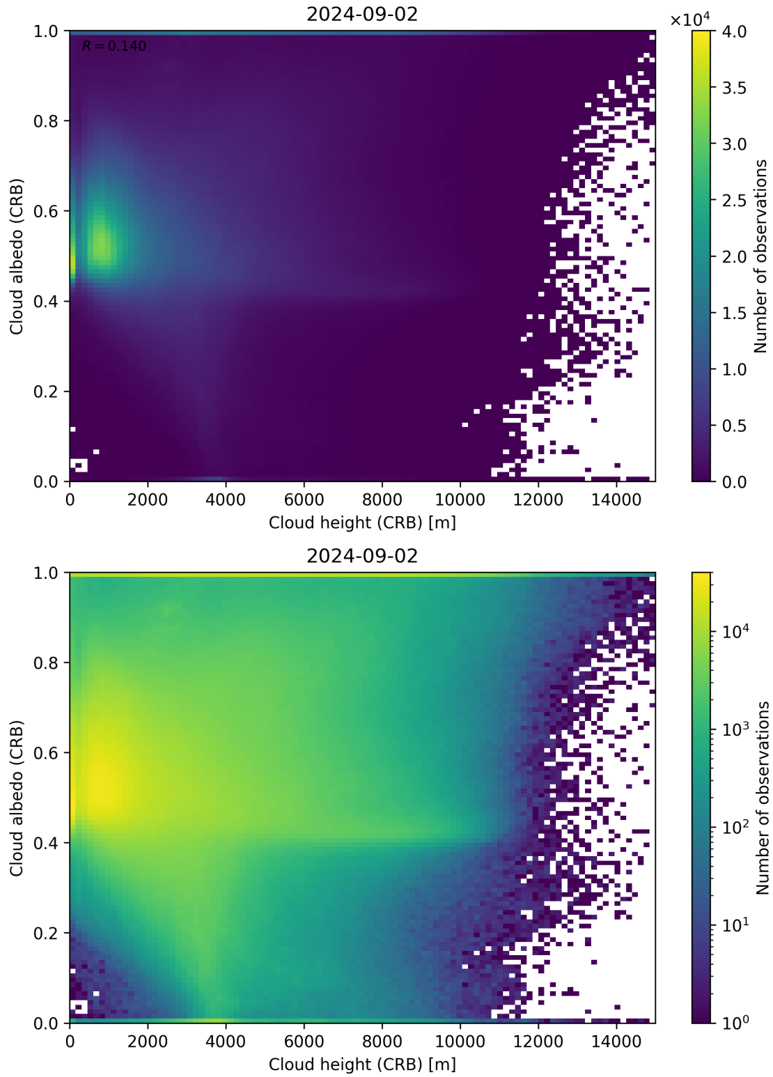
Figure 80: Scatter density plot of “Cloud height (CRB)” against “Cloud albedo (CRB)” for 2024-09-01 to 2024-09-03.
