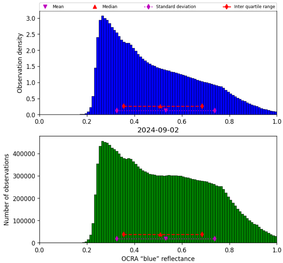
Figure 51: Histogram of “OCRA “blue” reflectance” for 2024-09-01 to 2024-09-03
