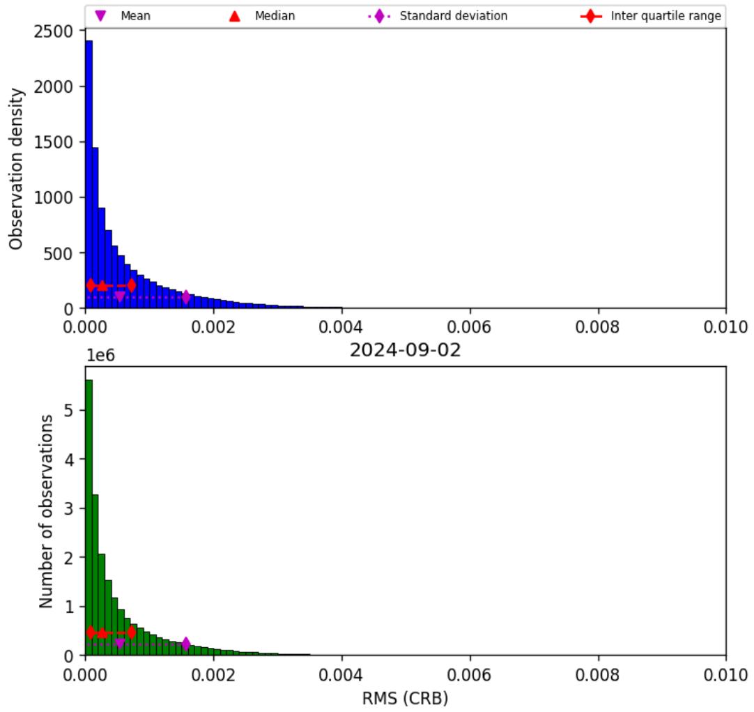
Figure 48: Histogram of “RMS (CRB)” for 2024-09-01 to 2024-09-03
