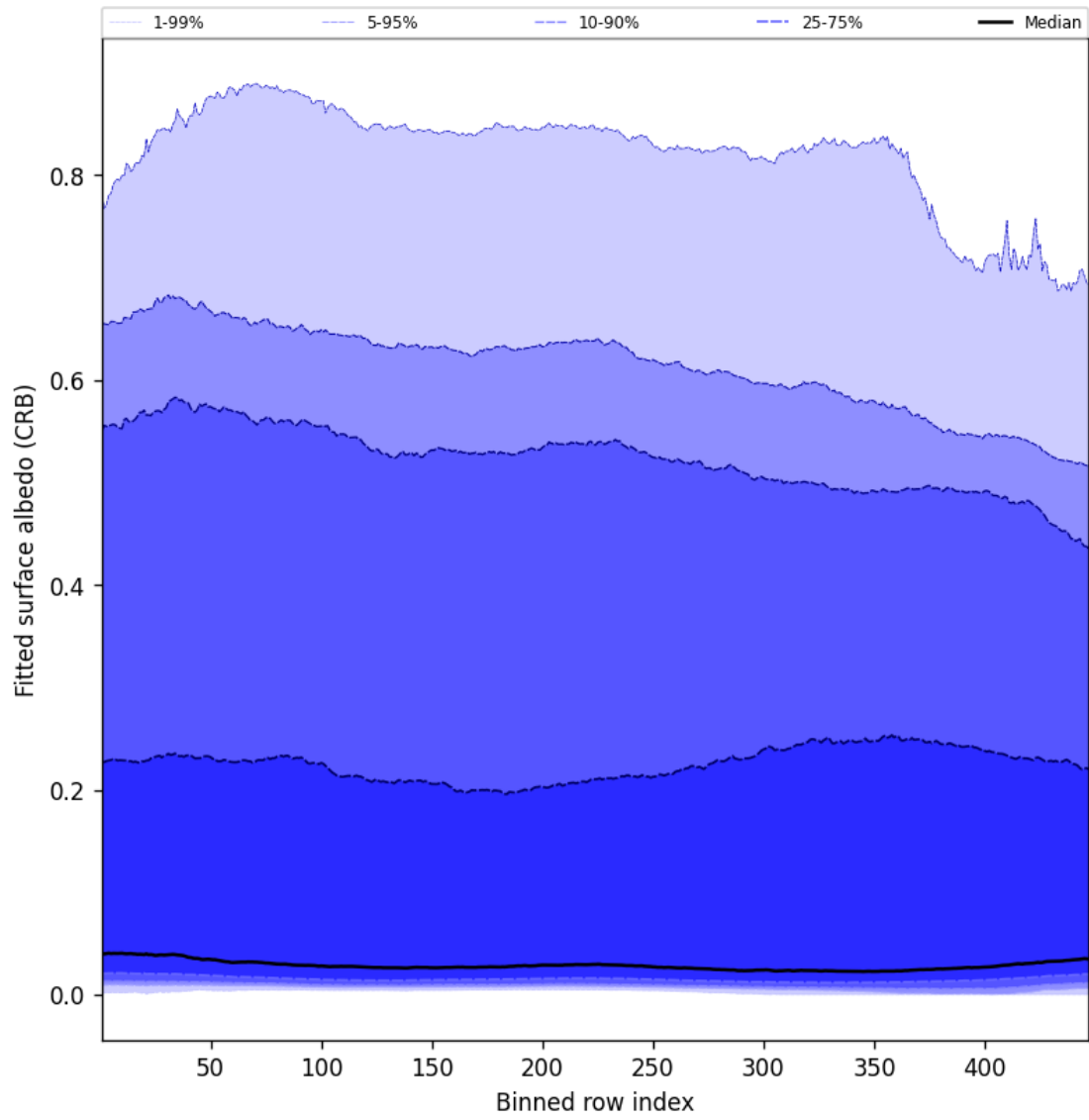
Figure 62: Along track statistics of “Fitted surface albedo (CRB)” for 2024-09-01 to 2024-09-03
