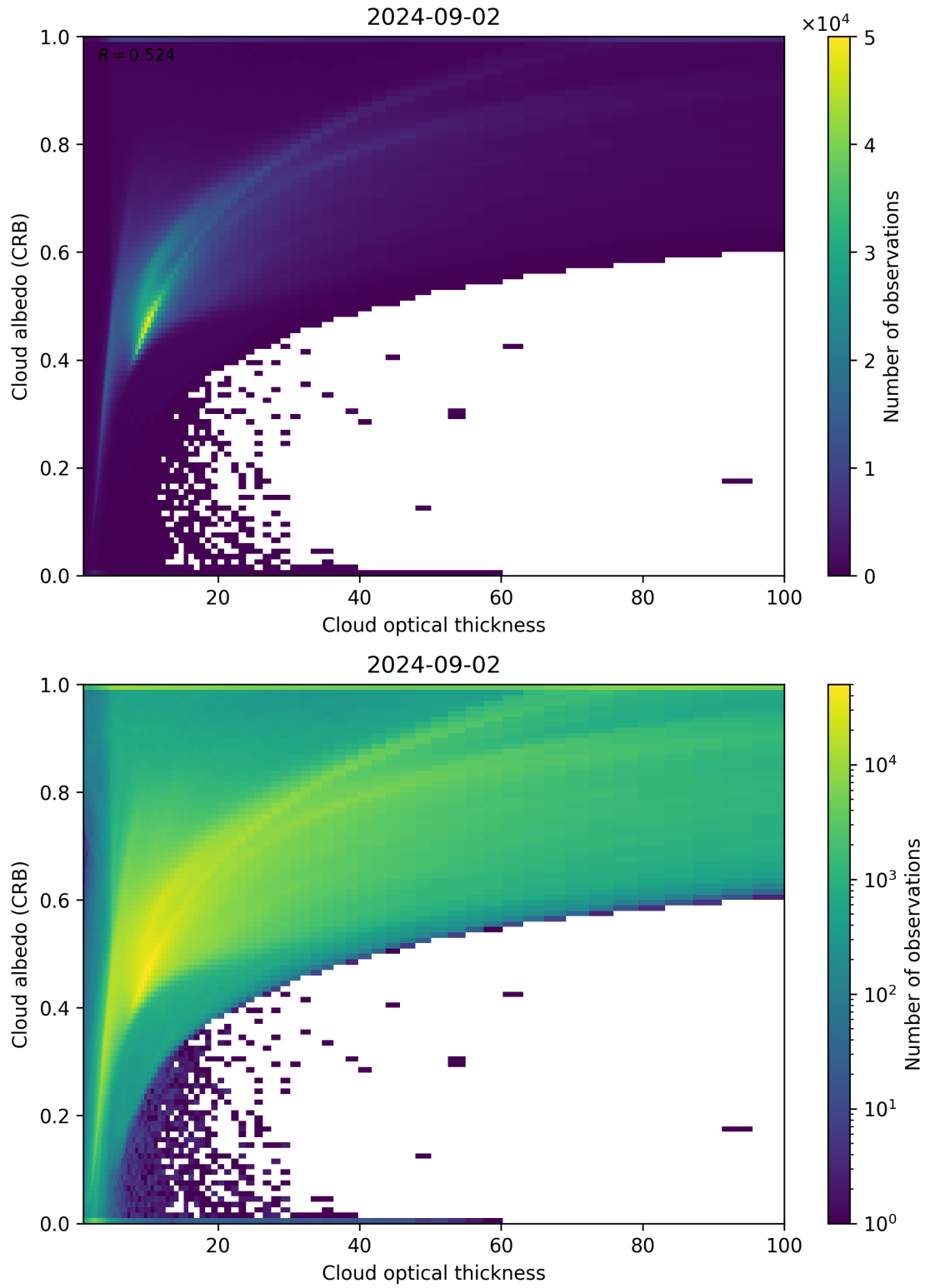
Figure 82: Scatter density plot of “Cloud optical thickness” against “Cloud albedo (CRB)” for 2024-09-01 to 2024-09-03.
