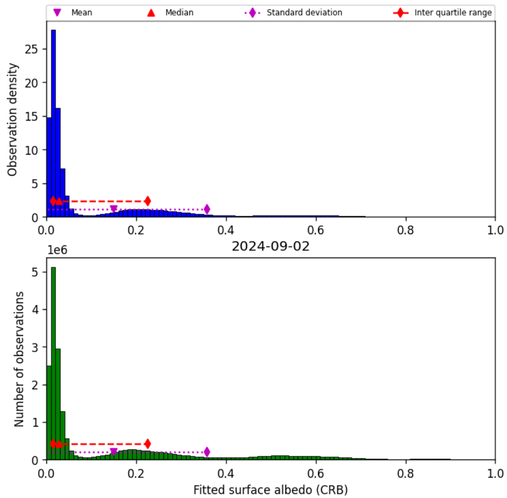
Figure 46: Histogram of “Fitted surface albedo (CRB)” for 2024-09-01 to 2024-09-03
