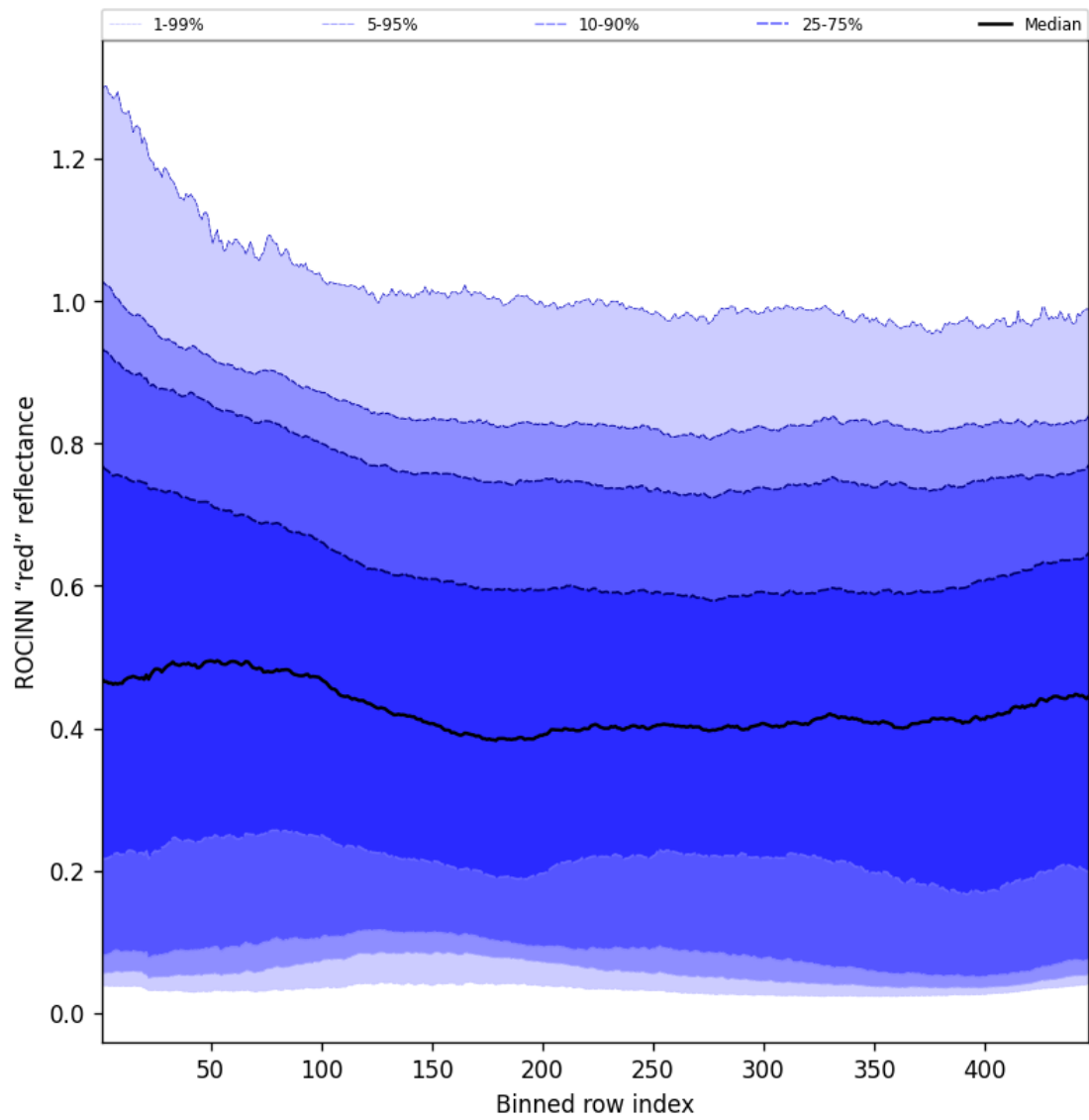
Figure 69: Along track statistics of “ROCINN “red” reflectance” for 2024-09-01 to 2024-09-03
