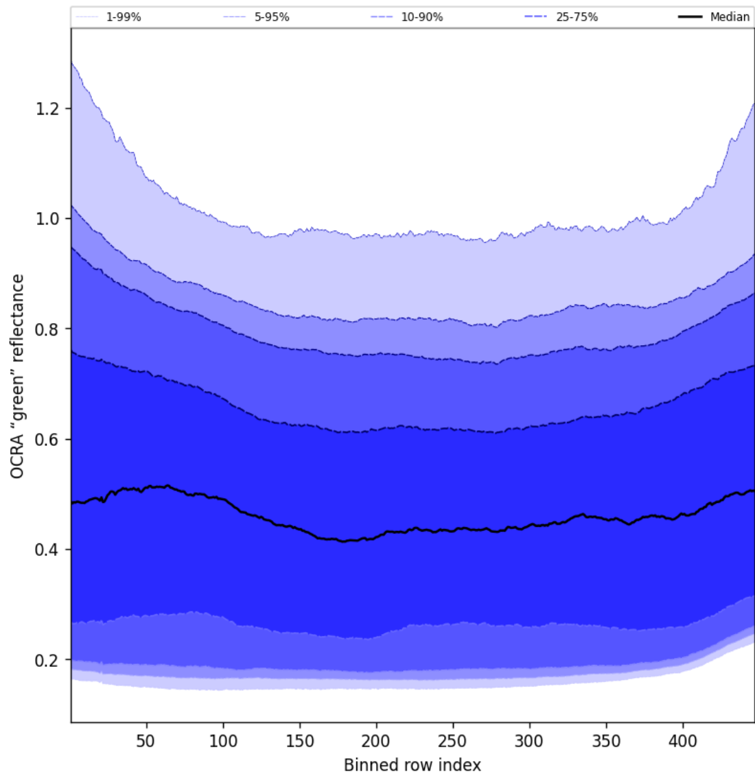
Figure 68: Along track statistics of "OCRA "green" reflectance" for 2024-09-01 to 2024-09-03
