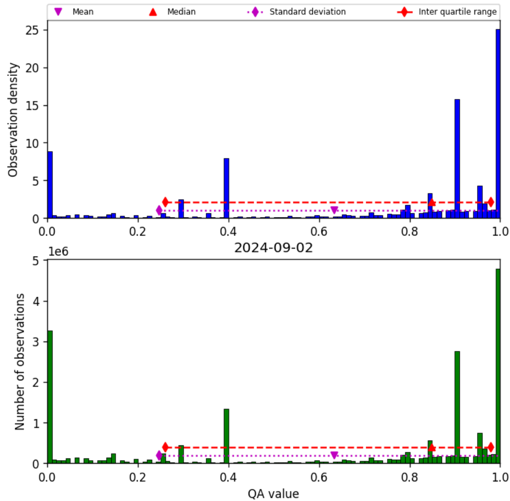
Figure 38: Histogram of “QA value” for 2024-09-01 to 2024-09-03
