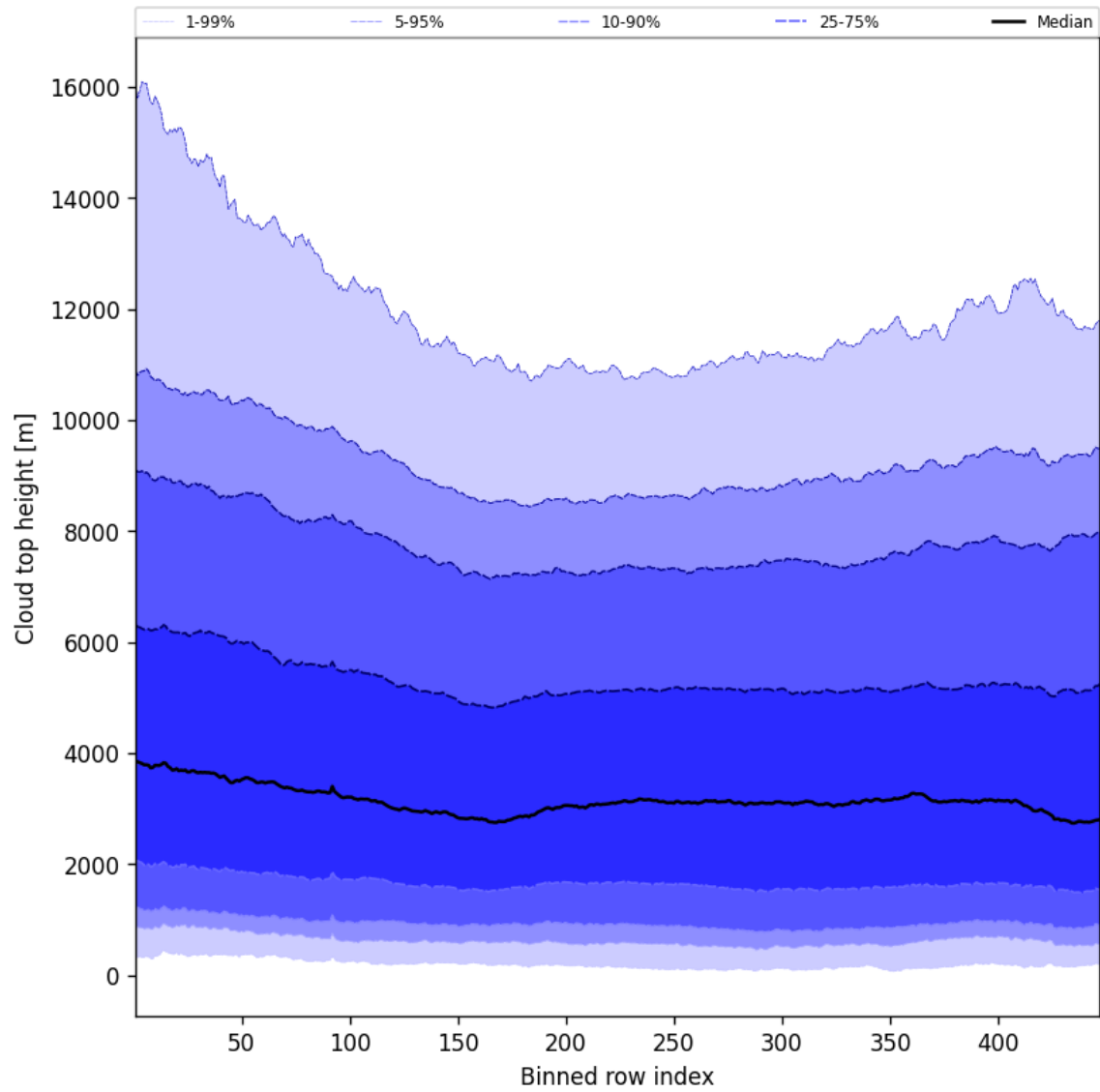
Figure 56: Along track statistics of “Cloud top height” for 2024-09-01 to 2024-09-03
