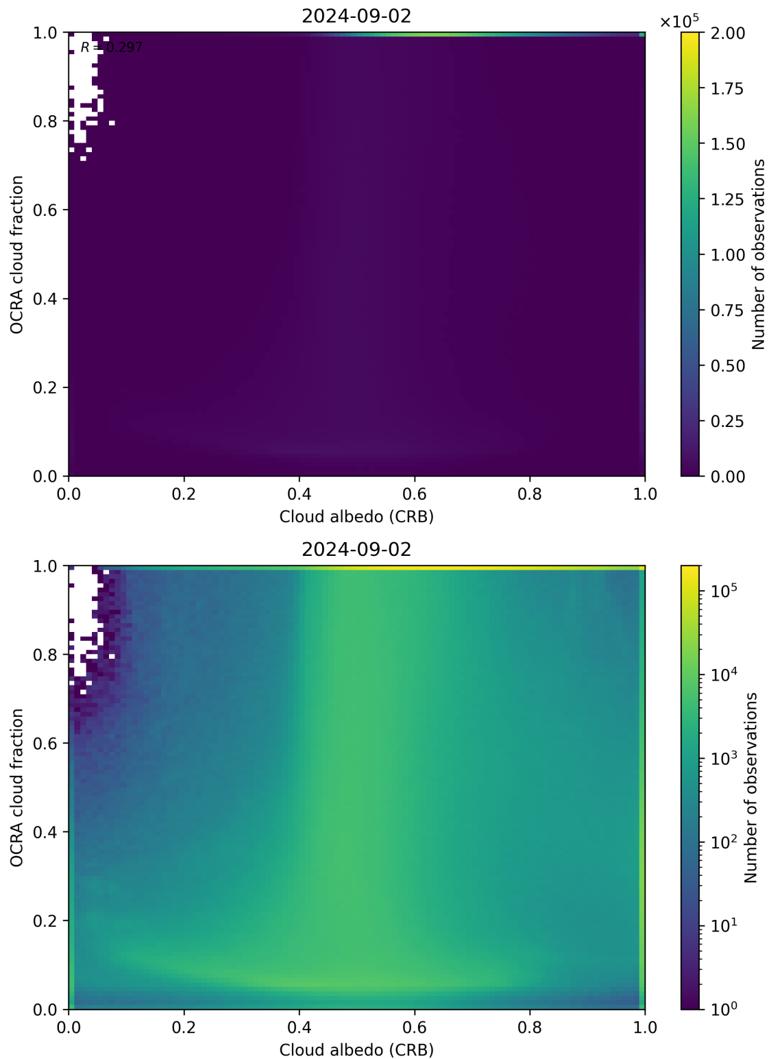
Figure 70: Scatter density plot of “Cloud albedo (CRB)” against “OCRA cloud fraction” for 2024-09-01 to 2024-09-03.
