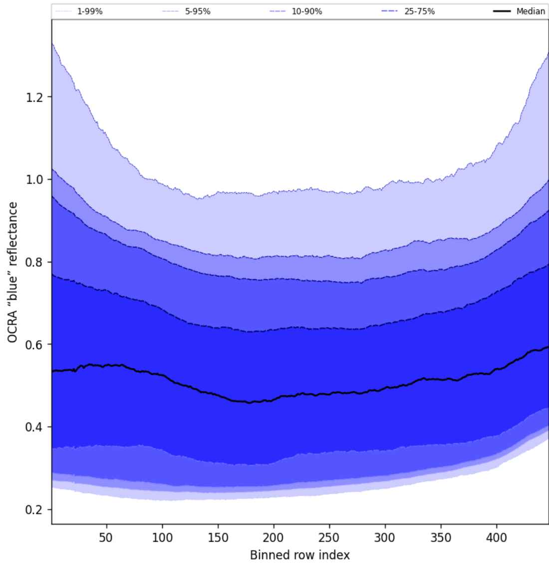
Figure 67: Along track statistics of “OCRA “blue” reflectance” for 2024-09-01 to 2024-09-03
