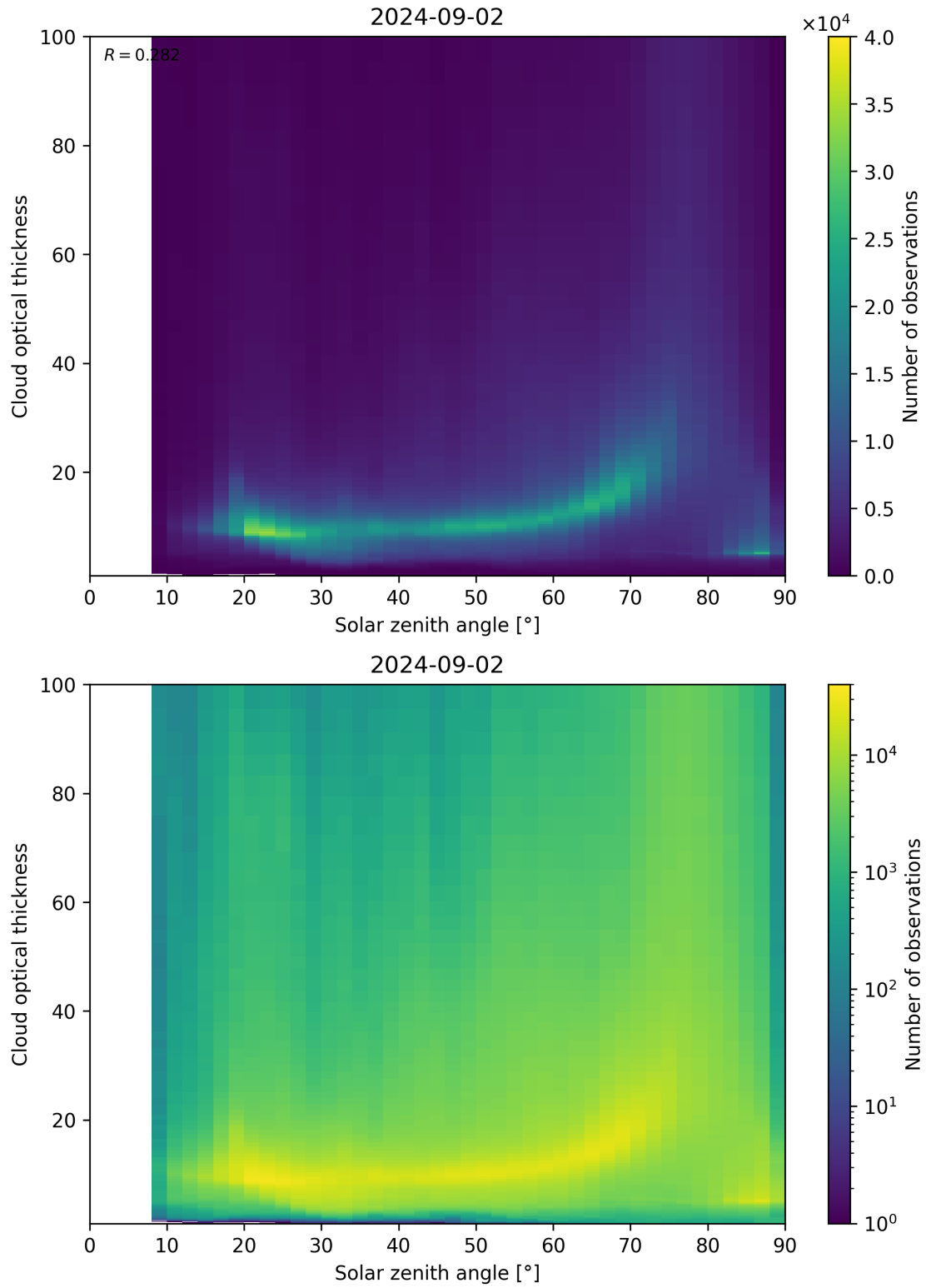
Figure 103: Scatter density plot of “Solar zenith angle” against “Cloud optical thickness” for 2024-09-01 to 2024-09-03.
