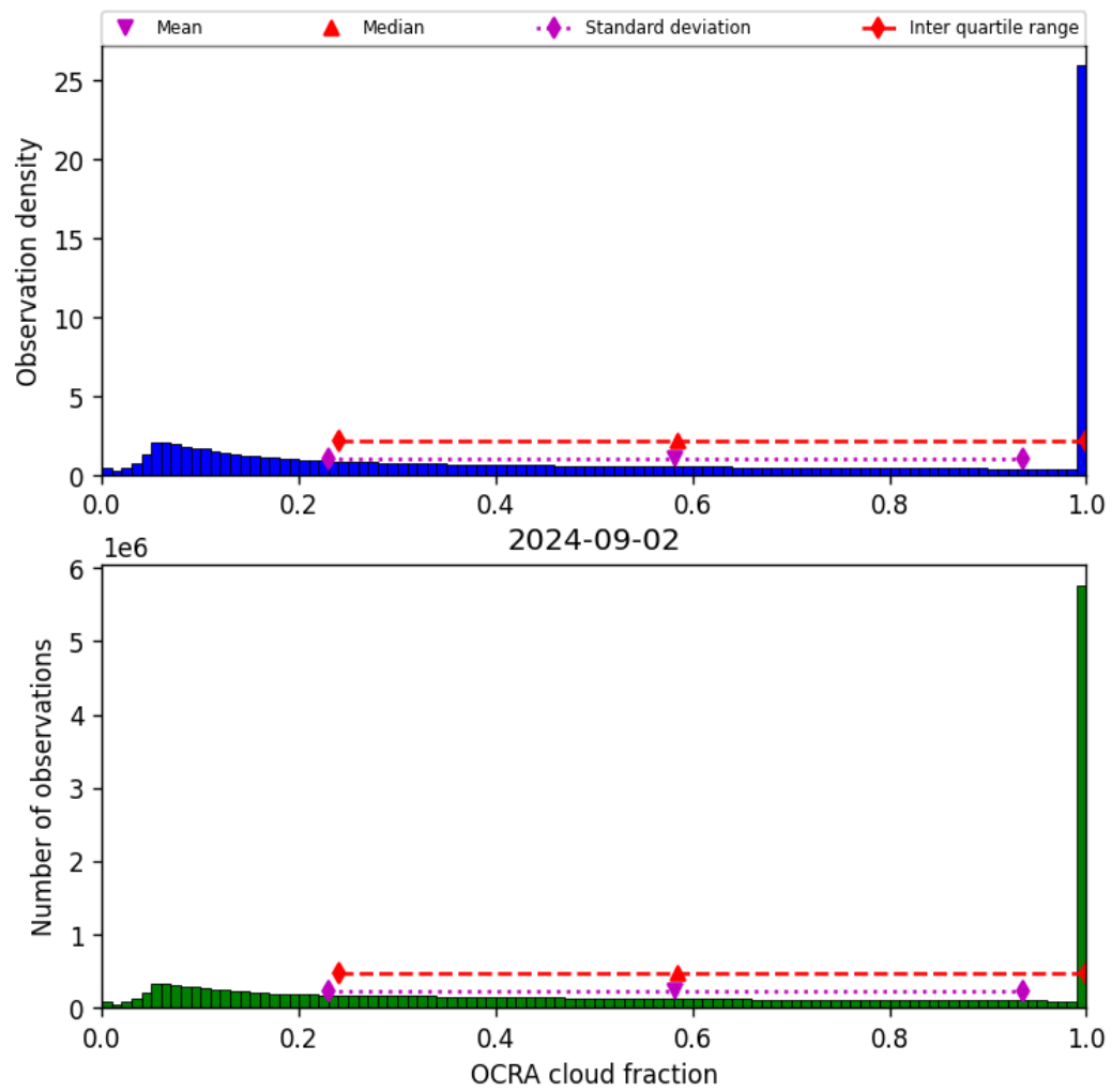
Figure 50: Histogram of “OCRA cloud fraction” for 2024-09-01 to 2024-09-03
