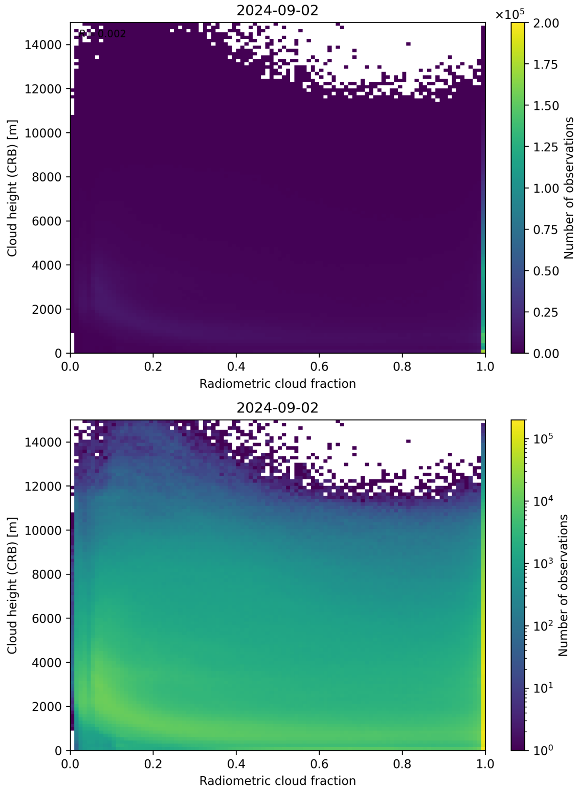
Figure 74: Scatter density plot of “Radiometric cloud fraction” against “Cloud height (CRB)” for 2024-09-01 to 2024-09-03.
