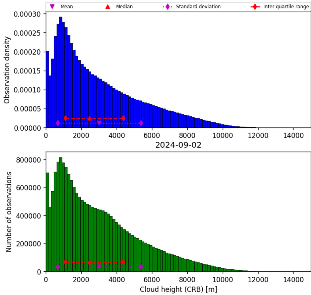
Figure 43: Histogram of “Cloud height (CRB)” for 2024-09-01 to 2024-09-03
