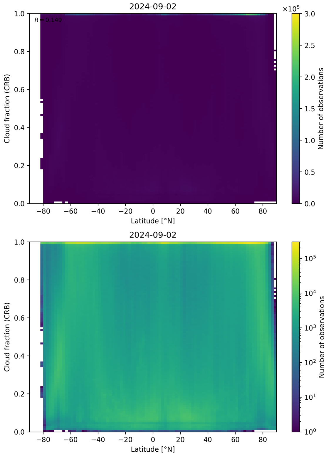
Figure 94: Scatter density plot of “Latitude” against “Cloud fraction (CRB)” for 2024-09-01 to 2024-09-03.
