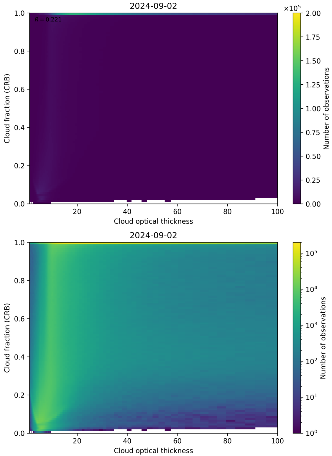
Figure 84: Scatter density plot of “Cloud optical thickness” against “Cloud fraction (CRB)” for 2024-09-01 to 2024-09-03.
