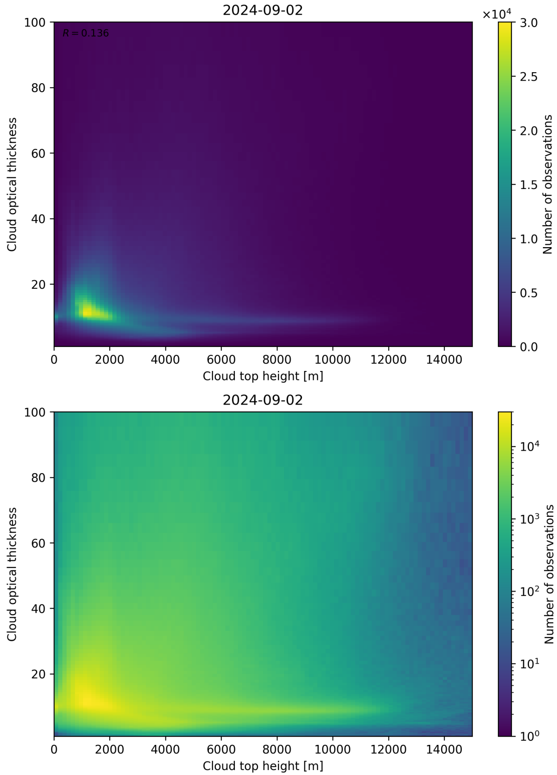
Figure 90: Scatter density plot of “Cloud top height” against “Cloud optical thickness” for 2024-09-01 to 2024-09-03.
