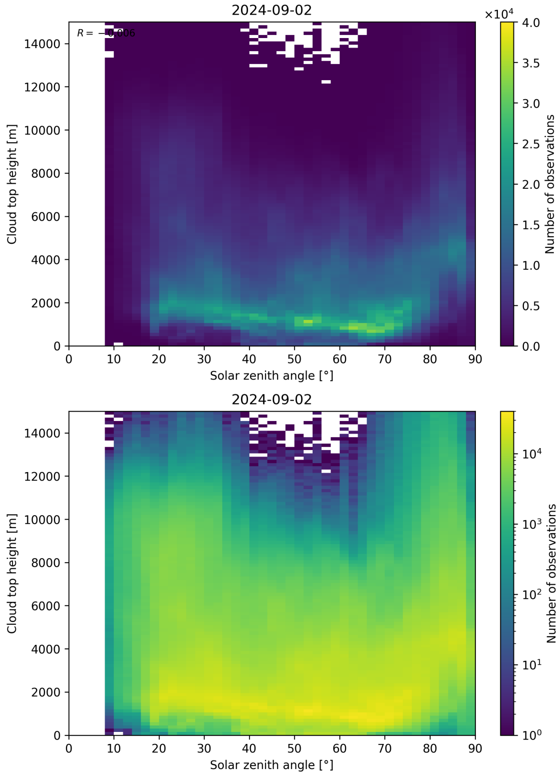
Figure 104: Scatter density plot of “Solar zenith angle” against “Cloud top height” for 2024-09-01 to 2024-09-03.
