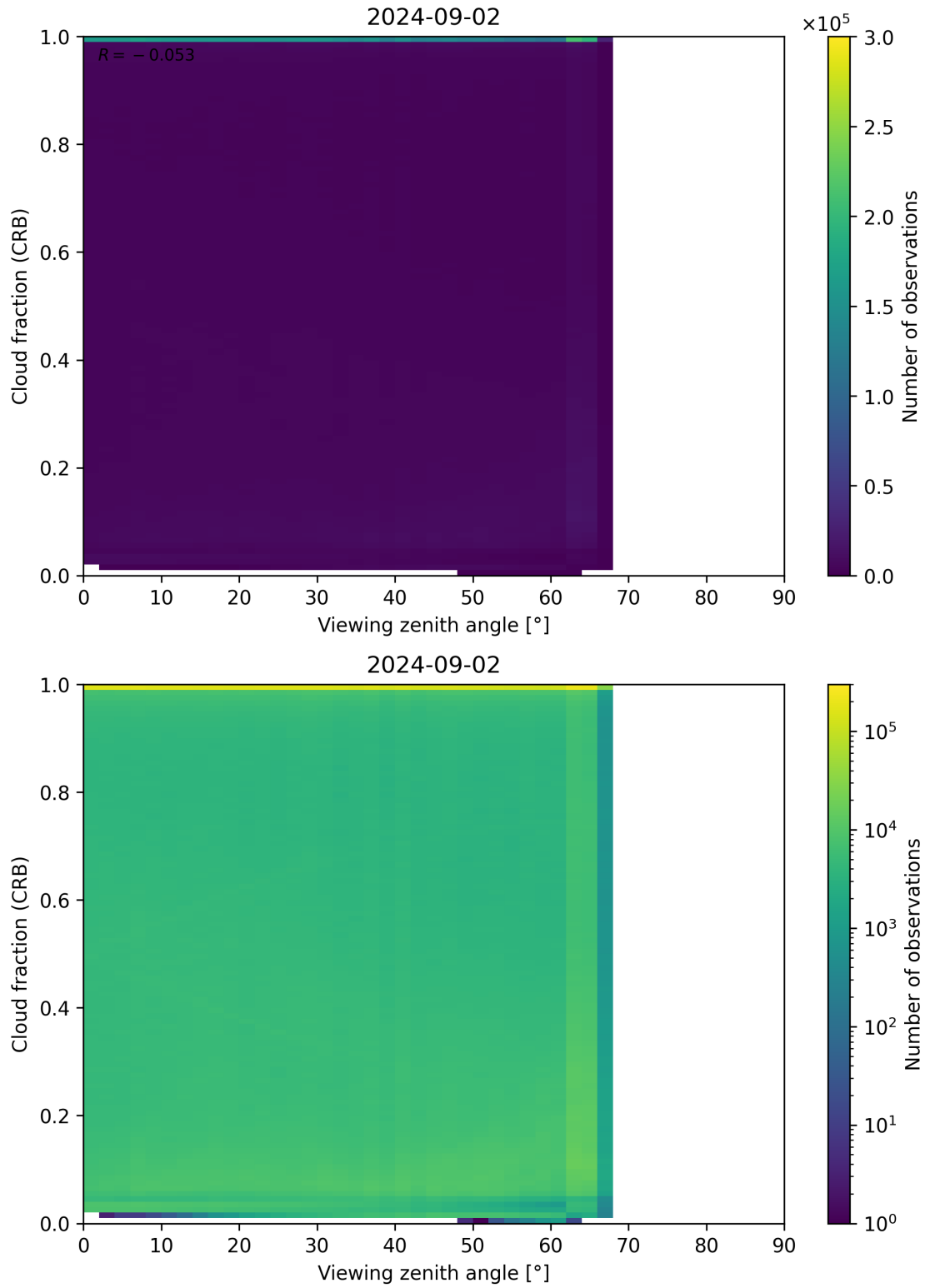
Figure 109: Scatter density plot of “Viewing zenith angle” against “Cloud fraction (CRB)” for 2024-09-01 to 2024-09-03.
