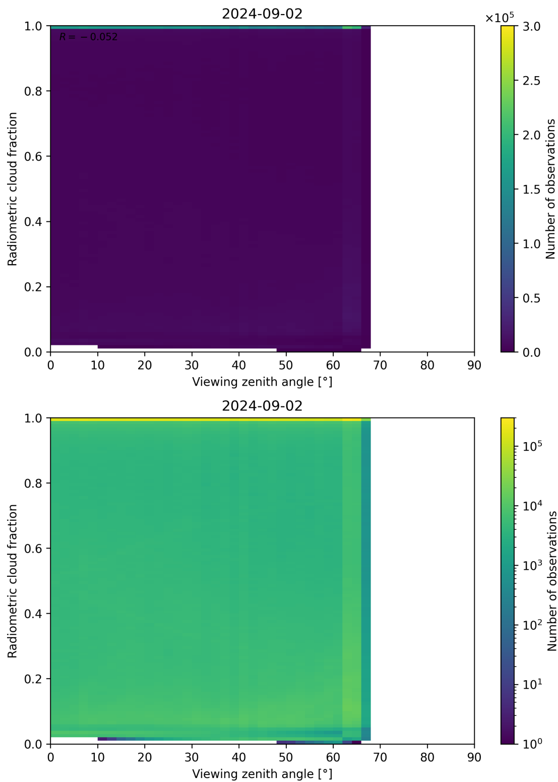
Figure 107: Scatter density plot of “Viewing zenith angle” against “Radiometric cloud fraction” for 2024-09-01 to 2024-09-03.
