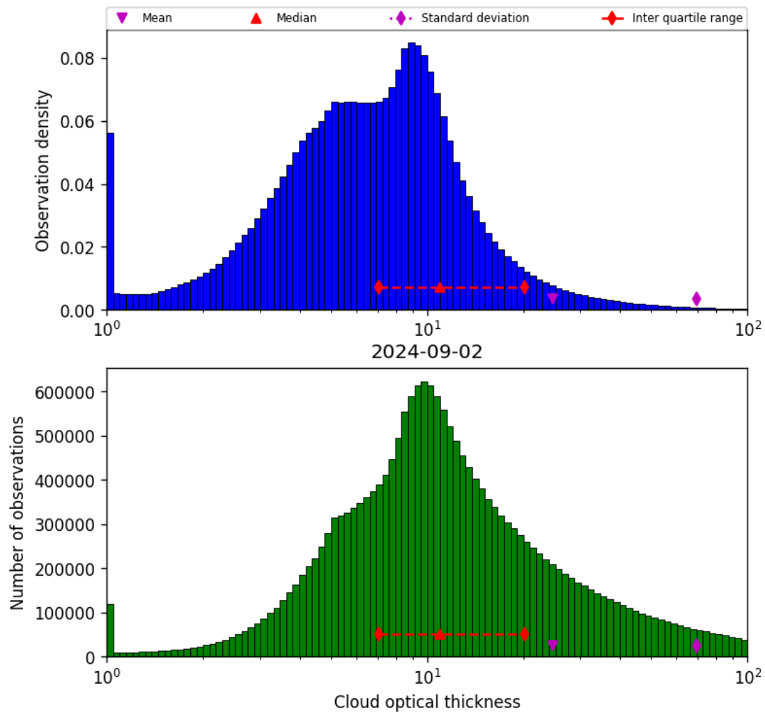
Figure 41: Histogram of “Cloud optical thickness” for 2024-09-01 to 2024-09-03
