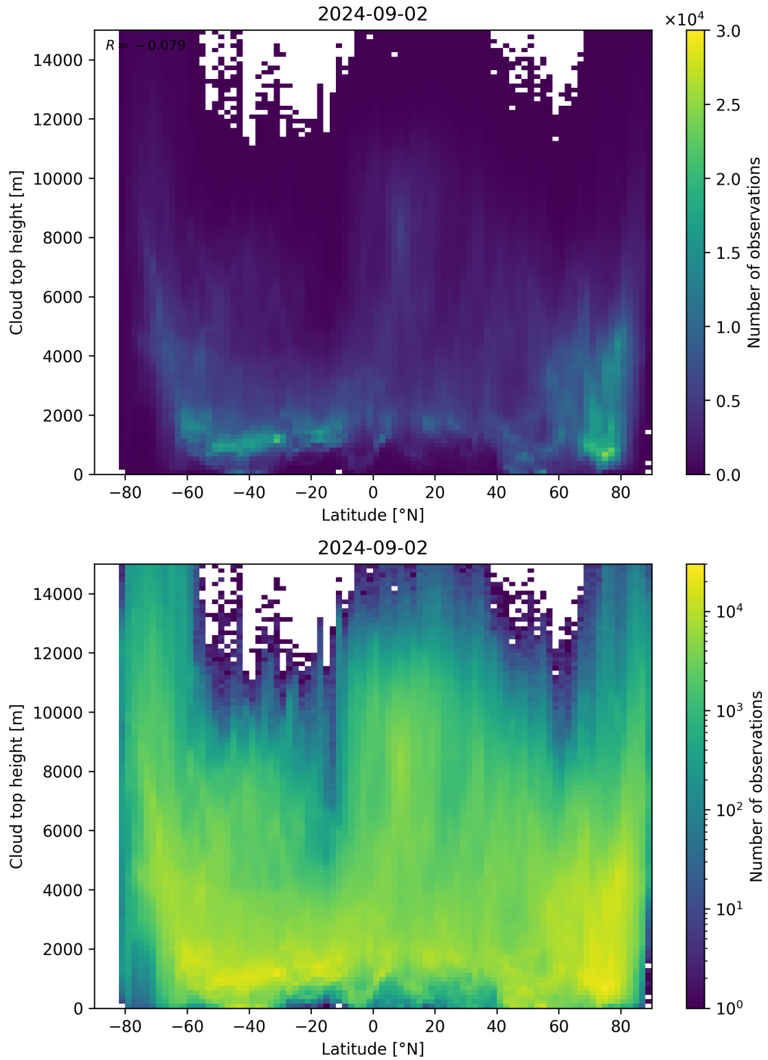
Figure 97: Scatter density plot of “Latitude” against “Cloud top height” for 2024-09-01 to 2024-09-03.
