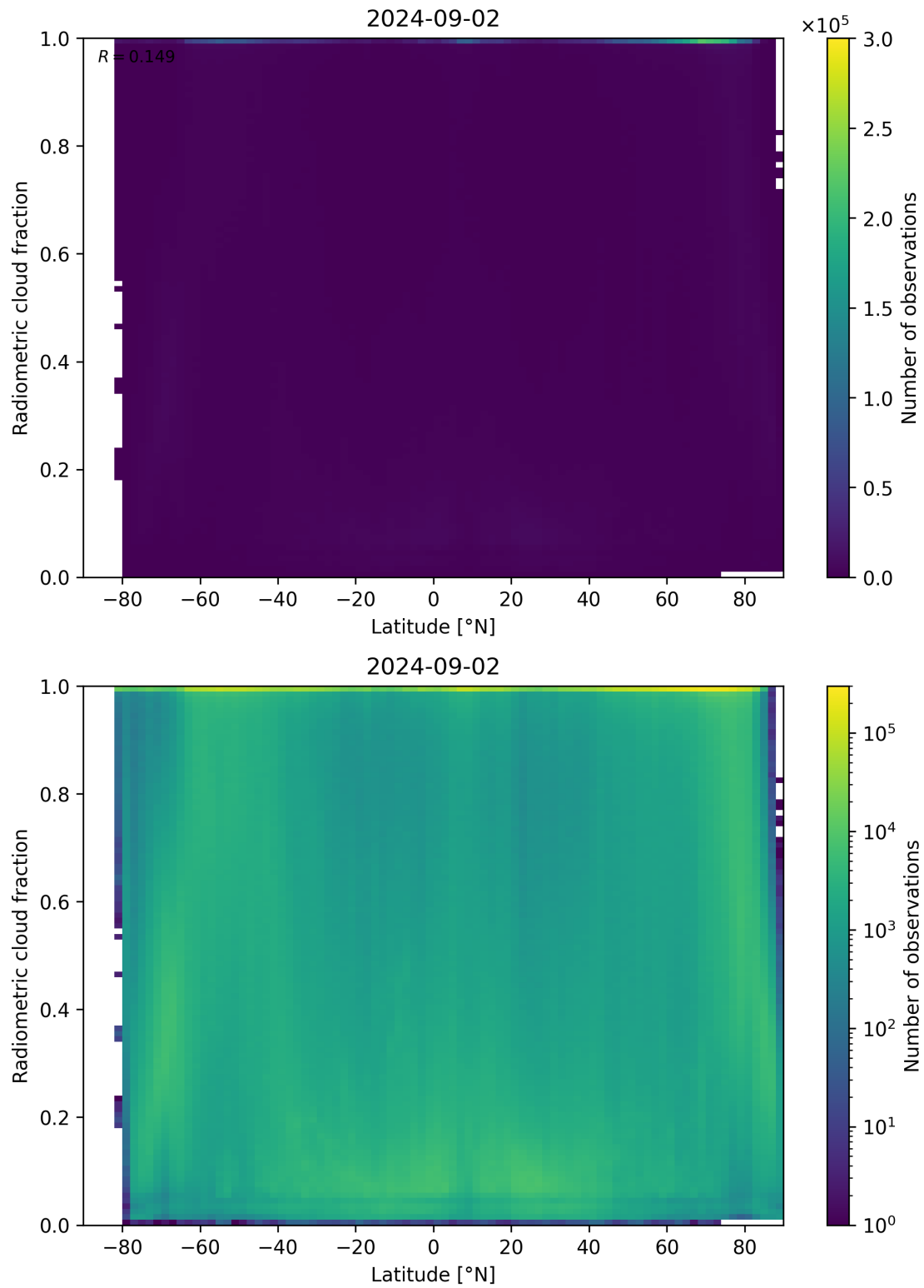
Figure 92: Scatter density plot of “Latitude” against “Radiometric cloud fraction” for 2024-09-01 to 2024-09-03.
