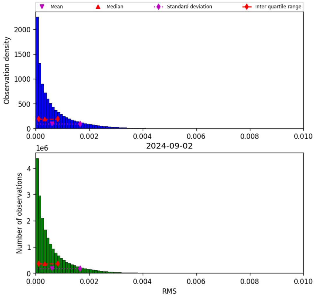
Figure 47: Histogram of “RMS” for 2024-09-01 to 2024-09-03
