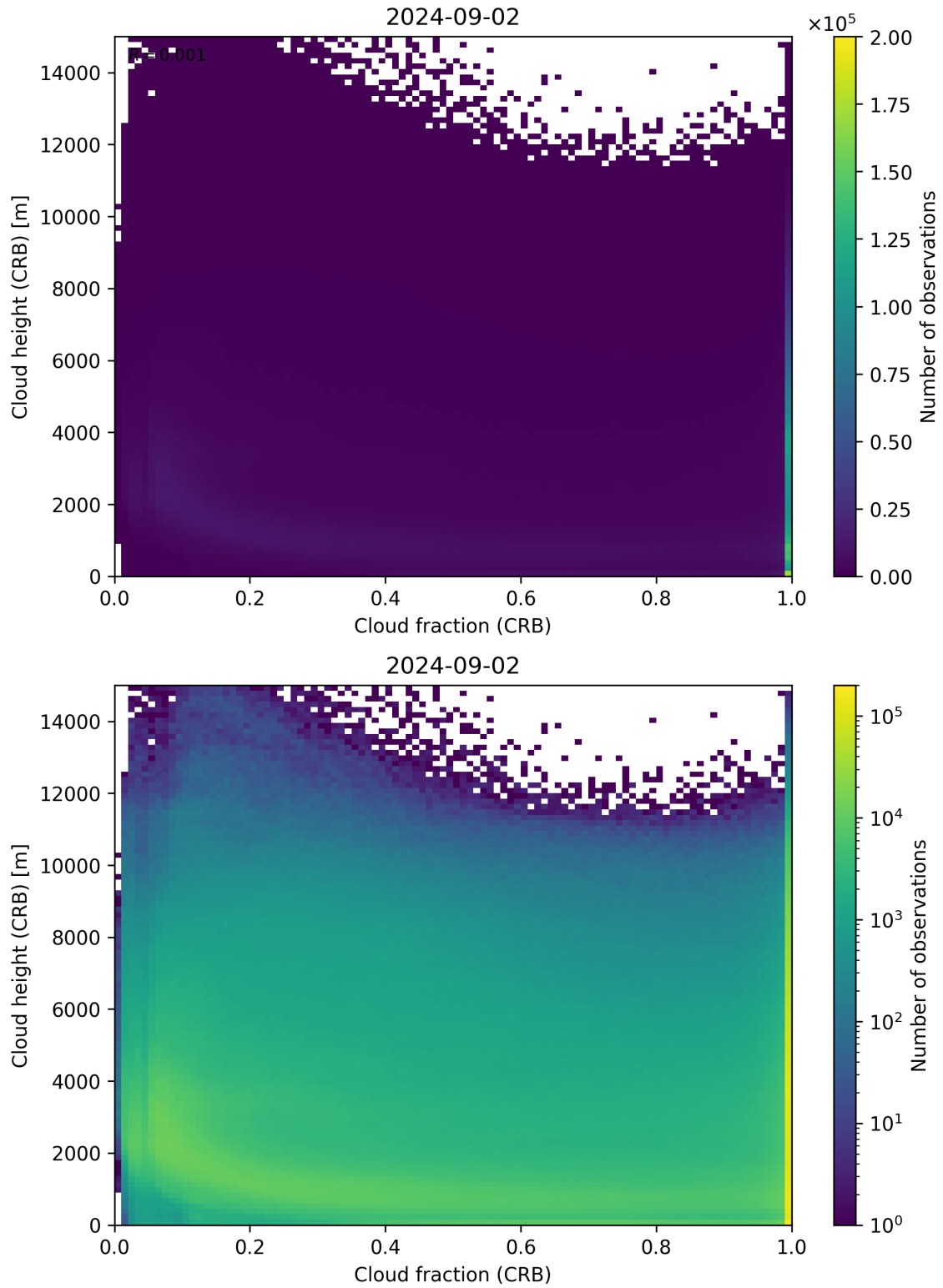
Figure 79: Scatter density plot of “Cloud fraction (CRB)” against “Cloud height (CRB)” for 2024-09-01 to 2024-09-03.
