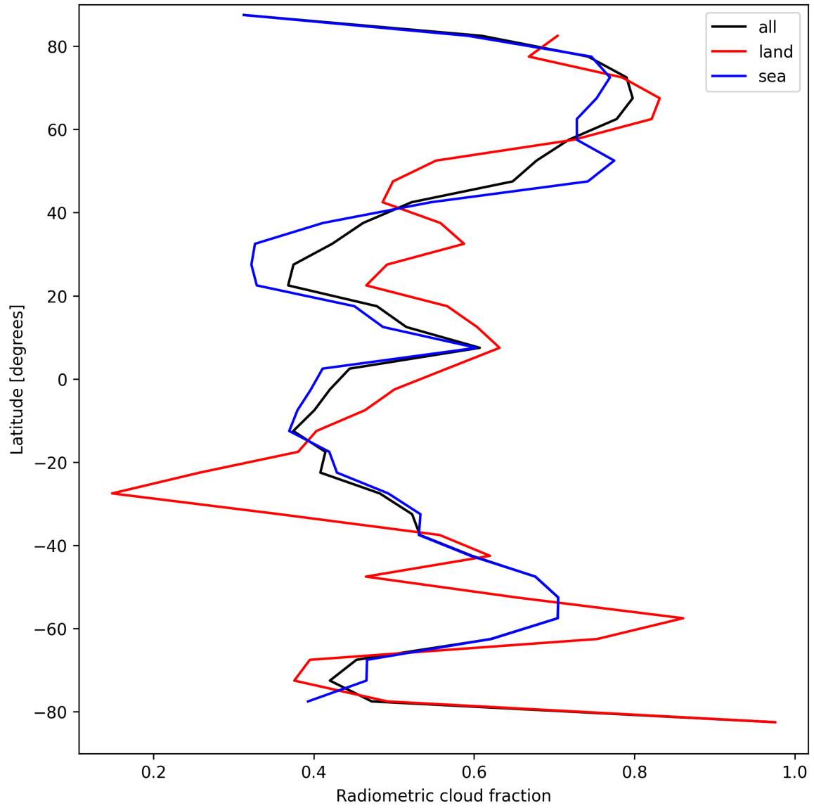
Figure 23: Zonal average of “Radiometric cloud fraction” for 2024-09-01 to 2024-09-03.
