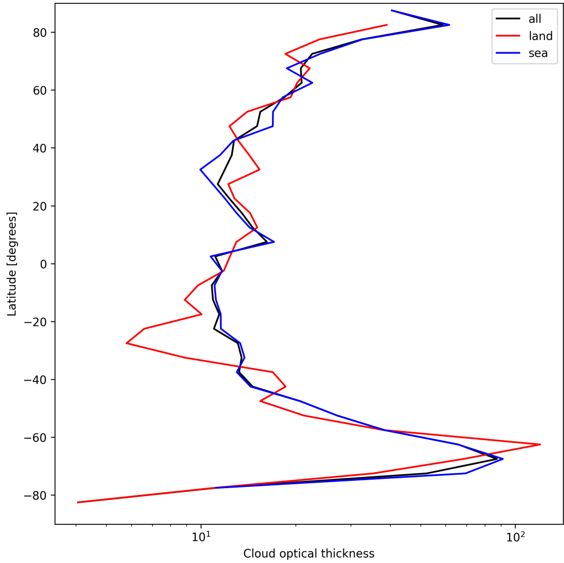
Figure 25: Zonal average of “Cloud optical thickness” for 2024-09-01 to 2024-09-03.
