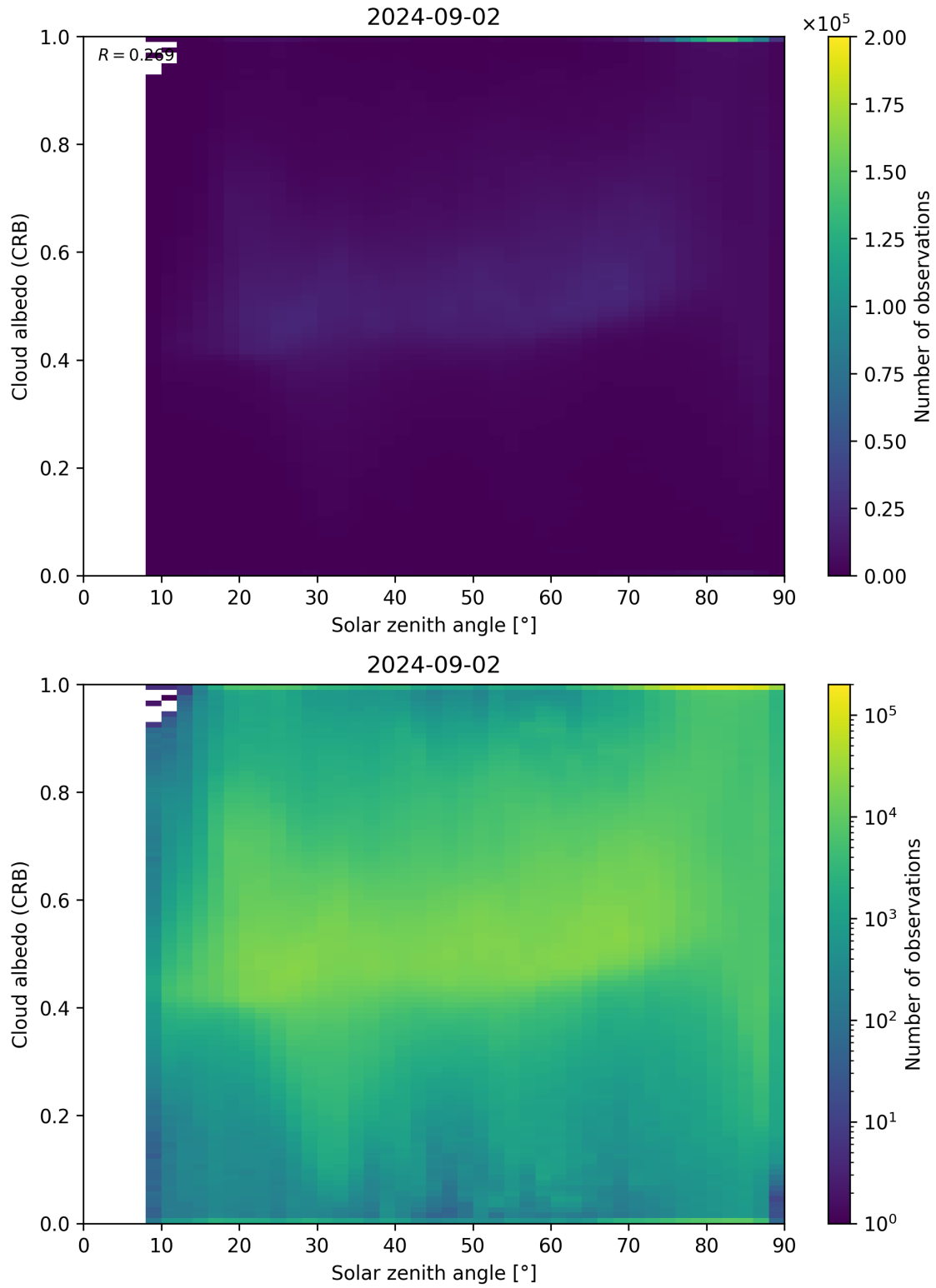
Figure 98: Scatter density plot of “Solar zenith angle” against “Cloud albedo (CRB)” for 2024-09-01 to 2024-09-03.
