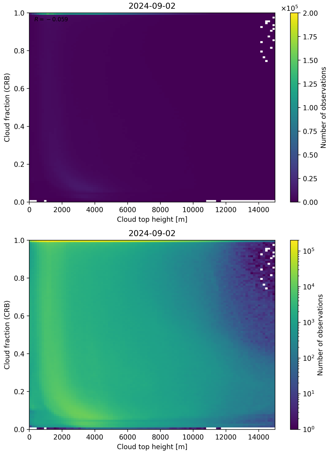
Figure 88: Scatter density plot of “Cloud top height” against “Cloud fraction (CRB)” for 2024-09-01 to 2024-09-03.
