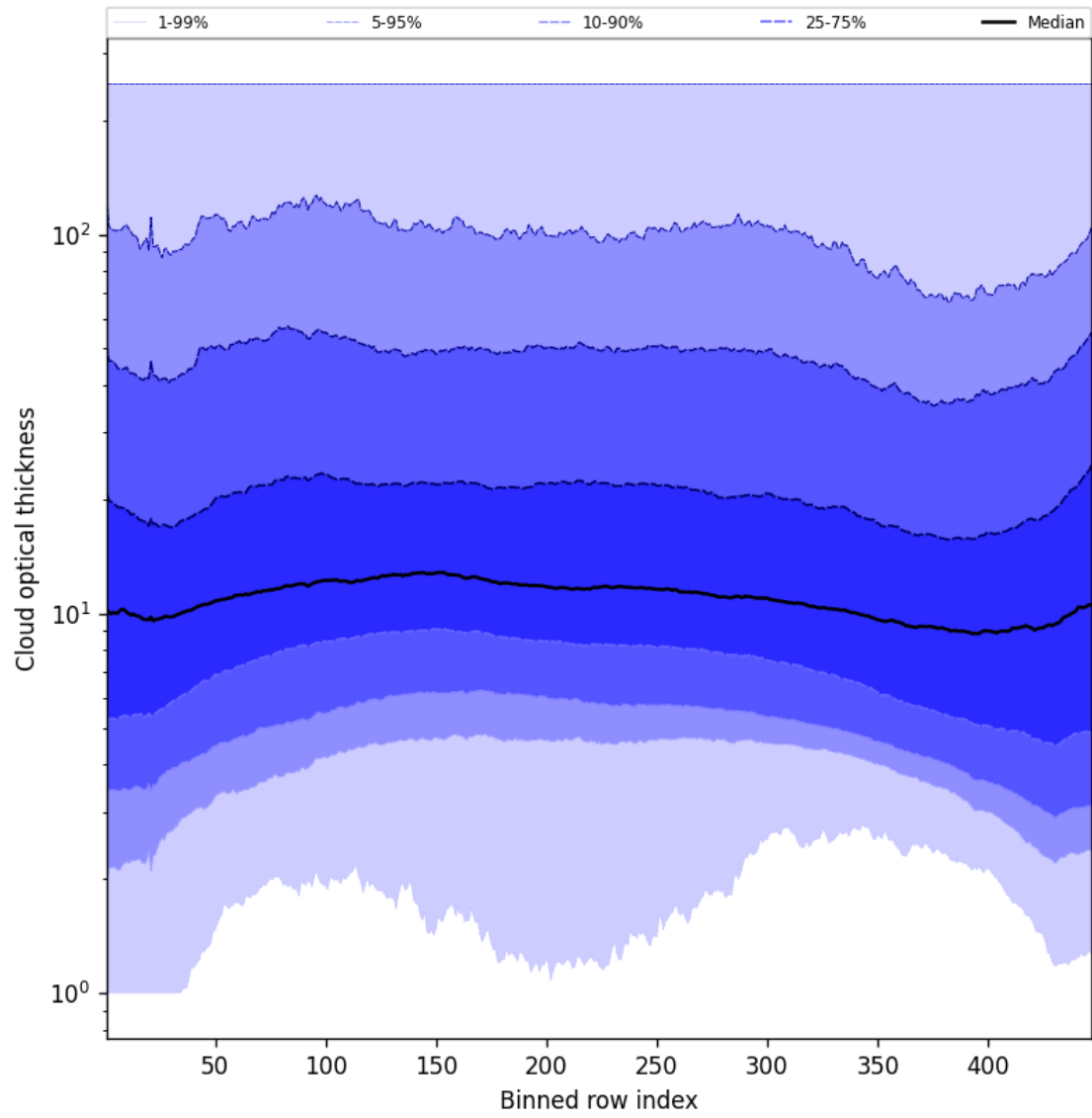
Figure 57: Along track statistics of “Cloud optical thickness” for 2024-09-01 to 2024-09-03
