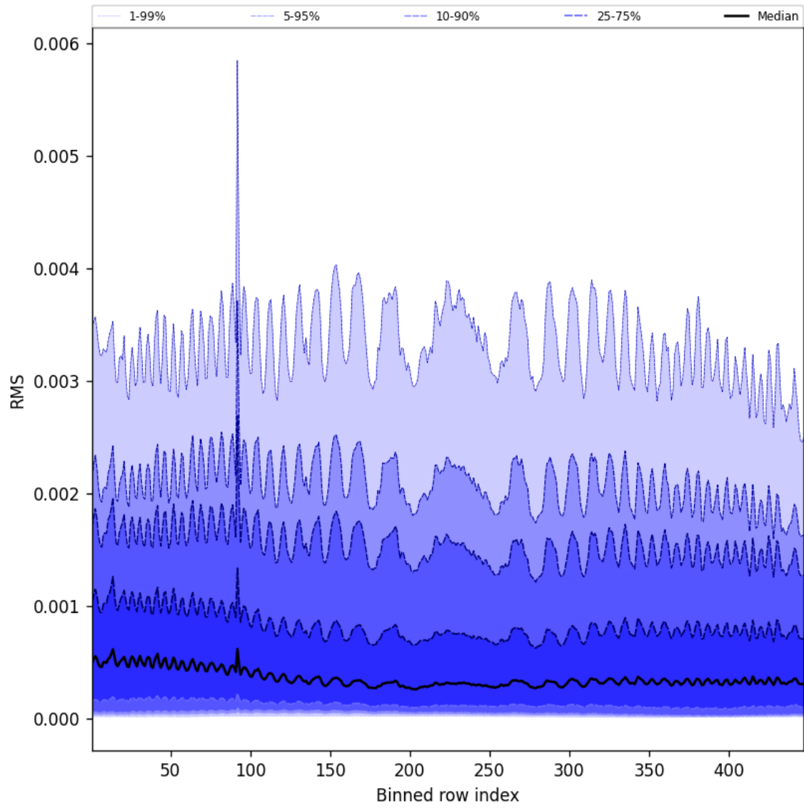
Figure 63: Along track statistics of “RMS” for 2024-09-01 to 2024-09-03
