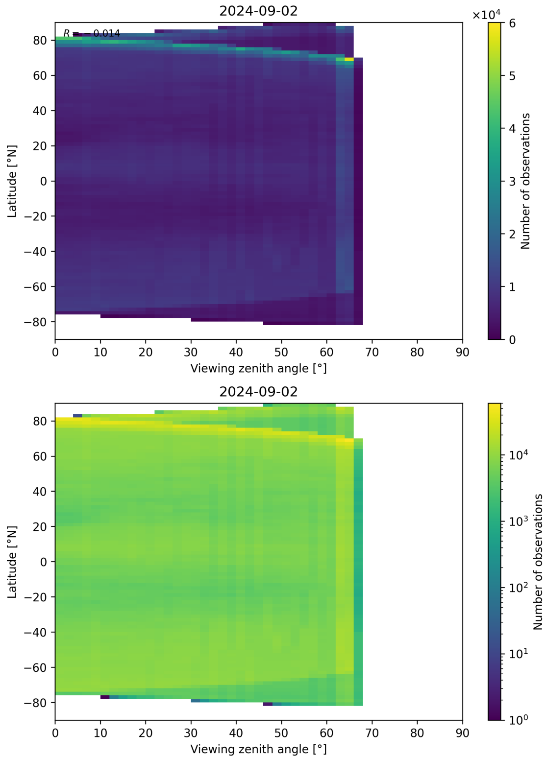
Figure 113: Scatter density plot of “Viewing zenith angle” against “Latitude” for 2024-09-01 to 2024-09-03.
