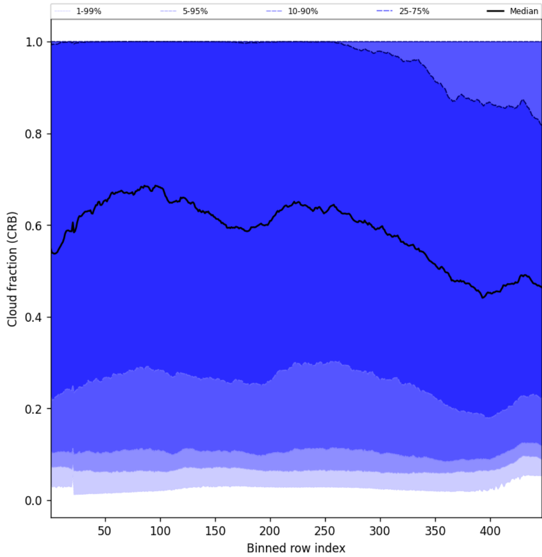
Figure 58: Along track statistics of “Cloud fraction (CRB)” for 2024-09-01 to 2024-09-03
