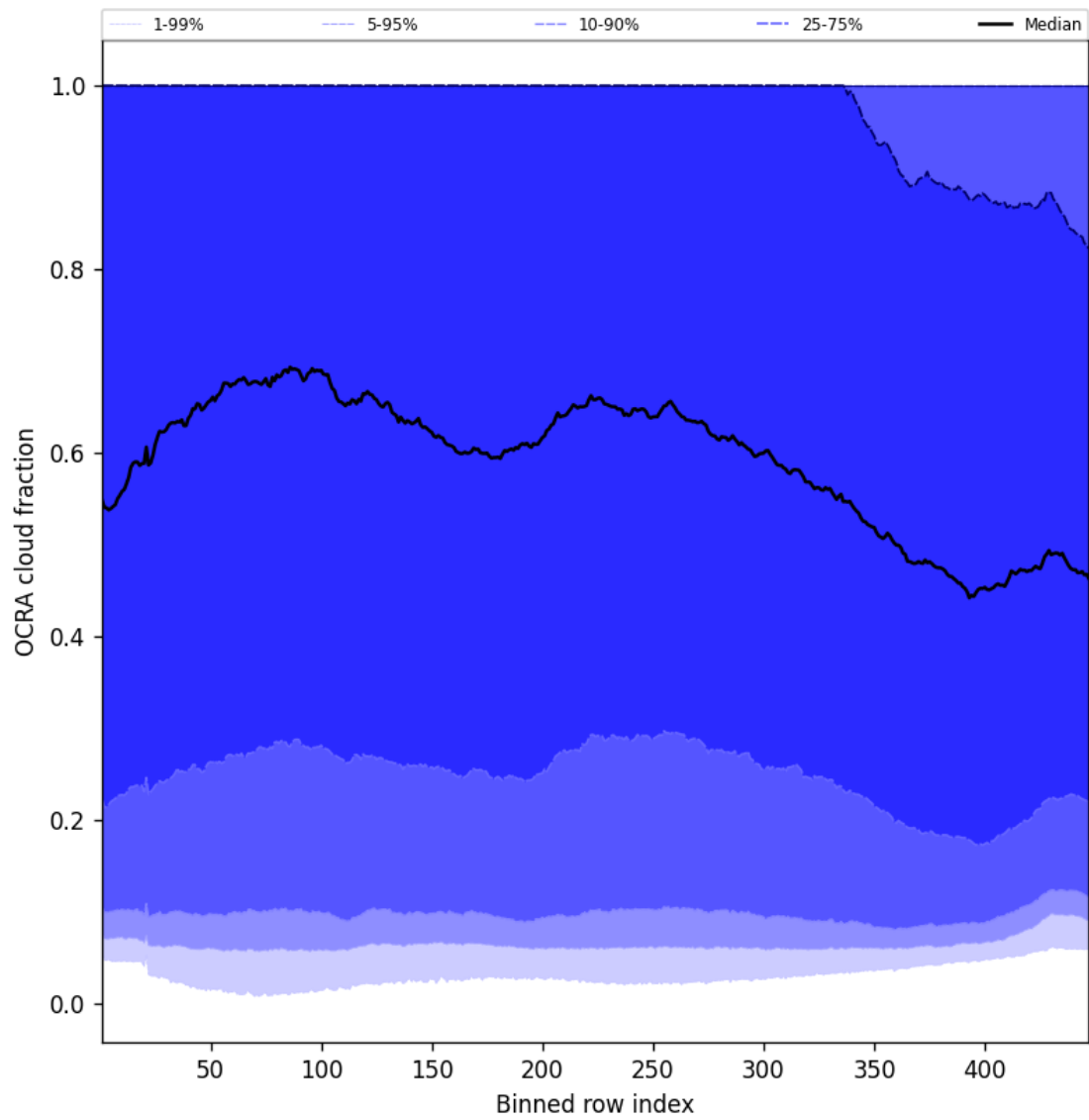
Figure 66: Along track statistics of “OCRA cloud fraction” for 2024-09-01 to 2024-09-03
