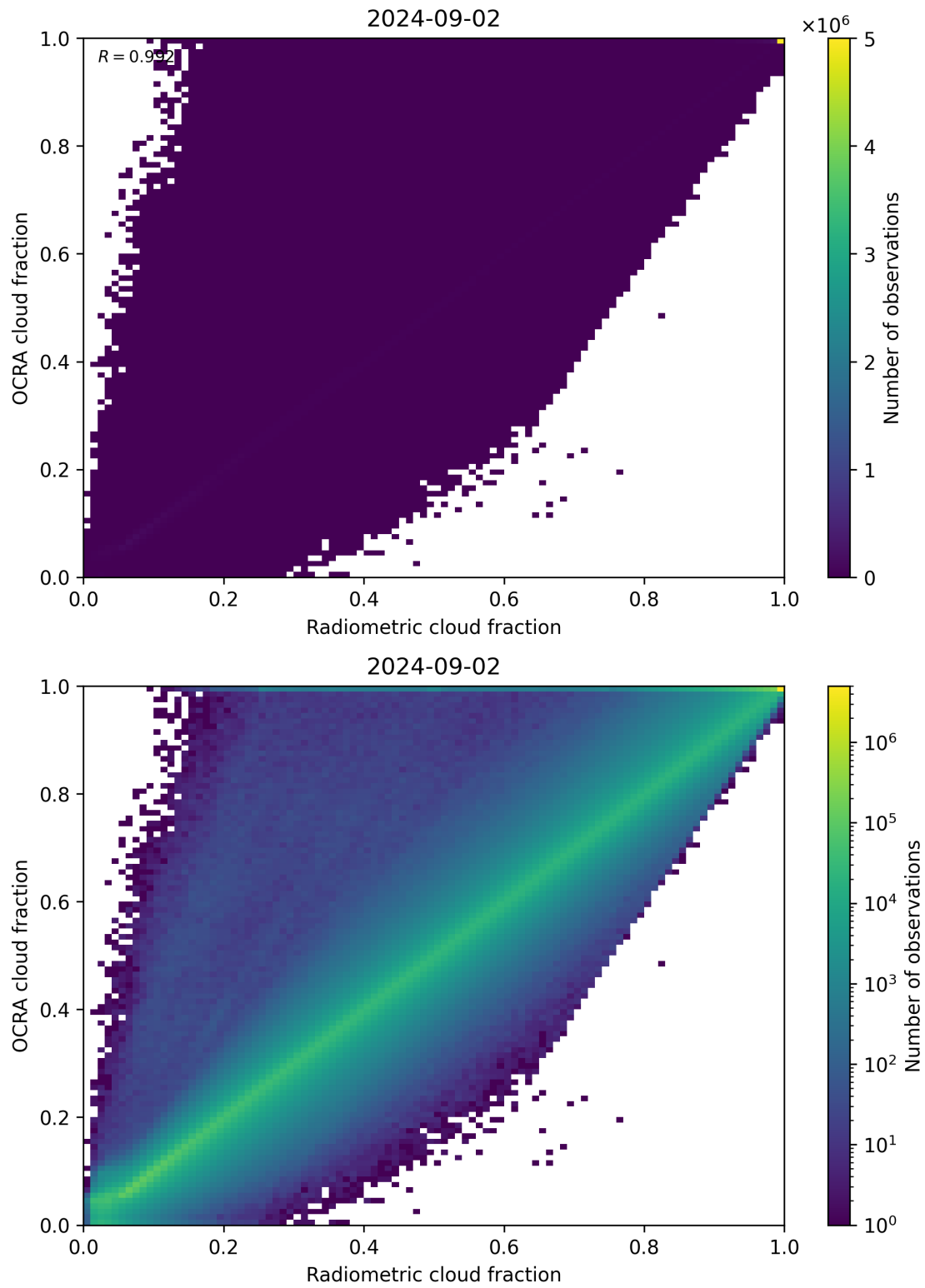
Figure 72: Scatter density plot of “Radiometric cloud fraction” against “OCRA cloud fraction” for 2024-09-01 to 2024-09-03.
