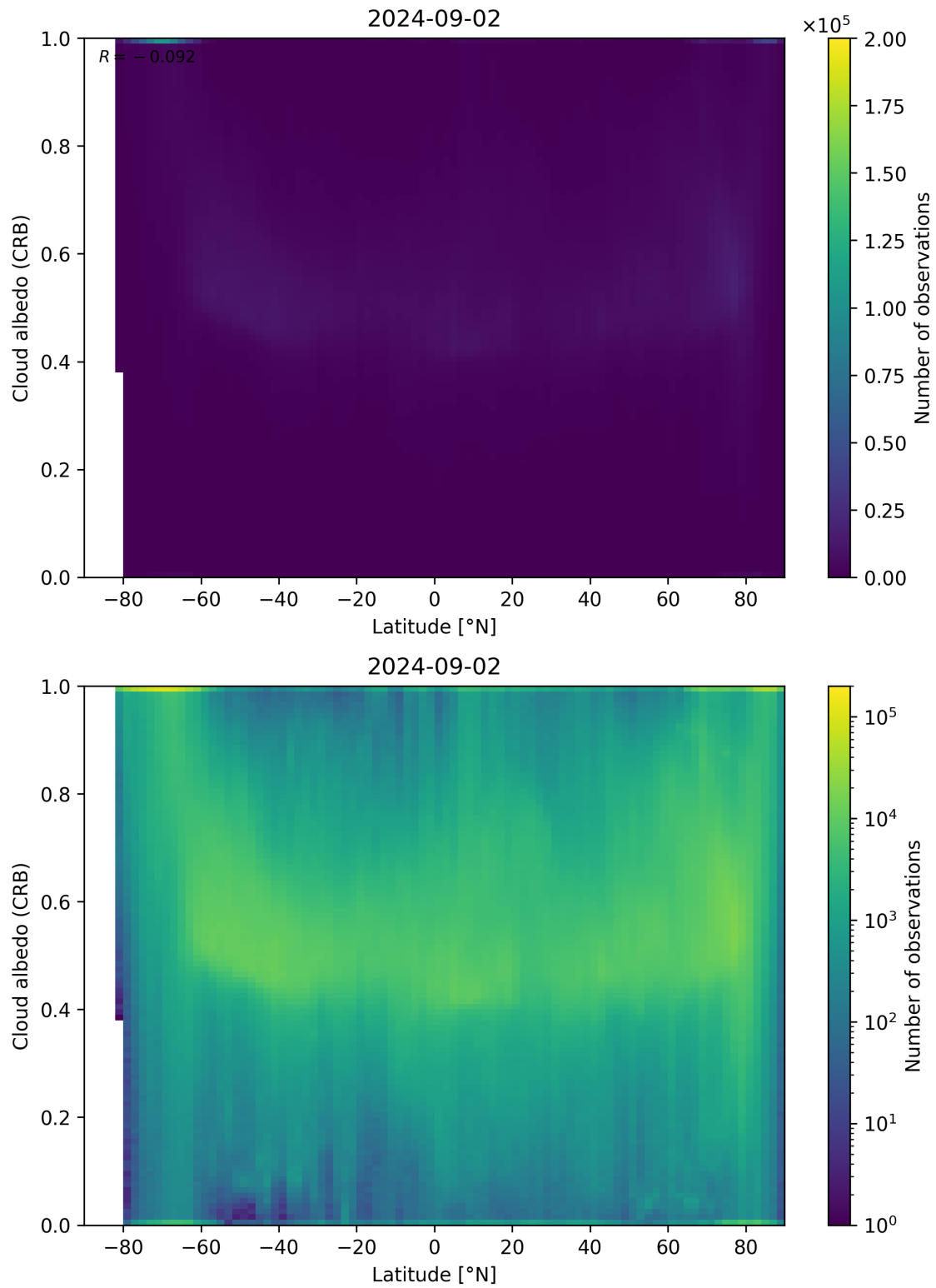
Figure 91: Scatter density plot of “Latitude” against “Cloud albedo (CRB)” for 2024-09-01 to 2024-09-03.
