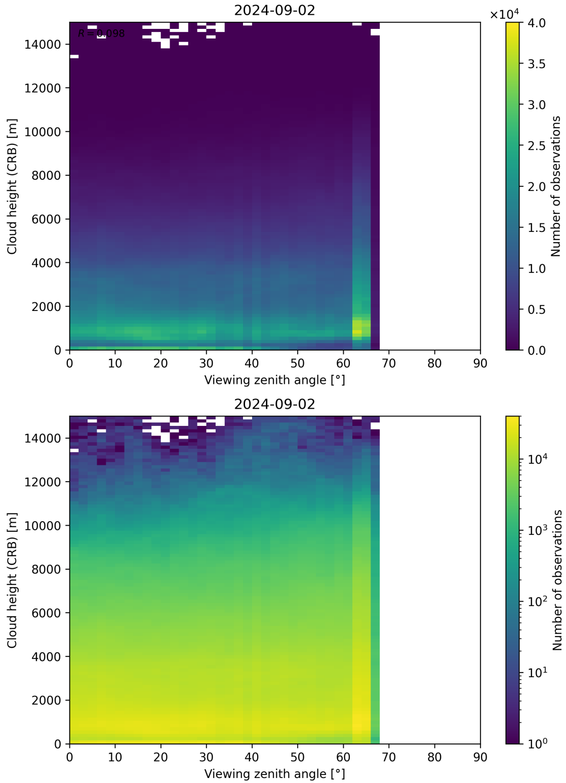
Figure 110: Scatter density plot of “Viewing zenith angle” against “Cloud height (CRB)” for 2024-09-01 to 2024-09-03.
