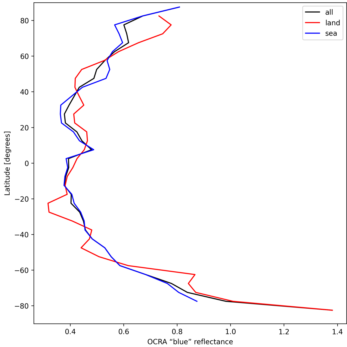
Figure 35: Zonal average of “OCRA “blue” reflectance” for 2024-09-01 to 2024-09-03.
