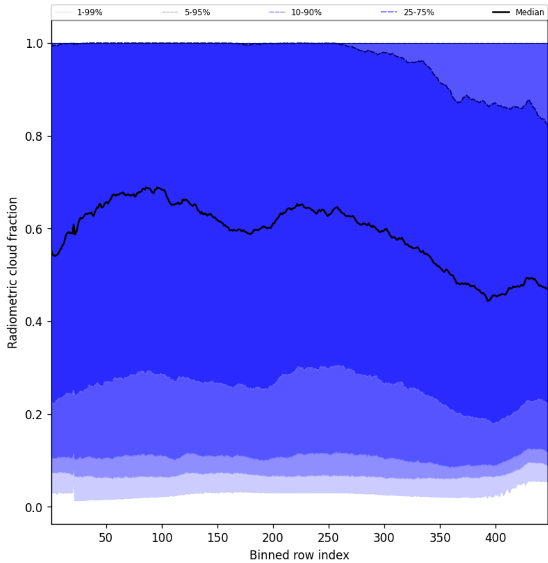
Figure 55: Along track statistics of “Radiometric cloud fraction” for 2024-09-01 to 2024-09-03
