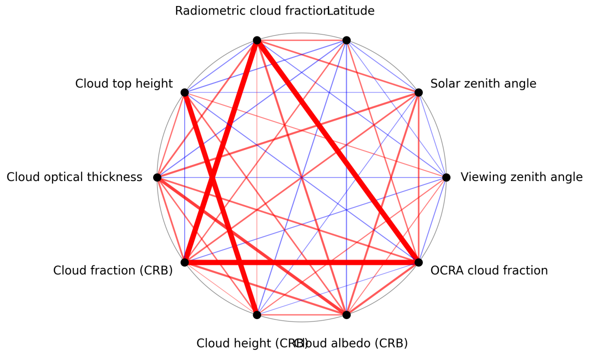
Figure 1: Map of correlation graph for 2024-09-01 to 2024-09-03.
