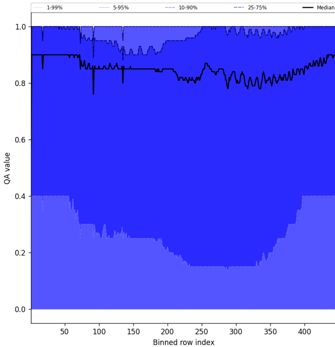
Figure 54: Along track statistics of “QA value” for 2024-09-01 to 2024-09-03
