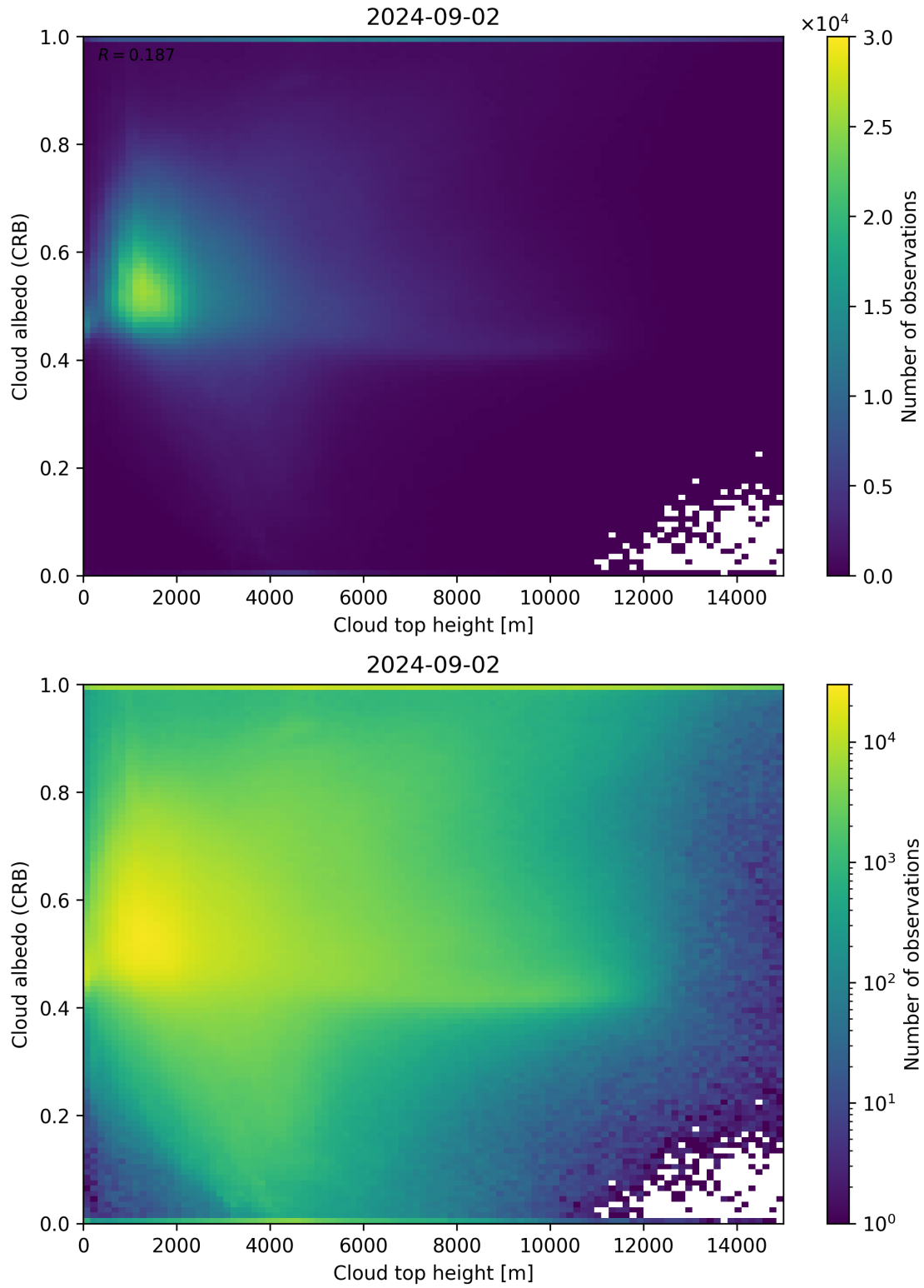
Figure 86: Scatter density plot of “Cloud top height” against “Cloud albedo (CRB)” for 2024-09-01 to 2024-09-03.
