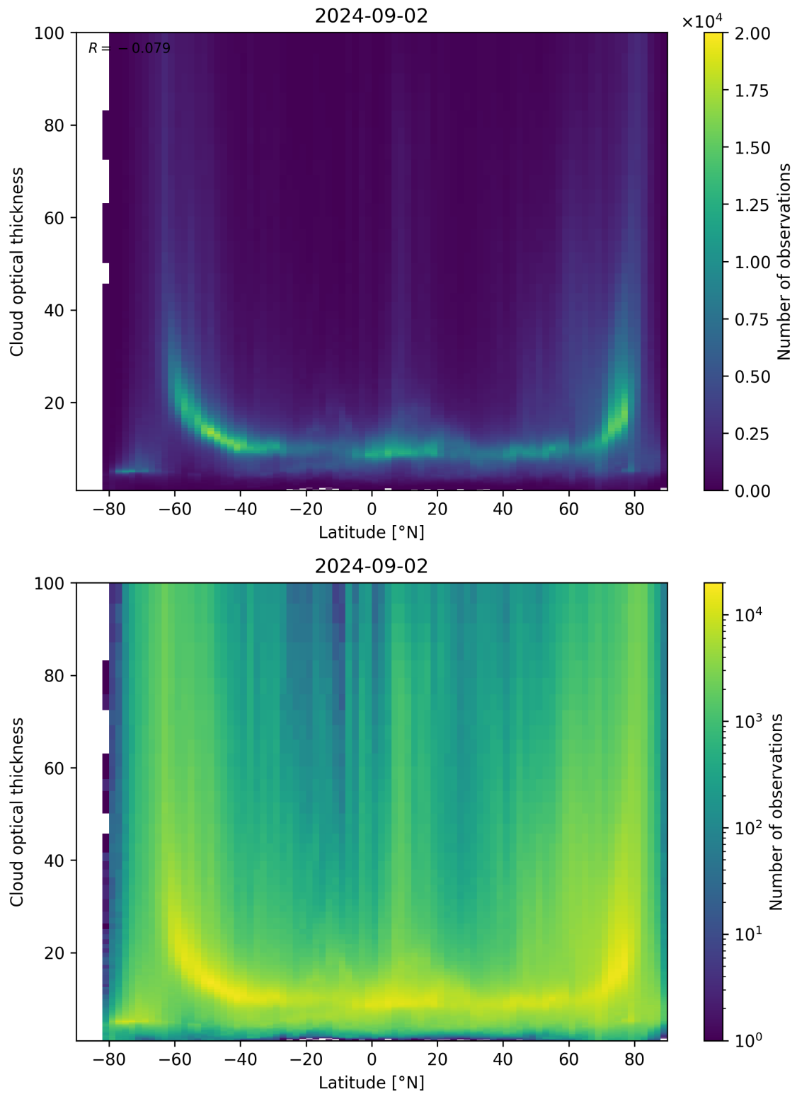
Figure 96: Scatter density plot of “Latitude” against “Cloud optical thickness” for 2024-09-01 to 2024-09-03.
