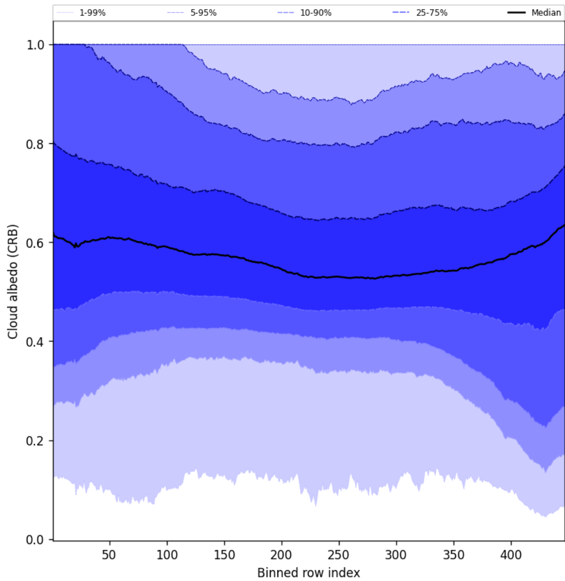
Figure 60: Along track statistics of “Cloud albedo (CRB)” for 2024-09-01 to 2024-09-03
