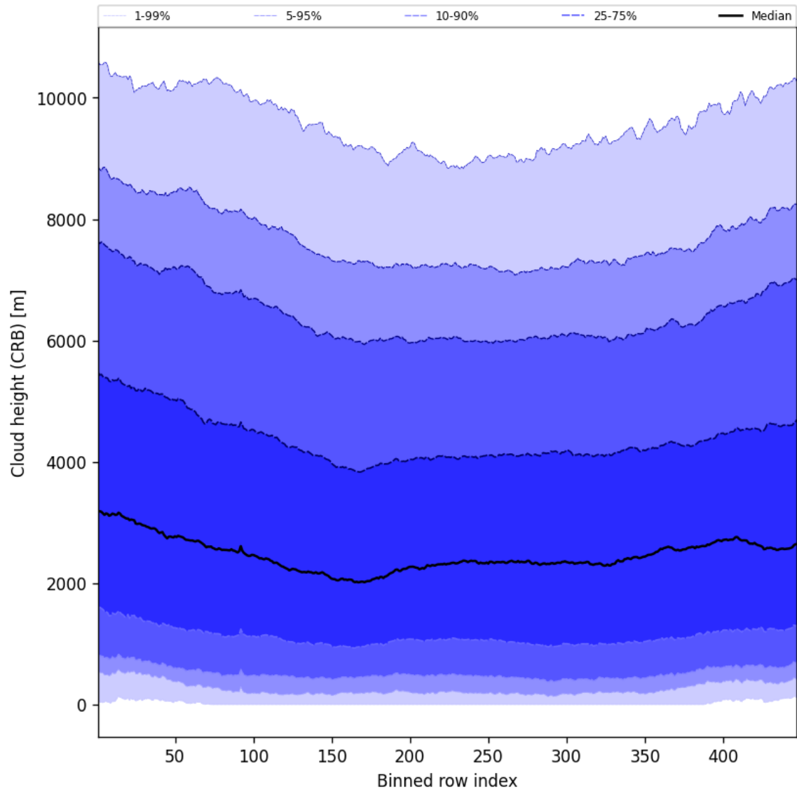
Figure 59: Along track statistics of “Cloud height (CRB)” for 2024-09-01 to 2024-09-03
