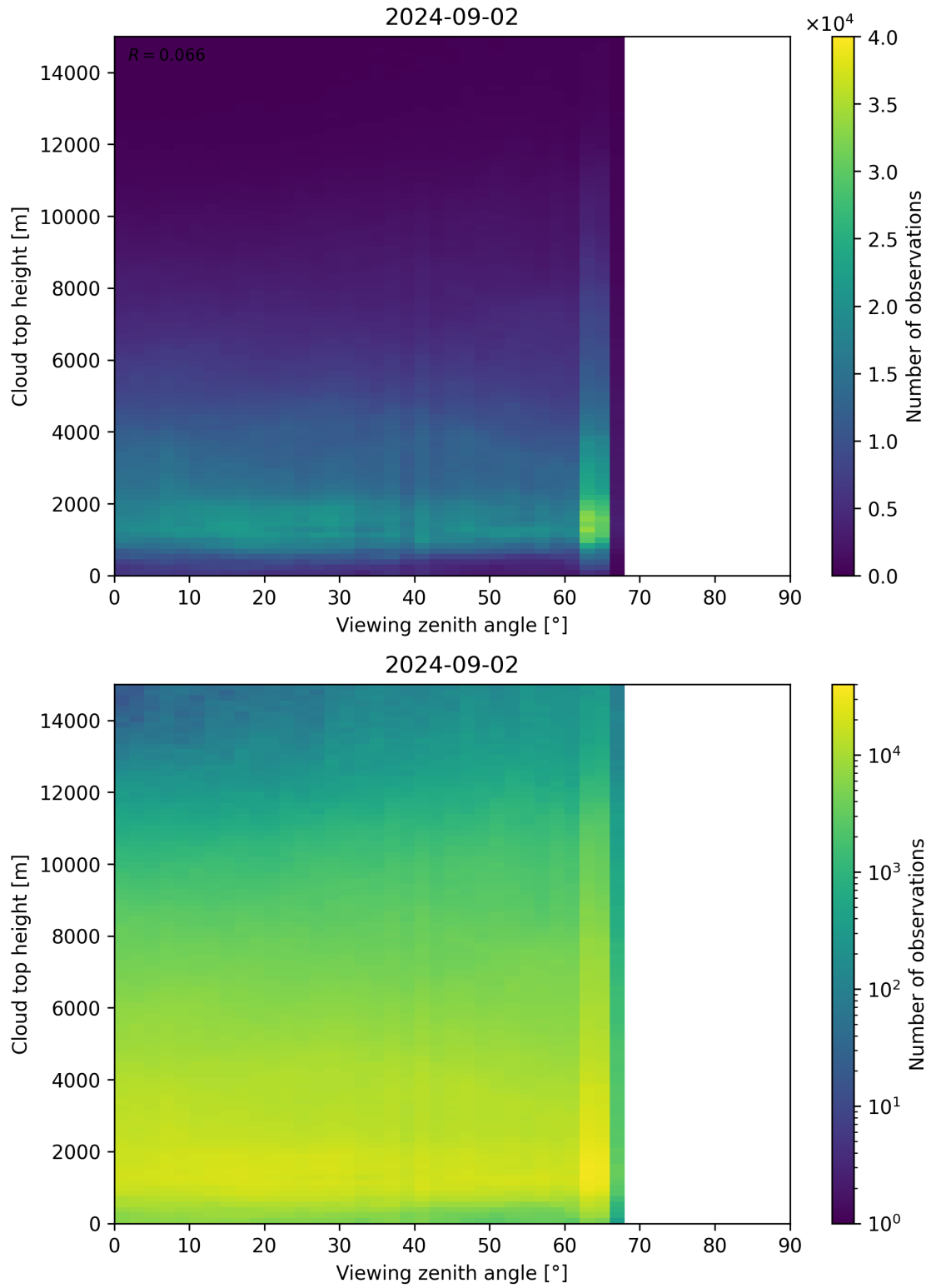
Figure 112: Scatter density plot of “Viewing zenith angle” against “Cloud top height” for 2024-09-01 to 2024-09-03.
