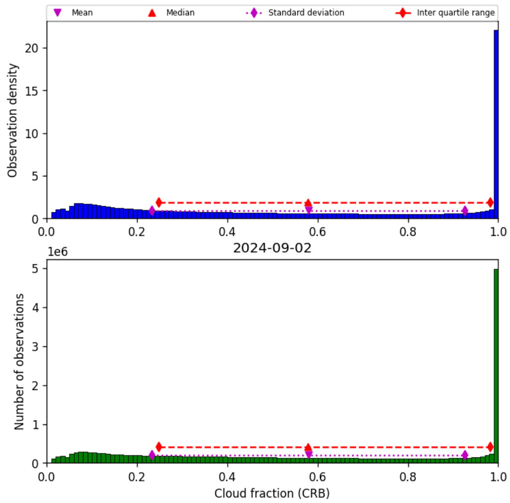
Figure 42: Histogram of “Cloud fraction (CRB)” for 2024-09-01 to 2024-09-03
