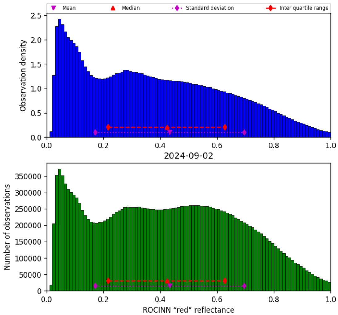
Figure 53: Histogram of “ROCINN “red” reflectance” for 2024-09-01 to 2024-09-03
