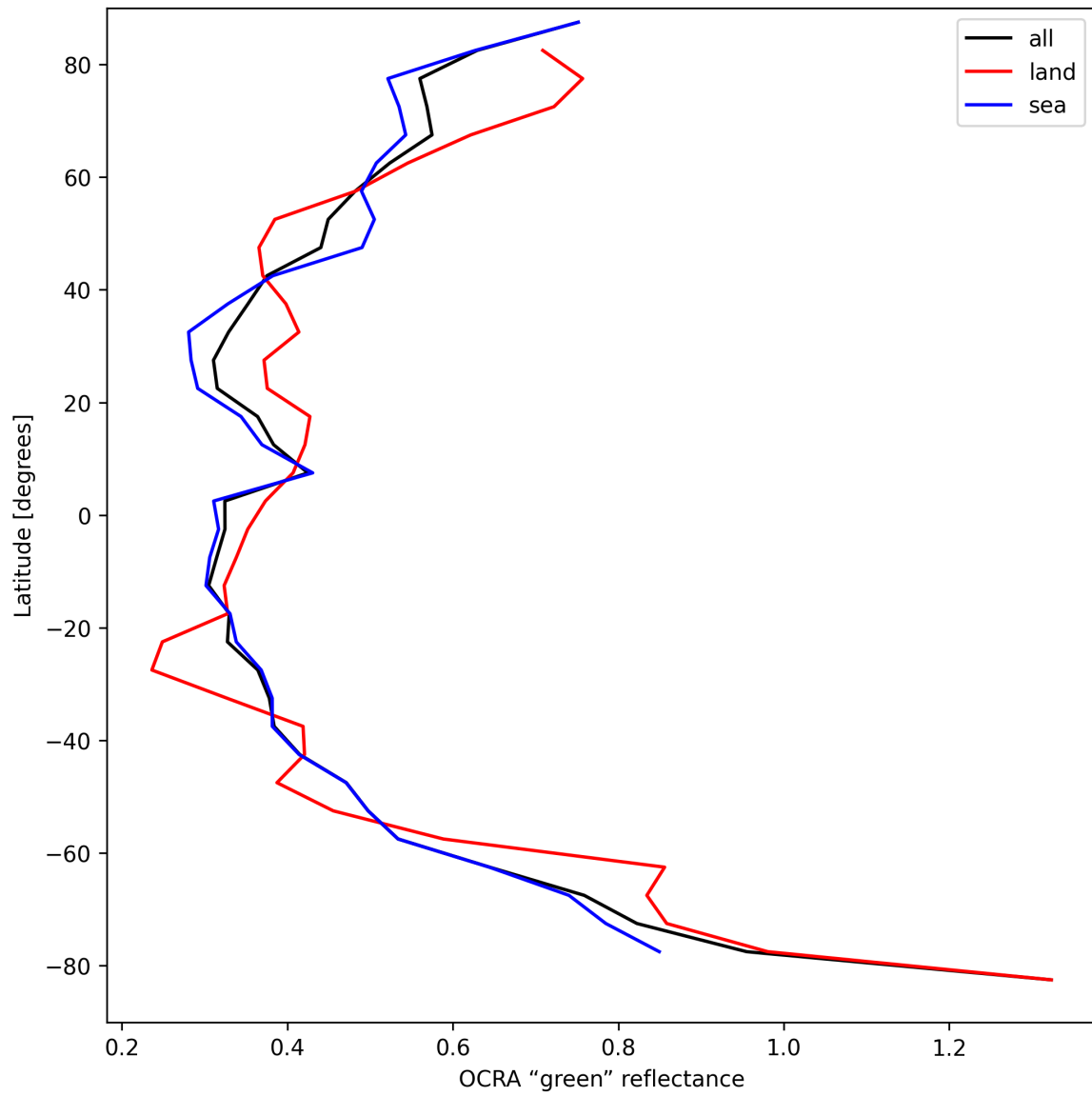
Figure 36: Zonal average of “OCRA “green” reflectance” for 2024-09-01 to 2024-09-03.
