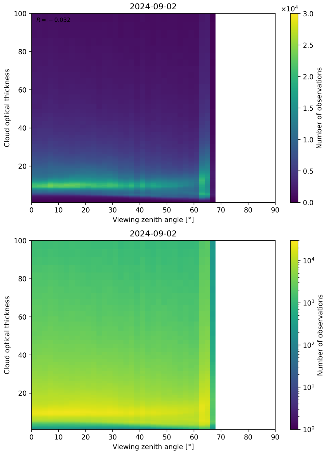
Figure 111: Scatter density plot of “Viewing zenith angle” against “Cloud optical thickness” for 2024-09-01 to 2024-09-03.
