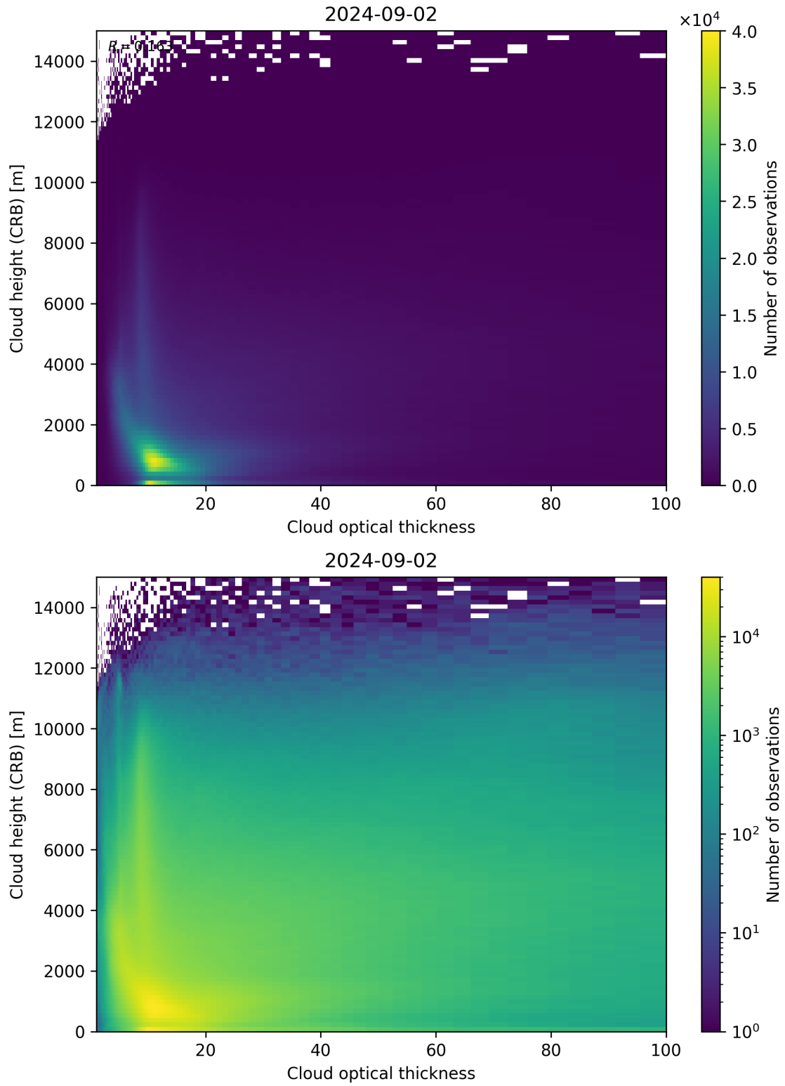
Figure 85: Scatter density plot of “Cloud optical thickness” against “Cloud height (CRB)” for 2024-09-01 to 2024-09-03.
