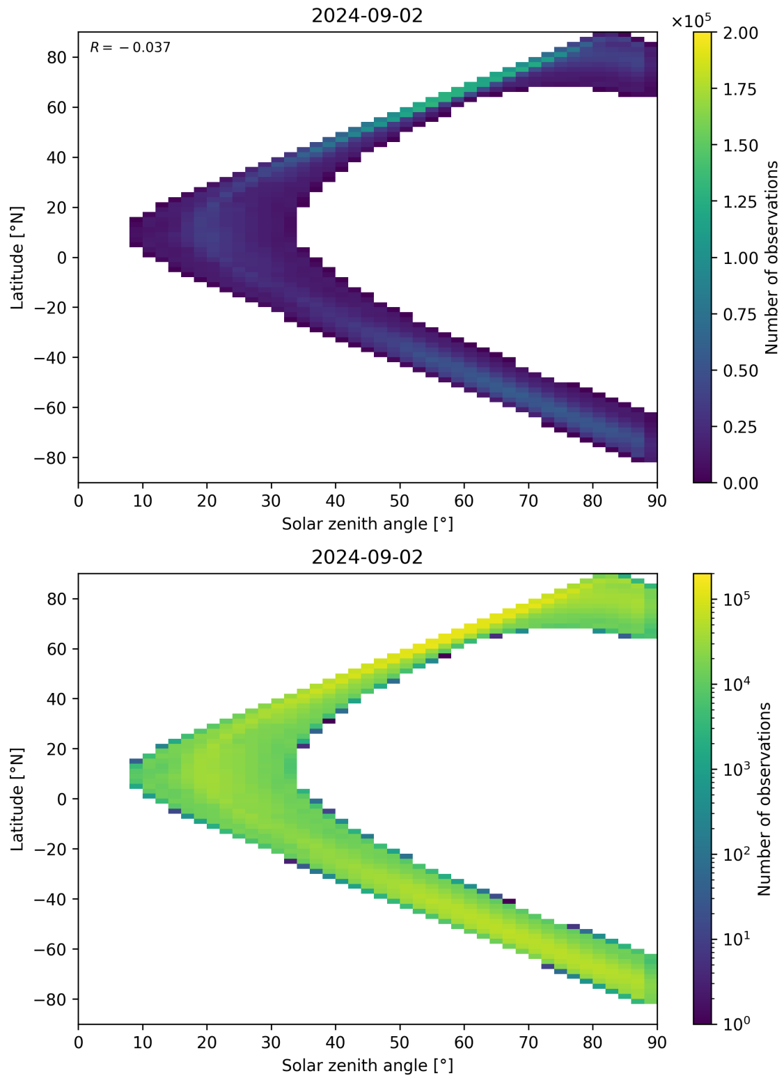
Figure 105: Scatter density plot of “Solar zenith angle” against “Latitude” for 2024-09-01 to 2024-09-03.
