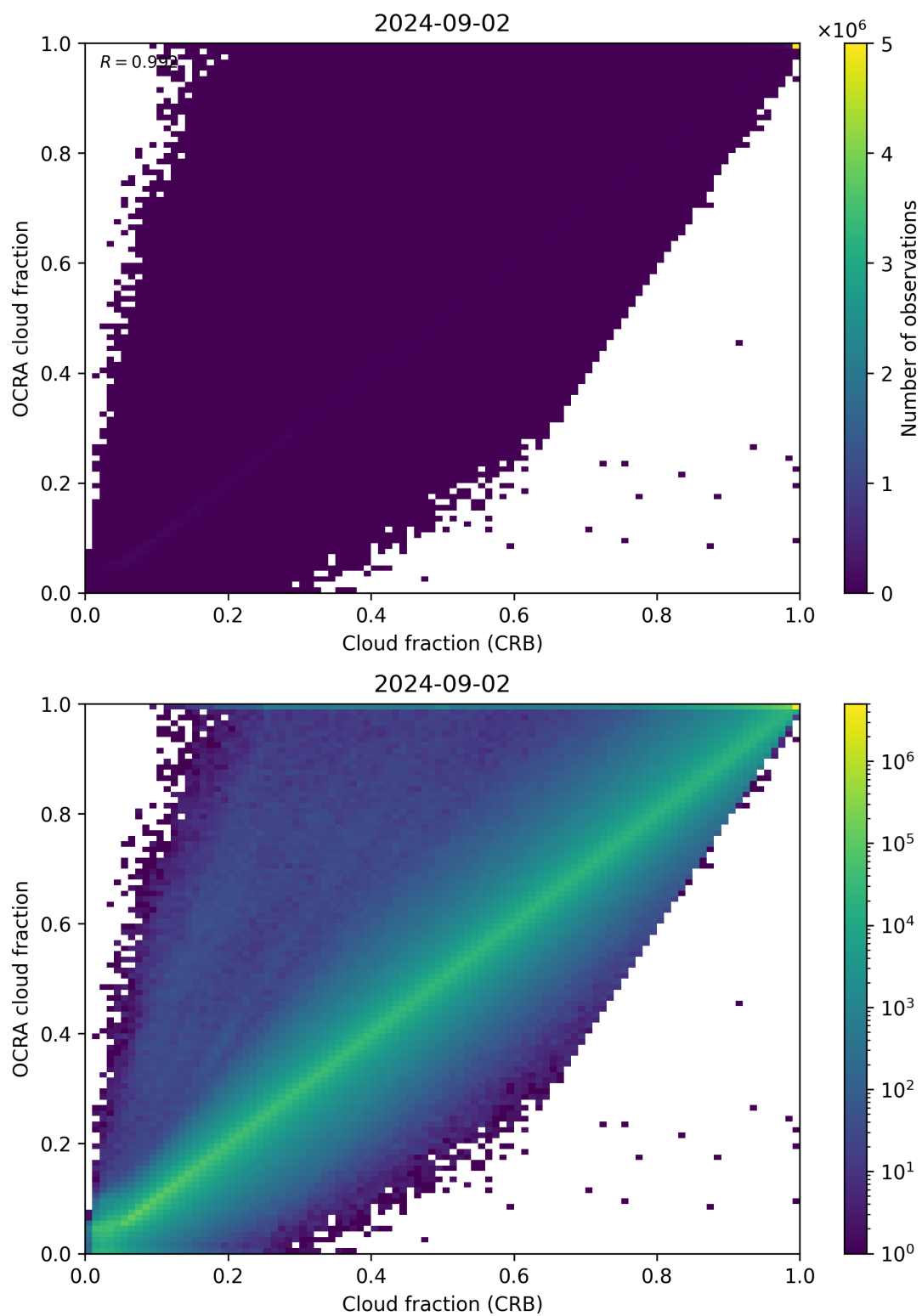
Figure 78: Scatter density plot of “Cloud fraction (CRB)” against “OCRA cloud fraction” for 2024-09-01 to 2024-09-03.
