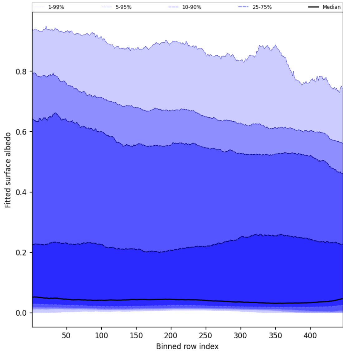
Figure 61: Along track statistics of “Fitted surface albedo” for 2024-09-01 to 2024-09-03
