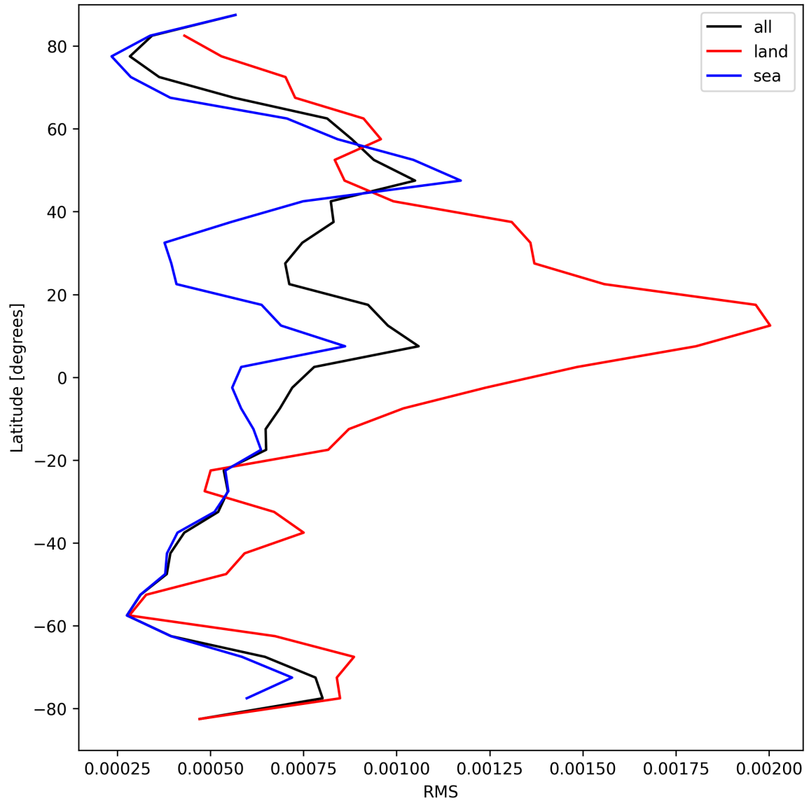
Figure 31: Zonal average of “RMS” for 2024-09-01 to 2024-09-03.
