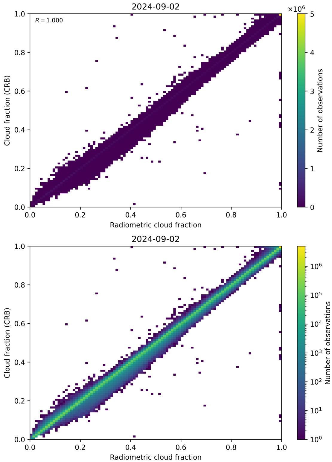
Figure 73: Scatter density plot of “Radiometric cloud fraction” against “Cloud fraction (CRB)” for 2024-09-01 to 2024-09-03.
