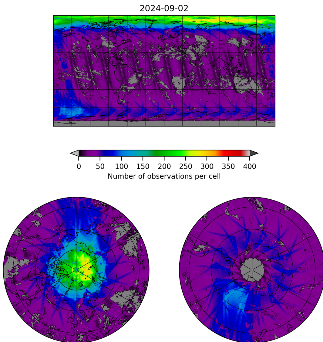
Figure 21: Map of the number of observations for 2024-09-01 to 2024-09-03
