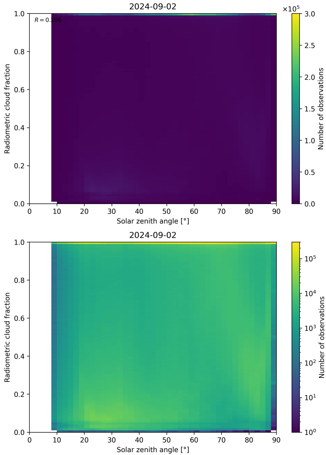
Figure 99: Scatter density plot of “Solar zenith angle” against “Radiometric cloud fraction” for 2024-09-01 to 2024-09-03.
