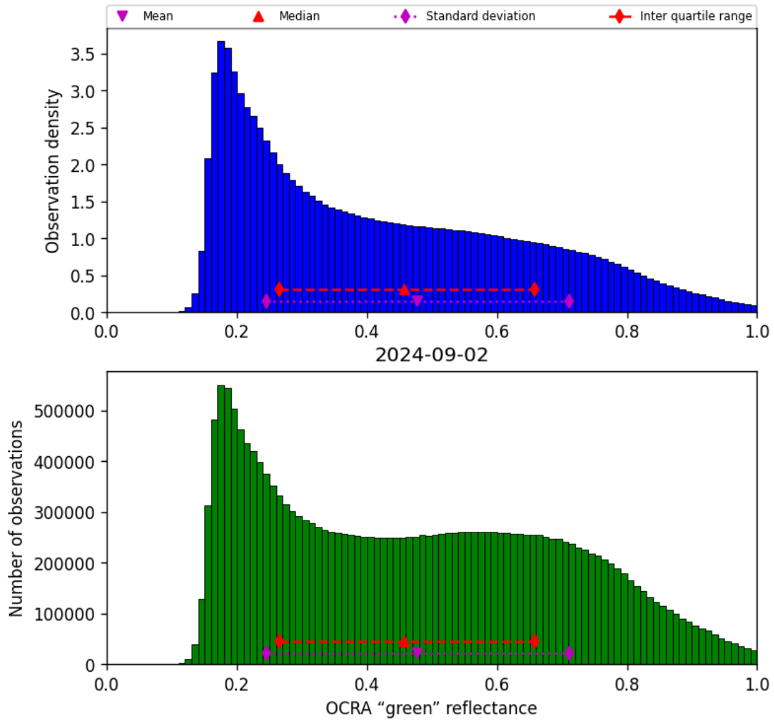
Figure 52: Histogram of “OCRA “green” reflectance” for 2024-09-01 to 2024-09-03
