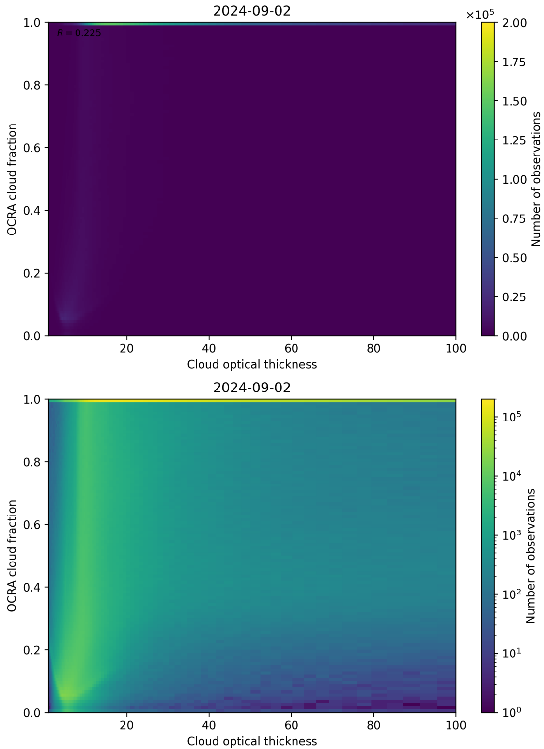
Figure 83: Scatter density plot of “Cloud optical thickness” against “OCRA cloud fraction” for 2024-09-01 to 2024-09-03.
