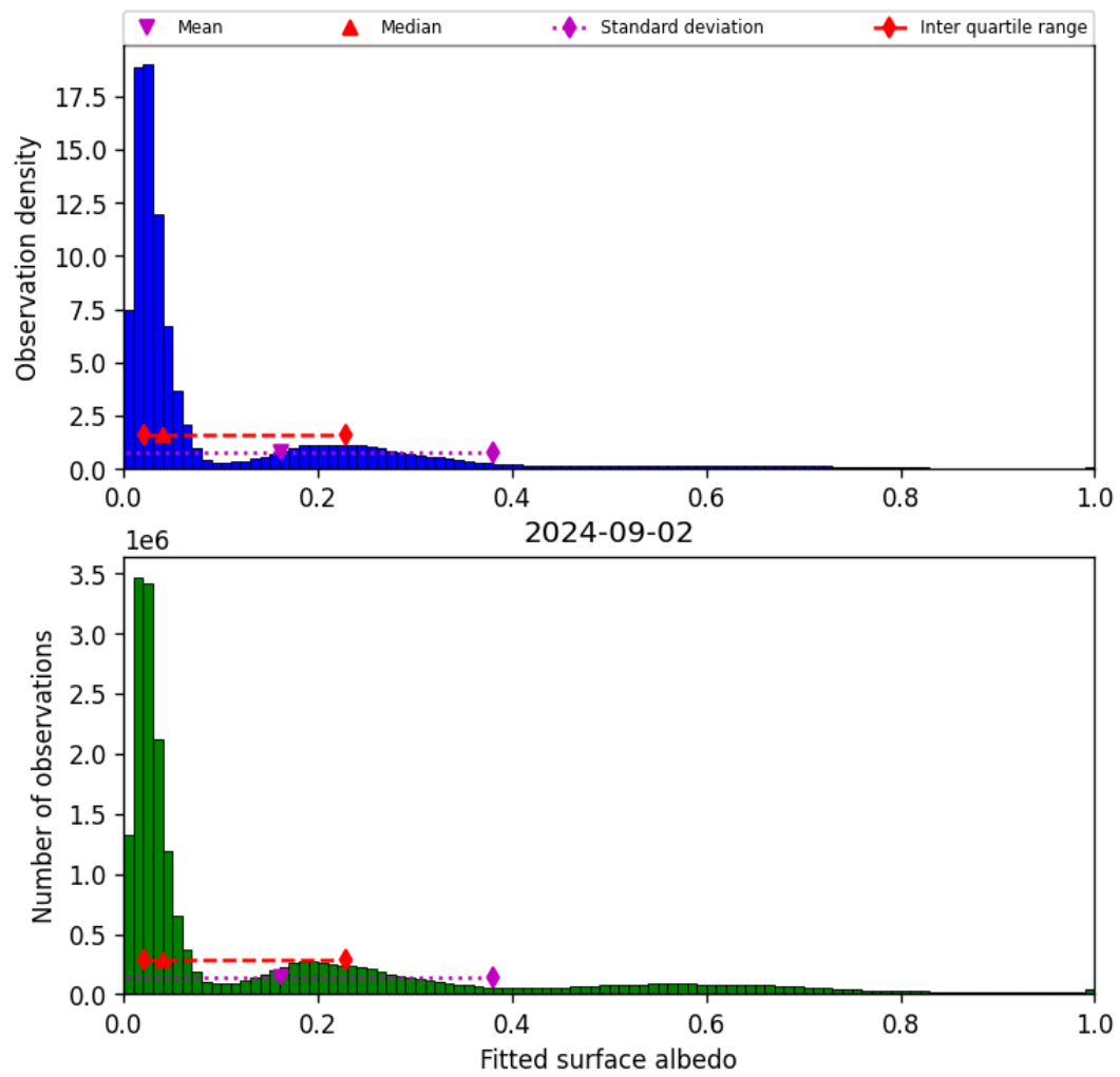
Figure 45: Histogram of “Fitted surface albedo” for 2024-09-01 to 2024-09-03
