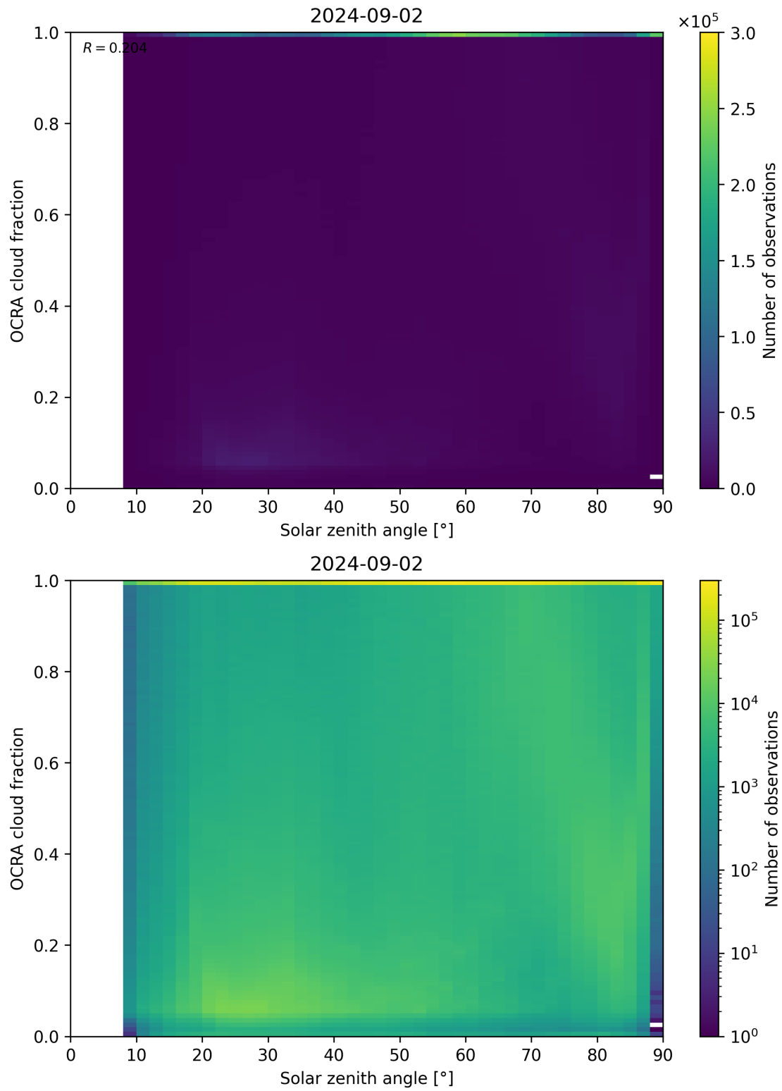
Figure 100: Scatter density plot of “Solar zenith angle” against “OCRA cloud fraction” for 2024-09-01 to 2024-09-03.
