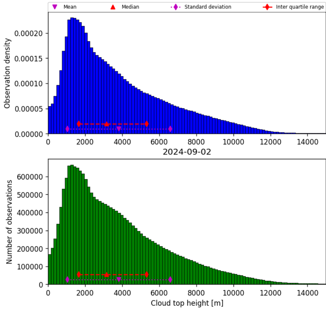
Figure 40: Histogram of “Cloud top height” for 2024-09-01 to 2024-09-03
