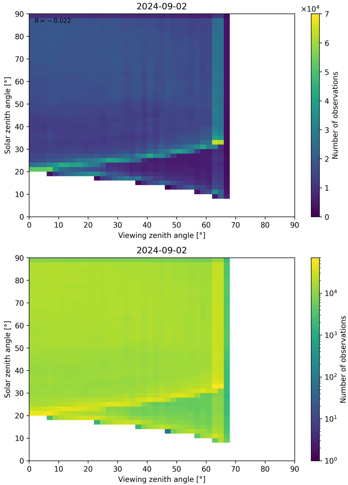
Figure 114: Scatter density plot of “Viewing zenith angle” against “Solar zenith angle” for 2024-09-01 to 2024-09-03.
