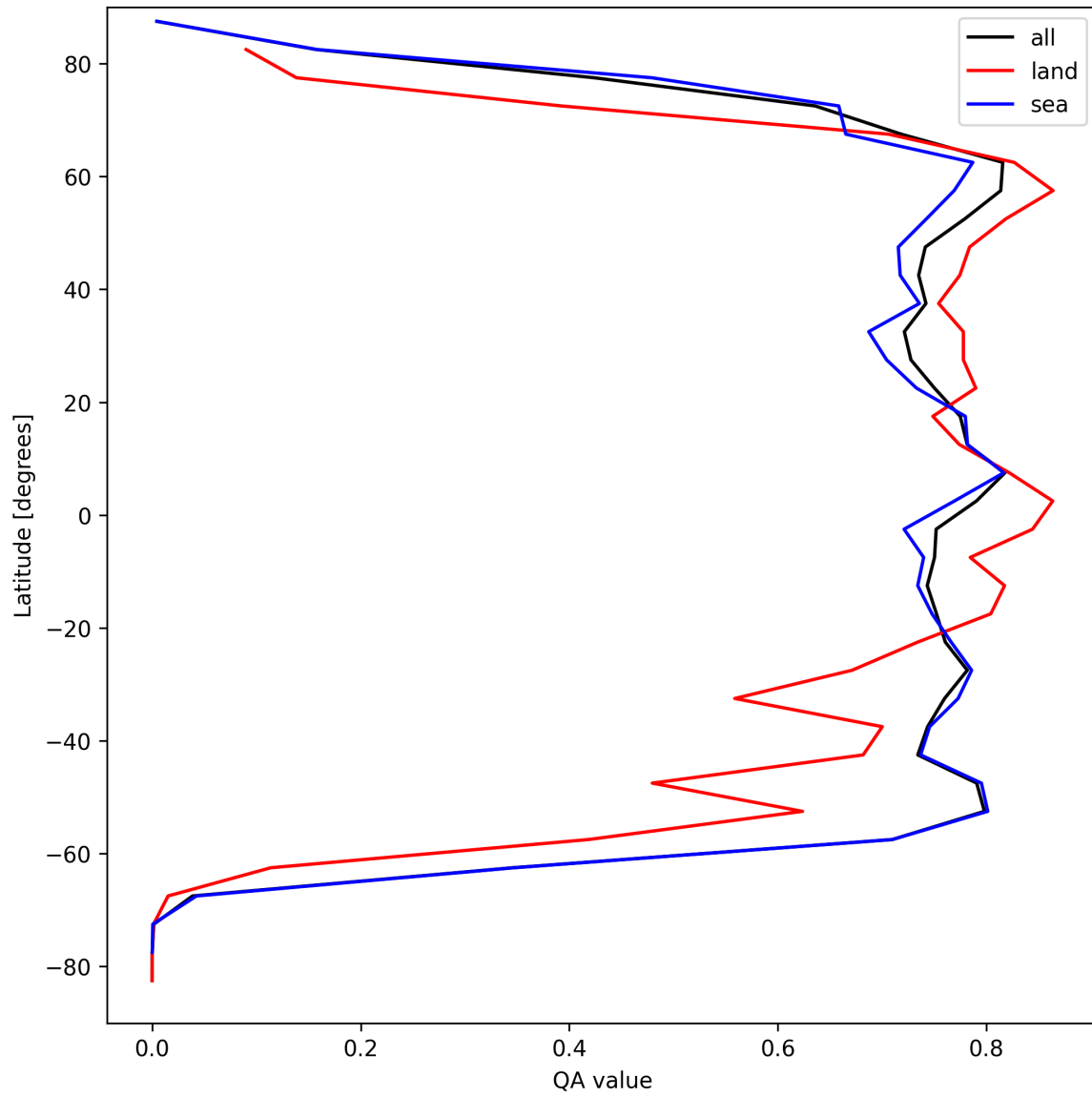
Figure 22: Zonal average of “QA value” for 2024-09-01 to 2024-09-03.
