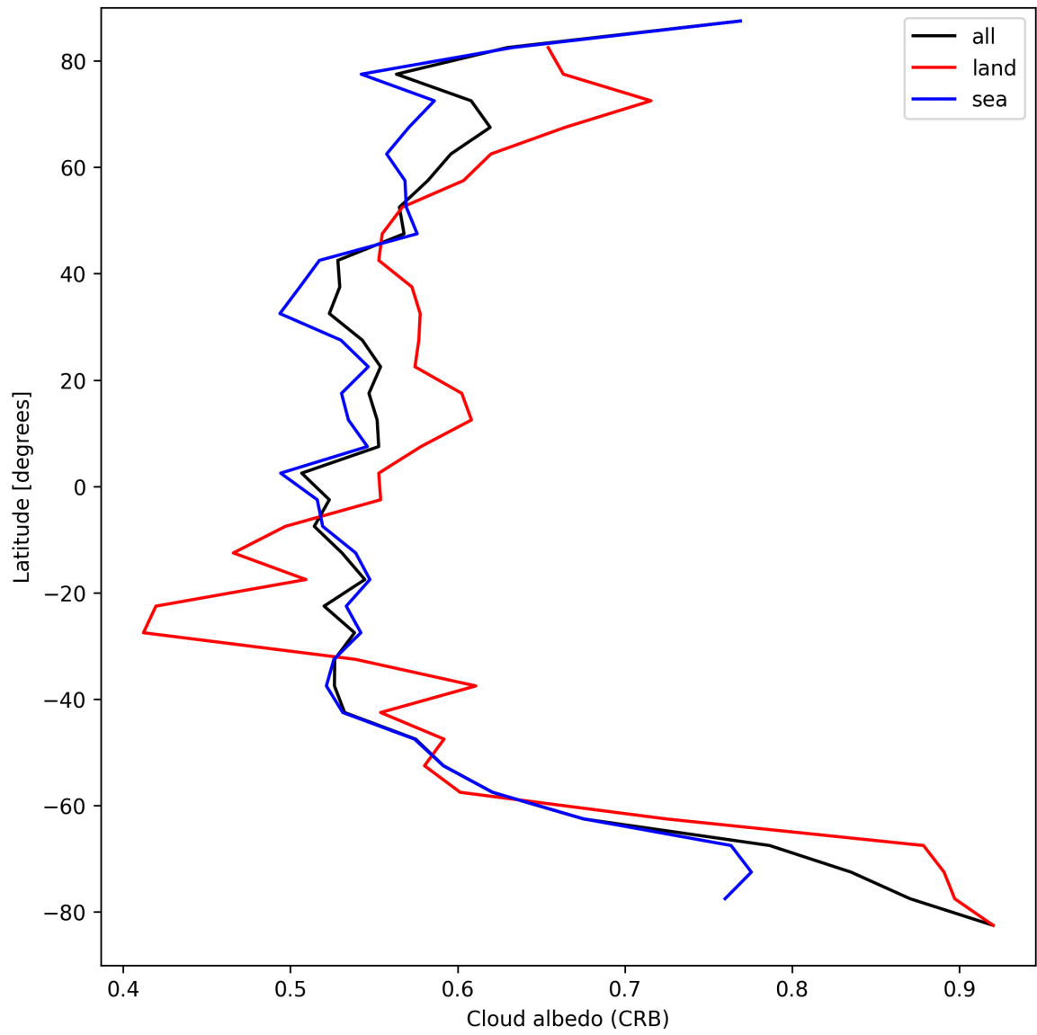
Figure 28: Zonal average of “Cloud albedo (CRB)” for 2024-09-01 to 2024-09-03.
