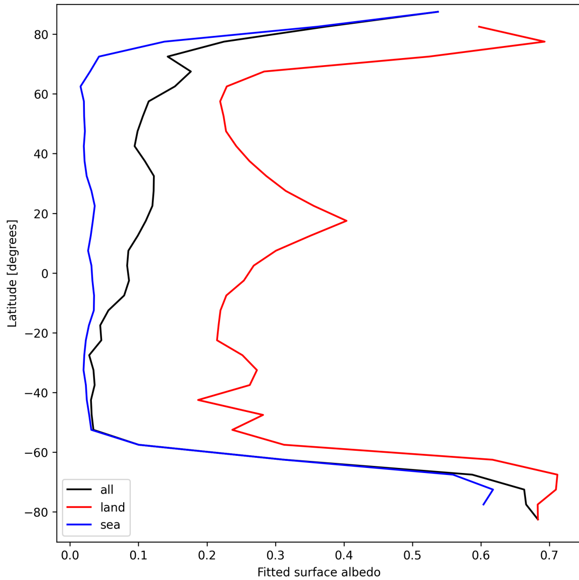
Figure 29: Zonal average of “Fitted surface albedo” for 2024-09-01 to 2024-09-03.
