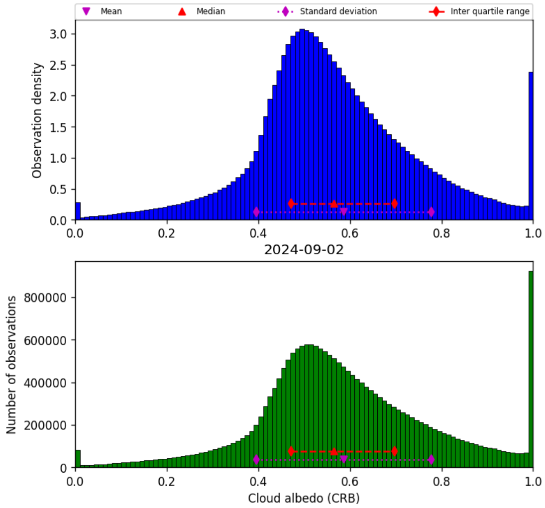
Figure 44: Histogram of “Cloud albedo (CRB)” for 2024-09-01 to 2024-09-03
