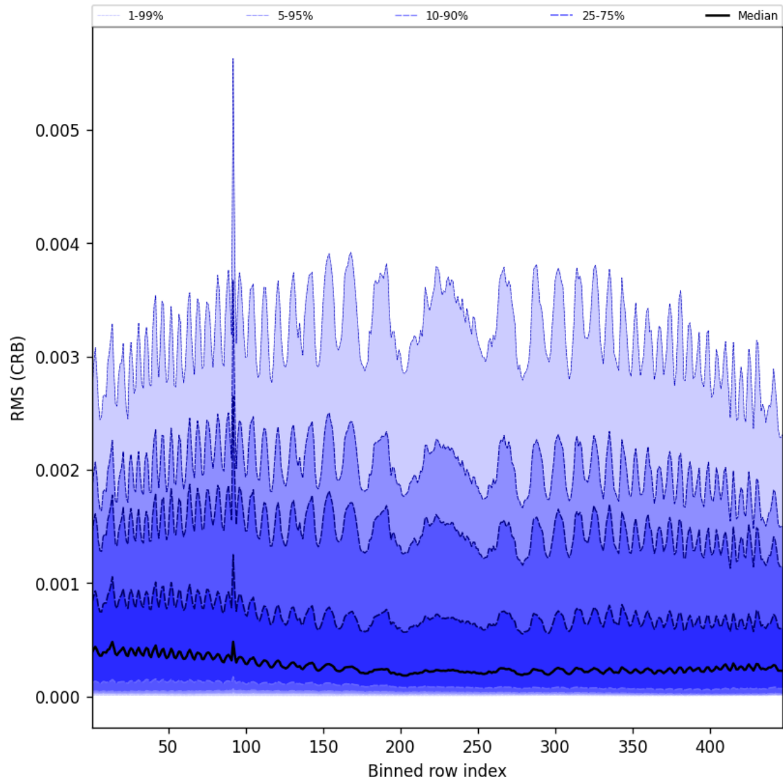
Figure 64: Along track statistics of “RMS (CRB)” for 2024-09-01 to 2024-09-03
