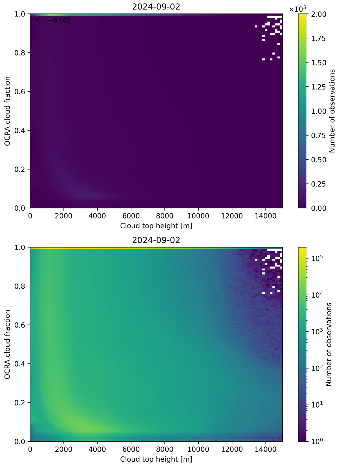
Figure 87: Scatter density plot of “Cloud top height” against “OCRA cloud fraction” for 2024-09-01 to 2024-09-03.
