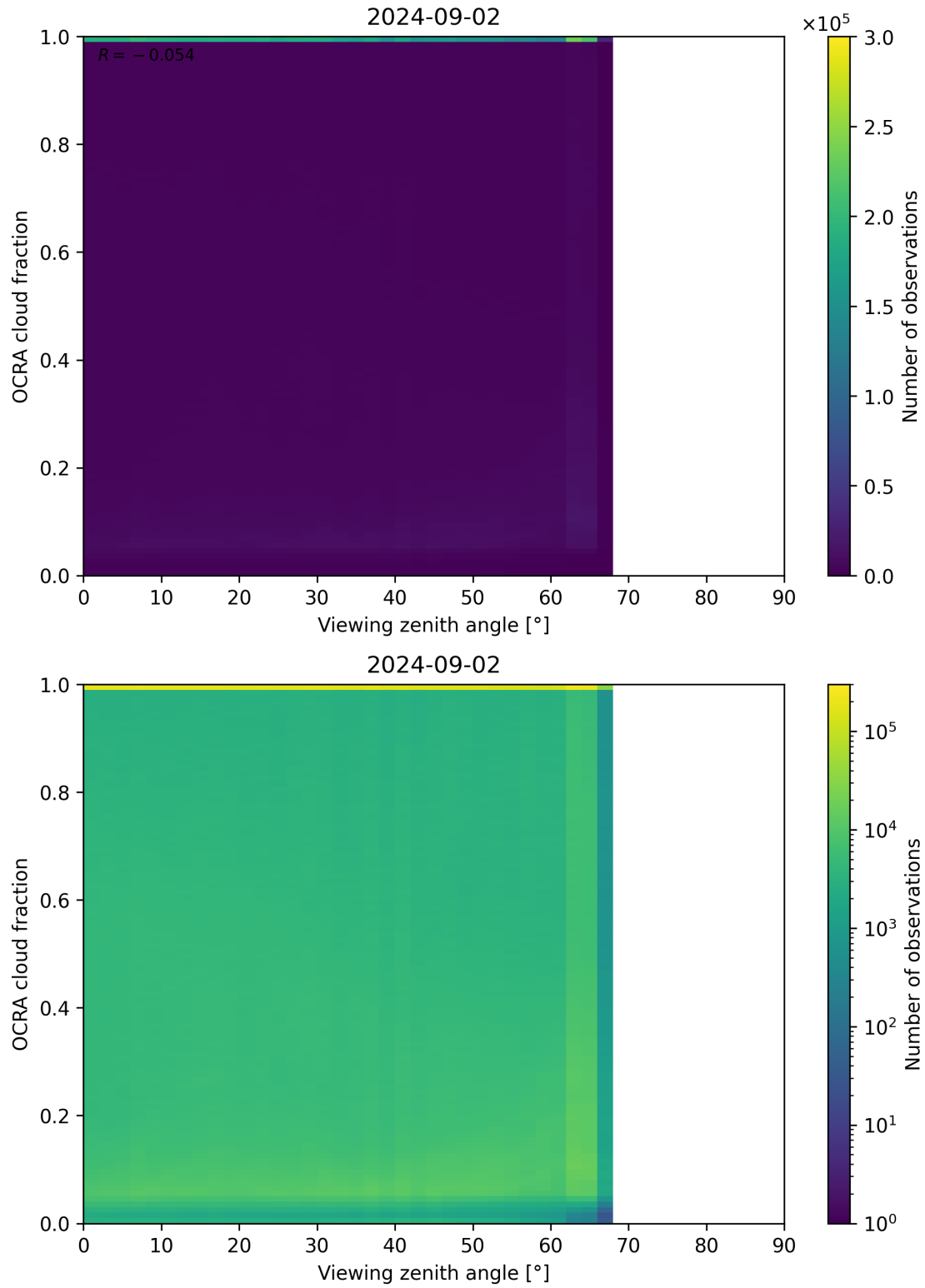
Figure 108: Scatter density plot of “Viewing zenith angle” against “OCRA cloud fraction” for 2024-09-01 to 2024-09-03.
