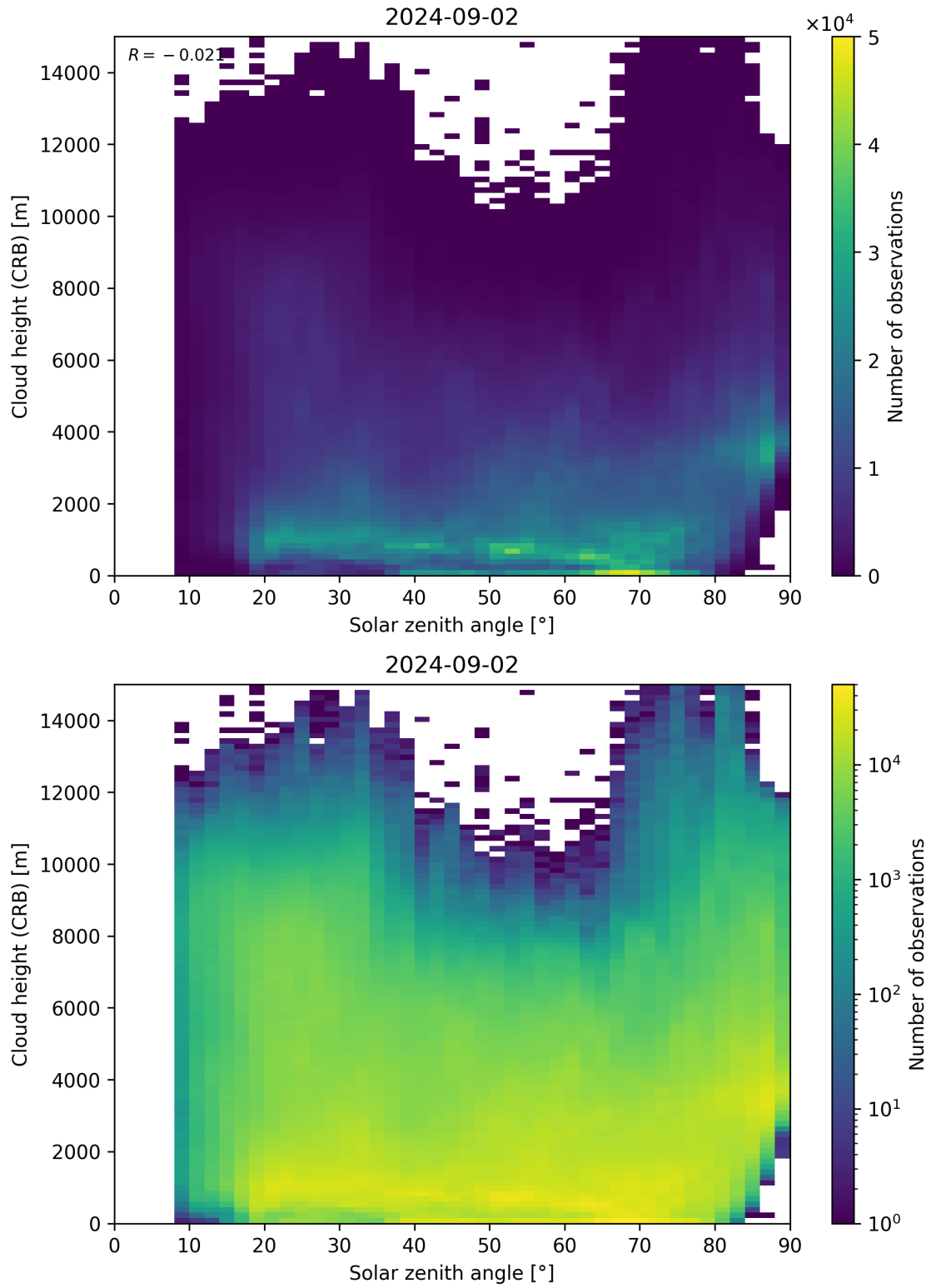
Figure 102: Scatter density plot of “Solar zenith angle” against “Cloud height (CRB)” for 2024-09-01 to 2024-09-03.
