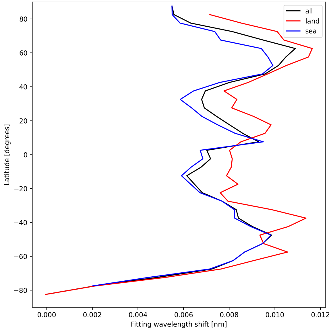
Figure 33: Zonal average of “Fitting wavelength shift” for 2024-09-01 to 2024-09-03.
