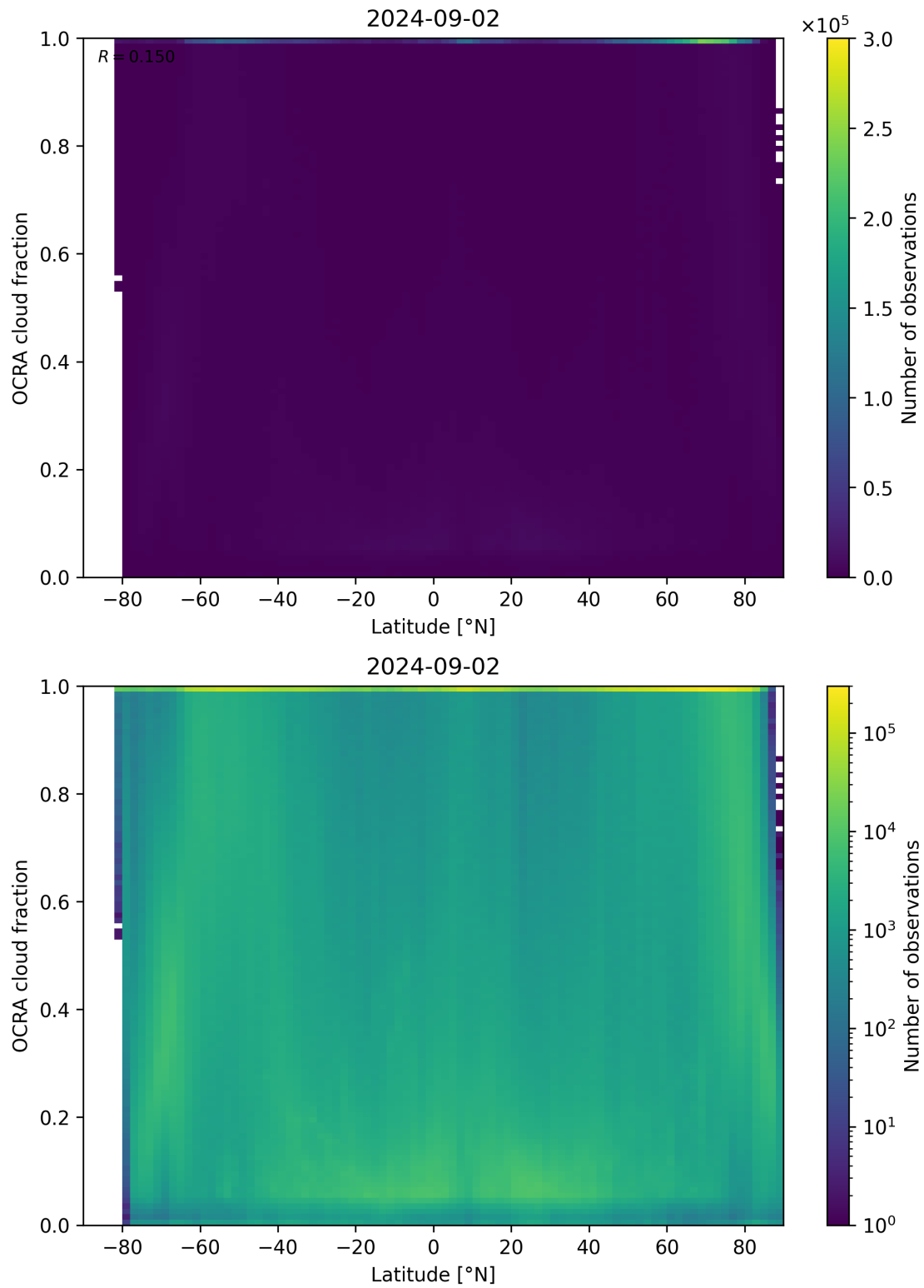
Figure 93: Scatter density plot of “Latitude” against “OCRA cloud fraction” for 2024-09-01 to 2024-09-03.
