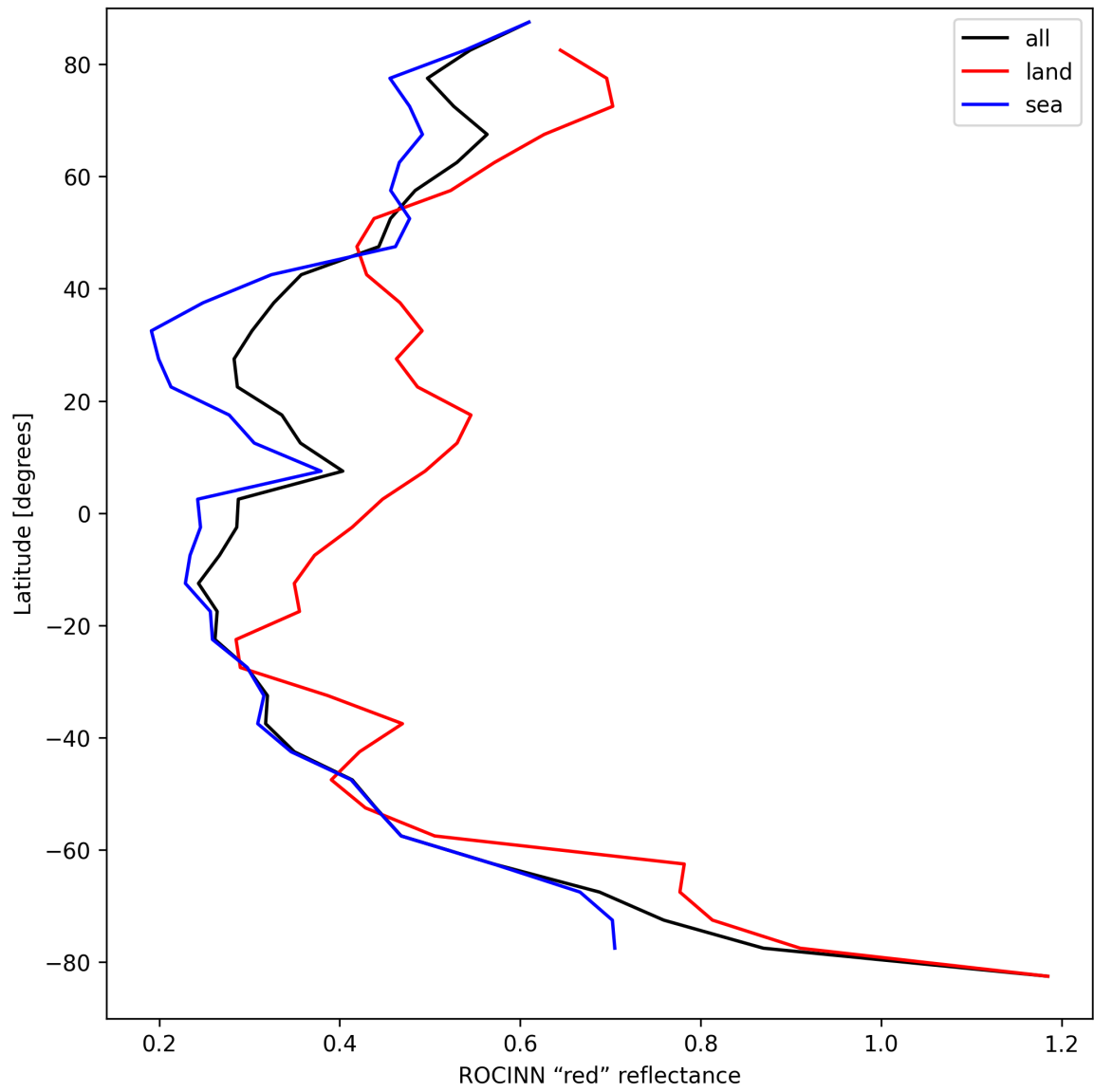
Figure 37: Zonal average of "ROCINN "red" reflectance" for 2024-09-01 to 2024-09-03.
