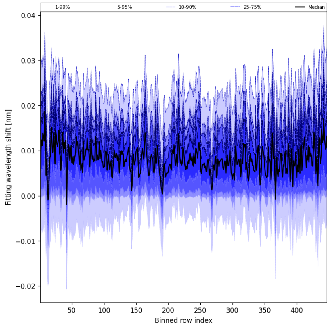
Figure 65: Along track statistics of “Fitting wavelength shift” for 2024-09-01 to 2024-09-03
