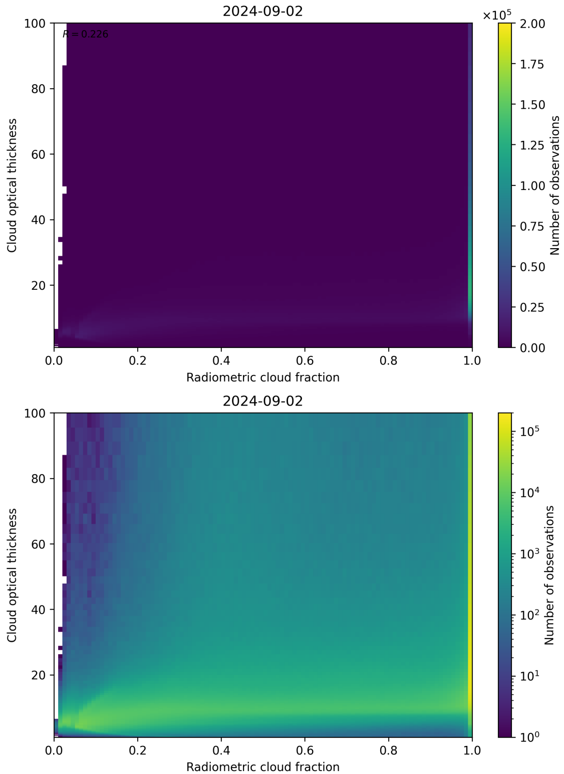
Figure 75: Scatter density plot of “Radiometric cloud fraction” against “Cloud optical thickness” for 2024-09-01 to 2024-09-03.
