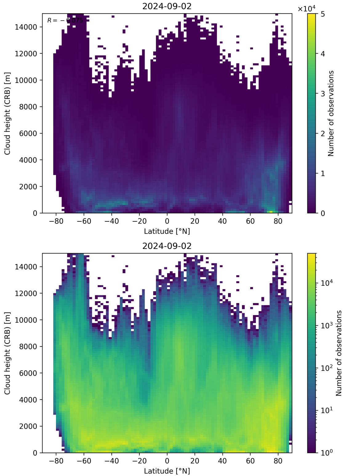
Figure 95: Scatter density plot of “Latitude” against “Cloud height (CRB)” for 2024-09-01 to 2024-09-03.
