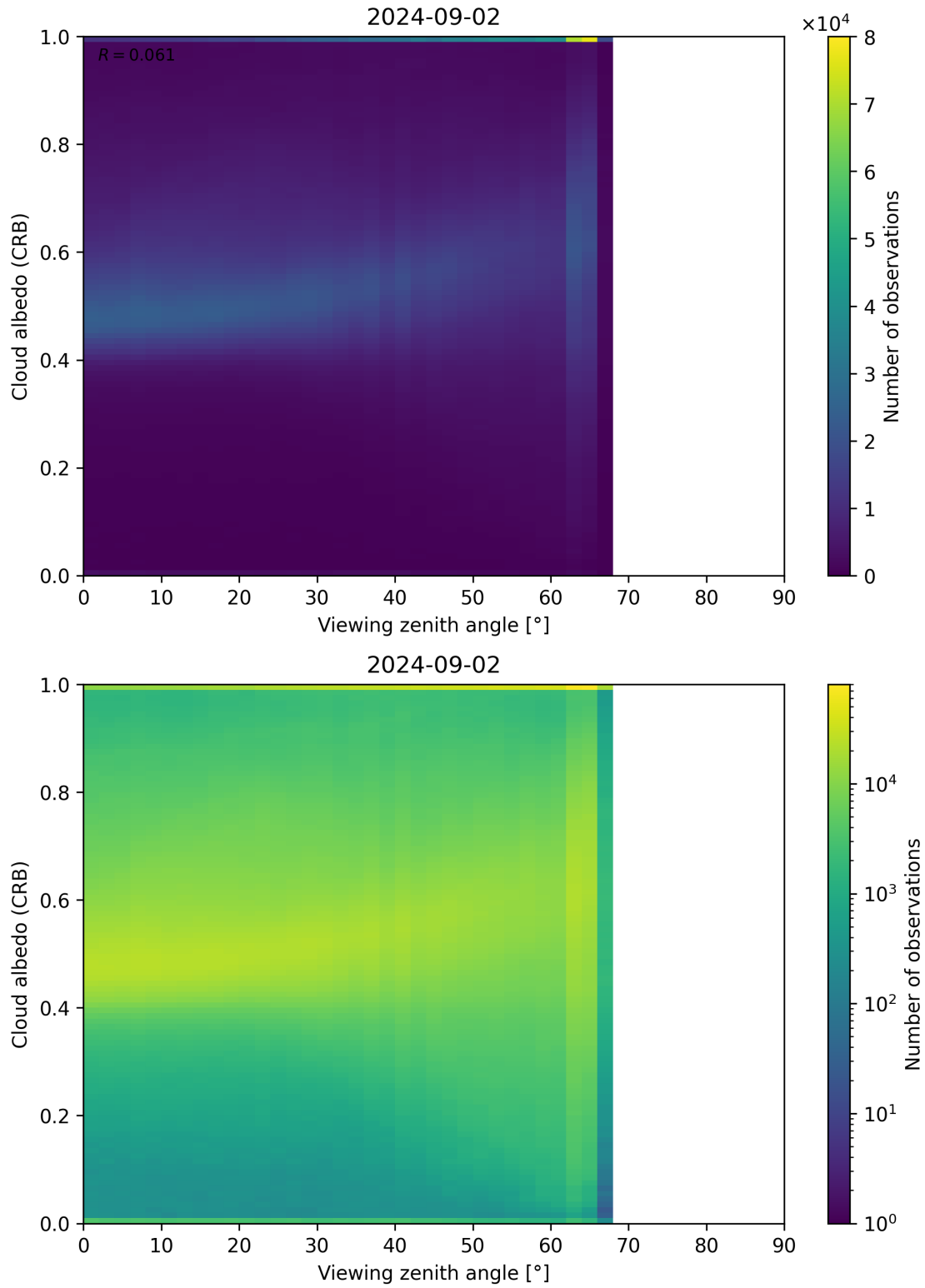
Figure 106: Scatter density plot of “Viewing zenith angle” against “Cloud albedo (CRB)” for 2024-09-01 to 2024-09-03.
