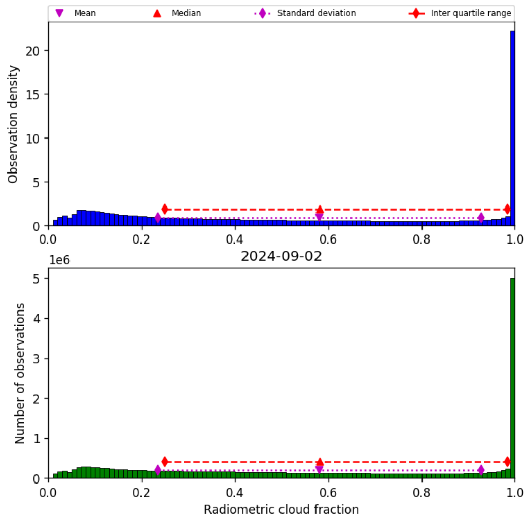
Figure 39: Histogram of “Radiometric cloud fraction” for 2024-09-01 to 2024-09-03
