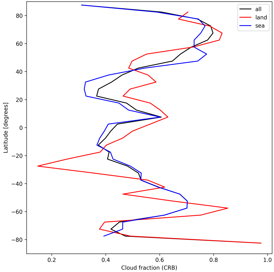
Figure 26: Zonal average of “Cloud fraction (CRB)” for 2024-09-01 to 2024-09-03.
