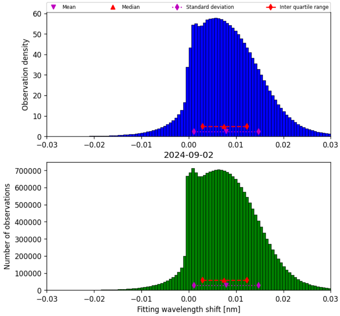
Figure 49: Histogram of “Fitting wavelength shift” for 2024-09-01 to 2024-09-03
