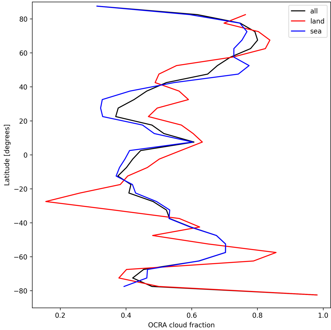
Figure 34: Zonal average of “OCRA cloud fraction” for 2024-09-01 to 2024-09-03.
