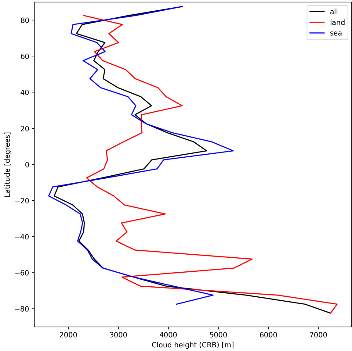
Figure 27: Zonal average of “Cloud height (CRB)” for 2024-09-01 to 2024-09-03.
