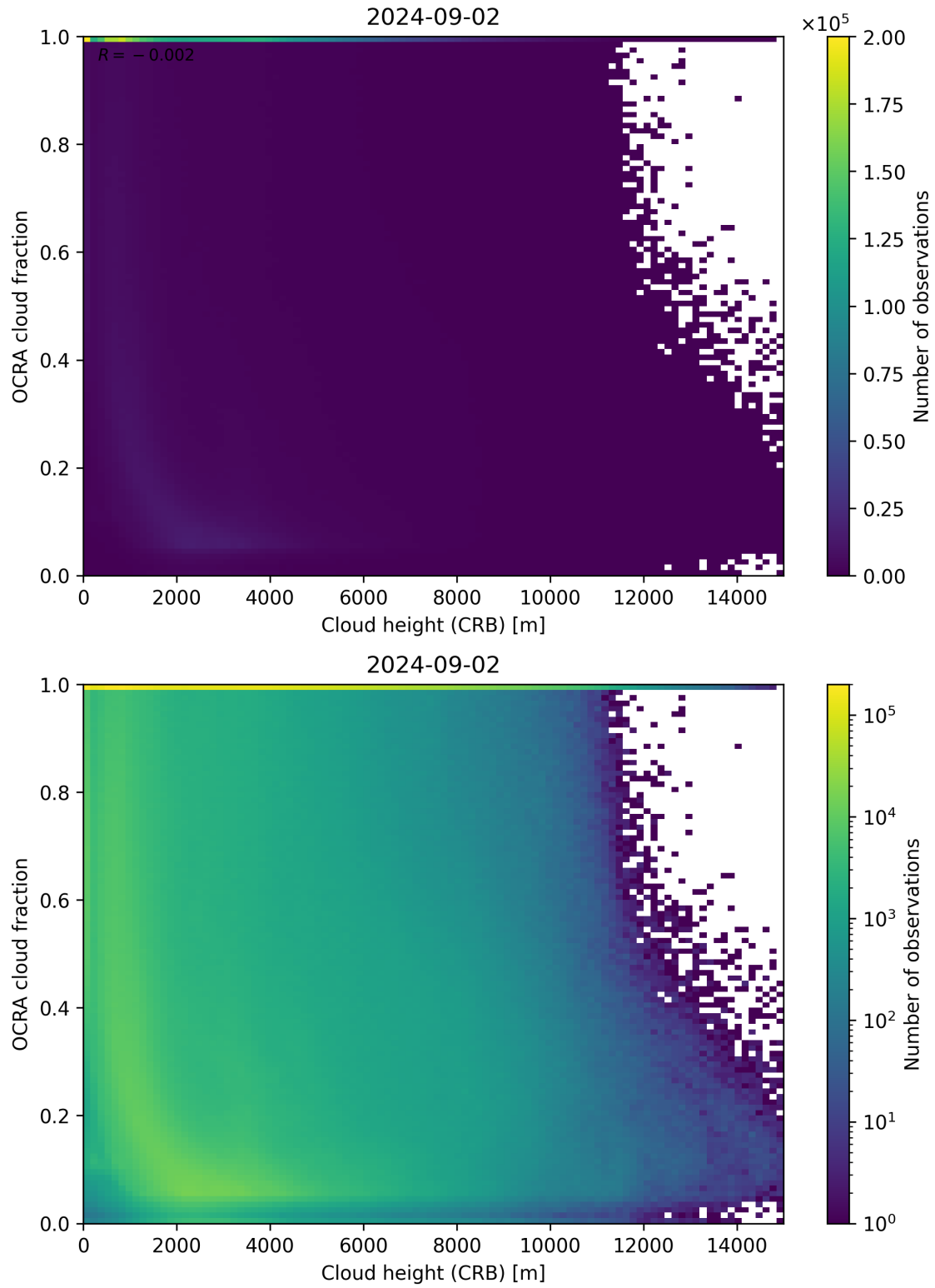
Figure 81: Scatter density plot of “Cloud height (CRB)” against “OCRA cloud fraction” for 2024-09-01 to 2024-09-03.
