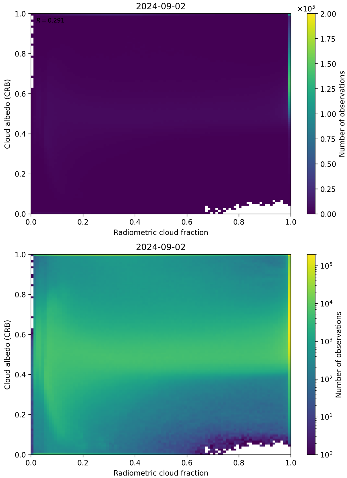
Figure 71: Scatter density plot of “Radiometric cloud fraction” against “Cloud albedo (CRB)” for 2024-09-01 to 2024-09-03.
