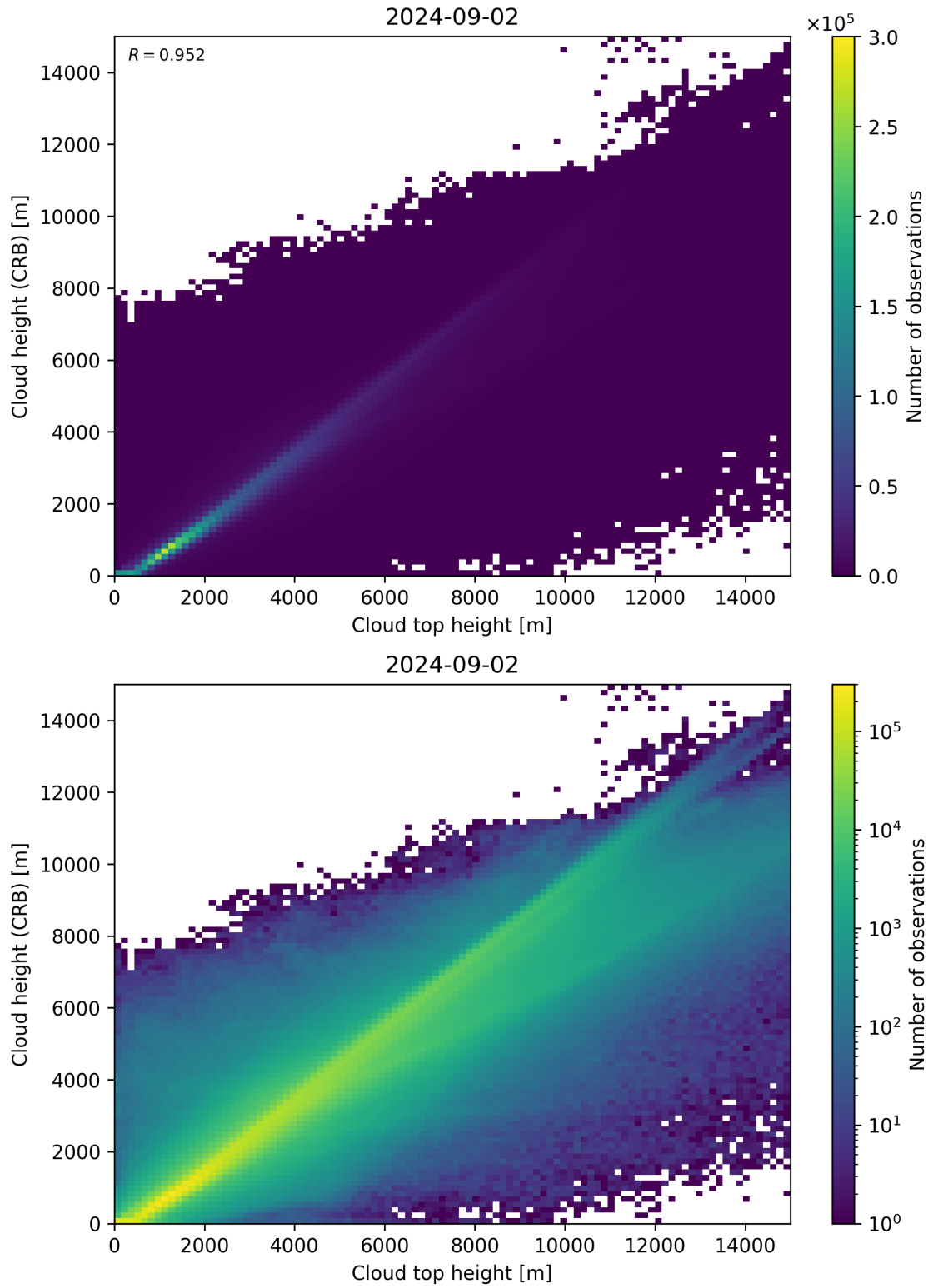
Figure 89: Scatter density plot of “Cloud top height” against “Cloud height (CRB)” for 2024-09-01 to 2024-09-03.
