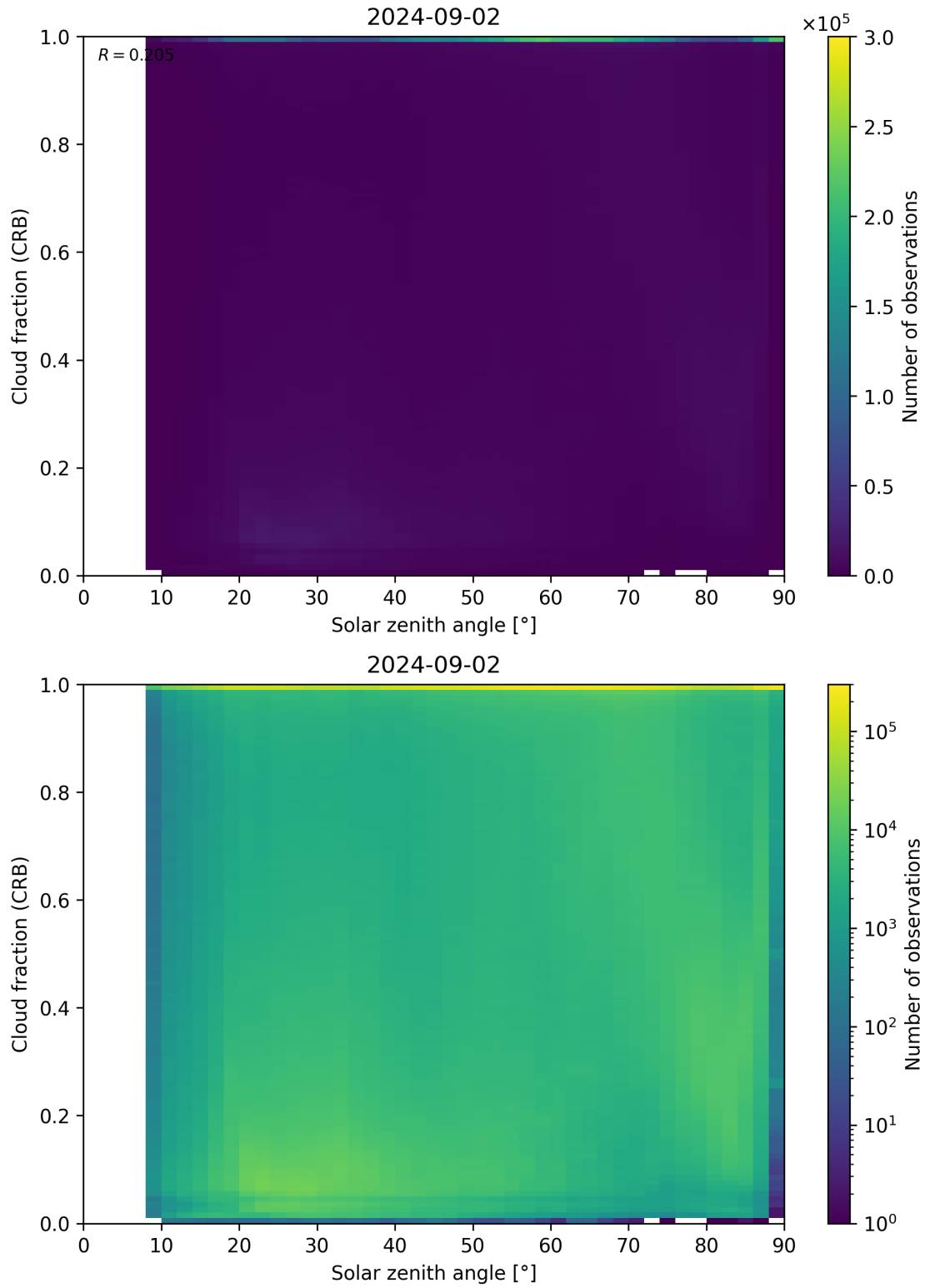
Figure 101: Scatter density plot of “Solar zenith angle” against “Cloud fraction (CRB)” for 2024-09-01 to 2024-09-03.
