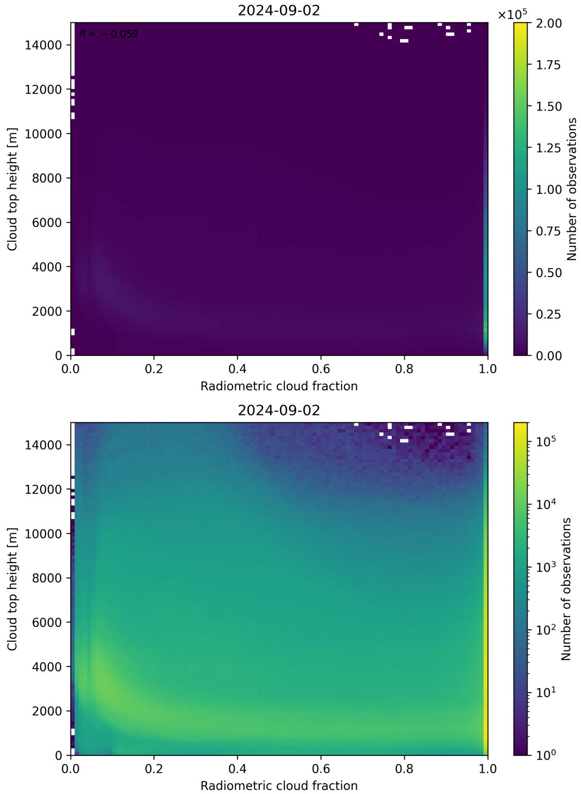
Figure 76: Scatter density plot of “Radiometric cloud fraction” against “Cloud top height” for 2024-09-01 to 2024-09-03.
