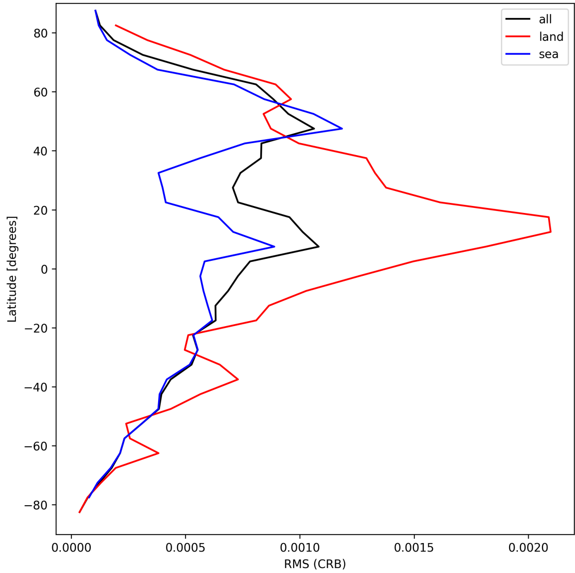
Figure 32: Zonal average of “RMS (CRB)” for 2024-09-01 to 2024-09-03.
