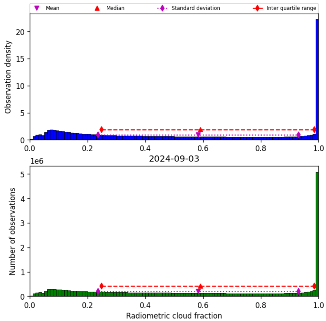
Figure 39: Histogram of “Radiometric cloud fraction” for 2024-09-02 to 2024-09-04
