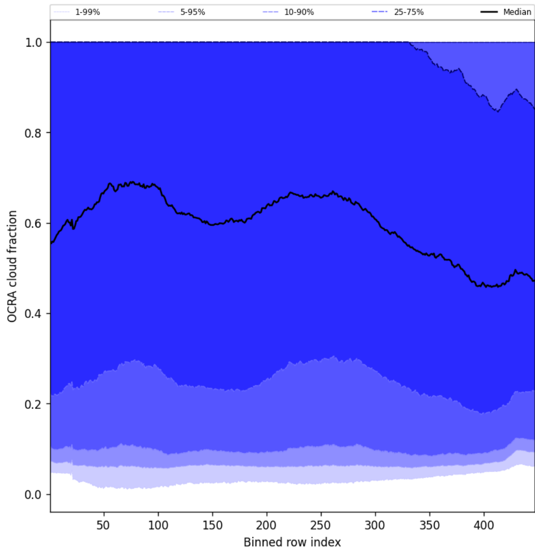
Figure 66: Along track statistics of “OCRA cloud fraction” for 2024-09-02 to 2024-09-04
