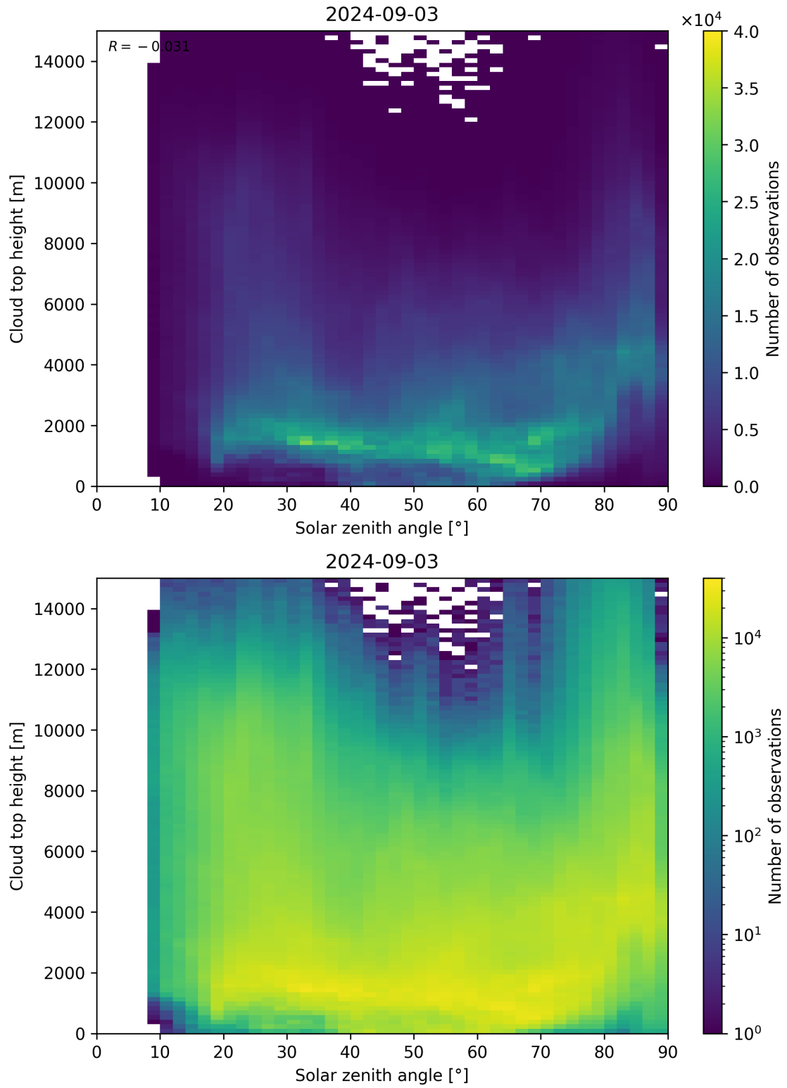
Figure 104: Scatter density plot of “Solar zenith angle” against “Cloud top height” for 2024-09-02 to 2024-09-04.
