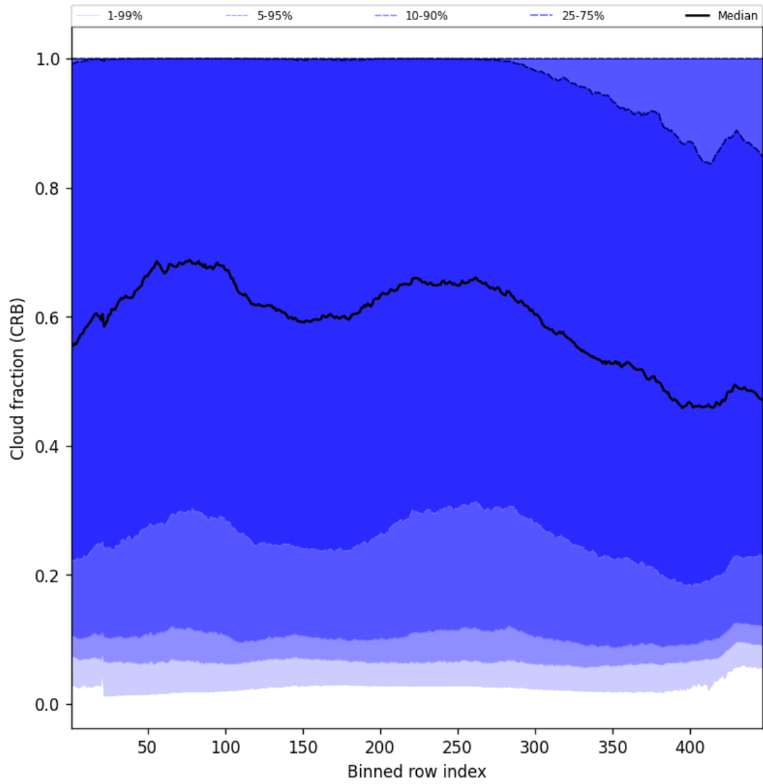
Figure 58: Along track statistics of “Cloud fraction (CRB)” for 2024-09-02 to 2024-09-04
