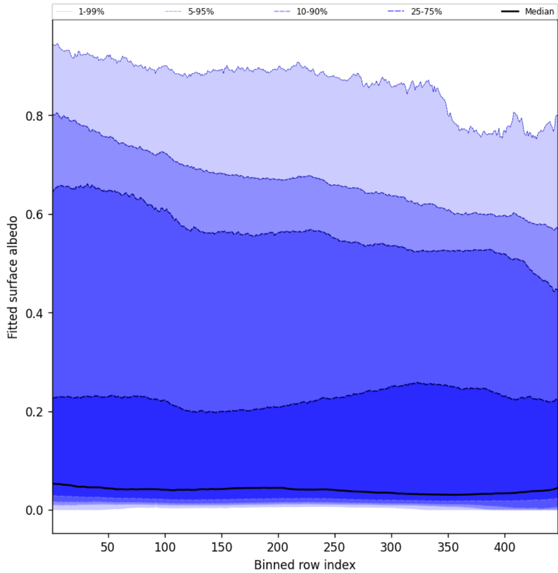
Figure 61: Along track statistics of “Fitted surface albedo” for 2024-09-02 to 2024-09-04
