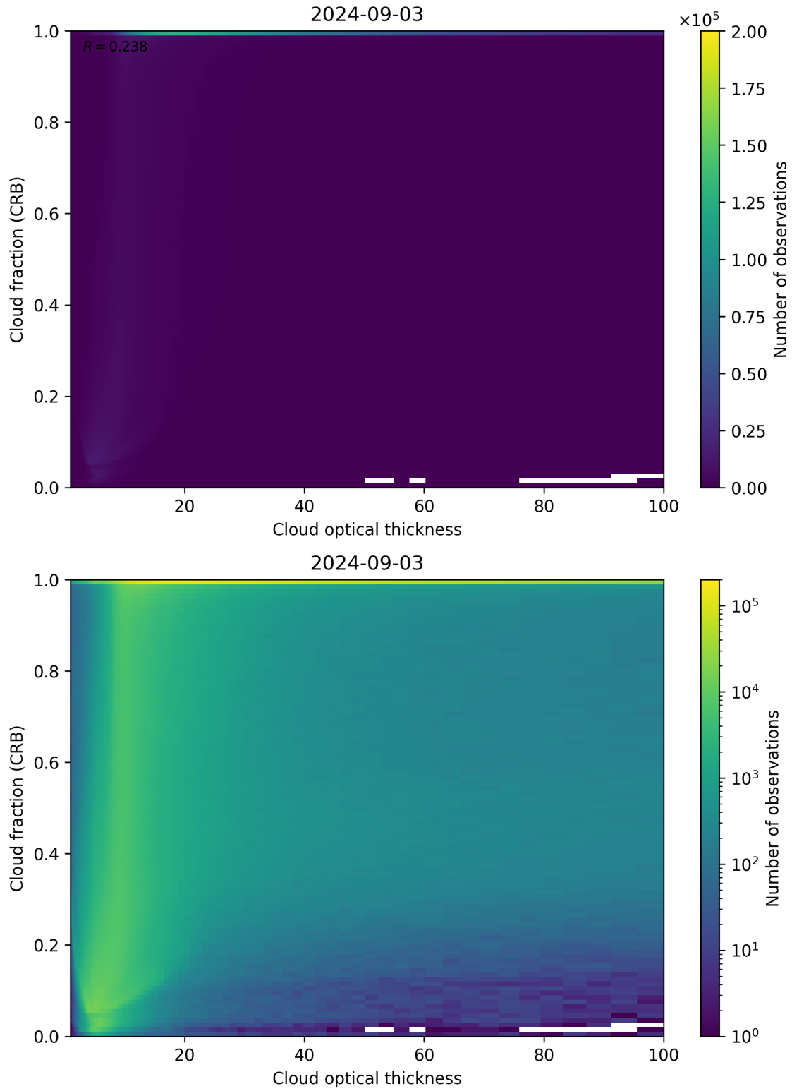
Figure 84: Scatter density plot of “Cloud optical thickness” against “Cloud fraction (CRB)” for 2024-09-02 to 2024-09-04.
