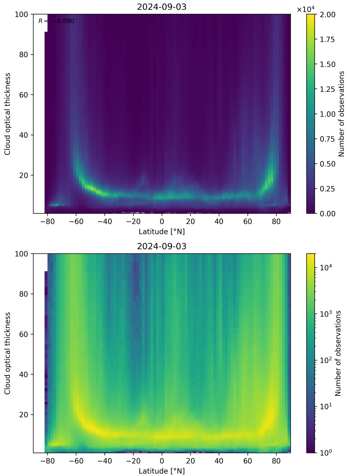
Figure 96: Scatter density plot of “Latitude” against “Cloud optical thickness” for 2024-09-02 to 2024-09-04.
