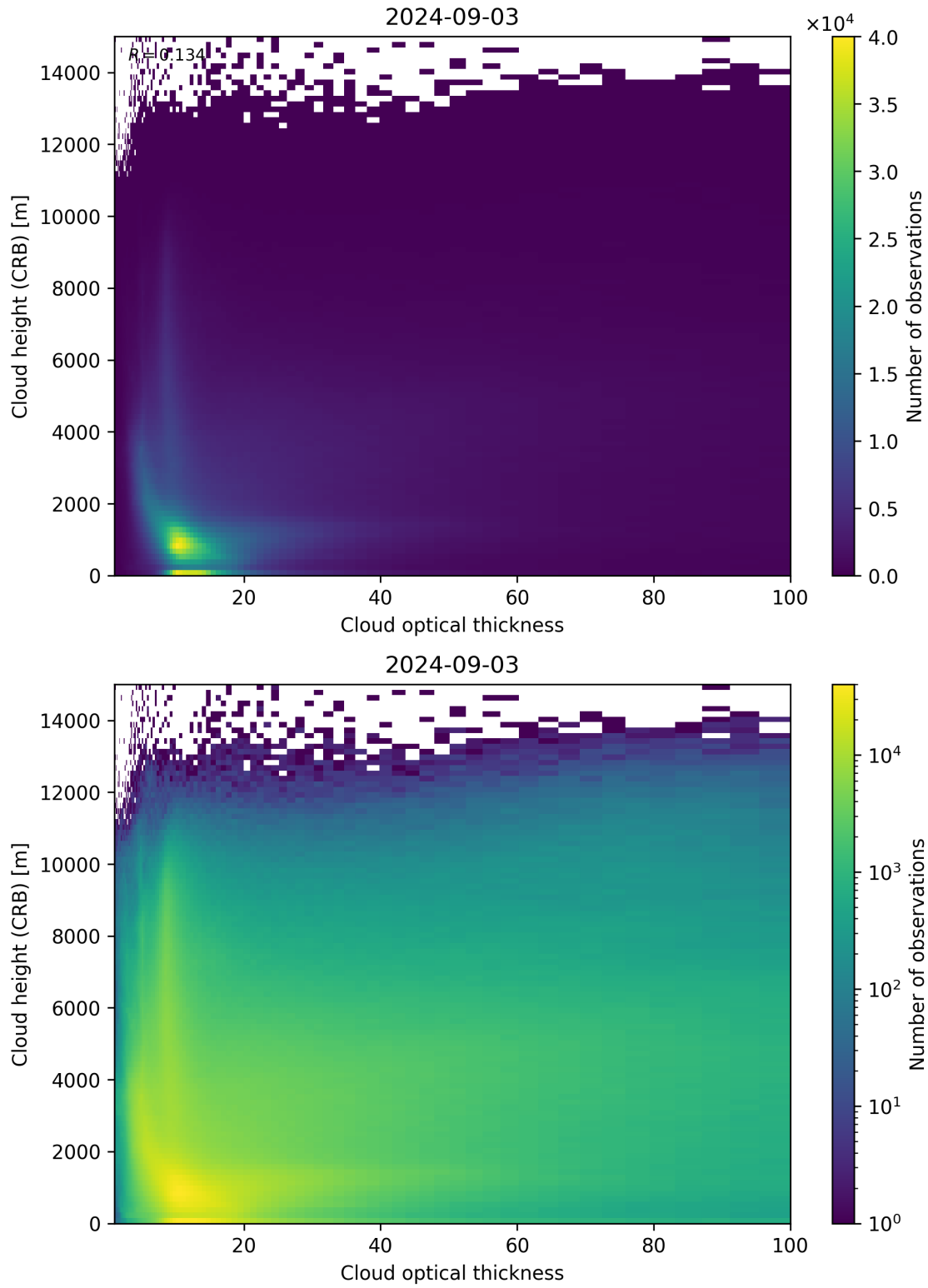
Figure 85: Scatter density plot of “Cloud optical thickness” against “Cloud height (CRB)” for 2024-09-02 to 2024-09-04.
