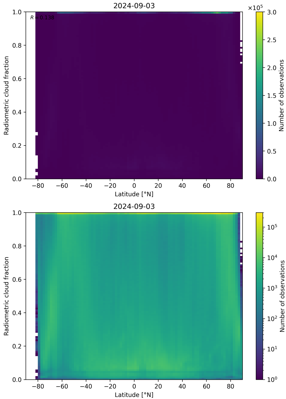
Figure 92: Scatter density plot of “Latitude” against “Radiometric cloud fraction” for 2024-09-02 to 2024-09-04.
