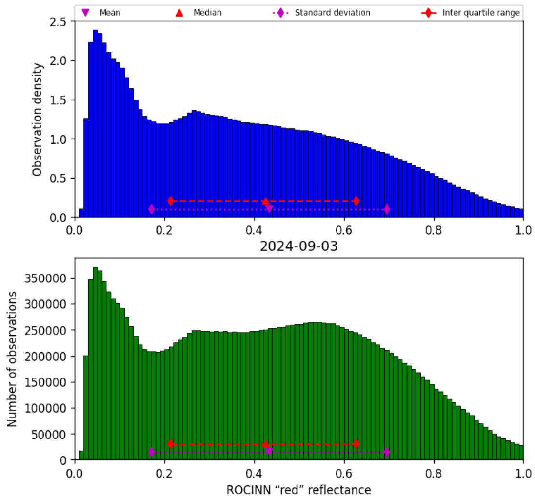
Figure 53: Histogram of “ROCINN “red” reflectance” for 2024-09-02 to 2024-09-04
