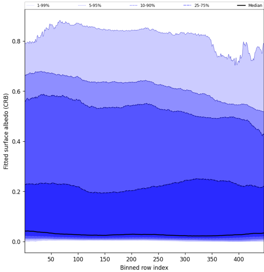
Figure 62: Along track statistics of “Fitted surface albedo (CRB)” for 2024-09-02 to 2024-09-04
