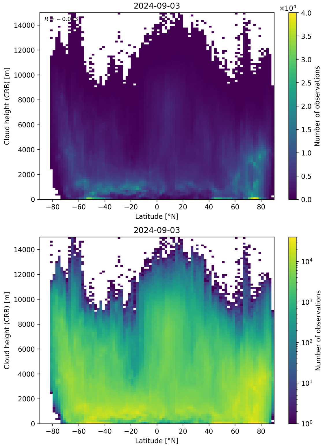
Figure 95: Scatter density plot of “Latitude” against “Cloud height (CRB)” for 2024-09-02 to 2024-09-04.
