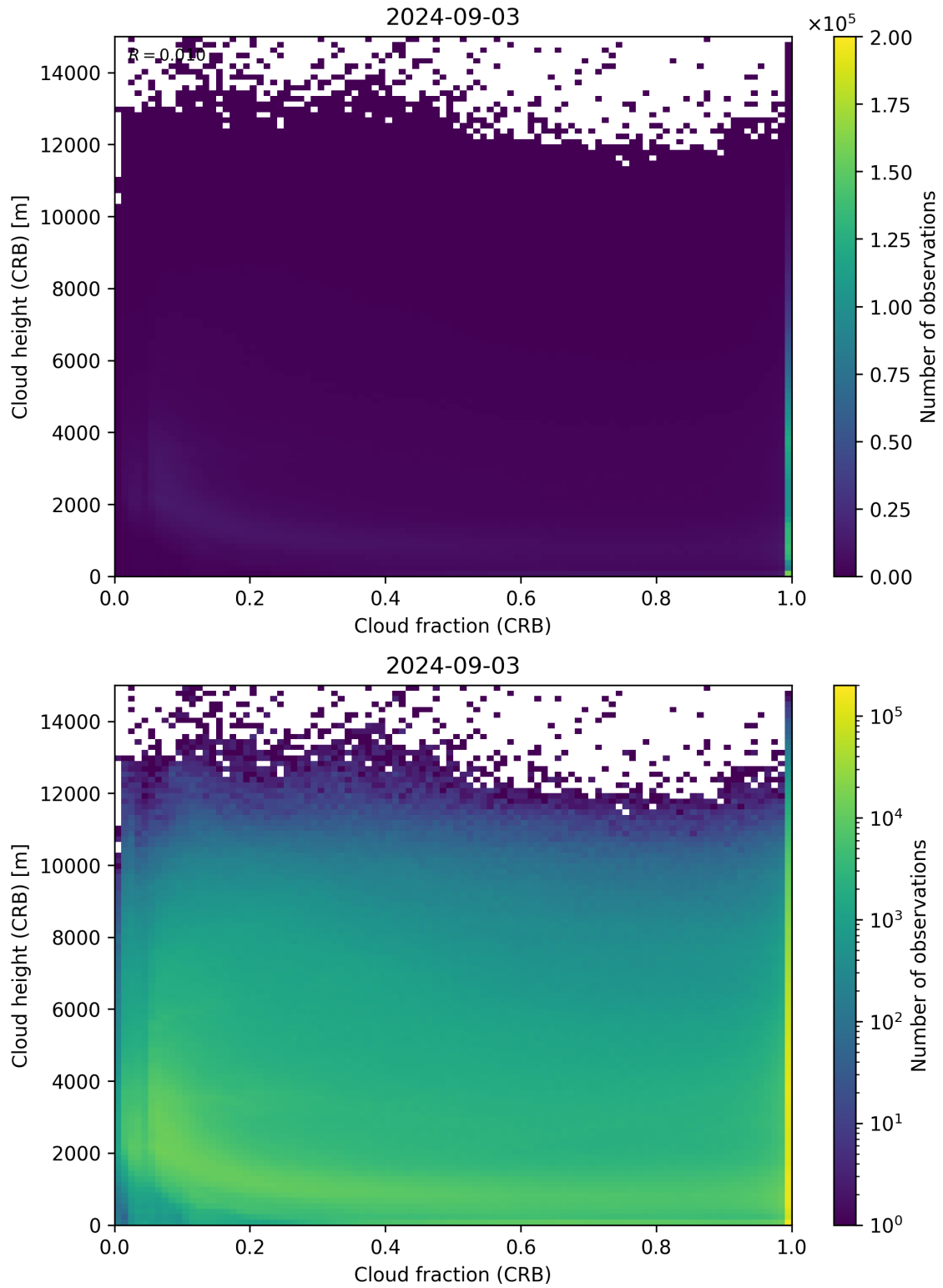
Figure 79: Scatter density plot of “Cloud fraction (CRB)” against “Cloud height (CRB)” for 2024-09-02 to 2024-09-04.
