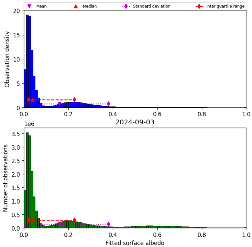
Figure 45: Histogram of “Fitted surface albedo” for 2024-09-02 to 2024-09-04
