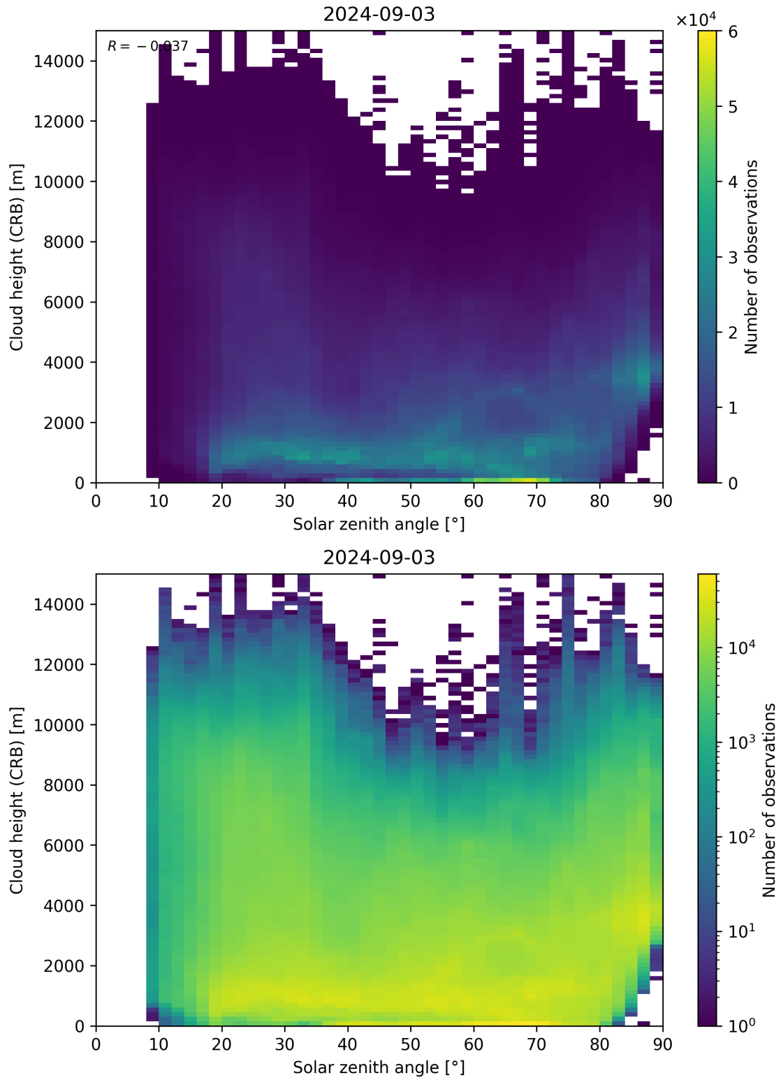
Figure 102: Scatter density plot of “Solar zenith angle” against “Cloud height (CRB)” for 2024-09-02 to 2024-09-04.
