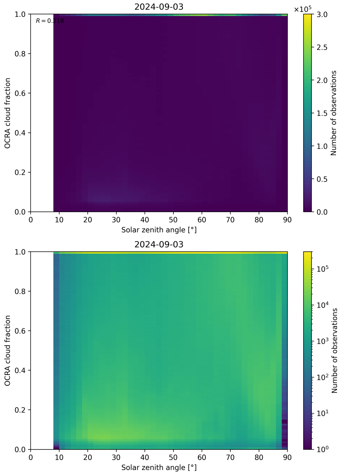
Figure 100: Scatter density plot of “Solar zenith angle” against “OCRA cloud fraction” for 2024-09-02 to 2024-09-04.
