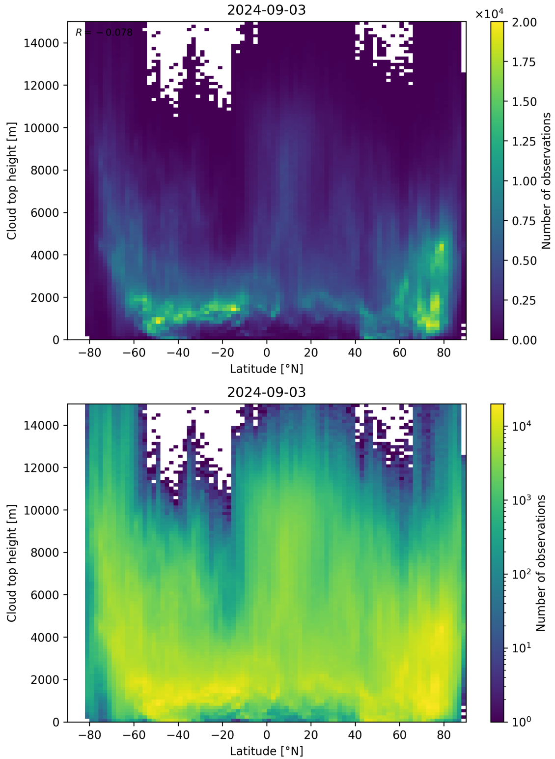
Figure 97: Scatter density plot of “Latitude” against “Cloud top height” for 2024-09-02 to 2024-09-04.
