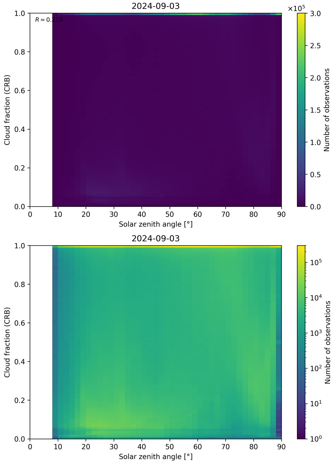
Figure 101: Scatter density plot of “Solar zenith angle” against “Cloud fraction (CRB)” for 2024-09-02 to 2024-09-04.
