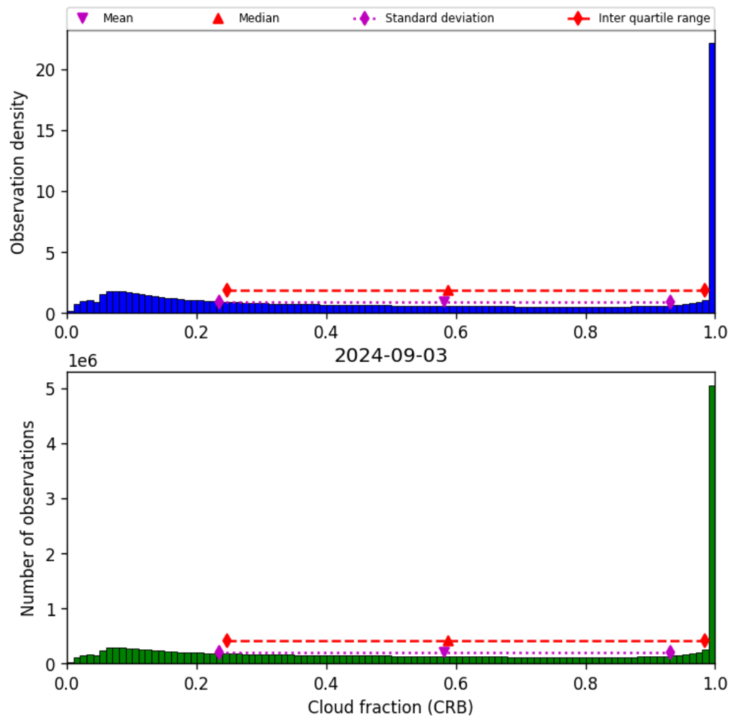
Figure 42: Histogram of “Cloud fraction (CRB)” for 2024-09-02 to 2024-09-04
