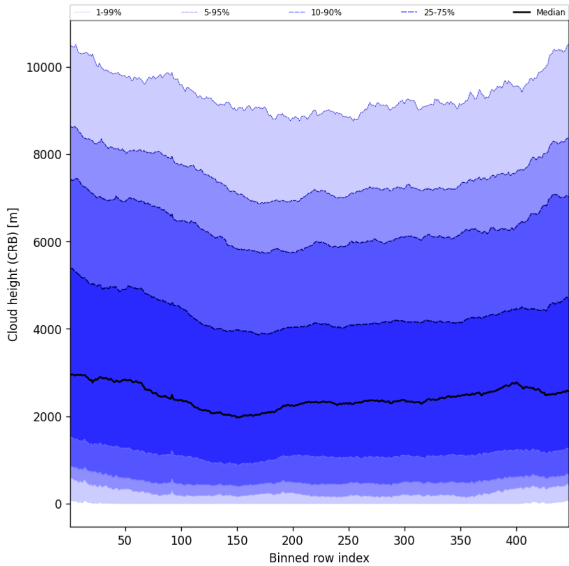
Figure 59: Along track statistics of “Cloud height (CRB)” for 2024-09-02 to 2024-09-04
