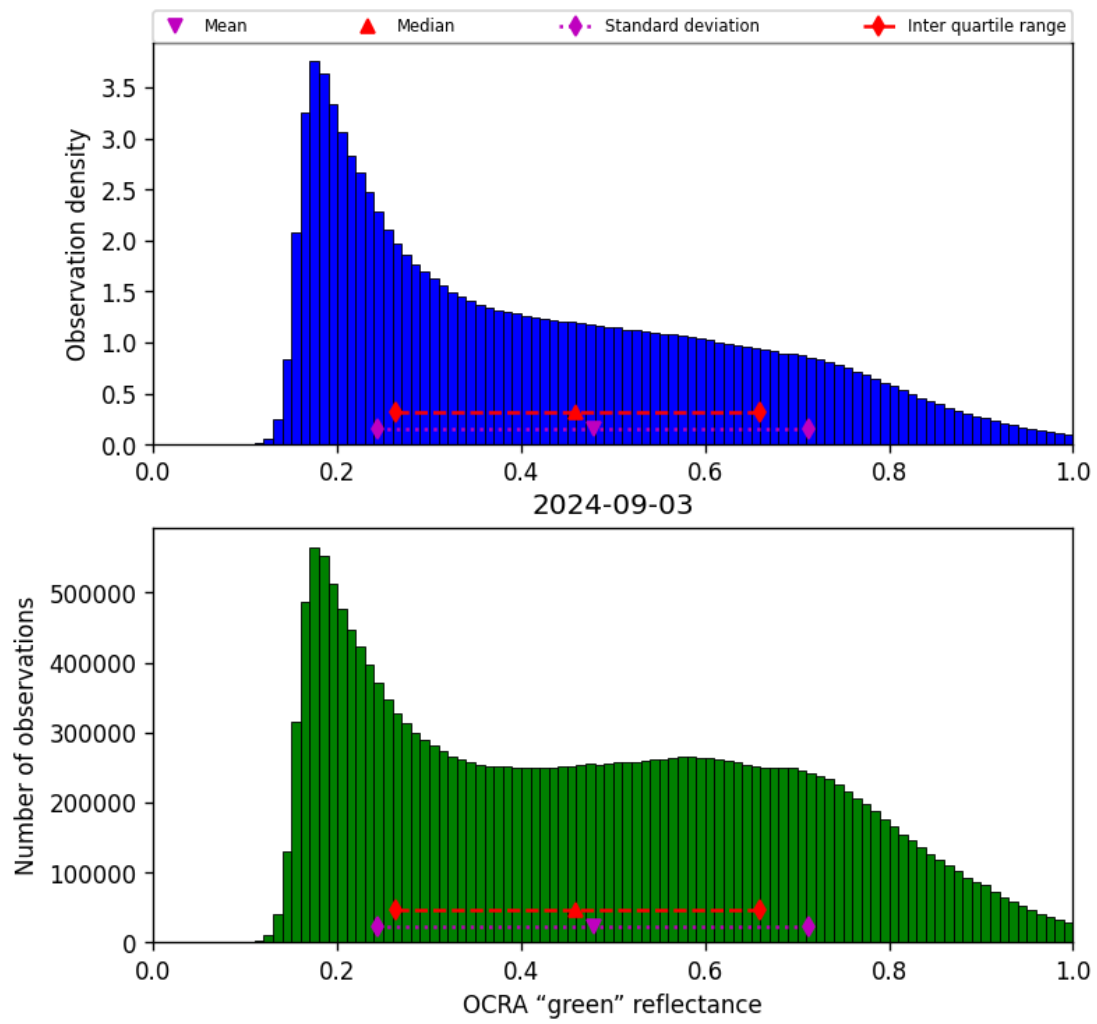
Figure 52: Histogram of “OCRA “green” reflectance” for 2024-09-02 to 2024-09-04
