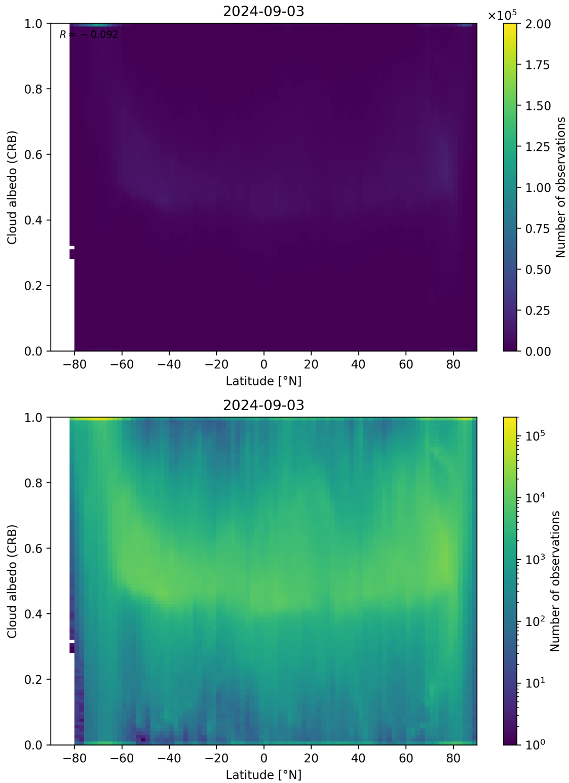
Figure 91: Scatter density plot of “Latitude” against “Cloud albedo (CRB)” for 2024-09-02 to 2024-09-04.
