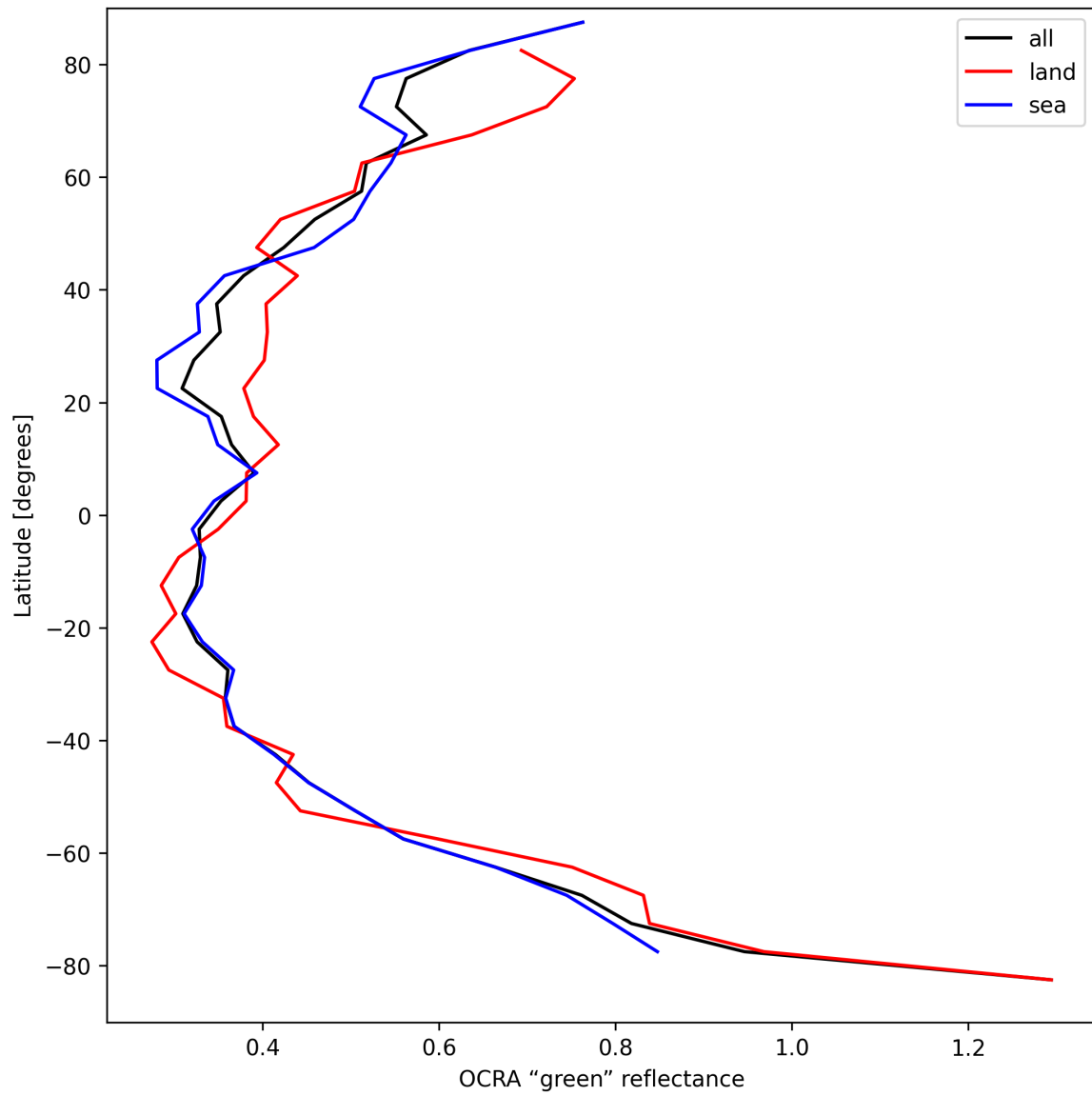
Figure 36: Zonal average of “OCRA “green” reflectance” for 2024-09-02 to 2024-09-04.
