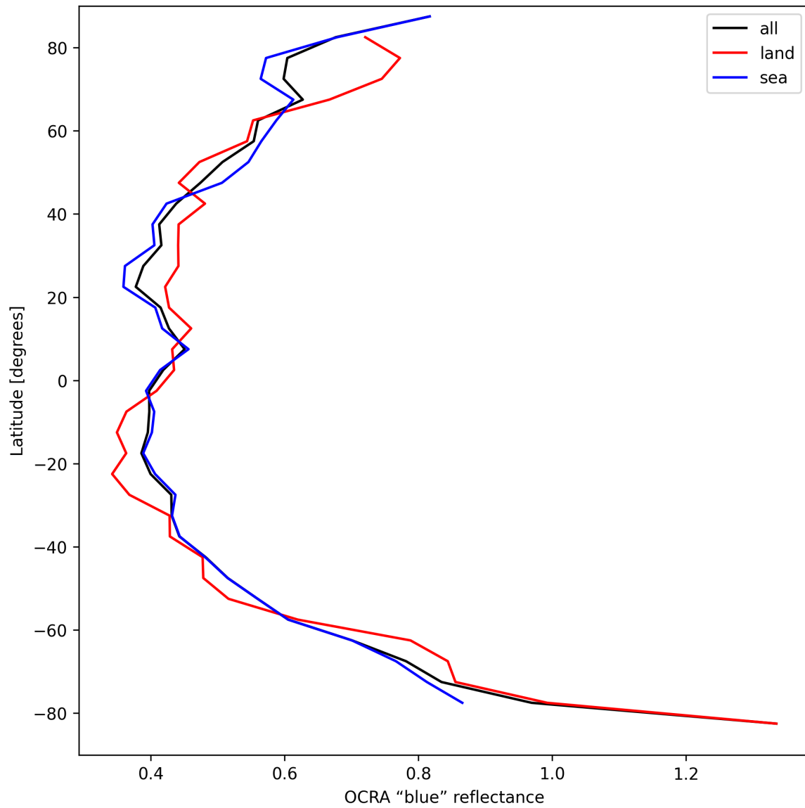
Figure 35: Zonal average of “OCRA “blue” reflectance” for 2024-09-02 to 2024-09-04.
