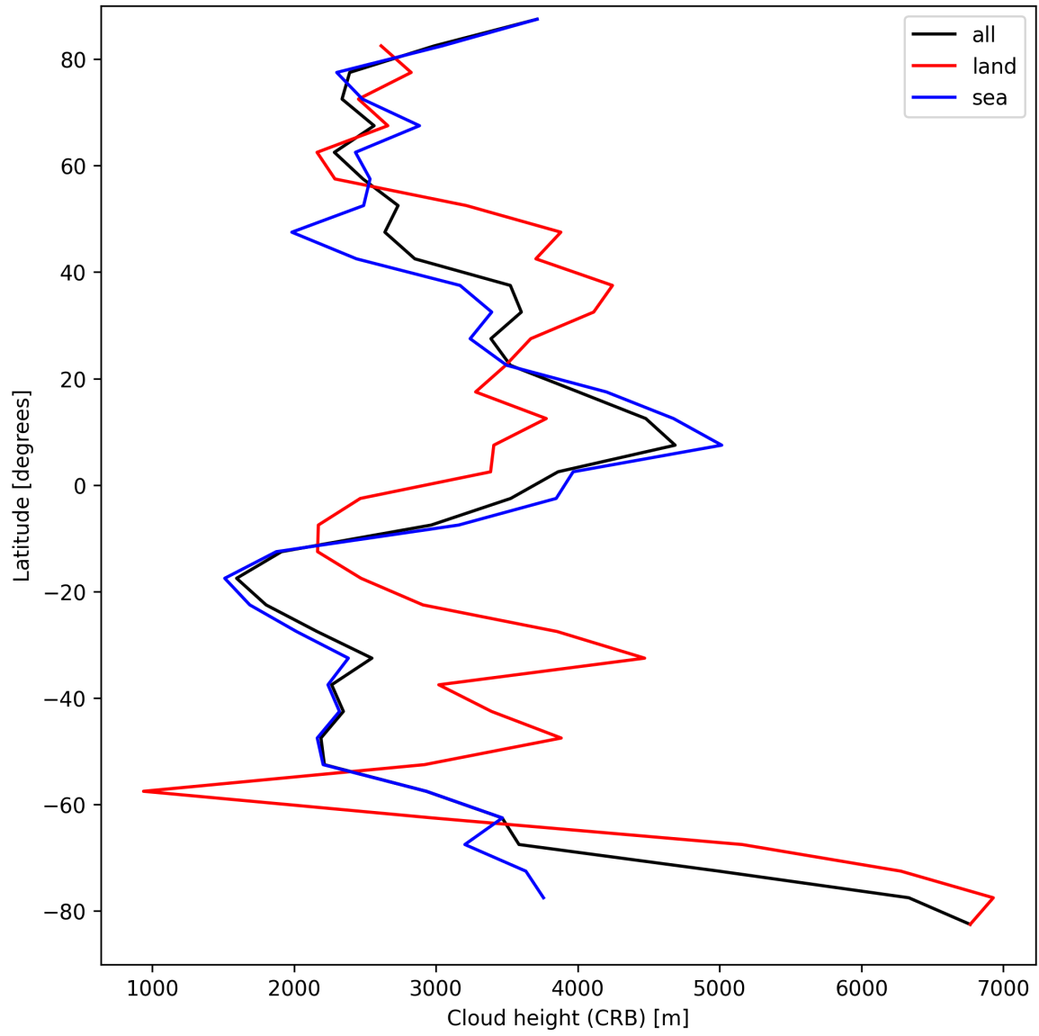
Figure 27: Zonal average of “Cloud height (CRB)” for 2024-09-02 to 2024-09-04.
