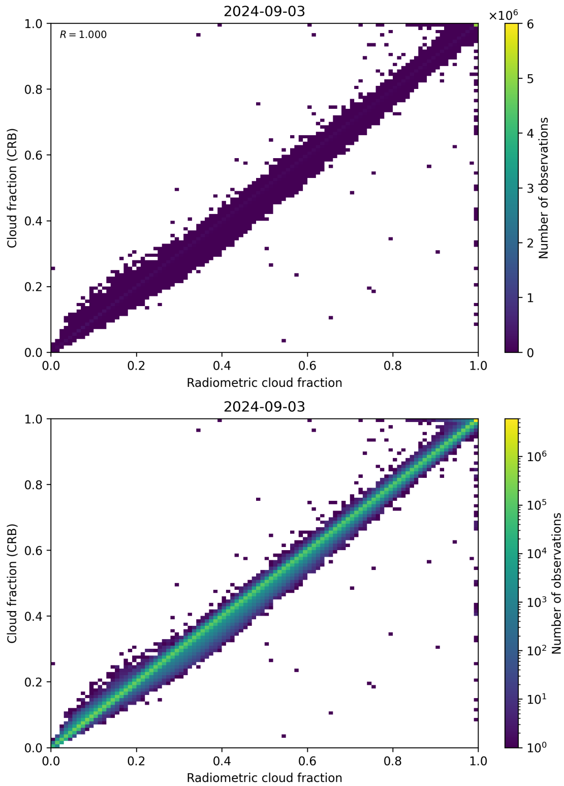
Figure 73: Scatter density plot of “Radiometric cloud fraction” against “Cloud fraction (CRB)” for 2024-09-02 to 2024-09-04.
