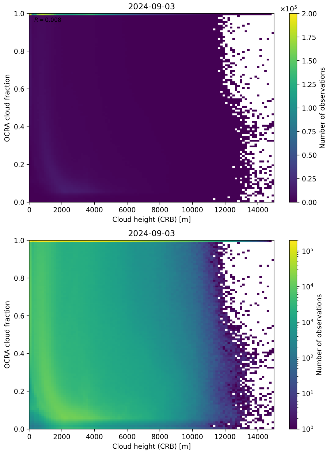
Figure 81: Scatter density plot of “Cloud height (CRB)” against “OCRA cloud fraction” for 2024-09-02 to 2024-09-04.
