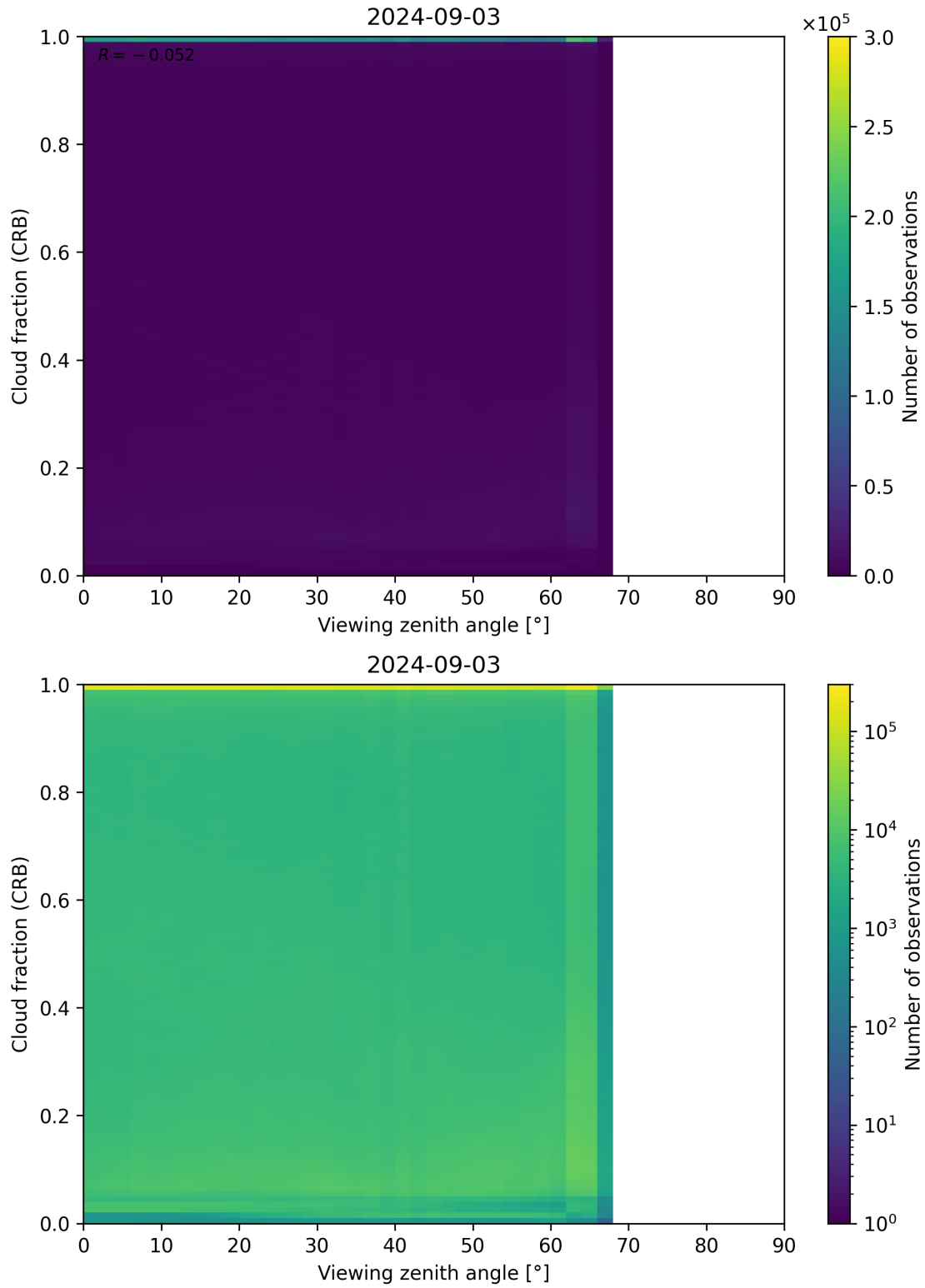
Figure 109: Scatter density plot of “Viewing zenith angle” against “Cloud fraction (CRB)” for 2024-09-02 to 2024-09-04.
