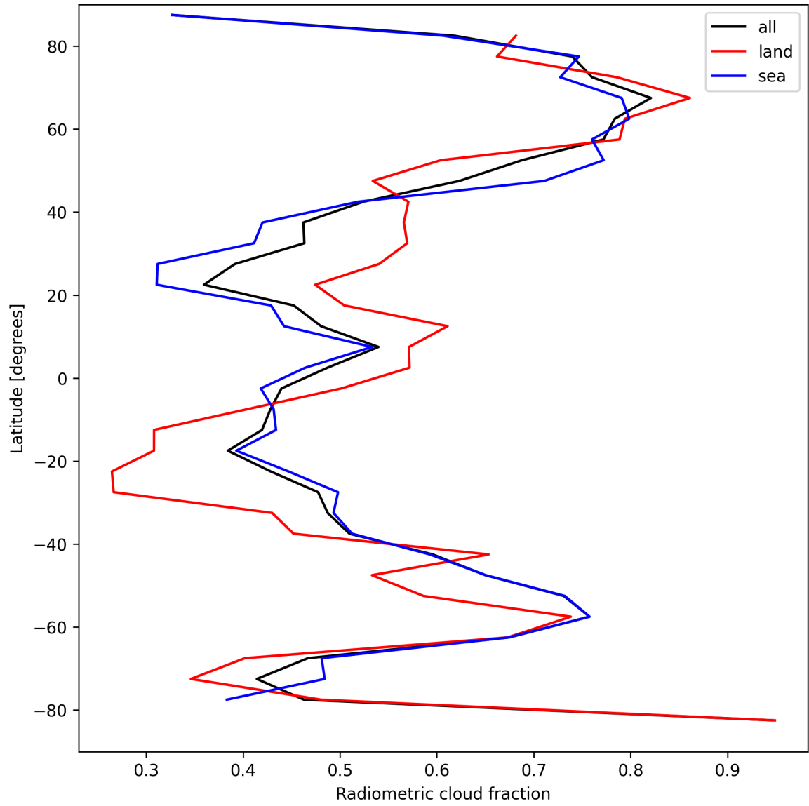
Figure 23: Zonal average of “Radiometric cloud fraction” for 2024-09-02 to 2024-09-04.
