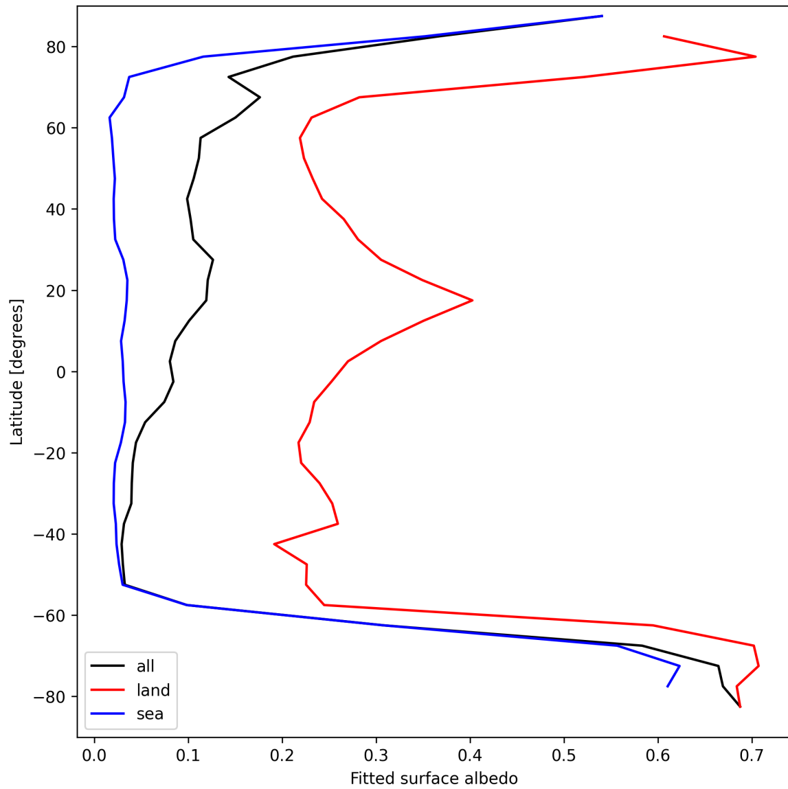
Figure 29: Zonal average of “Fitted surface albedo” for 2024-09-02 to 2024-09-04.
