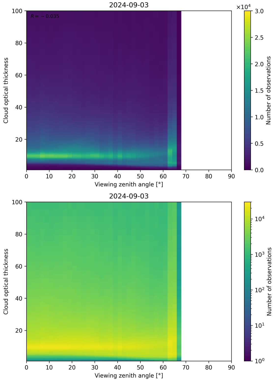
Figure 111: Scatter density plot of “Viewing zenith angle” against “Cloud optical thickness” for 2024-09-02 to 2024-09-04.
