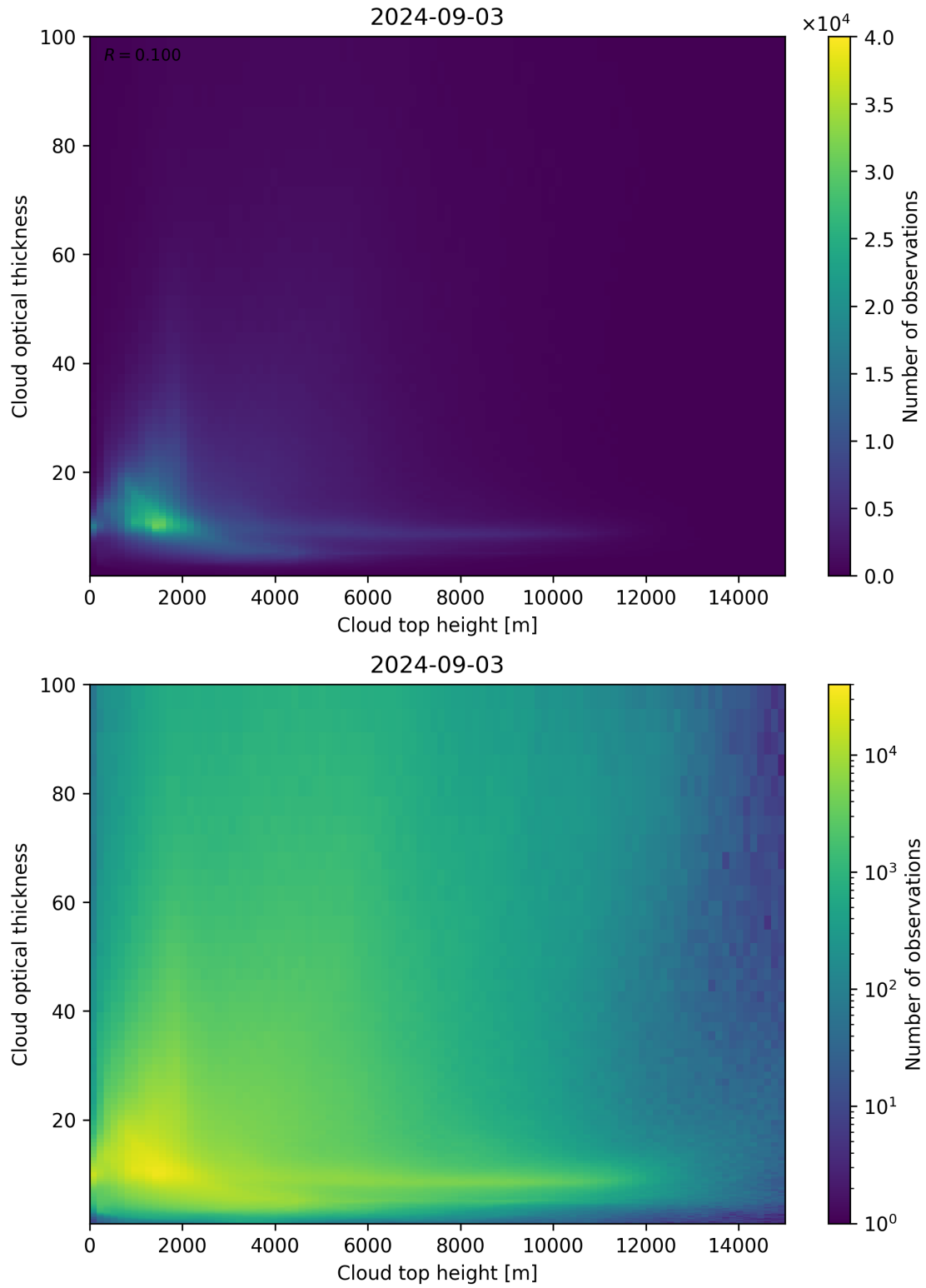
Figure 90: Scatter density plot of “Cloud top height” against “Cloud optical thickness” for 2024-09-02 to 2024-09-04.
