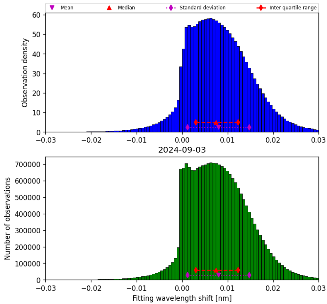
Figure 49: Histogram of “Fitting wavelength shift” for 2024-09-02 to 2024-09-04
