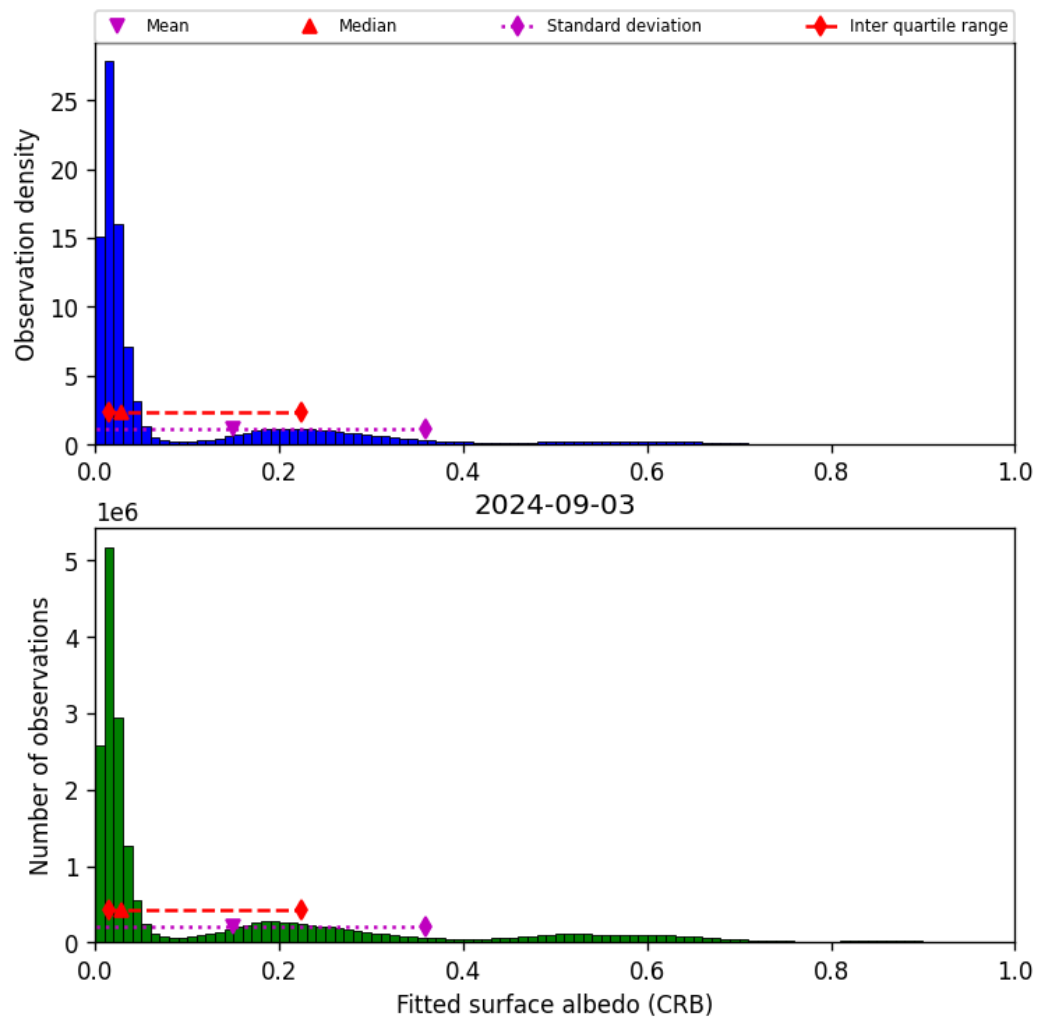
Figure 46: Histogram of “Fitted surface albedo (CRB)” for 2024-09-02 to 2024-09-04
