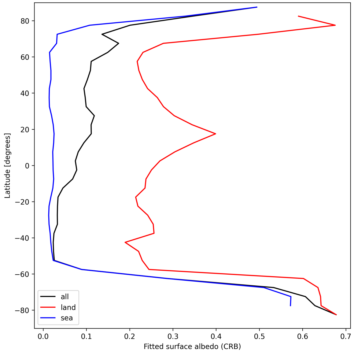
Figure 30: Zonal average of “Fitted surface albedo (CRB)” for 2024-09-02 to 2024-09-04.
