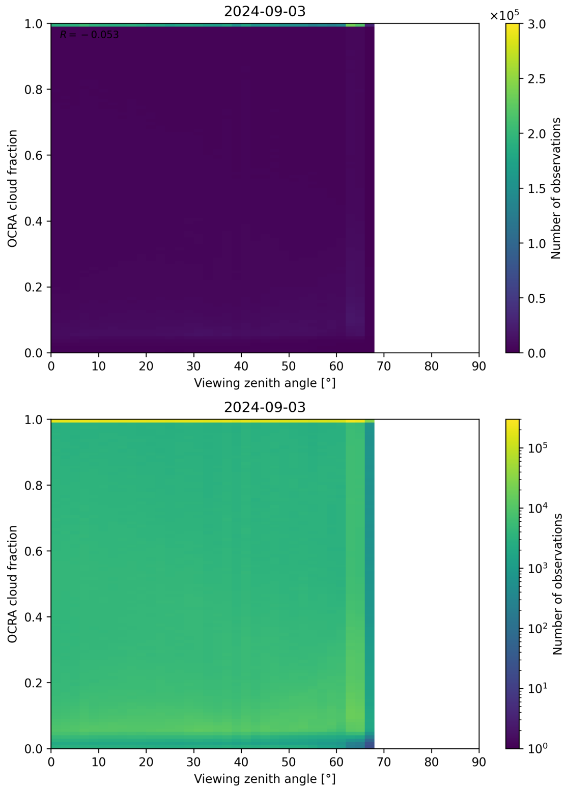
Figure 108: Scatter density plot of “Viewing zenith angle” against “OCRA cloud fraction” for 2024-09-02 to 2024-09-04.
