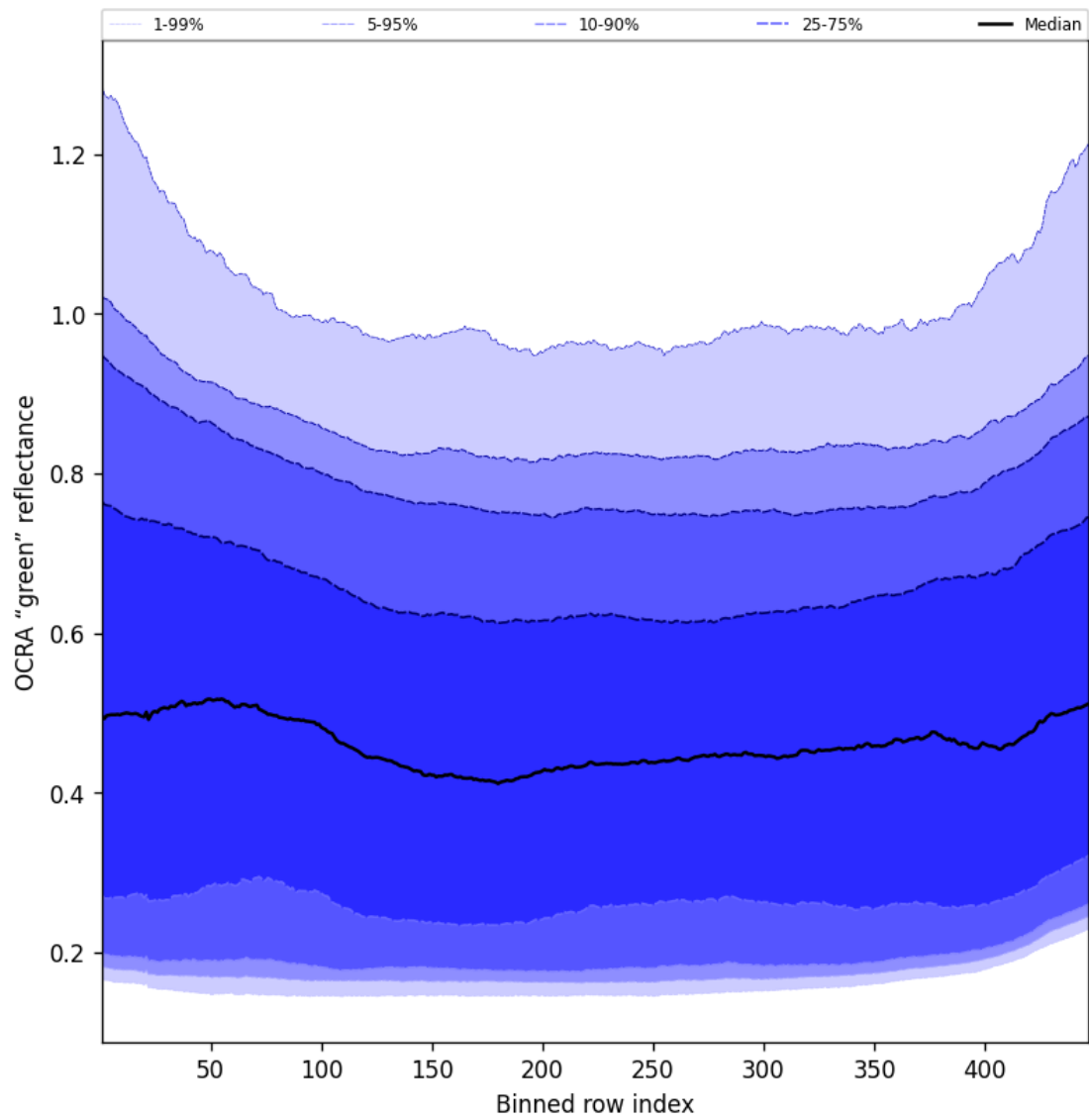
Figure 68: Along track statistics of “OCRA “green” reflectance” for 2024-09-02 to 2024-09-04
