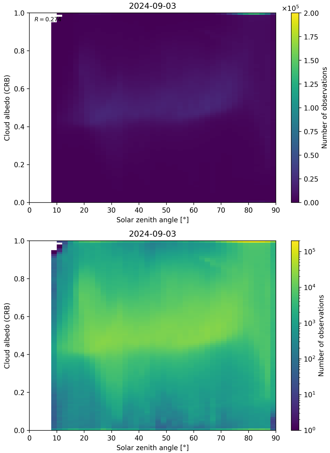
Figure 98: Scatter density plot of “Solar zenith angle” against “Cloud albedo (CRB)” for 2024-09-02 to 2024-09-04.
