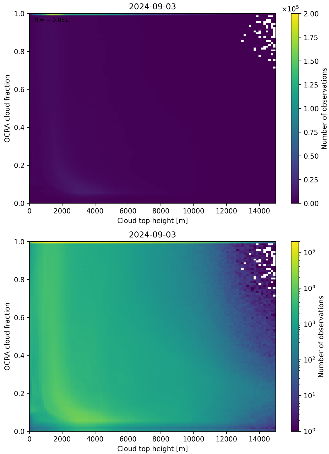
Figure 87: Scatter density plot of “Cloud top height” against “OCRA cloud fraction” for 2024-09-02 to 2024-09-04.
