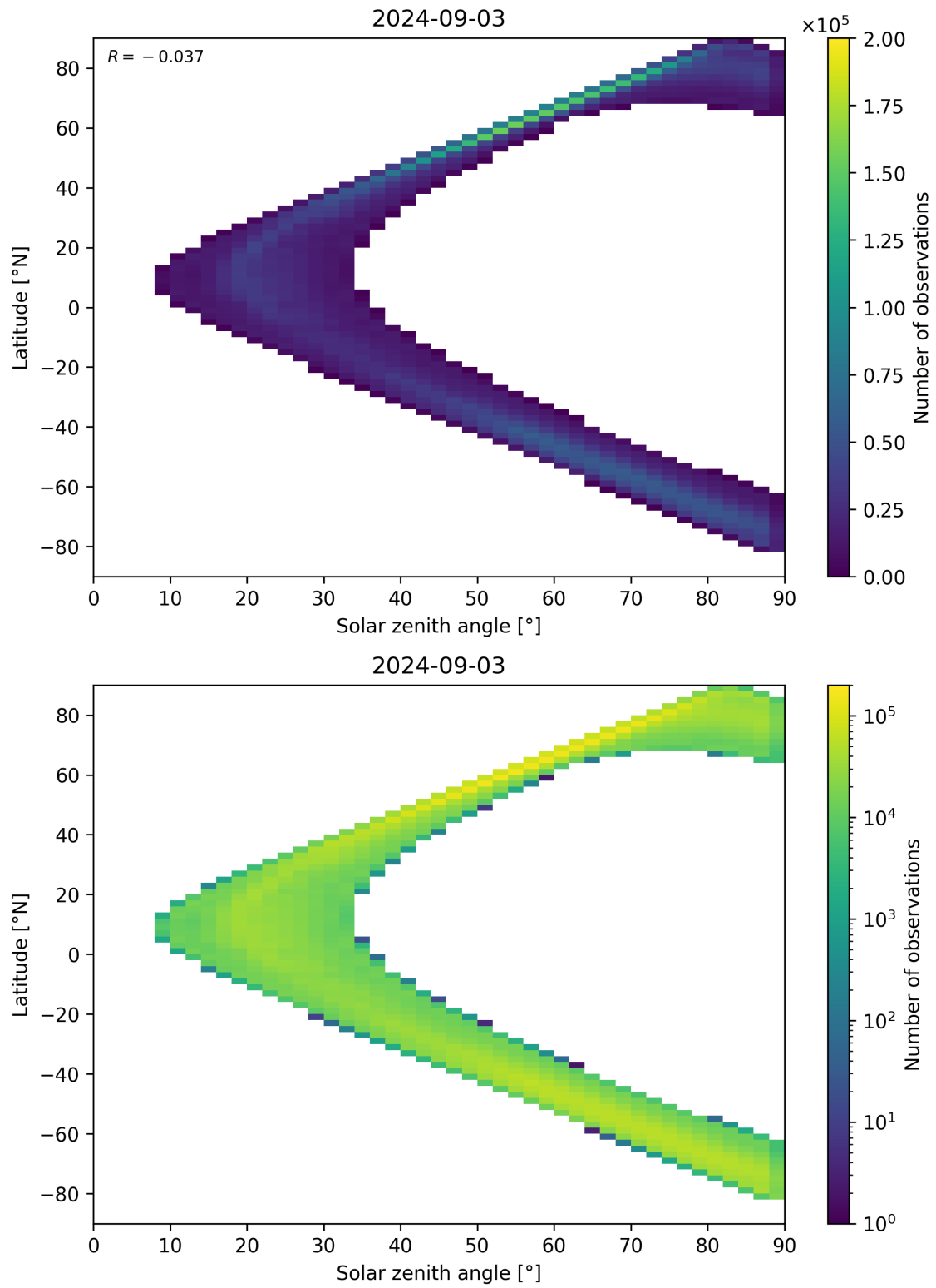
Figure 105: Scatter density plot of “Solar zenith angle” against “Latitude” for 2024-09-02 to 2024-09-04.
