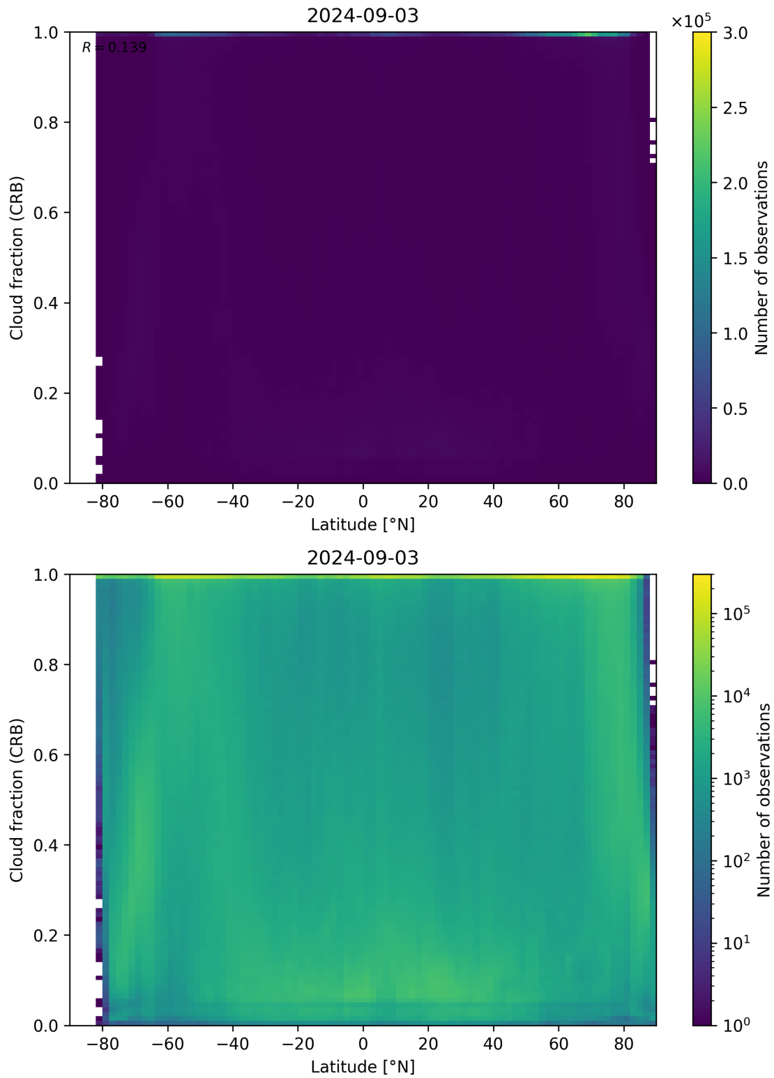
Figure 94: Scatter density plot of “Latitude” against “Cloud fraction (CRB)” for 2024-09-02 to 2024-09-04.
