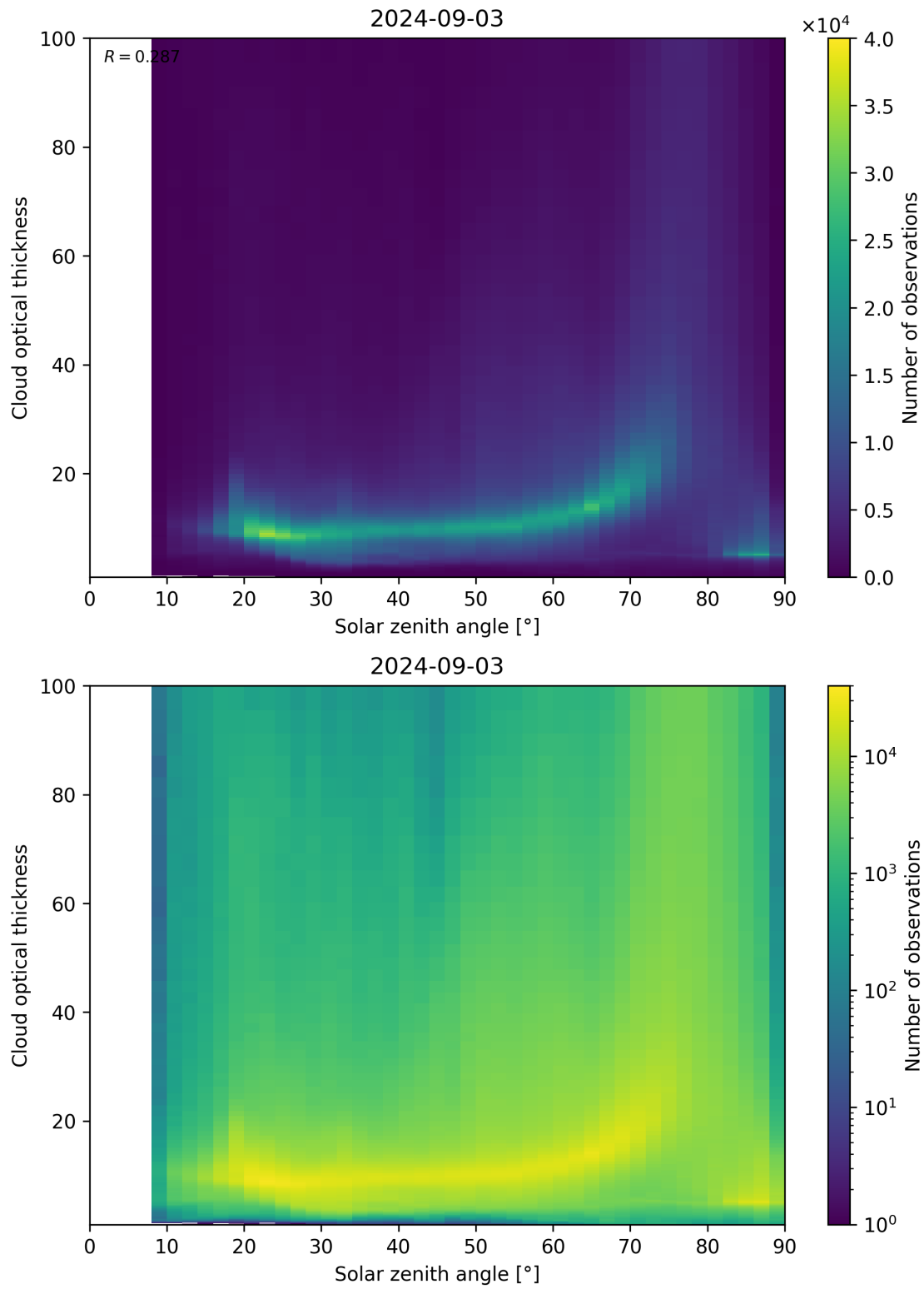
Figure 103: Scatter density plot of “Solar zenith angle” against “Cloud optical thickness” for 2024-09-02 to 2024-09-04.
