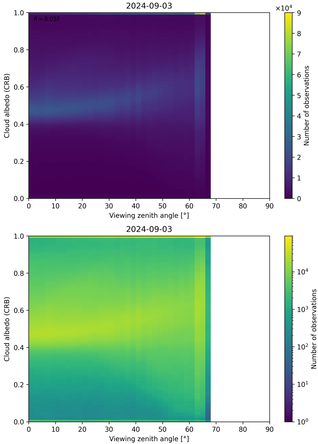
Figure 106: Scatter density plot of “Viewing zenith angle” against “Cloud albedo (CRB)” for 2024-09-02 to 2024-09-04.
