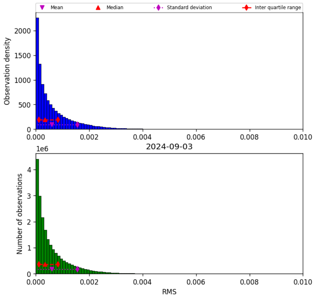
Figure 47: Histogram of “RMS” for 2024-09-02 to 2024-09-04
