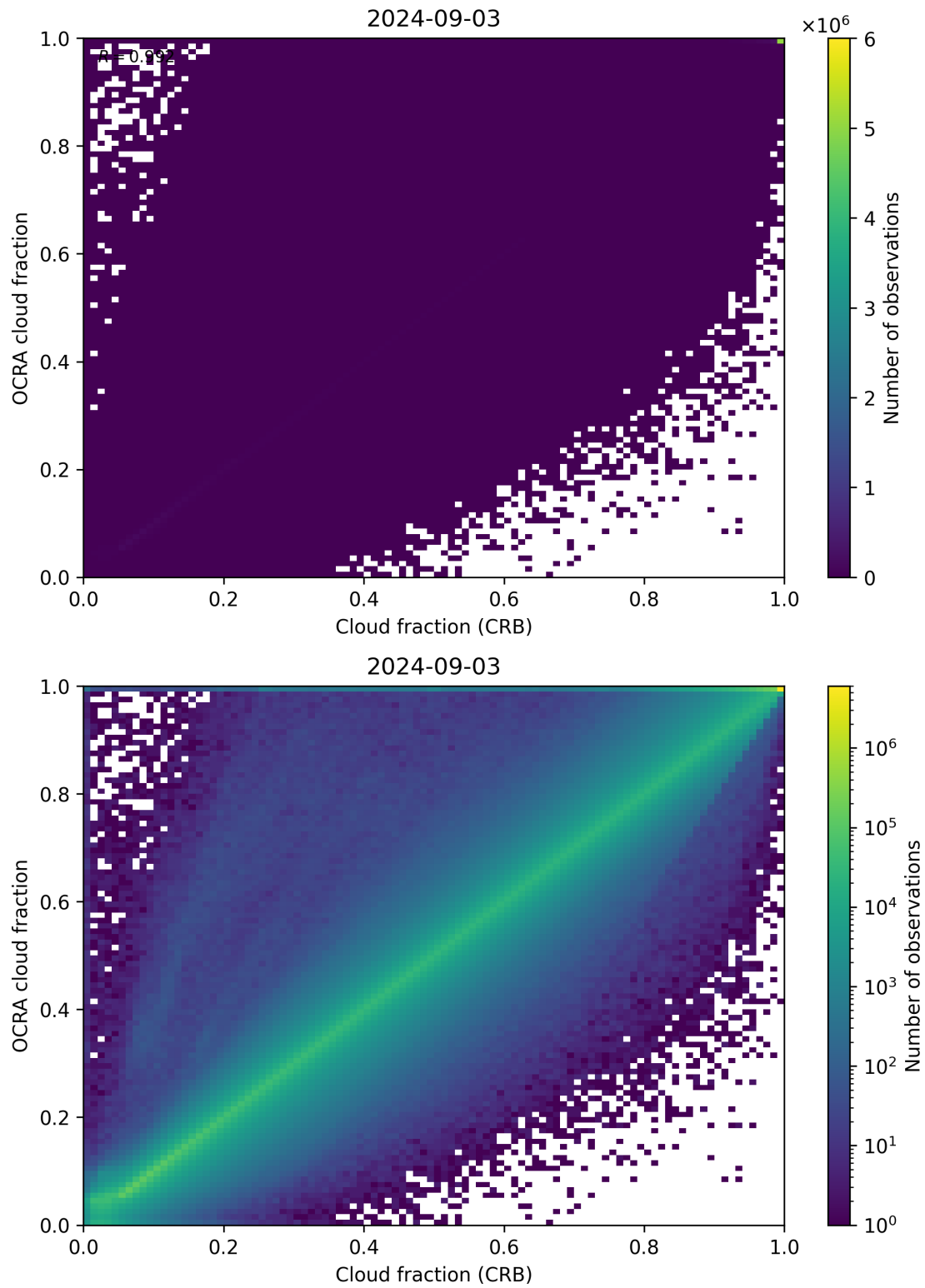
Figure 78: Scatter density plot of “Cloud fraction (CRB)” against “OCRA cloud fraction” for 2024-09-02 to 2024-09-04.
