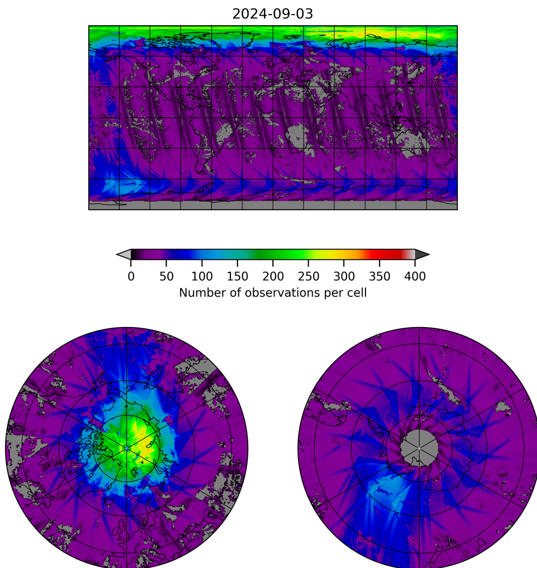
Figure 21: Map of the number of observations for 2024-09-02 to 2024-09-04
