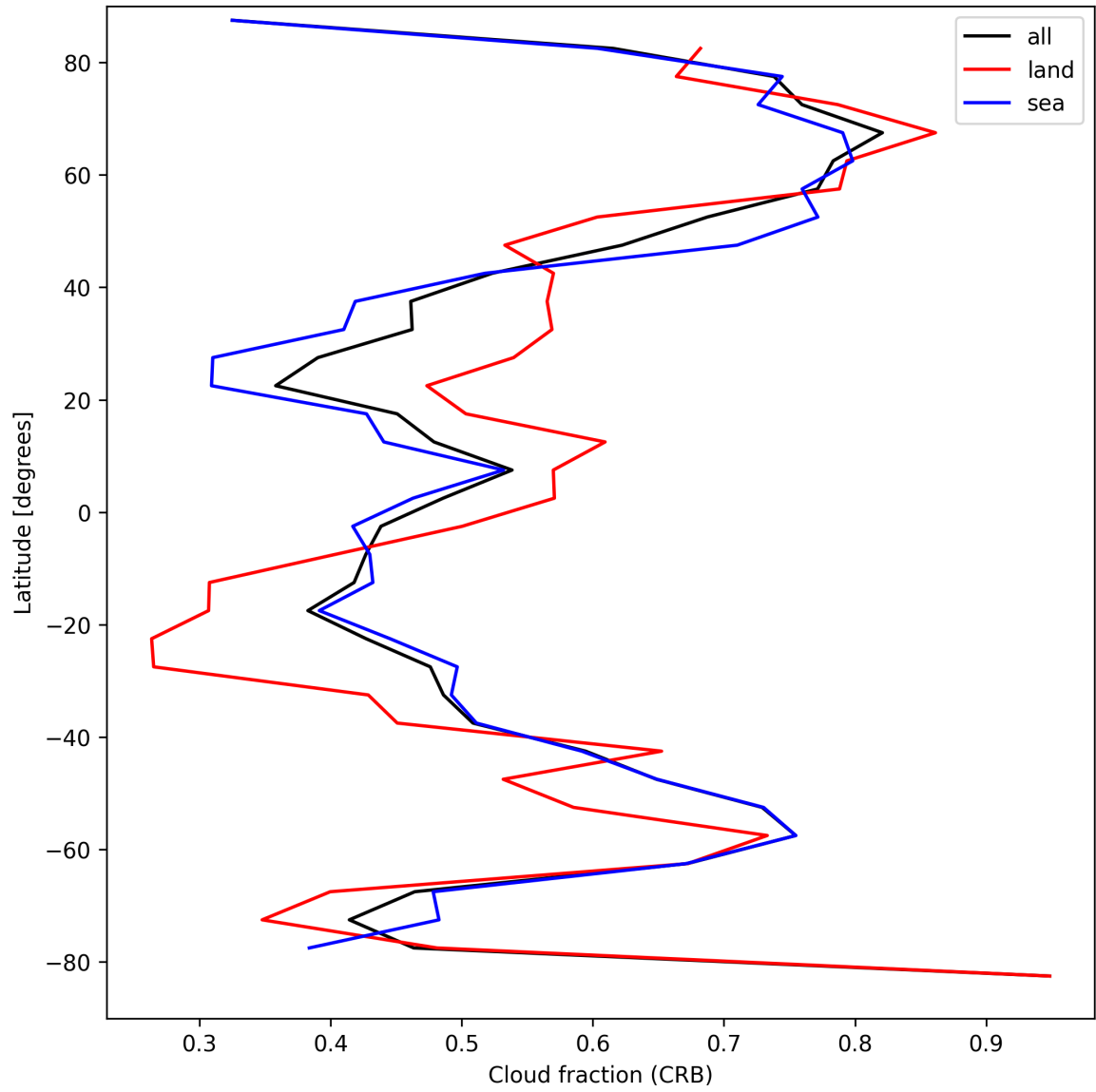
Figure 26: Zonal average of “Cloud fraction (CRB)” for 2024-09-02 to 2024-09-04.
