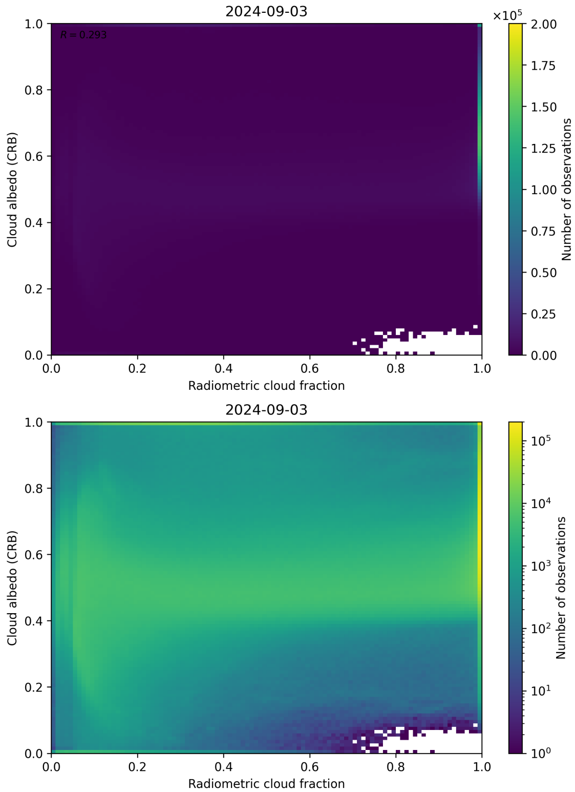
Figure 71: Scatter density plot of “Radiometric cloud fraction” against “Cloud albedo (CRB)” for 2024-09-02 to 2024-09-04.
