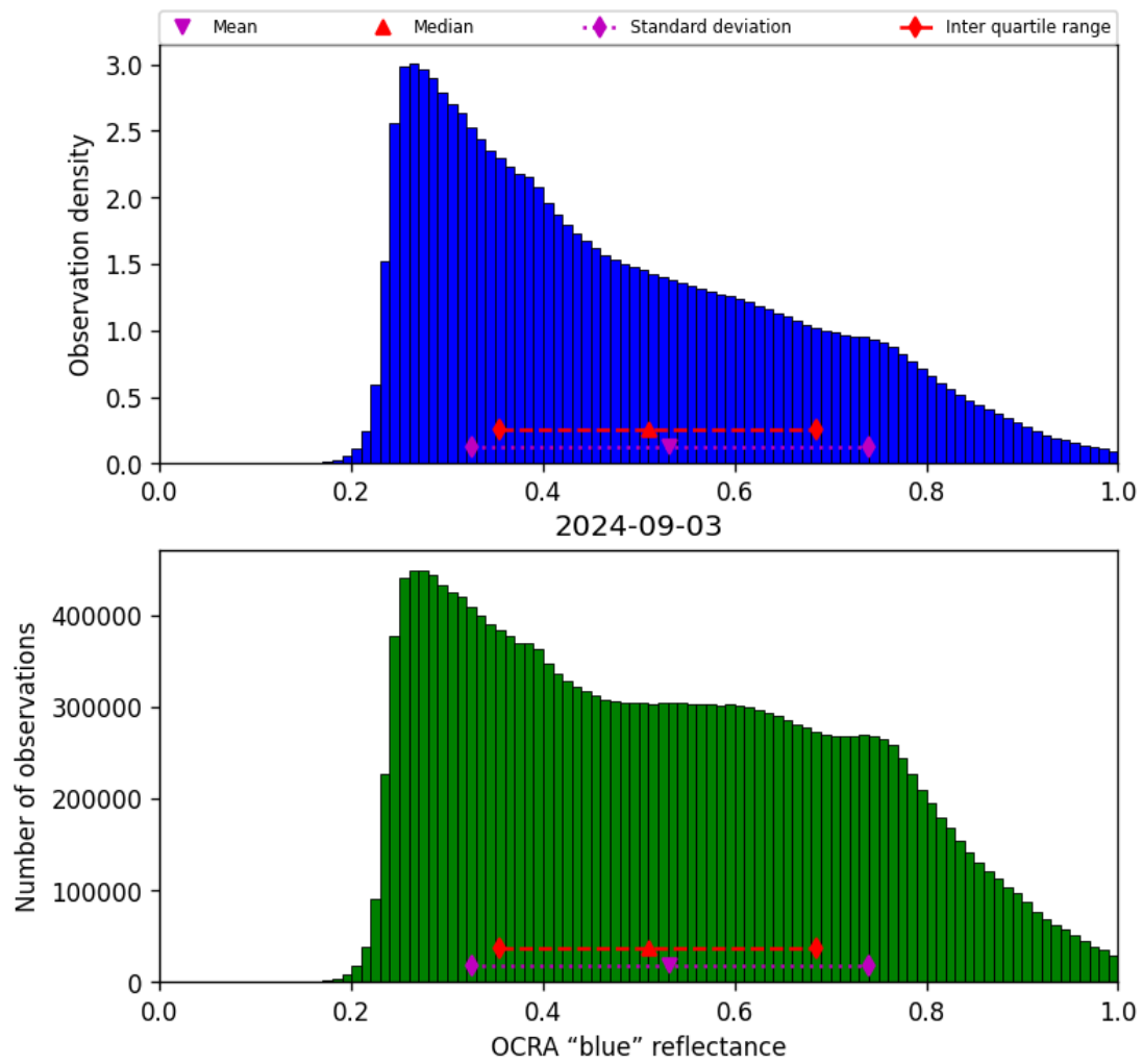
Figure 51: Histogram of “OCRA “blue” reflectance” for 2024-09-02 to 2024-09-04
