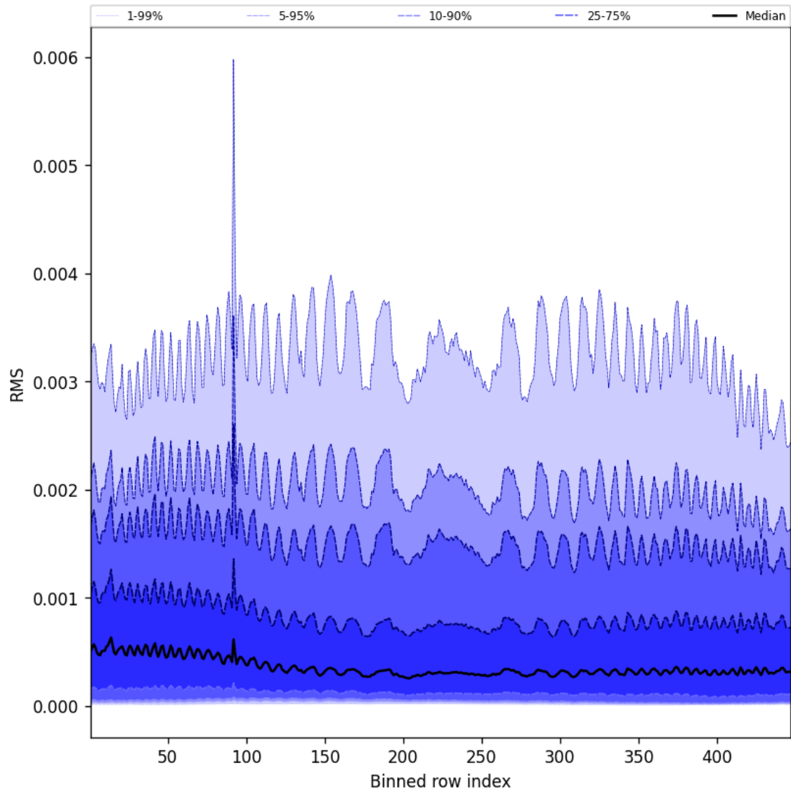
Figure 63: Along track statistics of “RMS” for 2024-09-02 to 2024-09-04
