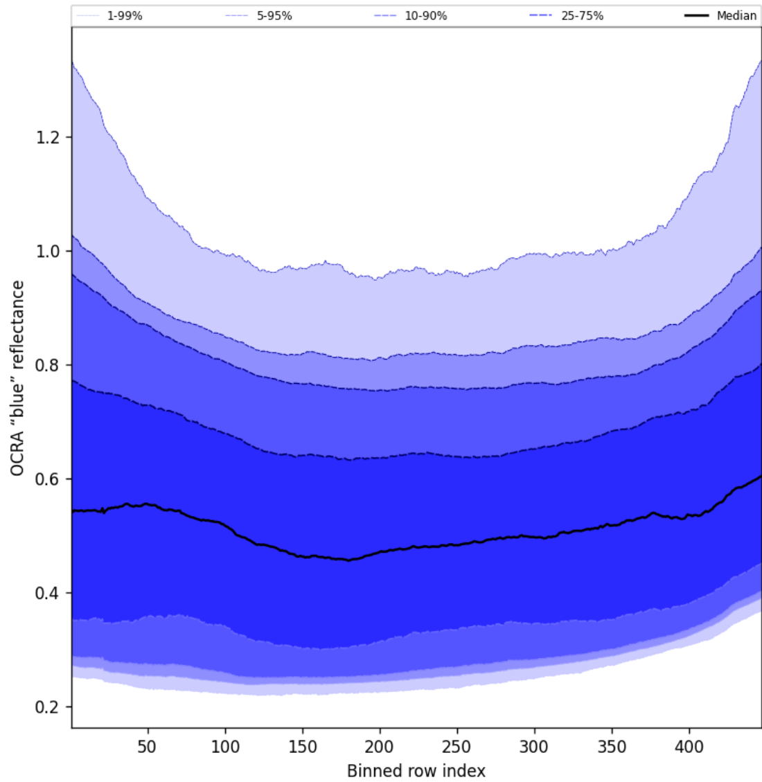
Figure 67: Along track statistics of “OCRA “blue” reflectance” for 2024-09-02 to 2024-09-04
