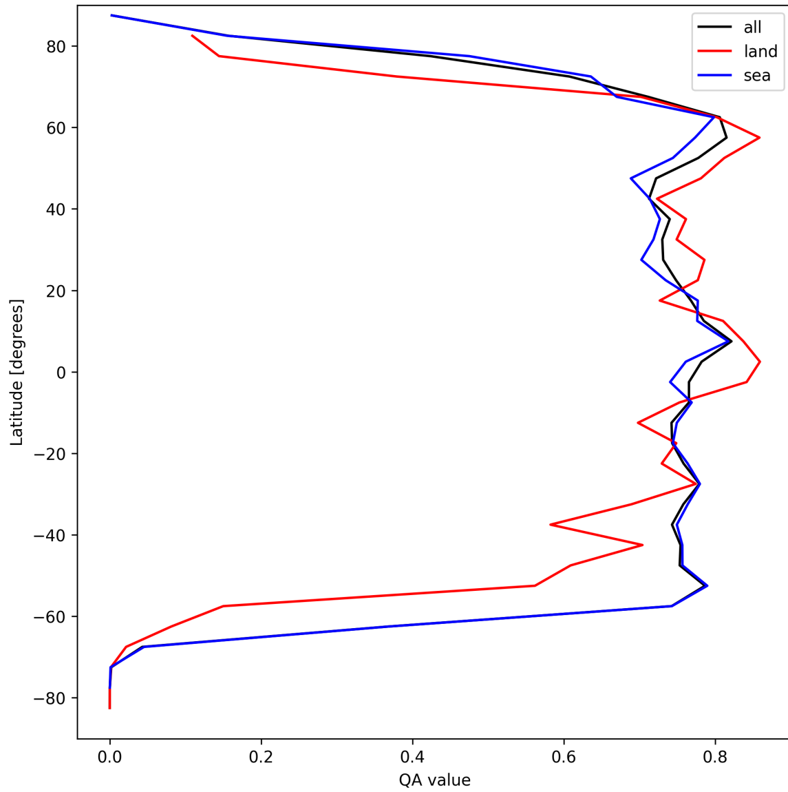
Figure 22: Zonal average of “QA value” for 2024-09-02 to 2024-09-04.
