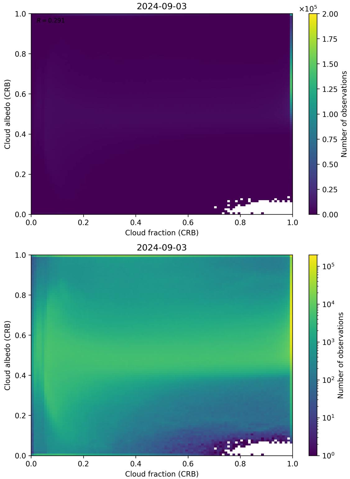
Figure 77: Scatter density plot of “Cloud fraction (CRB)” against “Cloud albedo (CRB)” for 2024-09-02 to 2024-09-04.
