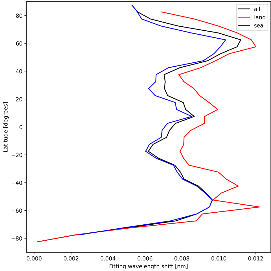
Figure 33: Zonal average of “Fitting wavelength shift” for 2024-09-02 to 2024-09-04.
