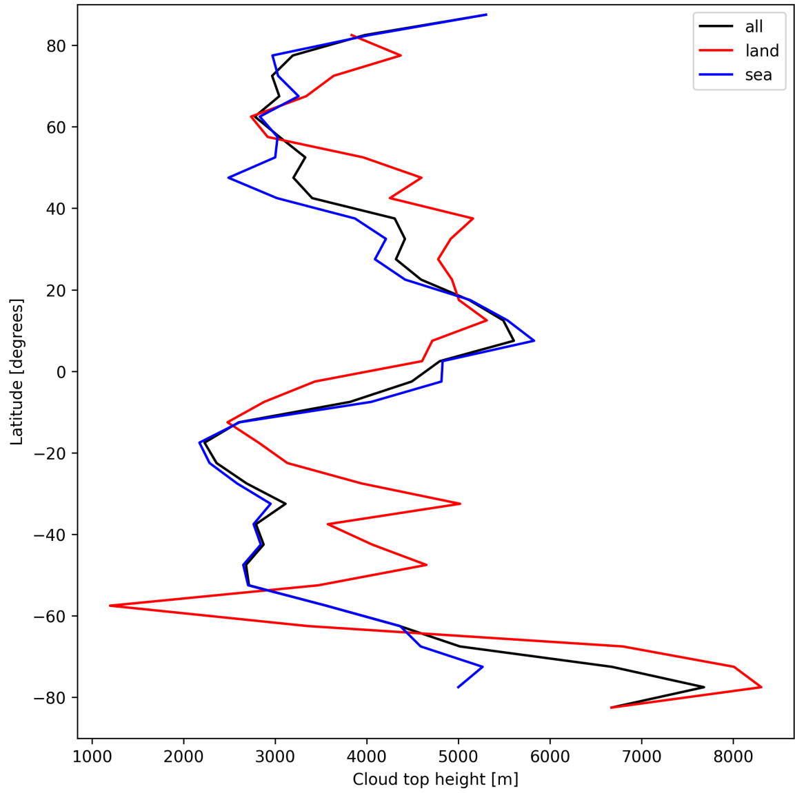
Figure 24: Zonal average of “Cloud top height” for 2024-09-02 to 2024-09-04.
