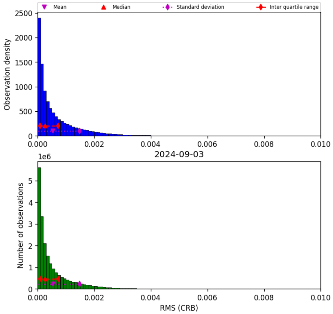
Figure 48: Histogram of “RMS (CRB)” for 2024-09-02 to 2024-09-04
