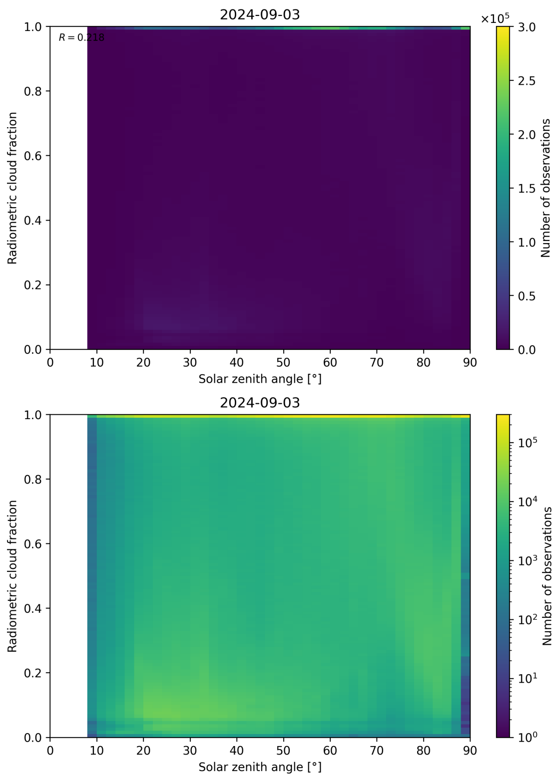
Figure 99: Scatter density plot of “Solar zenith angle” against “Radiometric cloud fraction” for 2024-09-02 to 2024-09-04.
