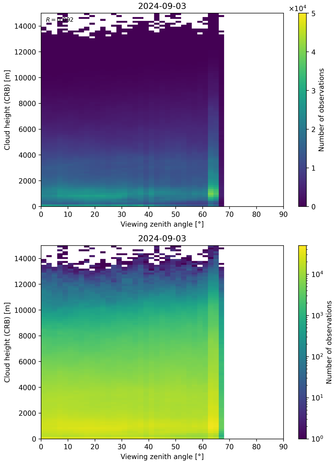
Figure 110: Scatter density plot of “Viewing zenith angle” against “Cloud height (CRB)” for 2024-09-02 to 2024-09-04.
