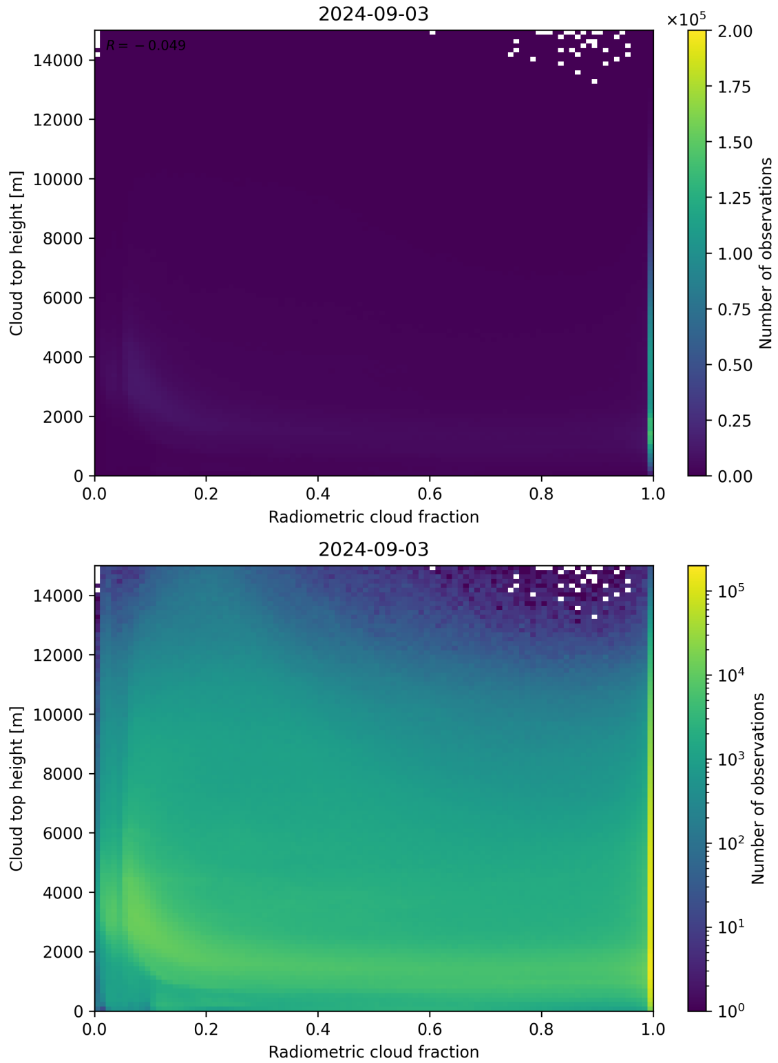
Figure 76: Scatter density plot of “Radiometric cloud fraction” against “Cloud top height” for 2024-09-02 to 2024-09-04.
