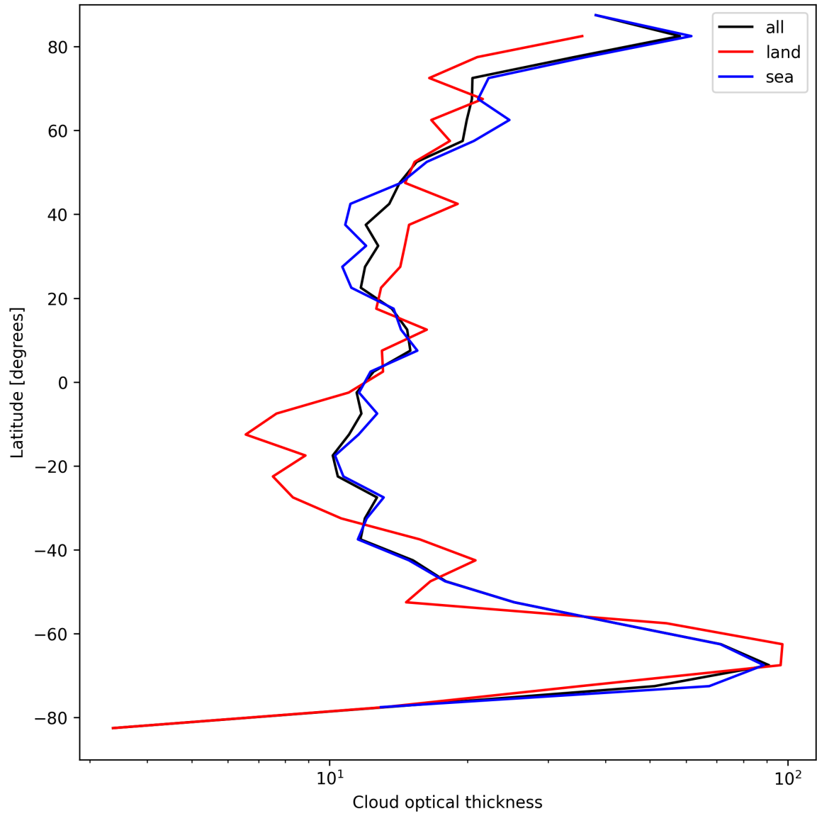
Figure 25: Zonal average of “Cloud optical thickness” for 2024-09-02 to 2024-09-04.
