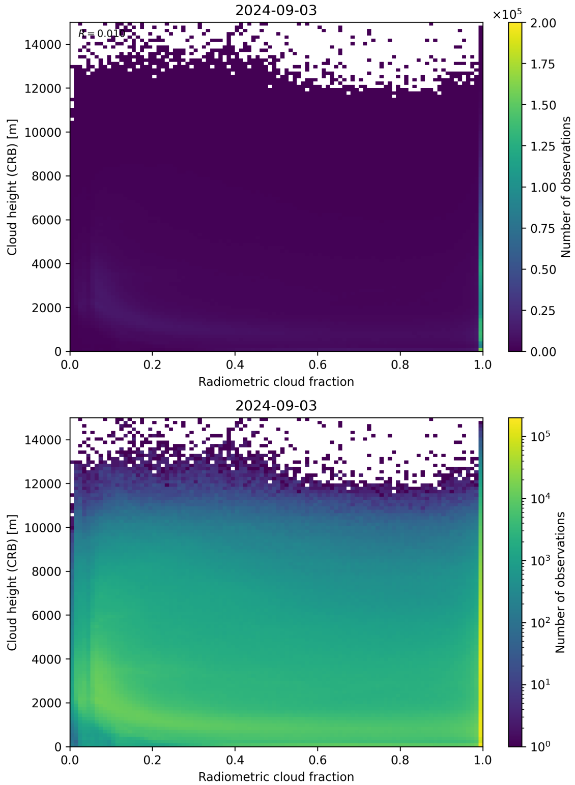
Figure 74: Scatter density plot of “Radiometric cloud fraction” against “Cloud height (CRB)” for 2024-09-02 to 2024-09-04.
