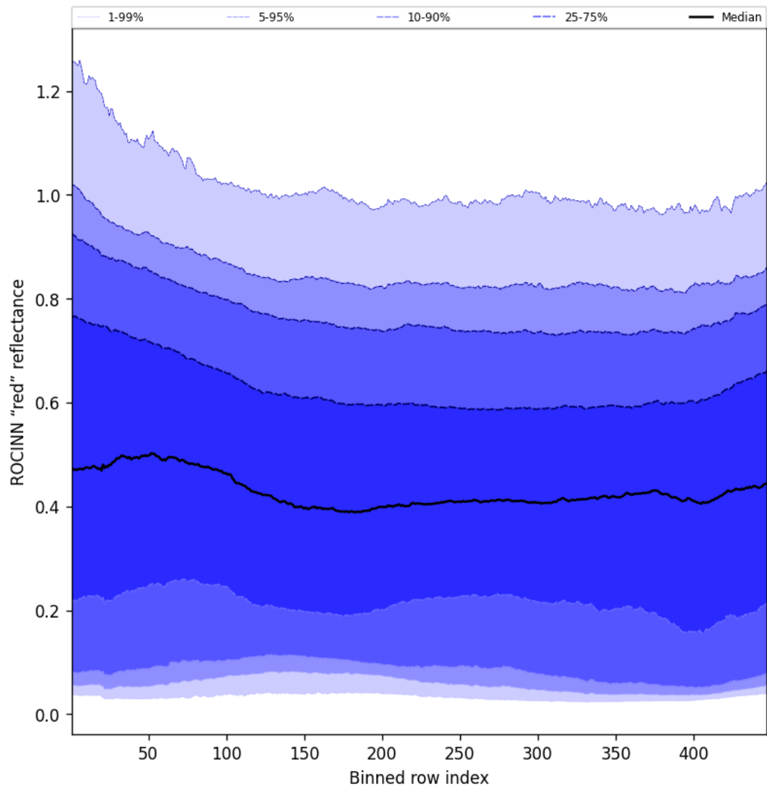
Figure 69: Along track statistics of “ROCINN “red” reflectance” for 2024-09-02 to 2024-09-04
