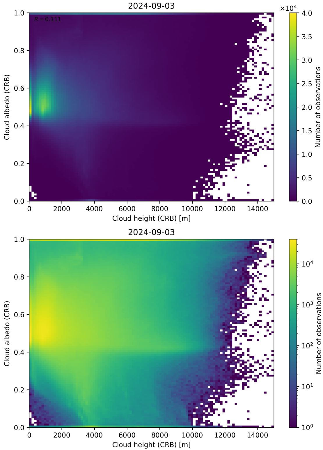
Figure 80: Scatter density plot of “Cloud height (CRB)” against “Cloud albedo (CRB)” for 2024-09-02 to 2024-09-04.
