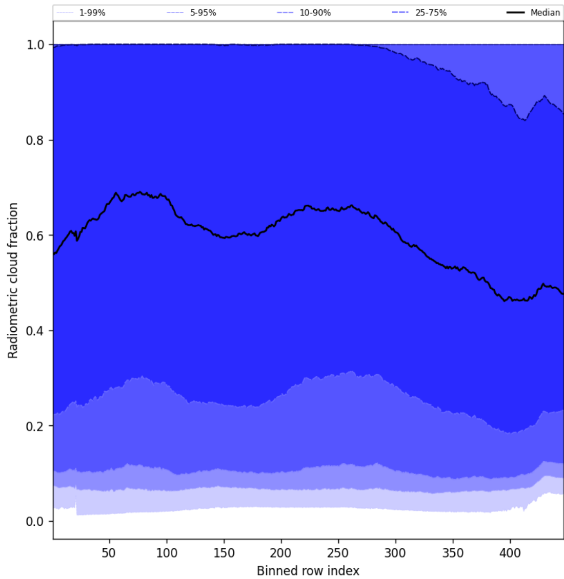
Figure 55: Along track statistics of “Radiometric cloud fraction” for 2024-09-02 to 2024-09-04
