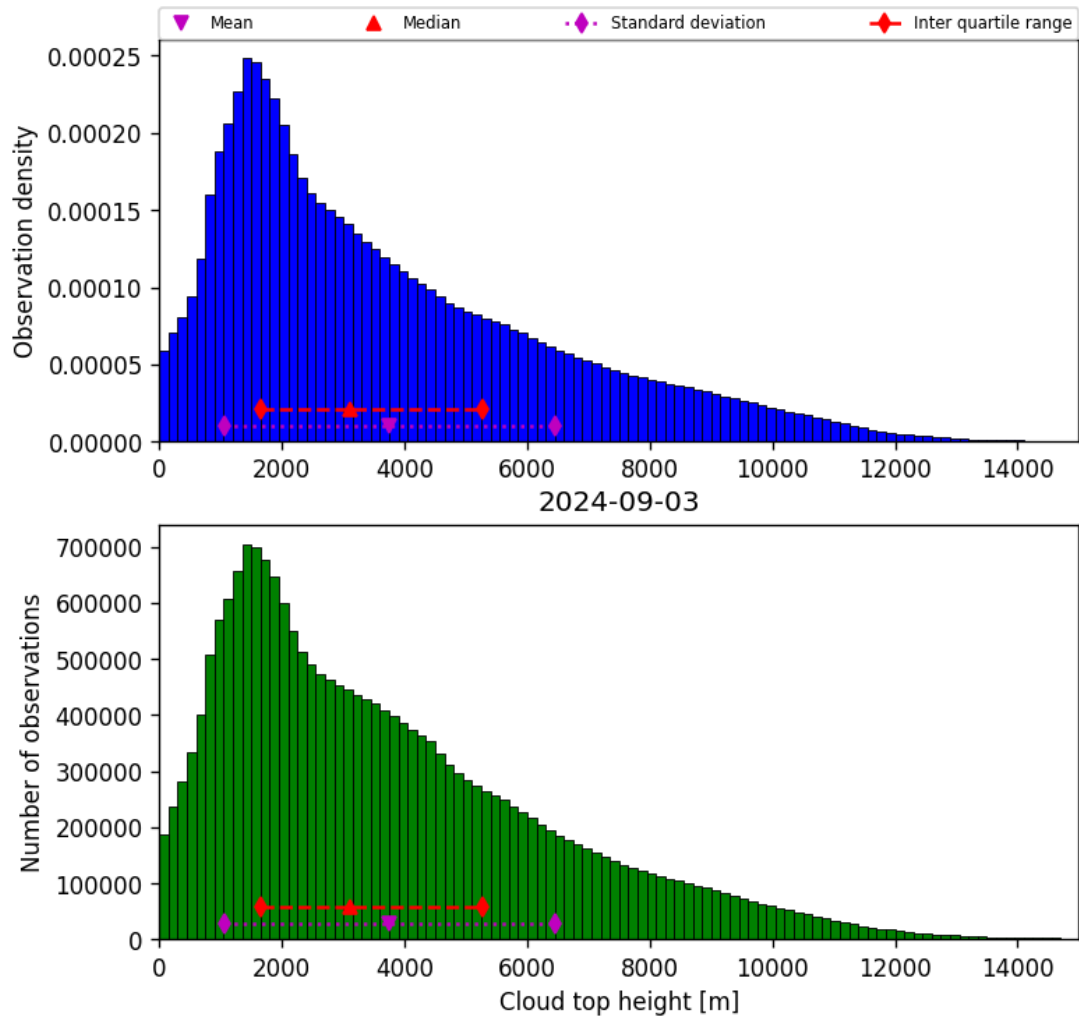
Figure 40: Histogram of “Cloud top height” for 2024-09-02 to 2024-09-04
