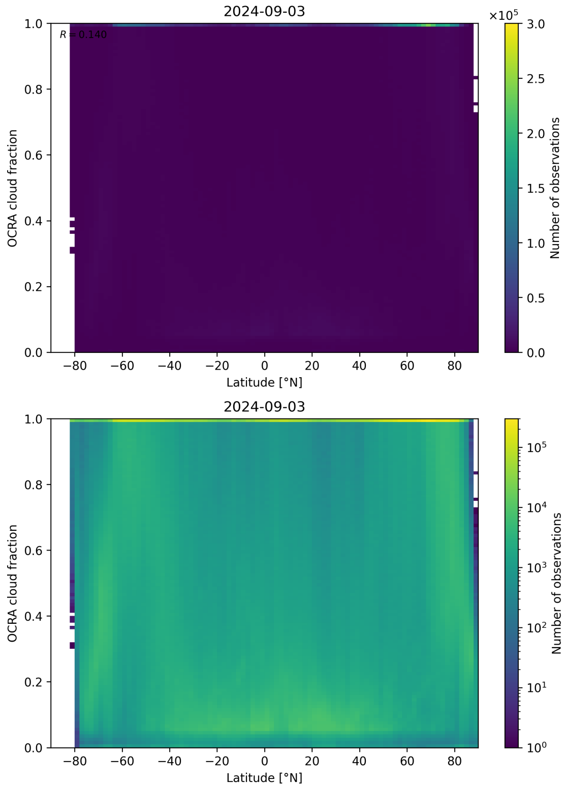
Figure 93: Scatter density plot of “Latitude” against “OCRA cloud fraction” for 2024-09-02 to 2024-09-04.
