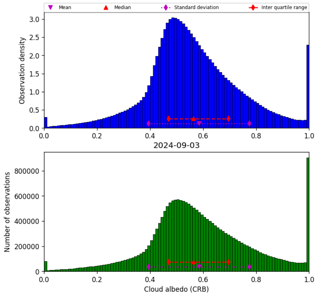
Figure 44: Histogram of “Cloud albedo (CRB)” for 2024-09-02 to 2024-09-04
