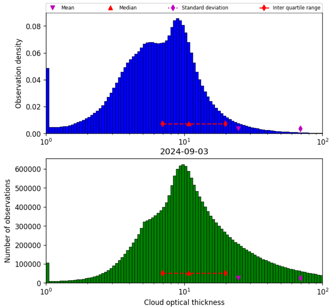
Figure 41: Histogram of “Cloud optical thickness” for 2024-09-02 to 2024-09-04
