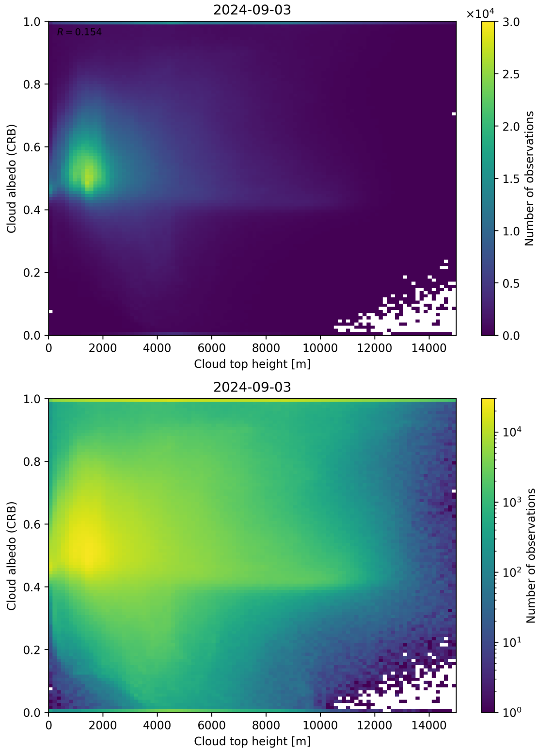
Figure 86: Scatter density plot of “Cloud top height” against “Cloud albedo (CRB)” for 2024-09-02 to 2024-09-04.
