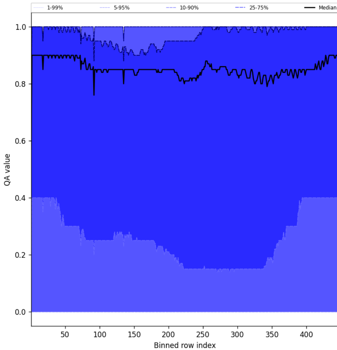
Figure 54: Along track statistics of “QA value” for 2024-09-02 to 2024-09-04
