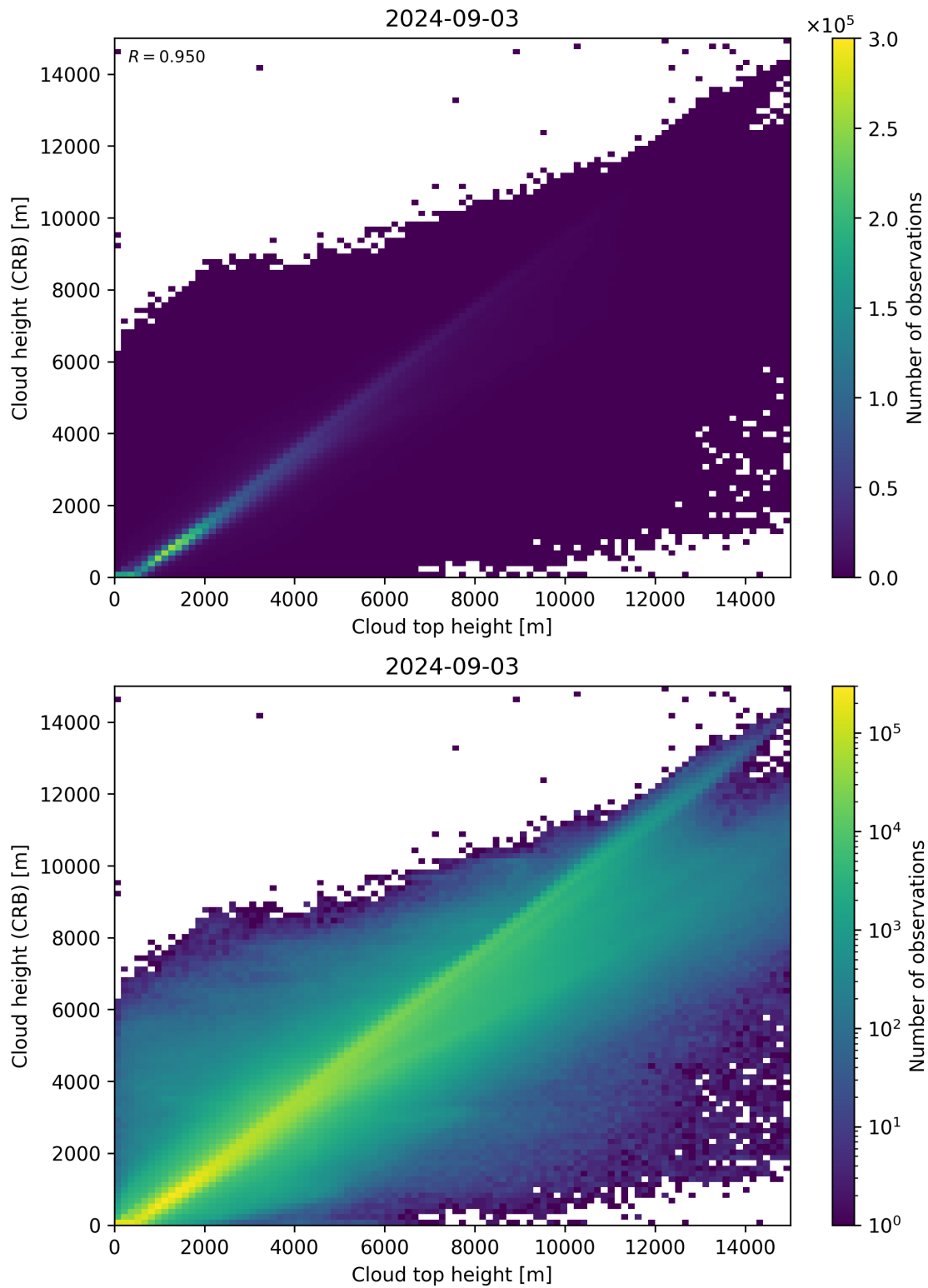
Figure 89: Scatter density plot of “Cloud top height” against “Cloud height (CRB)” for 2024-09-02 to 2024-09-04.
