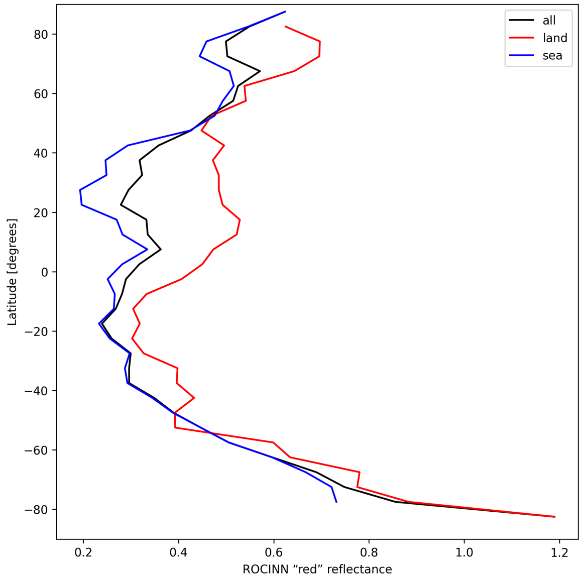
Figure 37: Zonal average of “ROCINN “red” reflectance” for 2024-09-02 to 2024-09-04.
