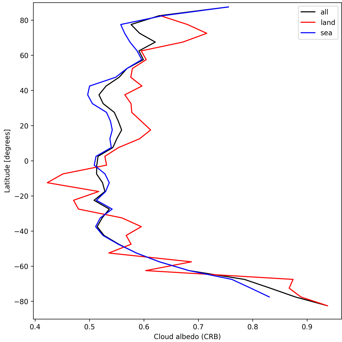
Figure 28: Zonal average of “Cloud albedo (CRB)” for 2024-09-02 to 2024-09-04.
