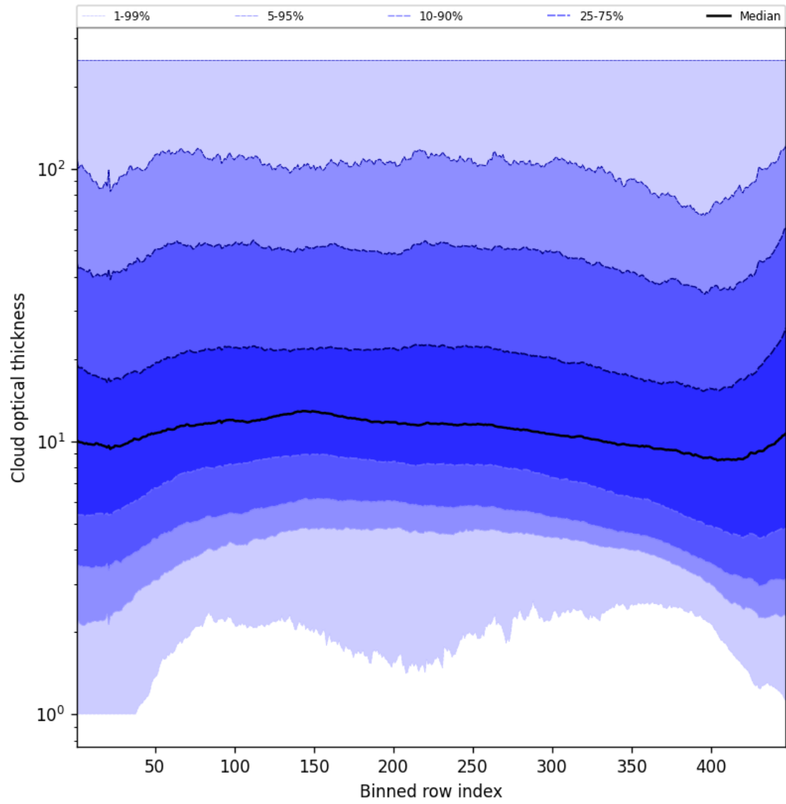
Figure 57: Along track statistics of “Cloud optical thickness” for 2024-09-02 to 2024-09-04
