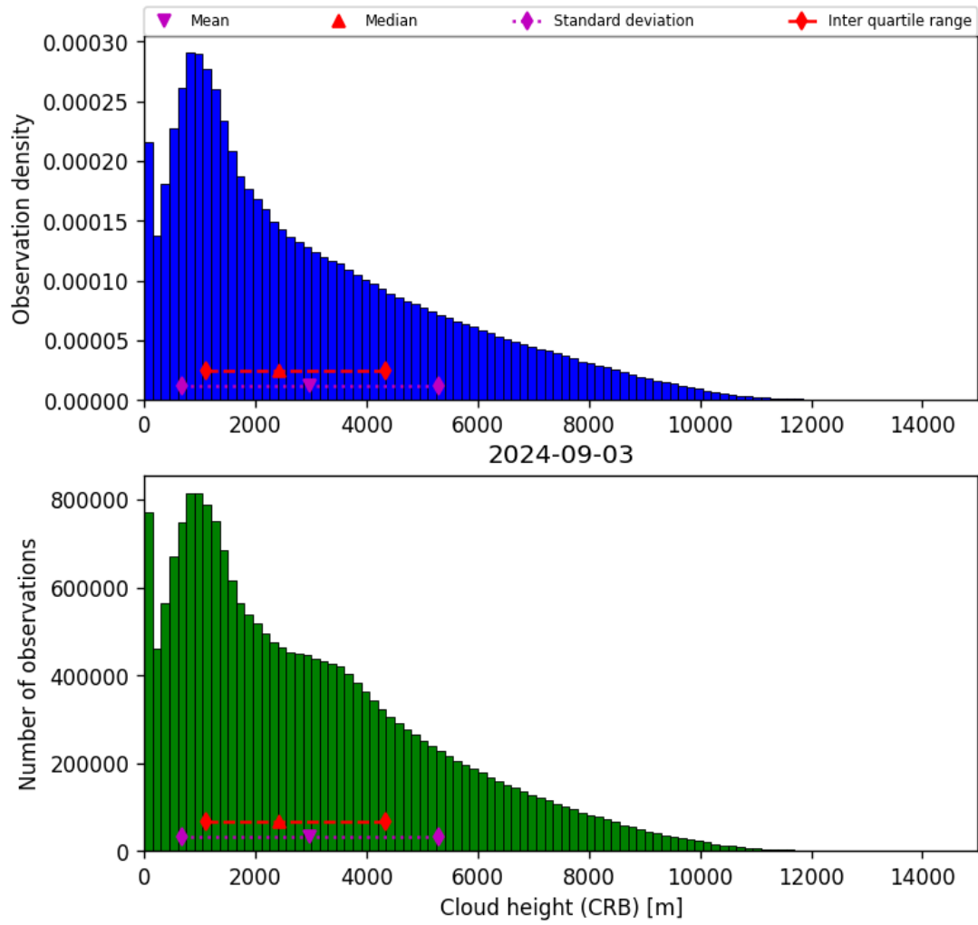
Figure 43: Histogram of “Cloud height (CRB)” for 2024-09-02 to 2024-09-04
