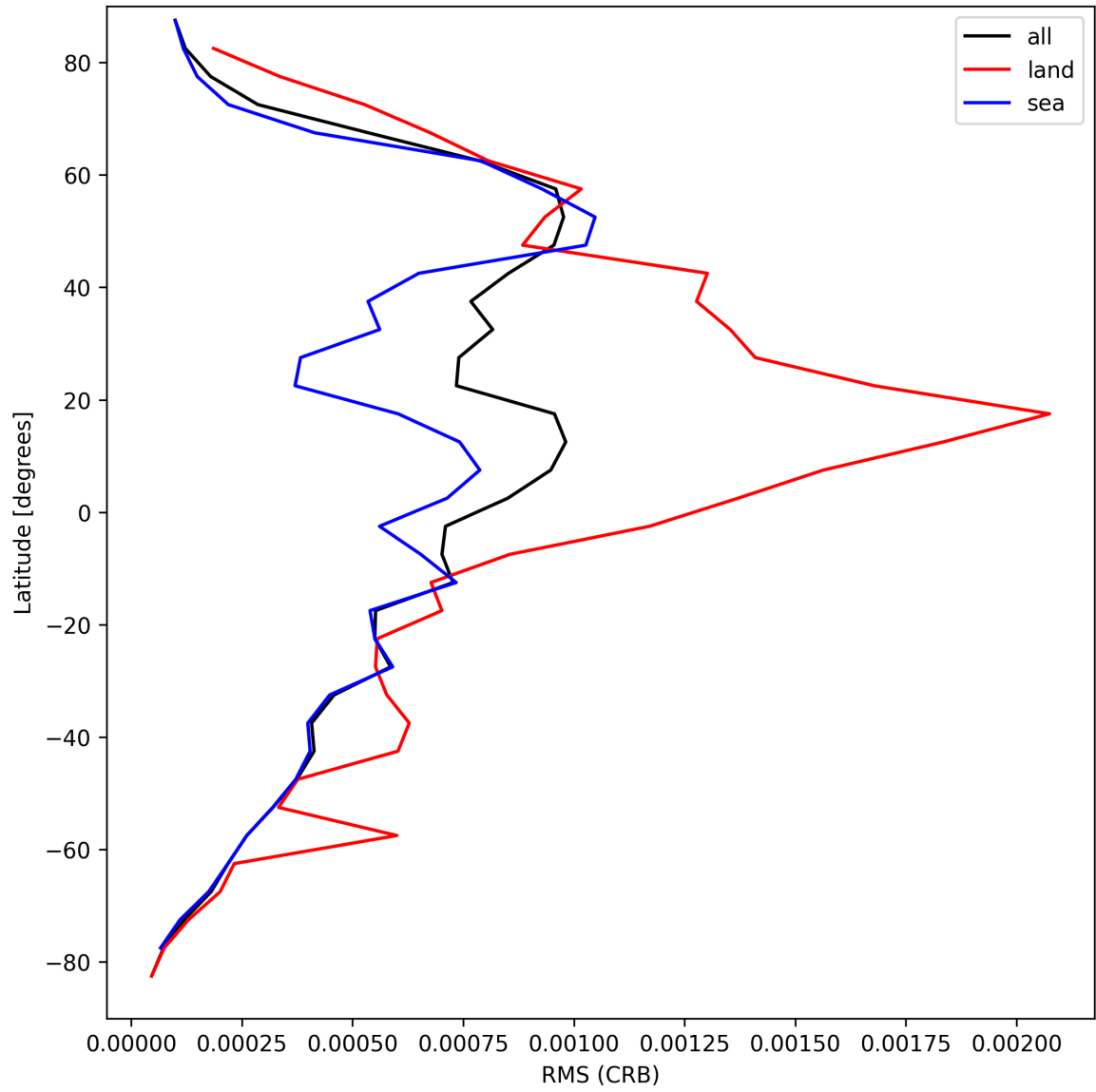
Figure 32: Zonal average of “RMS (CRB)” for 2024-09-02 to 2024-09-04.
