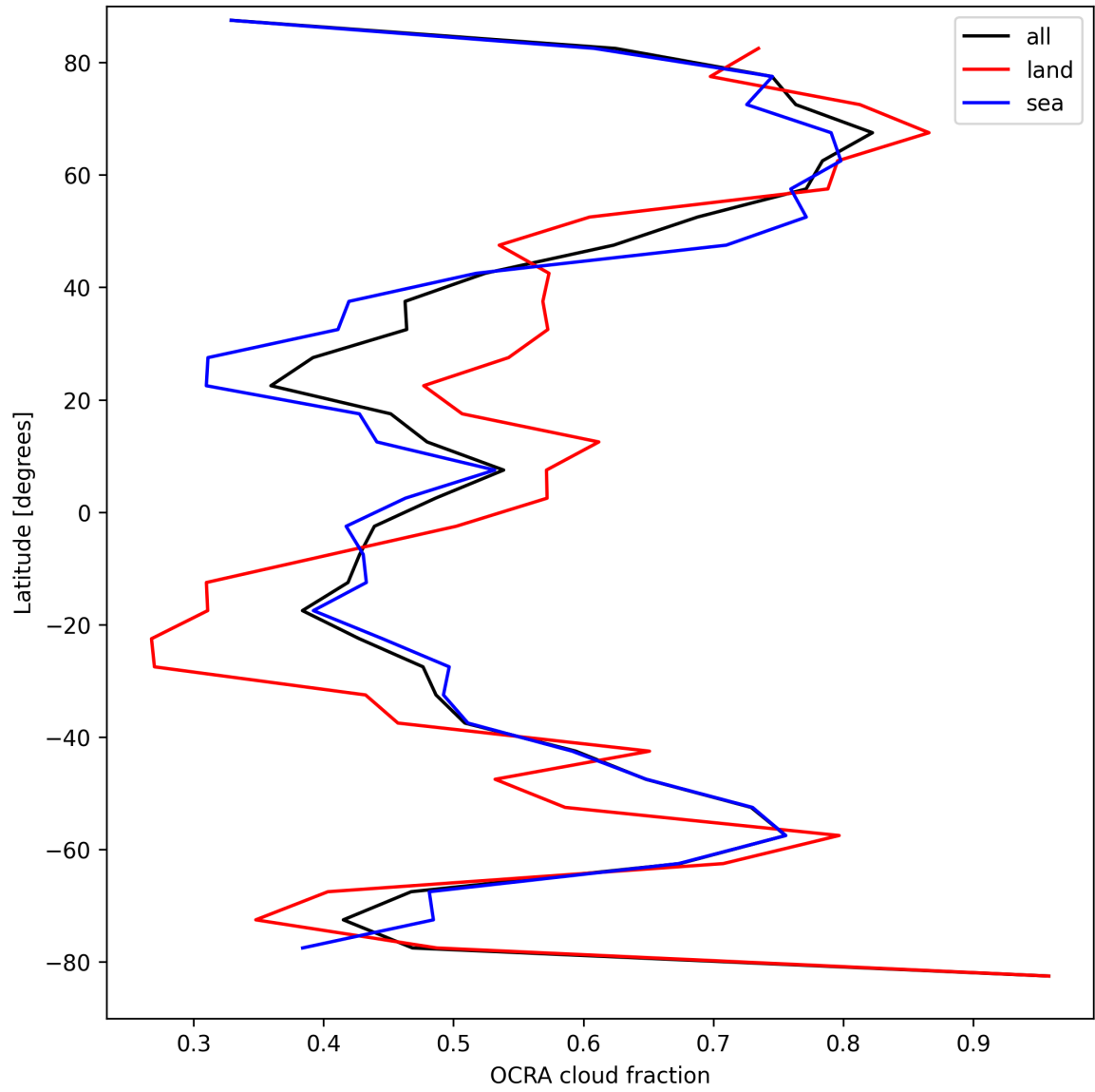
Figure 34: Zonal average of “OCRA cloud fraction” for 2024-09-02 to 2024-09-04.
