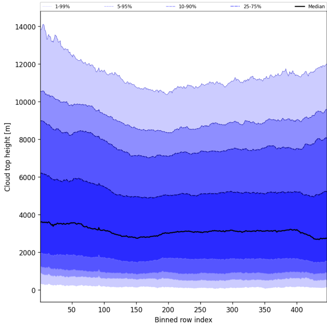
Figure 56: Along track statistics of “Cloud top height” for 2024-09-02 to 2024-09-04
