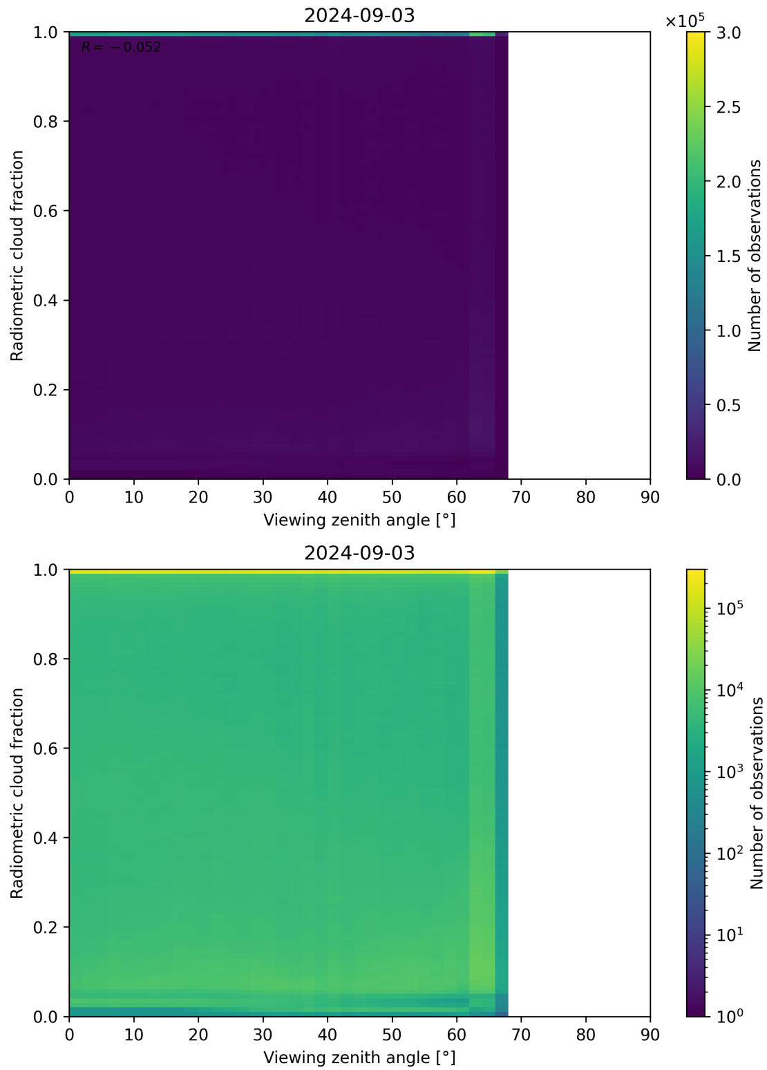
Figure 107: Scatter density plot of “Viewing zenith angle” against “Radiometric cloud fraction” for 2024-09-02 to 2024-09-04.
