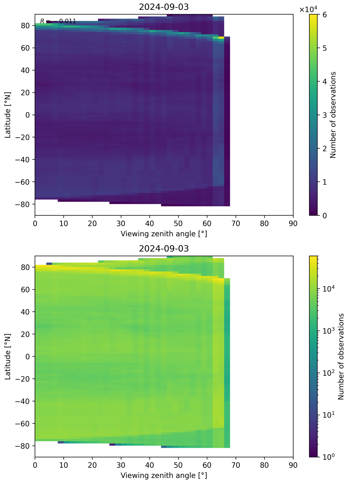
Figure 113: Scatter density plot of “Viewing zenith angle” against “Latitude” for 2024-09-02 to 2024-09-04.
