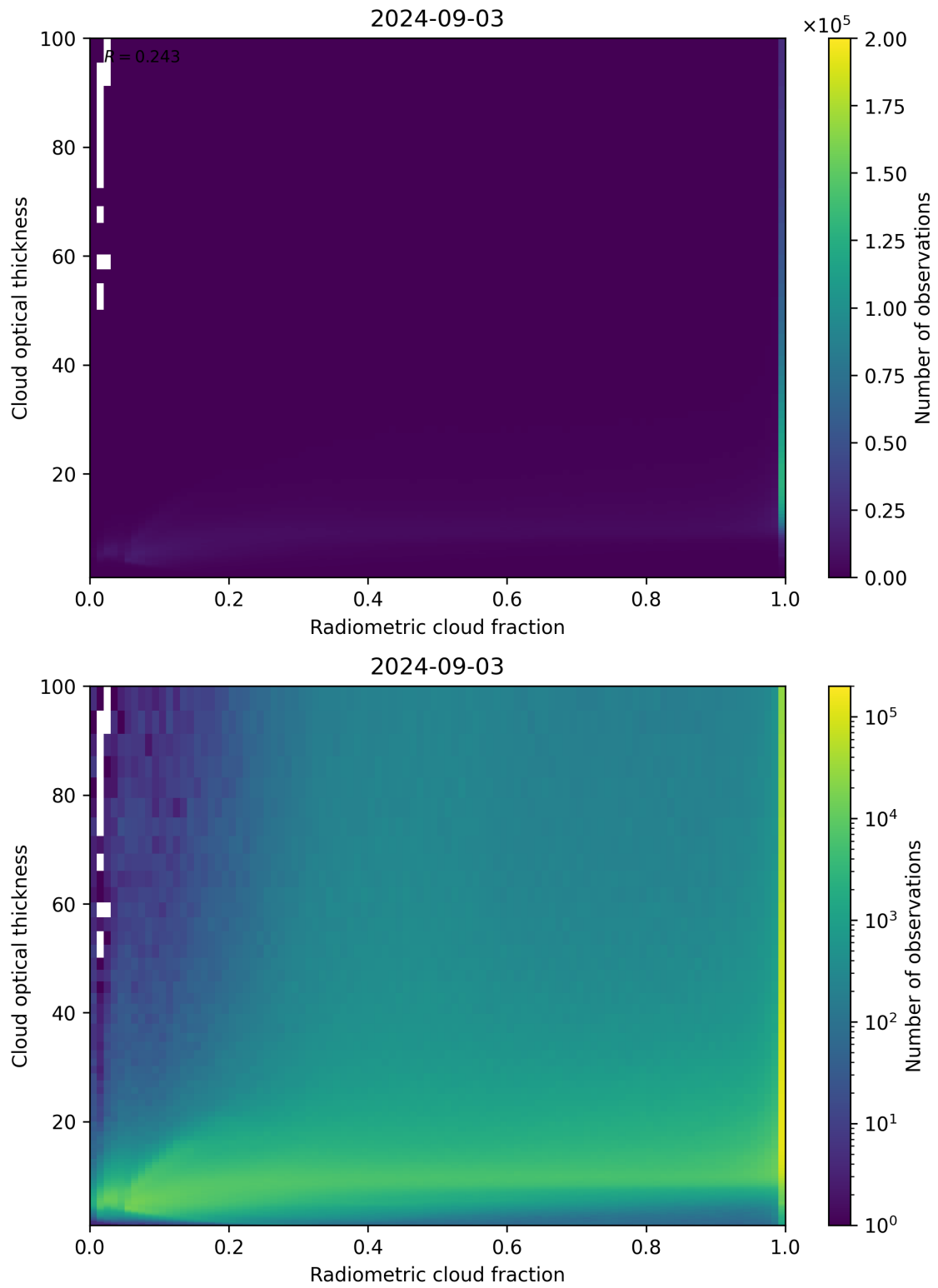
Figure 75: Scatter density plot of “Radiometric cloud fraction” against “Cloud optical thickness” for 2024-09-02 to 2024-09-04.
