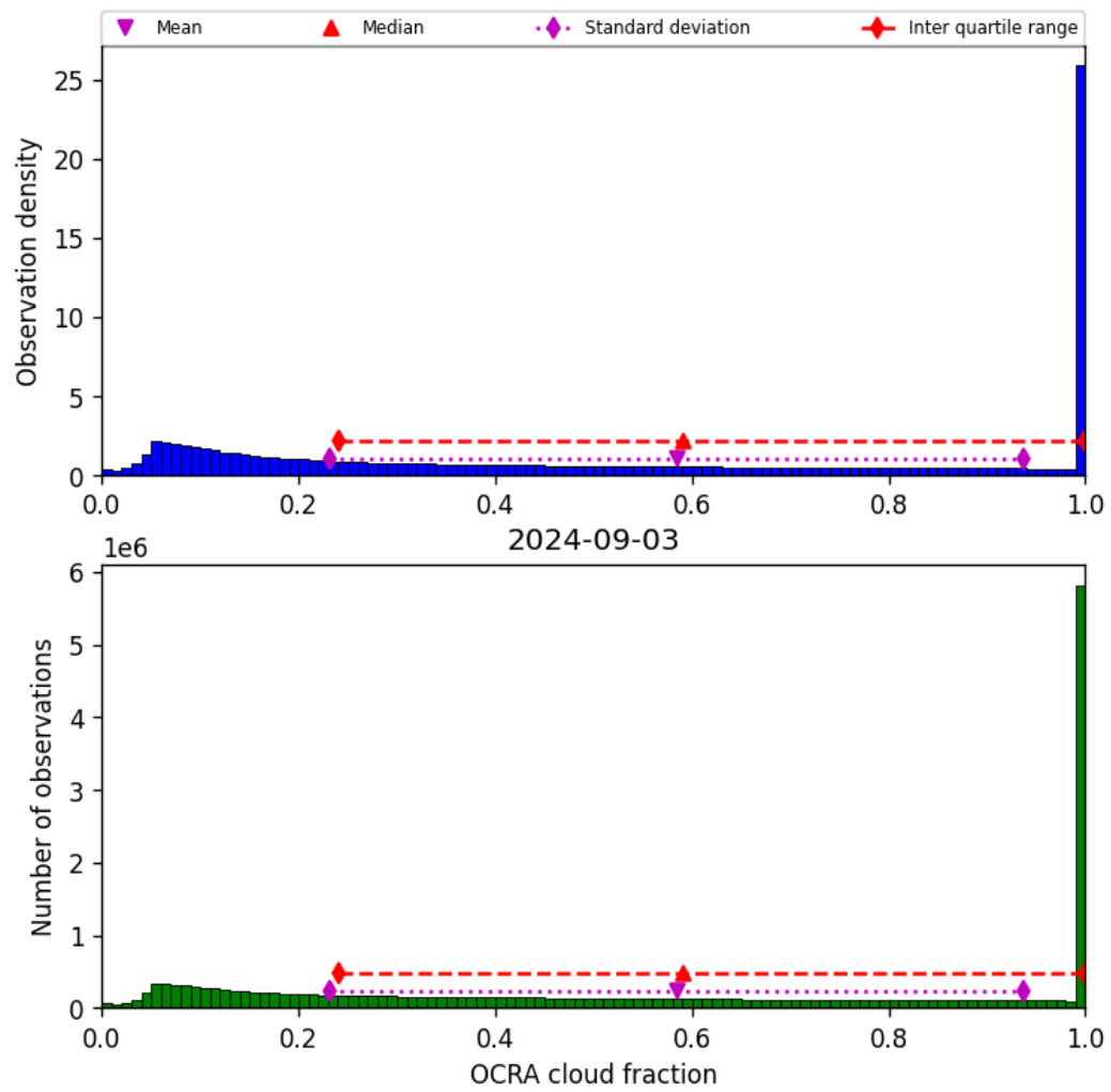
Figure 50: Histogram of “OCRA cloud fraction” for 2024-09-02 to 2024-09-04
