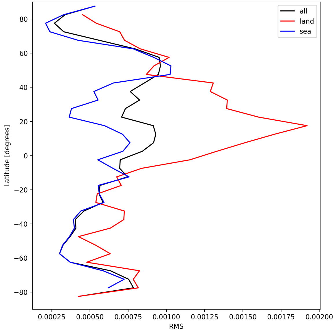
Figure 31: Zonal average of “RMS” for 2024-09-02 to 2024-09-04.
