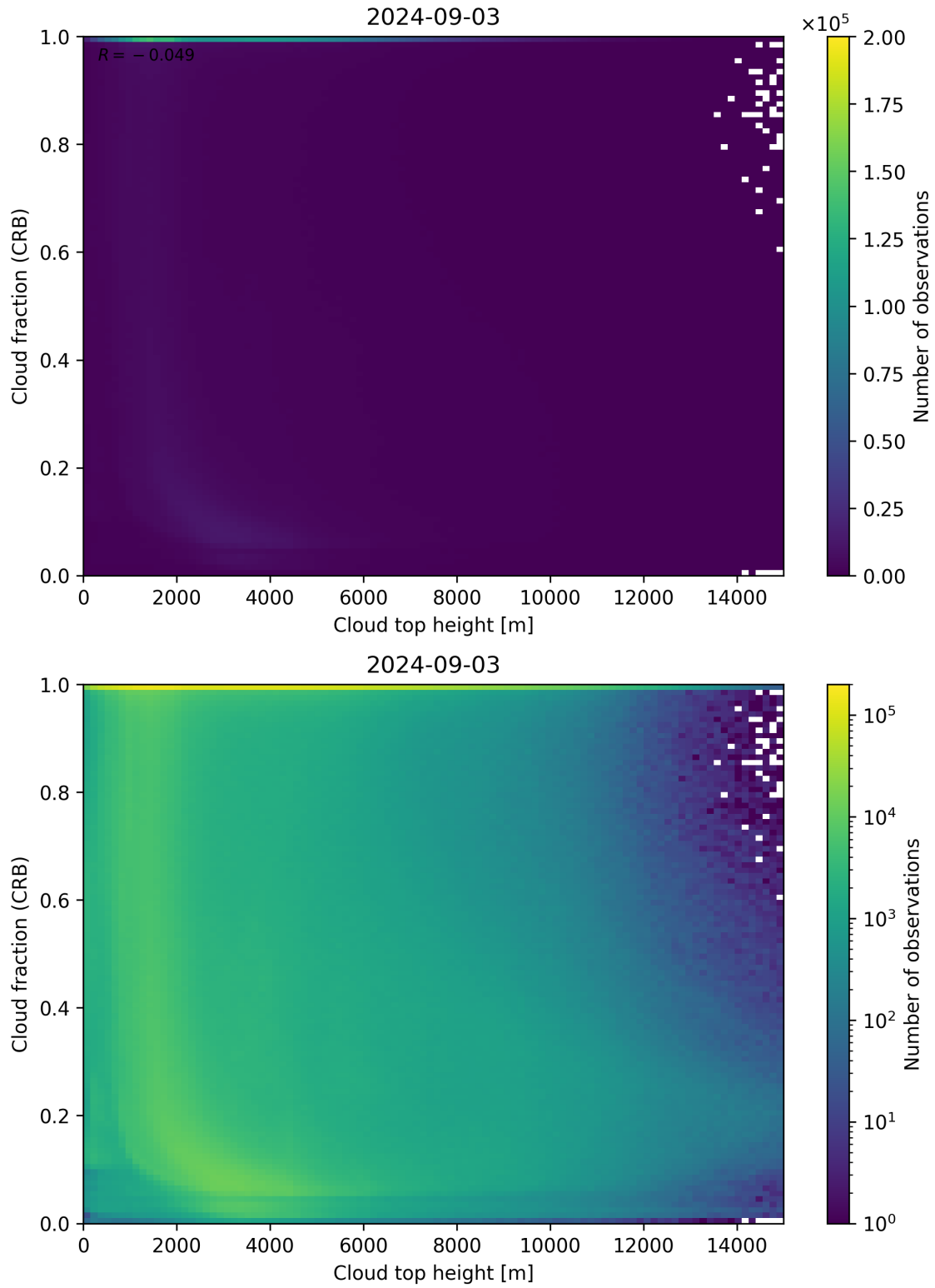
Figure 88: Scatter density plot of “Cloud top height” against “Cloud fraction (CRB)” for 2024-09-02 to 2024-09-04.
