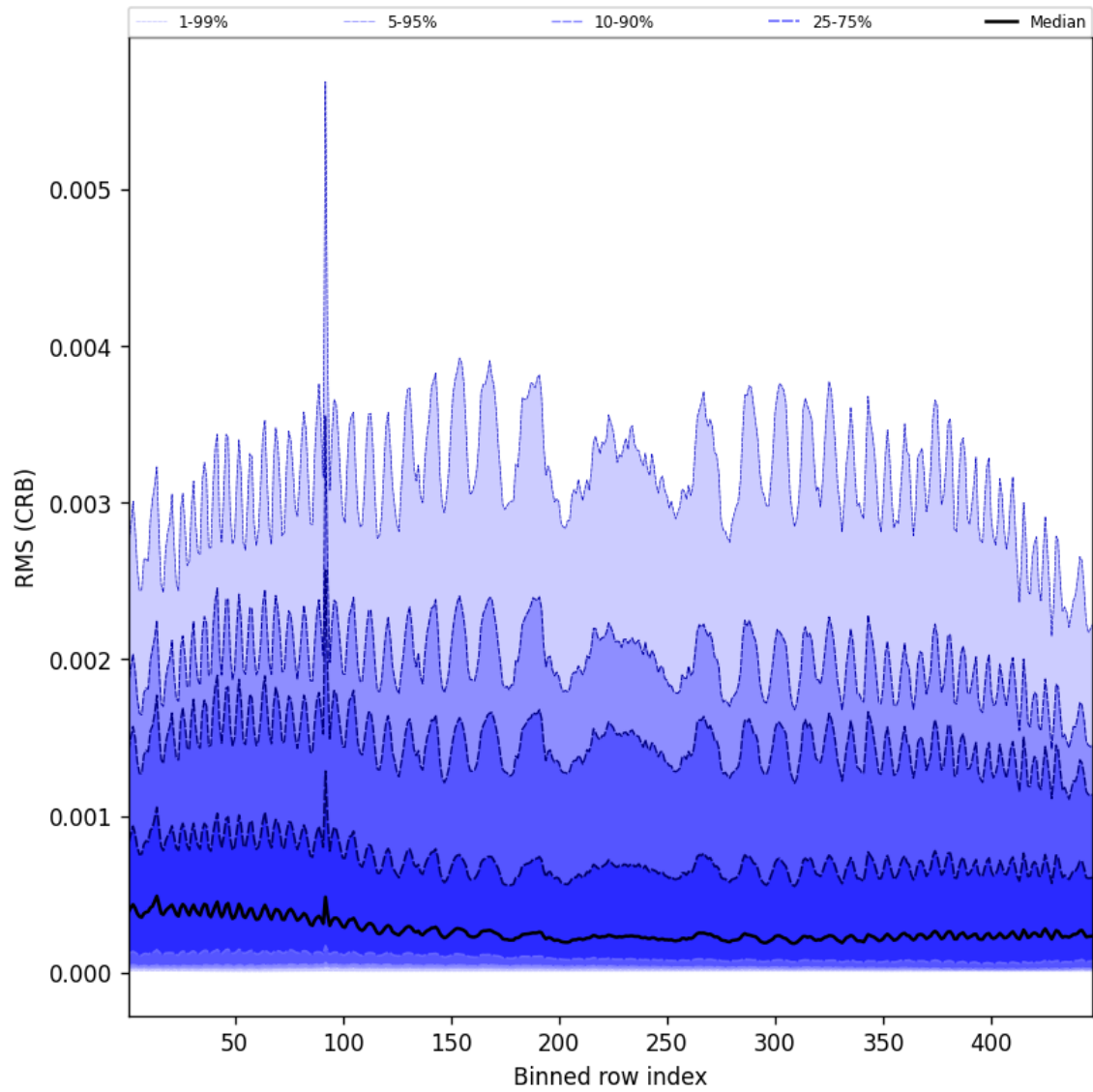
Figure 64: Along track statistics of “RMS (CRB)” for 2024-09-02 to 2024-09-04
