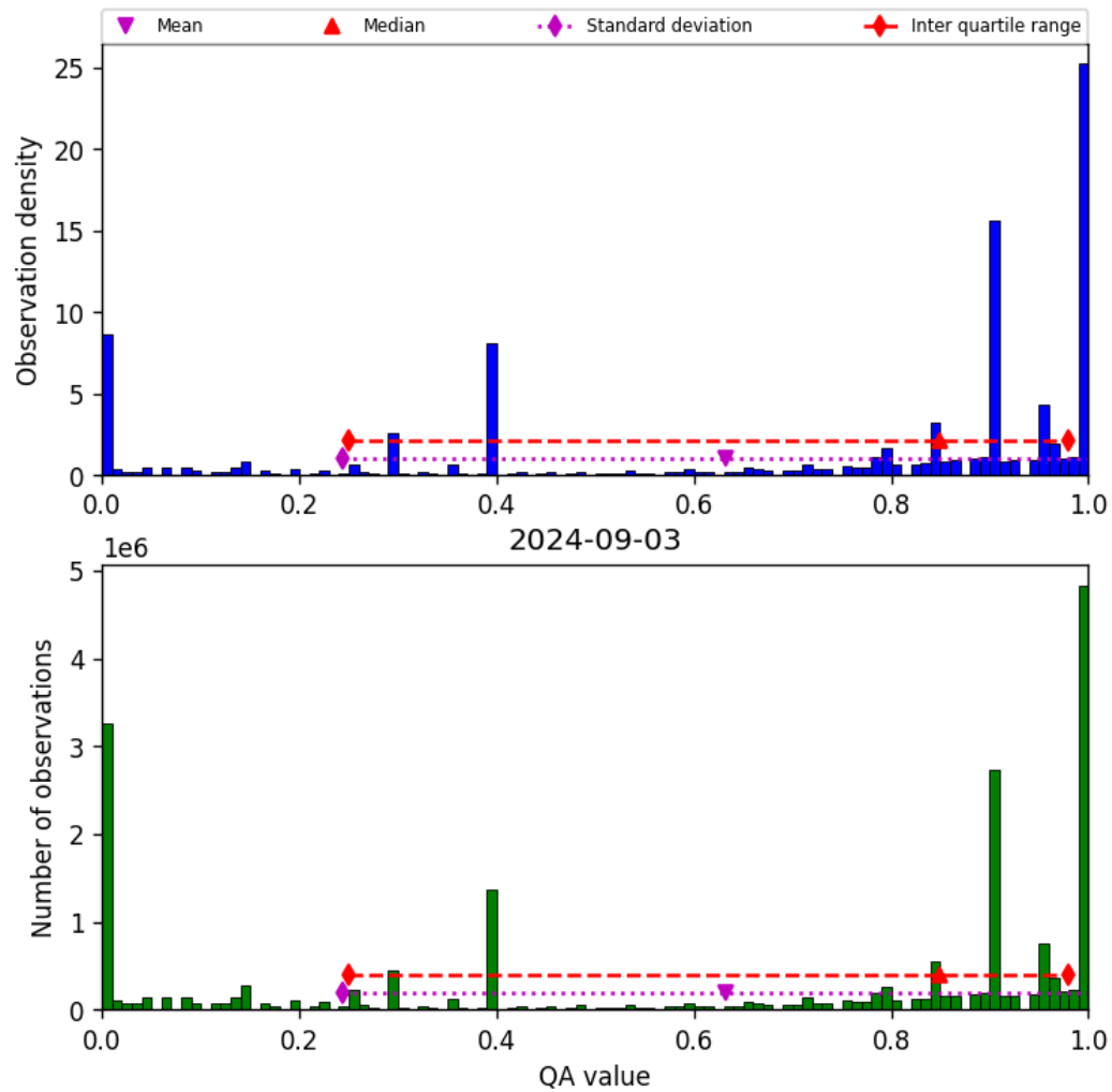
Figure 38: Histogram of “QA value” for 2024-09-02 to 2024-09-04
