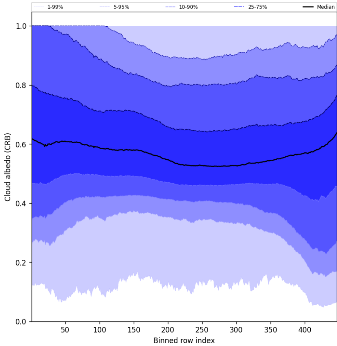
Figure 60: Along track statistics of “Cloud albedo (CRB)” for 2024-09-02 to 2024-09-04
