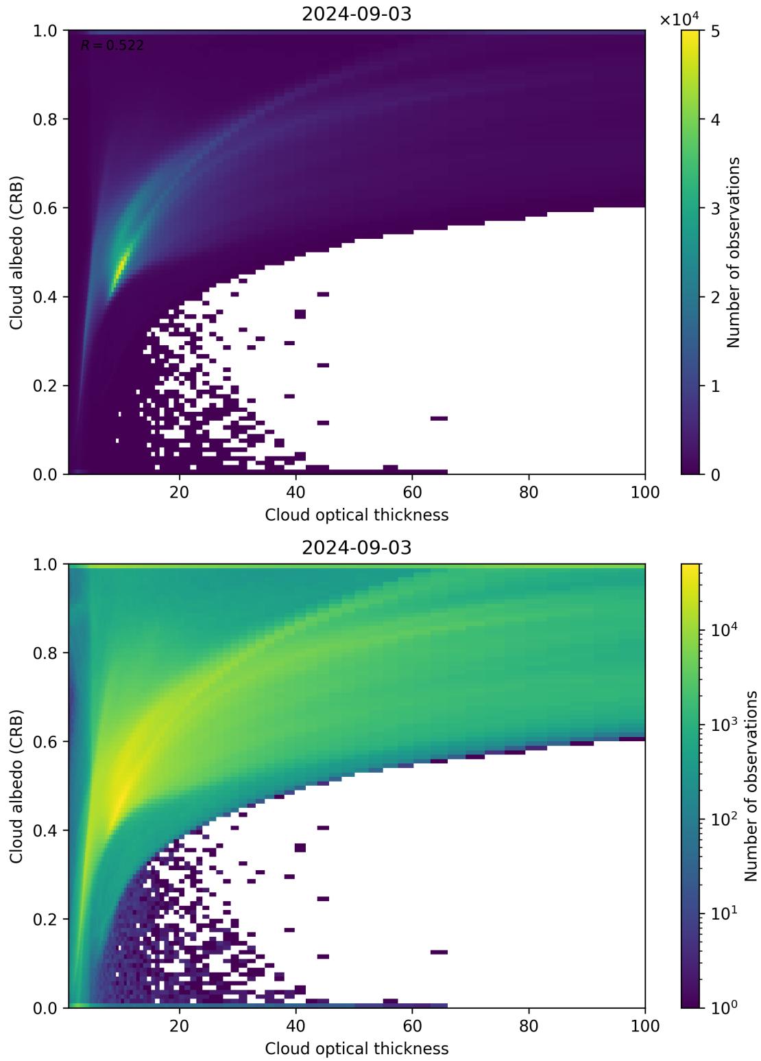
Figure 82: Scatter density plot of “Cloud optical thickness” against “Cloud albedo (CRB)” for 2024-09-02 to 2024-09-04.
