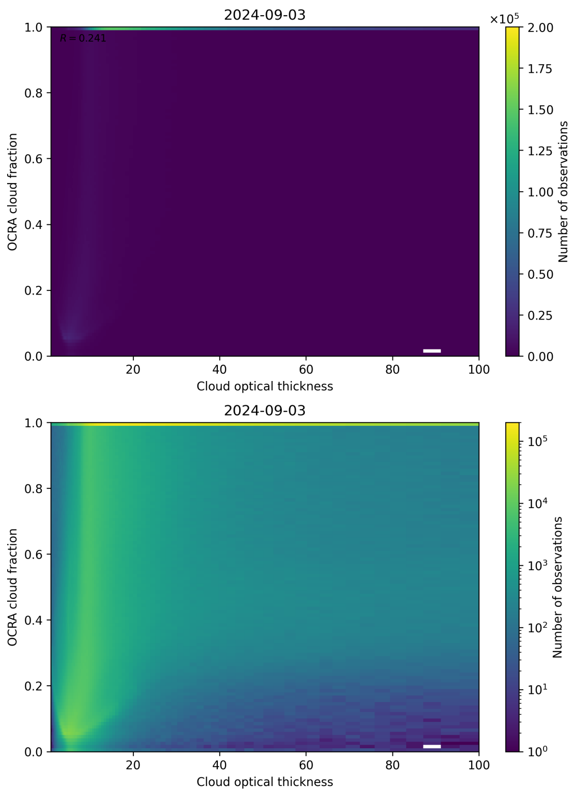
Figure 83: Scatter density plot of “Cloud optical thickness” against “OCRA cloud fraction” for 2024-09-02 to 2024-09-04.
