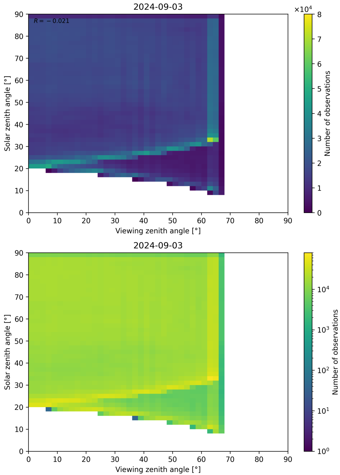
Figure 114: Scatter density plot of “Viewing zenith angle” against “Solar zenith angle” for 2024-09-02 to 2024-09-04.
