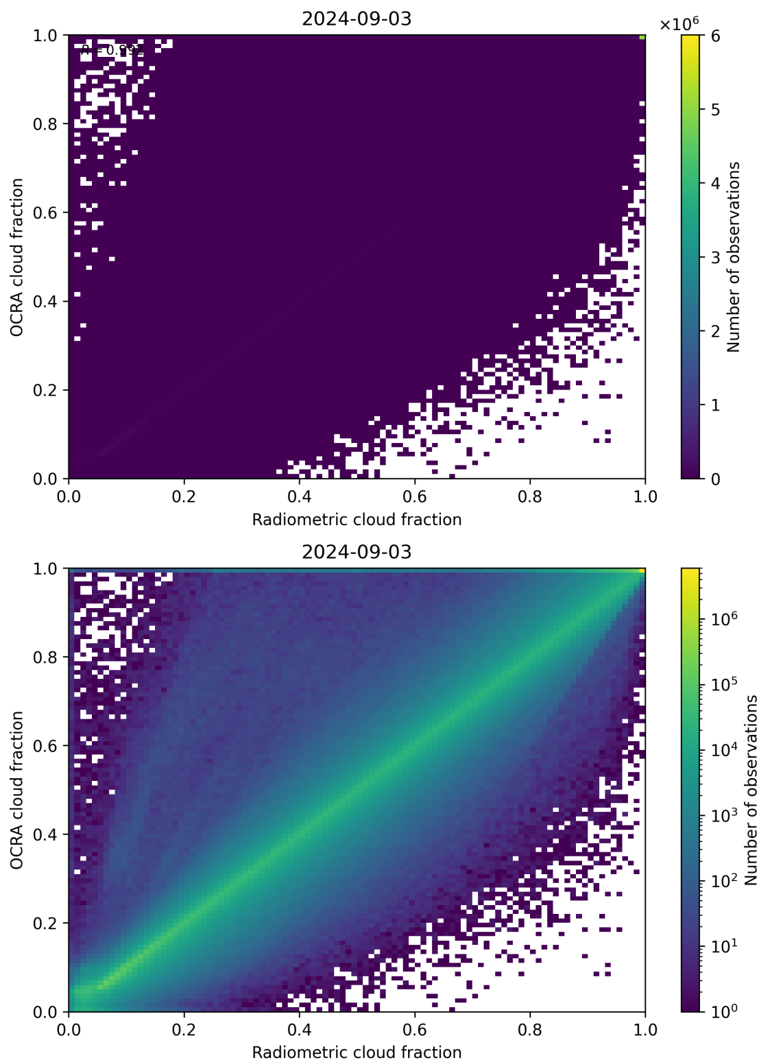
Figure 72: Scatter density plot of “Radiometric cloud fraction” against “OCRA cloud fraction” for 2024-09-02 to 2024-09-04.
