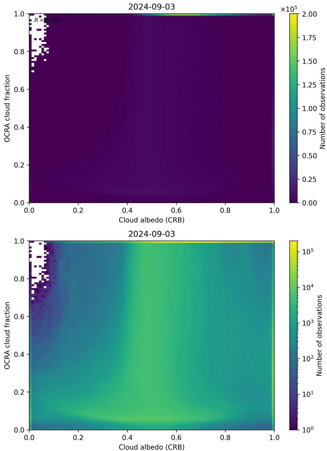
Figure 70: Scatter density plot of “Cloud albedo (CRB)” against “OCRA cloud fraction” for 2024-09-02 to 2024-09-04.
