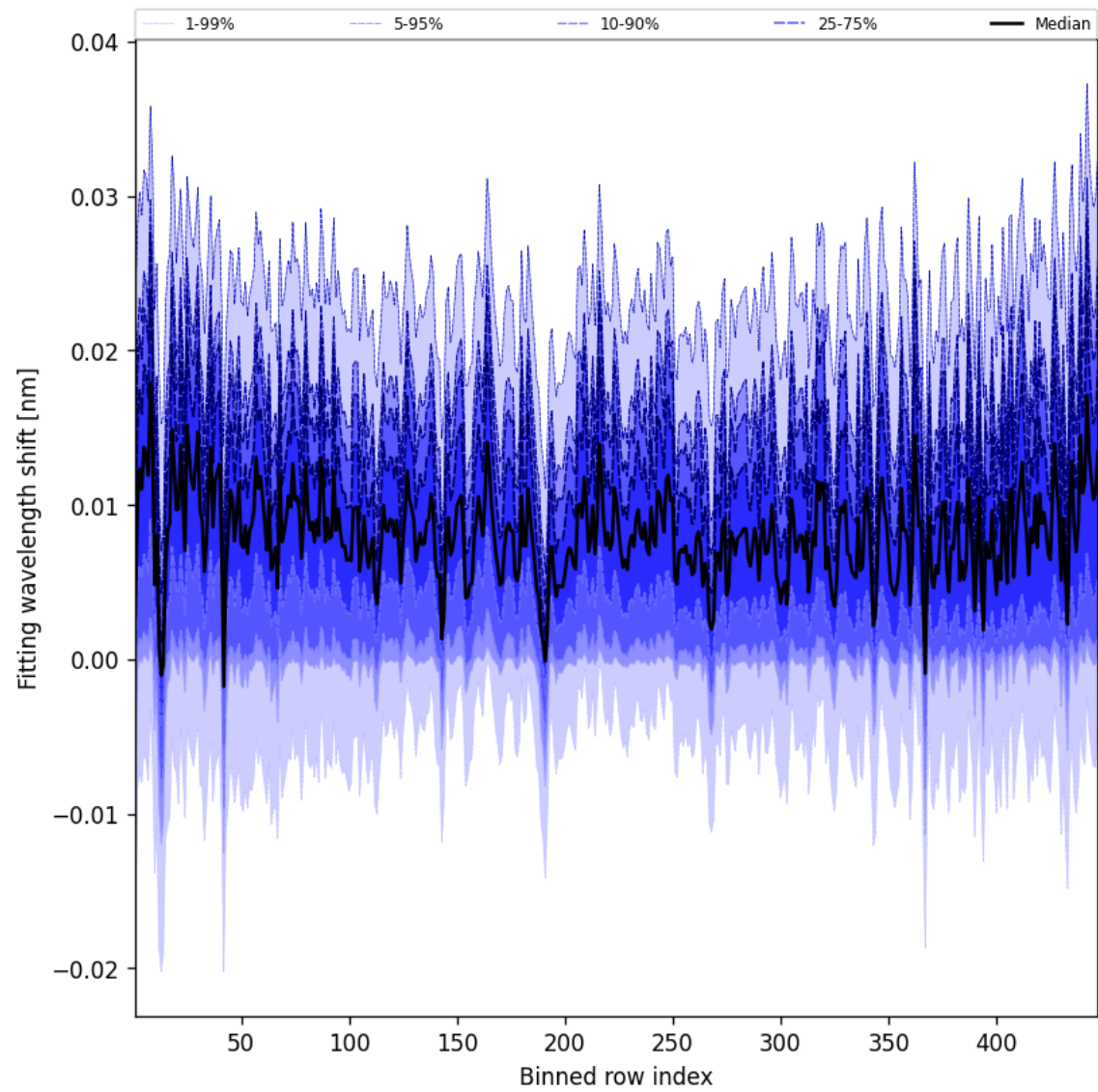
Figure 65: Along track statistics of “Fitting wavelength shift” for 2024-09-02 to 2024-09-04
