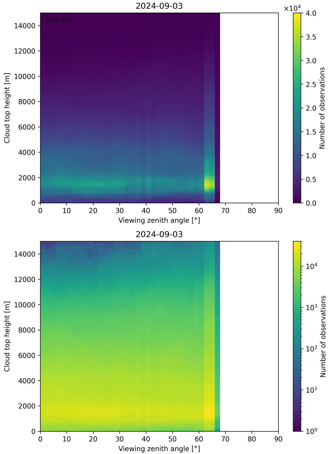
Figure 112: Scatter density plot of “Viewing zenith angle” against “Cloud top height” for 2024-09-02 to 2024-09-04.
