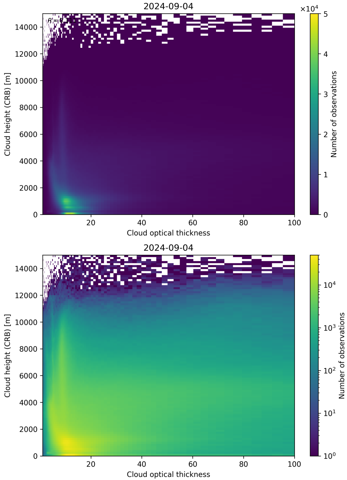
Figure 85: Scatter density plot of “Cloud optical thickness” against “Cloud height (CRB)” for 2024-09-03 to 2024-09-05.
