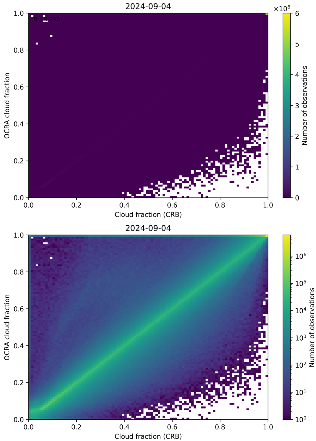
Figure 78: Scatter density plot of “Cloud fraction (CRB)” against “OCRA cloud fraction” for 2024-09-03 to 2024-09-05.
