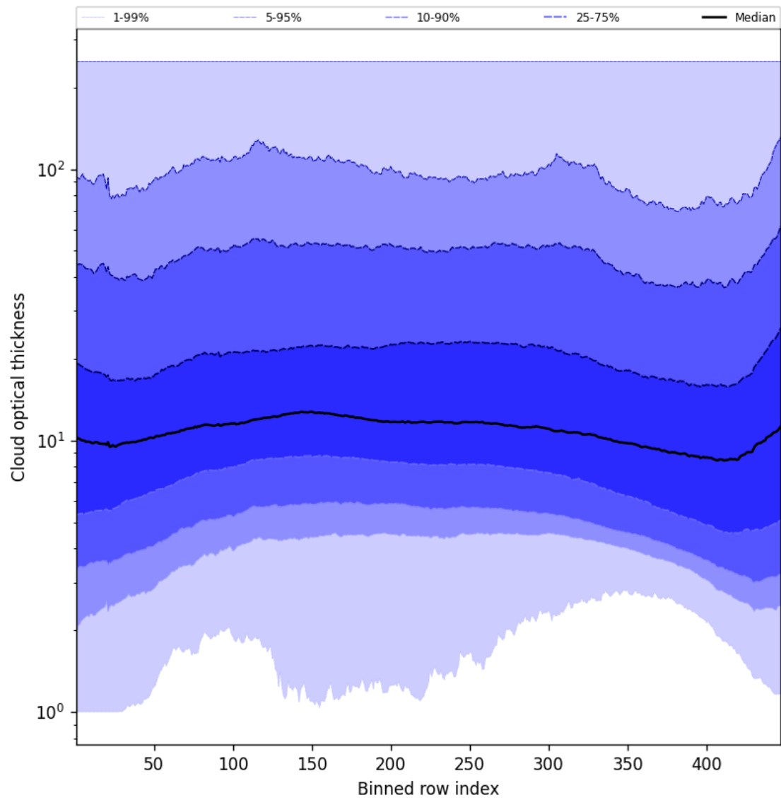
Figure 57: Along track statistics of “Cloud optical thickness” for 2024-09-03 to 2024-09-05
