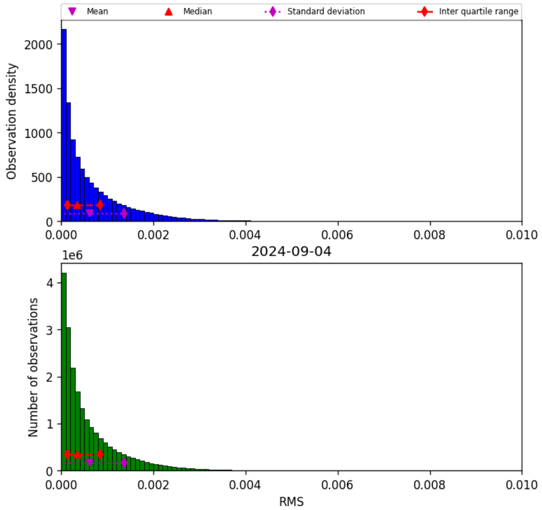
Figure 47: Histogram of “RMS” for 2024-09-03 to 2024-09-05
