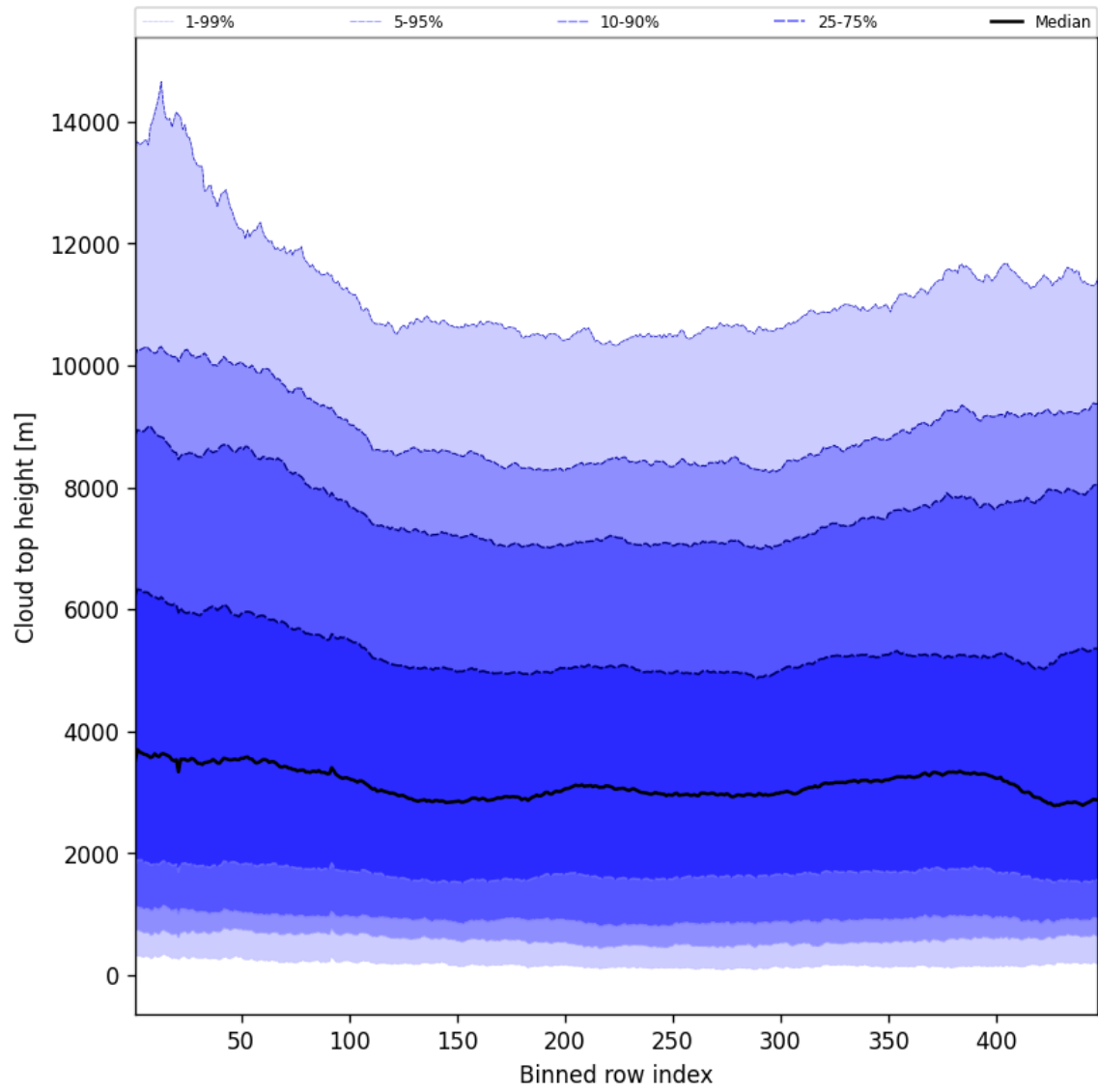
Figure 56: Along track statistics of “Cloud top height” for 2024-09-03 to 2024-09-05
