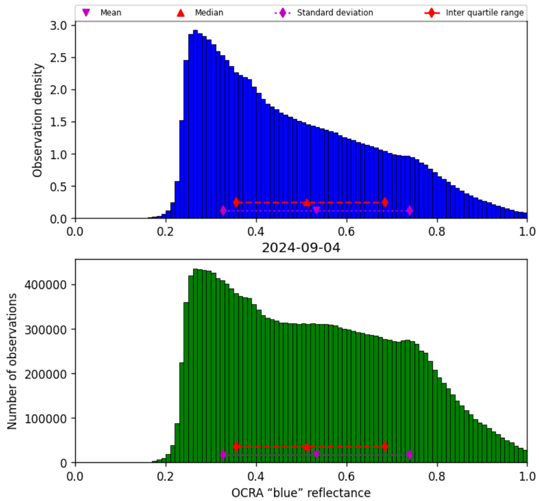
Figure 51: Histogram of “OCRA “blue” reflectance” for 2024-09-03 to 2024-09-05
