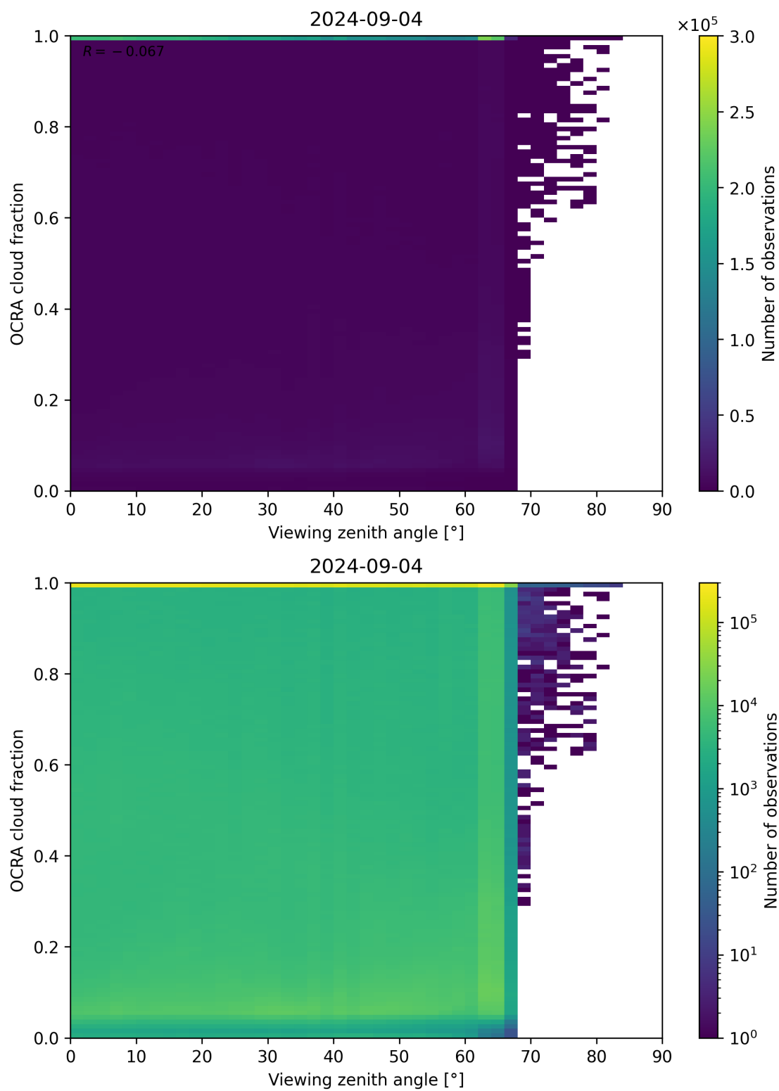
Figure 108: Scatter density plot of “Viewing zenith angle” against “OCRA cloud fraction” for 2024-09-03 to 2024-09-05.
