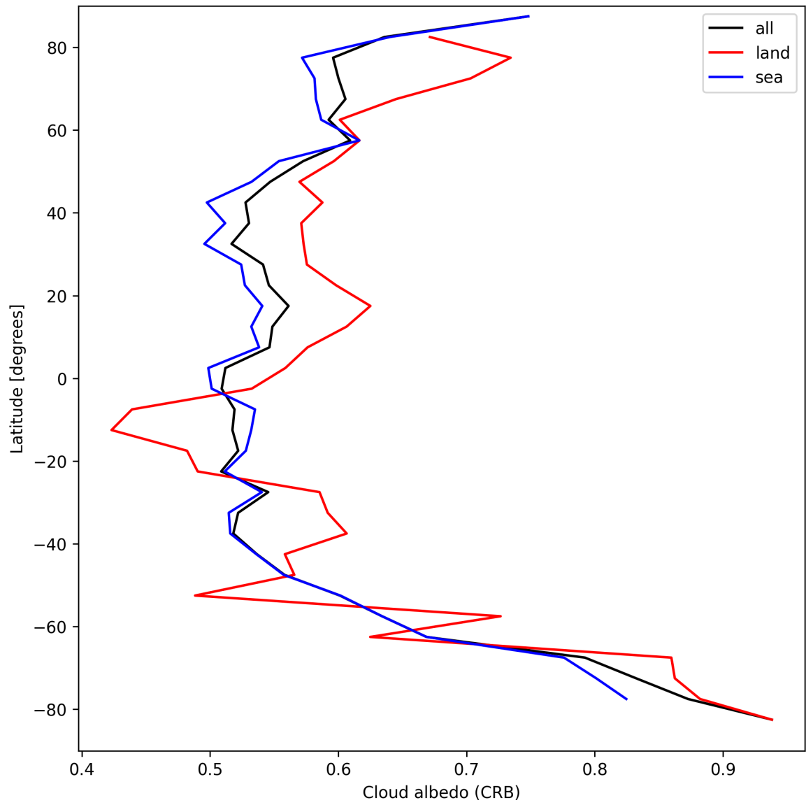
Figure 28: Zonal average of “Cloud albedo (CRB)” for 2024-09-03 to 2024-09-05.
