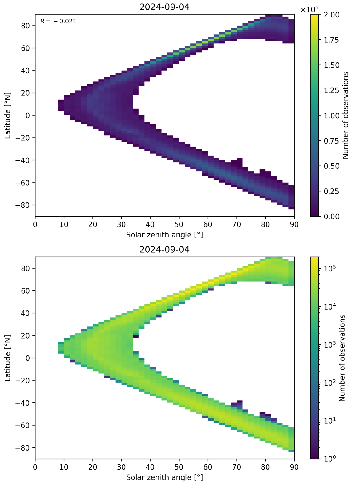
Figure 105: Scatter density plot of “Solar zenith angle” against “Latitude” for 2024-09-03 to 2024-09-05.
