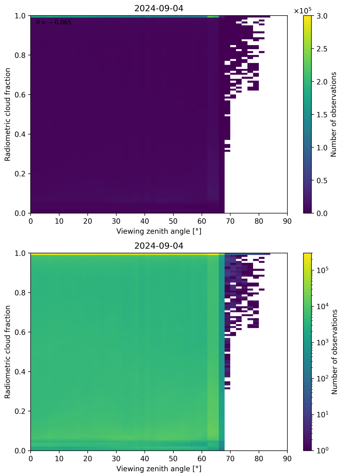
Figure 107: Scatter density plot of “Viewing zenith angle” against “Radiometric cloud fraction” for 2024-09-03 to 2024-09-05.
