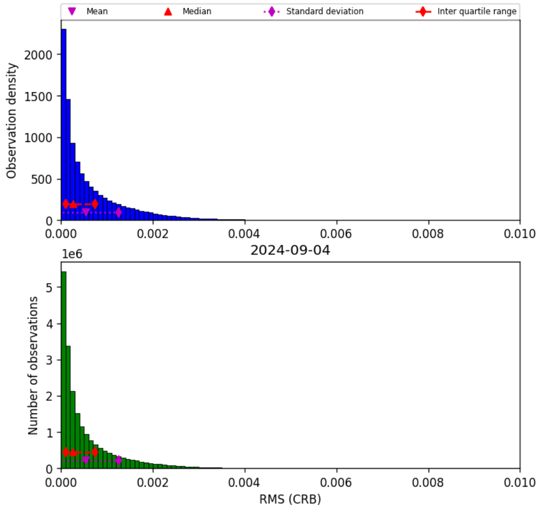
Figure 48: Histogram of “RMS (CRB)” for 2024-09-03 to 2024-09-05
