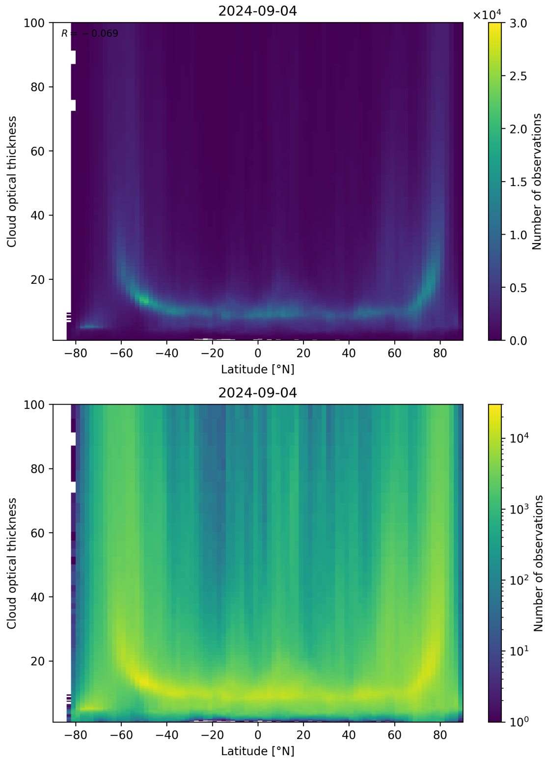
Figure 96: Scatter density plot of “Latitude” against “Cloud optical thickness” for 2024-09-03 to 2024-09-05.
