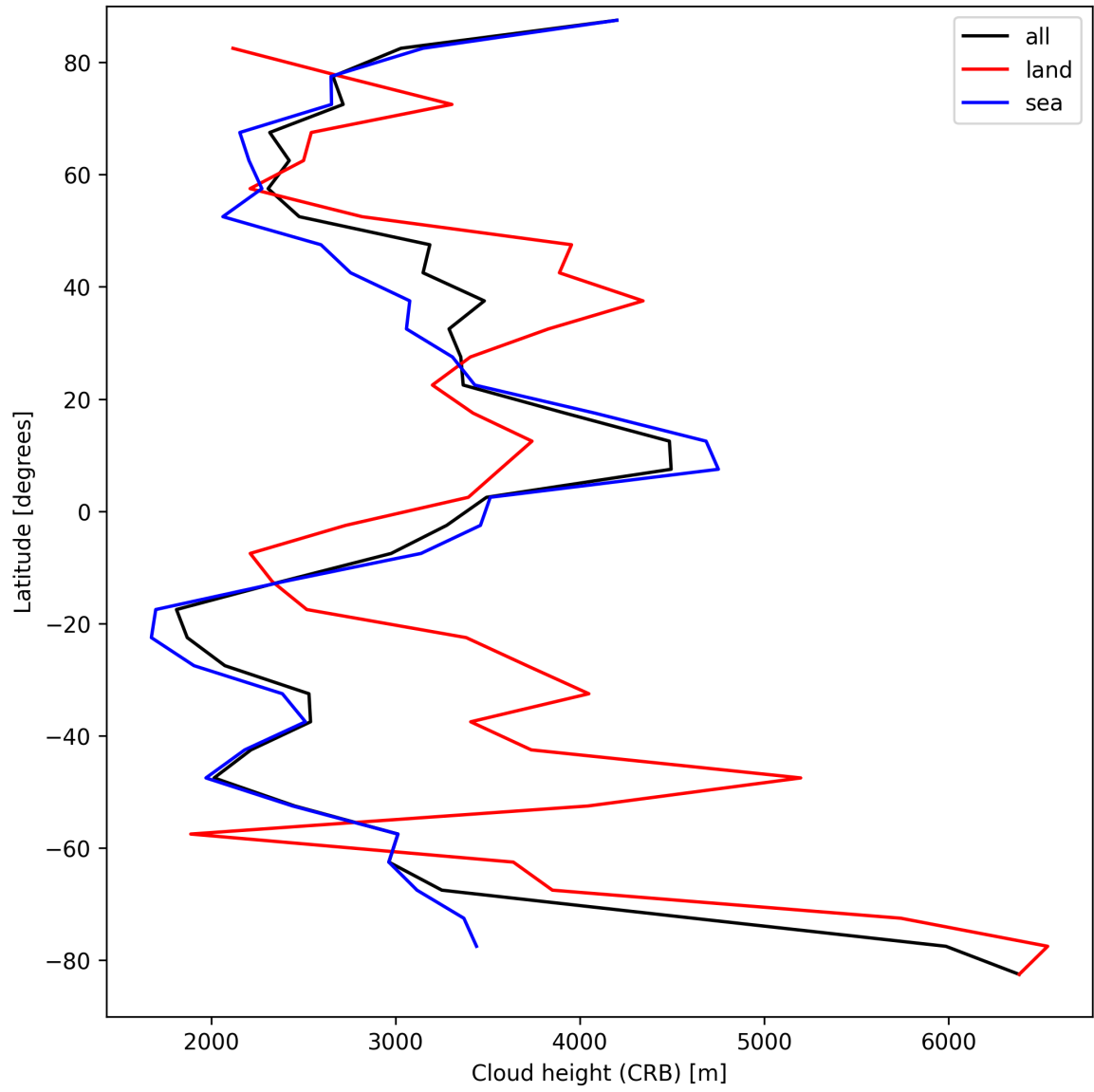
Figure 27: Zonal average of “Cloud height (CRB)” for 2024-09-03 to 2024-09-05.
