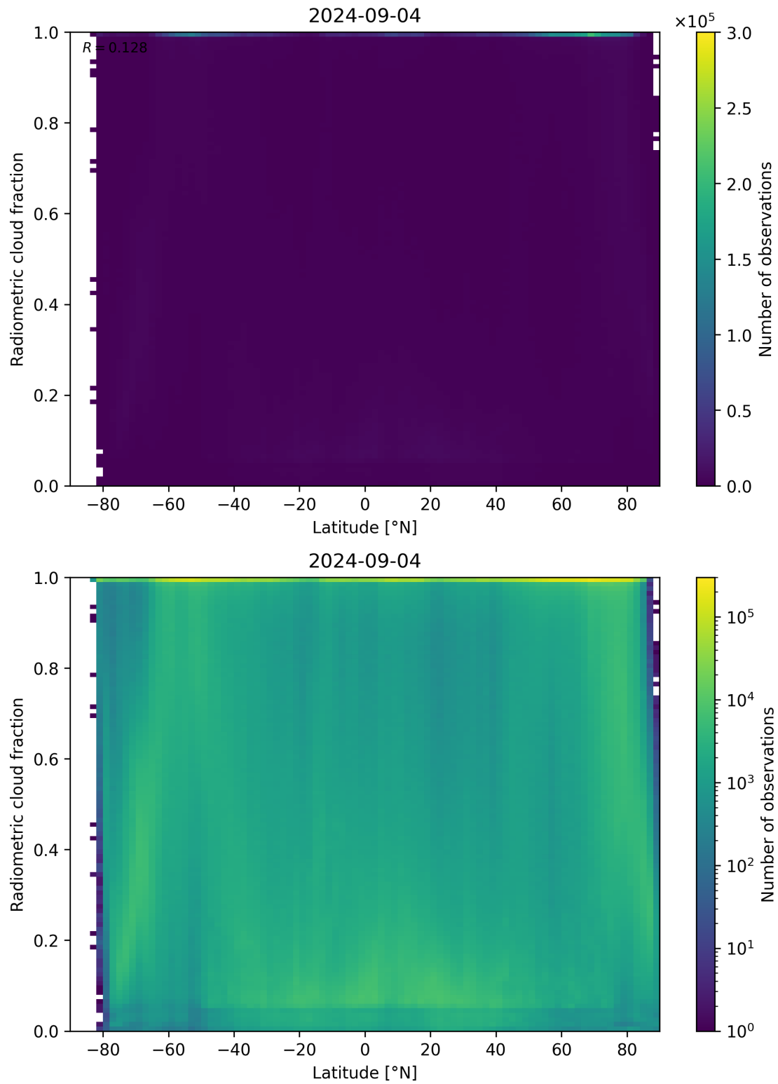
Figure 92: Scatter density plot of “Latitude” against “Radiometric cloud fraction” for 2024-09-03 to 2024-09-05.
