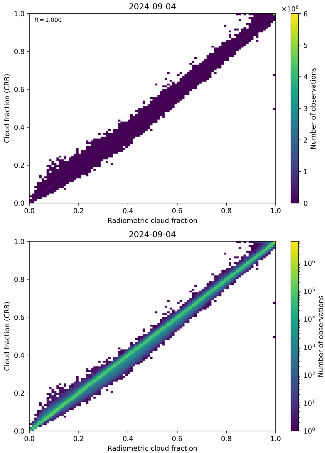
Figure 73: Scatter density plot of “Radiometric cloud fraction” against “Cloud fraction (CRB)” for 2024-09-03 to 2024-09-05.
