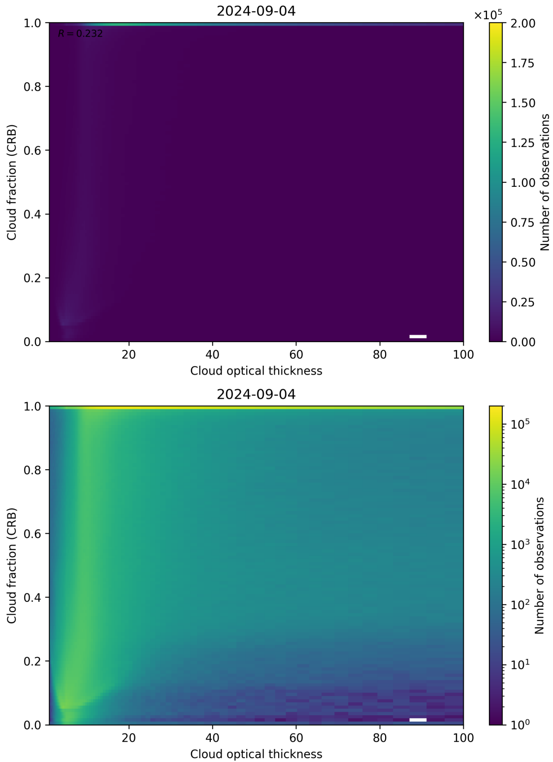
Figure 84: Scatter density plot of “Cloud optical thickness” against “Cloud fraction (CRB)” for 2024-09-03 to 2024-09-05.
