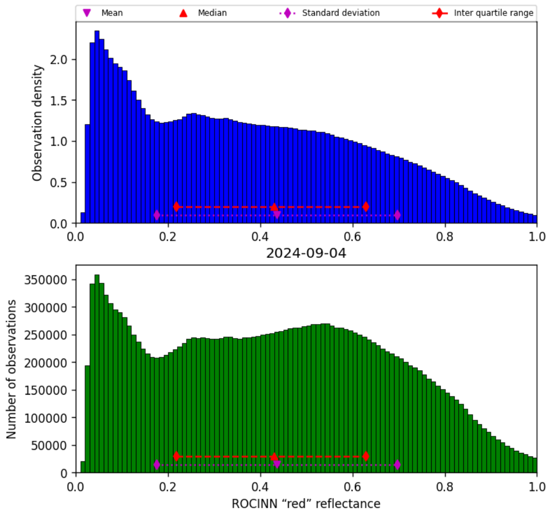
Figure 53: Histogram of “ROCINN “red” reflectance” for 2024-09-03 to 2024-09-05
