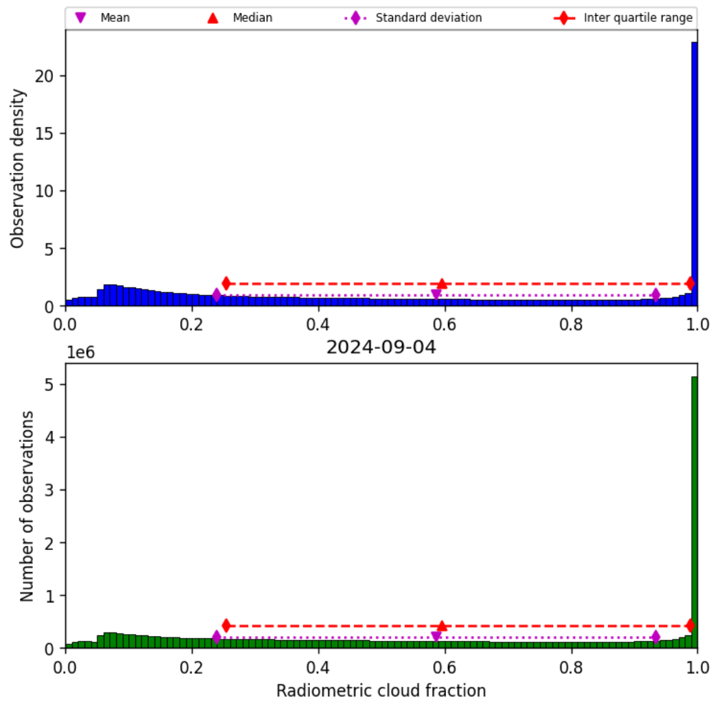
Figure 39: Histogram of “Radiometric cloud fraction” for 2024-09-03 to 2024-09-05
