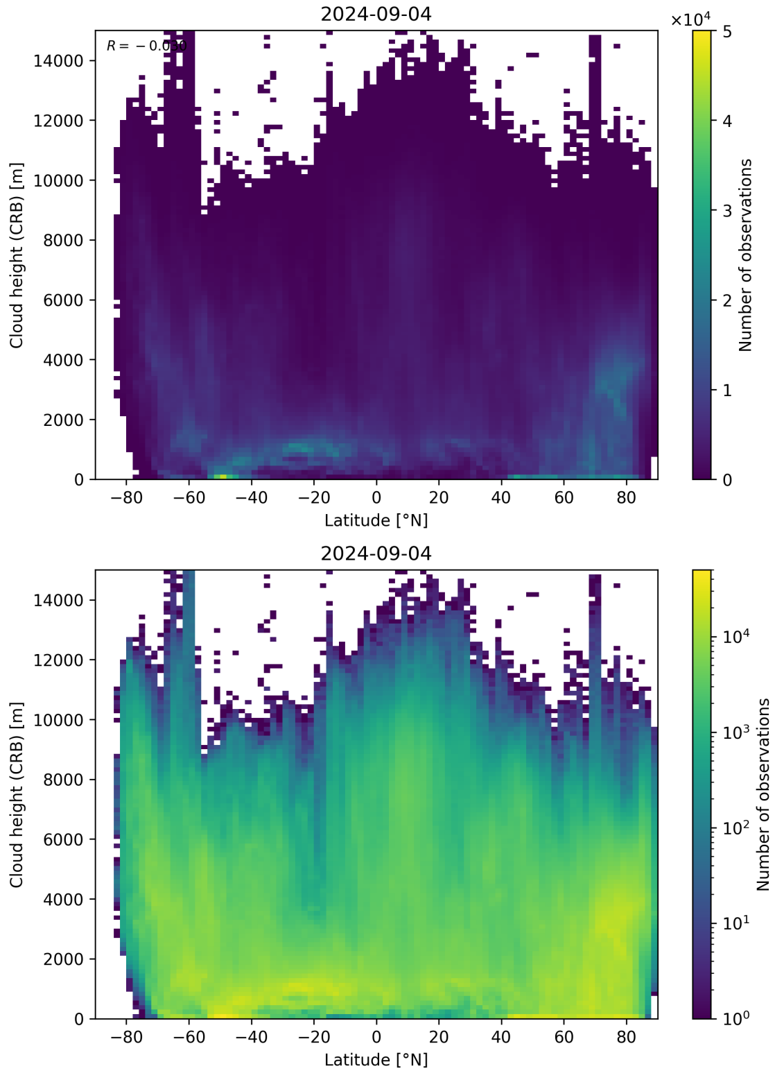
Figure 95: Scatter density plot of “Latitude” against “Cloud height (CRB)” for 2024-09-03 to 2024-09-05.
