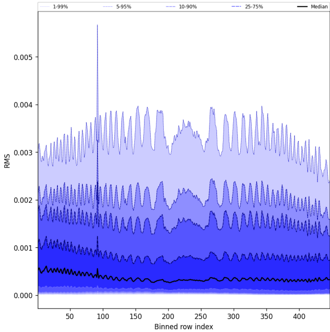
Figure 63: Along track statistics of “RMS” for 2024-09-03 to 2024-09-05
