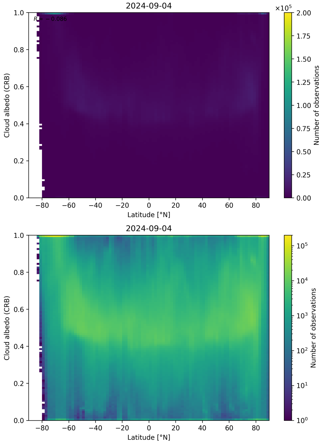
Figure 91: Scatter density plot of “Latitude” against “Cloud albedo (CRB)” for 2024-09-03 to 2024-09-05.
