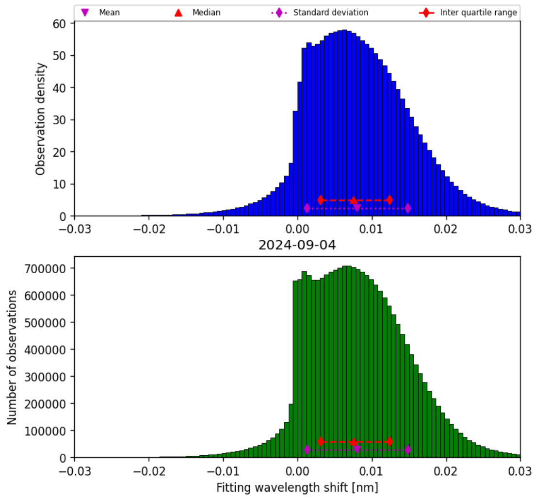
Figure 49: Histogram of “Fitting wavelength shift” for 2024-09-03 to 2024-09-05
