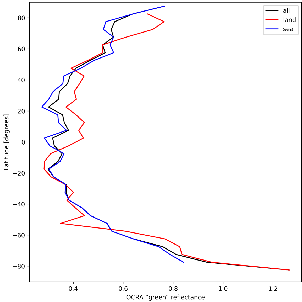
Figure 36: Zonal average of “OCRA “green” reflectance” for 2024-09-03 to 2024-09-05.
