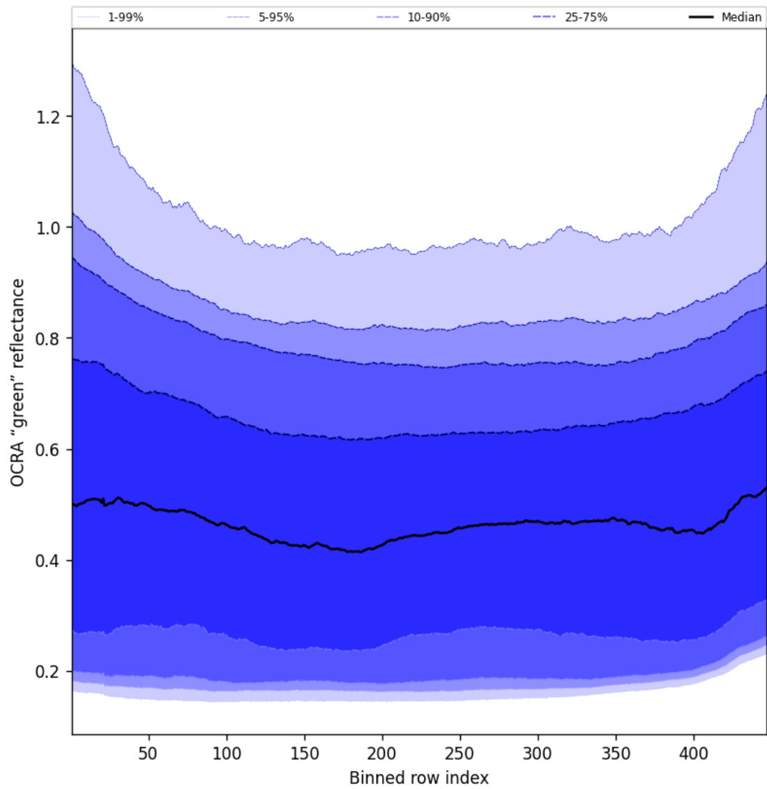
Figure 68: Along track statistics of “OCRA “green” reflectance” for 2024-09-03 to 2024-09-05
