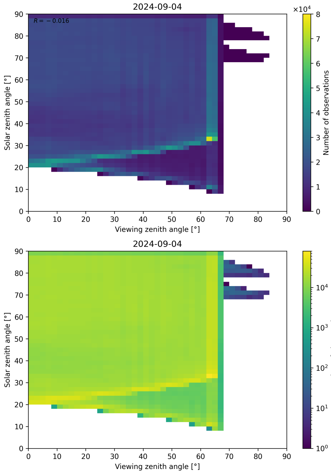
Figure 114: Scatter density plot of “Viewing zenith angle” against “Solar zenith angle” for 2024-09-03 to 2024-09-05.
