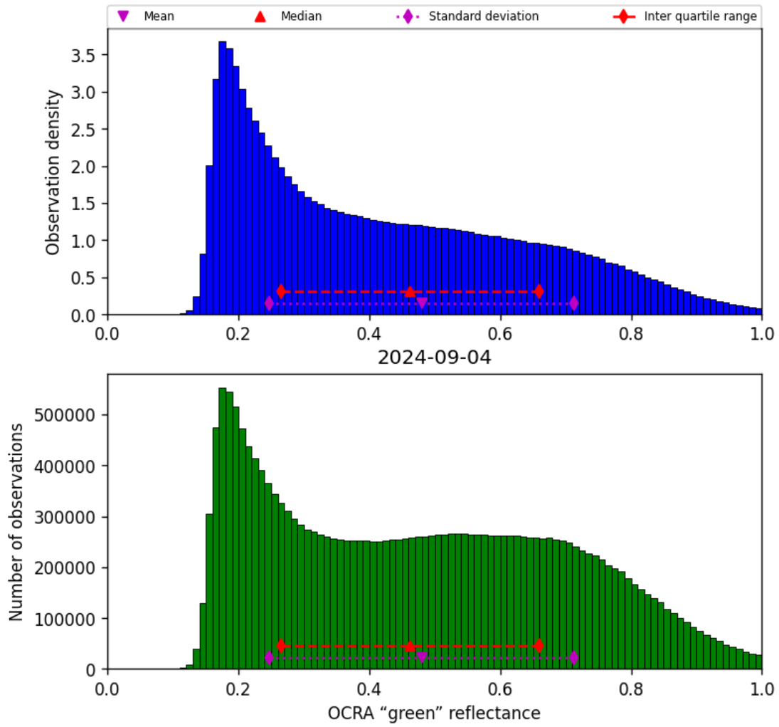
Figure 52: Histogram of “OCRA “green” reflectance” for 2024-09-03 to 2024-09-05
