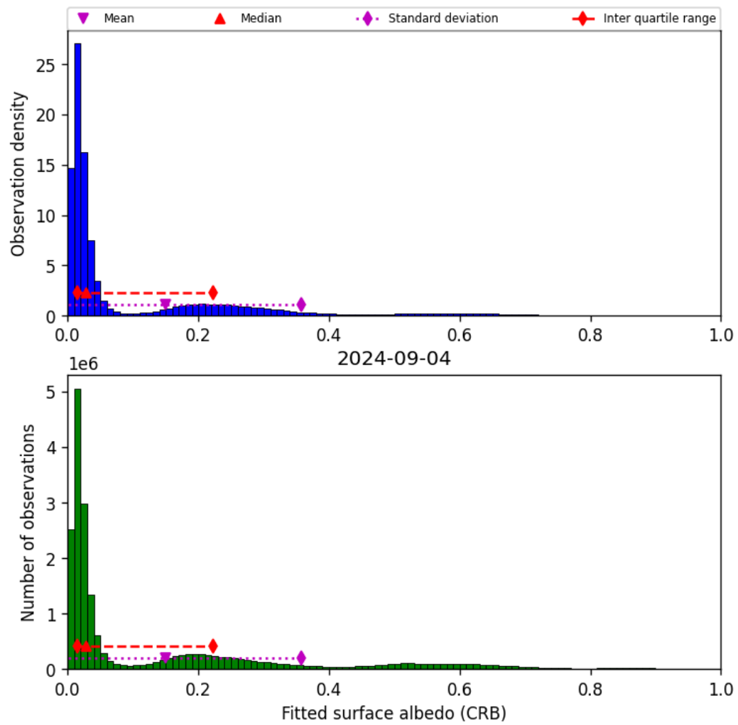
Figure 46: Histogram of “Fitted surface albedo (CRB)” for 2024-09-03 to 2024-09-05
