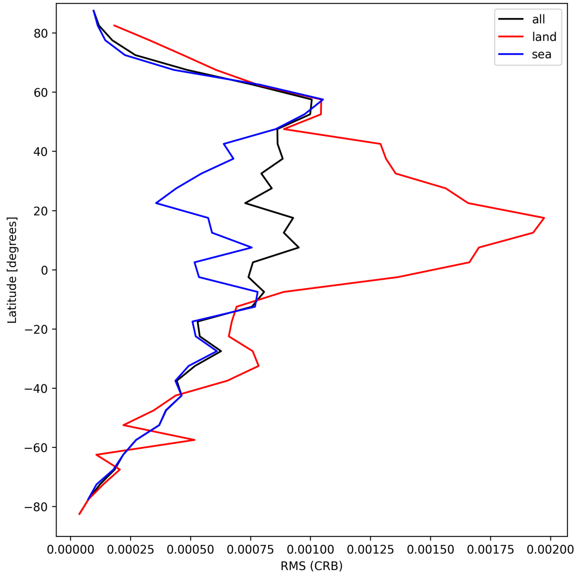
Figure 32: Zonal average of “RMS (CRB)” for 2024-09-03 to 2024-09-05.
