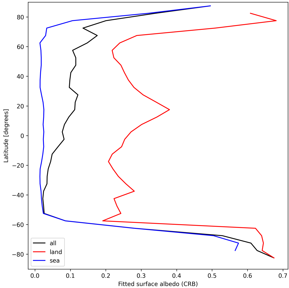
Figure 30: Zonal average of “Fitted surface albedo (CRB)” for 2024-09-03 to 2024-09-05.
