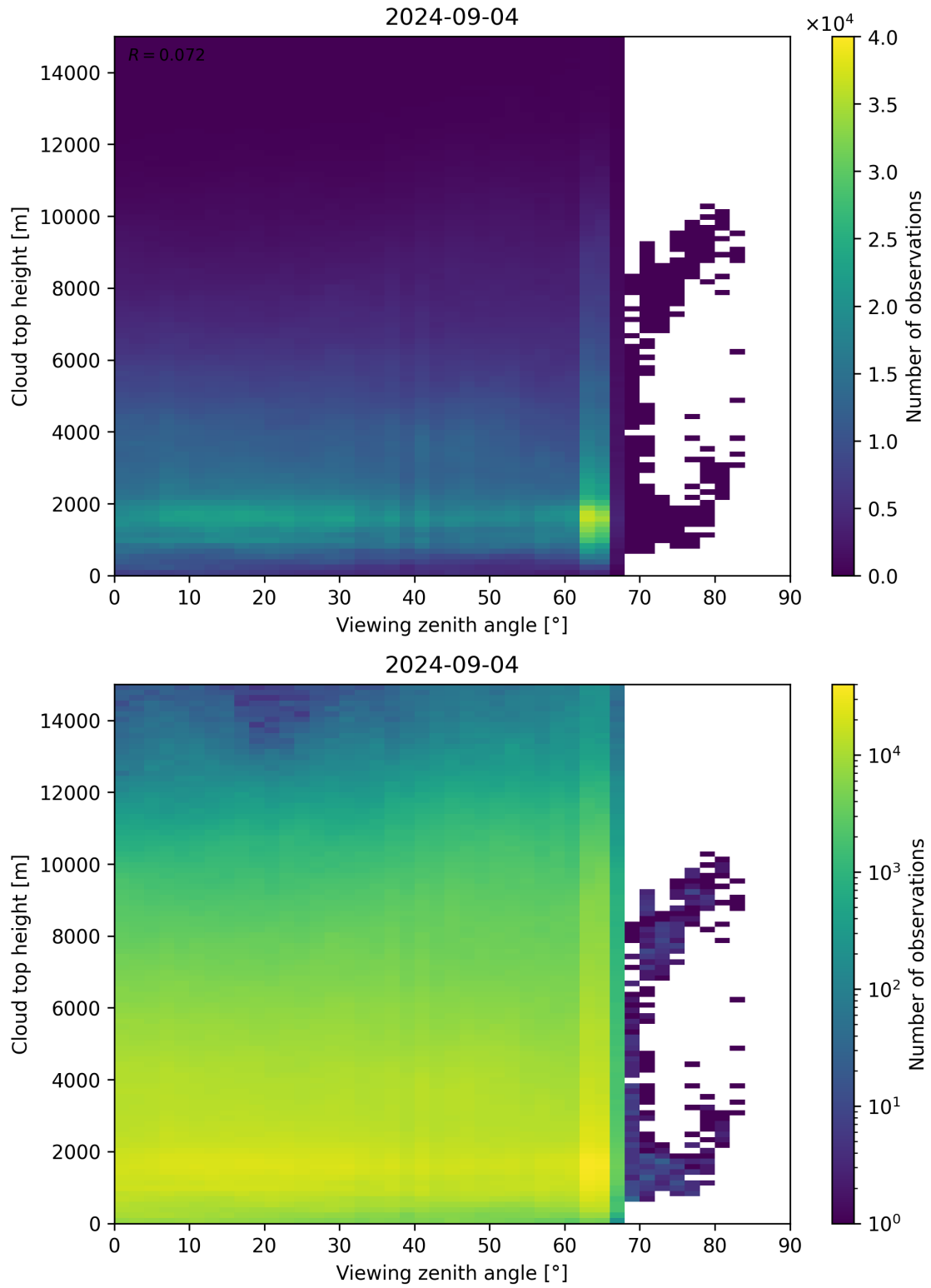
Figure 112: Scatter density plot of “Viewing zenith angle” against “Cloud top height” for 2024-09-03 to 2024-09-05.
