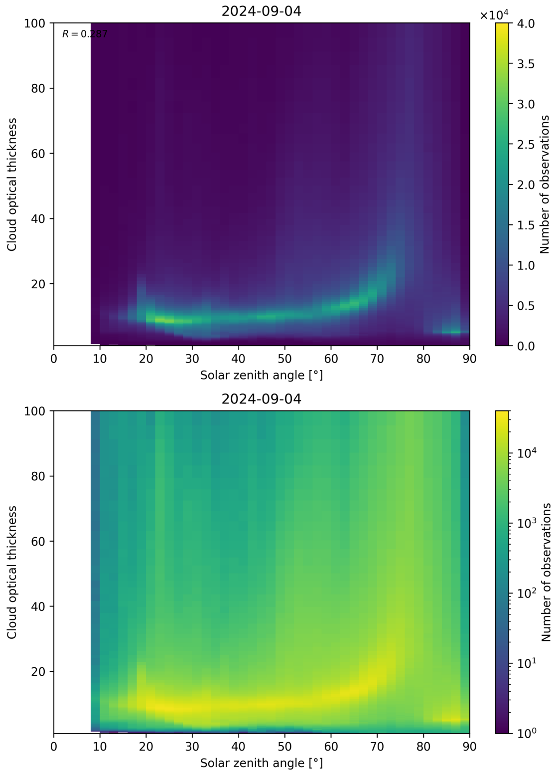
Figure 103: Scatter density plot of “Solar zenith angle” against “Cloud optical thickness” for 2024-09-03 to 2024-09-05.
