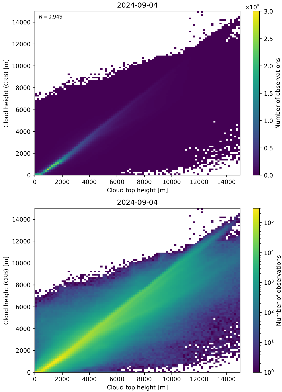
Figure 89: Scatter density plot of “Cloud top height” against “Cloud height (CRB)” for 2024-09-03 to 2024-09-05.
