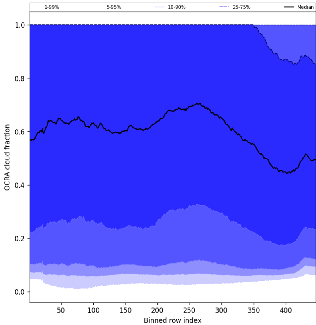
Figure 66: Along track statistics of “OCRA cloud fraction” for 2024-09-03 to 2024-09-05
