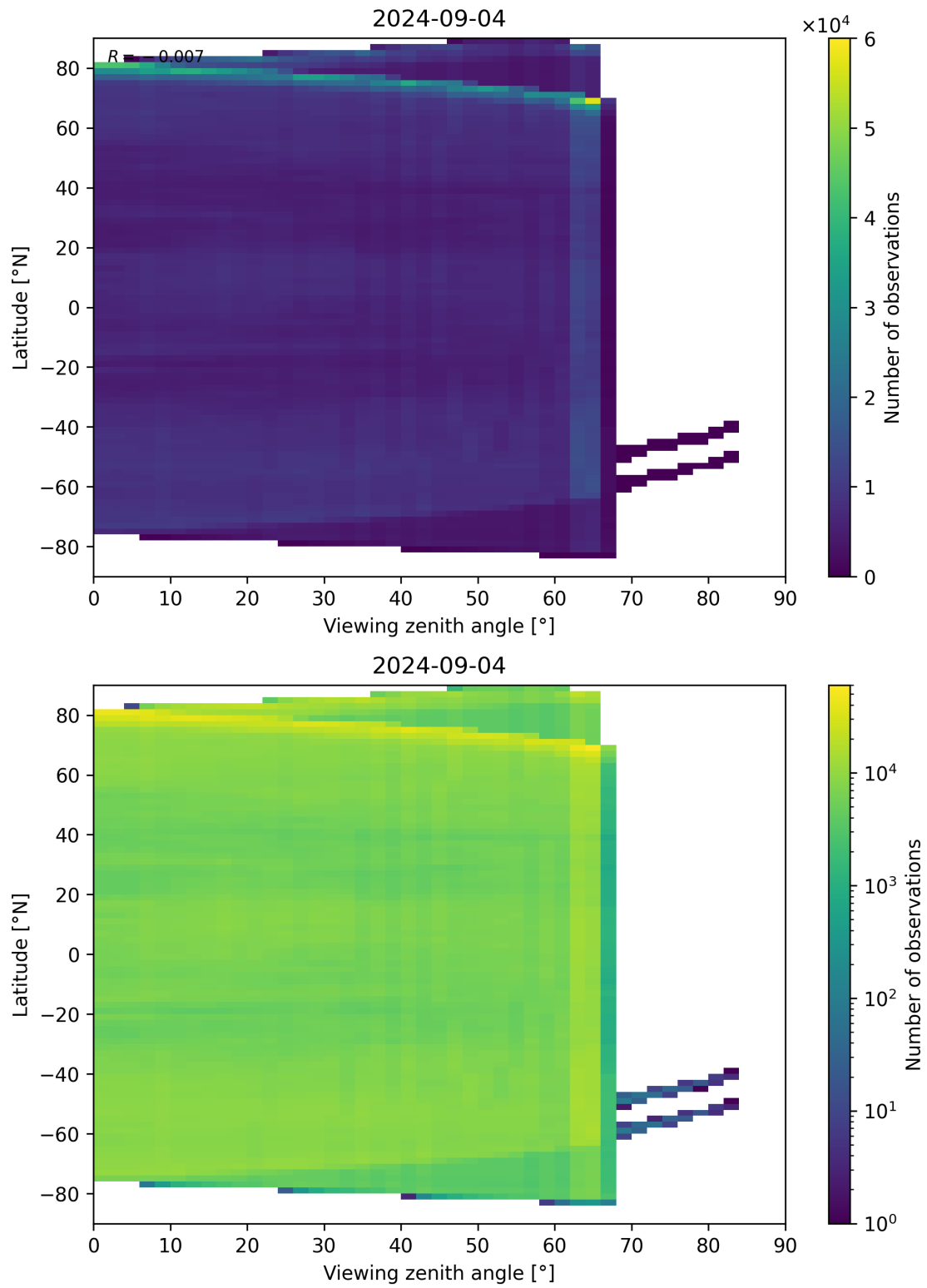
Figure 113: Scatter density plot of “Viewing zenith angle” against “Latitude” for 2024-09-03 to 2024-09-05.
