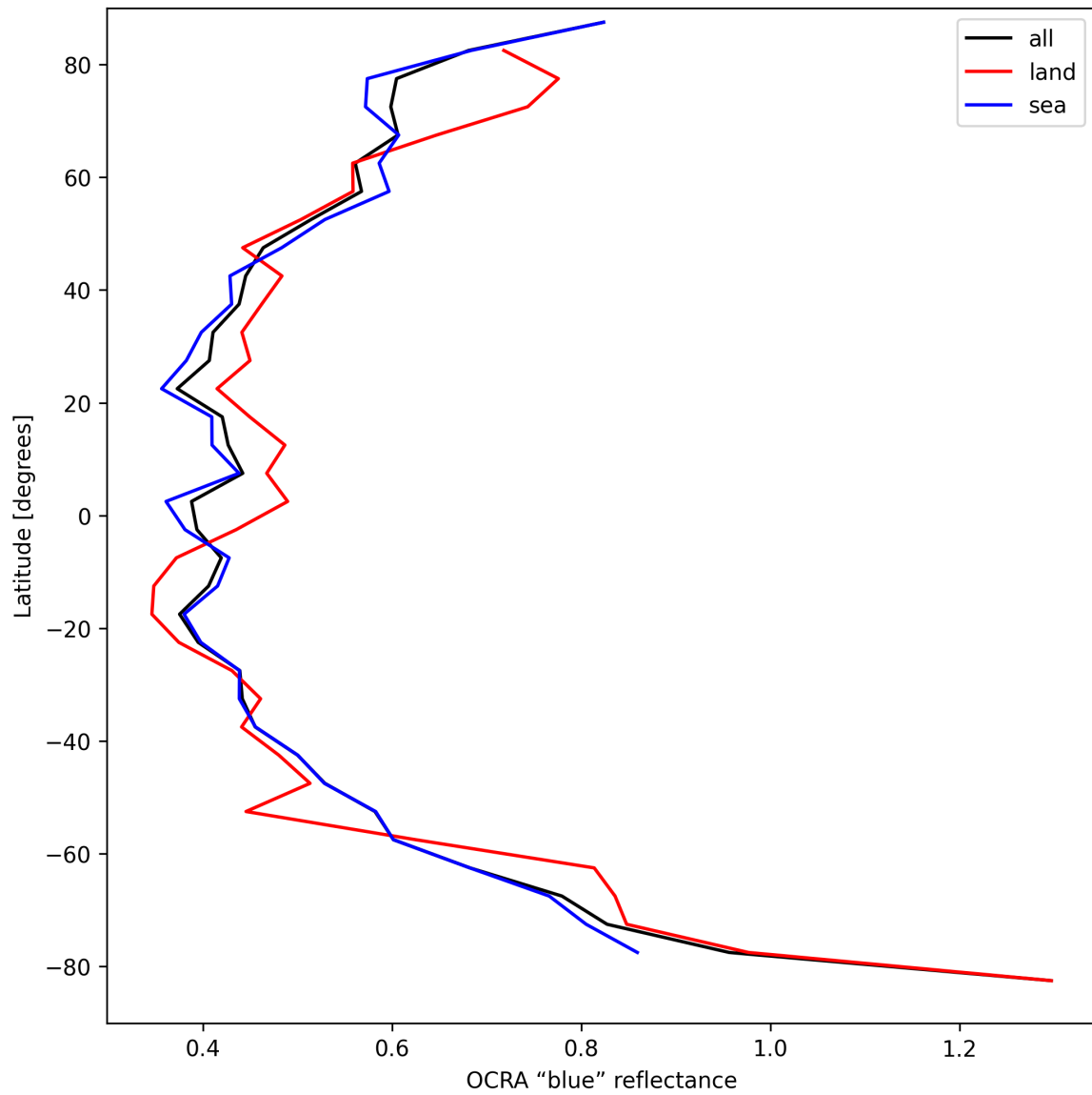
Figure 35: Zonal average of “OCRA “blue” reflectance” for 2024-09-03 to 2024-09-05.
