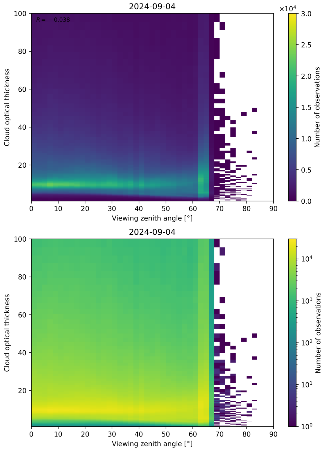
Figure 111: Scatter density plot of “Viewing zenith angle” against “Cloud optical thickness” for 2024-09-03 to 2024-09-05.
