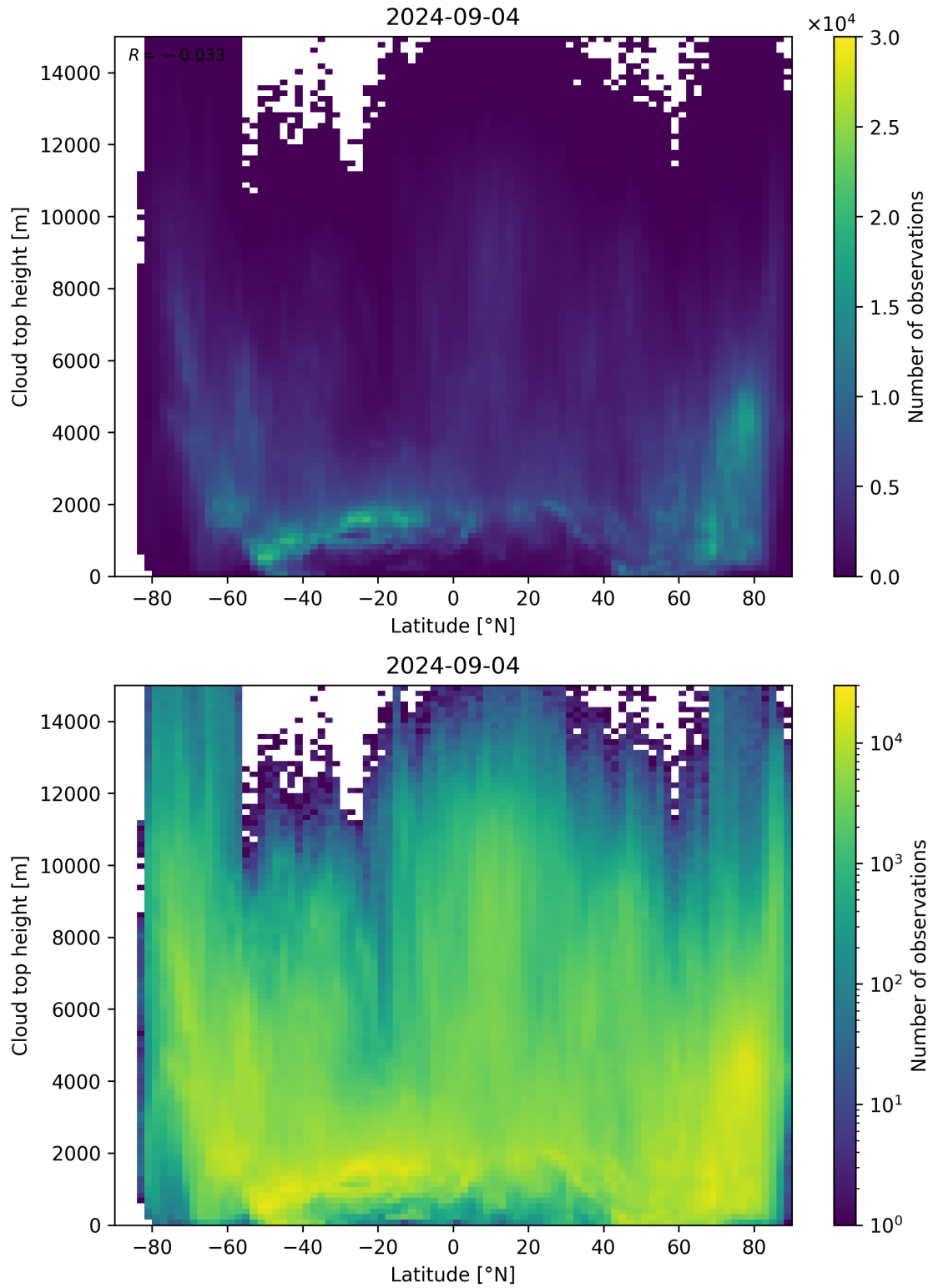
Figure 97: Scatter density plot of “Latitude” against “Cloud top height” for 2024-09-03 to 2024-09-05.
