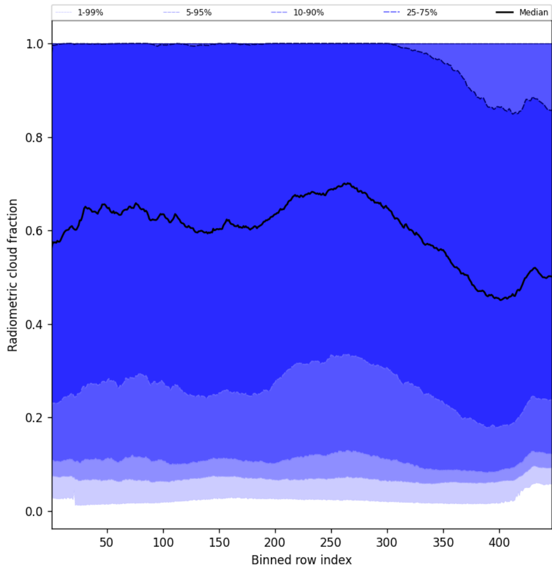
Figure 55: Along track statistics of “Radiometric cloud fraction” for 2024-09-03 to 2024-09-05
