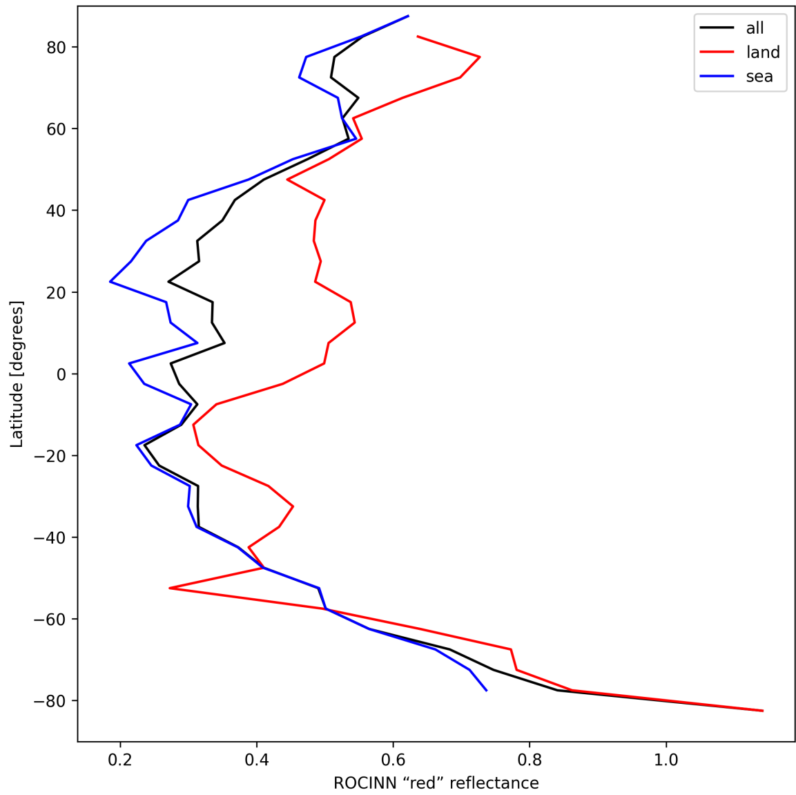
Figure 37: Zonal average of “ROCINN “red” reflectance” for 2024-09-03 to 2024-09-05.
