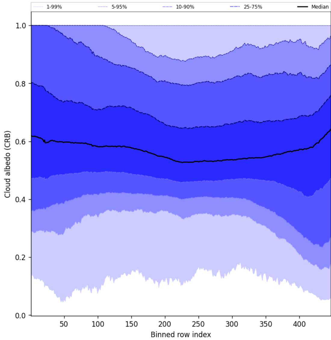
Figure 60: Along track statistics of “Cloud albedo (CRB)” for 2024-09-03 to 2024-09-05
