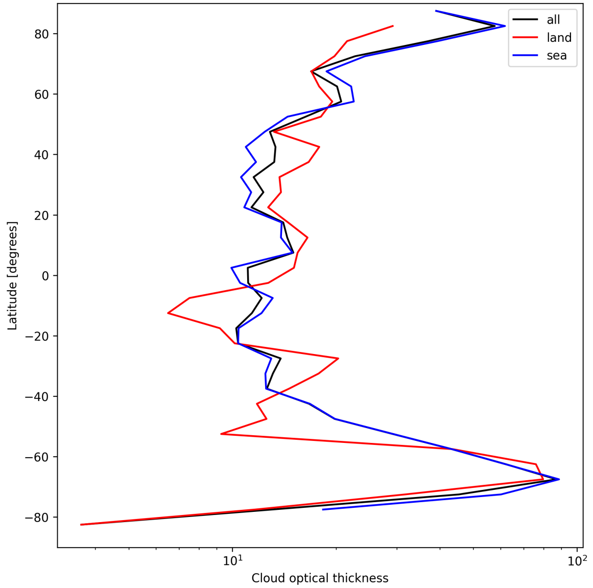
Figure 25: Zonal average of “Cloud optical thickness” for 2024-09-03 to 2024-09-05.
