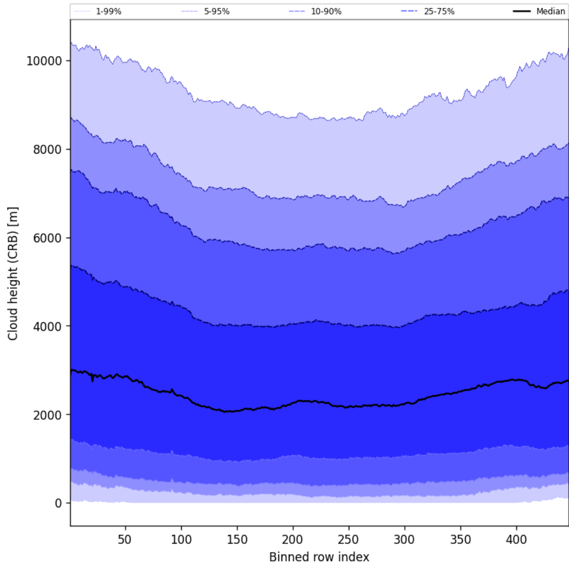
Figure 59: Along track statistics of “Cloud height (CRB)” for 2024-09-03 to 2024-09-05
