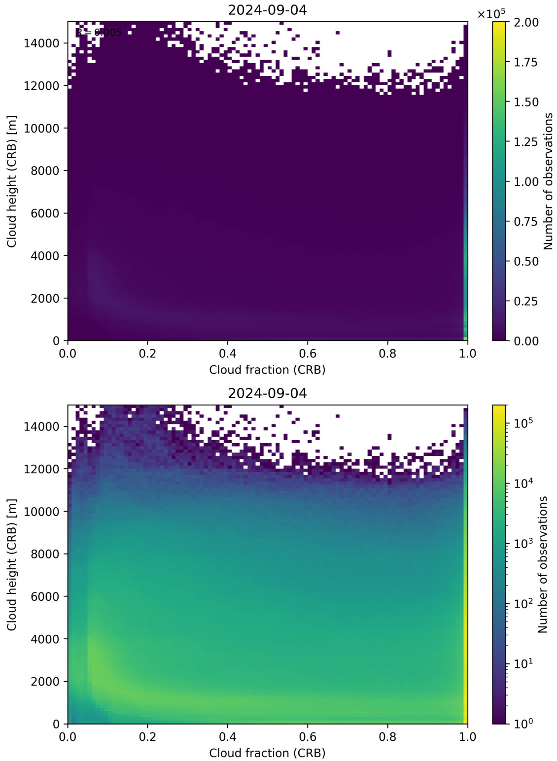
Figure 79: Scatter density plot of “Cloud fraction (CRB)” against “Cloud height (CRB)” for 2024-09-03 to 2024-09-05.
