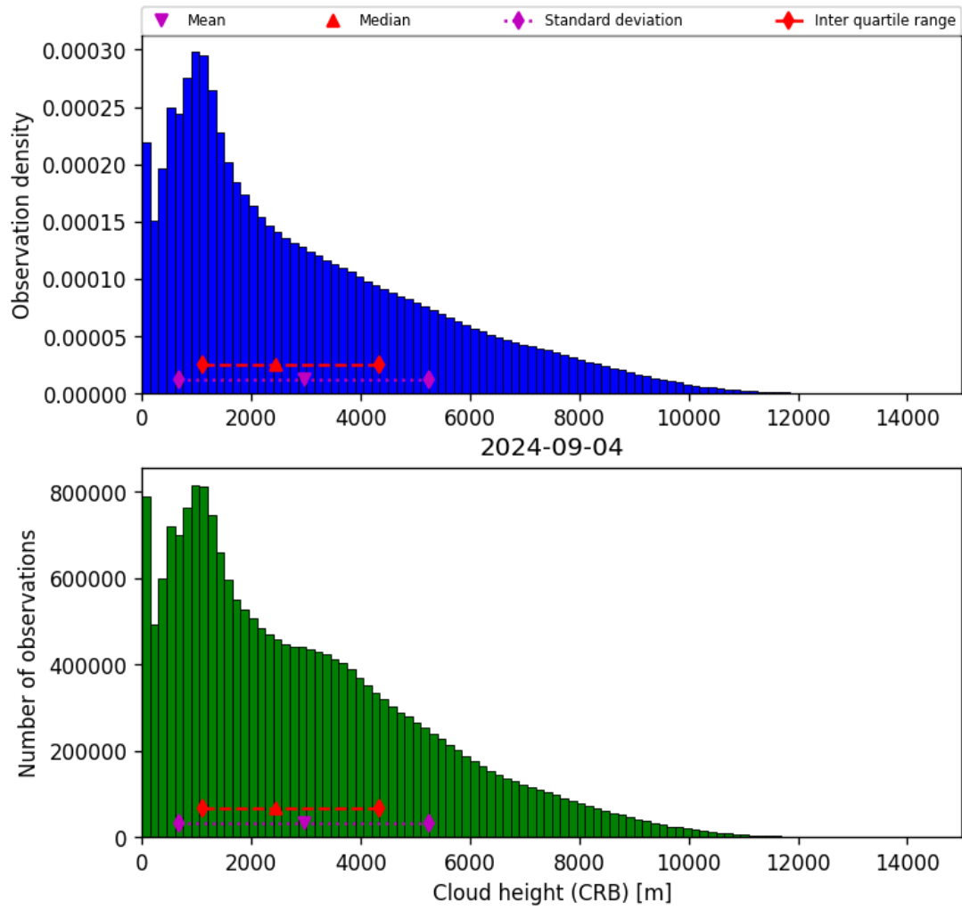
Figure 43: Histogram of “Cloud height (CRB)” for 2024-09-03 to 2024-09-05
