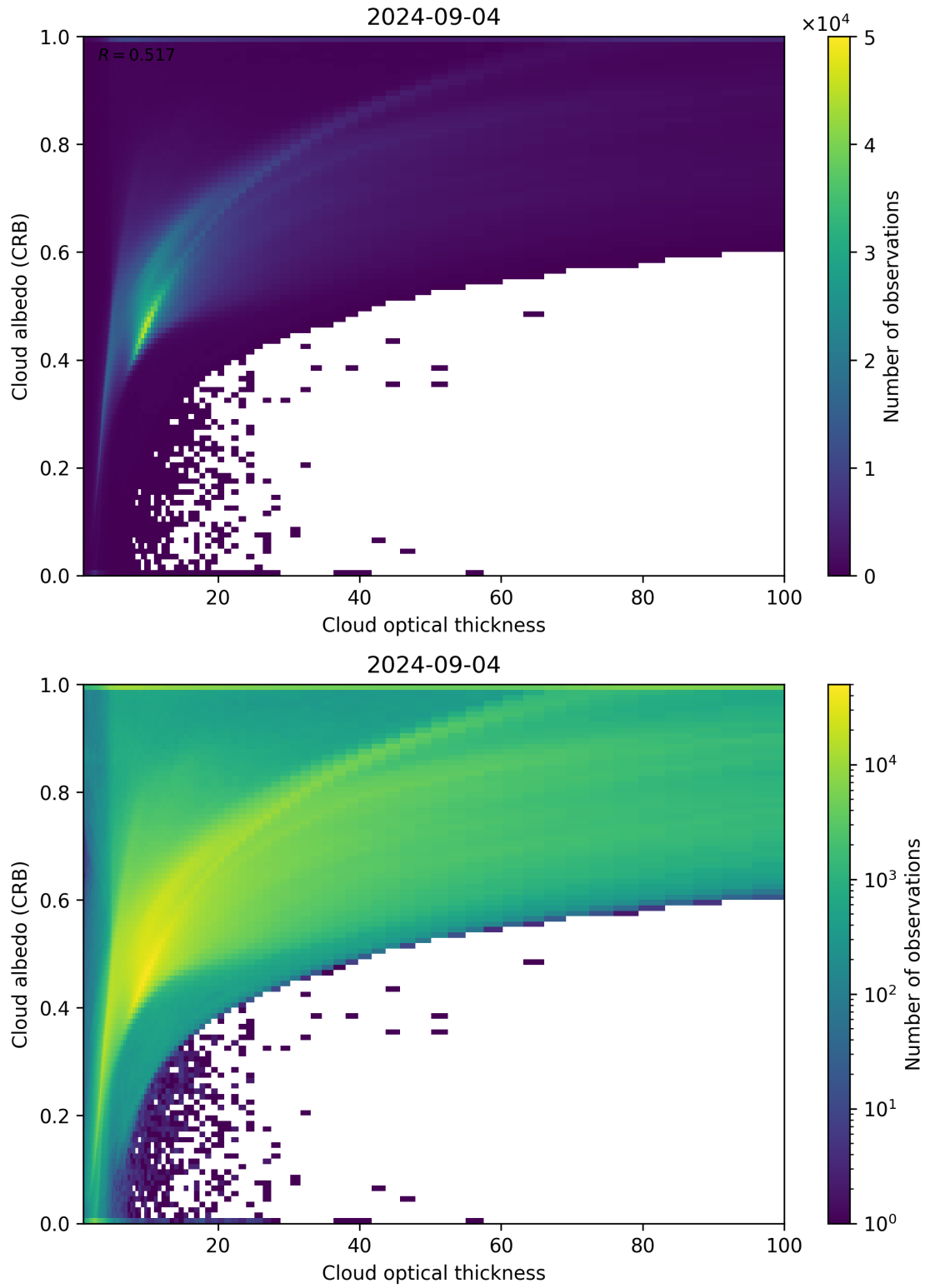
Figure 82: Scatter density plot of “Cloud optical thickness” against “Cloud albedo (CRB)” for 2024-09-03 to 2024-09-05.
