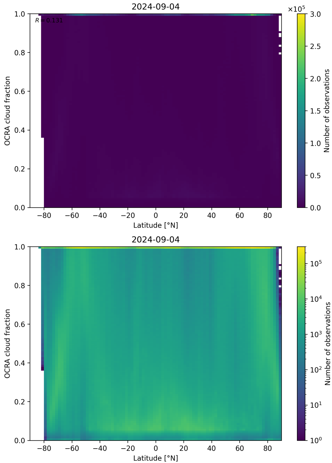
Figure 93: Scatter density plot of “Latitude” against “OCRA cloud fraction” for 2024-09-03 to 2024-09-05.
