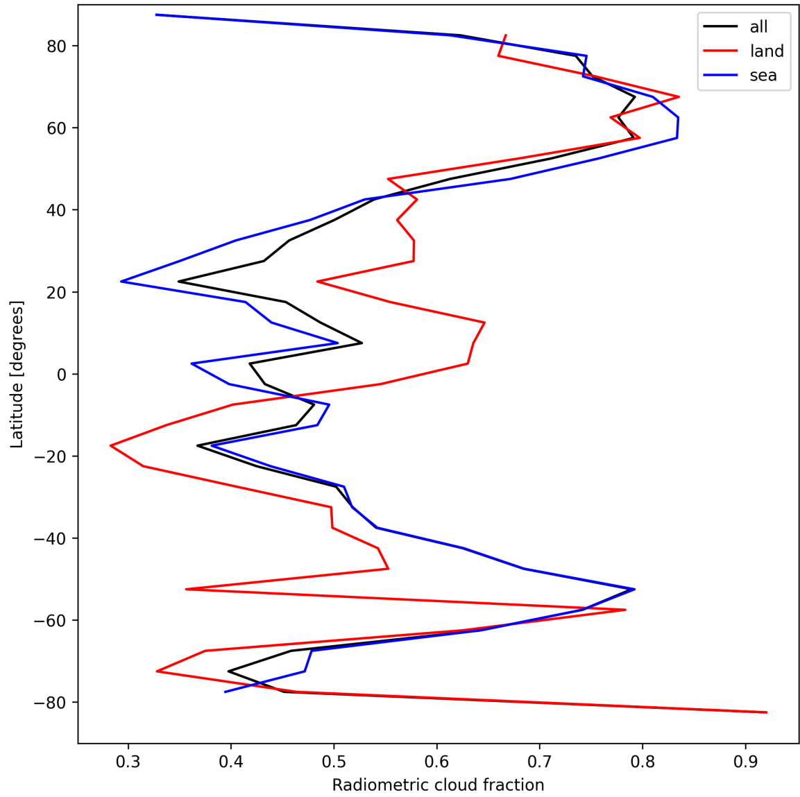
Figure 23: Zonal average of “Radiometric cloud fraction” for 2024-09-03 to 2024-09-05.
