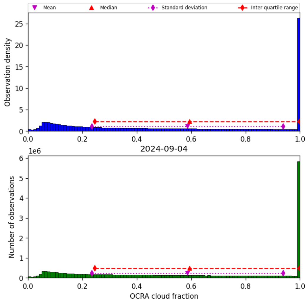
Figure 50: Histogram of “OCRA cloud fraction” for 2024-09-03 to 2024-09-05
