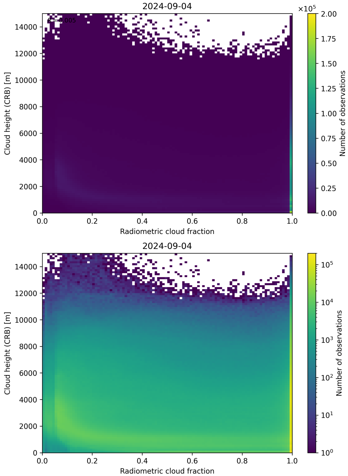
Figure 74: Scatter density plot of “Radiometric cloud fraction” against “Cloud height (CRB)” for 2024-09-03 to 2024-09-05.
