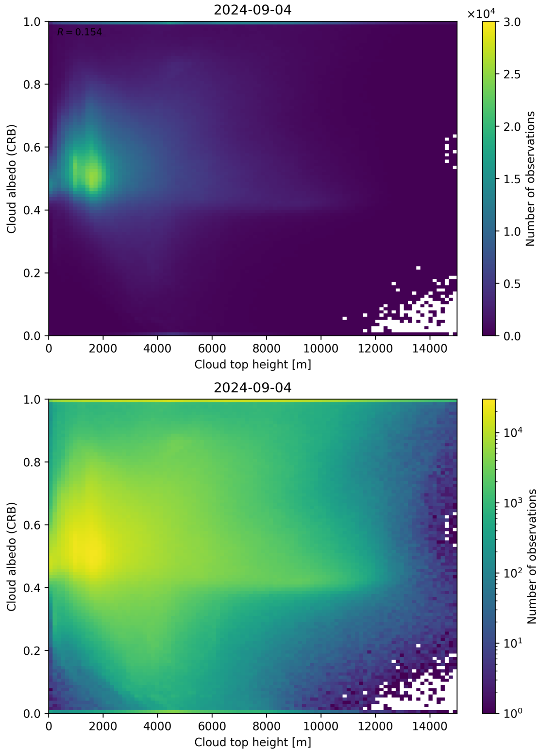
Figure 86: Scatter density plot of “Cloud top height” against “Cloud albedo (CRB)” for 2024-09-03 to 2024-09-05.
