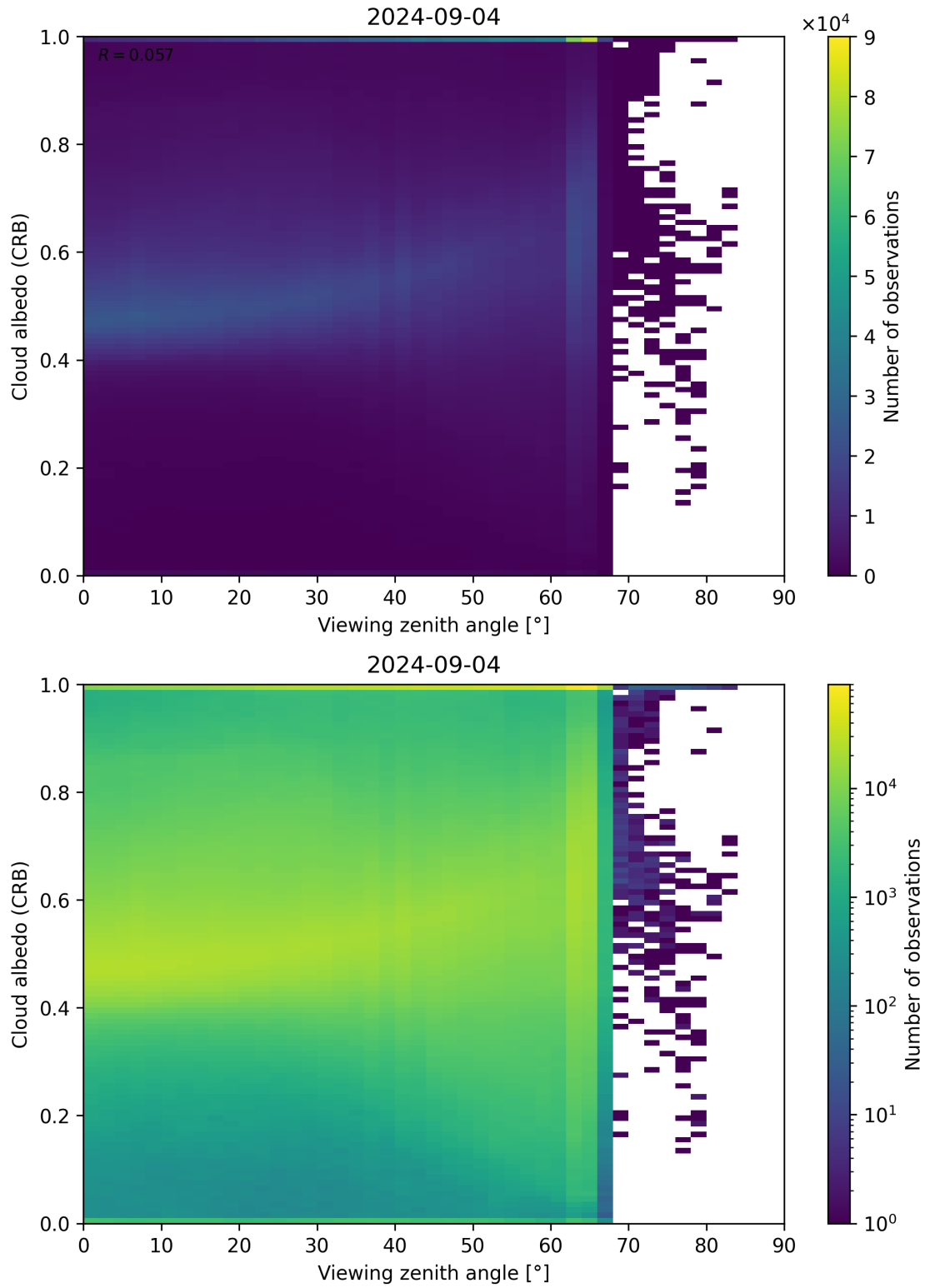
Figure 106: Scatter density plot of “Viewing zenith angle” against “Cloud albedo (CRB)” for 2024-09-03 to 2024-09-05.
