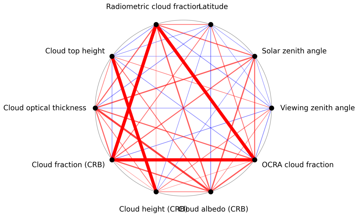
Figure 1: Map of correlation graph for 2024-09-03 to 2024-09-05.
