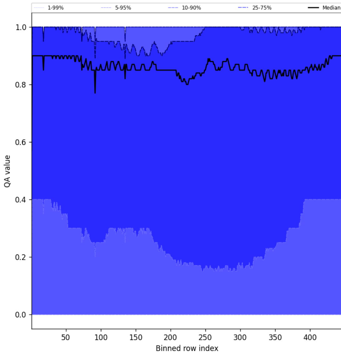
Figure 54: Along track statistics of “QA value” for 2024-09-03 to 2024-09-05
