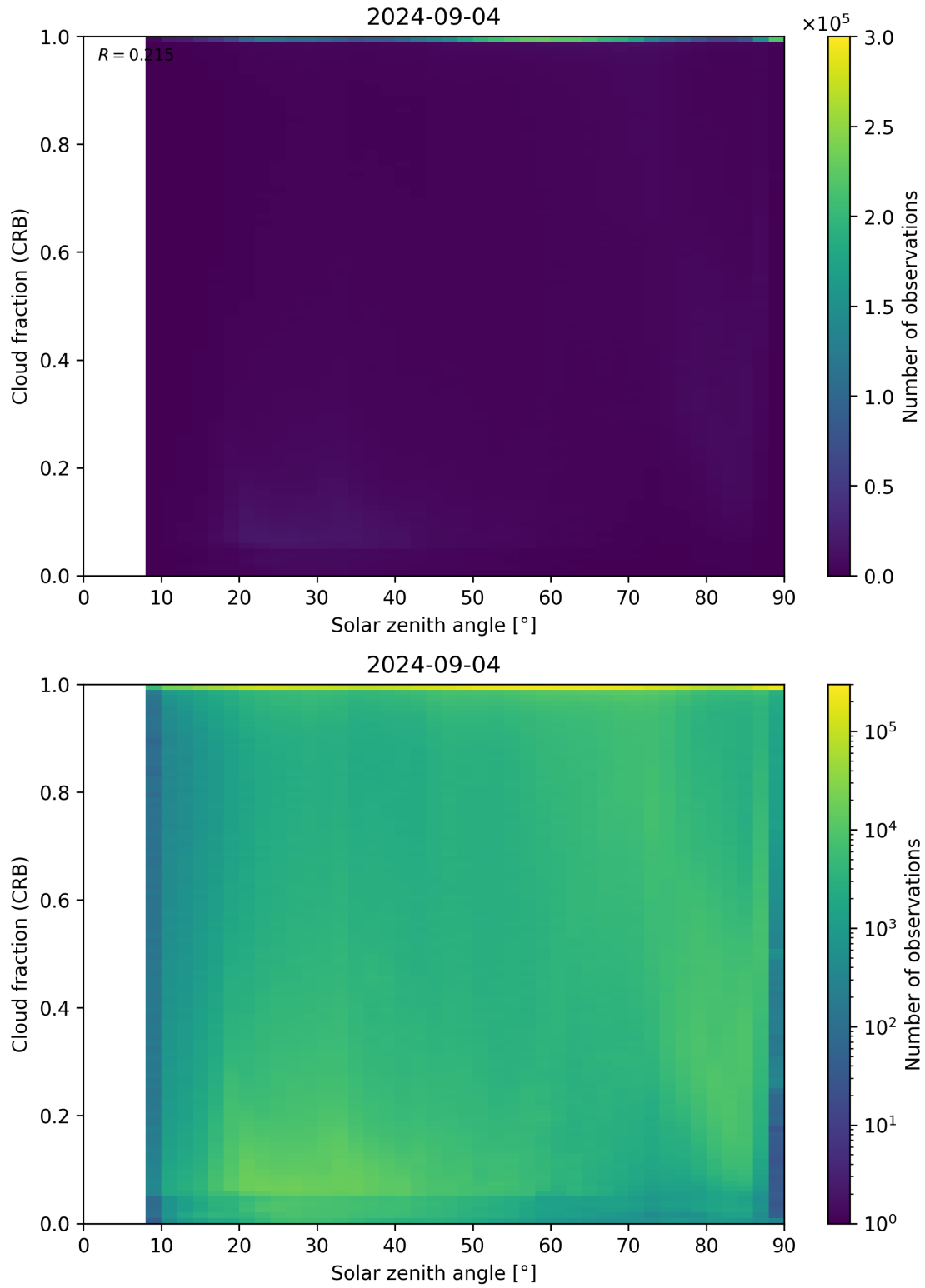
Figure 101: Scatter density plot of “Solar zenith angle” against “Cloud fraction (CRB)” for 2024-09-03 to 2024-09-05.
