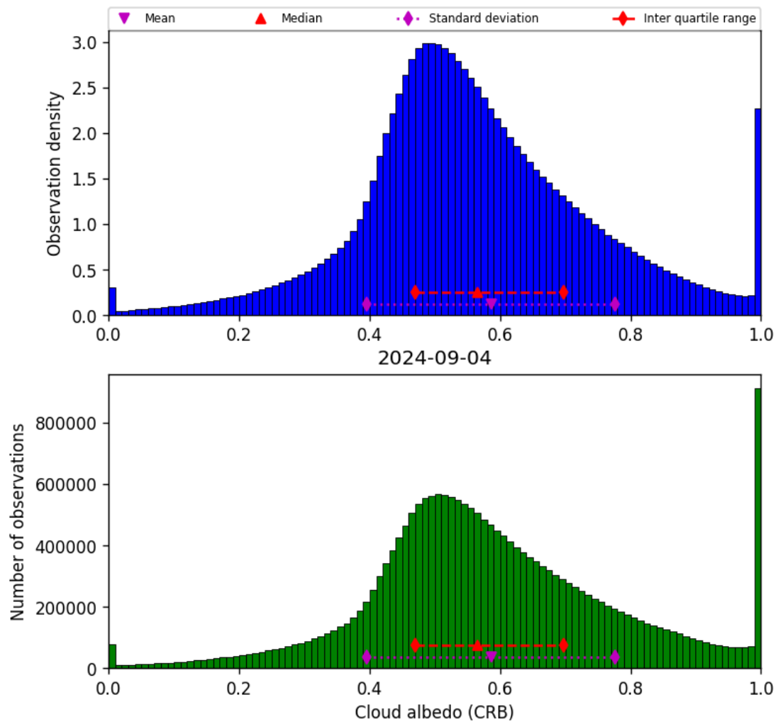
Figure 44: Histogram of “Cloud albedo (CRB)” for 2024-09-03 to 2024-09-05
