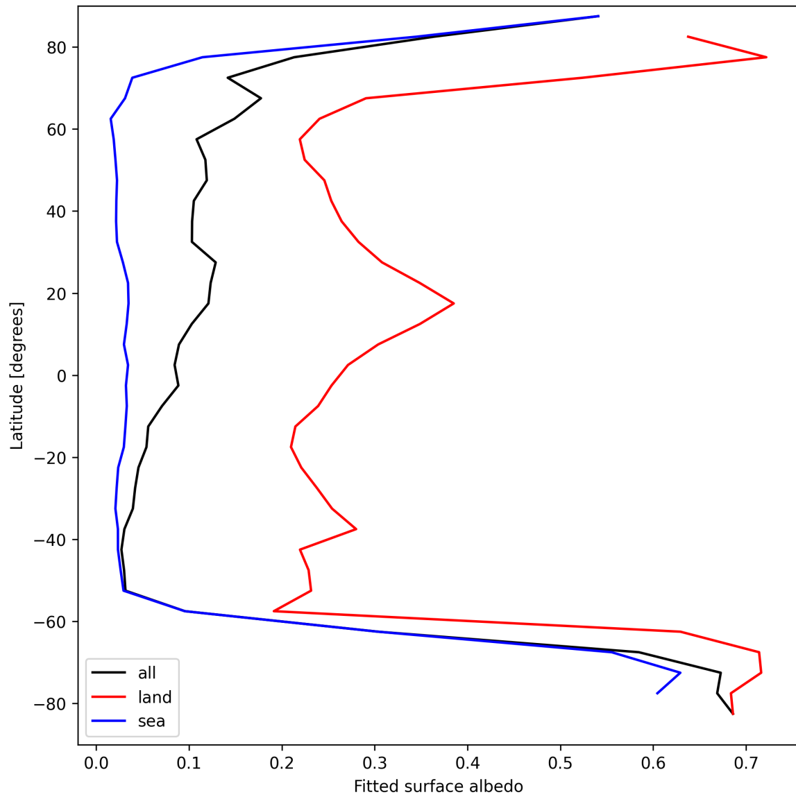
Figure 29: Zonal average of “Fitted surface albedo” for 2024-09-03 to 2024-09-05.
