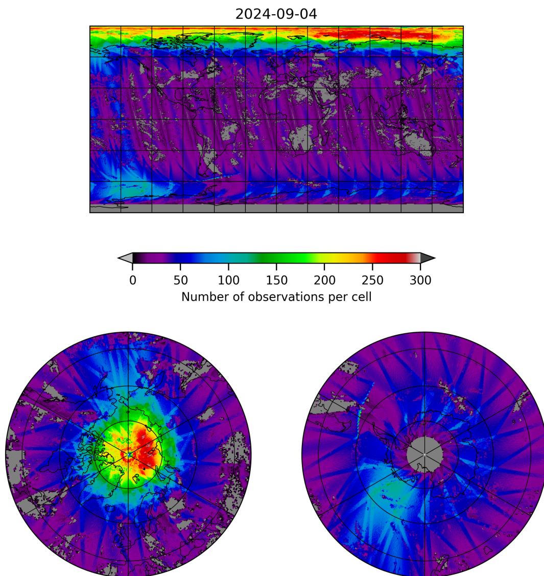
Figure 21: Map of the number of observations for 2024-09-03 to 2024-09-05
