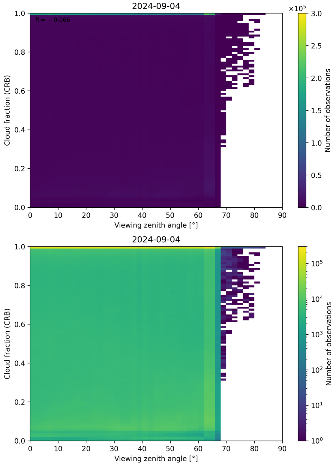
Figure 109: Scatter density plot of “Viewing zenith angle” against “Cloud fraction (CRB)” for 2024-09-03 to 2024-09-05.
