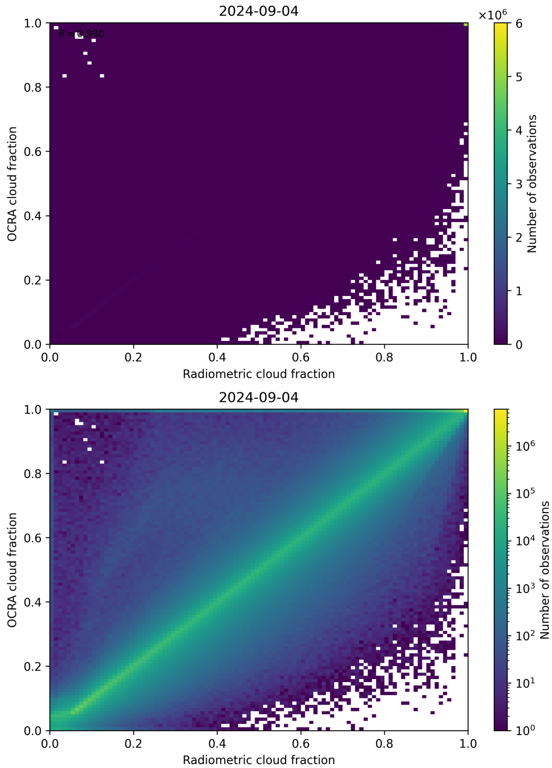
Figure 72: Scatter density plot of “Radiometric cloud fraction” against “OCRA cloud fraction” for 2024-09-03 to 2024-09-05.
