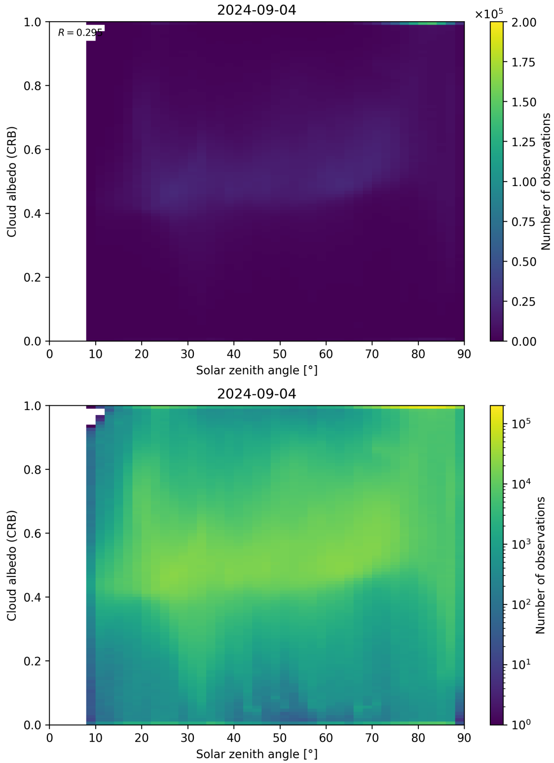
Figure 98: Scatter density plot of “Solar zenith angle” against “Cloud albedo (CRB)” for 2024-09-03 to 2024-09-05.
