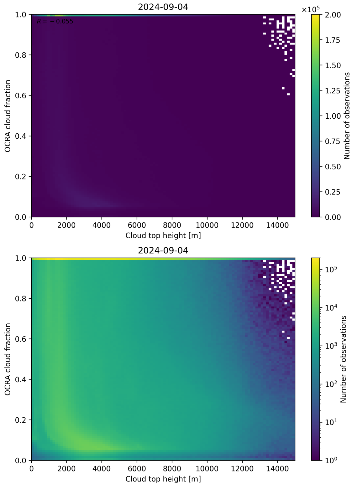
Figure 87: Scatter density plot of “Cloud top height” against “OCRA cloud fraction” for 2024-09-03 to 2024-09-05.
