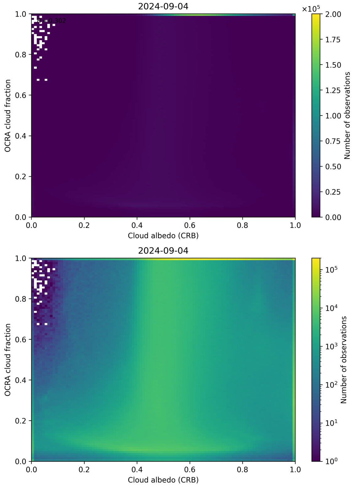
Figure 70: Scatter density plot of “Cloud albedo (CRB)” against “OCRA cloud fraction” for 2024-09-03 to 2024-09-05.
