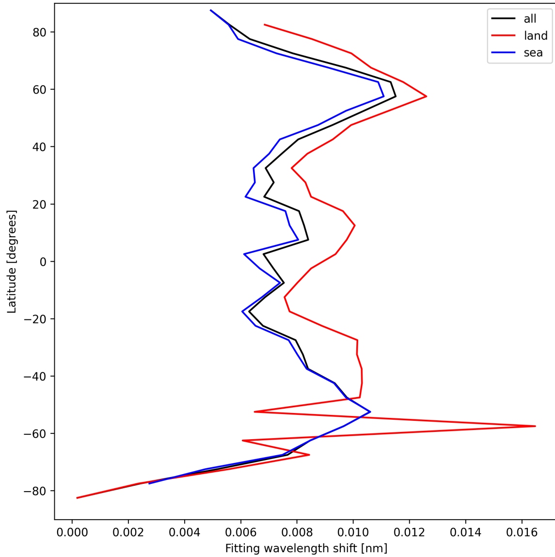
Figure 33: Zonal average of “Fitting wavelength shift” for 2024-09-03 to 2024-09-05.
