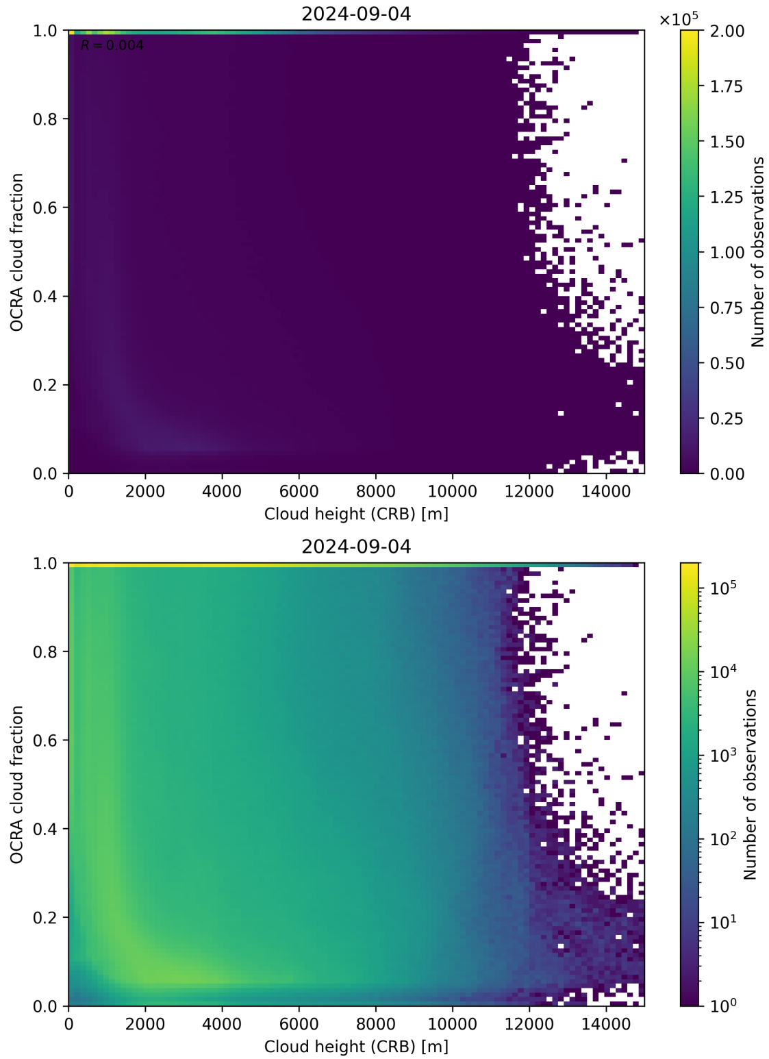
Figure 81: Scatter density plot of “Cloud height (CRB)” against “OCRA cloud fraction” for 2024-09-03 to 2024-09-05.
