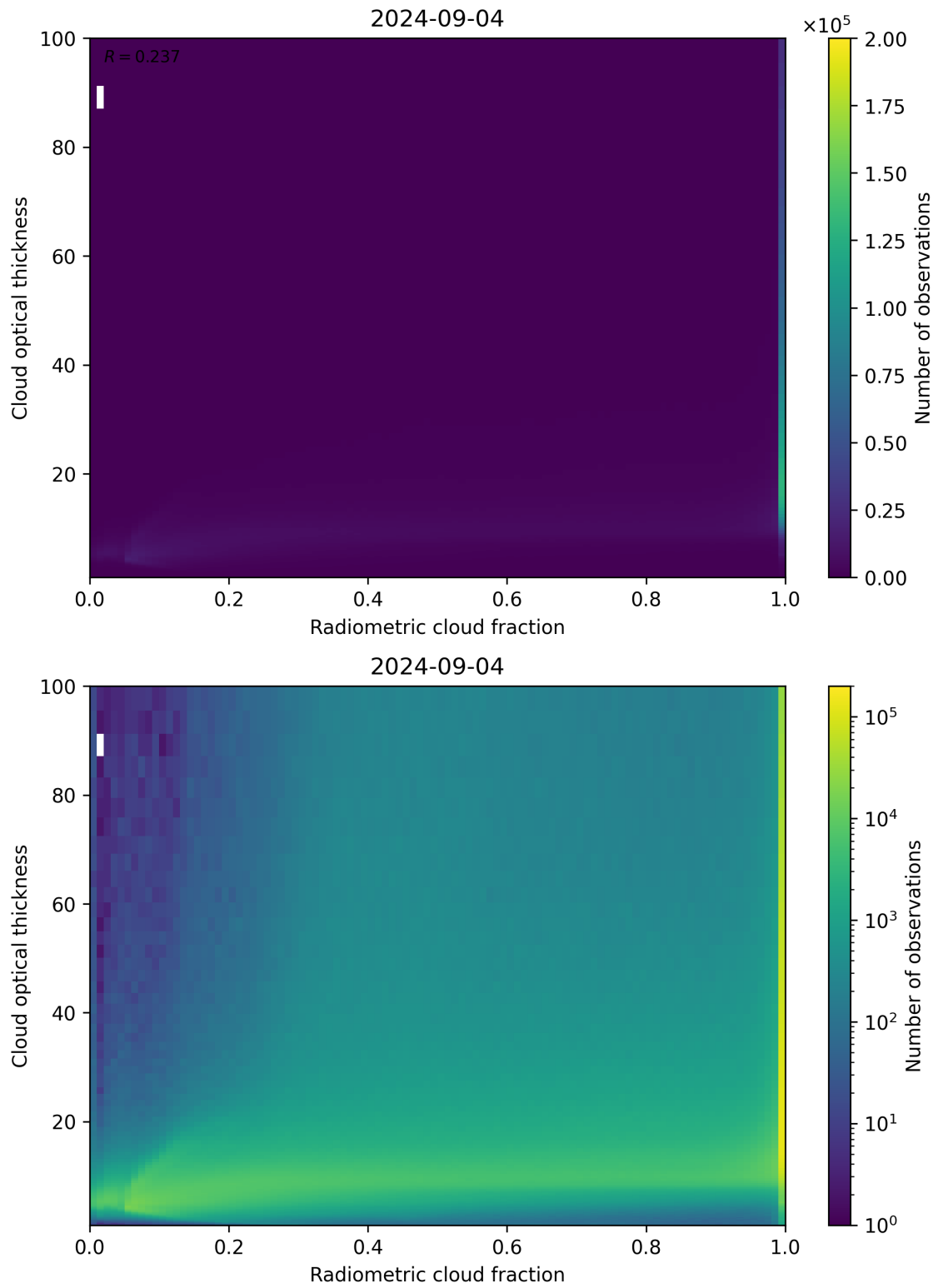
Figure 75: Scatter density plot of “Radiometric cloud fraction” against “Cloud optical thickness” for 2024-09-03 to 2024-09-05.
