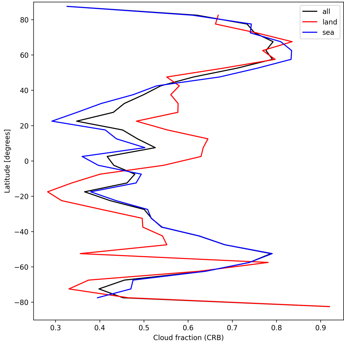
Figure 26: Zonal average of “Cloud fraction (CRB)” for 2024-09-03 to 2024-09-05.
