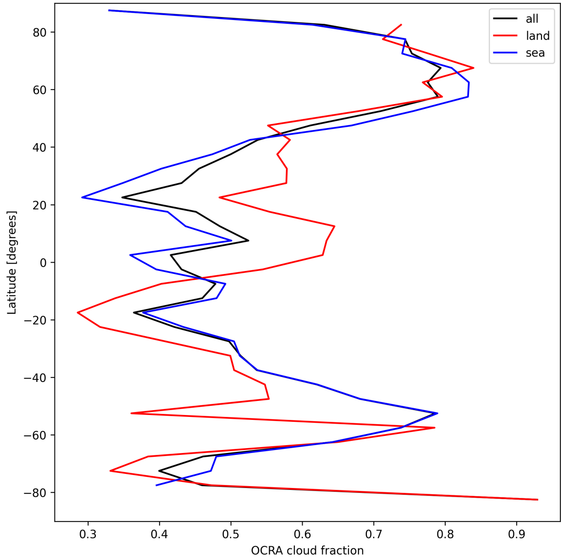
Figure 34: Zonal average of “OCRA cloud fraction” for 2024-09-03 to 2024-09-05.
