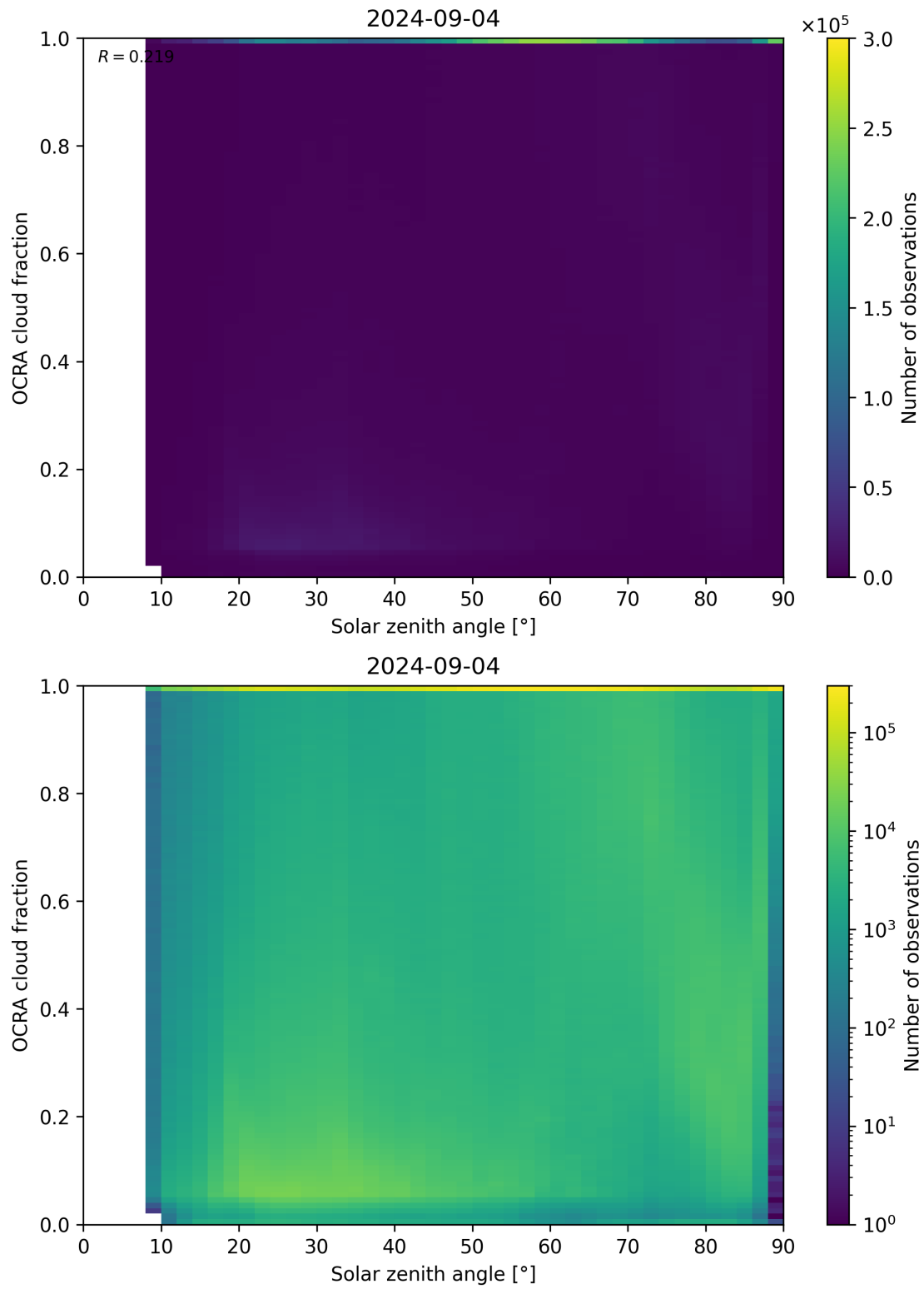
Figure 100: Scatter density plot of “Solar zenith angle” against “OCRA cloud fraction” for 2024-09-03 to 2024-09-05.
