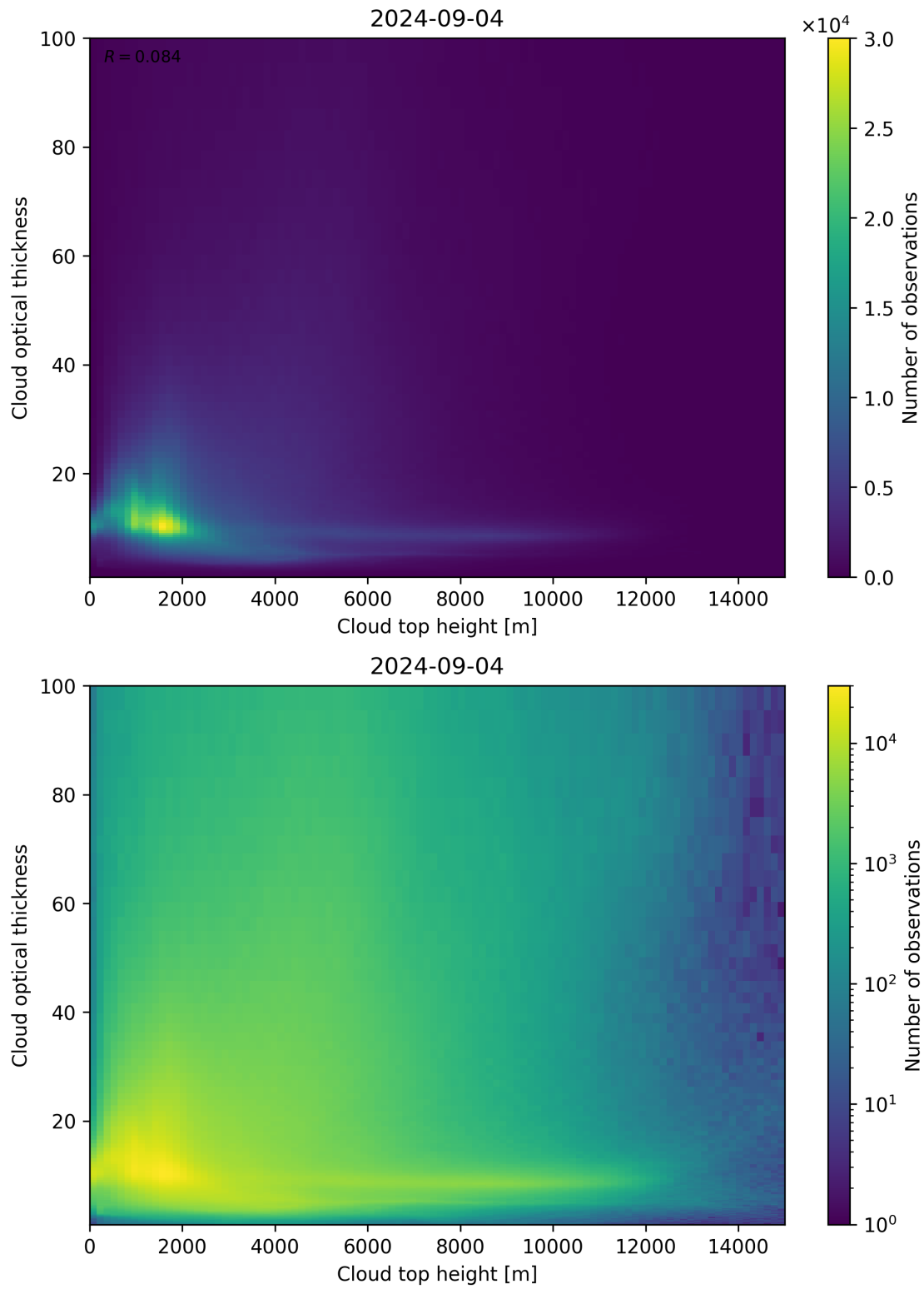
Figure 90: Scatter density plot of “Cloud top height” against “Cloud optical thickness” for 2024-09-03 to 2024-09-05.
