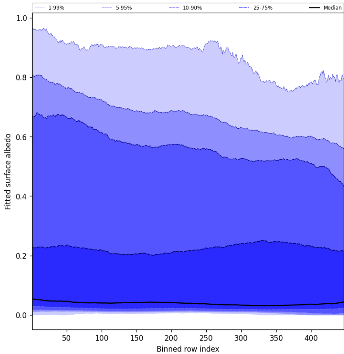
Figure 61: Along track statistics of “Fitted surface albedo” for 2024-09-03 to 2024-09-05
