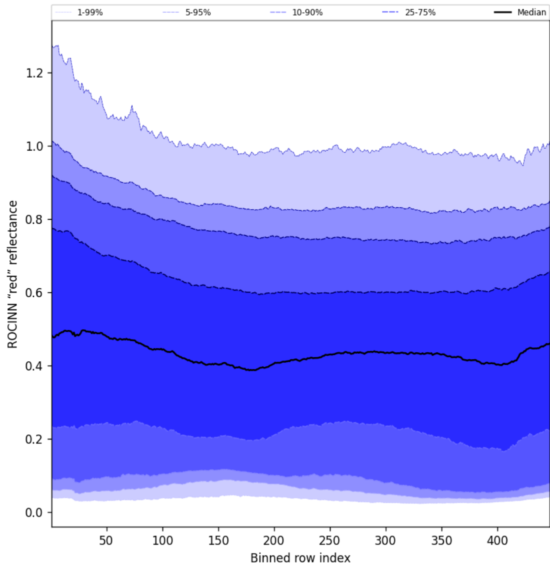
Figure 69: Along track statistics of “ROCINN “red” reflectance” for 2024-09-03 to 2024-09-05
