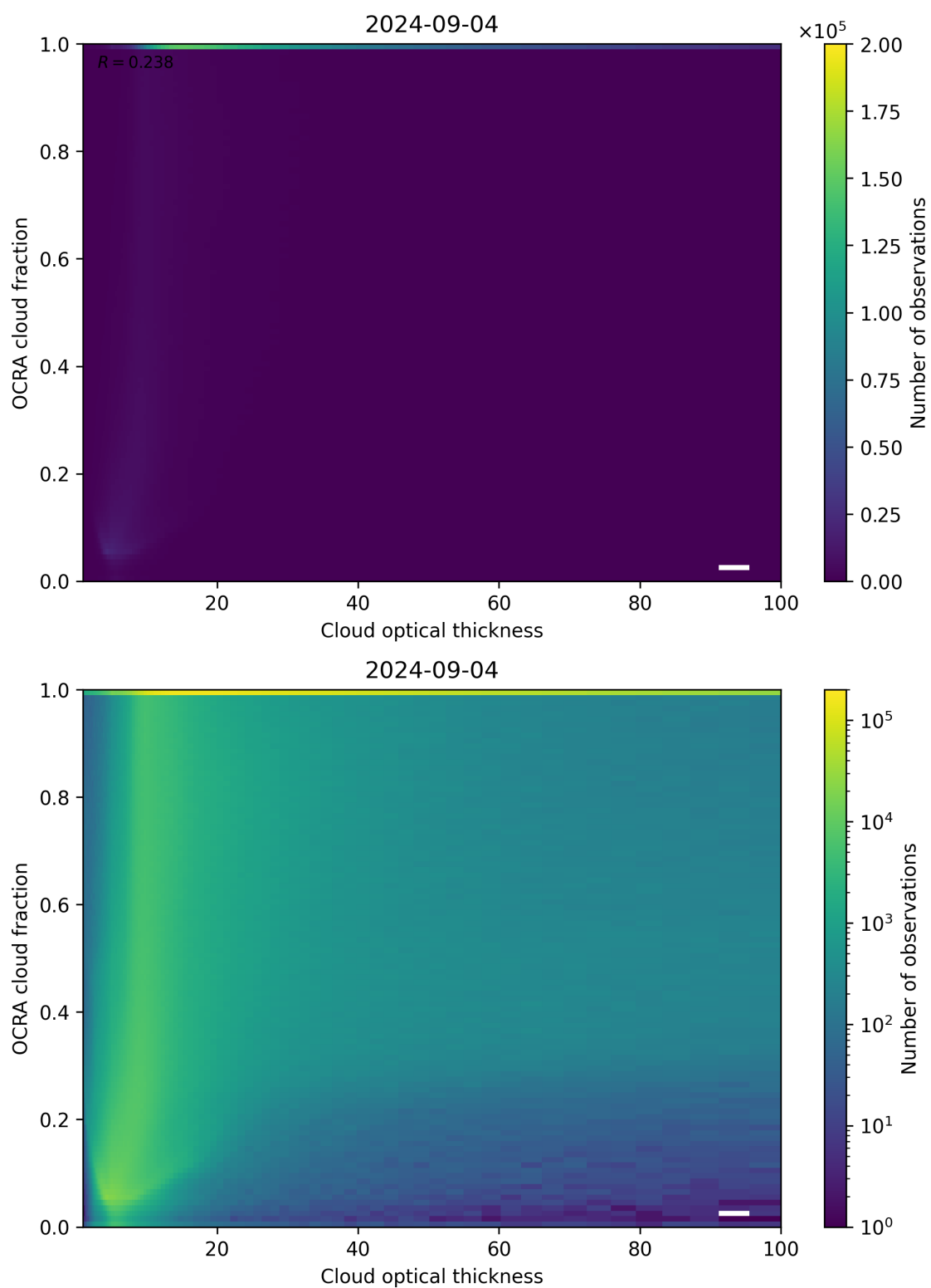
Figure 83: Scatter density plot of “Cloud optical thickness” against “OCRA cloud fraction” for 2024-09-03 to 2024-09-05.
