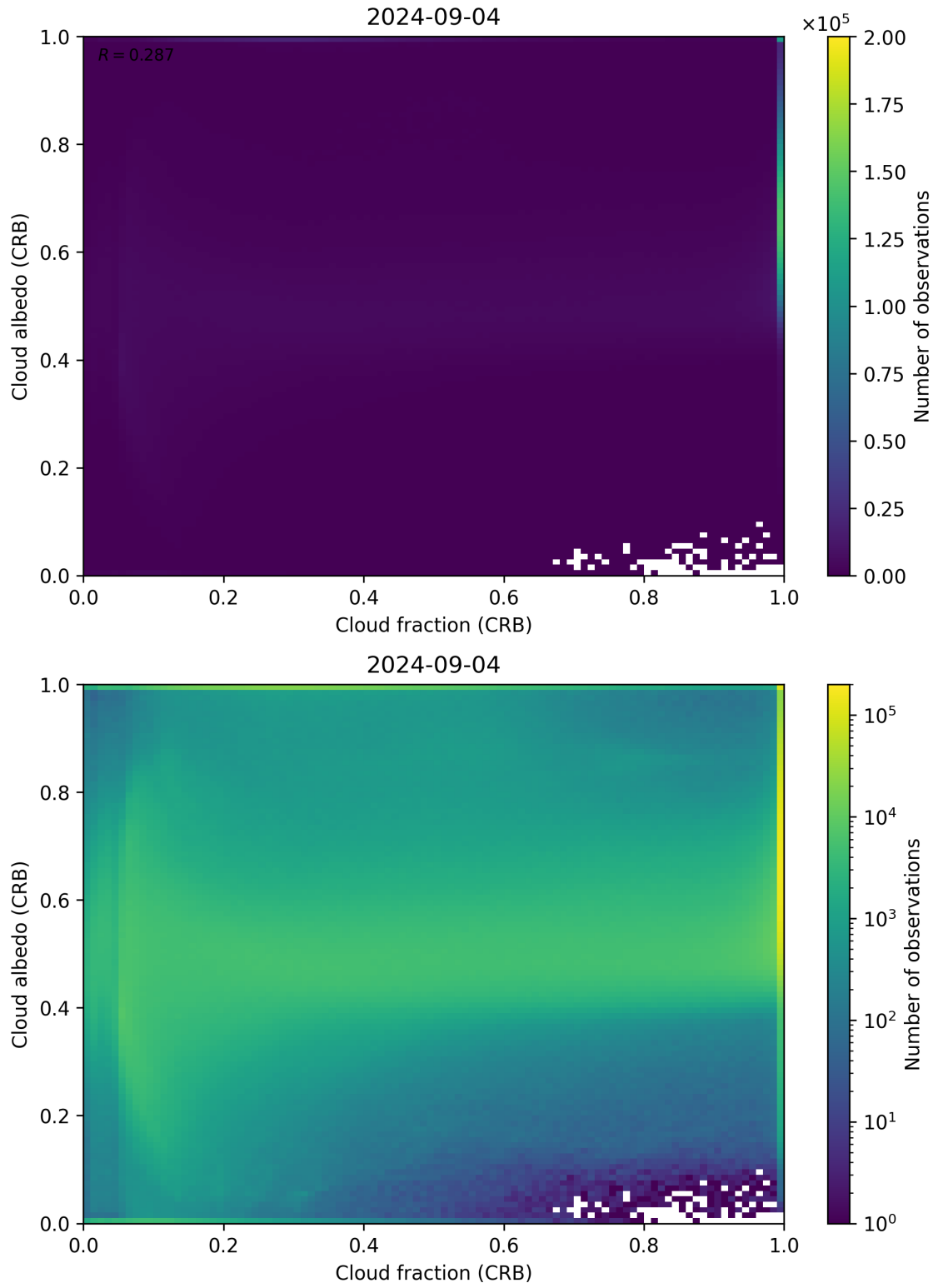
Figure 77: Scatter density plot of “Cloud fraction (CRB)” against “Cloud albedo (CRB)” for 2024-09-03 to 2024-09-05.
