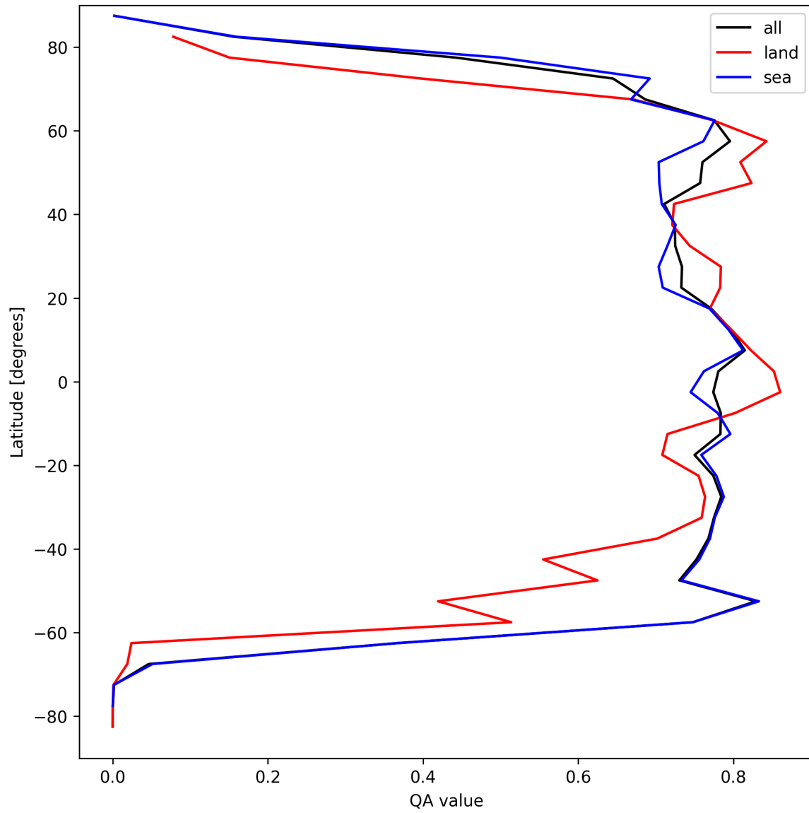
Figure 22: Zonal average of “QA value” for 2024-09-03 to 2024-09-05.
