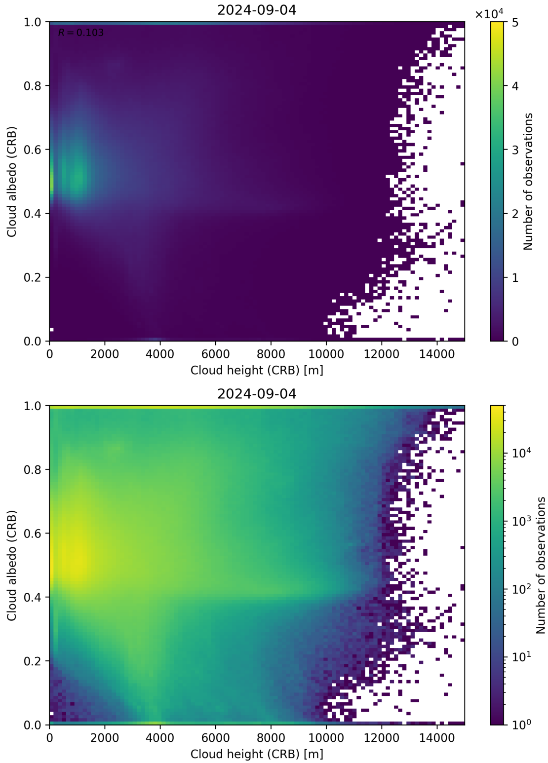
Figure 80: Scatter density plot of “Cloud height (CRB)” against “Cloud albedo (CRB)” for 2024-09-03 to 2024-09-05.
