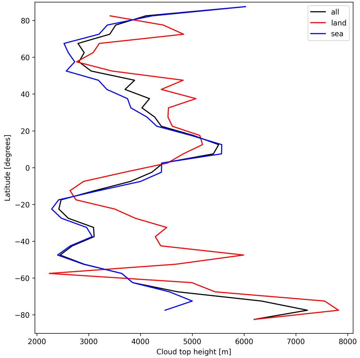
Figure 24: Zonal average of “Cloud top height” for 2024-09-03 to 2024-09-05.
