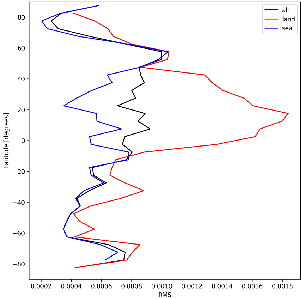
Figure 31: Zonal average of “RMS” for 2024-09-03 to 2024-09-05.
