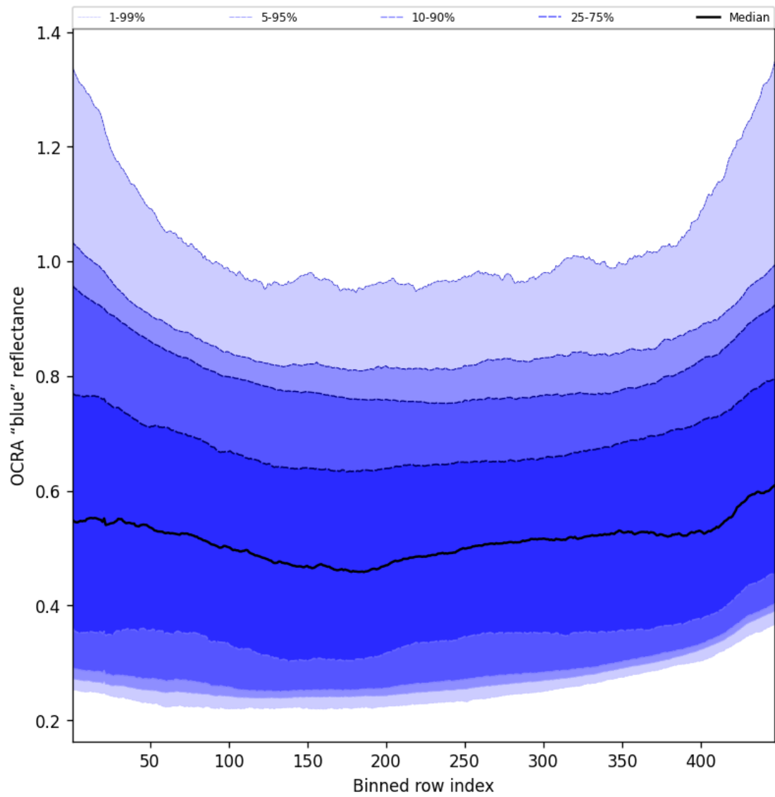
Figure 67: Along track statistics of “OCRA “blue” reflectance” for 2024-09-03 to 2024-09-05
