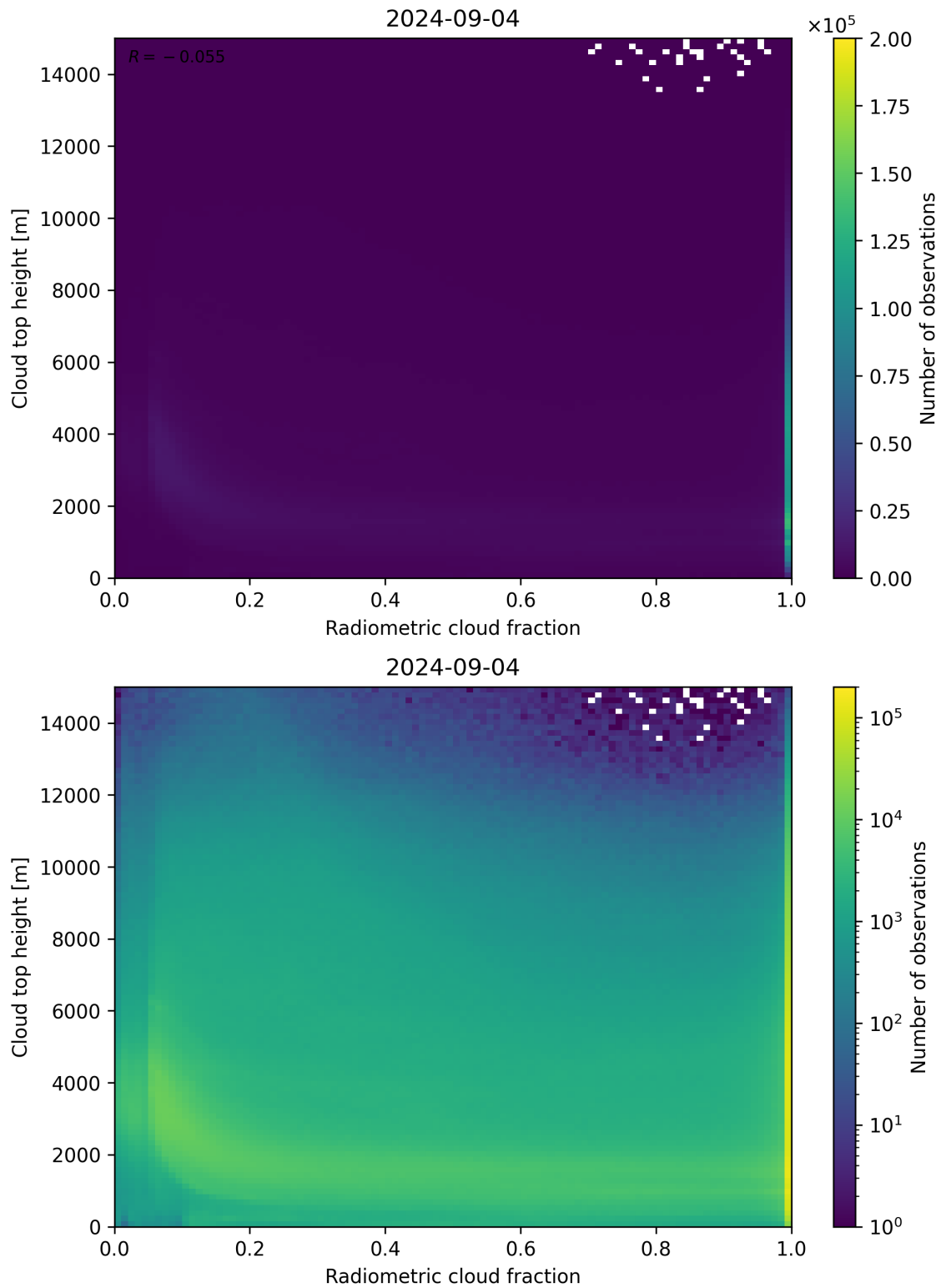
Figure 76: Scatter density plot of “Radiometric cloud fraction” against “Cloud top height” for 2024-09-03 to 2024-09-05.
