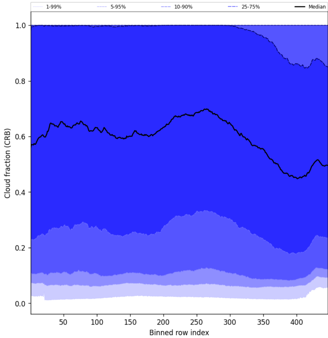
Figure 58: Along track statistics of “Cloud fraction (CRB)” for 2024-09-03 to 2024-09-05
