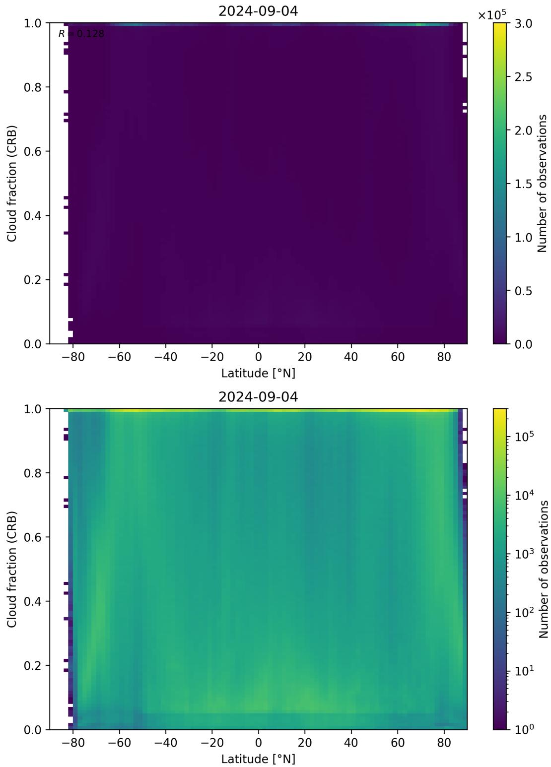
Figure 94: Scatter density plot of “Latitude” against “Cloud fraction (CRB)” for 2024-09-03 to 2024-09-05.
