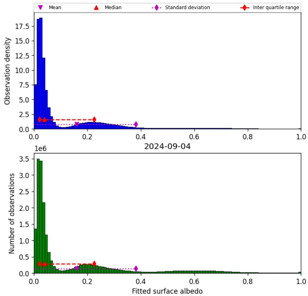
Figure 45: Histogram of “Fitted surface albedo” for 2024-09-03 to 2024-09-05
