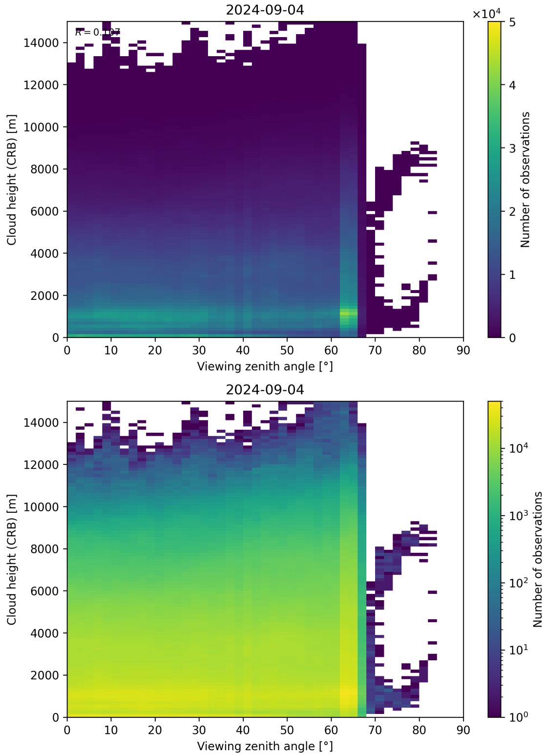
Figure 110: Scatter density plot of “Viewing zenith angle” against “Cloud height (CRB)” for 2024-09-03 to 2024-09-05.
