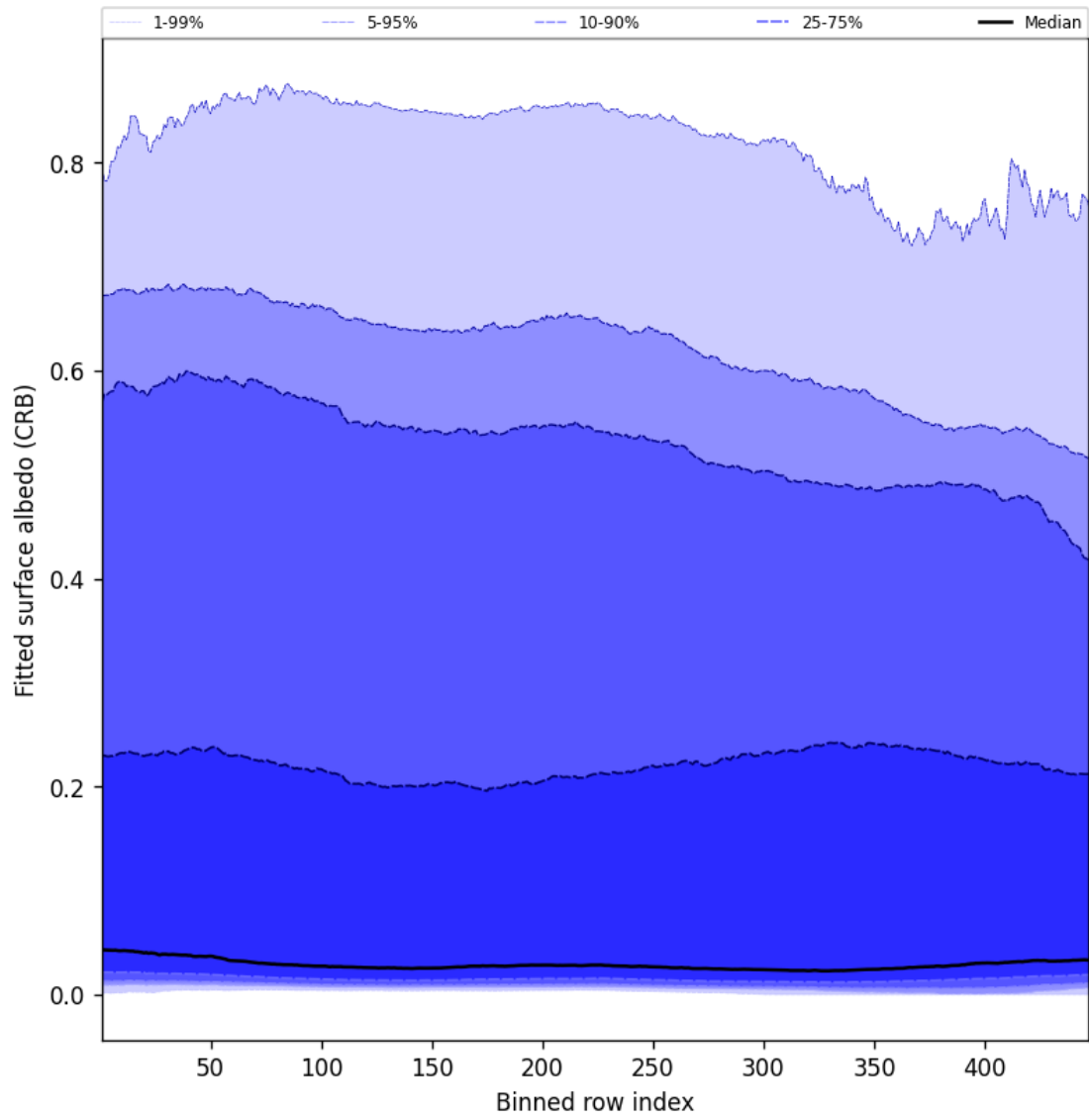
Figure 62: Along track statistics of “Fitted surface albedo (CRB)” for 2024-09-03 to 2024-09-05
