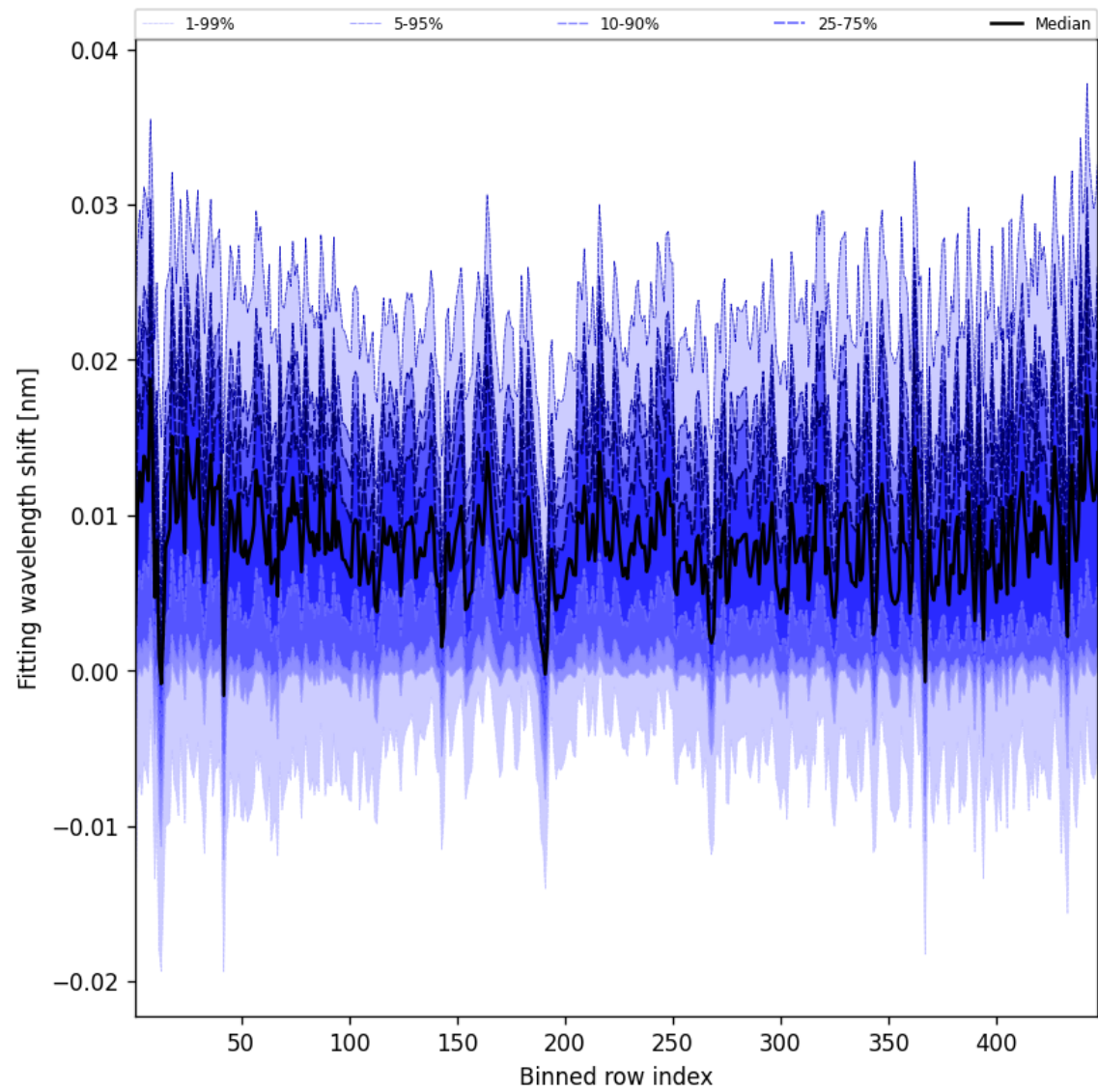
Figure 65: Along track statistics of “Fitting wavelength shift” for 2024-09-03 to 2024-09-05
