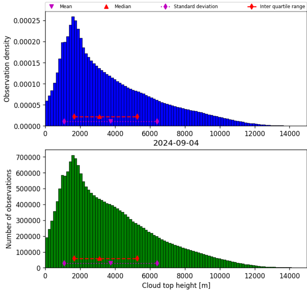
Figure 40: Histogram of “Cloud top height” for 2024-09-03 to 2024-09-05
