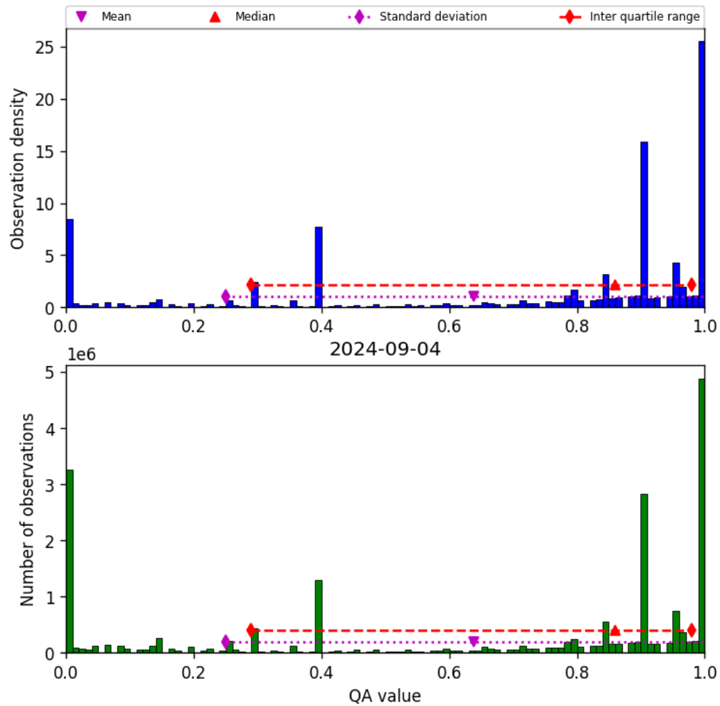
Figure 38: Histogram of “QA value” for 2024-09-03 to 2024-09-05
