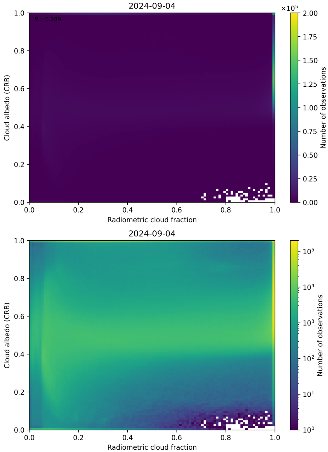
Figure 71: Scatter density plot of “Radiometric cloud fraction” against “Cloud albedo (CRB)” for 2024-09-03 to 2024-09-05.
