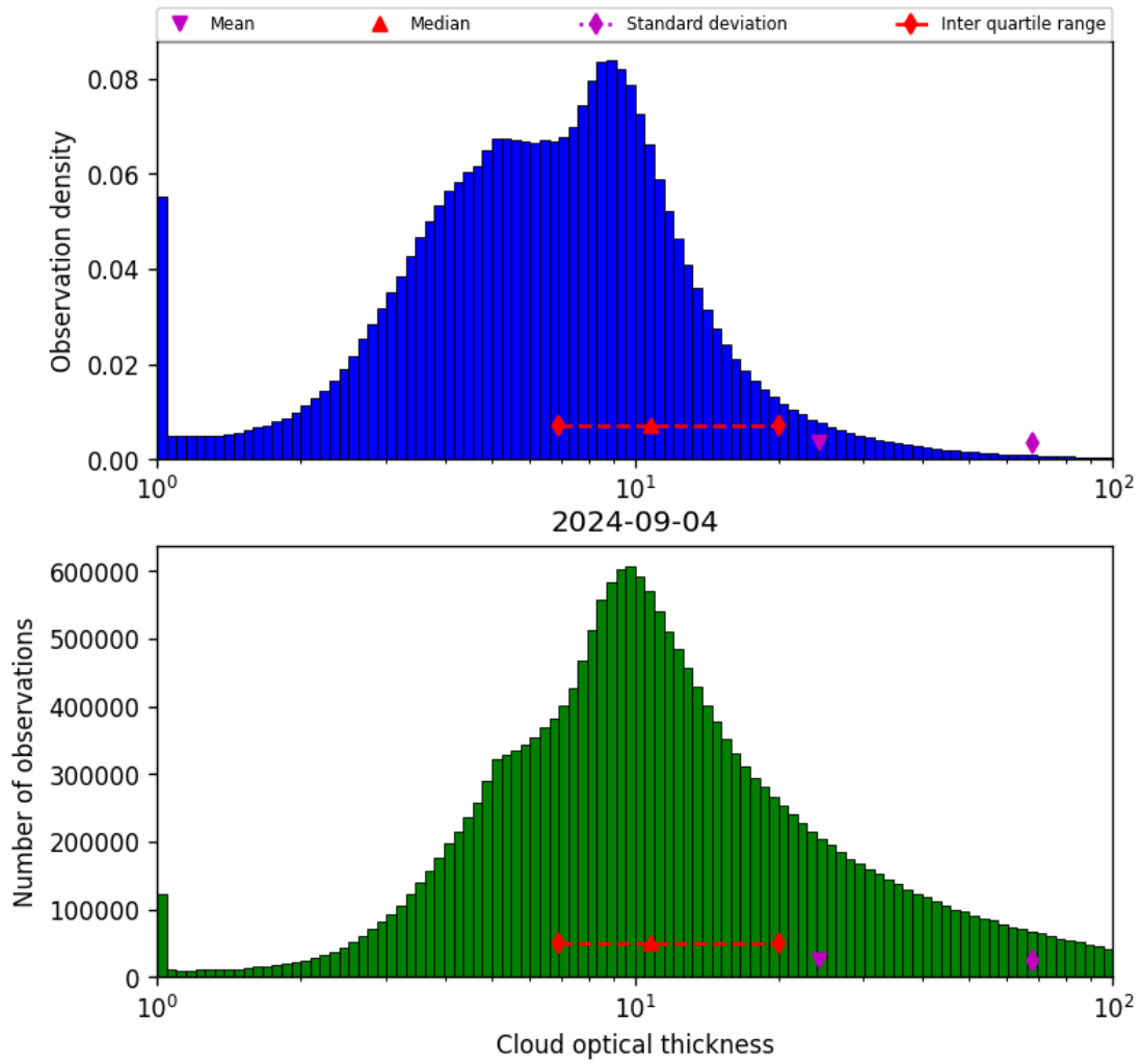
Figure 41: Histogram of “Cloud optical thickness” for 2024-09-03 to 2024-09-05
