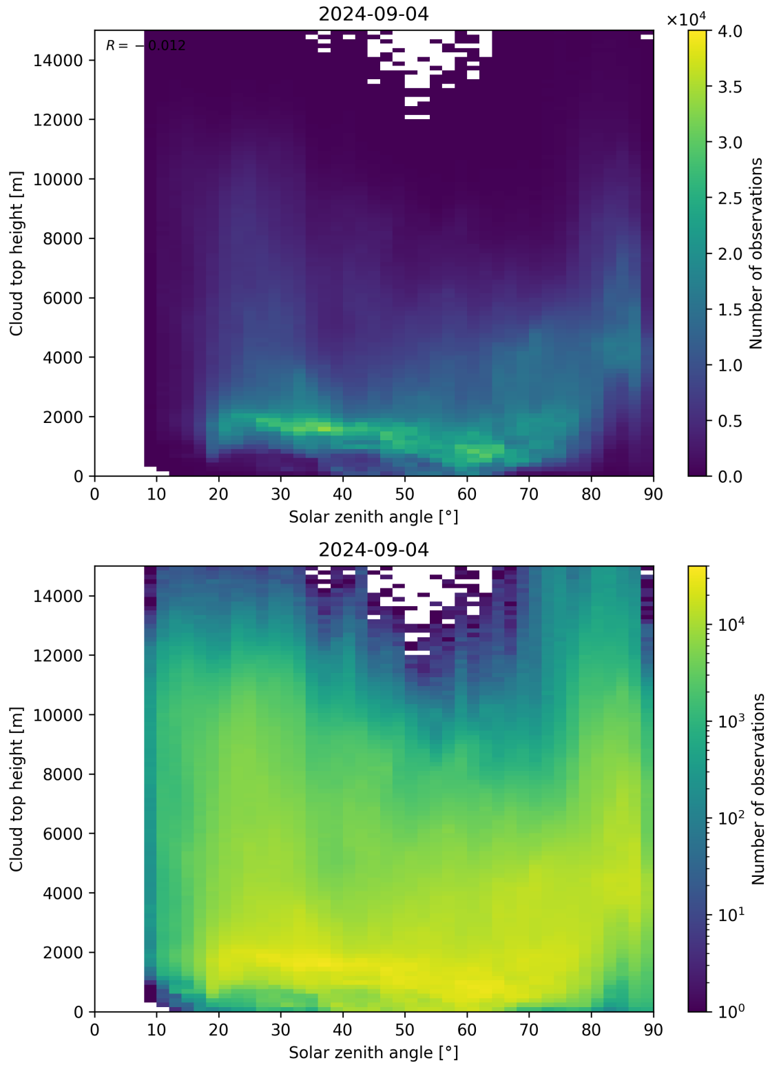
Figure 104: Scatter density plot of “Solar zenith angle” against “Cloud top height” for 2024-09-03 to 2024-09-05.
