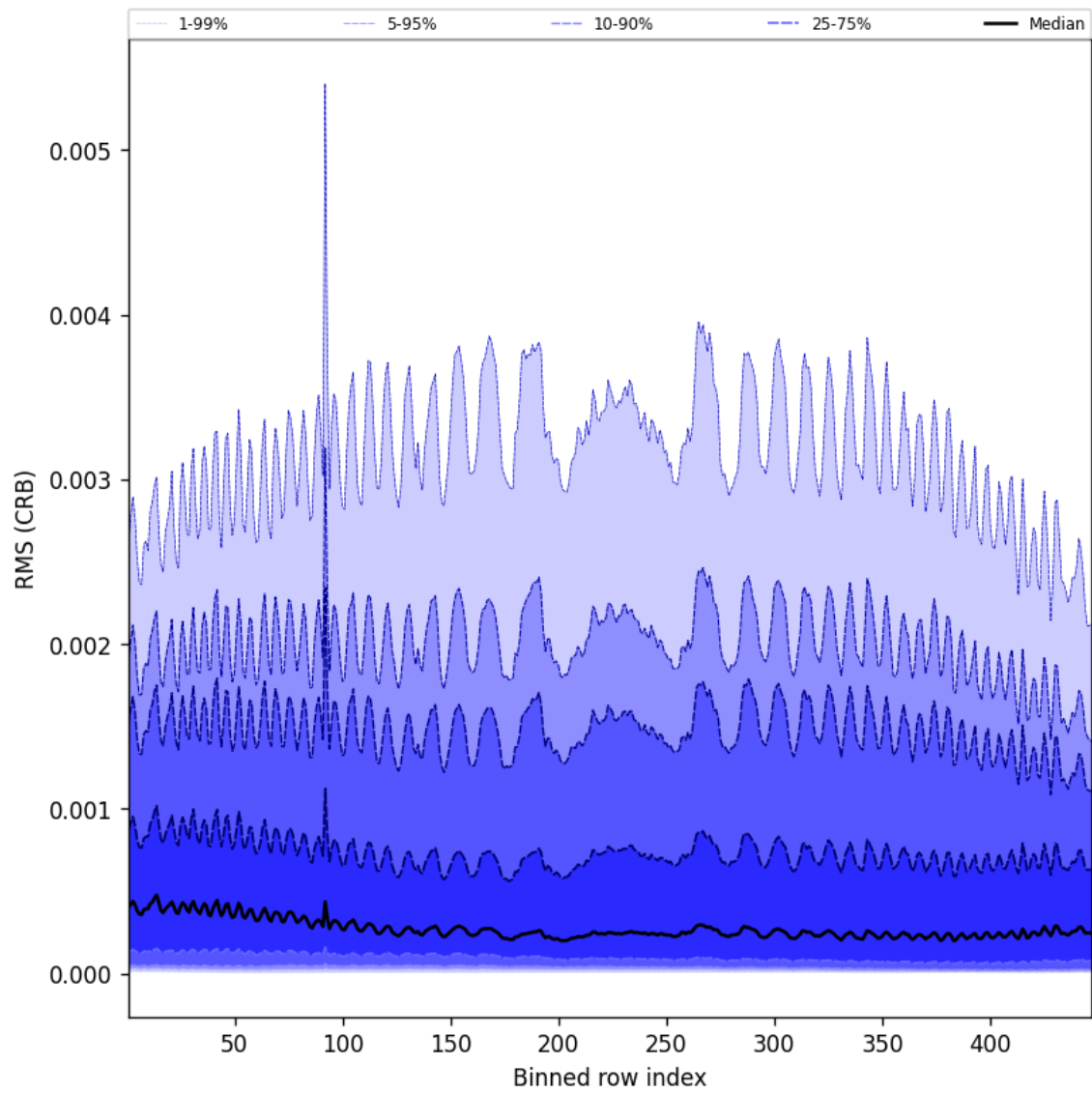
Figure 64: Along track statistics of “RMS (CRB)” for 2024-09-03 to 2024-09-05
