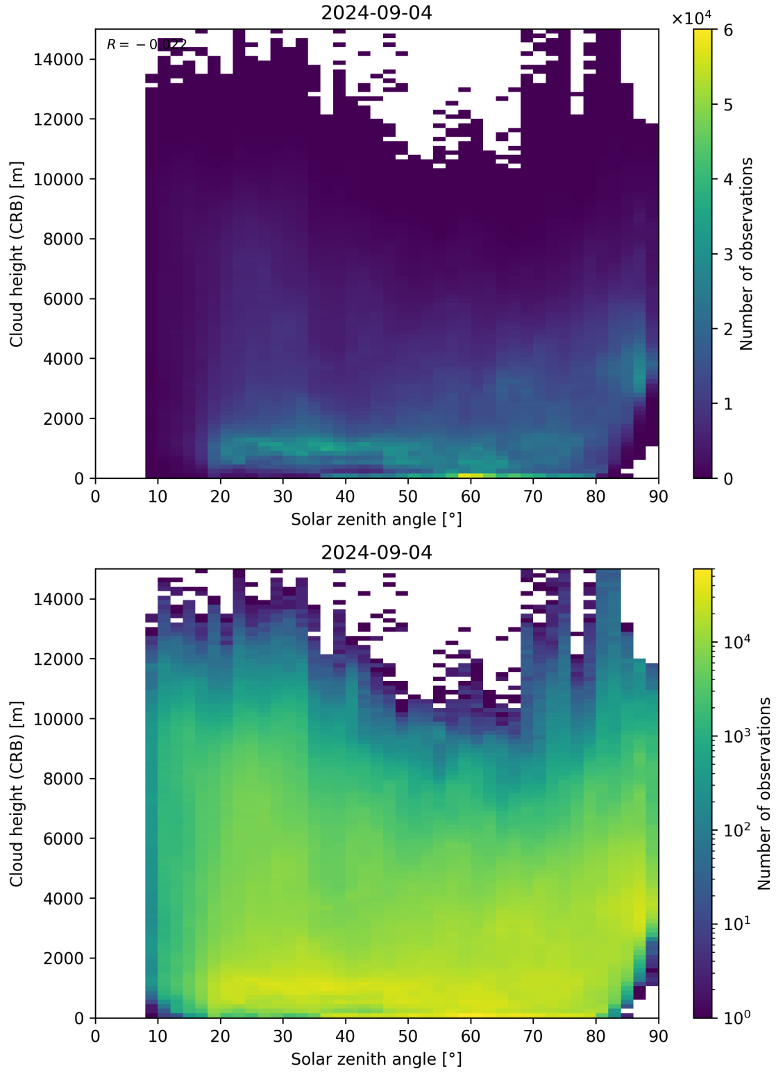
Figure 102: Scatter density plot of “Solar zenith angle” against “Cloud height (CRB)” for 2024-09-03 to 2024-09-05.
