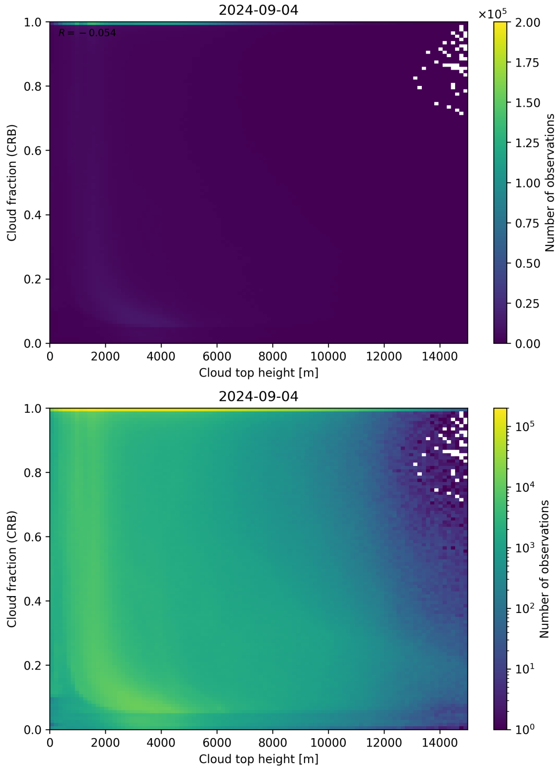
Figure 88: Scatter density plot of “Cloud top height” against “Cloud fraction (CRB)” for 2024-09-03 to 2024-09-05.
