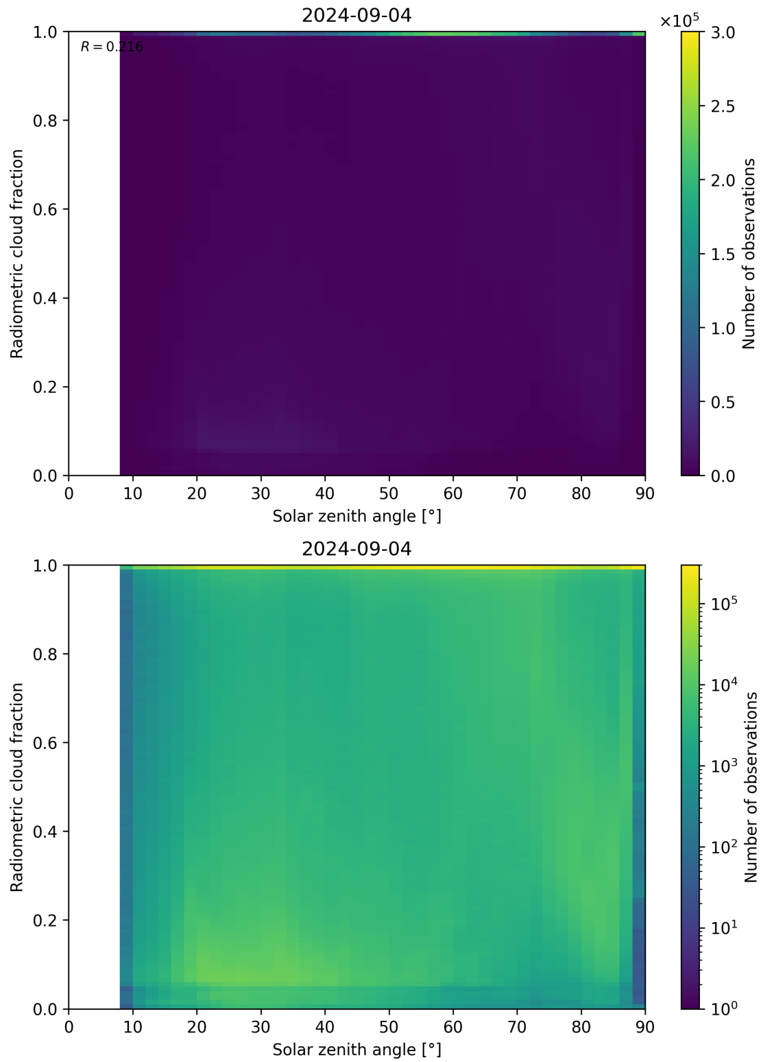
Figure 99: Scatter density plot of “Solar zenith angle” against “Radiometric cloud fraction” for 2024-09-03 to 2024-09-05.
