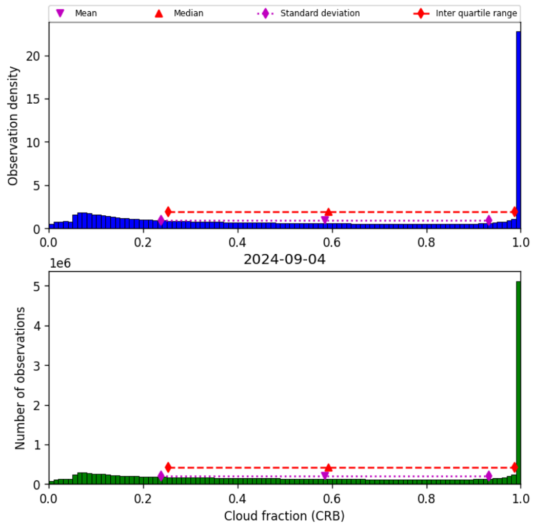
Figure 42: Histogram of “Cloud fraction (CRB)” for 2024-09-03 to 2024-09-05
