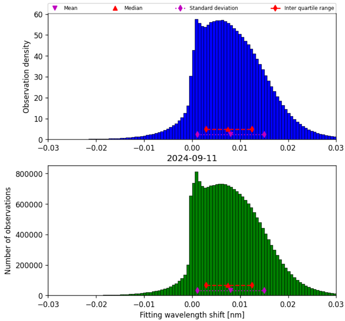
Figure 49: Histogram of “Fitting wavelength shift” for 2024-09-10 to 2024-09-12
