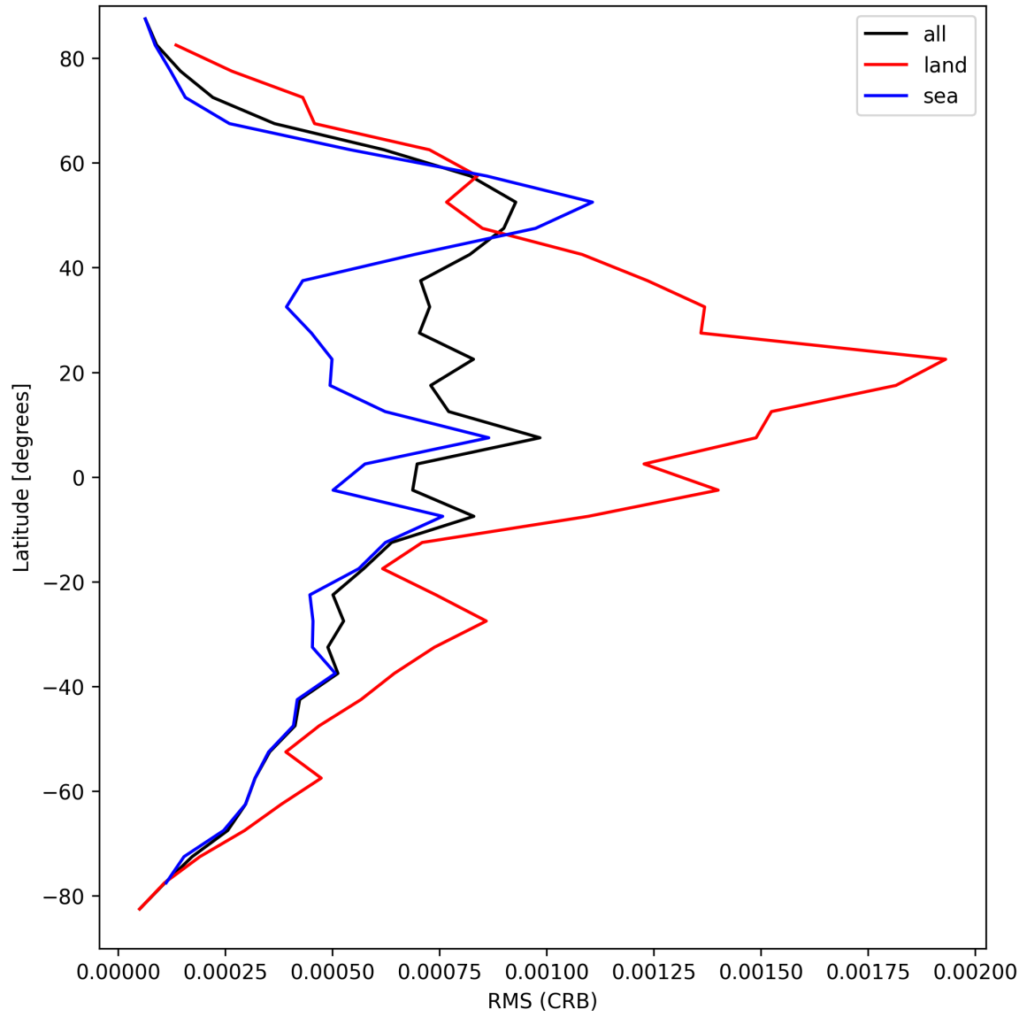
Figure 32: Zonal average of “RMS (CRB)” for 2024-09-10 to 2024-09-12.
