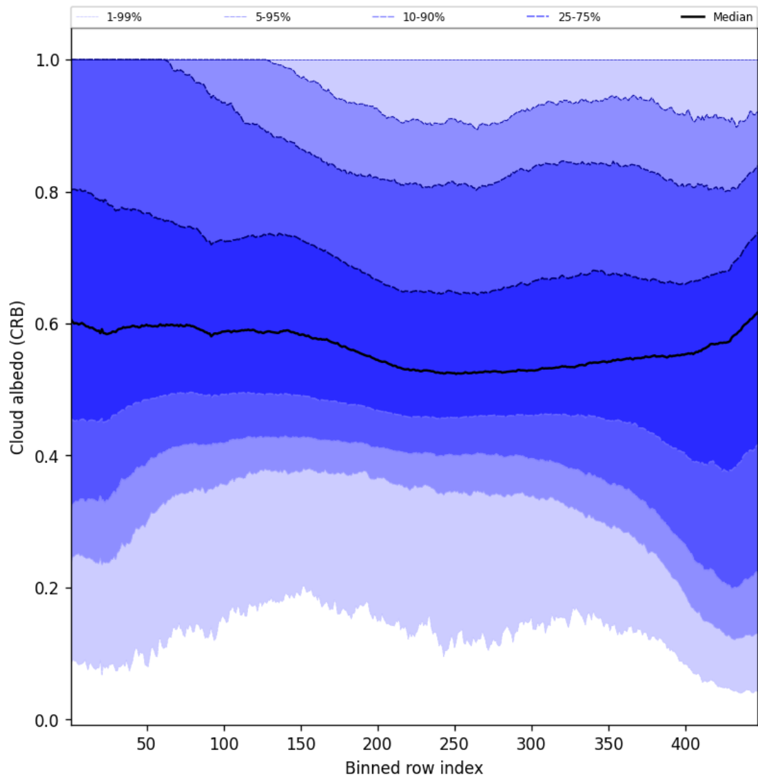
Figure 60: Along track statistics of “Cloud albedo (CRB)” for 2024-09-10 to 2024-09-12
