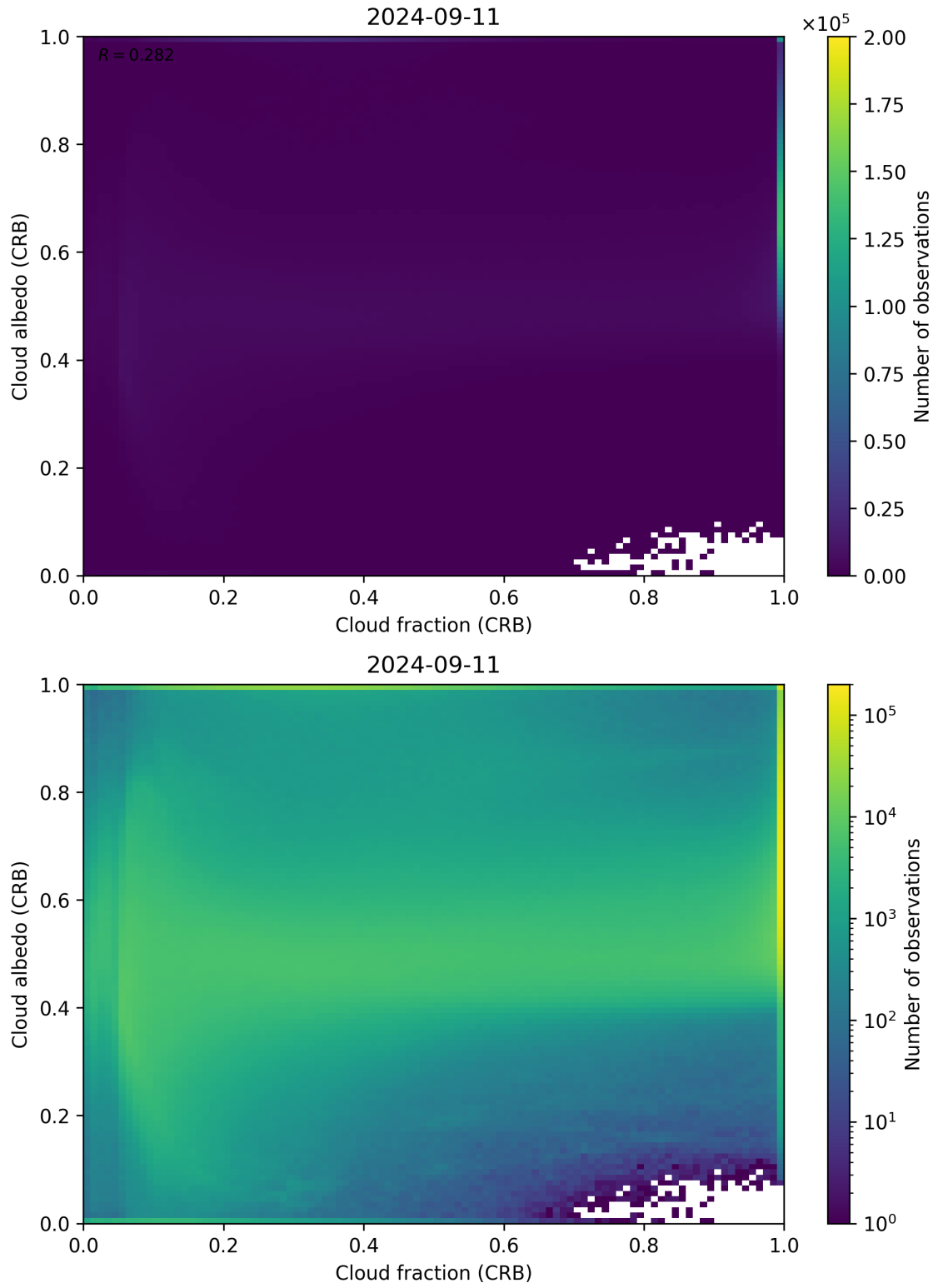
Figure 77: Scatter density plot of “Cloud fraction (CRB)” against “Cloud albedo (CRB)” for 2024-09-10 to 2024-09-12.
