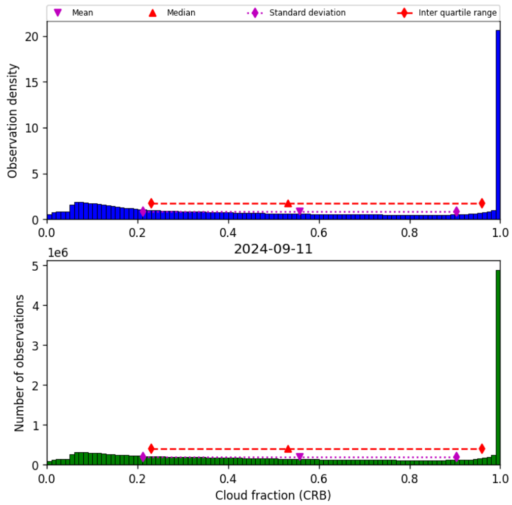
Figure 42: Histogram of “Cloud fraction (CRB)” for 2024-09-10 to 2024-09-12
