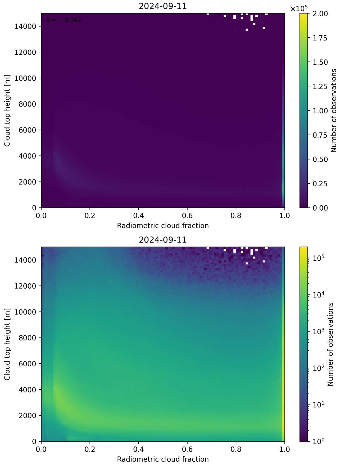
Figure 76: Scatter density plot of “Radiometric cloud fraction” against “Cloud top height” for 2024-09-10 to 2024-09-12.
