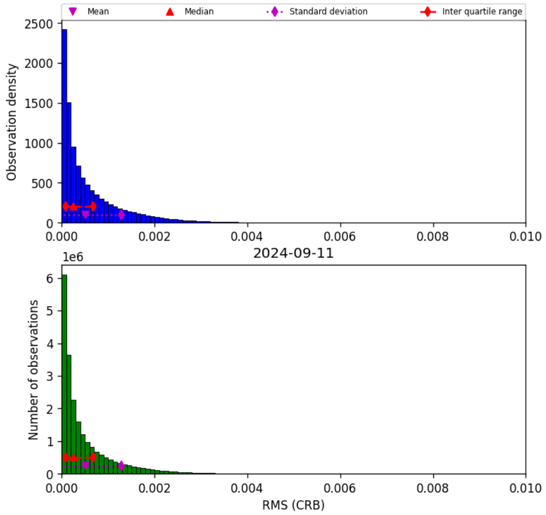
Figure 48: Histogram of “RMS (CRB)” for 2024-09-10 to 2024-09-12
