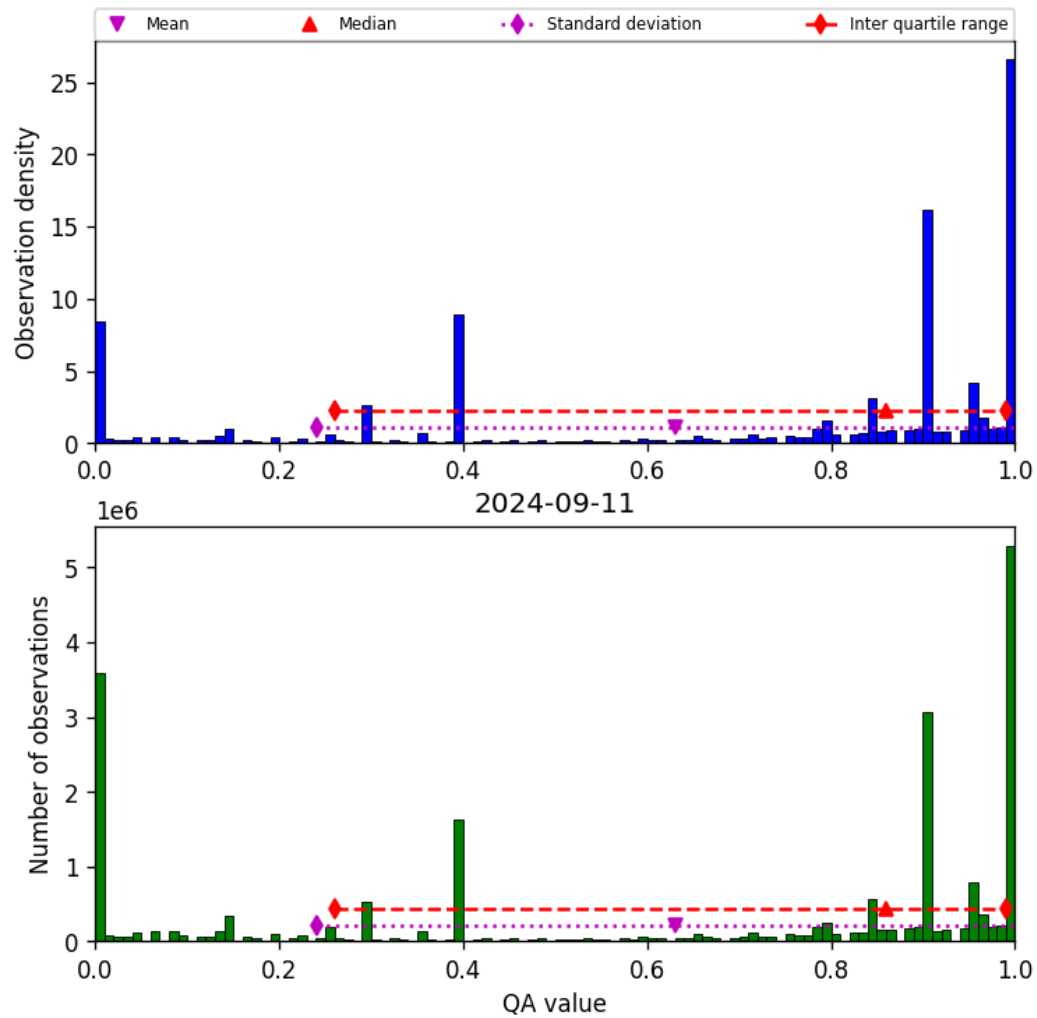
Figure 38: Histogram of “QA value” for 2024-09-10 to 2024-09-12
