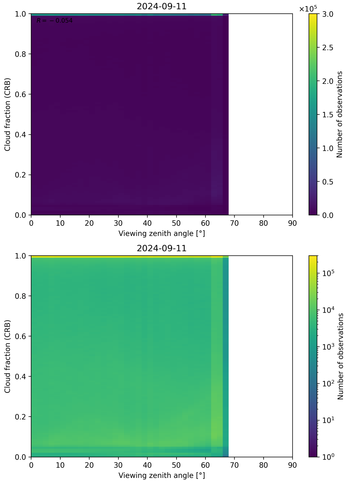
Figure 109: Scatter density plot of “Viewing zenith angle” against “Cloud fraction (CRB)” for 2024-09-10 to 2024-09-12.
