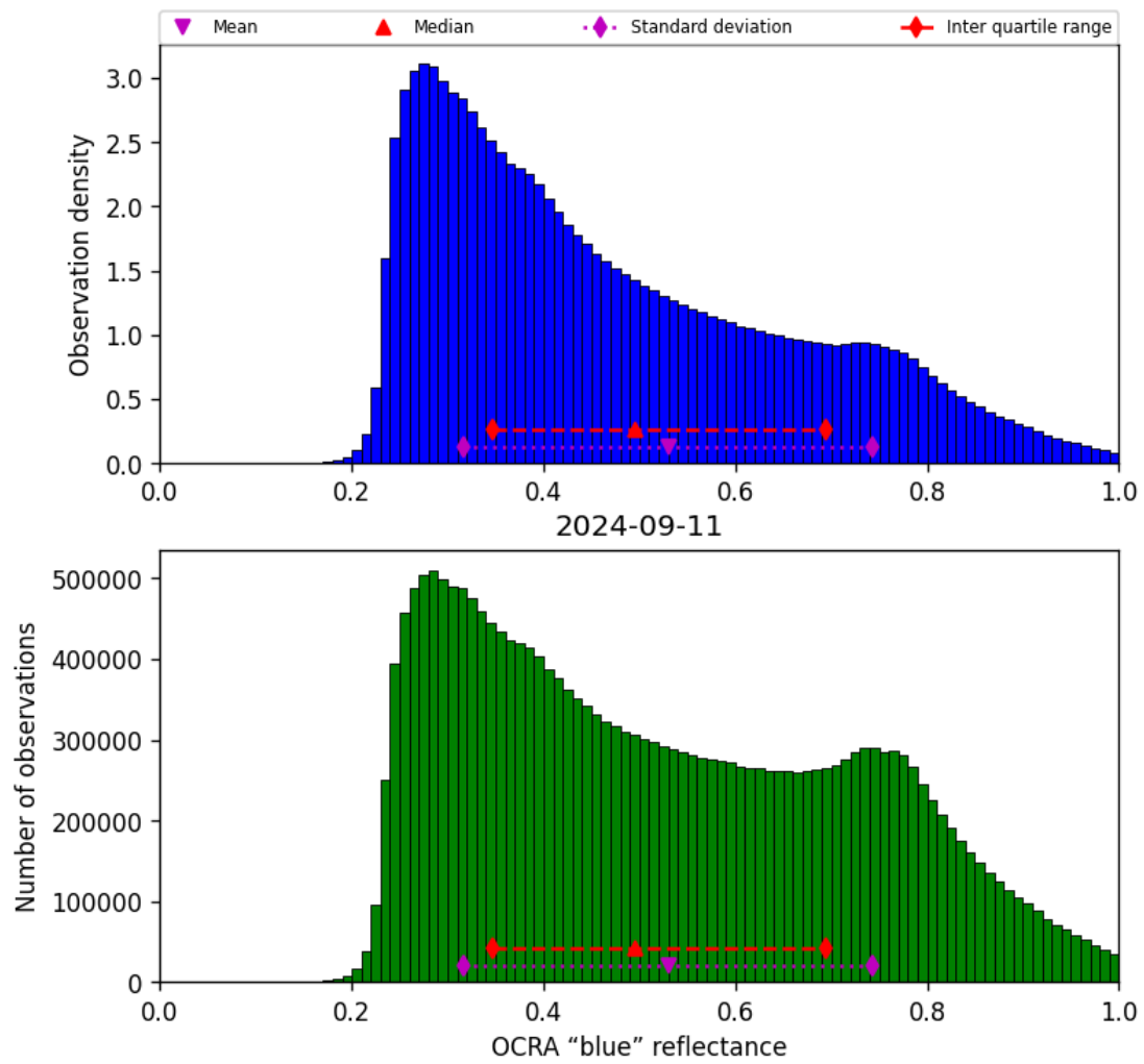
Figure 51: Histogram of “OCRA “blue” reflectance” for 2024-09-10 to 2024-09-12
