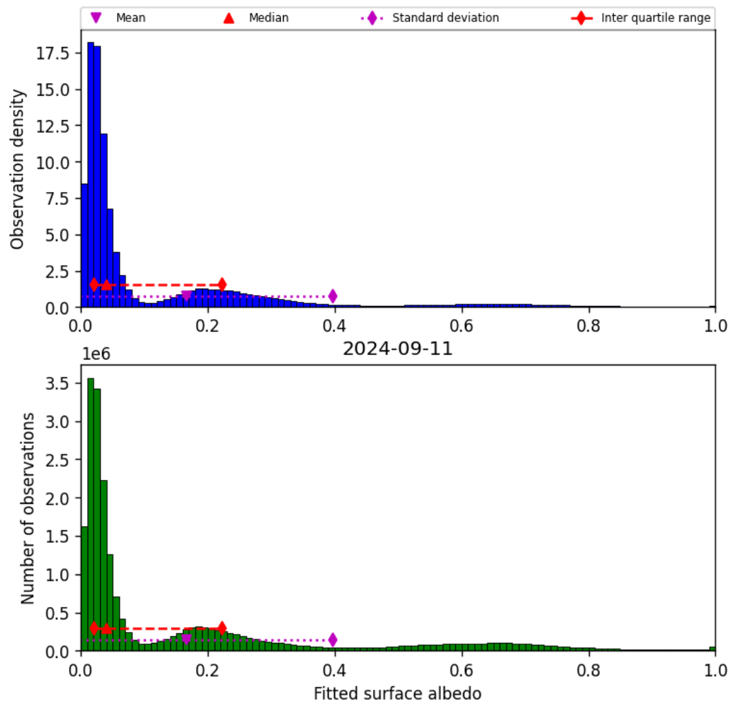
Figure 45: Histogram of “Fitted surface albedo” for 2024-09-10 to 2024-09-12
