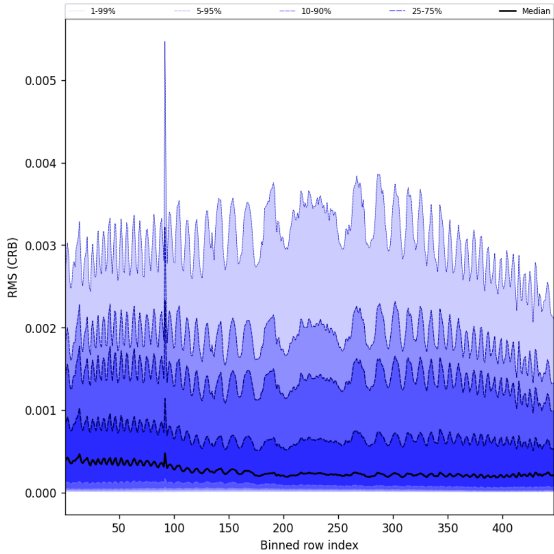
Figure 64: Along track statistics of “RMS (CRB)” for 2024-09-10 to 2024-09-12
