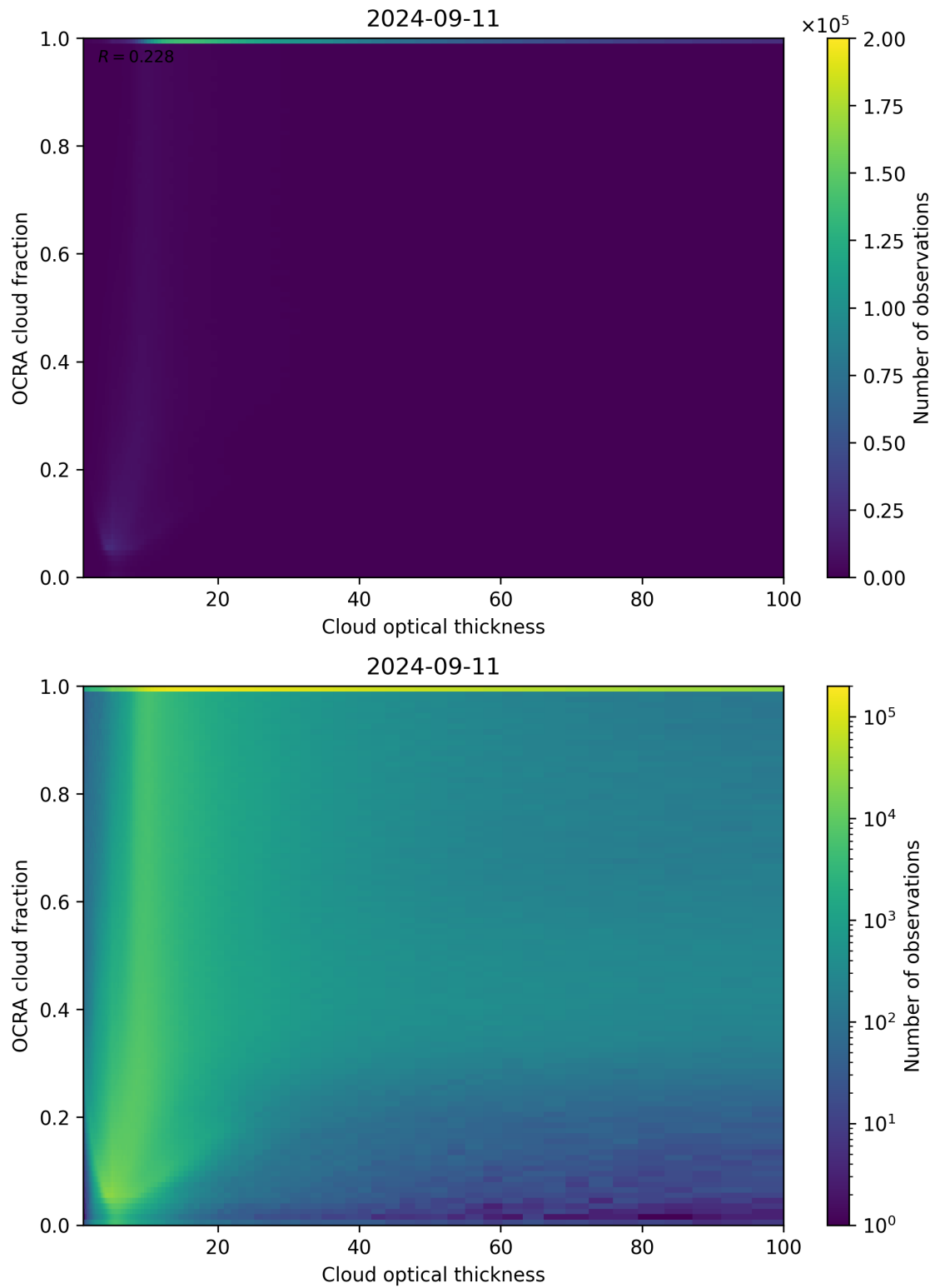
Figure 83: Scatter density plot of “Cloud optical thickness” against “OCRA cloud fraction” for 2024-09-10 to 2024-09-12.
