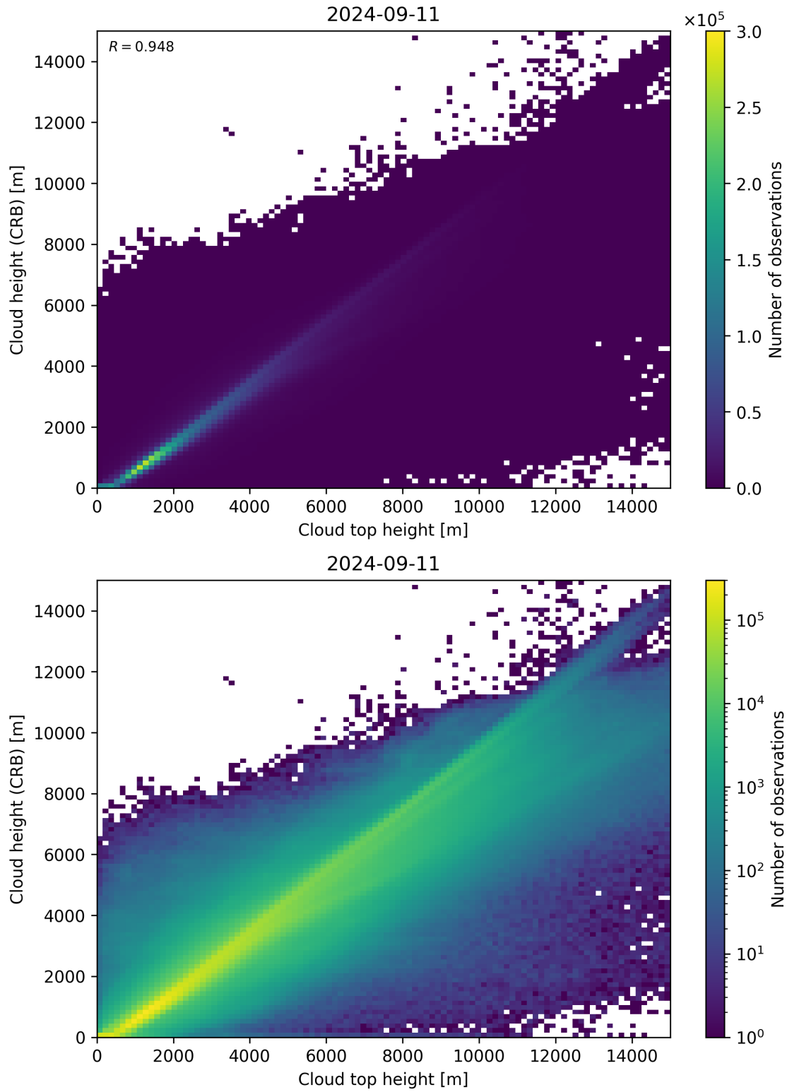
Figure 89: Scatter density plot of “Cloud top height” against “Cloud height (CRB)” for 2024-09-10 to 2024-09-12.
