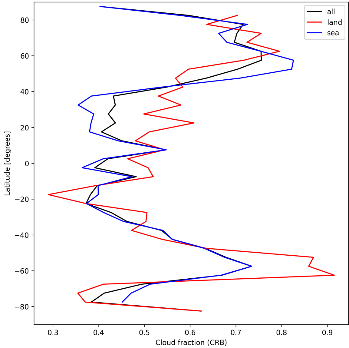
Figure 26: Zonal average of “Cloud fraction (CRB)” for 2024-09-10 to 2024-09-12.
