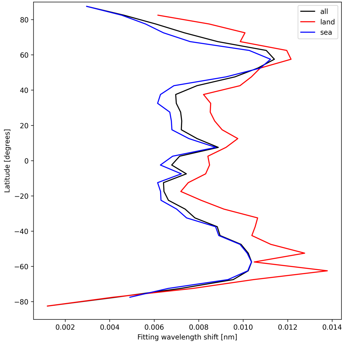
Figure 33: Zonal average of “Fitting wavelength shift” for 2024-09-10 to 2024-09-12.
