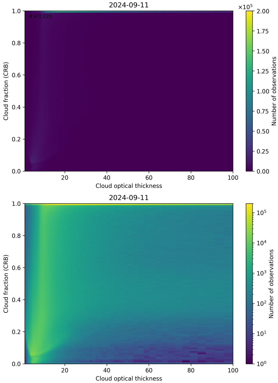
Figure 84: Scatter density plot of “Cloud optical thickness” against “Cloud fraction (CRB)” for 2024-09-10 to 2024-09-12.
