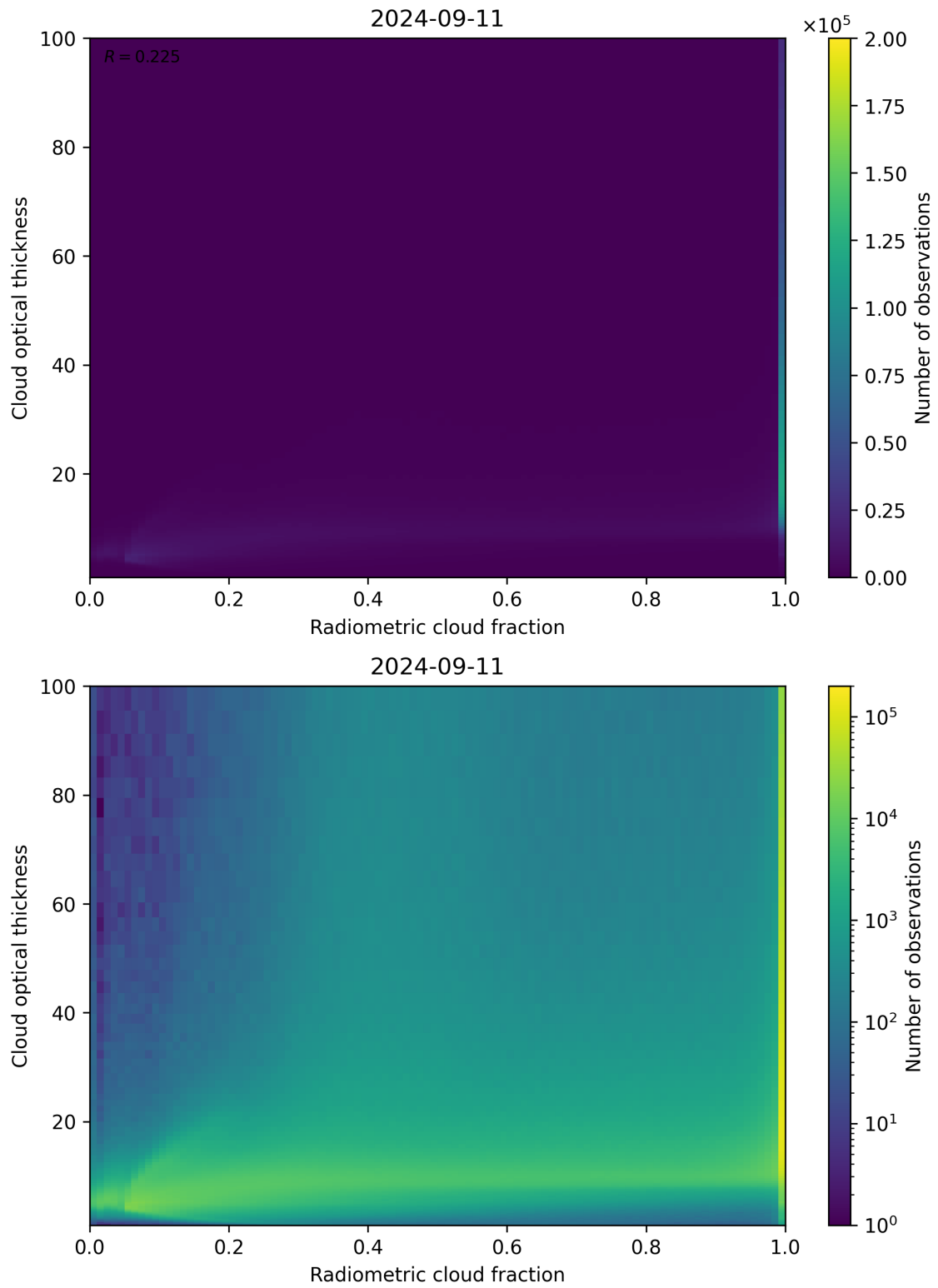
Figure 75: Scatter density plot of “Radiometric cloud fraction” against “Cloud optical thickness” for 2024-09-10 to 2024-09-12.
