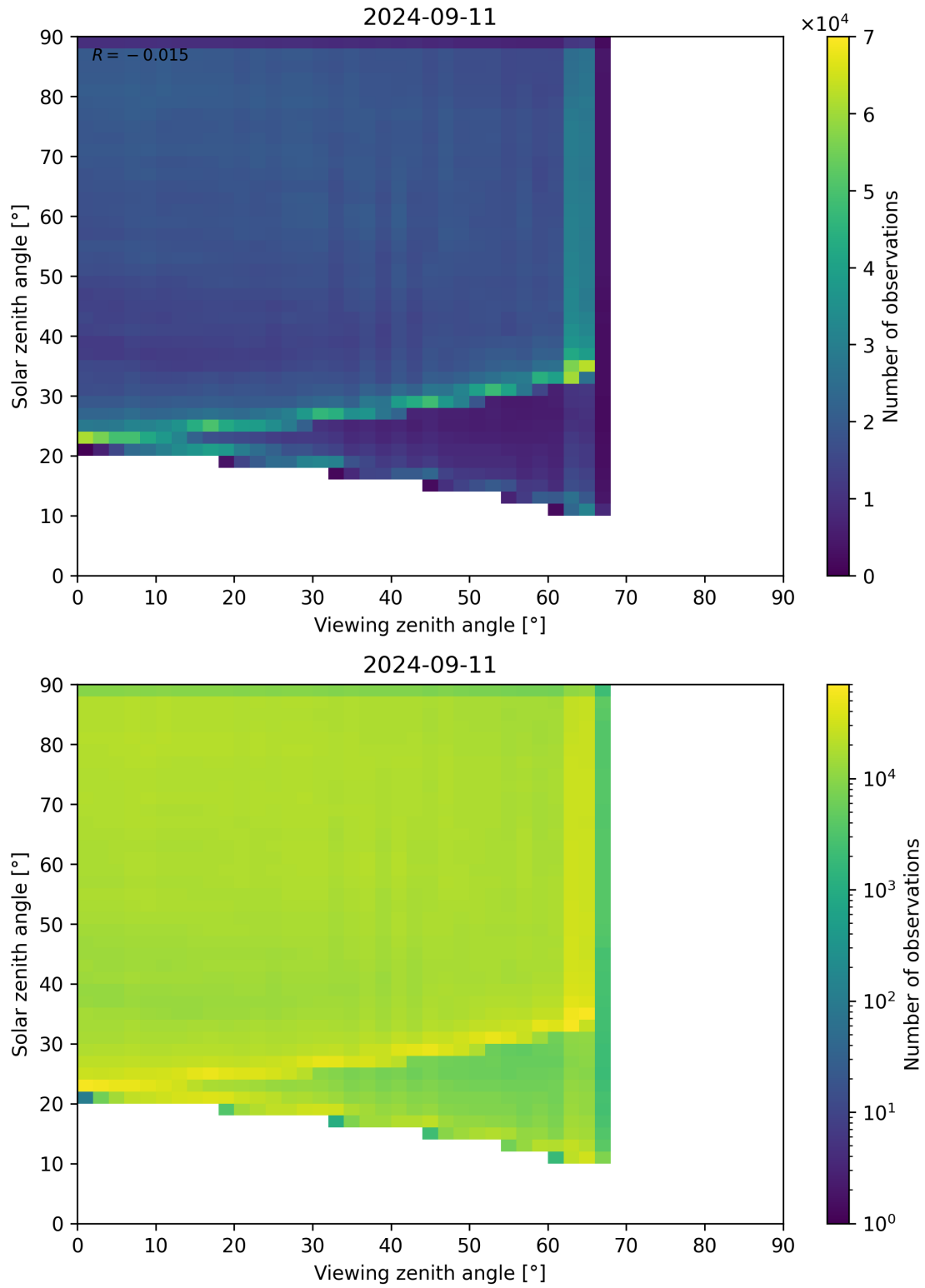
Figure 114: Scatter density plot of “Viewing zenith angle” against “Solar zenith angle” for 2024-09-10 to 2024-09-12.
