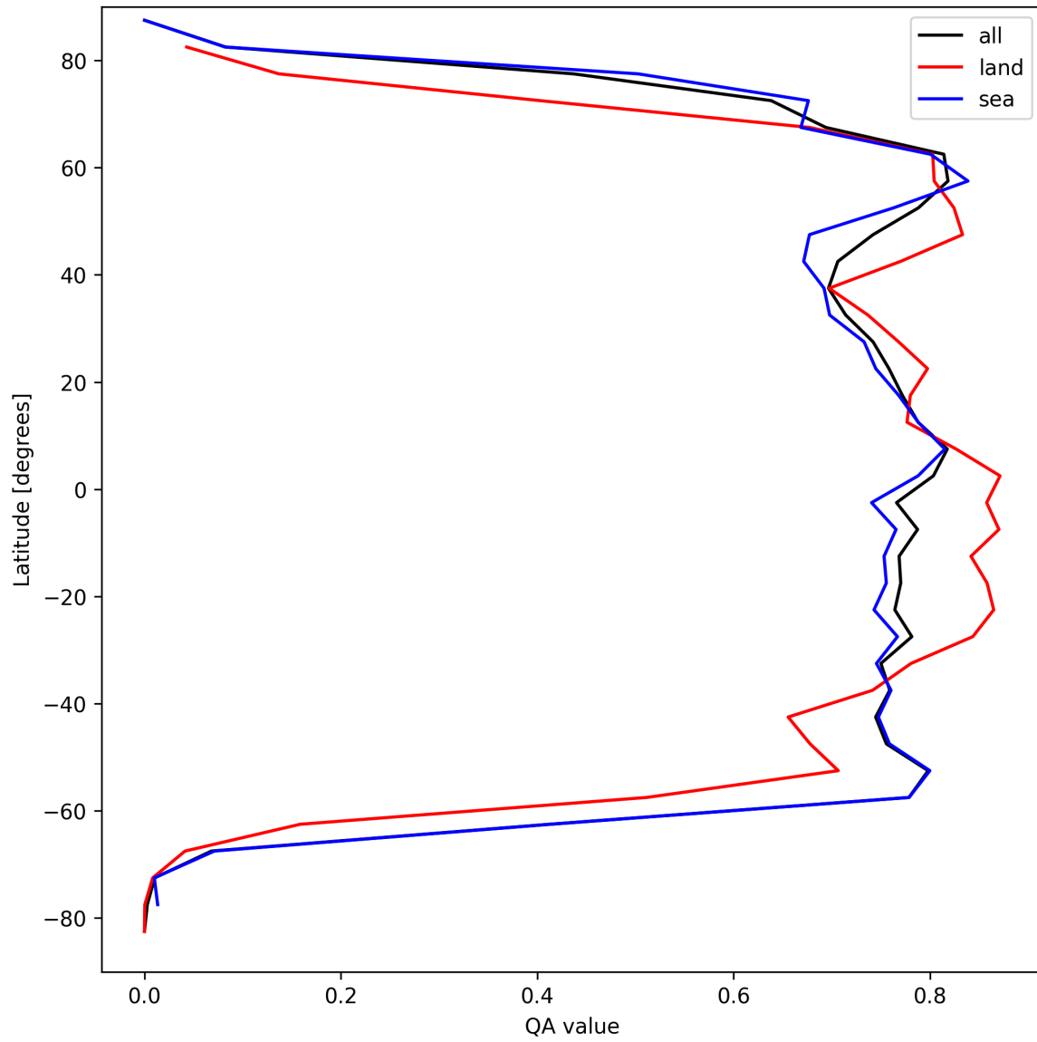
Figure 22: Zonal average of “QA value” for 2024-09-10 to 2024-09-12.
