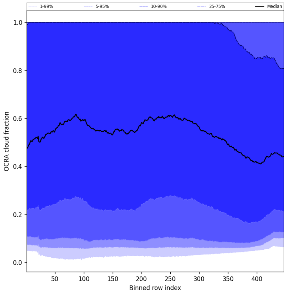
Figure 66: Along track statistics of “OCRA cloud fraction” for 2024-09-10 to 2024-09-12
