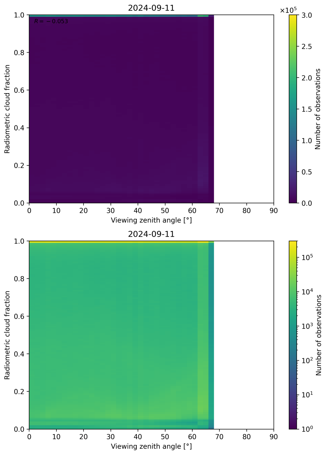
Figure 107: Scatter density plot of “Viewing zenith angle” against “Radiometric cloud fraction” for 2024-09-10 to 2024-09-12.
