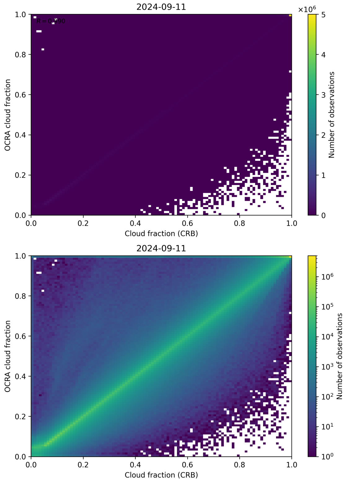
Figure 78: Scatter density plot of “Cloud fraction (CRB)” against “OCRA cloud fraction” for 2024-09-10 to 2024-09-12.
