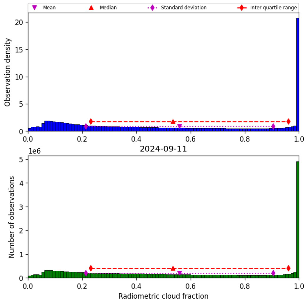
Figure 39: Histogram of “Radiometric cloud fraction” for 2024-09-10 to 2024-09-12
