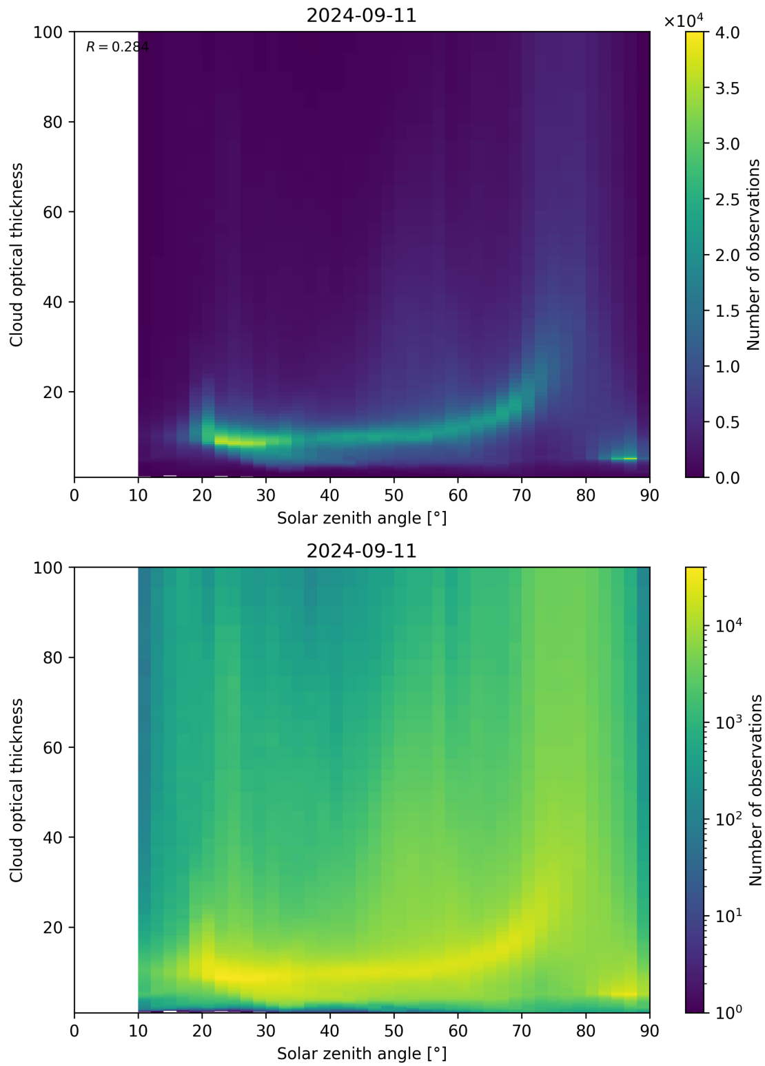
Figure 103: Scatter density plot of “Solar zenith angle” against “Cloud optical thickness” for 2024-09-10 to 2024-09-12.
