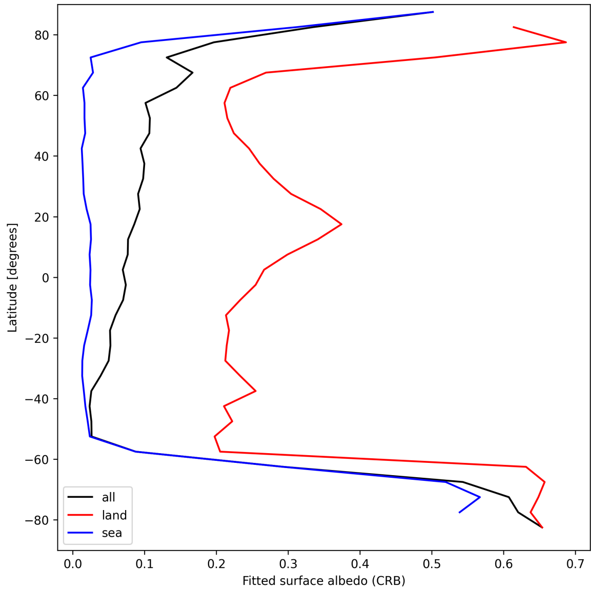
Figure 30: Zonal average of “Fitted surface albedo (CRB)” for 2024-09-10 to 2024-09-12.
