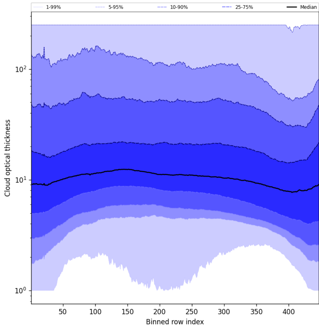
Figure 57: Along track statistics of “Cloud optical thickness” for 2024-09-10 to 2024-09-12
