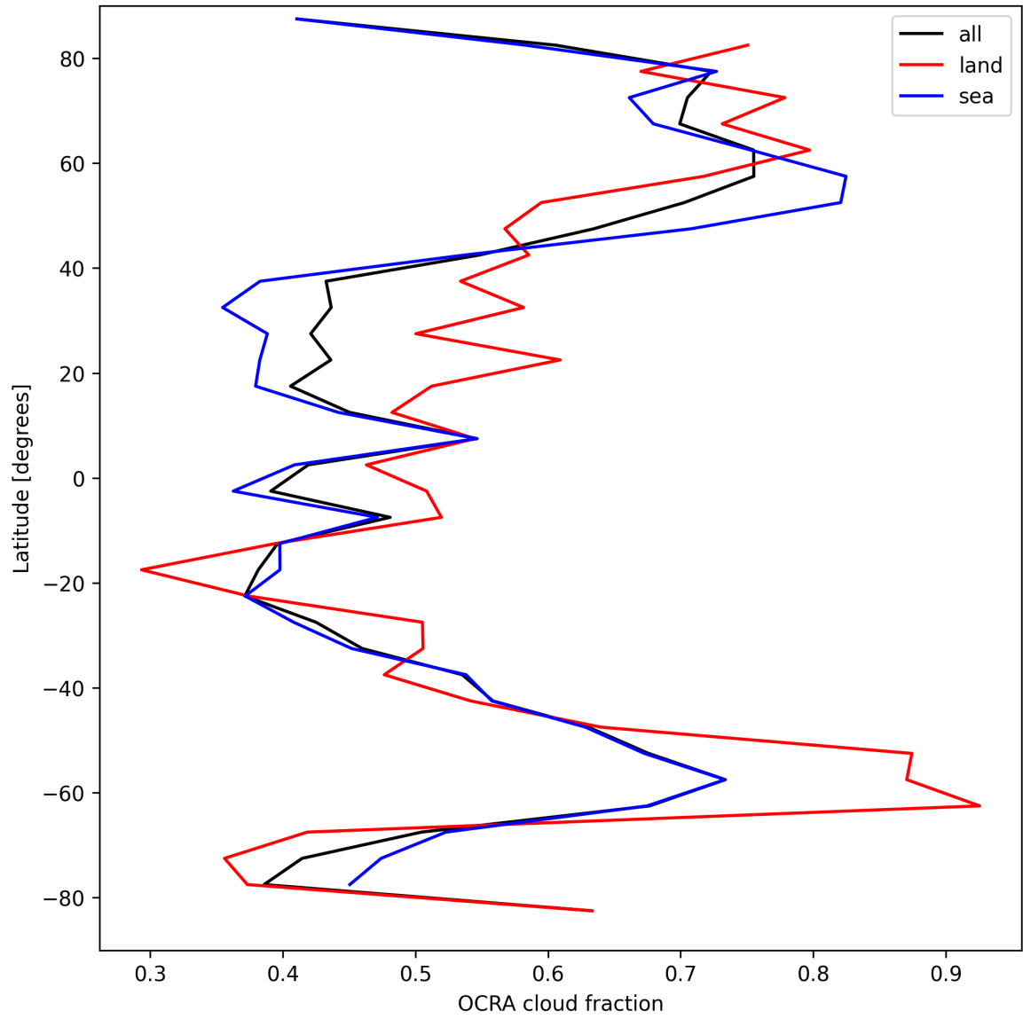
Figure 34: Zonal average of “OCRA cloud fraction” for 2024-09-10 to 2024-09-12.
