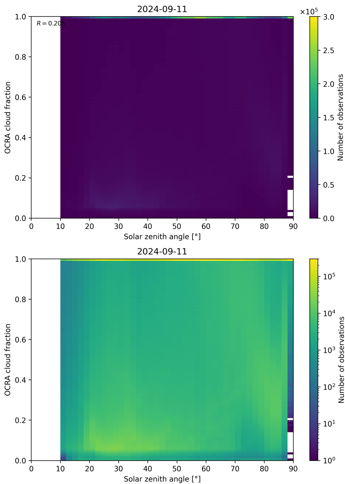
Figure 100: Scatter density plot of “Solar zenith angle” against “OCRA cloud fraction” for 2024-09-10 to 2024-09-12.
