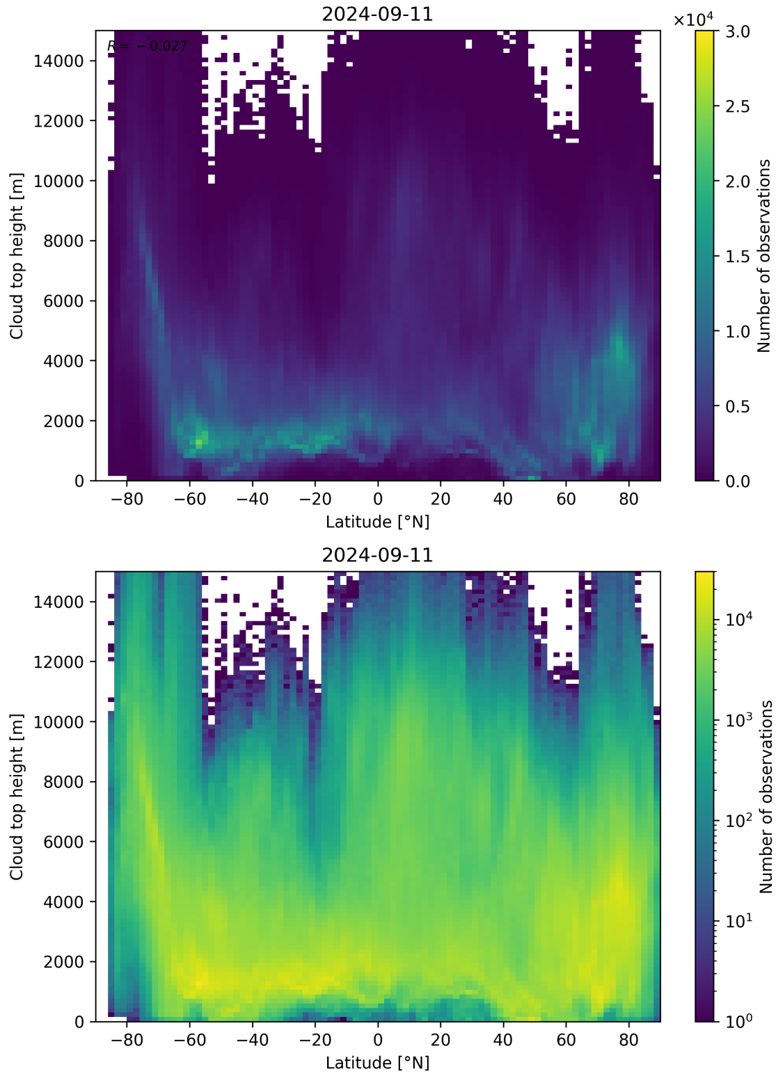
Figure 97: Scatter density plot of “Latitude” against “Cloud top height” for 2024-09-10 to 2024-09-12.
