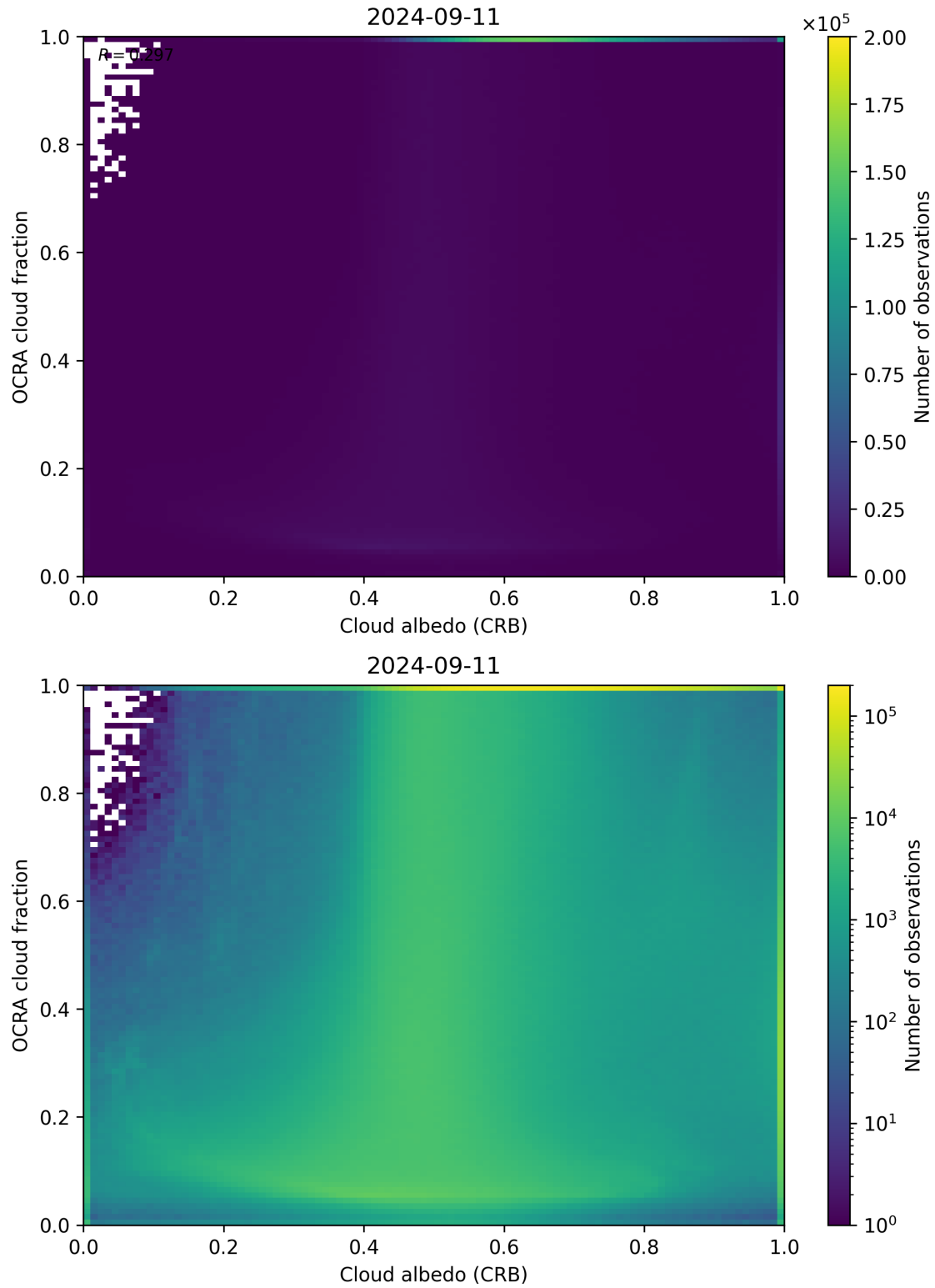
Figure 70: Scatter density plot of “Cloud albedo (CRB)” against “OCRA cloud fraction” for 2024-09-10 to 2024-09-12.
