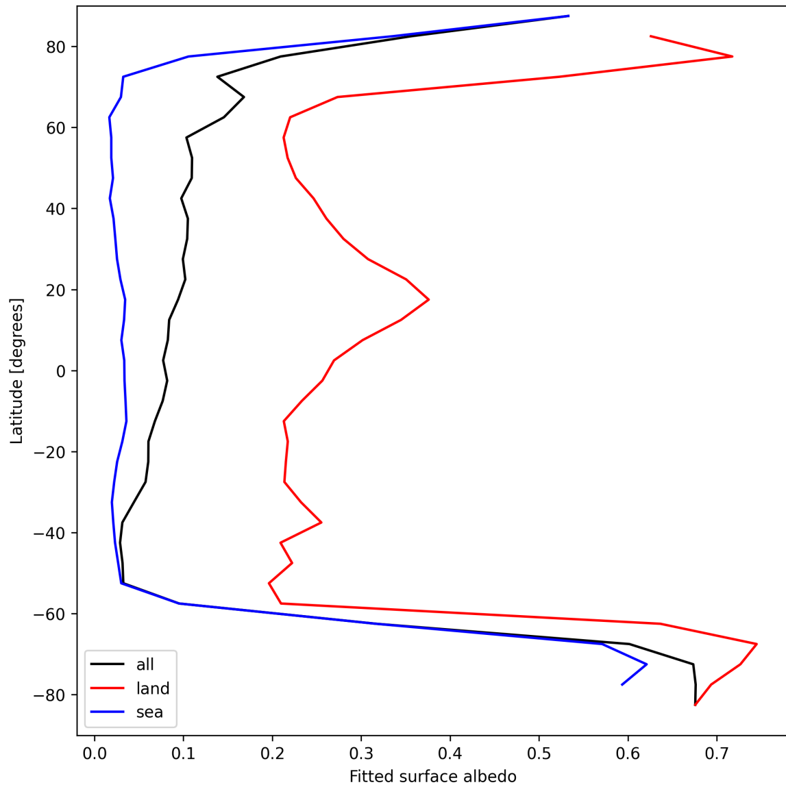
Figure 29: Zonal average of “Fitted surface albedo” for 2024-09-10 to 2024-09-12.
