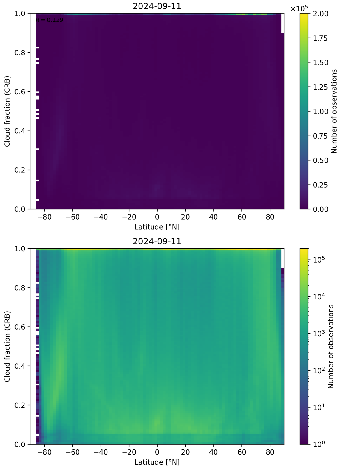
Figure 94: Scatter density plot of “Latitude” against “Cloud fraction (CRB)” for 2024-09-10 to 2024-09-12.
