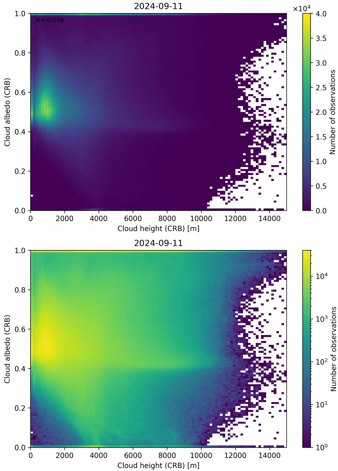
Figure 80: Scatter density plot of “Cloud height (CRB)” against “Cloud albedo (CRB)” for 2024-09-10 to 2024-09-12.
