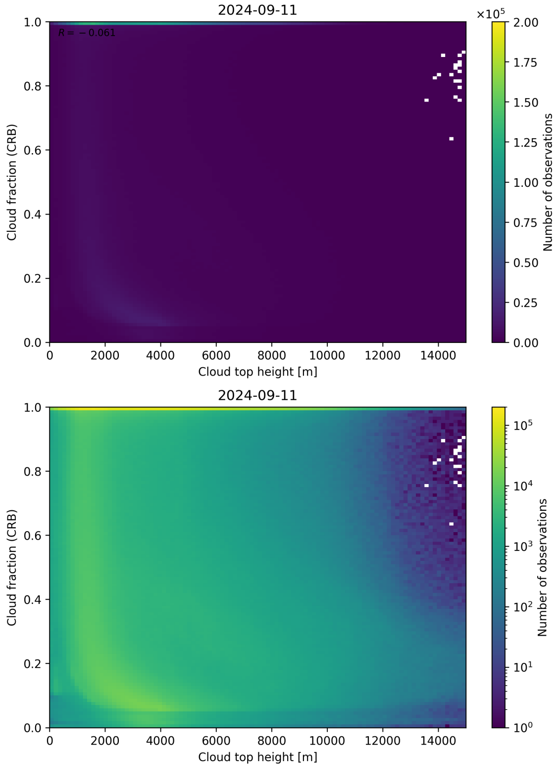
Figure 88: Scatter density plot of “Cloud top height” against “Cloud fraction (CRB)” for 2024-09-10 to 2024-09-12.
