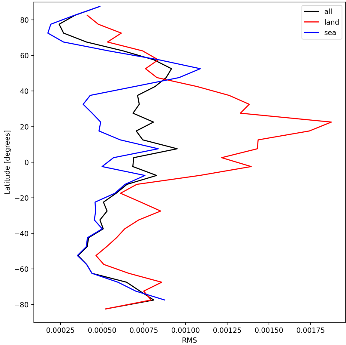
Figure 31: Zonal average of “RMS” for 2024-09-10 to 2024-09-12.
