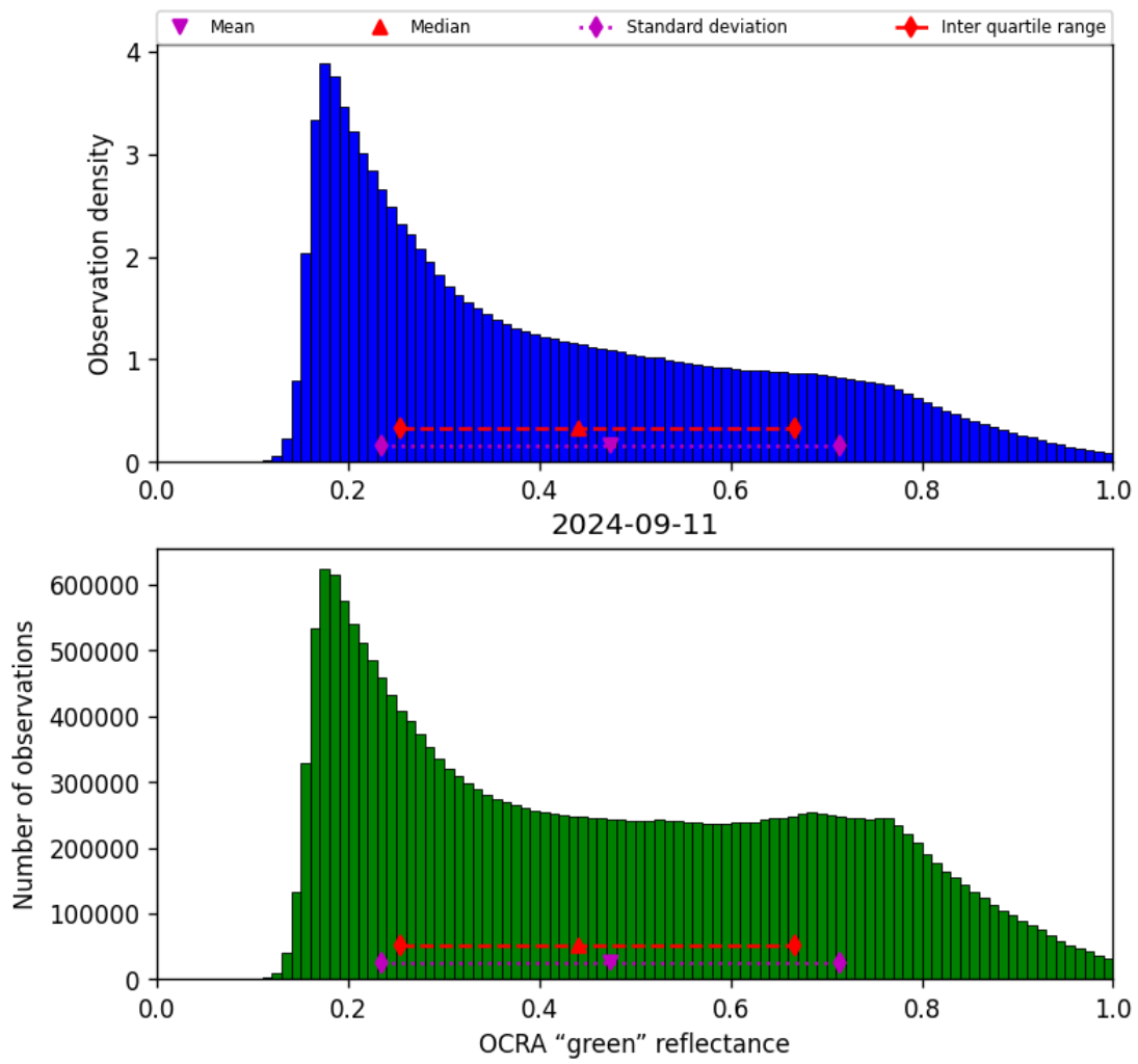
Figure 52: Histogram of “OCRA “green” reflectance” for 2024-09-10 to 2024-09-12
