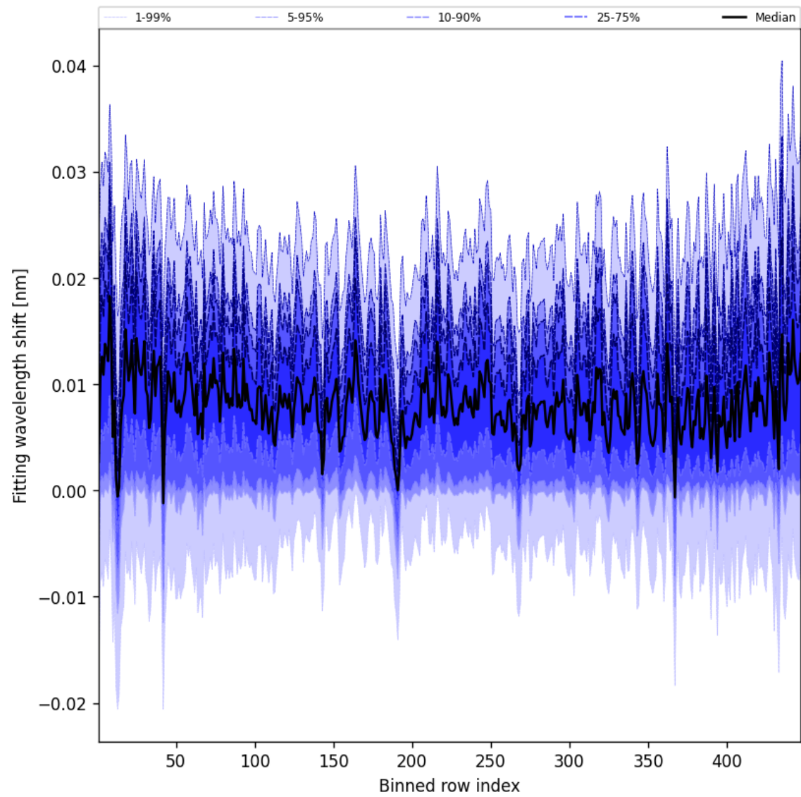
Figure 65: Along track statistics of “Fitting wavelength shift” for 2024-09-10 to 2024-09-12
