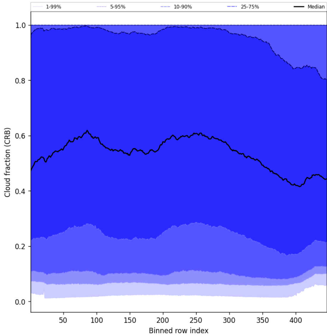
Figure 58: Along track statistics of “Cloud fraction (CRB)” for 2024-09-10 to 2024-09-12
