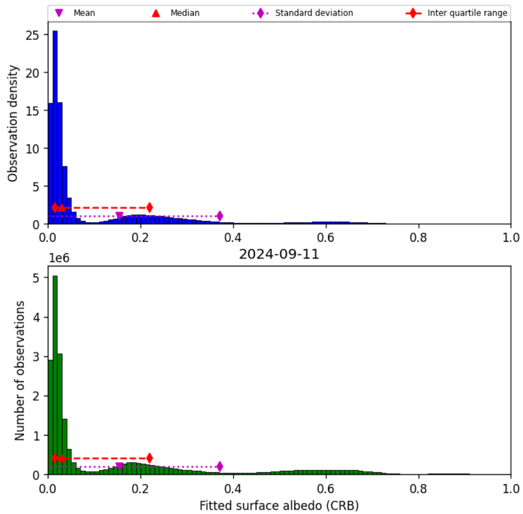
Figure 46: Histogram of “Fitted surface albedo (CRB)” for 2024-09-10 to 2024-09-12
