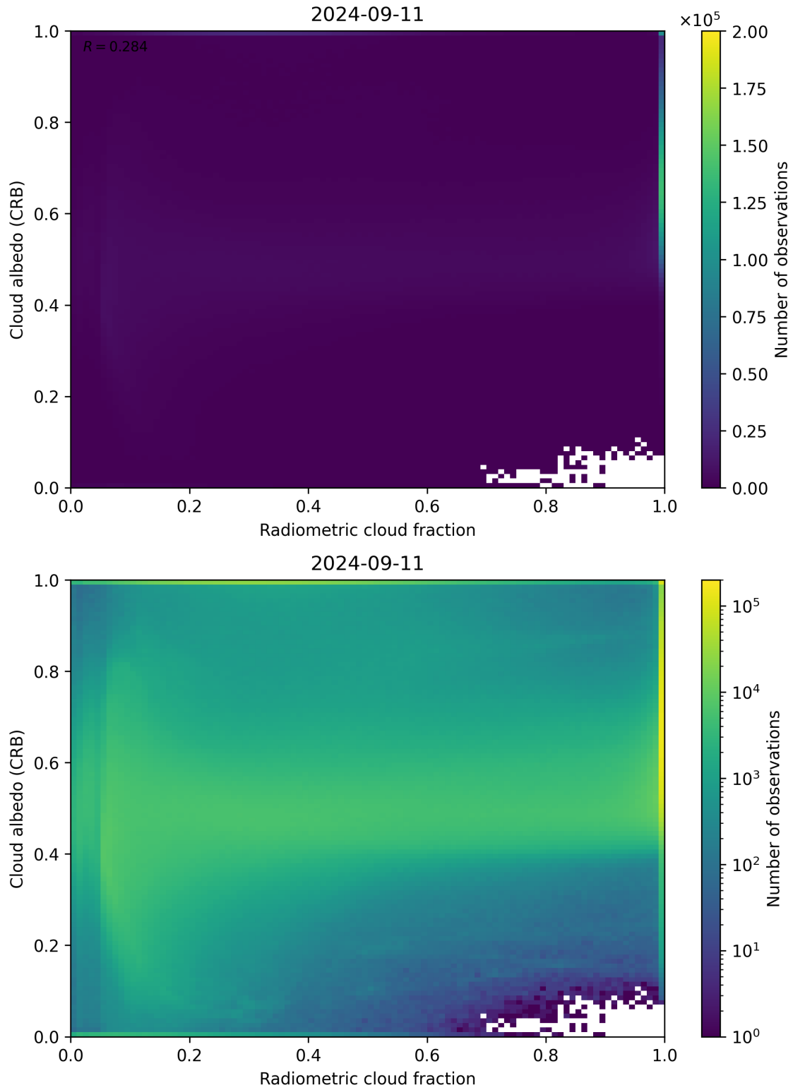
Figure 71: Scatter density plot of “Radiometric cloud fraction” against “Cloud albedo (CRB)” for 2024-09-10 to 2024-09-12.
