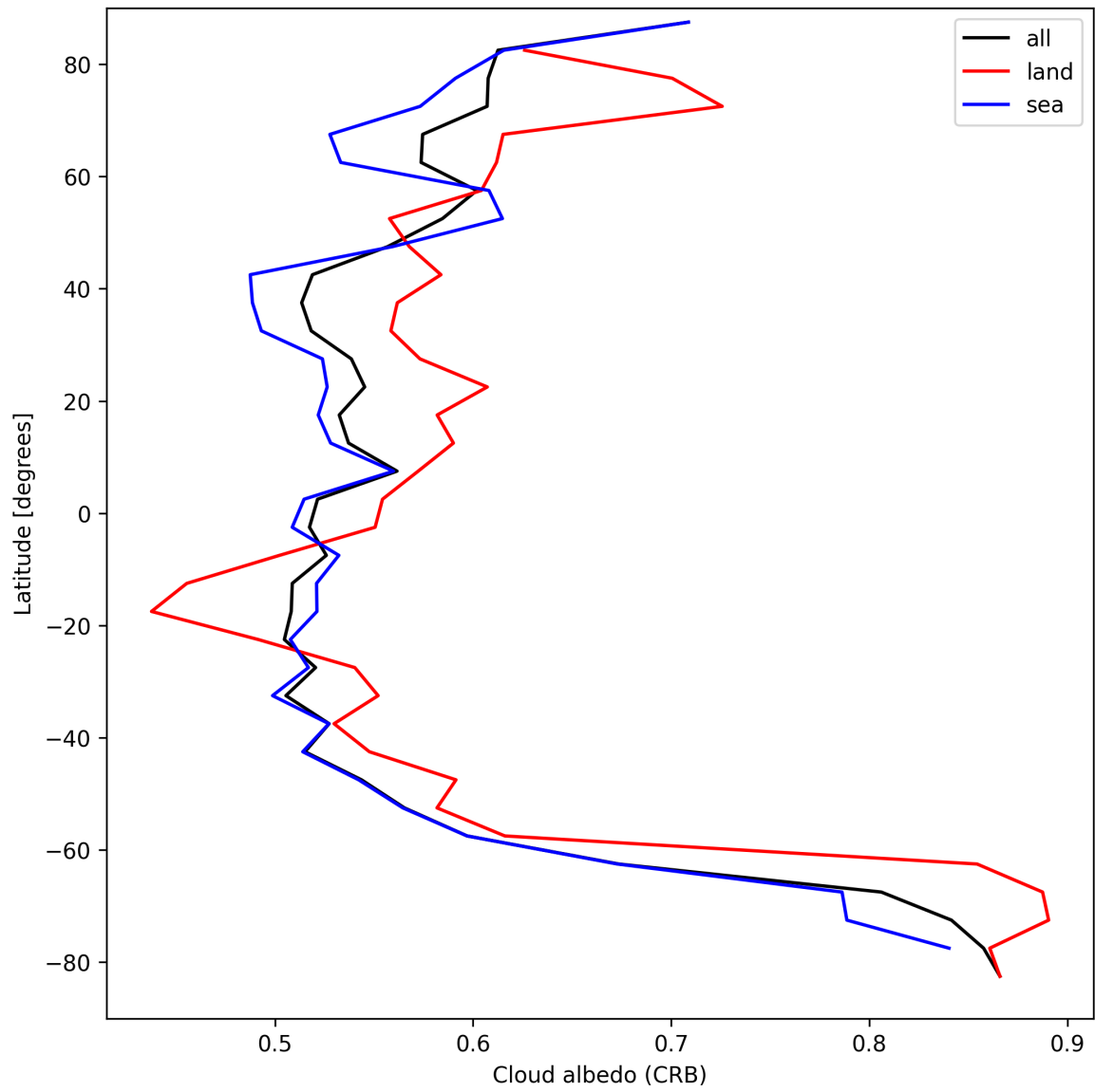
Figure 28: Zonal average of “Cloud albedo (CRB)” for 2024-09-10 to 2024-09-12.
