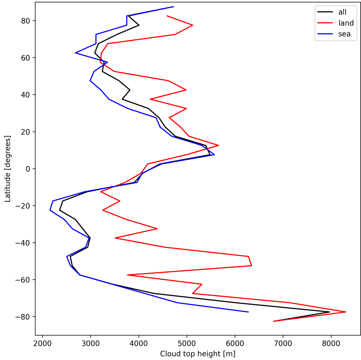
Figure 24: Zonal average of “Cloud top height” for 2024-09-10 to 2024-09-12.
