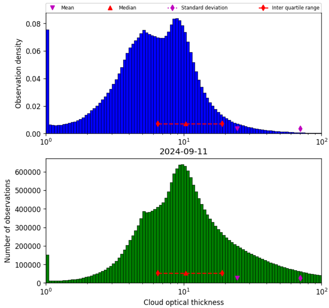
Figure 41: Histogram of “Cloud optical thickness” for 2024-09-10 to 2024-09-12
