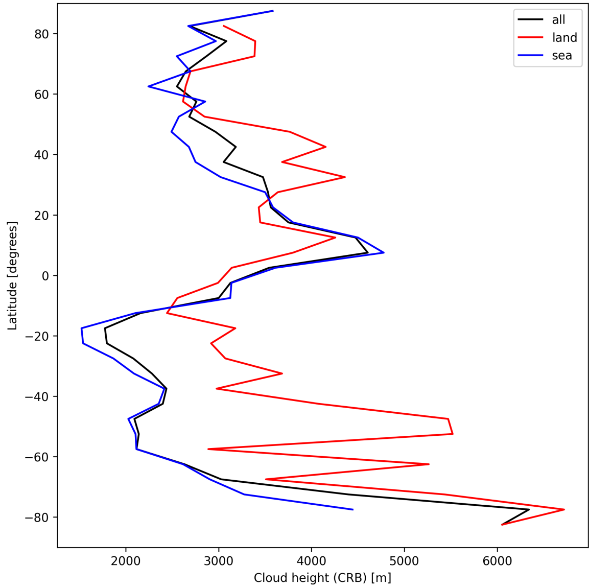
Figure 27: Zonal average of “Cloud height (CRB)” for 2024-09-10 to 2024-09-12.
