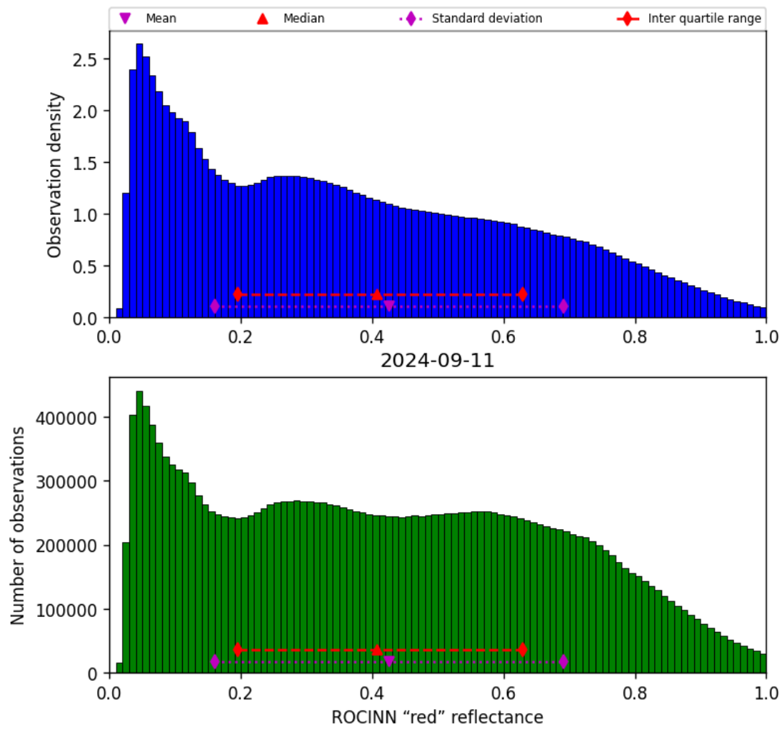
Figure 53: Histogram of “ROCINN “red” reflectance” for 2024-09-10 to 2024-09-12
