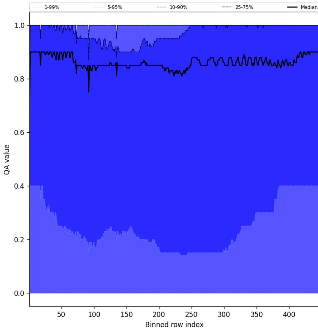
Figure 54: Along track statistics of “QA value” for 2024-09-10 to 2024-09-12
