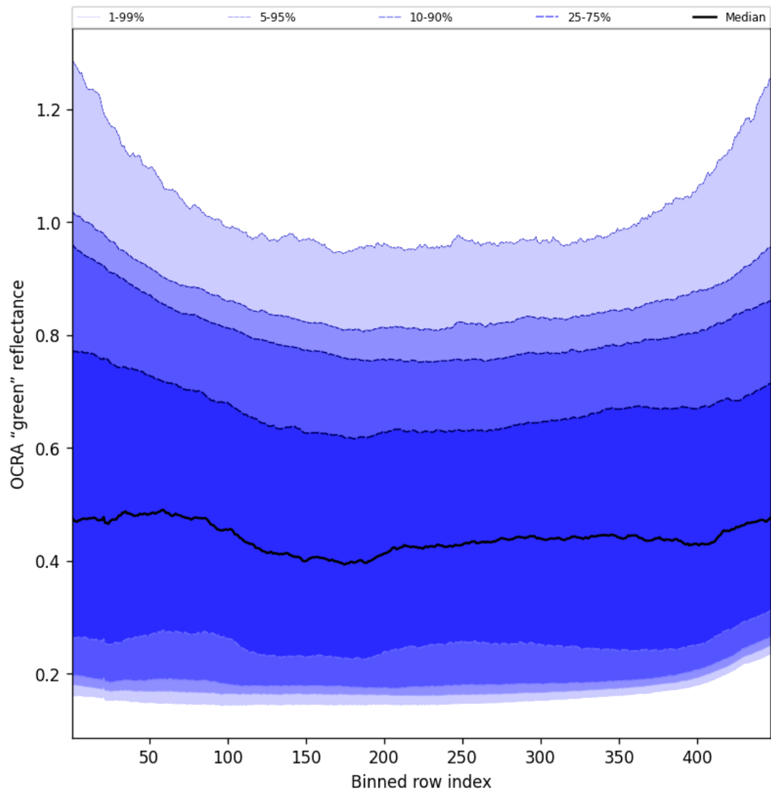
Figure 68: Along track statistics of “OCRA “green” reflectance” for 2024-09-10 to 2024-09-12
