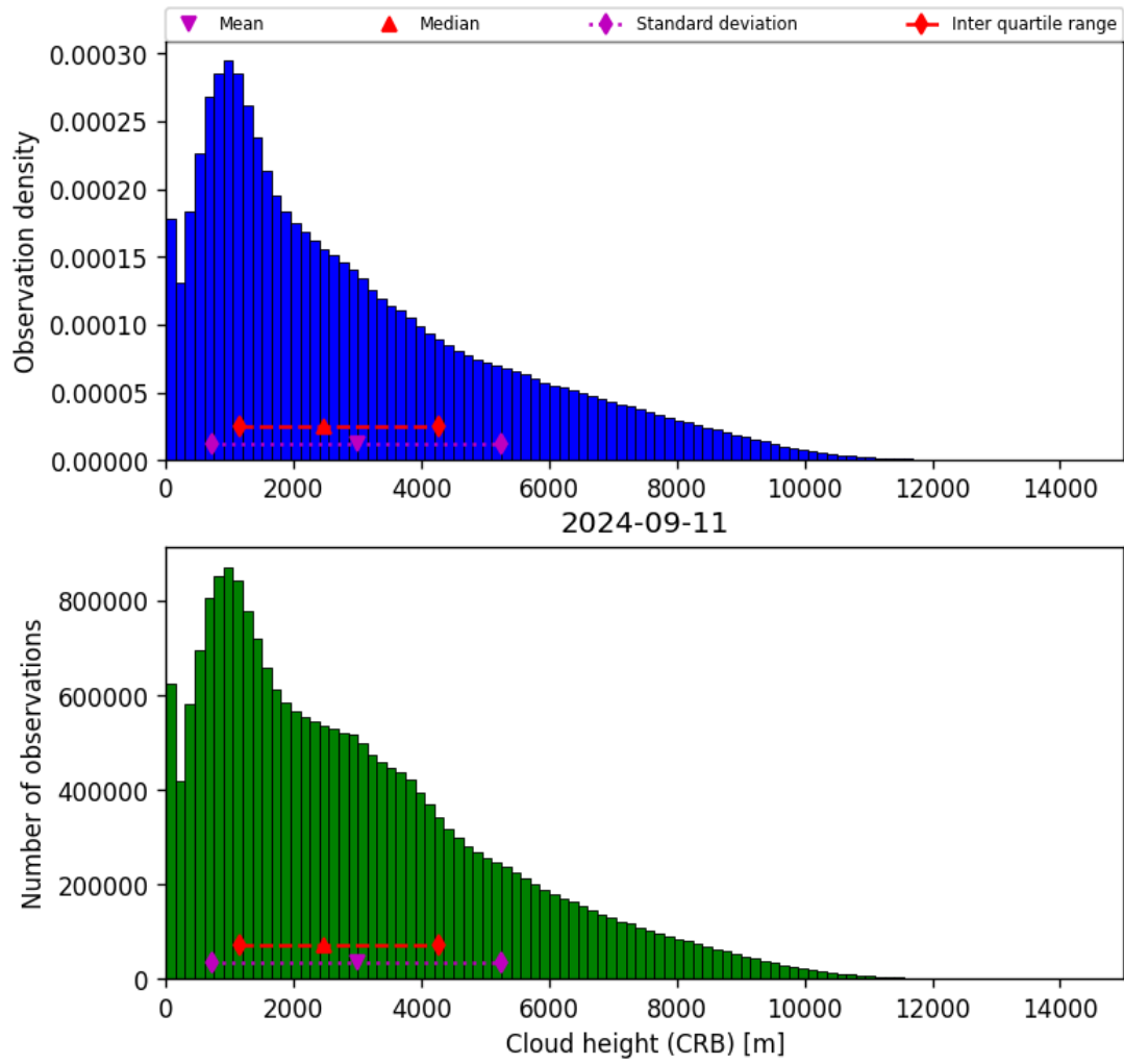
Figure 43: Histogram of “Cloud height (CRB)” for 2024-09-10 to 2024-09-12
