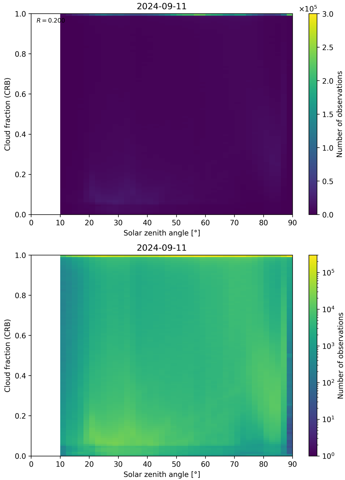
Figure 101: Scatter density plot of “Solar zenith angle” against “Cloud fraction (CRB)” for 2024-09-10 to 2024-09-12.
