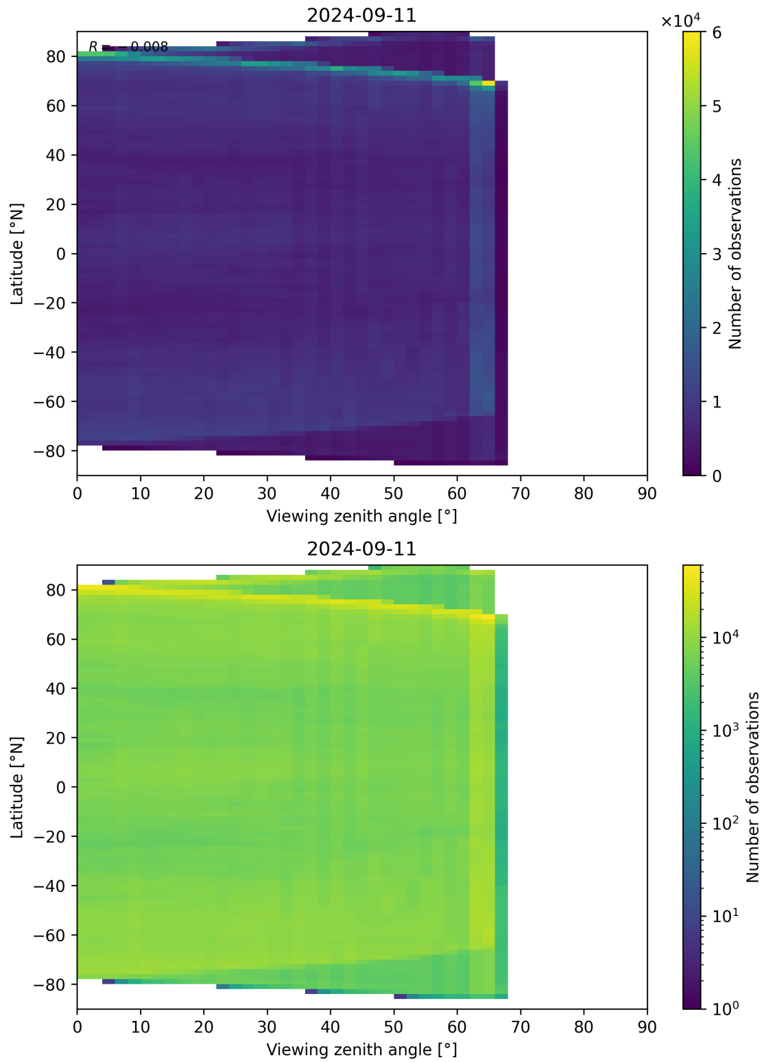
Figure 113: Scatter density plot of “Viewing zenith angle” against “Latitude” for 2024-09-10 to 2024-09-12.
