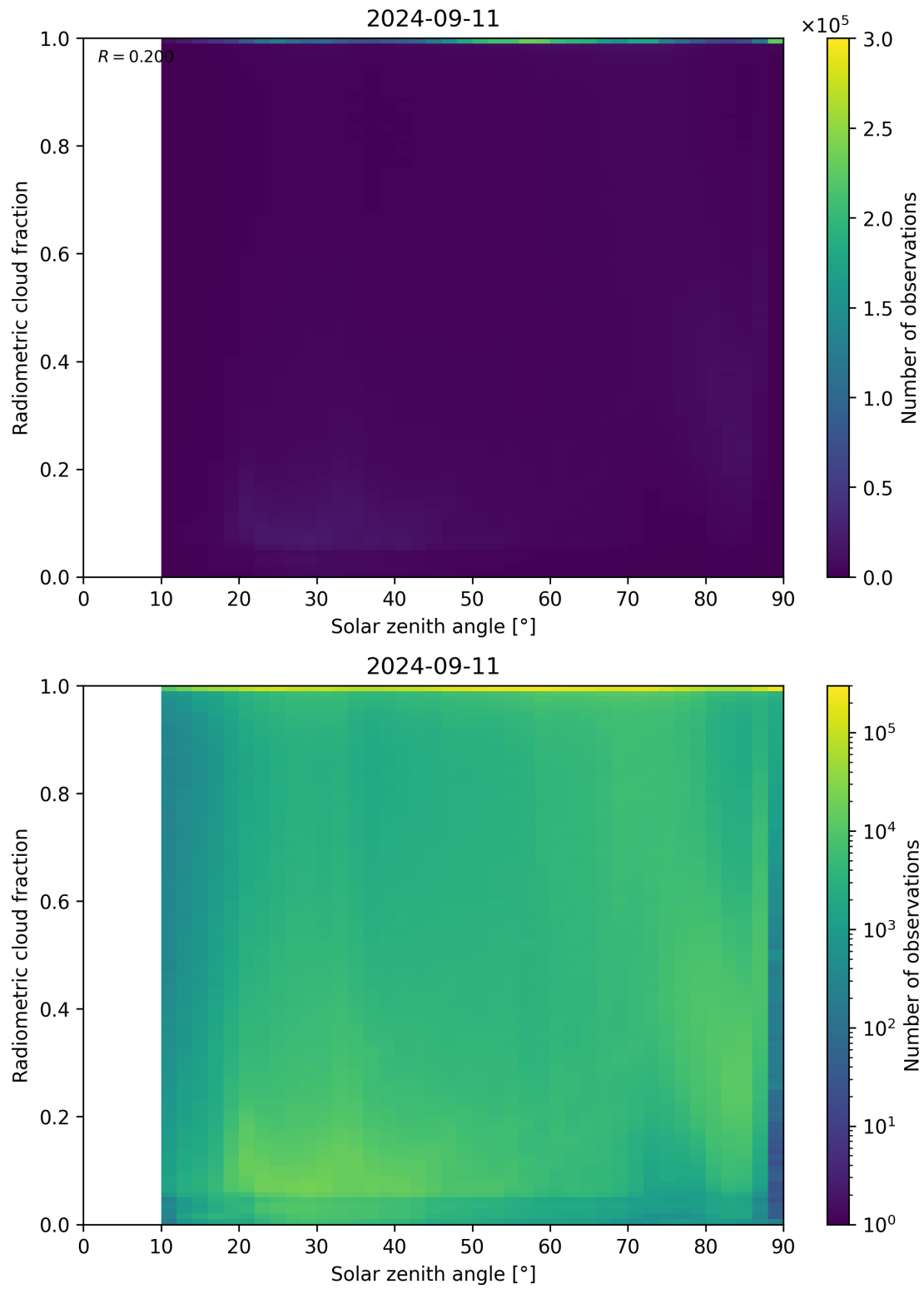
Figure 99: Scatter density plot of “Solar zenith angle” against “Radiometric cloud fraction” for 2024-09-10 to 2024-09-12.
