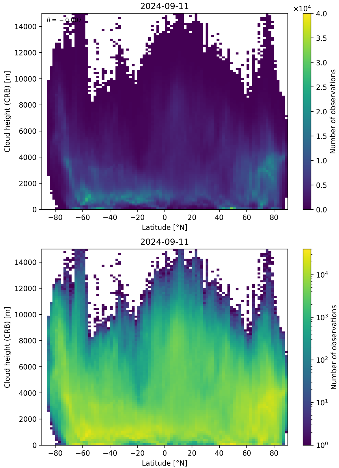
Figure 95: Scatter density plot of “Latitude” against “Cloud height (CRB)” for 2024-09-10 to 2024-09-12.
