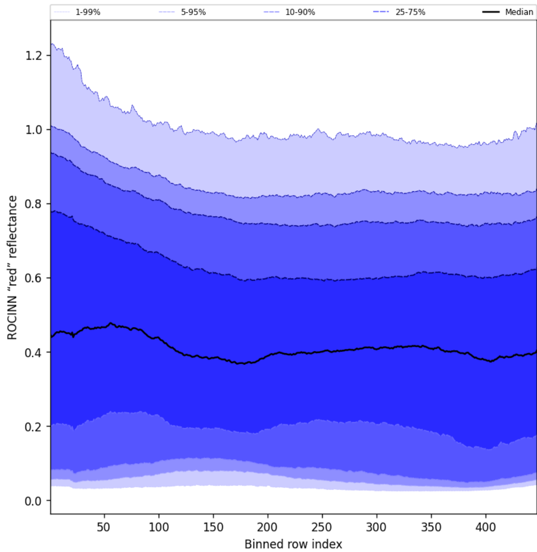
Figure 69: Along track statistics of “ROCINN “red” reflectance” for 2024-09-10 to 2024-09-12
