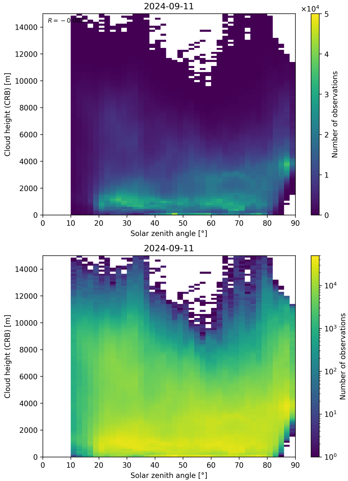
Figure 102: Scatter density plot of “Solar zenith angle” against “Cloud height (CRB)” for 2024-09-10 to 2024-09-12.
