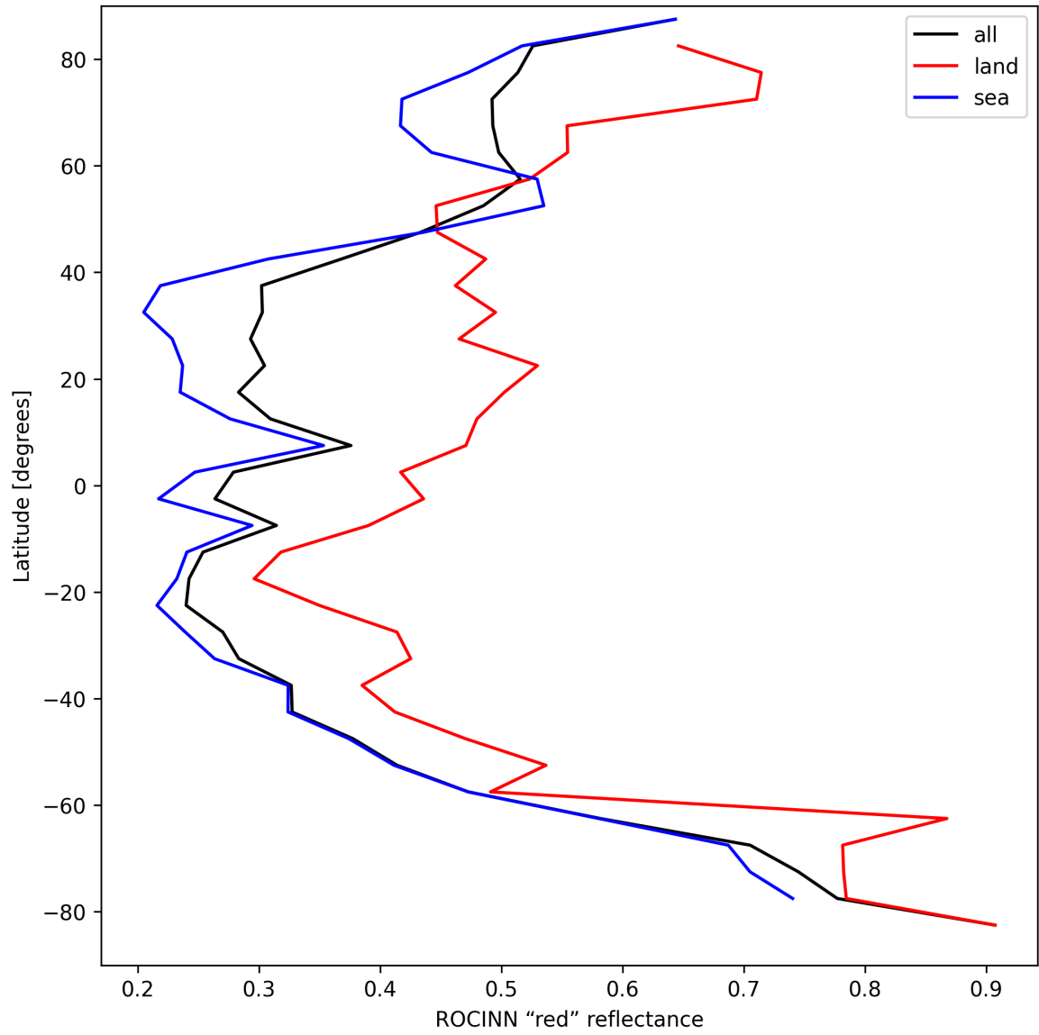
Figure 37: Zonal average of “ROCINN “red” reflectance” for 2024-09-10 to 2024-09-12.
