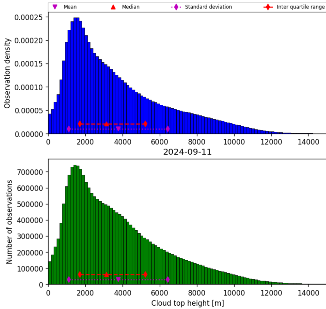
Figure 40: Histogram of “Cloud top height” for 2024-09-10 to 2024-09-12
