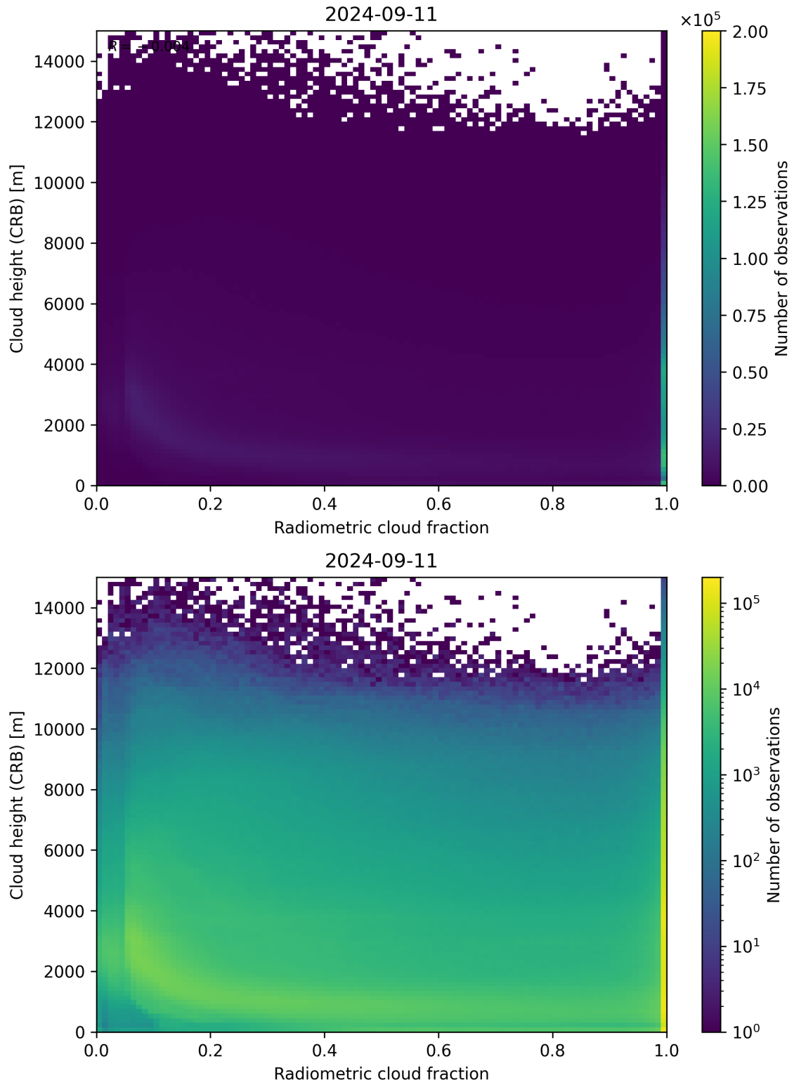
Figure 74: Scatter density plot of “Radiometric cloud fraction” against “Cloud height (CRB)” for 2024-09-10 to 2024-09-12.
