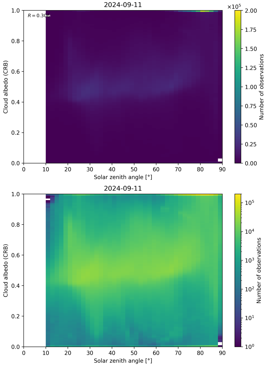
Figure 98: Scatter density plot of “Solar zenith angle” against “Cloud albedo (CRB)” for 2024-09-10 to 2024-09-12.
