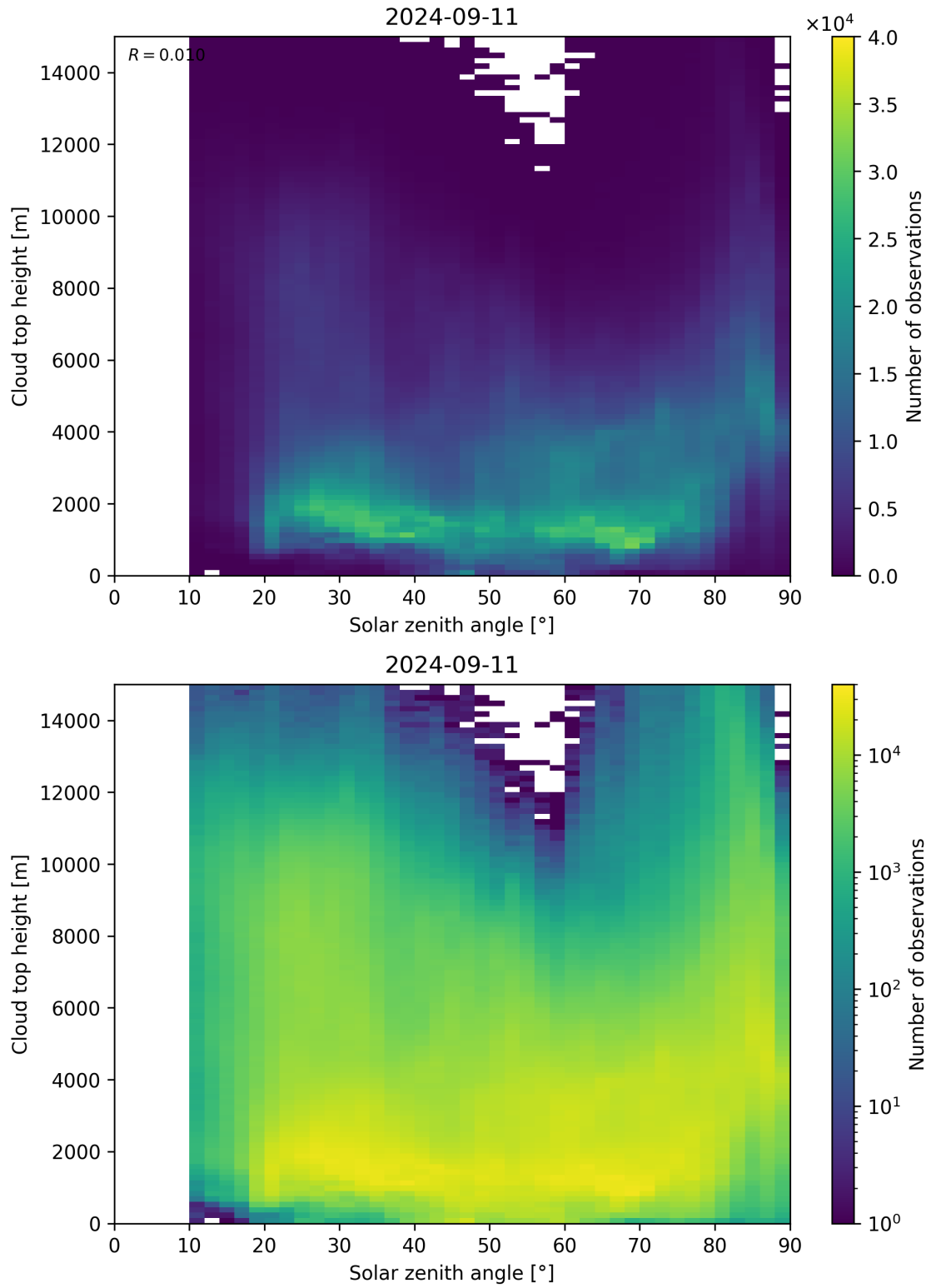
Figure 104: Scatter density plot of “Solar zenith angle” against “Cloud top height” for 2024-09-10 to 2024-09-12.
