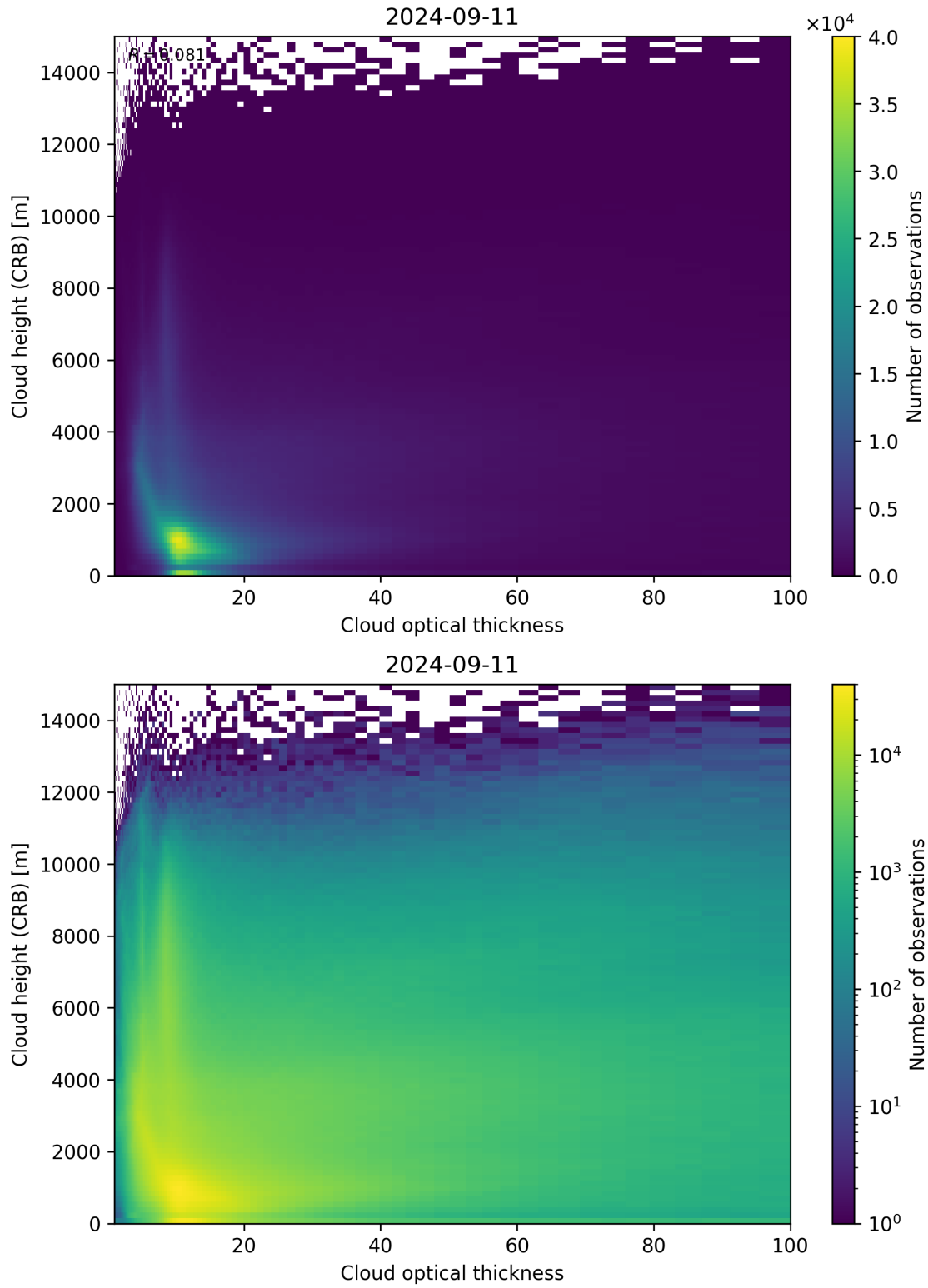
Figure 85: Scatter density plot of “Cloud optical thickness” against “Cloud height (CRB)” for 2024-09-10 to 2024-09-12.
