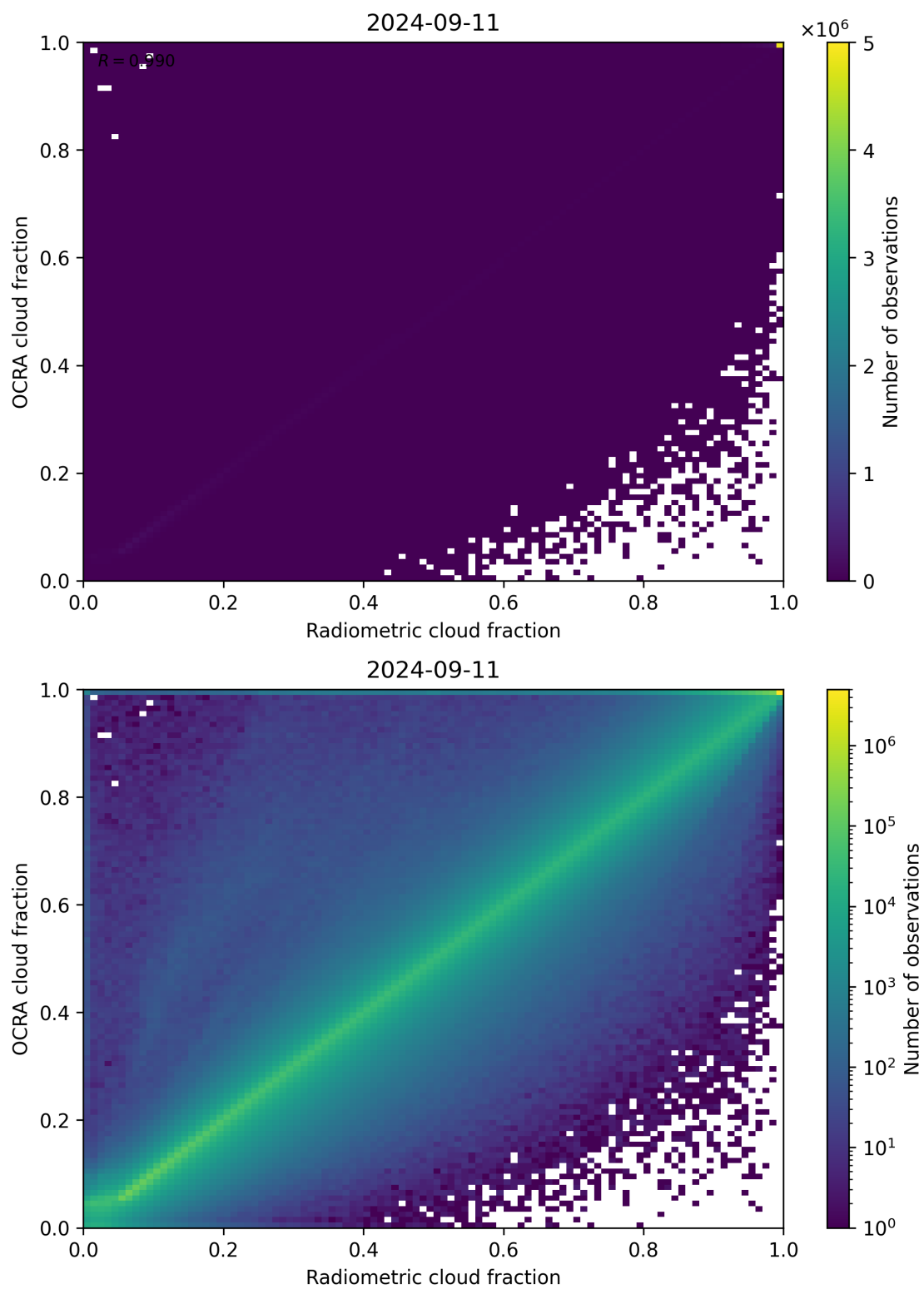
Figure 72: Scatter density plot of “Radiometric cloud fraction” against “OCRA cloud fraction” for 2024-09-10 to 2024-09-12.
