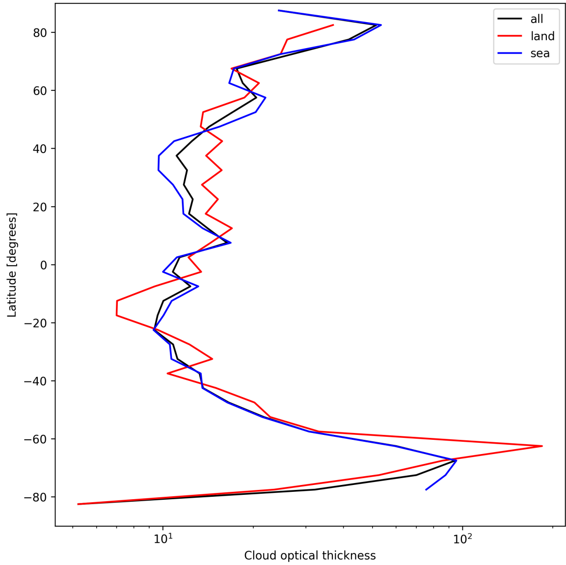
Figure 25: Zonal average of “Cloud optical thickness” for 2024-09-10 to 2024-09-12.
