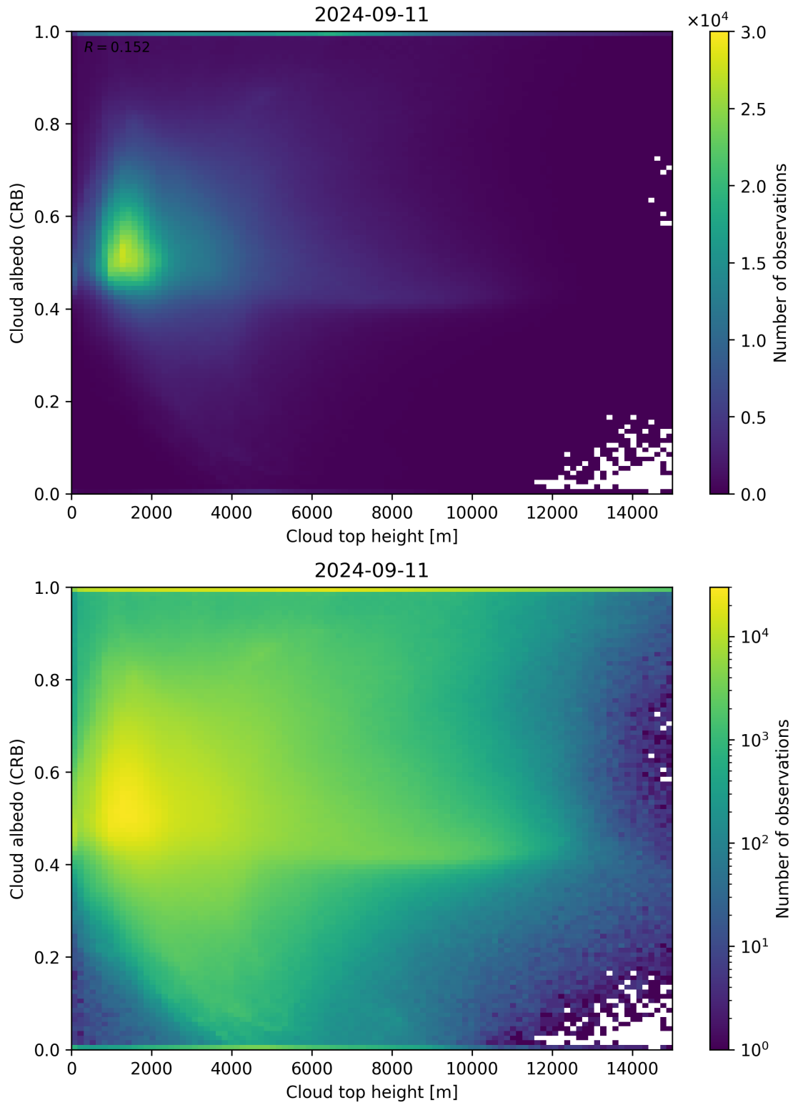
Figure 86: Scatter density plot of “Cloud top height” against “Cloud albedo (CRB)” for 2024-09-10 to 2024-09-12.
