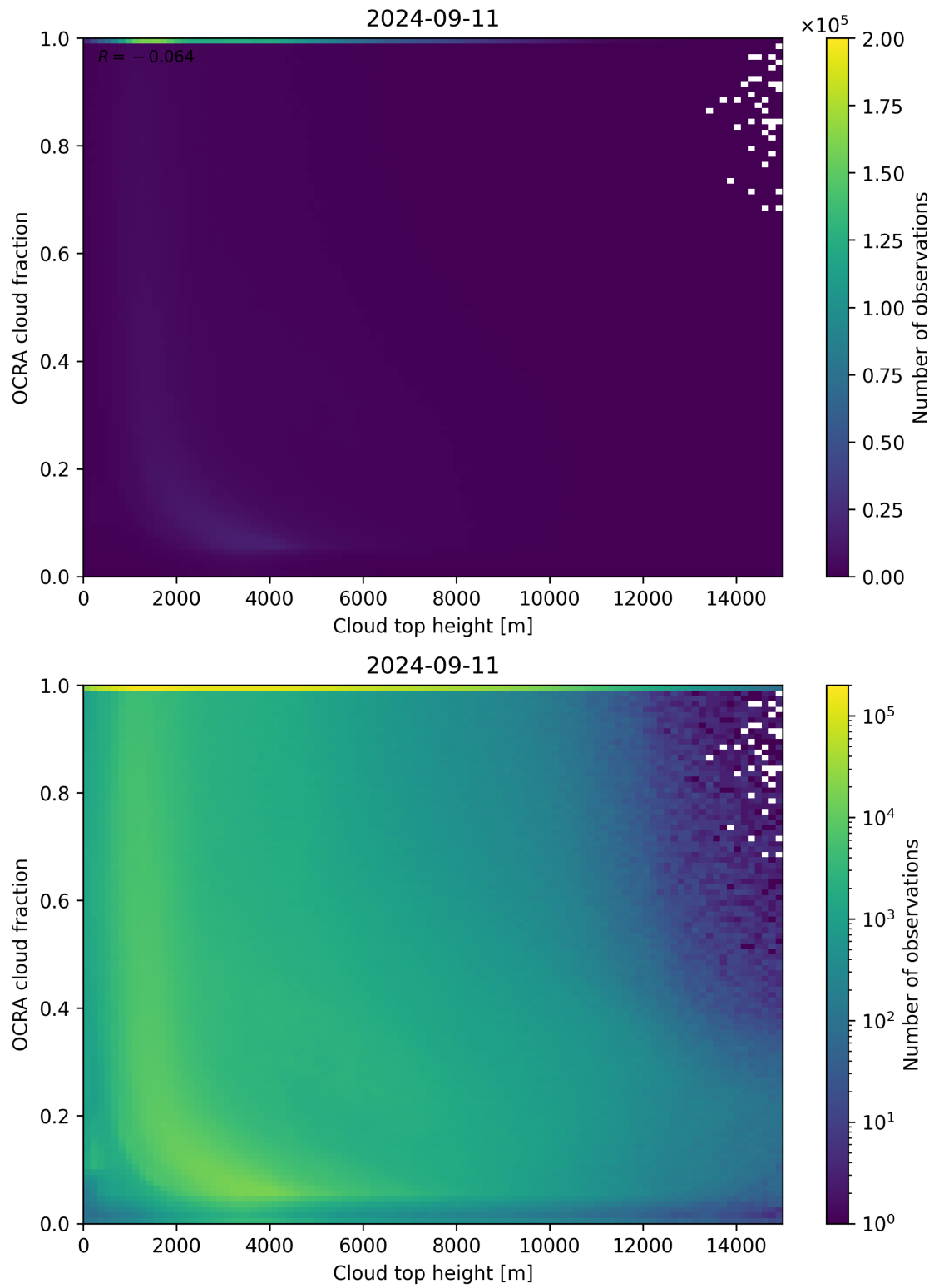
Figure 87: Scatter density plot of “Cloud top height” against “OCRA cloud fraction” for 2024-09-10 to 2024-09-12.
