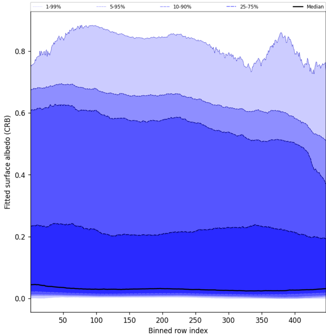
Figure 62: Along track statistics of “Fitted surface albedo (CRB)” for 2024-09-10 to 2024-09-12
