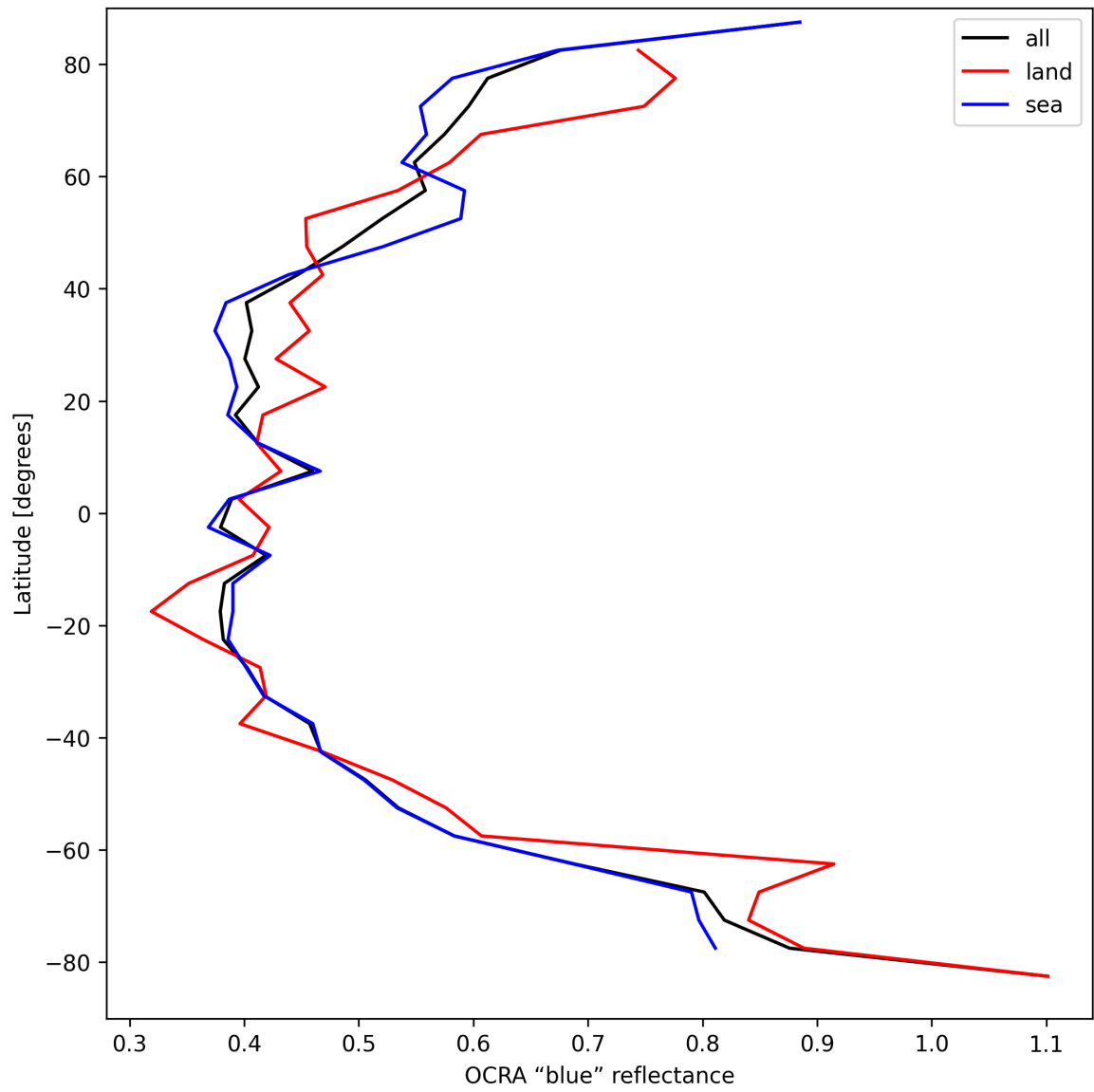
Figure 35: Zonal average of “OCRA “blue” reflectance” for 2024-09-10 to 2024-09-12.
