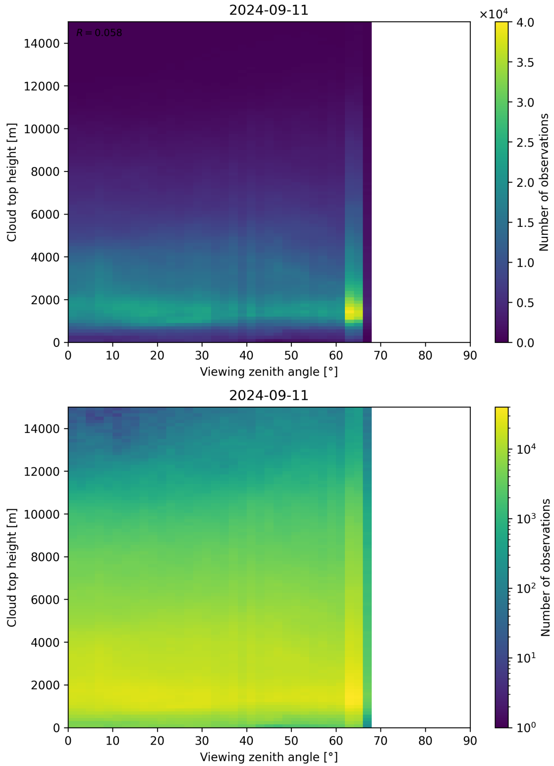
Figure 112: Scatter density plot of “Viewing zenith angle” against “Cloud top height” for 2024-09-10 to 2024-09-12.
