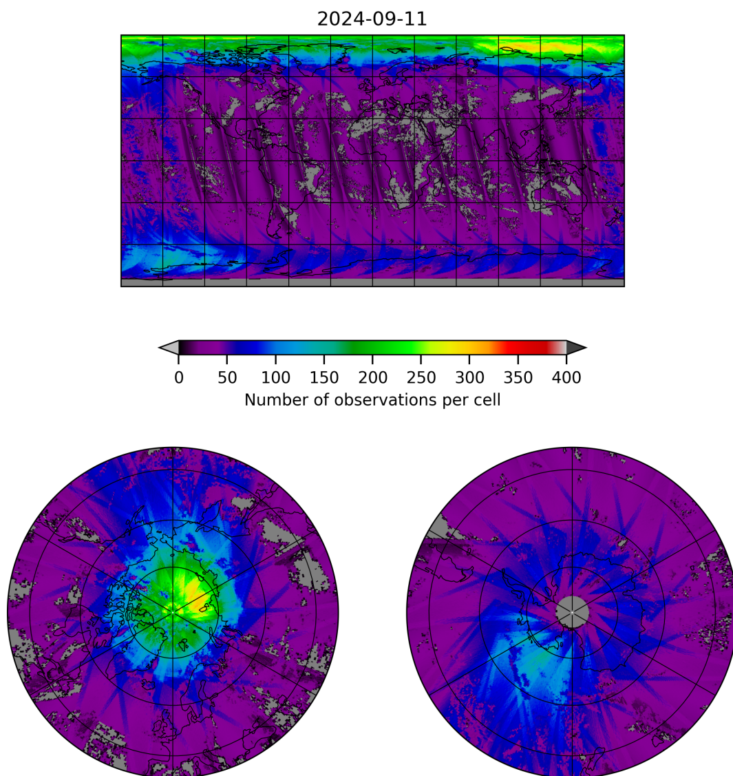
Figure 21: Map of the number of observations for 2024-09-10 to 2024-09-12
