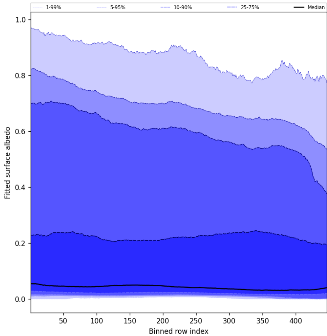
Figure 61: Along track statistics of “Fitted surface albedo” for 2024-09-10 to 2024-09-12
