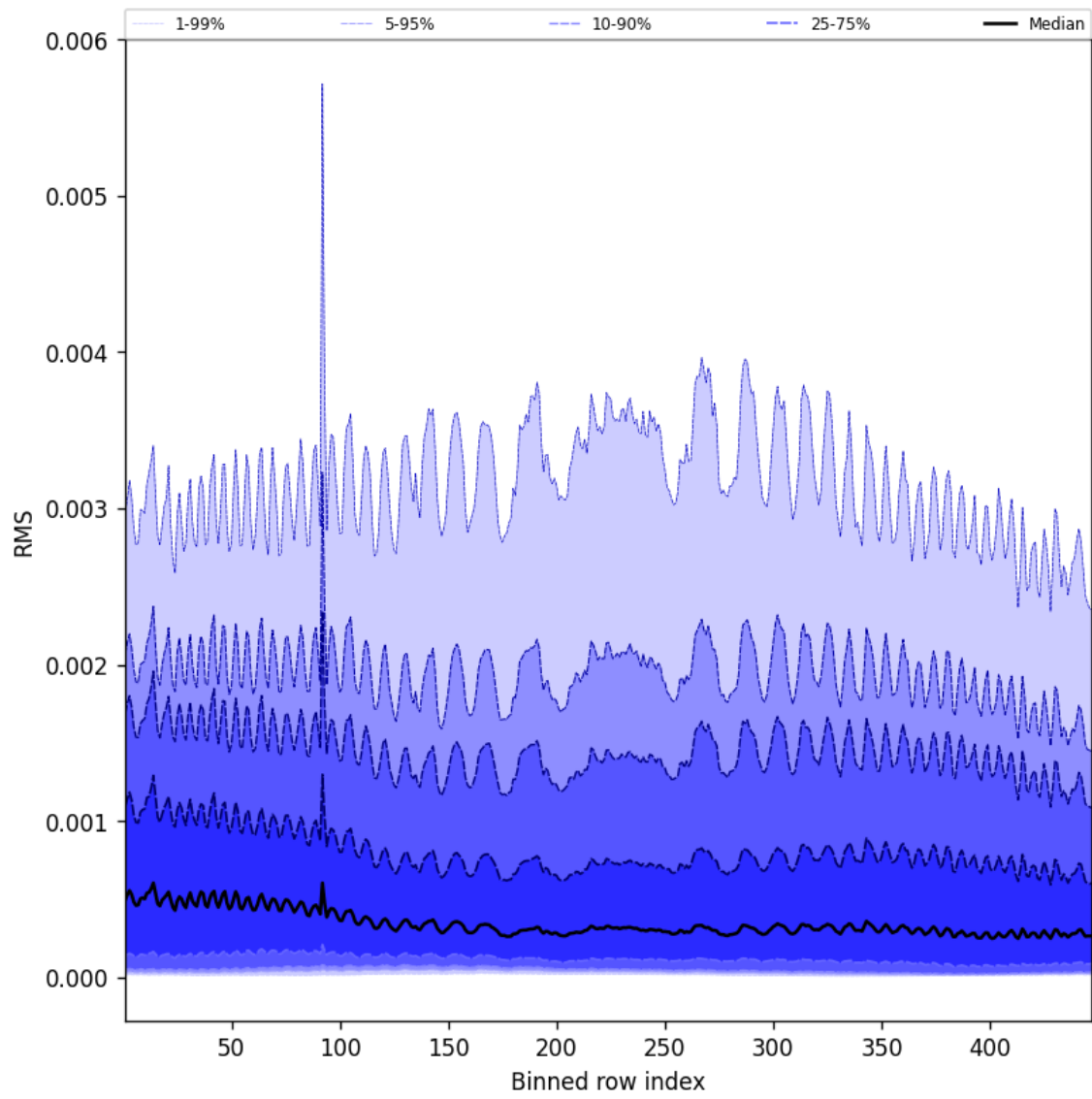
Figure 63: Along track statistics of “RMS” for 2024-09-10 to 2024-09-12
