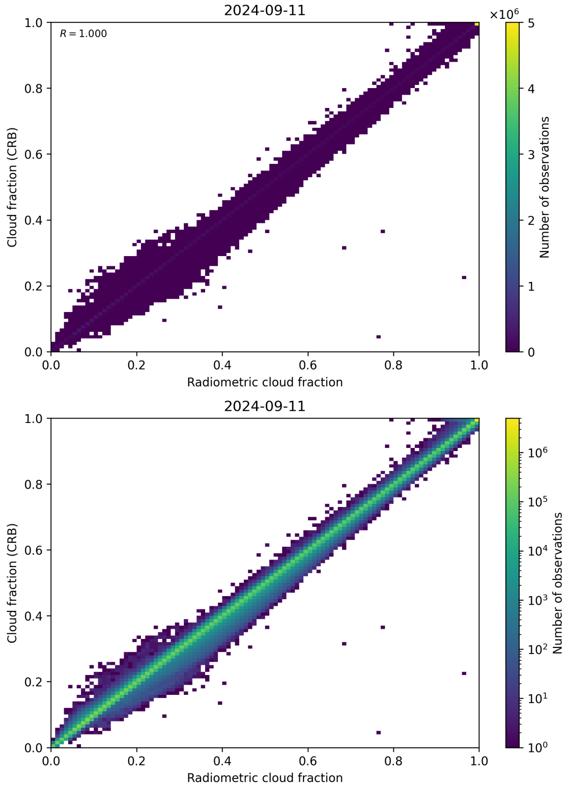
Figure 73: Scatter density plot of “Radiometric cloud fraction” against “Cloud fraction (CRB)” for 2024-09-10 to 2024-09-12.
