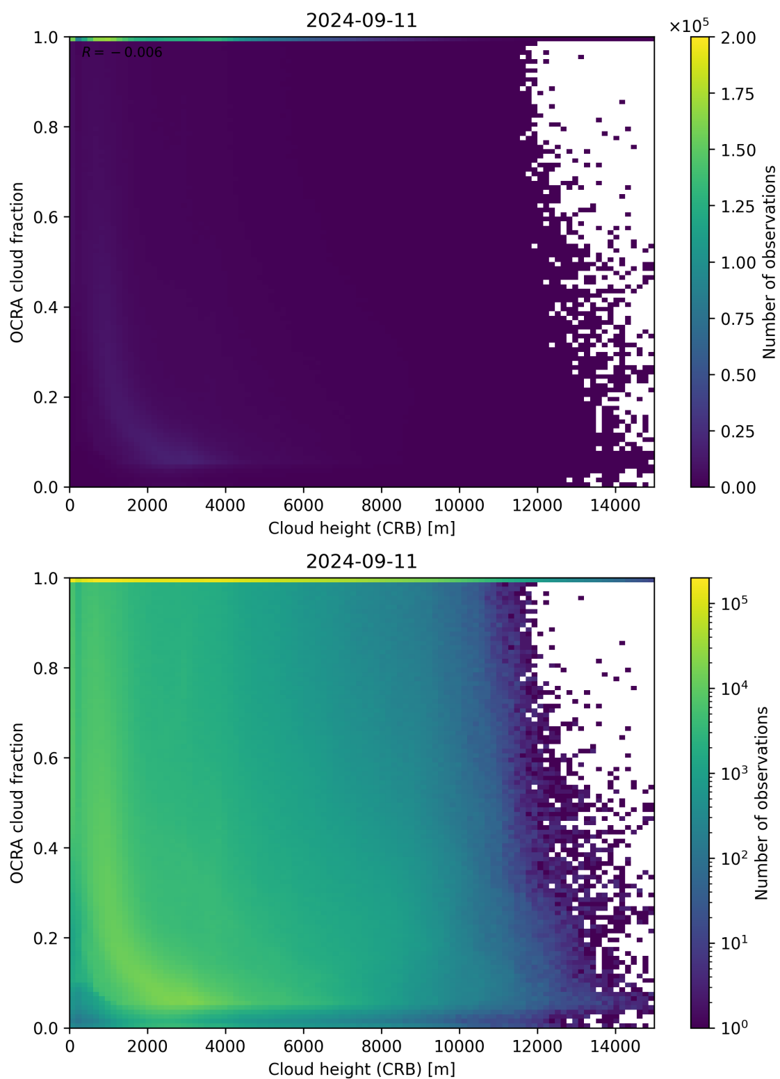
Figure 81: Scatter density plot of “Cloud height (CRB)” against “OCRA cloud fraction” for 2024-09-10 to 2024-09-12.
