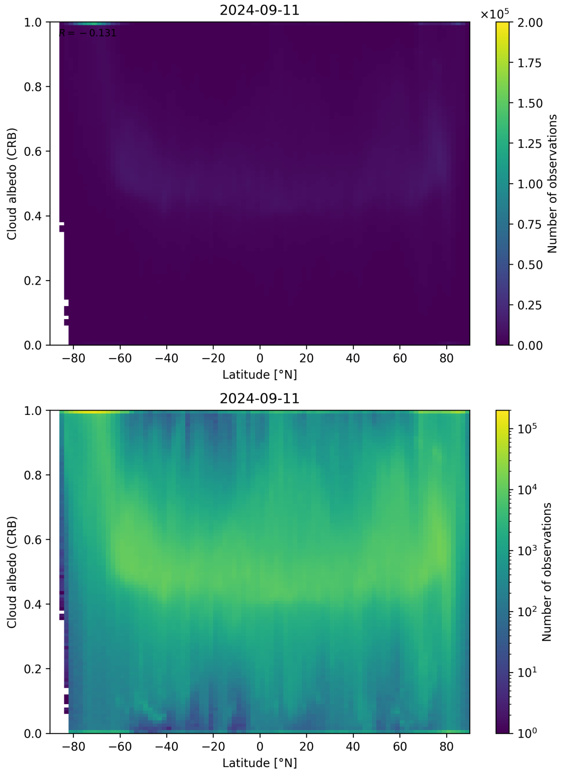
Figure 91: Scatter density plot of “Latitude” against “Cloud albedo (CRB)” for 2024-09-10 to 2024-09-12.
