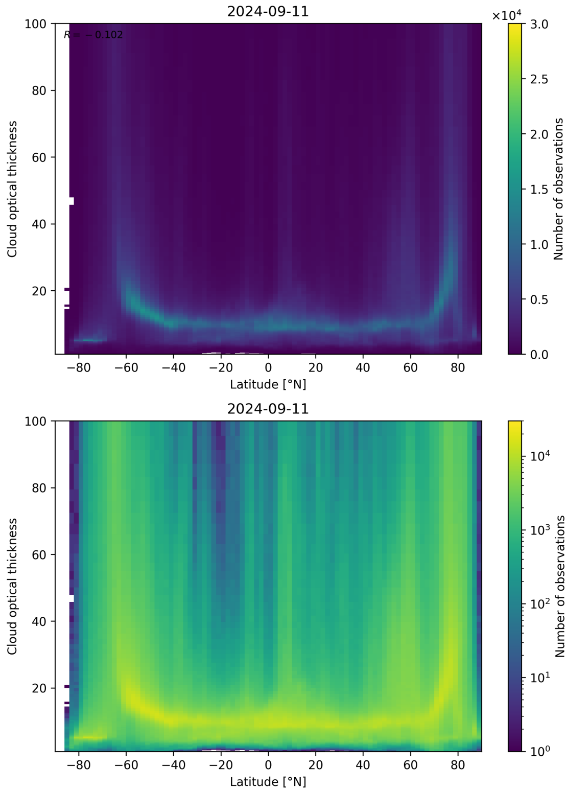
Figure 96: Scatter density plot of “Latitude” against “Cloud optical thickness” for 2024-09-10 to 2024-09-12.
