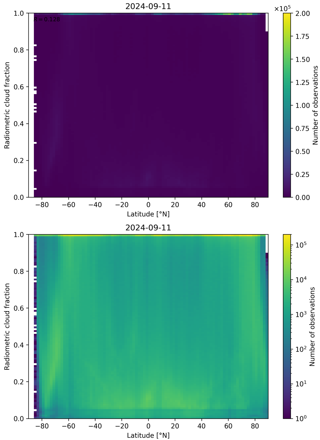
Figure 92: Scatter density plot of “Latitude” against “Radiometric cloud fraction” for 2024-09-10 to 2024-09-12.
