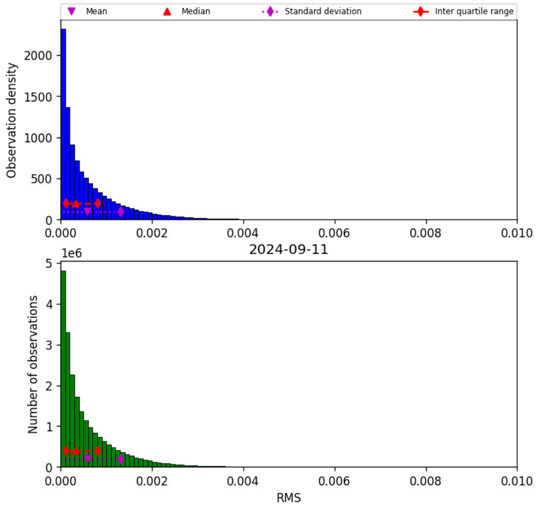
Figure 47: Histogram of “RMS” for 2024-09-10 to 2024-09-12
