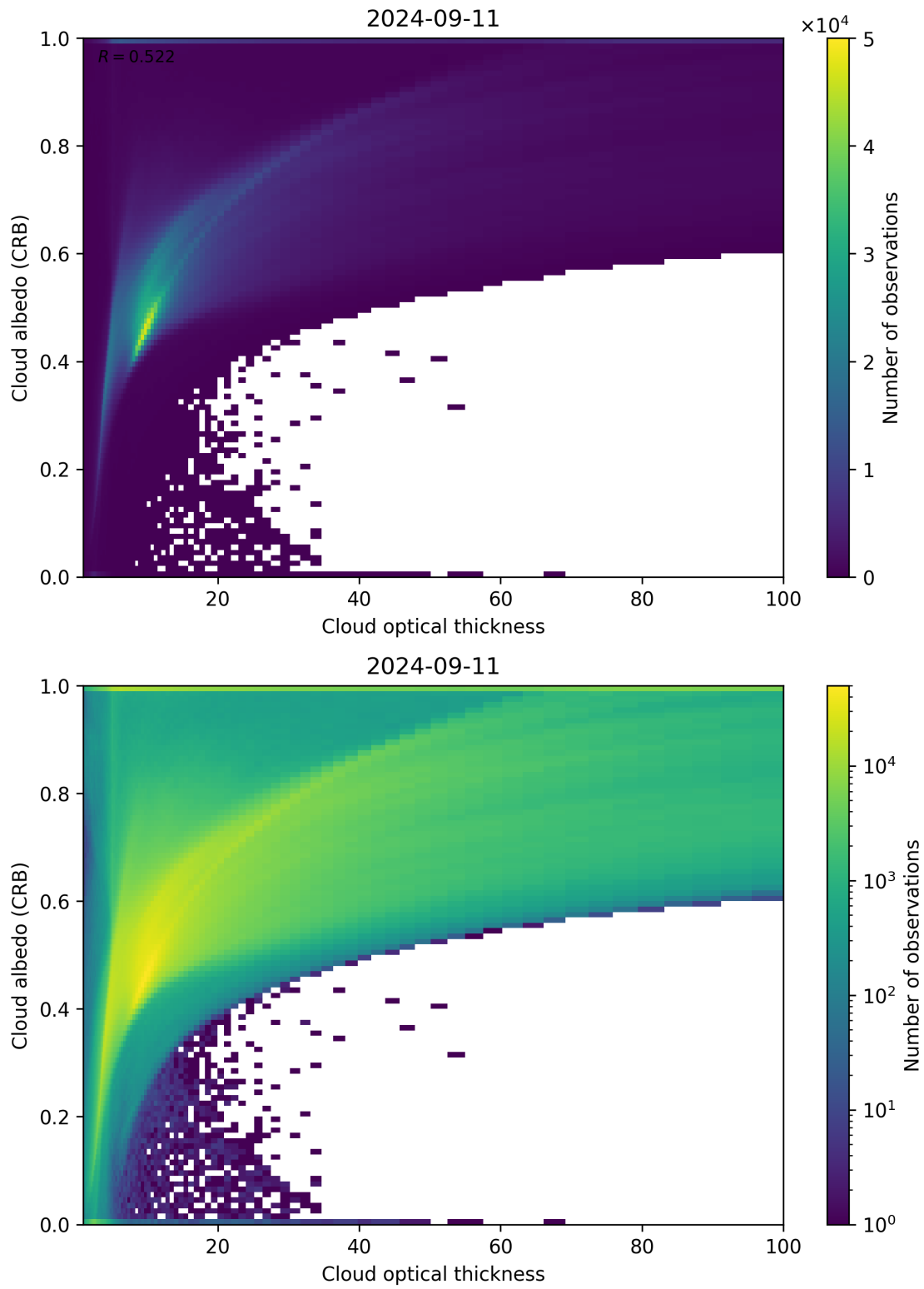
Figure 82: Scatter density plot of “Cloud optical thickness” against “Cloud albedo (CRB)” for 2024-09-10 to 2024-09-12.
