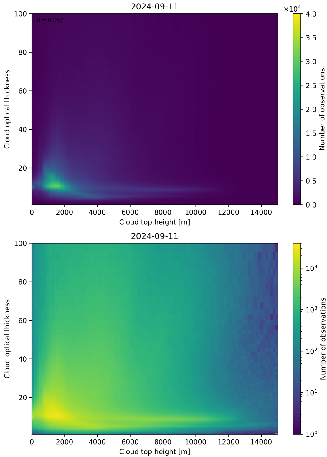
Figure 90: Scatter density plot of “Cloud top height” against “Cloud optical thickness” for 2024-09-10 to 2024-09-12.
