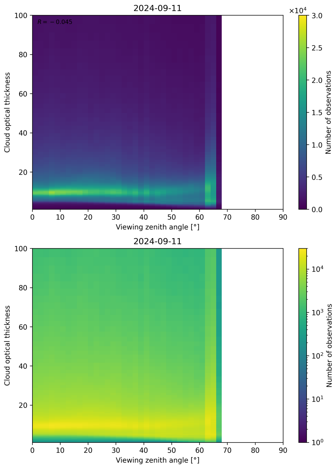
Figure 111: Scatter density plot of “Viewing zenith angle” against “Cloud optical thickness” for 2024-09-10 to 2024-09-12.
