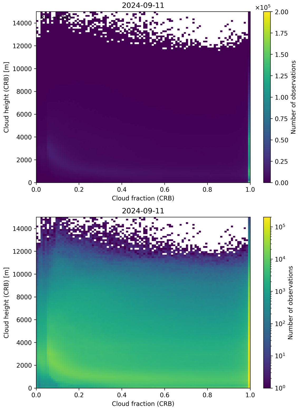
Figure 79: Scatter density plot of “Cloud fraction (CRB)” against “Cloud height (CRB)” for 2024-09-10 to 2024-09-12.
