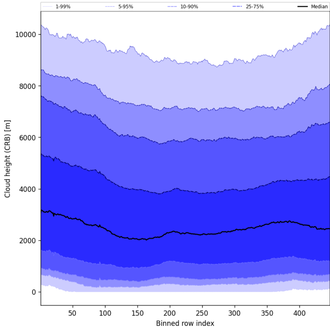
Figure 59: Along track statistics of “Cloud height (CRB)” for 2024-09-10 to 2024-09-12
