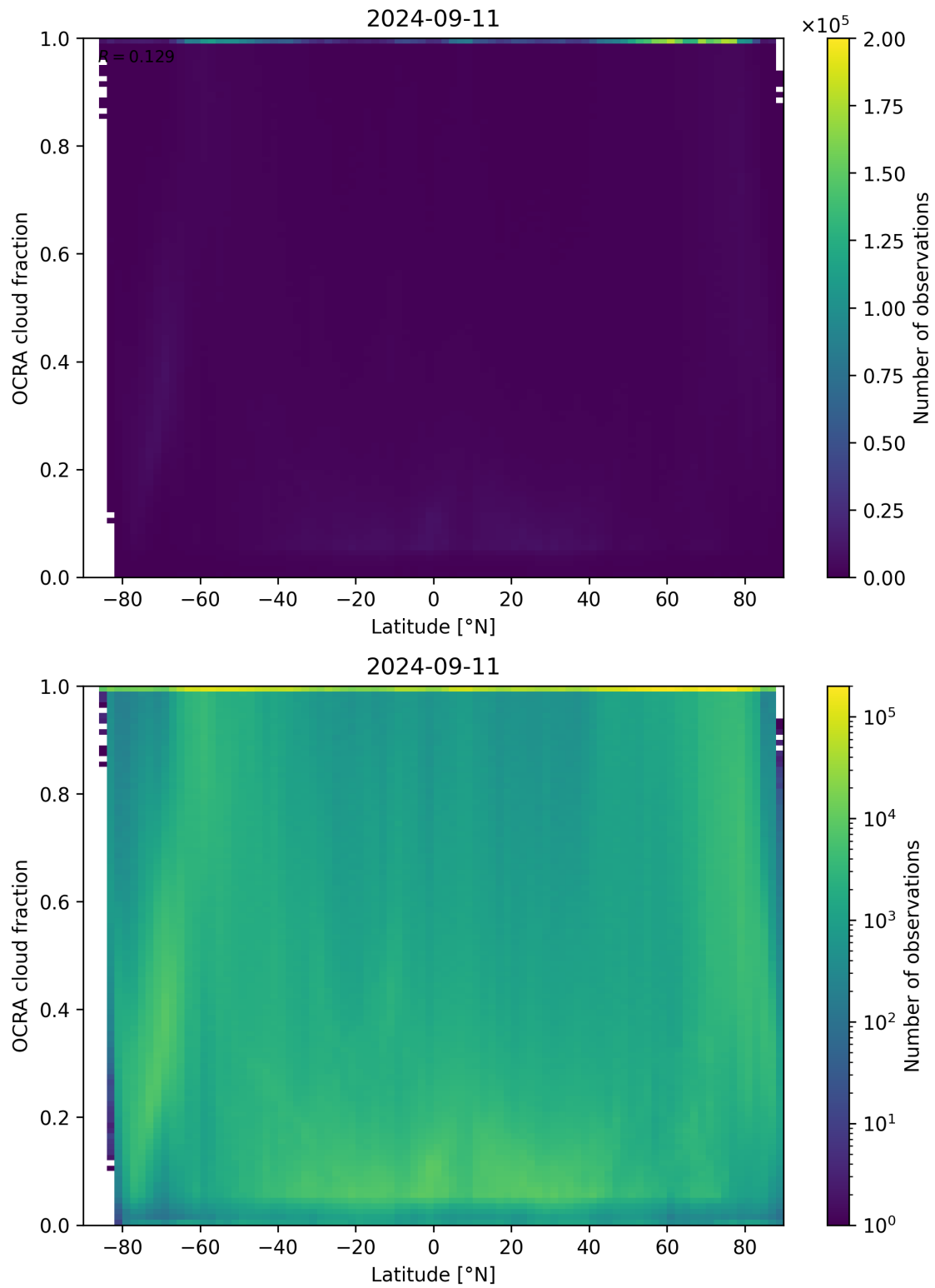
Figure 93: Scatter density plot of “Latitude” against “OCRA cloud fraction” for 2024-09-10 to 2024-09-12.
