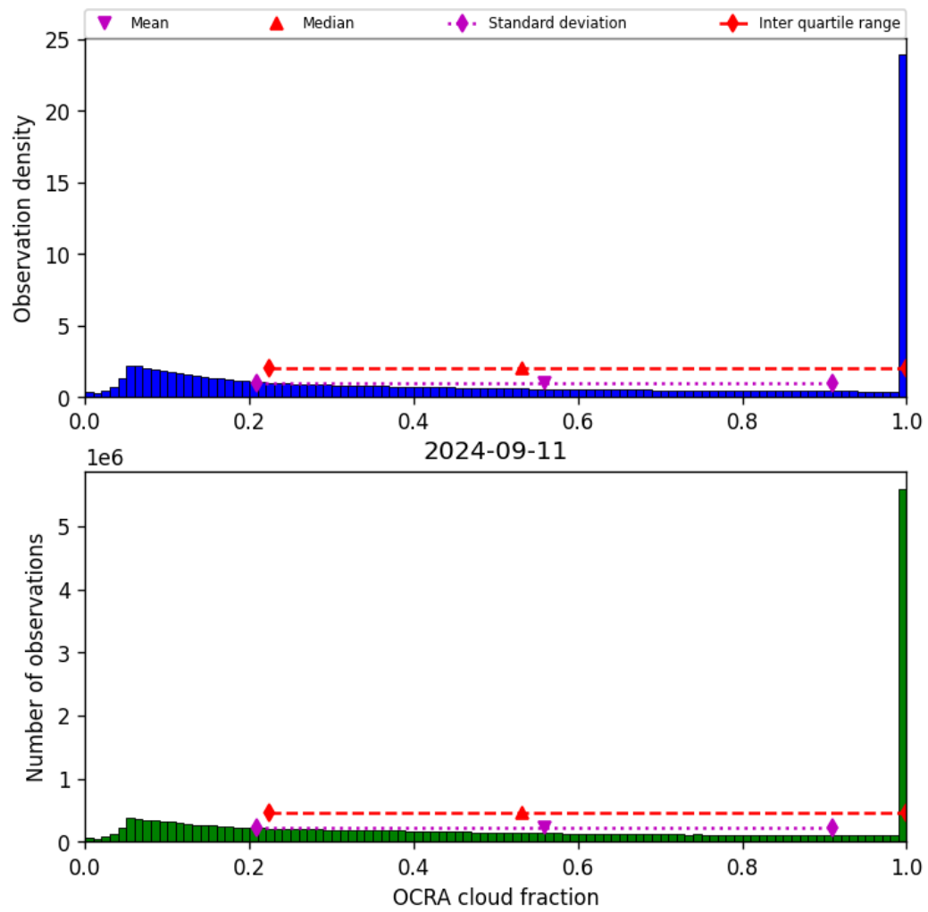
Figure 50: Histogram of “OCRA cloud fraction” for 2024-09-10 to 2024-09-12
