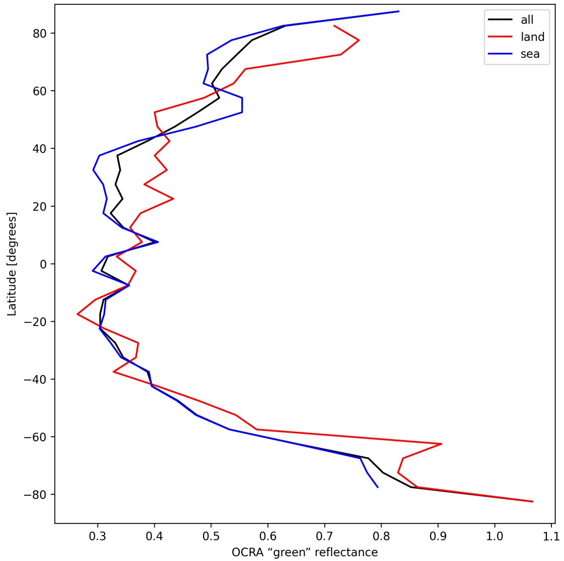
Figure 36: Zonal average of “OCRA “green” reflectance” for 2024-09-10 to 2024-09-12.
