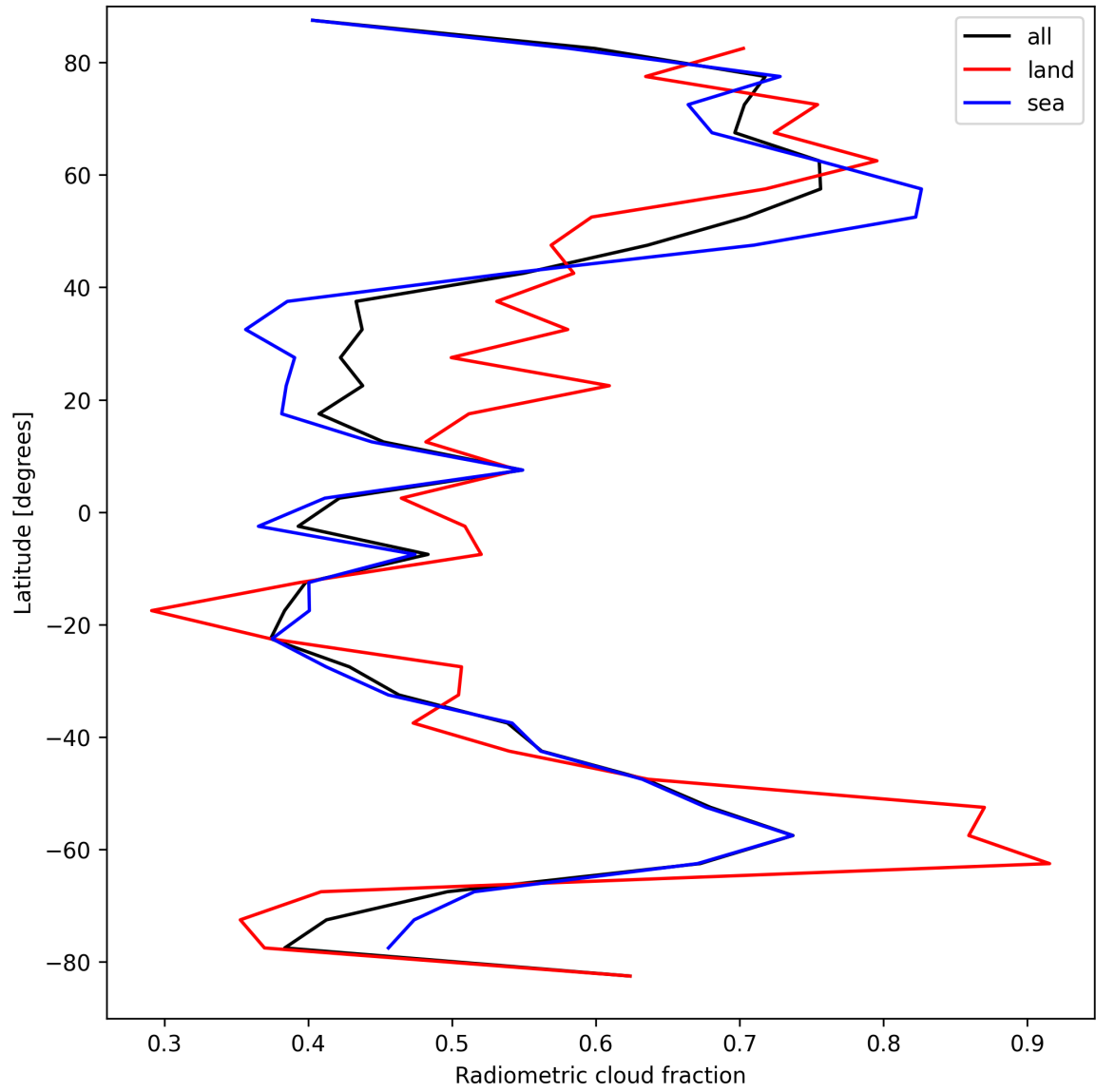
Figure 23: Zonal average of “Radiometric cloud fraction” for 2024-09-10 to 2024-09-12.
