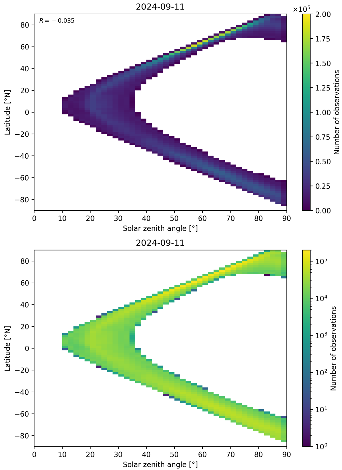
Figure 105: Scatter density plot of “Solar zenith angle” against “Latitude” for 2024-09-10 to 2024-09-12.
