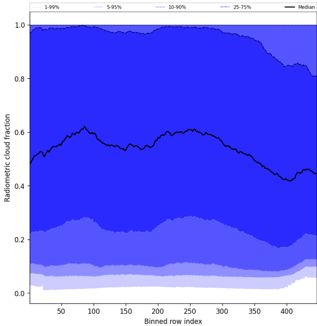
Figure 55: Along track statistics of “Radiometric cloud fraction” for 2024-09-10 to 2024-09-12
