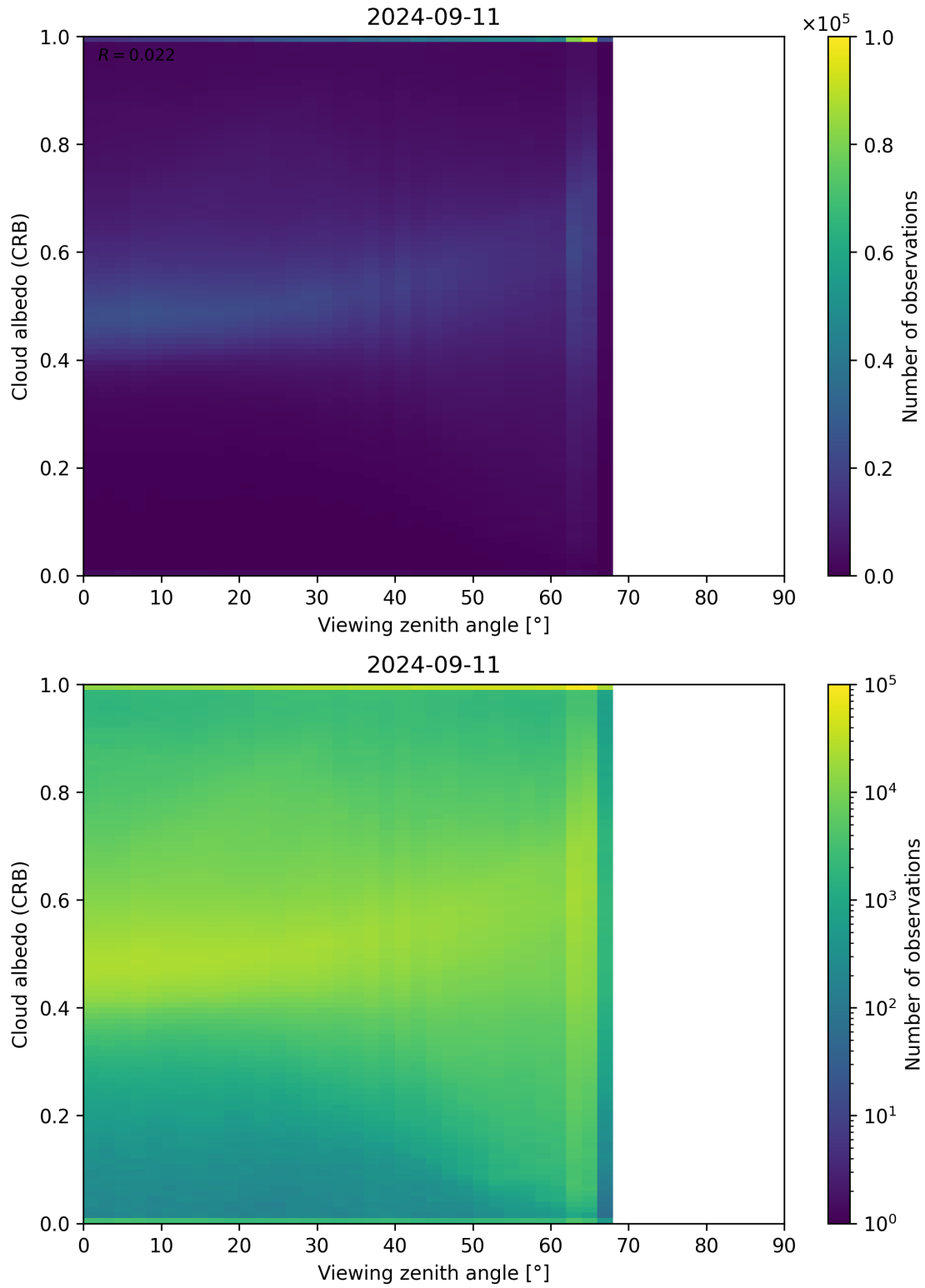
Figure 106: Scatter density plot of “Viewing zenith angle” against “Cloud albedo (CRB)” for 2024-09-10 to 2024-09-12.
