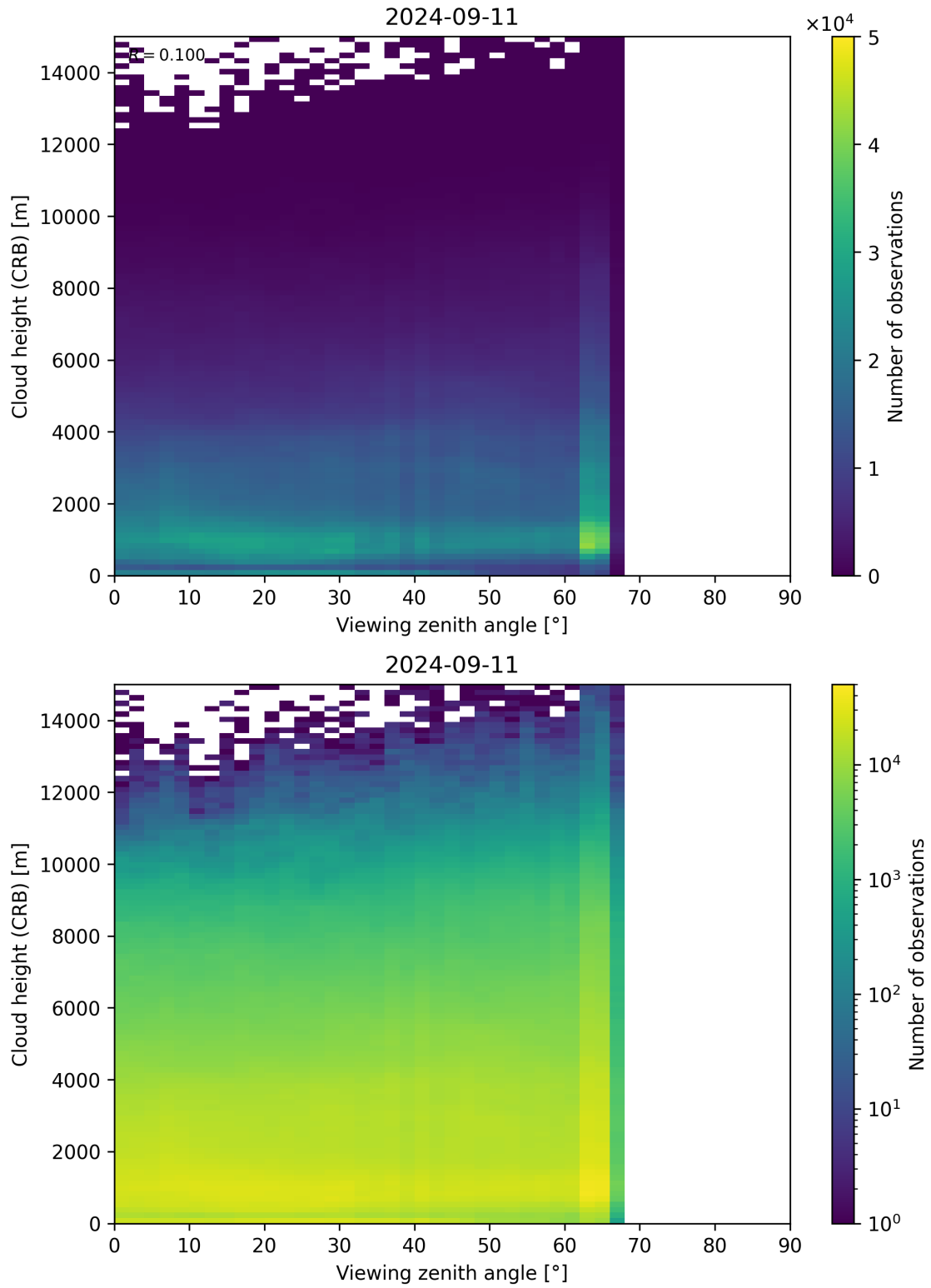
Figure 110: Scatter density plot of “Viewing zenith angle” against “Cloud height (CRB)” for 2024-09-10 to 2024-09-12.
