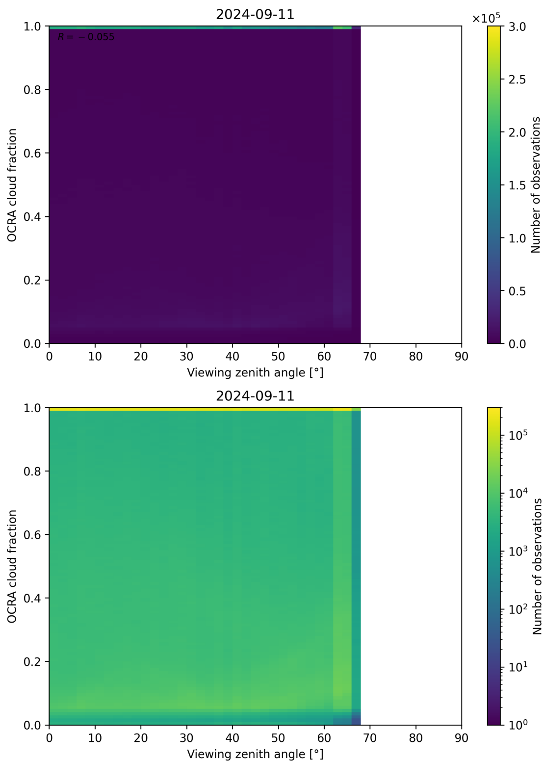
Figure 108: Scatter density plot of “Viewing zenith angle” against “OCRA cloud fraction” for 2024-09-10 to 2024-09-12.
