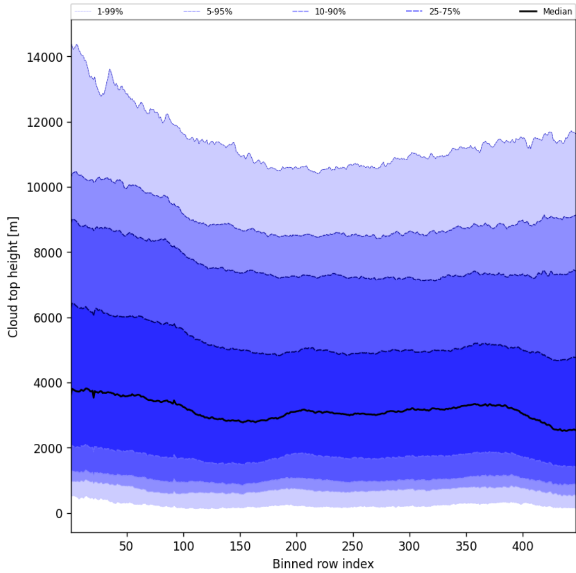
Figure 56: Along track statistics of “Cloud top height” for 2024-09-10 to 2024-09-12
