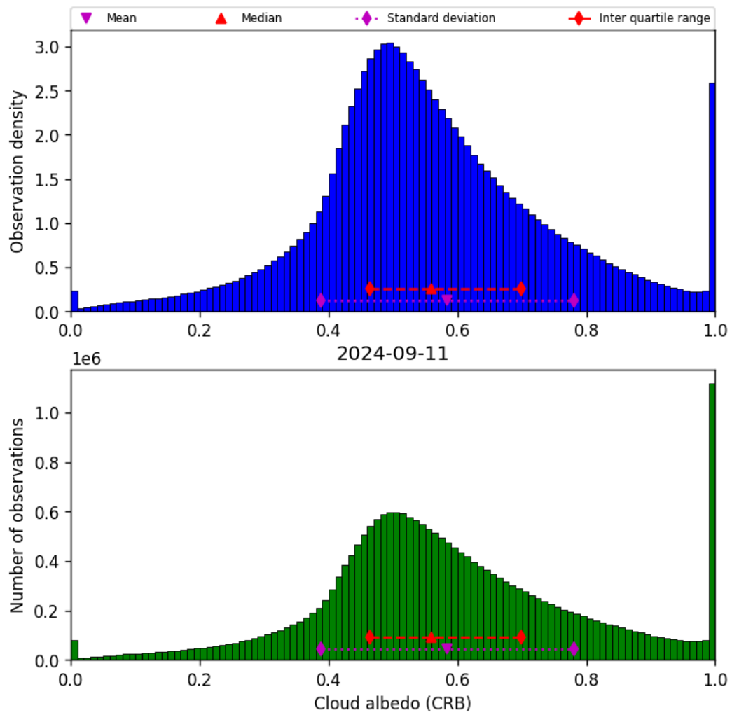
Figure 44: Histogram of “Cloud albedo (CRB)” for 2024-09-10 to 2024-09-12
