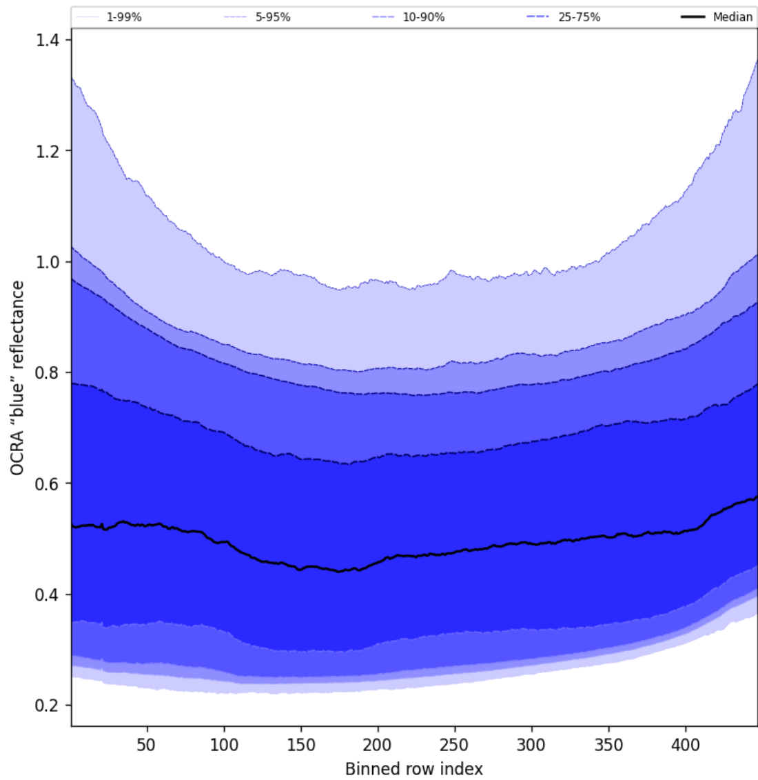
Figure 67: Along track statistics of “OCRA “blue” reflectance” for 2024-09-10 to 2024-09-12
