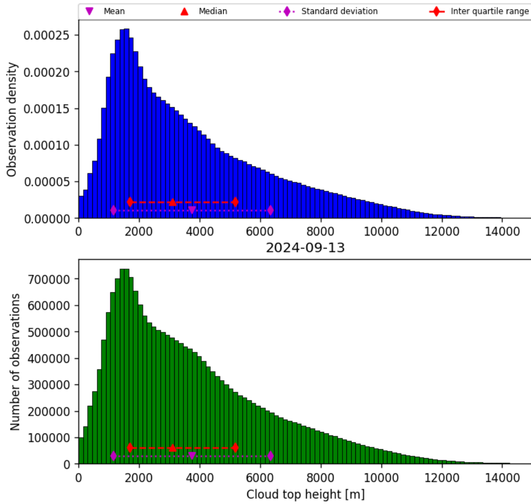
Figure 40: Histogram of “Cloud top height” for 2024-09-12 to 2024-09-14
