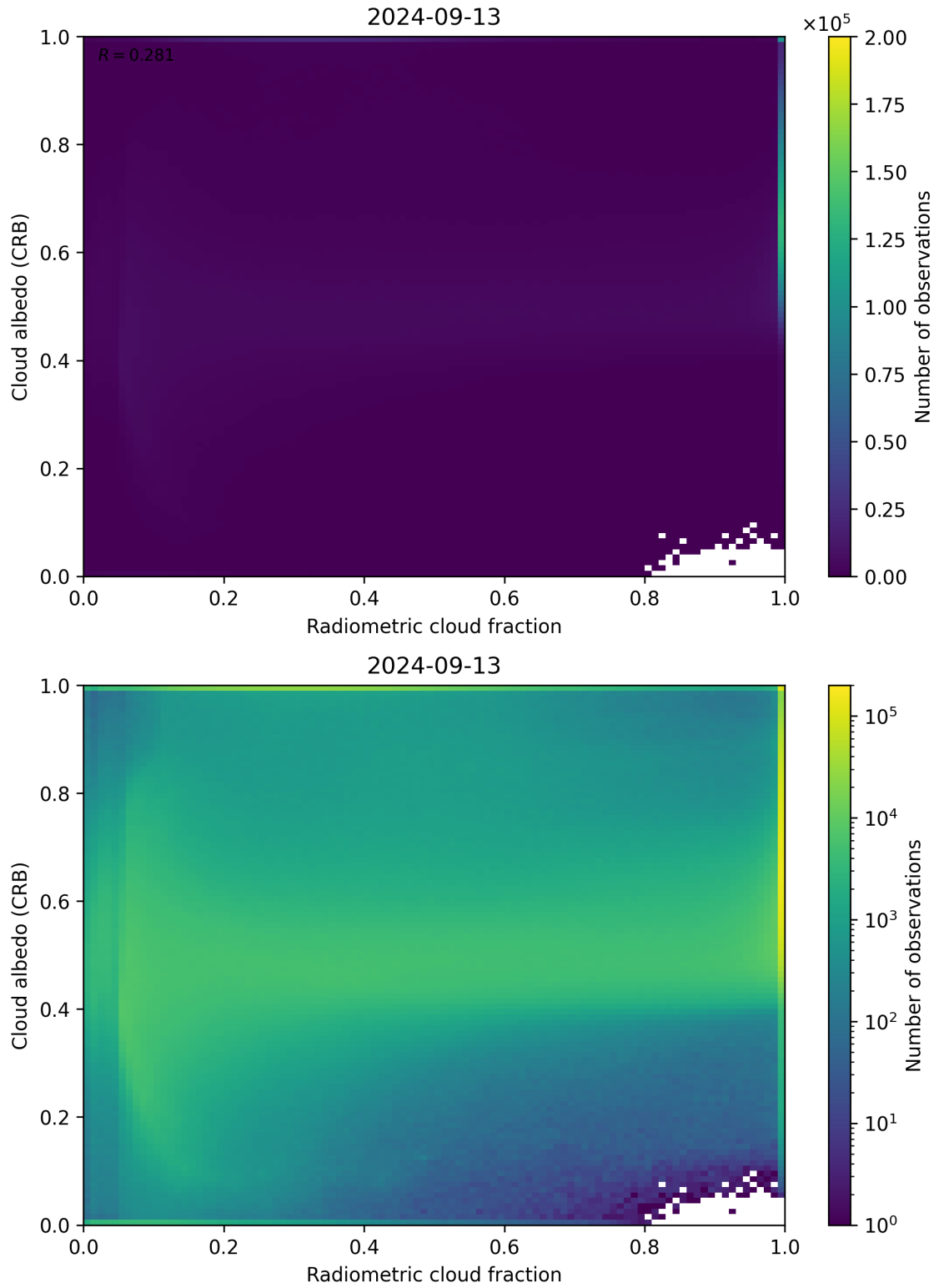
Figure 71: Scatter density plot of “Radiometric cloud fraction” against “Cloud albedo (CRB)” for 2024-09-12 to 2024-09-14.
