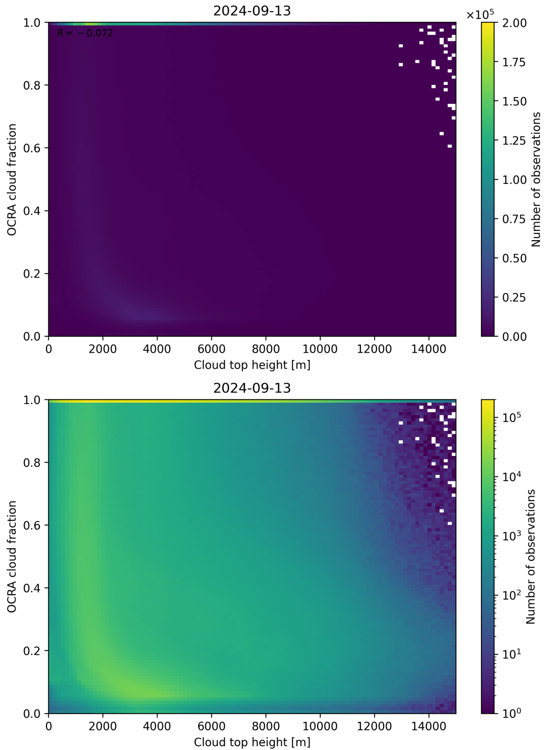
Figure 87: Scatter density plot of “Cloud top height” against “OCRA cloud fraction” for 2024-09-12 to 2024-09-14.
