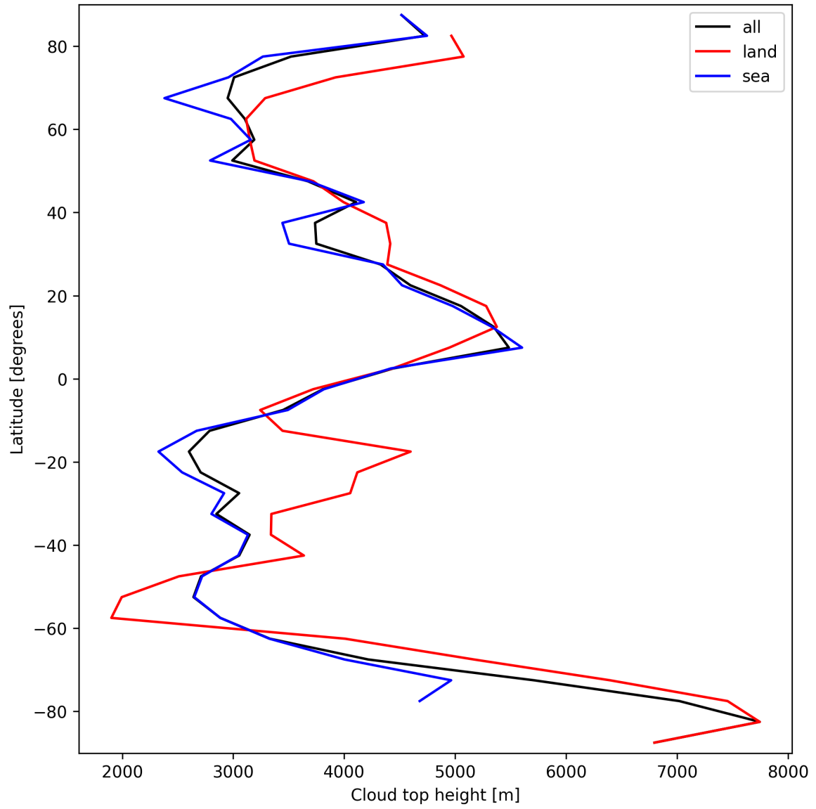
Figure 24: Zonal average of “Cloud top height” for 2024-09-12 to 2024-09-14.
