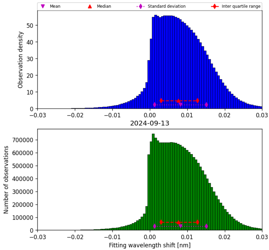
Figure 49: Histogram of “Fitting wavelength shift” for 2024-09-12 to 2024-09-14
