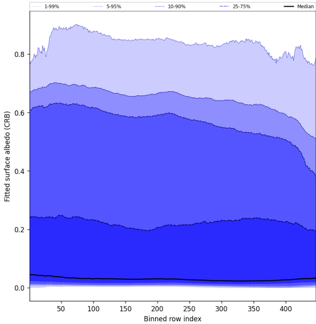
Figure 62: Along track statistics of “Fitted surface albedo (CRB)” for 2024-09-12 to 2024-09-14
