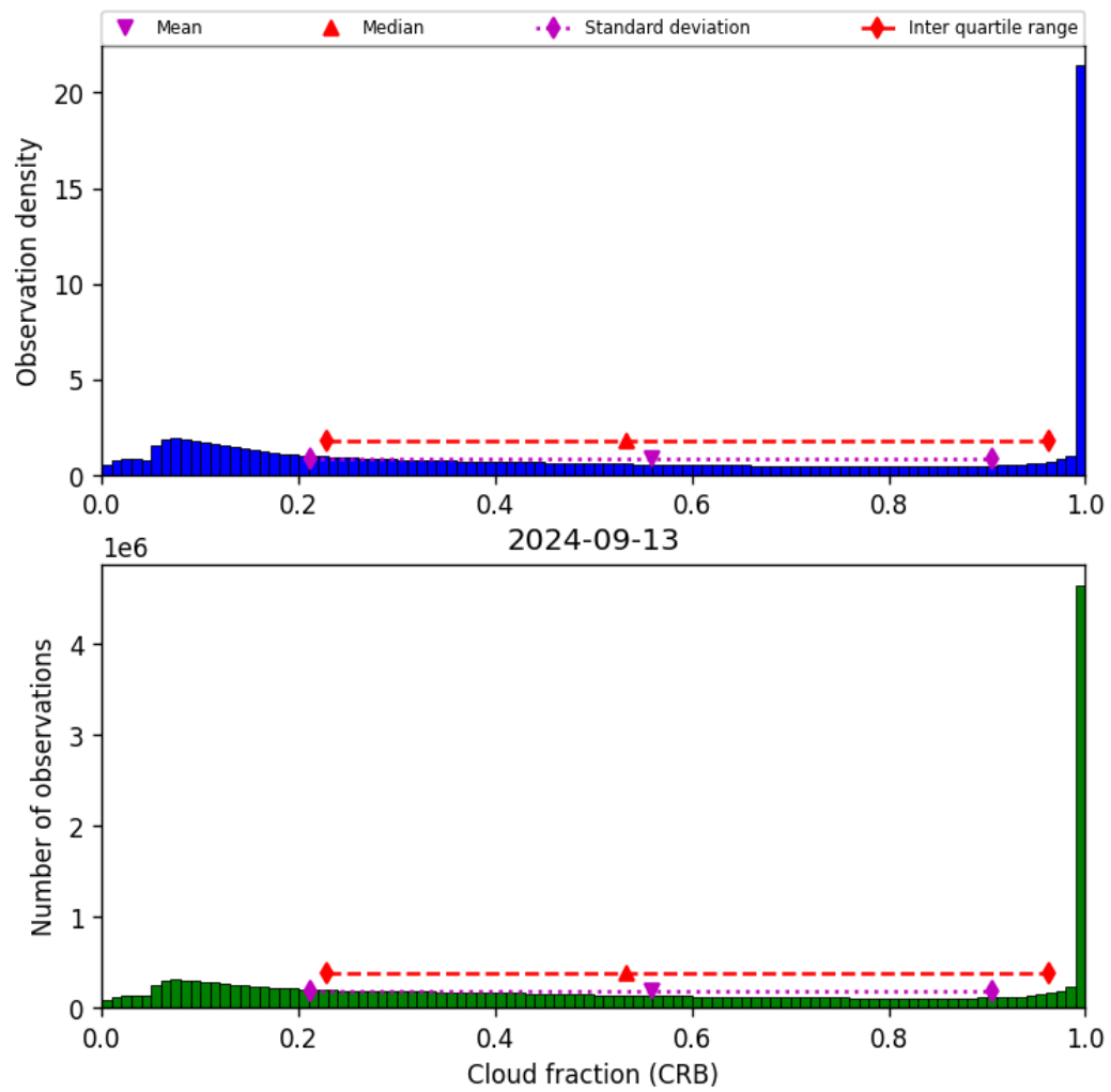
Figure 42: Histogram of “Cloud fraction (CRB)” for 2024-09-12 to 2024-09-14
