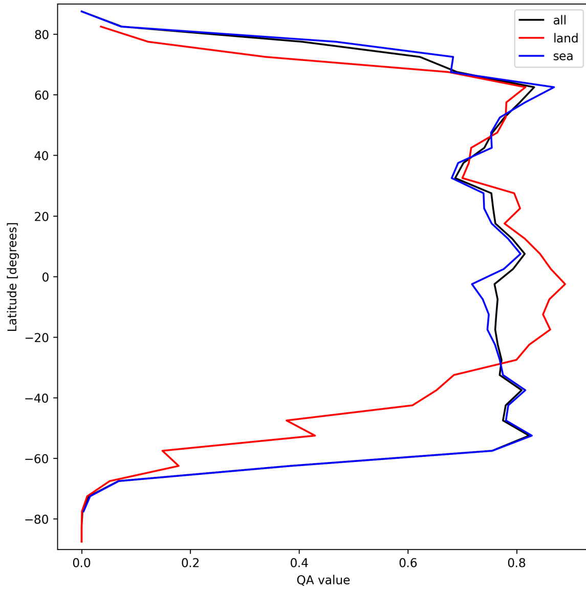
Figure 22: Zonal average of “QA value” for 2024-09-12 to 2024-09-14.
