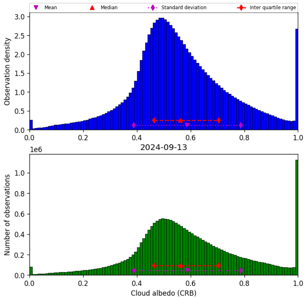
Figure 44: Histogram of “Cloud albedo (CRB)” for 2024-09-12 to 2024-09-14
