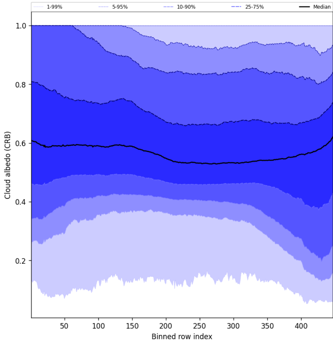
Figure 60: Along track statistics of “Cloud albedo (CRB)” for 2024-09-12 to 2024-09-14
