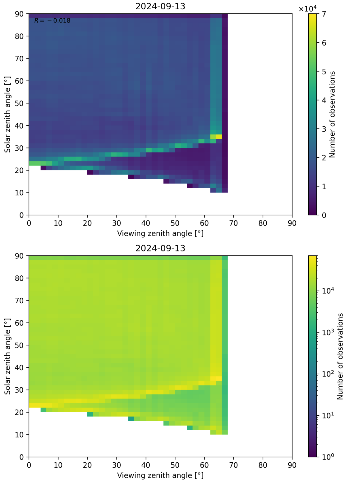
Figure 114: Scatter density plot of “Viewing zenith angle” against “Solar zenith angle” for 2024-09-12 to 2024-09-14.
