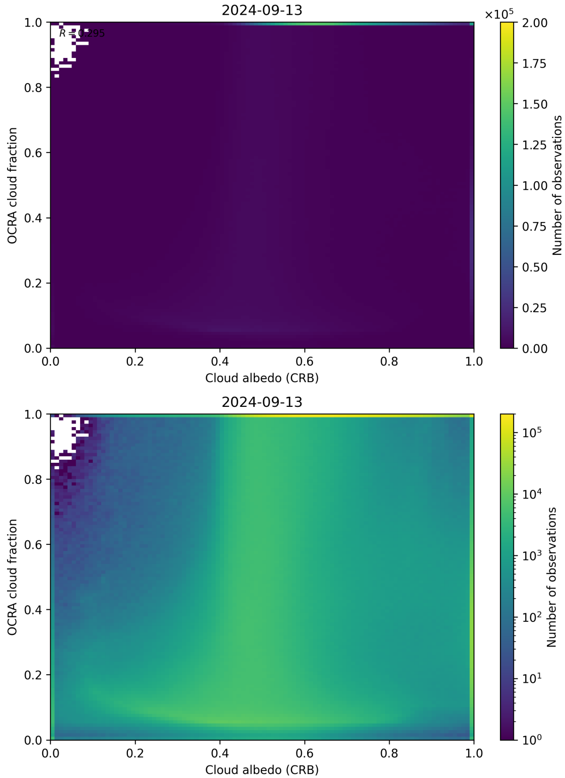
Figure 70: Scatter density plot of “Cloud albedo (CRB)” against “OCRA cloud fraction” for 2024-09-12 to 2024-09-14.
