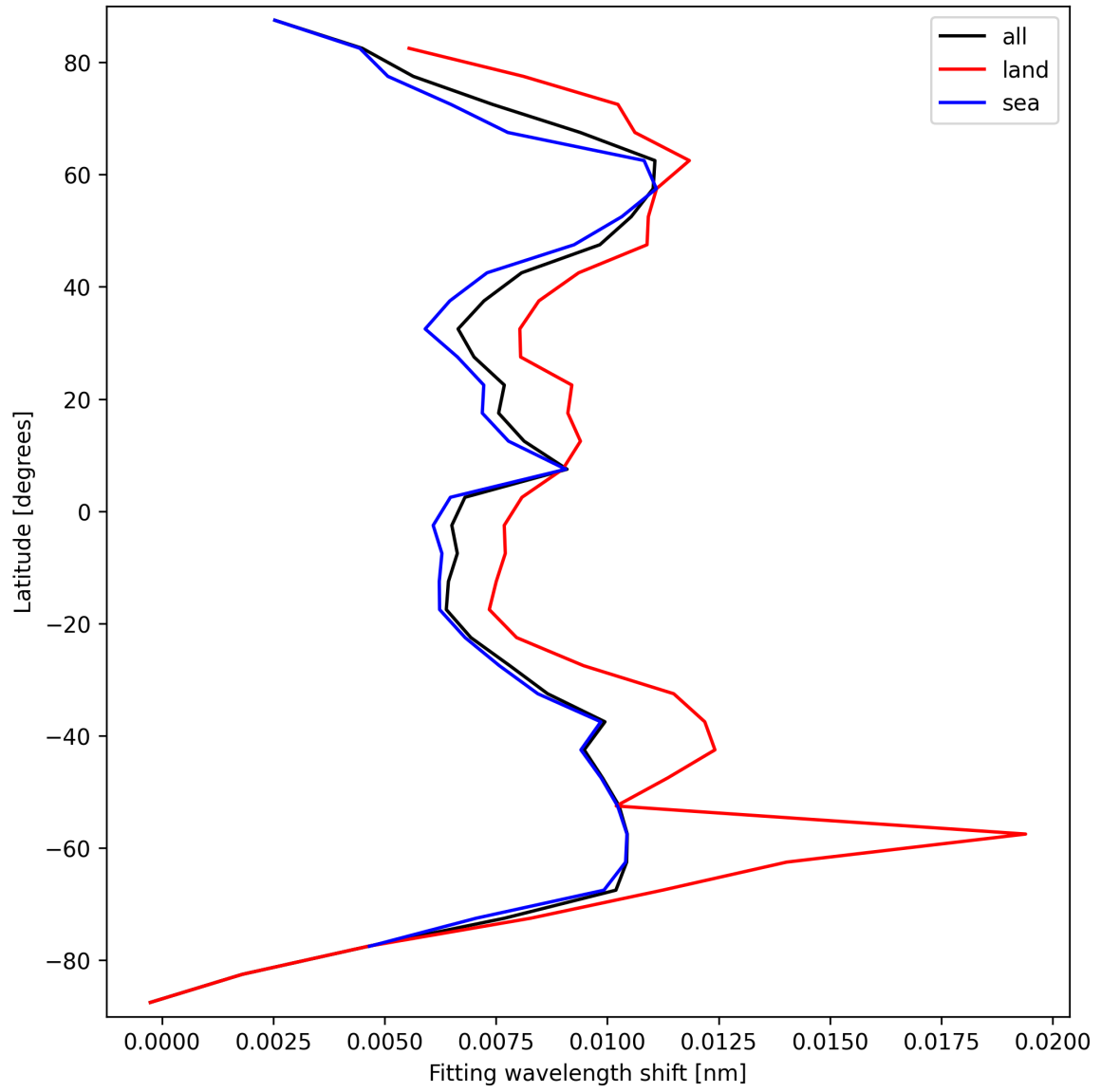
Figure 33: Zonal average of “Fitting wavelength shift” for 2024-09-12 to 2024-09-14.
