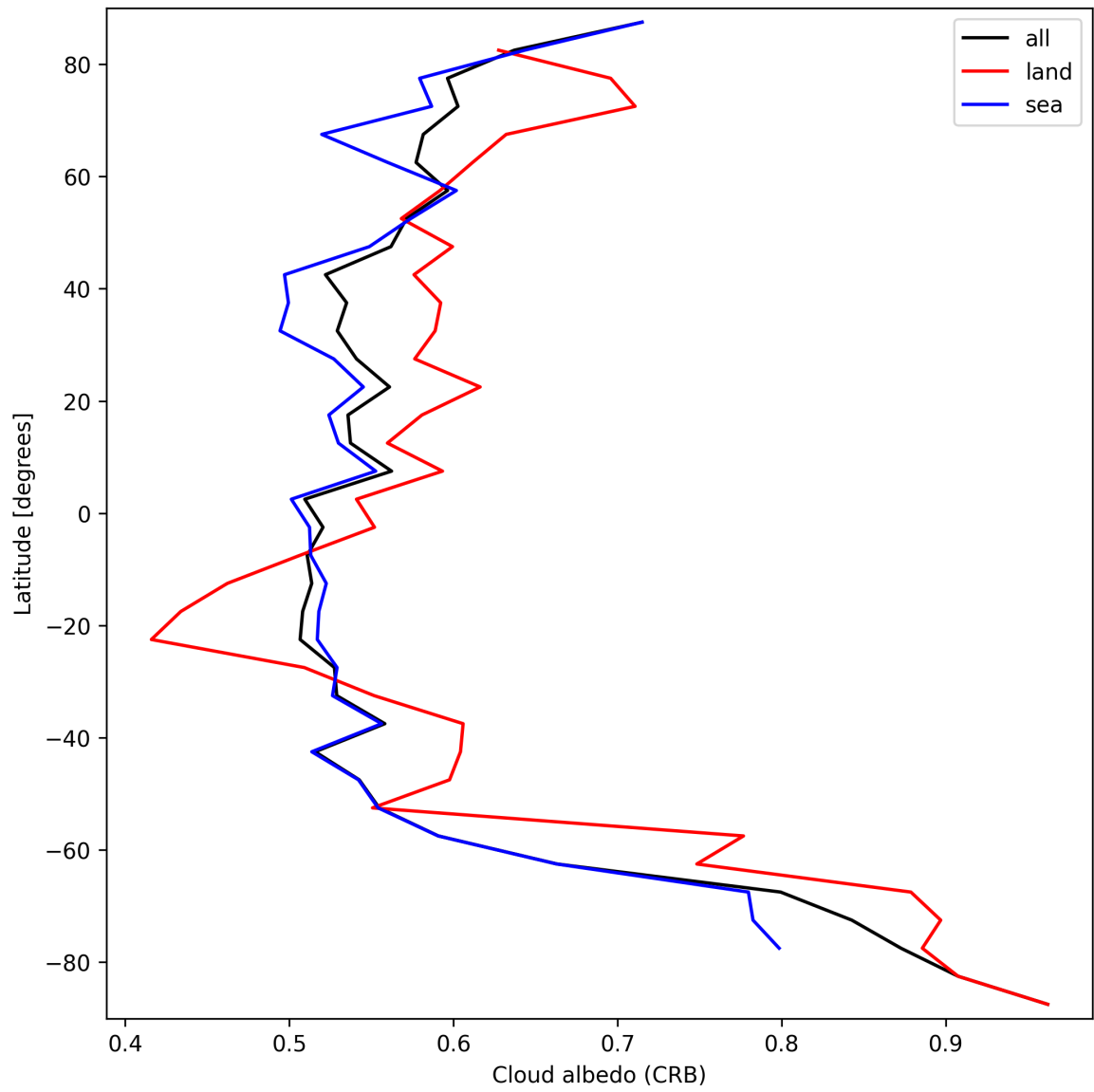
Figure 28: Zonal average of “Cloud albedo (CRB)” for 2024-09-12 to 2024-09-14.
