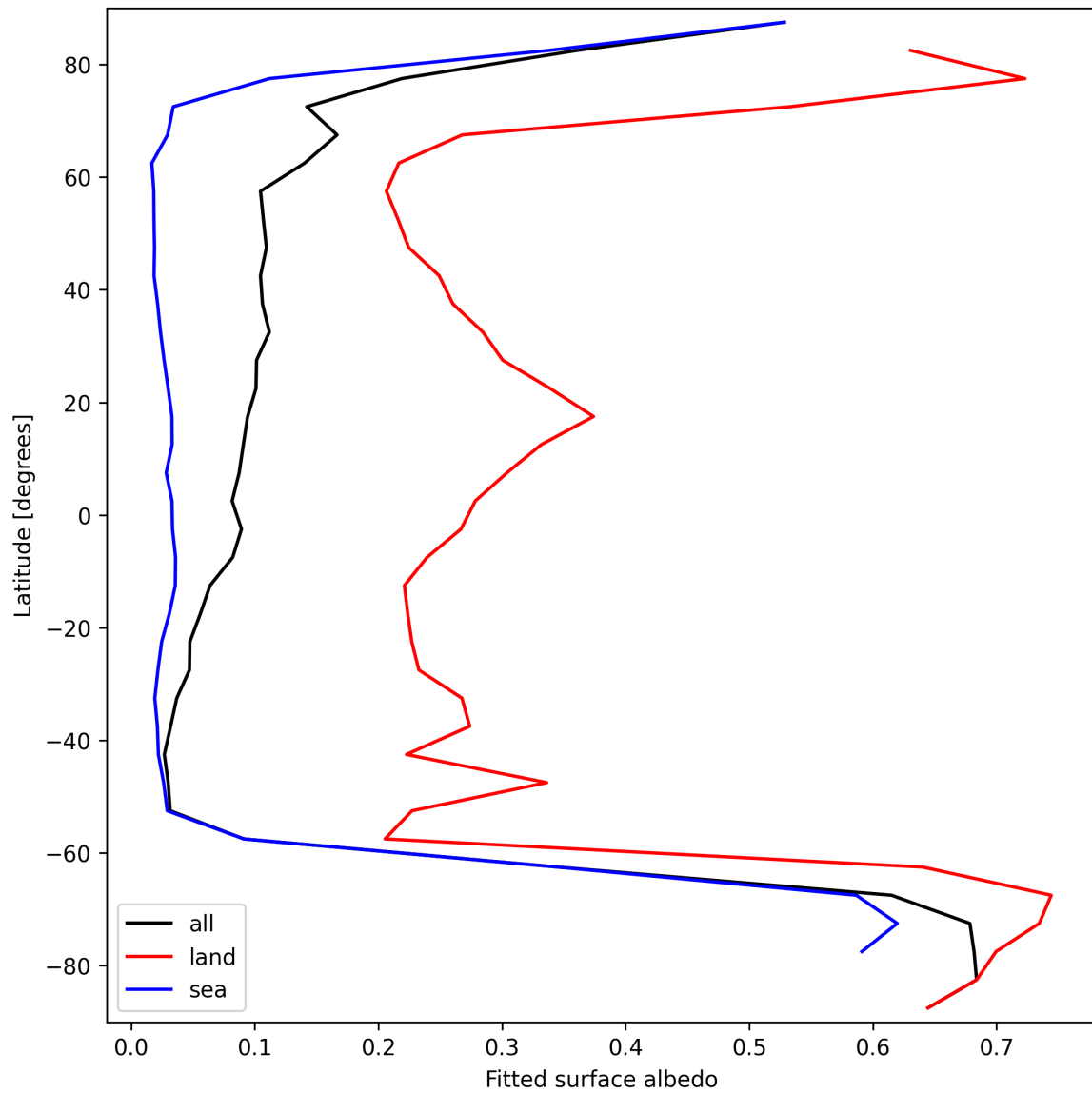
Figure 29: Zonal average of “Fitted surface albedo” for 2024-09-12 to 2024-09-14.
