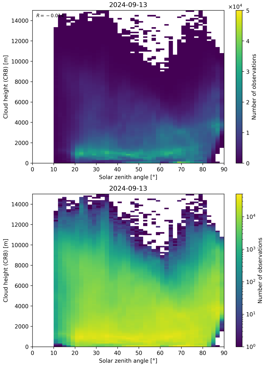
Figure 102: Scatter density plot of “Solar zenith angle” against “Cloud height (CRB)” for 2024-09-12 to 2024-09-14.
