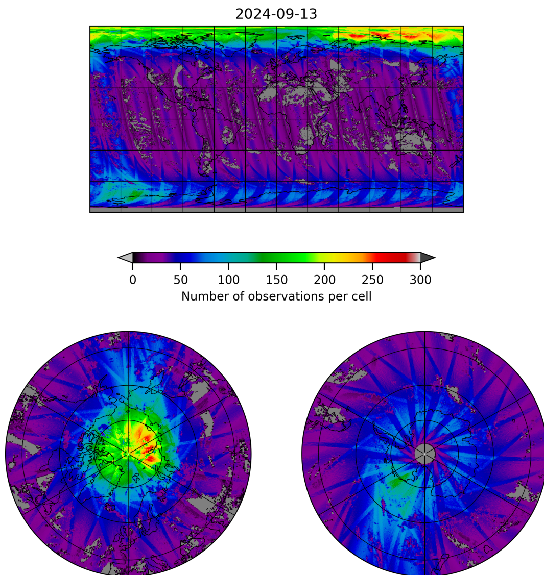
Figure 21: Map of the number of observations for 2024-09-12 to 2024-09-14
