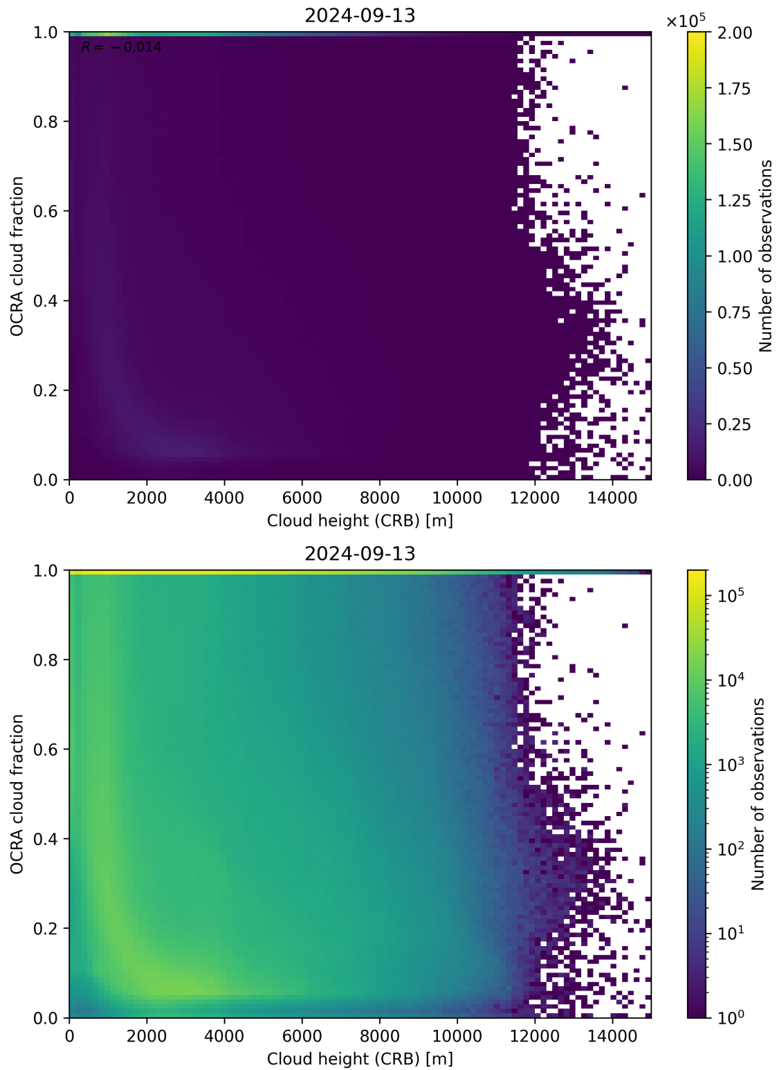
Figure 81: Scatter density plot of “Cloud height (CRB)” against “OCRA cloud fraction” for 2024-09-12 to 2024-09-14.
