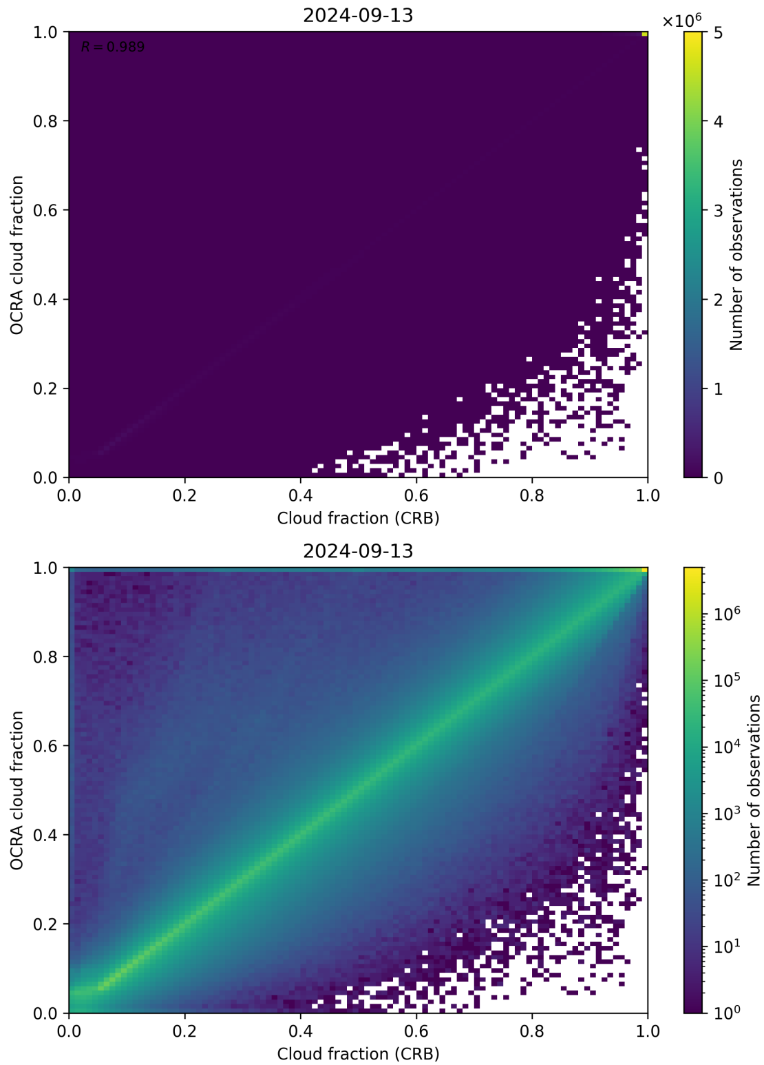
Figure 78: Scatter density plot of “Cloud fraction (CRB)” against “OCRA cloud fraction” for 2024-09-12 to 2024-09-14.
