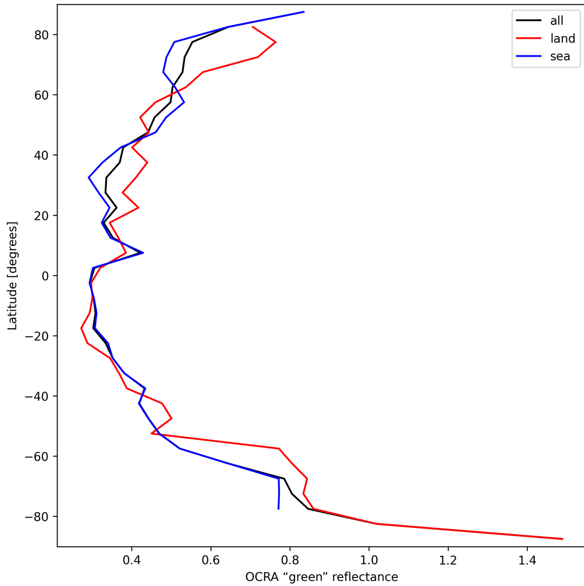
Figure 36: Zonal average of “OCRA “green” reflectance” for 2024-09-12 to 2024-09-14.
