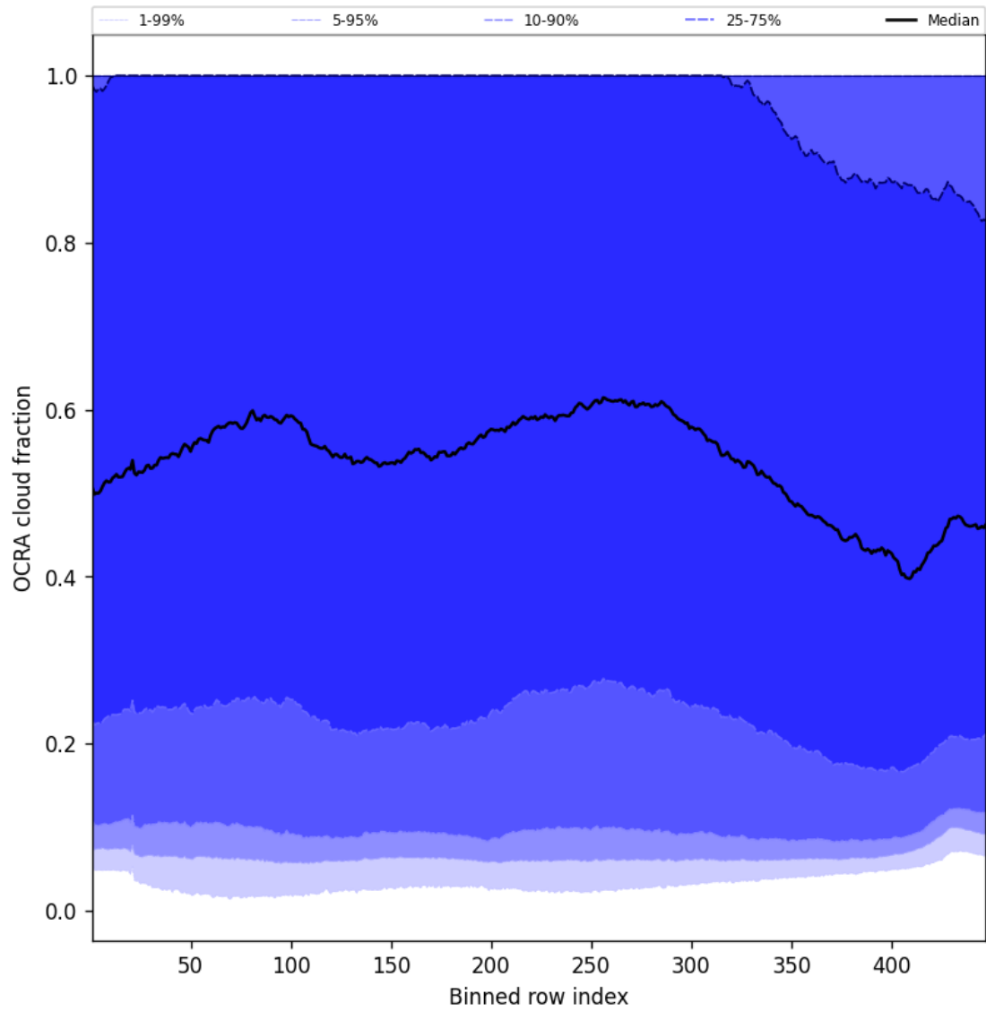
Figure 66: Along track statistics of “OCRA cloud fraction” for 2024-09-12 to 2024-09-14
