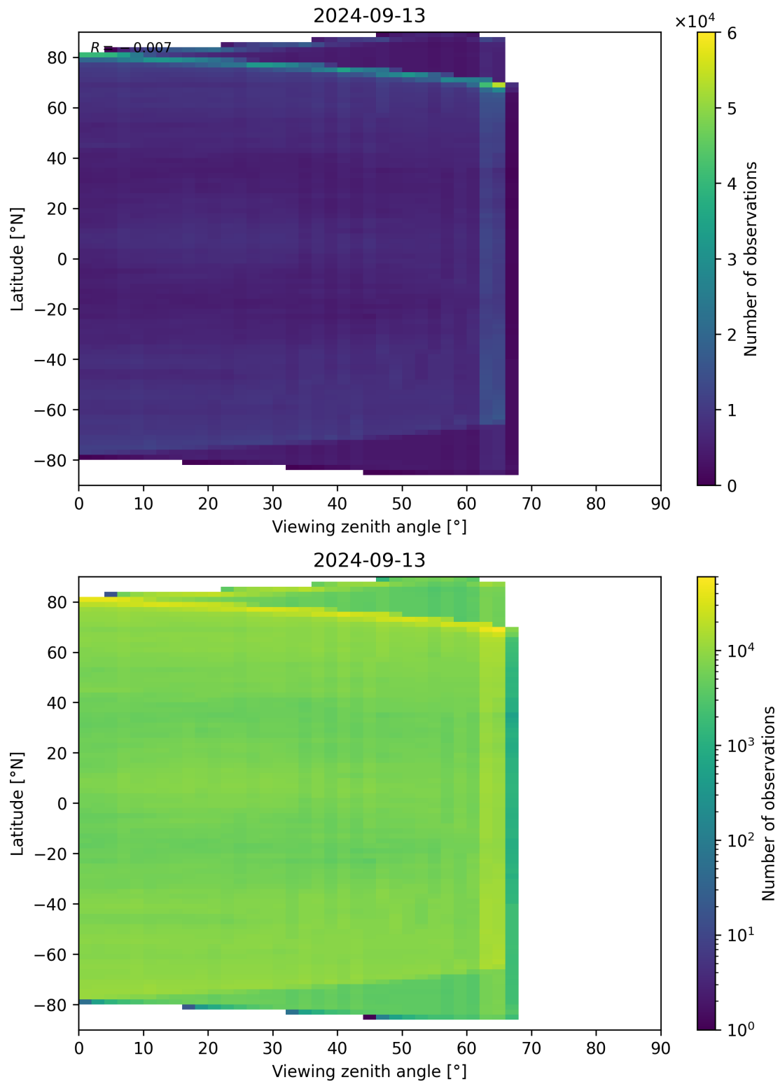
Figure 113: Scatter density plot of “Viewing zenith angle” against “Latitude” for 2024-09-12 to 2024-09-14.
