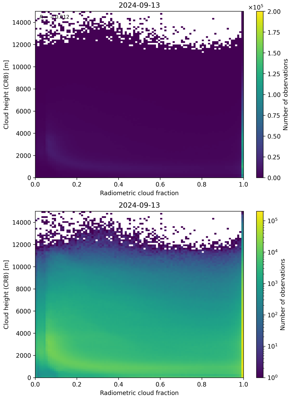
Figure 74: Scatter density plot of “Radiometric cloud fraction” against “Cloud height (CRB)” for 2024-09-12 to 2024-09-14.
