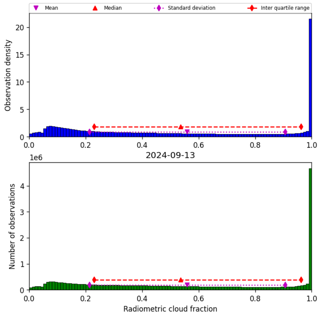
Figure 39: Histogram of “Radiometric cloud fraction” for 2024-09-12 to 2024-09-14
