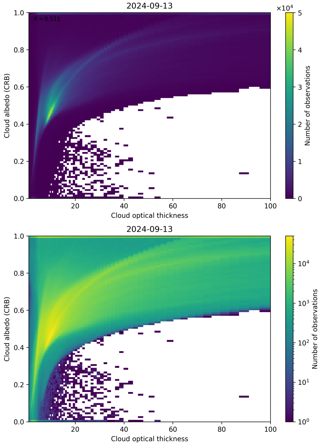
Figure 82: Scatter density plot of “Cloud optical thickness” against “Cloud albedo (CRB)” for 2024-09-12 to 2024-09-14.
