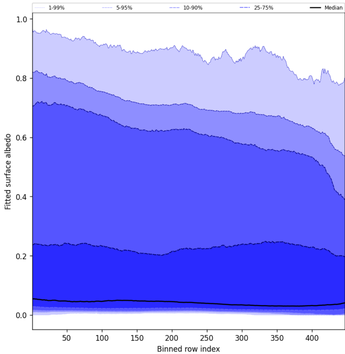
Figure 61: Along track statistics of “Fitted surface albedo” for 2024-09-12 to 2024-09-14
