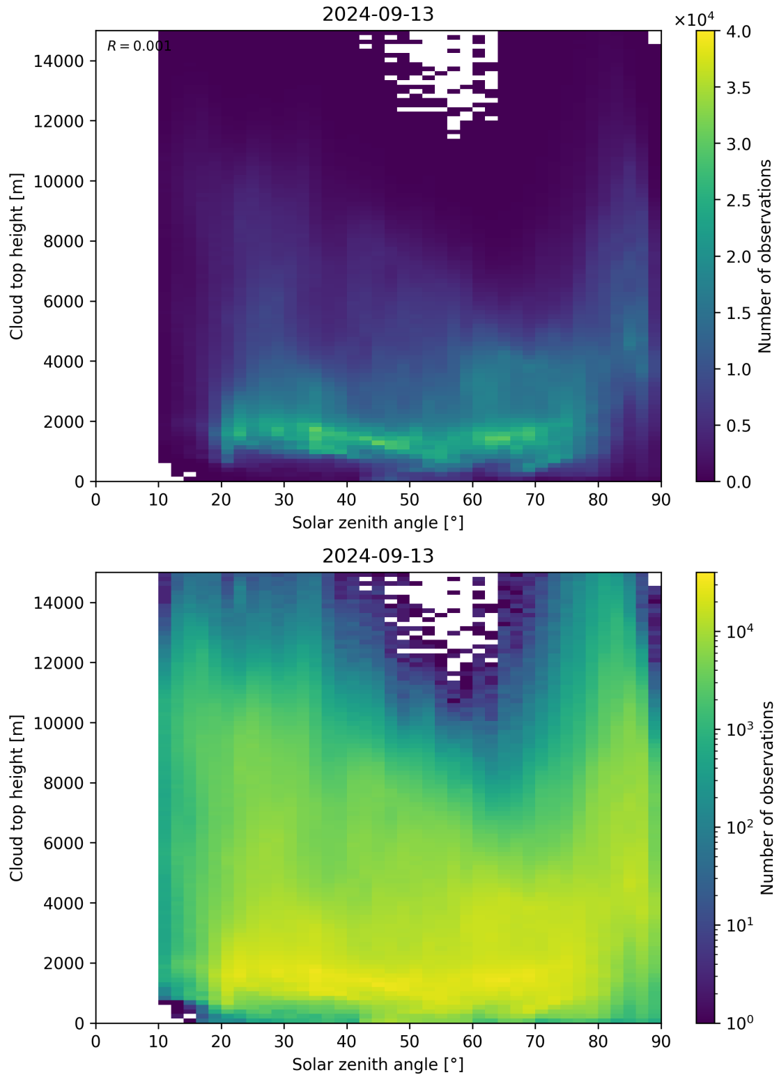
Figure 104: Scatter density plot of “Solar zenith angle” against “Cloud top height” for 2024-09-12 to 2024-09-14.
