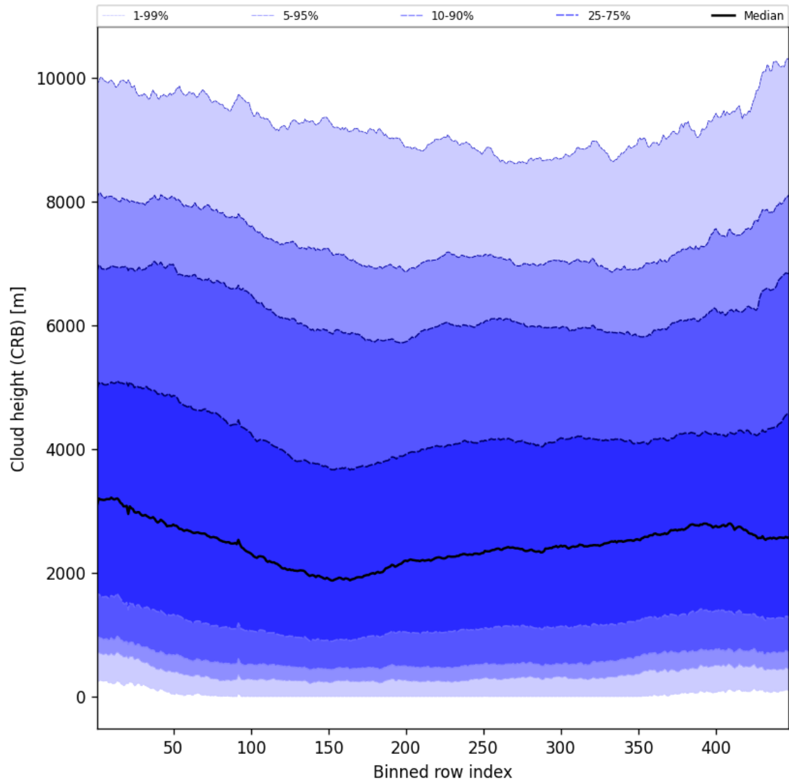
Figure 59: Along track statistics of “Cloud height (CRB)” for 2024-09-12 to 2024-09-14
