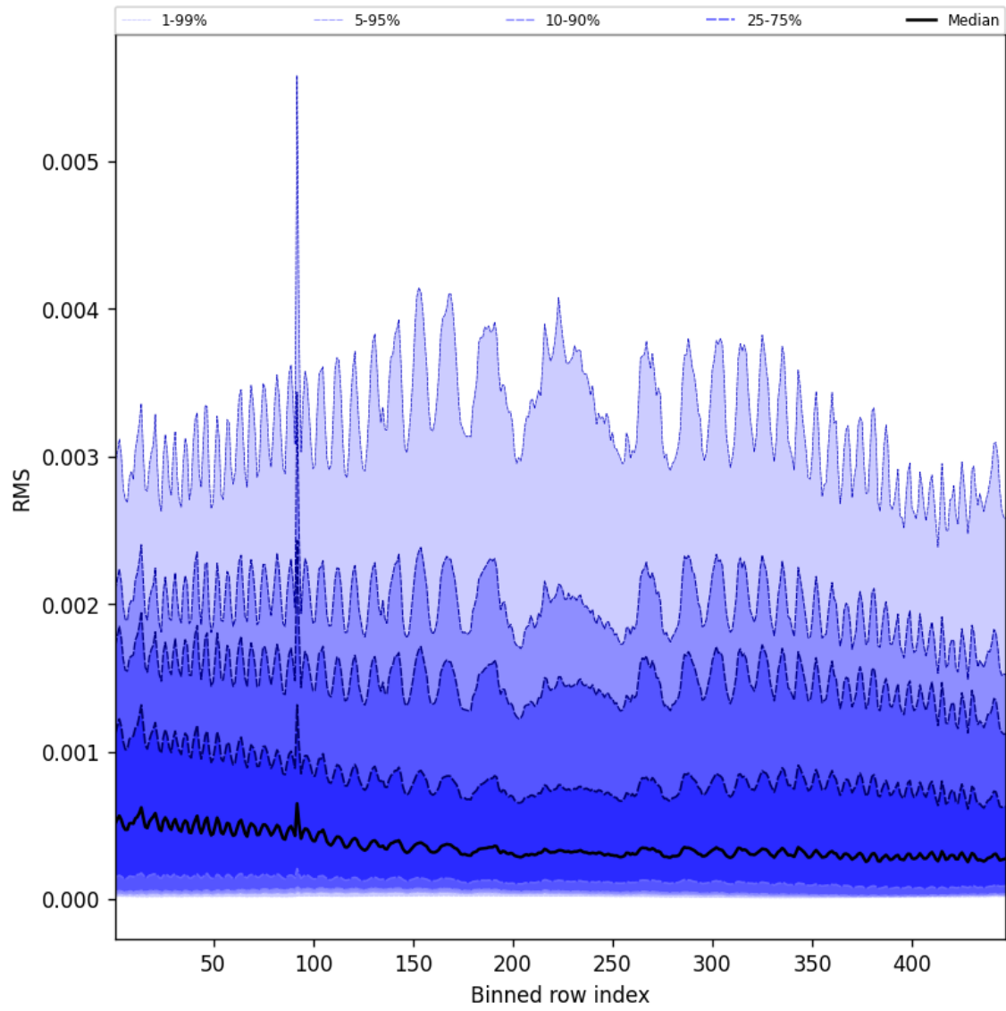
Figure 63: Along track statistics of “RMS” for 2024-09-12 to 2024-09-14
