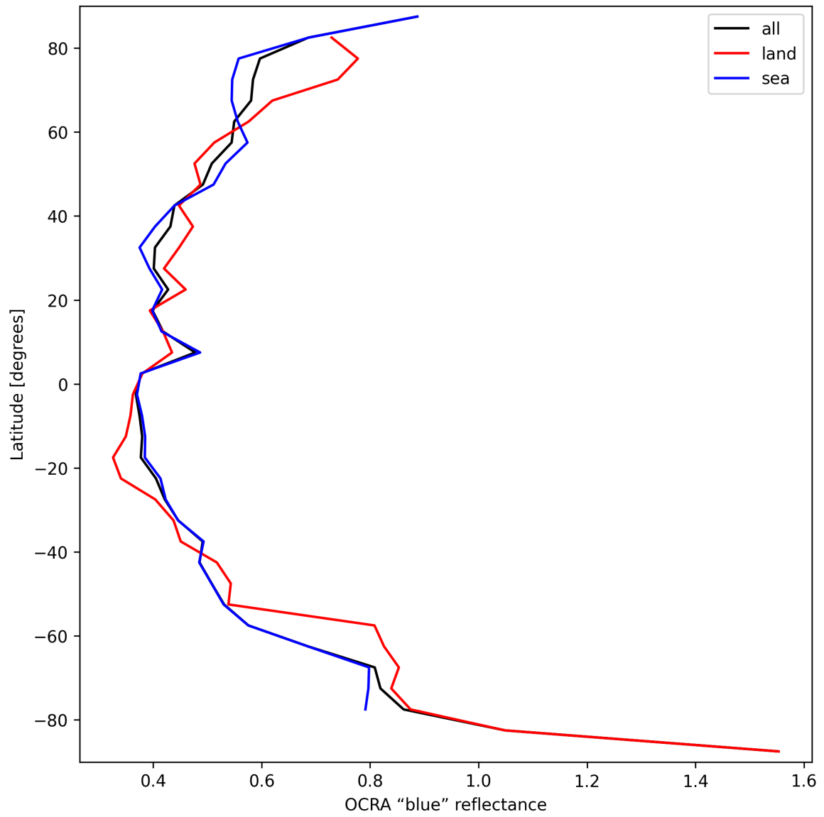
Figure 35: Zonal average of “OCRA “blue” reflectance” for 2024-09-12 to 2024-09-14.
