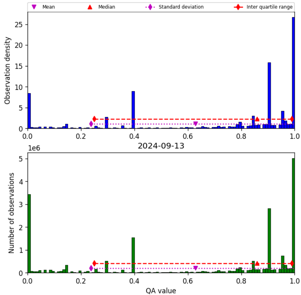
Figure 38: Histogram of “QA value” for 2024-09-12 to 2024-09-14
