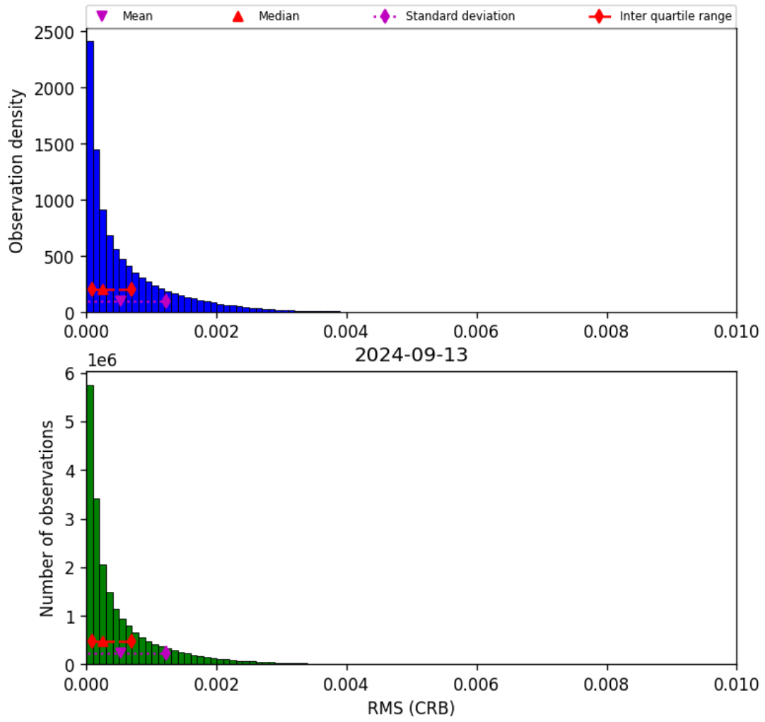
Figure 48: Histogram of “RMS (CRB)” for 2024-09-12 to 2024-09-14
