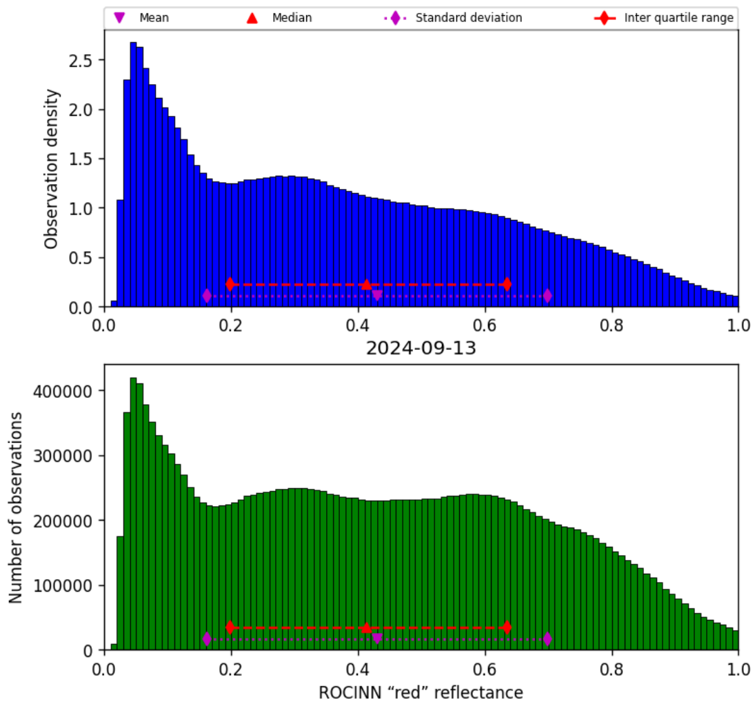
Figure 53: Histogram of “ROCINN “red” reflectance” for 2024-09-12 to 2024-09-14
