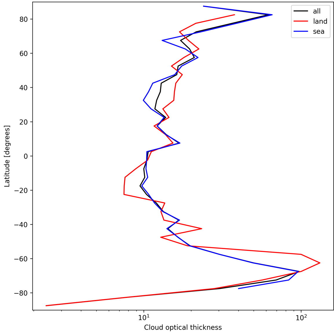
Figure 25: Zonal average of “Cloud optical thickness” for 2024-09-12 to 2024-09-14.
