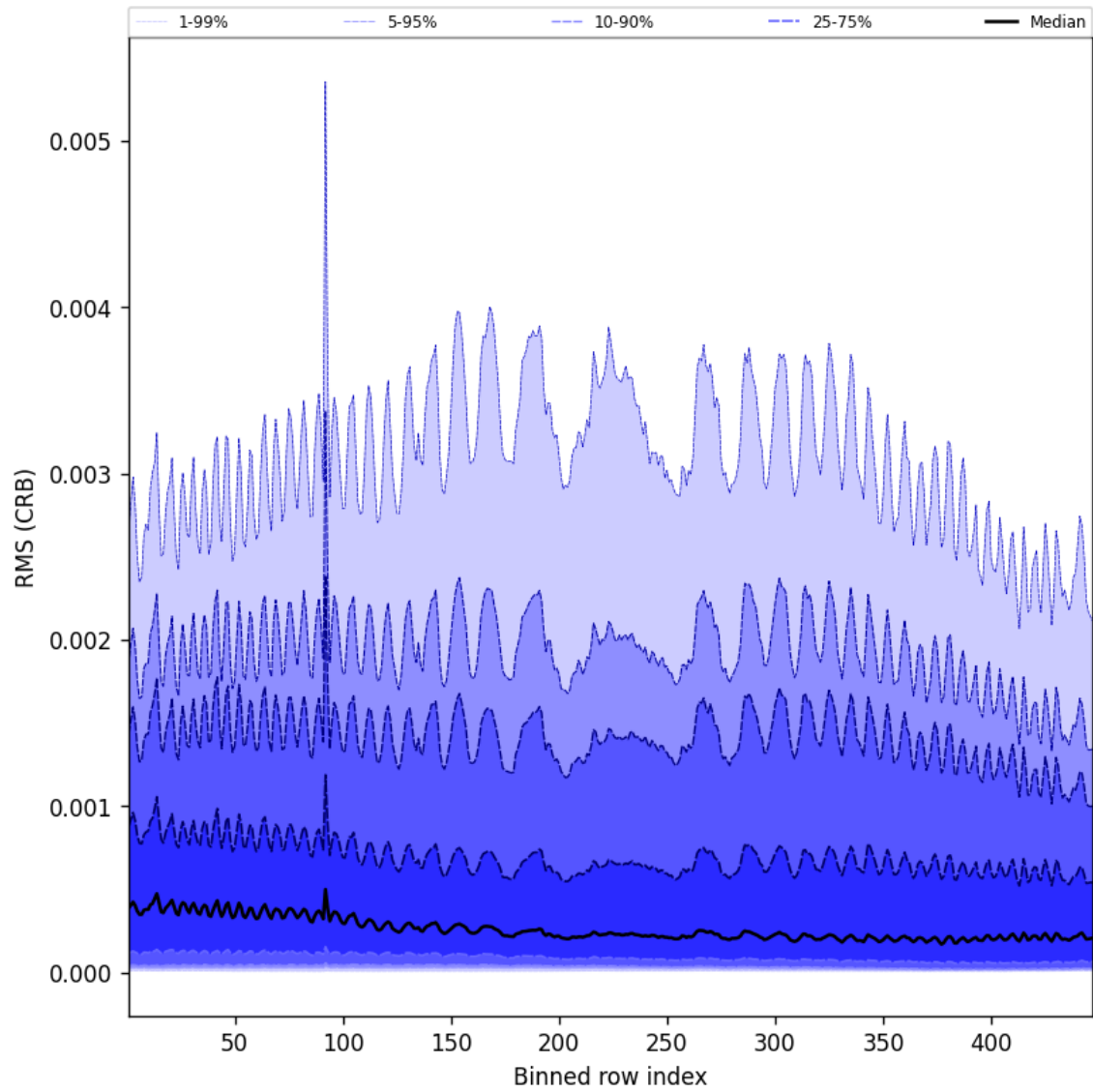
Figure 64: Along track statistics of “RMS (CRB)” for 2024-09-12 to 2024-09-14
