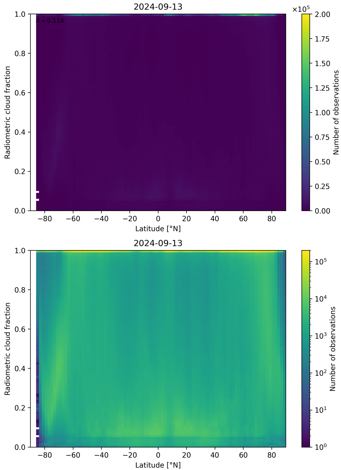
Figure 92: Scatter density plot of “Latitude” against “Radiometric cloud fraction” for 2024-09-12 to 2024-09-14.
