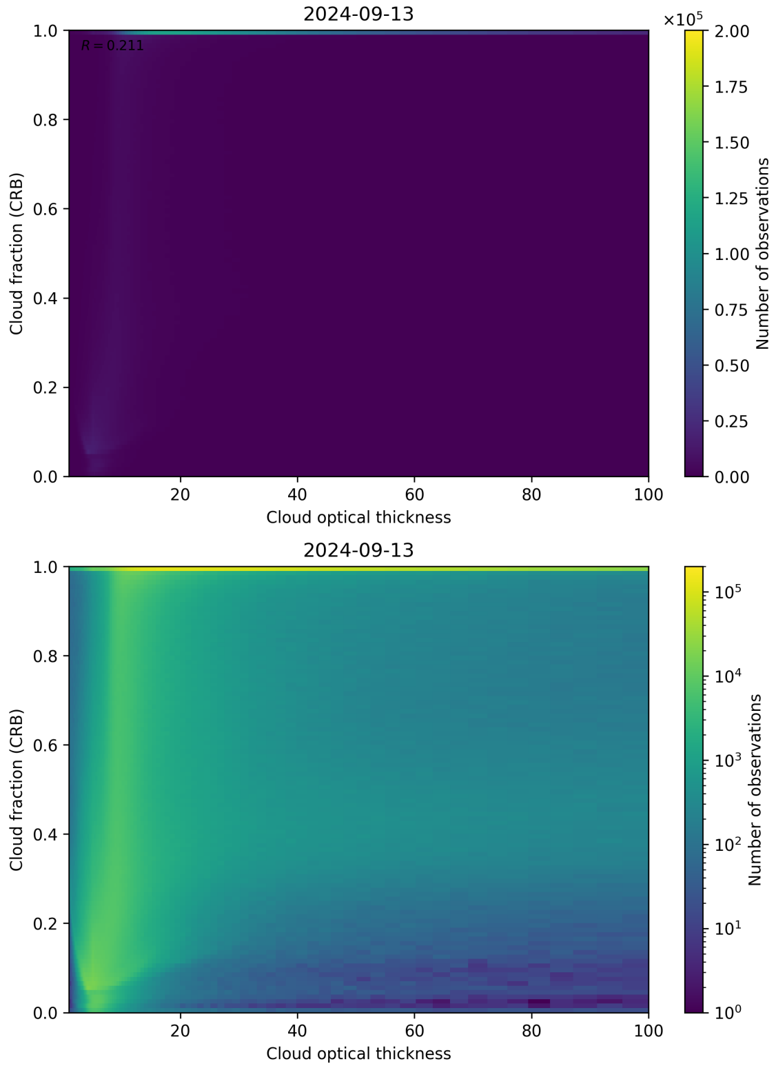
Figure 84: Scatter density plot of “Cloud optical thickness” against “Cloud fraction (CRB)” for 2024-09-12 to 2024-09-14.
