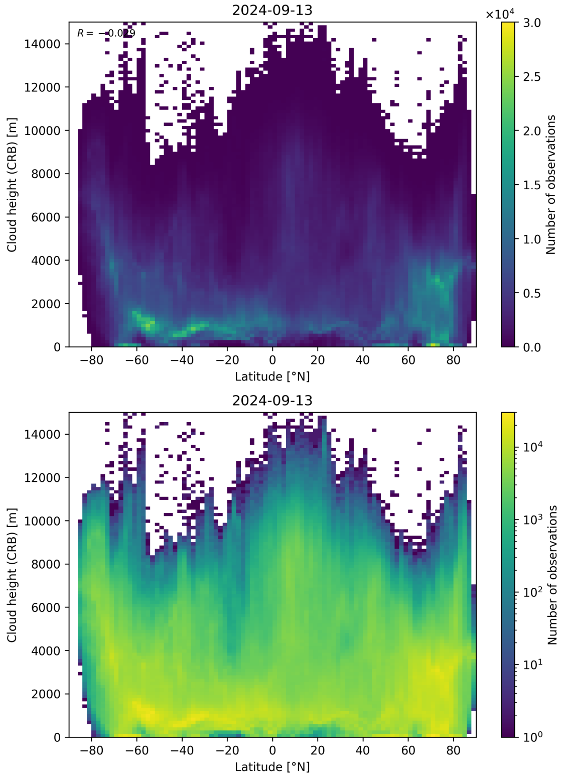
Figure 95: Scatter density plot of “Latitude” against “Cloud height (CRB)” for 2024-09-12 to 2024-09-14.
