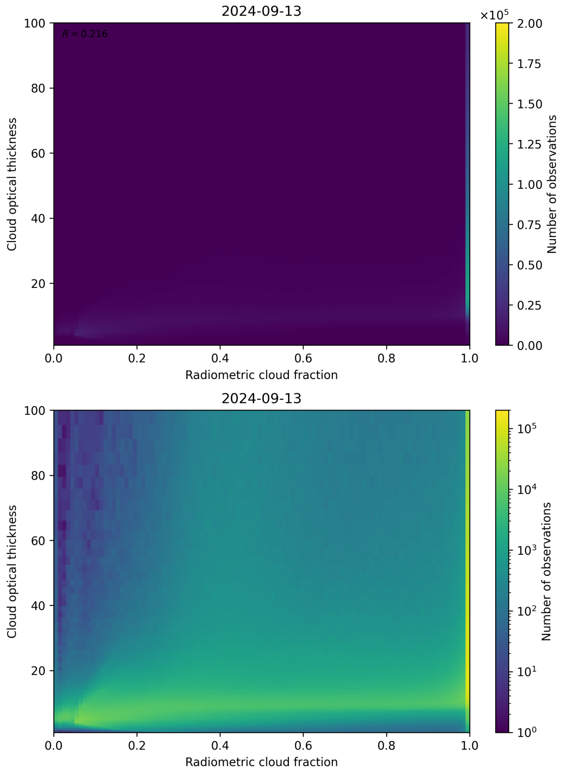
Figure 75: Scatter density plot of “Radiometric cloud fraction” against “Cloud optical thickness” for 2024-09-12 to 2024-09-14.
