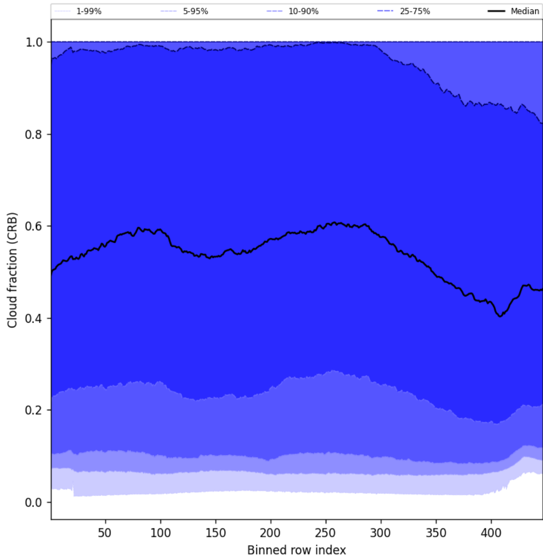
Figure 58: Along track statistics of “Cloud fraction (CRB)” for 2024-09-12 to 2024-09-14
