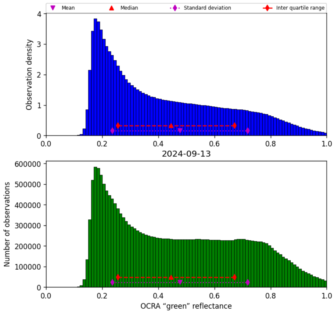
Figure 52: Histogram of “OCRA “green” reflectance” for 2024-09-12 to 2024-09-14
