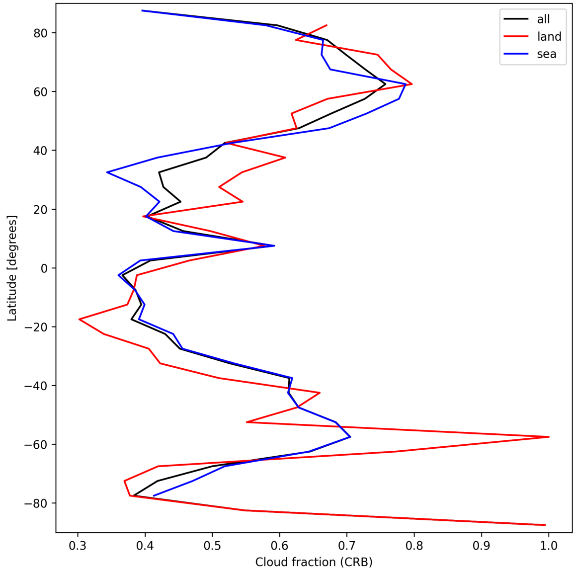
Figure 26: Zonal average of “Cloud fraction (CRB)” for 2024-09-12 to 2024-09-14.
