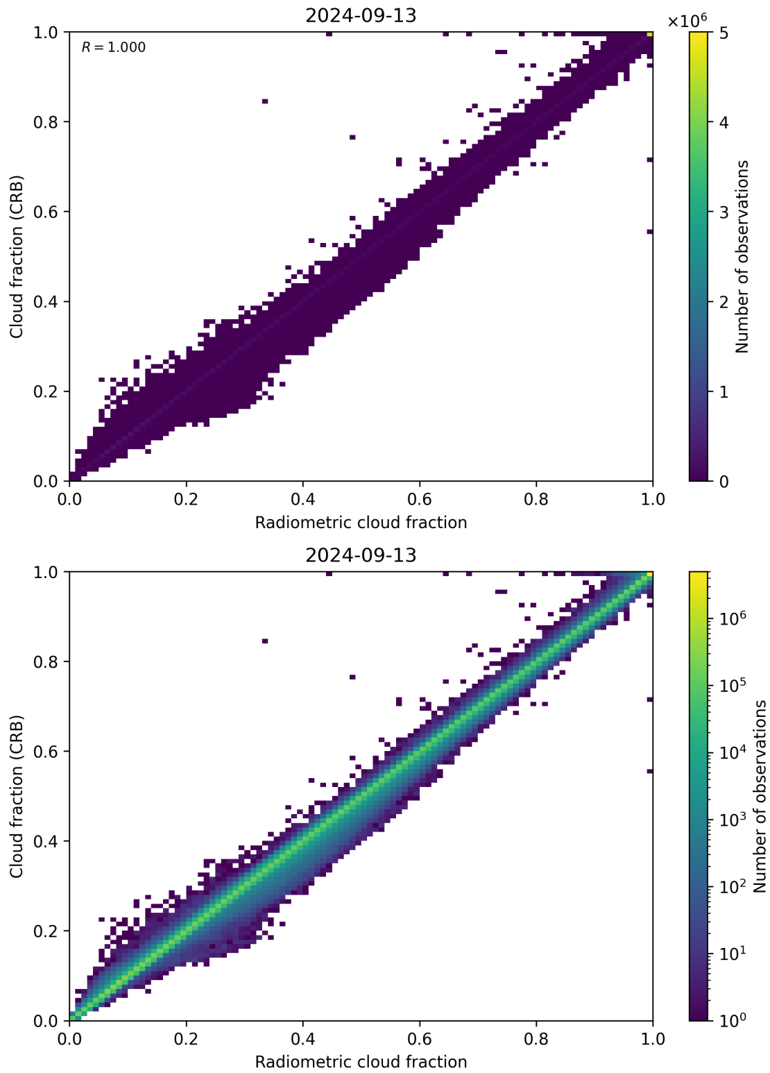
Figure 73: Scatter density plot of “Radiometric cloud fraction” against “Cloud fraction (CRB)” for 2024-09-12 to 2024-09-14.
