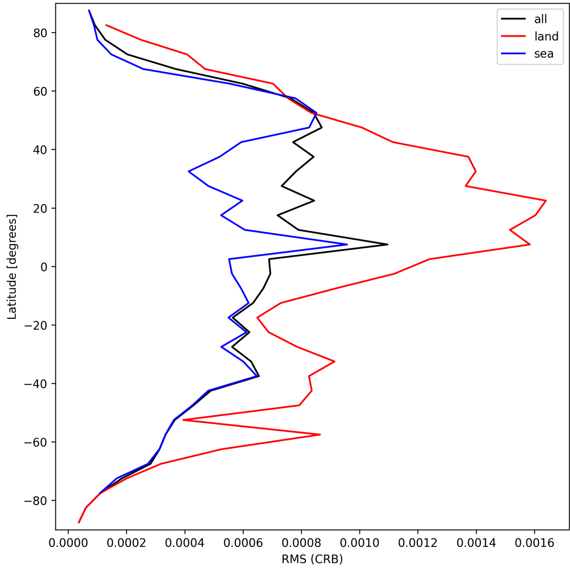
Figure 32: Zonal average of “RMS (CRB)” for 2024-09-12 to 2024-09-14.
