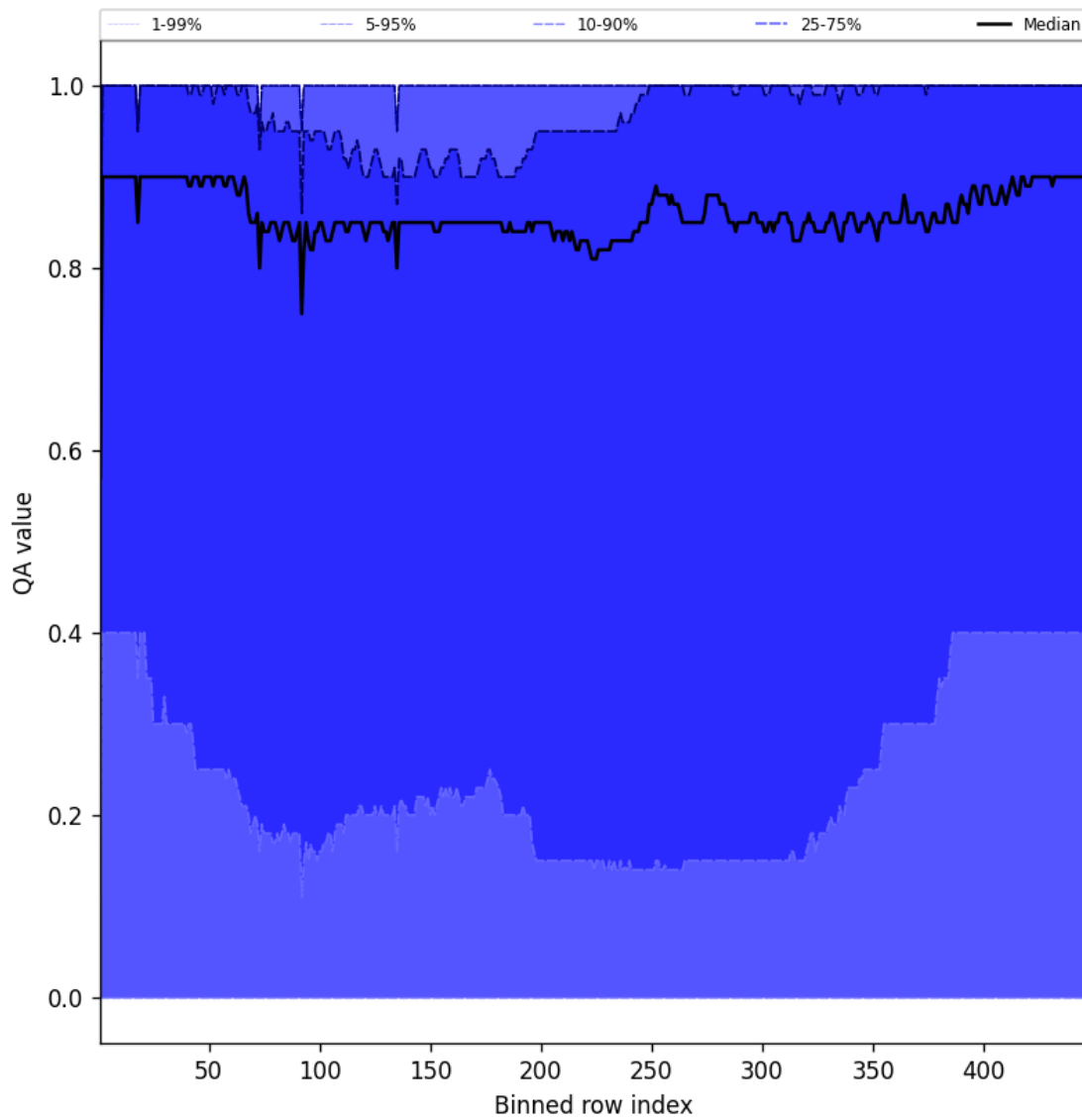
Figure 54: Along track statistics of “QA value” for 2024-09-12 to 2024-09-14
