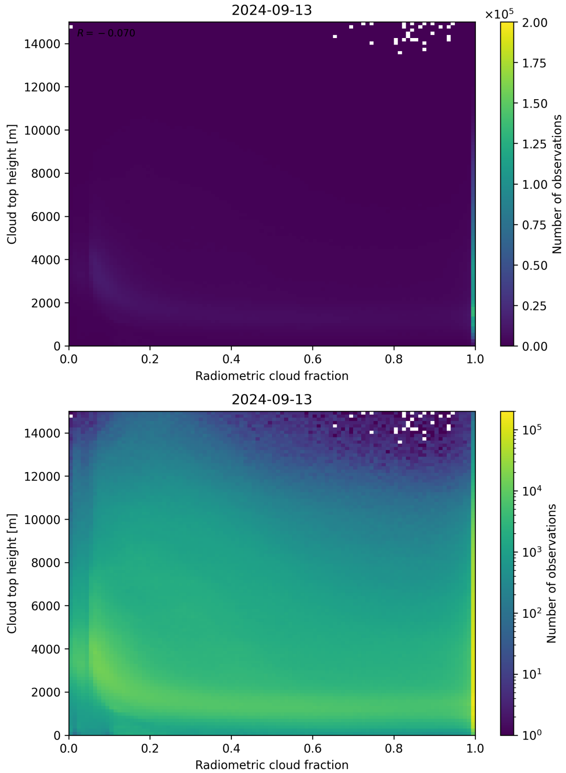
Figure 76: Scatter density plot of “Radiometric cloud fraction” against “Cloud top height” for 2024-09-12 to 2024-09-14.
