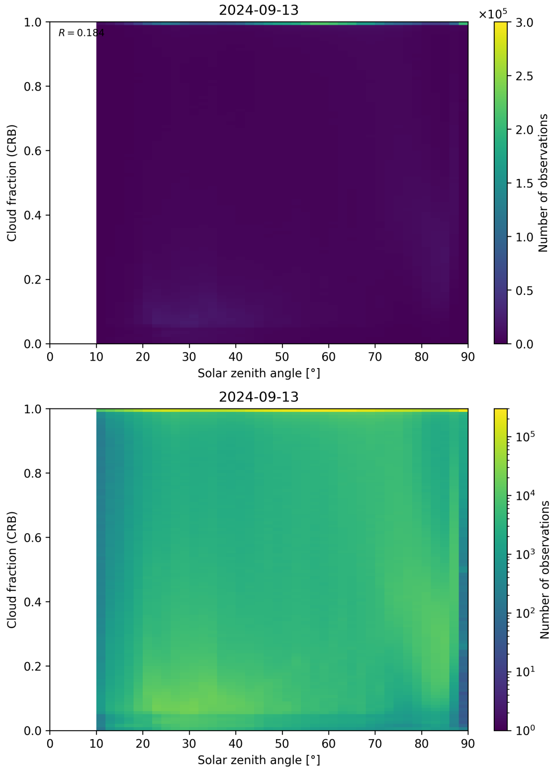
Figure 101: Scatter density plot of “Solar zenith angle” against “Cloud fraction (CRB)” for 2024-09-12 to 2024-09-14.
