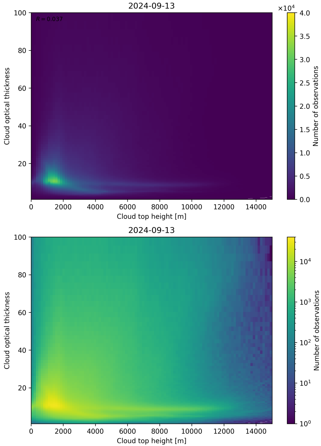
Figure 90: Scatter density plot of “Cloud top height” against “Cloud optical thickness” for 2024-09-12 to 2024-09-14.
