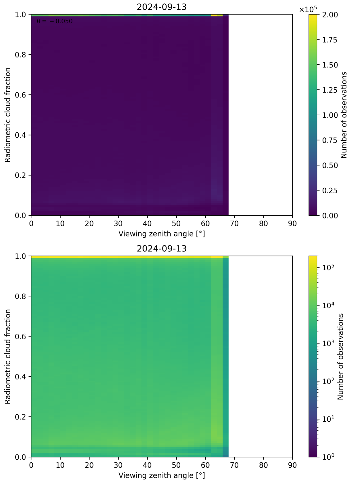
Figure 107: Scatter density plot of “Viewing zenith angle” against “Radiometric cloud fraction” for 2024-09-12 to 2024-09-14.
