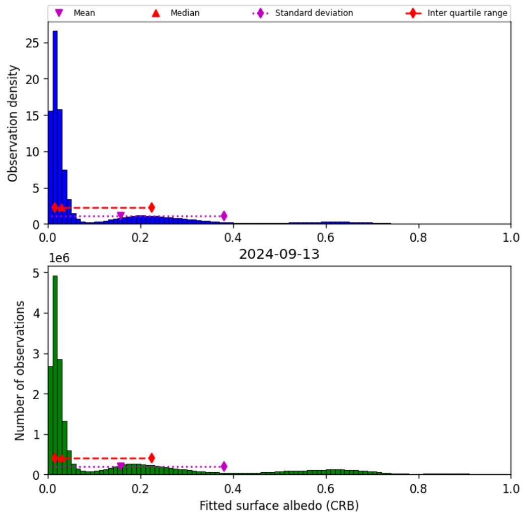
Figure 46: Histogram of “Fitted surface albedo (CRB)” for 2024-09-12 to 2024-09-14
