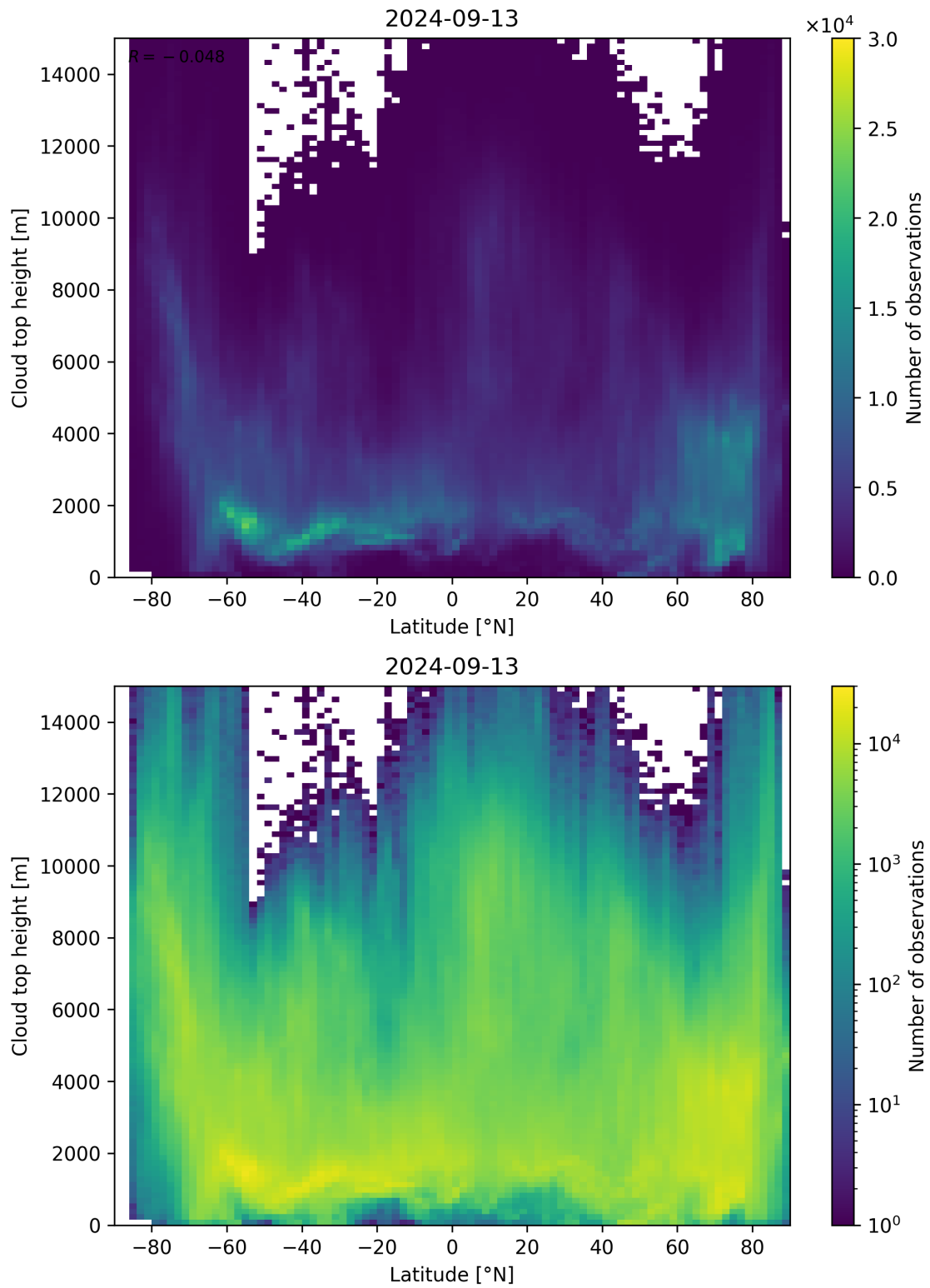
Figure 97: Scatter density plot of “Latitude” against “Cloud top height” for 2024-09-12 to 2024-09-14.
