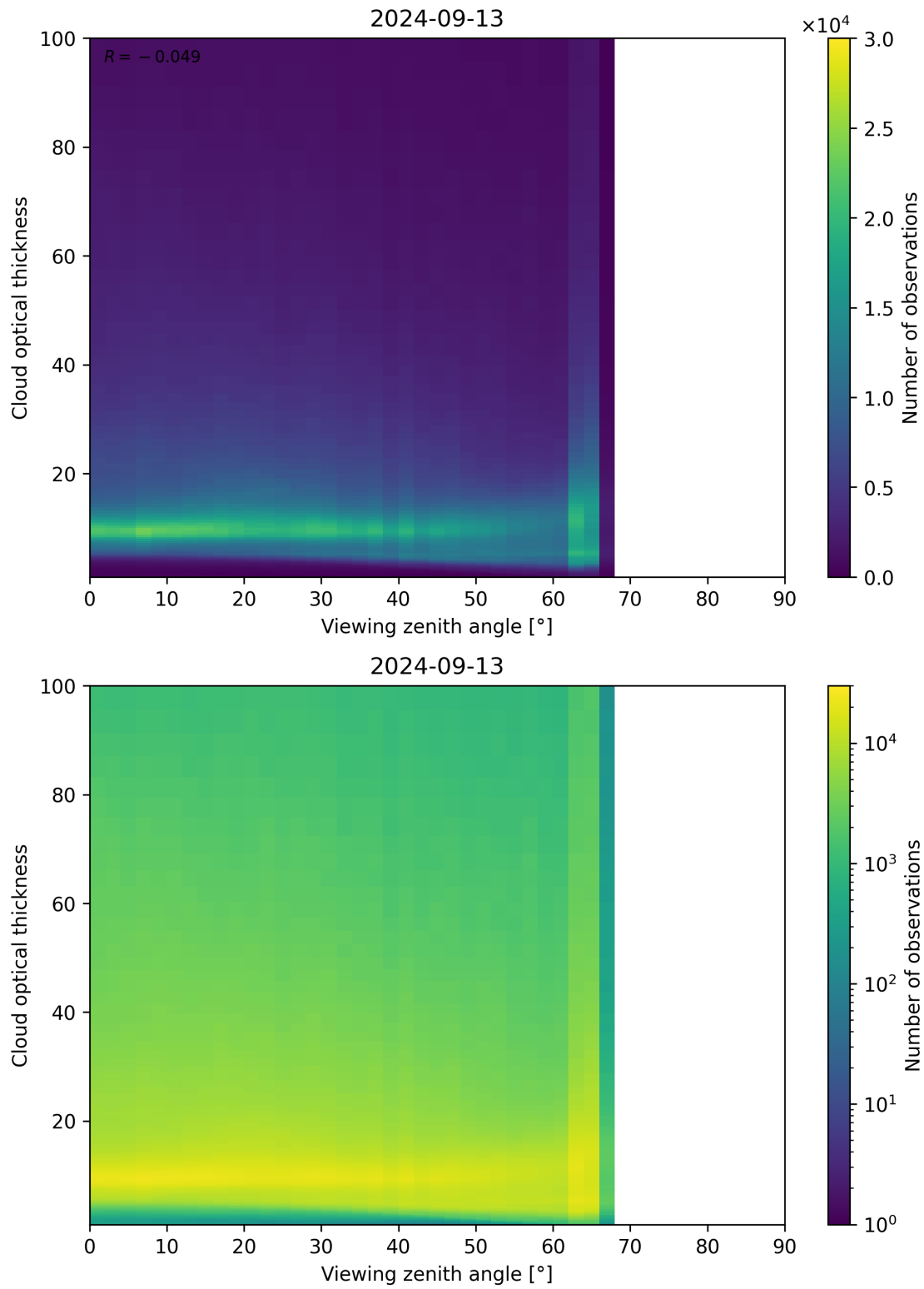
Figure 111: Scatter density plot of “Viewing zenith angle” against “Cloud optical thickness” for 2024-09-12 to 2024-09-14.
