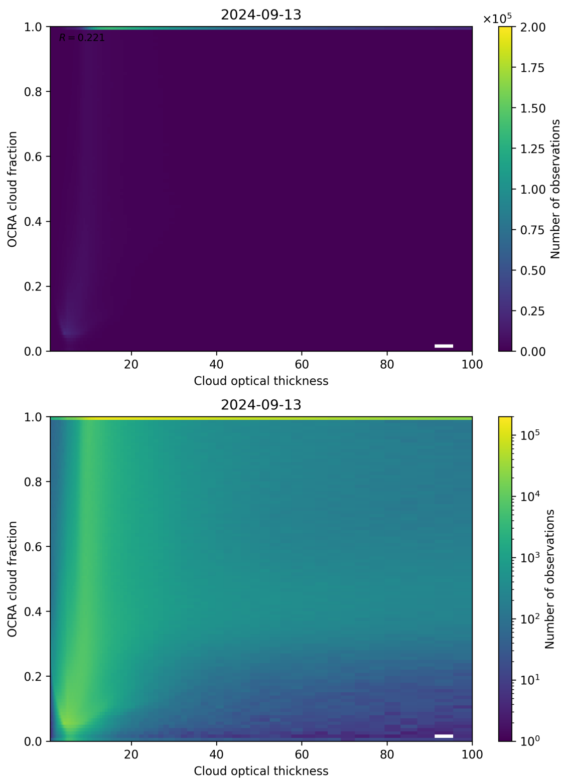
Figure 83: Scatter density plot of “Cloud optical thickness” against “OCRA cloud fraction” for 2024-09-12 to 2024-09-14.
