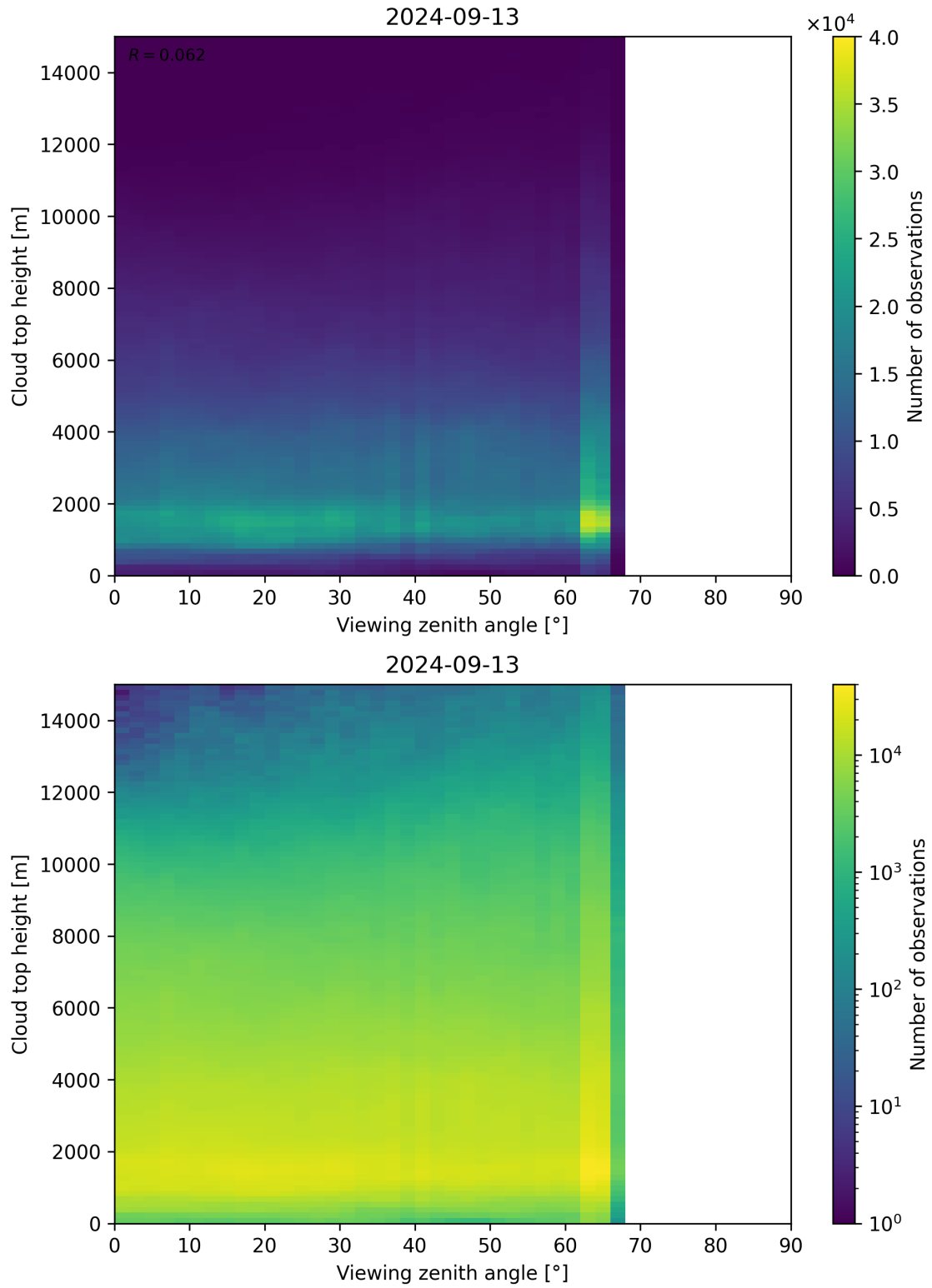
Figure 112: Scatter density plot of “Viewing zenith angle” against “Cloud top height” for 2024-09-12 to 2024-09-14.
