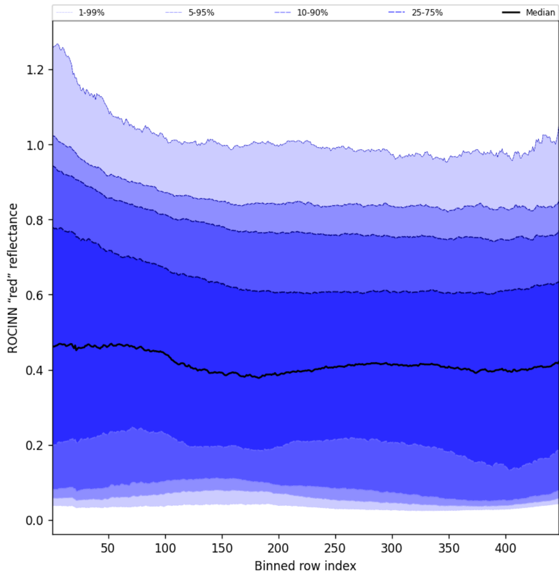
Figure 69: Along track statistics of “ROCINN “red” reflectance” for 2024-09-12 to 2024-09-14
