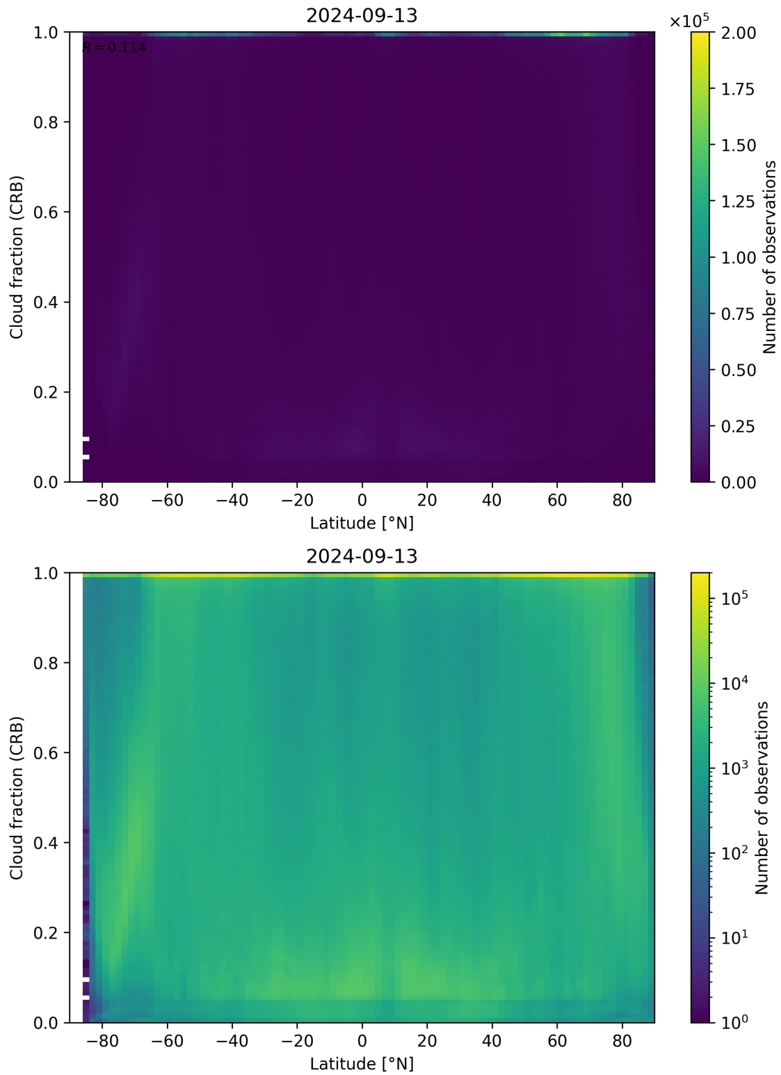
Figure 94: Scatter density plot of “Latitude” against “Cloud fraction (CRB)” for 2024-09-12 to 2024-09-14.
