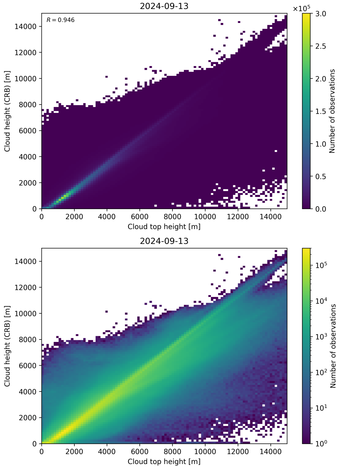
Figure 89: Scatter density plot of “Cloud top height” against “Cloud height (CRB)” for 2024-09-12 to 2024-09-14.
