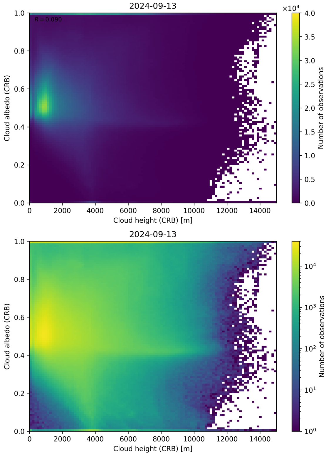
Figure 80: Scatter density plot of “Cloud height (CRB)” against “Cloud albedo (CRB)” for 2024-09-12 to 2024-09-14.
