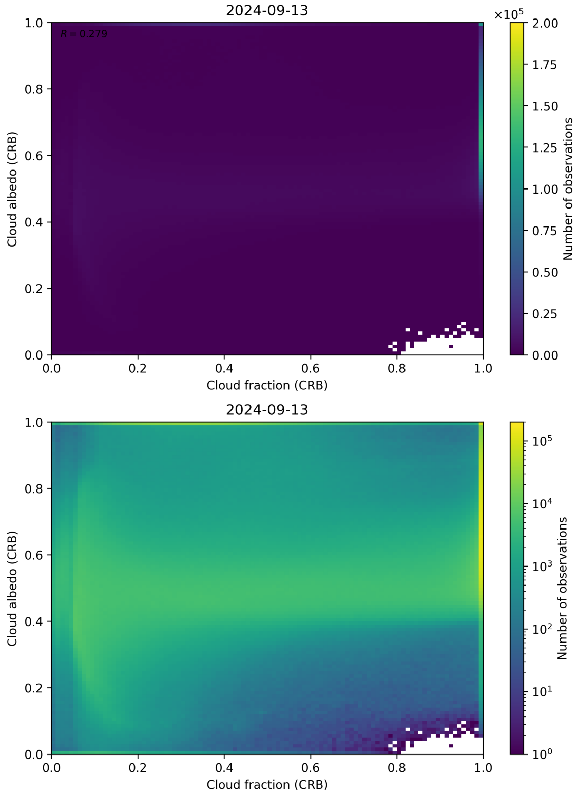
Figure 77: Scatter density plot of “Cloud fraction (CRB)” against “Cloud albedo (CRB)” for 2024-09-12 to 2024-09-14.
