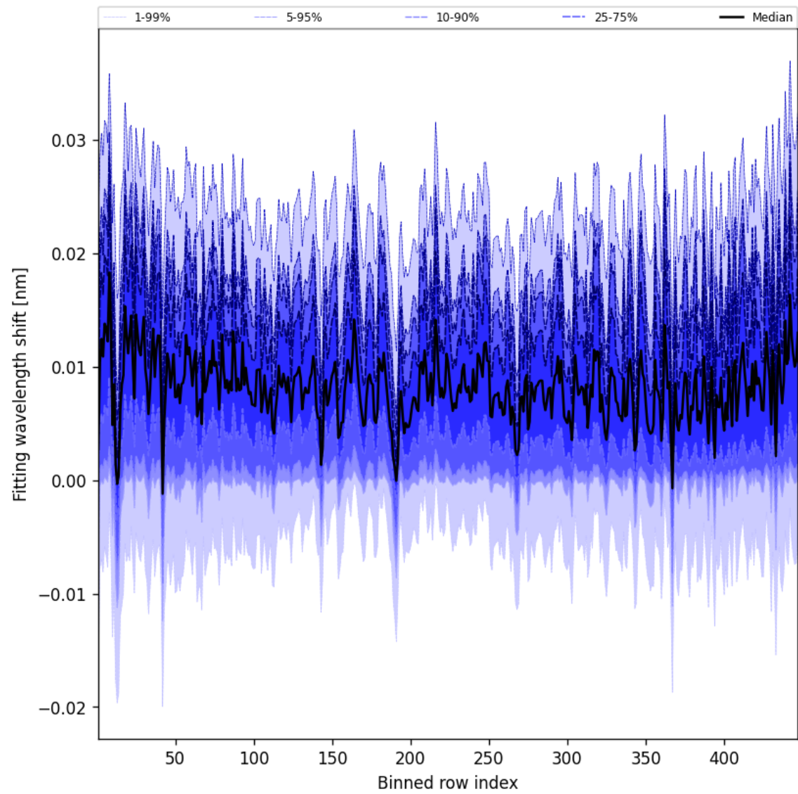
Figure 65: Along track statistics of “Fitting wavelength shift” for 2024-09-12 to 2024-09-14
