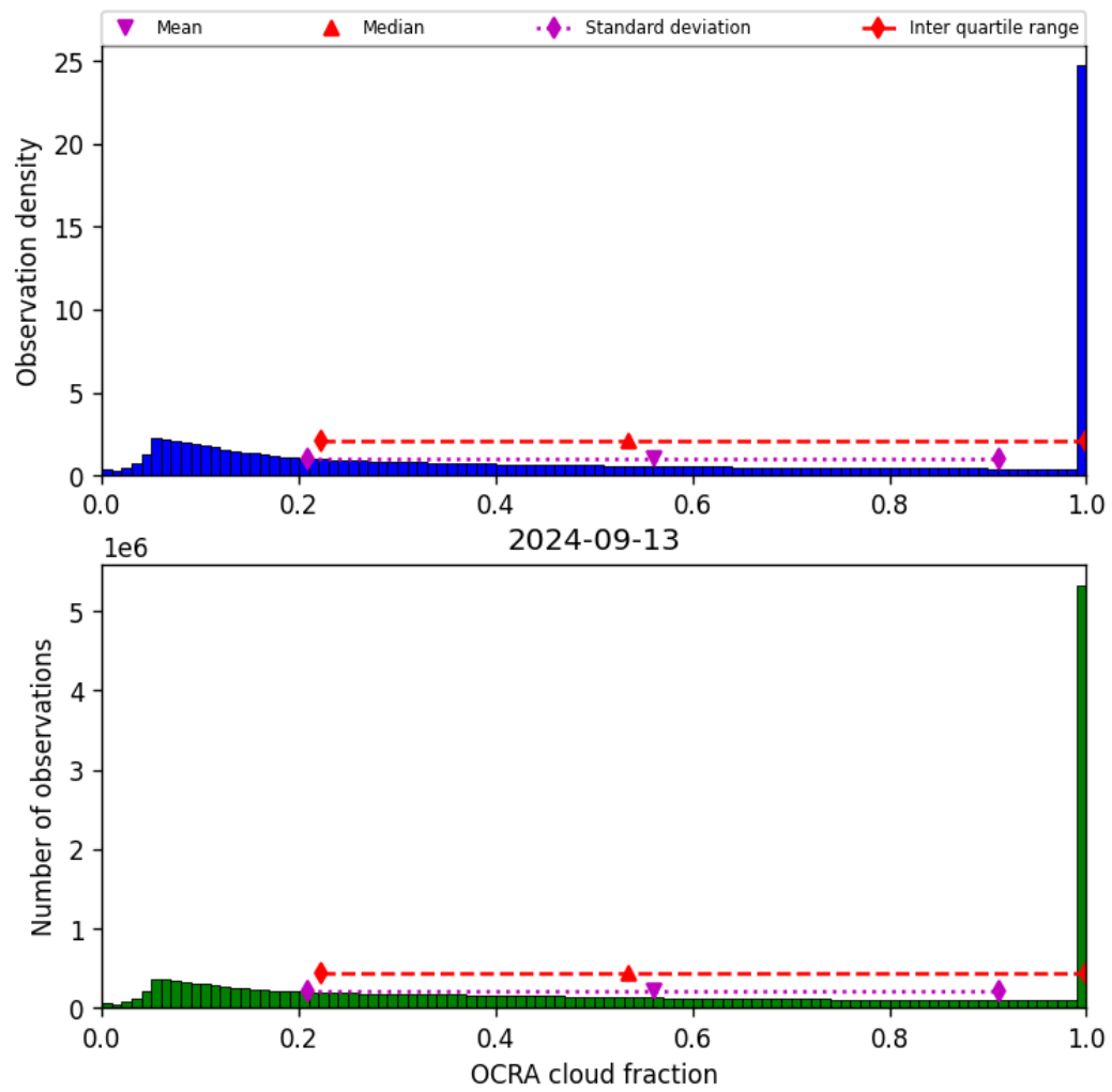
Figure 50: Histogram of “OCRA cloud fraction” for 2024-09-12 to 2024-09-14
