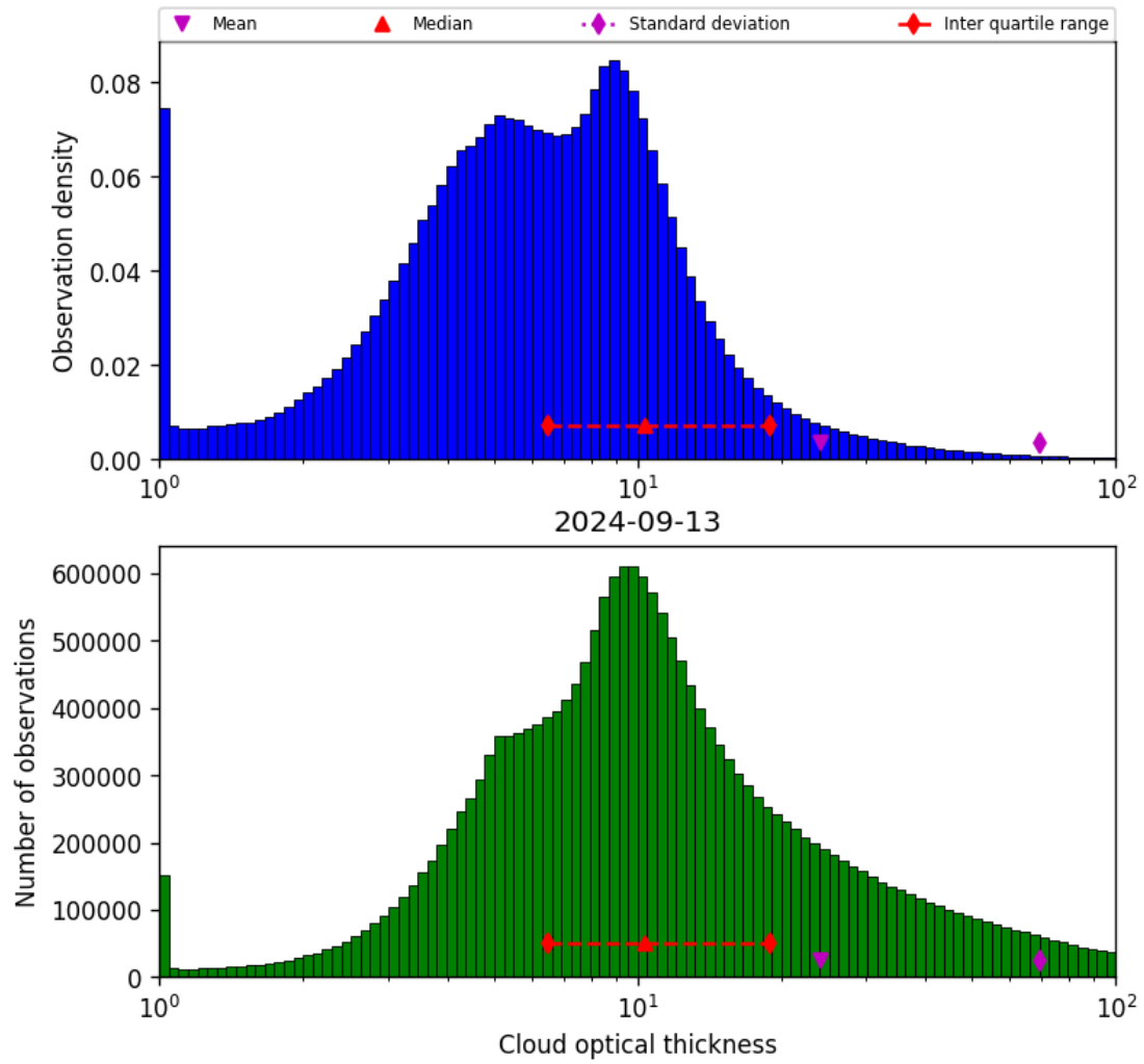
Figure 41: Histogram of “Cloud optical thickness” for 2024-09-12 to 2024-09-14
