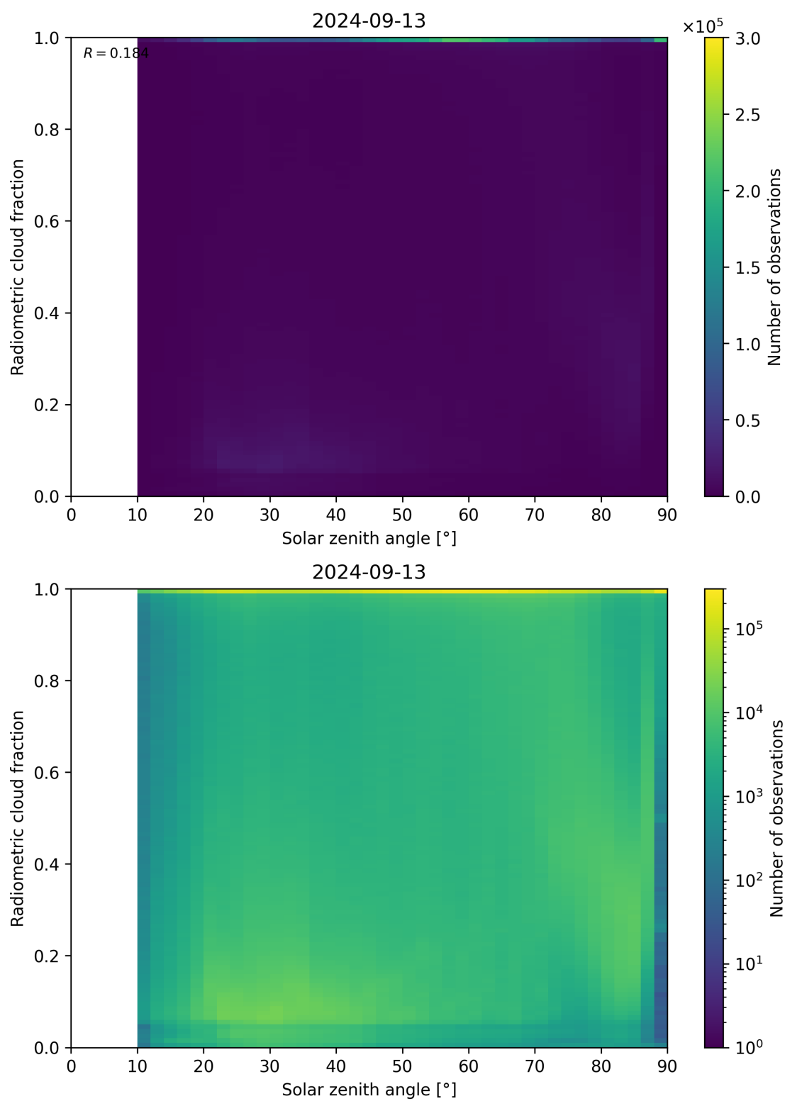
Figure 99: Scatter density plot of “Solar zenith angle” against “Radiometric cloud fraction” for 2024-09-12 to 2024-09-14.
