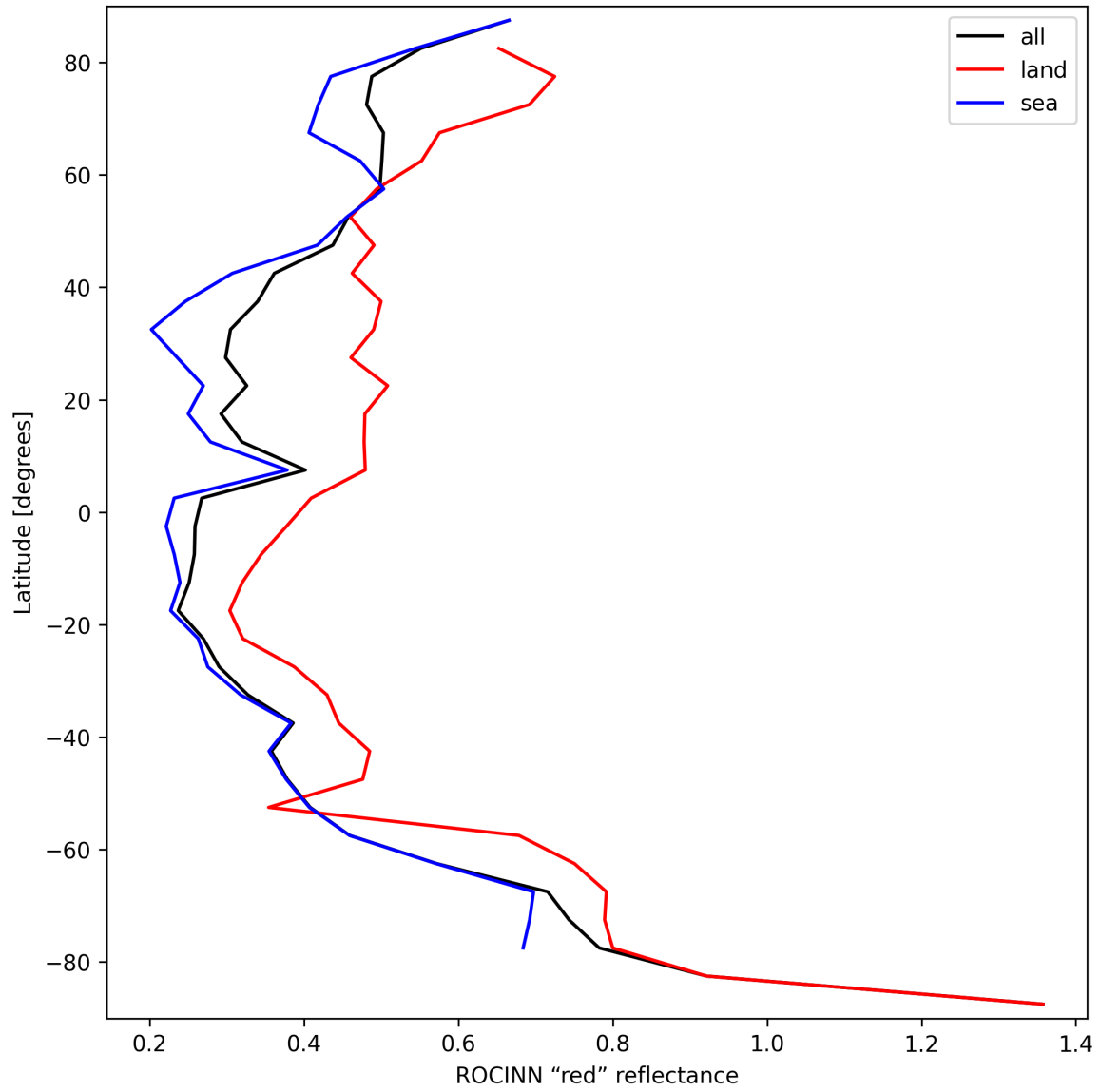
Figure 37: Zonal average of “ROCINN “red” reflectance” for 2024-09-12 to 2024-09-14.
