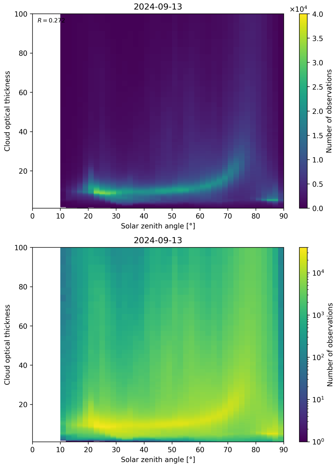
Figure 103: Scatter density plot of “Solar zenith angle” against “Cloud optical thickness” for 2024-09-12 to 2024-09-14.
