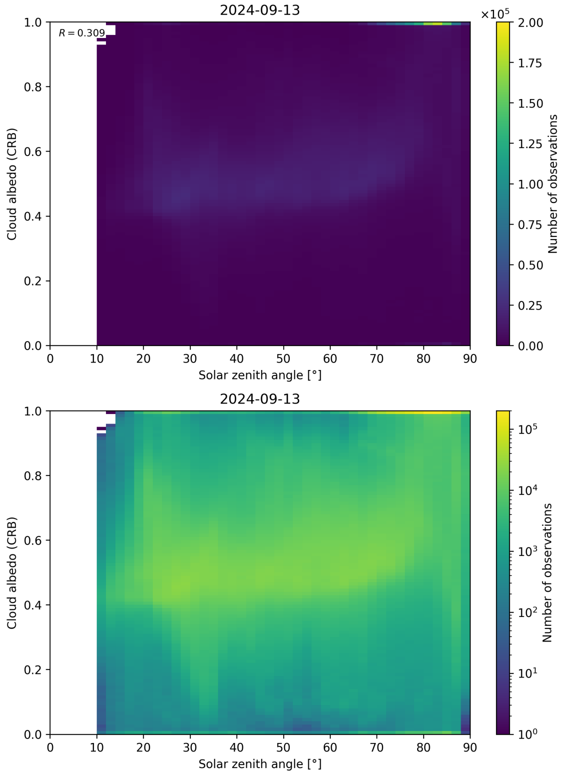
Figure 98: Scatter density plot of “Solar zenith angle” against “Cloud albedo (CRB)” for 2024-09-12 to 2024-09-14.
