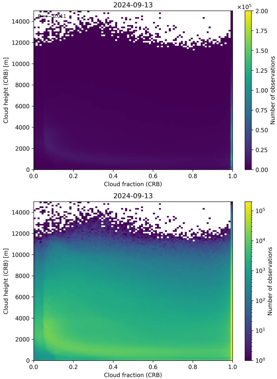
Figure 79: Scatter density plot of “Cloud fraction (CRB)” against “Cloud height (CRB)” for 2024-09-12 to 2024-09-14.
