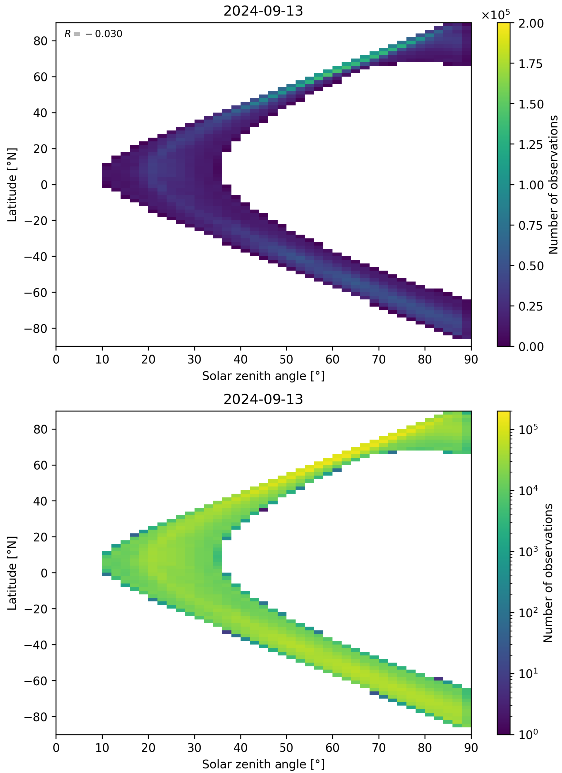
Figure 105: Scatter density plot of “Solar zenith angle” against “Latitude” for 2024-09-12 to 2024-09-14.
