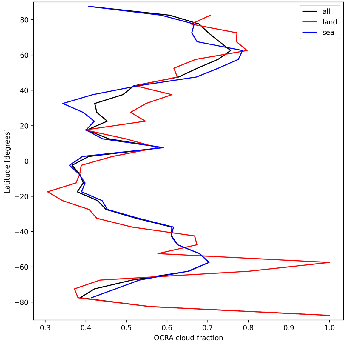
Figure 34: Zonal average of “OCRA cloud fraction” for 2024-09-12 to 2024-09-14.
