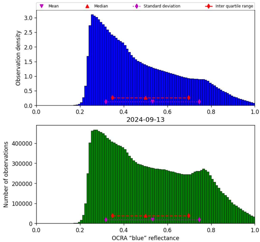
Figure 51: Histogram of “OCRA “blue” reflectance” for 2024-09-12 to 2024-09-14
