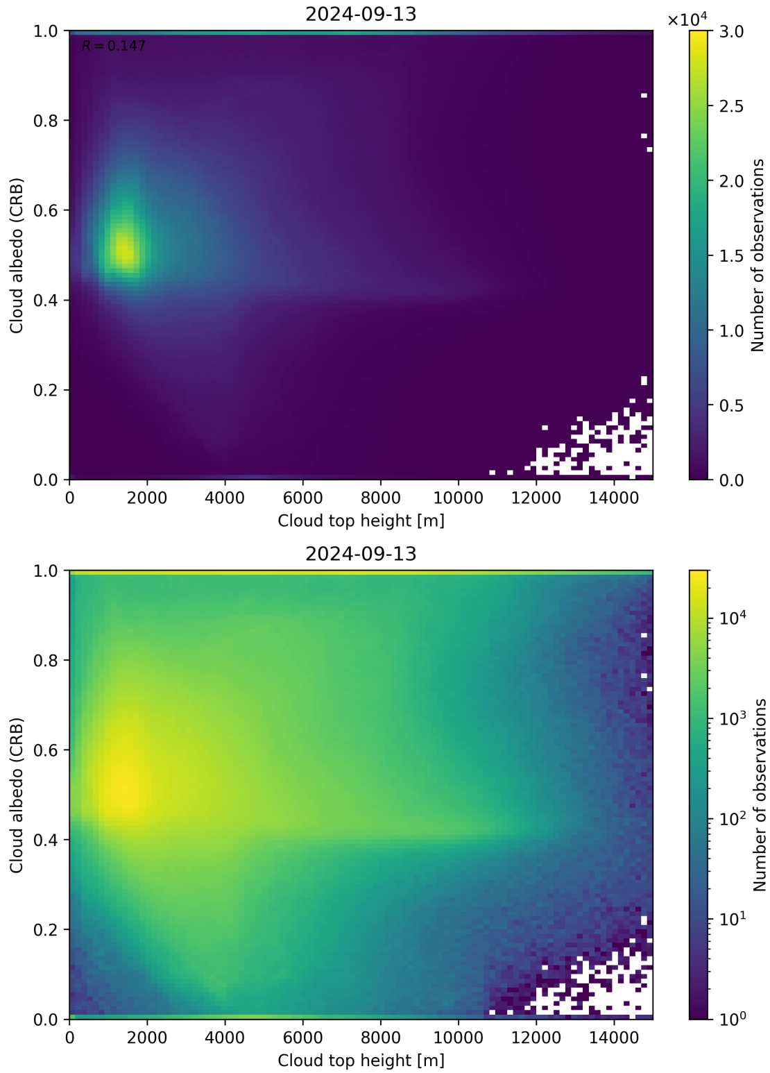
Figure 86: Scatter density plot of “Cloud top height” against “Cloud albedo (CRB)” for 2024-09-12 to 2024-09-14.
