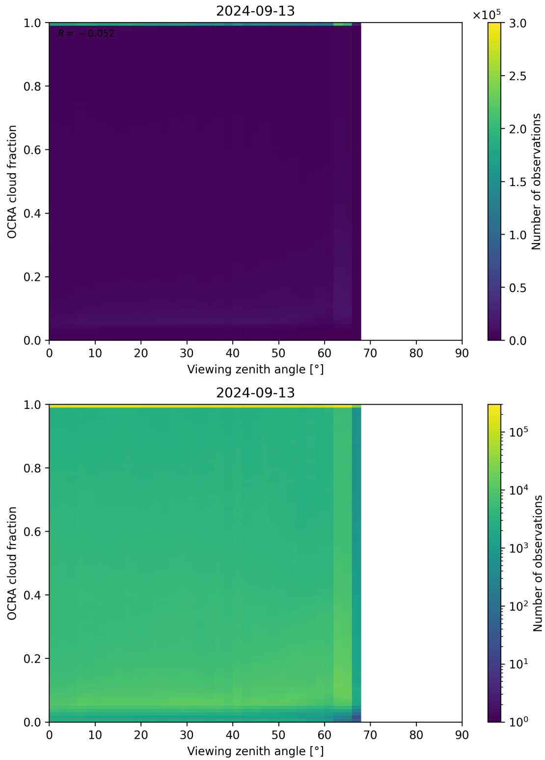
Figure 108: Scatter density plot of “Viewing zenith angle” against “OCRA cloud fraction” for 2024-09-12 to 2024-09-14.
