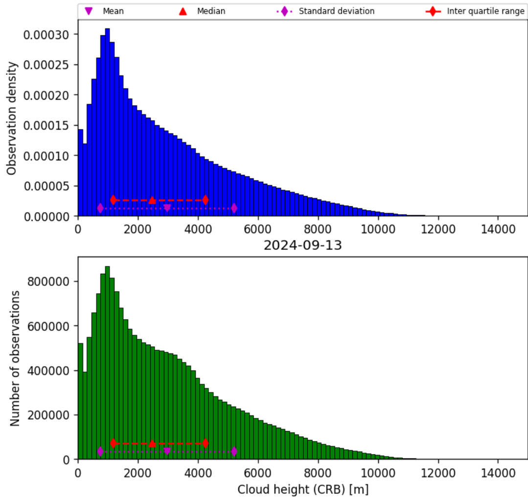
Figure 43: Histogram of “Cloud height (CRB)” for 2024-09-12 to 2024-09-14
