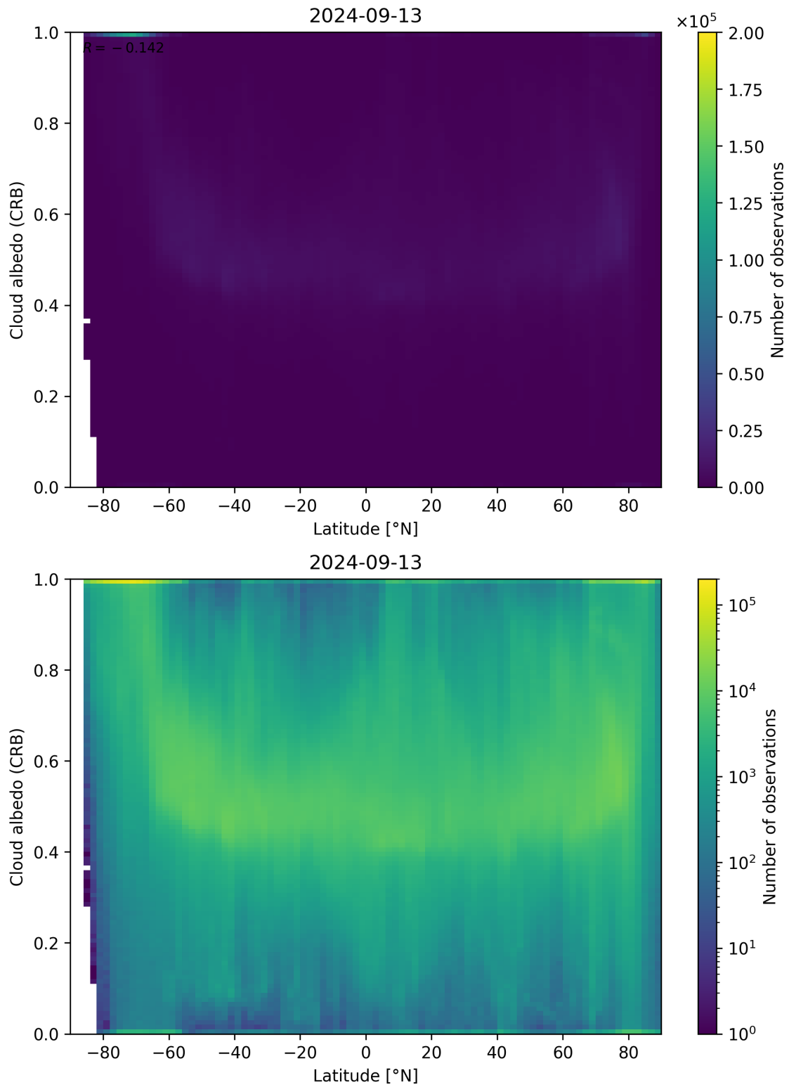
Figure 91: Scatter density plot of “Latitude” against “Cloud albedo (CRB)” for 2024-09-12 to 2024-09-14.
