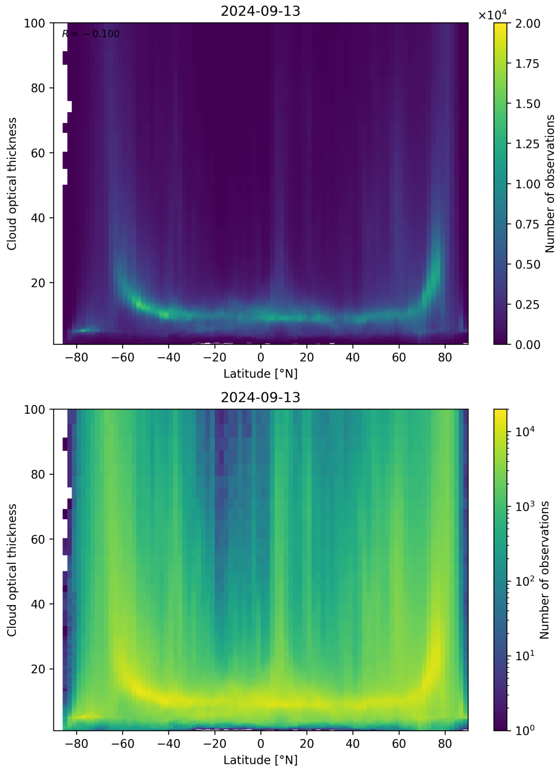
Figure 96: Scatter density plot of “Latitude” against “Cloud optical thickness” for 2024-09-12 to 2024-09-14.
