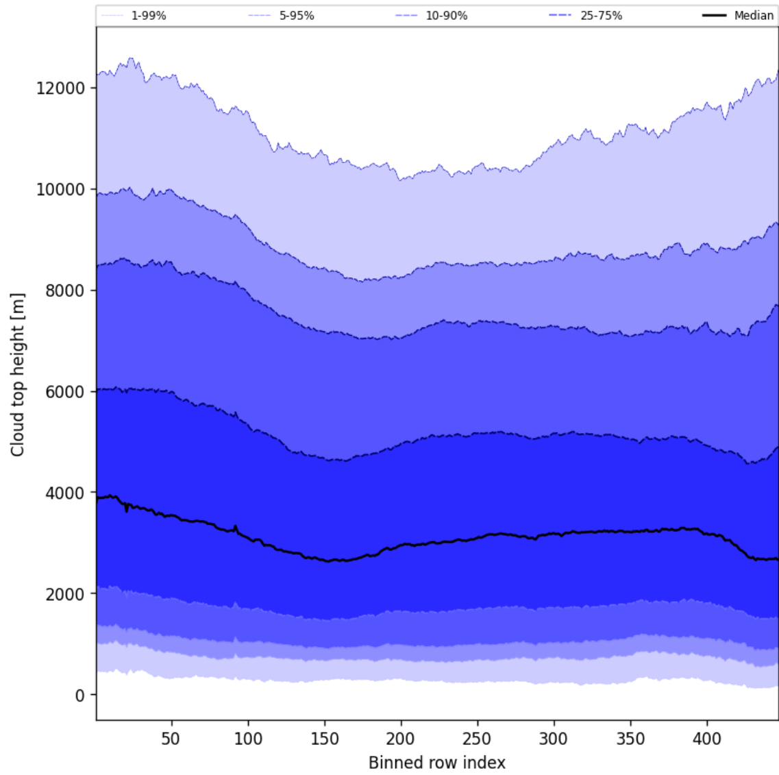
Figure 56: Along track statistics of “Cloud top height” for 2024-09-12 to 2024-09-14
