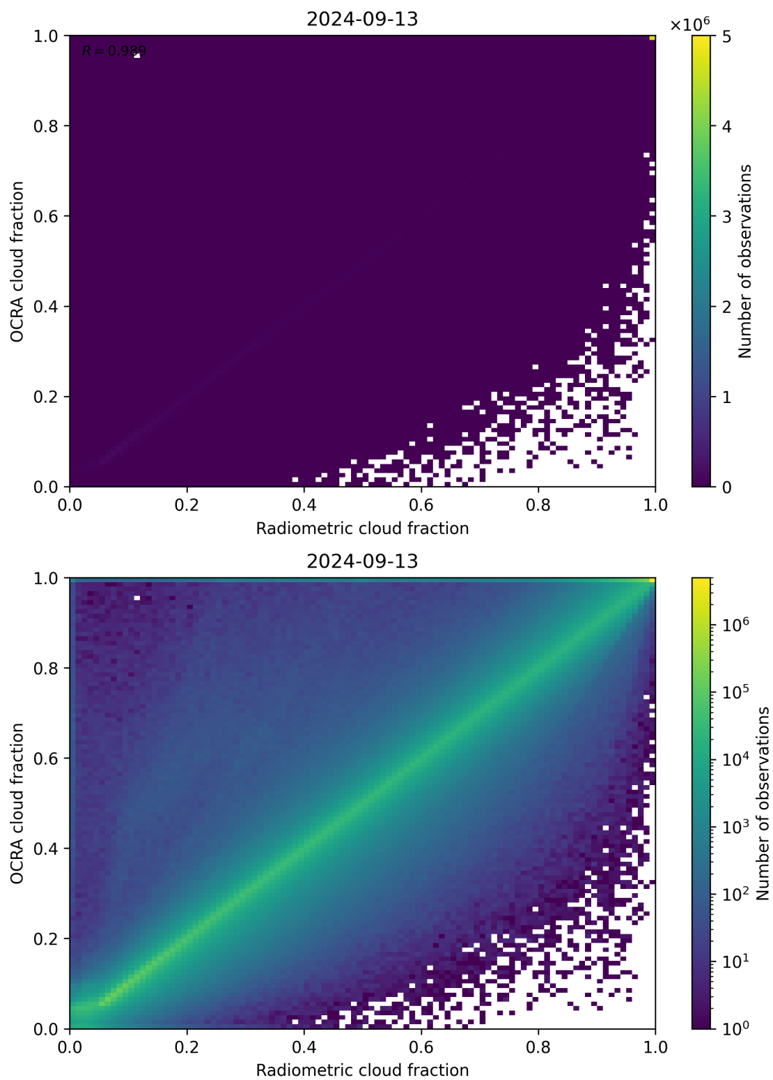
Figure 72: Scatter density plot of “Radiometric cloud fraction” against “OCRA cloud fraction” for 2024-09-12 to 2024-09-14.
