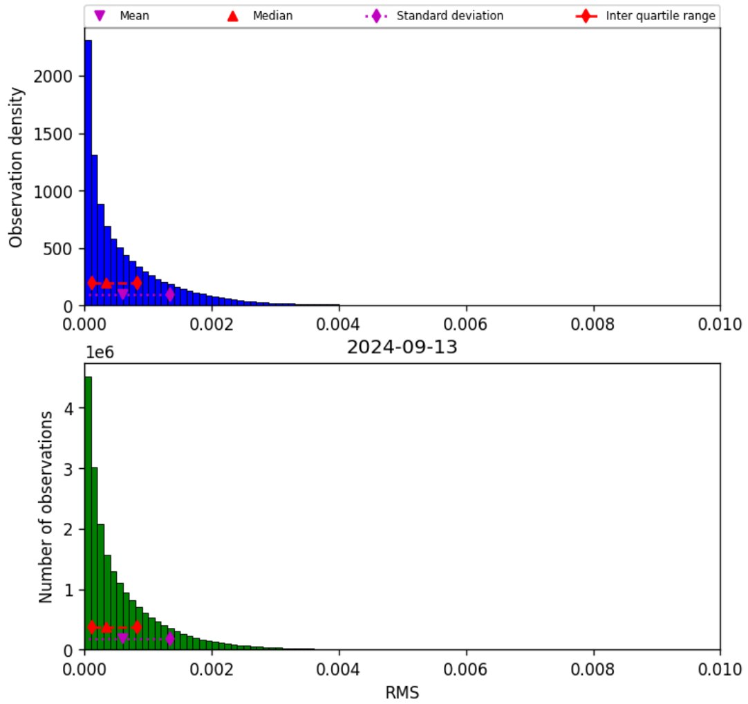
Figure 47: Histogram of “RMS” for 2024-09-12 to 2024-09-14
