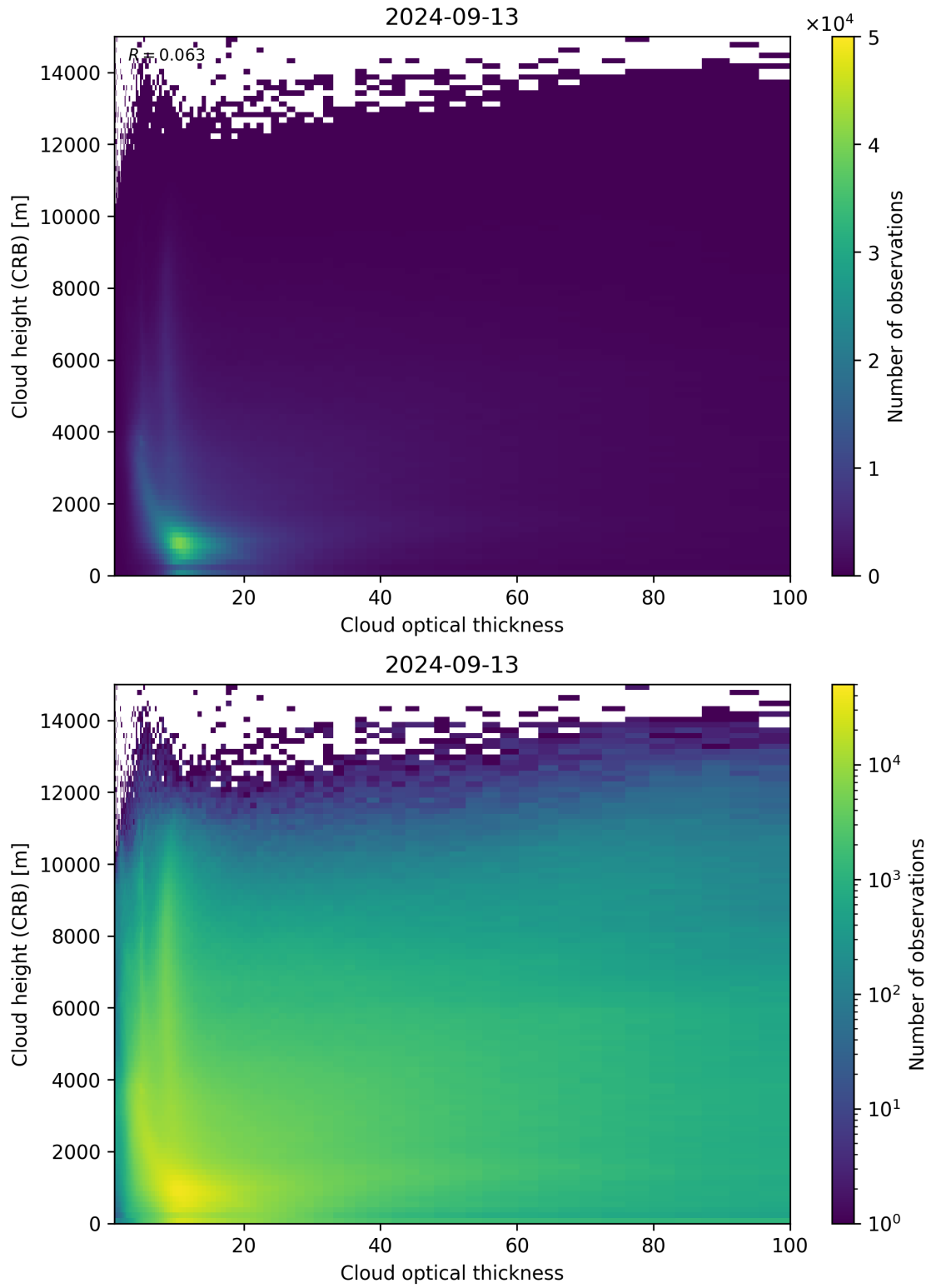
Figure 85: Scatter density plot of “Cloud optical thickness” against “Cloud height (CRB)” for 2024-09-12 to 2024-09-14.
