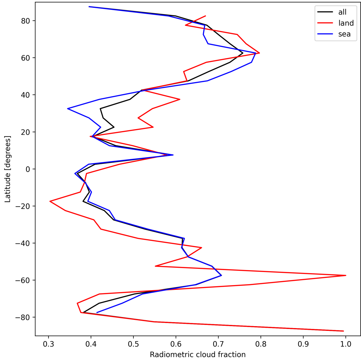
Figure 23: Zonal average of “Radiometric cloud fraction” for 2024-09-12 to 2024-09-14.
