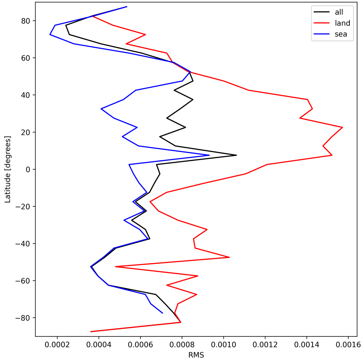
Figure 31: Zonal average of “RMS” for 2024-09-12 to 2024-09-14.
