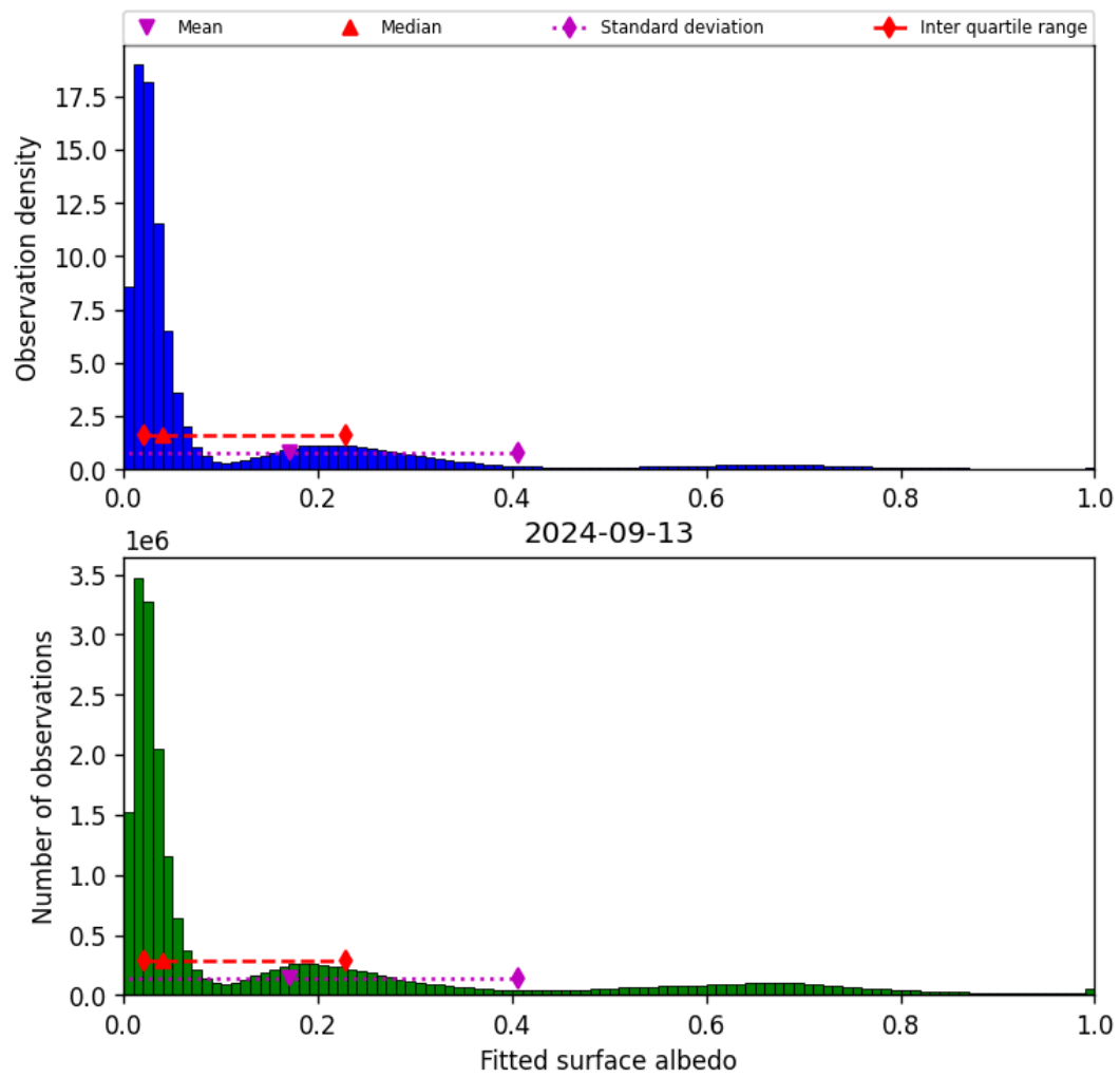
Figure 45: Histogram of “Fitted surface albedo” for 2024-09-12 to 2024-09-14
