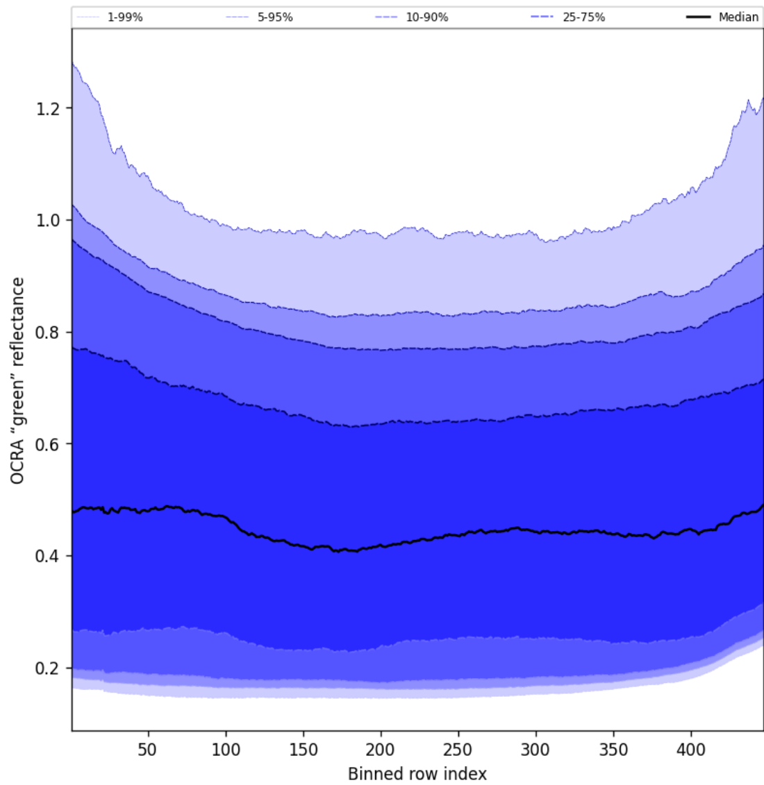
Figure 68: Along track statistics of “OCRA “green” reflectance” for 2024-09-12 to 2024-09-14
