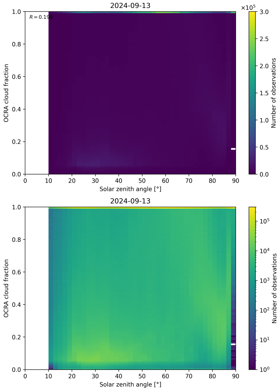
Figure 100: Scatter density plot of “Solar zenith angle” against “OCRA cloud fraction” for 2024-09-12 to 2024-09-14.
