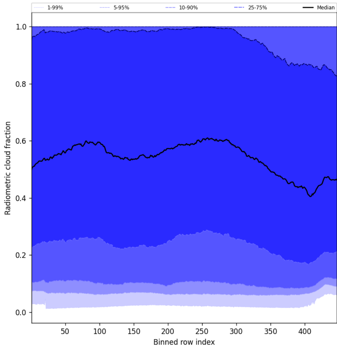
Figure 55: Along track statistics of “Radiometric cloud fraction” for 2024-09-12 to 2024-09-14
