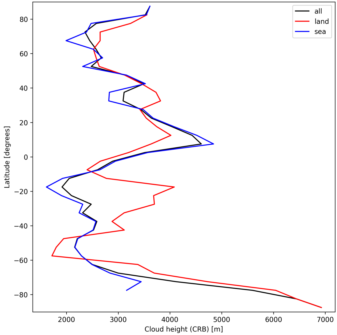
Figure 27: Zonal average of “Cloud height (CRB)” for 2024-09-12 to 2024-09-14.
