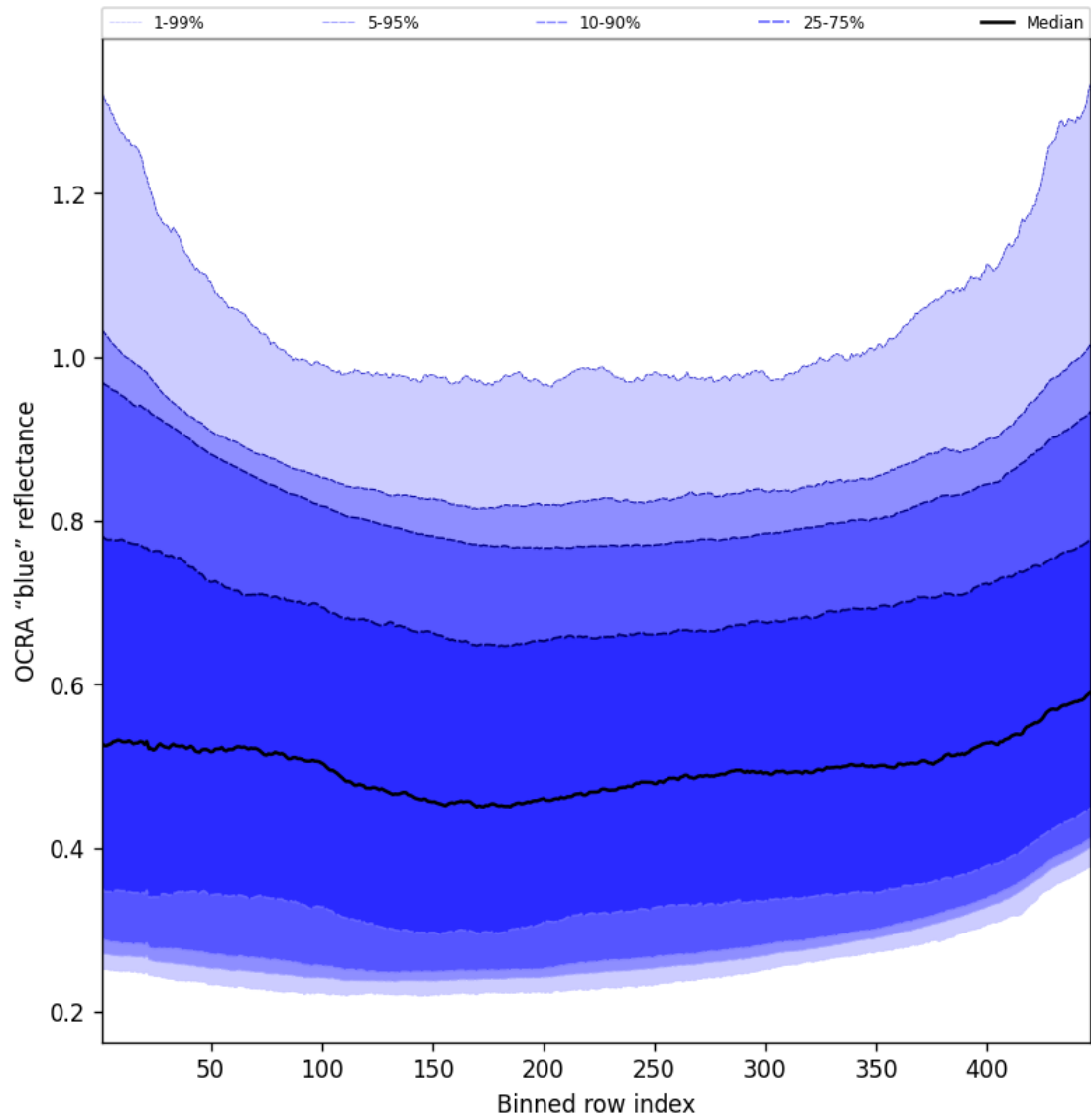
Figure 67: Along track statistics of “OCRA “blue” reflectance” for 2024-09-12 to 2024-09-14
