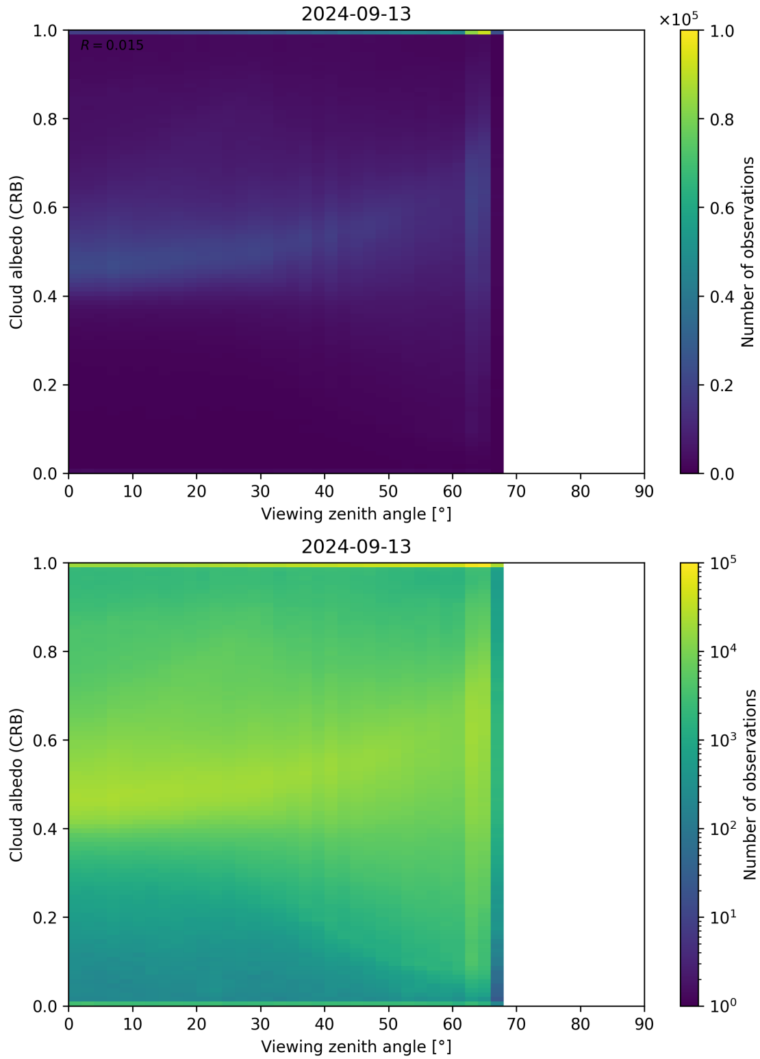
Figure 106: Scatter density plot of “Viewing zenith angle” against “Cloud albedo (CRB)” for 2024-09-12 to 2024-09-14.
