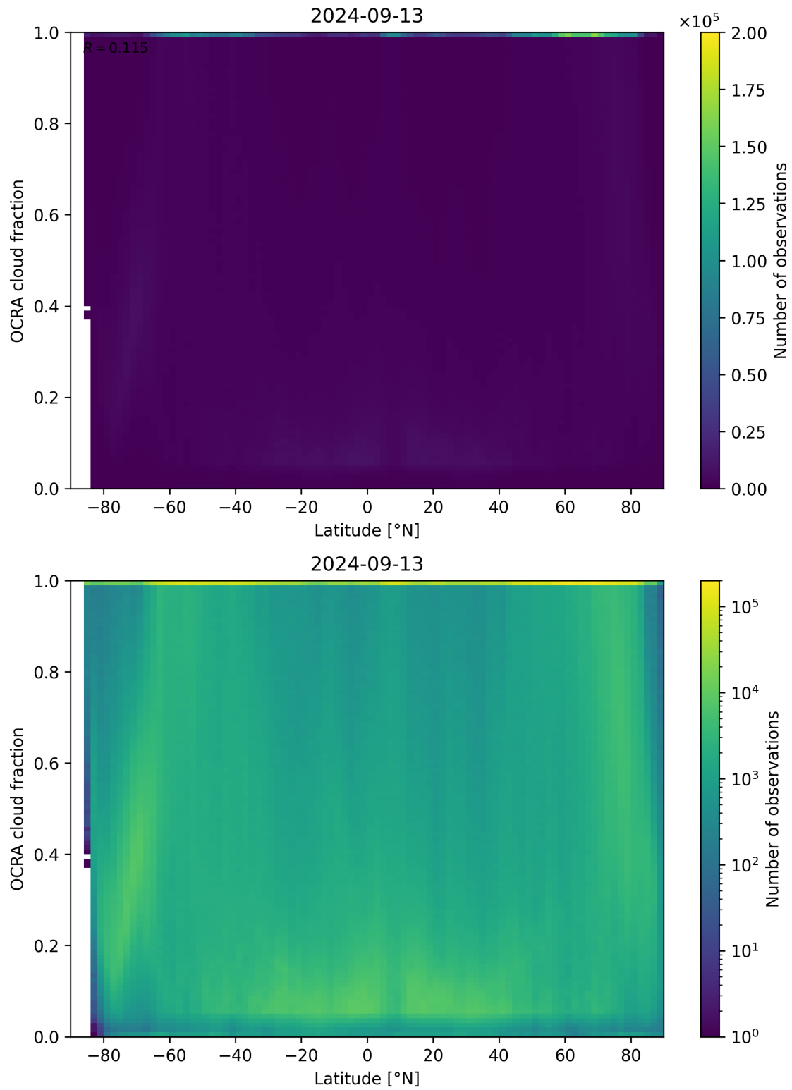
Figure 93: Scatter density plot of “Latitude” against “OCRA cloud fraction” for 2024-09-12 to 2024-09-14.
