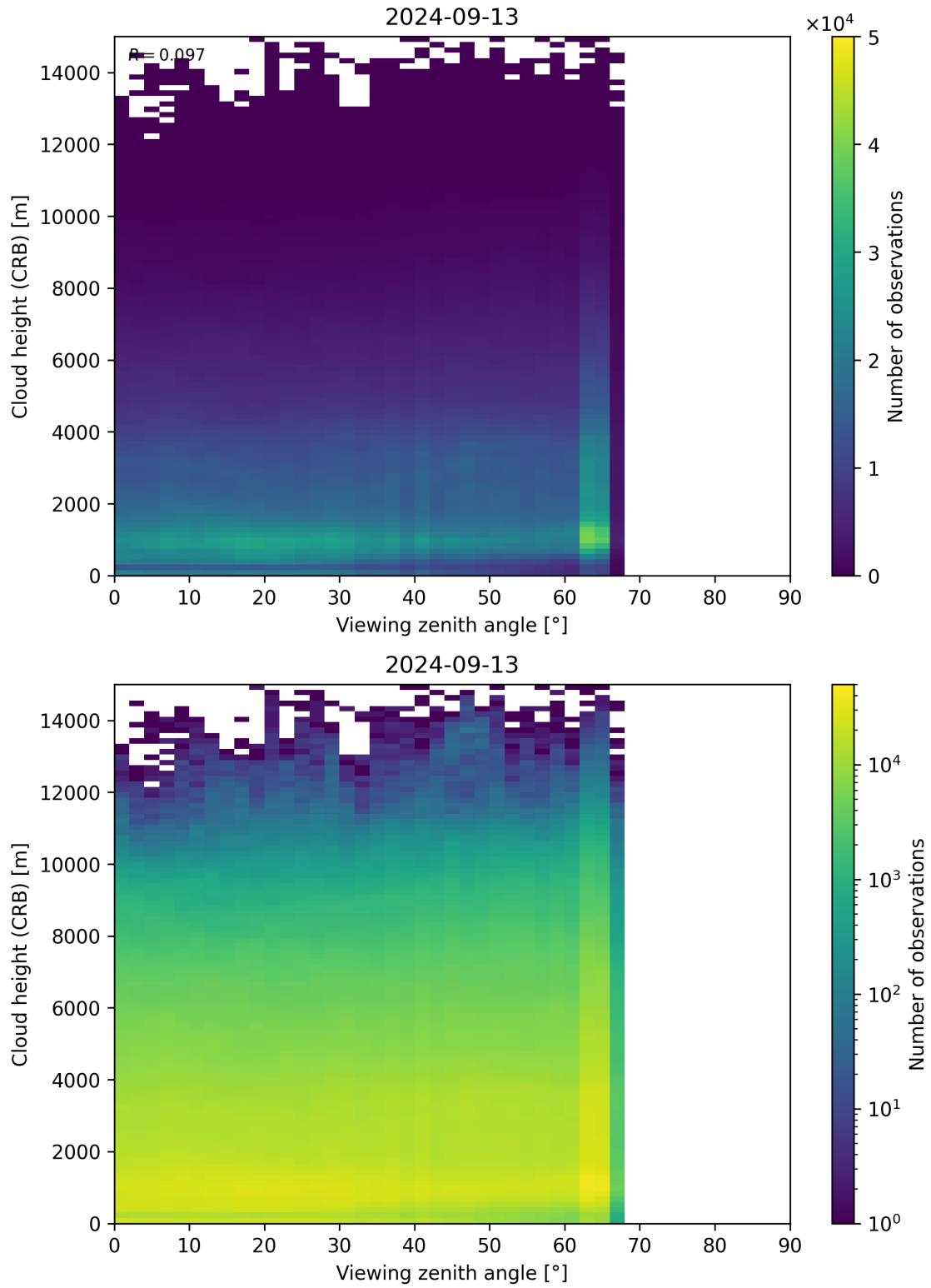
Figure 110: Scatter density plot of “Viewing zenith angle” against “Cloud height (CRB)” for 2024-09-12 to 2024-09-14.
