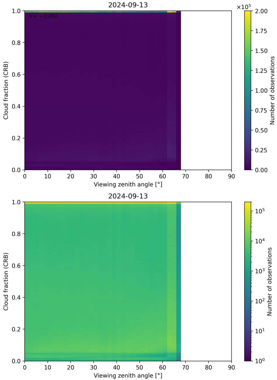
Figure 109: Scatter density plot of “Viewing zenith angle” against “Cloud fraction (CRB)” for 2024-09-12 to 2024-09-14.
