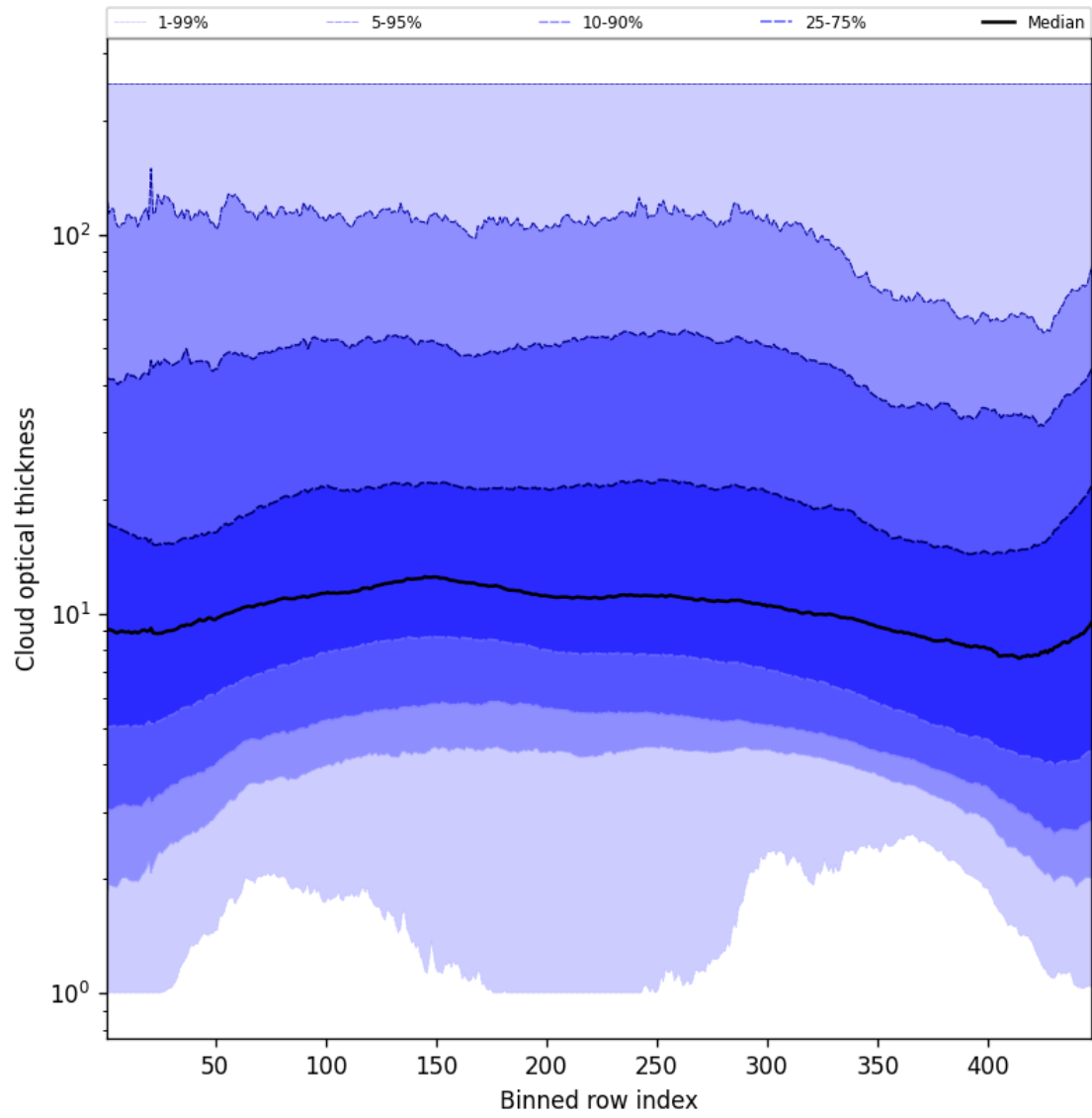
Figure 57: Along track statistics of “Cloud optical thickness” for 2024-09-12 to 2024-09-14
