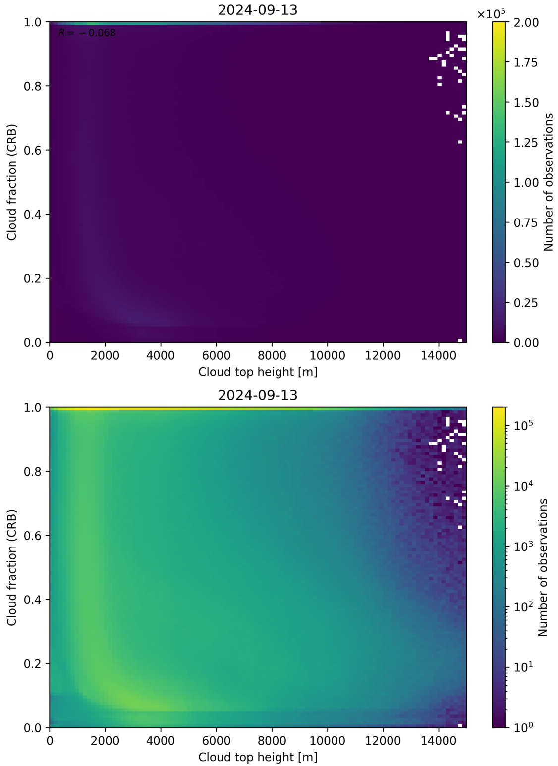
Figure 88: Scatter density plot of “Cloud top height” against “Cloud fraction (CRB)” for 2024-09-12 to 2024-09-14.
