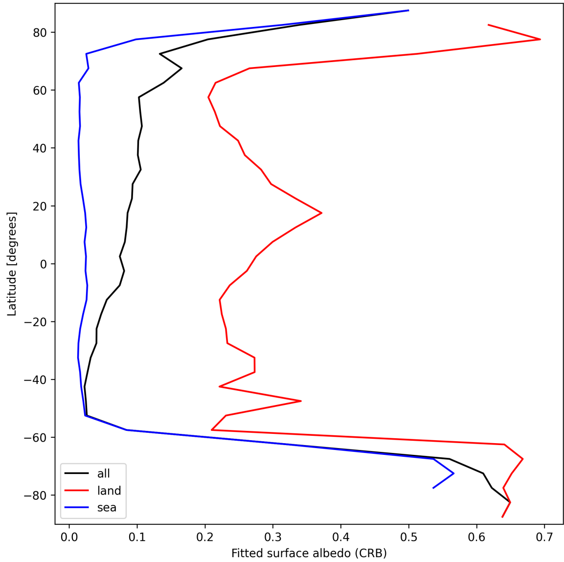
Figure 30: Zonal average of “Fitted surface albedo (CRB)” for 2024-09-12 to 2024-09-14.
