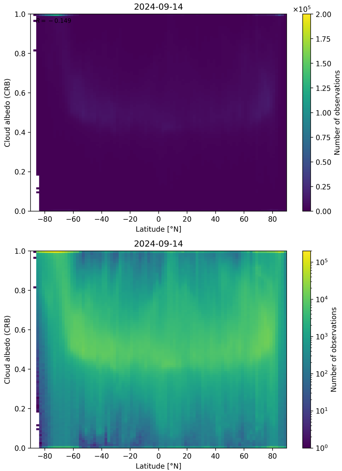
Figure 91: Scatter density plot of “Latitude” against “Cloud albedo (CRB)” for 2024-09-13 to 2024-09-15.
