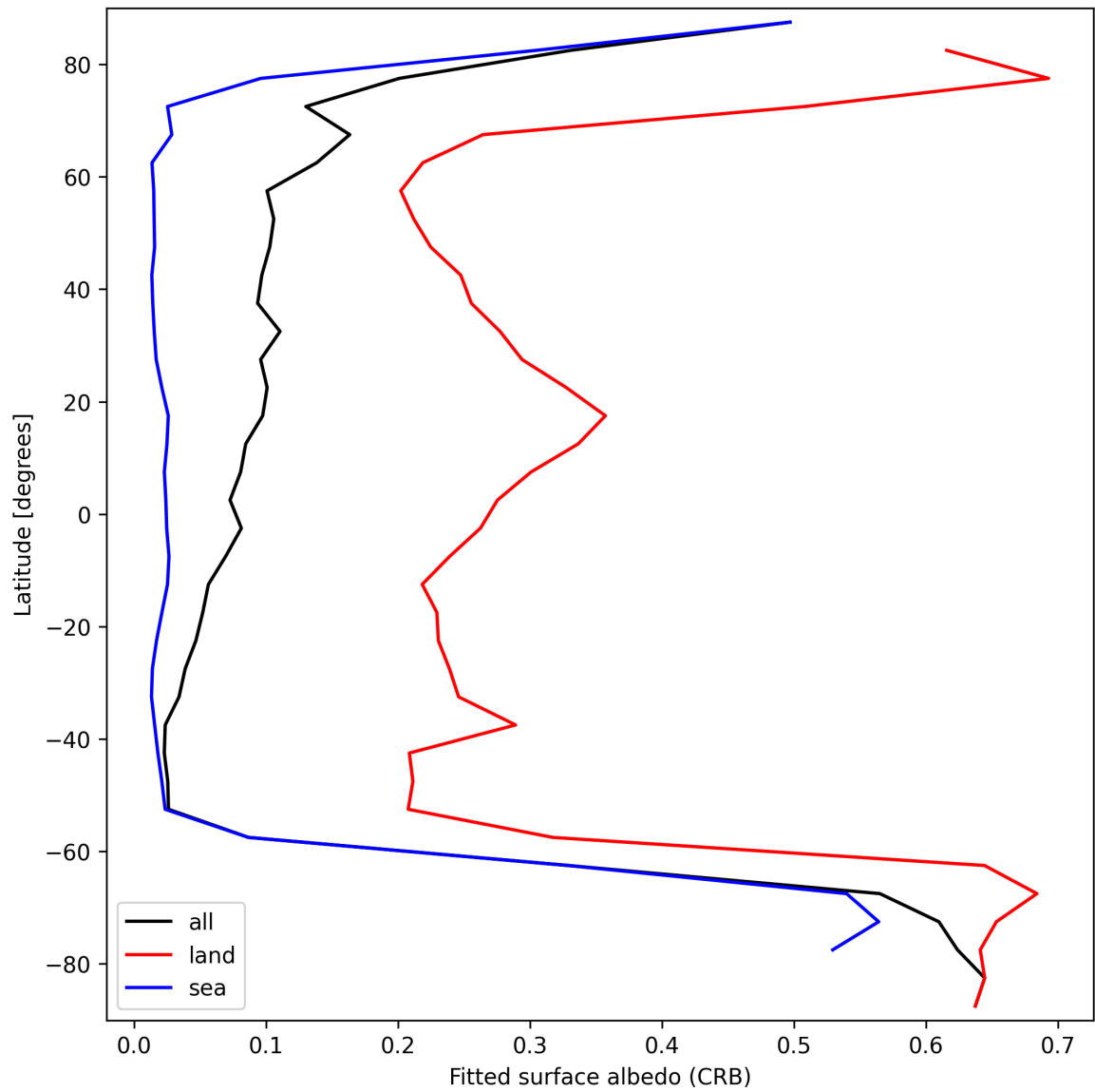
Figure 30: Zonal average of “Fitted surface albedo (CRB)” for 2024-09-13 to 2024-09-15.
