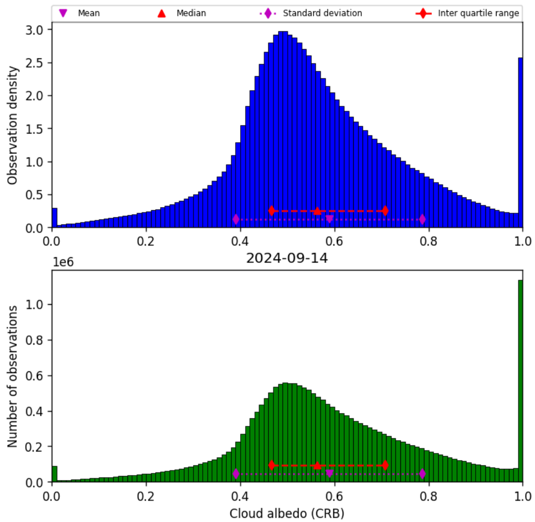
Figure 44: Histogram of “Cloud albedo (CRB)” for 2024-09-13 to 2024-09-15
