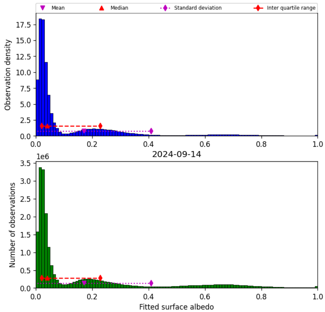
Figure 45: Histogram of “Fitted surface albedo” for 2024-09-13 to 2024-09-15
