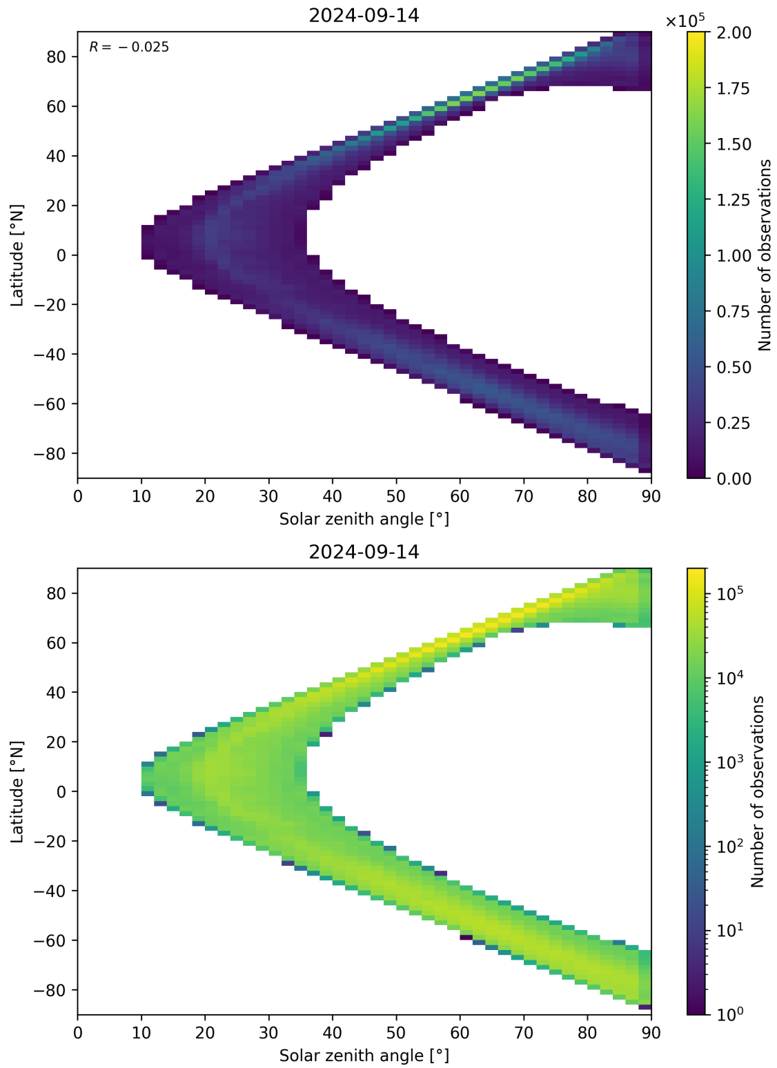
Figure 105: Scatter density plot of “Solar zenith angle” against “Latitude” for 2024-09-13 to 2024-09-15.
