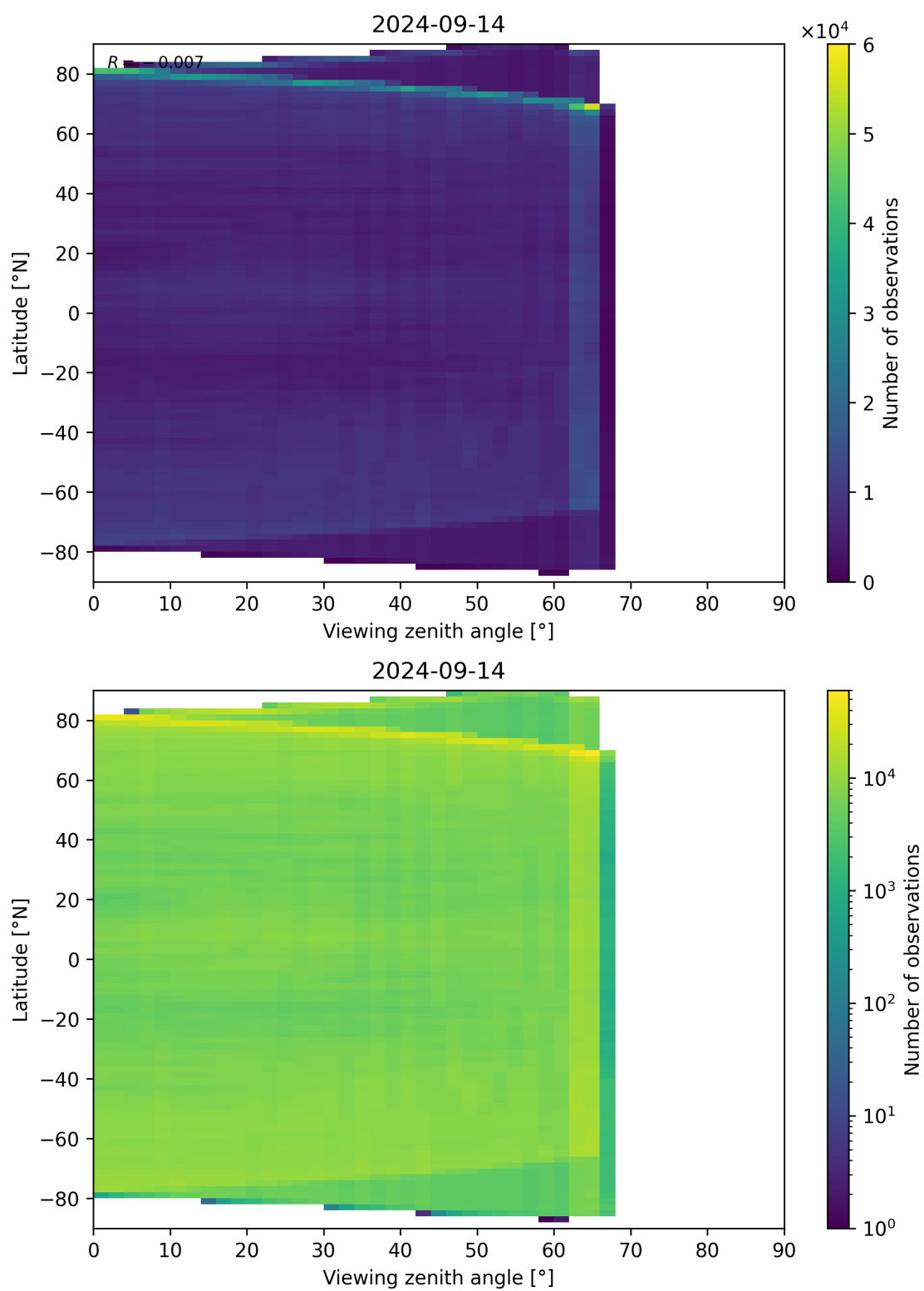
Figure 113: Scatter density plot of “Viewing zenith angle” against “Latitude” for 2024-09-13 to 2024-09-15.
