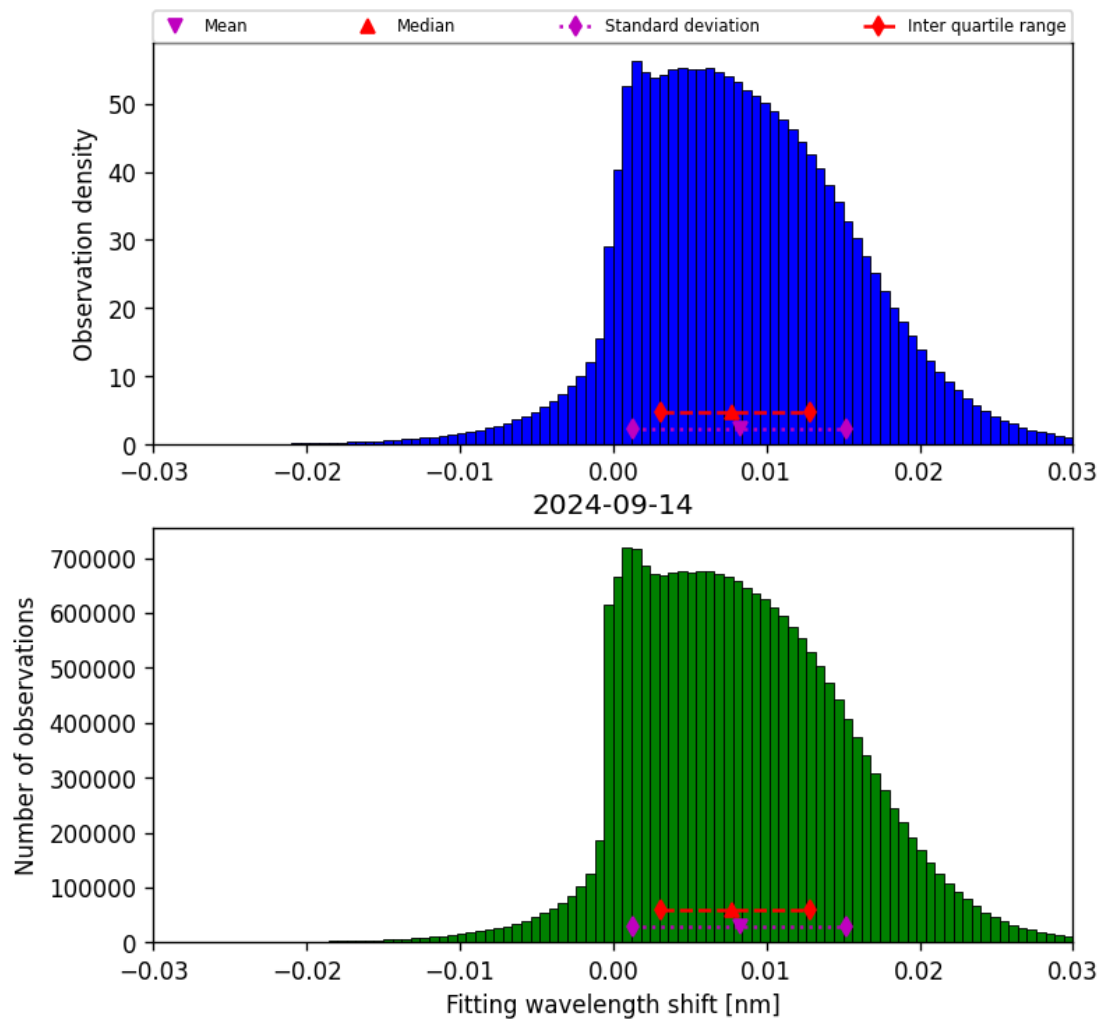
Figure 49: Histogram of “Fitting wavelength shift” for 2024-09-13 to 2024-09-15
