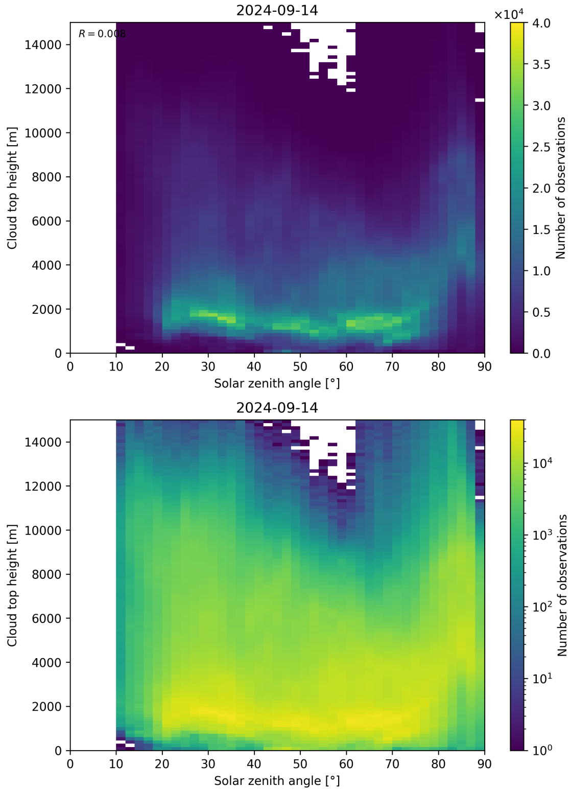
Figure 104: Scatter density plot of “Solar zenith angle” against “Cloud top height” for 2024-09-13 to 2024-09-15.
