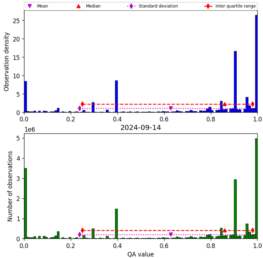
Figure 38: Histogram of “QA value” for 2024-09-13 to 2024-09-15
