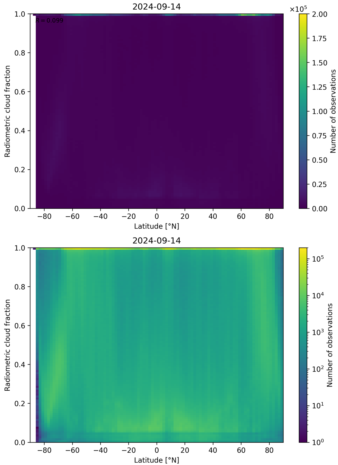
Figure 92: Scatter density plot of “Latitude” against “Radiometric cloud fraction” for 2024-09-13 to 2024-09-15.
