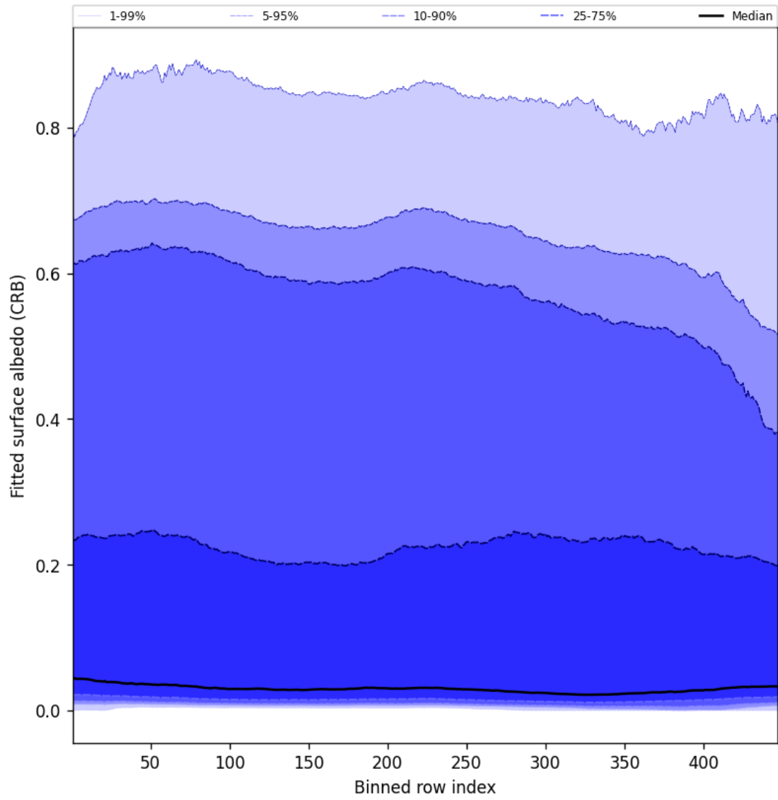
Figure 62: Along track statistics of “Fitted surface albedo (CRB)” for 2024-09-13 to 2024-09-15
