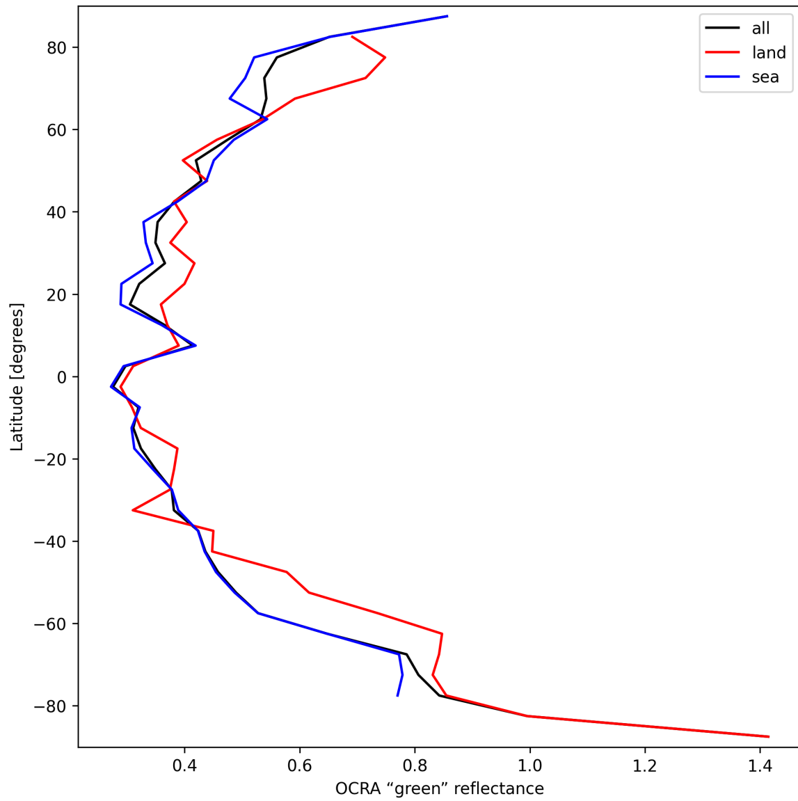
Figure 36: Zonal average of “OCRA “green” reflectance” for 2024-09-13 to 2024-09-15.
