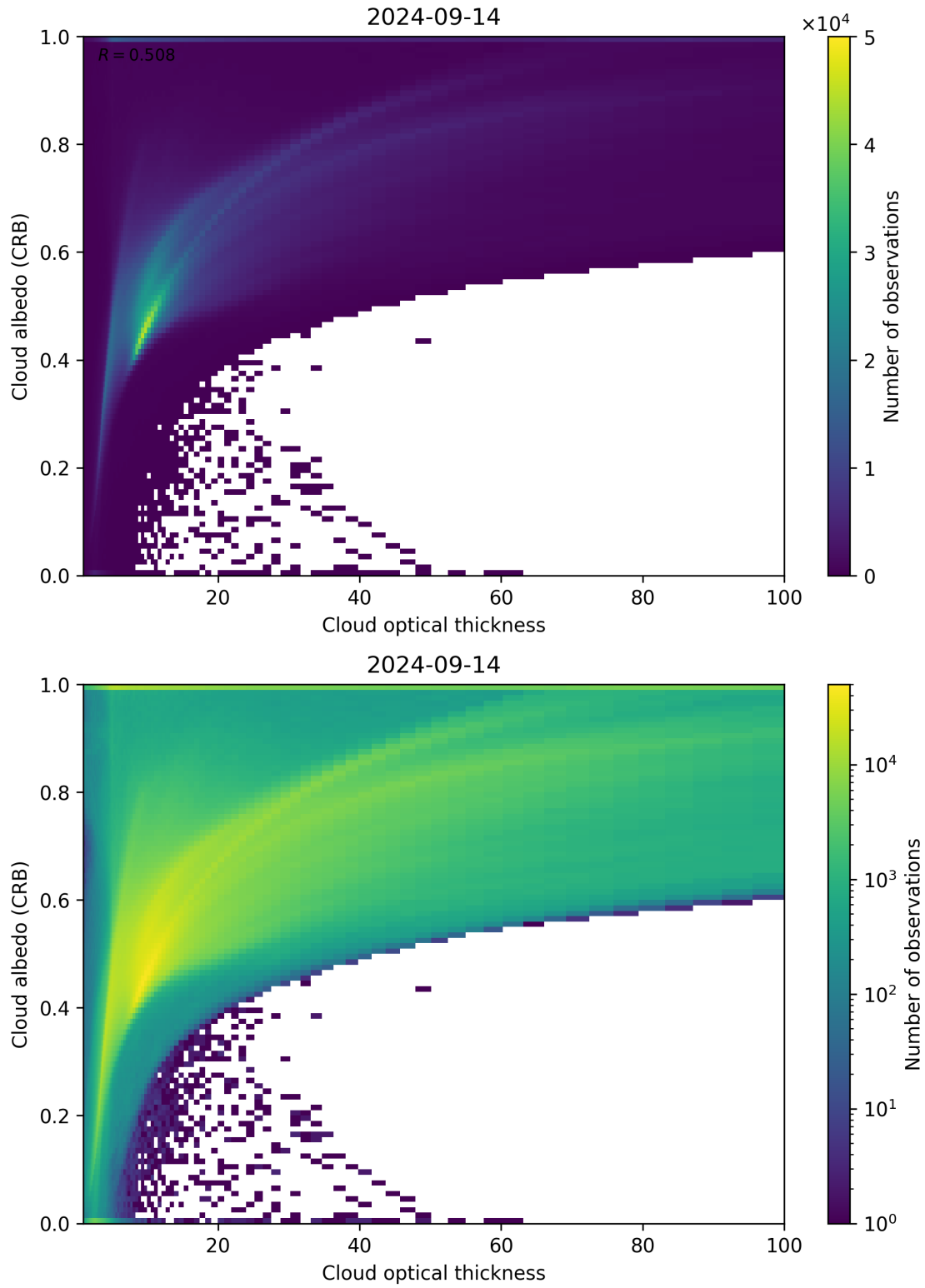
Figure 82: Scatter density plot of “Cloud optical thickness” against “Cloud albedo (CRB)” for 2024-09-13 to 2024-09-15.
