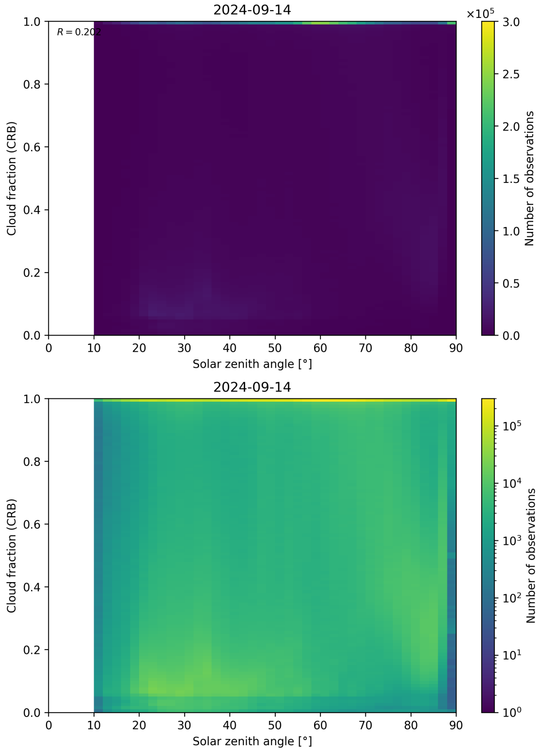
Figure 101: Scatter density plot of “Solar zenith angle” against “Cloud fraction (CRB)” for 2024-09-13 to 2024-09-15.
