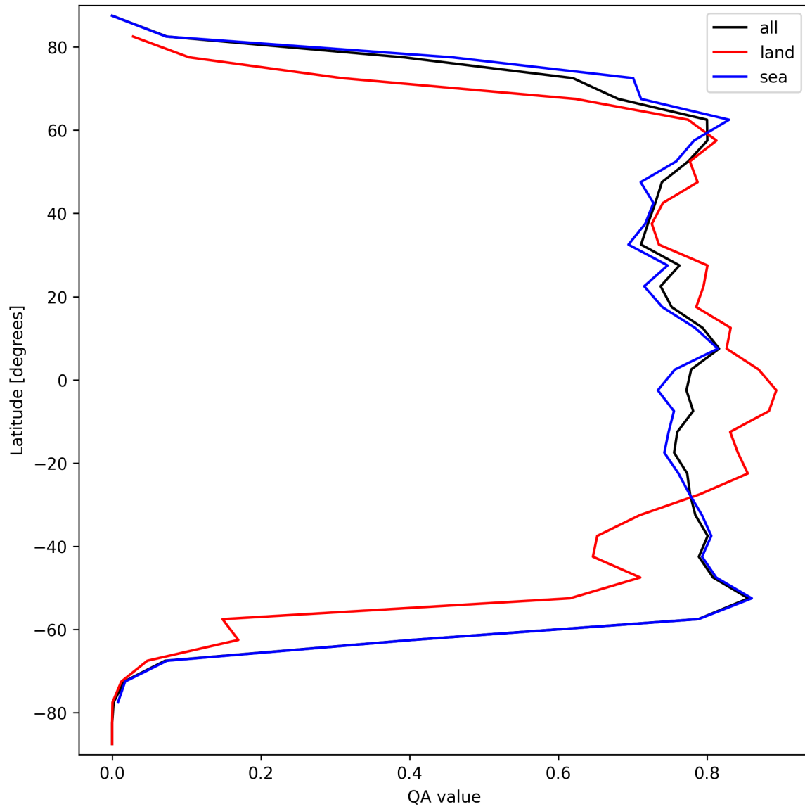
Figure 22: Zonal average of “QA value” for 2024-09-13 to 2024-09-15.
