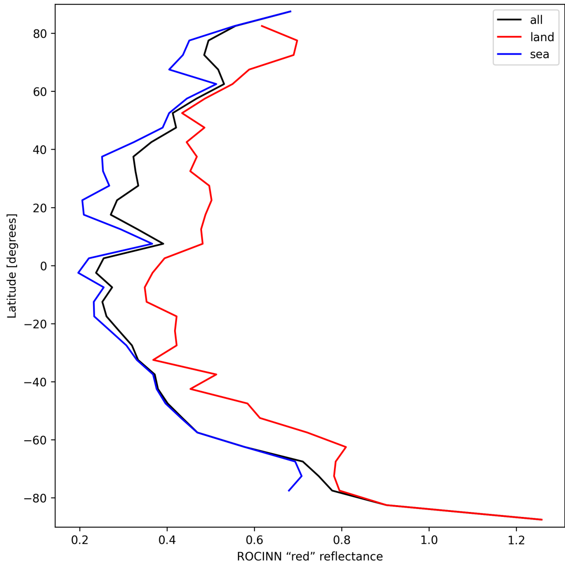
Figure 37: Zonal average of “ROCINN “red” reflectance” for 2024-09-13 to 2024-09-15.
