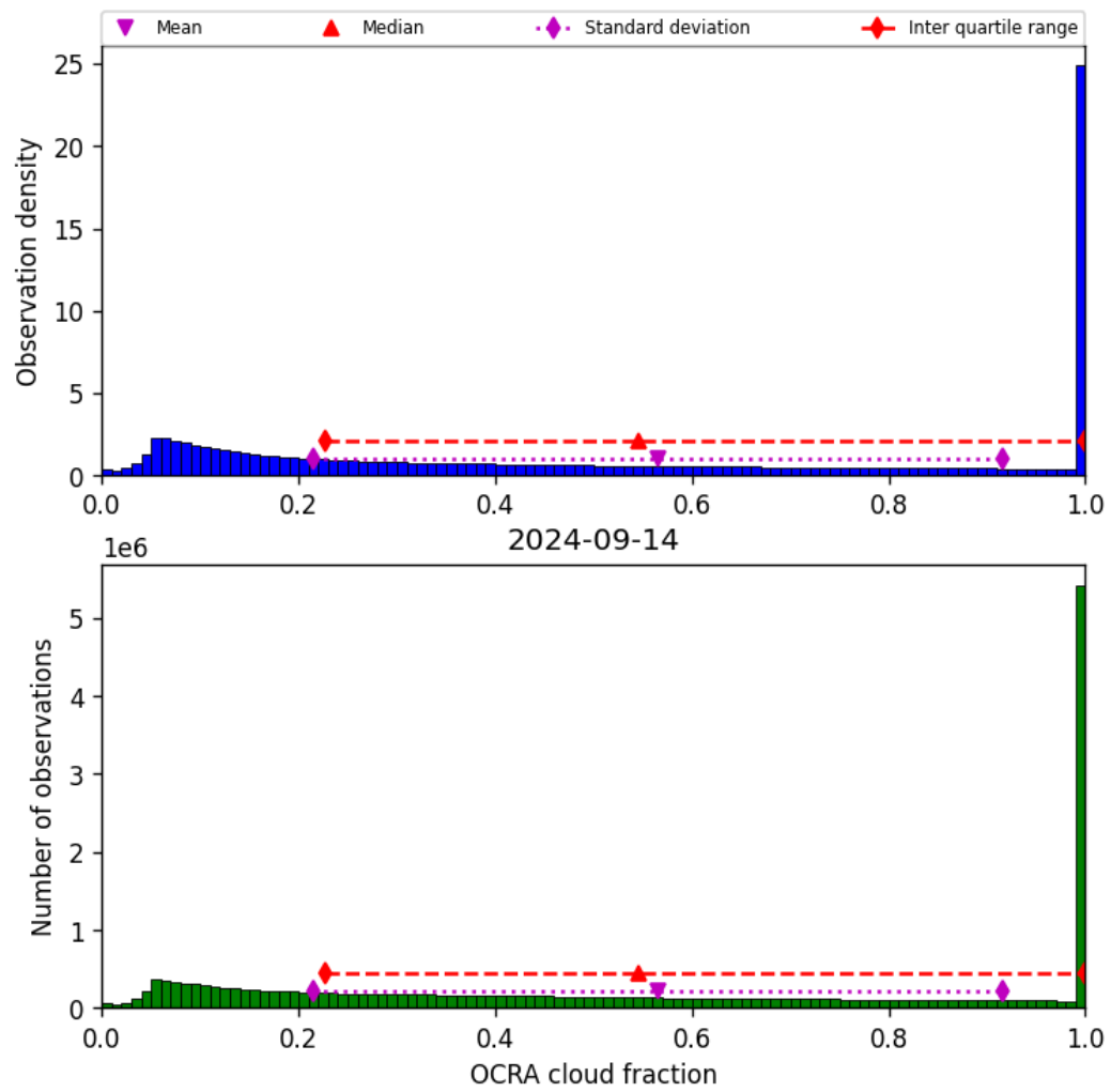
Figure 50: Histogram of “OCRA cloud fraction” for 2024-09-13 to 2024-09-15
