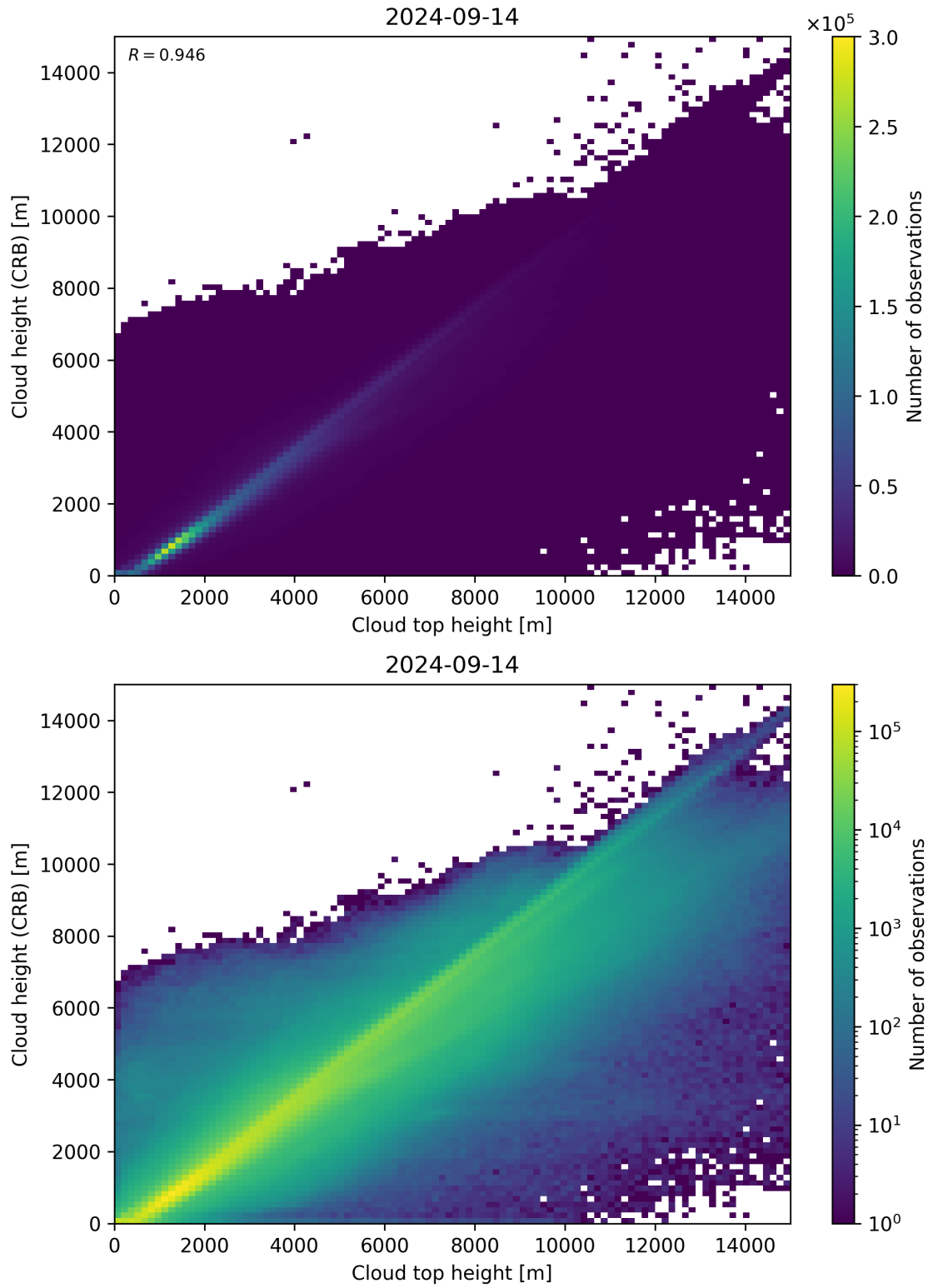
Figure 89: Scatter density plot of “Cloud top height” against “Cloud height (CRB)” for 2024-09-13 to 2024-09-15.
