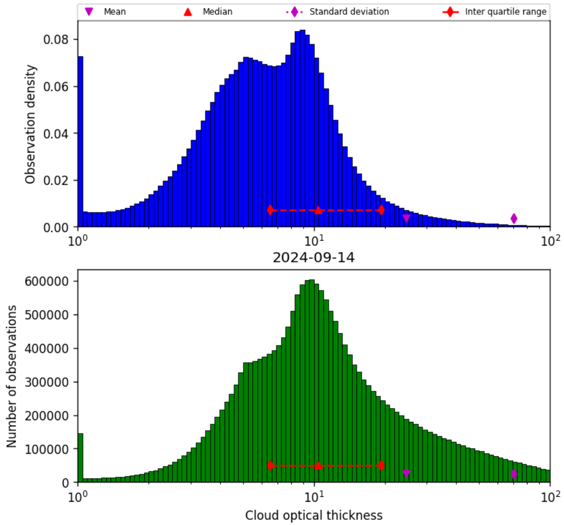
Figure 41: Histogram of “Cloud optical thickness” for 2024-09-13 to 2024-09-15
