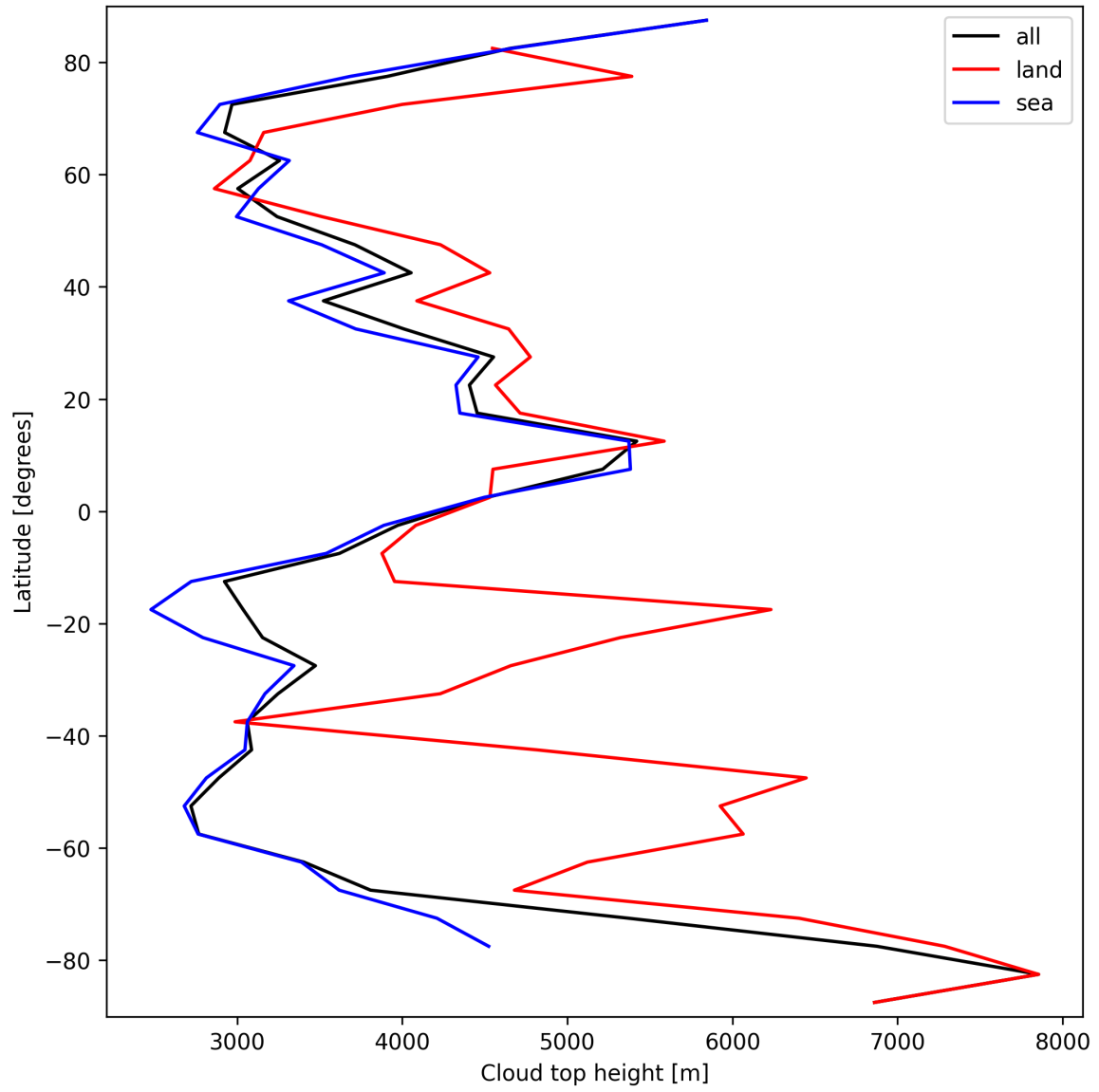
Figure 24: Zonal average of “Cloud top height” for 2024-09-13 to 2024-09-15.
