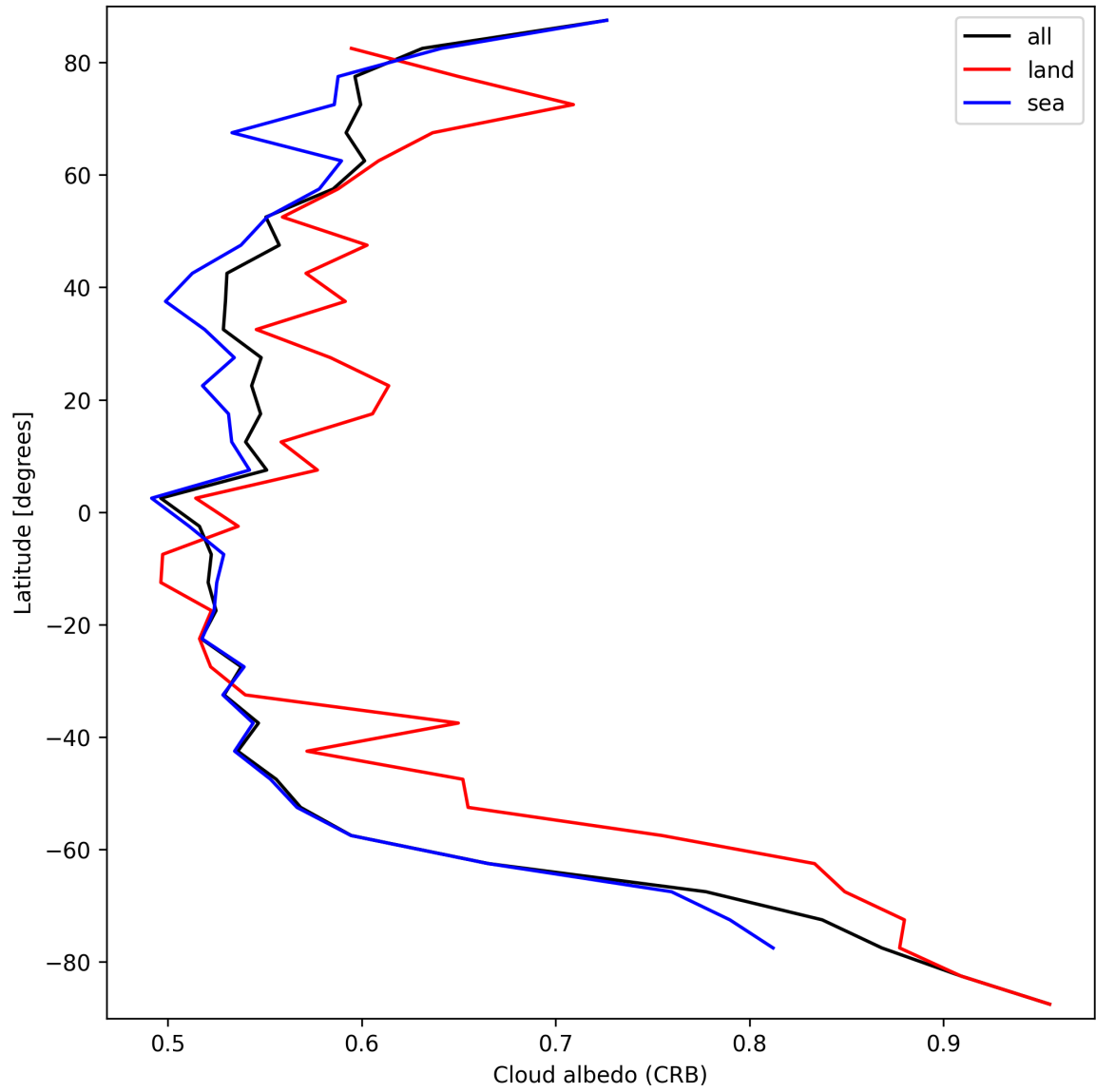
Figure 28: Zonal average of “Cloud albedo (CRB)” for 2024-09-13 to 2024-09-15.
