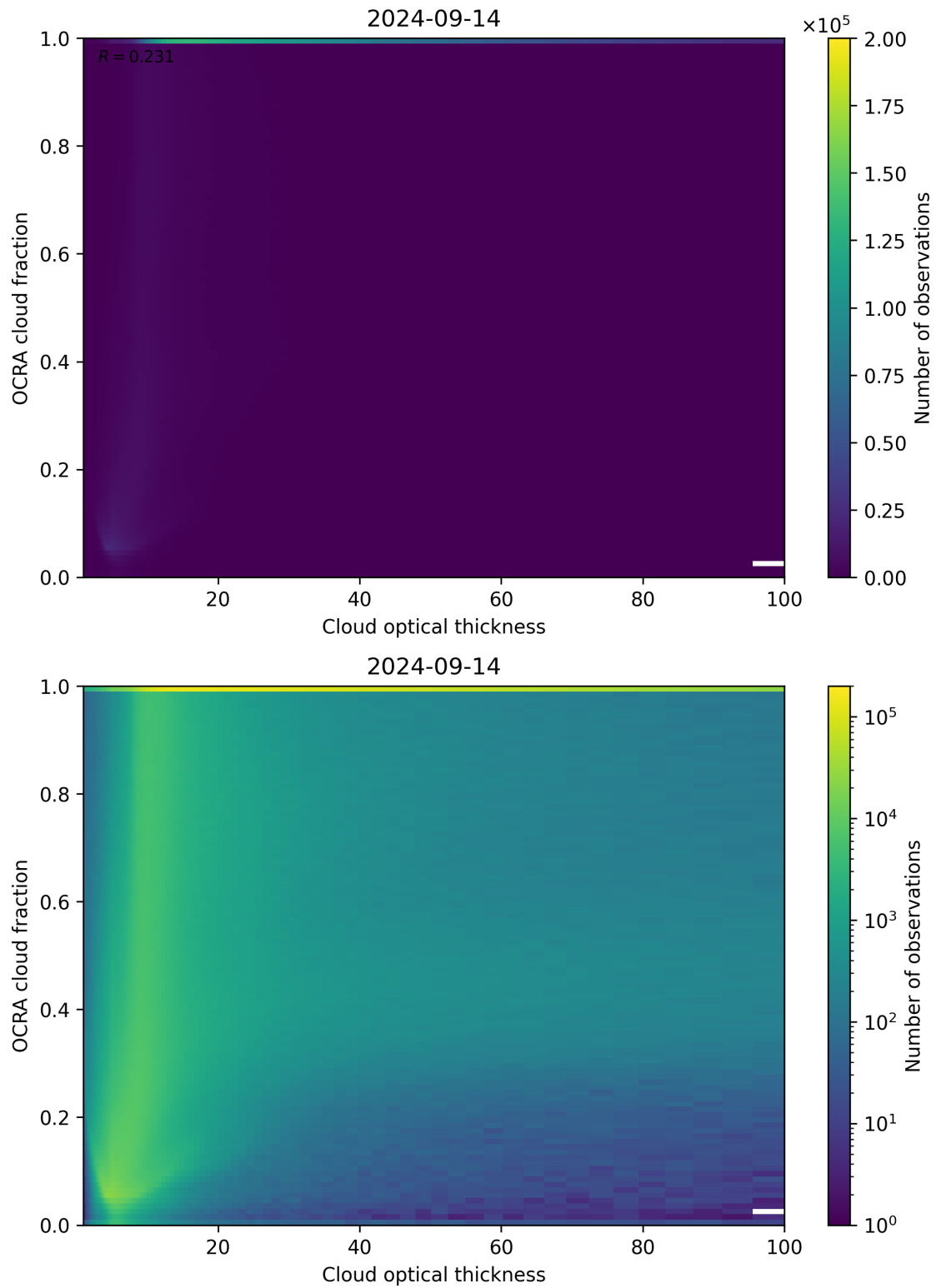
Figure 83: Scatter density plot of “Cloud optical thickness” against “OCRA cloud fraction” for 2024-09-13 to 2024-09-15.
