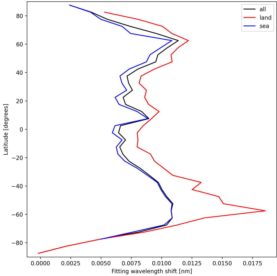
Figure 33: Zonal average of “Fitting wavelength shift” for 2024-09-13 to 2024-09-15.
