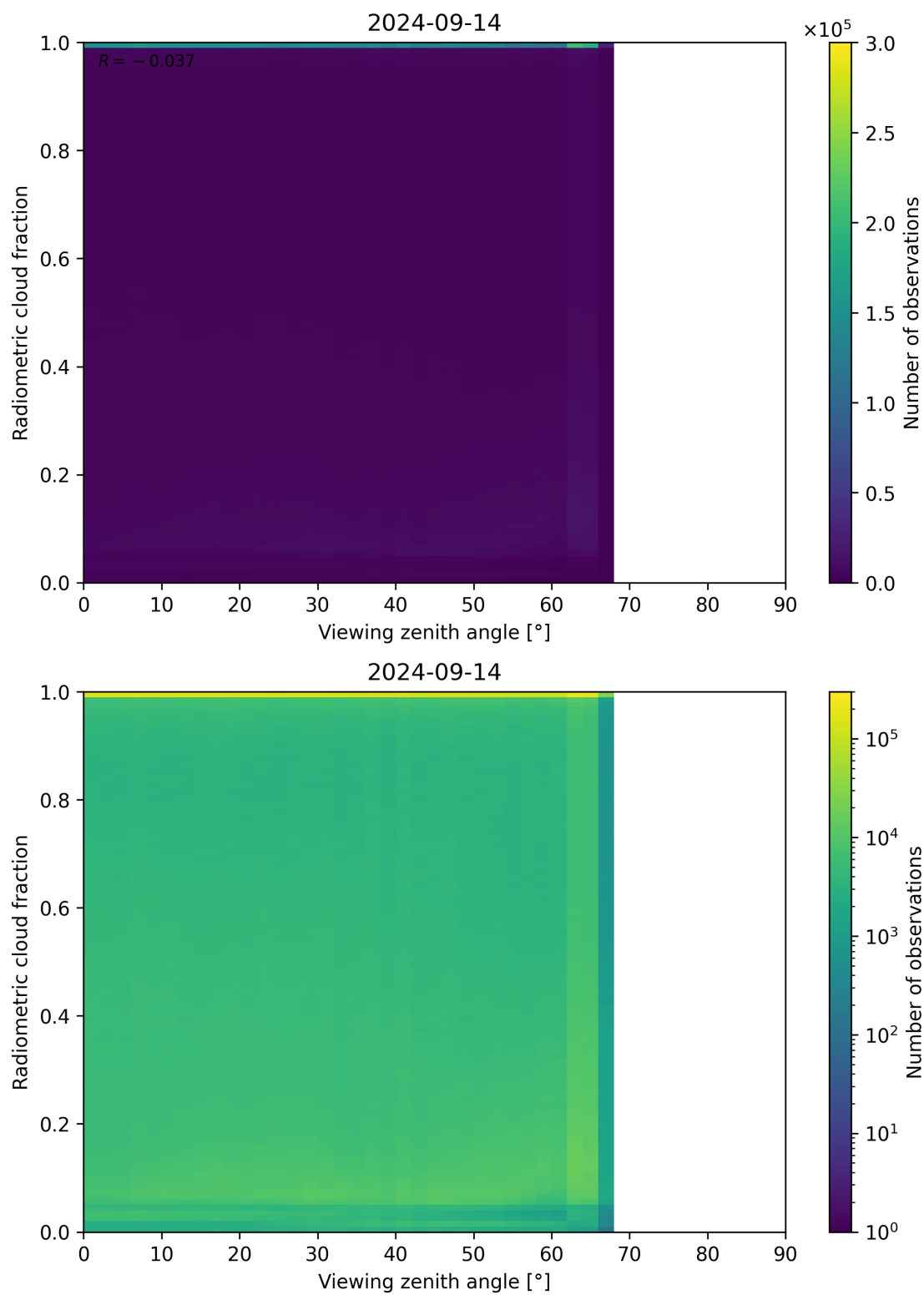
Figure 107: Scatter density plot of “Viewing zenith angle” against “Radiometric cloud fraction” for 2024-09-13 to 2024-09-15.
