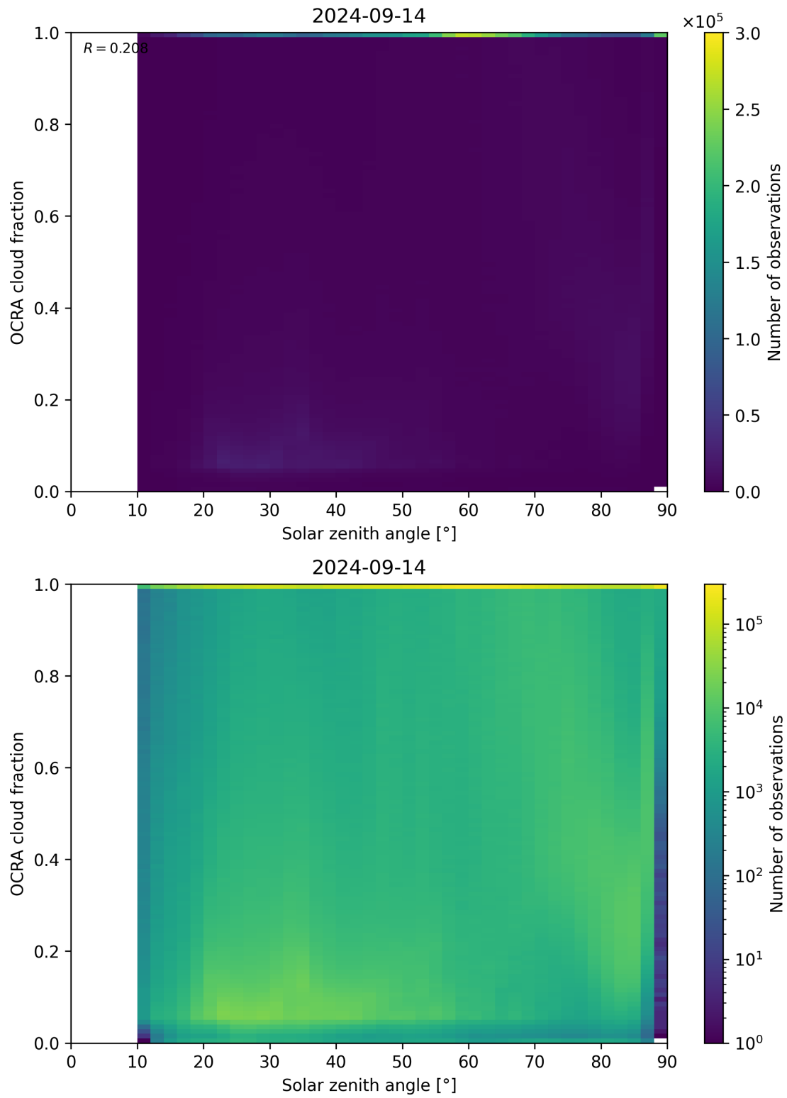
Figure 100: Scatter density plot of “Solar zenith angle” against “OCRA cloud fraction” for 2024-09-13 to 2024-09-15.
