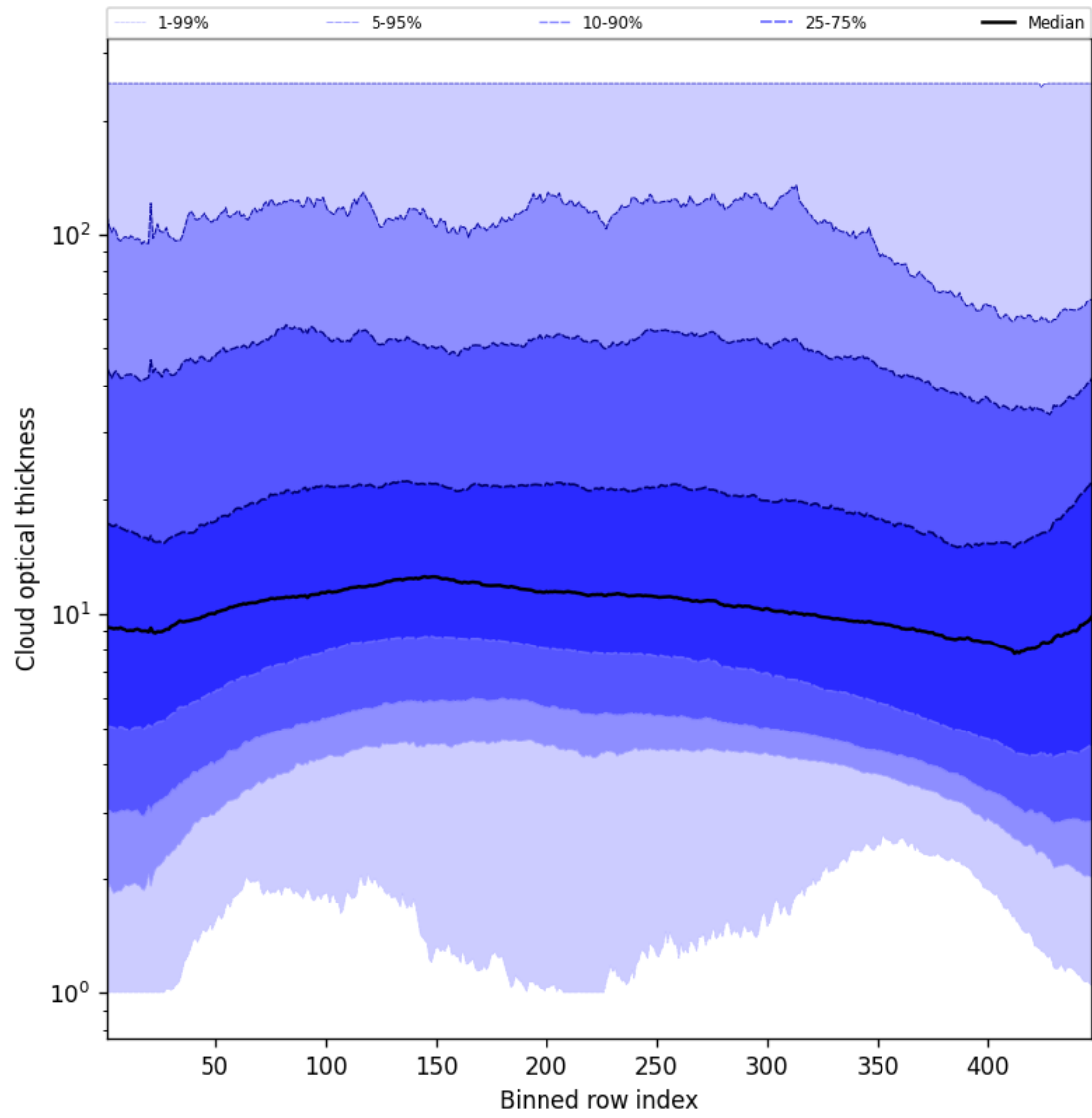
Figure 57: Along track statistics of “Cloud optical thickness” for 2024-09-13 to 2024-09-15
