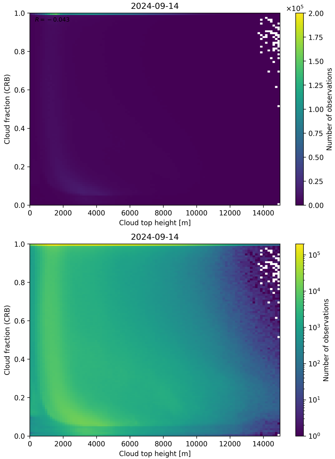
Figure 88: Scatter density plot of “Cloud top height” against “Cloud fraction (CRB)” for 2024-09-13 to 2024-09-15.
