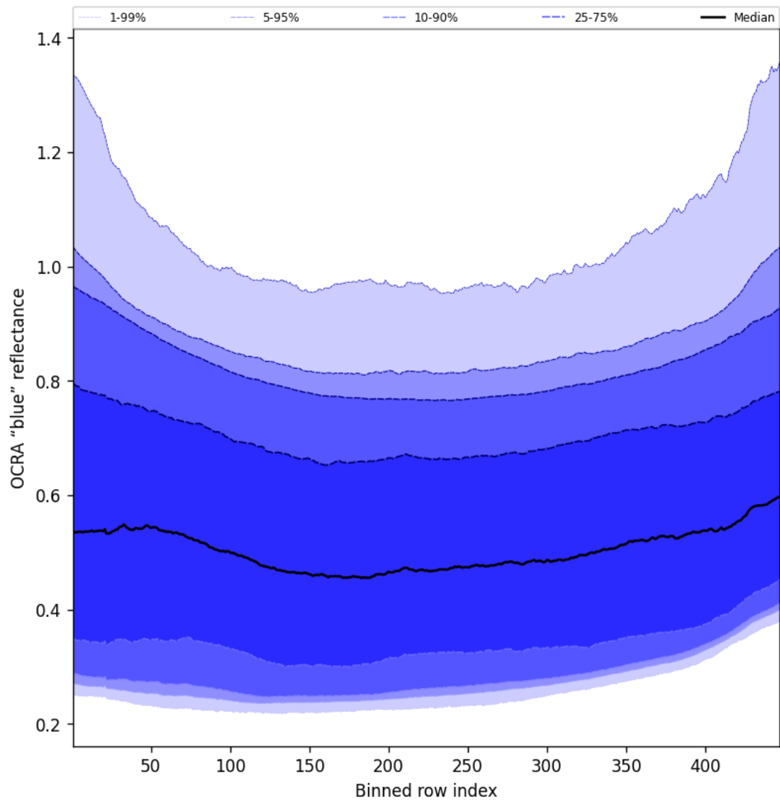
Figure 67: Along track statistics of “OCRA “blue” reflectance” for 2024-09-13 to 2024-09-15
