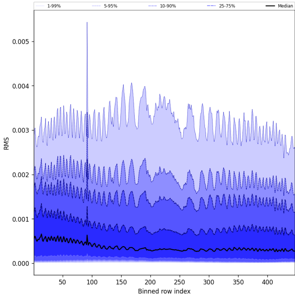
Figure 63: Along track statistics of “RMS” for 2024-09-13 to 2024-09-15
