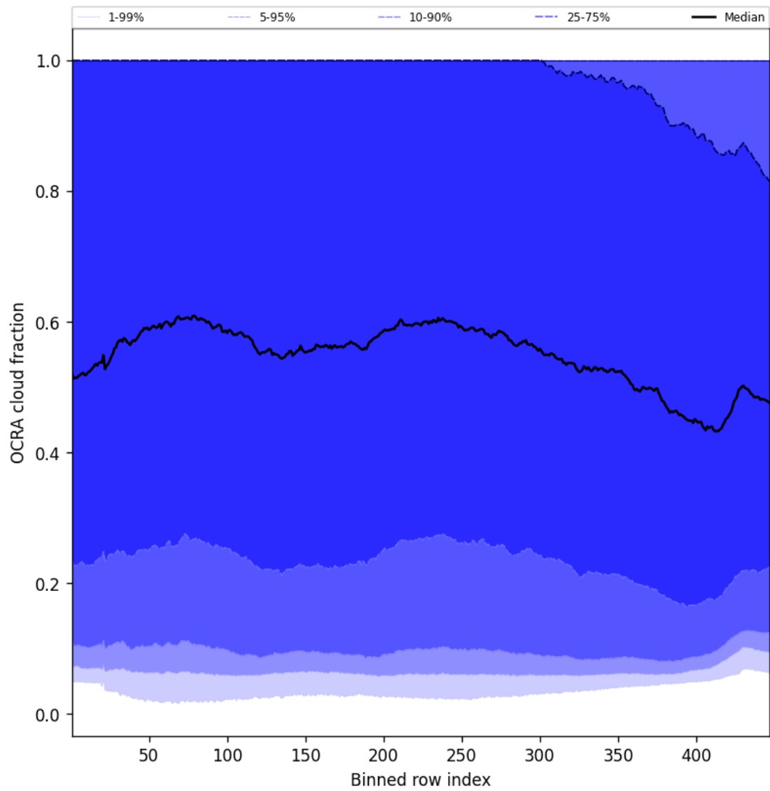
Figure 66: Along track statistics of “OCRA cloud fraction” for 2024-09-13 to 2024-09-15
