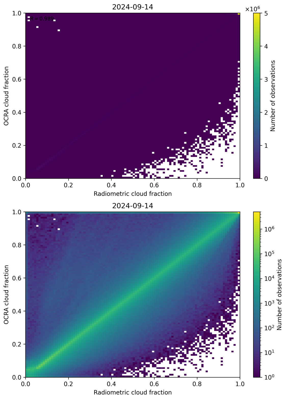
Figure 72: Scatter density plot of “Radiometric cloud fraction” against “OCRA cloud fraction” for 2024-09-13 to 2024-09-15.
