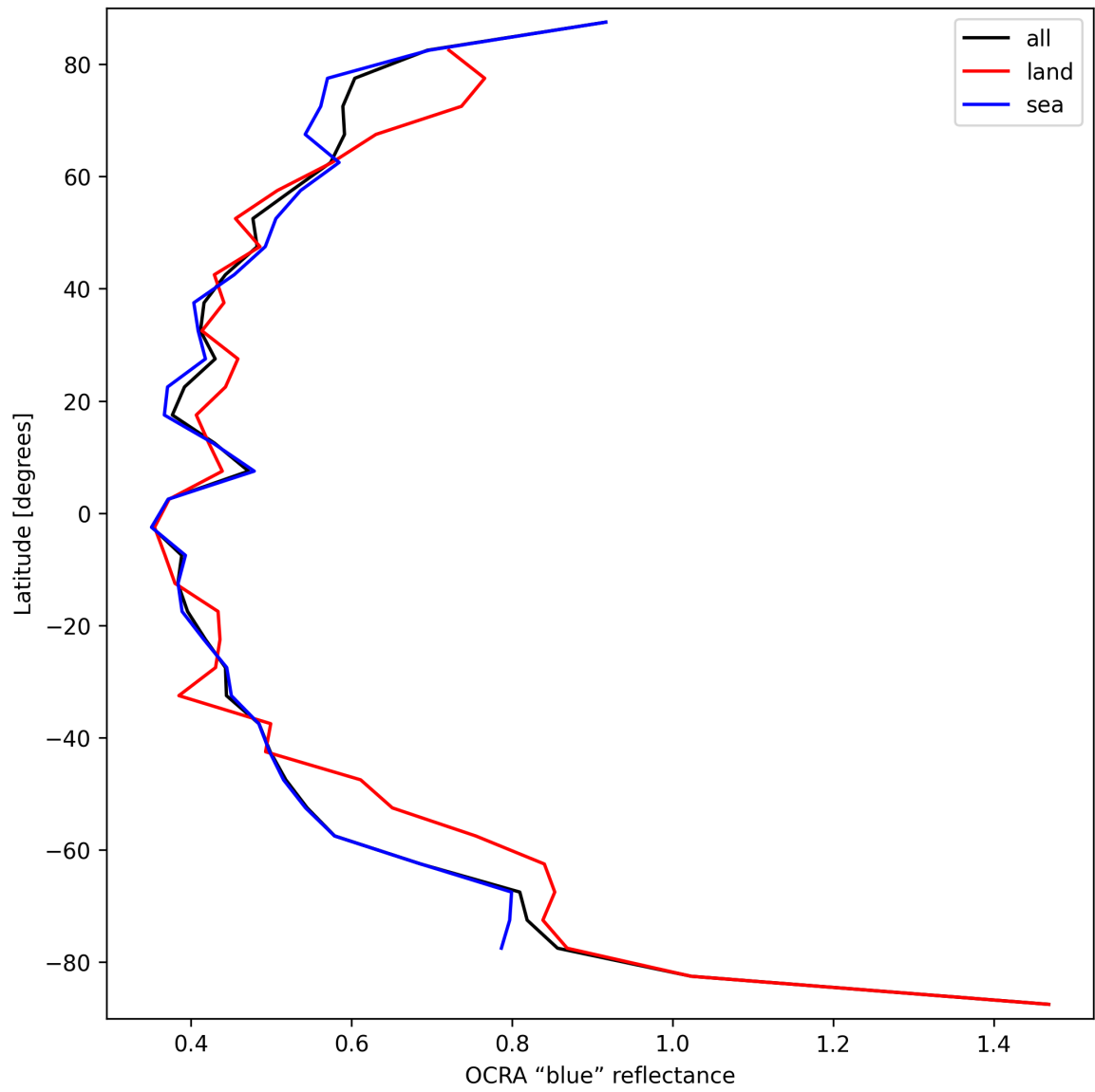
Figure 35: Zonal average of “OCRA “blue” reflectance” for 2024-09-13 to 2024-09-15.
