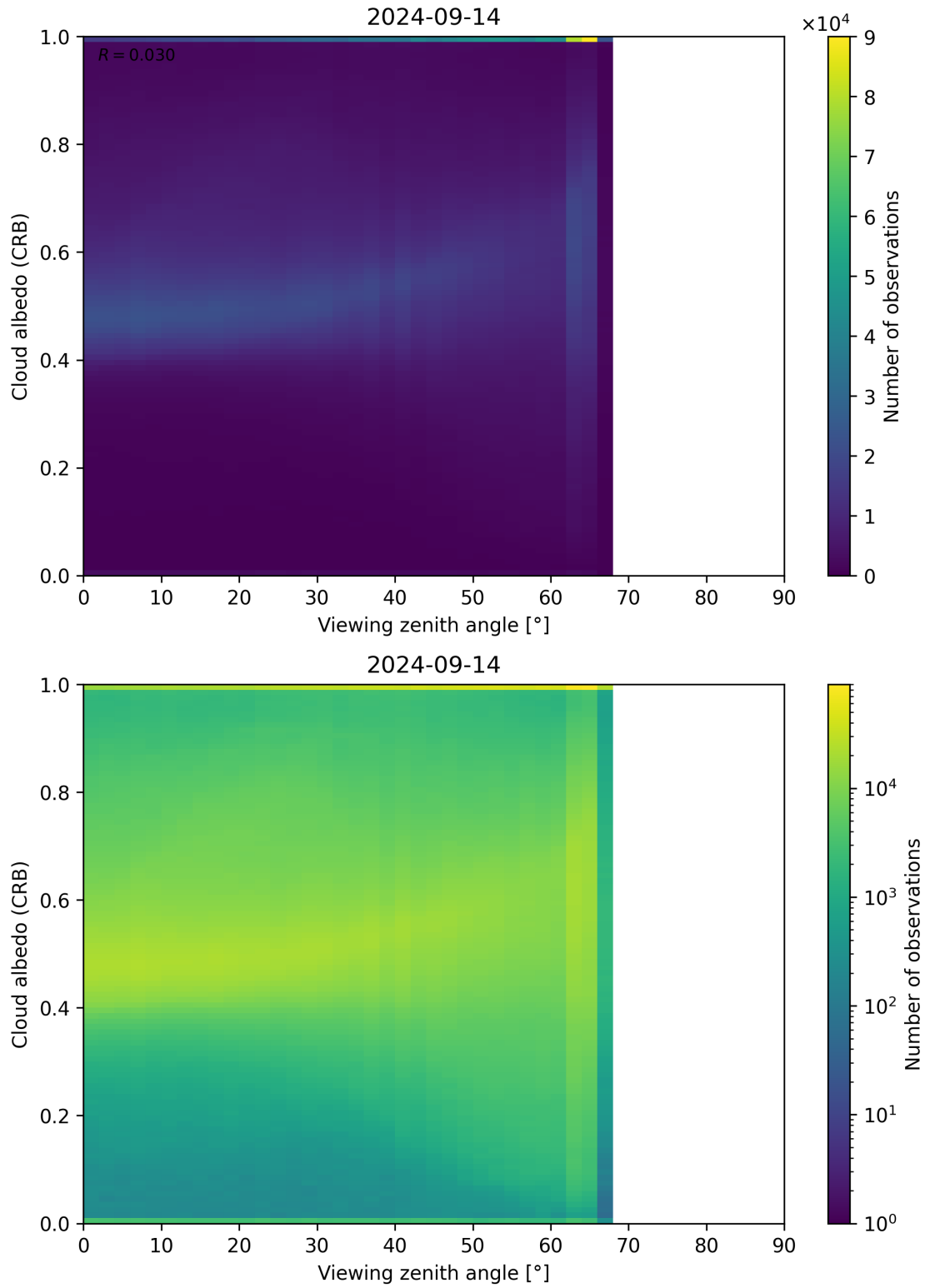
Figure 106: Scatter density plot of “Viewing zenith angle” against “Cloud albedo (CRB)” for 2024-09-13 to 2024-09-15.
