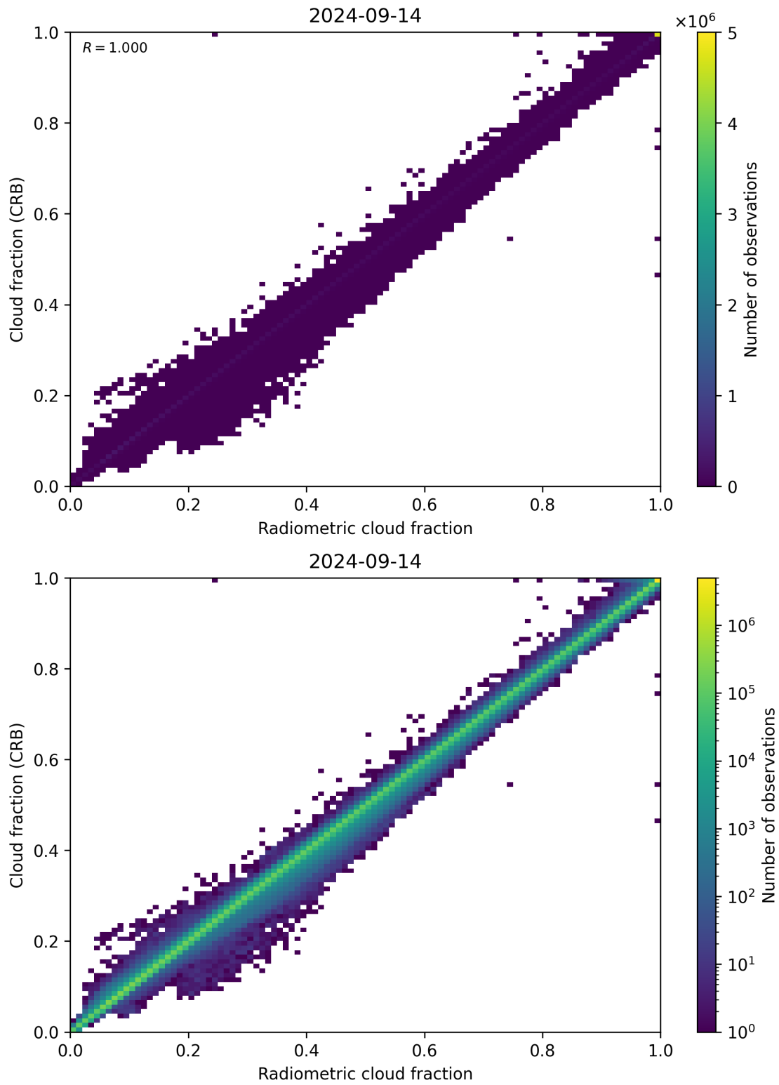
Figure 73: Scatter density plot of “Radiometric cloud fraction” against “Cloud fraction (CRB)” for 2024-09-13 to 2024-09-15.
