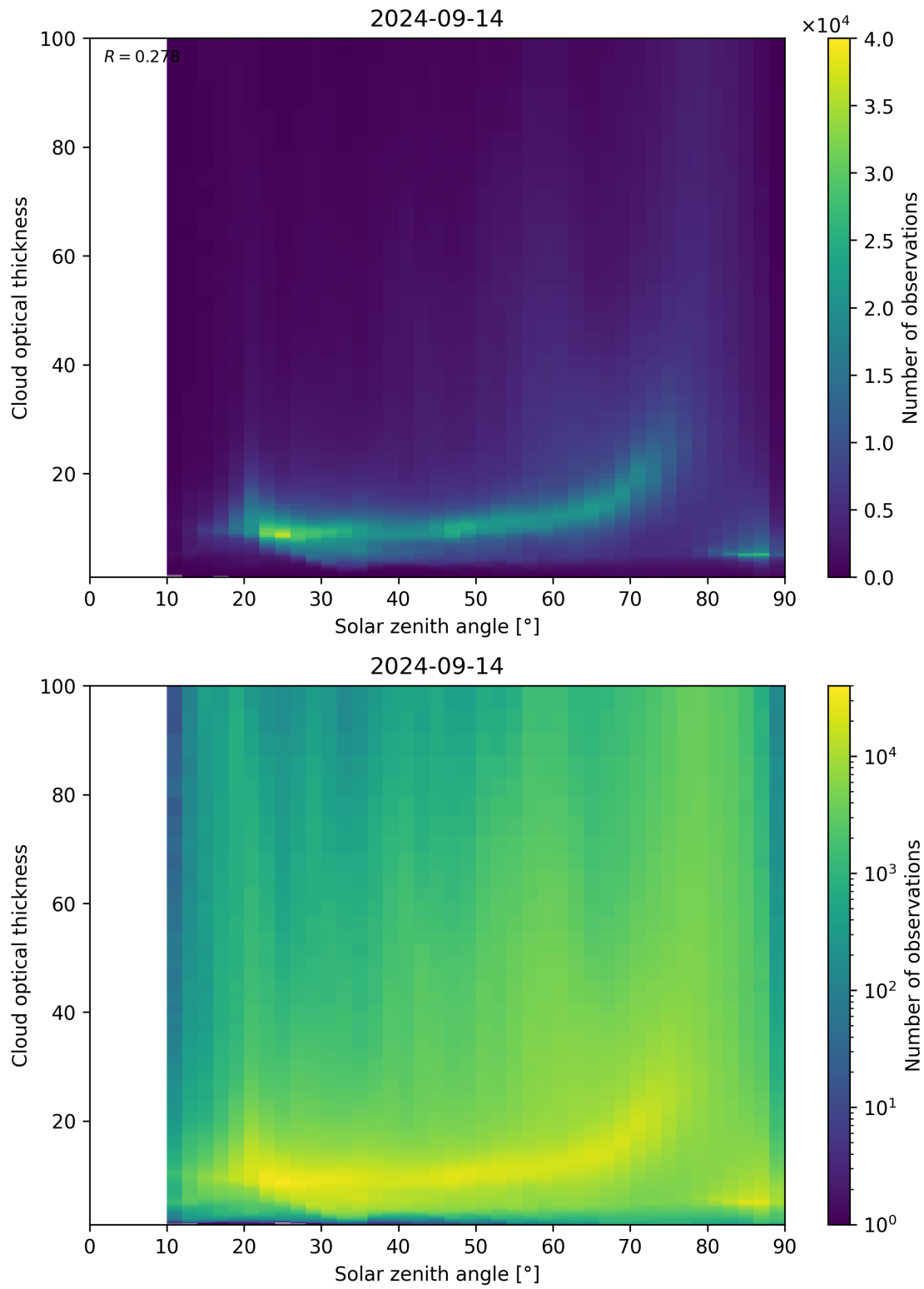
Figure 103: Scatter density plot of “Solar zenith angle” against “Cloud optical thickness” for 2024-09-13 to 2024-09-15.
