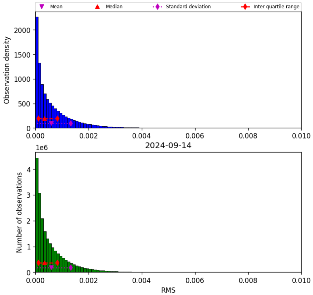
Figure 47: Histogram of “RMS” for 2024-09-13 to 2024-09-15
