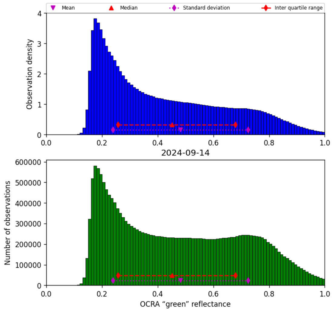
Figure 52: Histogram of “OCRA “green” reflectance” for 2024-09-13 to 2024-09-15
