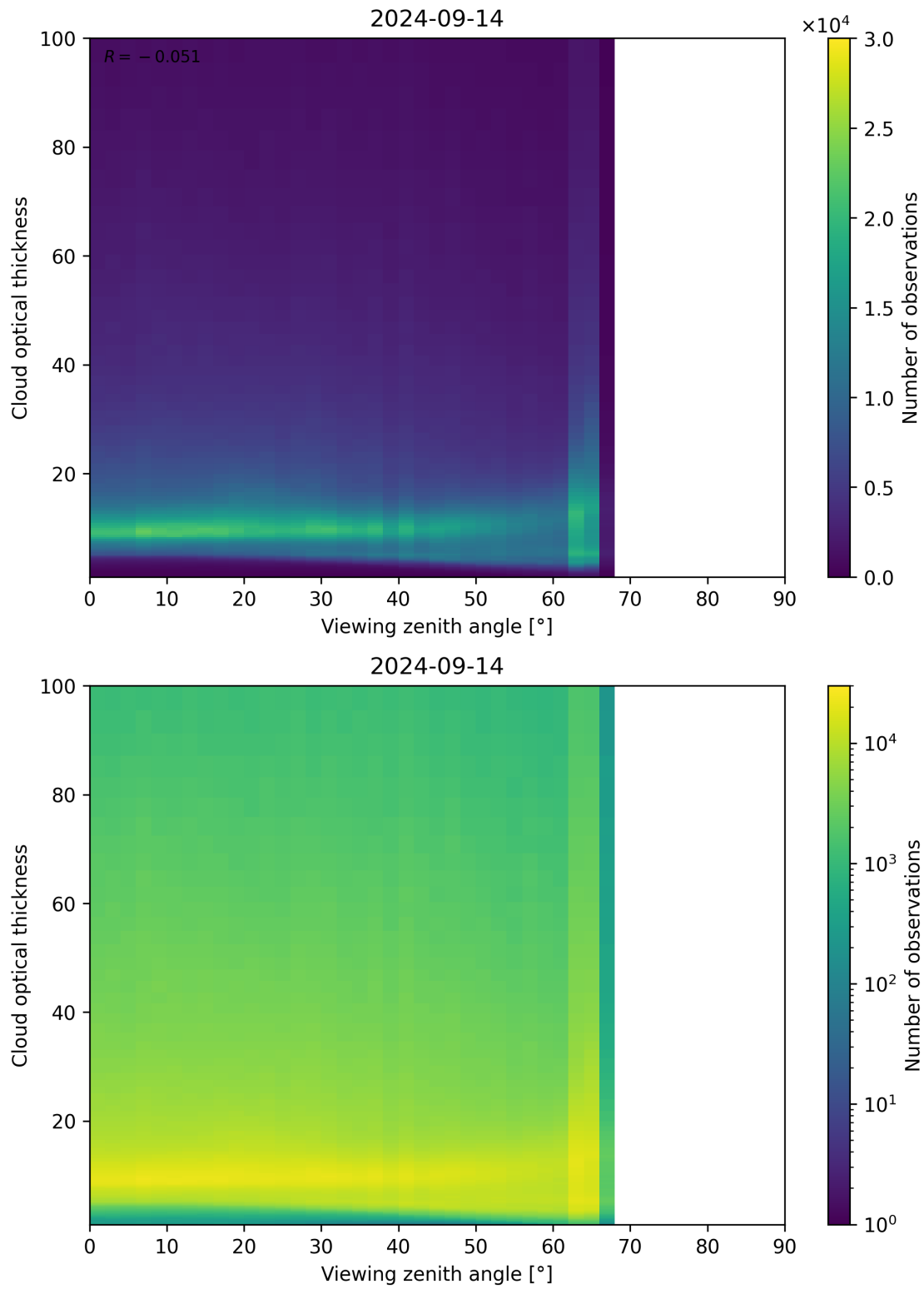
Figure 111: Scatter density plot of “Viewing zenith angle” against “Cloud optical thickness” for 2024-09-13 to 2024-09-15.
