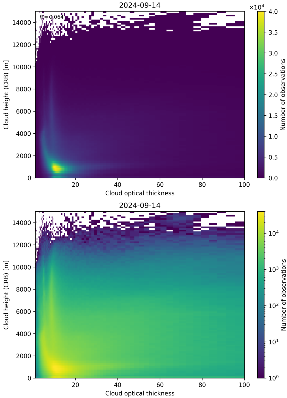
Figure 85: Scatter density plot of “Cloud optical thickness” against “Cloud height (CRB)” for 2024-09-13 to 2024-09-15.
