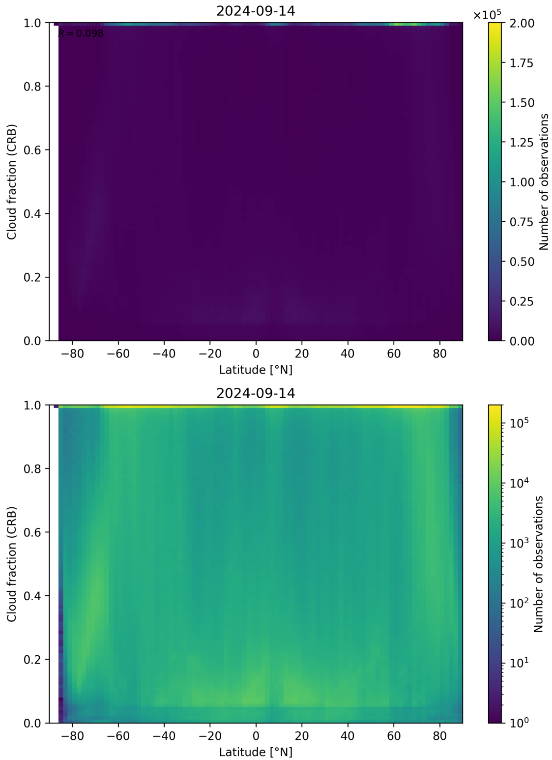
Figure 94: Scatter density plot of “Latitude” against “Cloud fraction (CRB)” for 2024-09-13 to 2024-09-15.
