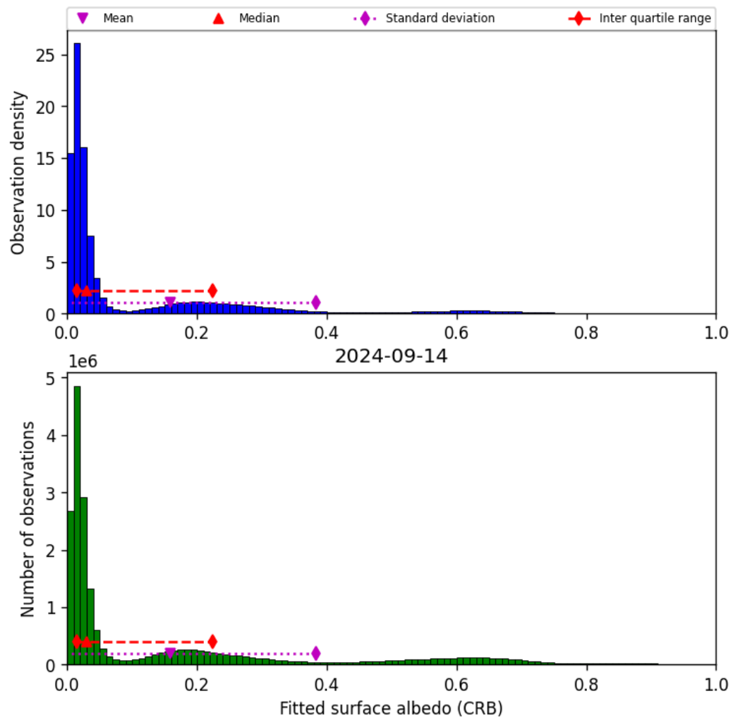
Figure 46: Histogram of “Fitted surface albedo (CRB)” for 2024-09-13 to 2024-09-15
