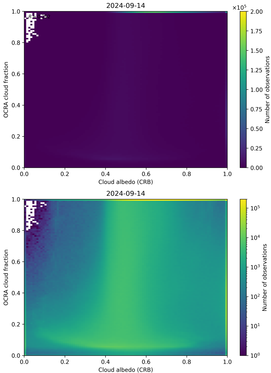
Figure 70: Scatter density plot of “Cloud albedo (CRB)” against “OCRA cloud fraction” for 2024-09-13 to 2024-09-15.
