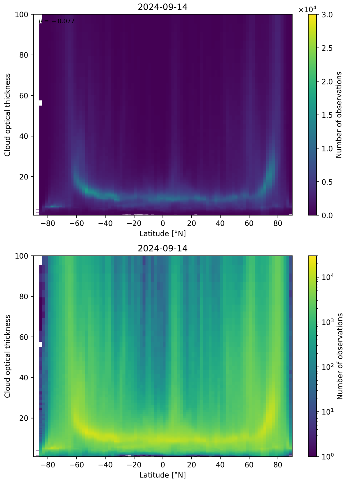
Figure 96: Scatter density plot of “Latitude” against “Cloud optical thickness” for 2024-09-13 to 2024-09-15.
