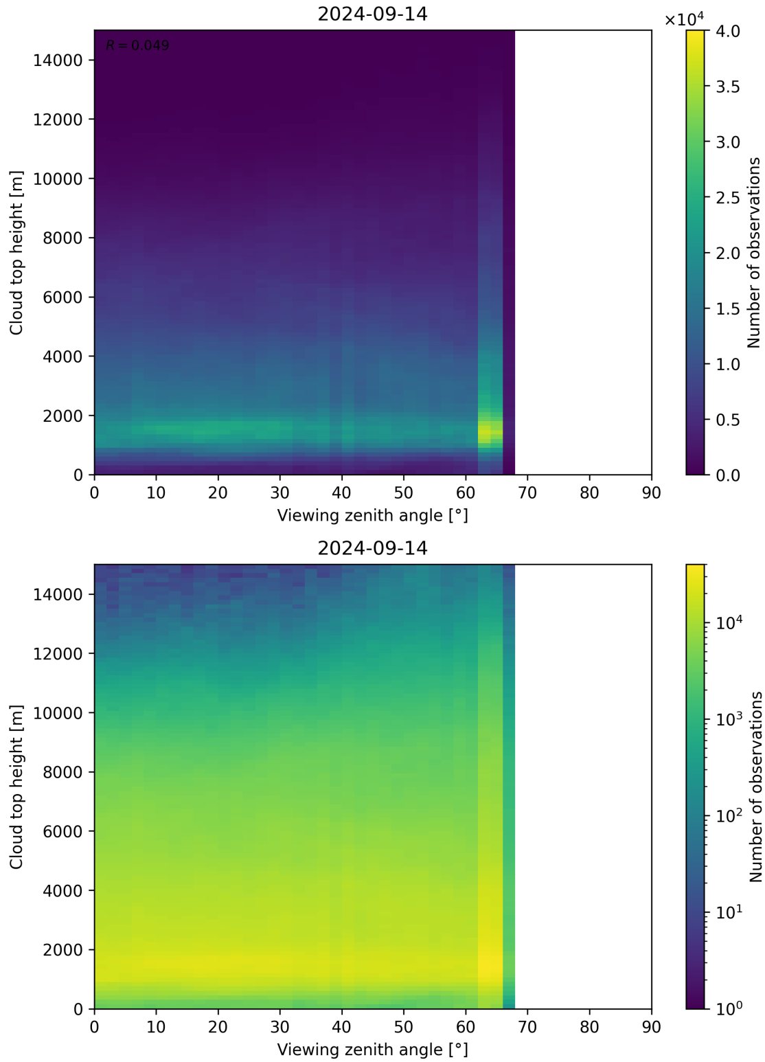
Figure 112: Scatter density plot of “Viewing zenith angle” against “Cloud top height” for 2024-09-13 to 2024-09-15.
