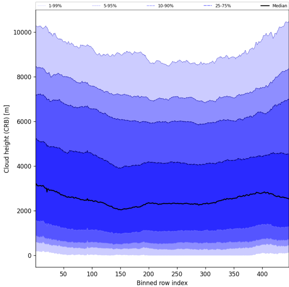
Figure 59: Along track statistics of “Cloud height (CRB)” for 2024-09-13 to 2024-09-15
