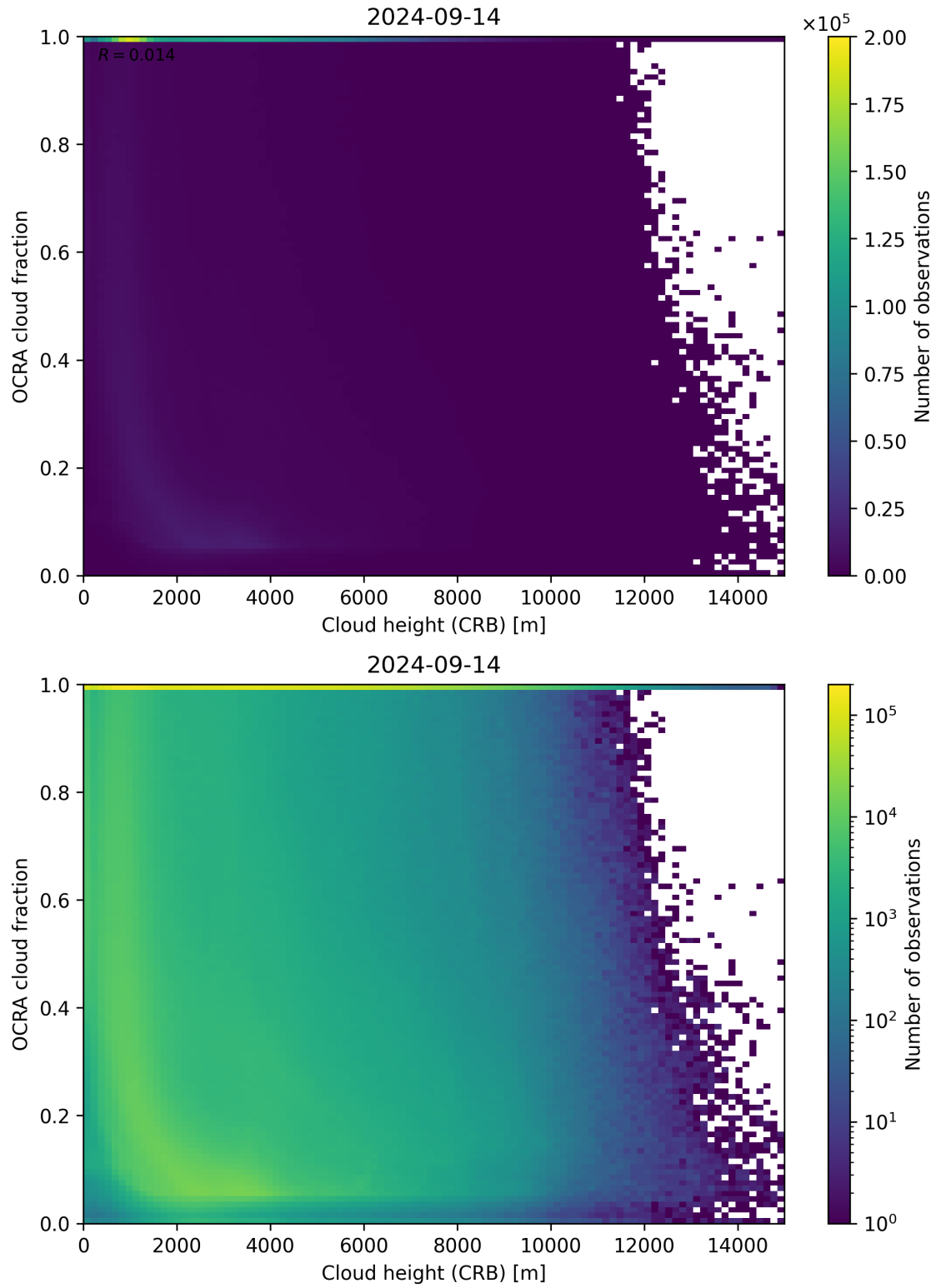
Figure 81: Scatter density plot of “Cloud height (CRB)” against “OCRA cloud fraction” for 2024-09-13 to 2024-09-15.
