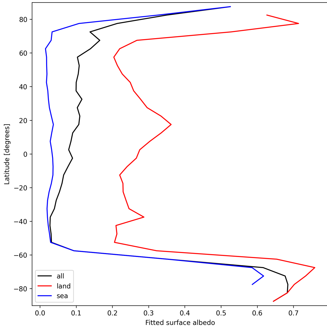
Figure 29: Zonal average of “Fitted surface albedo” for 2024-09-13 to 2024-09-15.
