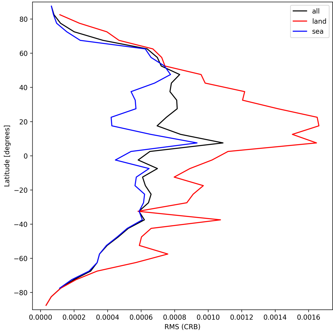
Figure 32: Zonal average of “RMS (CRB)” for 2024-09-13 to 2024-09-15.
