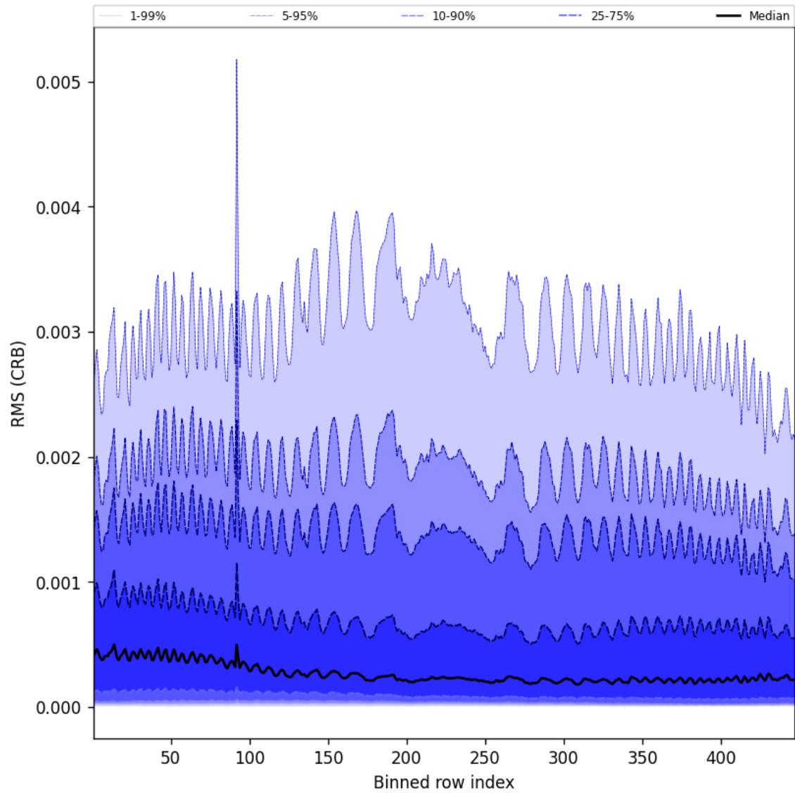
Figure 64: Along track statistics of “RMS (CRB)” for 2024-09-13 to 2024-09-15
