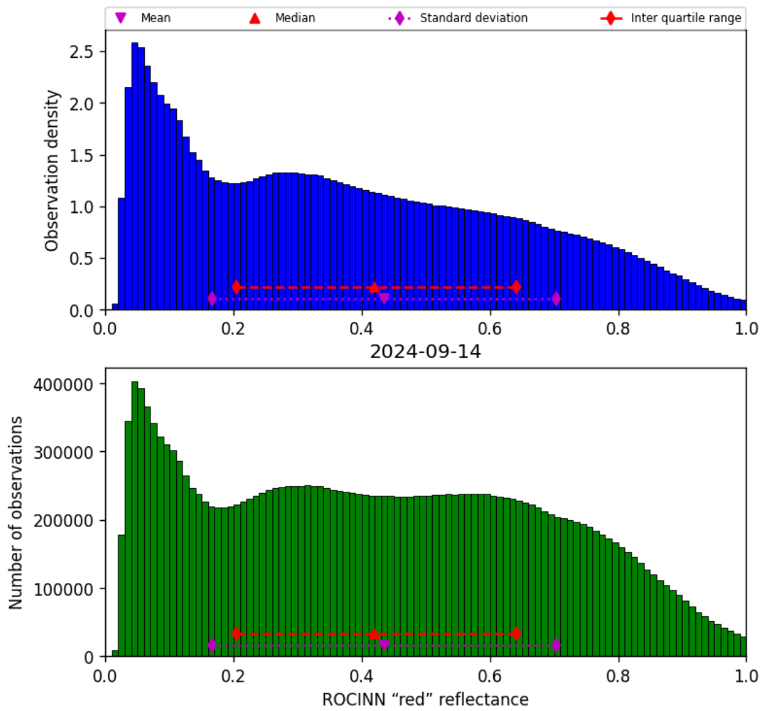
Figure 53: Histogram of “ROCINN “red” reflectance” for 2024-09-13 to 2024-09-15
