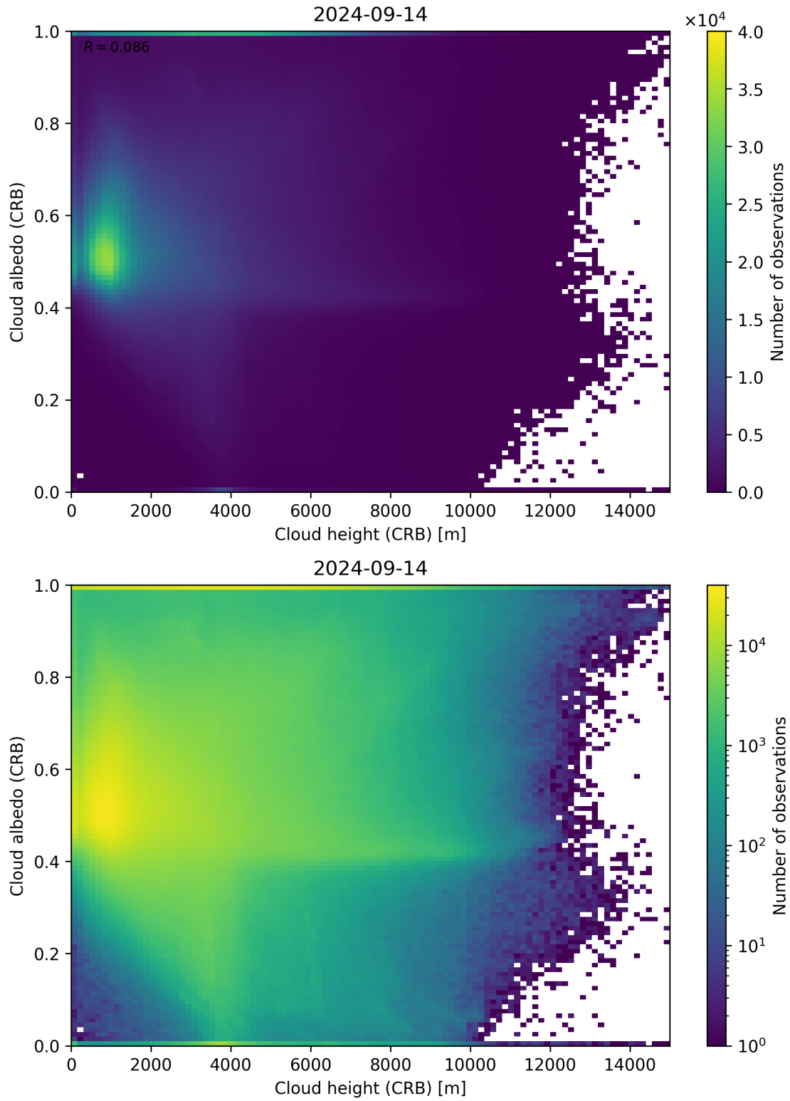
Figure 80: Scatter density plot of “Cloud height (CRB)” against “Cloud albedo (CRB)” for 2024-09-13 to 2024-09-15.
