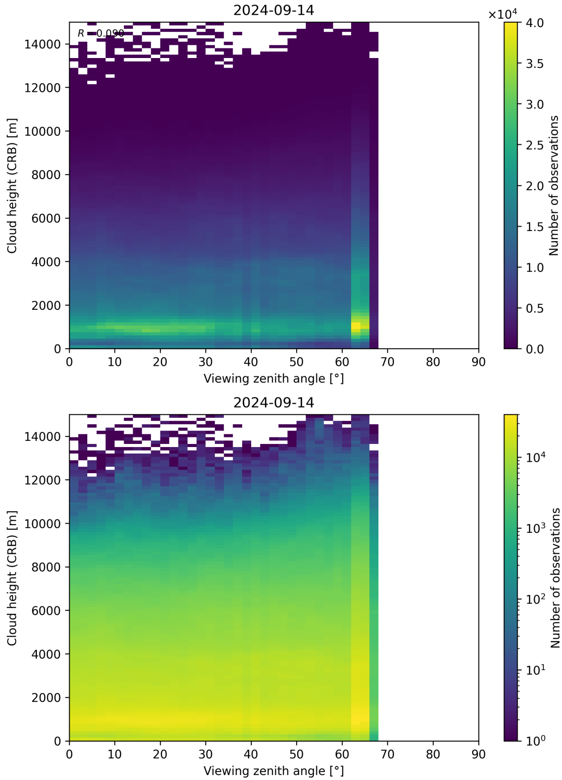
Figure 110: Scatter density plot of “Viewing zenith angle” against “Cloud height (CRB)” for 2024-09-13 to 2024-09-15.
