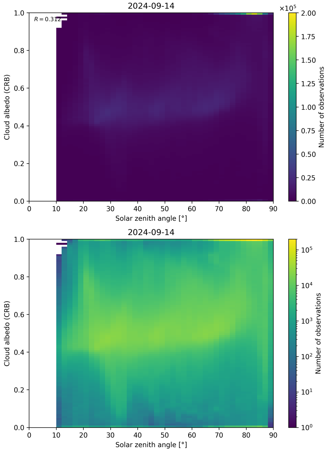
Figure 98: Scatter density plot of “Solar zenith angle” against “Cloud albedo (CRB)” for 2024-09-13 to 2024-09-15.
