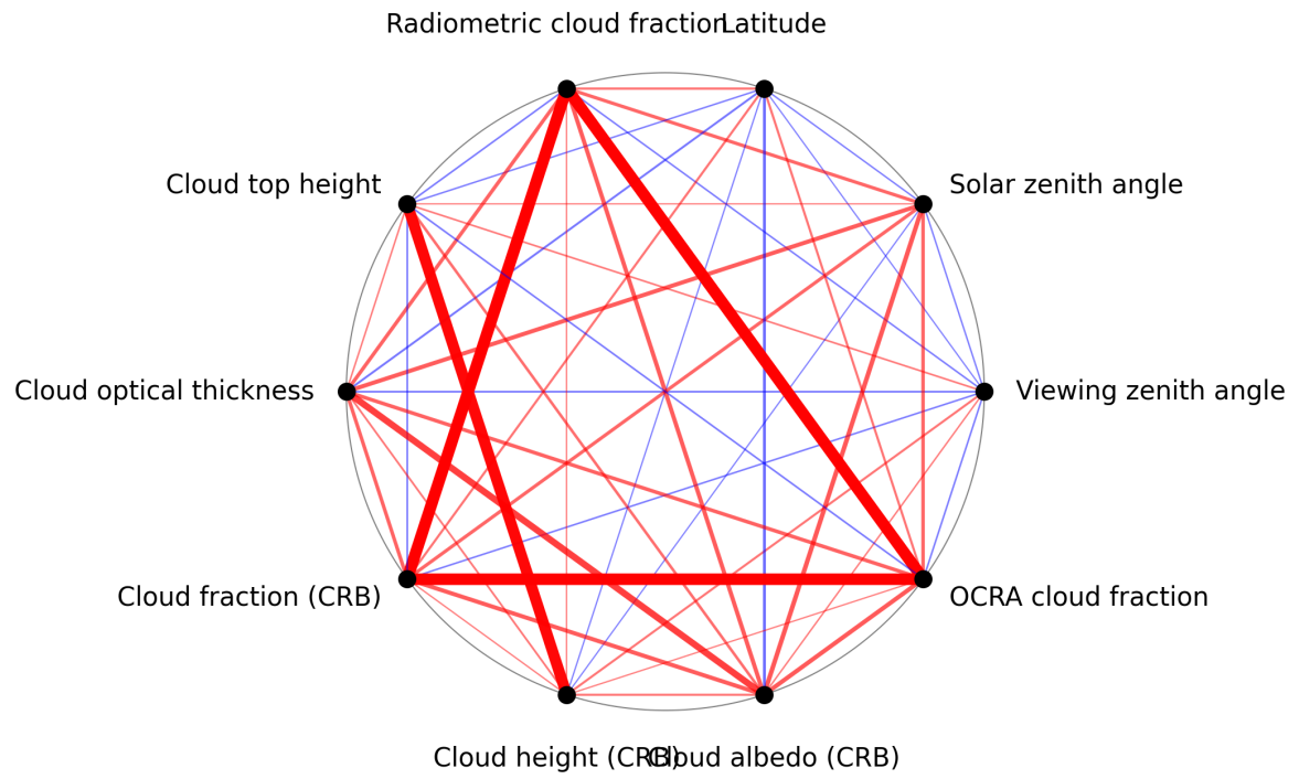
Figure 1: Map of correlation graph for 2024-09-13 to 2024-09-15.
