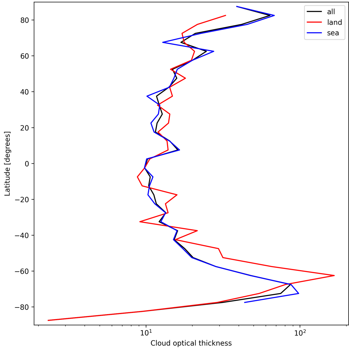
Figure 25: Zonal average of “Cloud optical thickness” for 2024-09-13 to 2024-09-15.
