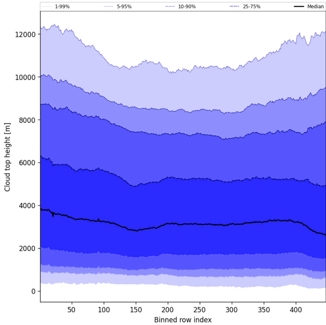
Figure 56: Along track statistics of “Cloud top height” for 2024-09-13 to 2024-09-15
