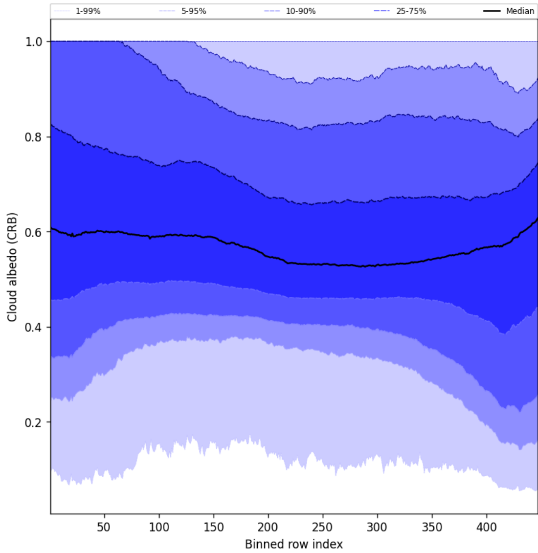
Figure 60: Along track statistics of “Cloud albedo (CRB)” for 2024-09-13 to 2024-09-15
