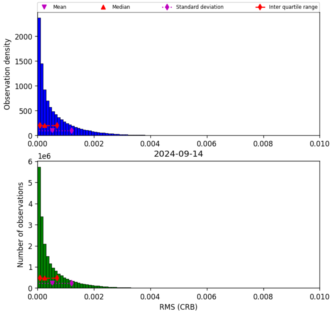
Figure 48: Histogram of “RMS (CRB)” for 2024-09-13 to 2024-09-15
