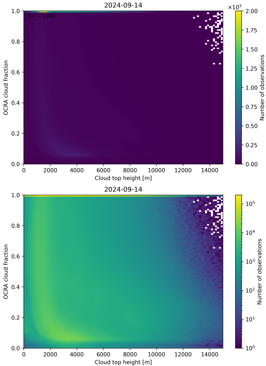
Figure 87: Scatter density plot of “Cloud top height” against “OCRA cloud fraction” for 2024-09-13 to 2024-09-15.
