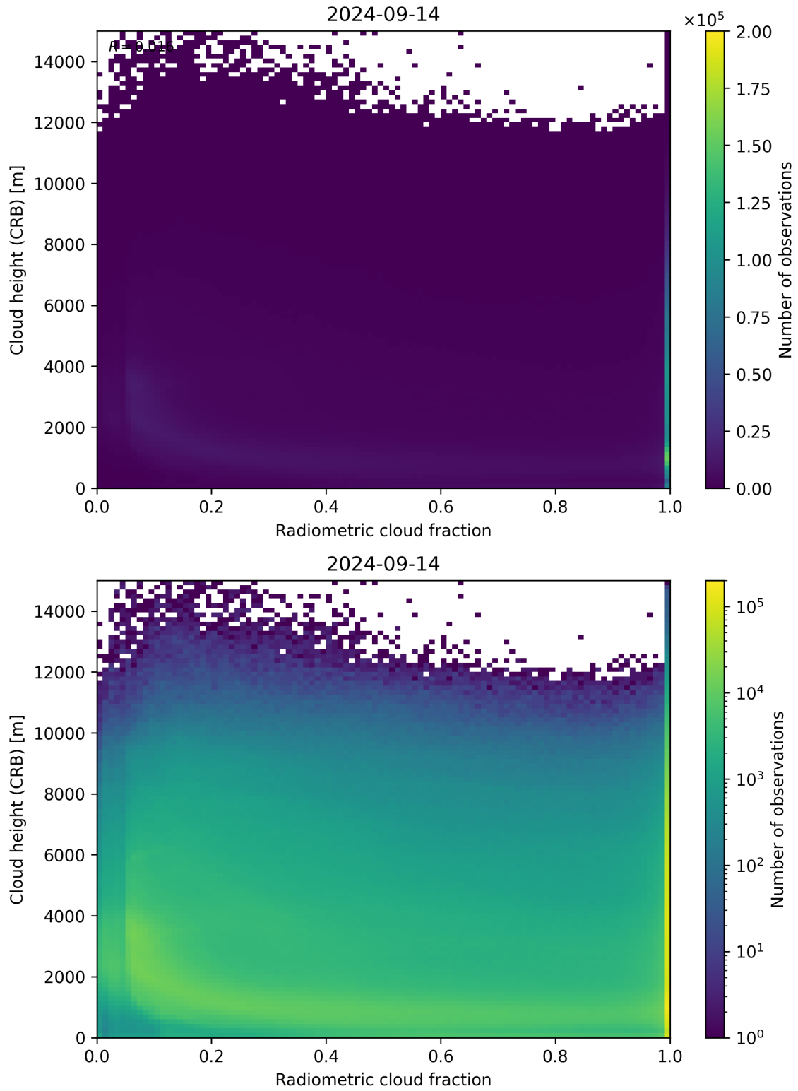
Figure 74: Scatter density plot of “Radiometric cloud fraction” against “Cloud height (CRB)” for 2024-09-13 to 2024-09-15.
