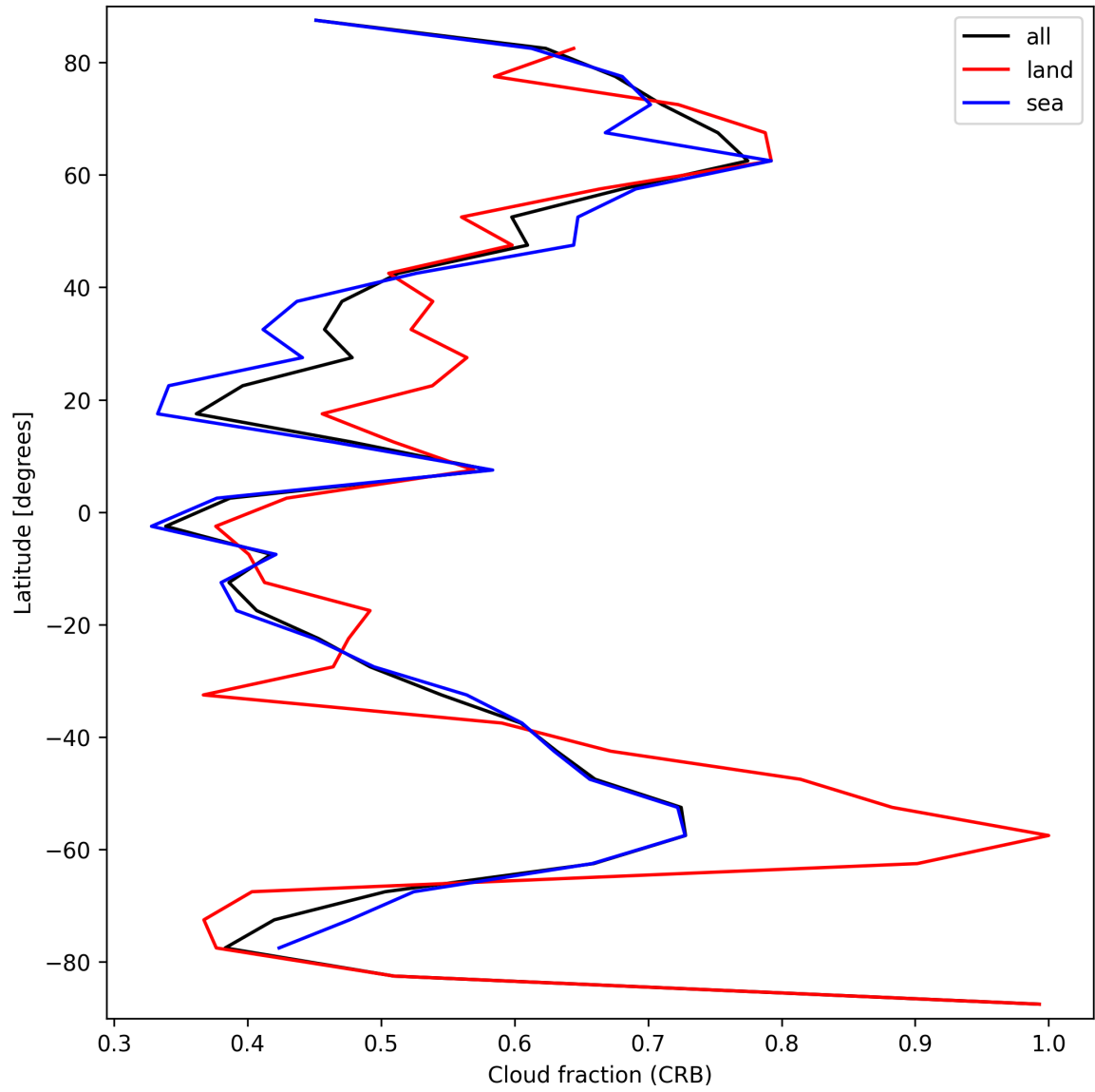
Figure 26: Zonal average of “Cloud fraction (CRB)” for 2024-09-13 to 2024-09-15.
