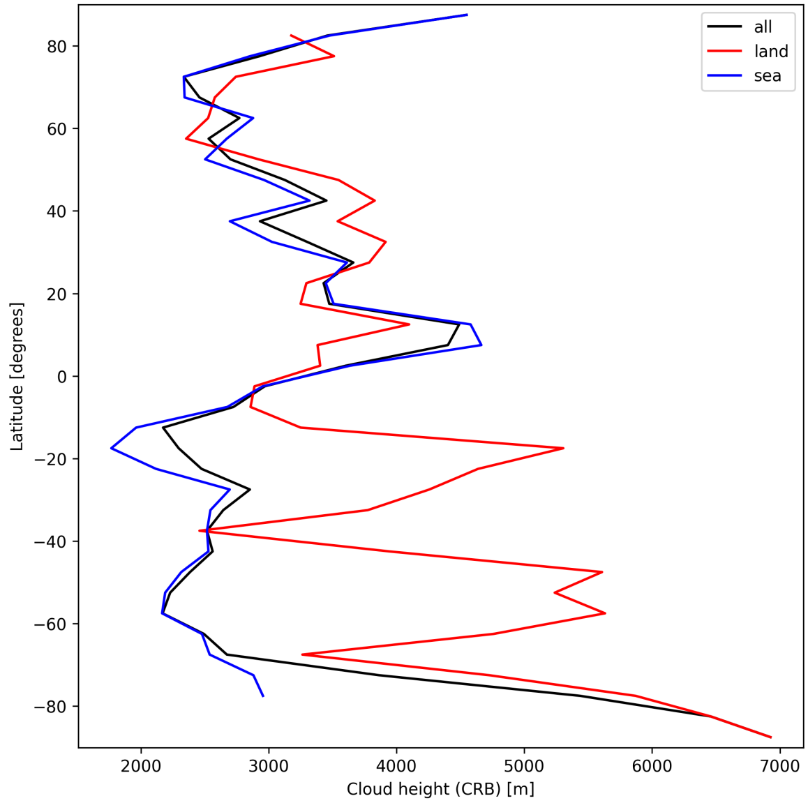
Figure 27: Zonal average of “Cloud height (CRB)” for 2024-09-13 to 2024-09-15.
