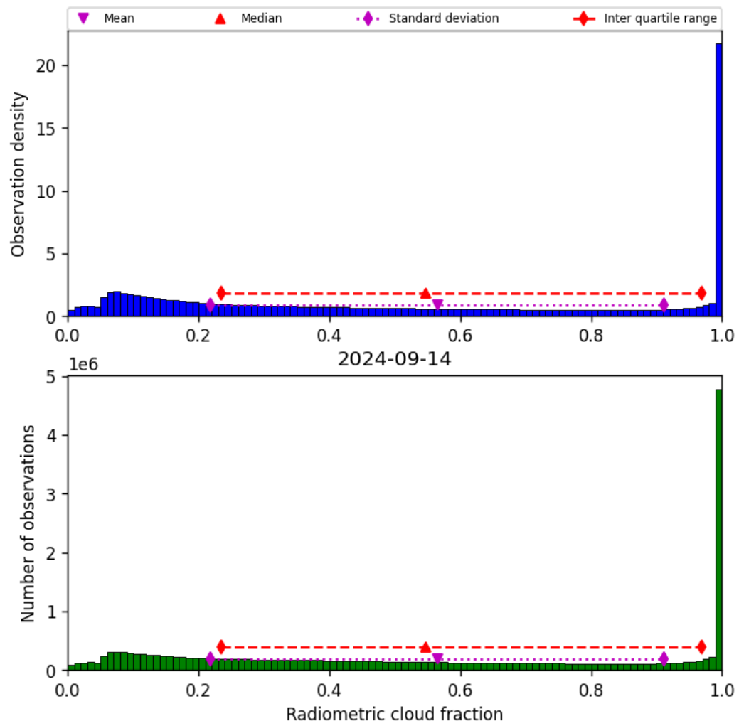
Figure 39: Histogram of “Radiometric cloud fraction” for 2024-09-13 to 2024-09-15
