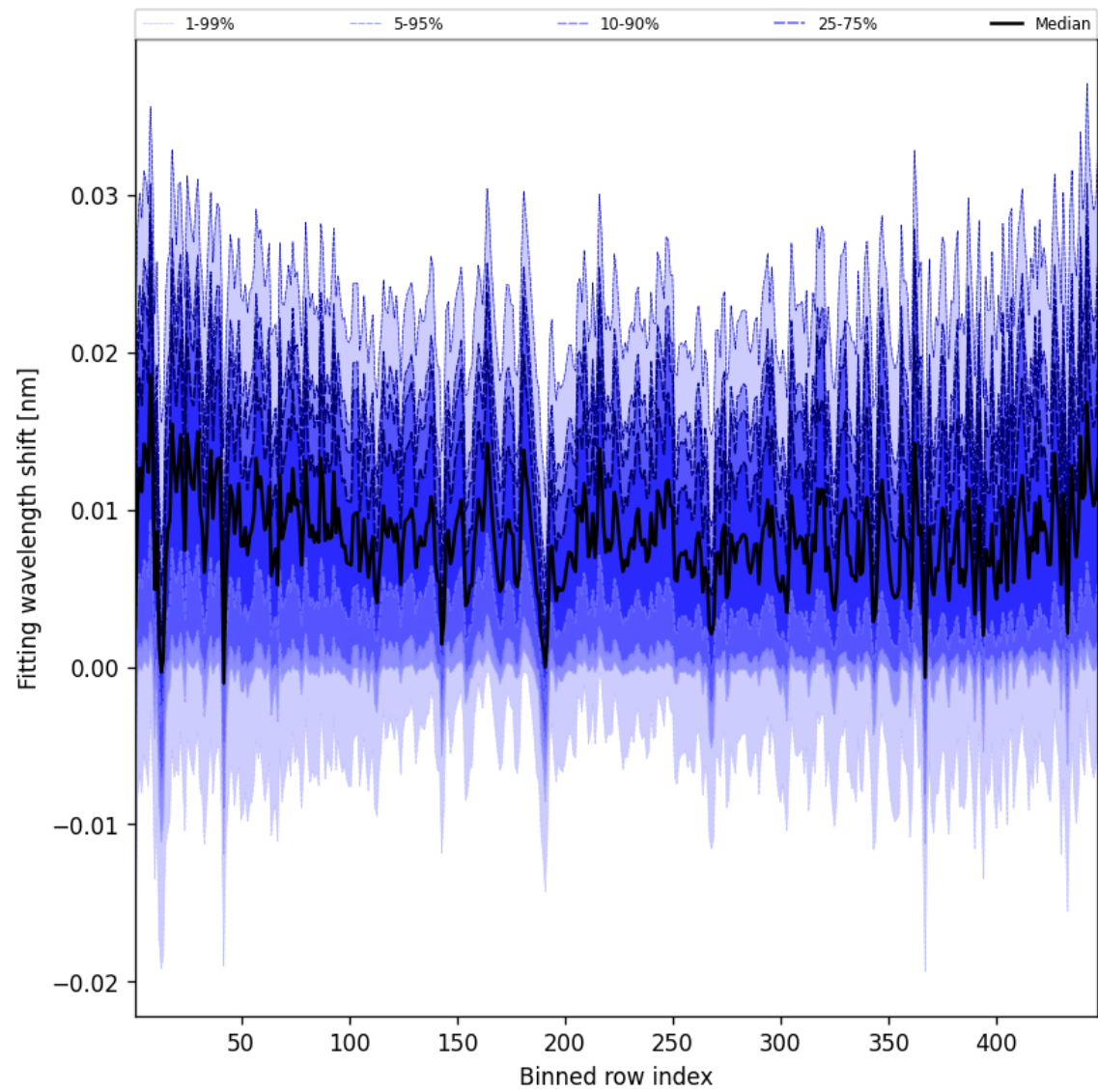
Figure 65: Along track statistics of “Fitting wavelength shift” for 2024-09-13 to 2024-09-15
