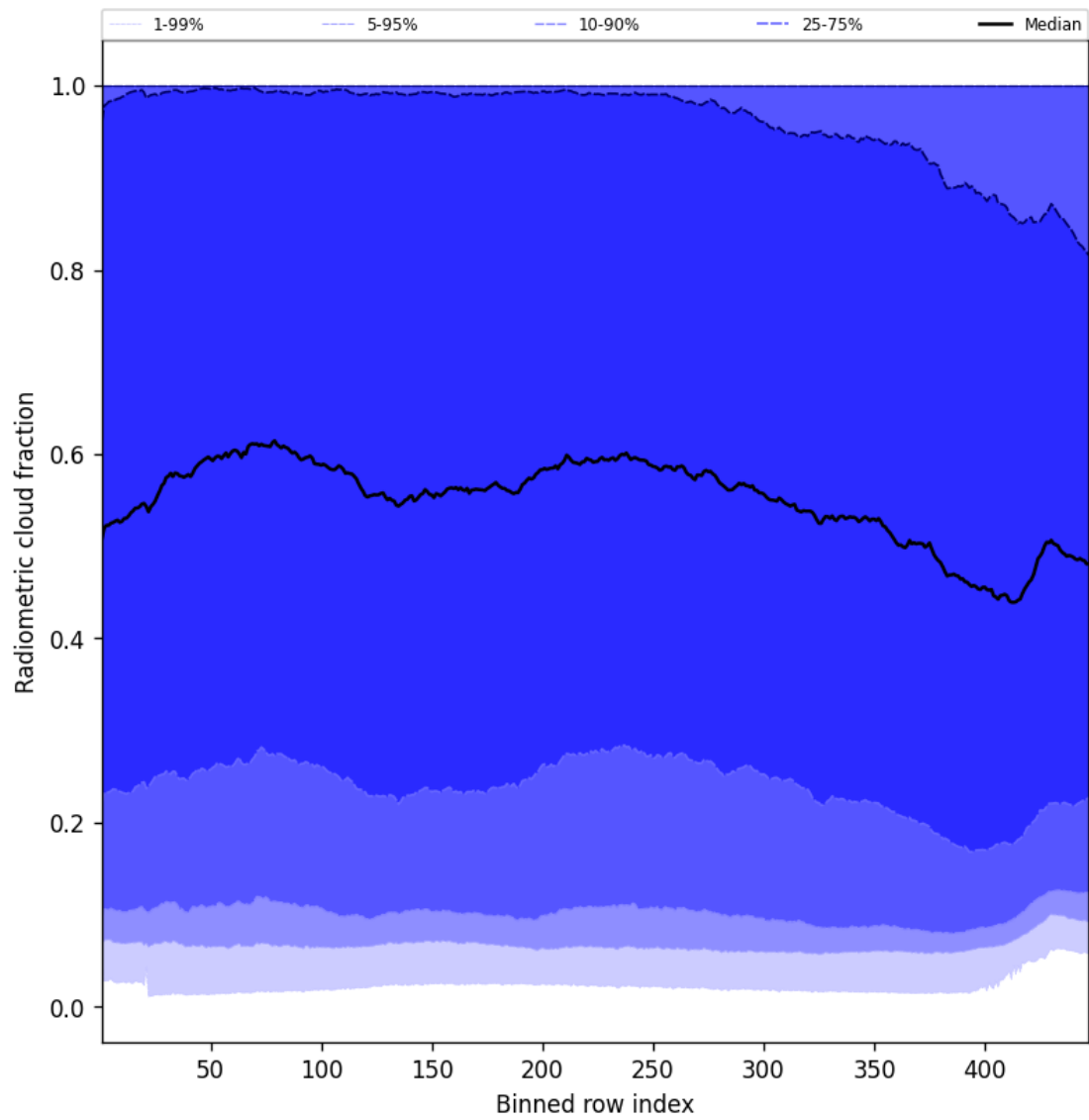
Figure 55: Along track statistics of “Radiometric cloud fraction” for 2024-09-13 to 2024-09-15
