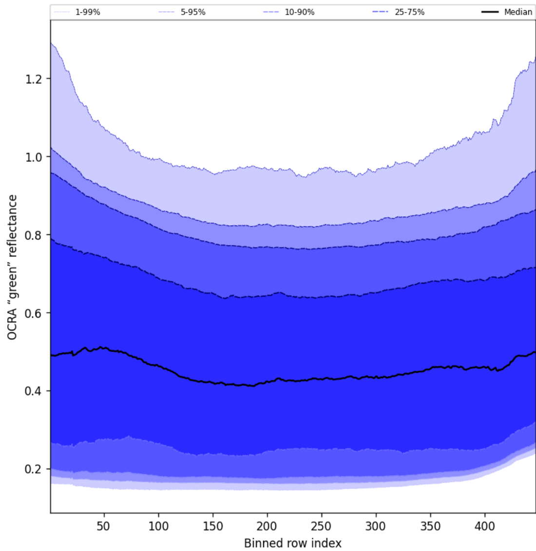
Figure 68: Along track statistics of “OCRA “green” reflectance” for 2024-09-13 to 2024-09-15
