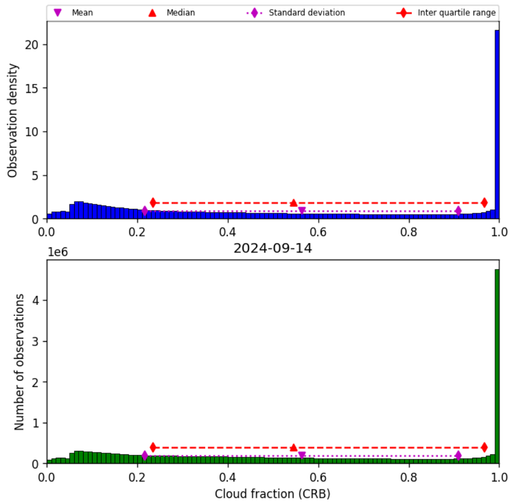
Figure 42: Histogram of “Cloud fraction (CRB)” for 2024-09-13 to 2024-09-15
