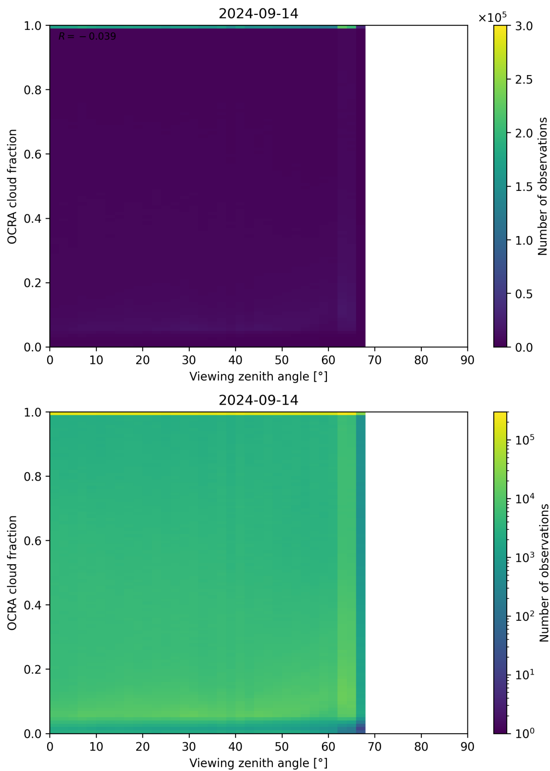
Figure 108: Scatter density plot of “Viewing zenith angle” against “OCRA cloud fraction” for 2024-09-13 to 2024-09-15.
