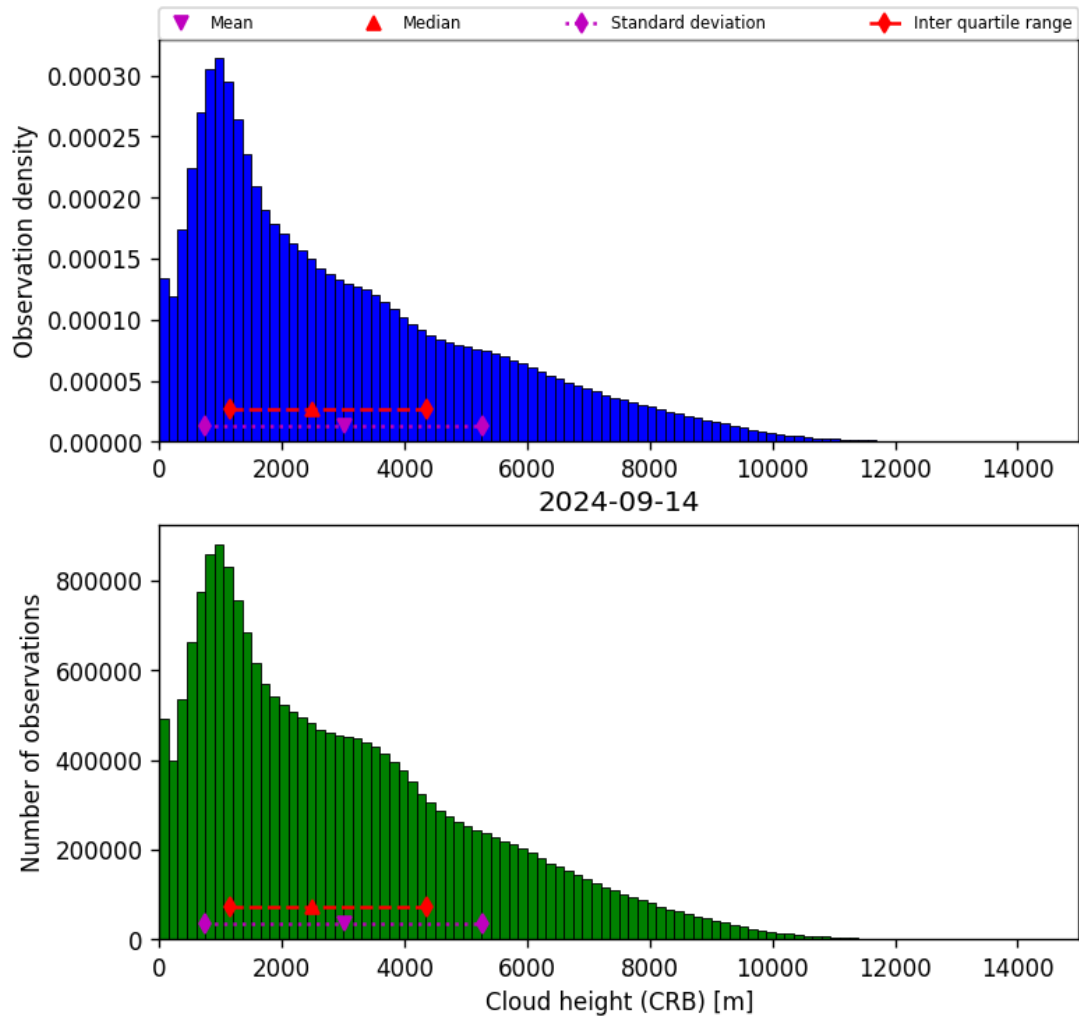
Figure 43: Histogram of “Cloud height (CRB)” for 2024-09-13 to 2024-09-15
