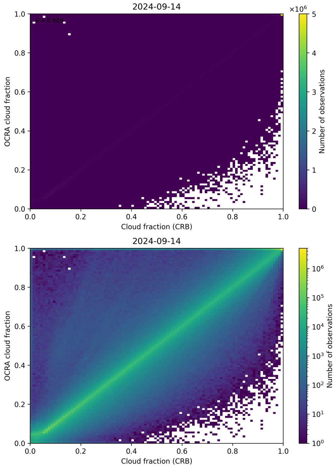
Figure 78: Scatter density plot of “Cloud fraction (CRB)” against “OCRA cloud fraction” for 2024-09-13 to 2024-09-15.
