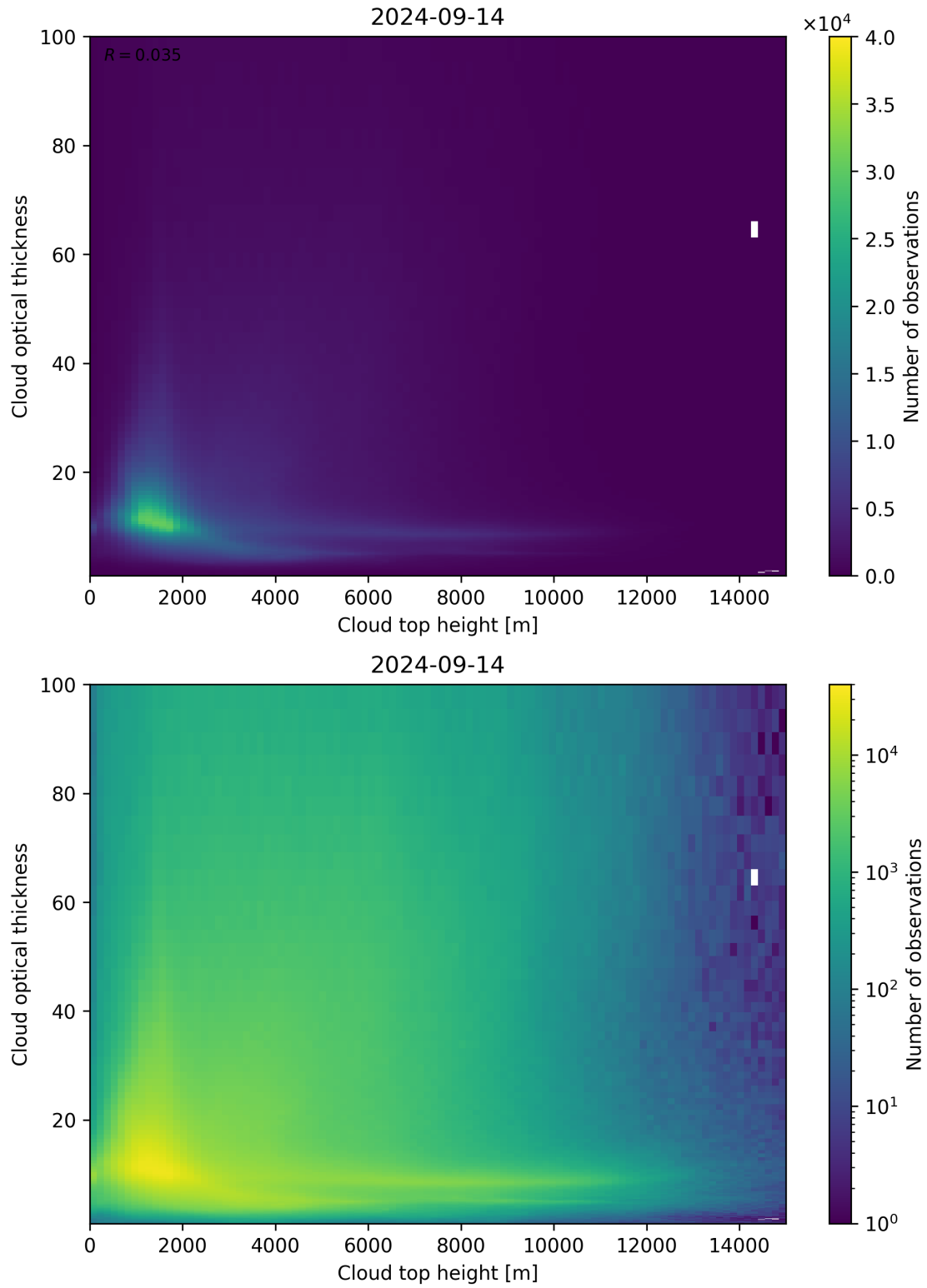
Figure 90: Scatter density plot of “Cloud top height” against “Cloud optical thickness” for 2024-09-13 to 2024-09-15.
