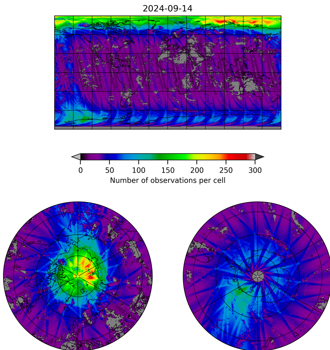
Figure 21: Map of the number of observations for 2024-09-13 to 2024-09-15
