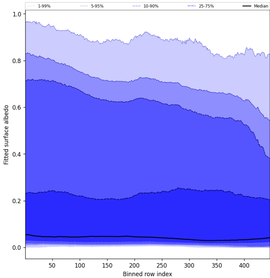
Figure 61: Along track statistics of “Fitted surface albedo” for 2024-09-13 to 2024-09-15
