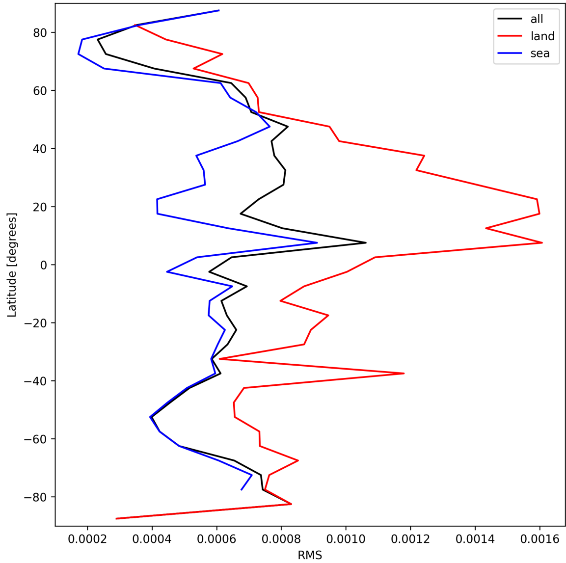
Figure 31: Zonal average of “RMS” for 2024-09-13 to 2024-09-15.
