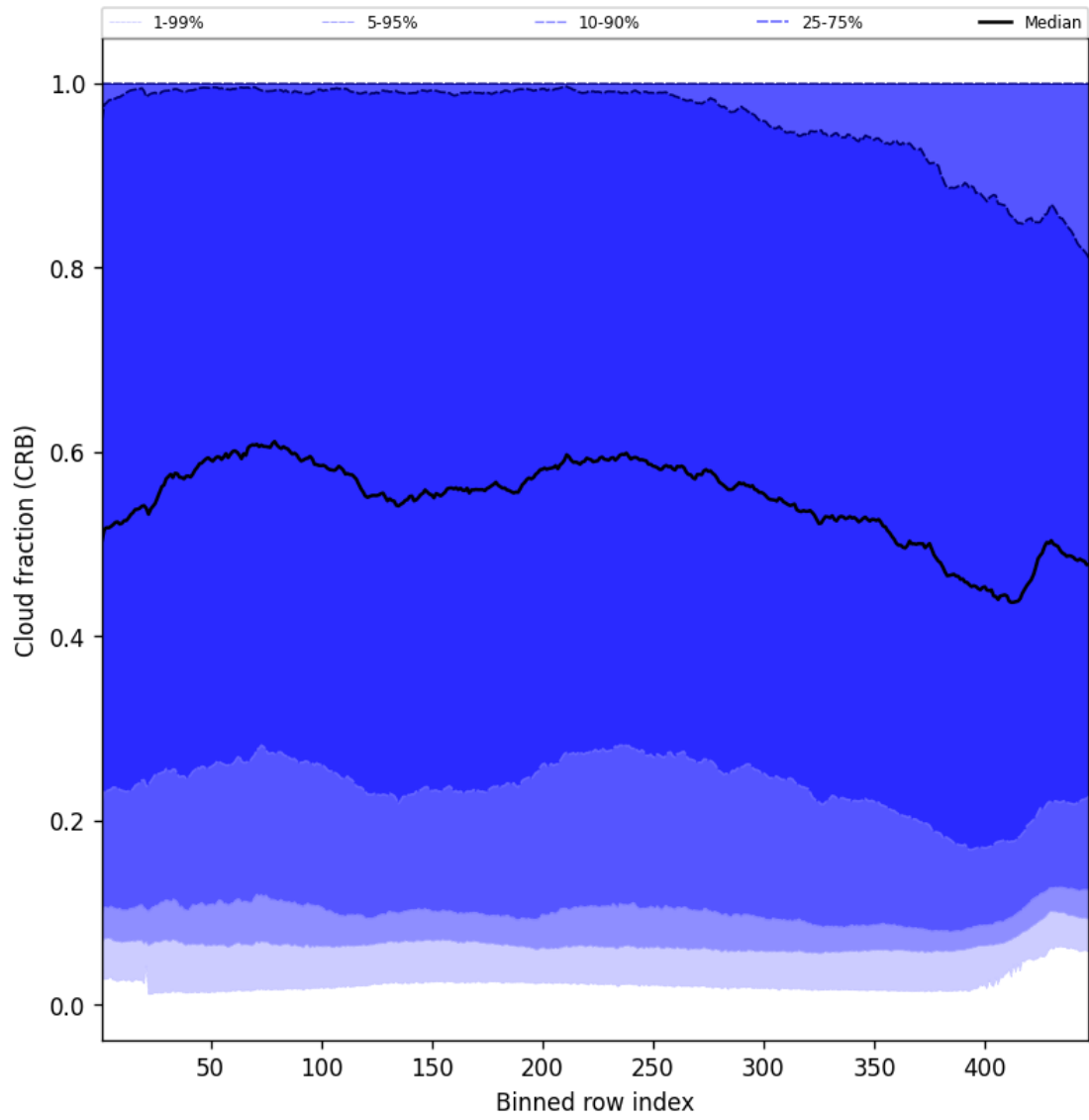
Figure 58: Along track statistics of “Cloud fraction (CRB)” for 2024-09-13 to 2024-09-15
