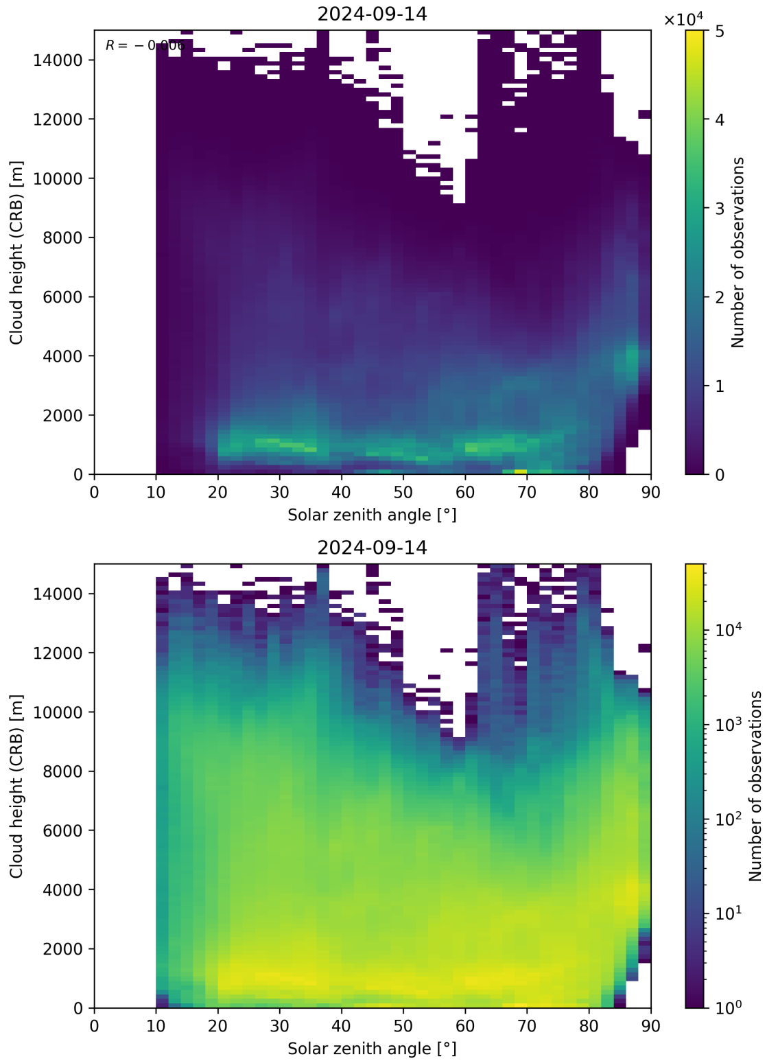
Figure 102: Scatter density plot of “Solar zenith angle” against “Cloud height (CRB)” for 2024-09-13 to 2024-09-15.
