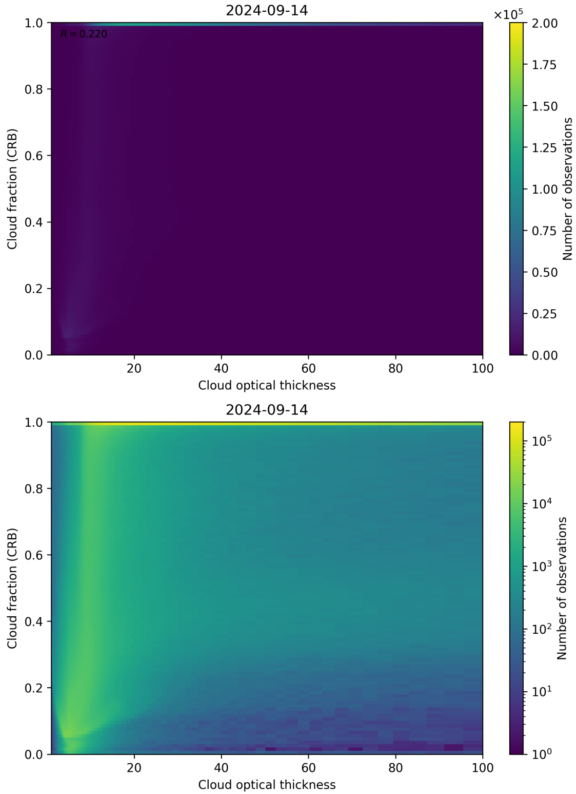
Figure 84: Scatter density plot of “Cloud optical thickness” against “Cloud fraction (CRB)” for 2024-09-13 to 2024-09-15.
