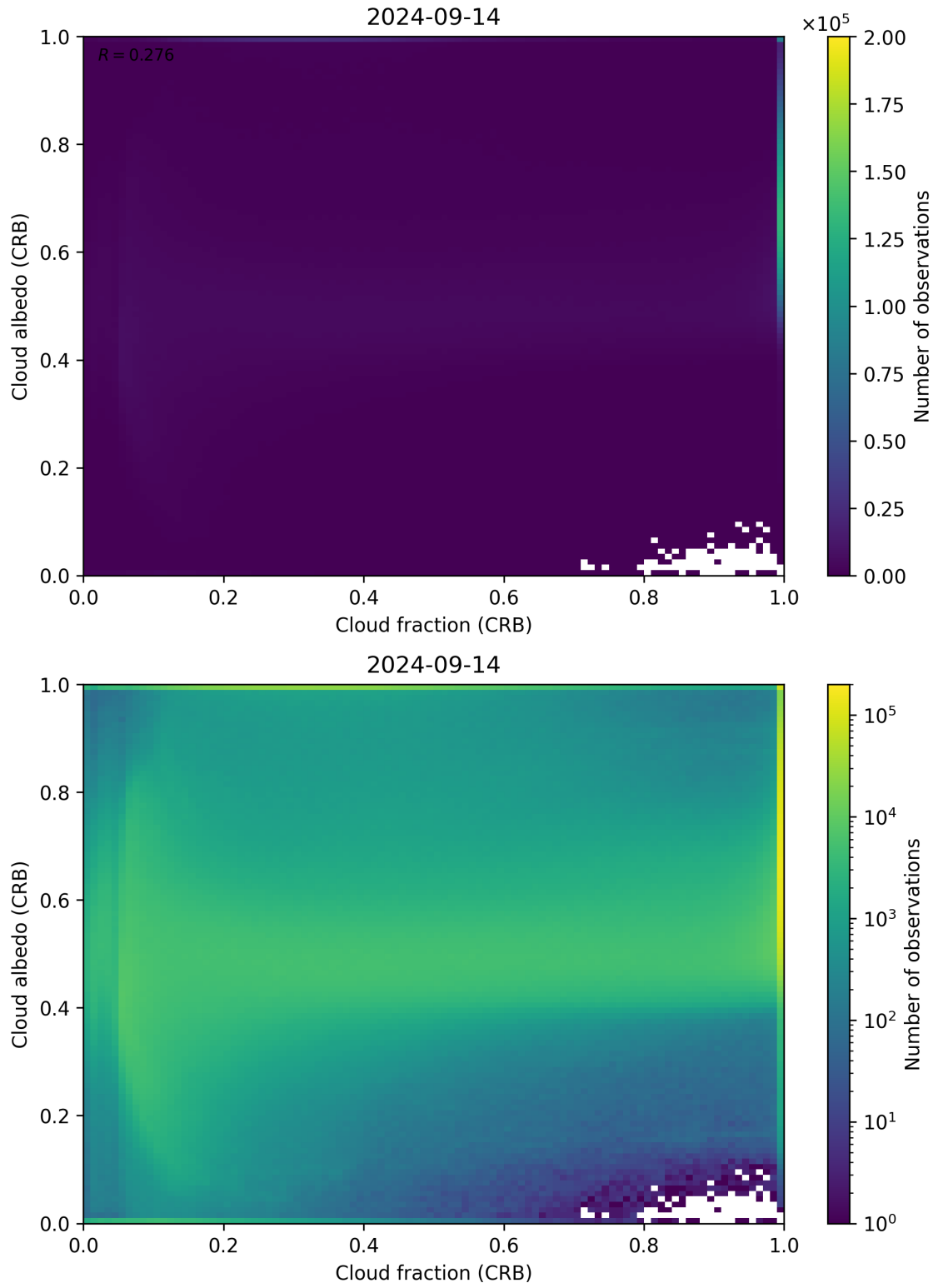
Figure 77: Scatter density plot of “Cloud fraction (CRB)” against “Cloud albedo (CRB)” for 2024-09-13 to 2024-09-15.
