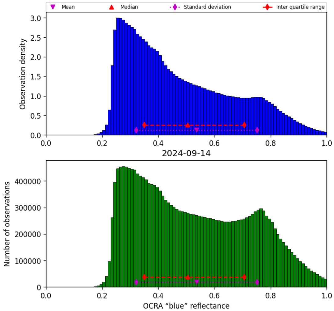
Figure 51: Histogram of “OCRA “blue” reflectance” for 2024-09-13 to 2024-09-15
