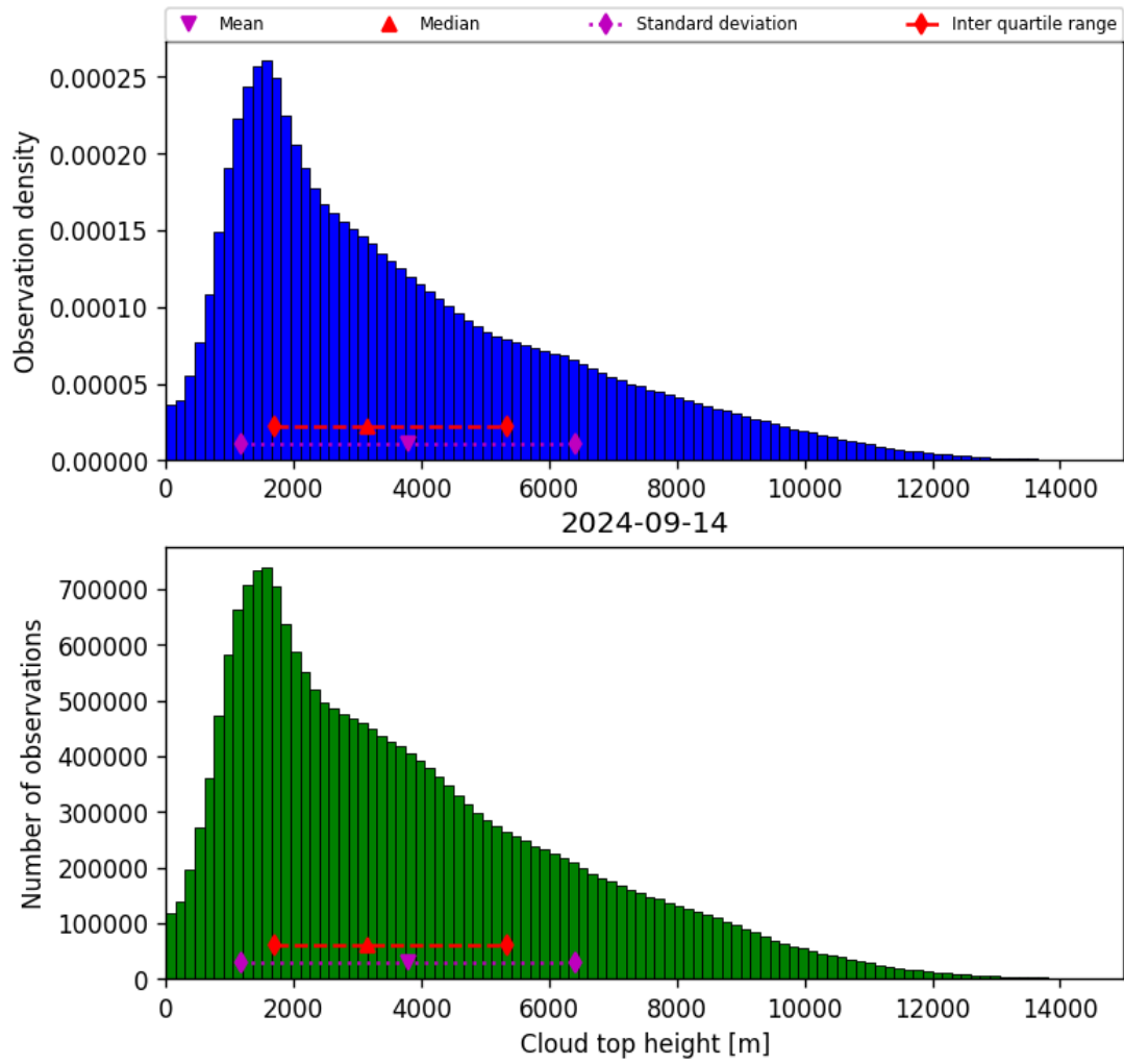
Figure 40: Histogram of “Cloud top height” for 2024-09-13 to 2024-09-15
