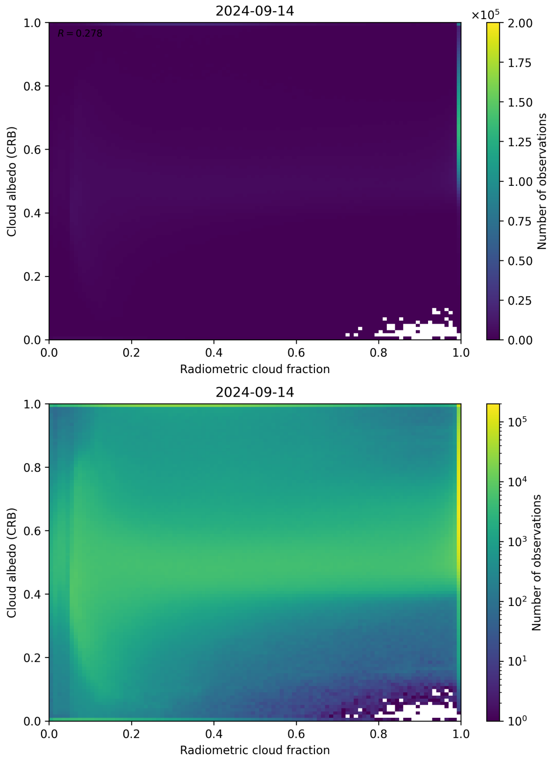
Figure 71: Scatter density plot of “Radiometric cloud fraction” against “Cloud albedo (CRB)” for 2024-09-13 to 2024-09-15.
