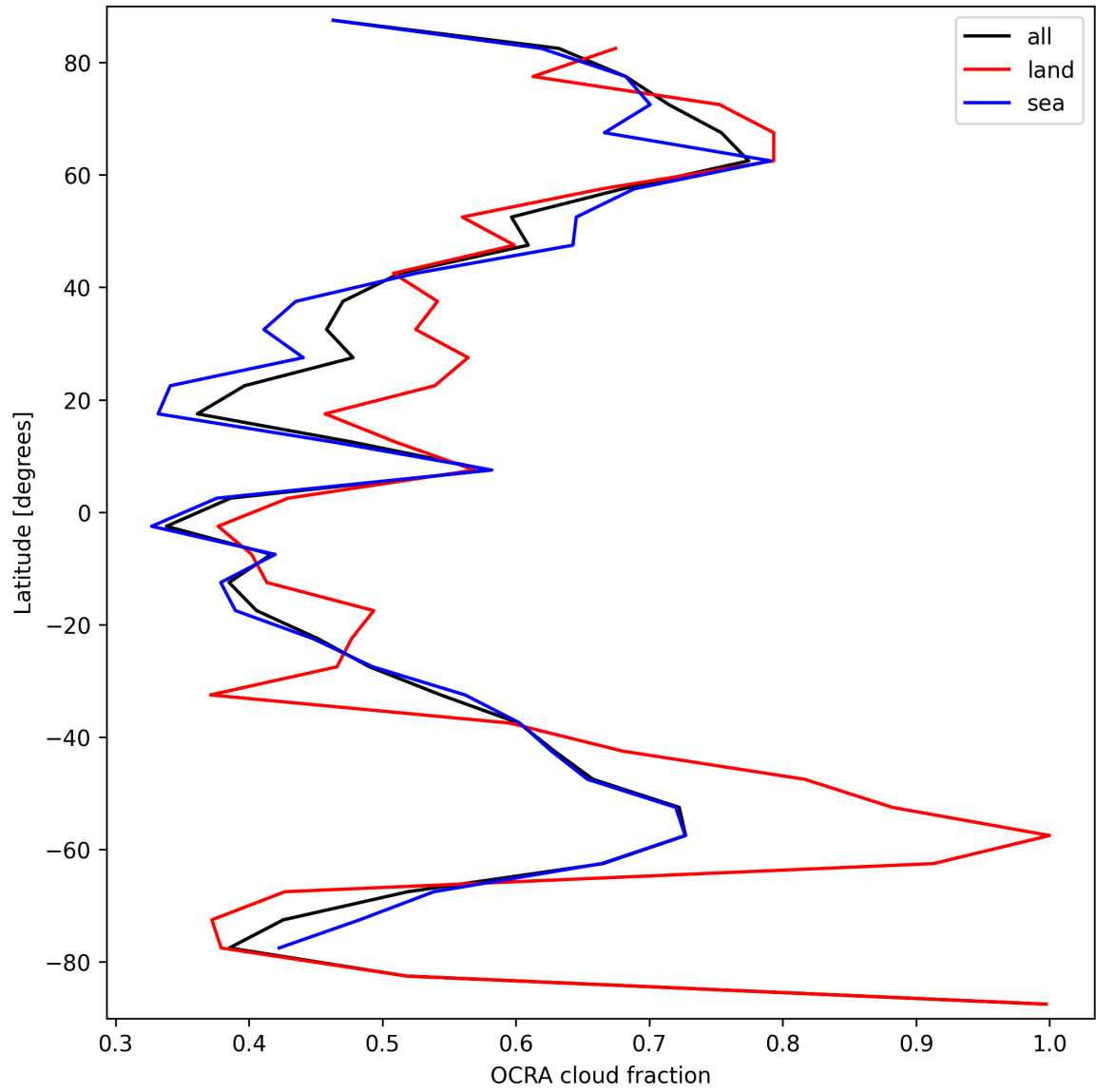
Figure 34: Zonal average of “OCRA cloud fraction” for 2024-09-13 to 2024-09-15.
