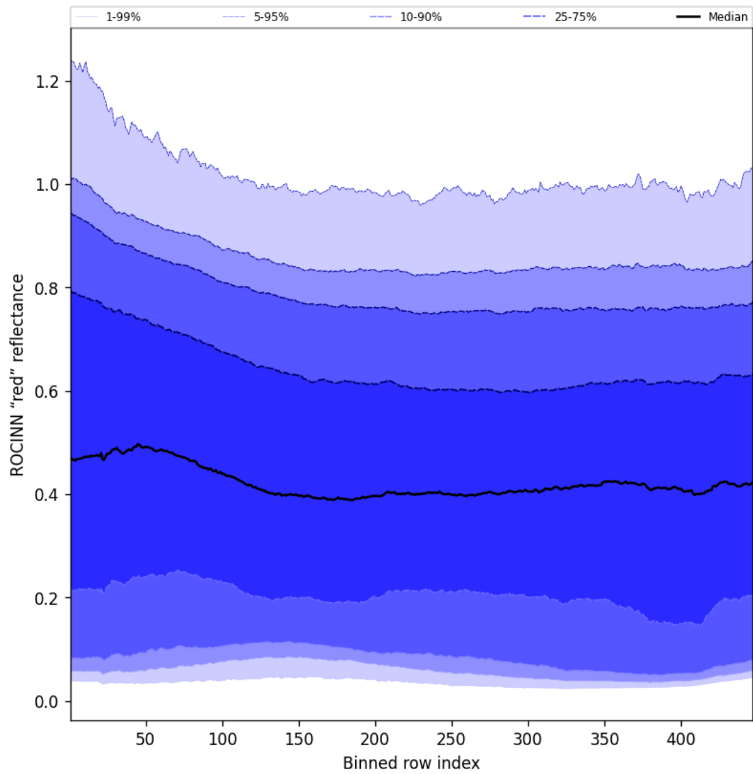
Figure 69: Along track statistics of “ROCINN “red” reflectance” for 2024-09-13 to 2024-09-15
