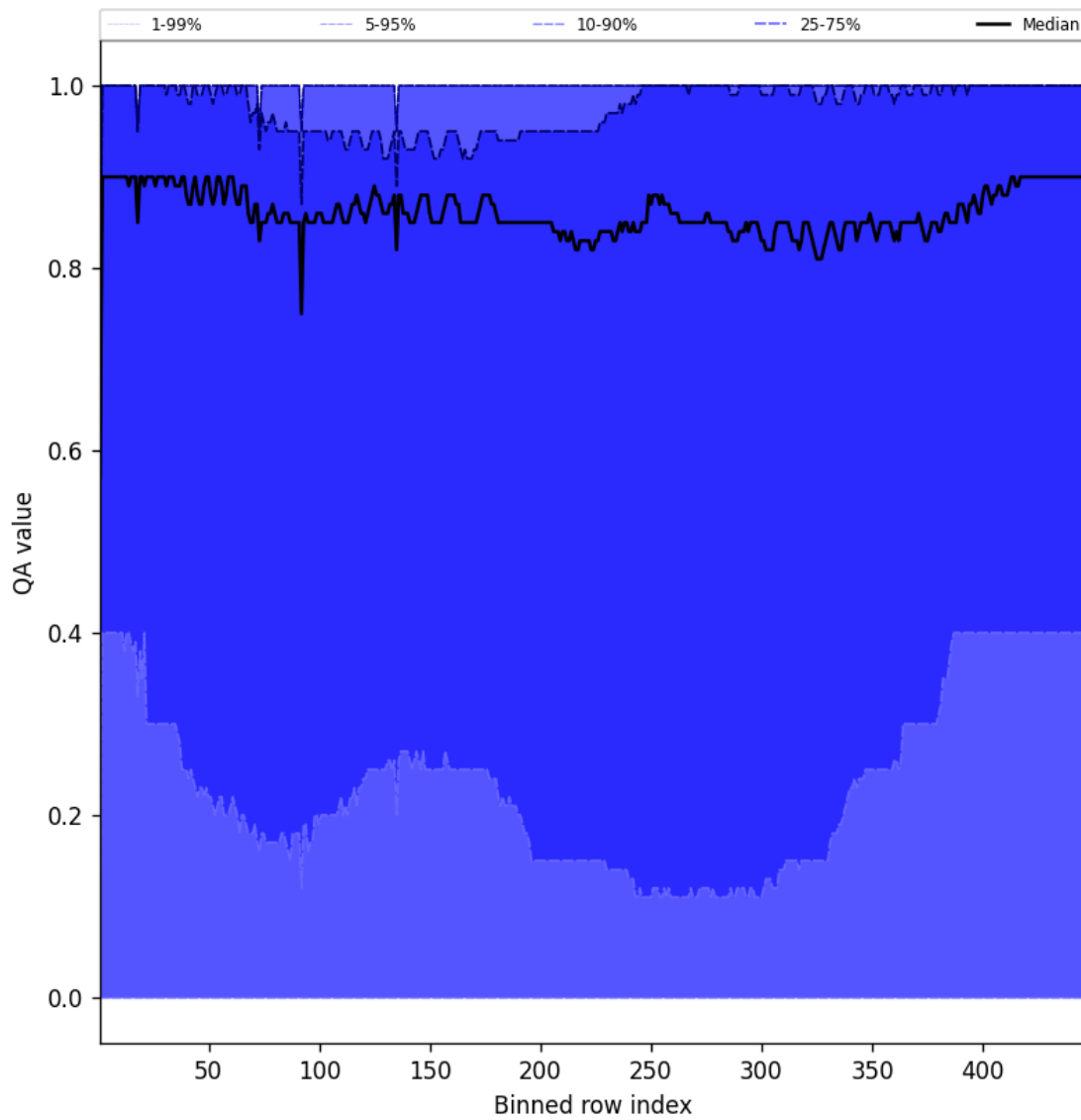
Figure 54: Along track statistics of “QA value” for 2024-09-13 to 2024-09-15
