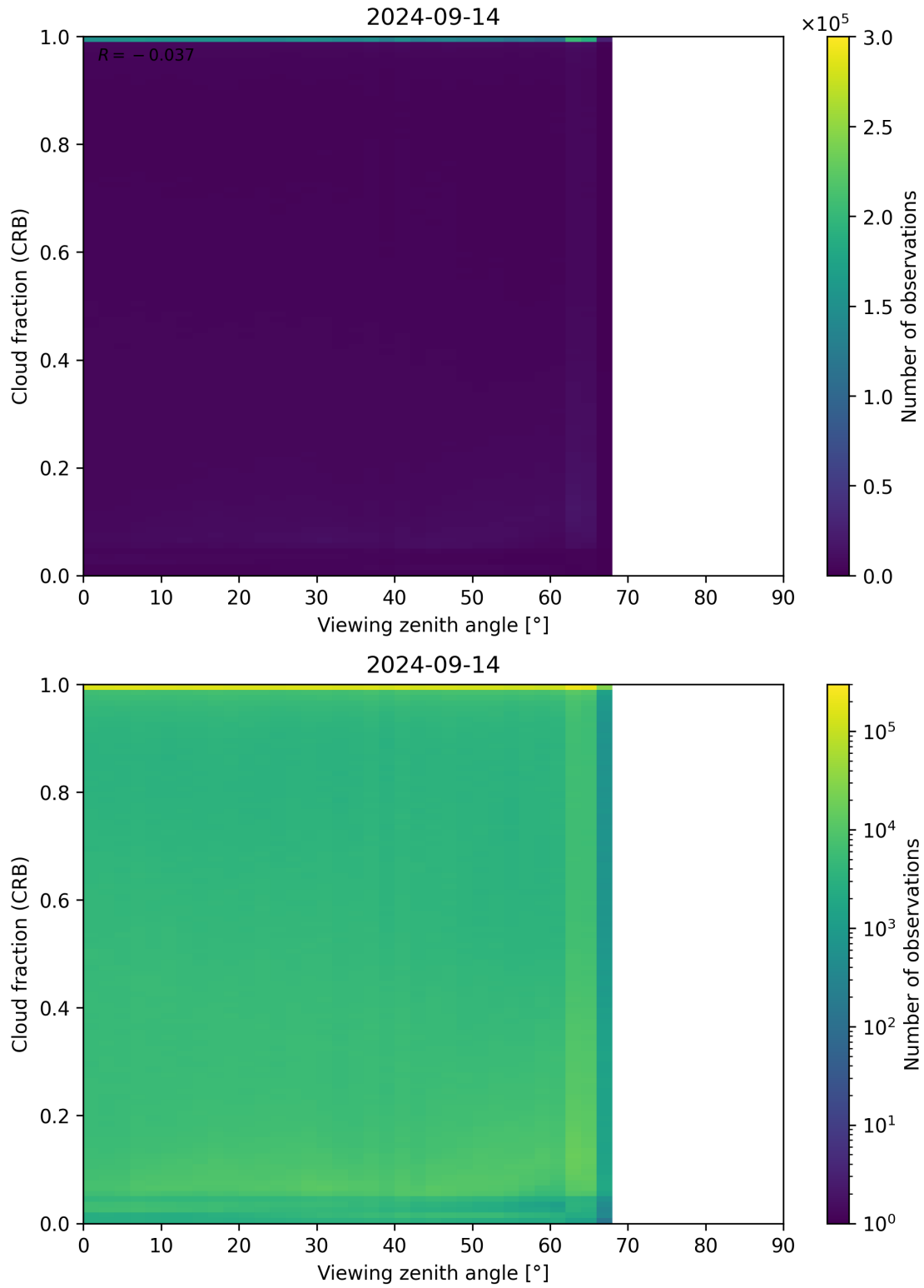
Figure 109: Scatter density plot of “Viewing zenith angle” against “Cloud fraction (CRB)” for 2024-09-13 to 2024-09-15.
