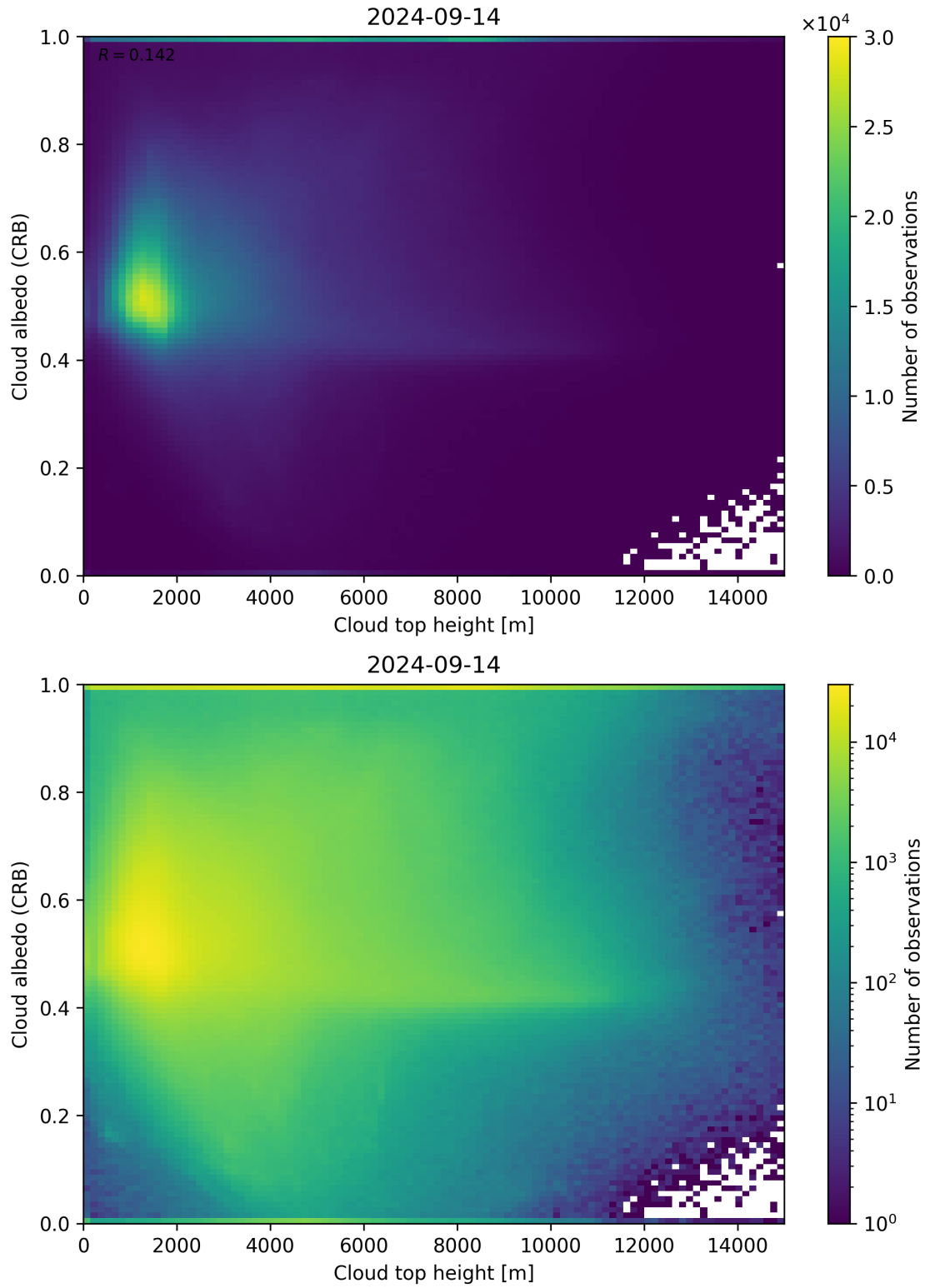
Figure 86: Scatter density plot of “Cloud top height” against “Cloud albedo (CRB)” for 2024-09-13 to 2024-09-15.
