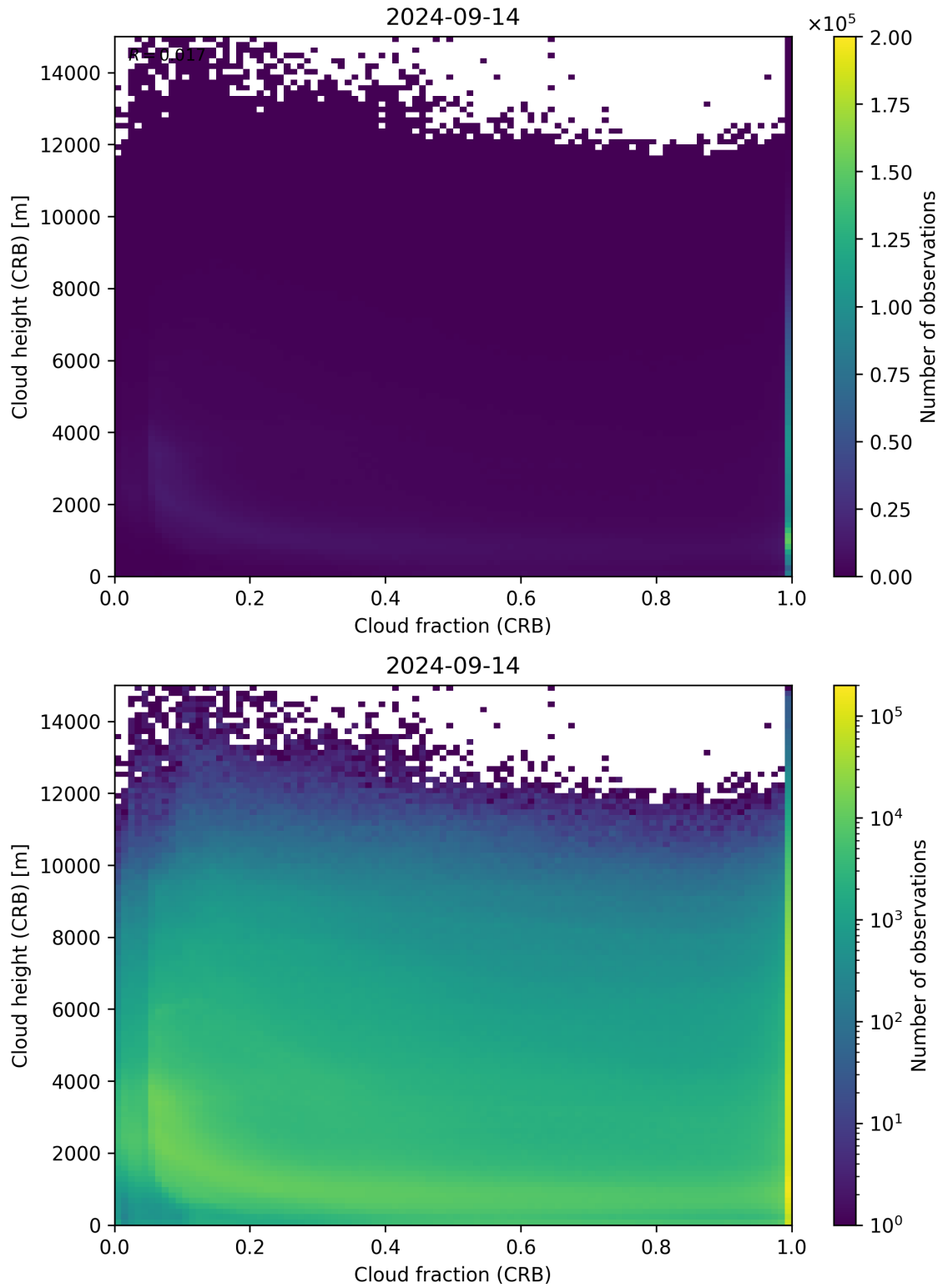
Figure 79: Scatter density plot of “Cloud fraction (CRB)” against “Cloud height (CRB)” for 2024-09-13 to 2024-09-15.
