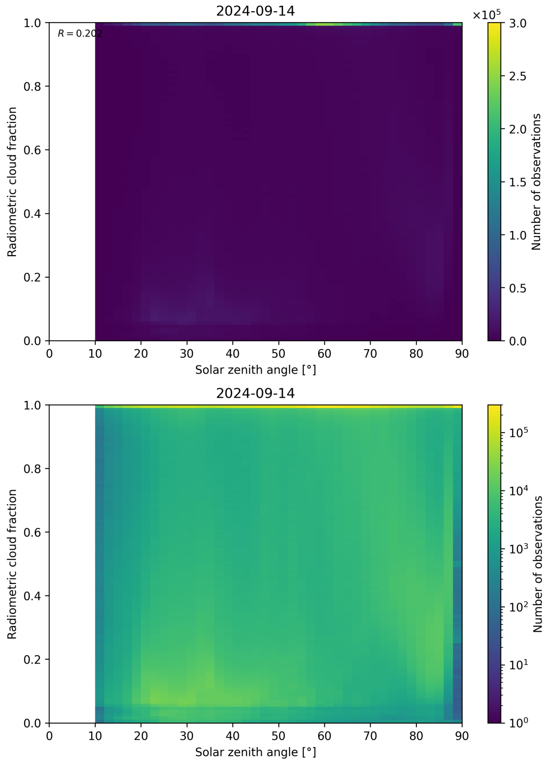
Figure 99: Scatter density plot of “Solar zenith angle” against “Radiometric cloud fraction” for 2024-09-13 to 2024-09-15.
