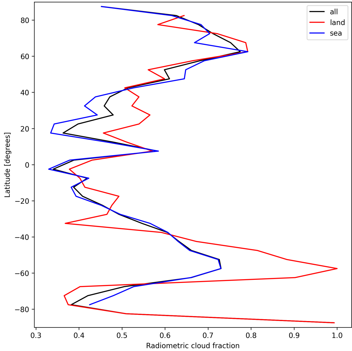
Figure 23: Zonal average of “Radiometric cloud fraction” for 2024-09-13 to 2024-09-15.
