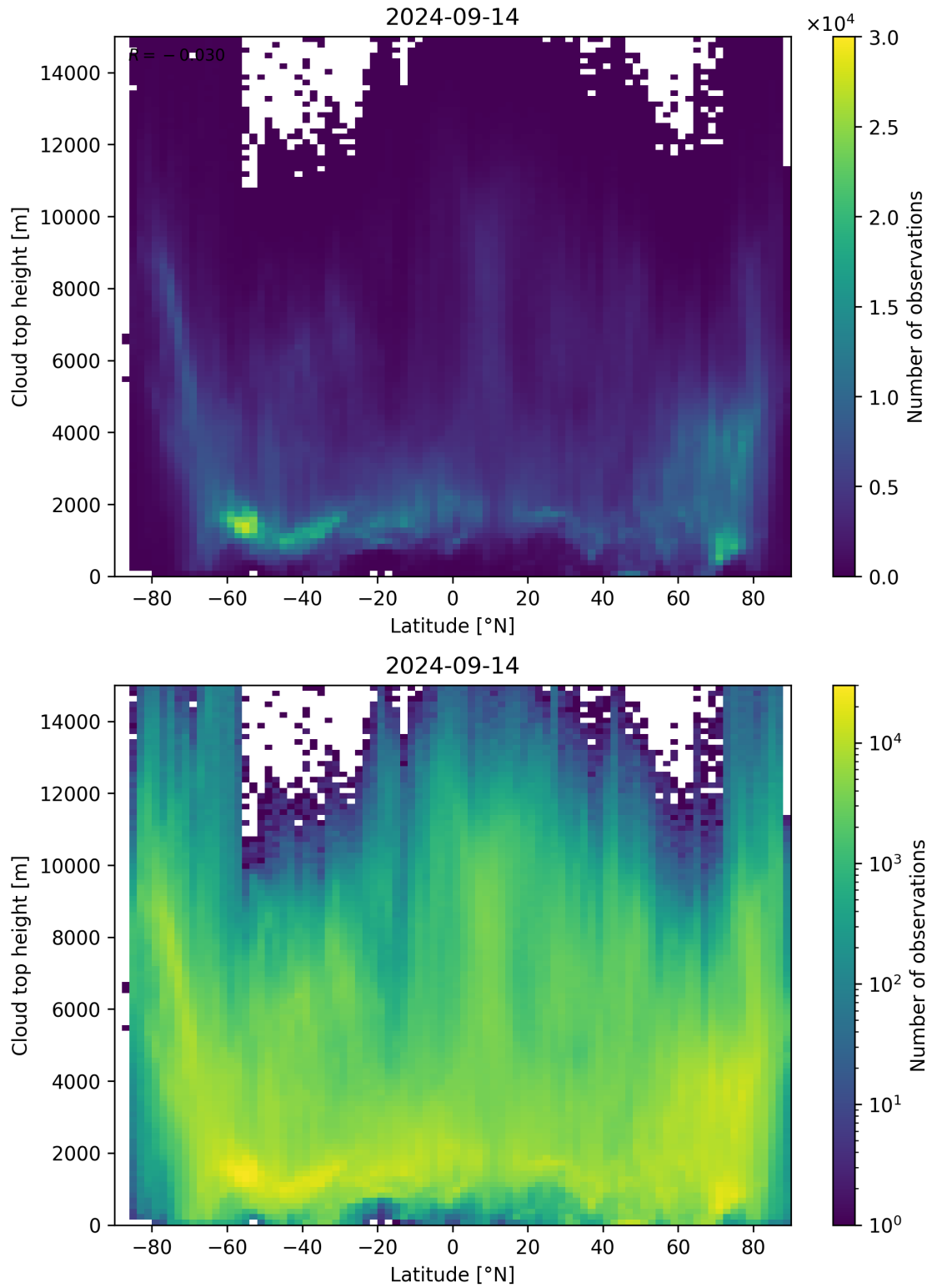
Figure 97: Scatter density plot of “Latitude” against “Cloud top height” for 2024-09-13 to 2024-09-15.
