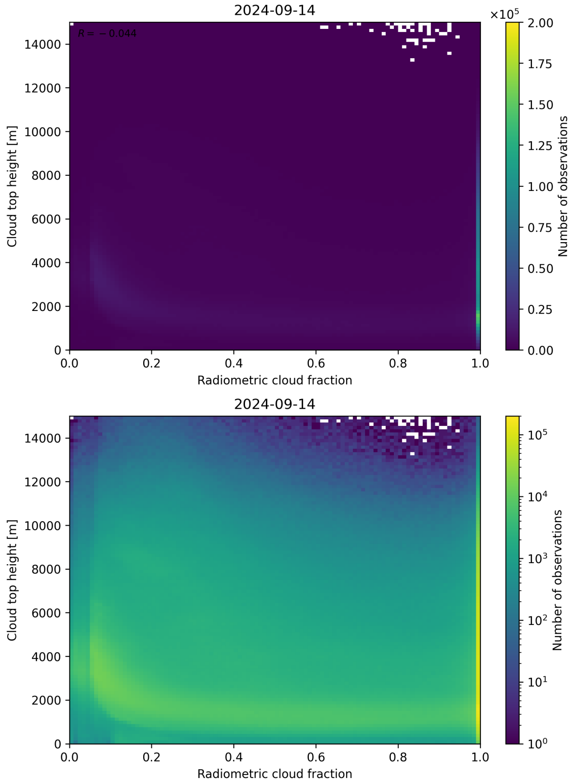
Figure 76: Scatter density plot of “Radiometric cloud fraction” against “Cloud top height” for 2024-09-13 to 2024-09-15.
