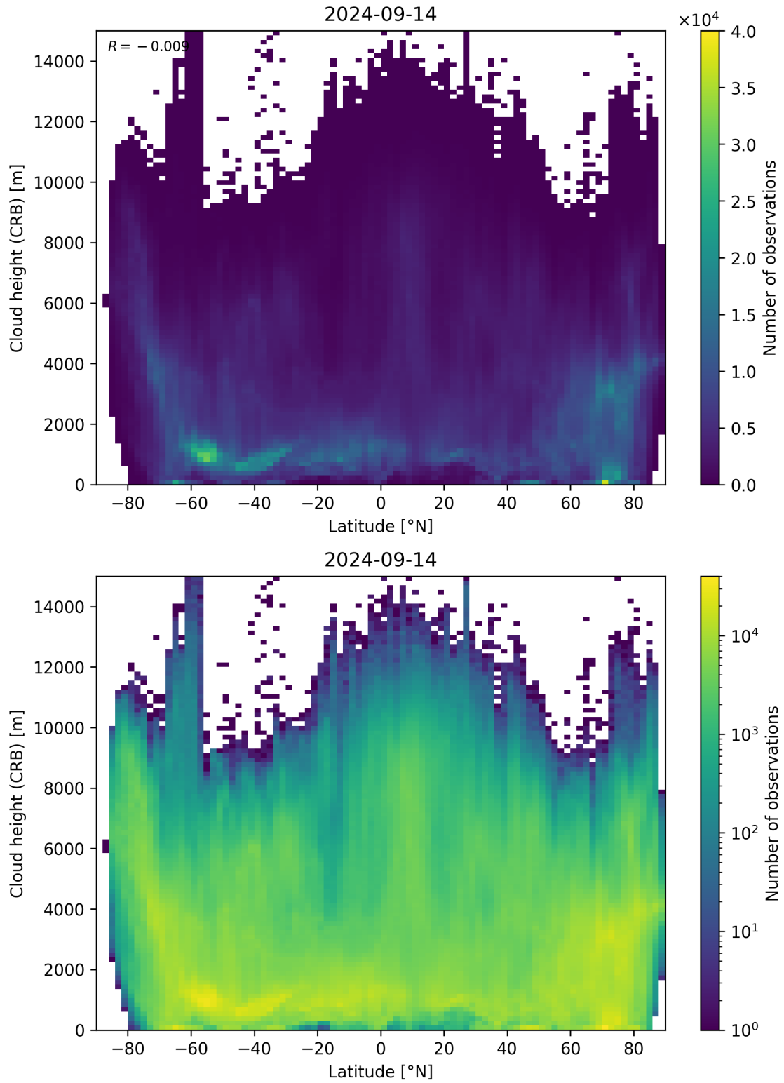
Figure 95: Scatter density plot of “Latitude” against “Cloud height (CRB)” for 2024-09-13 to 2024-09-15.
