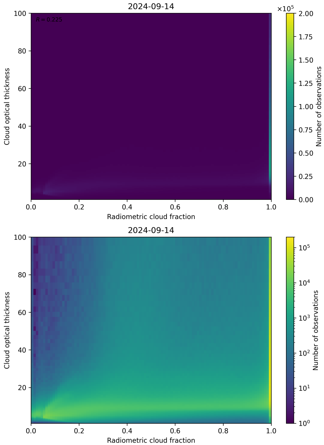
Figure 75: Scatter density plot of “Radiometric cloud fraction” against “Cloud optical thickness” for 2024-09-13 to 2024-09-15.
