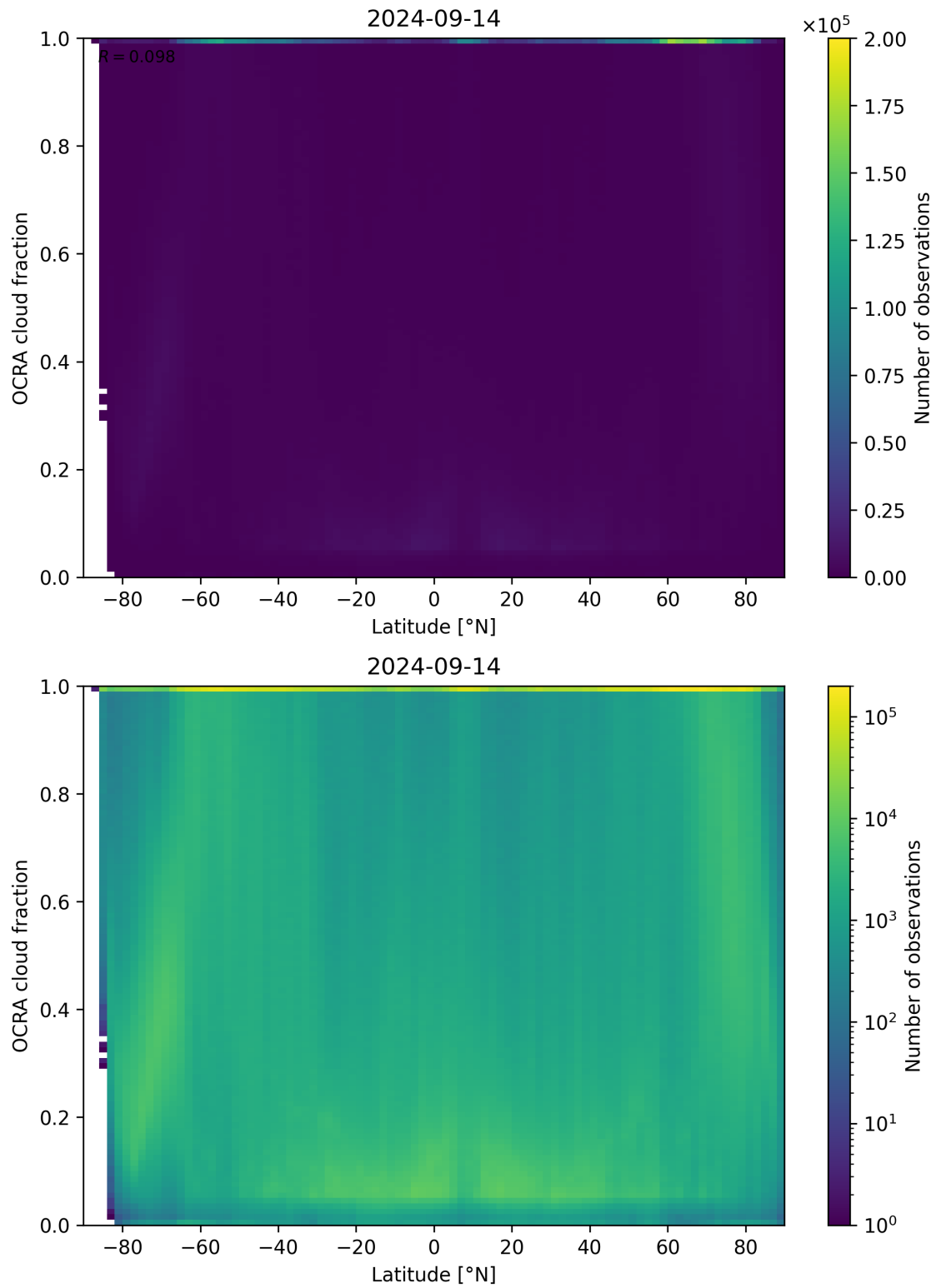
Figure 93: Scatter density plot of “Latitude” against “OCRA cloud fraction” for 2024-09-13 to 2024-09-15.
