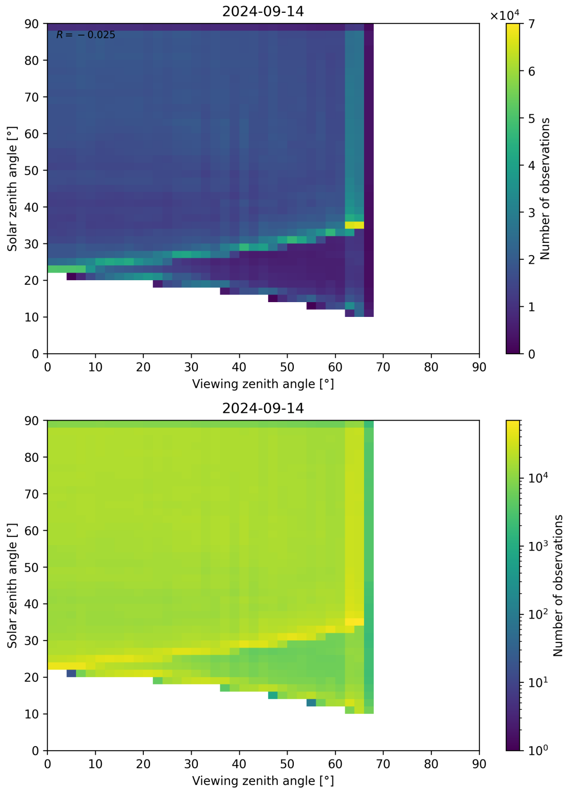
Figure 114: Scatter density plot of “Viewing zenith angle” against “Solar zenith angle” for 2024-09-13 to 2024-09-15.
