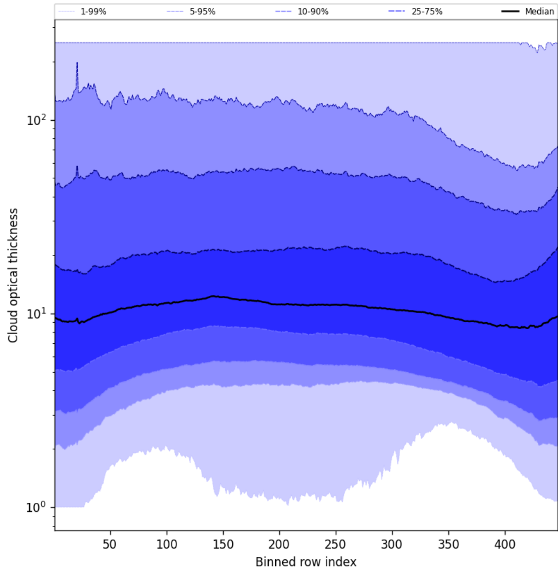
Figure 57: Along track statistics of “Cloud optical thickness” for 2024-09-14 to 2024-09-16
