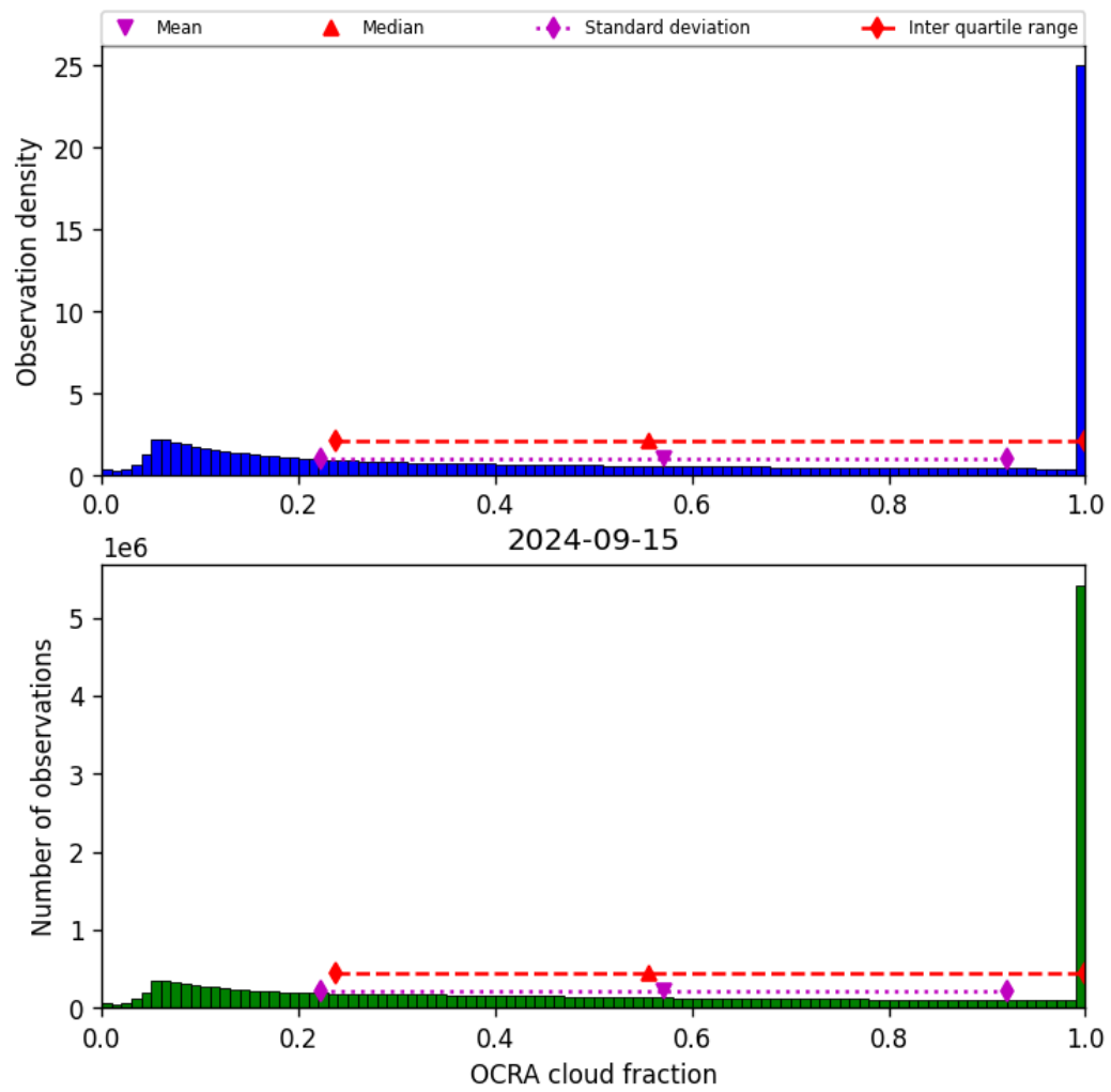
Figure 50: Histogram of “OCRA cloud fraction” for 2024-09-14 to 2024-09-16
