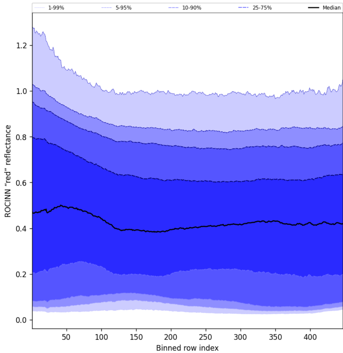
Figure 69: Along track statistics of “ROCINN “red” reflectance” for 2024-09-14 to 2024-09-16
