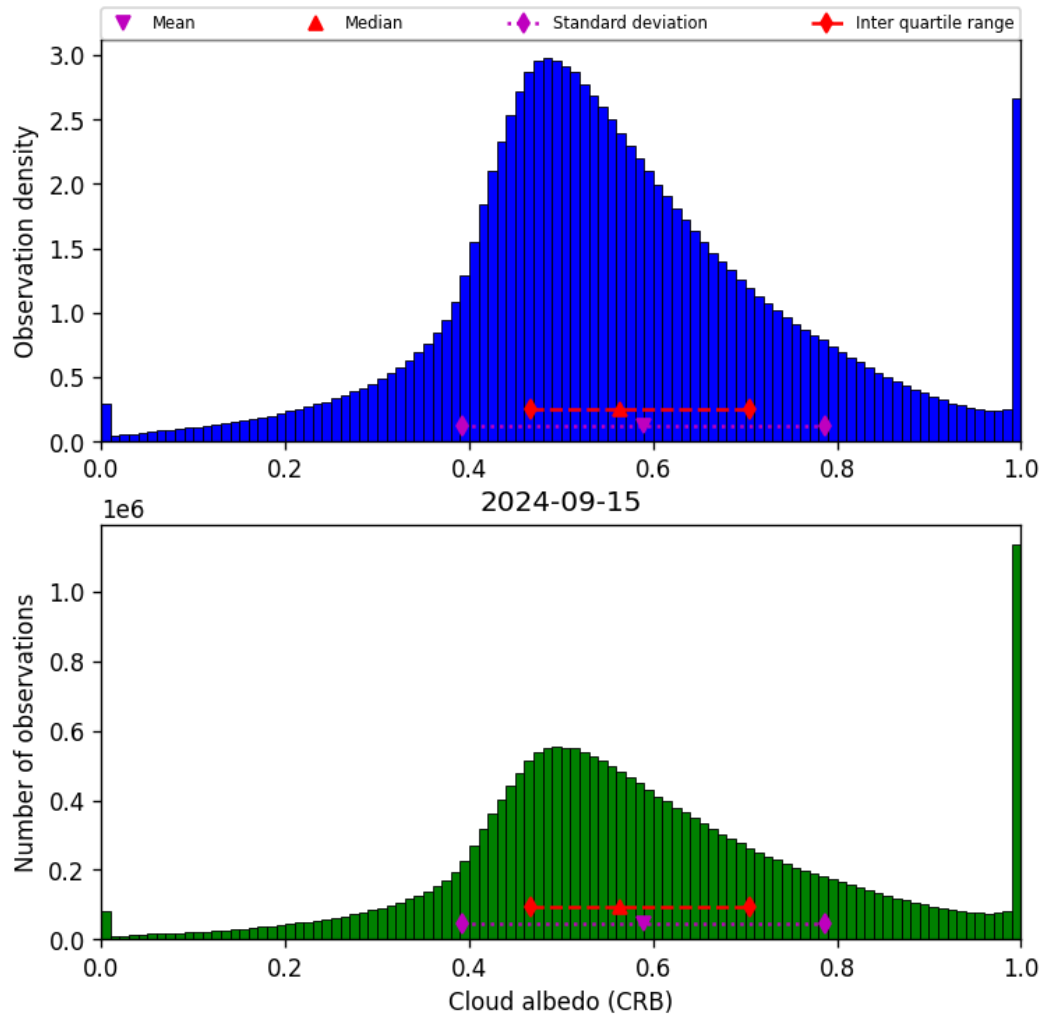
Figure 44: Histogram of “Cloud albedo (CRB)” for 2024-09-14 to 2024-09-16
