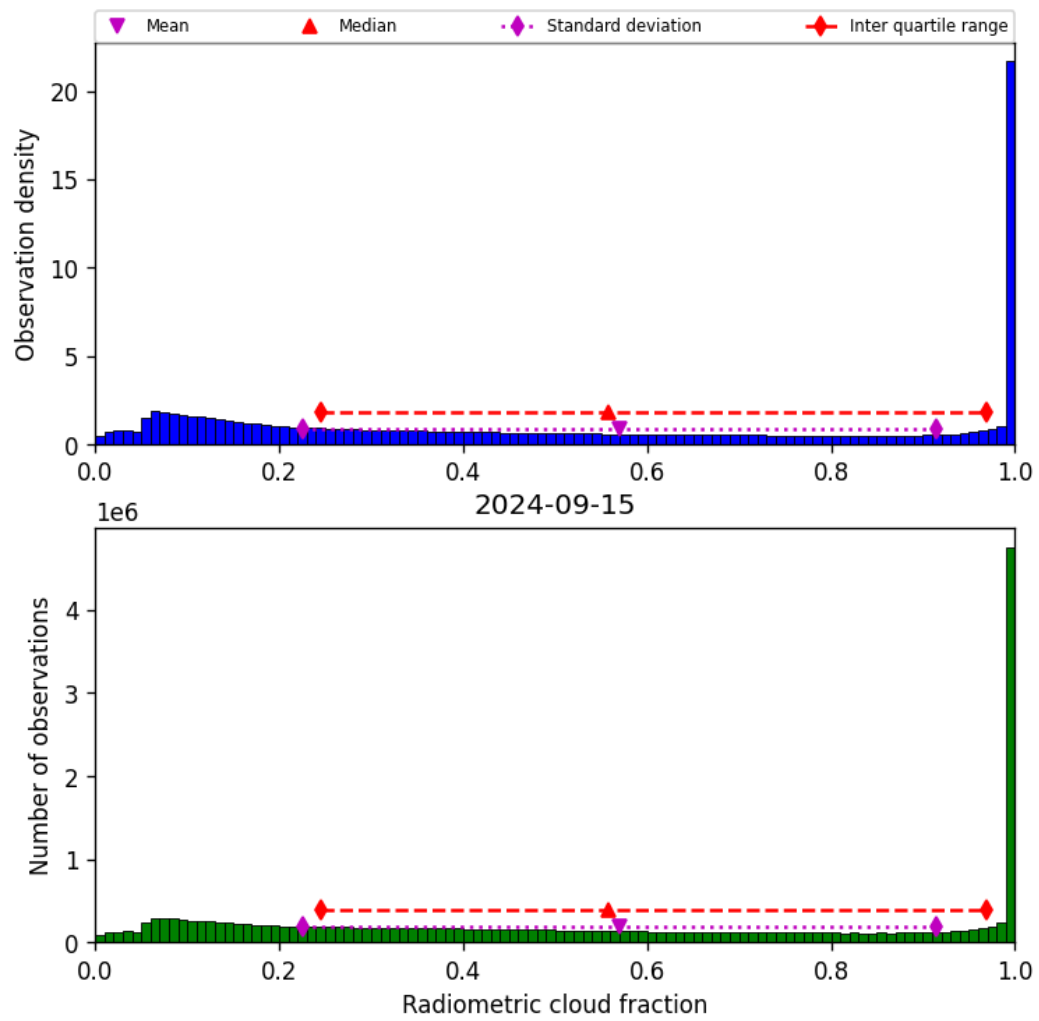
Figure 39: Histogram of “Radiometric cloud fraction” for 2024-09-14 to 2024-09-16
