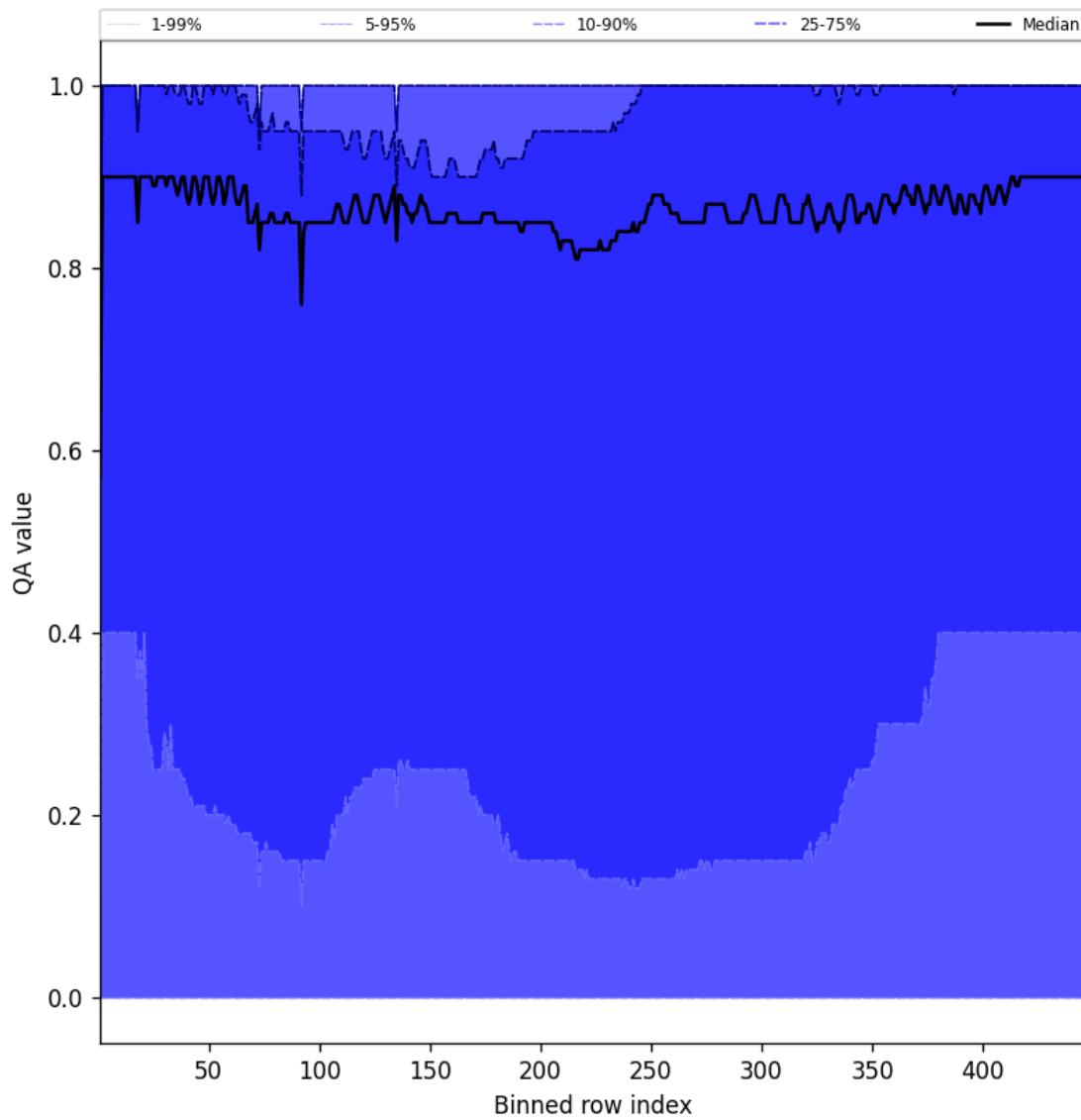
Figure 54: Along track statistics of “QA value” for 2024-09-14 to 2024-09-16
