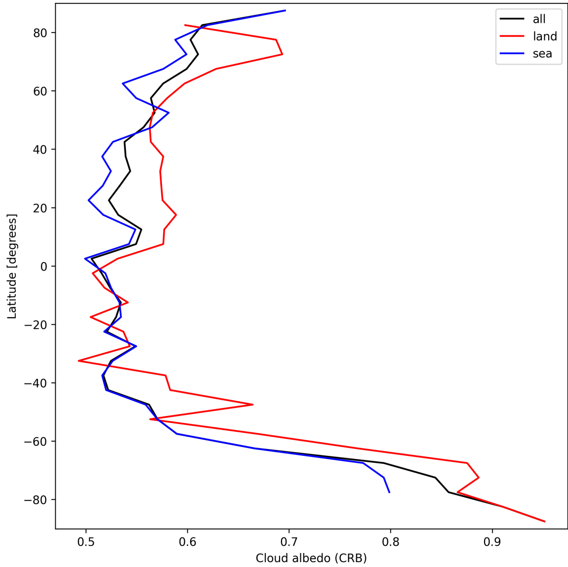
Figure 28: Zonal average of “Cloud albedo (CRB)” for 2024-09-14 to 2024-09-16.
