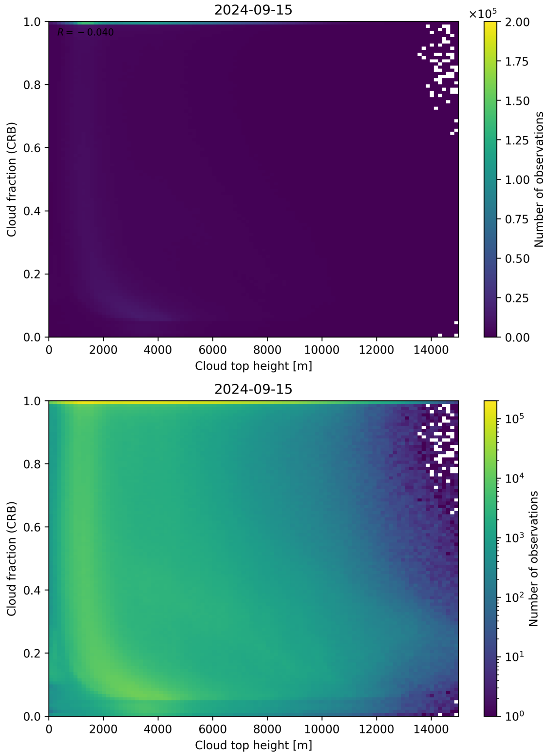
Figure 88: Scatter density plot of “Cloud top height” against “Cloud fraction (CRB)” for 2024-09-14 to 2024-09-16.
