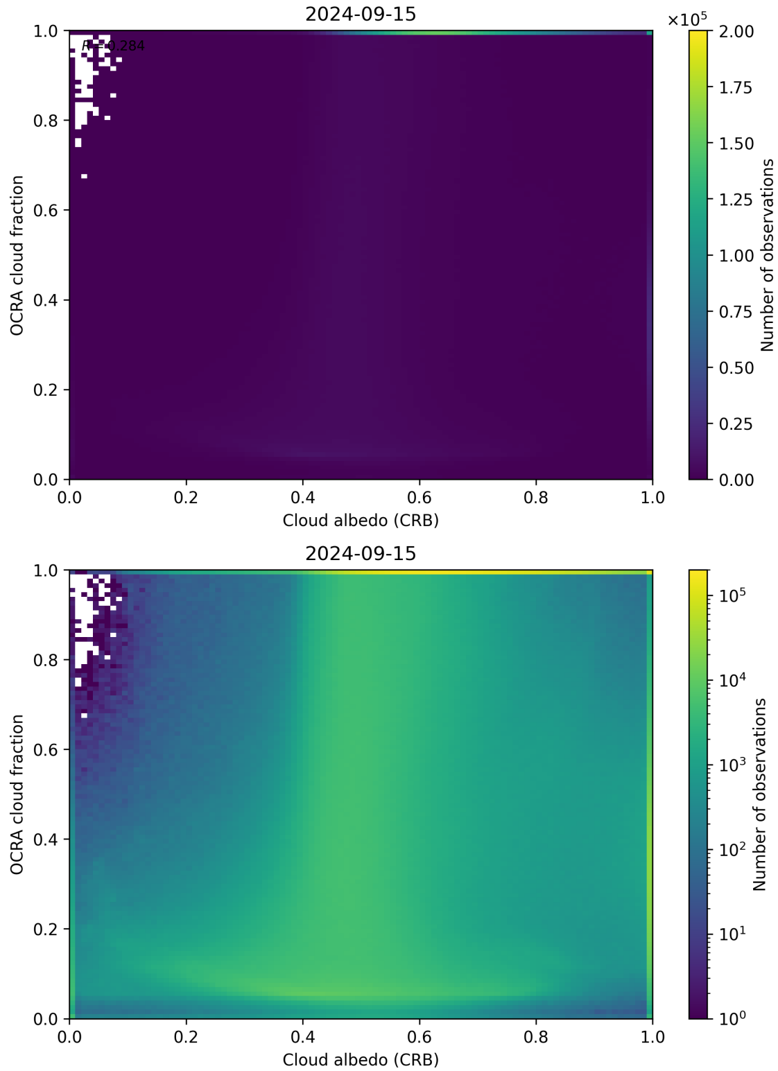
Figure 70: Scatter density plot of “Cloud albedo (CRB)” against “OCRA cloud fraction” for 2024-09-14 to 2024-09-16.
