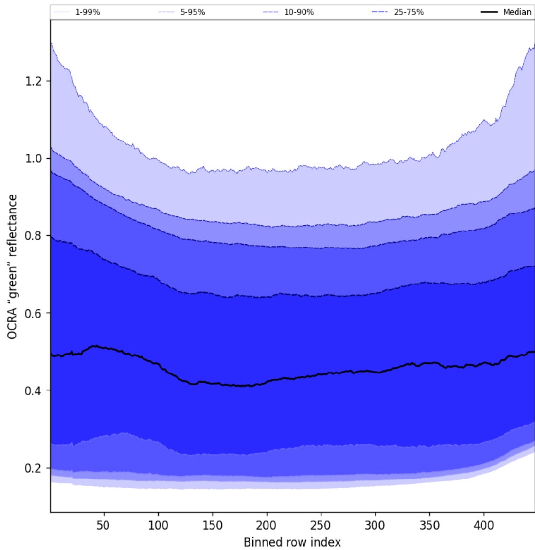
Figure 68: Along track statistics of “OCRA “green” reflectance” for 2024-09-14 to 2024-09-16
