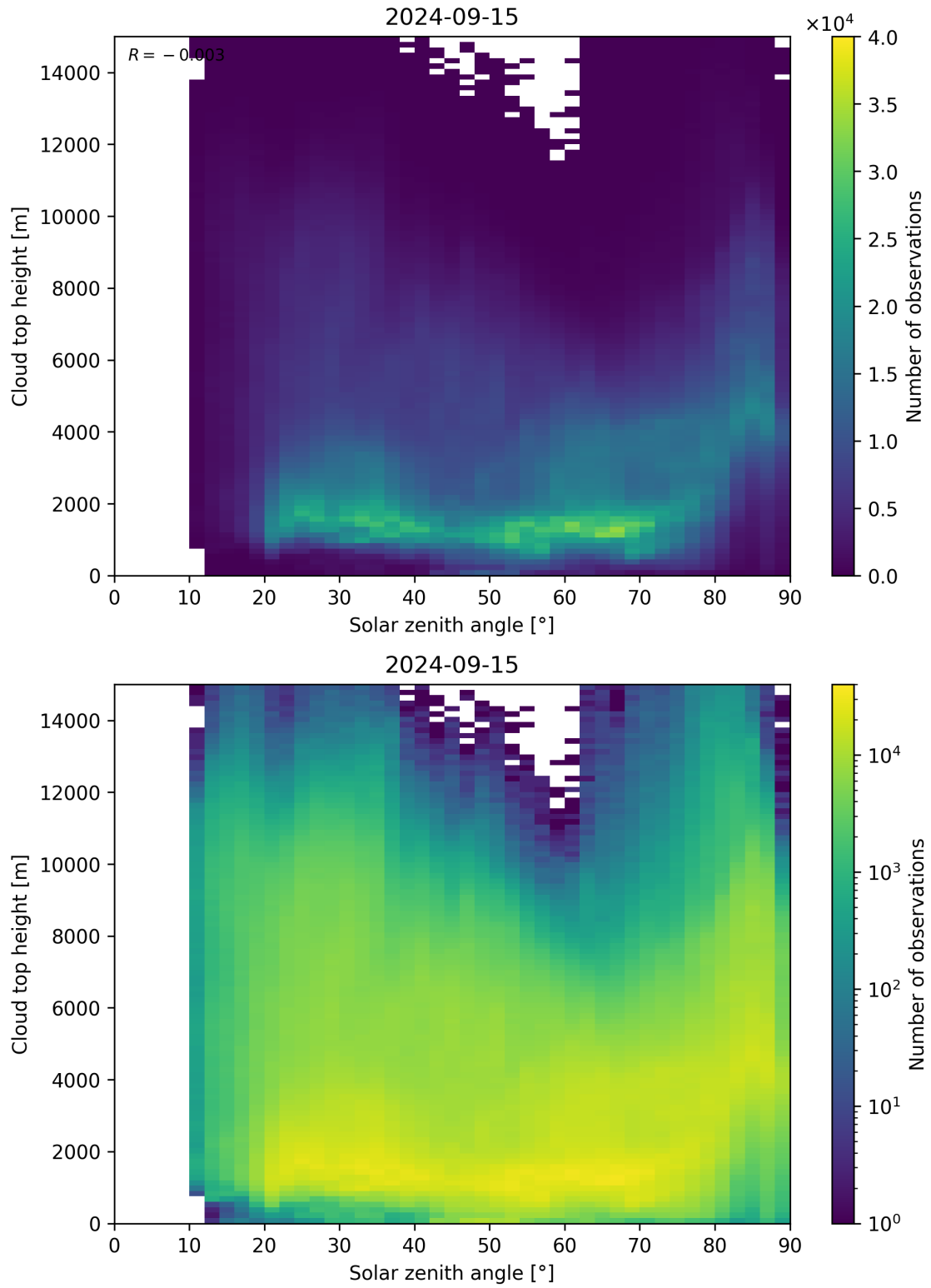
Figure 104: Scatter density plot of “Solar zenith angle” against “Cloud top height” for 2024-09-14 to 2024-09-16.
