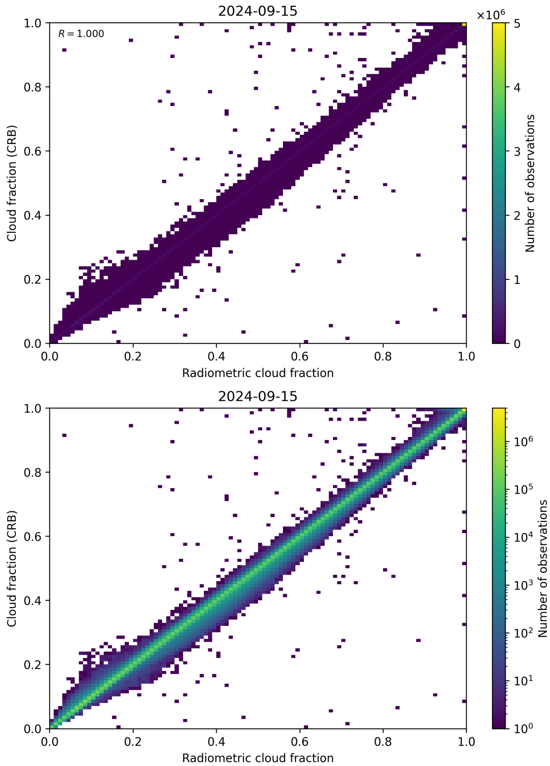
Figure 73: Scatter density plot of “Radiometric cloud fraction” against “Cloud fraction (CRB)” for 2024-09-14 to 2024-09-16.
