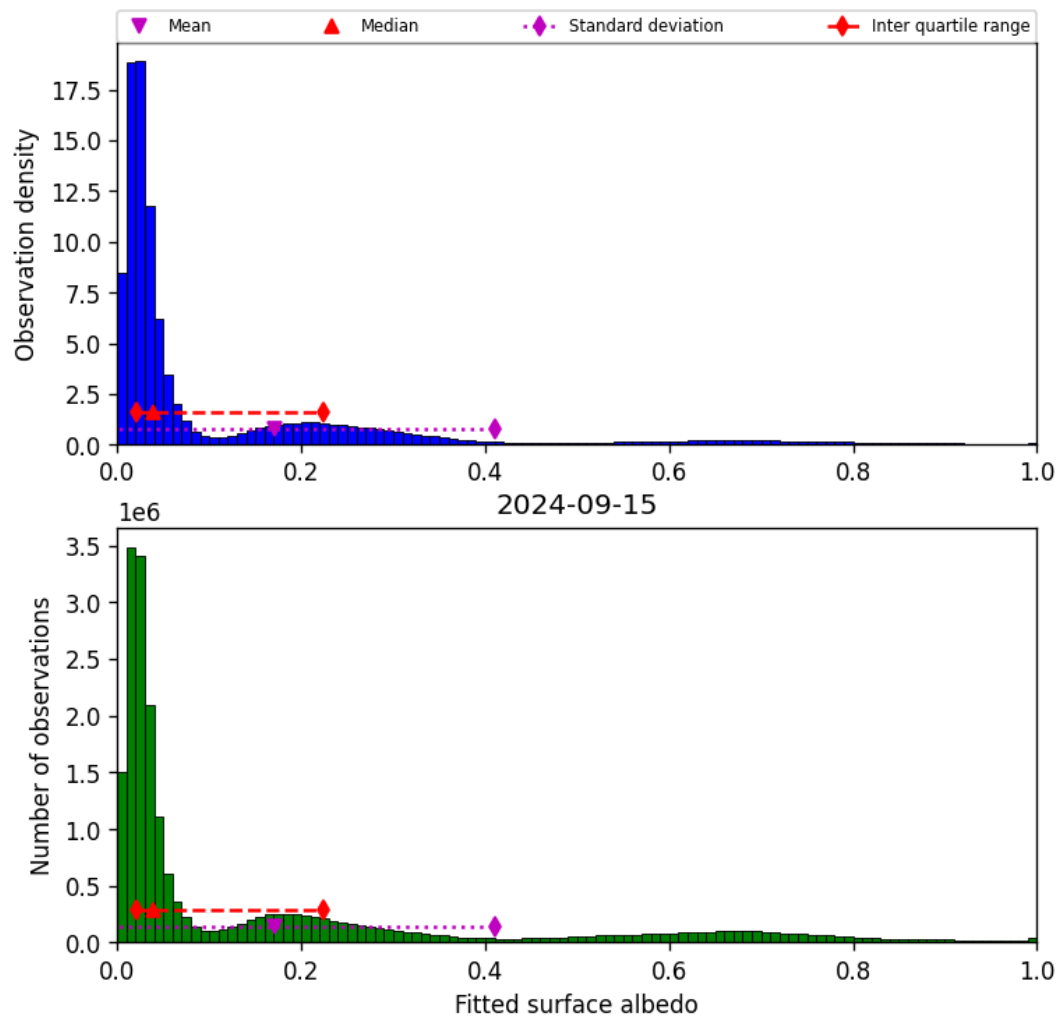
Figure 45: Histogram of “Fitted surface albedo” for 2024-09-14 to 2024-09-16
