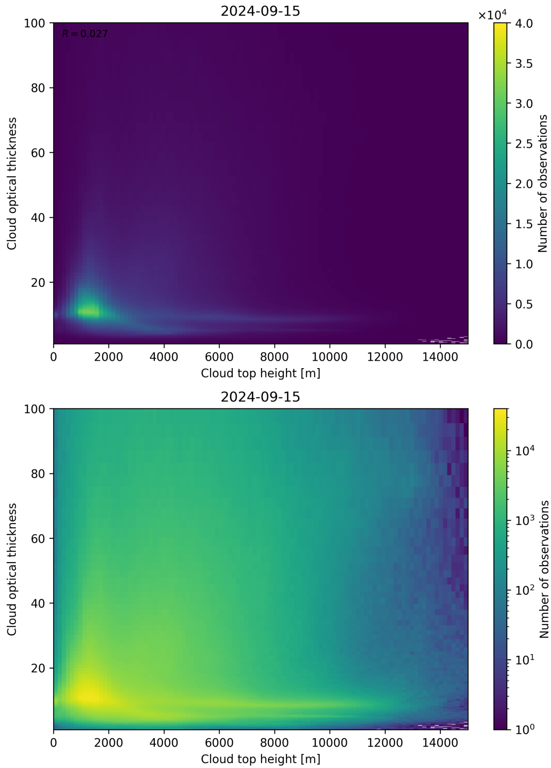
Figure 90: Scatter density plot of “Cloud top height” against “Cloud optical thickness” for 2024-09-14 to 2024-09-16.
