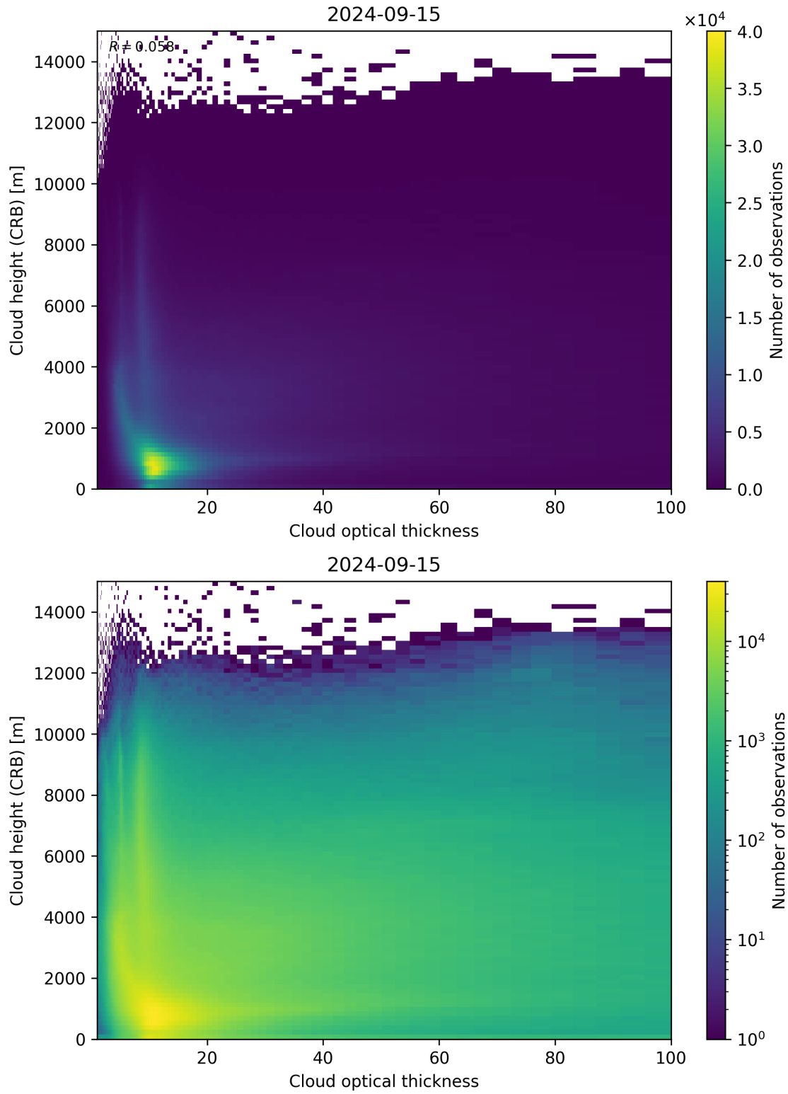
Figure 85: Scatter density plot of “Cloud optical thickness” against “Cloud height (CRB)” for 2024-09-14 to 2024-09-16.
