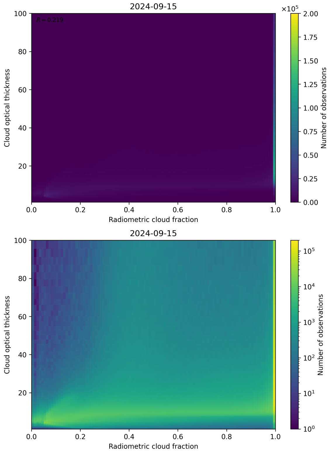
Figure 75: Scatter density plot of “Radiometric cloud fraction” against “Cloud optical thickness” for 2024-09-14 to 2024-09-16.
