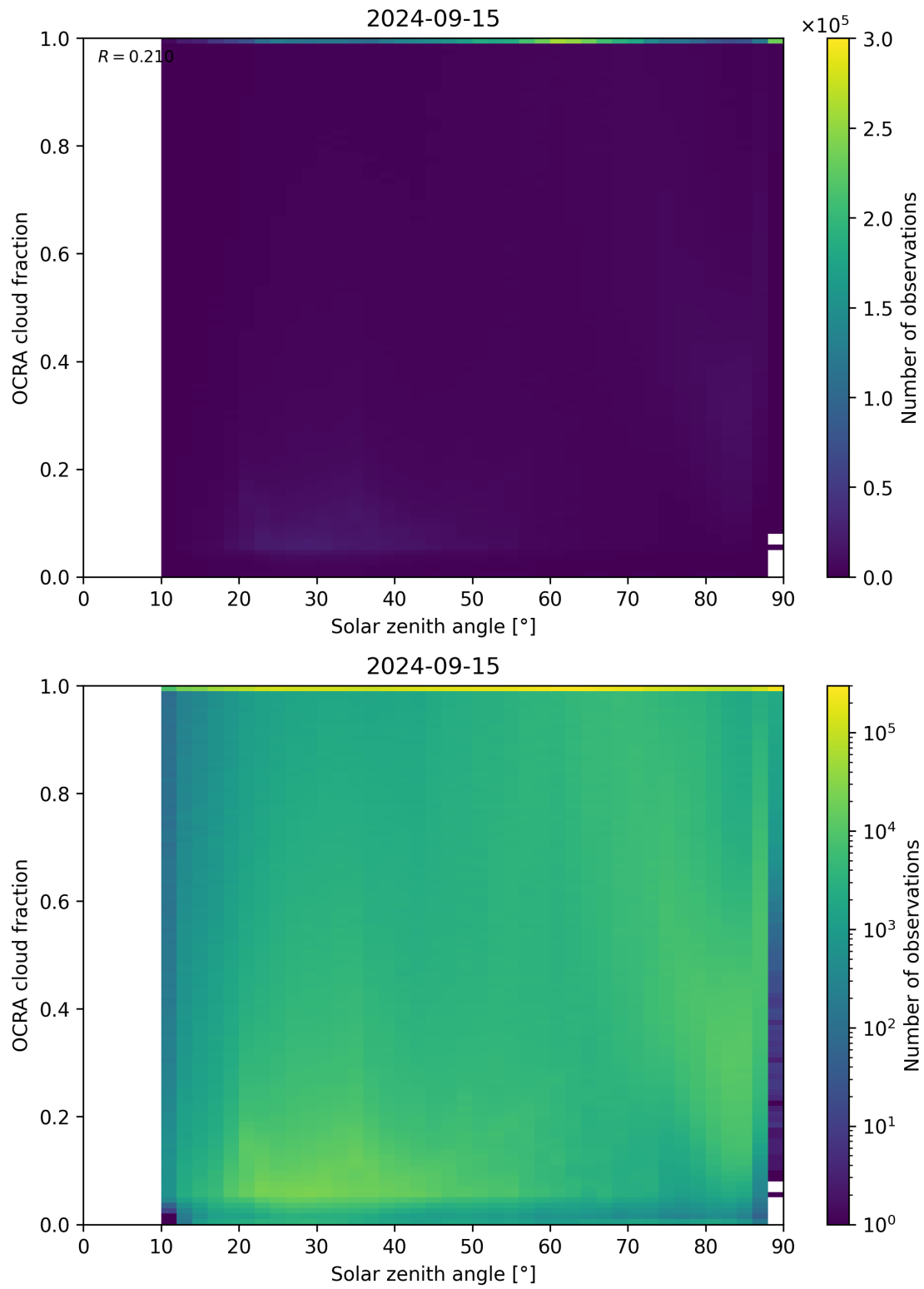
Figure 100: Scatter density plot of “Solar zenith angle” against “OCRA cloud fraction” for 2024-09-14 to 2024-09-16.
