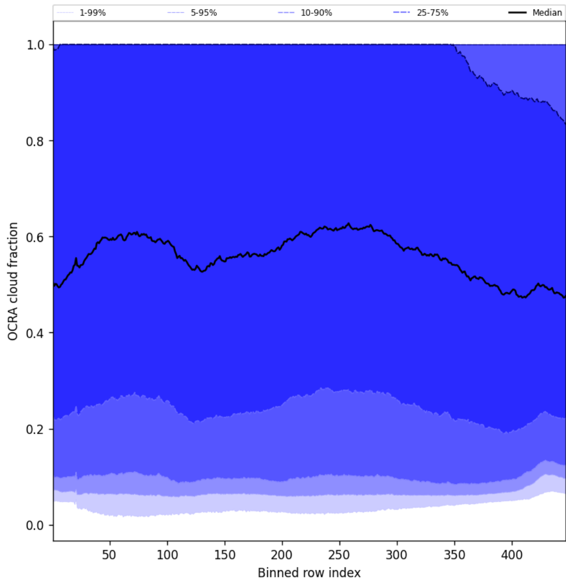
Figure 66: Along track statistics of “OCRA cloud fraction” for 2024-09-14 to 2024-09-16
