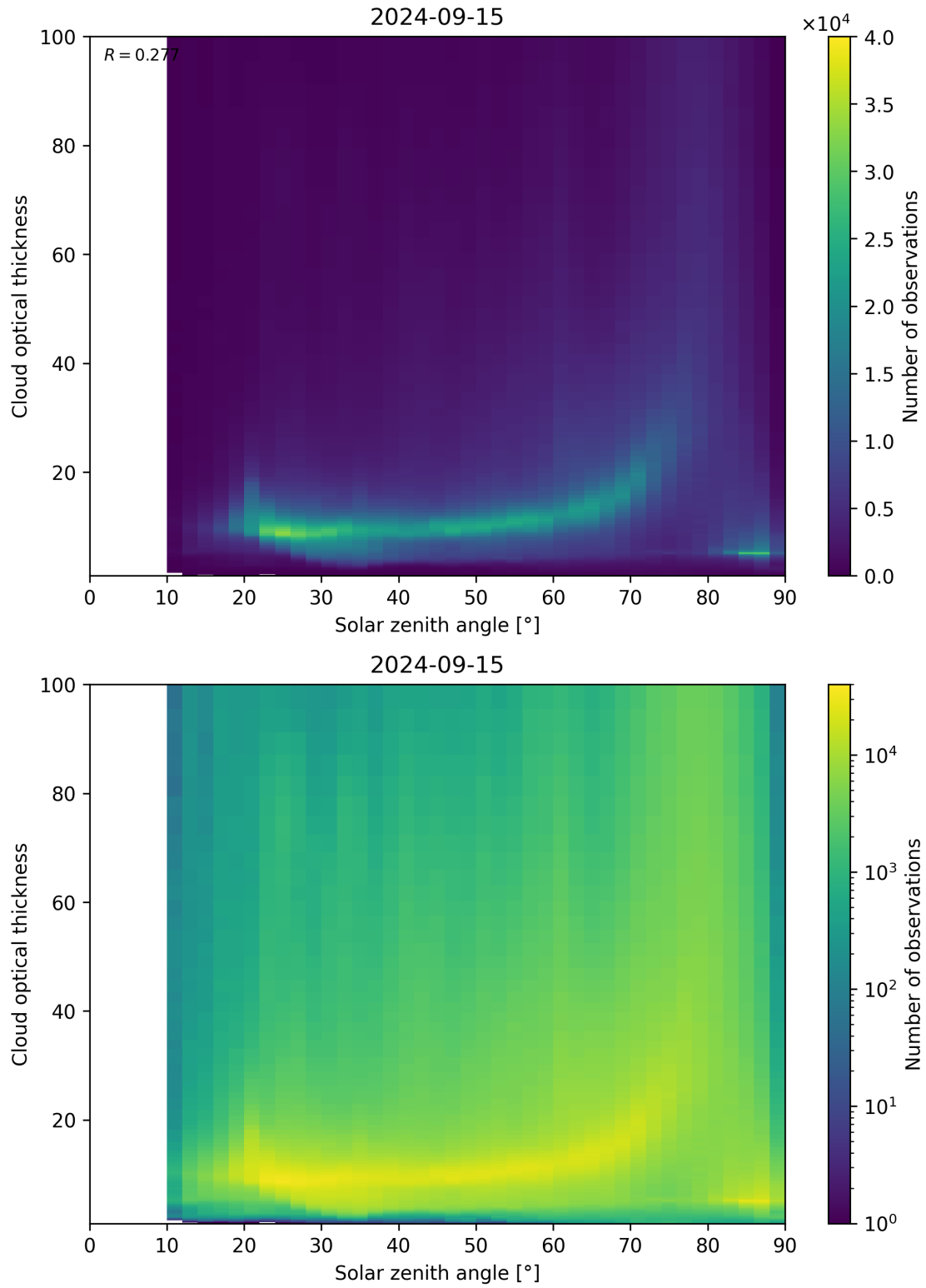
Figure 103: Scatter density plot of “Solar zenith angle” against “Cloud optical thickness” for 2024-09-14 to 2024-09-16.
