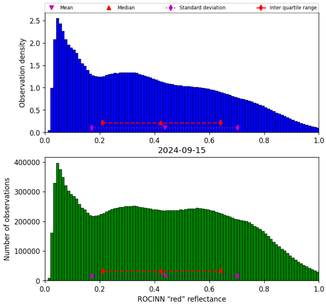
Figure 53: Histogram of “ROCINN “red” reflectance” for 2024-09-14 to 2024-09-16
