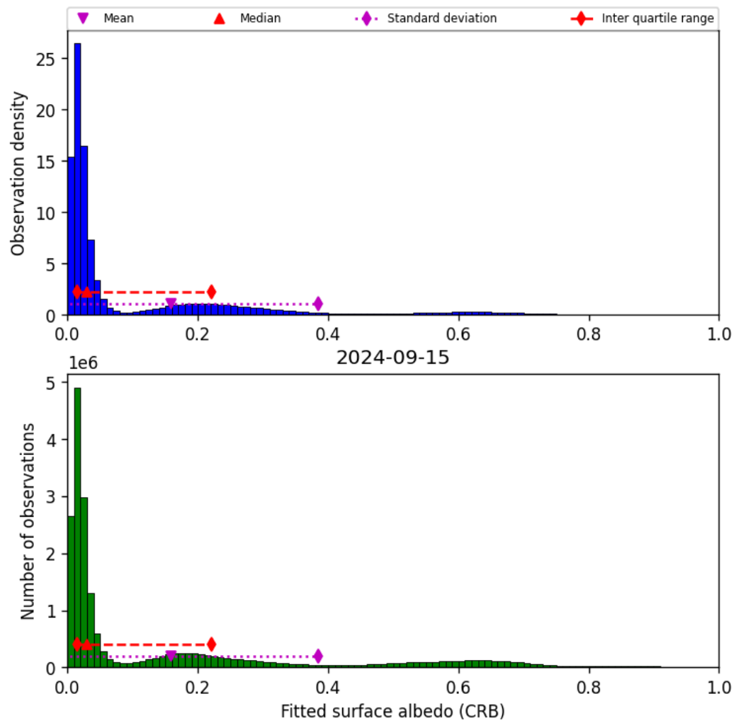
Figure 46: Histogram of “Fitted surface albedo (CRB)” for 2024-09-14 to 2024-09-16
