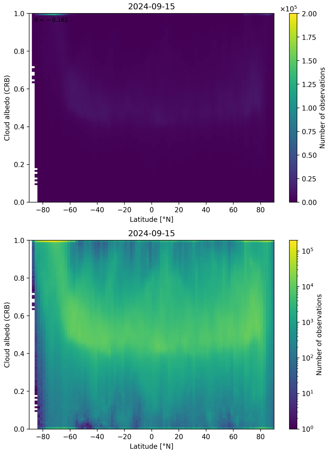
Figure 91: Scatter density plot of “Latitude” against “Cloud albedo (CRB)” for 2024-09-14 to 2024-09-16.
