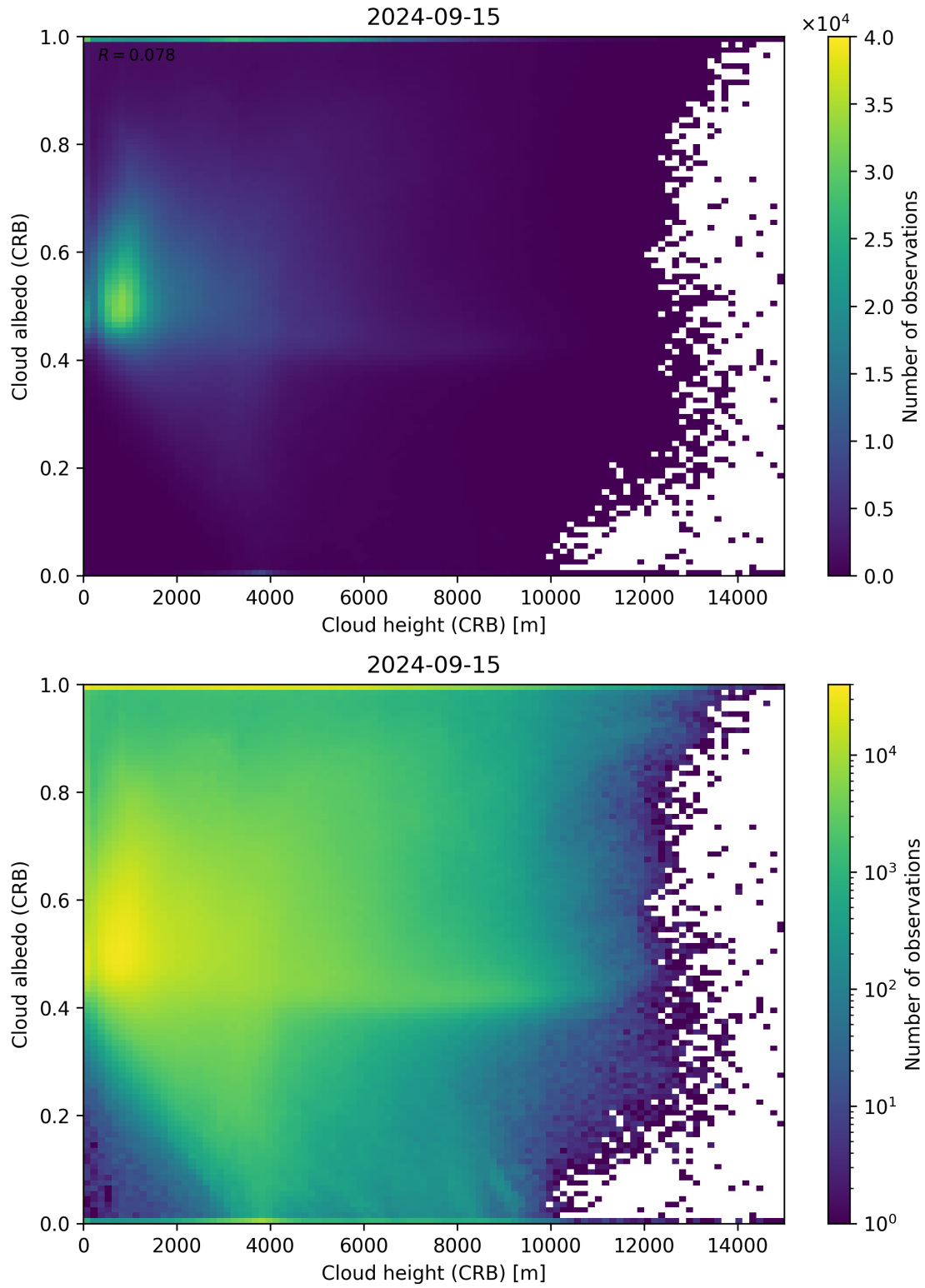
Figure 80: Scatter density plot of “Cloud height (CRB)” against “Cloud albedo (CRB)” for 2024-09-14 to 2024-09-16.
