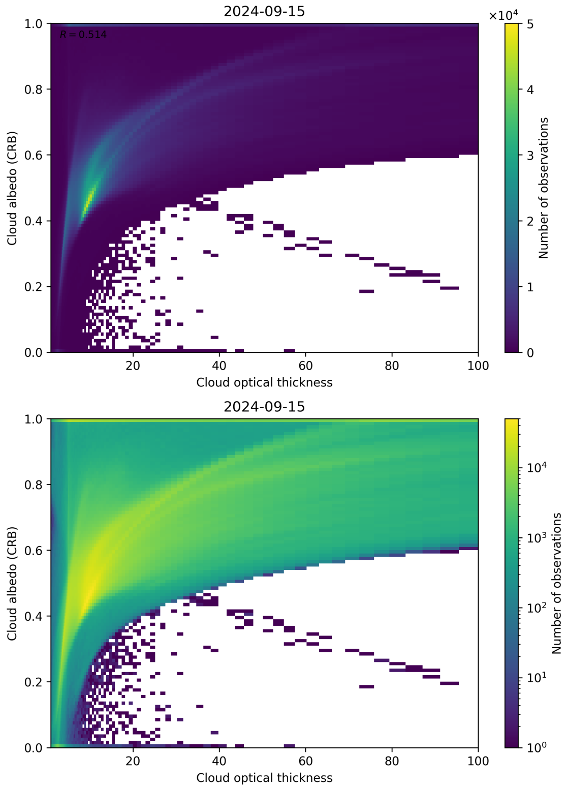
Figure 82: Scatter density plot of “Cloud optical thickness” against “Cloud albedo (CRB)” for 2024-09-14 to 2024-09-16.
