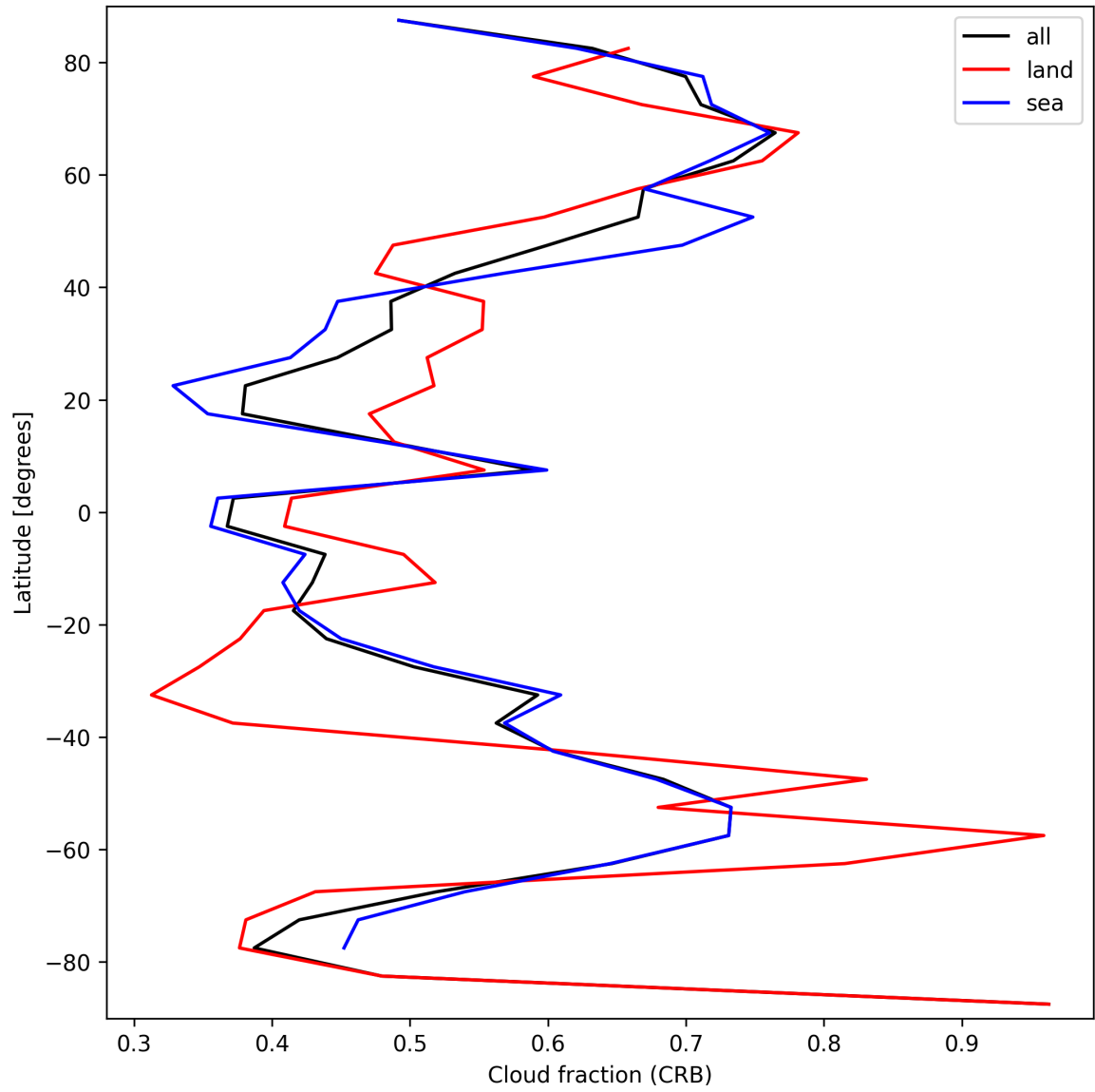
Figure 26: Zonal average of “Cloud fraction (CRB)” for 2024-09-14 to 2024-09-16.
