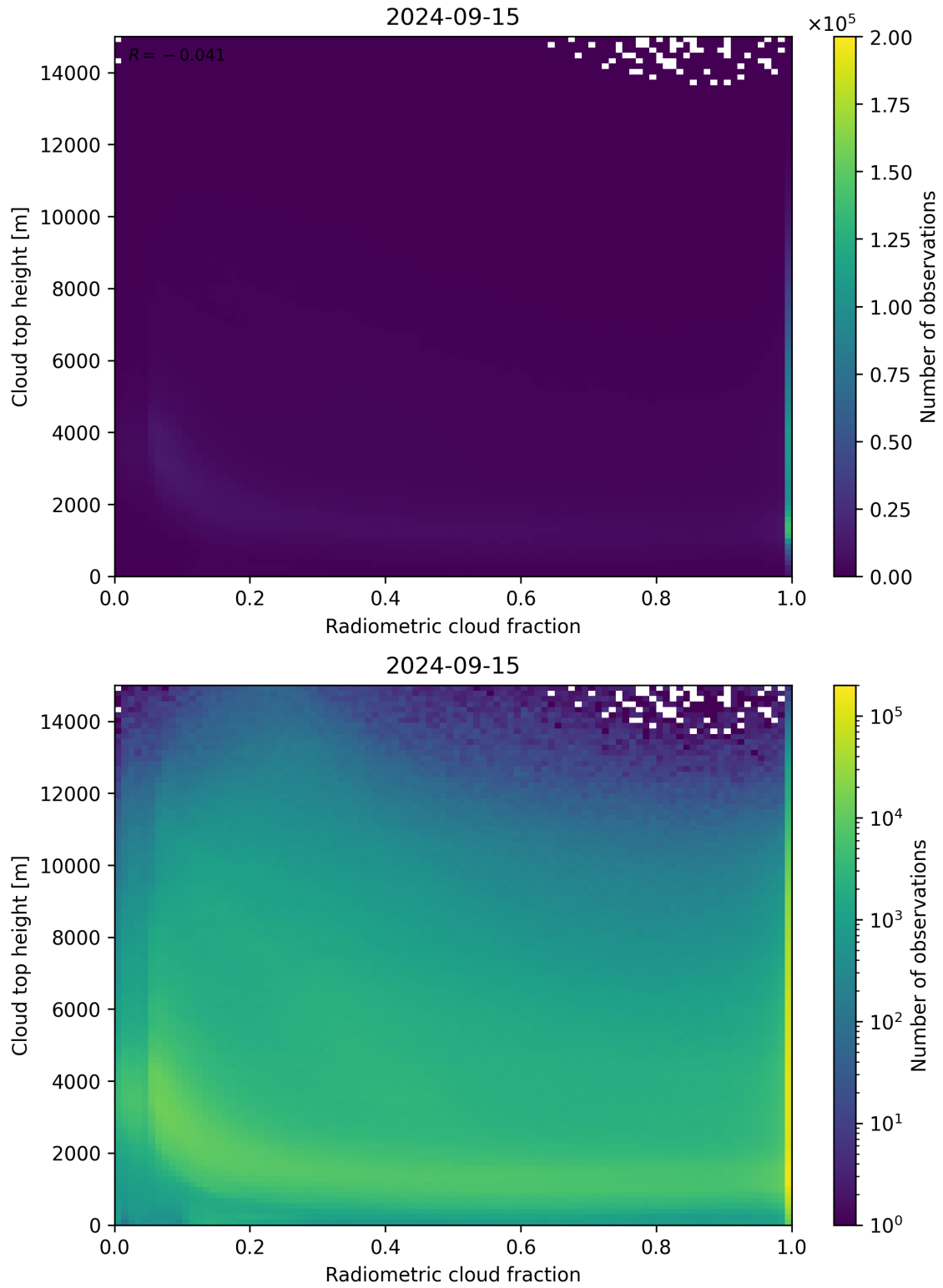
Figure 76: Scatter density plot of “Radiometric cloud fraction” against “Cloud top height” for 2024-09-14 to 2024-09-16.
