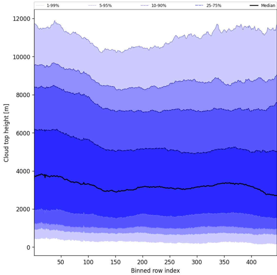
Figure 56: Along track statistics of “Cloud top height” for 2024-09-14 to 2024-09-16
