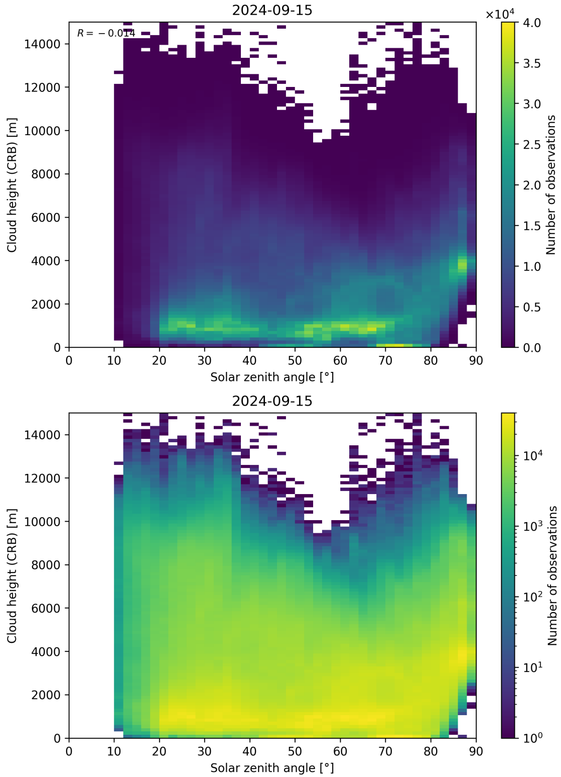
Figure 102: Scatter density plot of “Solar zenith angle” against “Cloud height (CRB)” for 2024-09-14 to 2024-09-16.
