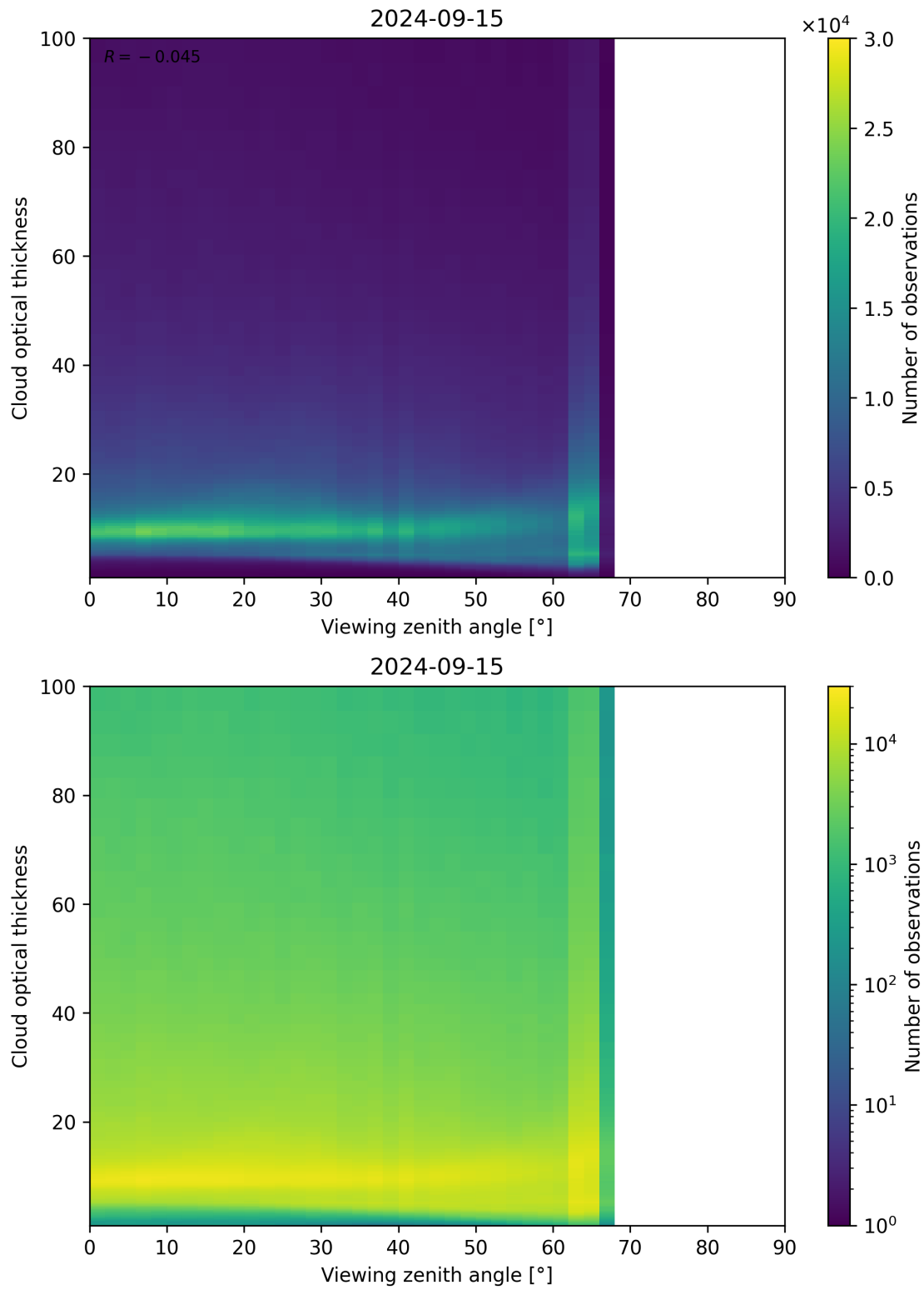
Figure 111: Scatter density plot of “Viewing zenith angle” against “Cloud optical thickness” for 2024-09-14 to 2024-09-16.
