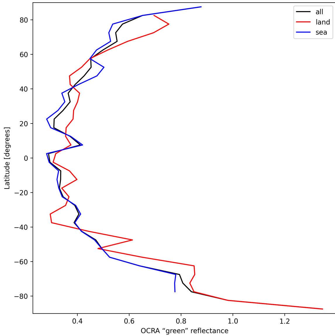
Figure 36: Zonal average of “OCRA “green” reflectance” for 2024-09-14 to 2024-09-16.
