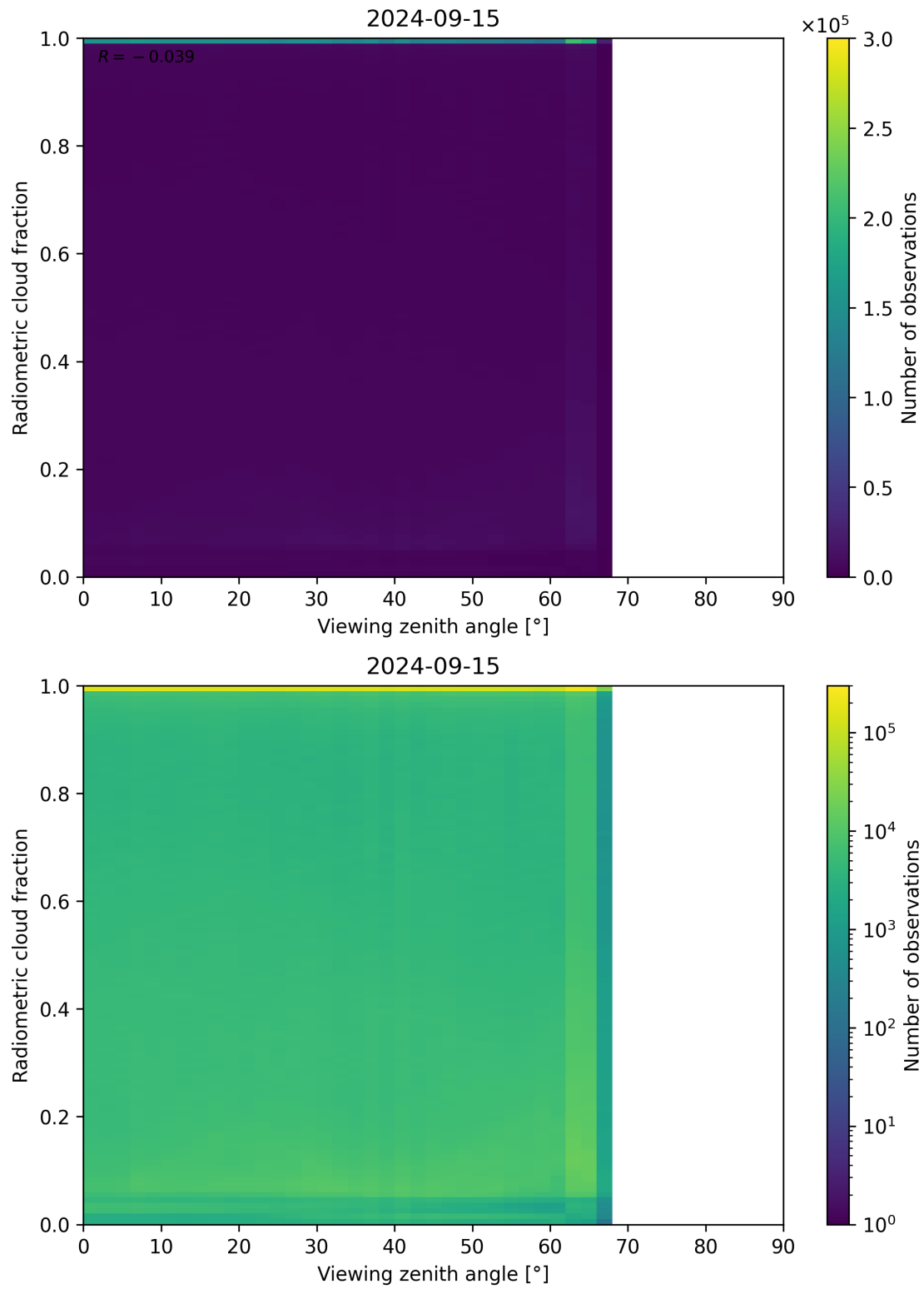
Figure 107: Scatter density plot of “Viewing zenith angle” against “Radiometric cloud fraction” for 2024-09-14 to 2024-09-16.
