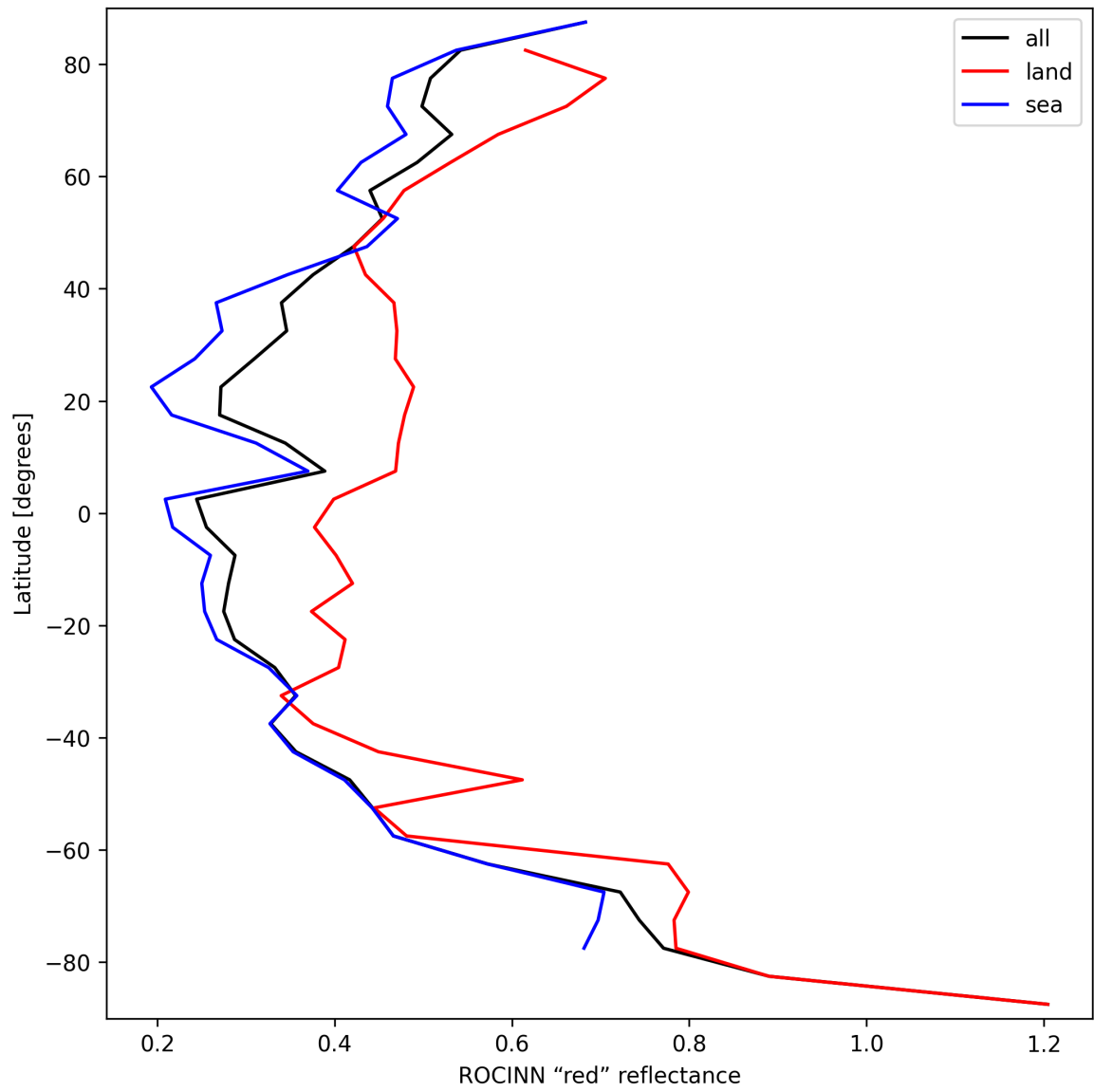
Figure 37: Zonal average of “ROCINN “red” reflectance” for 2024-09-14 to 2024-09-16.
