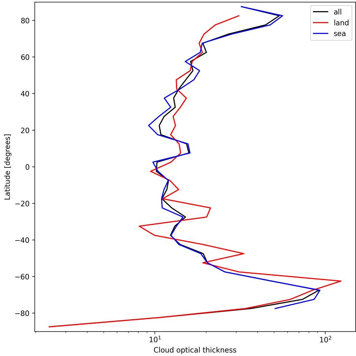
Figure 25: Zonal average of “Cloud optical thickness” for 2024-09-14 to 2024-09-16.
