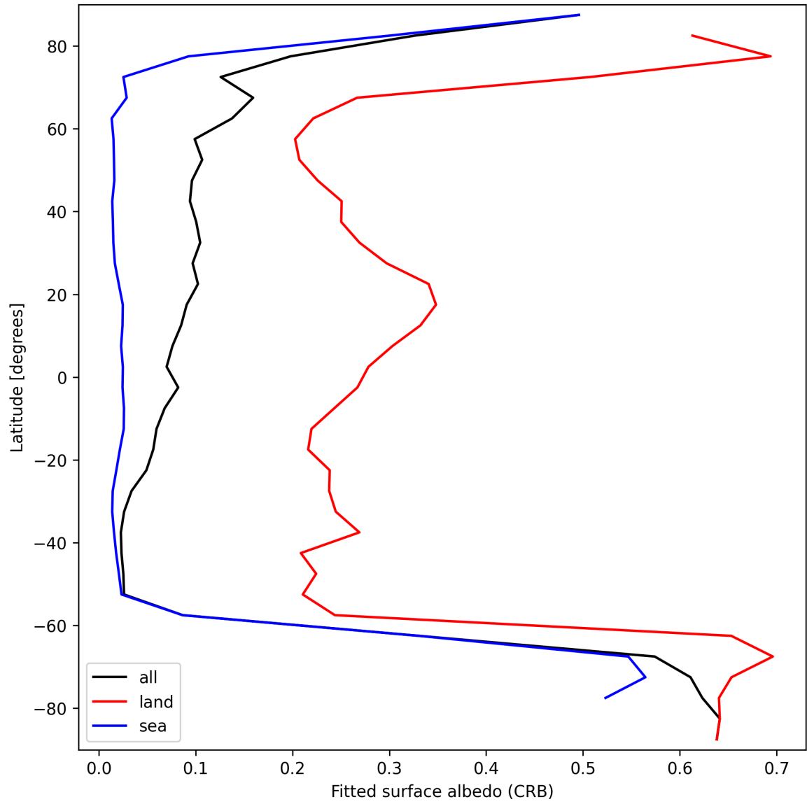
Figure 30: Zonal average of “Fitted surface albedo (CRB)” for 2024-09-14 to 2024-09-16.
