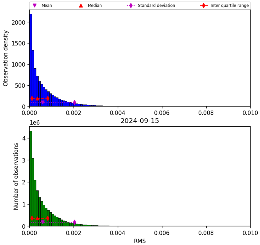
Figure 47: Histogram of “RMS” for 2024-09-14 to 2024-09-16
