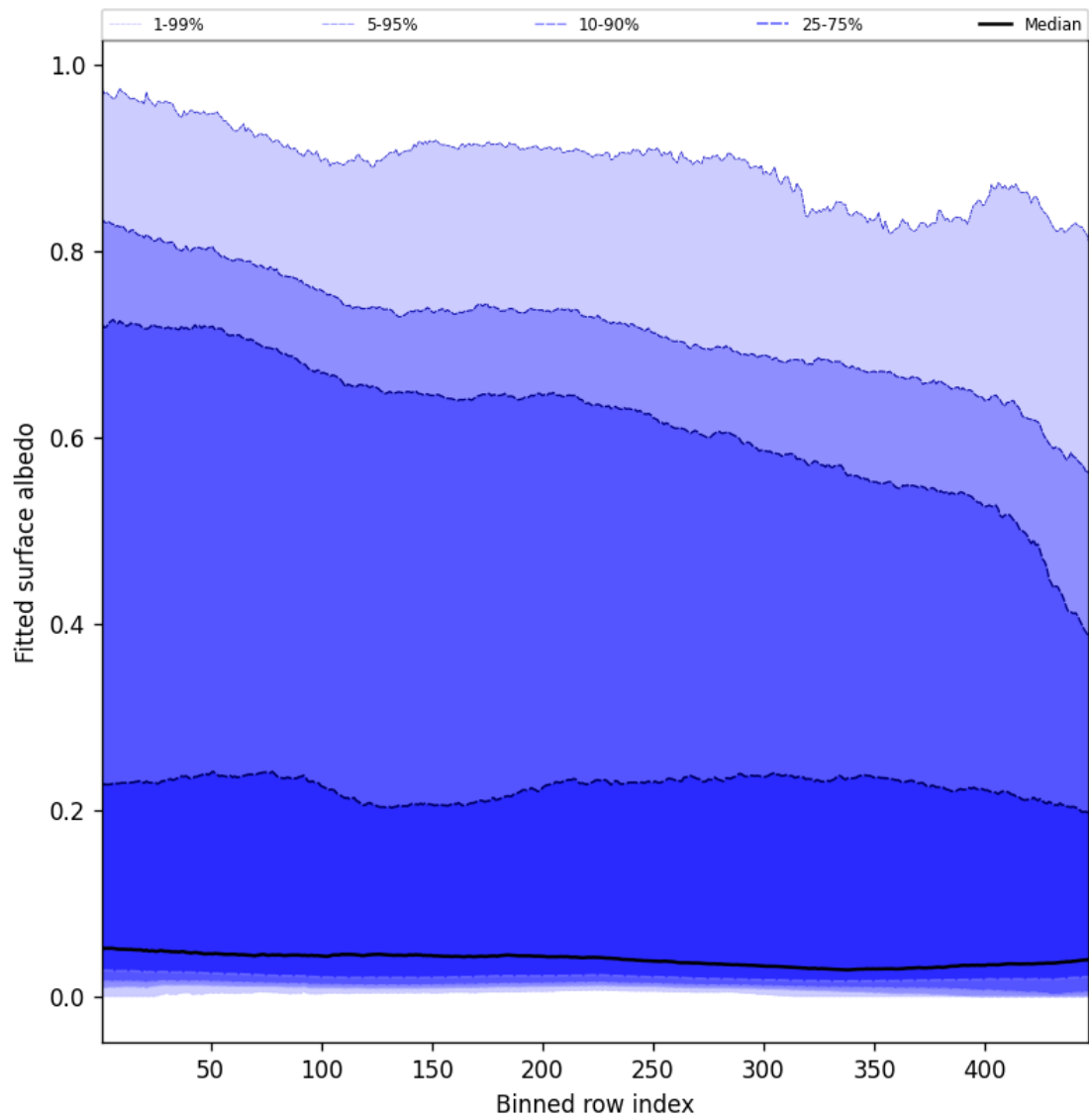
Figure 61: Along track statistics of “Fitted surface albedo” for 2024-09-14 to 2024-09-16
