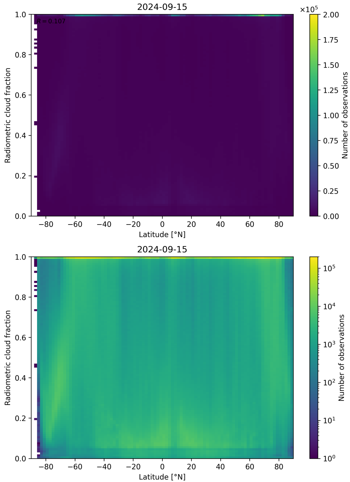
Figure 92: Scatter density plot of “Latitude” against “Radiometric cloud fraction” for 2024-09-14 to 2024-09-16.
