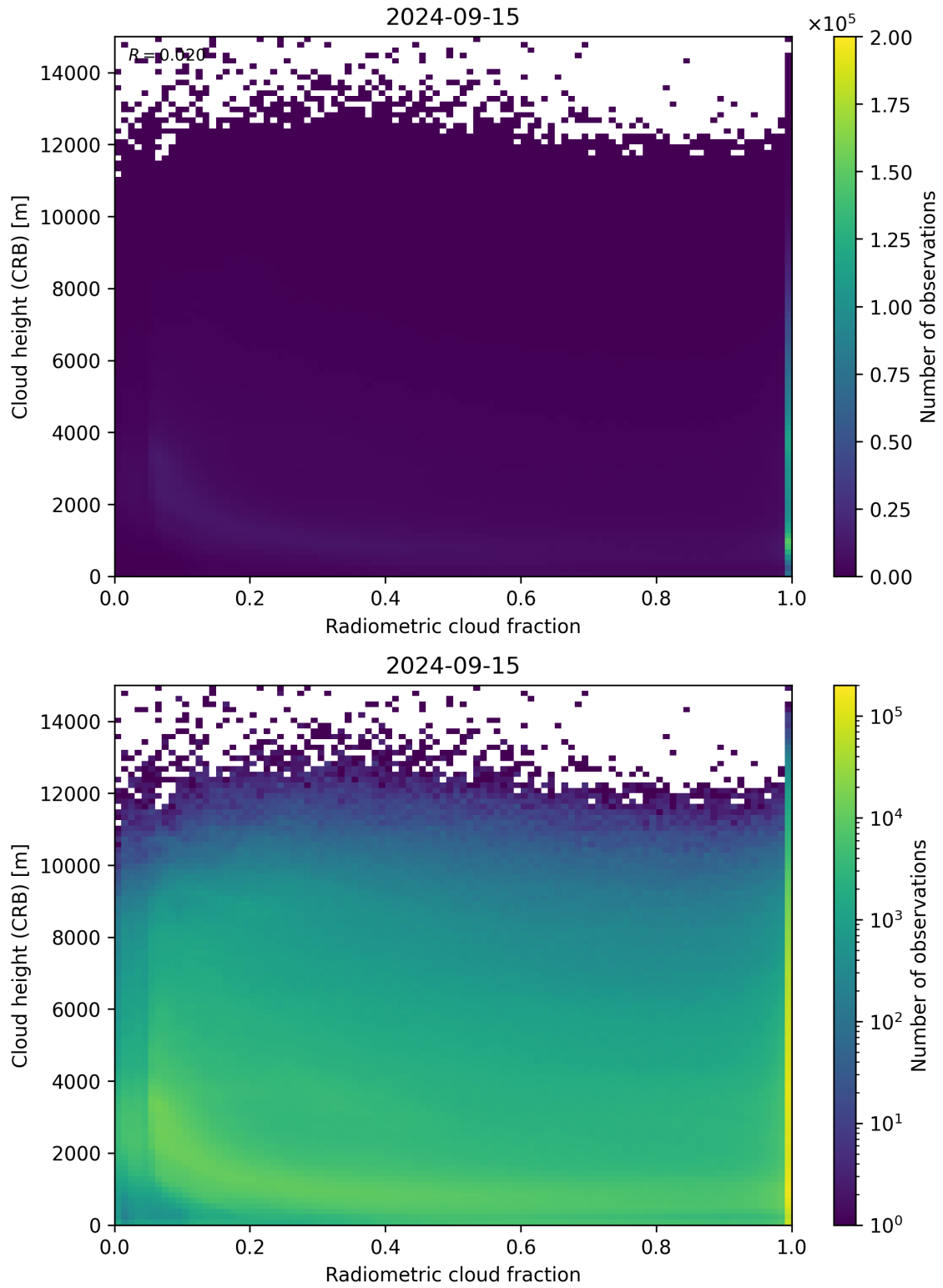
Figure 74: Scatter density plot of “Radiometric cloud fraction” against “Cloud height (CRB)” for 2024-09-14 to 2024-09-16.
