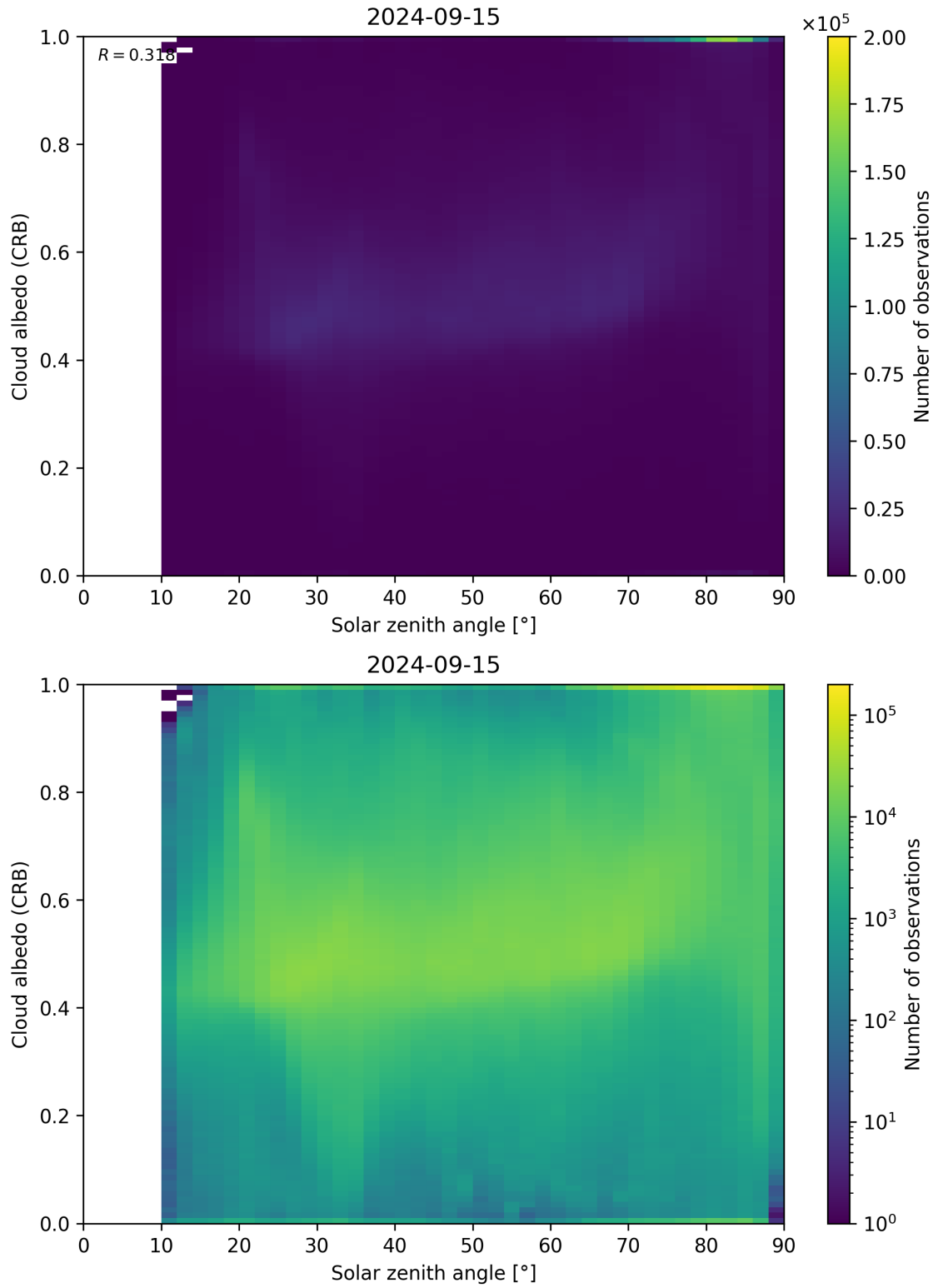
Figure 98: Scatter density plot of “Solar zenith angle” against “Cloud albedo (CRB)” for 2024-09-14 to 2024-09-16.
