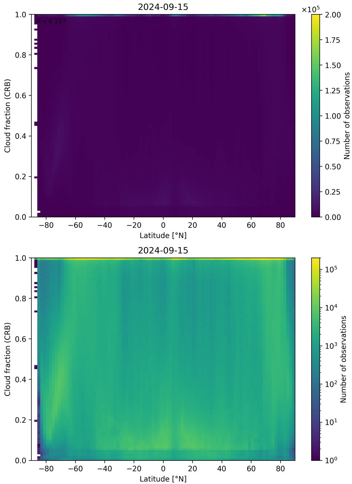
Figure 94: Scatter density plot of “Latitude” against “Cloud fraction (CRB)” for 2024-09-14 to 2024-09-16.
