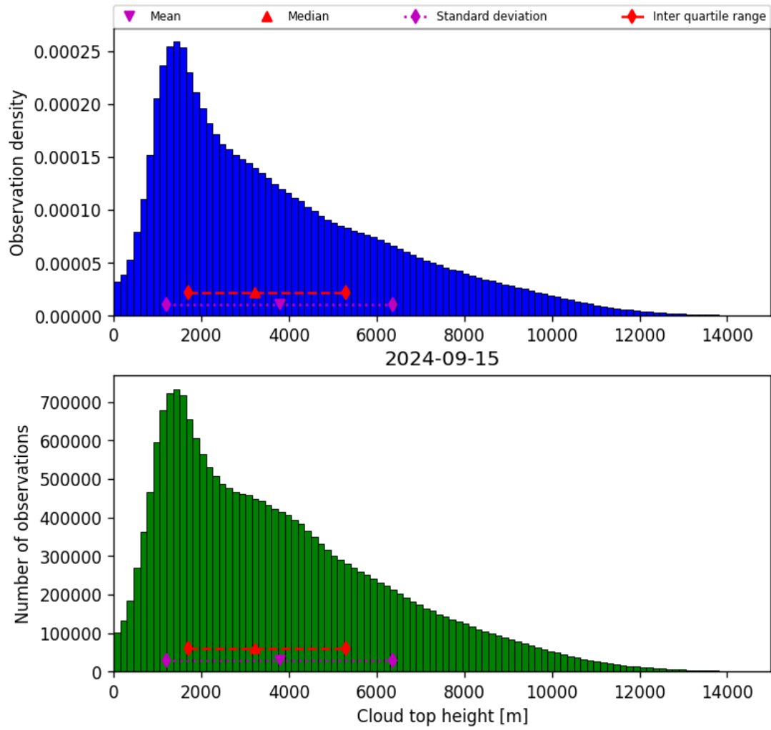
Figure 40: Histogram of “Cloud top height” for 2024-09-14 to 2024-09-16
