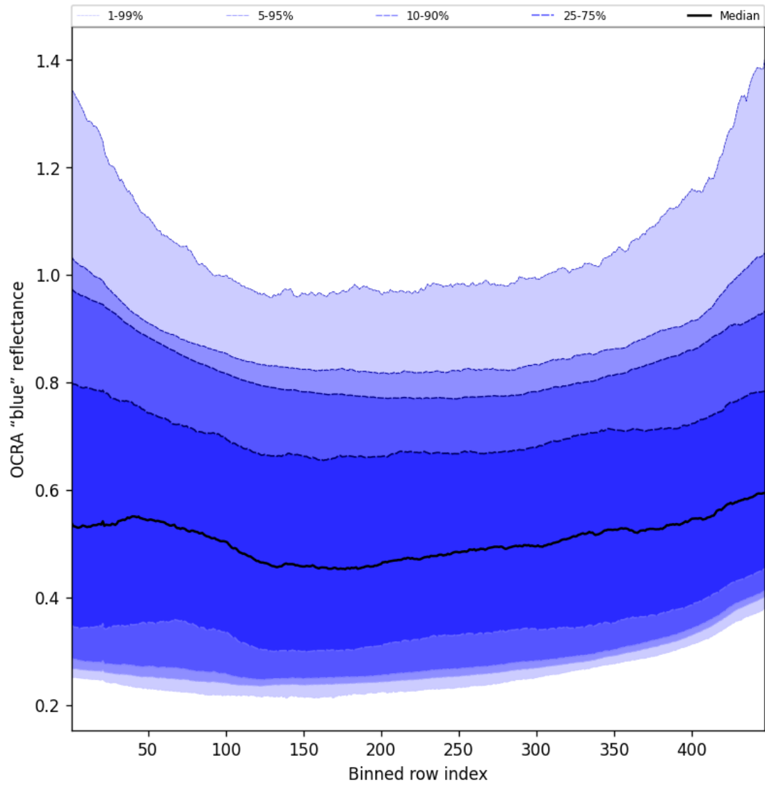
Figure 67: Along track statistics of "OCRA "blue" reflectance" for 2024-09-14 to 2024-09-16
