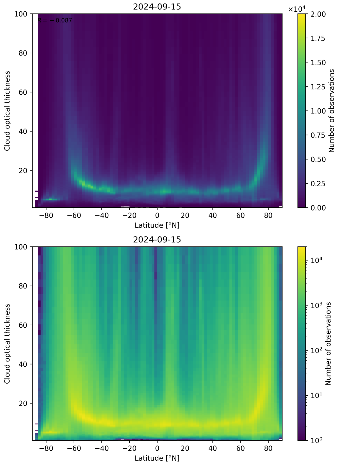
Figure 96: Scatter density plot of “Latitude” against “Cloud optical thickness” for 2024-09-14 to 2024-09-16.
