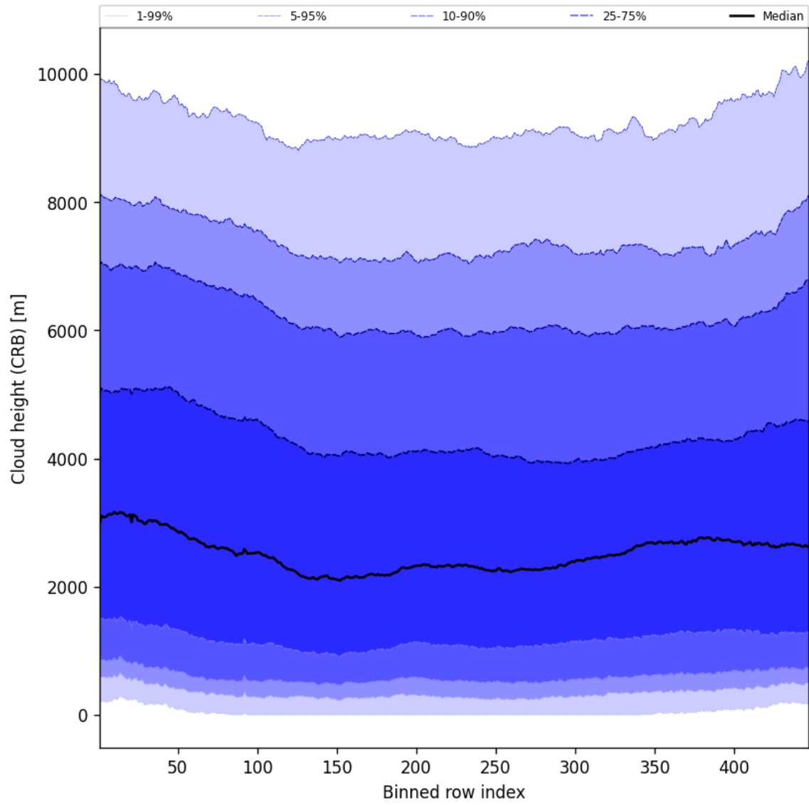
Figure 59: Along track statistics of “Cloud height (CRB)” for 2024-09-14 to 2024-09-16
