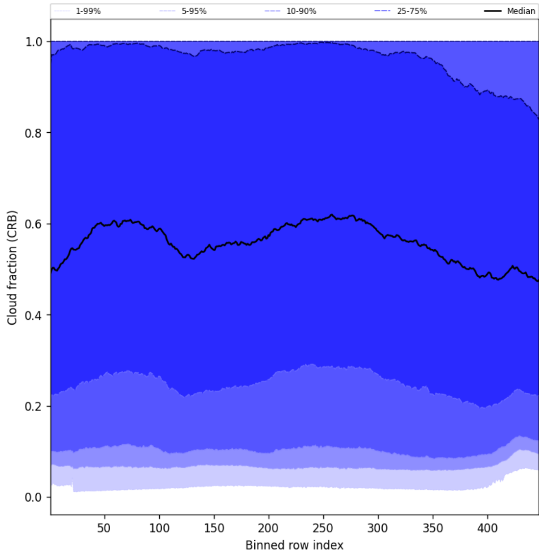
Figure 58: Along track statistics of “Cloud fraction (CRB)” for 2024-09-14 to 2024-09-16
