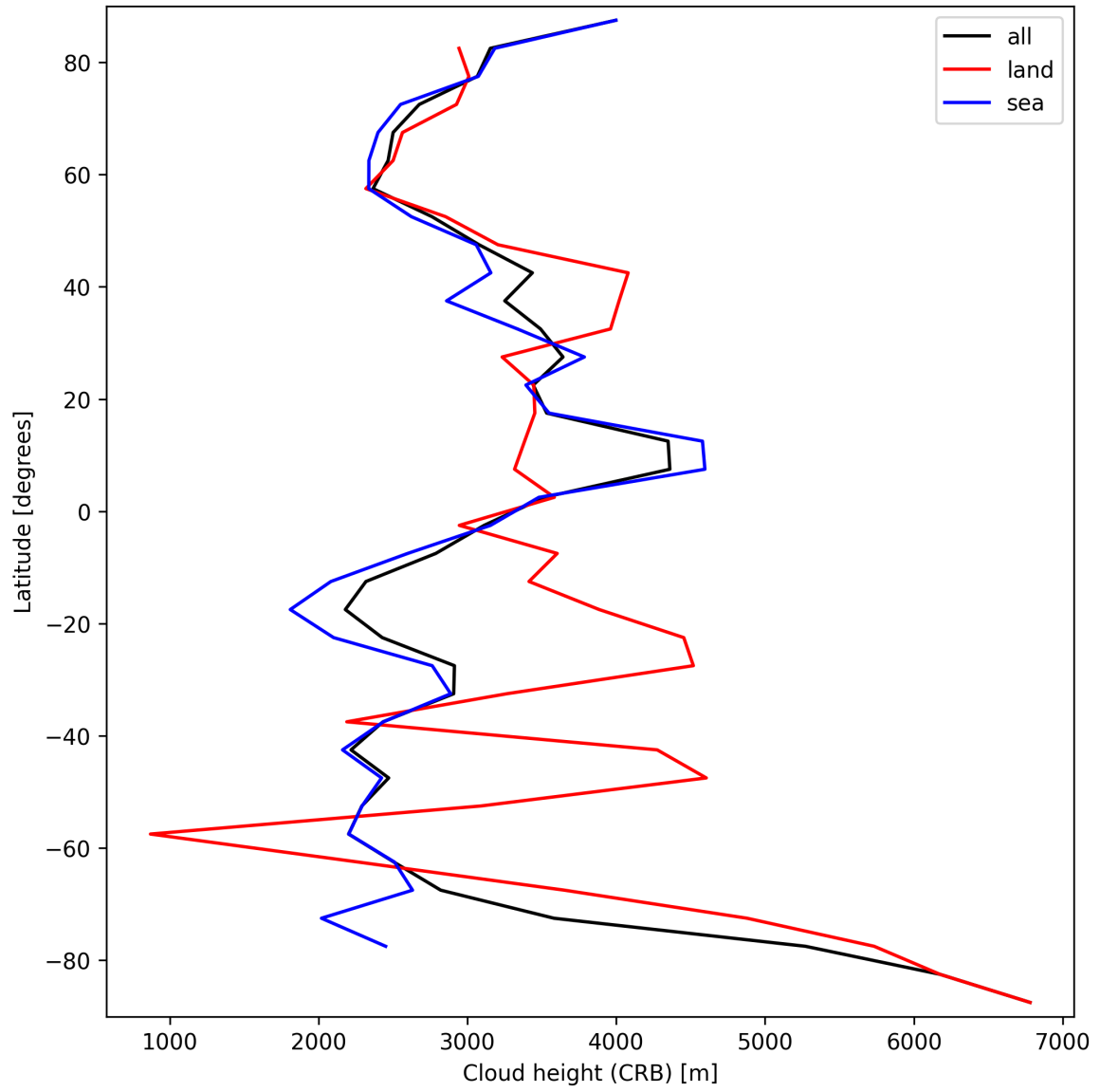
Figure 27: Zonal average of “Cloud height (CRB)” for 2024-09-14 to 2024-09-16.
