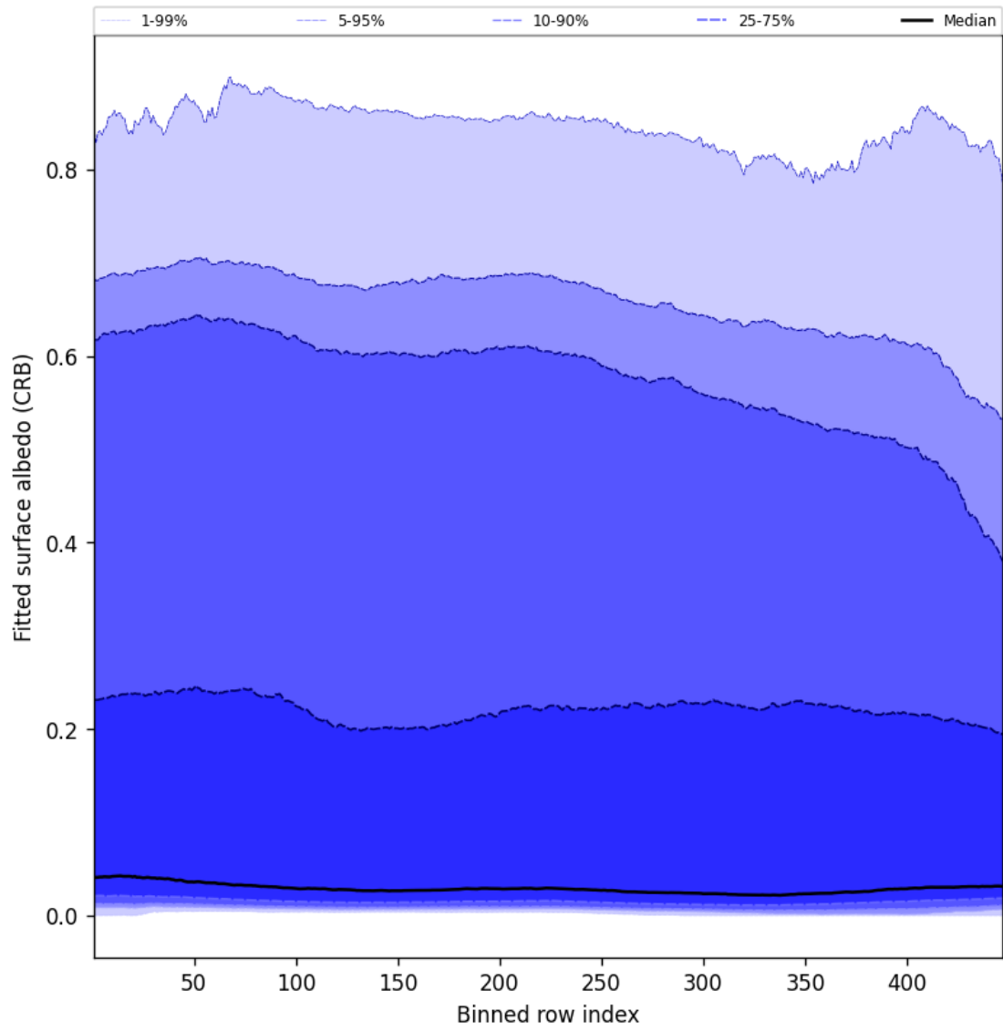
Figure 62: Along track statistics of “Fitted surface albedo (CRB)” for 2024-09-14 to 2024-09-16
