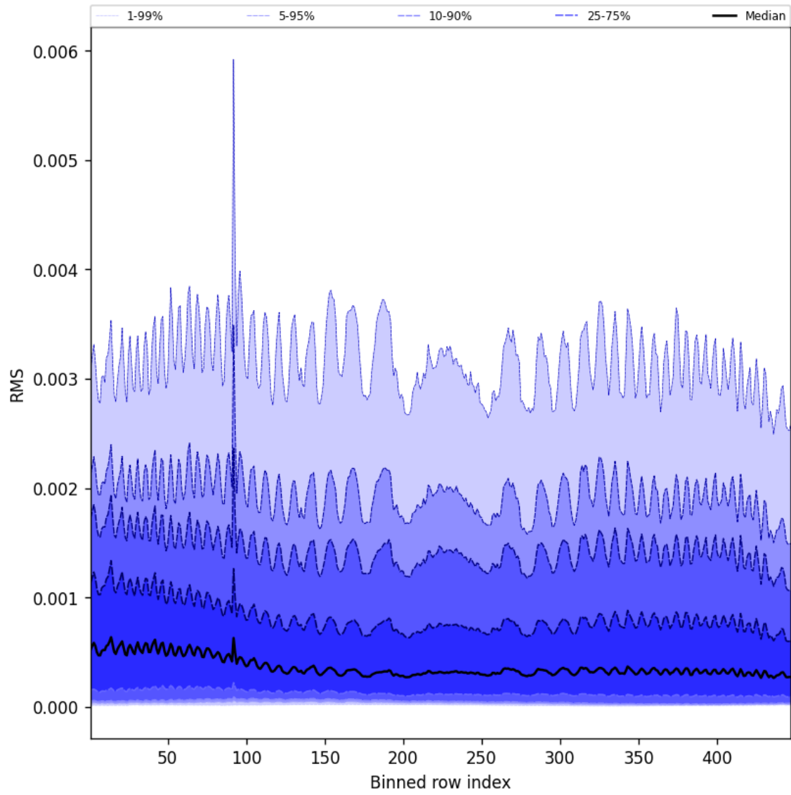
Figure 63: Along track statistics of “RMS” for 2024-09-14 to 2024-09-16
