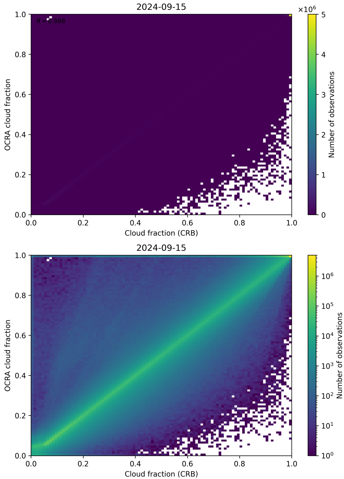
Figure 78: Scatter density plot of “Cloud fraction (CRB)” against “OCRA cloud fraction” for 2024-09-14 to 2024-09-16.
