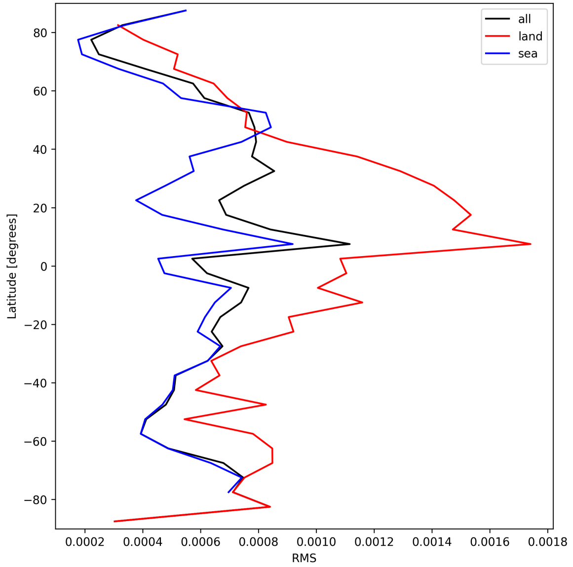
Figure 31: Zonal average of “RMS” for 2024-09-14 to 2024-09-16.
