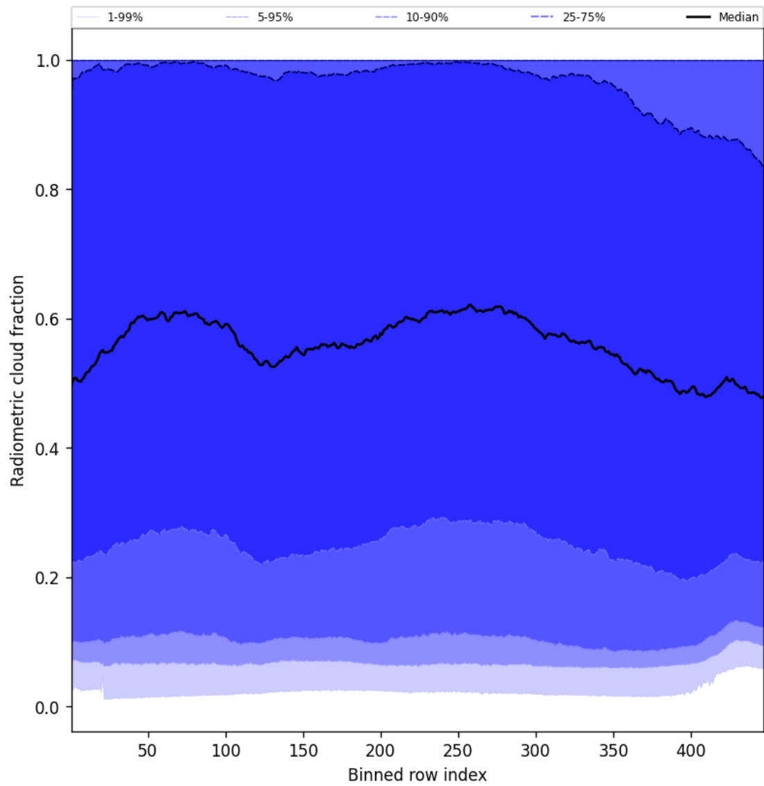
Figure 55: Along track statistics of “Radiometric cloud fraction” for 2024-09-14 to 2024-09-16
