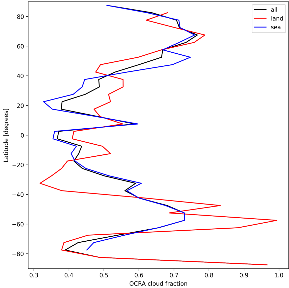
Figure 34: Zonal average of “OCRA cloud fraction” for 2024-09-14 to 2024-09-16.
