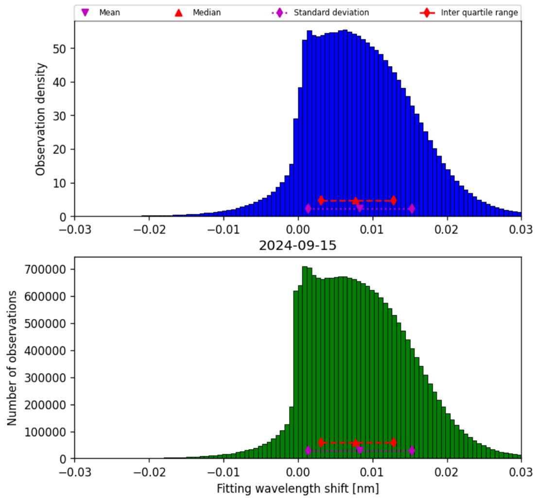
Figure 49: Histogram of “Fitting wavelength shift” for 2024-09-14 to 2024-09-16
