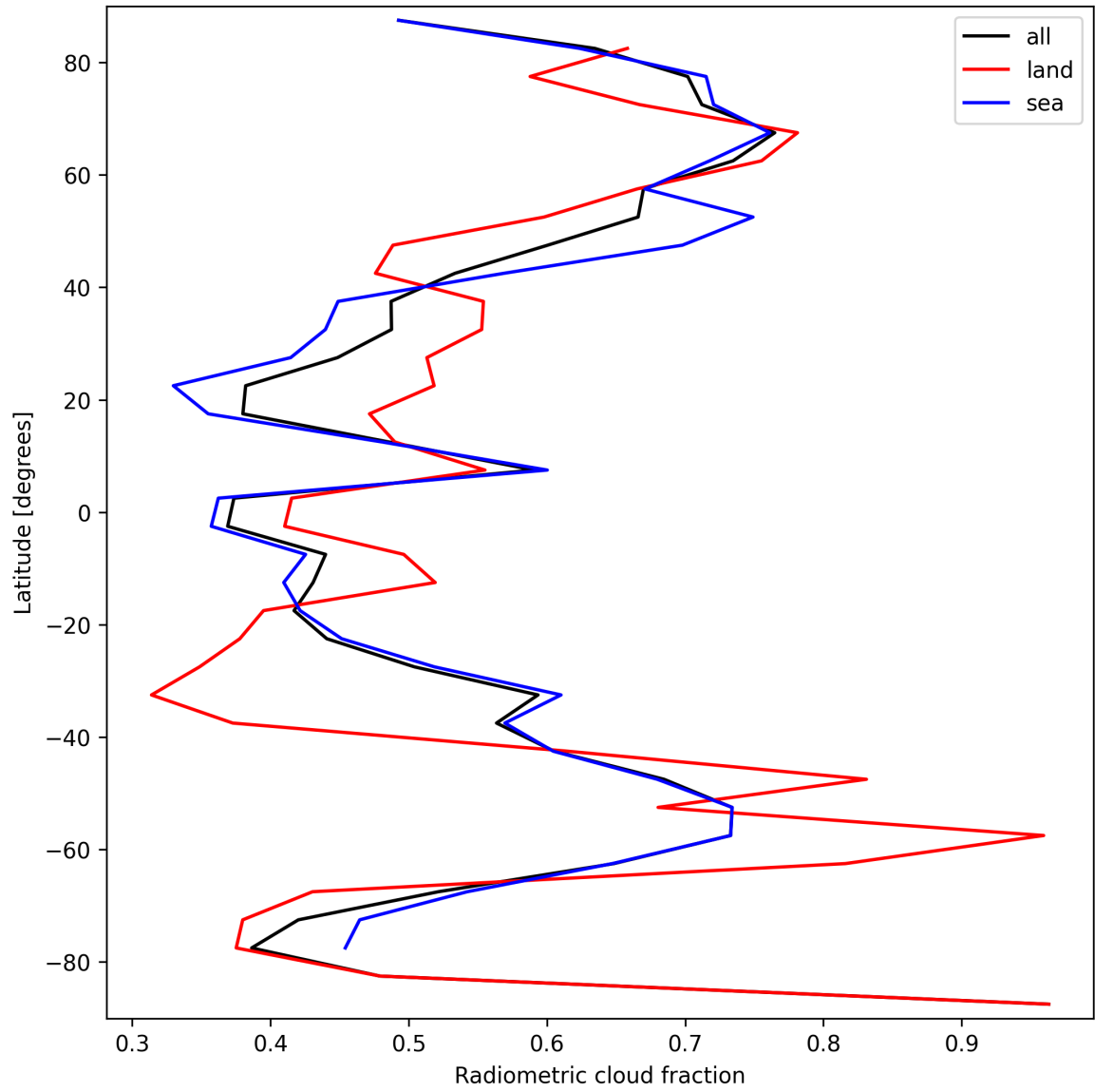
Figure 23: Zonal average of “Radiometric cloud fraction” for 2024-09-14 to 2024-09-16.
