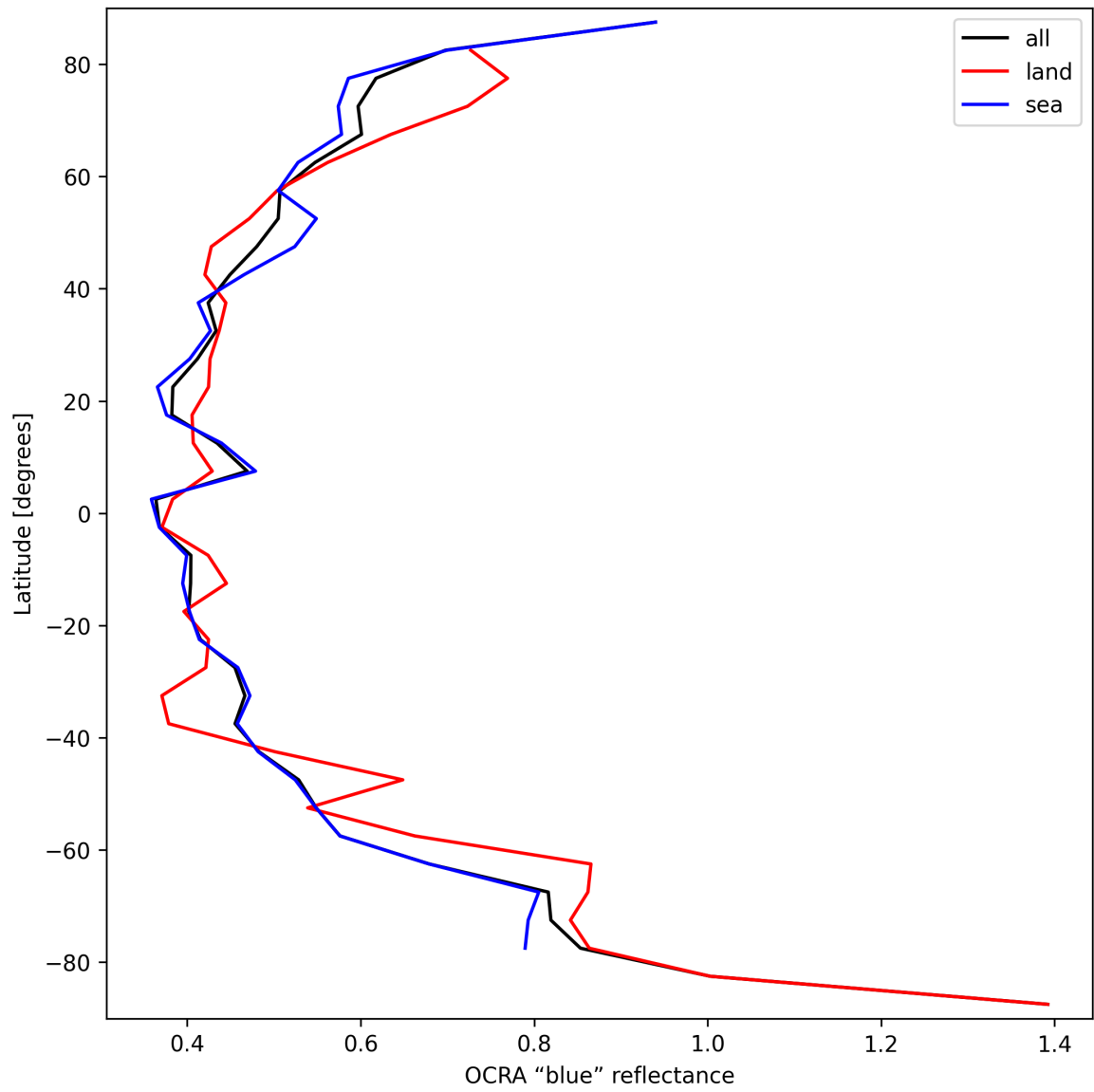
Figure 35: Zonal average of “OCRA “blue” reflectance” for 2024-09-14 to 2024-09-16.
