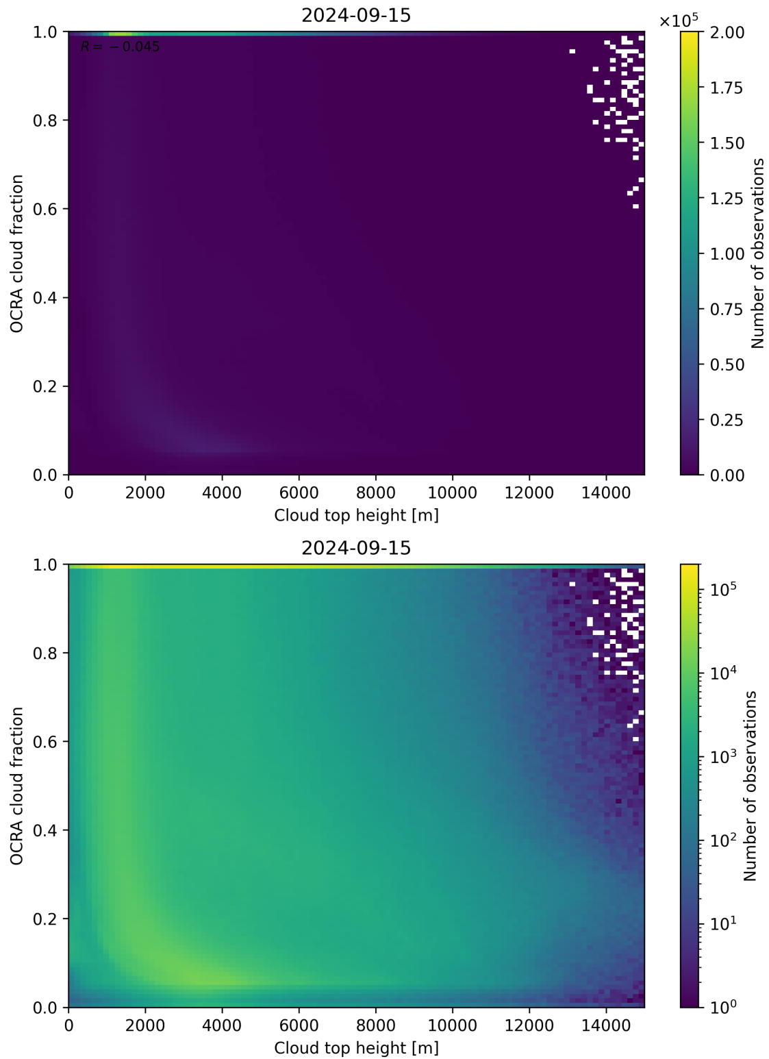
Figure 87: Scatter density plot of “Cloud top height” against “OCRA cloud fraction” for 2024-09-14 to 2024-09-16.
