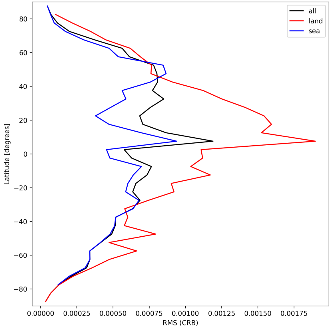
Figure 32: Zonal average of “RMS (CRB)” for 2024-09-14 to 2024-09-16.
