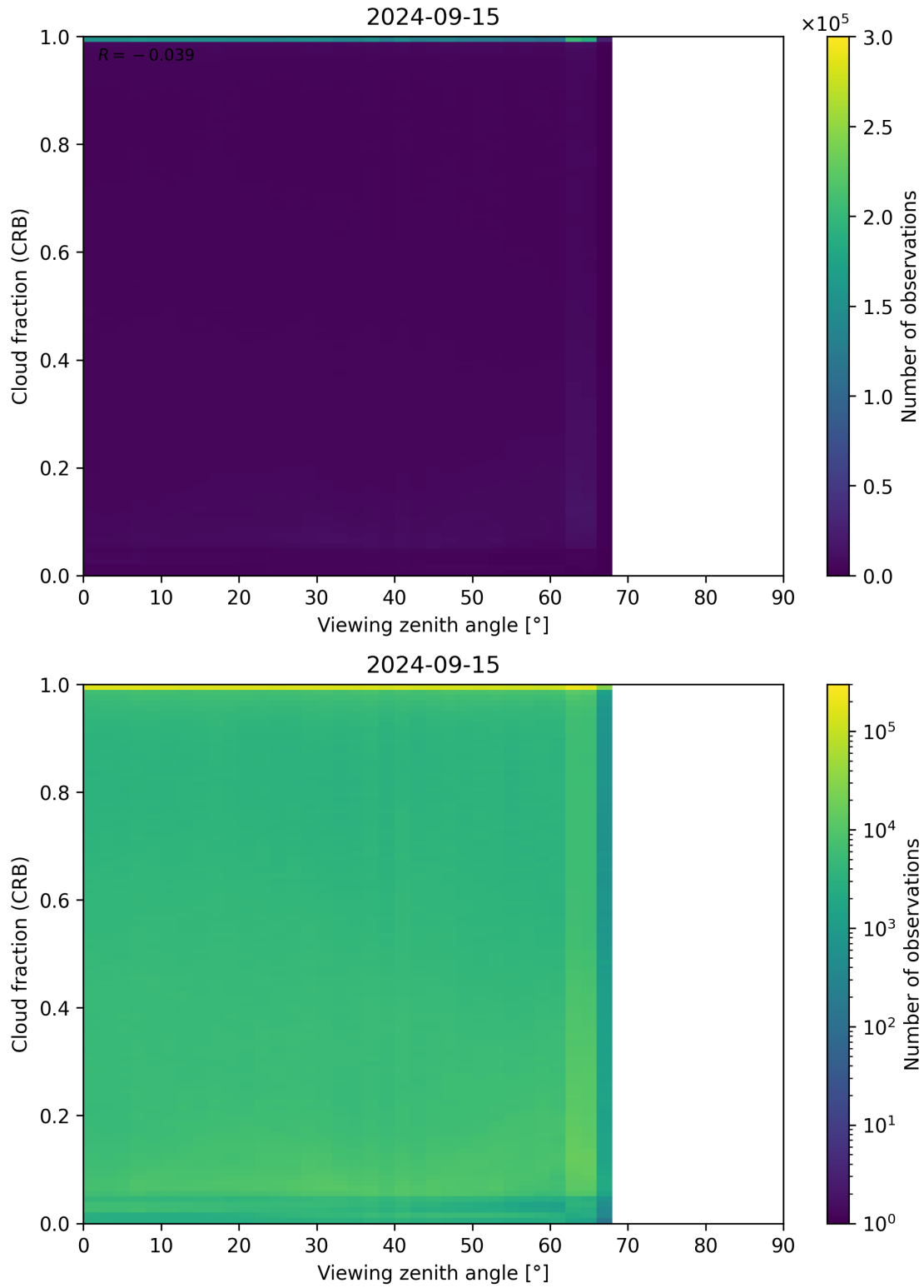
Figure 109: Scatter density plot of “Viewing zenith angle” against “Cloud fraction (CRB)” for 2024-09-14 to 2024-09-16.
