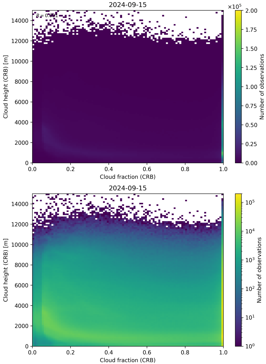
Figure 79: Scatter density plot of “Cloud fraction (CRB)” against “Cloud height (CRB)” for 2024-09-14 to 2024-09-16.
