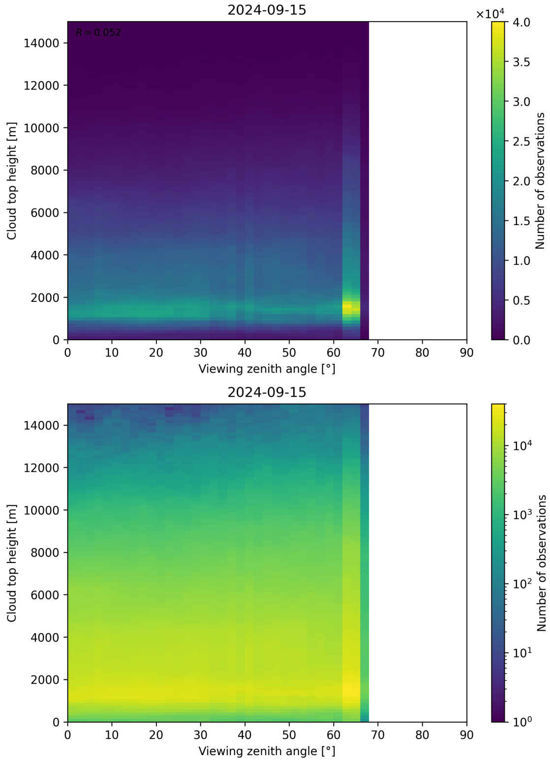
Figure 112: Scatter density plot of “Viewing zenith angle” against “Cloud top height” for 2024-09-14 to 2024-09-16.
