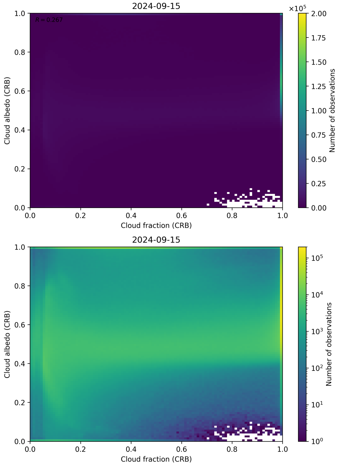
Figure 77: Scatter density plot of “Cloud fraction (CRB)” against “Cloud albedo (CRB)” for 2024-09-14 to 2024-09-16.
