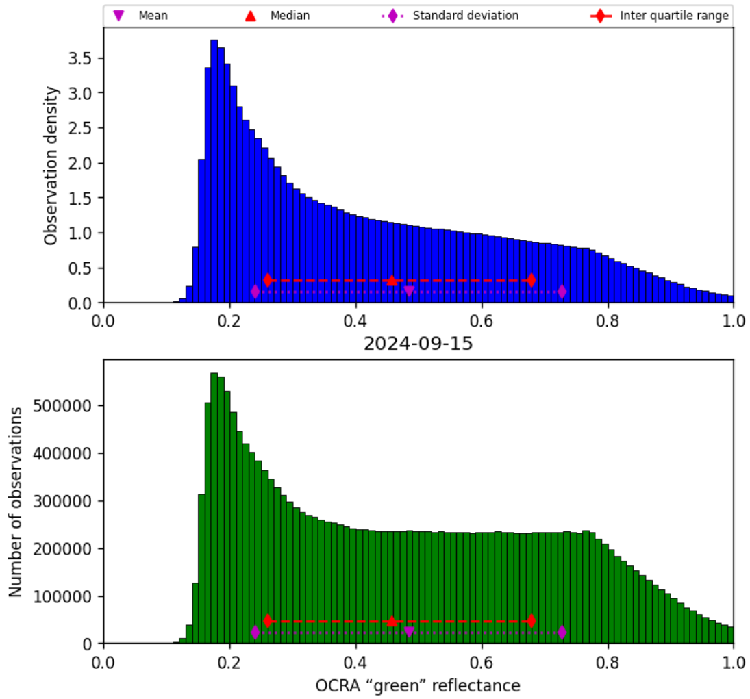
Figure 52: Histogram of “OCRA “green” reflectance” for 2024-09-14 to 2024-09-16
