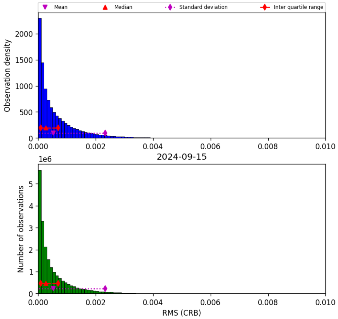
Figure 48: Histogram of “RMS (CRB)” for 2024-09-14 to 2024-09-16
