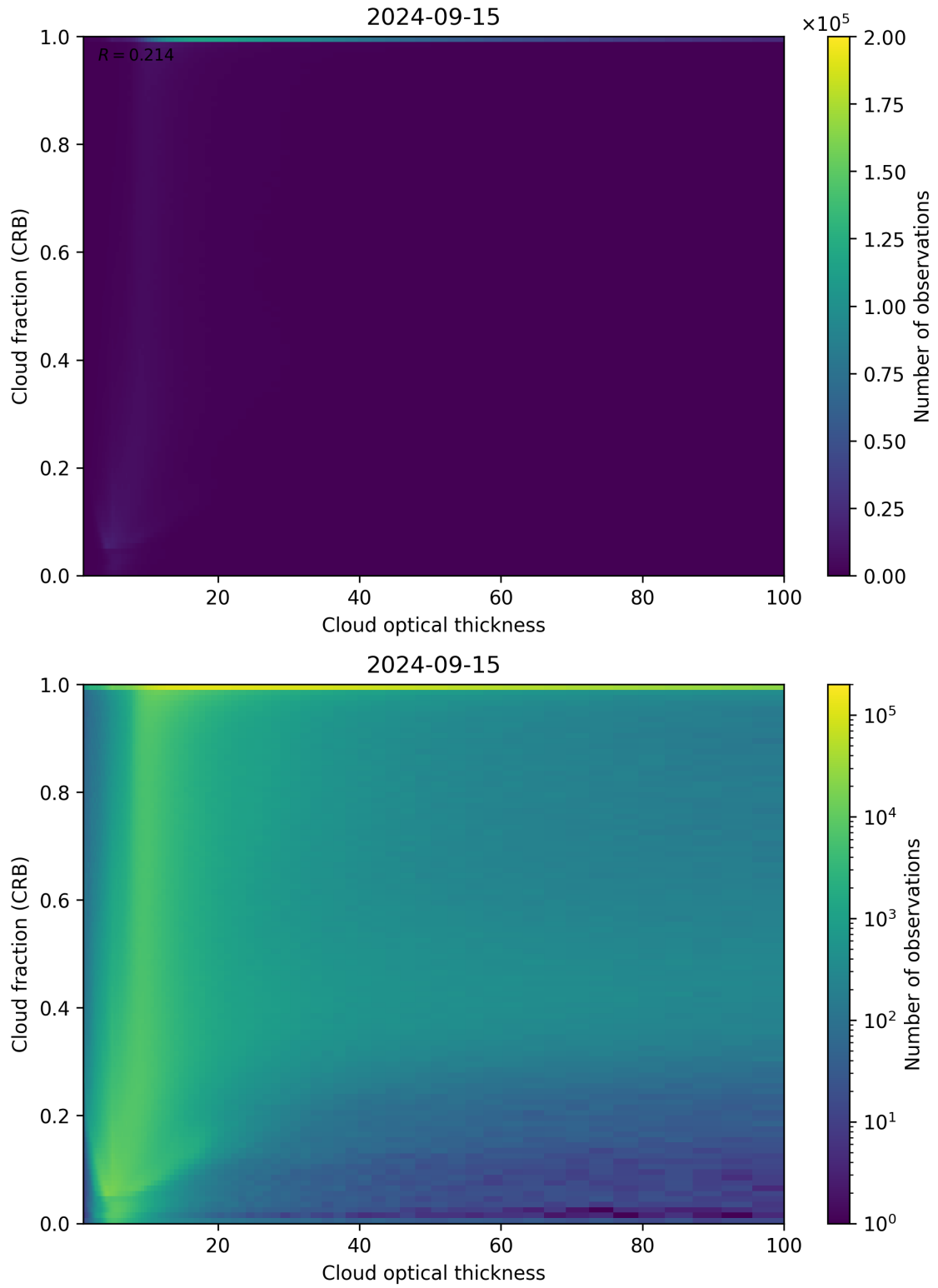
Figure 84: Scatter density plot of “Cloud optical thickness” against “Cloud fraction (CRB)” for 2024-09-14 to 2024-09-16.
