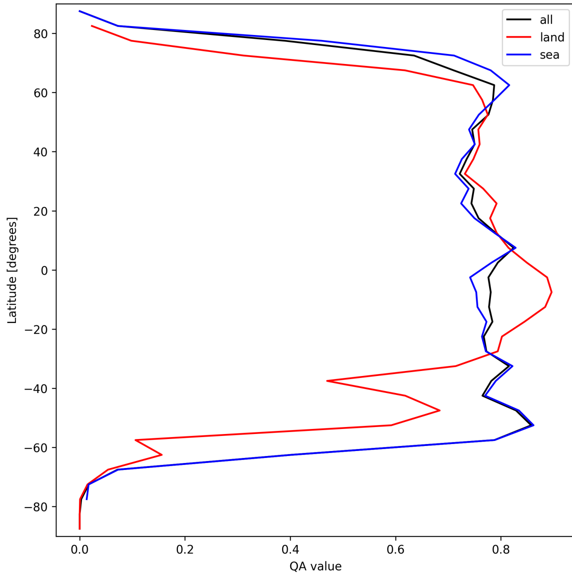
Figure 22: Zonal average of “QA value” for 2024-09-14 to 2024-09-16.
