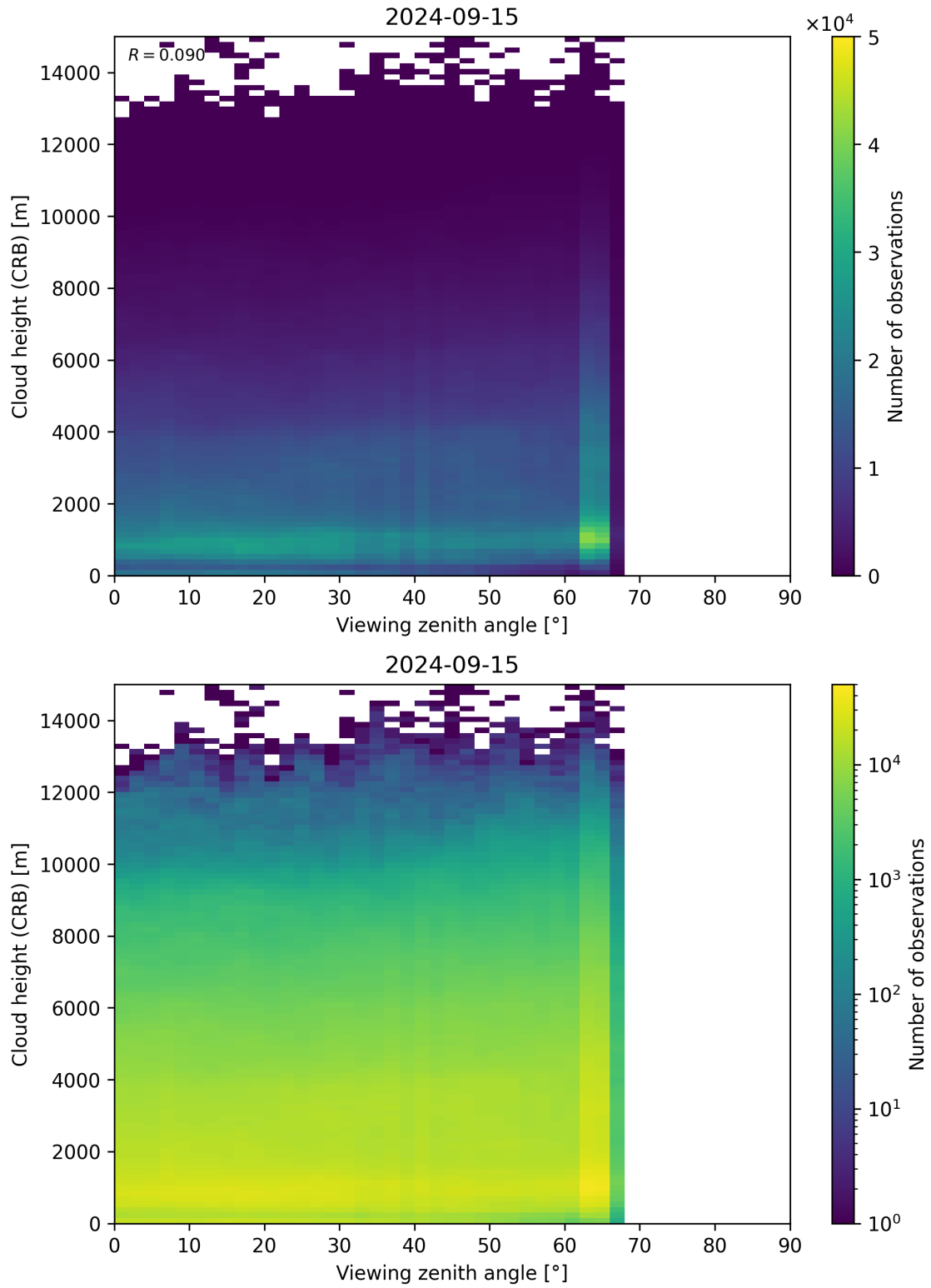
Figure 110: Scatter density plot of “Viewing zenith angle” against “Cloud height (CRB)” for 2024-09-14 to 2024-09-16.
