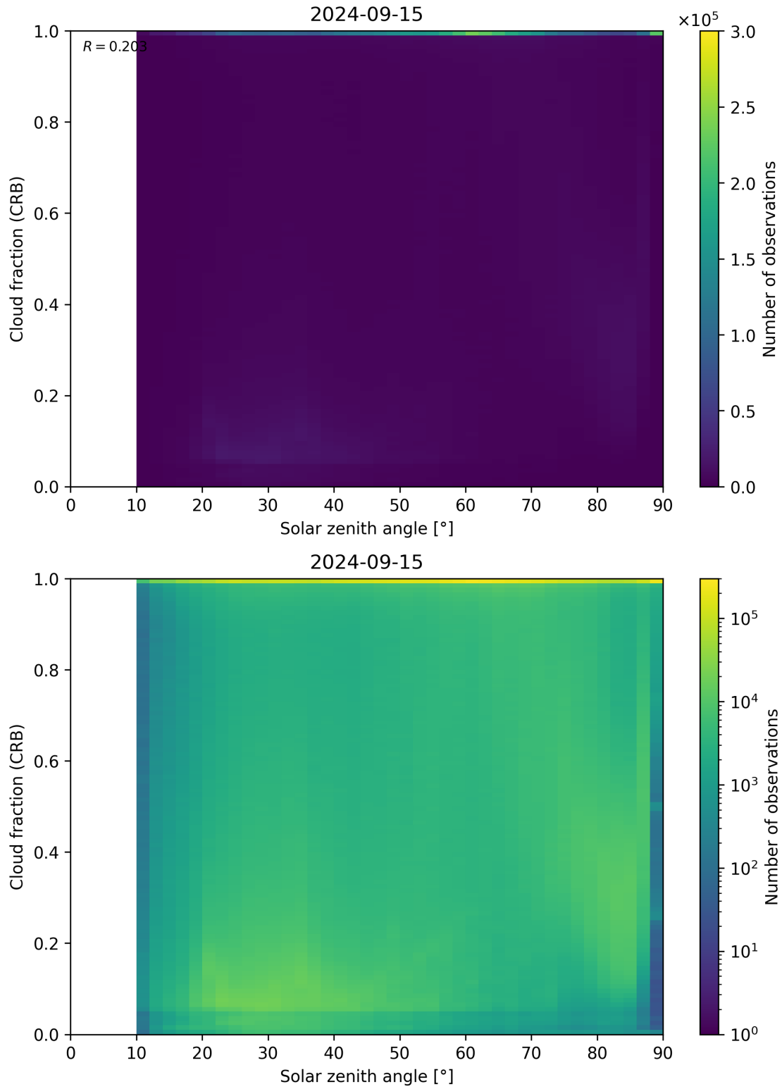
Figure 101: Scatter density plot of “Solar zenith angle” against “Cloud fraction (CRB)” for 2024-09-14 to 2024-09-16.
