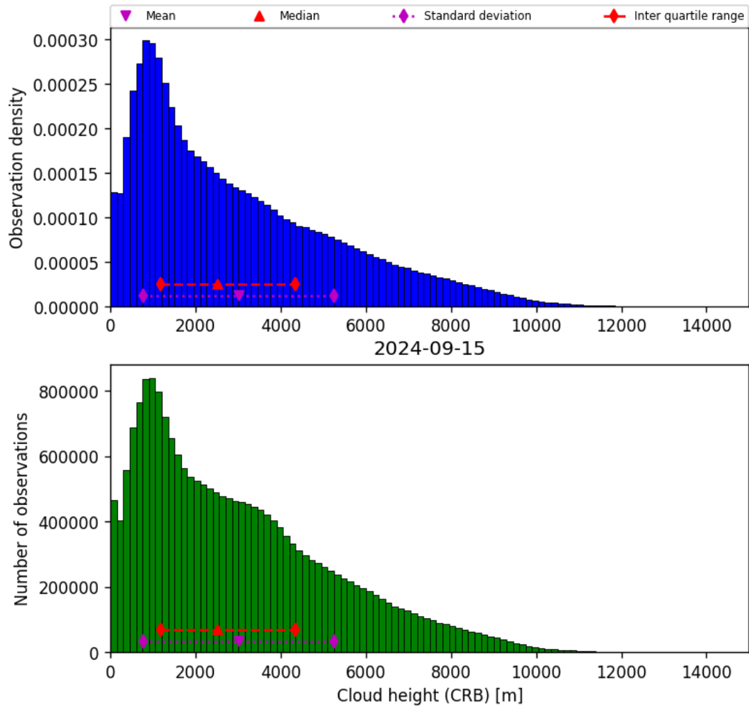
Figure 43: Histogram of “Cloud height (CRB)” for 2024-09-14 to 2024-09-16
