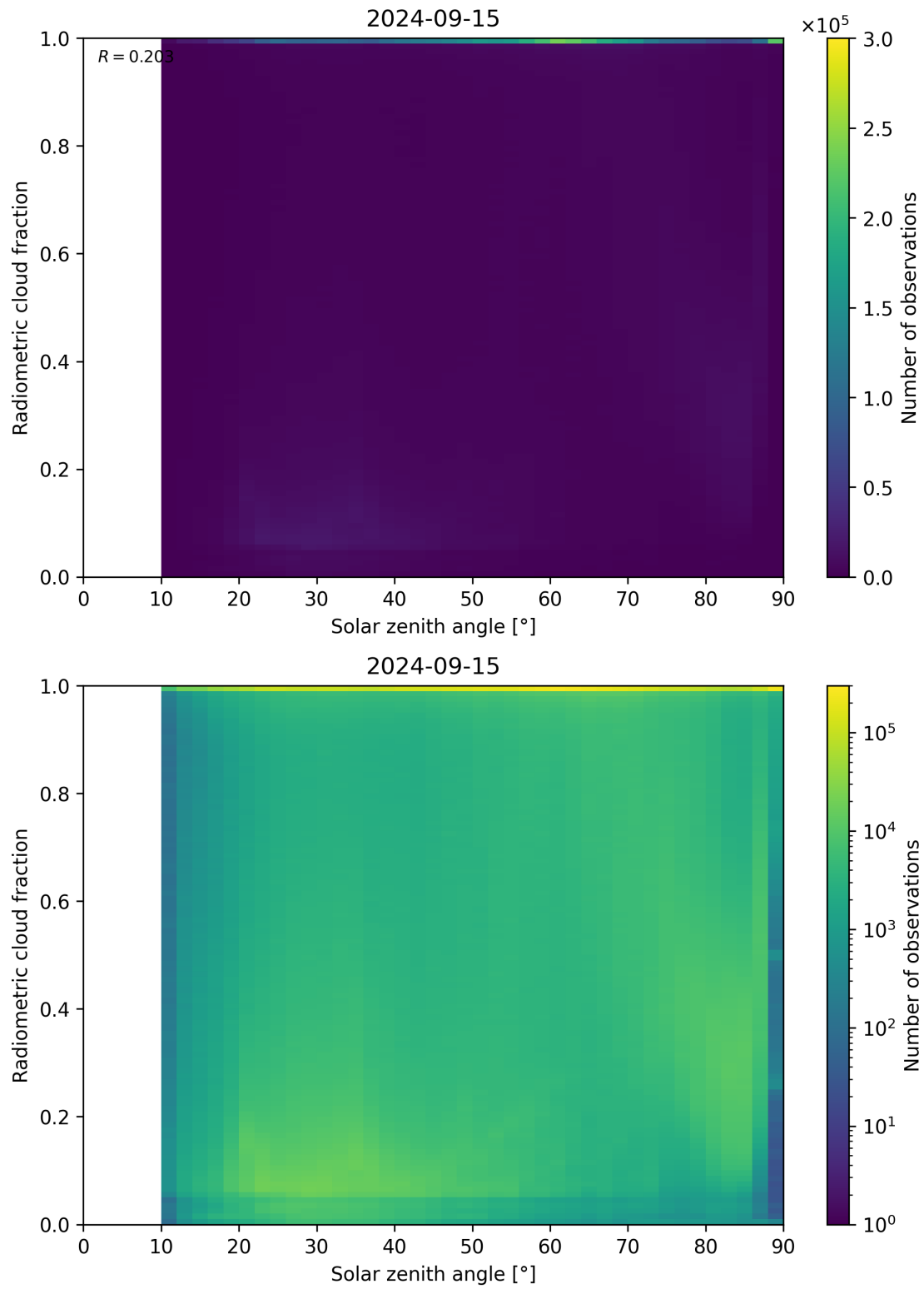
Figure 99: Scatter density plot of “Solar zenith angle” against “Radiometric cloud fraction” for 2024-09-14 to 2024-09-16.
