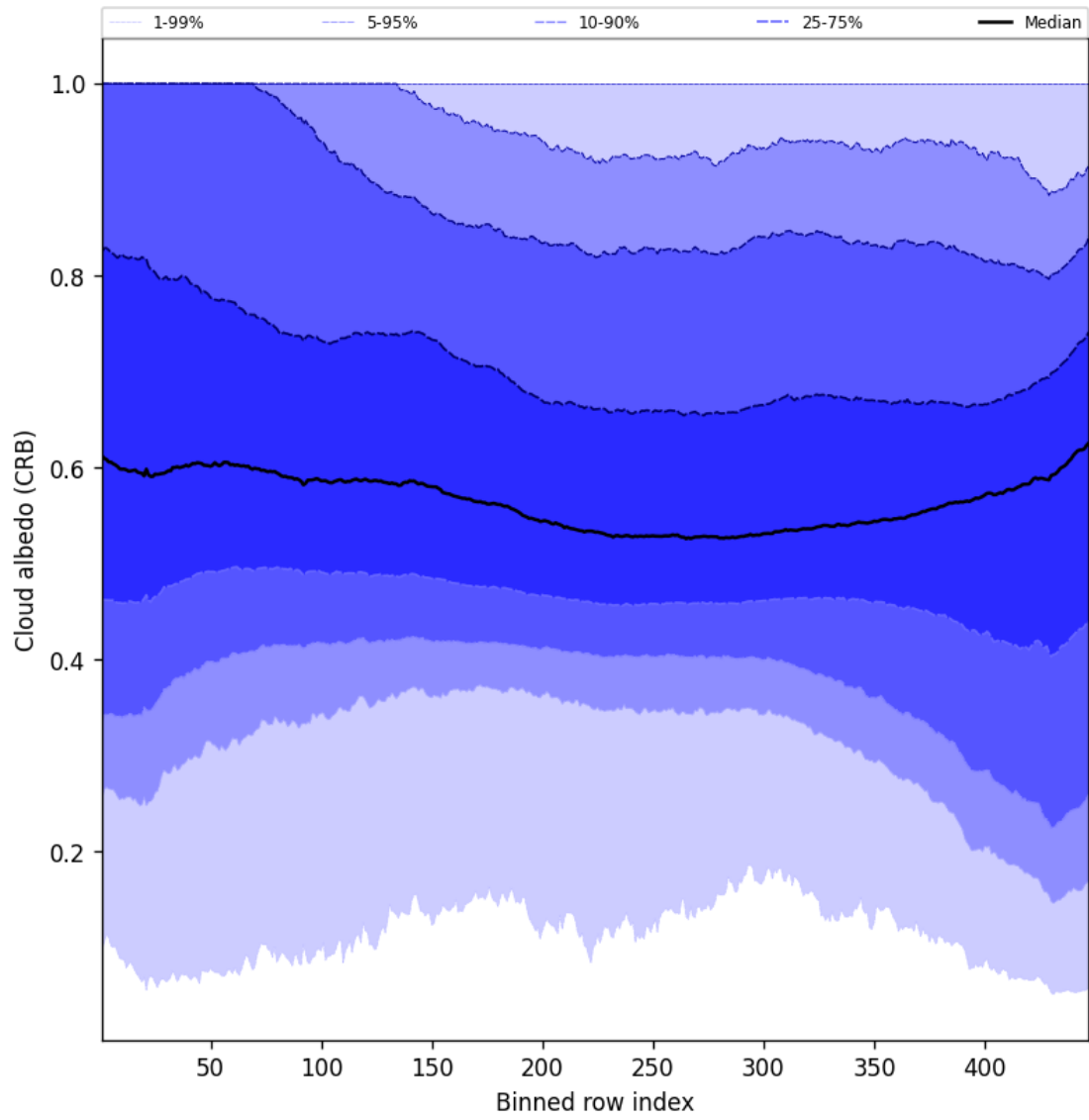
Figure 60: Along track statistics of “Cloud albedo (CRB)” for 2024-09-14 to 2024-09-16
