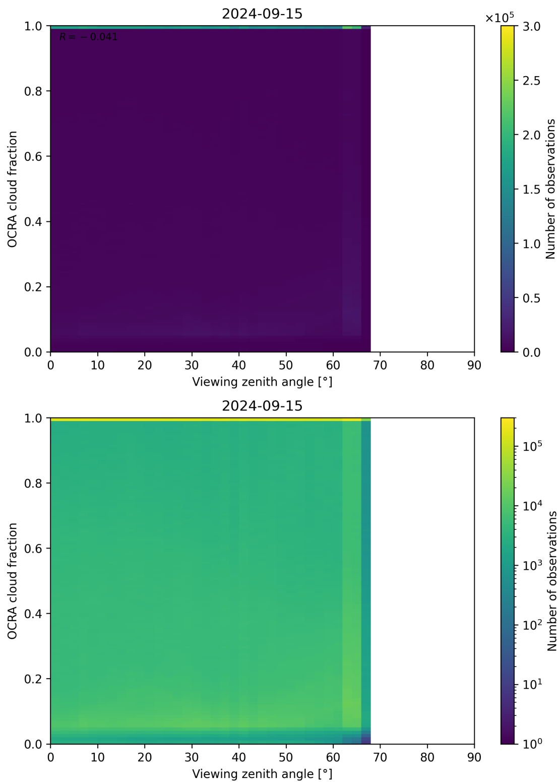
Figure 108: Scatter density plot of “Viewing zenith angle” against “OCRA cloud fraction” for 2024-09-14 to 2024-09-16.
