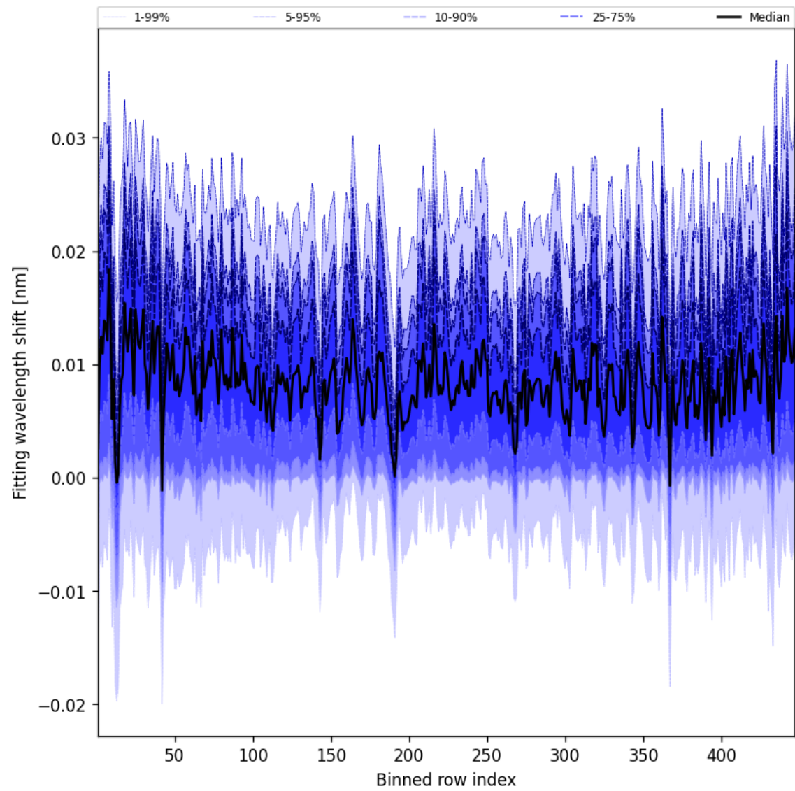
Figure 65: Along track statistics of “Fitting wavelength shift” for 2024-09-14 to 2024-09-16
