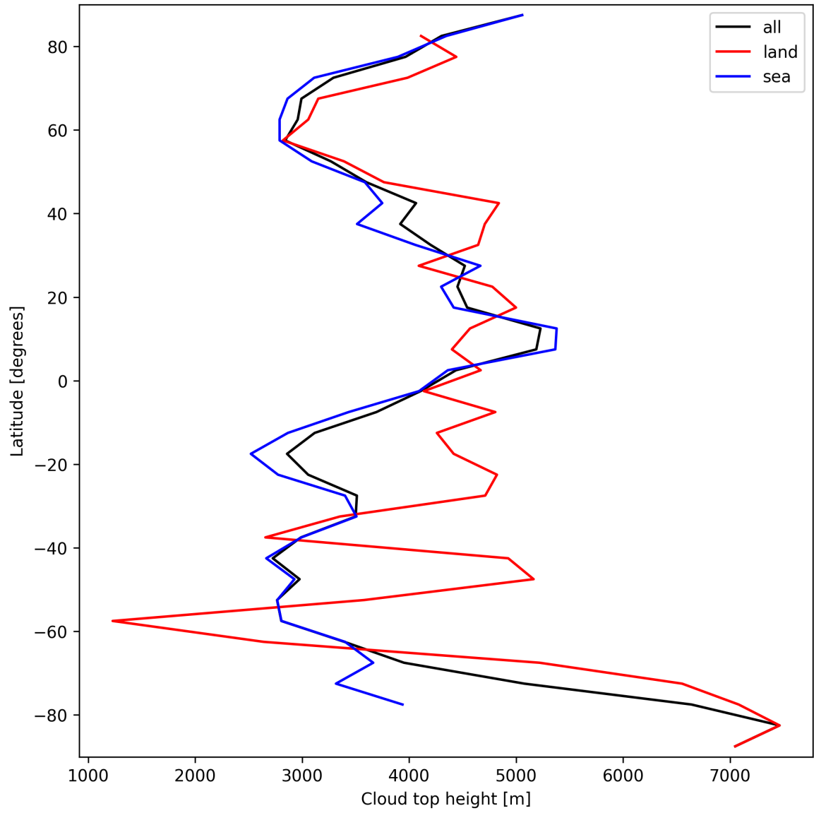
Figure 24: Zonal average of “Cloud top height” for 2024-09-14 to 2024-09-16.
