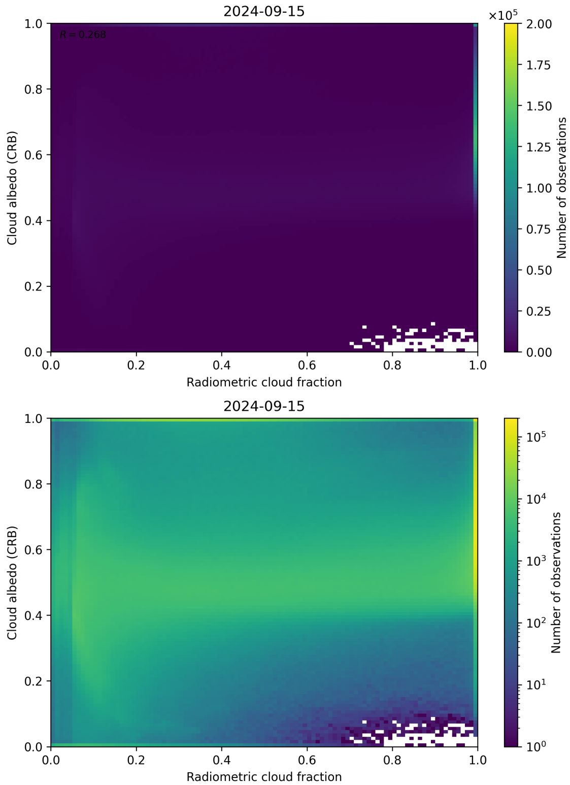
Figure 71: Scatter density plot of “Radiometric cloud fraction” against “Cloud albedo (CRB)” for 2024-09-14 to 2024-09-16.
