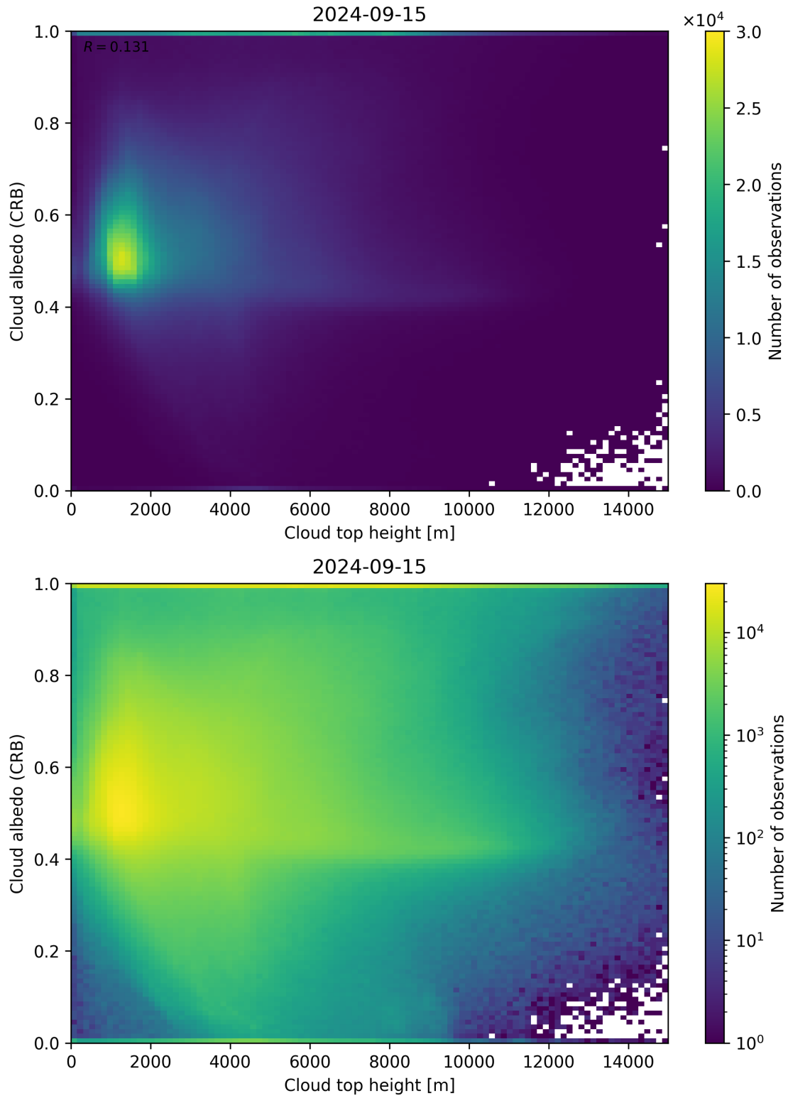
Figure 86: Scatter density plot of “Cloud top height” against “Cloud albedo (CRB)” for 2024-09-14 to 2024-09-16.
