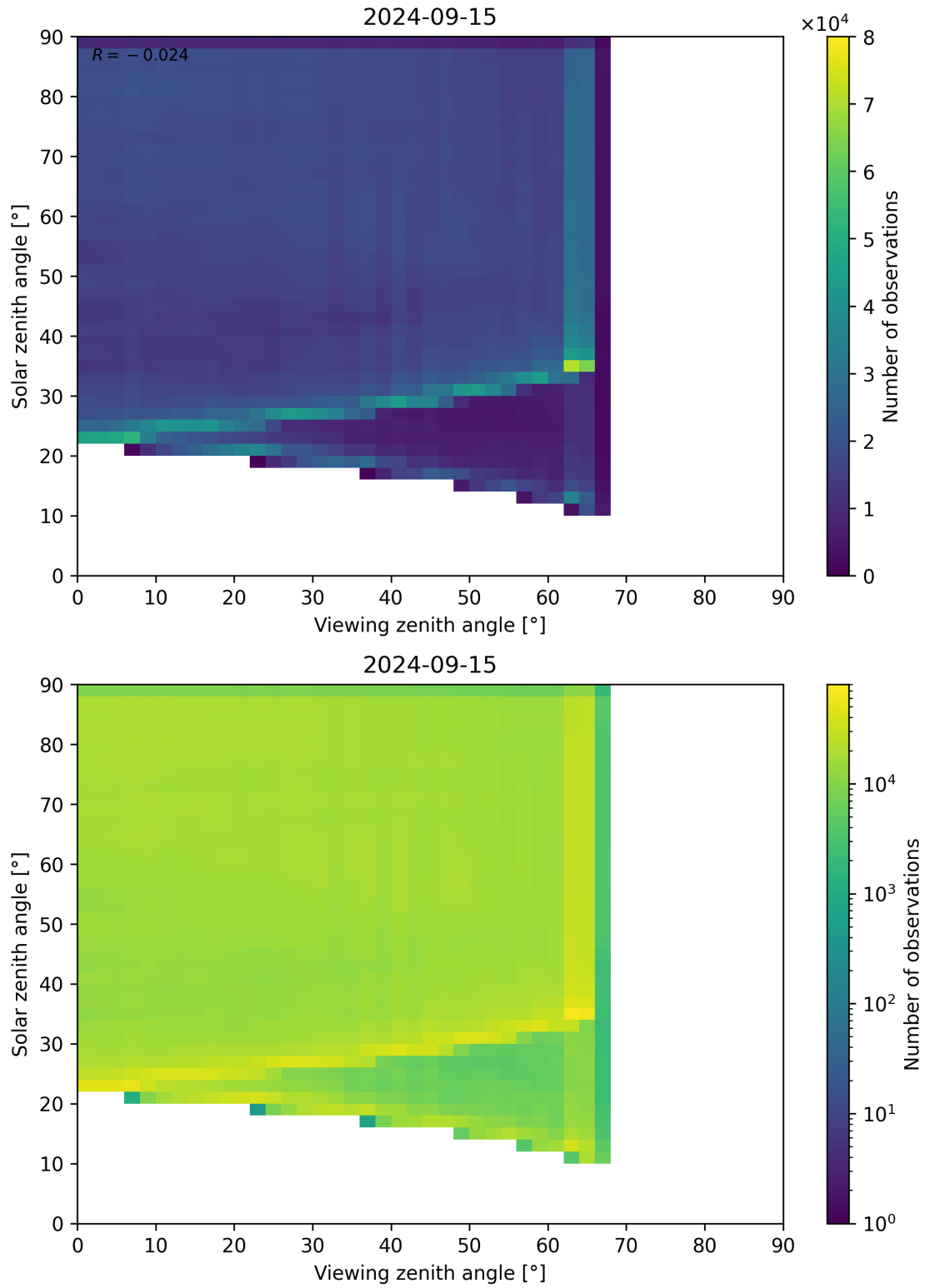
Figure 114: Scatter density plot of “Viewing zenith angle” against “Solar zenith angle” for 2024-09-14 to 2024-09-16.
