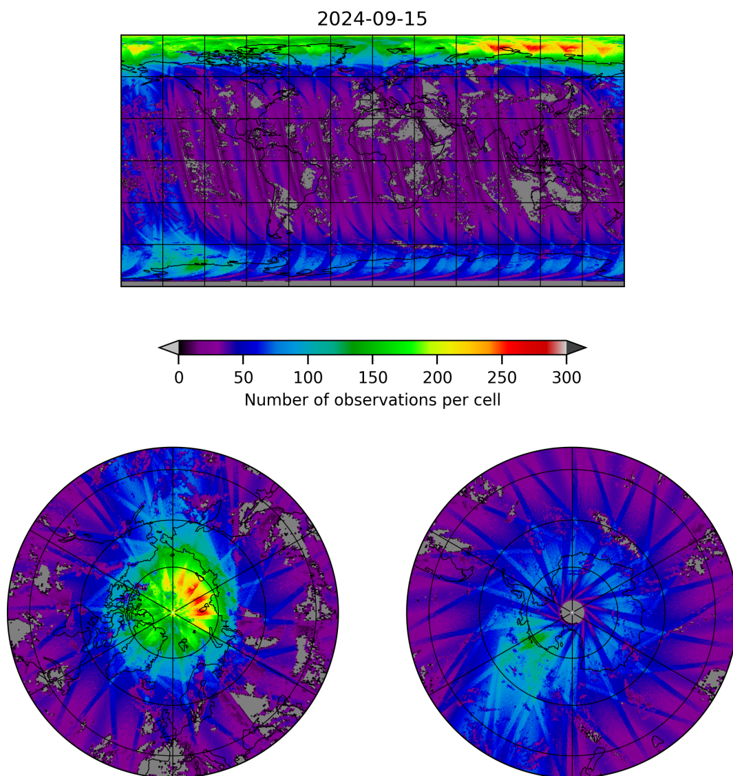
Figure 21: Map of the number of observations for 2024-09-14 to 2024-09-16
