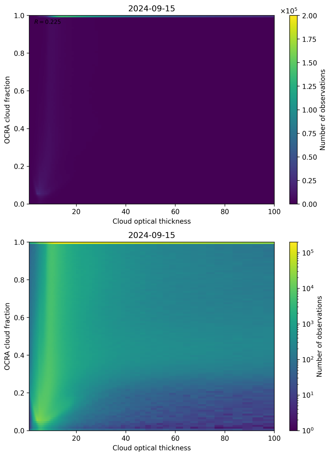
Figure 83: Scatter density plot of “Cloud optical thickness” against “OCRA cloud fraction” for 2024-09-14 to 2024-09-16.
