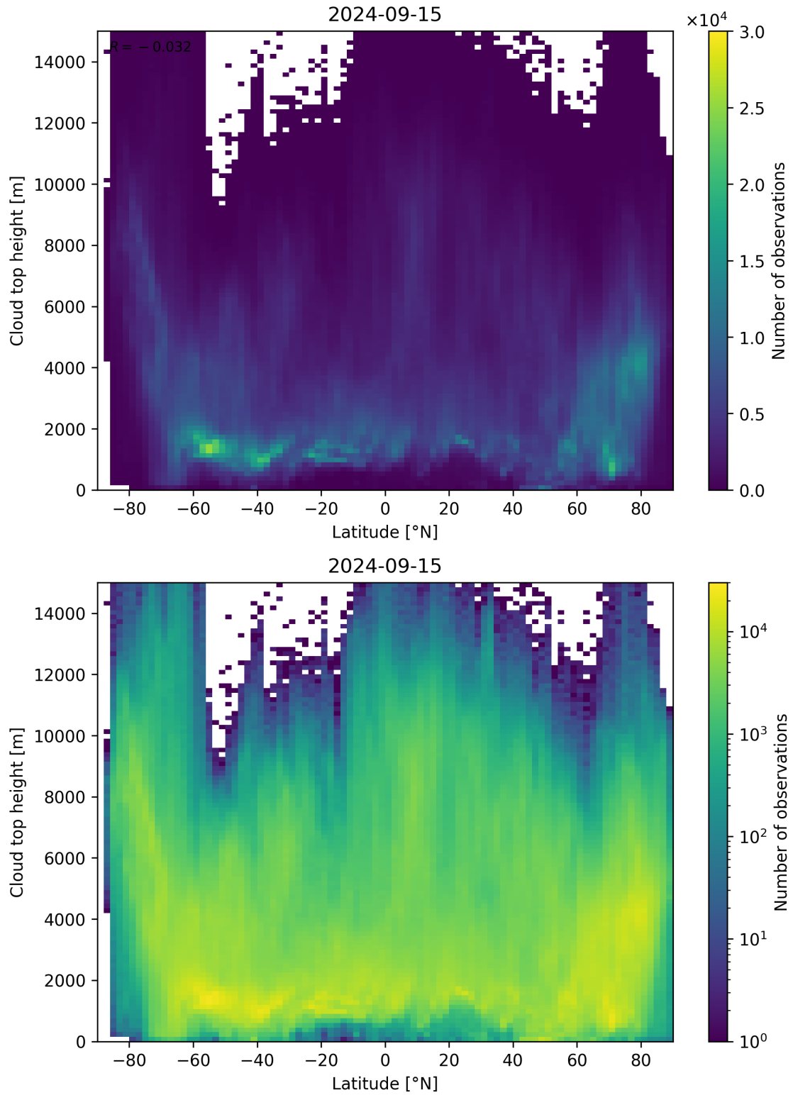
Figure 97: Scatter density plot of “Latitude” against “Cloud top height” for 2024-09-14 to 2024-09-16.
