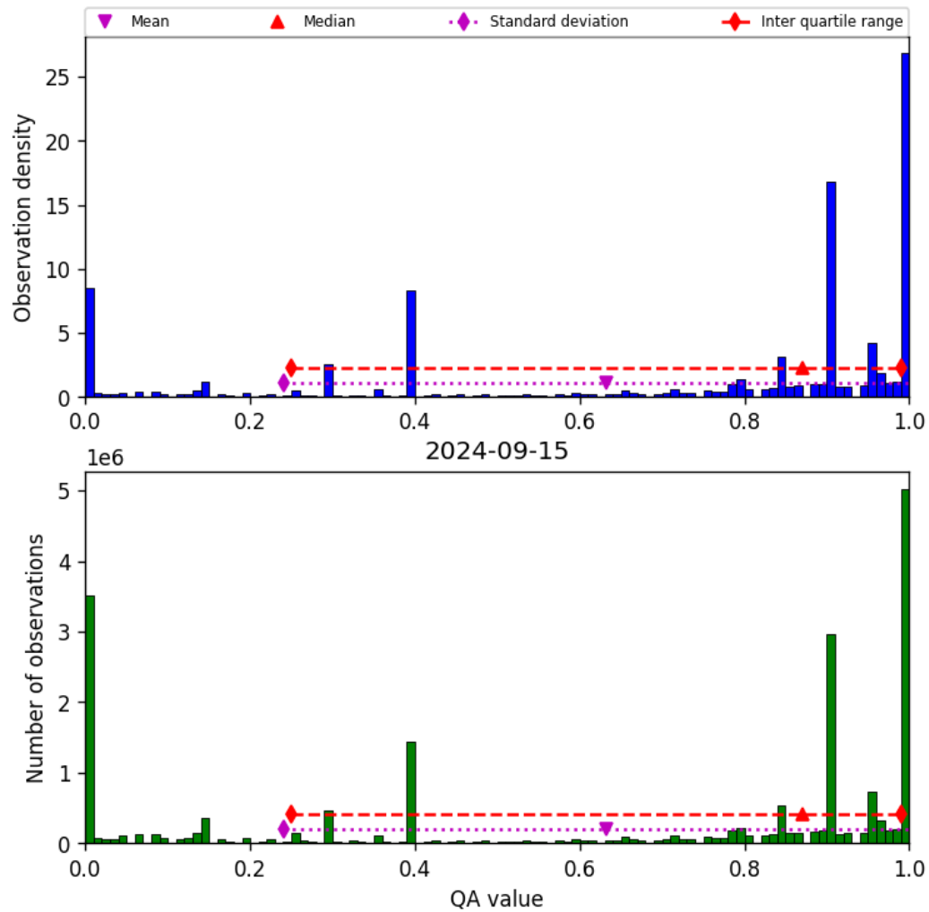
Figure 38: Histogram of “QA value” for 2024-09-14 to 2024-09-16
