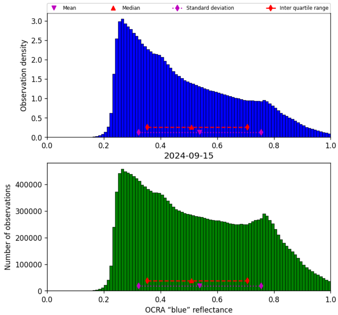
Figure 51: Histogram of “OCRA “blue” reflectance” for 2024-09-14 to 2024-09-16
