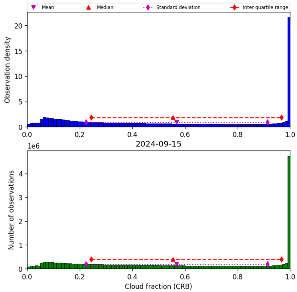
Figure 42: Histogram of “Cloud fraction (CRB)” for 2024-09-14 to 2024-09-16
