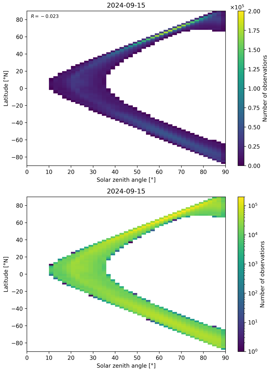
Figure 105: Scatter density plot of “Solar zenith angle” against “Latitude” for 2024-09-14 to 2024-09-16.
