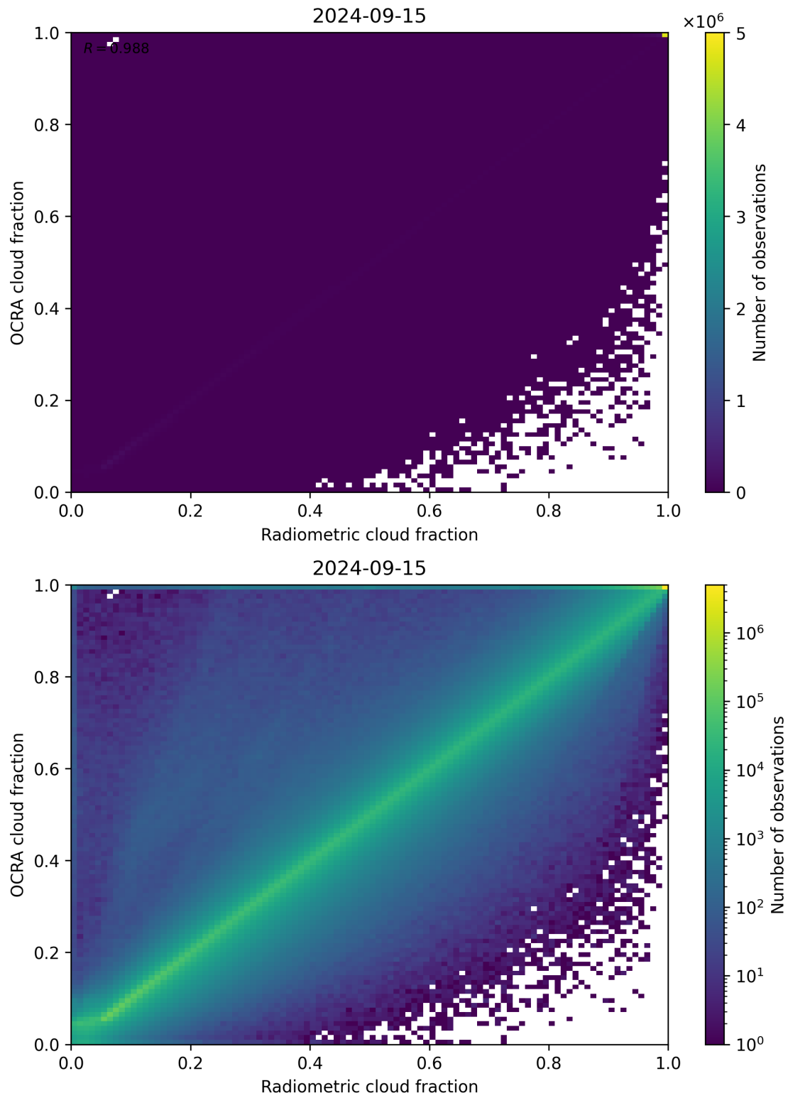
Figure 72: Scatter density plot of “Radiometric cloud fraction” against “OCRA cloud fraction” for 2024-09-14 to 2024-09-16.
