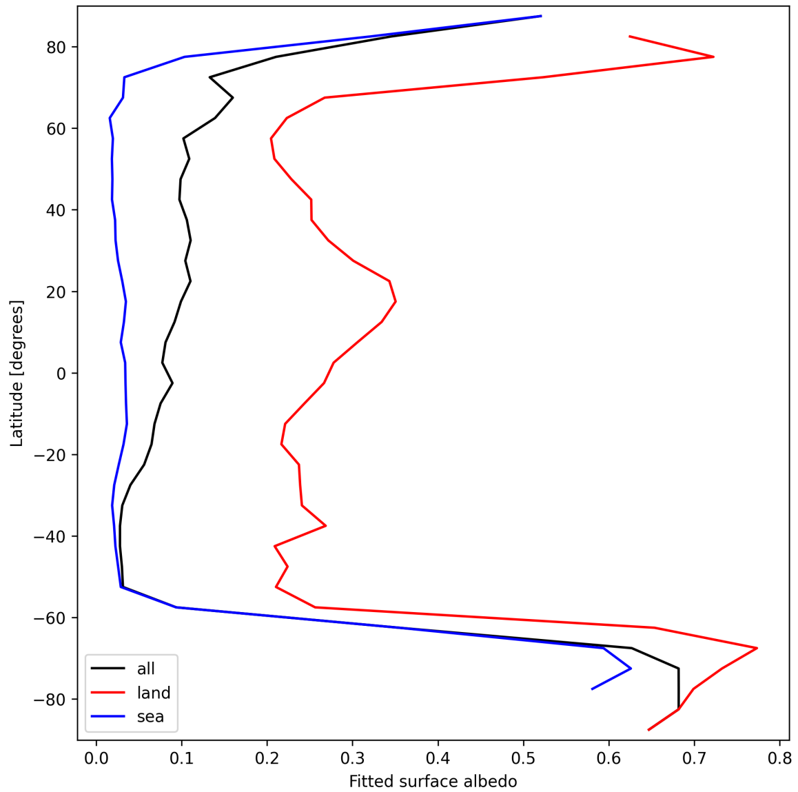
Figure 29: Zonal average of “Fitted surface albedo” for 2024-09-14 to 2024-09-16.
