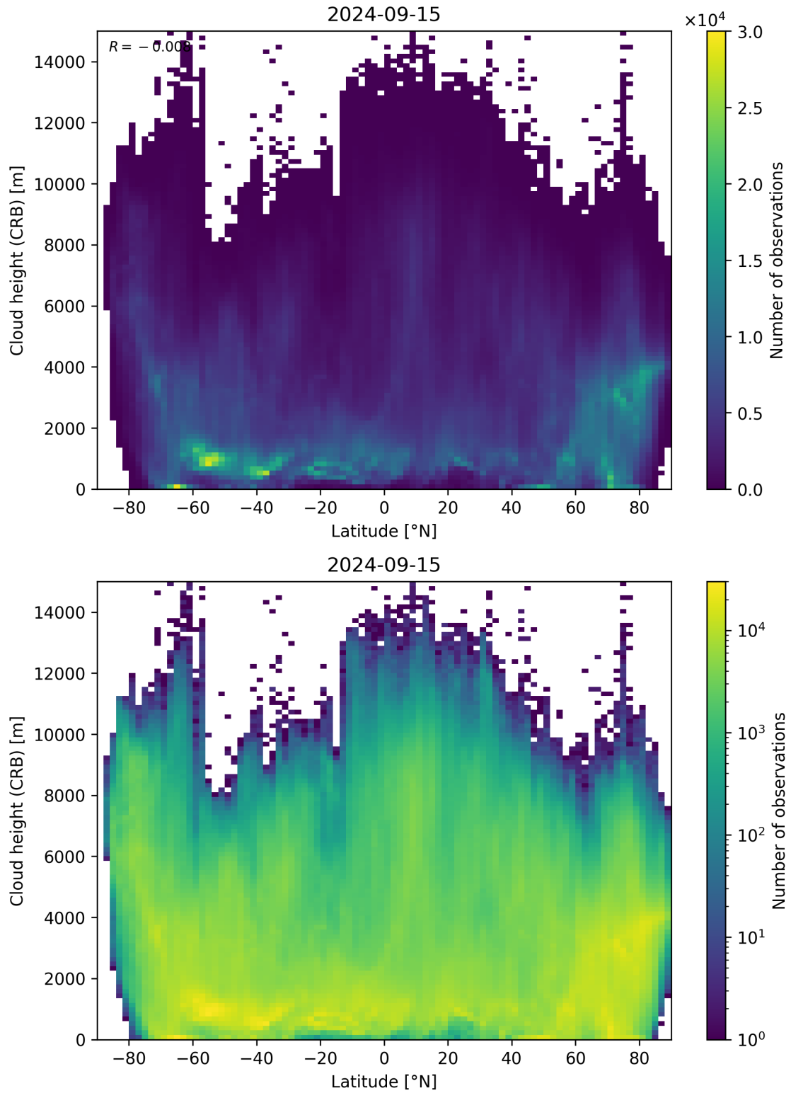
Figure 95: Scatter density plot of “Latitude” against “Cloud height (CRB)” for 2024-09-14 to 2024-09-16.
