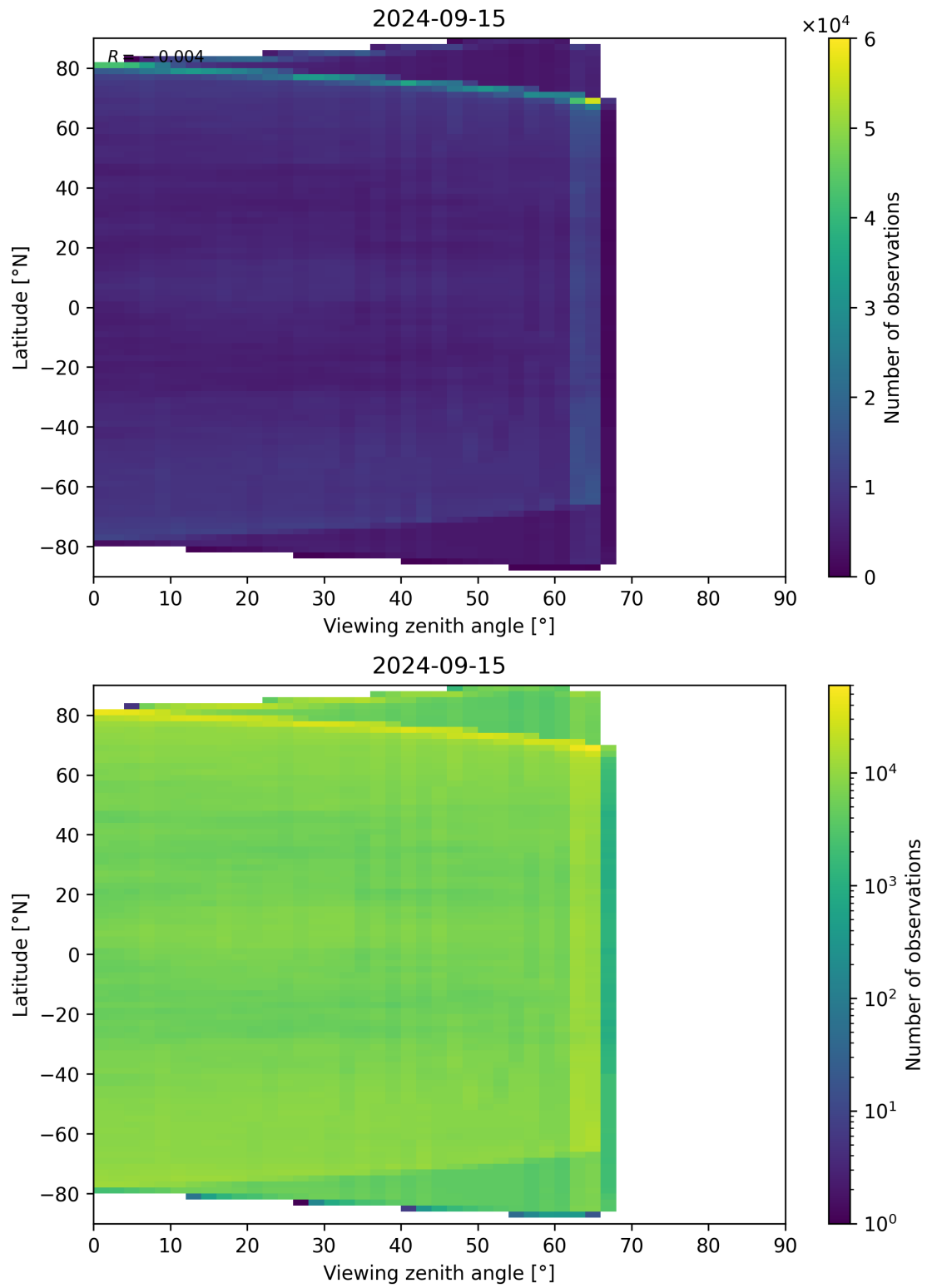
Figure 113: Scatter density plot of “Viewing zenith angle” against “Latitude” for 2024-09-14 to 2024-09-16.
