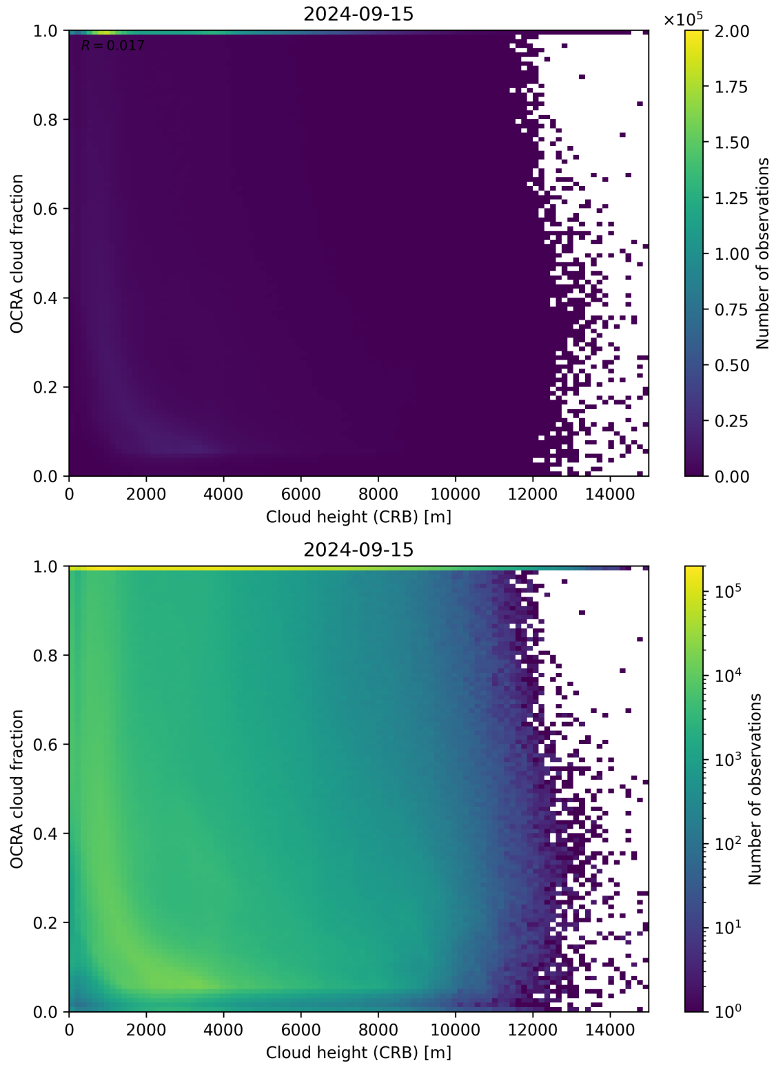
Figure 81: Scatter density plot of “Cloud height (CRB)” against “OCRA cloud fraction” for 2024-09-14 to 2024-09-16.
