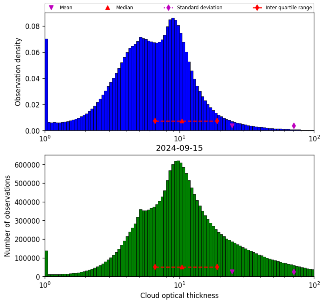
Figure 41: Histogram of “Cloud optical thickness” for 2024-09-14 to 2024-09-16
