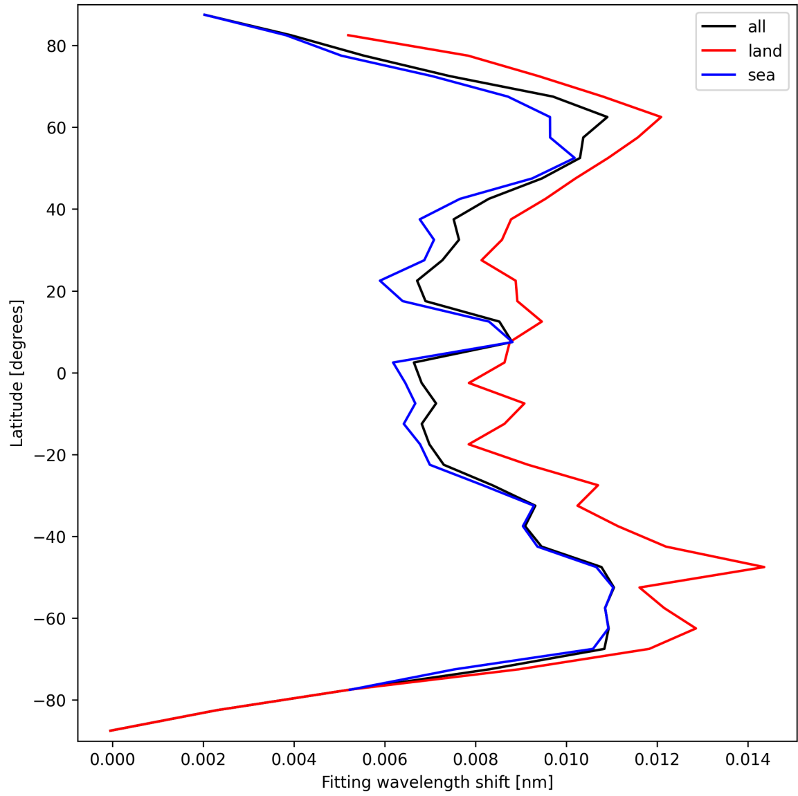
Figure 33: Zonal average of “Fitting wavelength shift” for 2024-09-14 to 2024-09-16.
