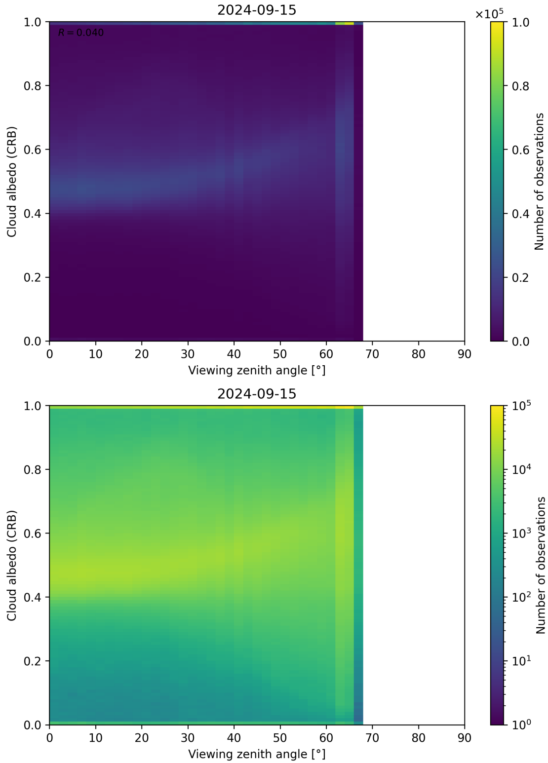
Figure 106: Scatter density plot of “Viewing zenith angle” against “Cloud albedo (CRB)” for 2024-09-14 to 2024-09-16.
