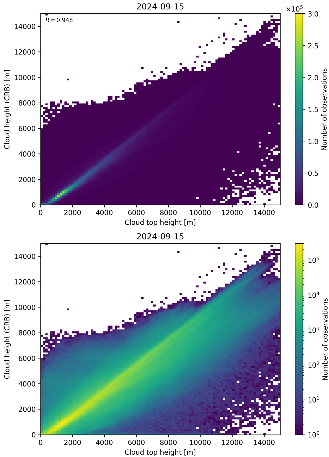
Figure 89: Scatter density plot of “Cloud top height” against “Cloud height (CRB)” for 2024-09-14 to 2024-09-16.
