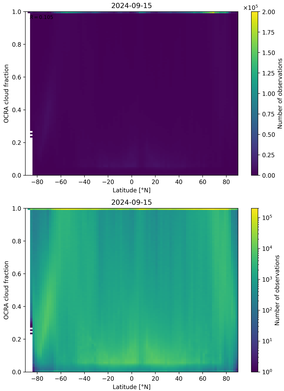
Figure 93: Scatter density plot of “Latitude” against “OCRA cloud fraction” for 2024-09-14 to 2024-09-16.
