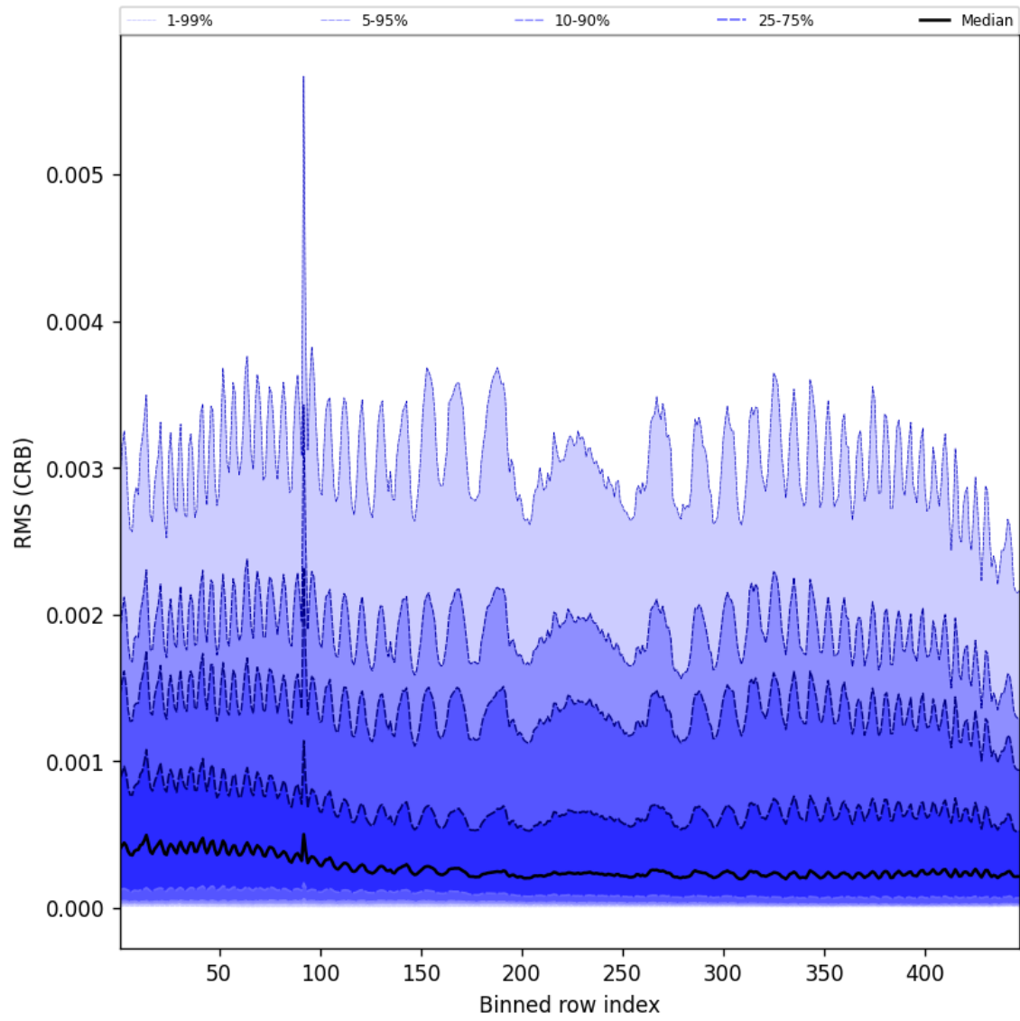
Figure 64: Along track statistics of “RMS (CRB)” for 2024-09-14 to 2024-09-16
