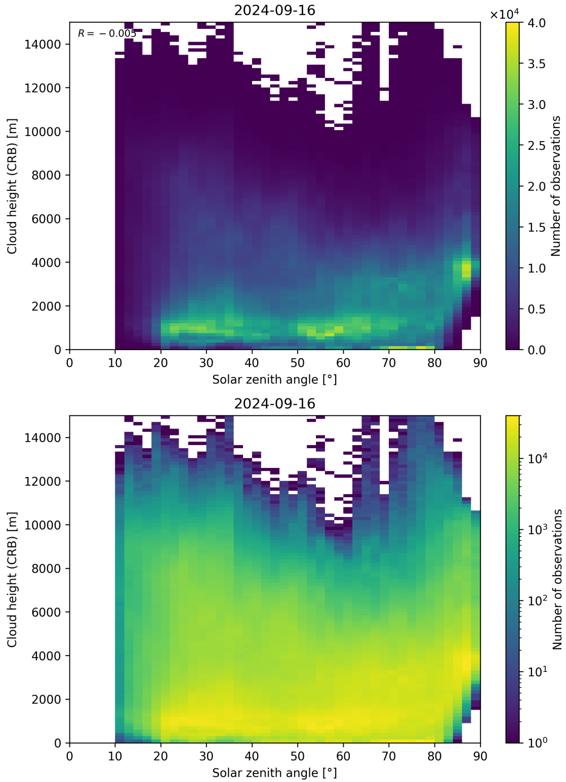
Figure 102: Scatter density plot of “Solar zenith angle” against “Cloud height (CRB)” for 2024-09-15 to 2024-09-17.
