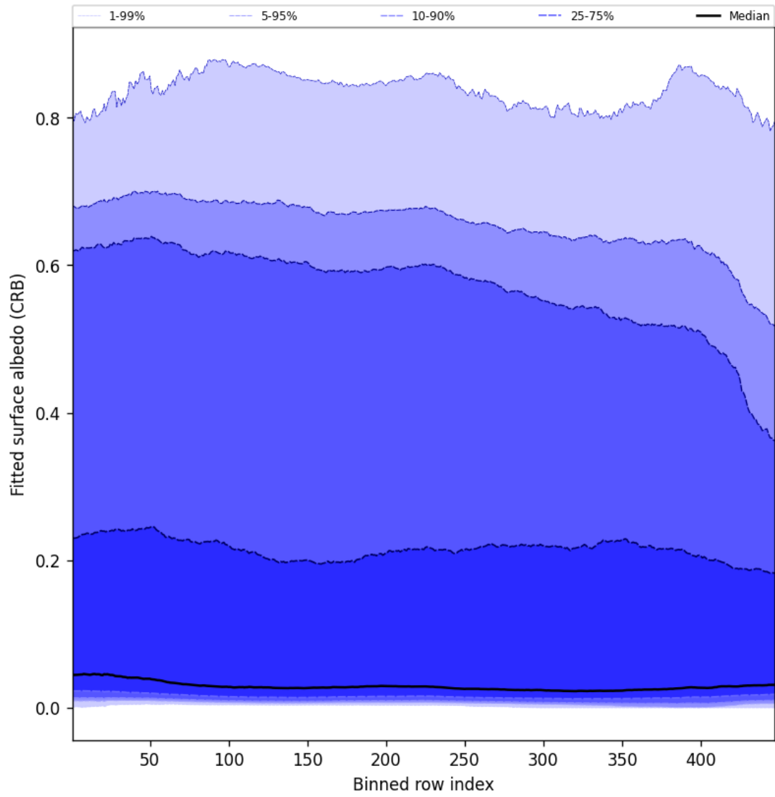
Figure 62: Along track statistics of “Fitted surface albedo (CRB)” for 2024-09-15 to 2024-09-17
