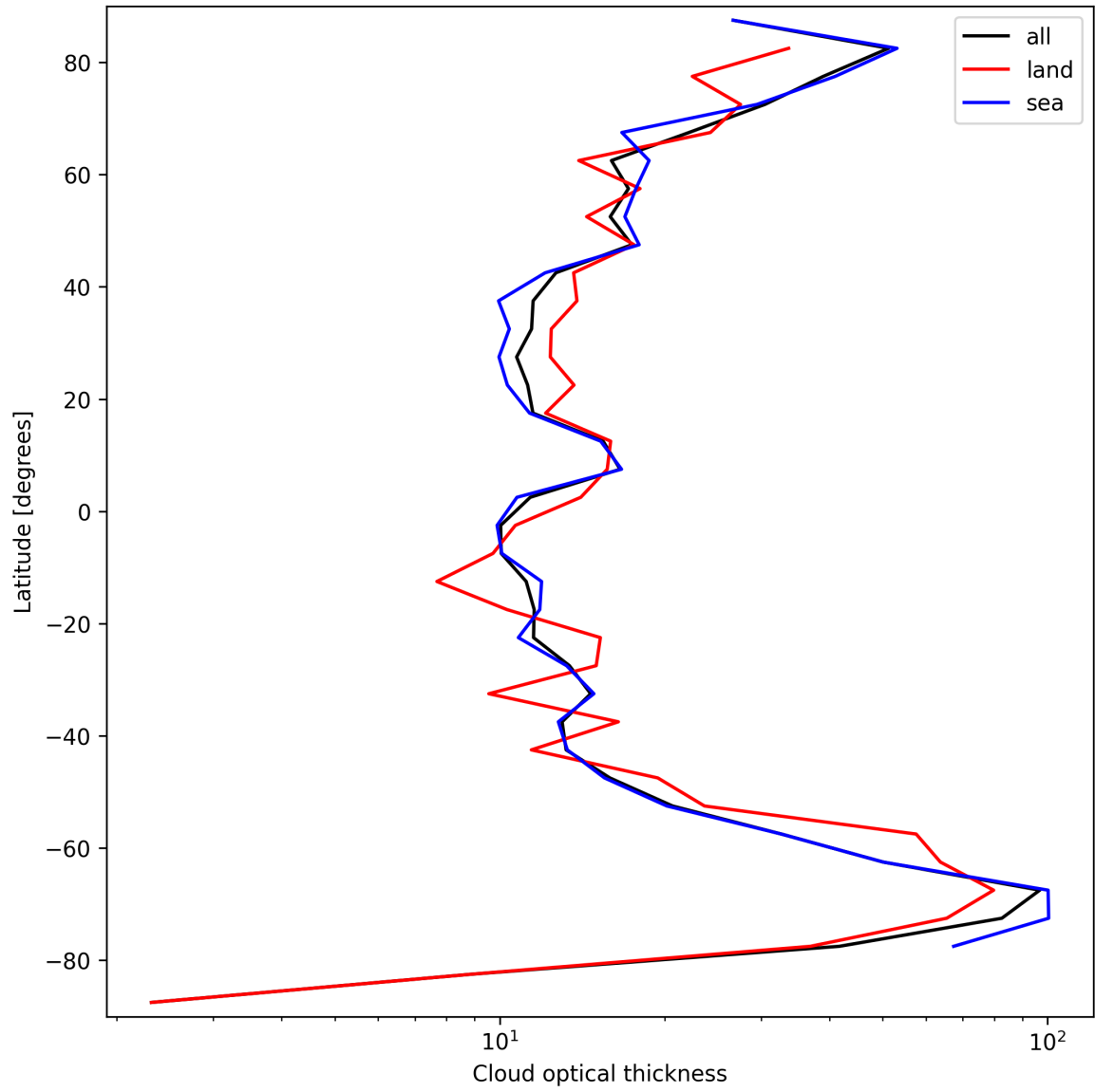
Figure 25: Zonal average of “Cloud optical thickness” for 2024-09-15 to 2024-09-17.
