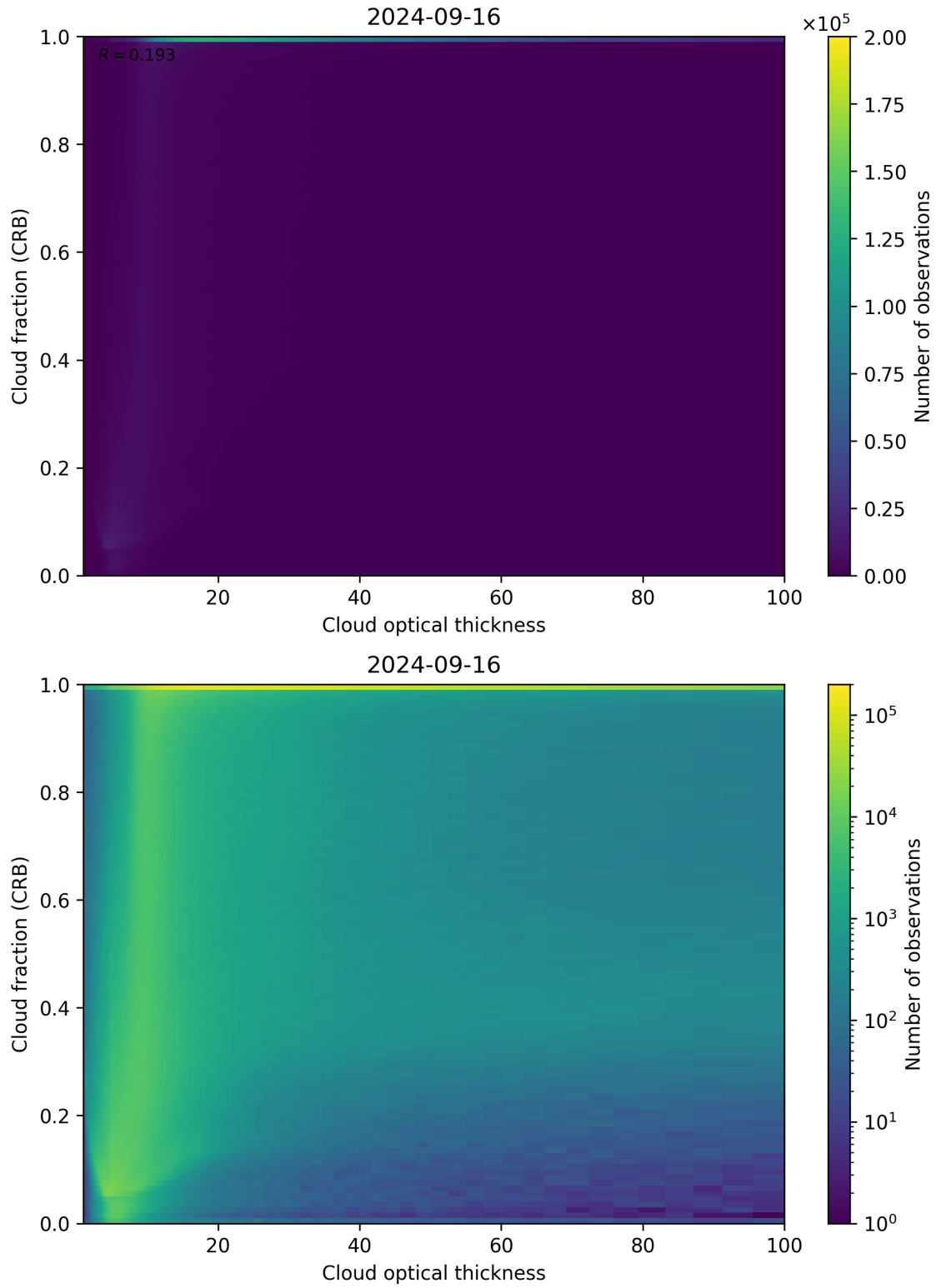
Figure 84: Scatter density plot of “Cloud optical thickness” against “Cloud fraction (CRB)” for 2024-09-15 to 2024-09-17.
