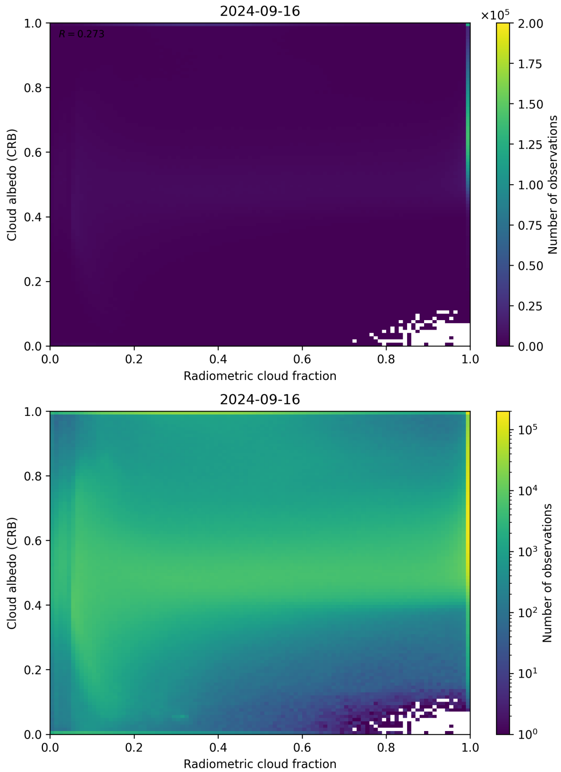
Figure 71: Scatter density plot of “Radiometric cloud fraction” against “Cloud albedo (CRB)” for 2024-09-15 to 2024-09-17.
