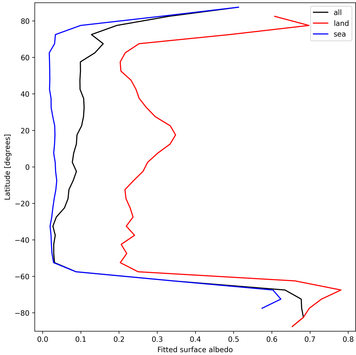
Figure 29: Zonal average of “Fitted surface albedo” for 2024-09-15 to 2024-09-17.
