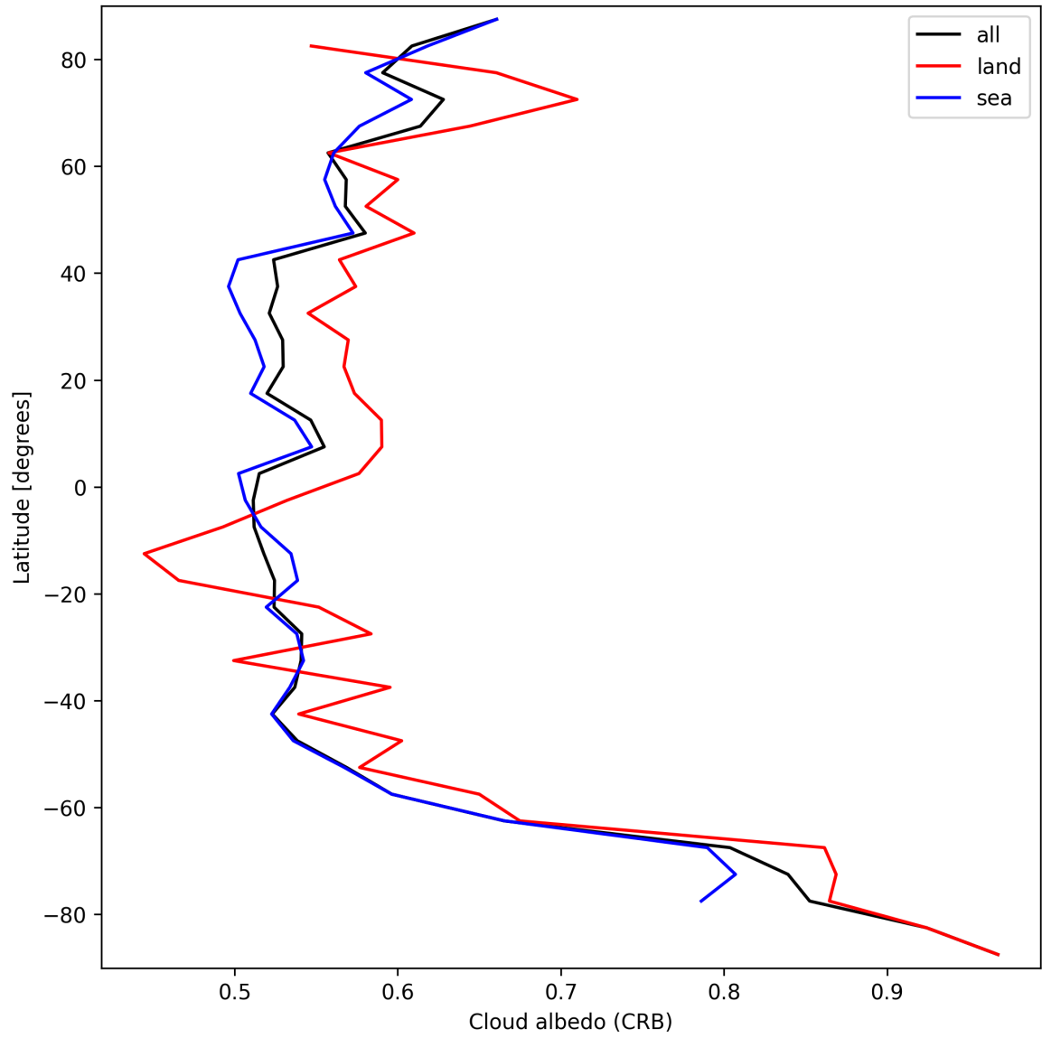
Figure 28: Zonal average of “Cloud albedo (CRB)” for 2024-09-15 to 2024-09-17.
