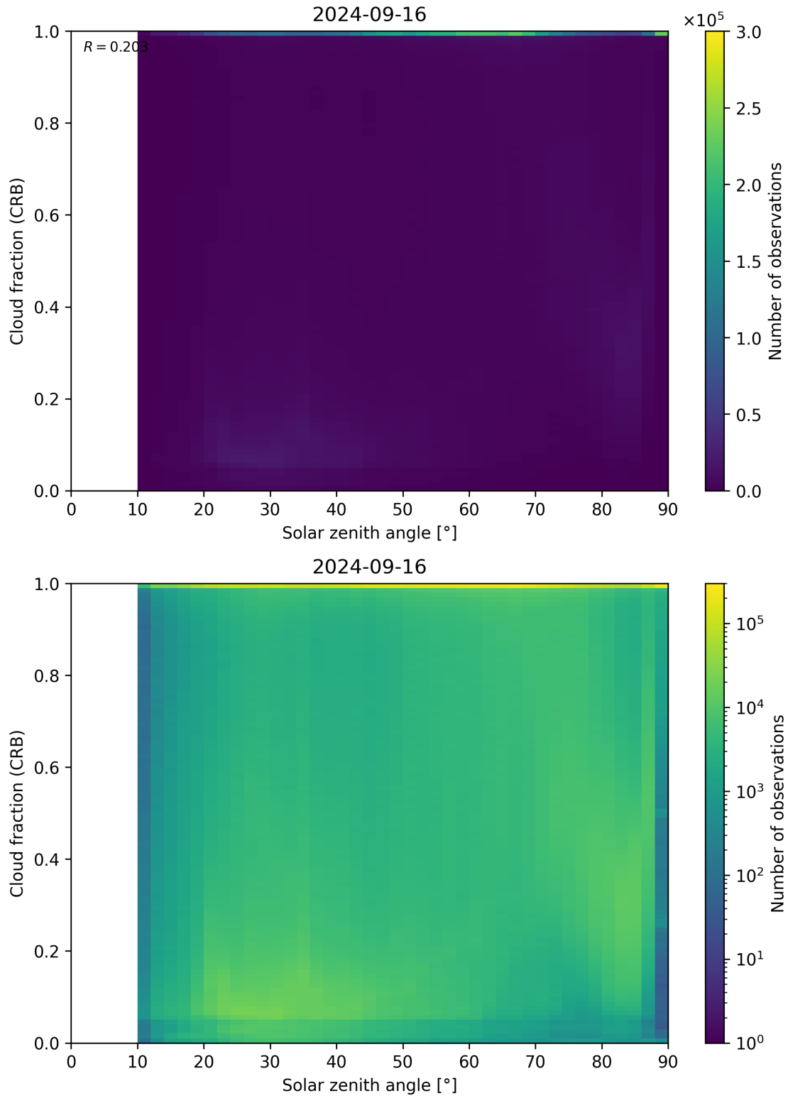
Figure 101: Scatter density plot of “Solar zenith angle” against “Cloud fraction (CRB)” for 2024-09-15 to 2024-09-17.
