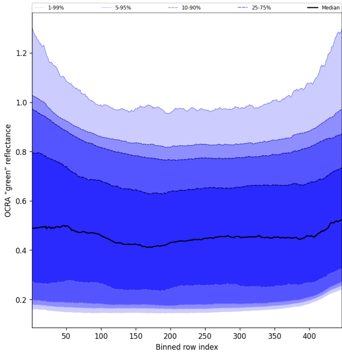
Figure 68: Along track statistics of "OCRA "green" reflectance" for 2024-09-15 to 2024-09-17
