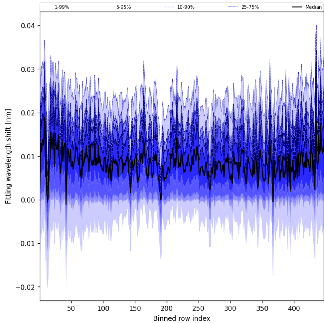
Figure 65: Along track statistics of “Fitting wavelength shift” for 2024-09-15 to 2024-09-17
