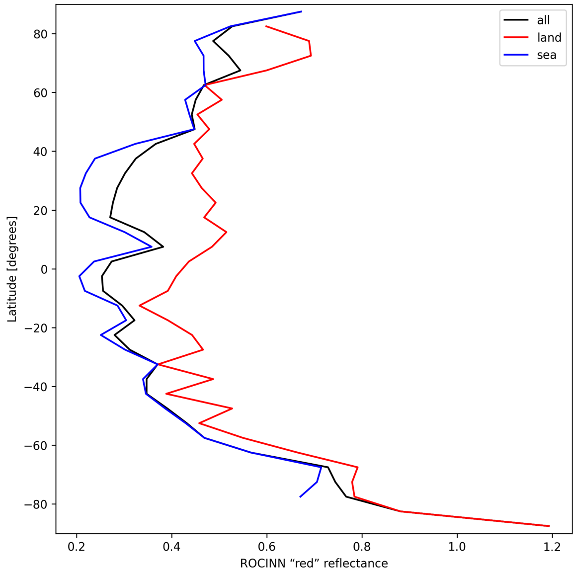
Figure 37: Zonal average of “ROCINN “red” reflectance” for 2024-09-15 to 2024-09-17.
