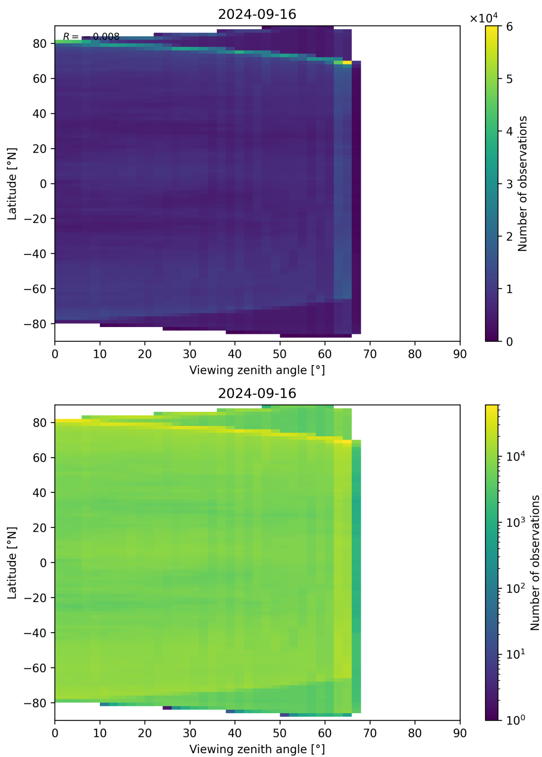
Figure 113: Scatter density plot of “Viewing zenith angle” against “Latitude” for 2024-09-15 to 2024-09-17.
