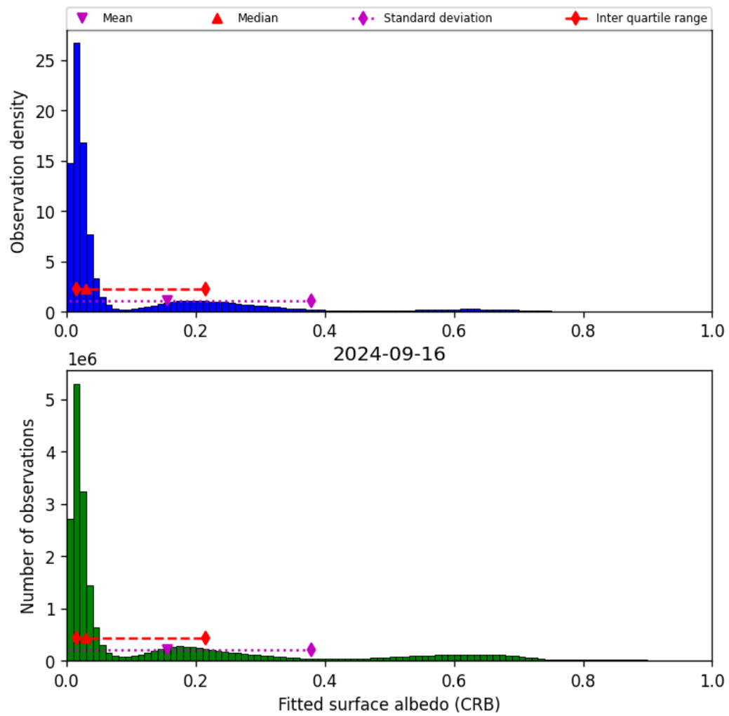
Figure 46: Histogram of “Fitted surface albedo (CRB)” for 2024-09-15 to 2024-09-17
