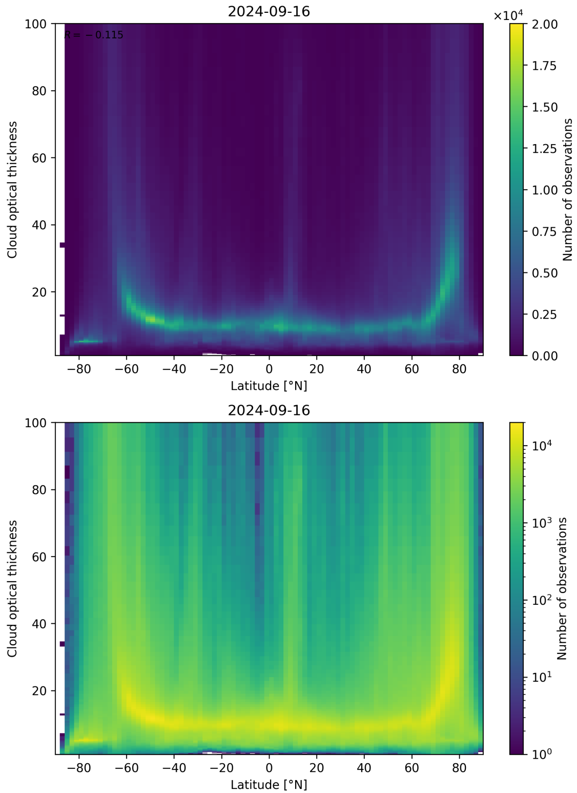
Figure 96: Scatter density plot of “Latitude” against “Cloud optical thickness” for 2024-09-15 to 2024-09-17.
