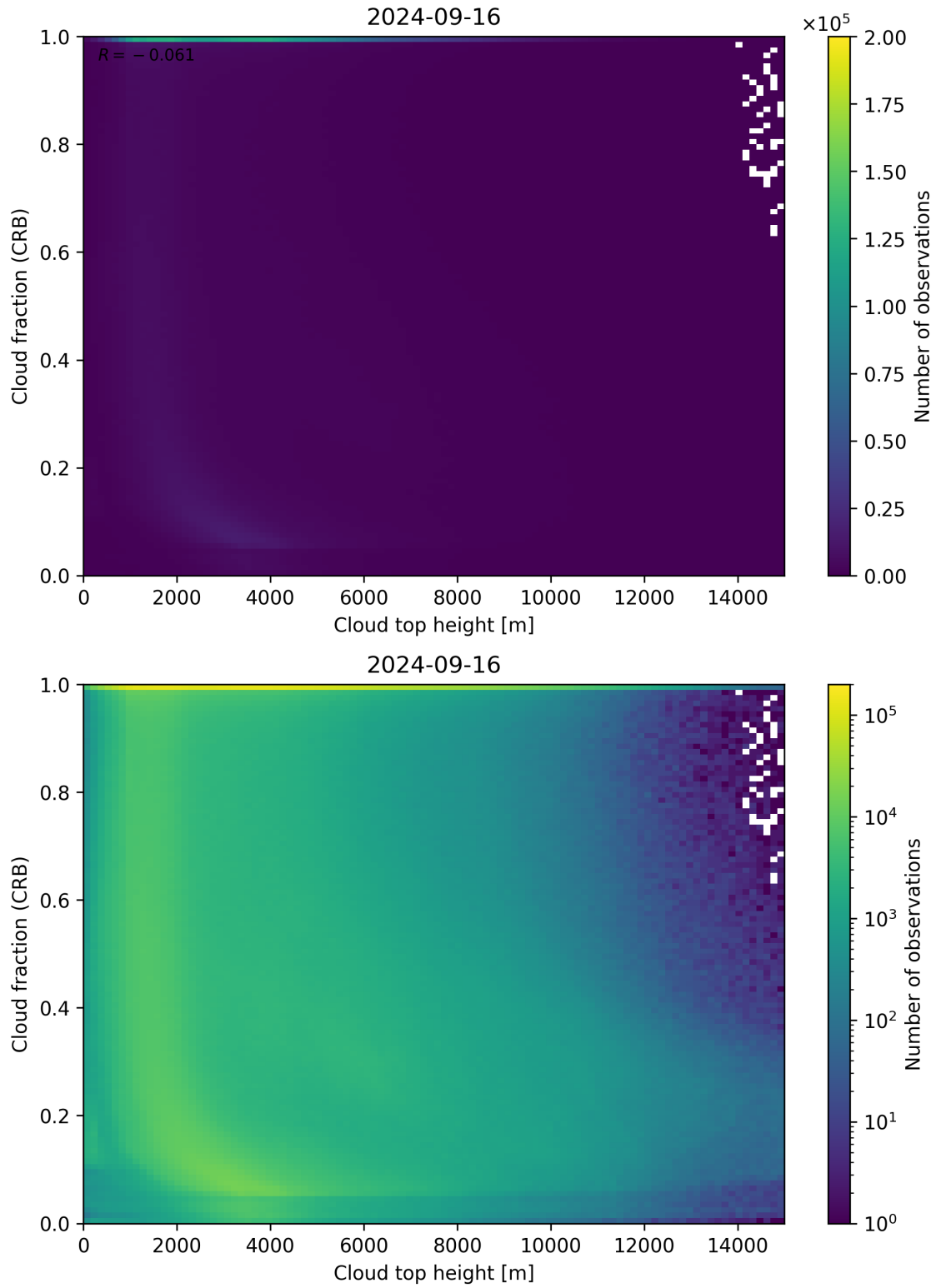
Figure 88: Scatter density plot of “Cloud top height” against “Cloud fraction (CRB)” for 2024-09-15 to 2024-09-17.
