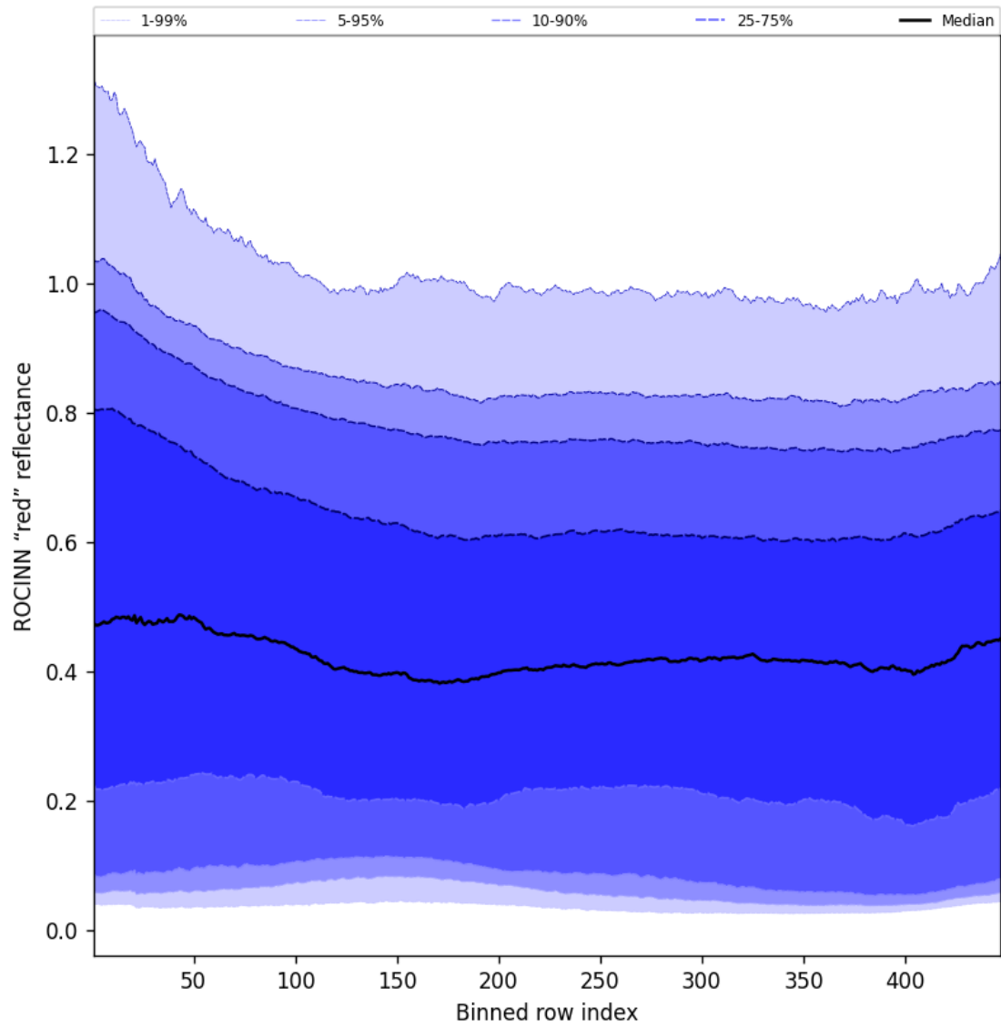
Figure 69: Along track statistics of “ROCINN “red” reflectance” for 2024-09-15 to 2024-09-17
