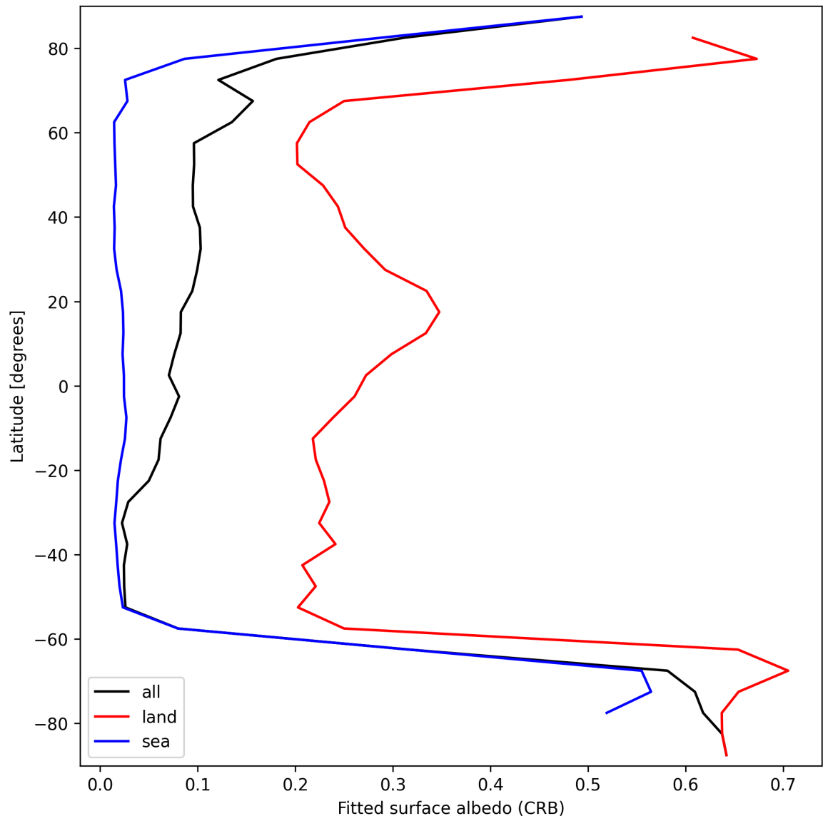
Figure 30: Zonal average of “Fitted surface albedo (CRB)” for 2024-09-15 to 2024-09-17.
