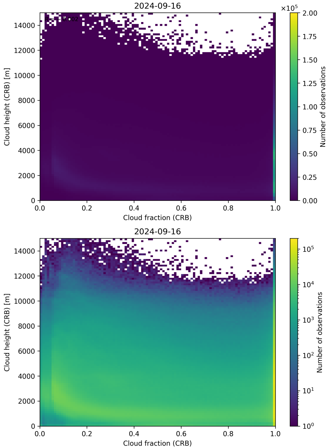
Figure 79: Scatter density plot of “Cloud fraction (CRB)” against “Cloud height (CRB)” for 2024-09-15 to 2024-09-17.
