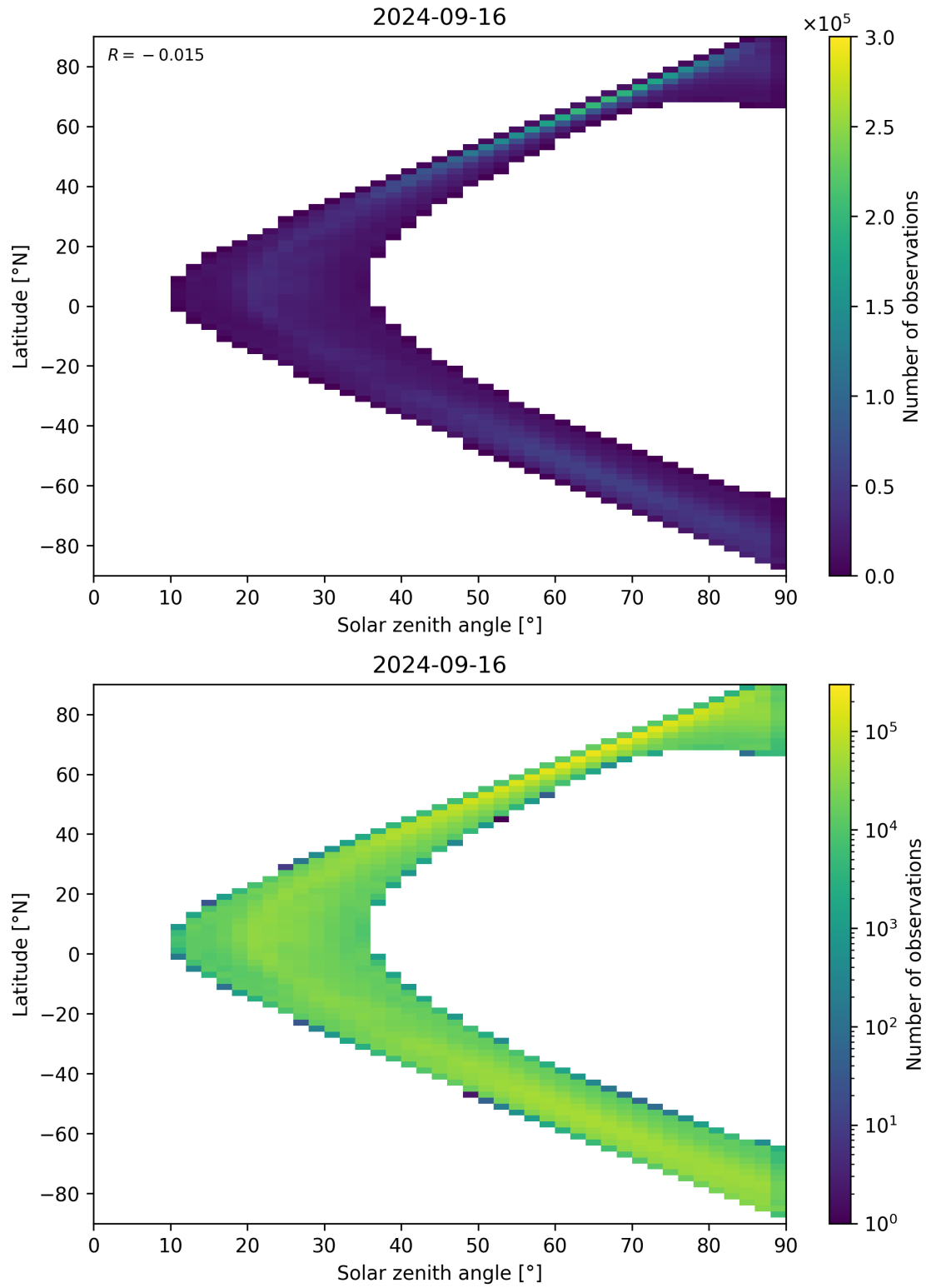
Figure 105: Scatter density plot of “Solar zenith angle” against “Latitude” for 2024-09-15 to 2024-09-17.
