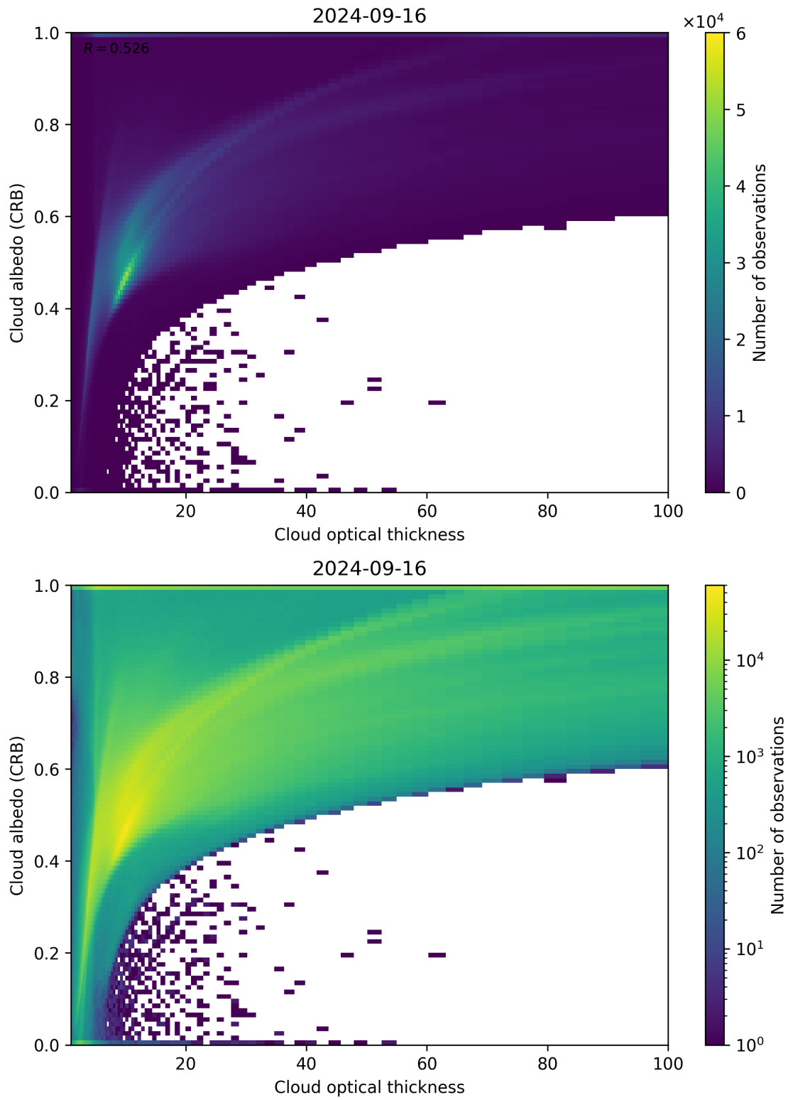
Figure 82: Scatter density plot of “Cloud optical thickness” against “Cloud albedo (CRB)” for 2024-09-15 to 2024-09-17.
