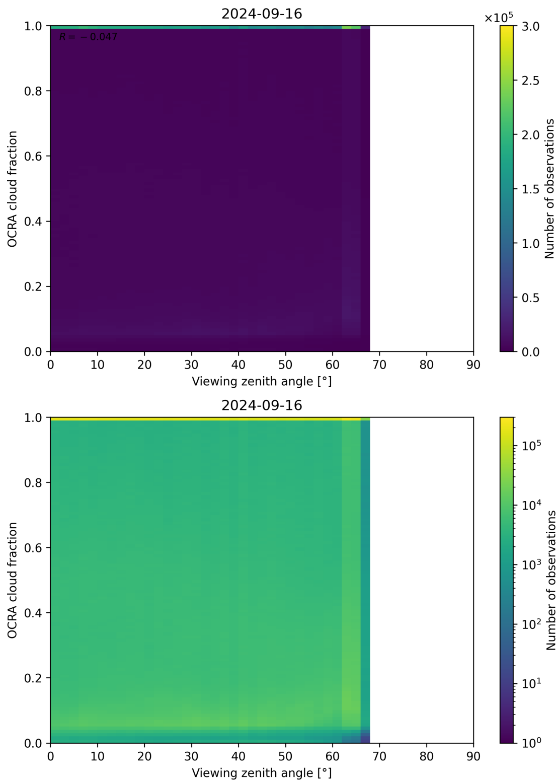
Figure 108: Scatter density plot of “Viewing zenith angle” against “OCRA cloud fraction” for 2024-09-15 to 2024-09-17.
