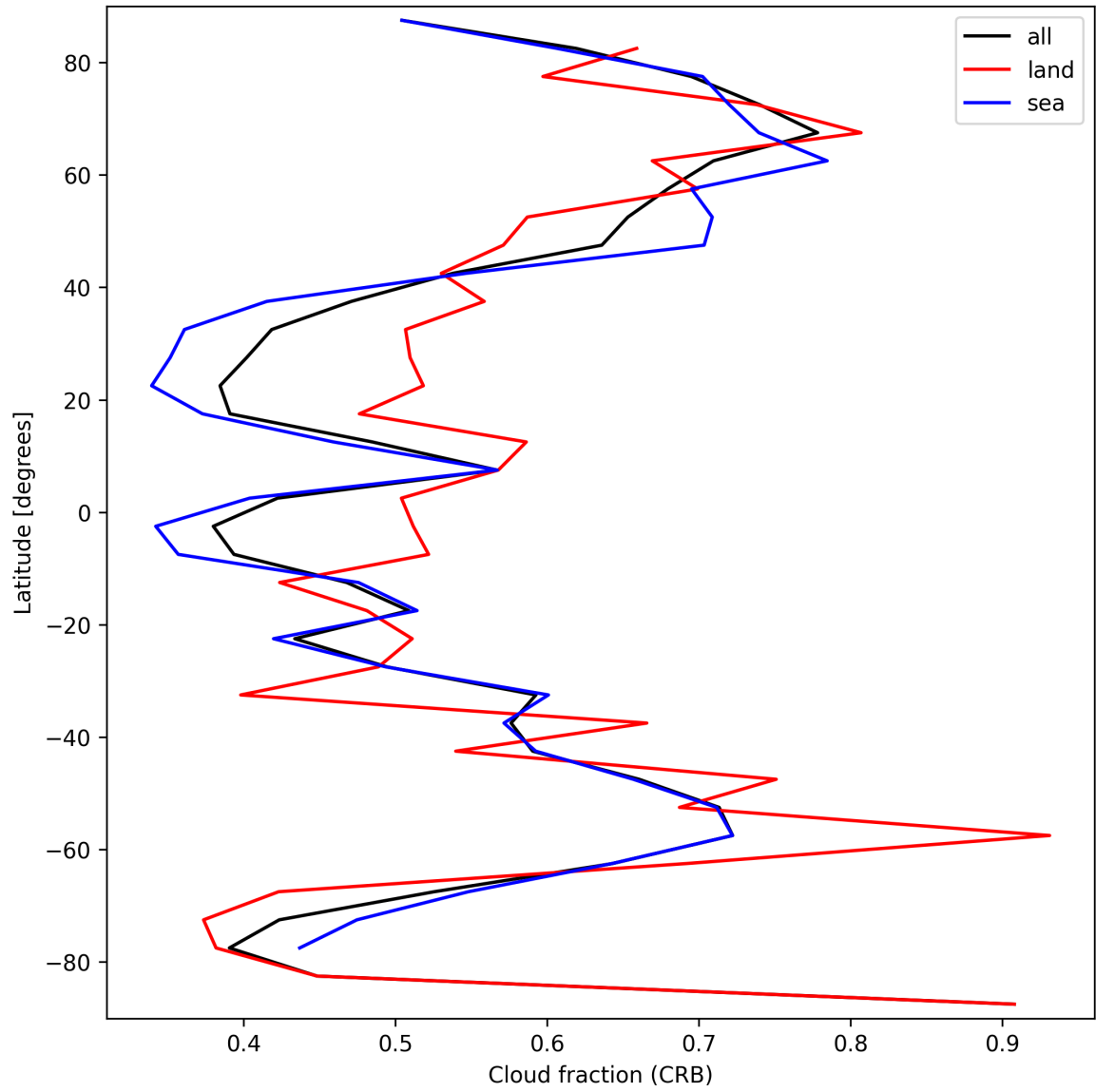
Figure 26: Zonal average of “Cloud fraction (CRB)” for 2024-09-15 to 2024-09-17.
