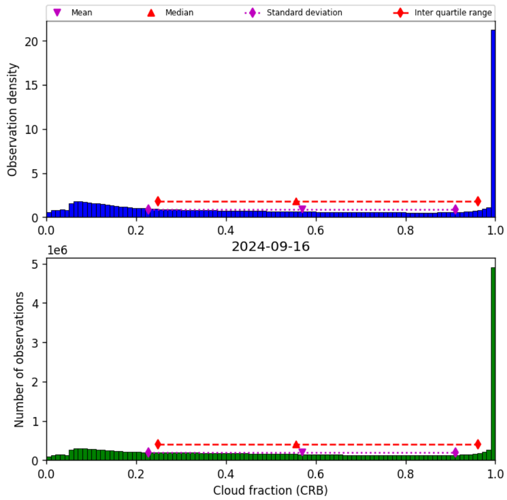
Figure 42: Histogram of “Cloud fraction (CRB)” for 2024-09-15 to 2024-09-17
