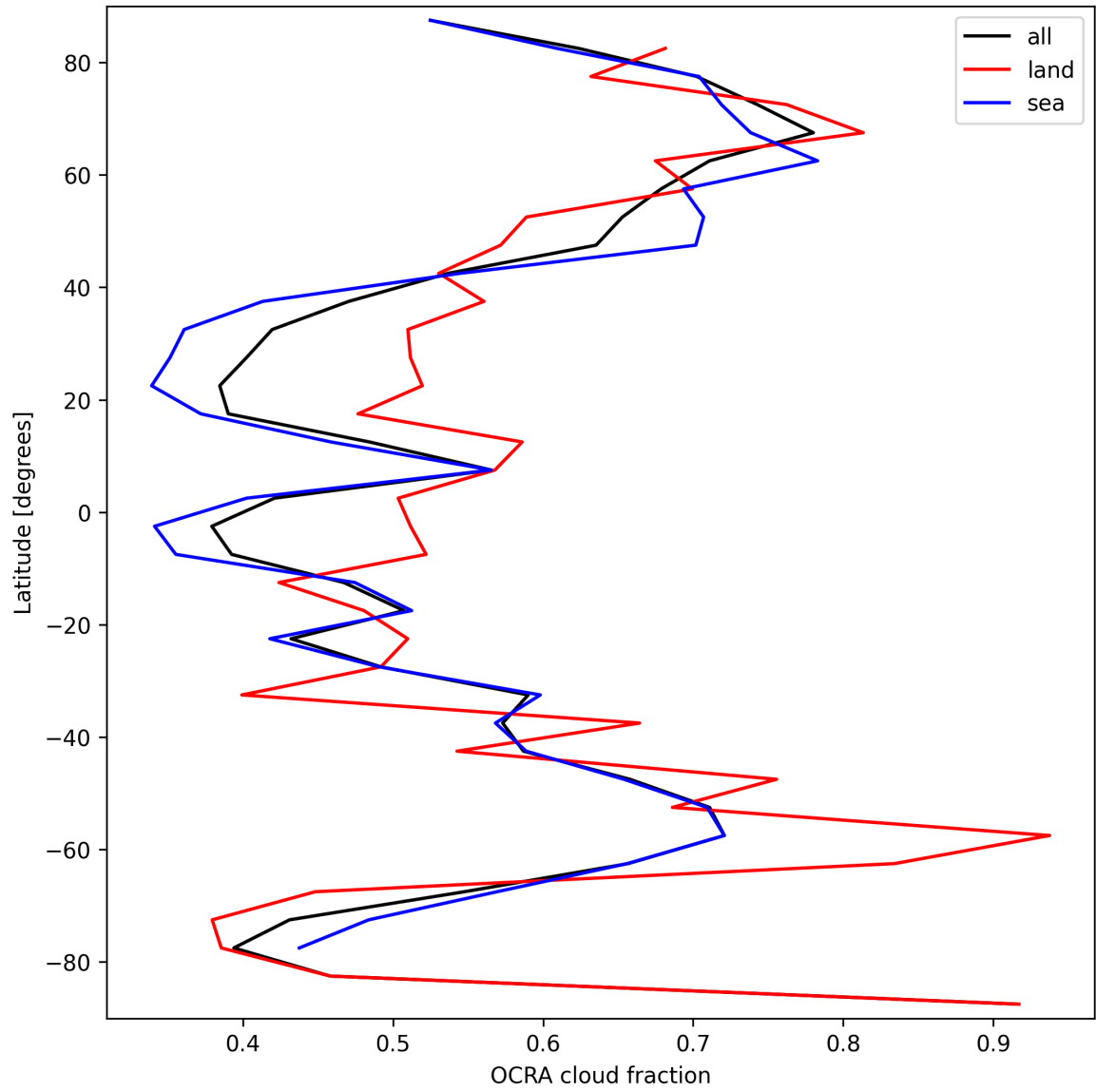
Figure 34: Zonal average of “OCRA cloud fraction” for 2024-09-15 to 2024-09-17.
