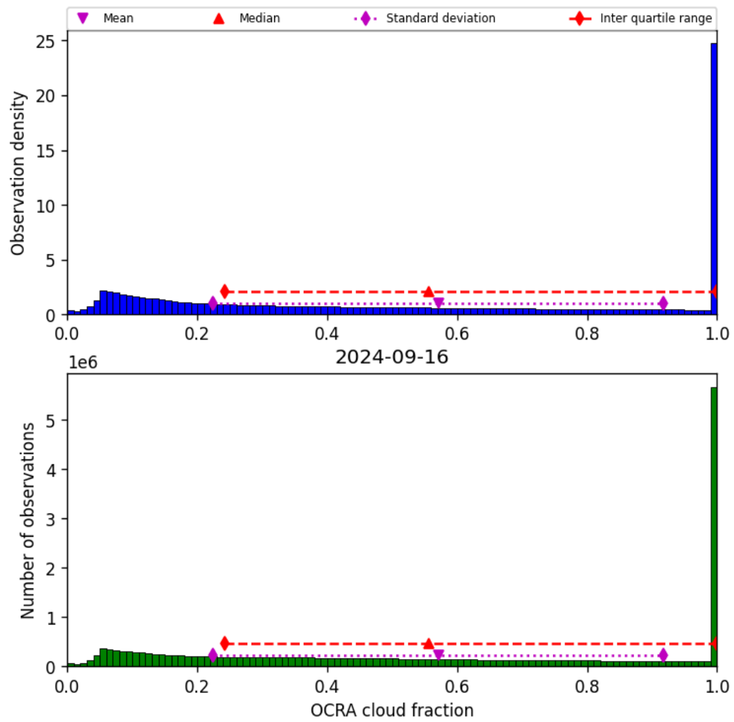
Figure 50: Histogram of “OCRA cloud fraction” for 2024-09-15 to 2024-09-17
