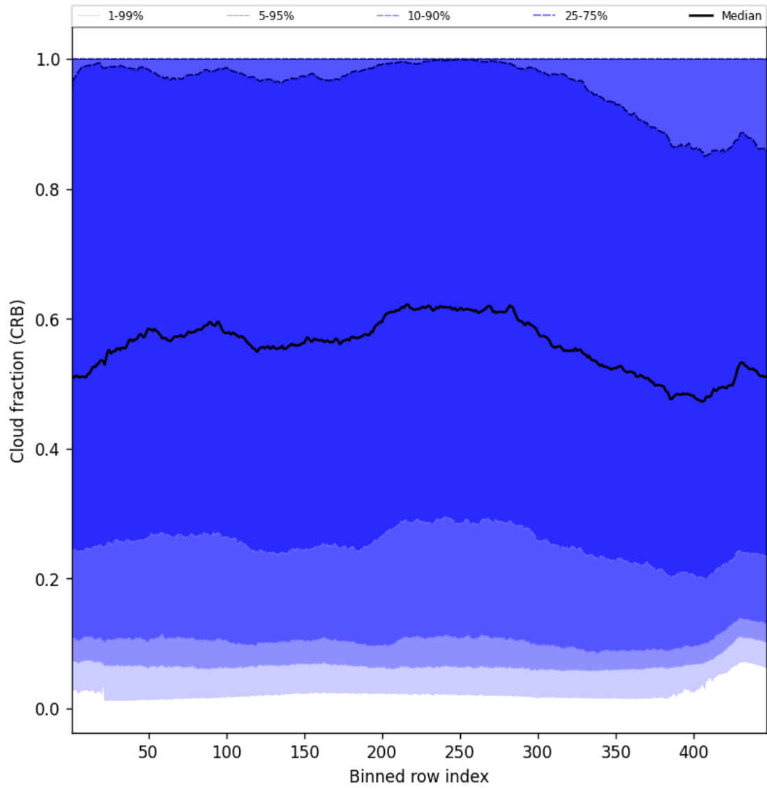
Figure 58: Along track statistics of “Cloud fraction (CRB)” for 2024-09-15 to 2024-09-17
