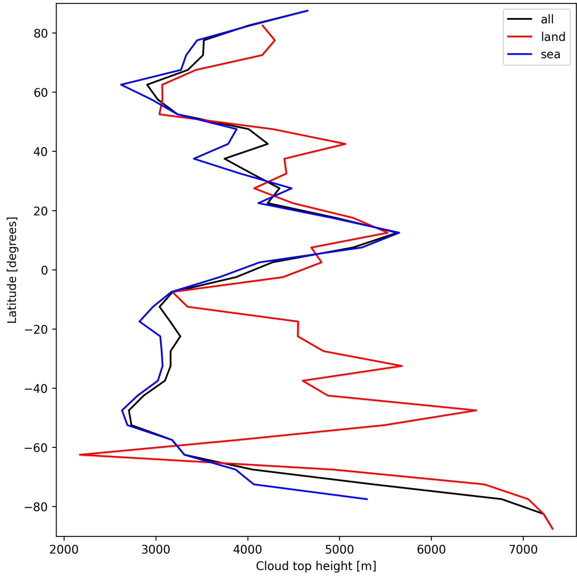
Figure 24: Zonal average of “Cloud top height” for 2024-09-15 to 2024-09-17.
