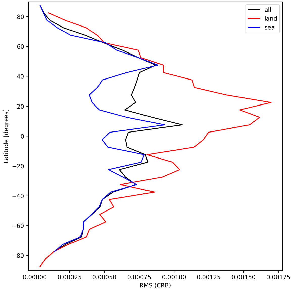
Figure 32: Zonal average of “RMS (CRB)” for 2024-09-15 to 2024-09-17.
