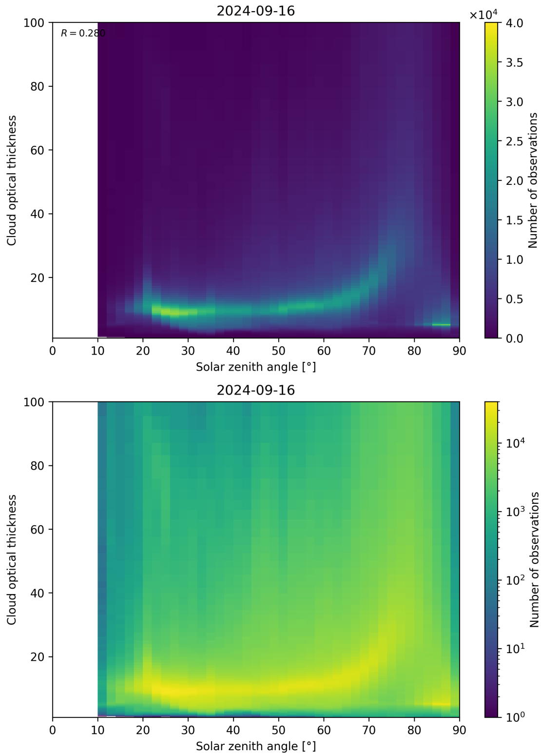
Figure 103: Scatter density plot of “Solar zenith angle” against “Cloud optical thickness” for 2024-09-15 to 2024-09-17.
