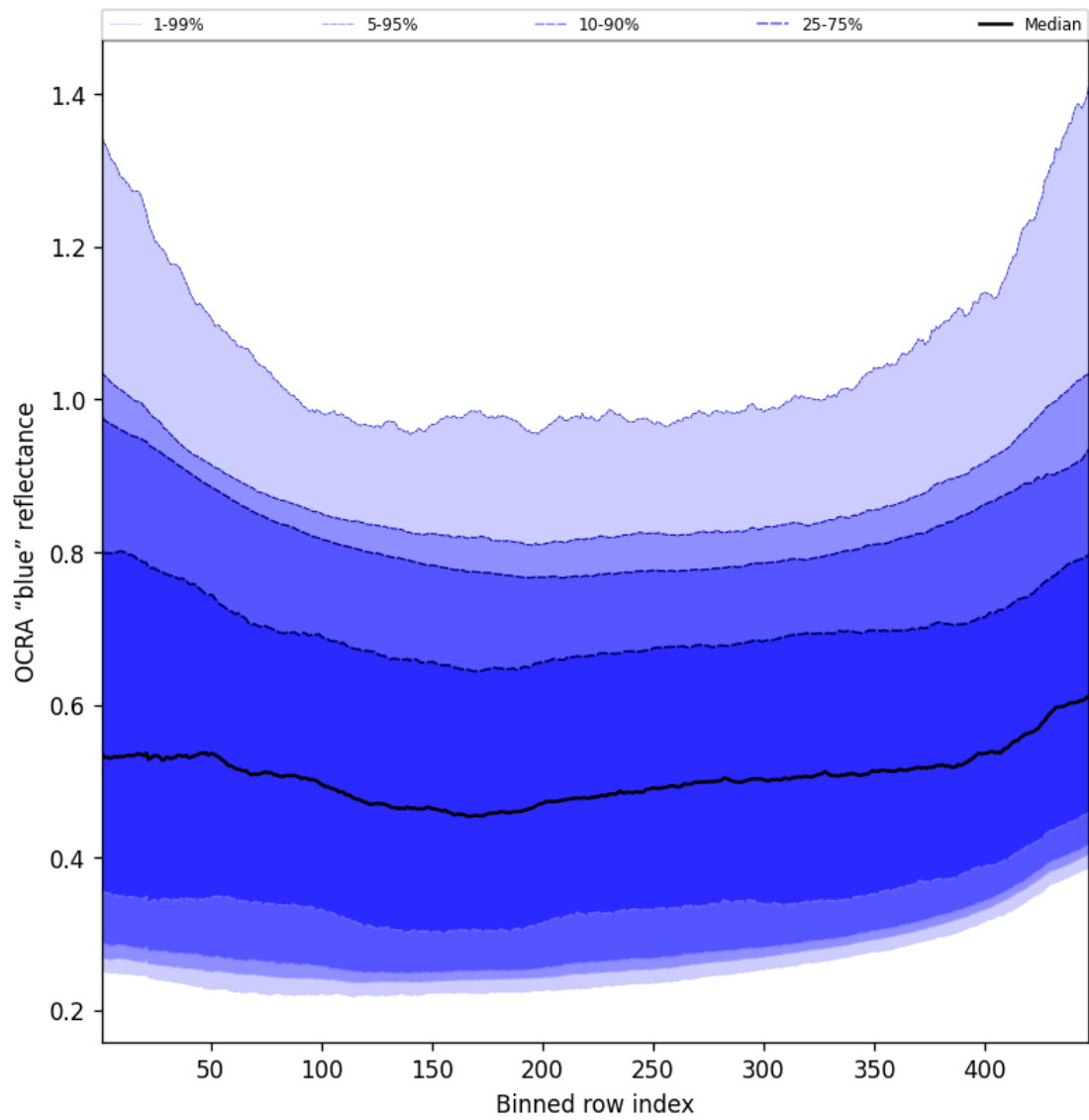
Figure 67: Along track statistics of “OCRA “blue” reflectance” for 2024-09-15 to 2024-09-17
