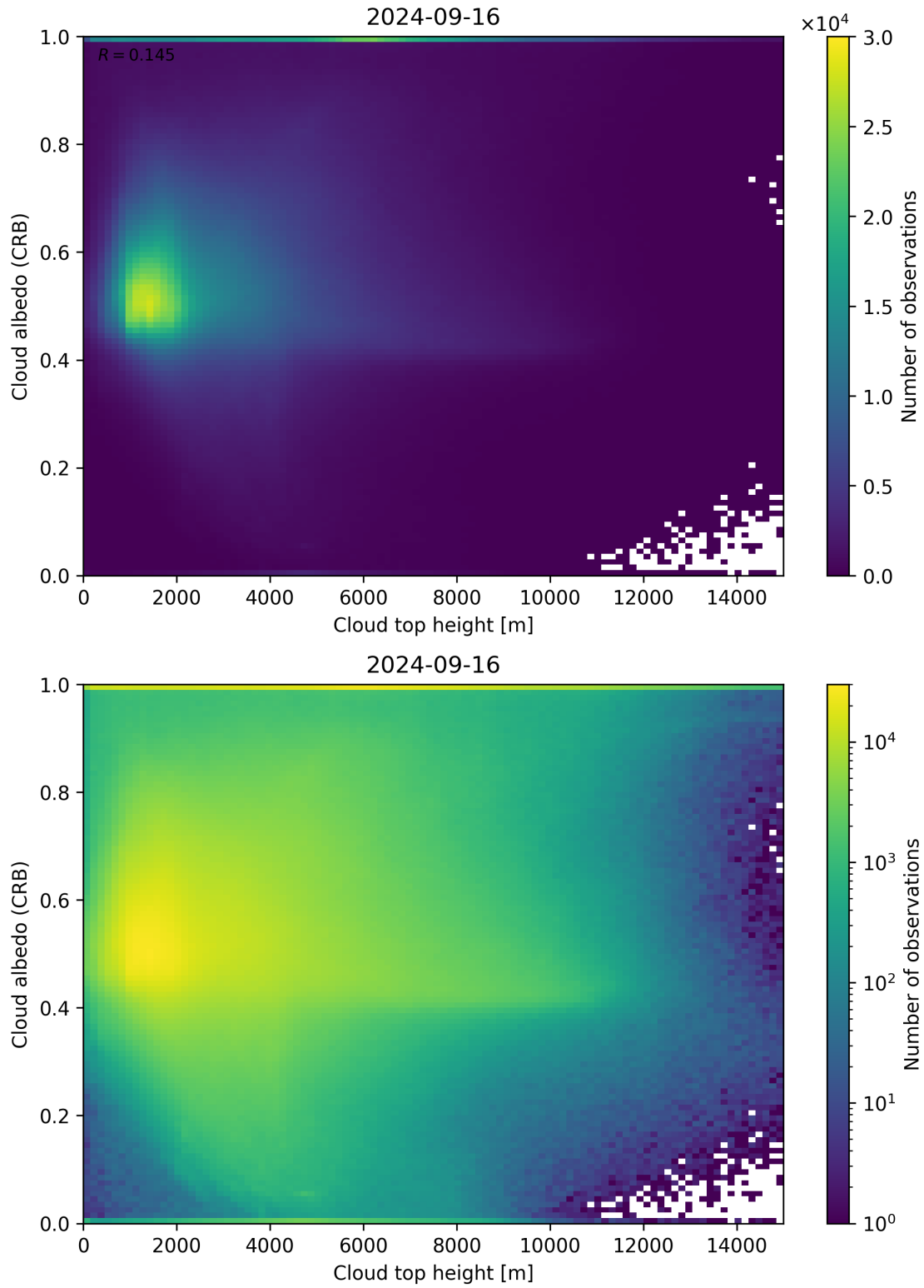
Figure 86: Scatter density plot of “Cloud top height” against “Cloud albedo (CRB)” for 2024-09-15 to 2024-09-17.
