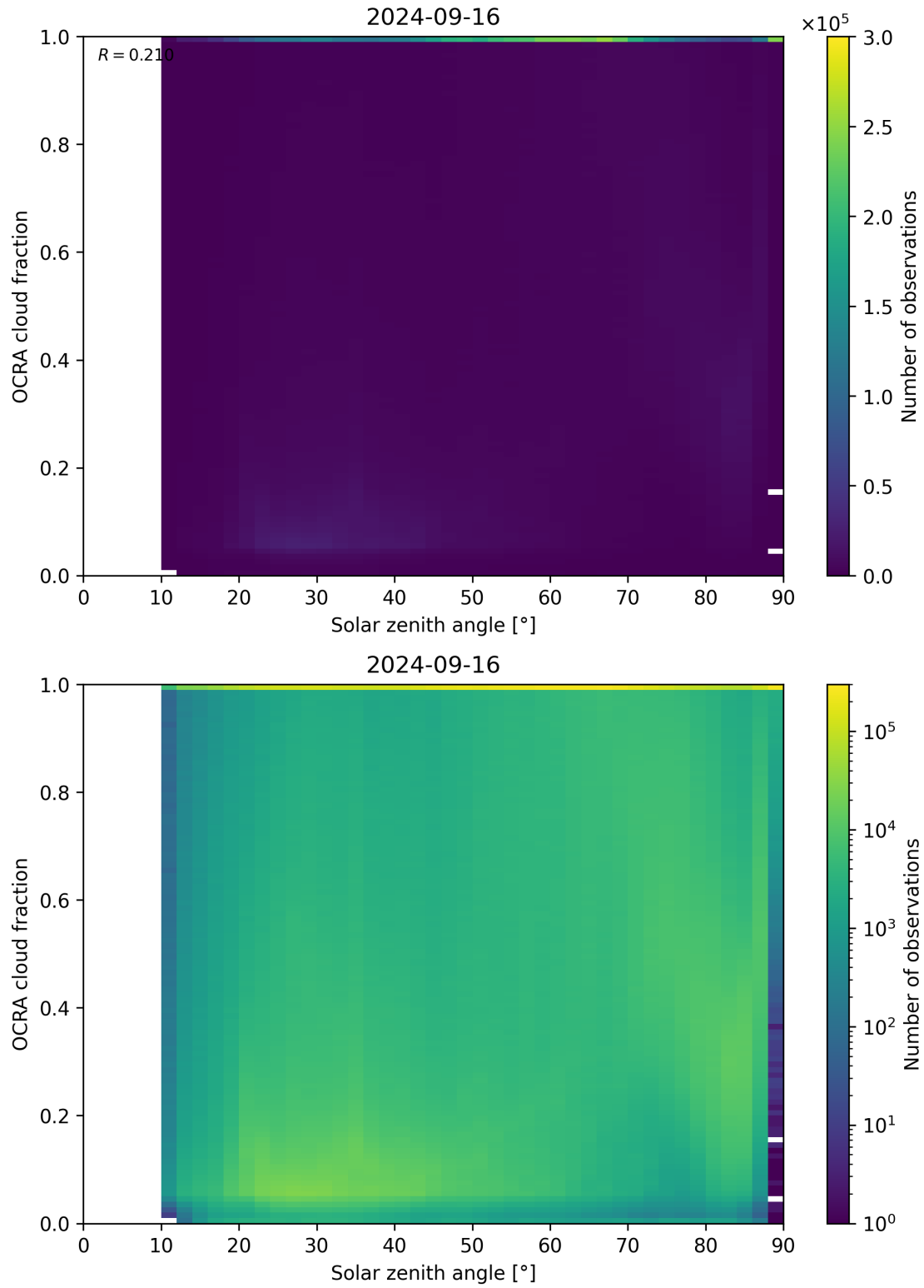
Figure 100: Scatter density plot of “Solar zenith angle” against “OCRA cloud fraction” for 2024-09-15 to 2024-09-17.
