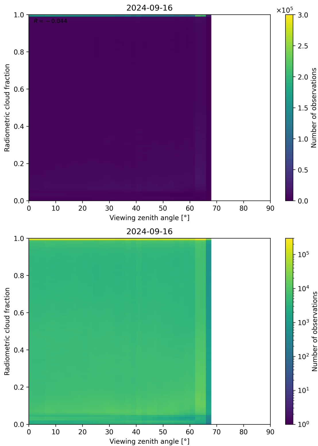
Figure 107: Scatter density plot of “Viewing zenith angle” against “Radiometric cloud fraction” for 2024-09-15 to 2024-09-17.
