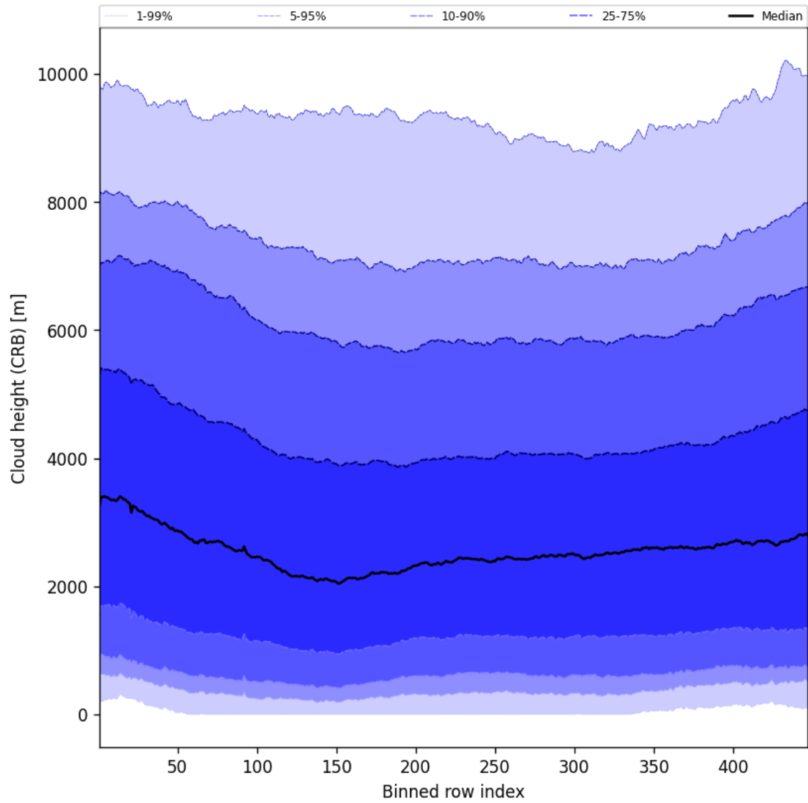
Figure 59: Along track statistics of “Cloud height (CRB)” for 2024-09-15 to 2024-09-17
