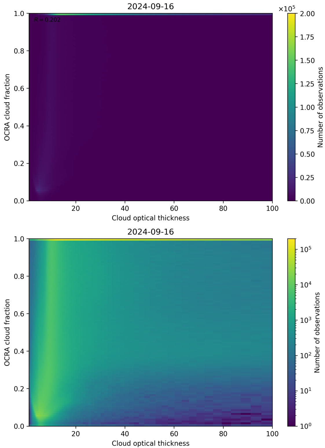
Figure 83: Scatter density plot of “Cloud optical thickness” against “OCRA cloud fraction” for 2024-09-15 to 2024-09-17.
