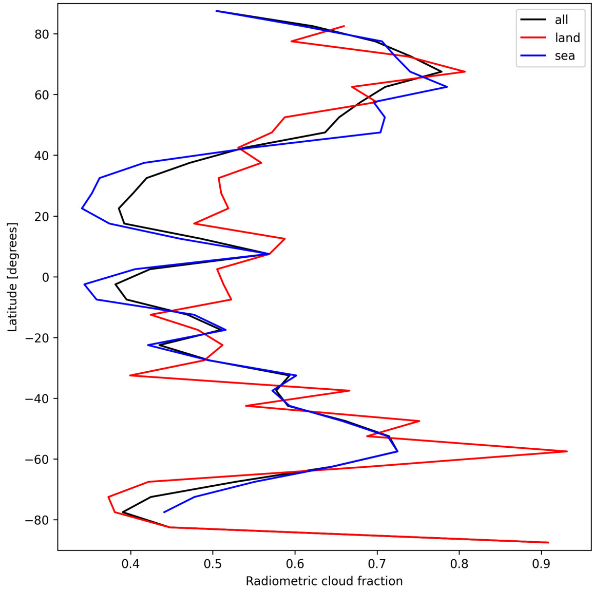
Figure 23: Zonal average of “Radiometric cloud fraction” for 2024-09-15 to 2024-09-17.
