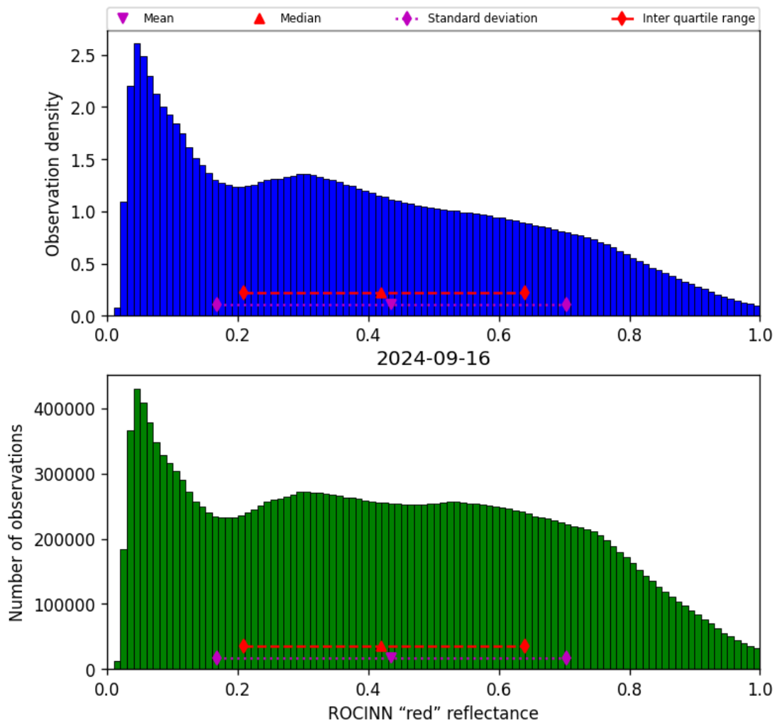
Figure 53: Histogram of “ROCINN “red” reflectance” for 2024-09-15 to 2024-09-17
