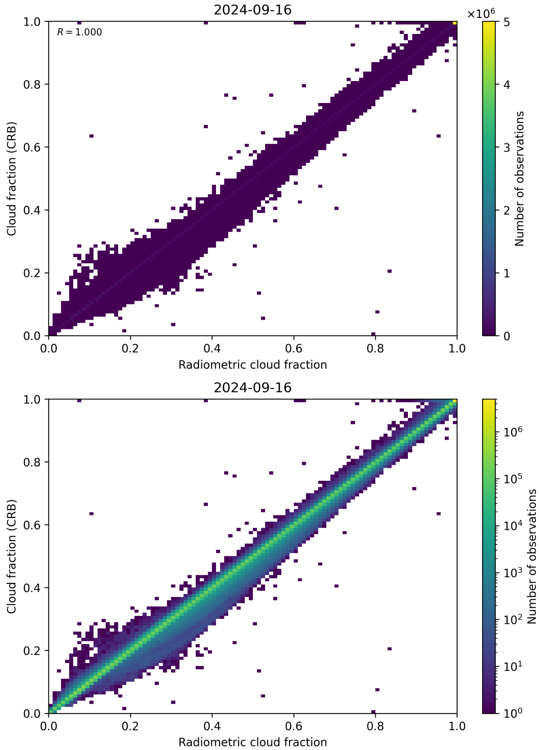
Figure 73: Scatter density plot of “Radiometric cloud fraction” against “Cloud fraction (CRB)” for 2024-09-15 to 2024-09-17.
