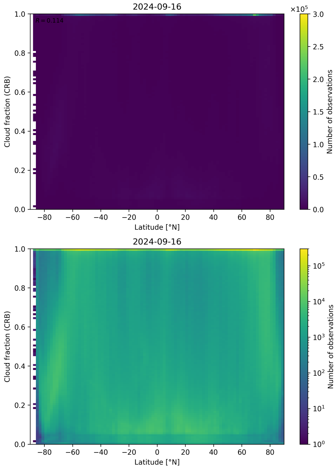
Figure 94: Scatter density plot of “Latitude” against “Cloud fraction (CRB)” for 2024-09-15 to 2024-09-17.
