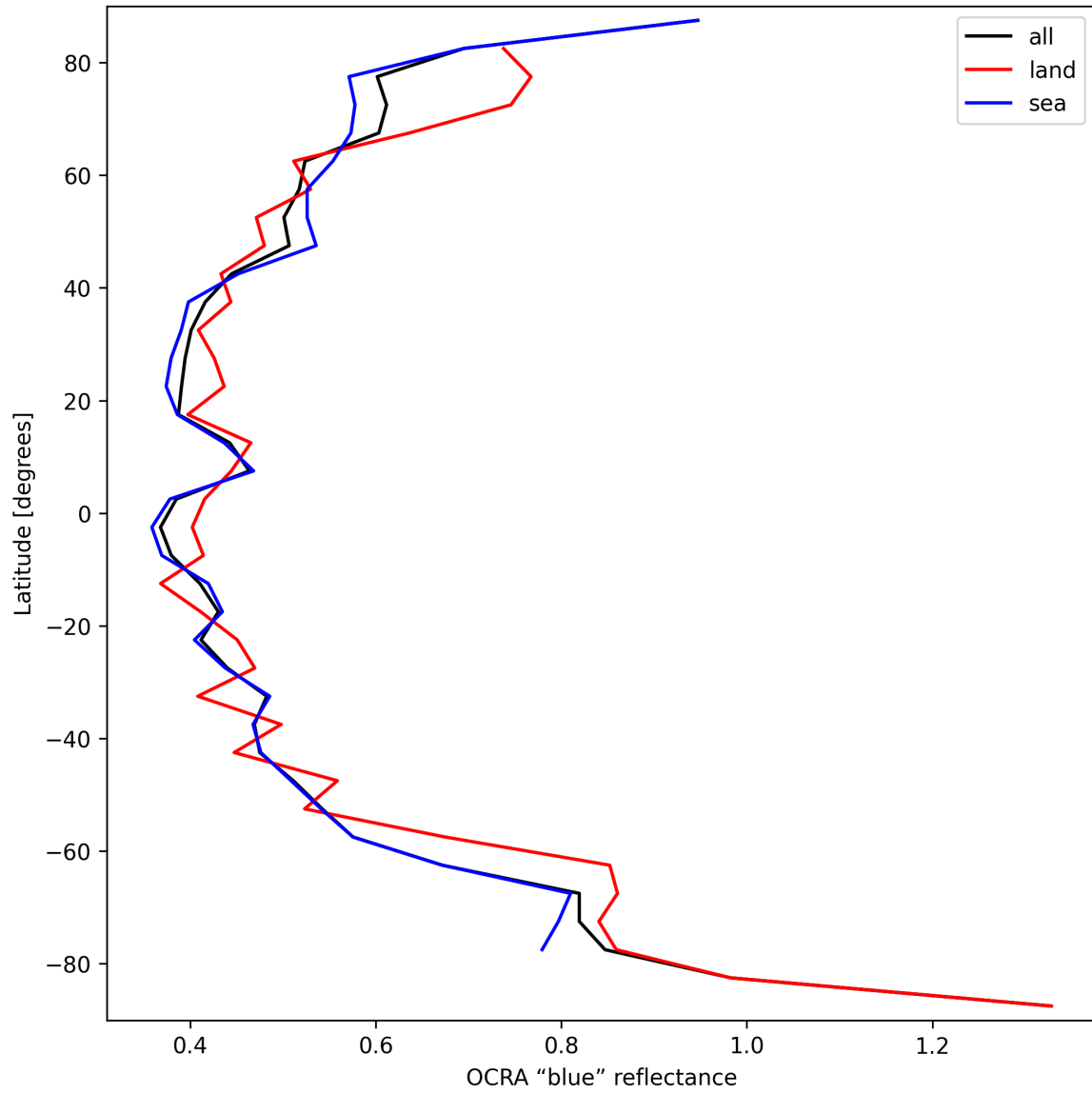
Figure 35: Zonal average of “OCRA “blue” reflectance” for 2024-09-15 to 2024-09-17.
