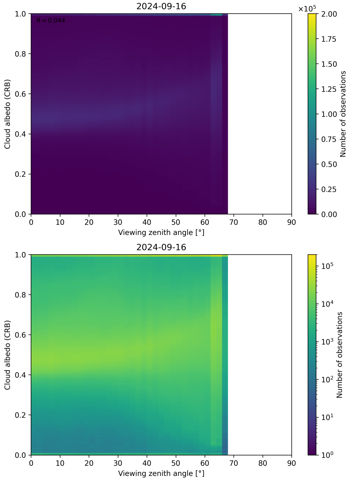
Figure 106: Scatter density plot of “Viewing zenith angle” against “Cloud albedo (CRB)” for 2024-09-15 to 2024-09-17.
