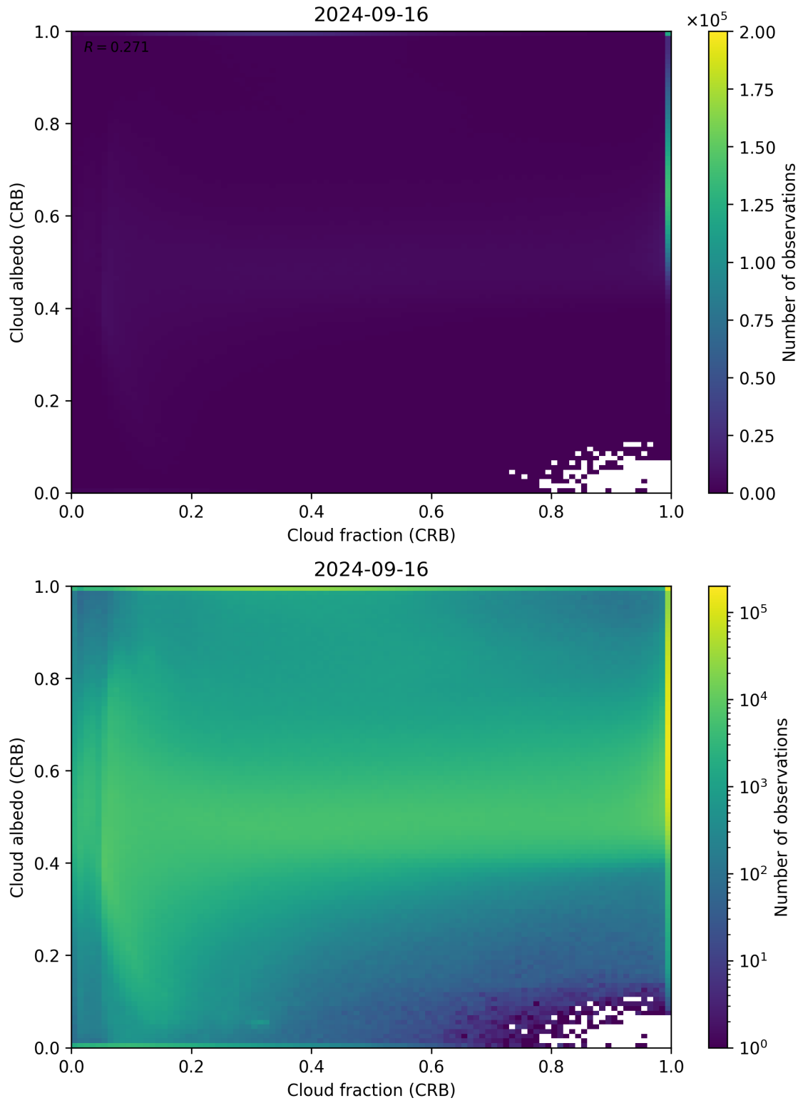
Figure 77: Scatter density plot of “Cloud fraction (CRB)” against “Cloud albedo (CRB)” for 2024-09-15 to 2024-09-17.
