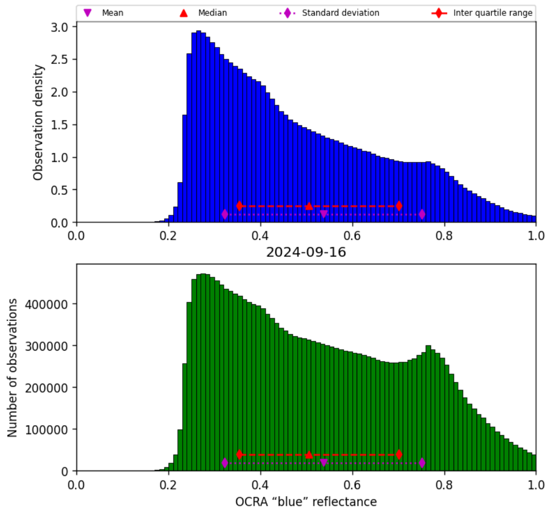
Figure 51: Histogram of “OCRA “blue” reflectance” for 2024-09-15 to 2024-09-17
