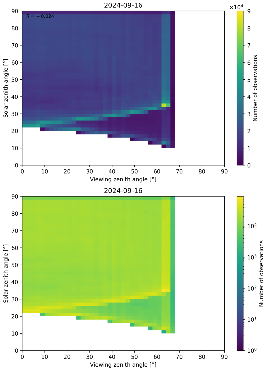
Figure 114: Scatter density plot of “Viewing zenith angle” against “Solar zenith angle” for 2024-09-15 to 2024-09-17.
