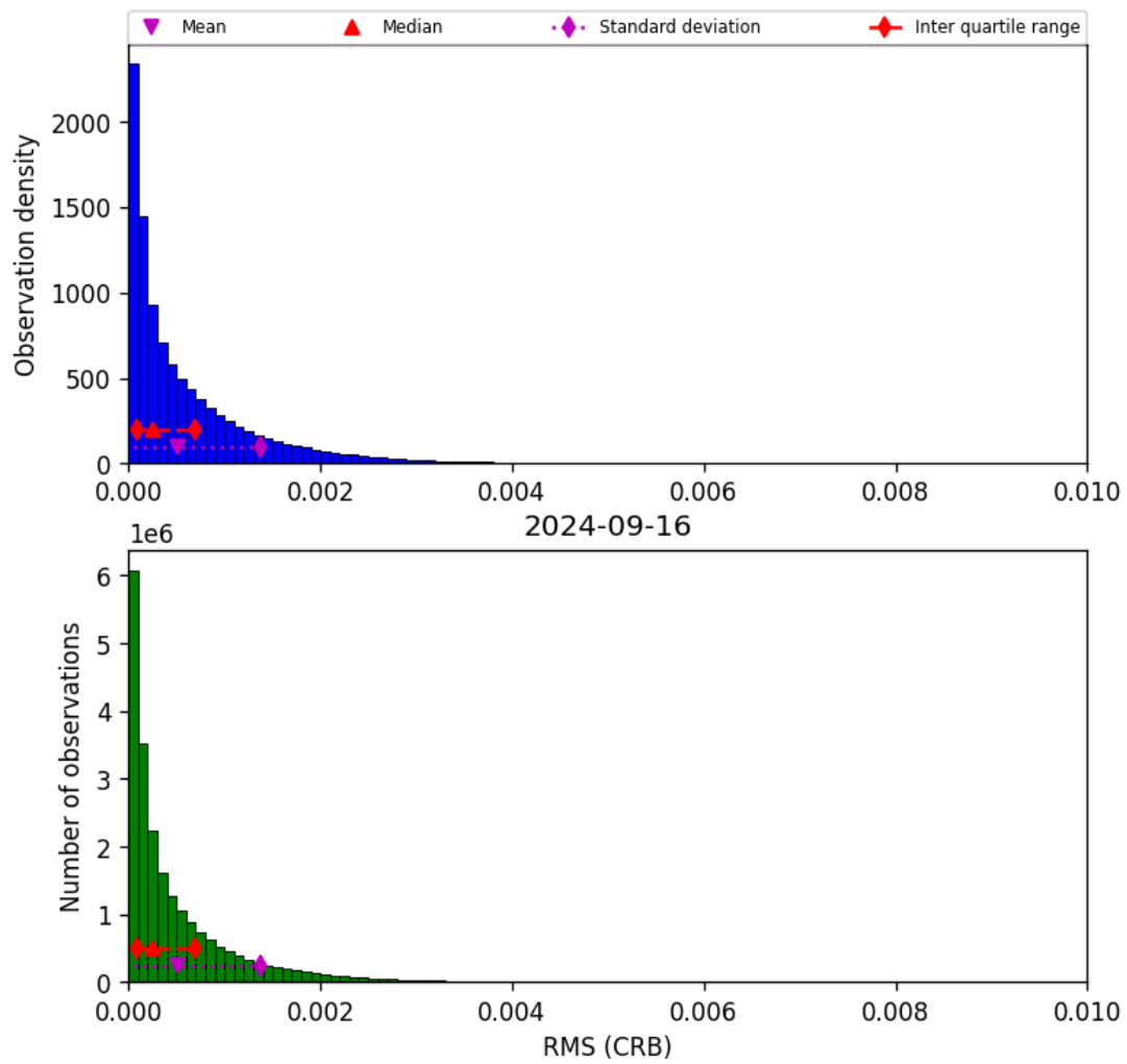
Figure 48: Histogram of “RMS (CRB)” for 2024-09-15 to 2024-09-17
