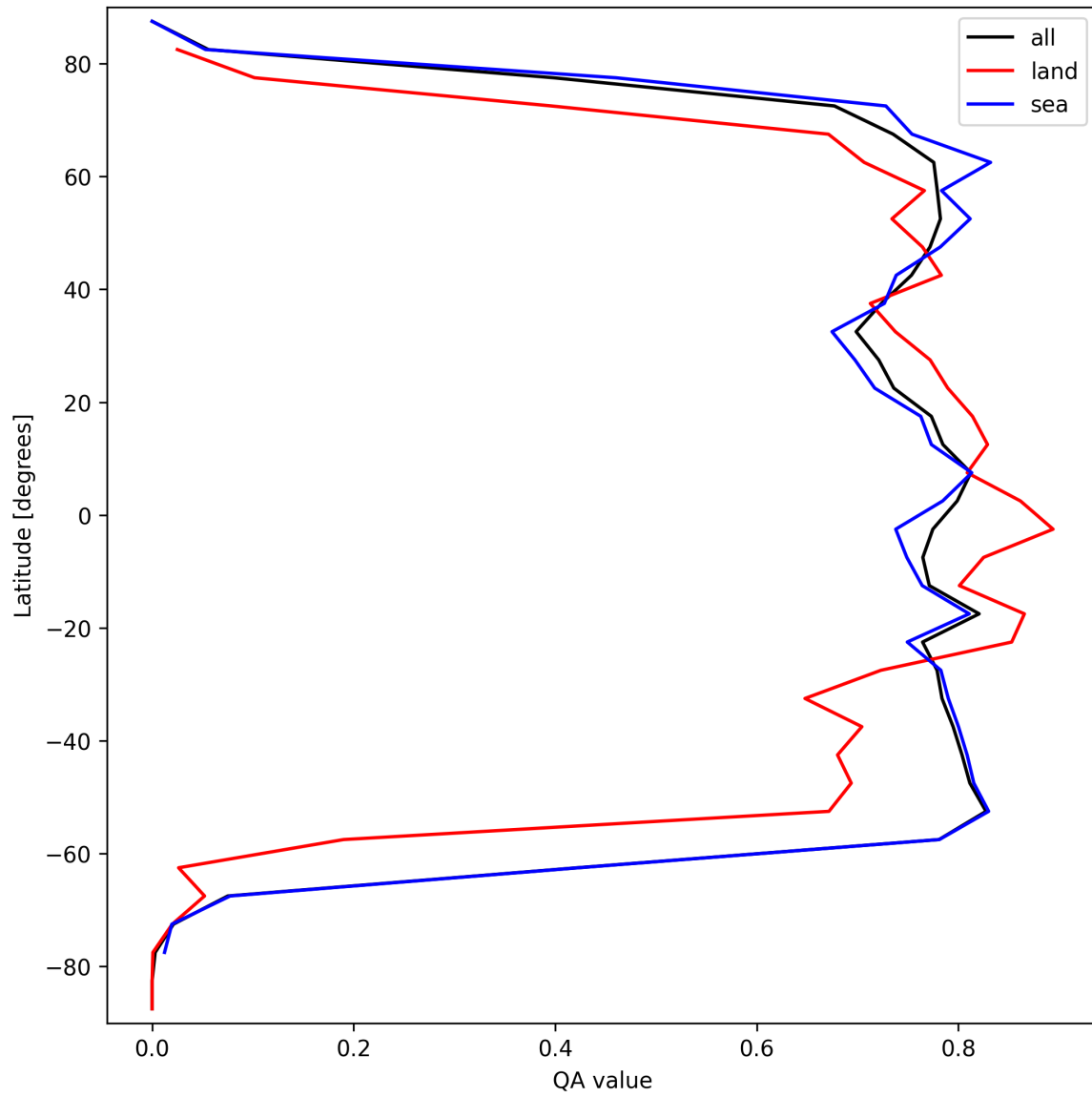
Figure 22: Zonal average of “QA value” for 2024-09-15 to 2024-09-17.
