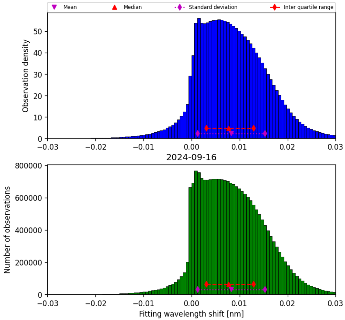
Figure 49: Histogram of “Fitting wavelength shift” for 2024-09-15 to 2024-09-17
