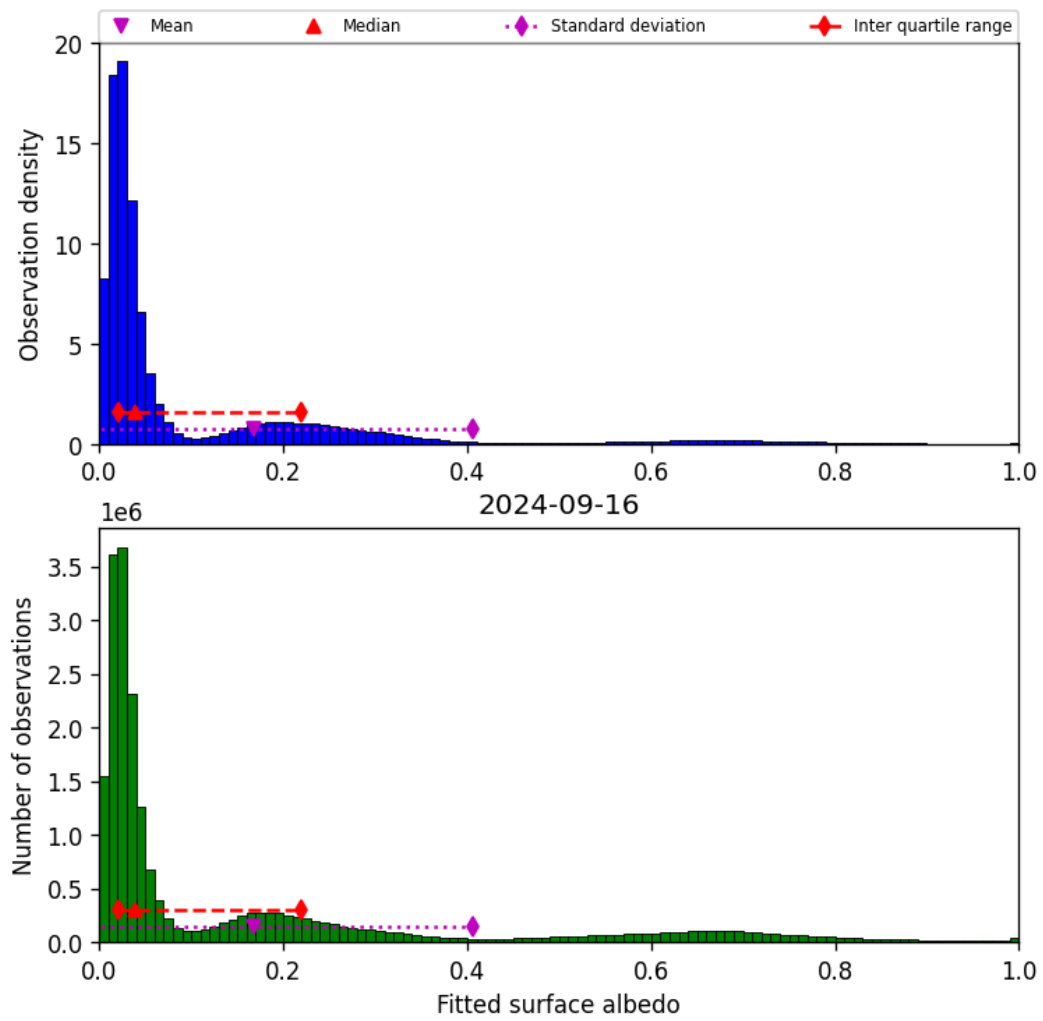
Figure 45: Histogram of “Fitted surface albedo” for 2024-09-15 to 2024-09-17
