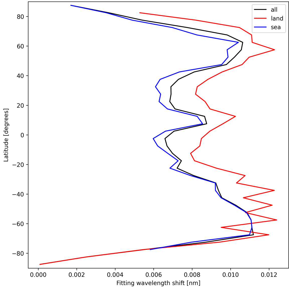
Figure 33: Zonal average of “Fitting wavelength shift” for 2024-09-15 to 2024-09-17.
