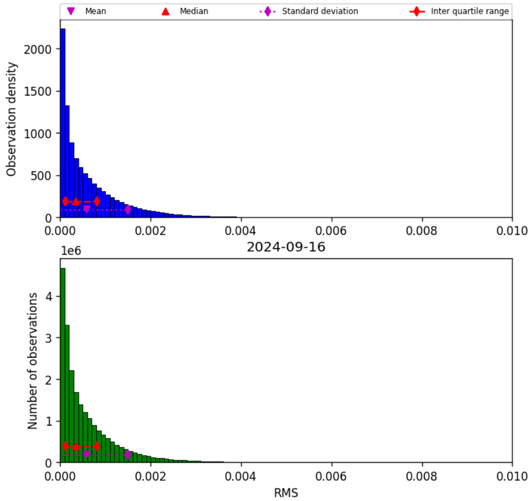
Figure 47: Histogram of “RMS” for 2024-09-15 to 2024-09-17
