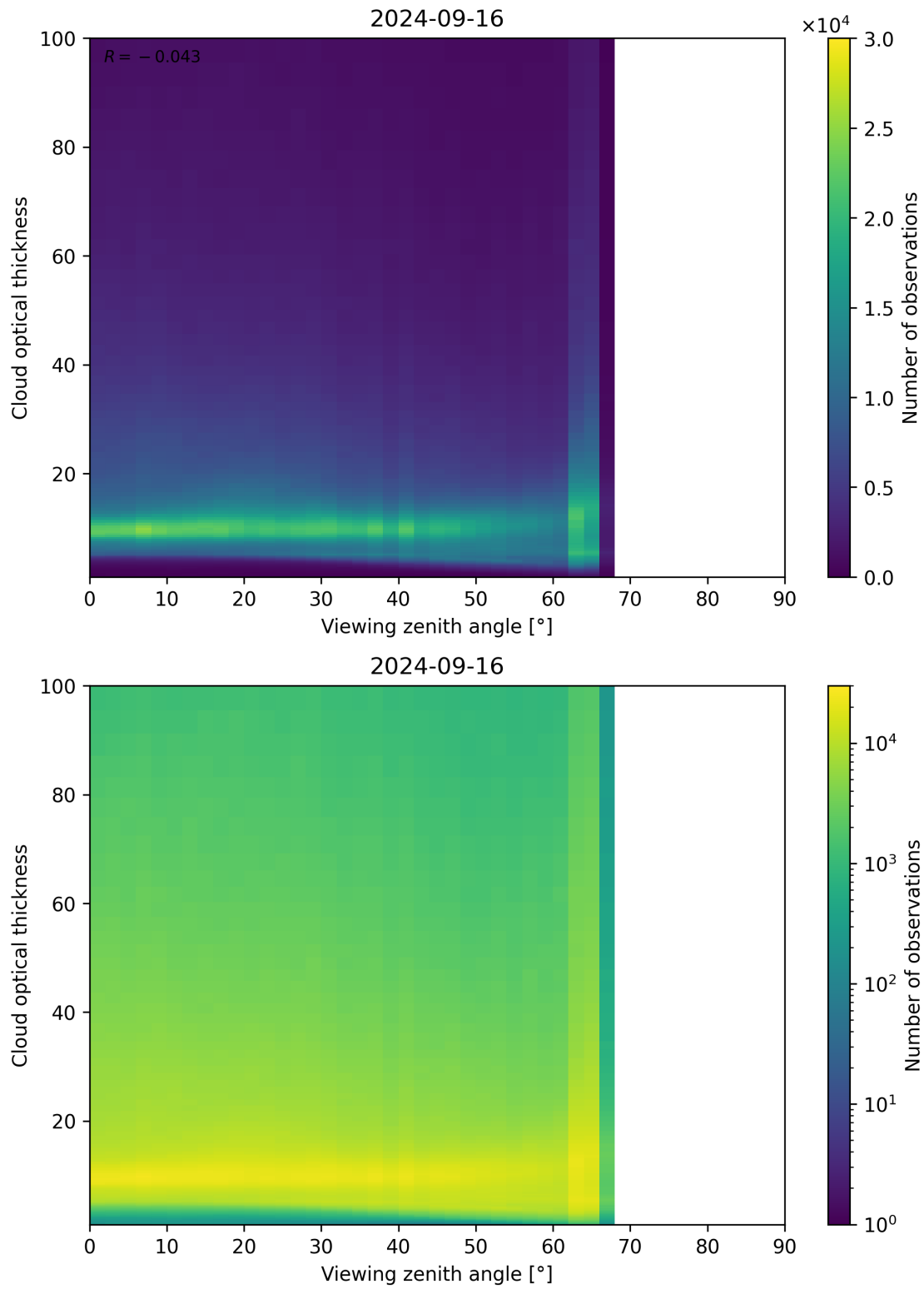
Figure 111: Scatter density plot of “Viewing zenith angle” against “Cloud optical thickness” for 2024-09-15 to 2024-09-17.
