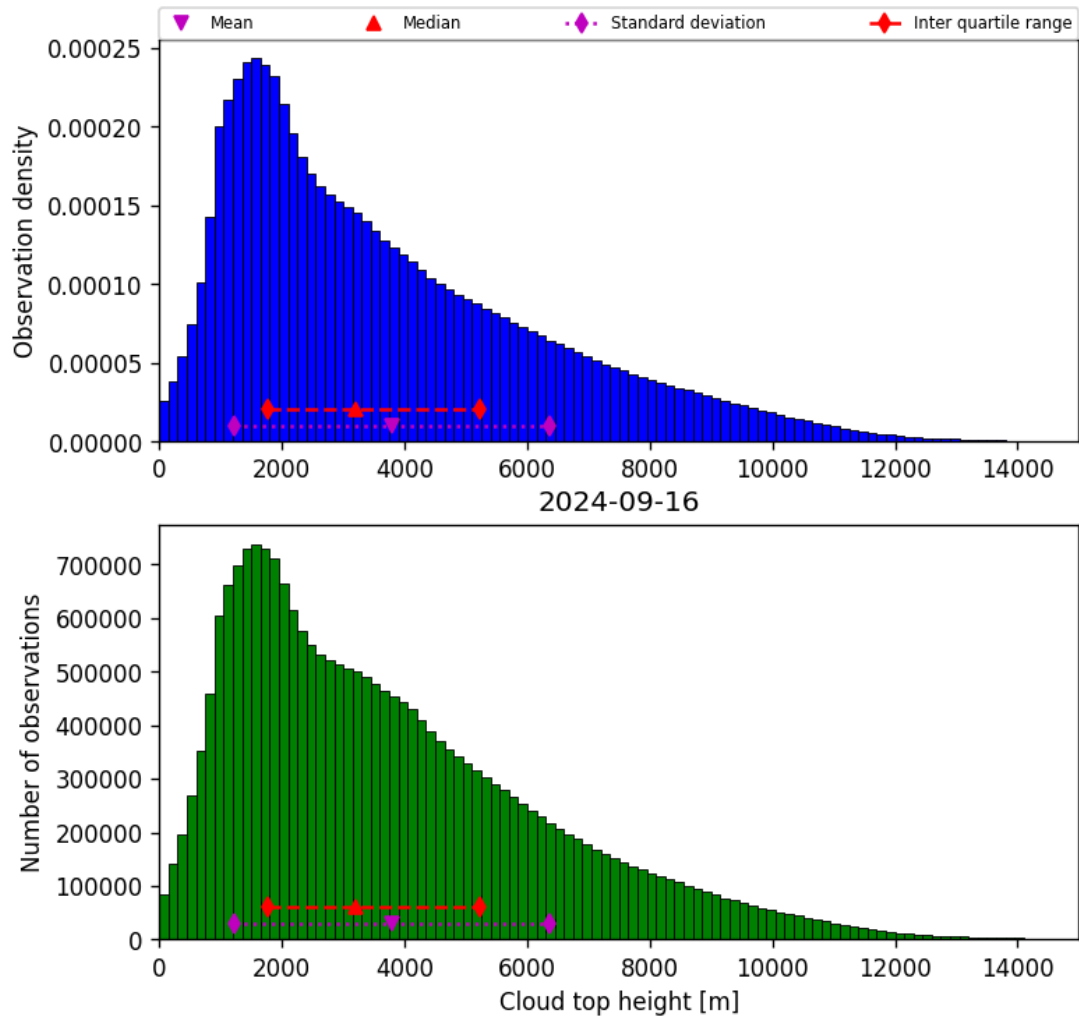
Figure 40: Histogram of “Cloud top height” for 2024-09-15 to 2024-09-17
