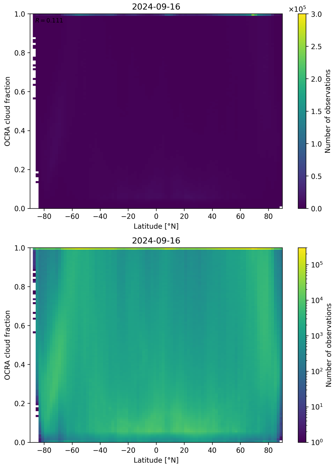
Figure 93: Scatter density plot of “Latitude” against “OCRA cloud fraction” for 2024-09-15 to 2024-09-17.
