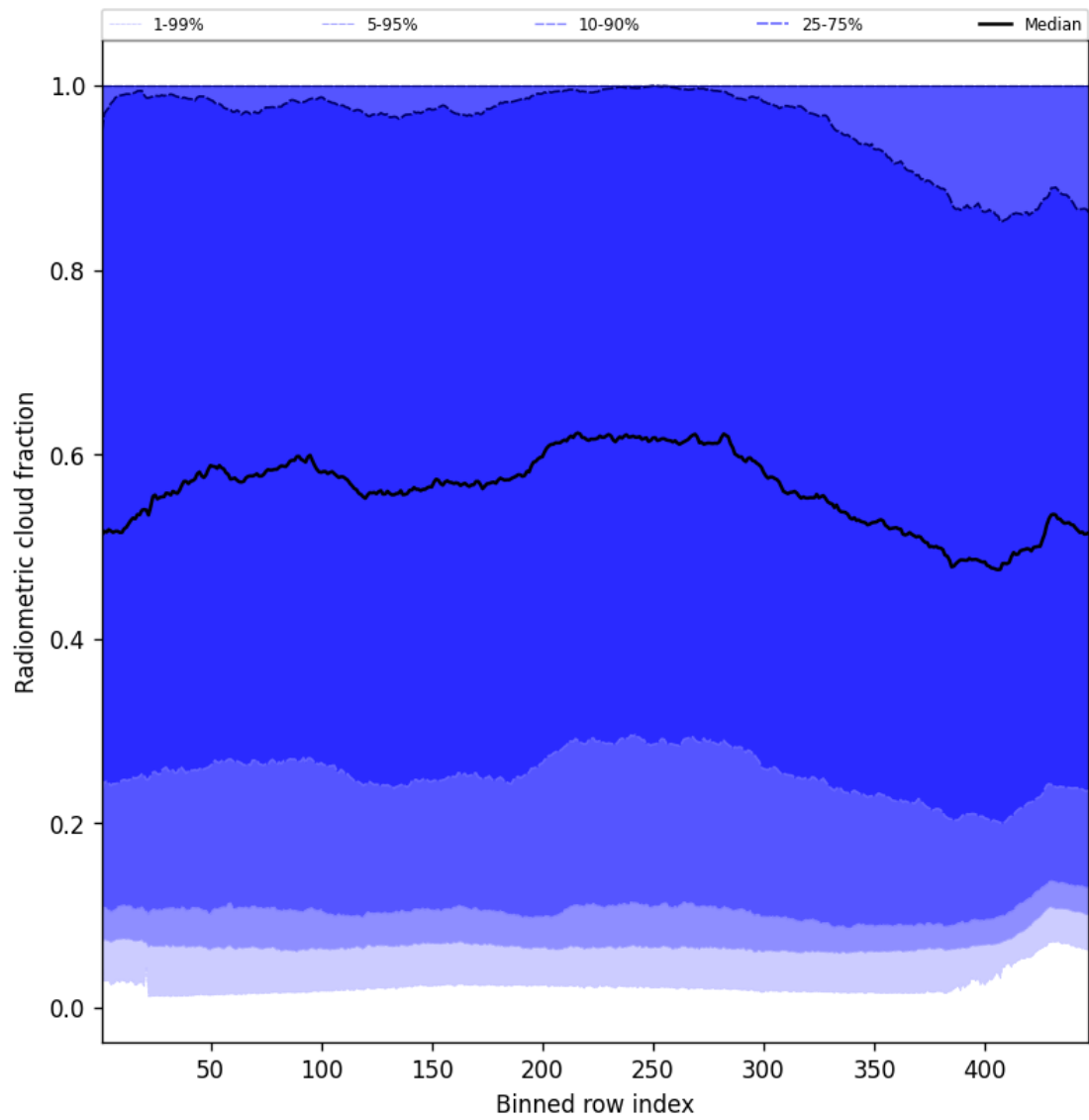
Figure 55: Along track statistics of “Radiometric cloud fraction” for 2024-09-15 to 2024-09-17
