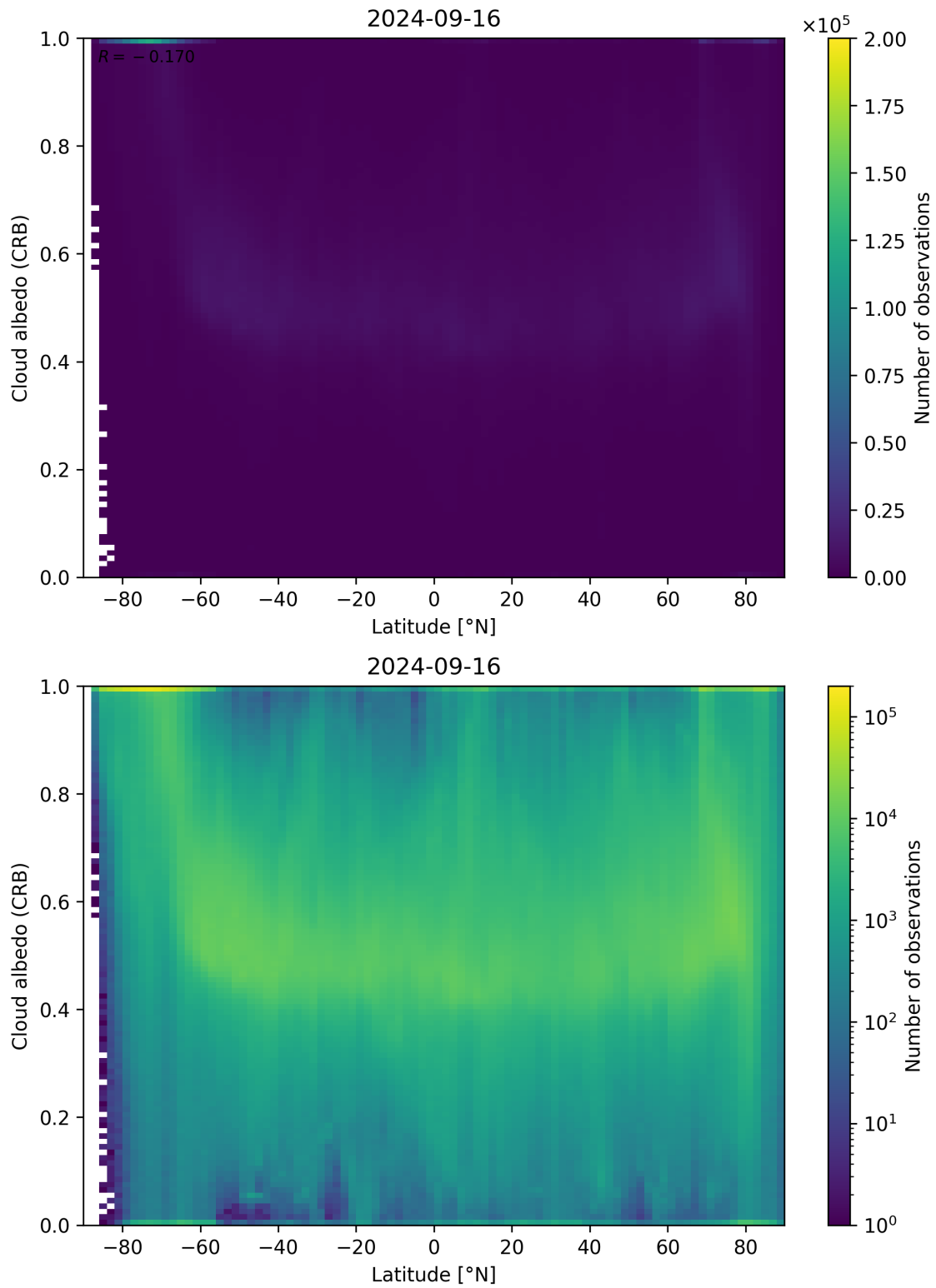
Figure 91: Scatter density plot of “Latitude” against “Cloud albedo (CRB)” for 2024-09-15 to 2024-09-17.
