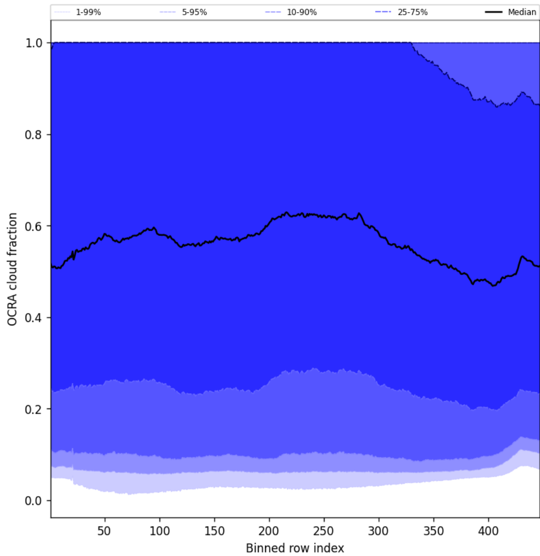
Figure 66: Along track statistics of “OCRA cloud fraction” for 2024-09-15 to 2024-09-17
