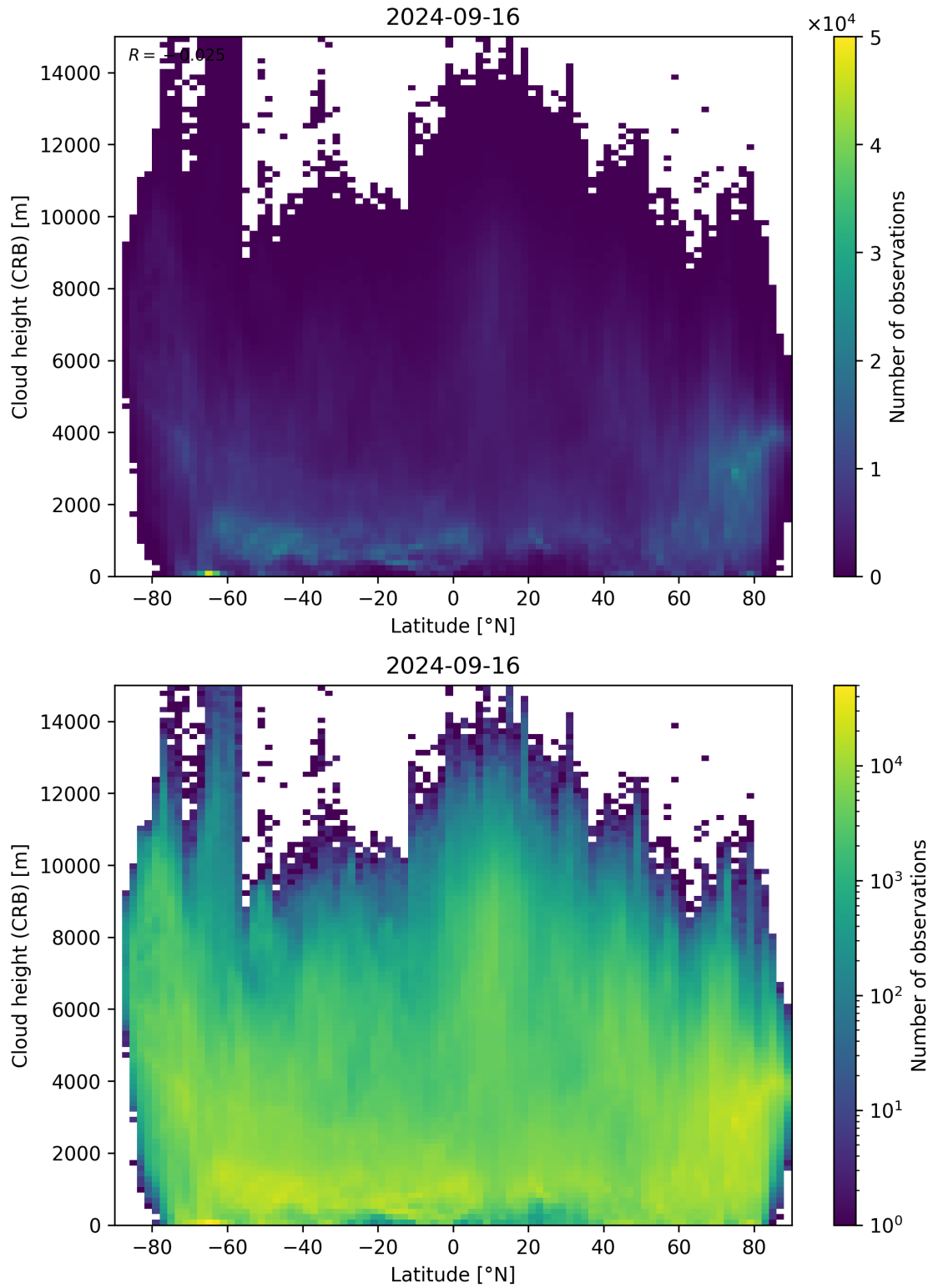
Figure 95: Scatter density plot of “Latitude” against “Cloud height (CRB)” for 2024-09-15 to 2024-09-17.
