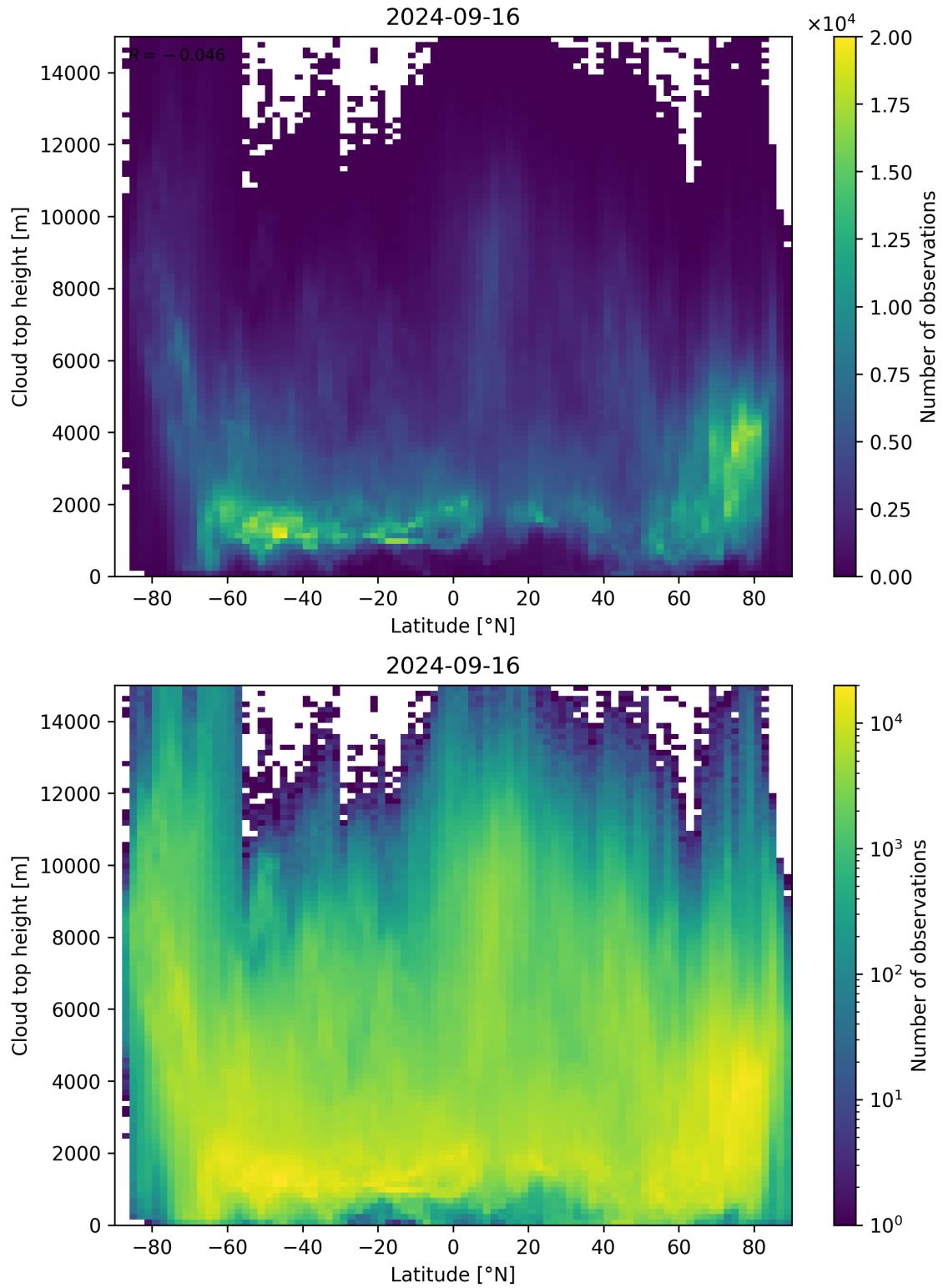
Figure 97: Scatter density plot of “Latitude” against “Cloud top height” for 2024-09-15 to 2024-09-17.
