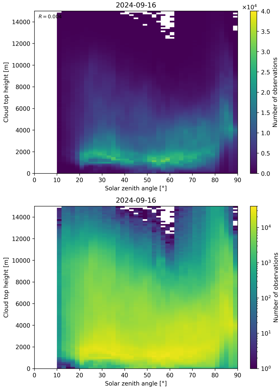
Figure 104: Scatter density plot of “Solar zenith angle” against “Cloud top height” for 2024-09-15 to 2024-09-17.
