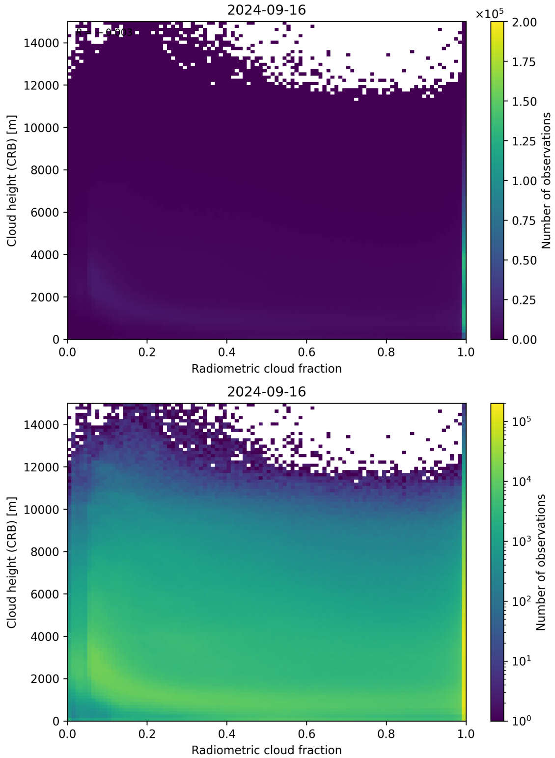
Figure 74: Scatter density plot of “Radiometric cloud fraction” against “Cloud height (CRB)” for 2024-09-15 to 2024-09-17.
