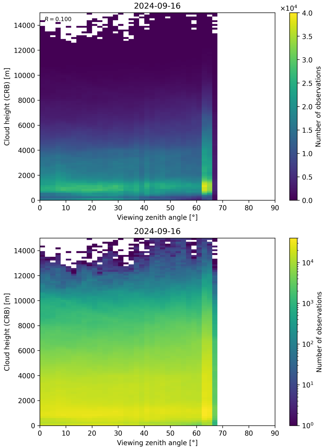
Figure 110: Scatter density plot of “Viewing zenith angle” against “Cloud height (CRB)” for 2024-09-15 to 2024-09-17.
