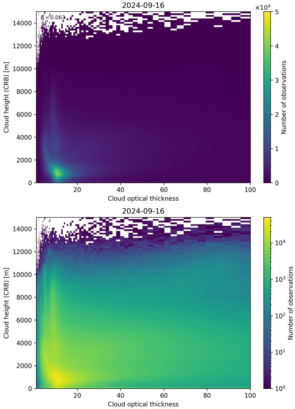
Figure 85: Scatter density plot of “Cloud optical thickness” against “Cloud height (CRB)” for 2024-09-15 to 2024-09-17.
