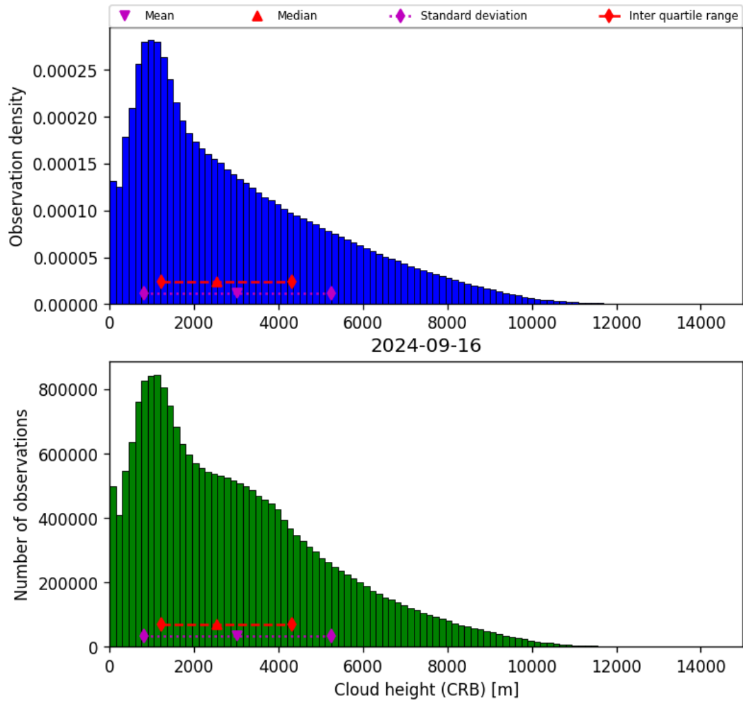
Figure 43: Histogram of “Cloud height (CRB)” for 2024-09-15 to 2024-09-17
