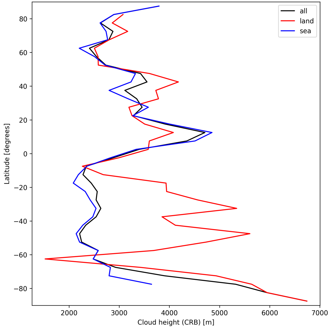
Figure 27: Zonal average of “Cloud height (CRB)” for 2024-09-15 to 2024-09-17.
