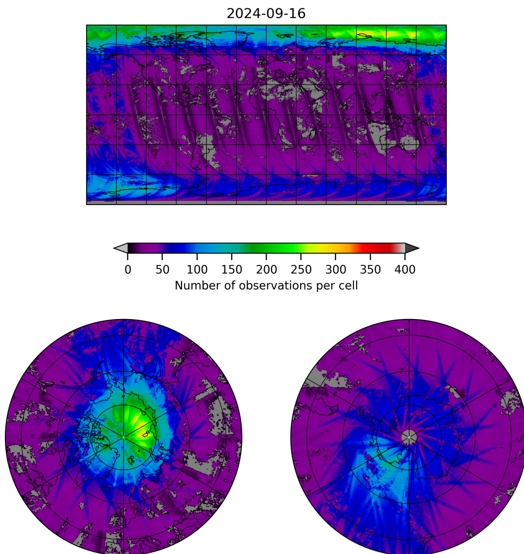
Figure 21: Map of the number of observations for 2024-09-15 to 2024-09-17
