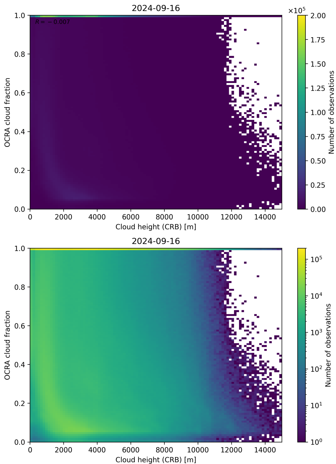
Figure 81: Scatter density plot of “Cloud height (CRB)” against “OCRA cloud fraction” for 2024-09-15 to 2024-09-17.
