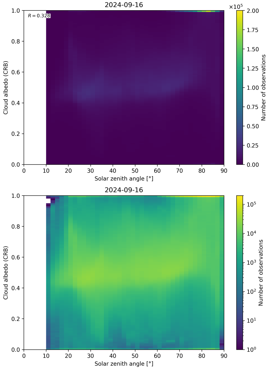
Figure 98: Scatter density plot of “Solar zenith angle” against “Cloud albedo (CRB)” for 2024-09-15 to 2024-09-17.
