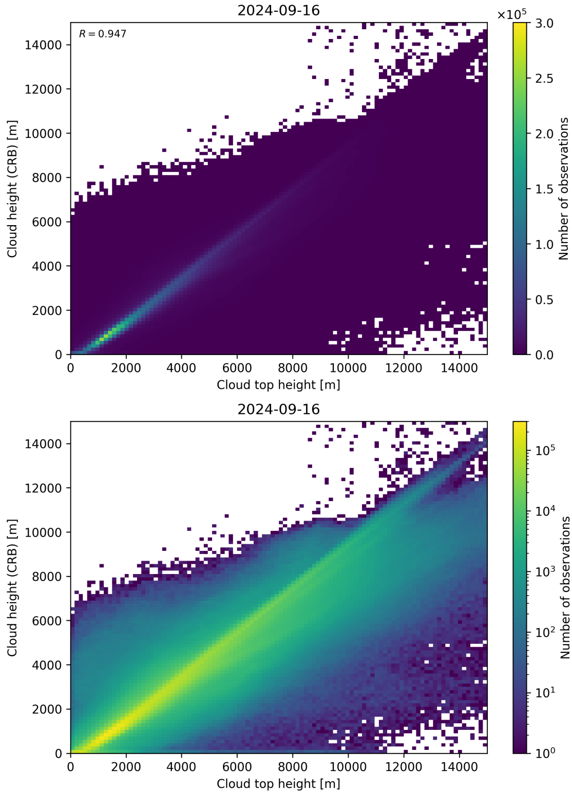
Figure 89: Scatter density plot of “Cloud top height” against “Cloud height (CRB)” for 2024-09-15 to 2024-09-17.
