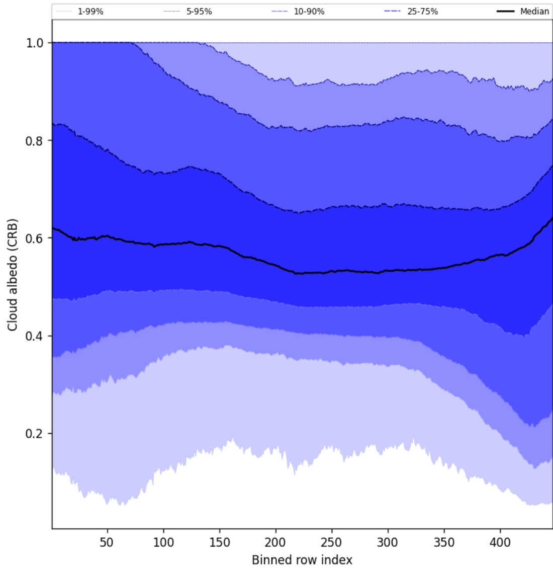
Figure 60: Along track statistics of “Cloud albedo (CRB)” for 2024-09-15 to 2024-09-17
