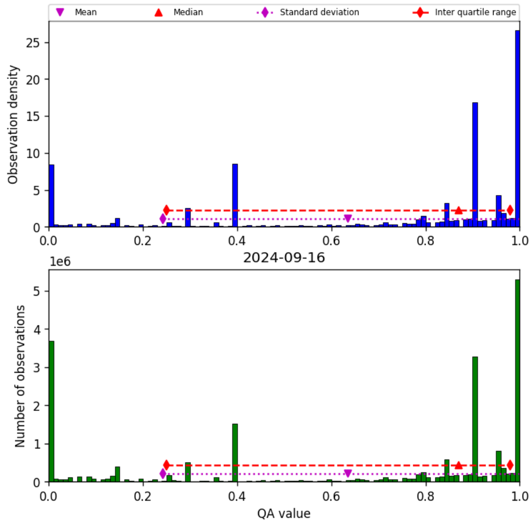
Figure 38: Histogram of “QA value” for 2024-09-15 to 2024-09-17
