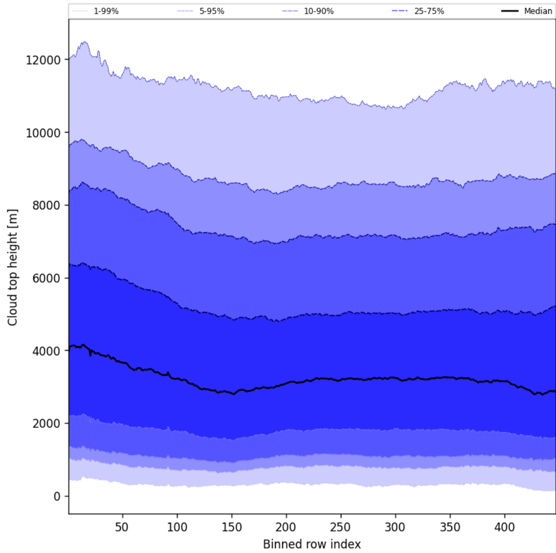
Figure 56: Along track statistics of “Cloud top height” for 2024-09-15 to 2024-09-17
