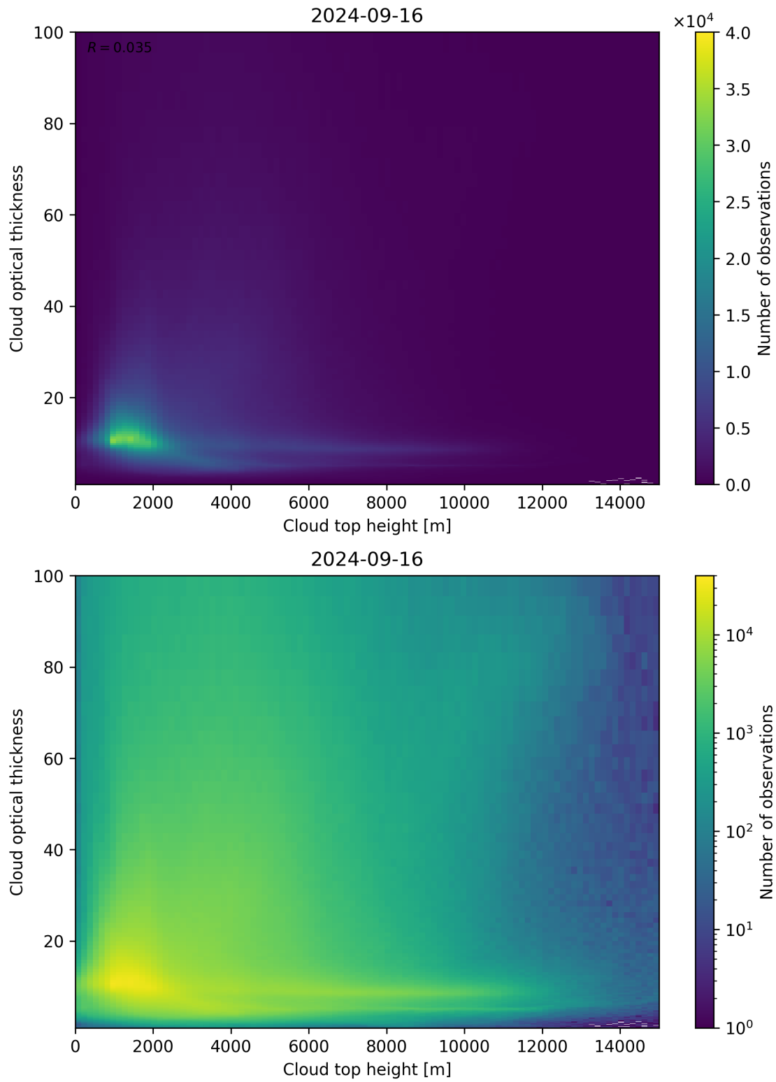
Figure 90: Scatter density plot of “Cloud top height” against “Cloud optical thickness” for 2024-09-15 to 2024-09-17.
