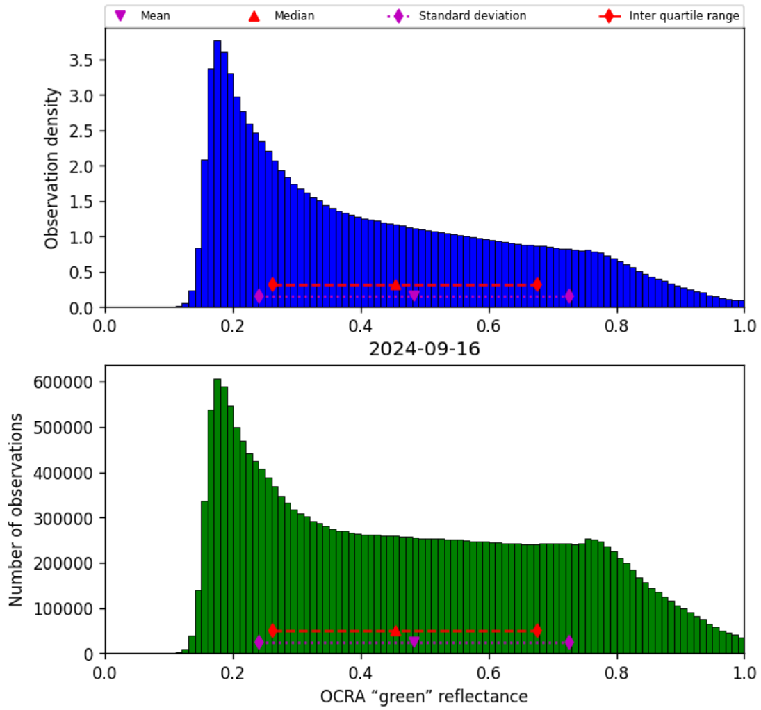
Figure 52: Histogram of “OCRA “green” reflectance” for 2024-09-15 to 2024-09-17
