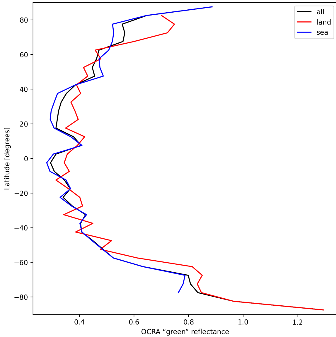
Figure 36: Zonal average of “OCRA “green” reflectance” for 2024-09-15 to 2024-09-17.
