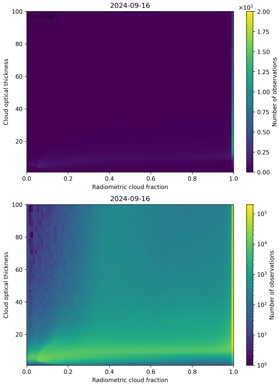
Figure 75: Scatter density plot of “Radiometric cloud fraction” against “Cloud optical thickness” for 2024-09-15 to 2024-09-17.
