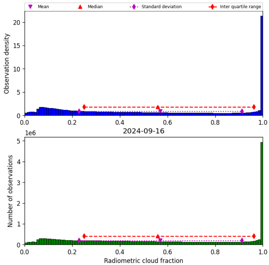
Figure 39: Histogram of “Radiometric cloud fraction” for 2024-09-15 to 2024-09-17
