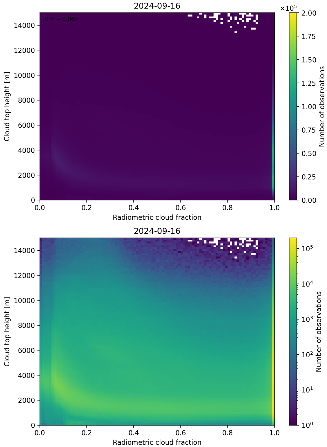
Figure 76: Scatter density plot of “Radiometric cloud fraction” against “Cloud top height” for 2024-09-15 to 2024-09-17.
