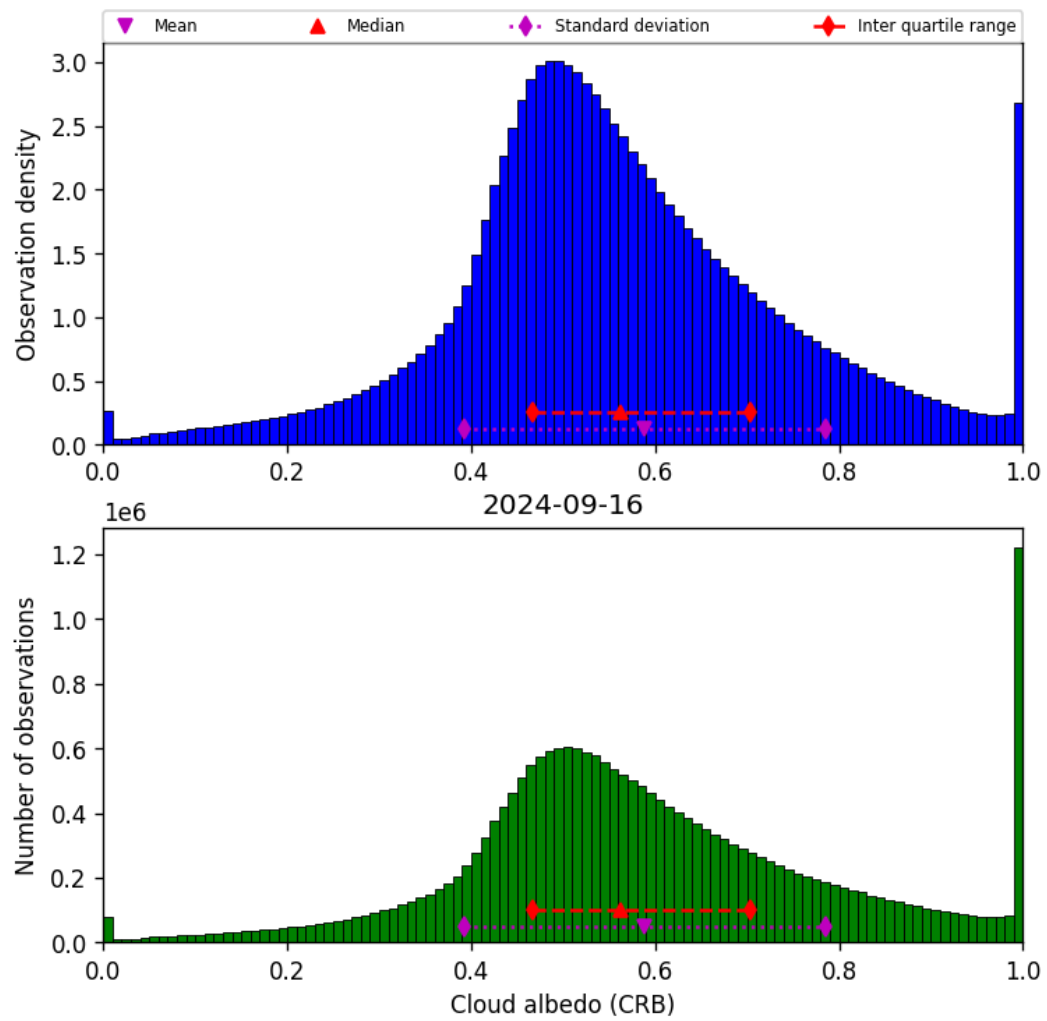
Figure 44: Histogram of “Cloud albedo (CRB)” for 2024-09-15 to 2024-09-17
