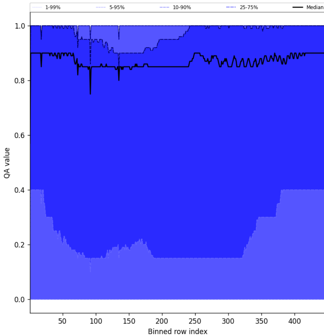
Figure 54: Along track statistics of “QA value” for 2024-09-15 to 2024-09-17
