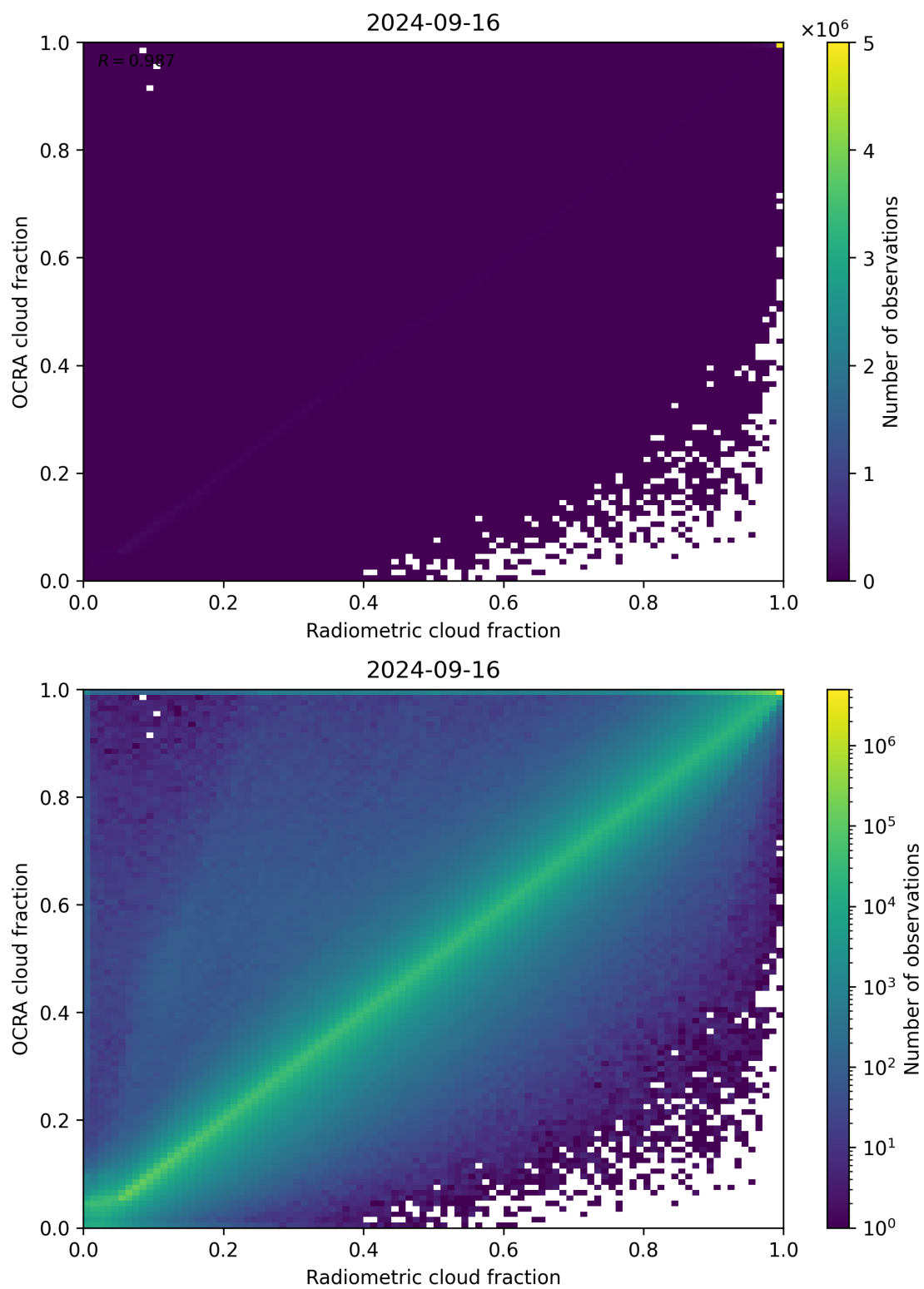
Figure 72: Scatter density plot of “Radiometric cloud fraction” against “OCRA cloud fraction” for 2024-09-15 to 2024-09-17.
