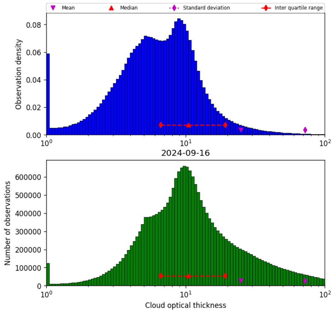
Figure 41: Histogram of “Cloud optical thickness” for 2024-09-15 to 2024-09-17
