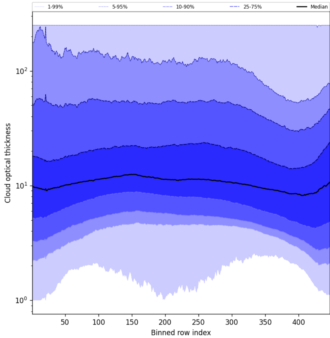
Figure 57: Along track statistics of “Cloud optical thickness” for 2024-09-15 to 2024-09-17
