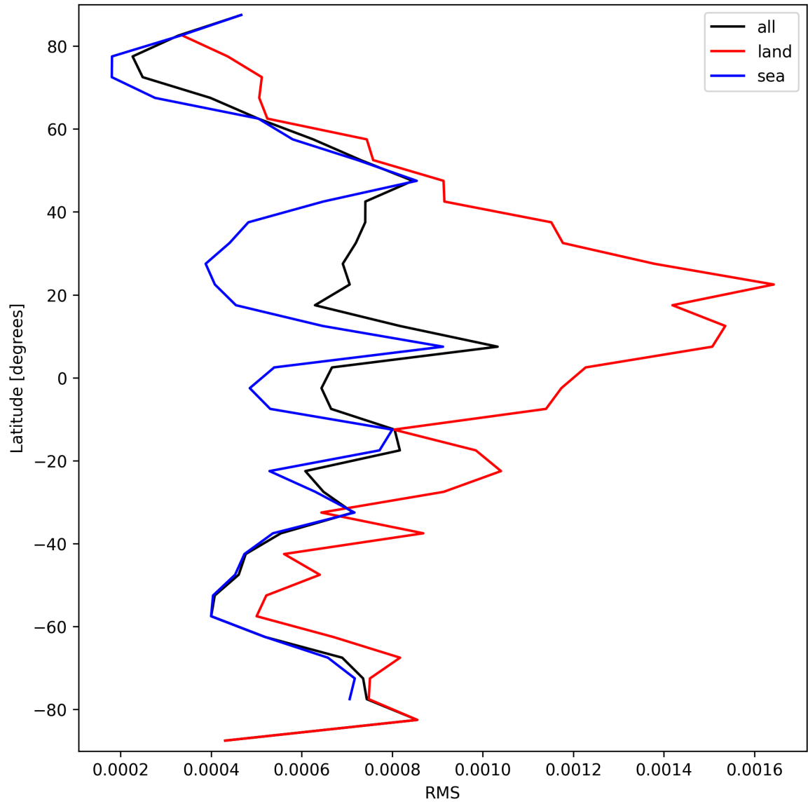
Figure 31: Zonal average of “RMS” for 2024-09-15 to 2024-09-17.
