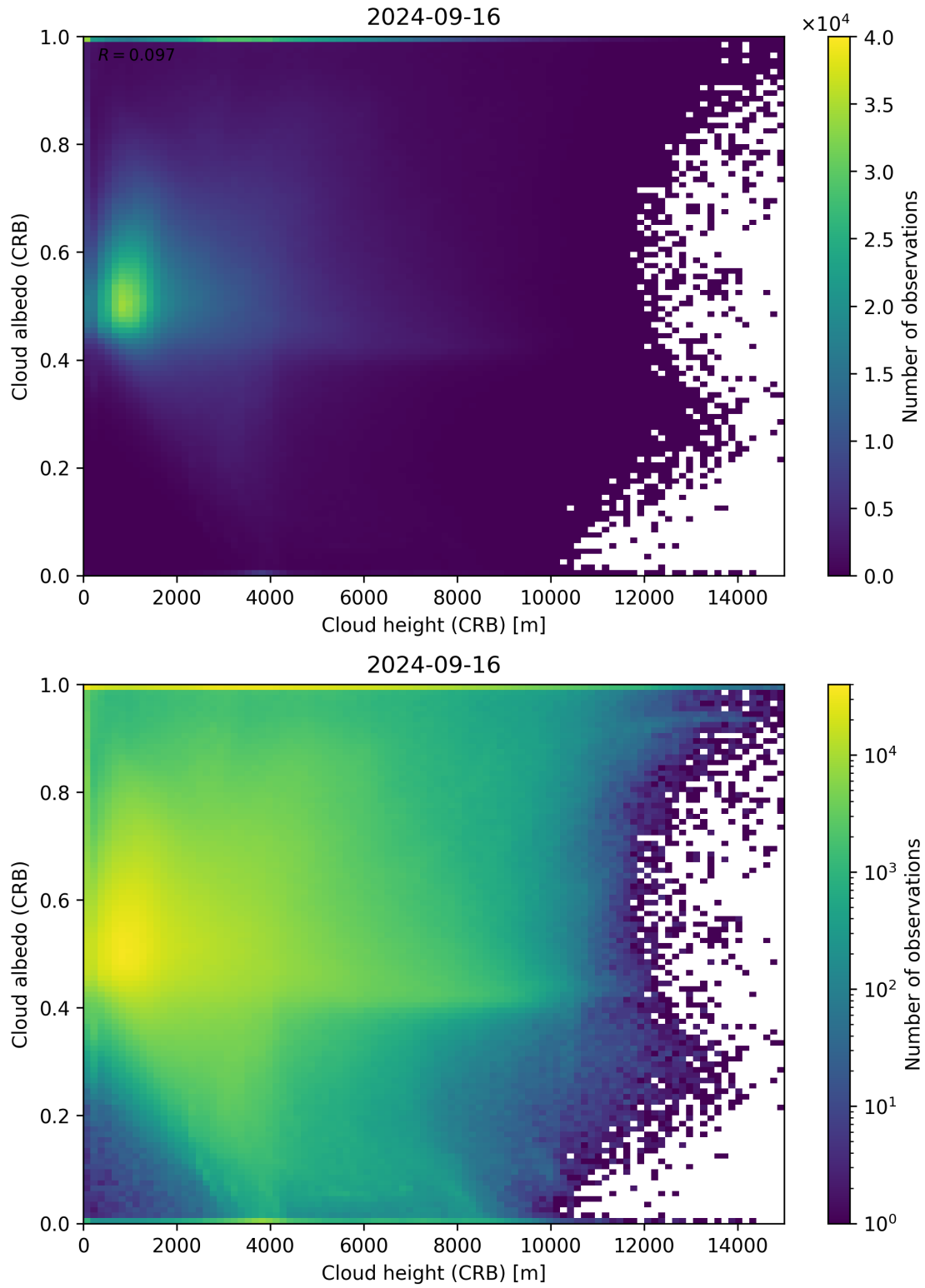
Figure 80: Scatter density plot of “Cloud height (CRB)” against “Cloud albedo (CRB)” for 2024-09-15 to 2024-09-17.
