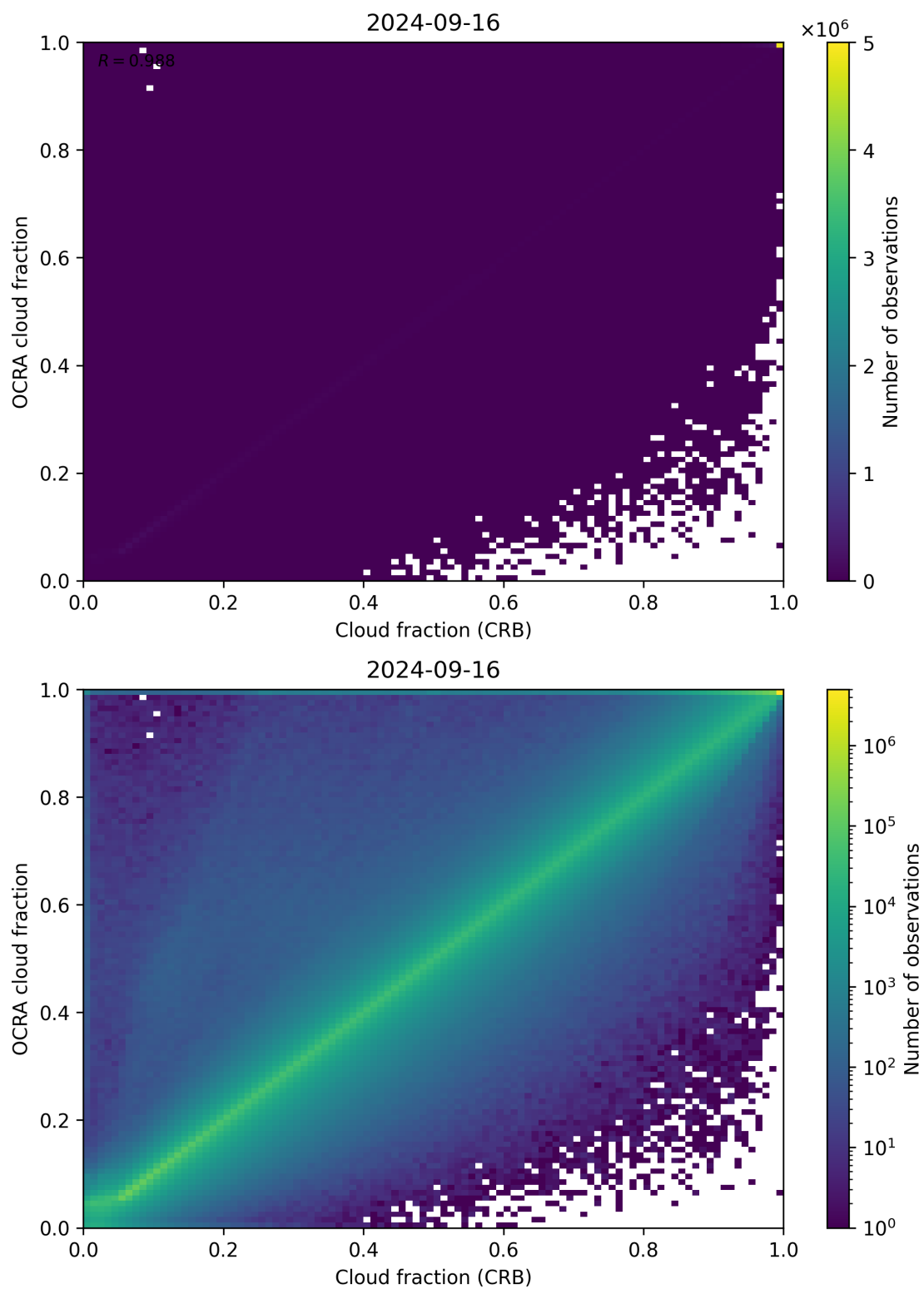
Figure 78: Scatter density plot of “Cloud fraction (CRB)” against “OCRA cloud fraction” for 2024-09-15 to 2024-09-17.
