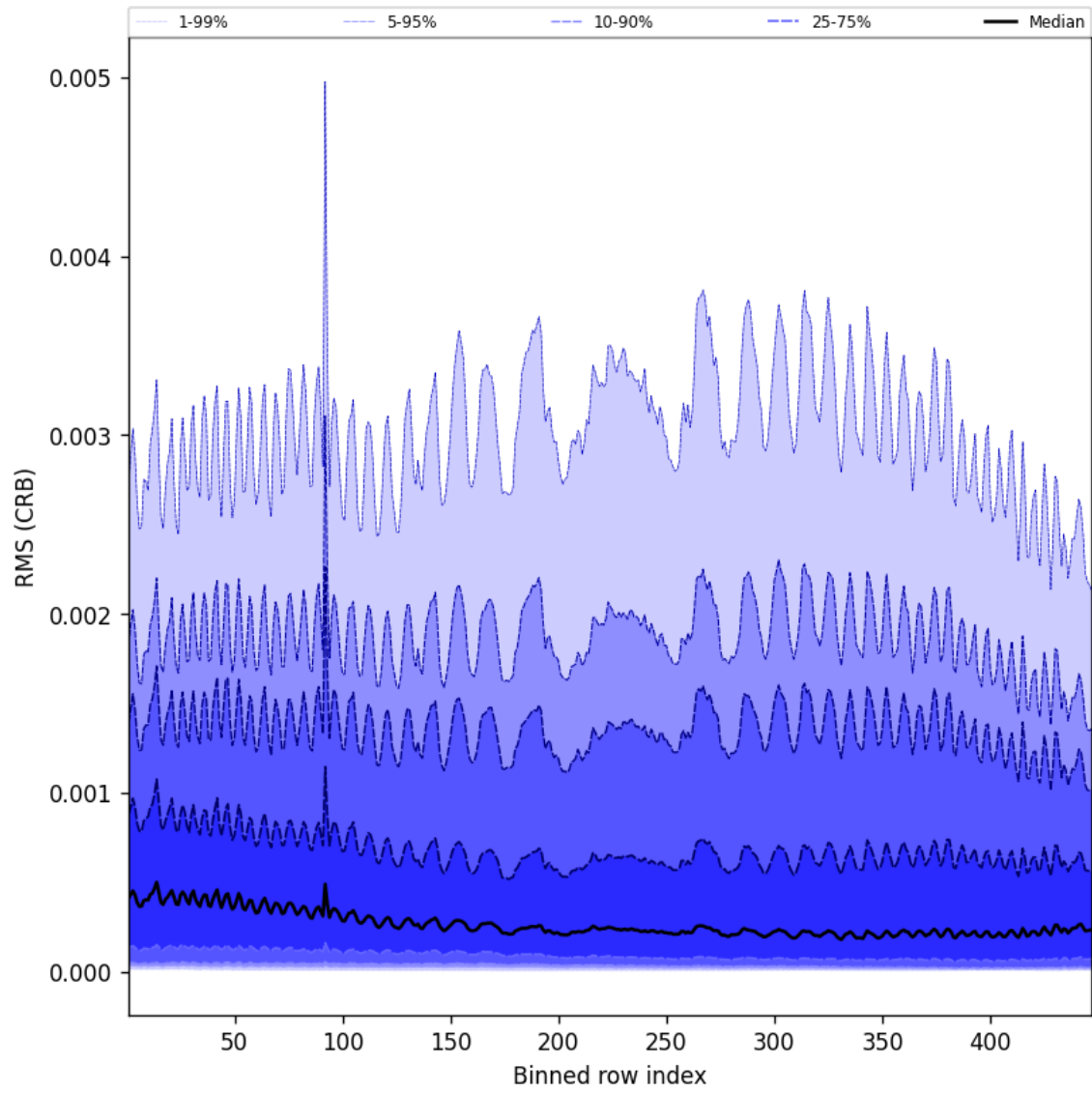
Figure 64: Along track statistics of “RMS (CRB)” for 2024-09-15 to 2024-09-17
