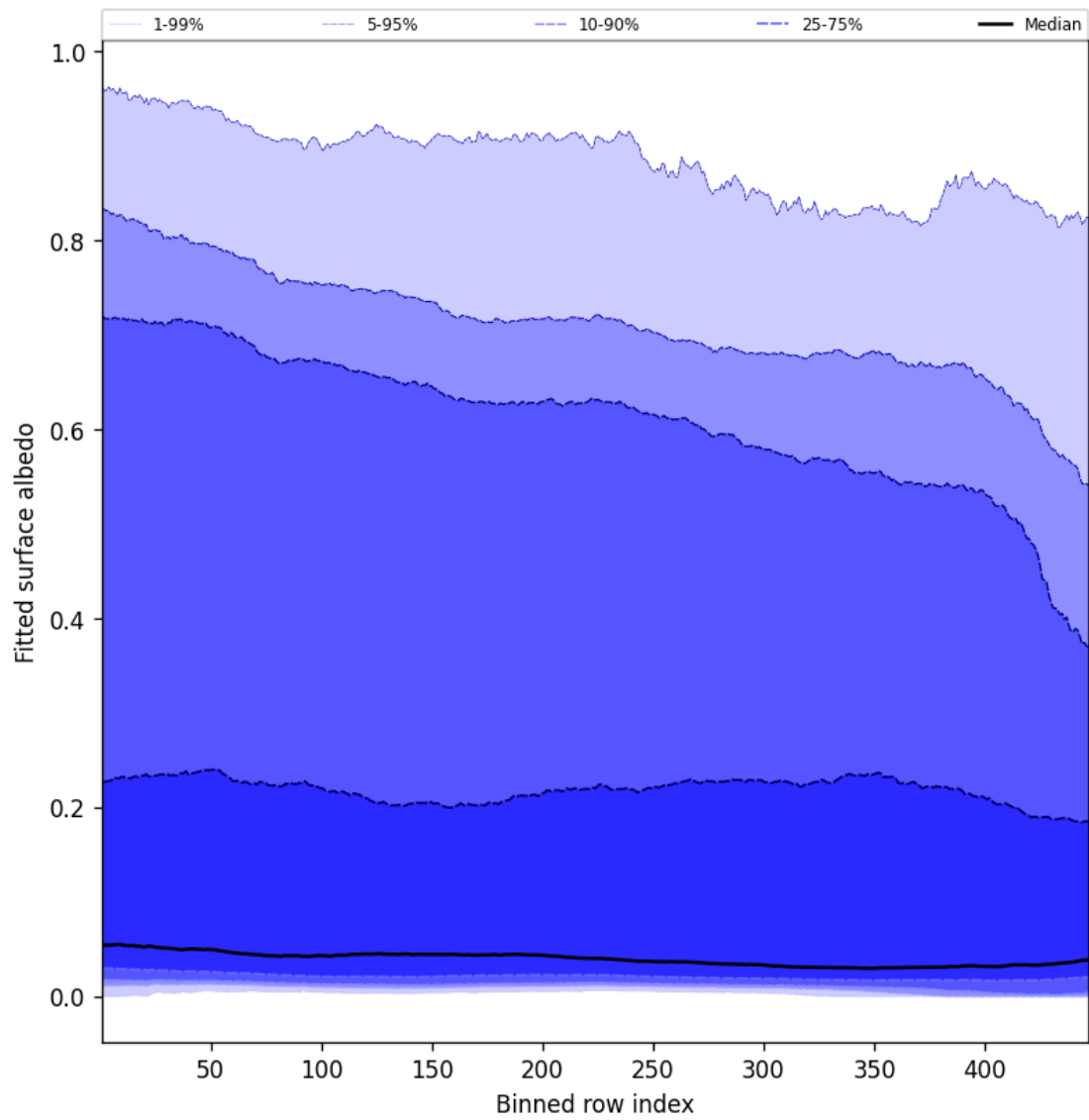
Figure 61: Along track statistics of “Fitted surface albedo” for 2024-09-15 to 2024-09-17
