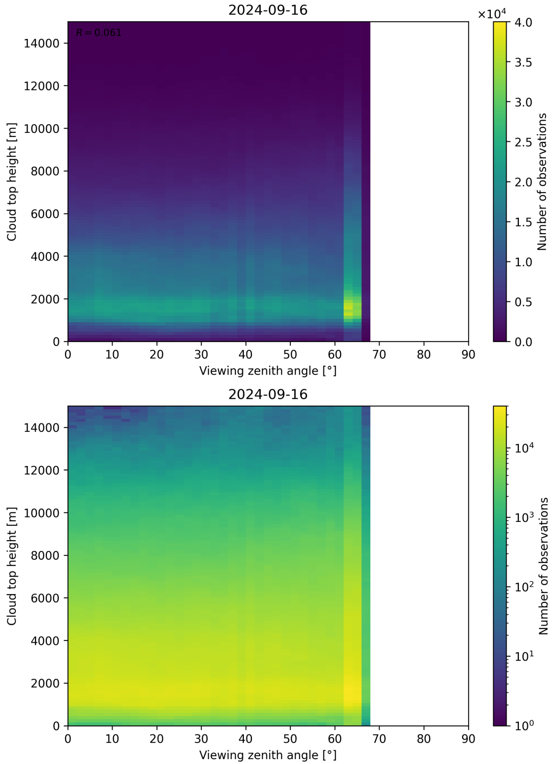
Figure 112: Scatter density plot of “Viewing zenith angle” against “Cloud top height” for 2024-09-15 to 2024-09-17.
