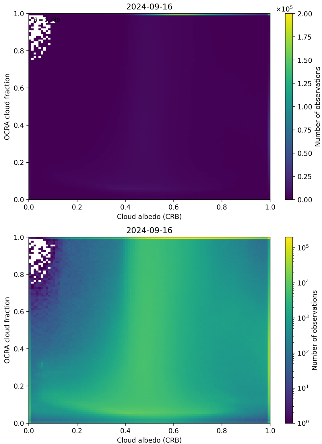
Figure 70: Scatter density plot of “Cloud albedo (CRB)” against “OCRA cloud fraction” for 2024-09-15 to 2024-09-17.
