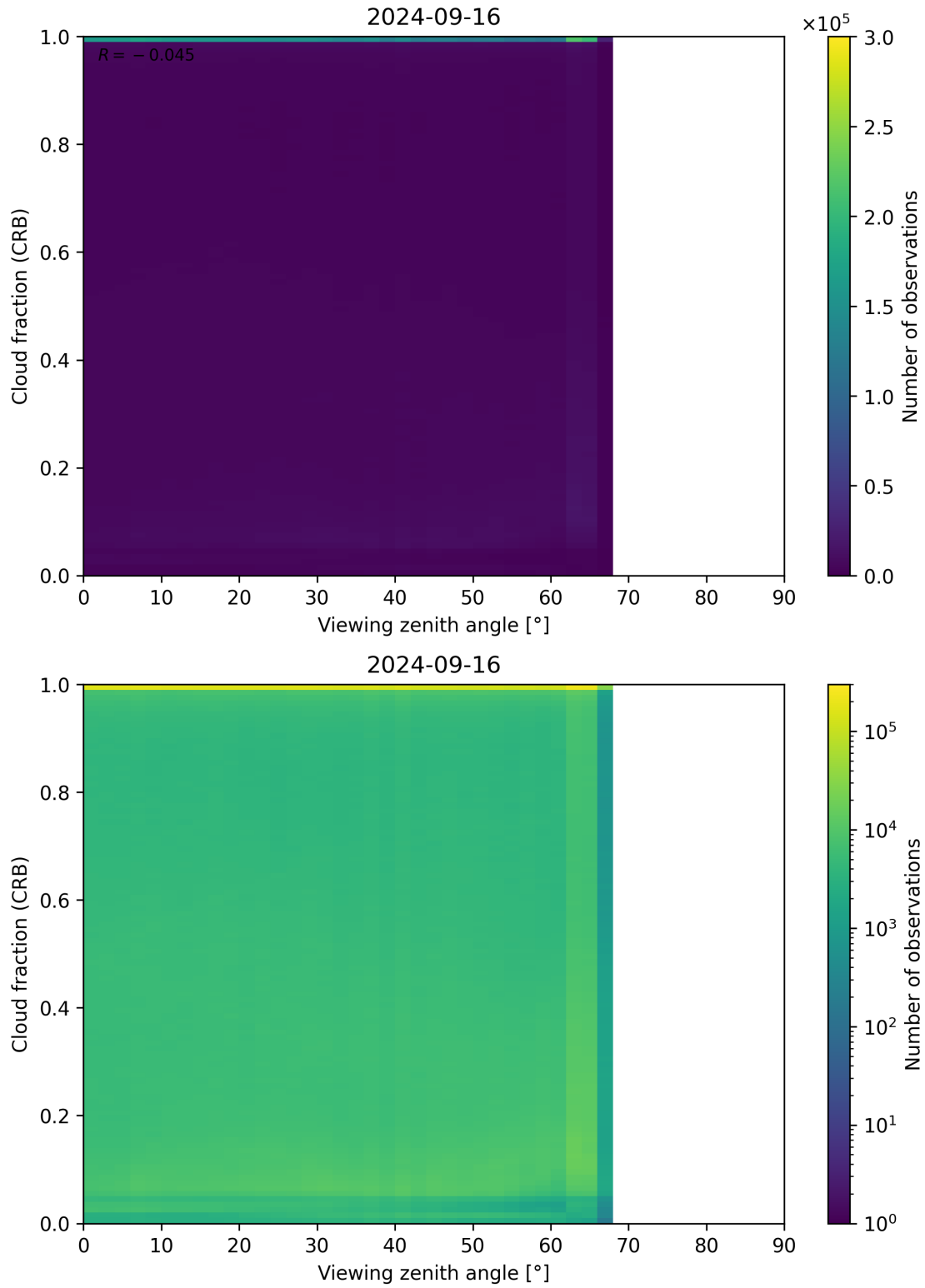
Figure 109: Scatter density plot of “Viewing zenith angle” against “Cloud fraction (CRB)” for 2024-09-15 to 2024-09-17.
