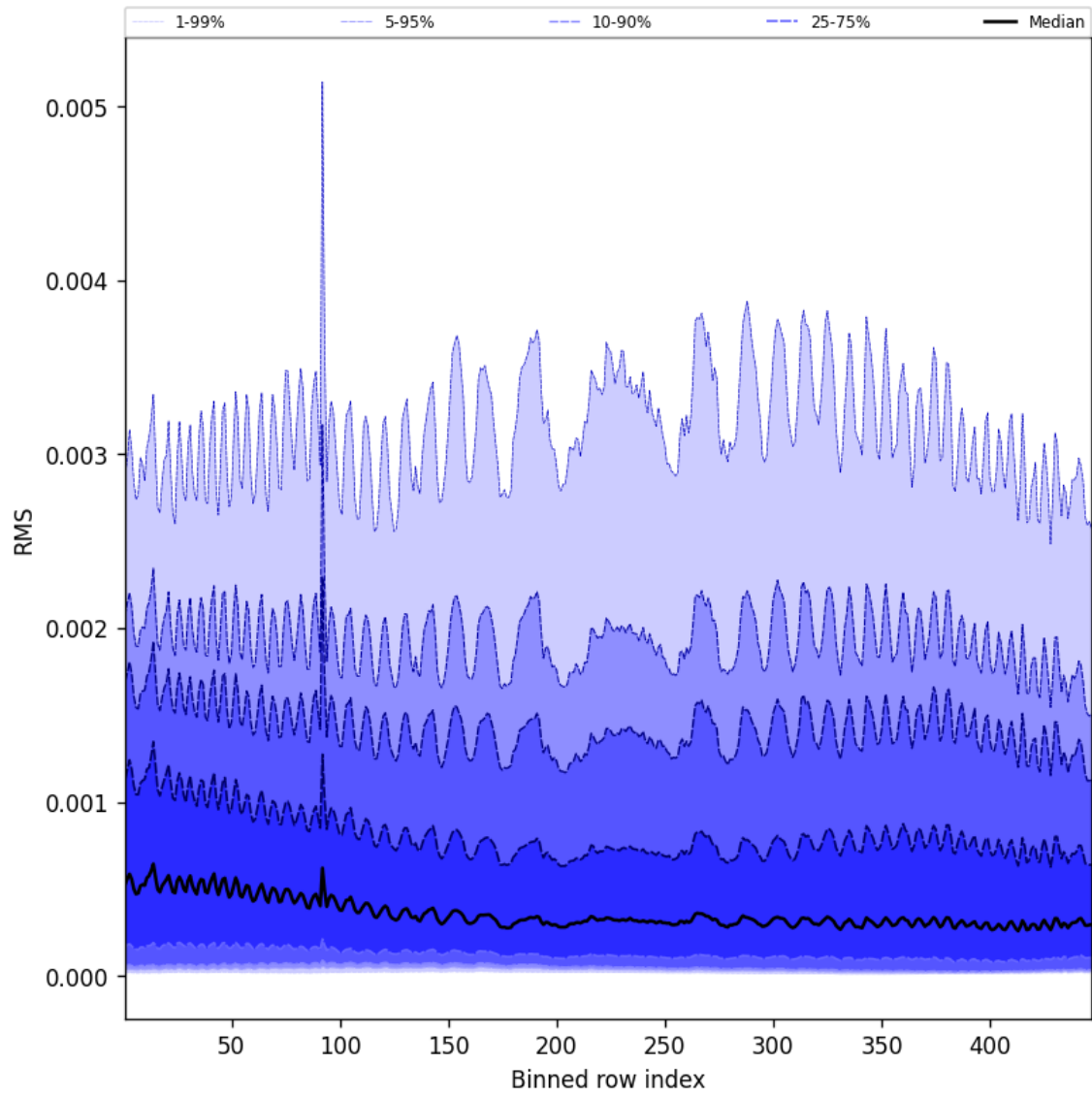
Figure 63: Along track statistics of “RMS” for 2024-09-15 to 2024-09-17
