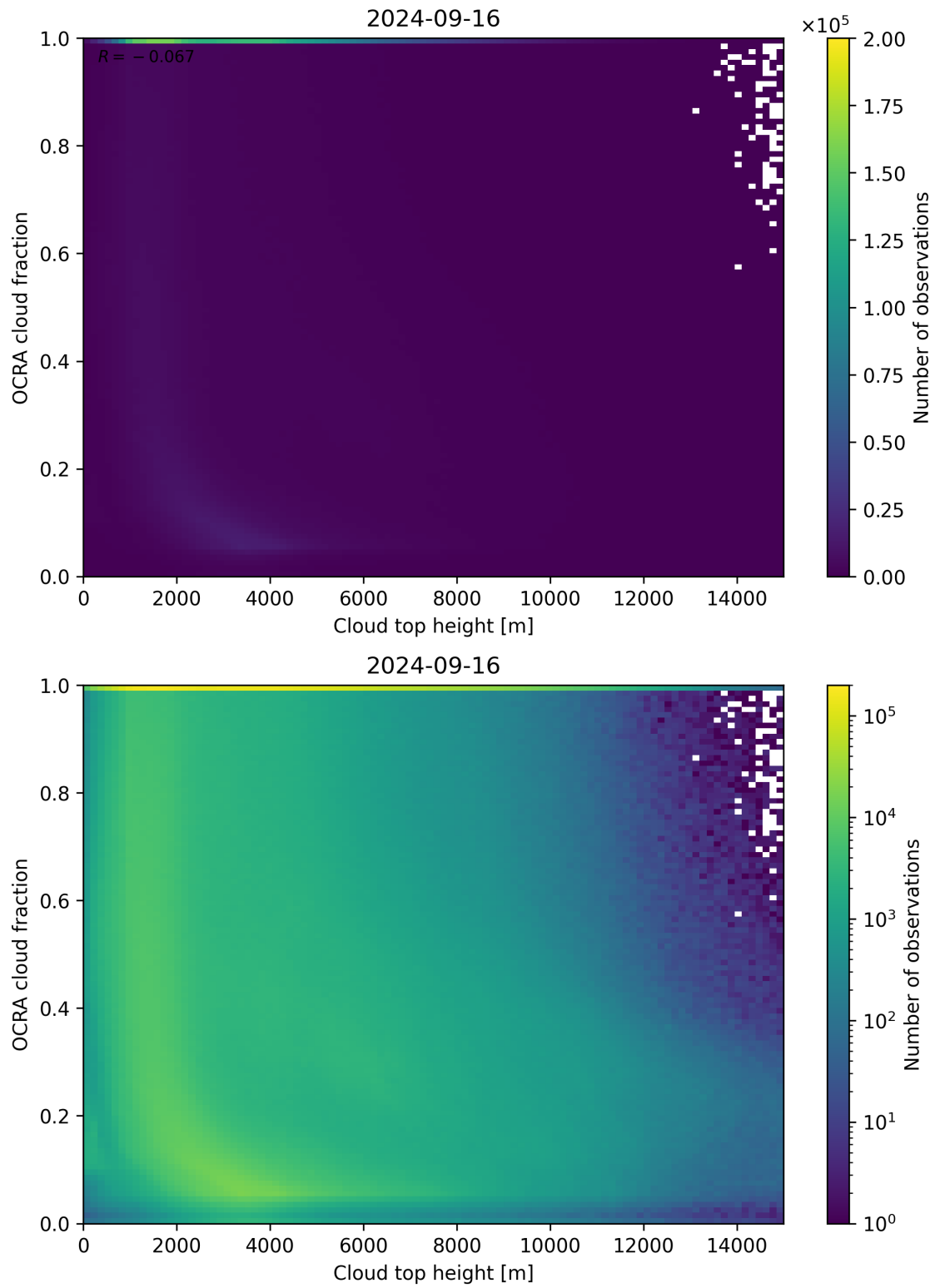
Figure 87: Scatter density plot of “Cloud top height” against “OCRA cloud fraction” for 2024-09-15 to 2024-09-17.
