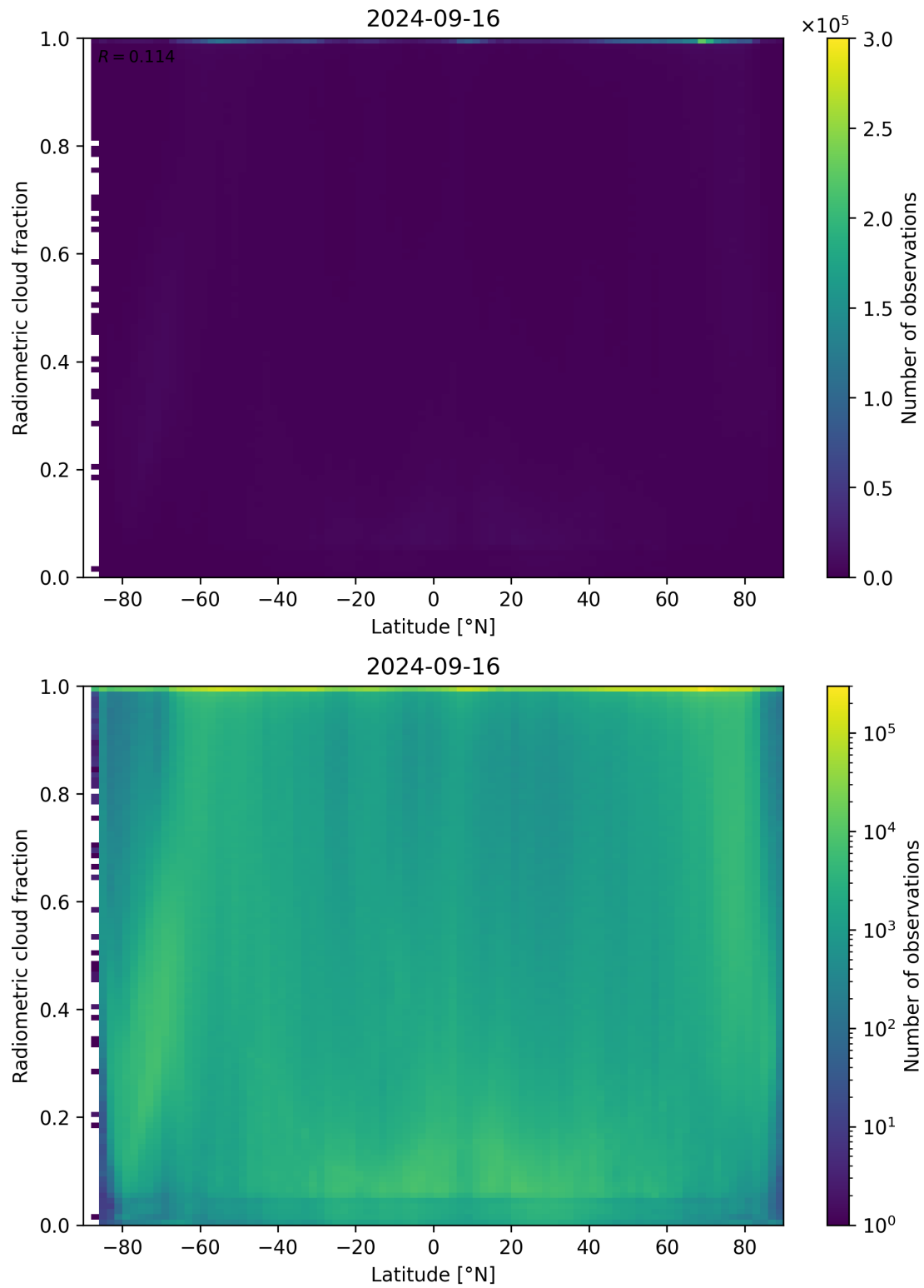
Figure 92: Scatter density plot of “Latitude” against “Radiometric cloud fraction” for 2024-09-15 to 2024-09-17.
