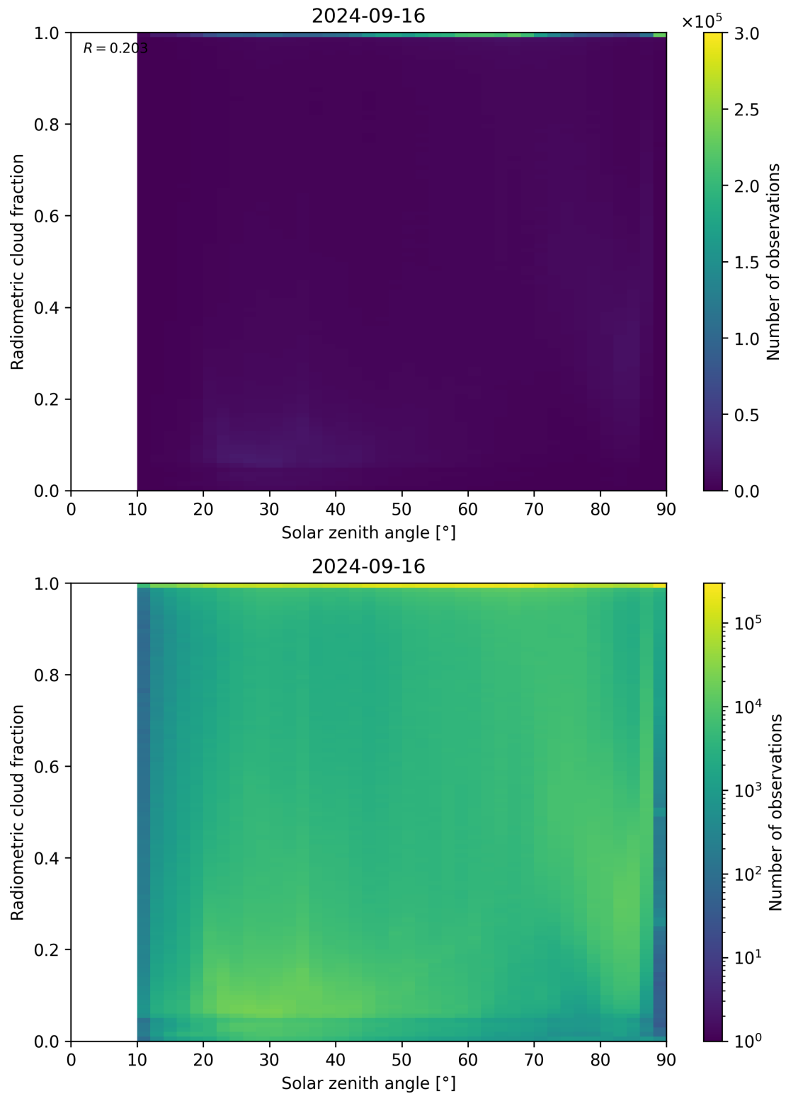
Figure 99: Scatter density plot of “Solar zenith angle” against “Radiometric cloud fraction” for 2024-09-15 to 2024-09-17.
