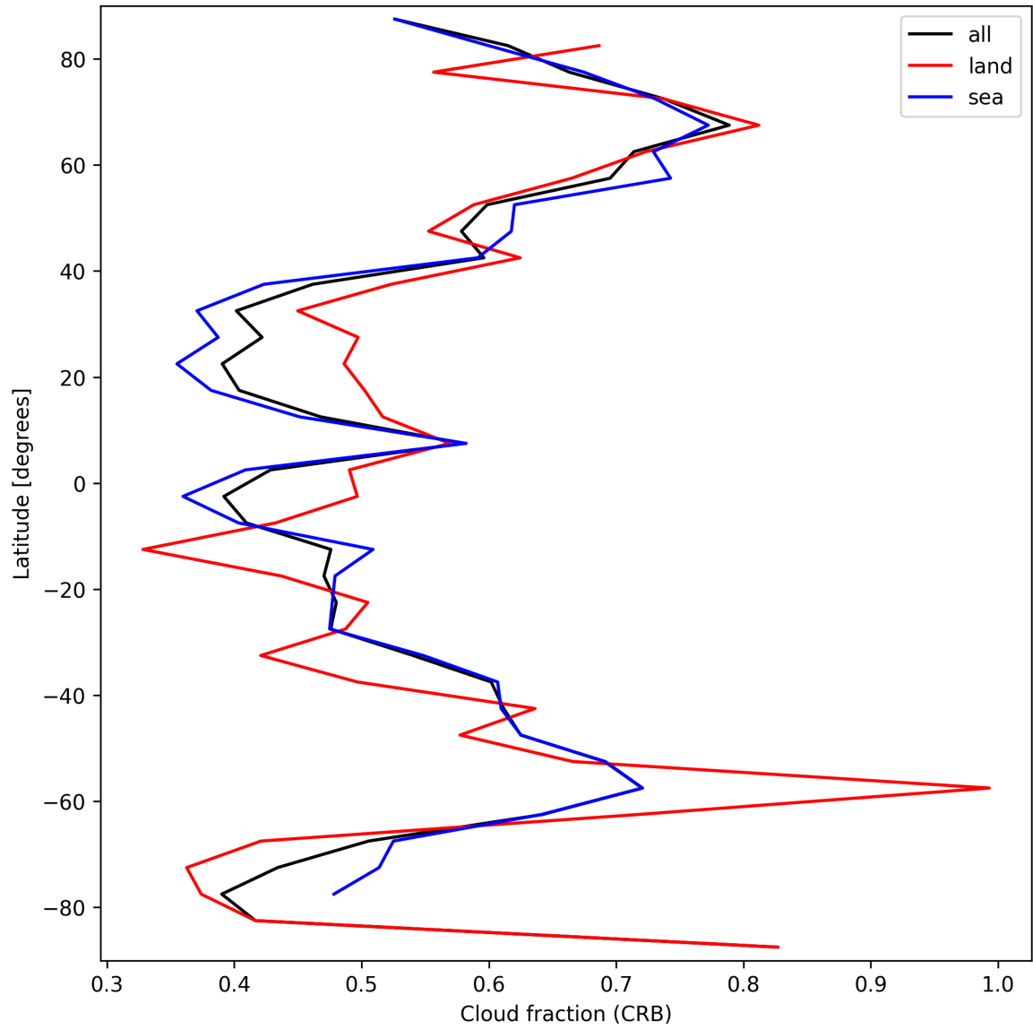
Figure 26: Zonal average of “Cloud fraction (CRB)” for 2024-09-17 to 2024-09-18.
