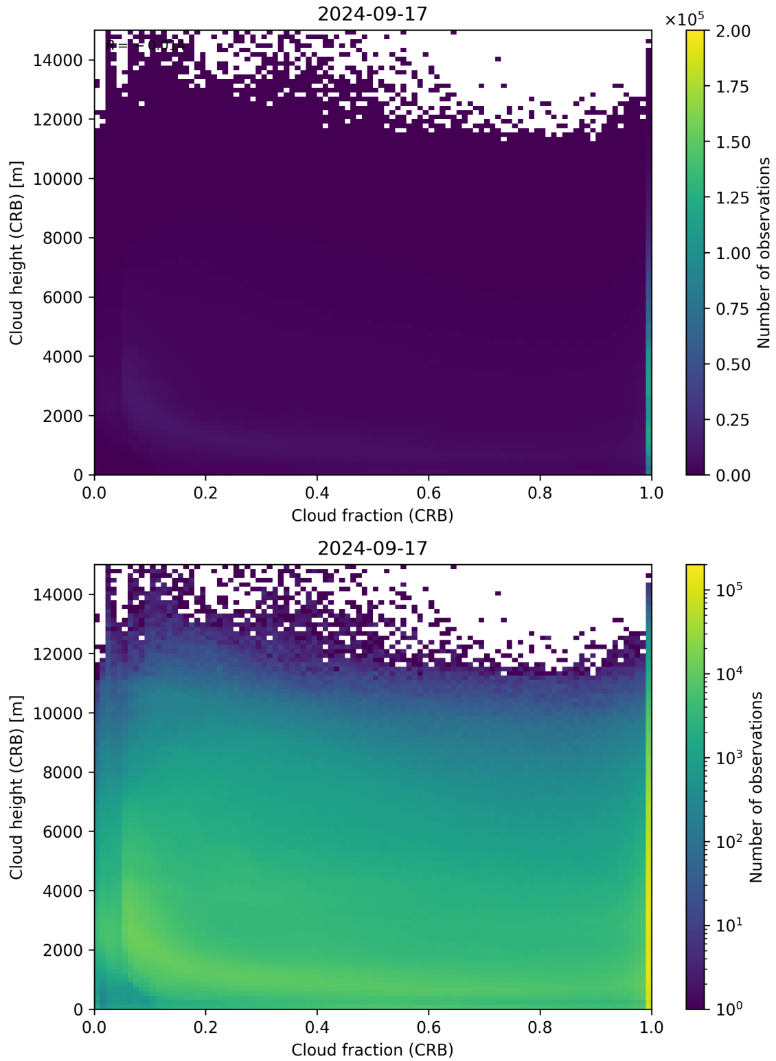
Figure 79: Scatter density plot of “Cloud fraction (CRB)” against “Cloud height (CRB)” for 2024-09-17 to 2024-09-18.
