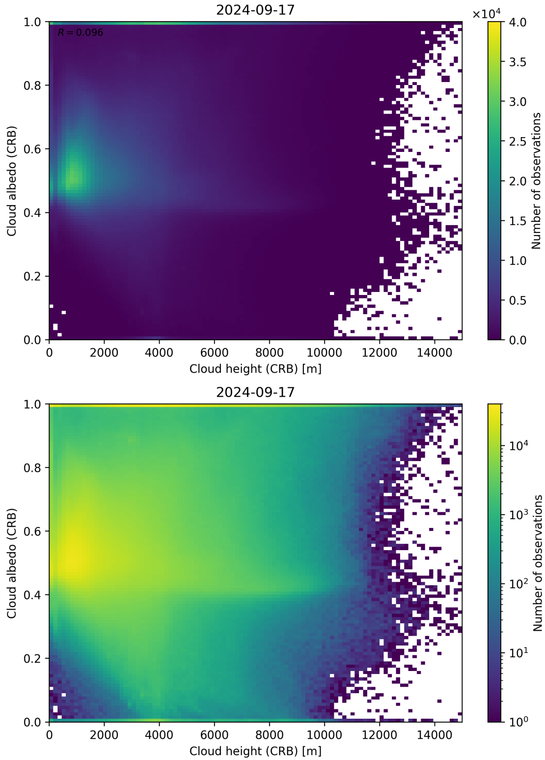
Figure 80: Scatter density plot of “Cloud height (CRB)” against “Cloud albedo (CRB)” for 2024-09-17 to 2024-09-18.
