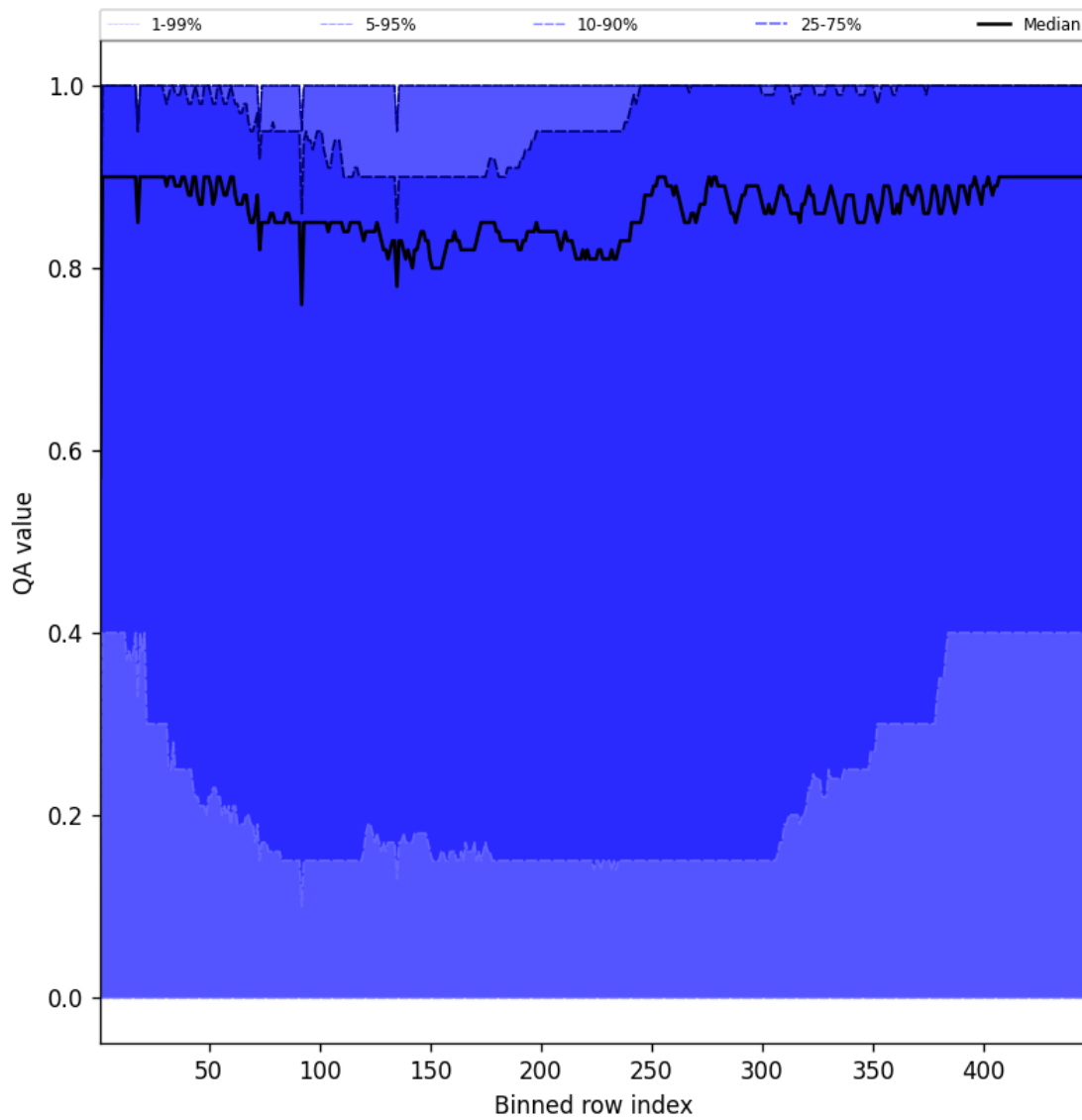
Figure 54: Along track statistics of “QA value” for 2024-09-17 to 2024-09-18
