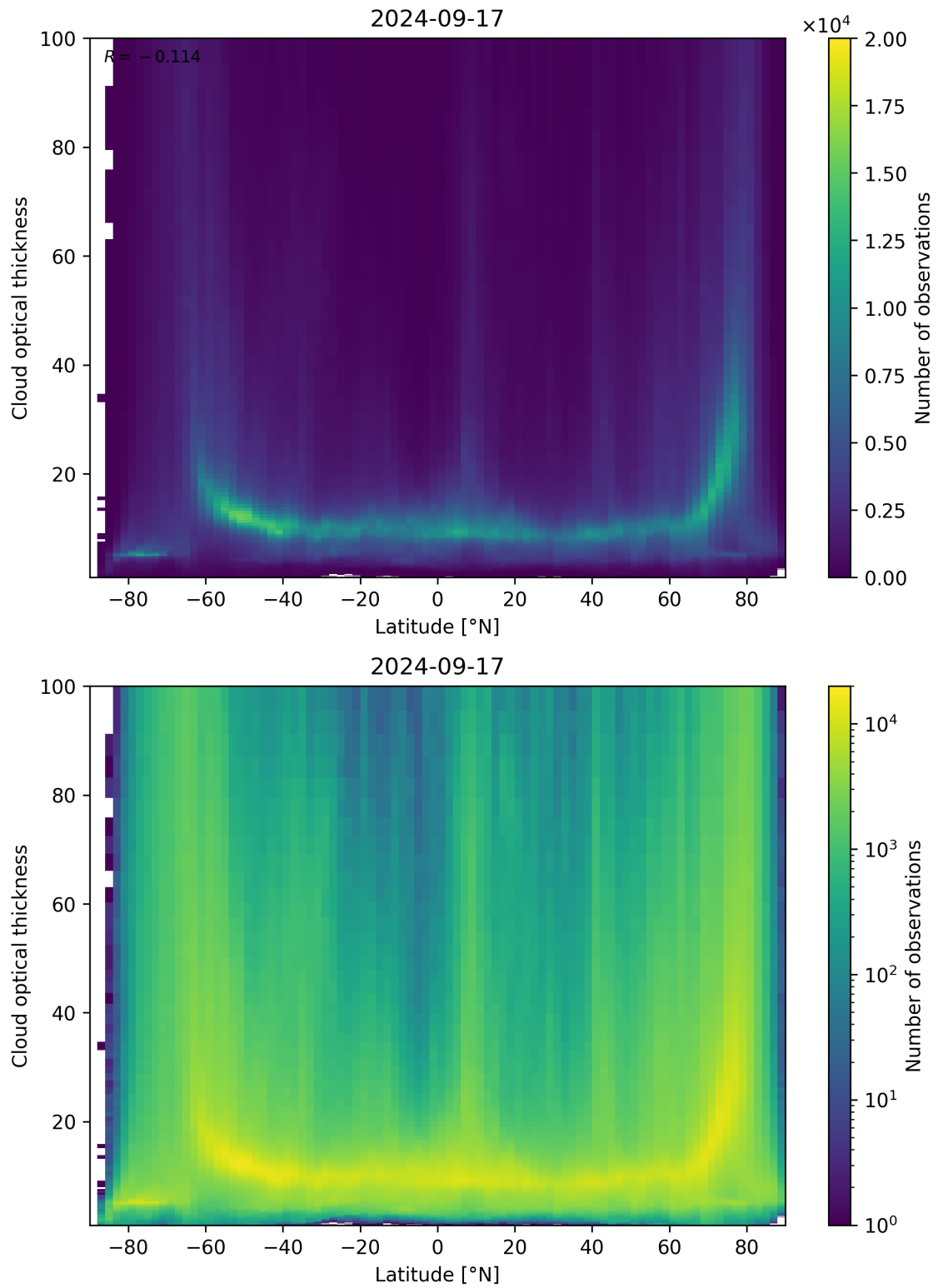
Figure 96: Scatter density plot of “Latitude” against “Cloud optical thickness” for 2024-09-17 to 2024-09-18.
