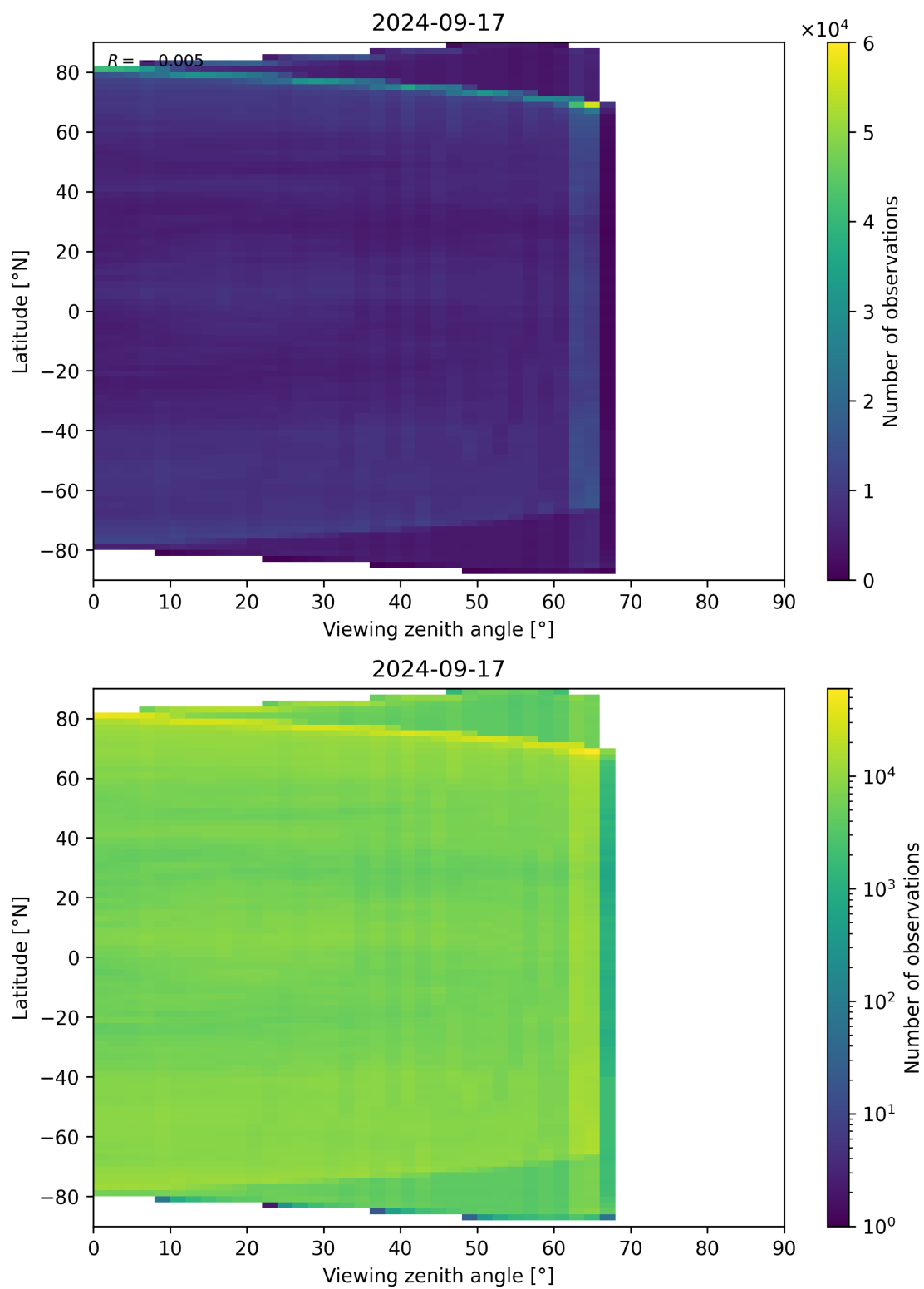
Figure 113: Scatter density plot of “Viewing zenith angle” against “Latitude” for 2024-09-17 to 2024-09-18.
