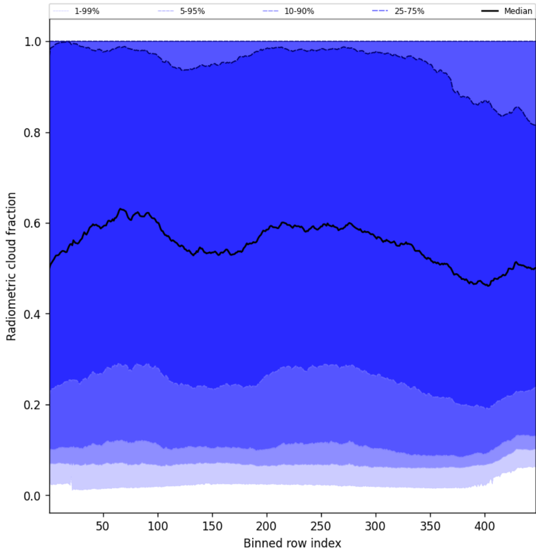
Figure 55: Along track statistics of “Radiometric cloud fraction” for 2024-09-17 to 2024-09-18
