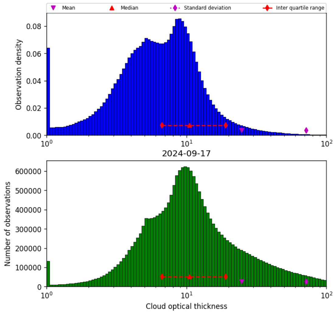
Figure 41: Histogram of “Cloud optical thickness” for 2024-09-17 to 2024-09-18
