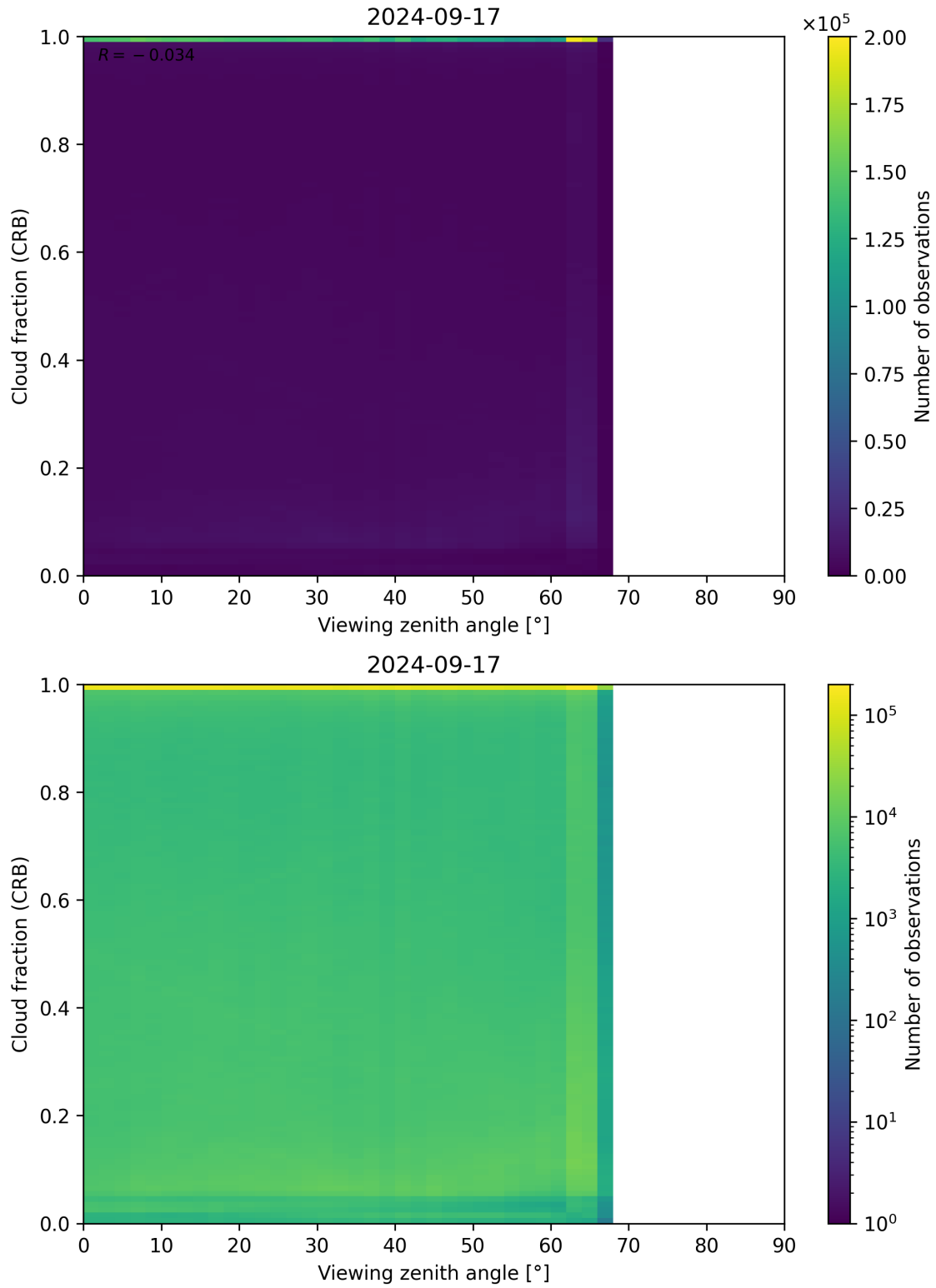
Figure 109: Scatter density plot of “Viewing zenith angle” against “Cloud fraction (CRB)” for 2024-09-17 to 2024-09-18.
