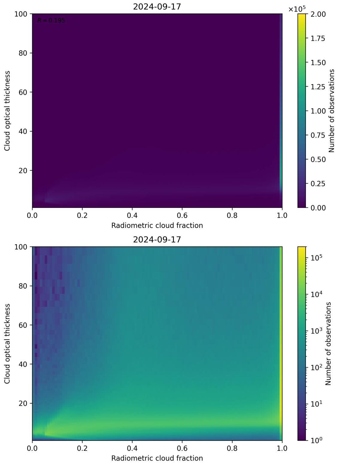
Figure 75: Scatter density plot of “Radiometric cloud fraction” against “Cloud optical thickness” for 2024-09-17 to 2024-09-18.
