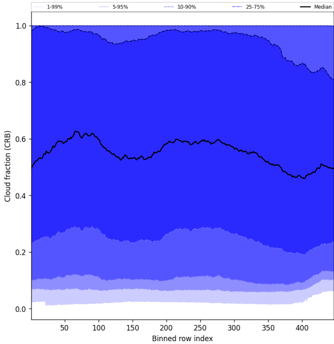
Figure 58: Along track statistics of “Cloud fraction (CRB)” for 2024-09-17 to 2024-09-18
