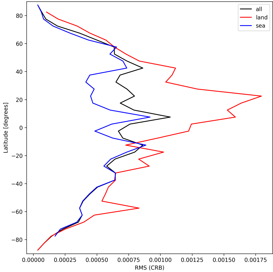
Figure 32: Zonal average of “RMS (CRB)” for 2024-09-17 to 2024-09-18.
