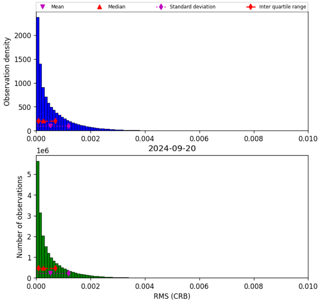
Figure 48: Histogram of “RMS (CRB)” for 2024-09-19 to 2024-09-21
