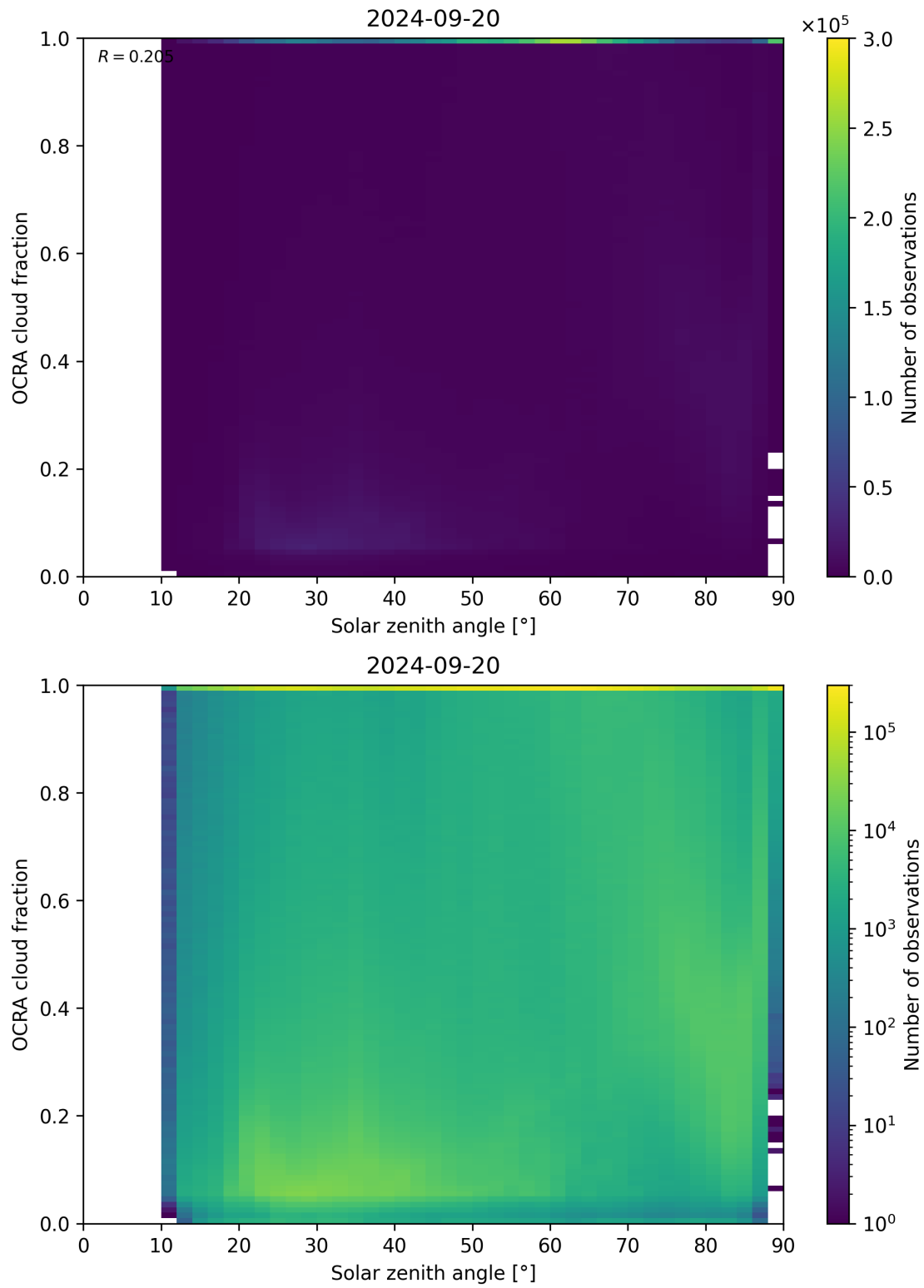
Figure 100: Scatter density plot of “Solar zenith angle” against “OCRA cloud fraction” for 2024-09-19 to 2024-09-21.
