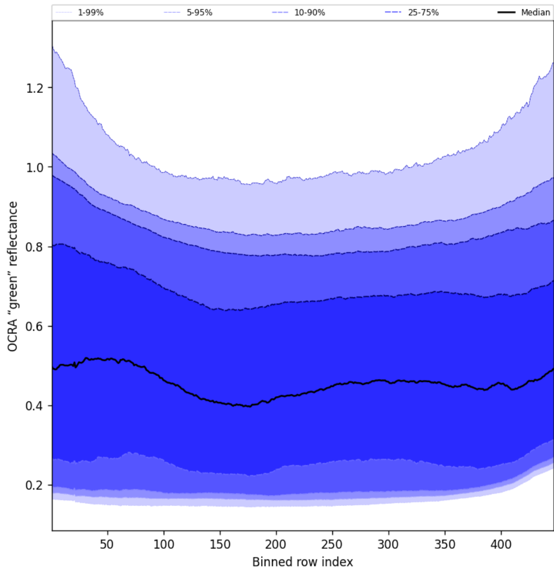
Figure 68: Along track statistics of “OCRA “green” reflectance” for 2024-09-19 to 2024-09-21
