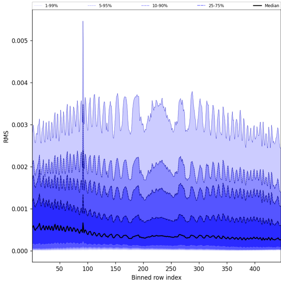
Figure 63: Along track statistics of “RMS” for 2024-09-19 to 2024-09-21
