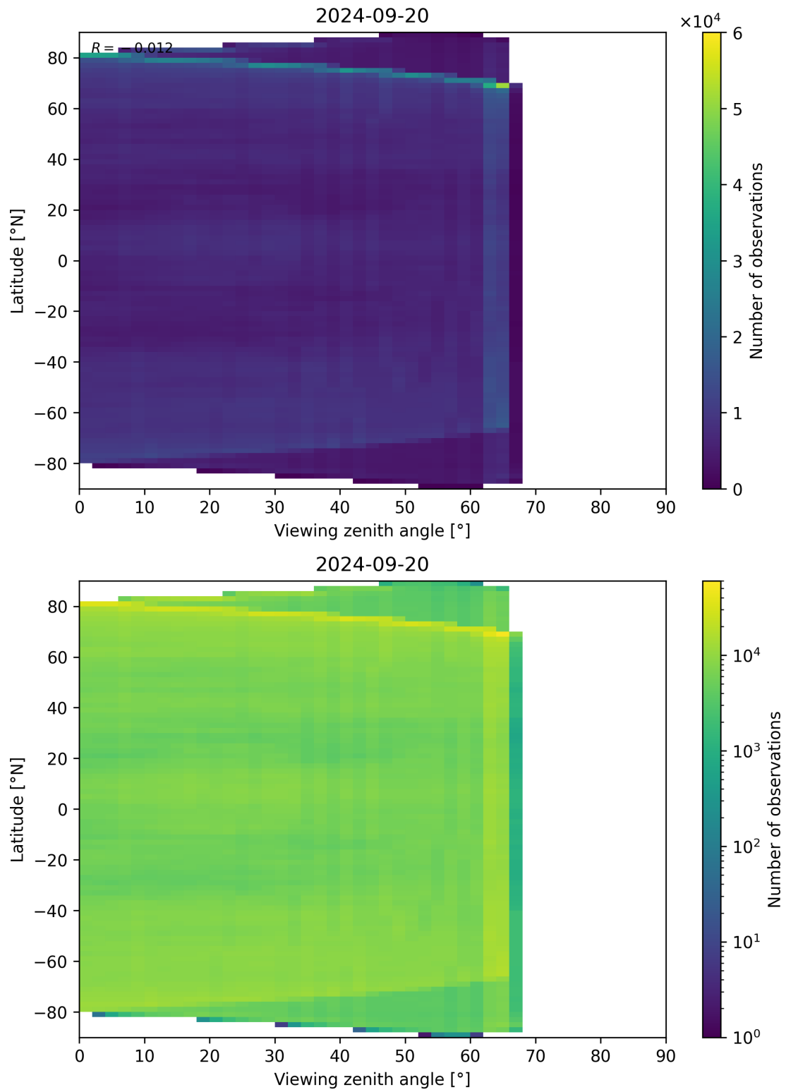
Figure 113: Scatter density plot of “Viewing zenith angle” against “Latitude” for 2024-09-19 to 2024-09-21.
