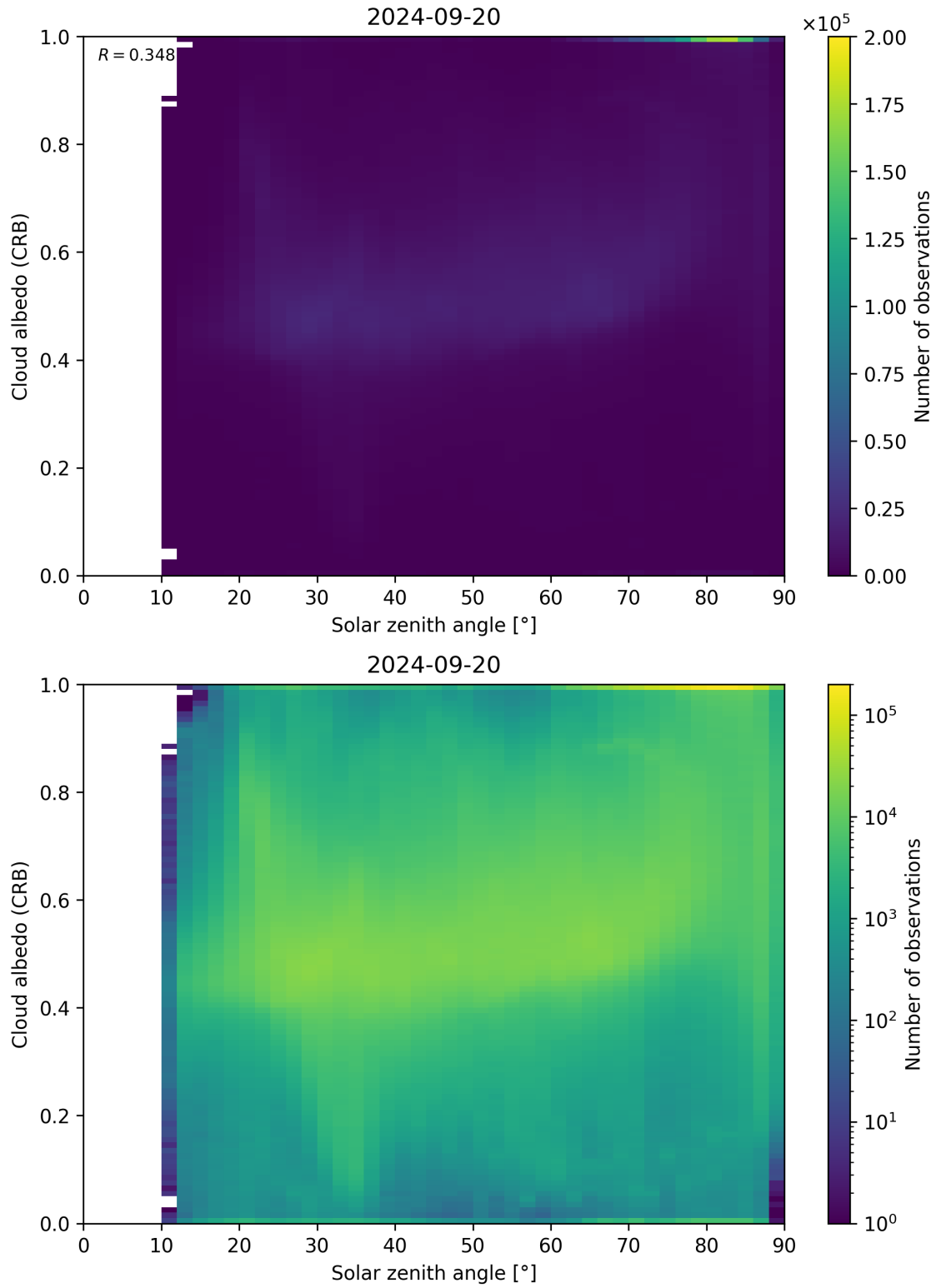
Figure 98: Scatter density plot of “Solar zenith angle” against “Cloud albedo (CRB)” for 2024-09-19 to 2024-09-21.
