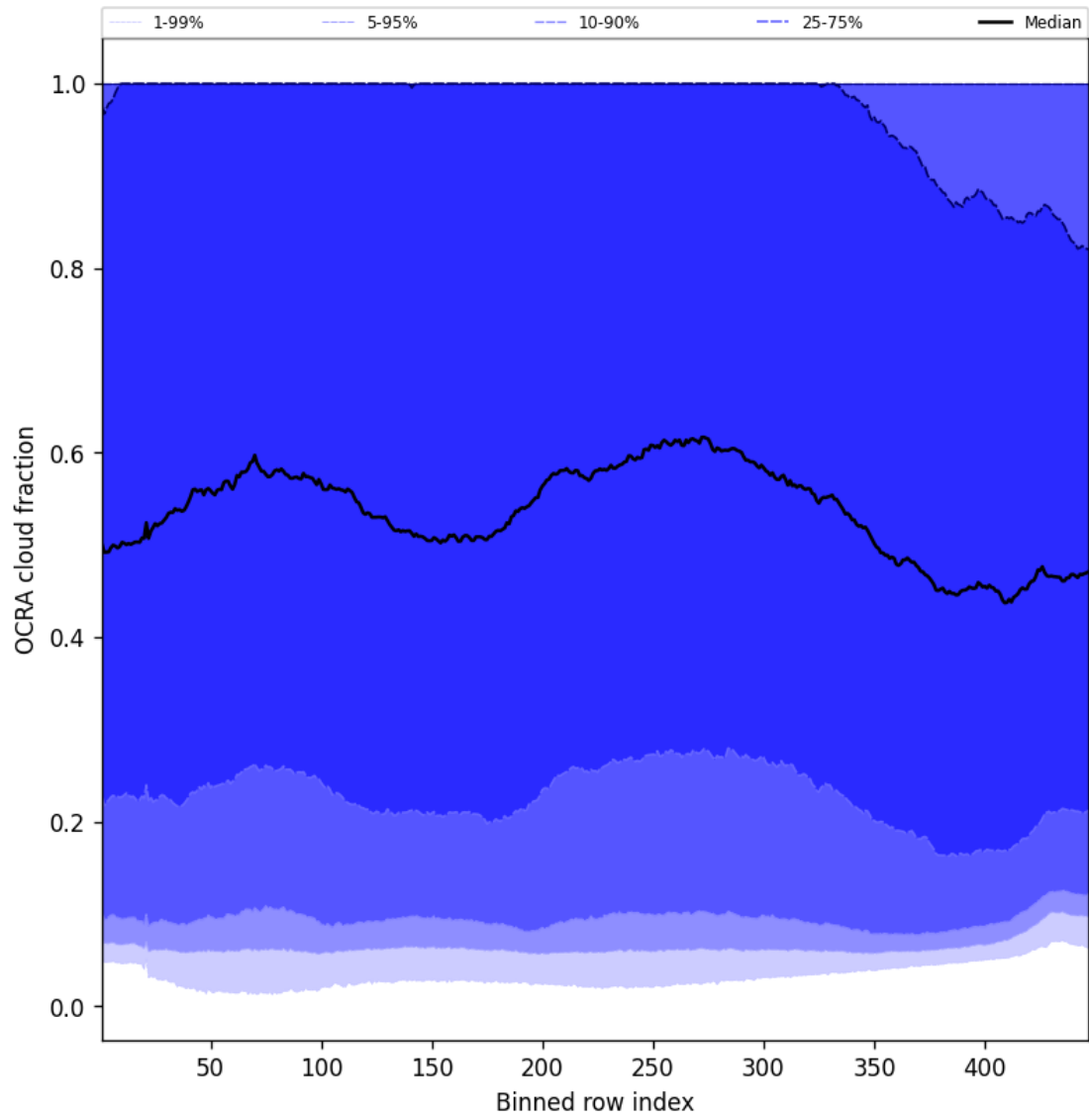
Figure 66: Along track statistics of “OCRA cloud fraction” for 2024-09-19 to 2024-09-21
