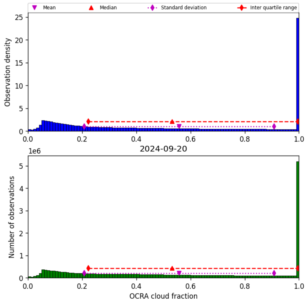
Figure 50: Histogram of “OCRA cloud fraction” for 2024-09-19 to 2024-09-21
