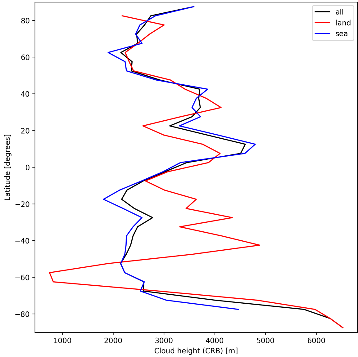
Figure 27: Zonal average of “Cloud height (CRB)” for 2024-09-19 to 2024-09-21.
