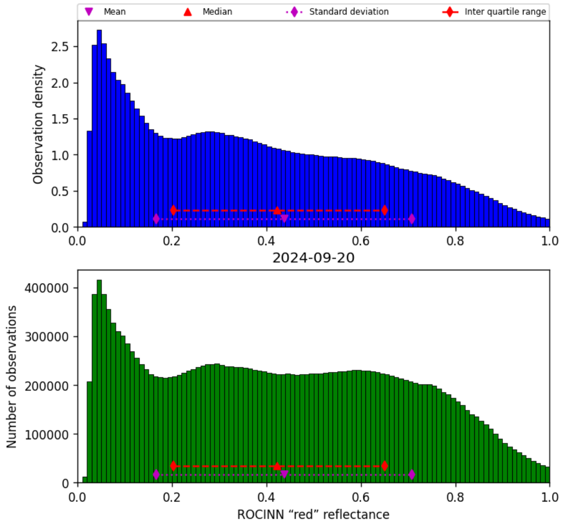
Figure 53: Histogram of “ROCINN “red” reflectance” for 2024-09-19 to 2024-09-21
