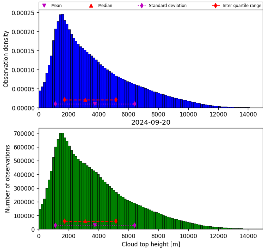
Figure 40: Histogram of “Cloud top height” for 2024-09-19 to 2024-09-21
