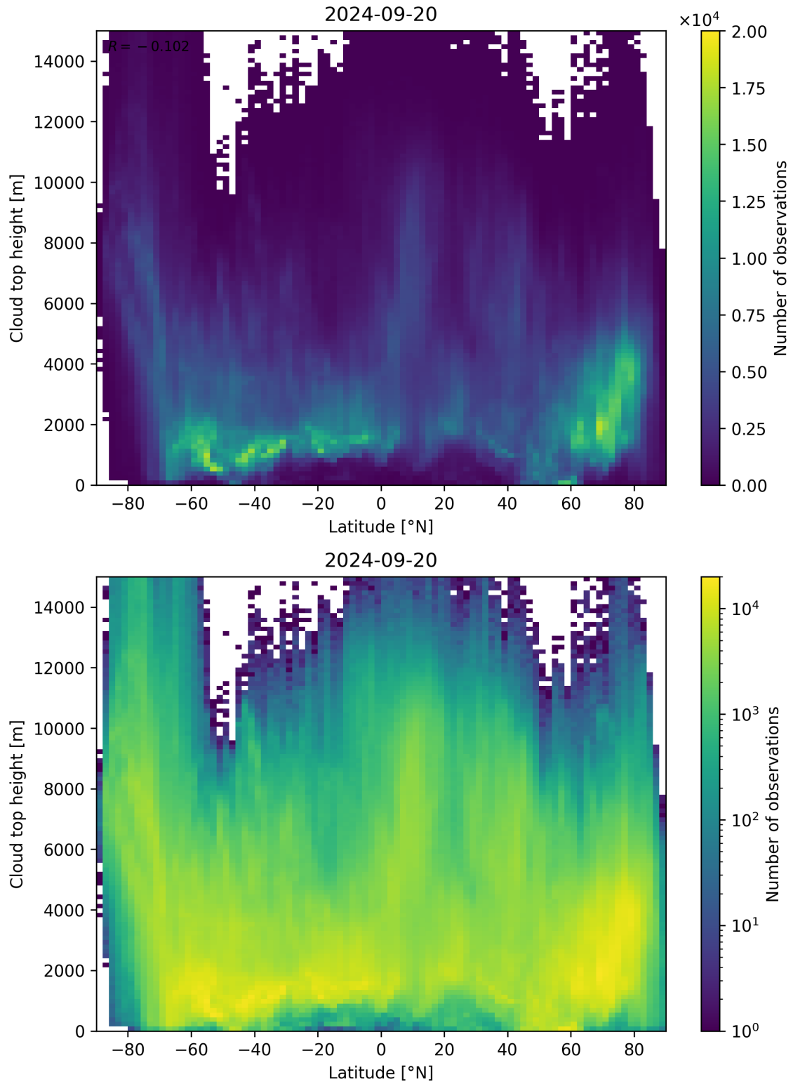
Figure 97: Scatter density plot of “Latitude” against “Cloud top height” for 2024-09-19 to 2024-09-21.
