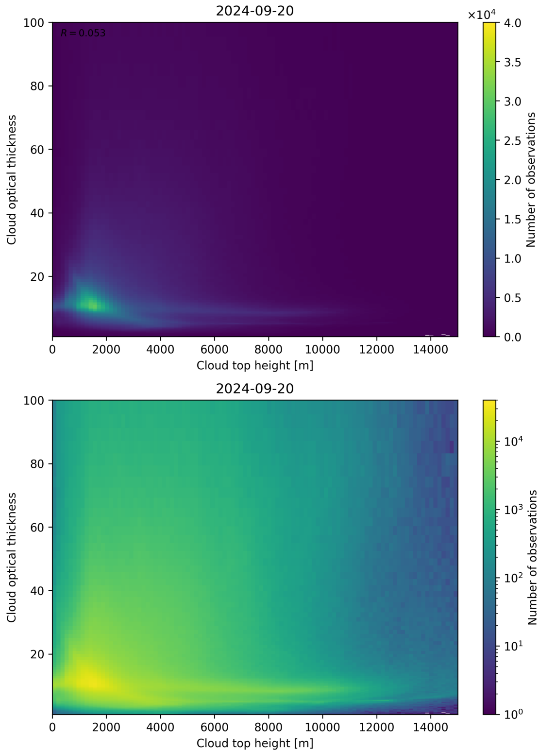
Figure 90: Scatter density plot of “Cloud top height” against “Cloud optical thickness” for 2024-09-19 to 2024-09-21.
