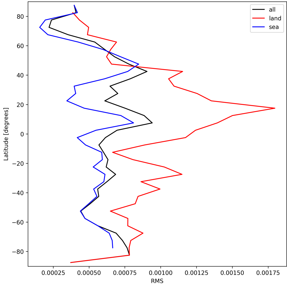
Figure 31: Zonal average of “RMS” for 2024-09-19 to 2024-09-21.
