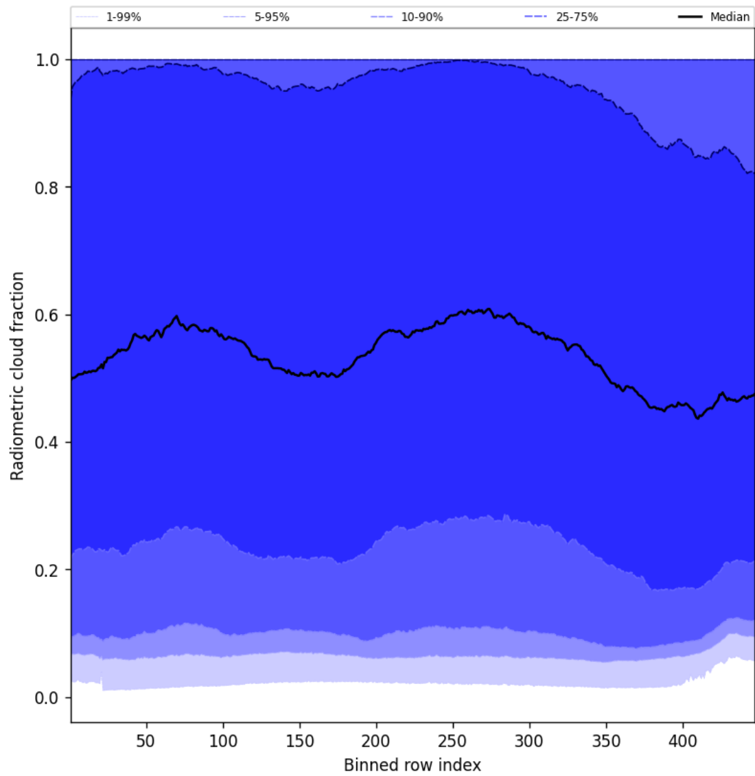
Figure 55: Along track statistics of "Radiometric cloud fraction" for 2024-09-19 to 2024-09-21
