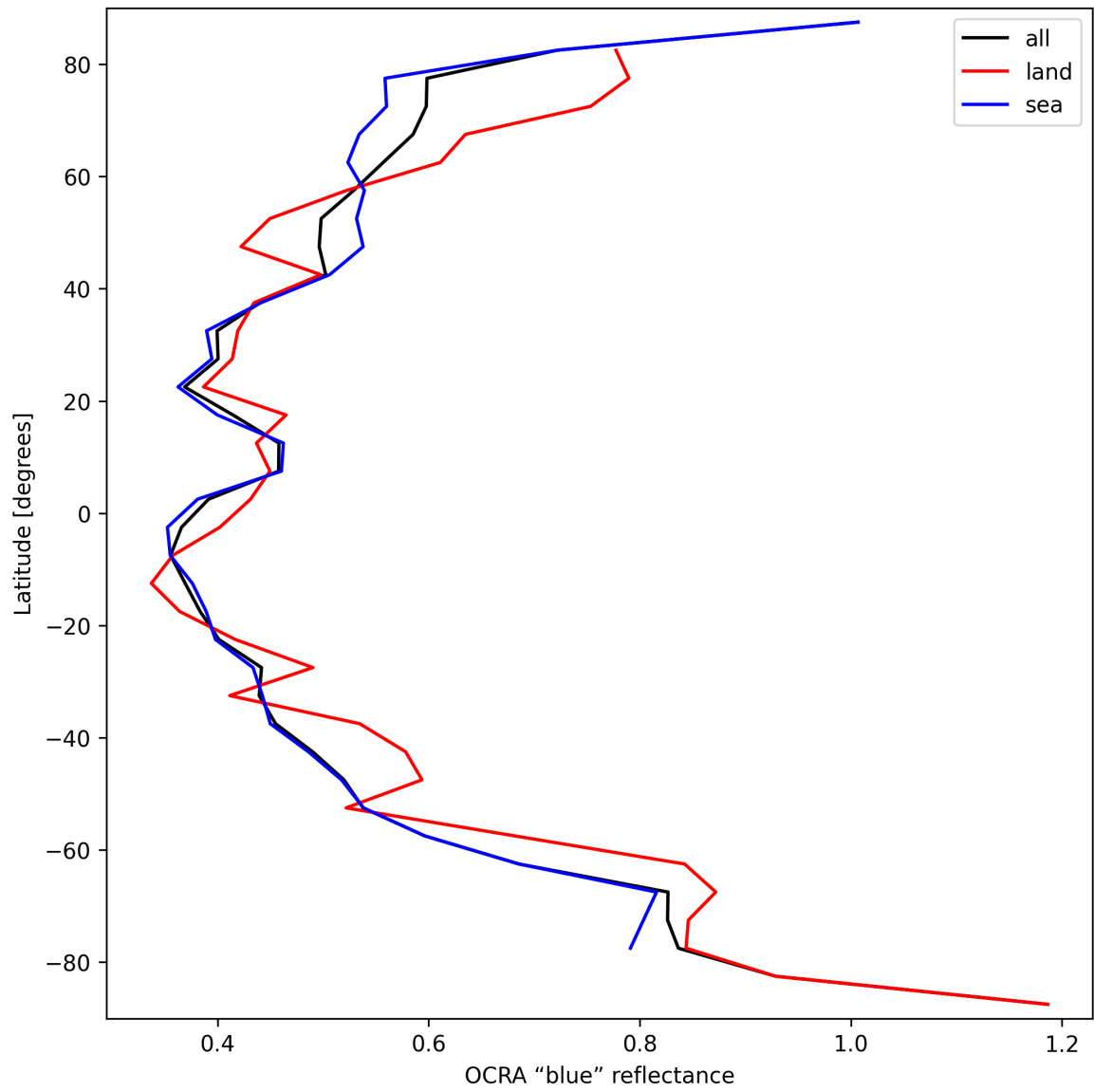
Figure 35: Zonal average of “OCRA “blue” reflectance” for 2024-09-19 to 2024-09-21.
