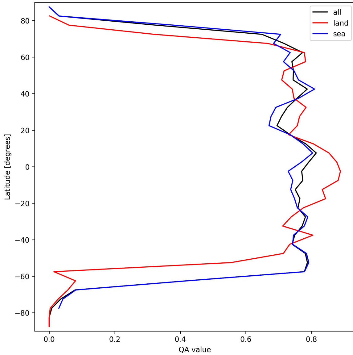
Figure 22: Zonal average of “QA value” for 2024-09-19 to 2024-09-21.
