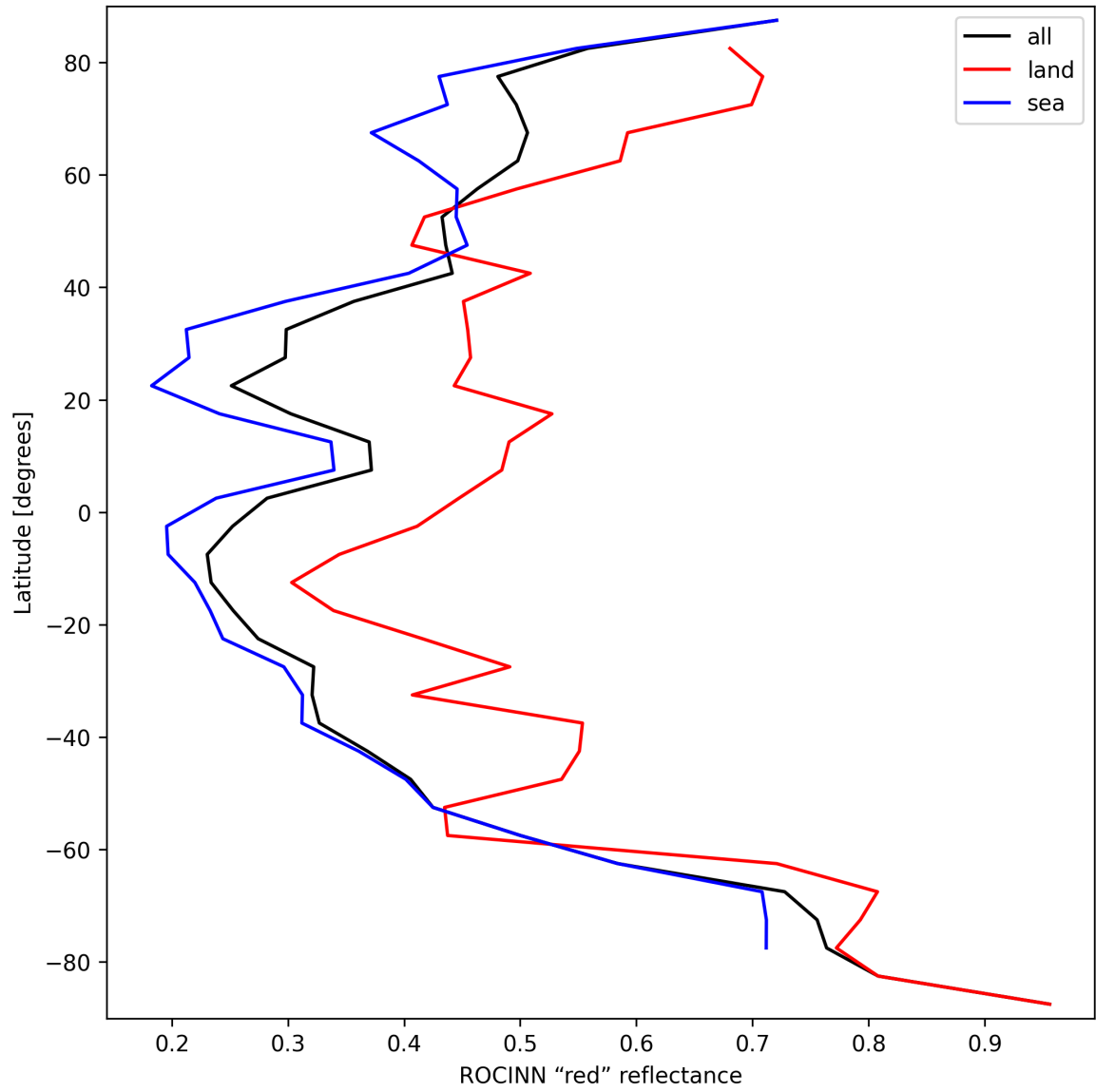
Figure 37: Zonal average of “ROCINN “red” reflectance” for 2024-09-19 to 2024-09-21.
