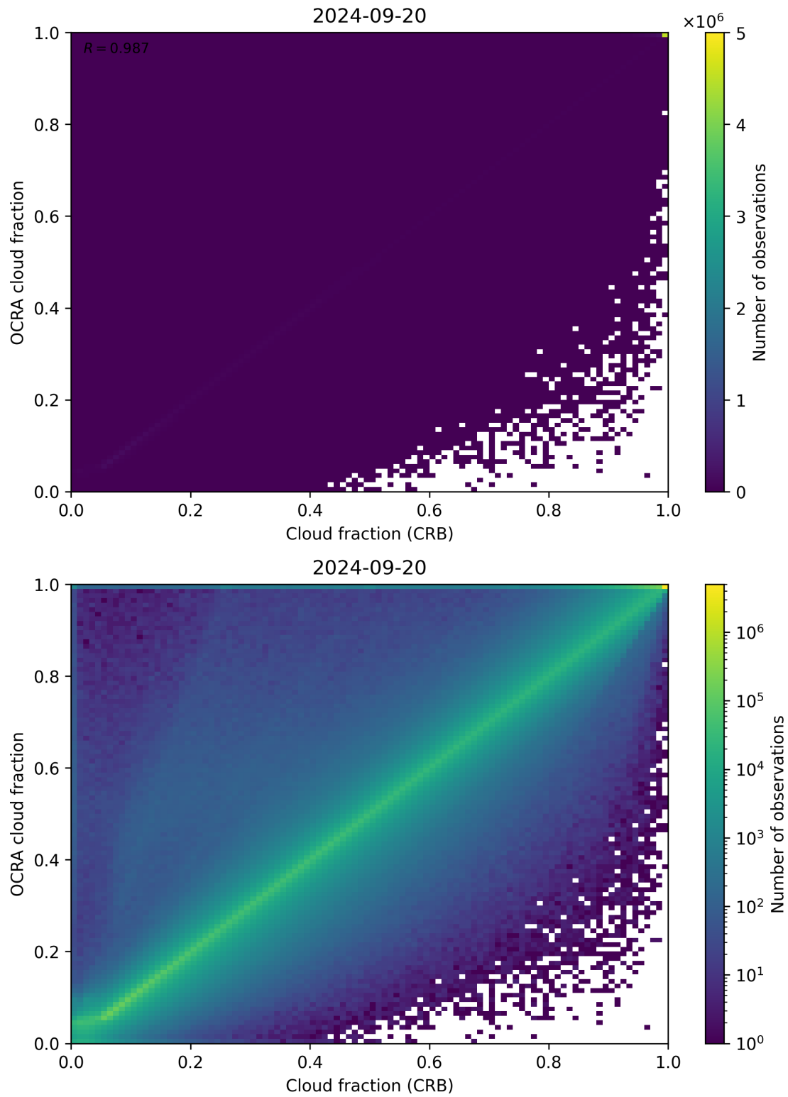
Figure 78: Scatter density plot of “Cloud fraction (CRB)” against “OCRA cloud fraction” for 2024-09-19 to 2024-09-21.
