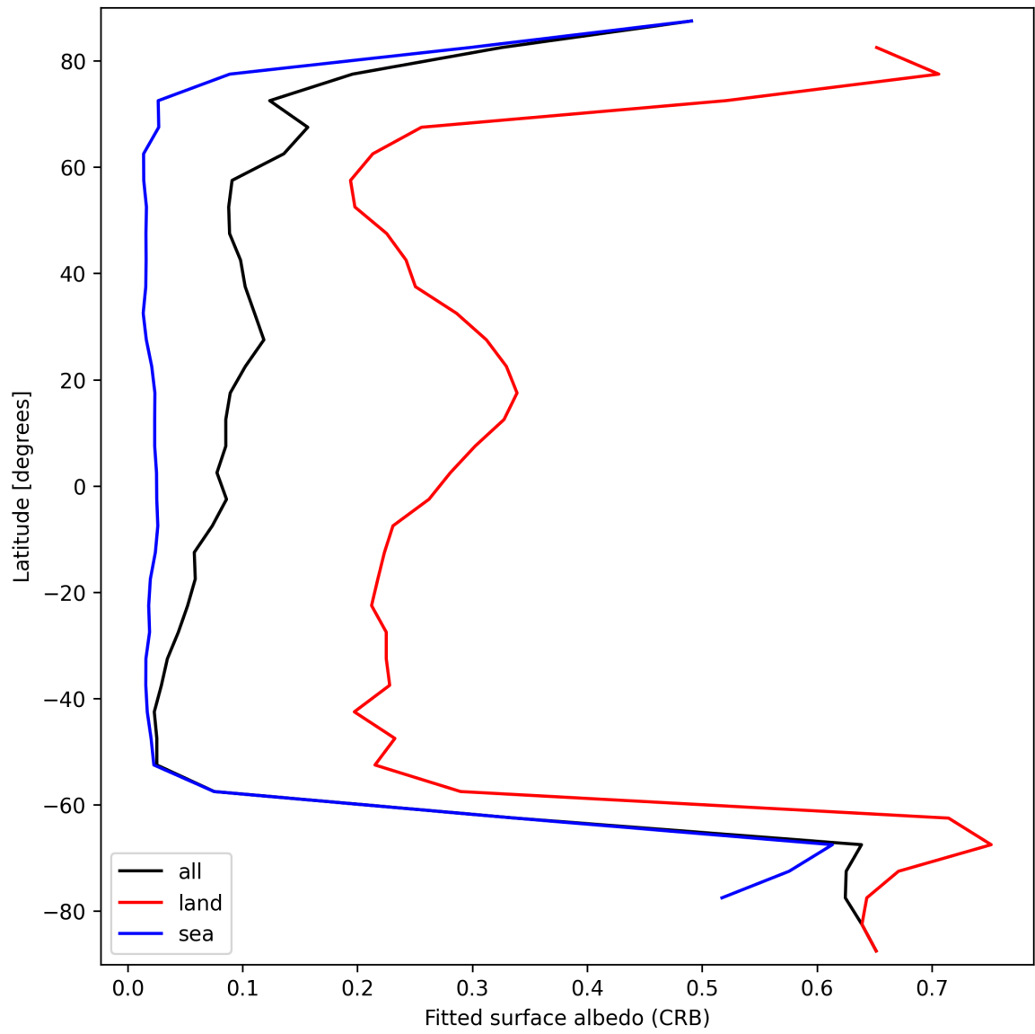
Figure 30: Zonal average of "Fitted surface albedo (CRB)" for 2024-09-19 to 2024-09-21.
