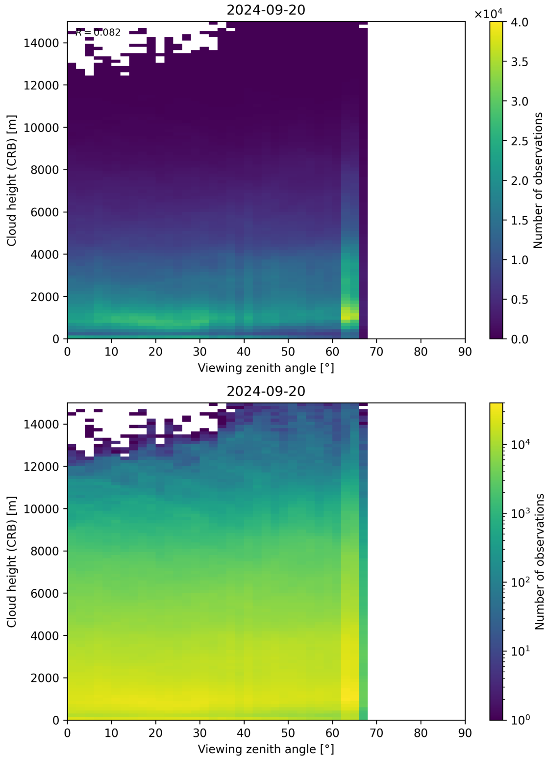
Figure 110: Scatter density plot of “Viewing zenith angle” against “Cloud height (CRB)” for 2024-09-19 to 2024-09-21.
