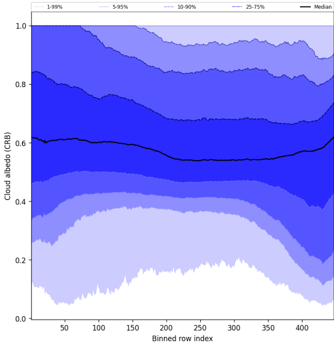
Figure 60: Along track statistics of “Cloud albedo (CRB)” for 2024-09-19 to 2024-09-21
