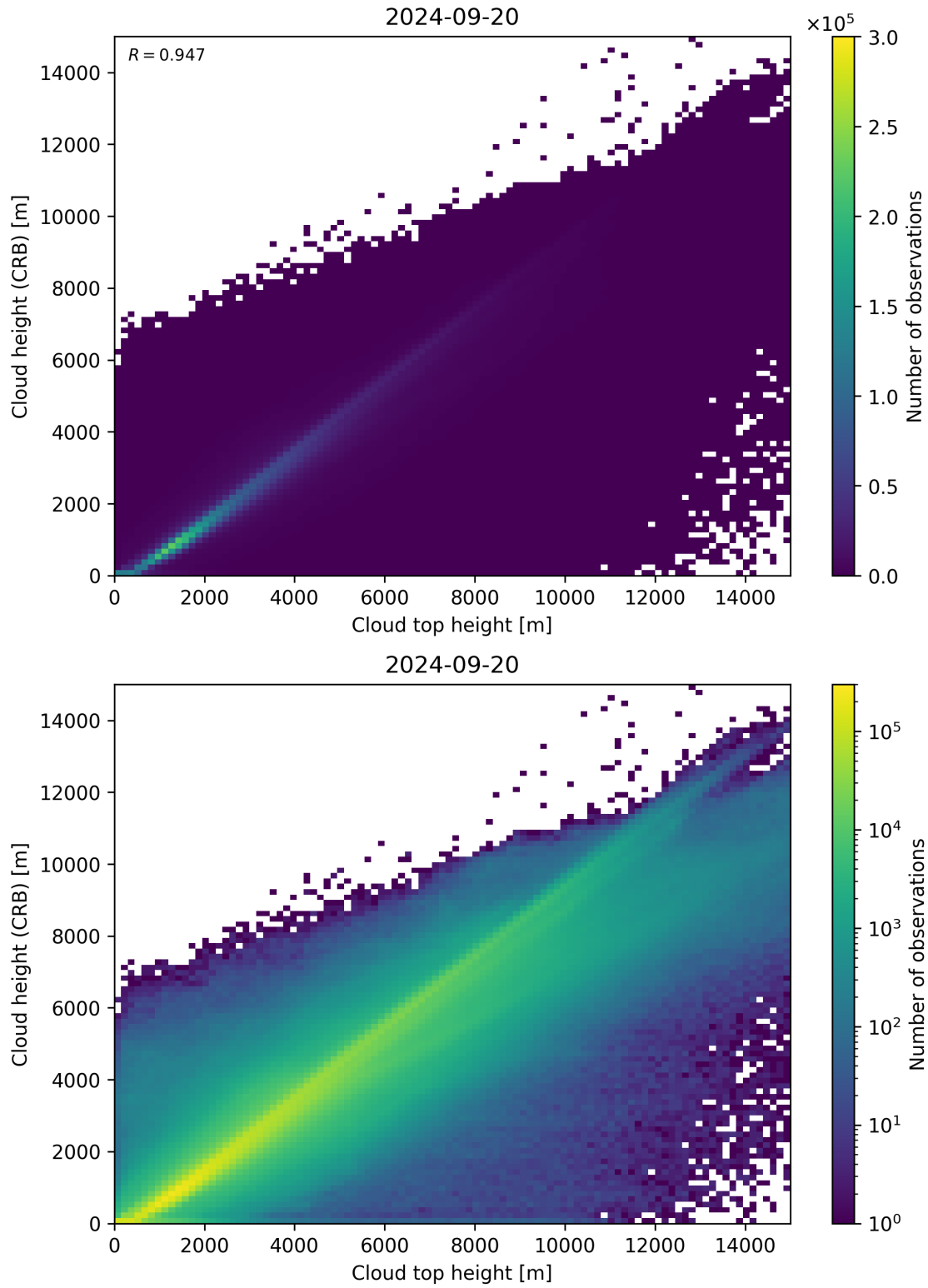
Figure 89: Scatter density plot of “Cloud top height” against “Cloud height (CRB)” for 2024-09-19 to 2024-09-21.
