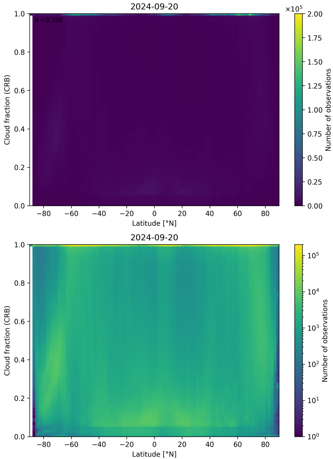
Figure 94: Scatter density plot of “Latitude” against “Cloud fraction (CRB)” for 2024-09-19 to 2024-09-21.
