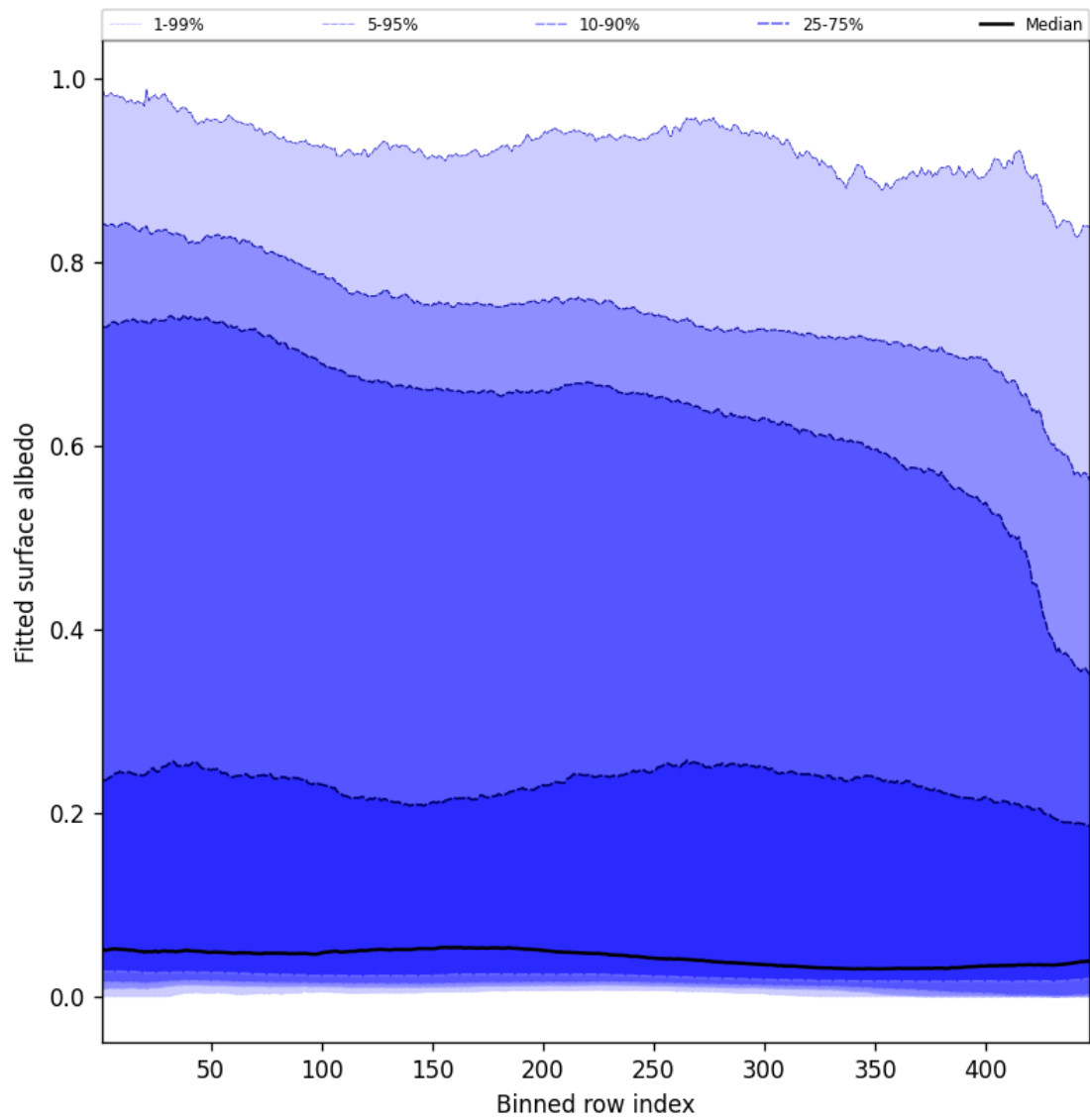
Figure 61: Along track statistics of “Fitted surface albedo” for 2024-09-19 to 2024-09-21
