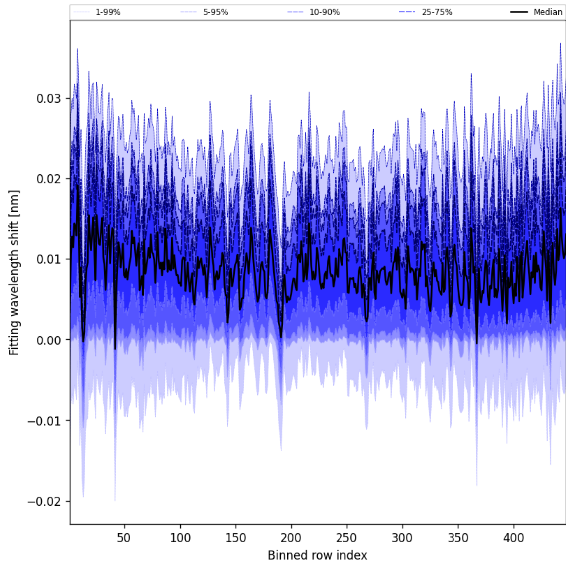
Figure 65: Along track statistics of “Fitting wavelength shift” for 2024-09-19 to 2024-09-21
