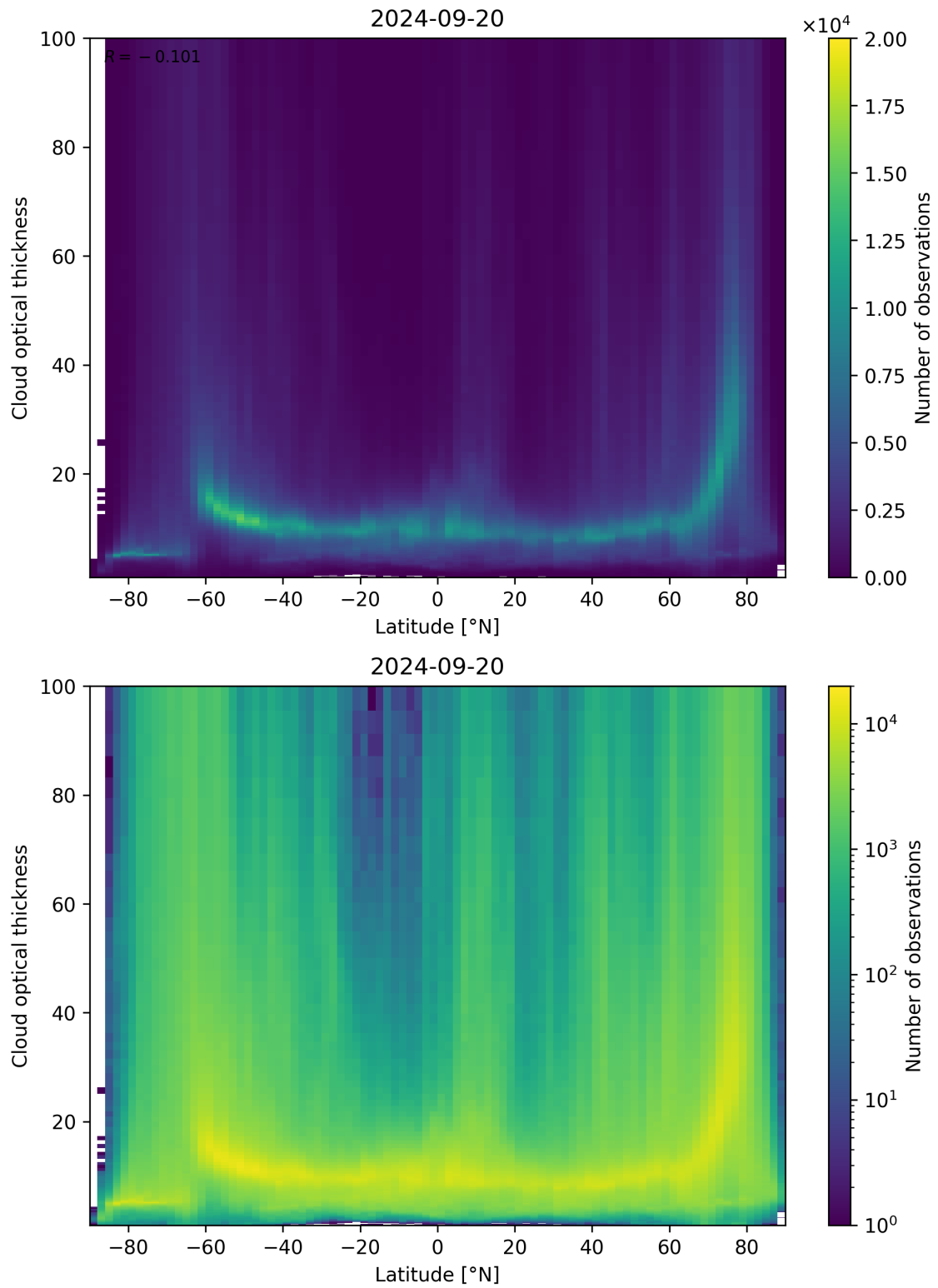
Figure 96: Scatter density plot of “Latitude” against “Cloud optical thickness” for 2024-09-19 to 2024-09-21.
