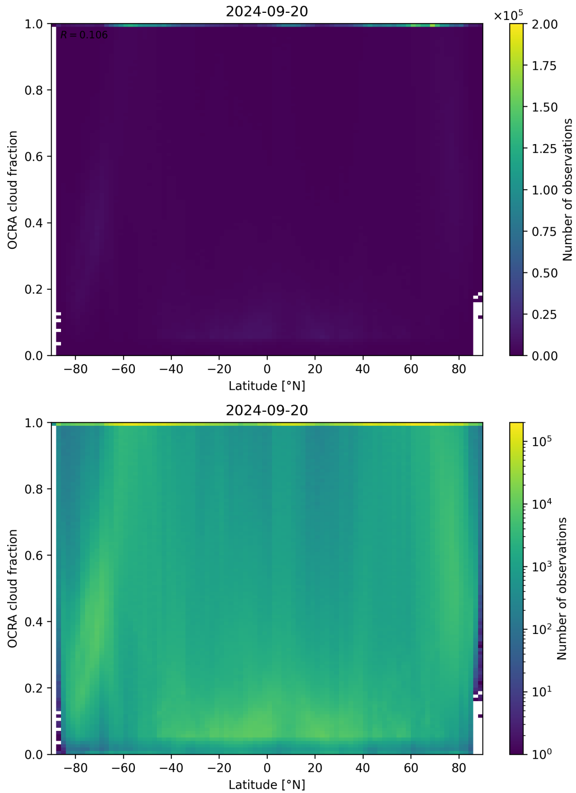
Figure 93: Scatter density plot of “Latitude” against “OCRA cloud fraction” for 2024-09-19 to 2024-09-21.
