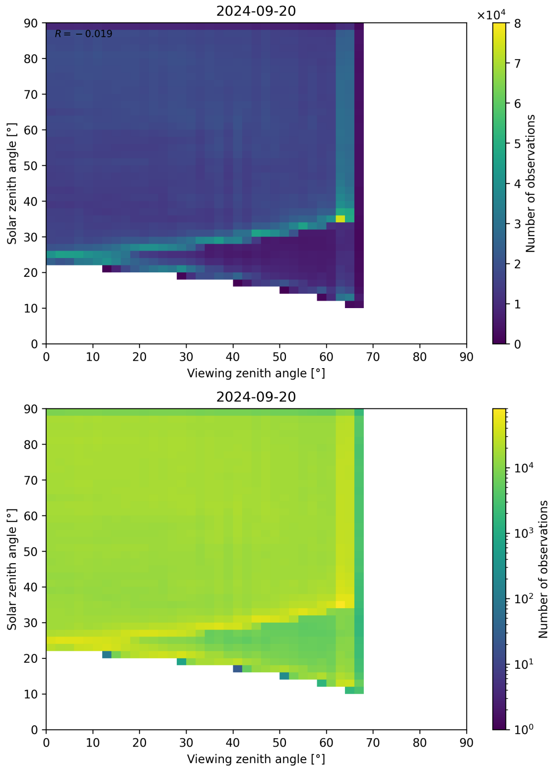
Figure 114: Scatter density plot of “Viewing zenith angle” against “Solar zenith angle” for 2024-09-19 to 2024-09-21.
