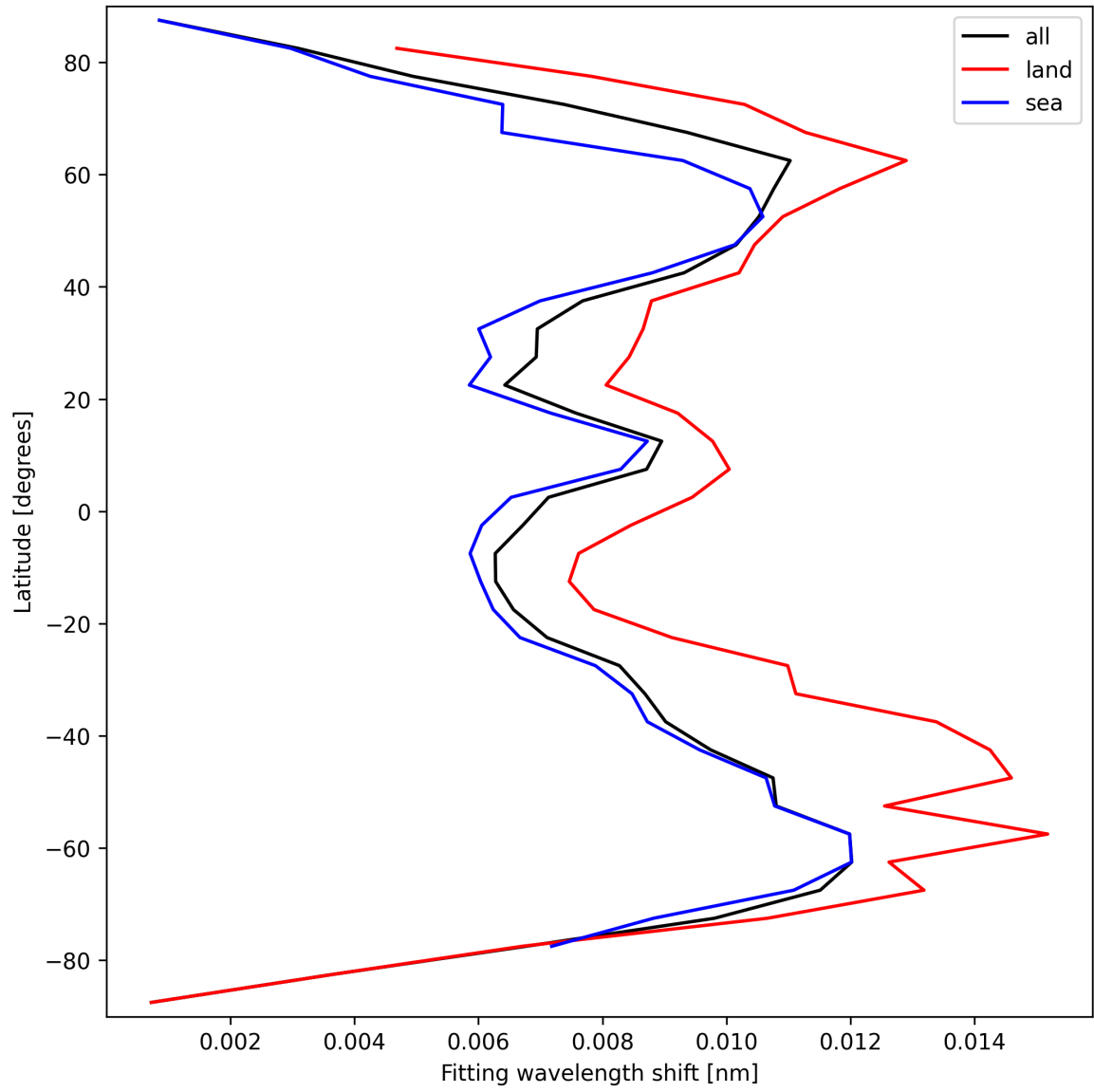
Figure 33: Zonal average of “Fitting wavelength shift” for 2024-09-19 to 2024-09-21.
