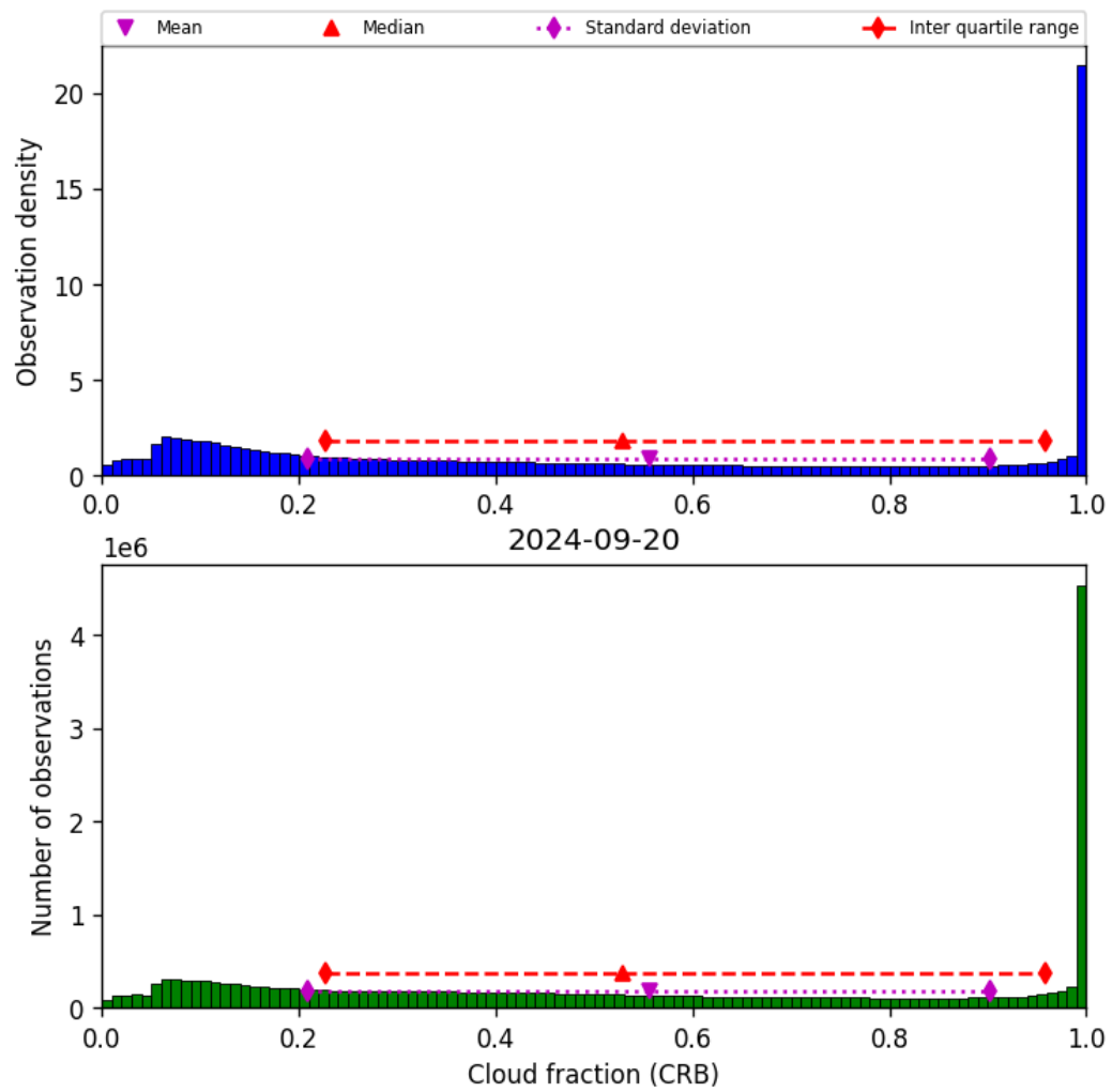
Figure 42: Histogram of “Cloud fraction (CRB)” for 2024-09-19 to 2024-09-21
