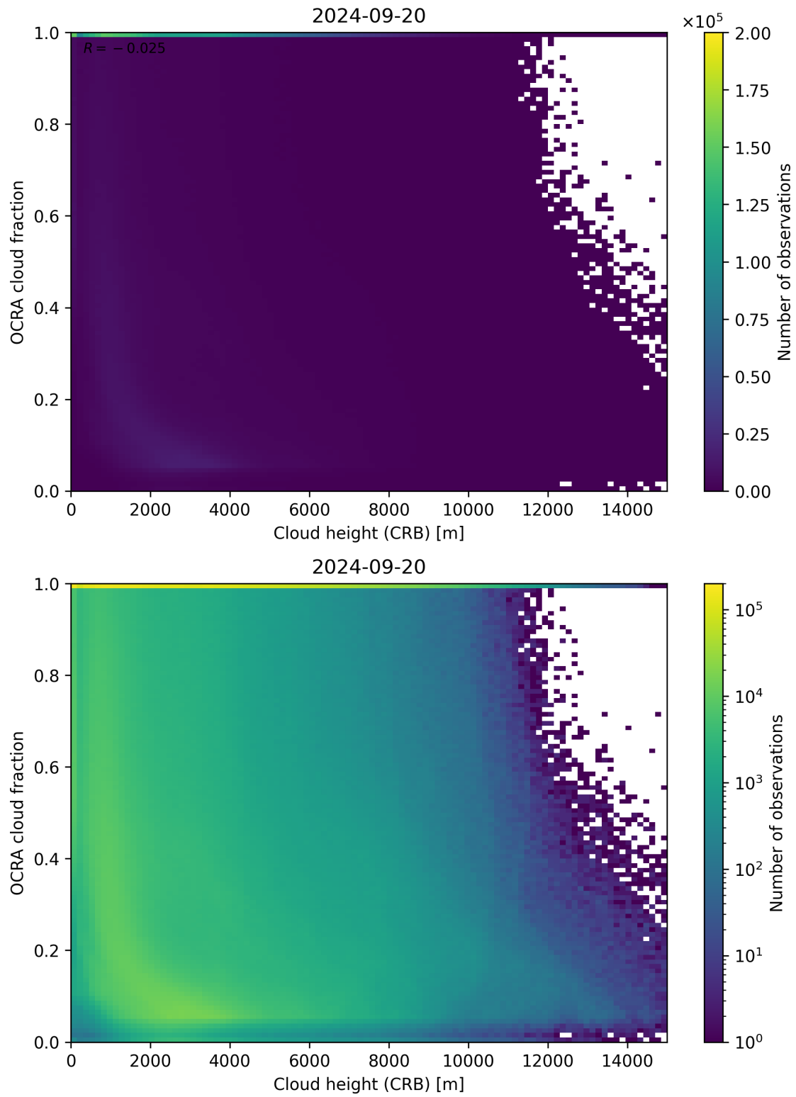
Figure 81: Scatter density plot of “Cloud height (CRB)” against “OCRA cloud fraction” for 2024-09-19 to 2024-09-21.
