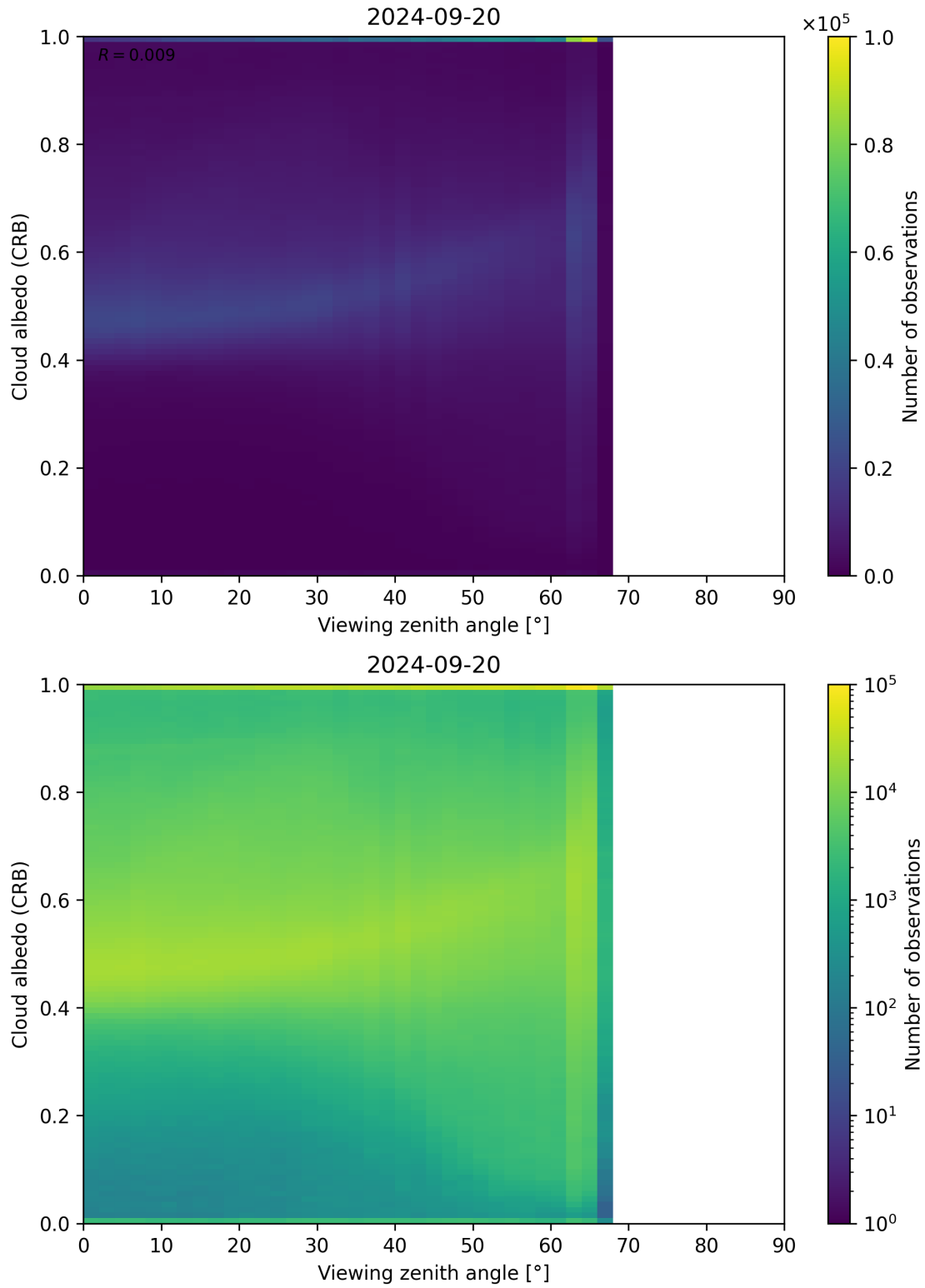
Figure 106: Scatter density plot of “Viewing zenith angle” against “Cloud albedo (CRB)” for 2024-09-19 to 2024-09-21.
