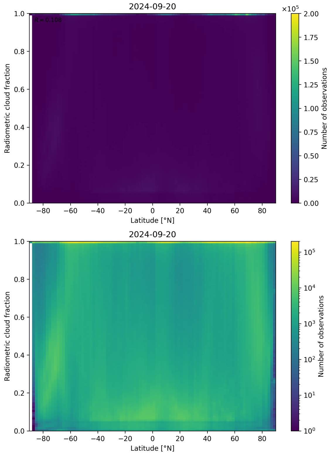
Figure 92: Scatter density plot of “Latitude” against “Radiometric cloud fraction” for 2024-09-19 to 2024-09-21.
