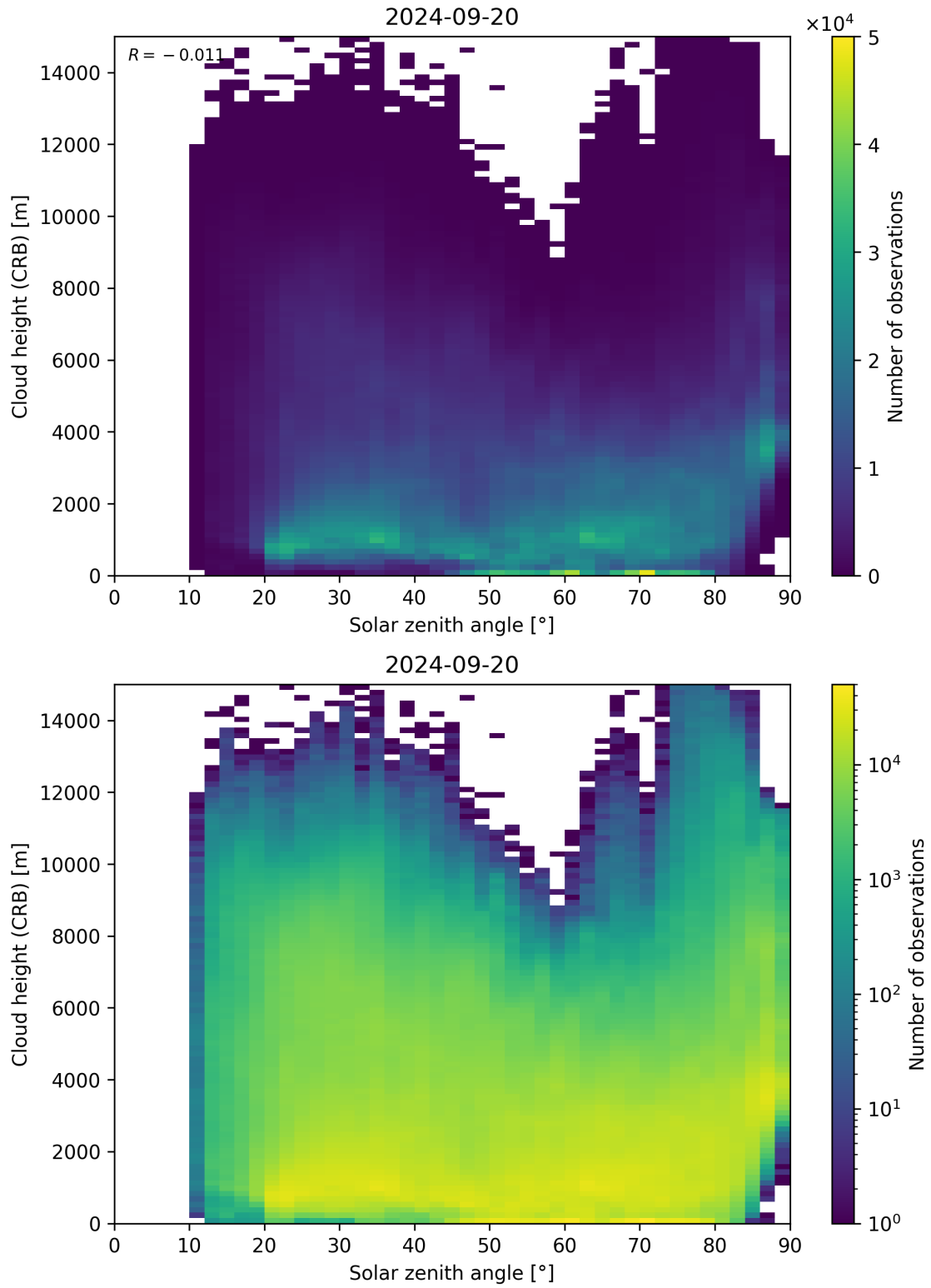
Figure 102: Scatter density plot of “Solar zenith angle” against “Cloud height (CRB)” for 2024-09-19 to 2024-09-21.
