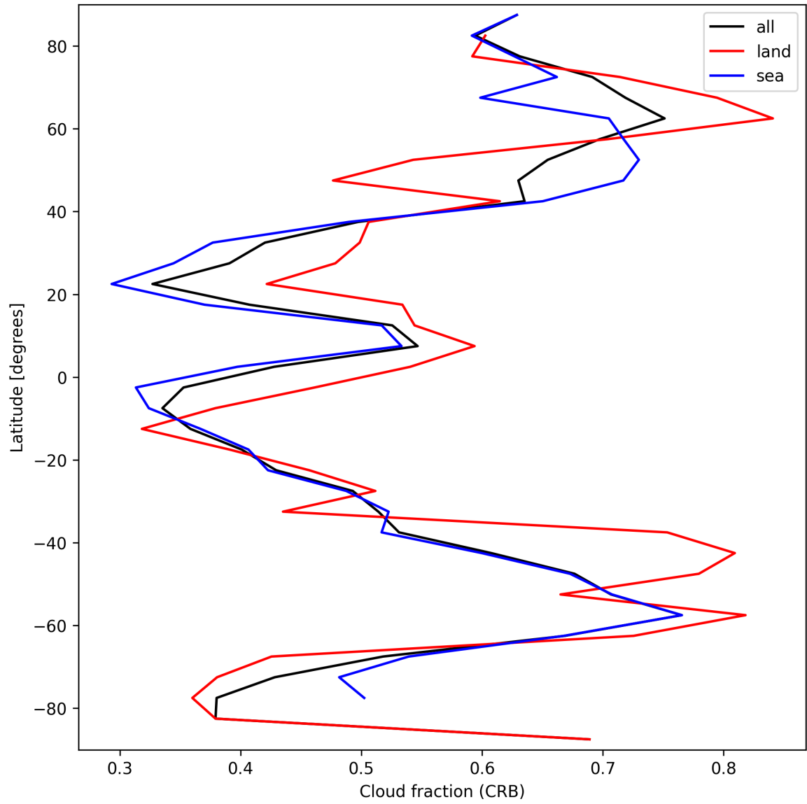
Figure 26: Zonal average of “Cloud fraction (CRB)” for 2024-09-19 to 2024-09-21.
