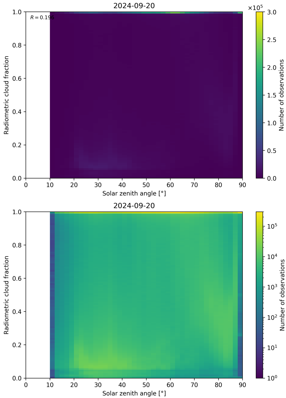
Figure 99: Scatter density plot of “Solar zenith angle” against “Radiometric cloud fraction” for 2024-09-19 to 2024-09-21.
