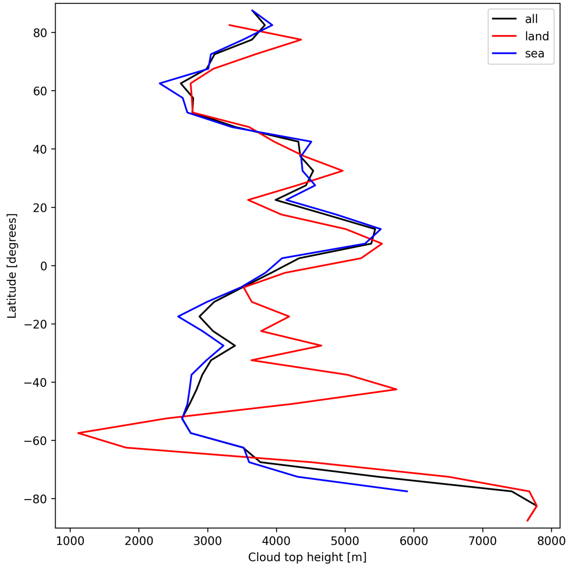
Figure 24: Zonal average of “Cloud top height” for 2024-09-19 to 2024-09-21.
