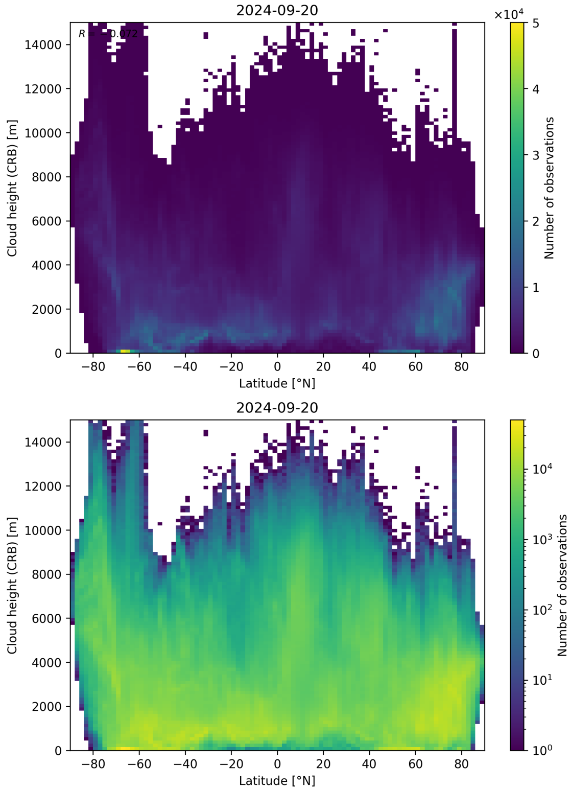
Figure 95: Scatter density plot of “Latitude” against “Cloud height (CRB)” for 2024-09-19 to 2024-09-21.
