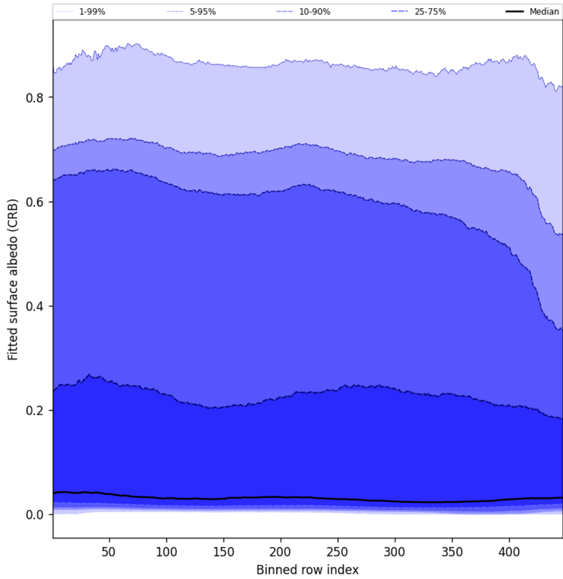
Figure 62: Along track statistics of “Fitted surface albedo (CRB)” for 2024-09-19 to 2024-09-21
