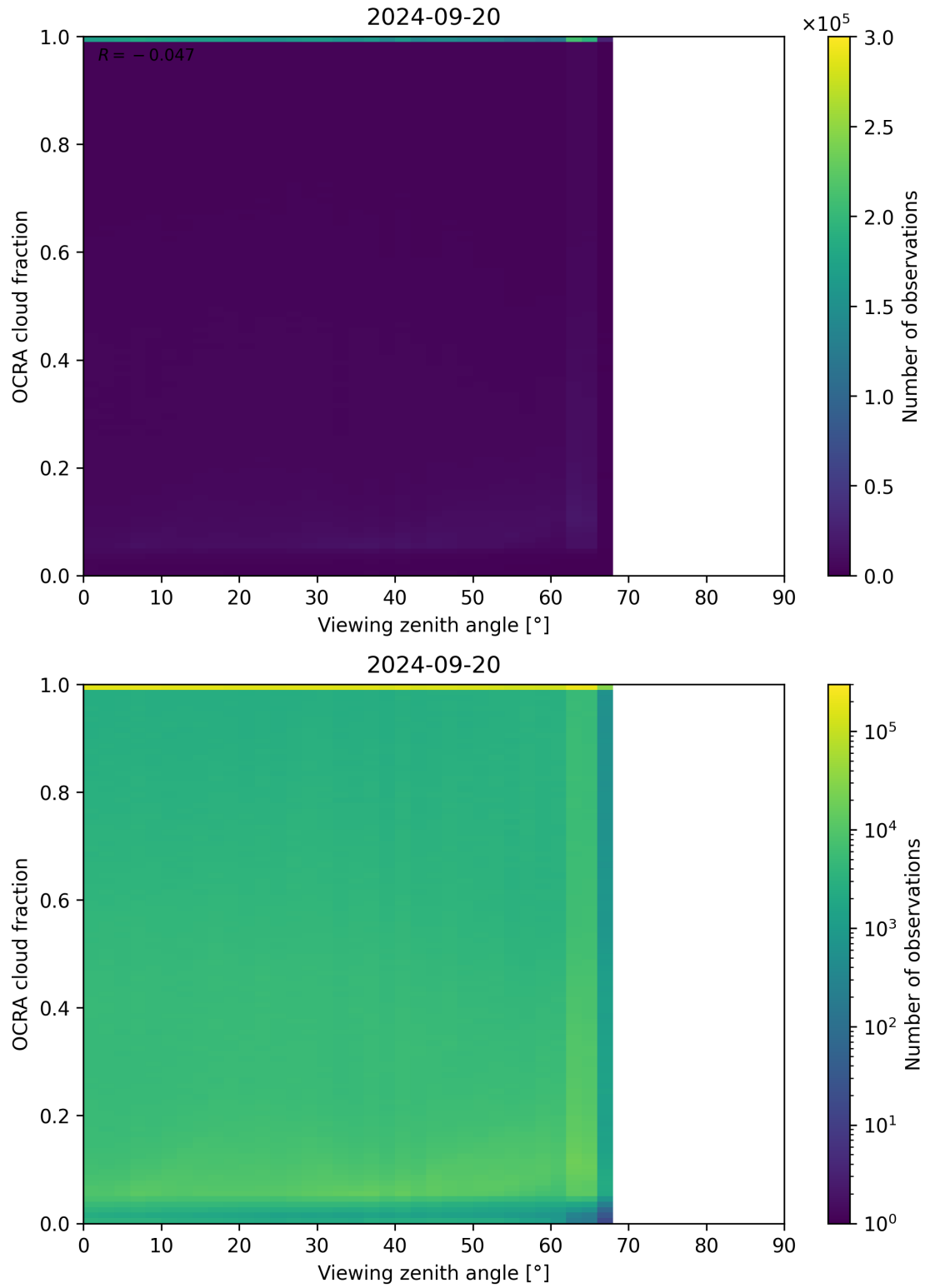
Figure 108: Scatter density plot of “Viewing zenith angle” against “OCRA cloud fraction” for 2024-09-19 to 2024-09-21.
