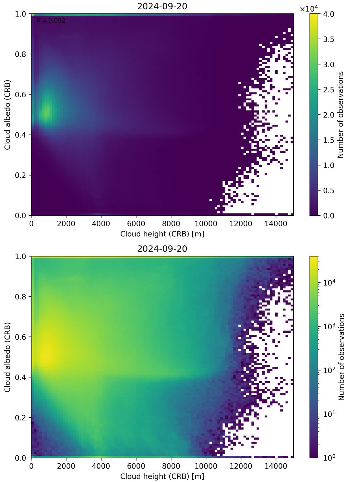
Figure 80: Scatter density plot of “Cloud height (CRB)” against “Cloud albedo (CRB)” for 2024-09-19 to 2024-09-21.
