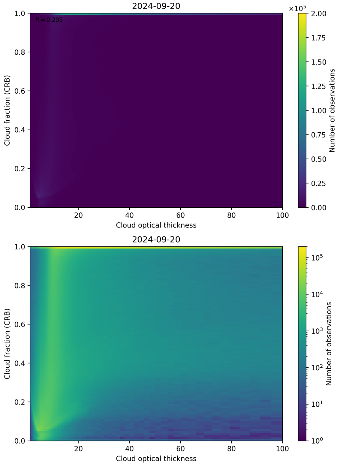
Figure 84: Scatter density plot of “Cloud optical thickness” against “Cloud fraction (CRB)” for 2024-09-19 to 2024-09-21.
