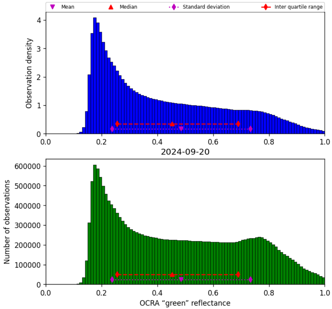
Figure 52: Histogram of “OCRA “green” reflectance” for 2024-09-19 to 2024-09-21
