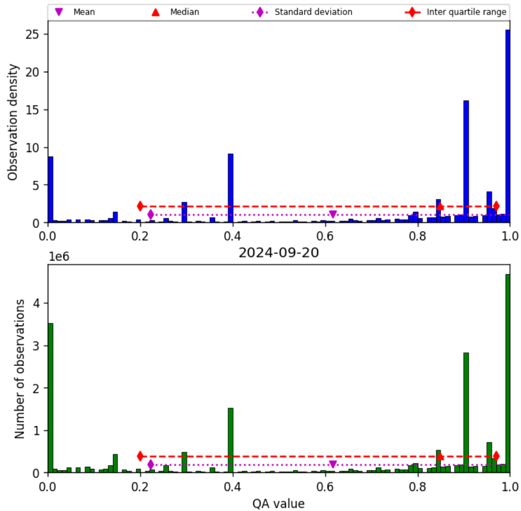
Figure 38: Histogram of “QA value” for 2024-09-19 to 2024-09-21
