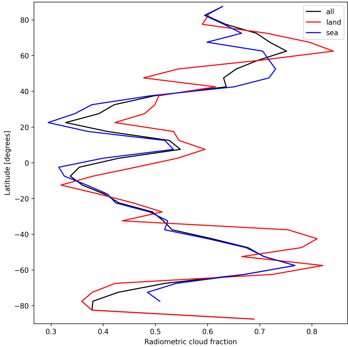
Figure 23: Zonal average of “Radiometric cloud fraction” for 2024-09-19 to 2024-09-21.
