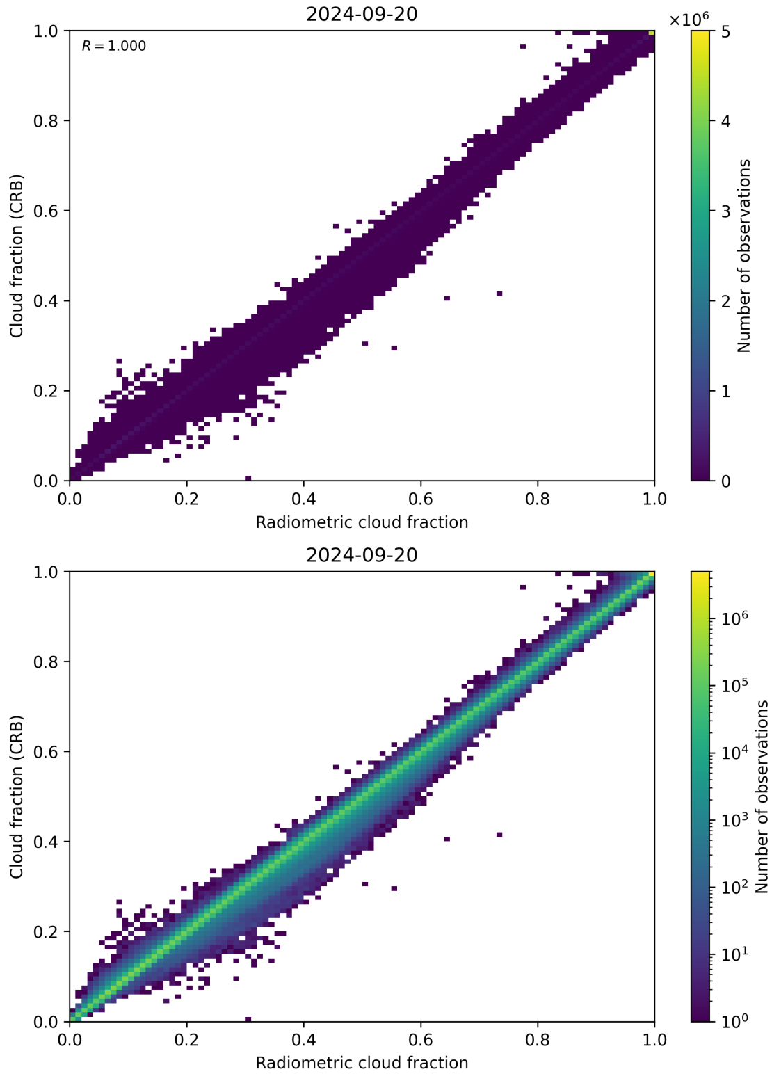
Figure 73: Scatter density plot of “Radiometric cloud fraction” against “Cloud fraction (CRB)” for 2024-09-19 to 2024-09-21.
