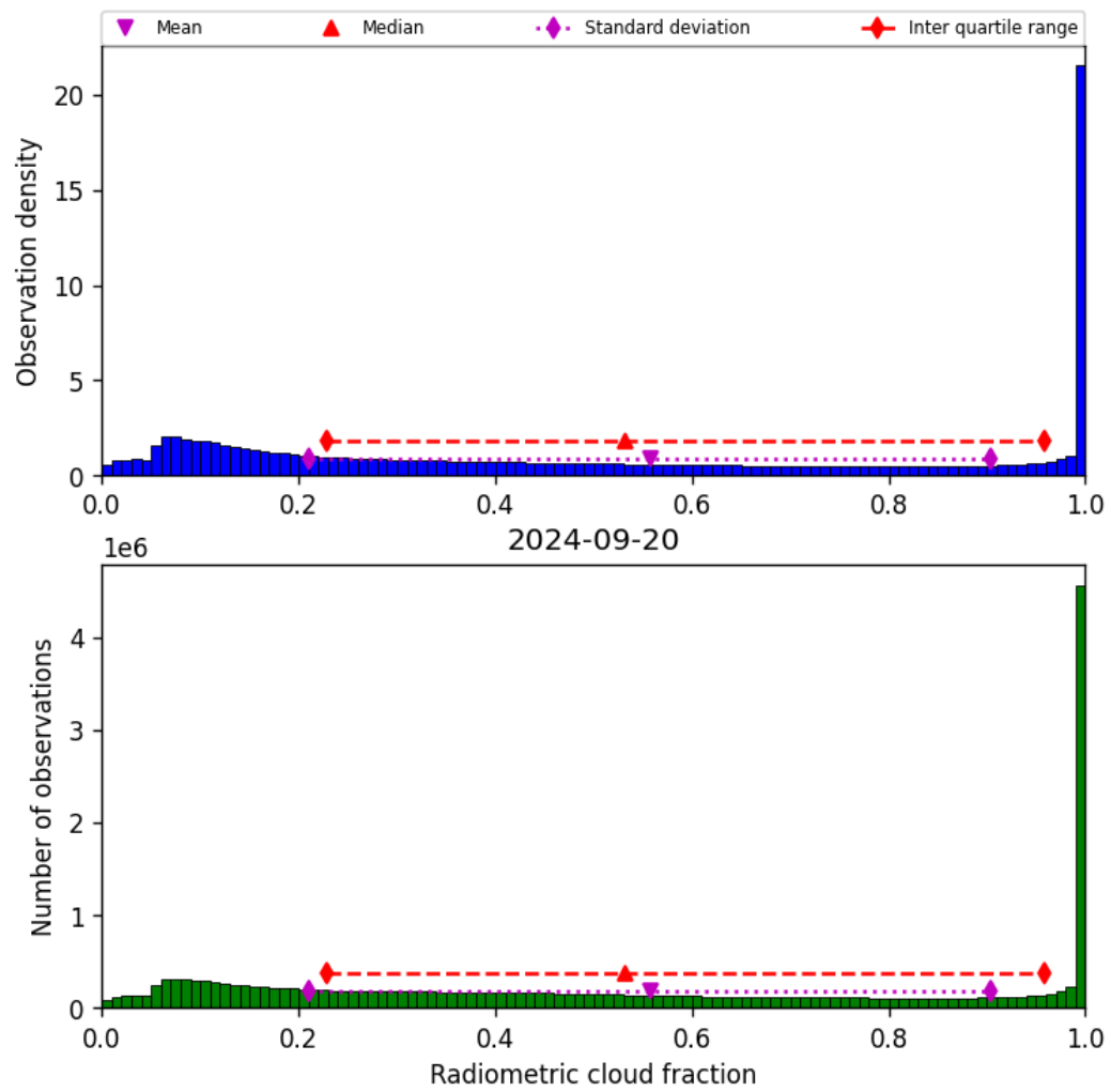
Figure 39: Histogram of “Radiometric cloud fraction” for 2024-09-19 to 2024-09-21
