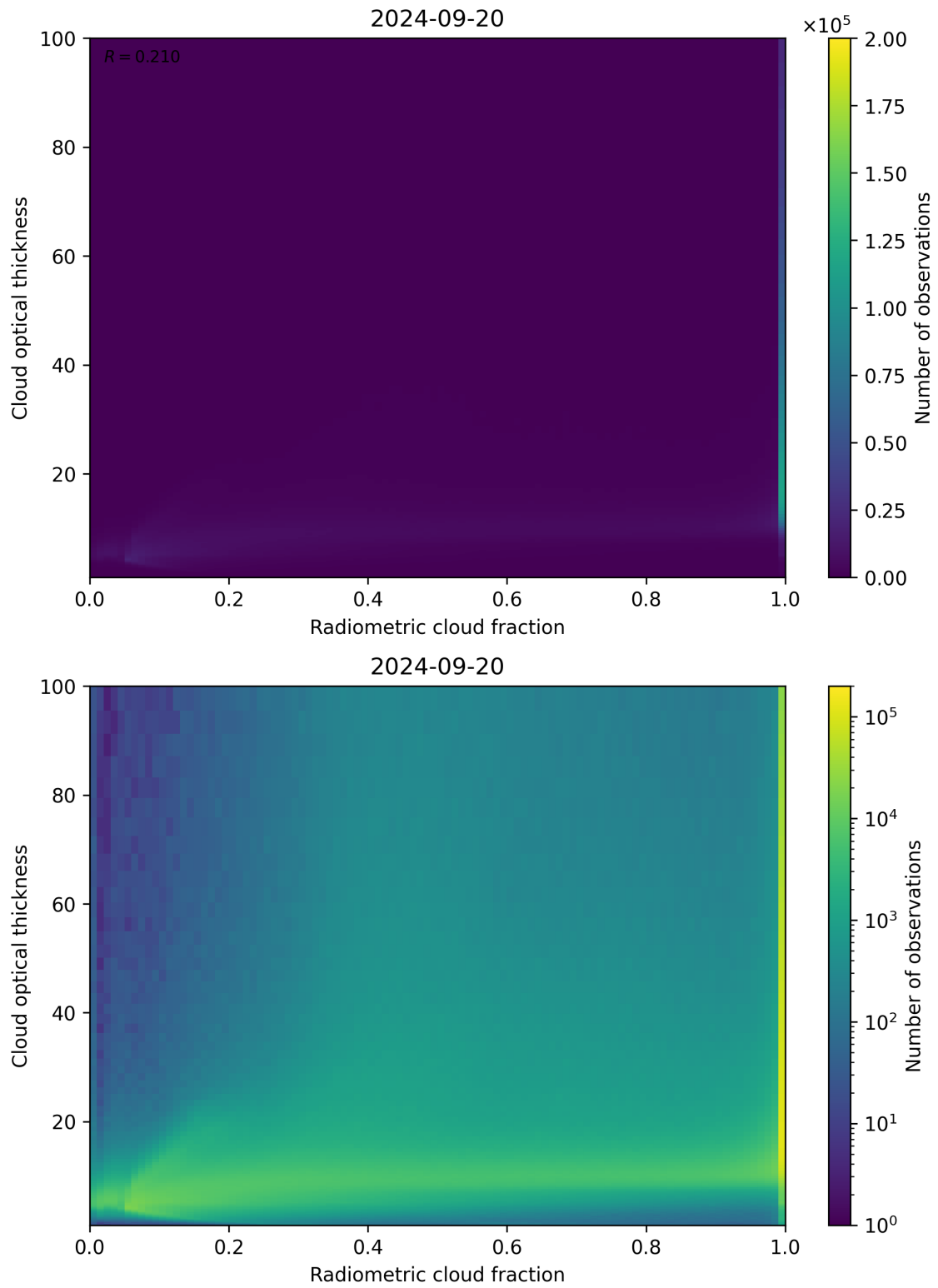
Figure 75: Scatter density plot of “Radiometric cloud fraction” against “Cloud optical thickness” for 2024-09-19 to 2024-09-21.
