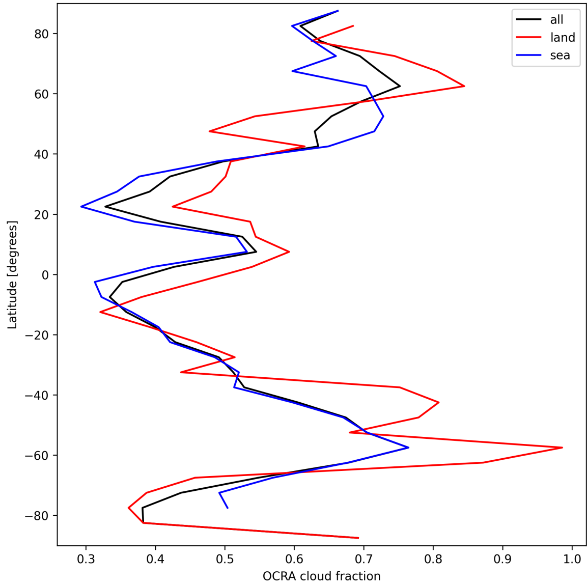
Figure 34: Zonal average of “OCRA cloud fraction” for 2024-09-19 to 2024-09-21.
