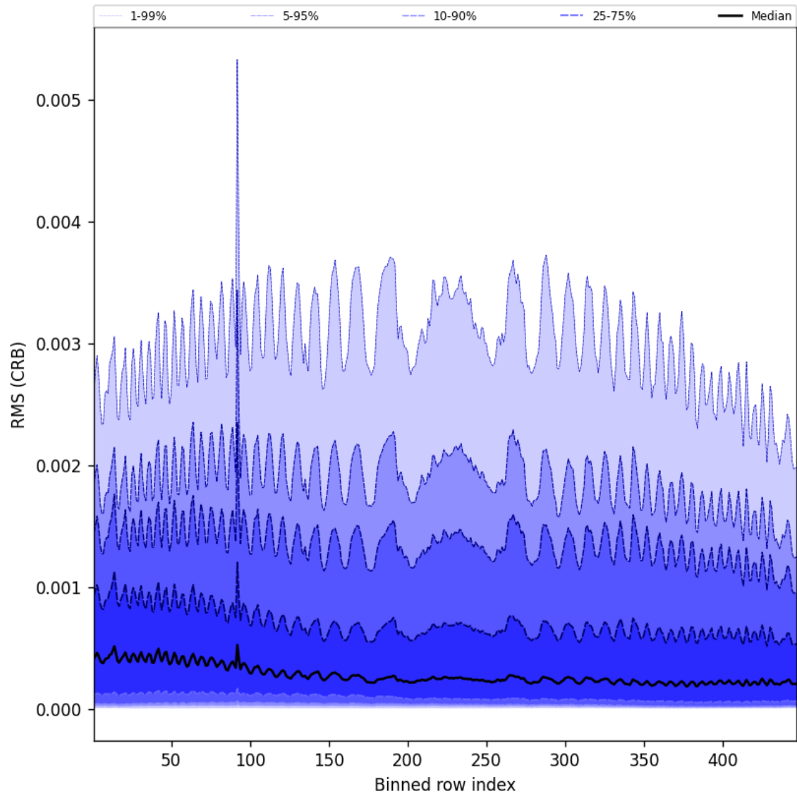
Figure 64: Along track statistics of “RMS (CRB)” for 2024-09-19 to 2024-09-21
