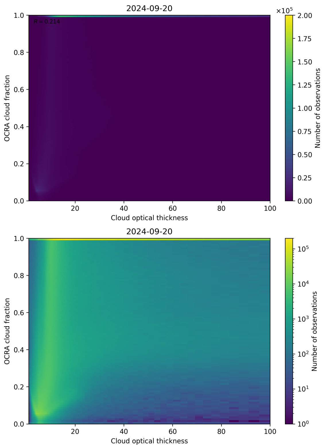
Figure 83: Scatter density plot of “Cloud optical thickness” against “OCRA cloud fraction” for 2024-09-19 to 2024-09-21.
