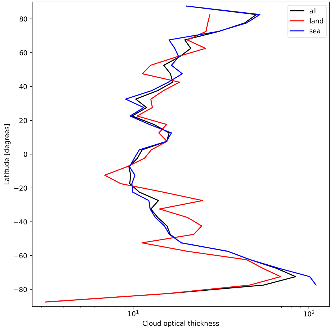
Figure 25: Zonal average of “Cloud optical thickness” for 2024-09-19 to 2024-09-21.
