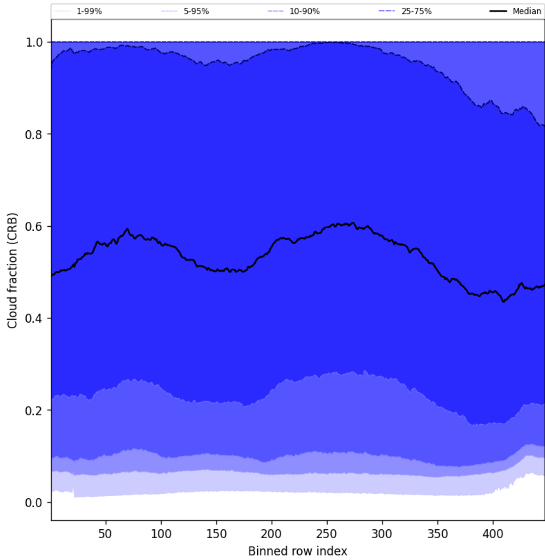
Figure 58: Along track statistics of “Cloud fraction (CRB)” for 2024-09-19 to 2024-09-21
