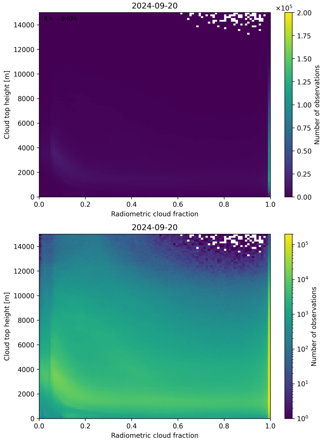
Figure 76: Scatter density plot of “Radiometric cloud fraction” against “Cloud top height” for 2024-09-19 to 2024-09-21.
