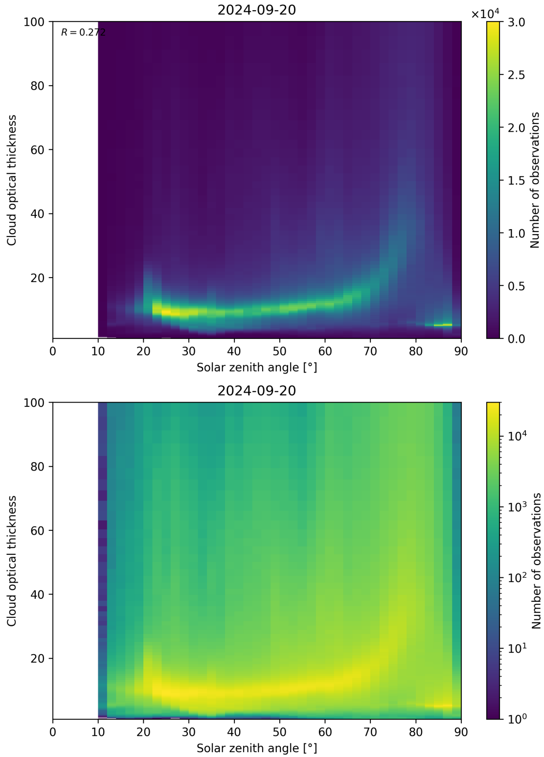
Figure 103: Scatter density plot of “Solar zenith angle” against “Cloud optical thickness” for 2024-09-19 to 2024-09-21.
