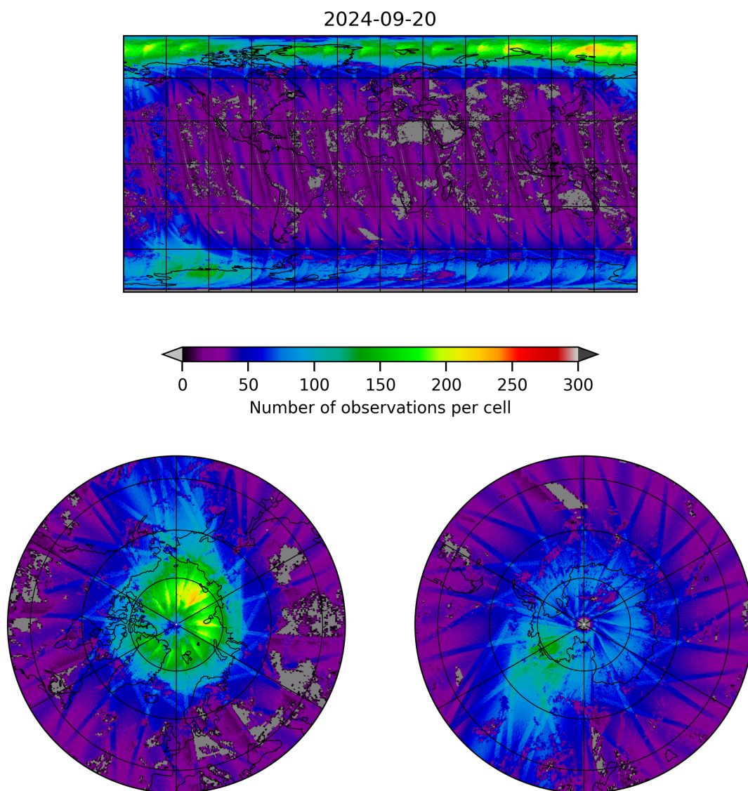
Figure 21: Map of the number of observations for 2024-09-19 to 2024-09-21
