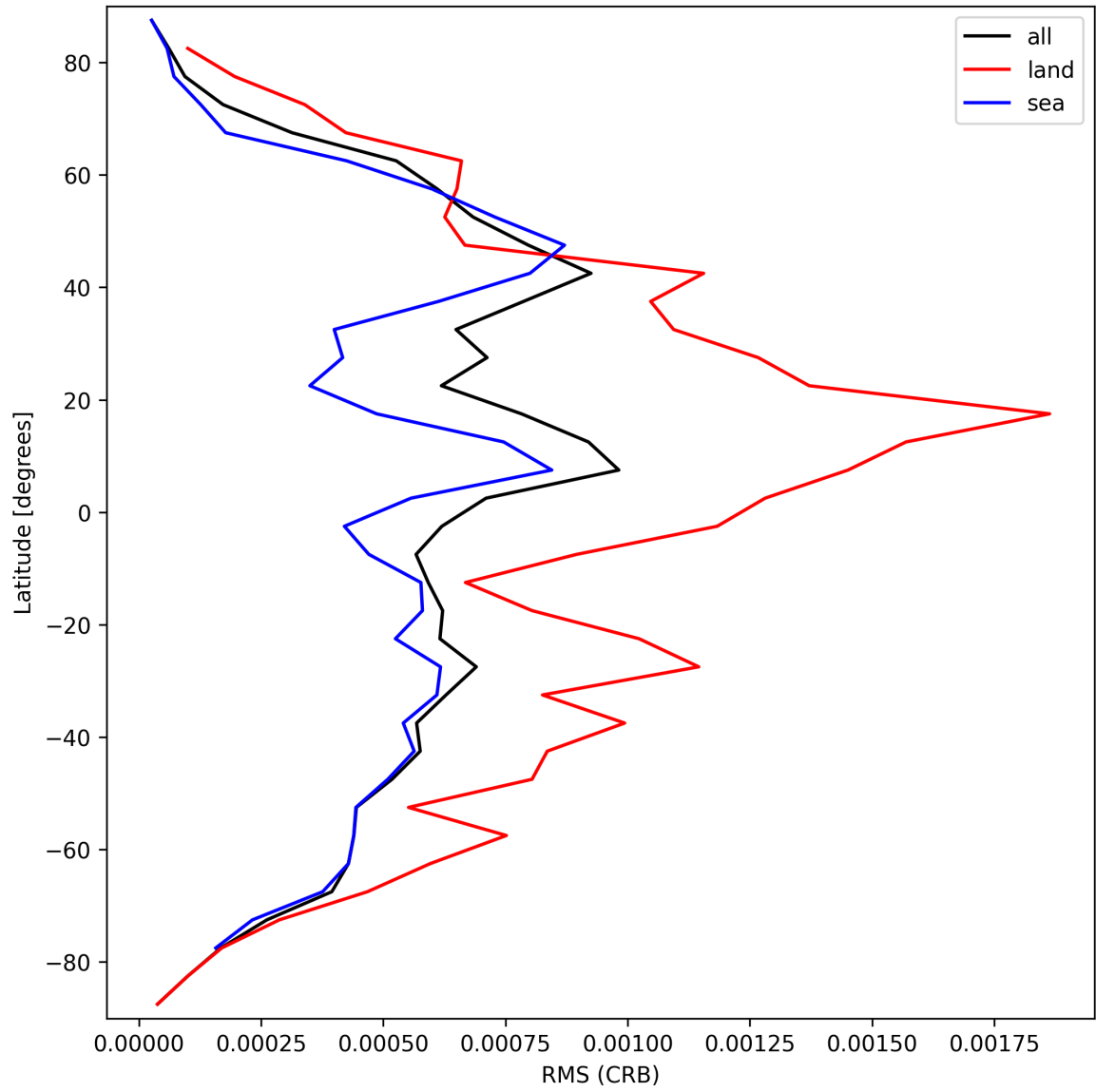
Figure 32: Zonal average of “RMS (CRB)” for 2024-09-19 to 2024-09-21.
