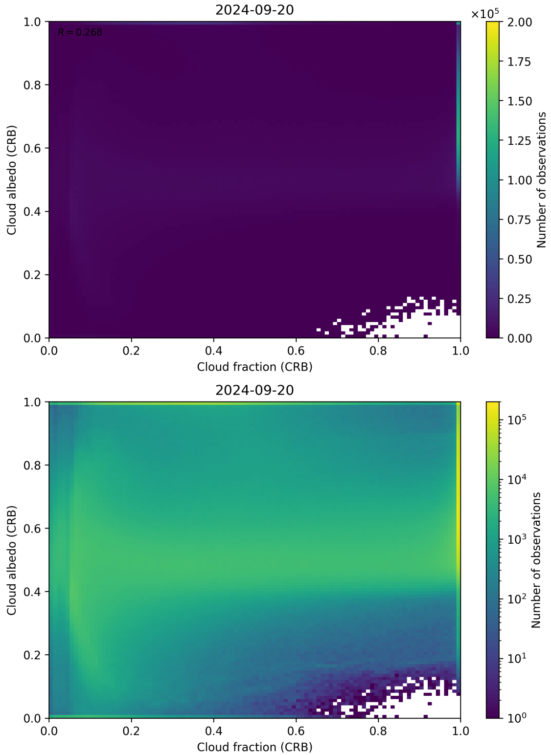
Figure 77: Scatter density plot of “Cloud fraction (CRB)” against “Cloud albedo (CRB)” for 2024-09-19 to 2024-09-21.
