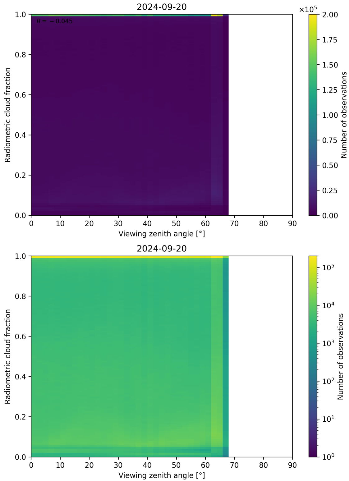
Figure 107: Scatter density plot of “Viewing zenith angle” against “Radiometric cloud fraction” for 2024-09-19 to 2024-09-21.
