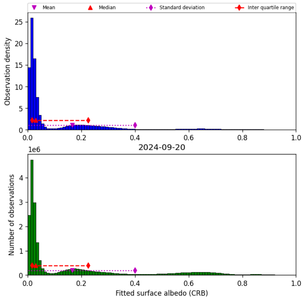
Figure 46: Histogram of “Fitted surface albedo (CRB)” for 2024-09-19 to 2024-09-21
