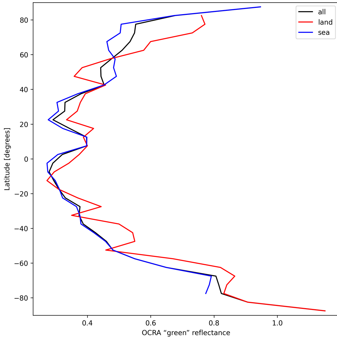
Figure 36: Zonal average of “OCRA “green” reflectance” for 2024-09-19 to 2024-09-21.
