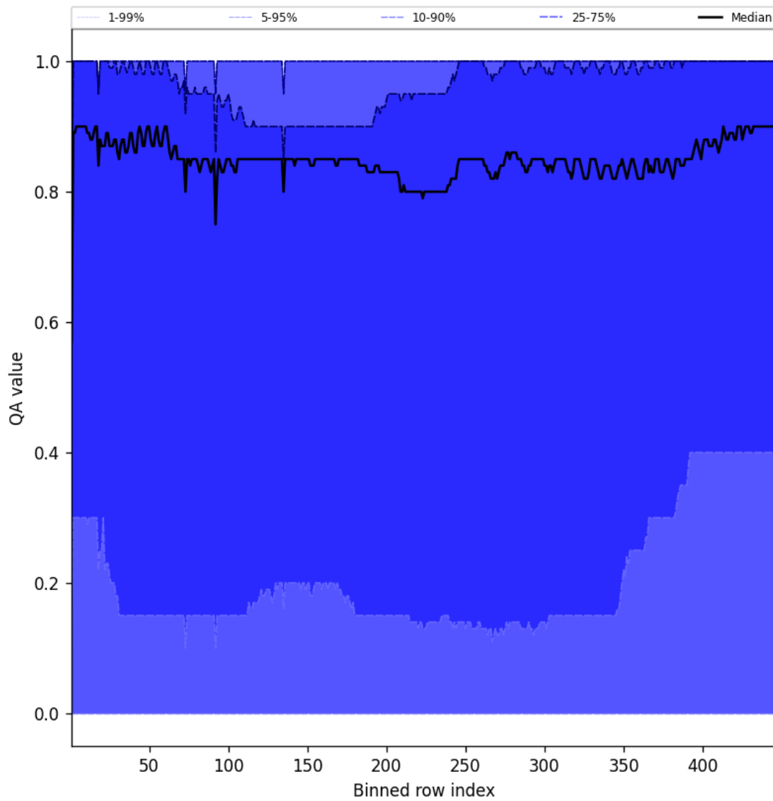
Figure 54: Along track statistics of “QA value” for 2024-09-19 to 2024-09-21
