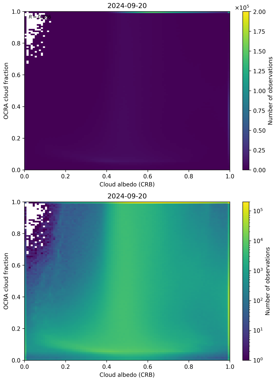
Figure 70: Scatter density plot of “Cloud albedo (CRB)” against “OCRA cloud fraction” for 2024-09-19 to 2024-09-21.
