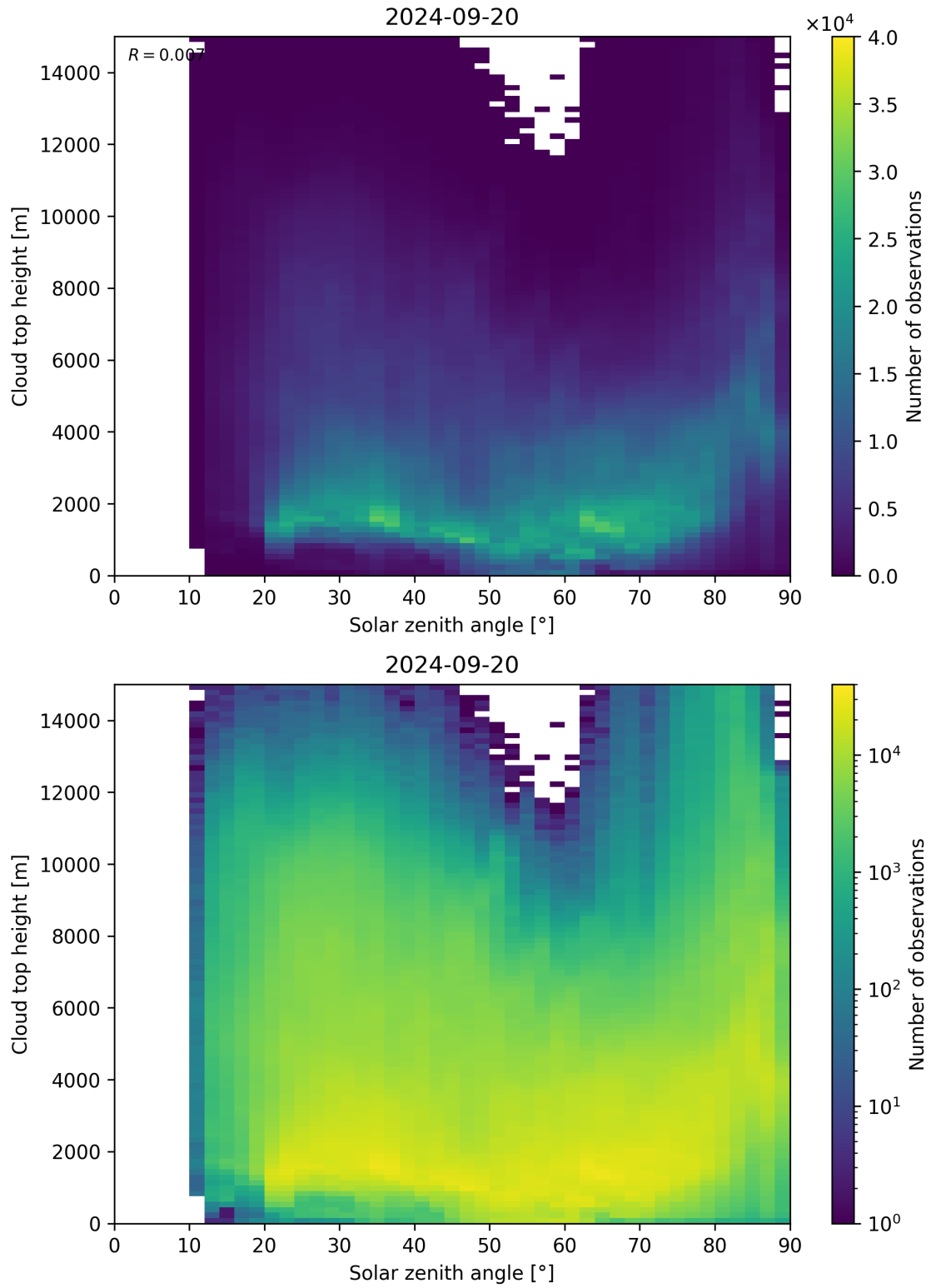
Figure 104: Scatter density plot of “Solar zenith angle” against “Cloud top height” for 2024-09-19 to 2024-09-21.
