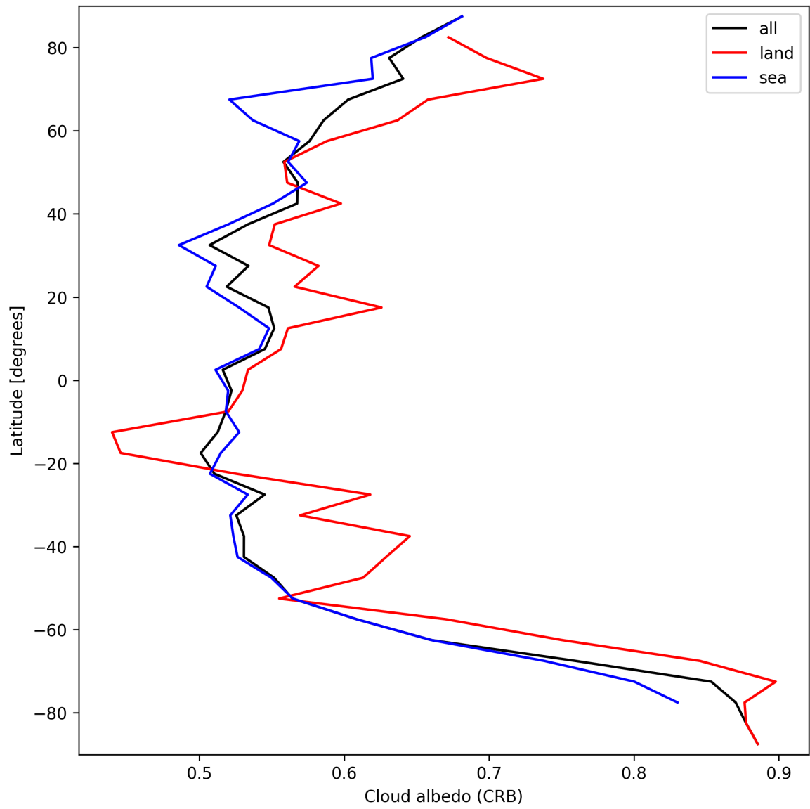
Figure 28: Zonal average of “Cloud albedo (CRB)” for 2024-09-19 to 2024-09-21.
