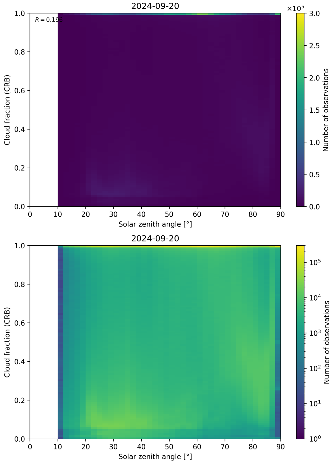
Figure 101: Scatter density plot of “Solar zenith angle” against “Cloud fraction (CRB)” for 2024-09-19 to 2024-09-21.
