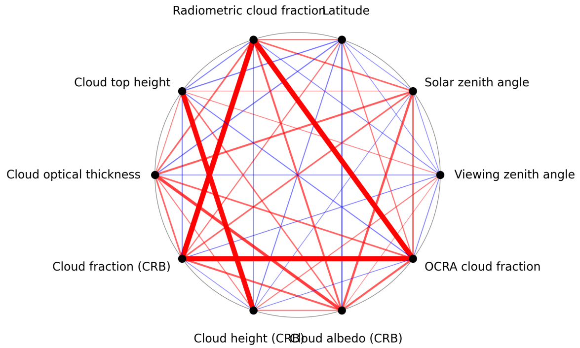
Figure 1: Map of correlation graph for 2024-09-19 to 2024-09-21.
