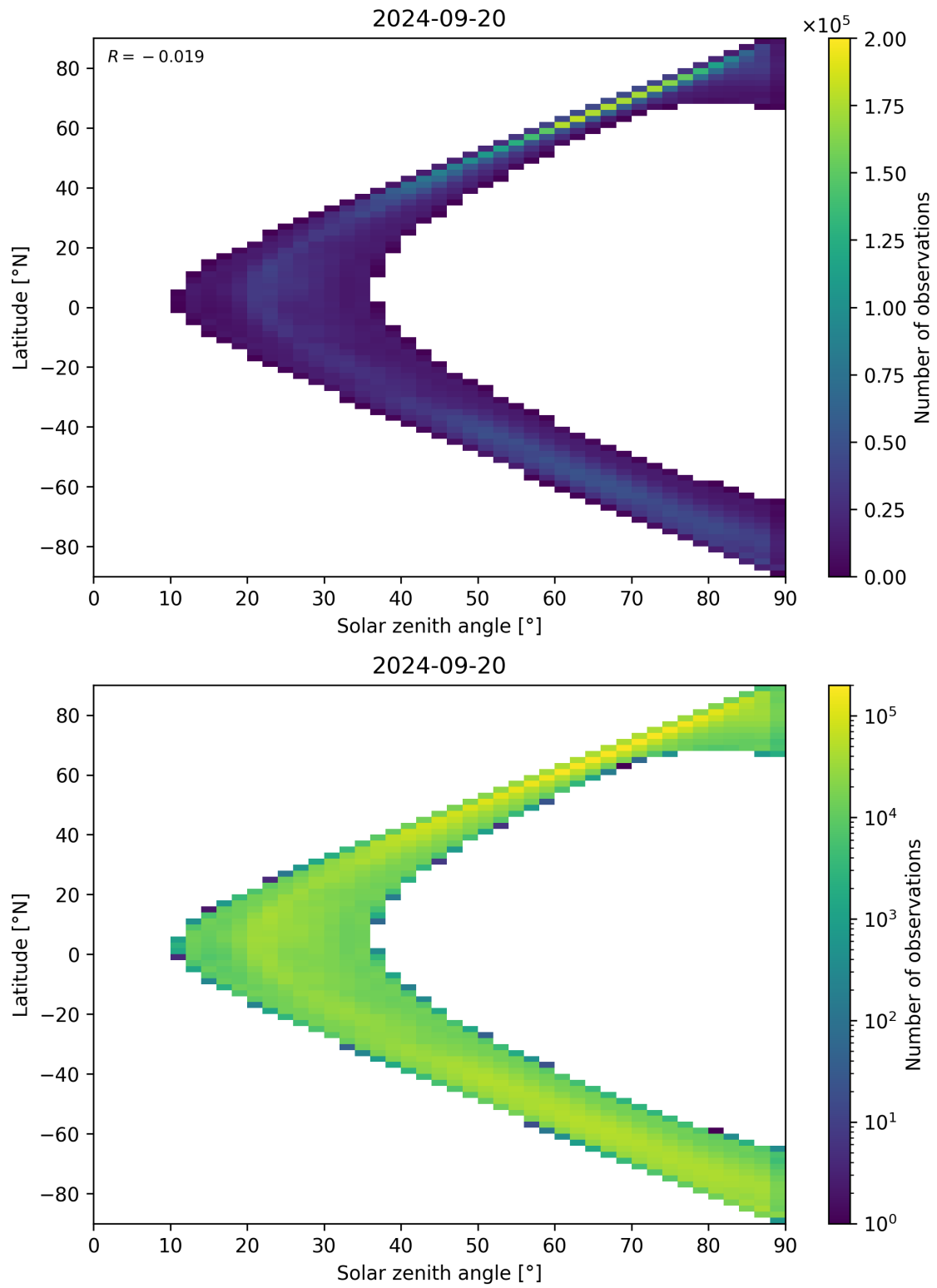
Figure 105: Scatter density plot of “Solar zenith angle” against “Latitude” for 2024-09-19 to 2024-09-21.
