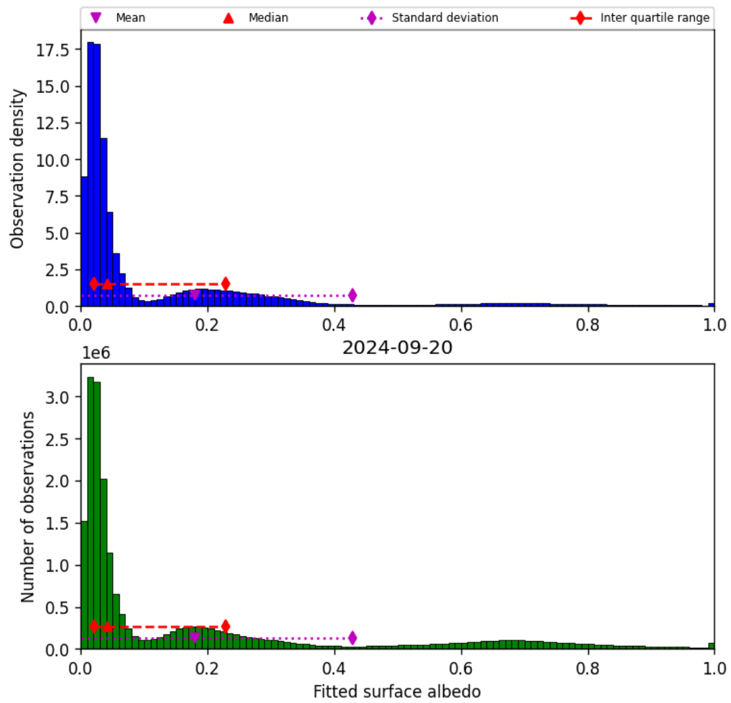
Figure 45: Histogram of “Fitted surface albedo” for 2024-09-19 to 2024-09-21
