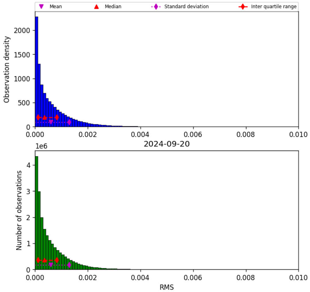
Figure 47: Histogram of “RMS” for 2024-09-19 to 2024-09-21
