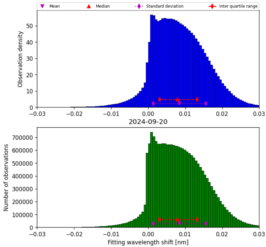
Figure 49: Histogram of “Fitting wavelength shift” for 2024-09-19 to 2024-09-21
