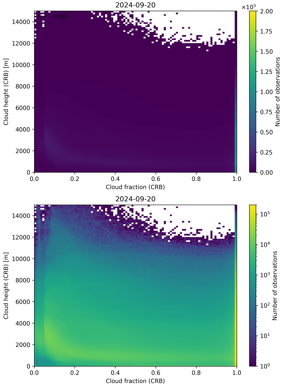
Figure 79: Scatter density plot of “Cloud fraction (CRB)” against “Cloud height (CRB)” for 2024-09-19 to 2024-09-21.
