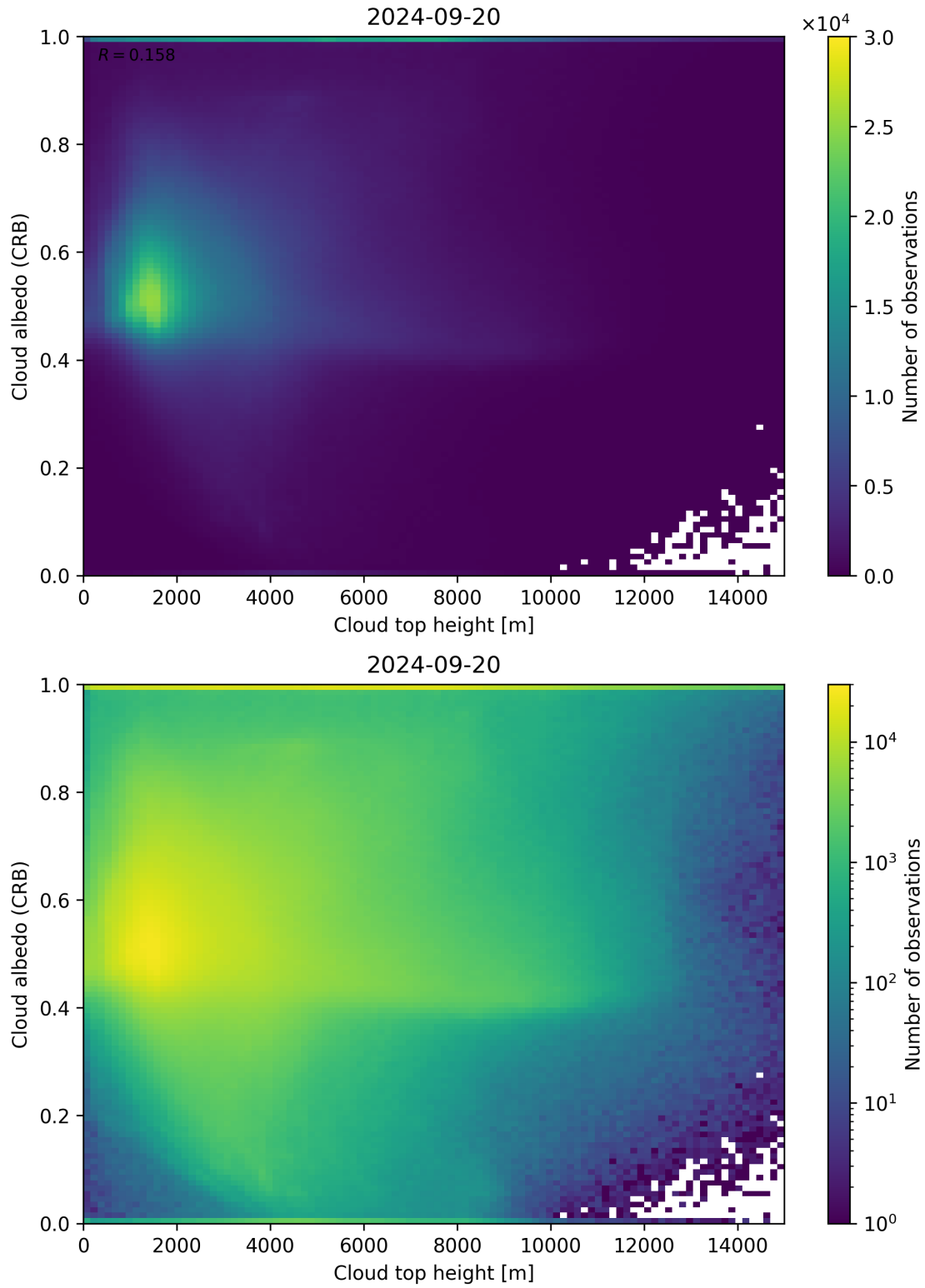
Figure 86: Scatter density plot of “Cloud top height” against “Cloud albedo (CRB)” for 2024-09-19 to 2024-09-21.
