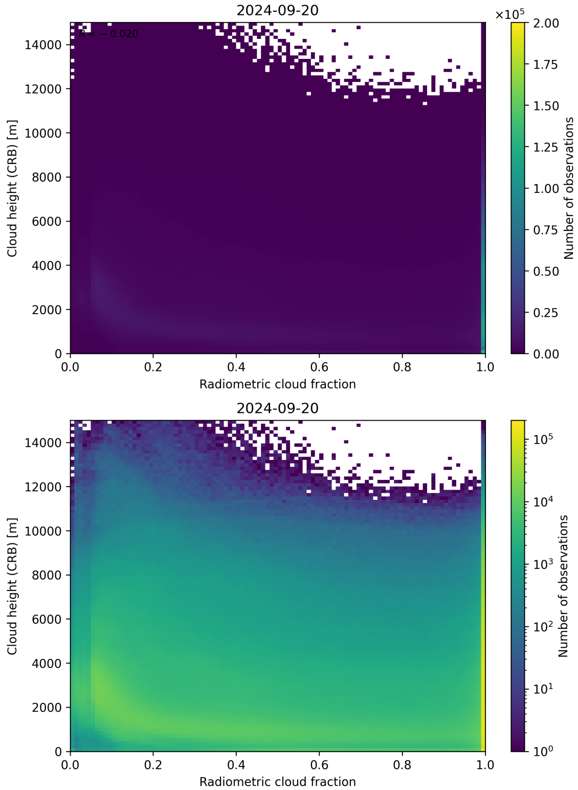
Figure 74: Scatter density plot of “Radiometric cloud fraction” against “Cloud height (CRB)” for 2024-09-19 to 2024-09-21.
