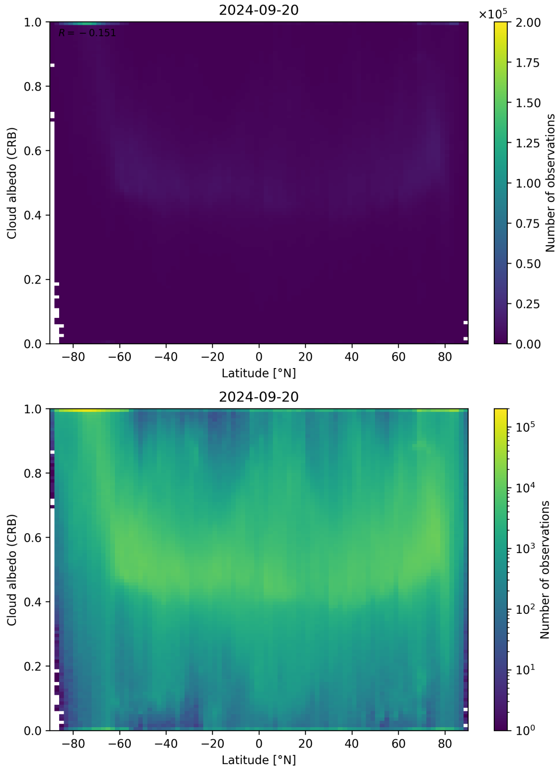
Figure 91: Scatter density plot of “Latitude” against “Cloud albedo (CRB)” for 2024-09-19 to 2024-09-21.
