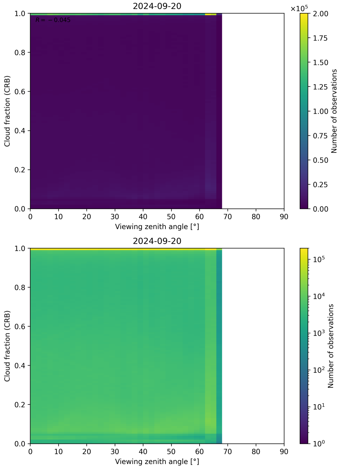
Figure 109: Scatter density plot of “Viewing zenith angle” against “Cloud fraction (CRB)” for 2024-09-19 to 2024-09-21.
