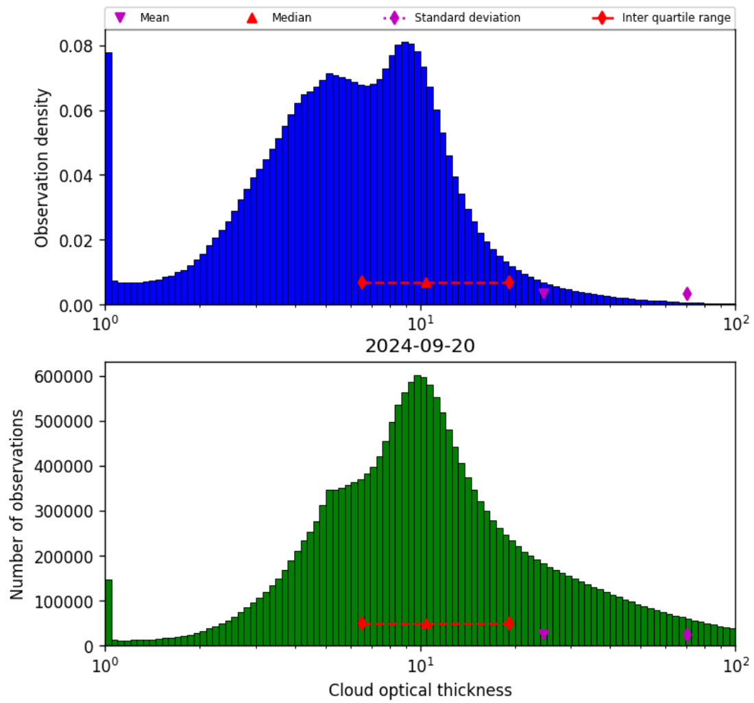
Figure 41: Histogram of “Cloud optical thickness” for 2024-09-19 to 2024-09-21
