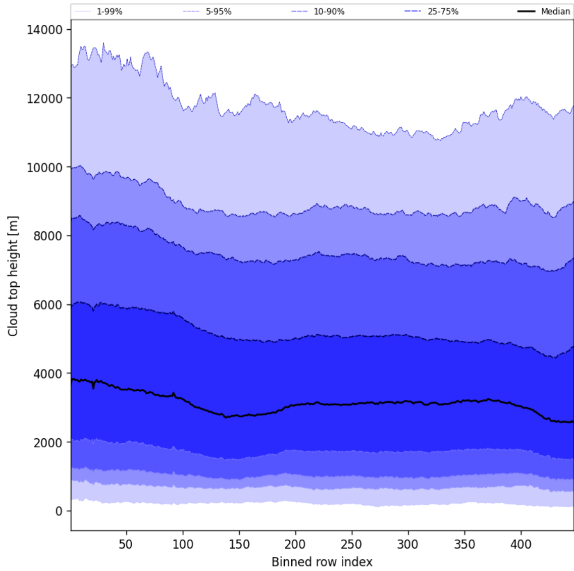
Figure 56: Along track statistics of “Cloud top height” for 2024-09-19 to 2024-09-21
