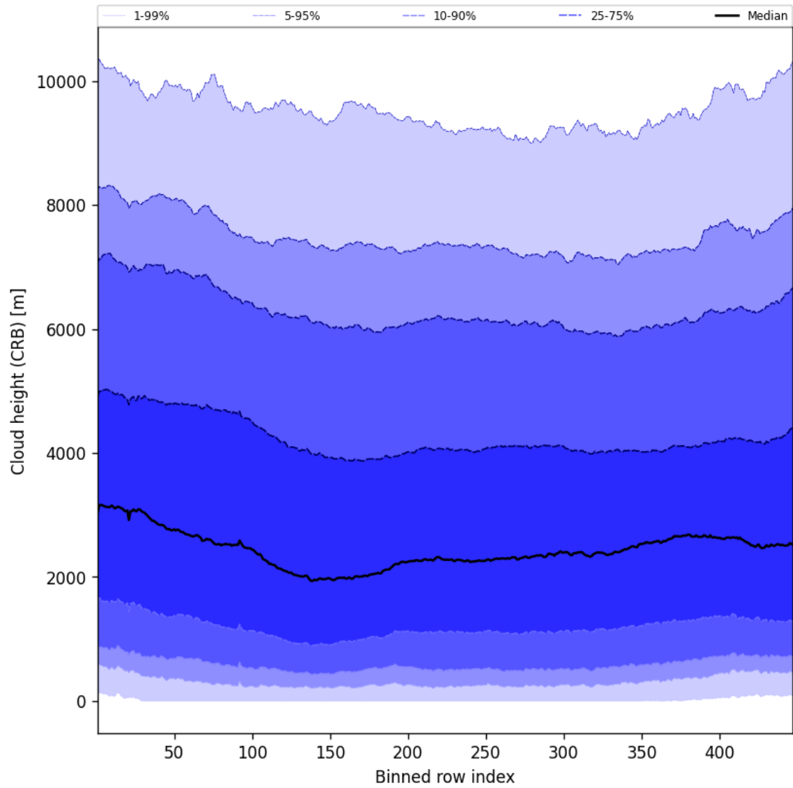
Figure 59: Along track statistics of “Cloud height (CRB)” for 2024-09-19 to 2024-09-21
