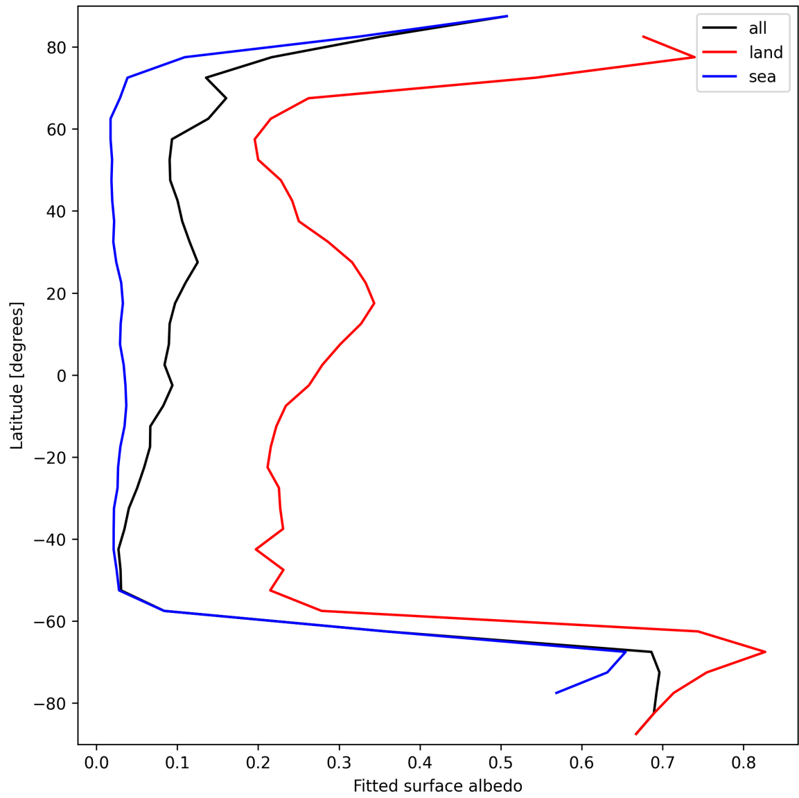
Figure 29: Zonal average of “Fitted surface albedo” for 2024-09-19 to 2024-09-21.
