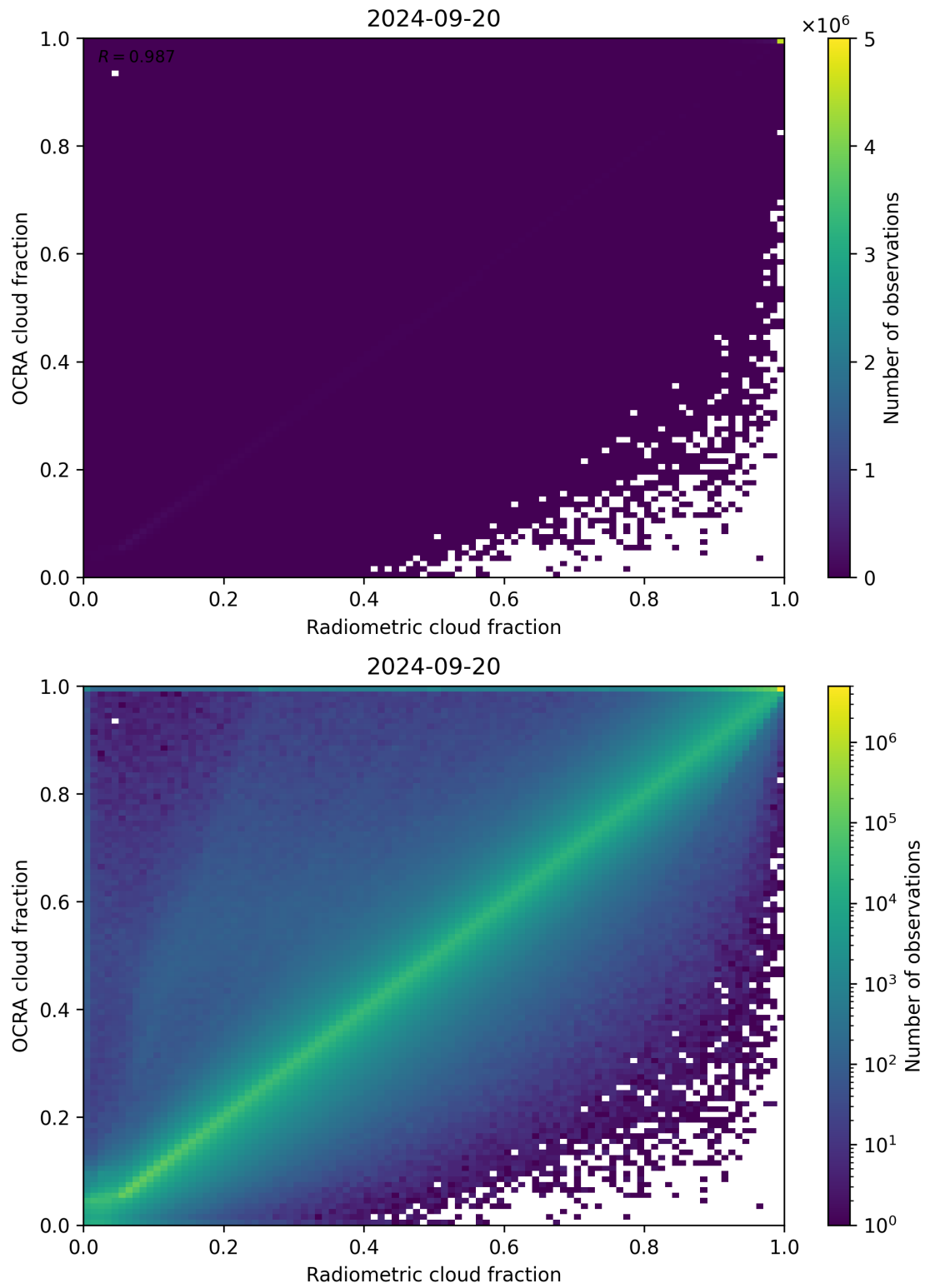
Figure 72: Scatter density plot of “Radiometric cloud fraction” against “OCRA cloud fraction” for 2024-09-19 to 2024-09-21.
