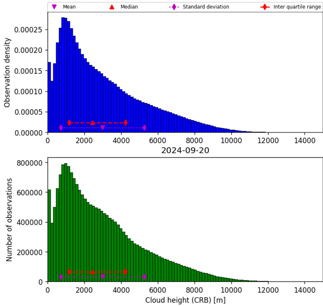
Figure 43: Histogram of “Cloud height (CRB)” for 2024-09-19 to 2024-09-21
