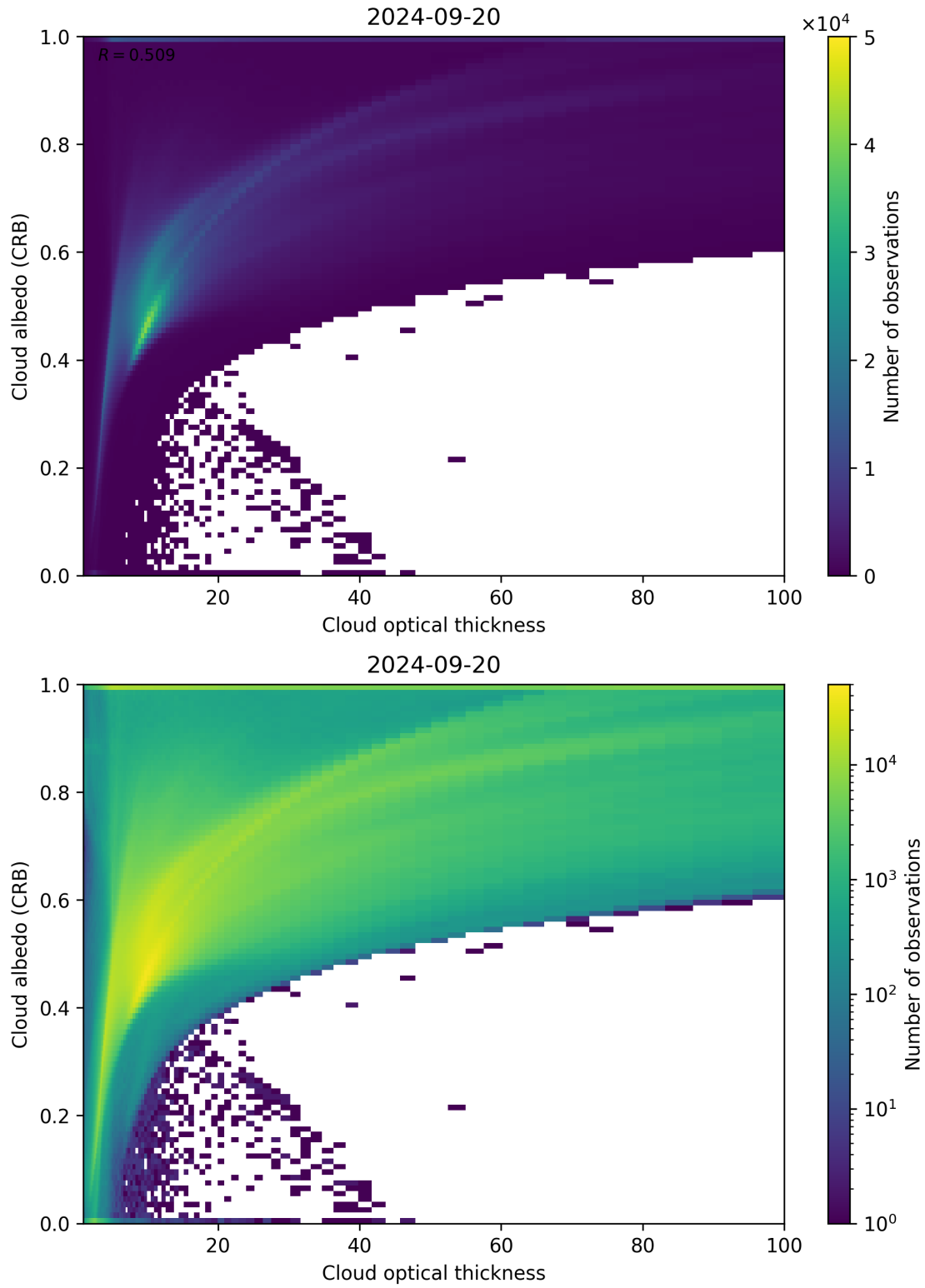
Figure 82: Scatter density plot of “Cloud optical thickness” against “Cloud albedo (CRB)” for 2024-09-19 to 2024-09-21.
