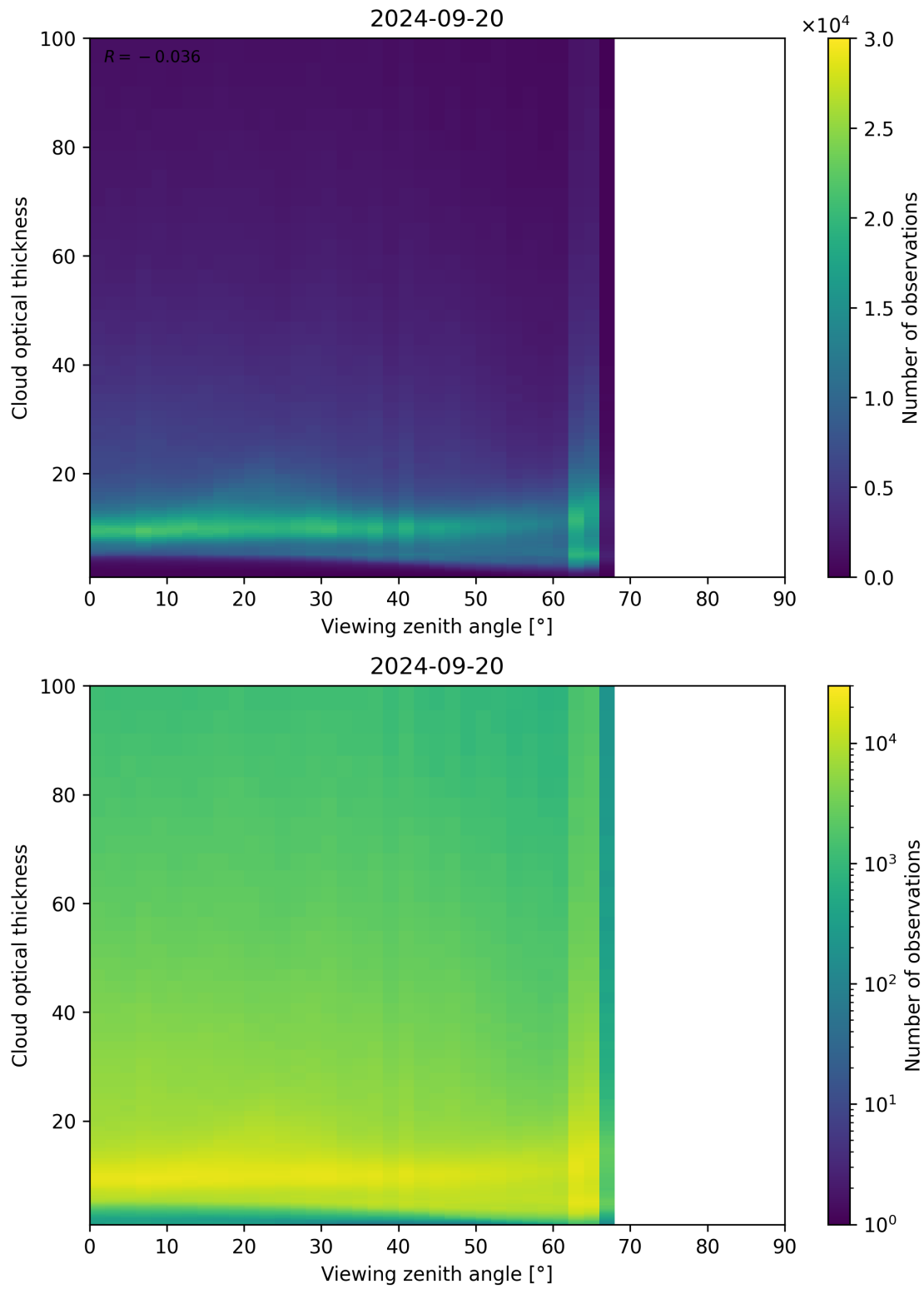
Figure 111: Scatter density plot of “Viewing zenith angle” against “Cloud optical thickness” for 2024-09-19 to 2024-09-21.
