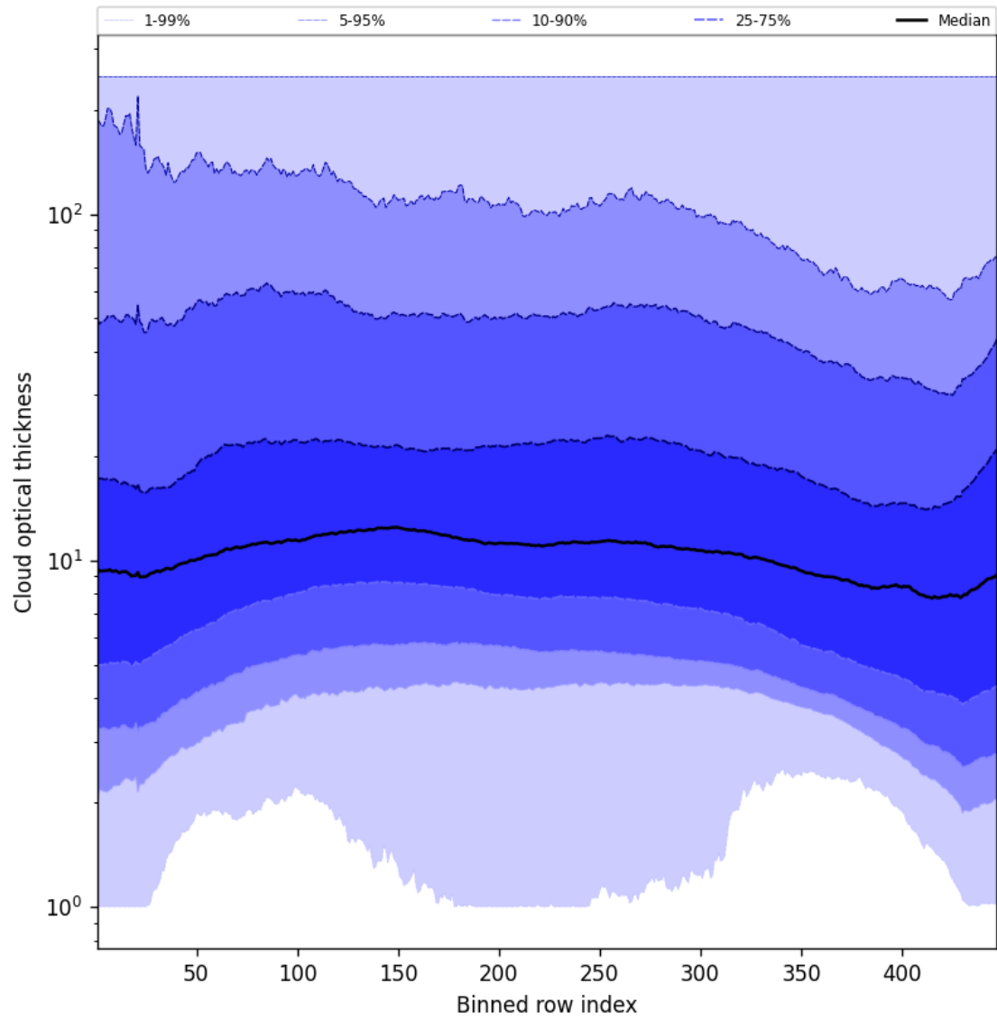
Figure 57: Along track statistics of “Cloud optical thickness” for 2024-09-19 to 2024-09-21
