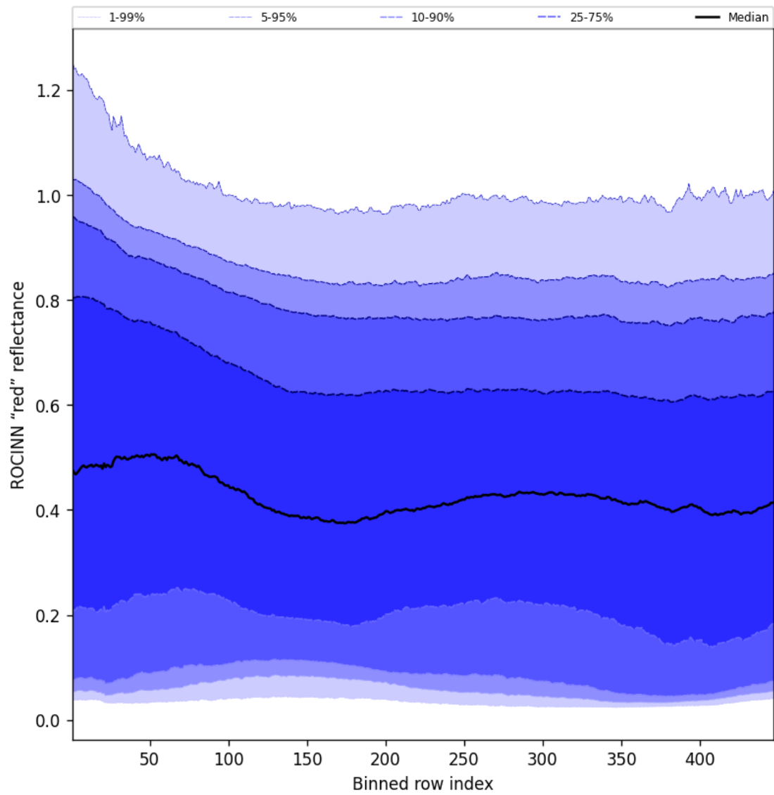
Figure 69: Along track statistics of “ROCINN “red” reflectance” for 2024-09-19 to 2024-09-21
