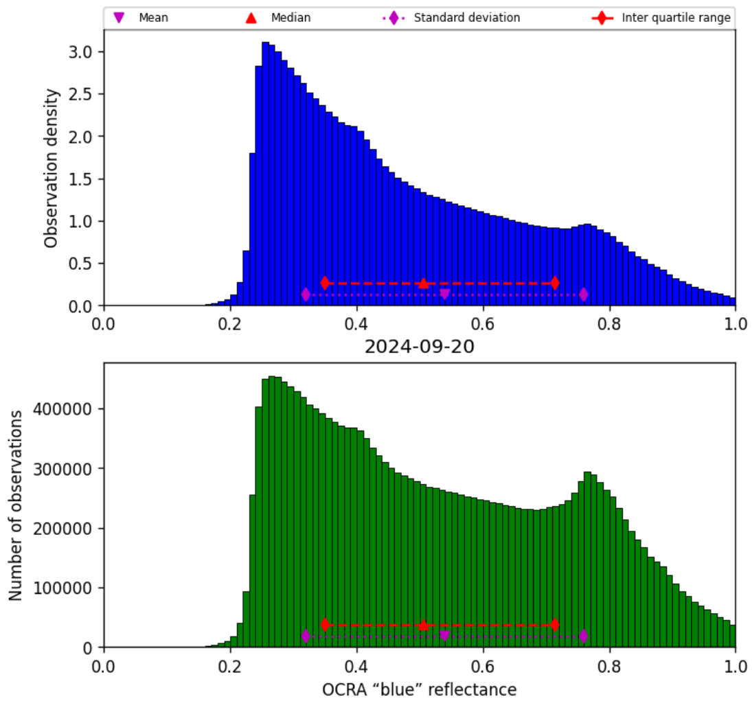
Figure 51: Histogram of “OCRA “blue” reflectance” for 2024-09-19 to 2024-09-21
