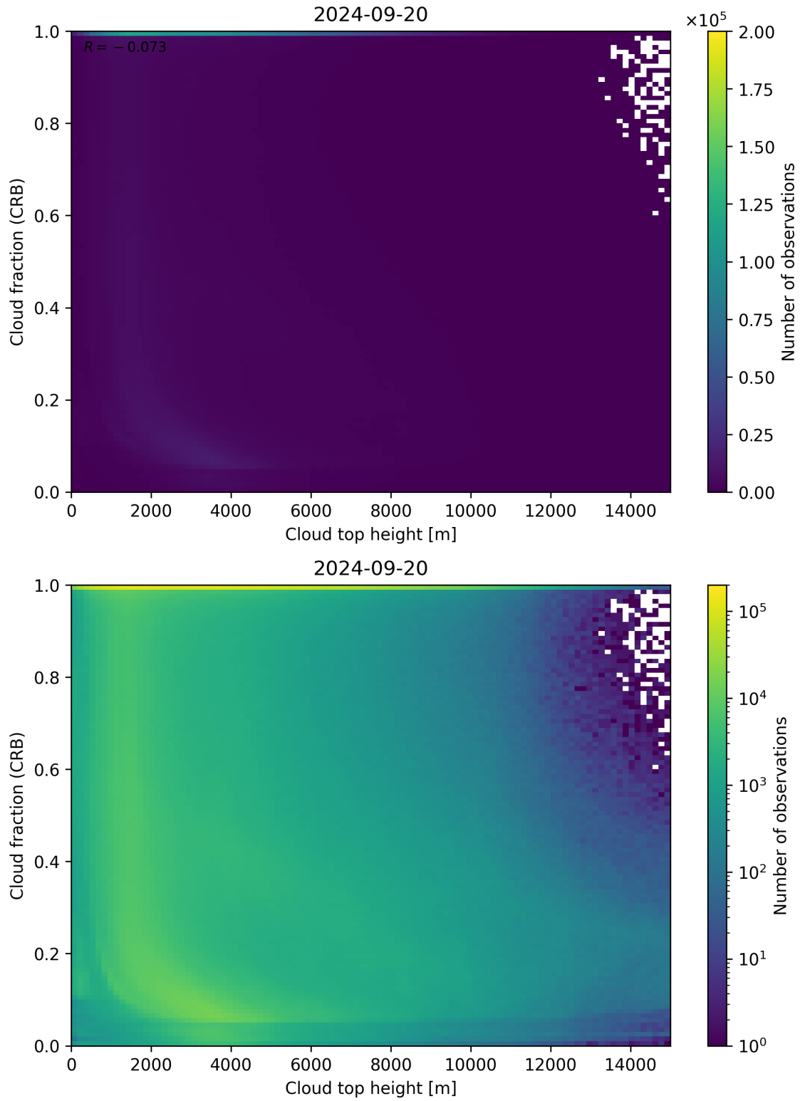
Figure 88: Scatter density plot of “Cloud top height” against “Cloud fraction (CRB)” for 2024-09-19 to 2024-09-21.
