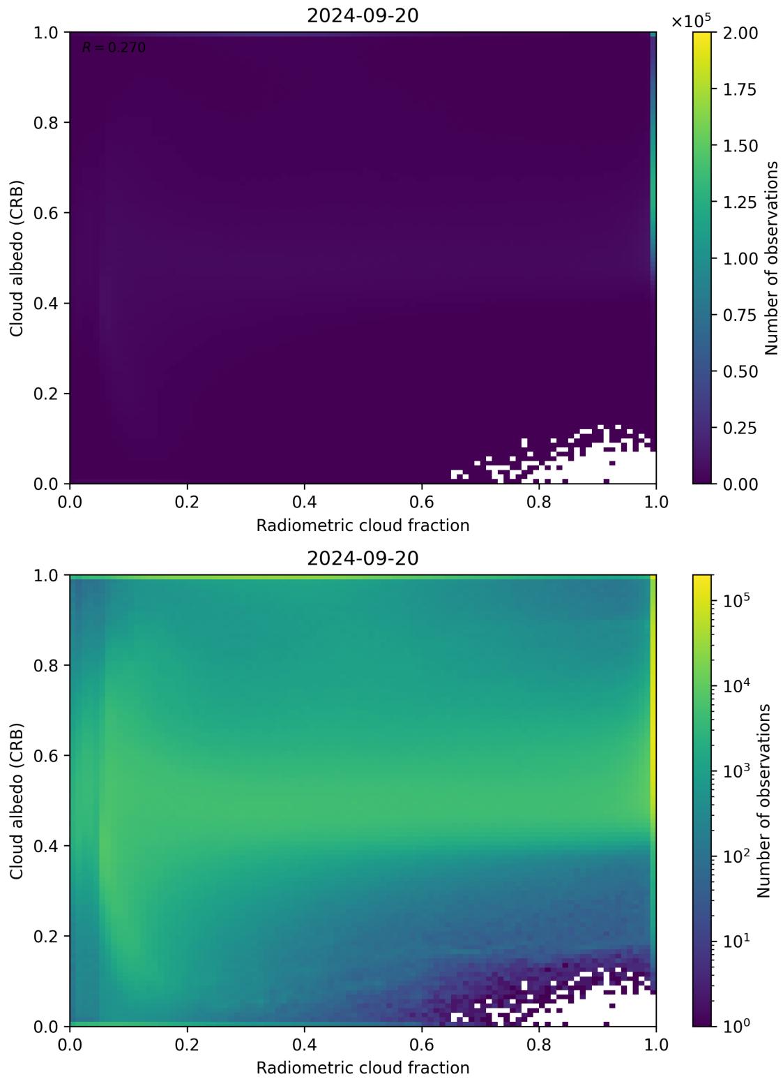
Figure 71: Scatter density plot of “Radiometric cloud fraction” against “Cloud albedo (CRB)” for 2024-09-19 to 2024-09-21.
