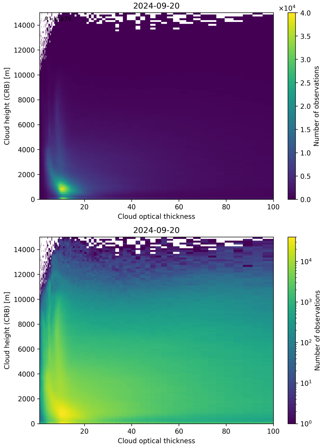
Figure 85: Scatter density plot of “Cloud optical thickness” against “Cloud height (CRB)” for 2024-09-19 to 2024-09-21.
