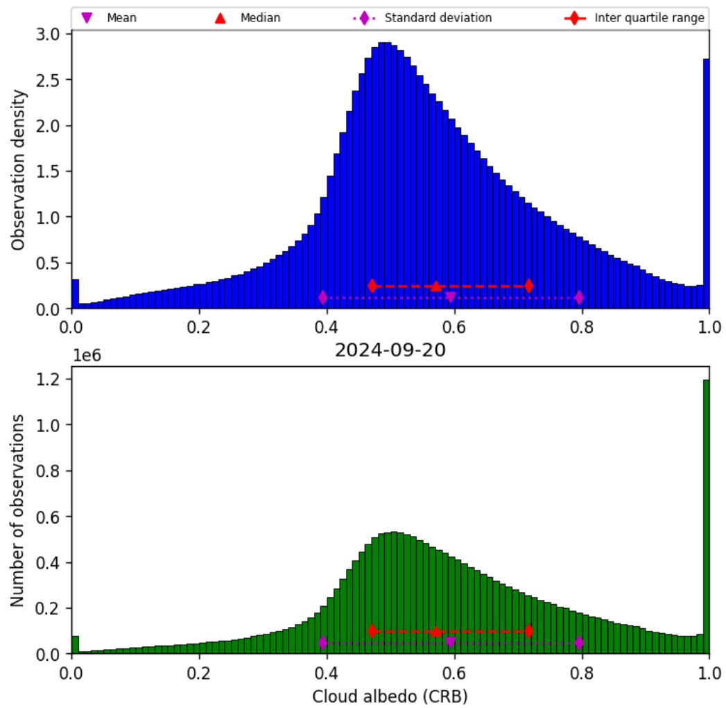
Figure 44: Histogram of “Cloud albedo (CRB)” for 2024-09-19 to 2024-09-21
