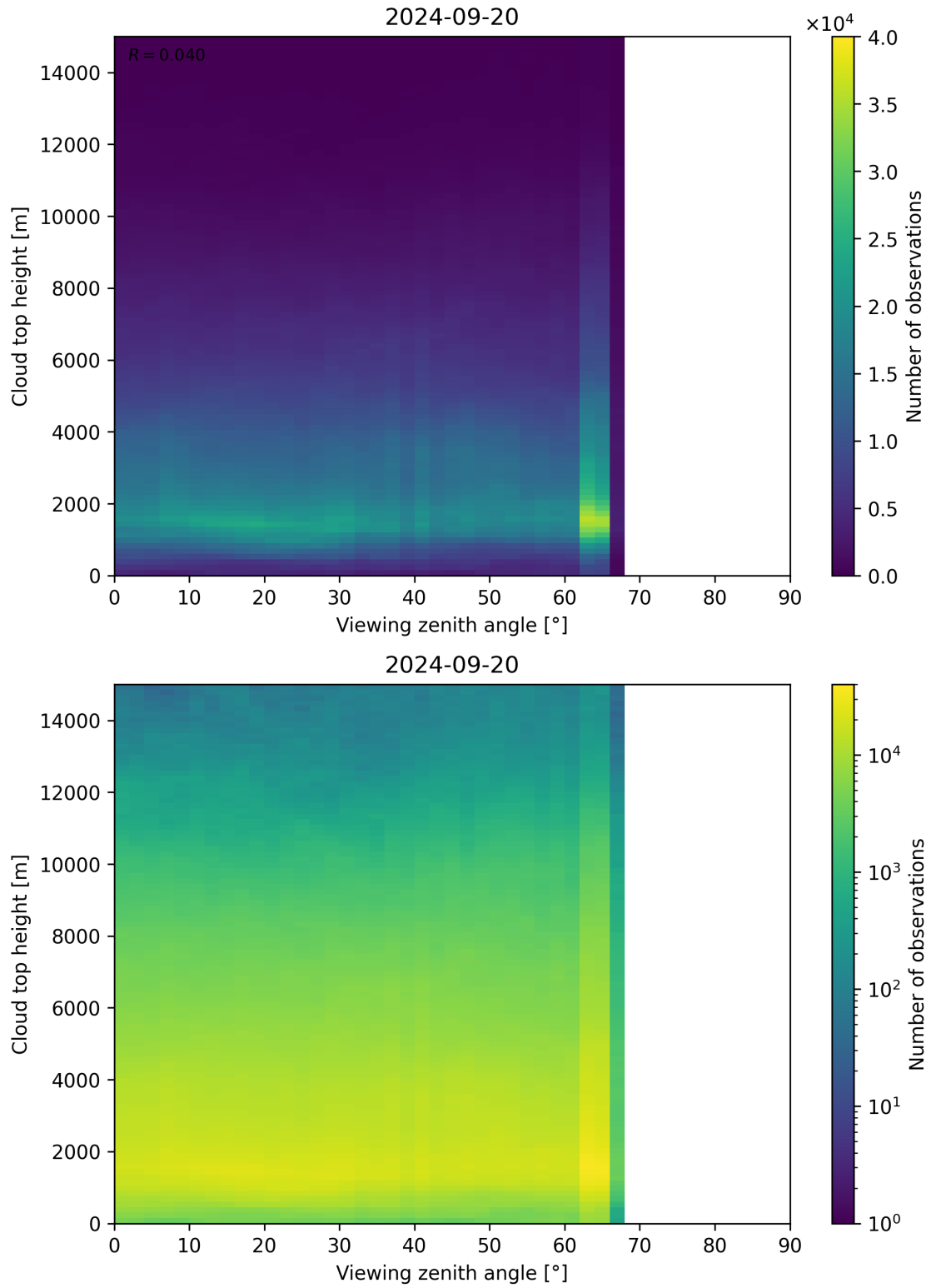
Figure 112: Scatter density plot of “Viewing zenith angle” against “Cloud top height” for 2024-09-19 to 2024-09-21.
