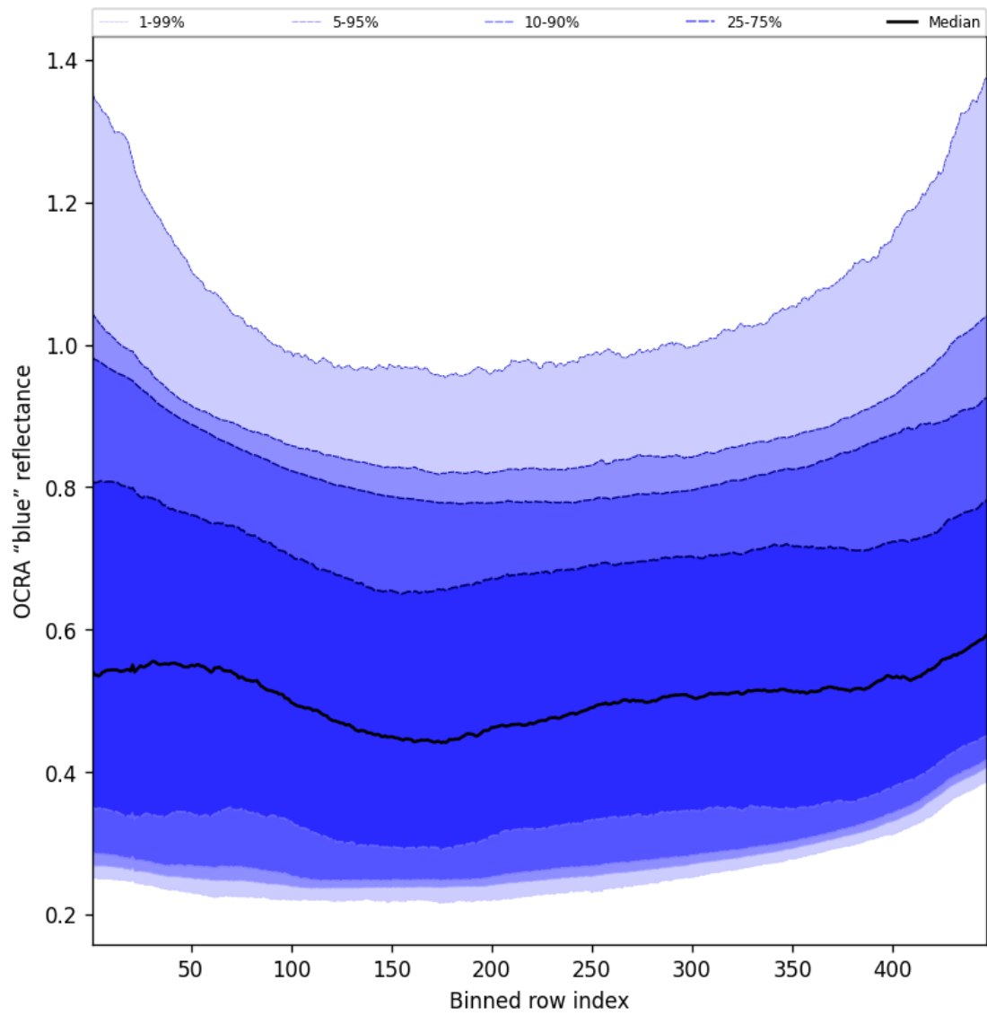
Figure 67: Along track statistics of “OCRA “blue” reflectance” for 2024-09-19 to 2024-09-21
