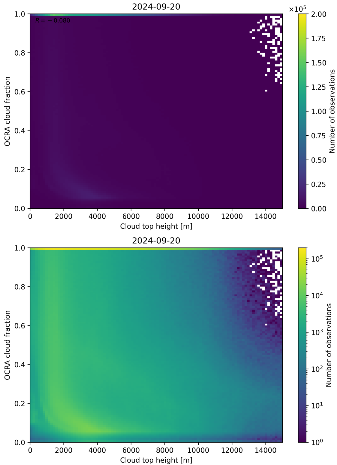
Figure 87: Scatter density plot of “Cloud top height” against “OCRA cloud fraction” for 2024-09-19 to 2024-09-21.
