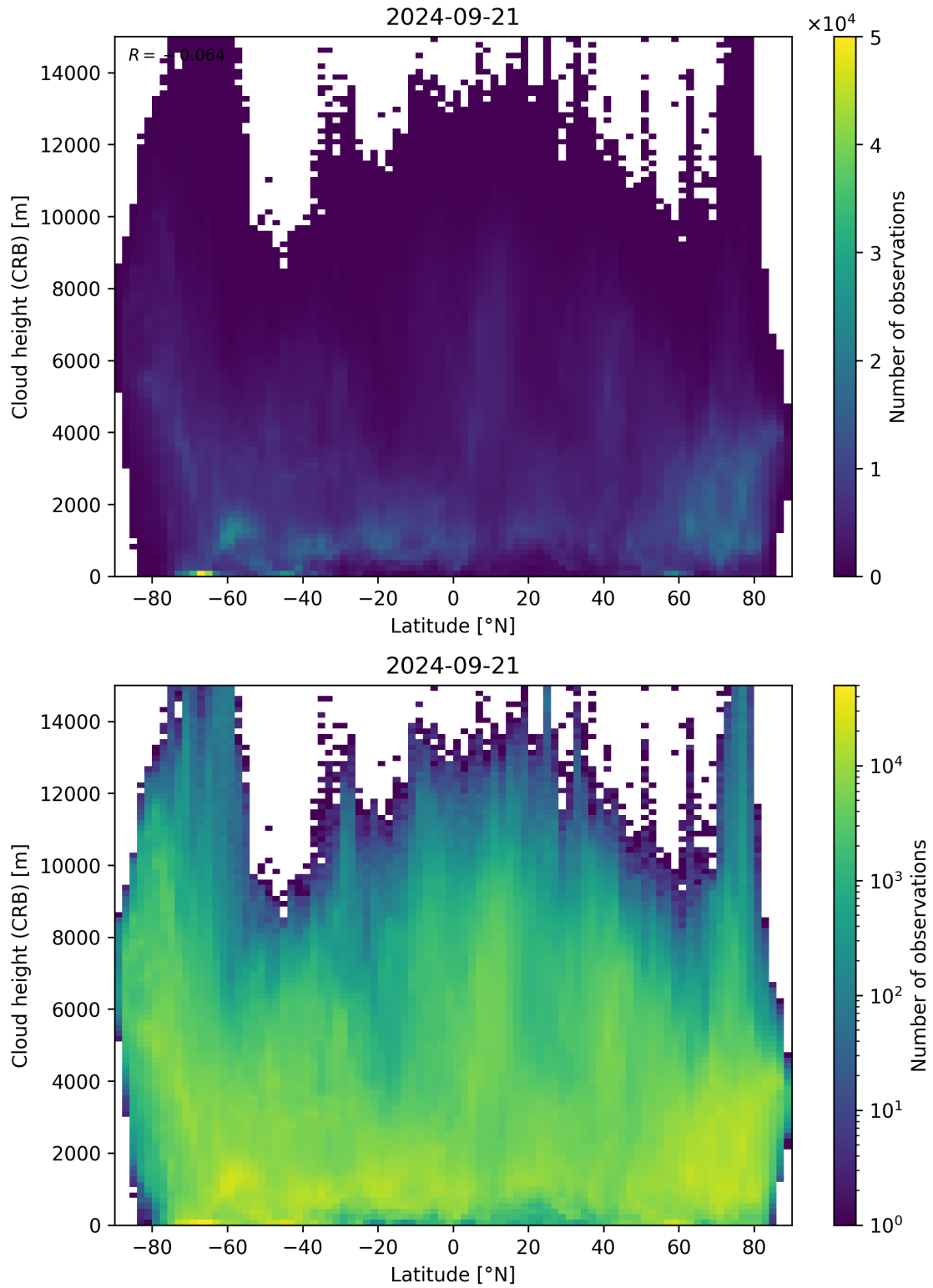
Figure 95: Scatter density plot of “Latitude” against “Cloud height (CRB)” for 2024-09-20 to 2024-09-22.
