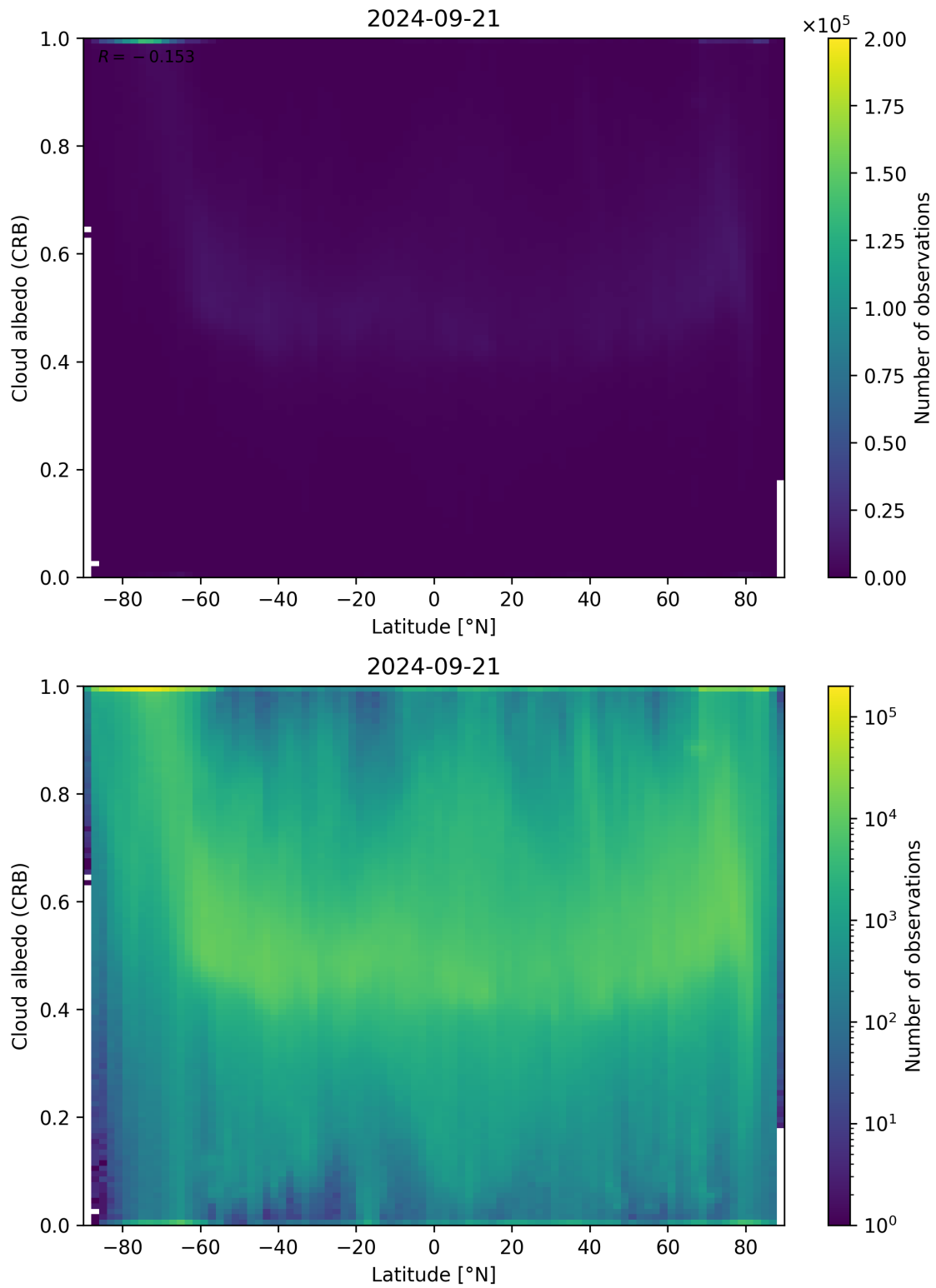
Figure 91: Scatter density plot of “Latitude” against “Cloud albedo (CRB)” for 2024-09-20 to 2024-09-22.
