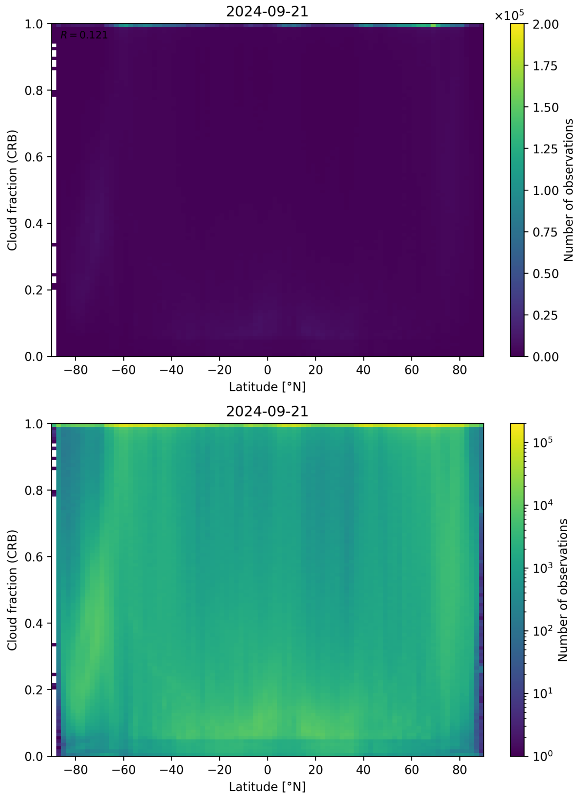
Figure 94: Scatter density plot of “Latitude” against “Cloud fraction (CRB)” for 2024-09-20 to 2024-09-22.
