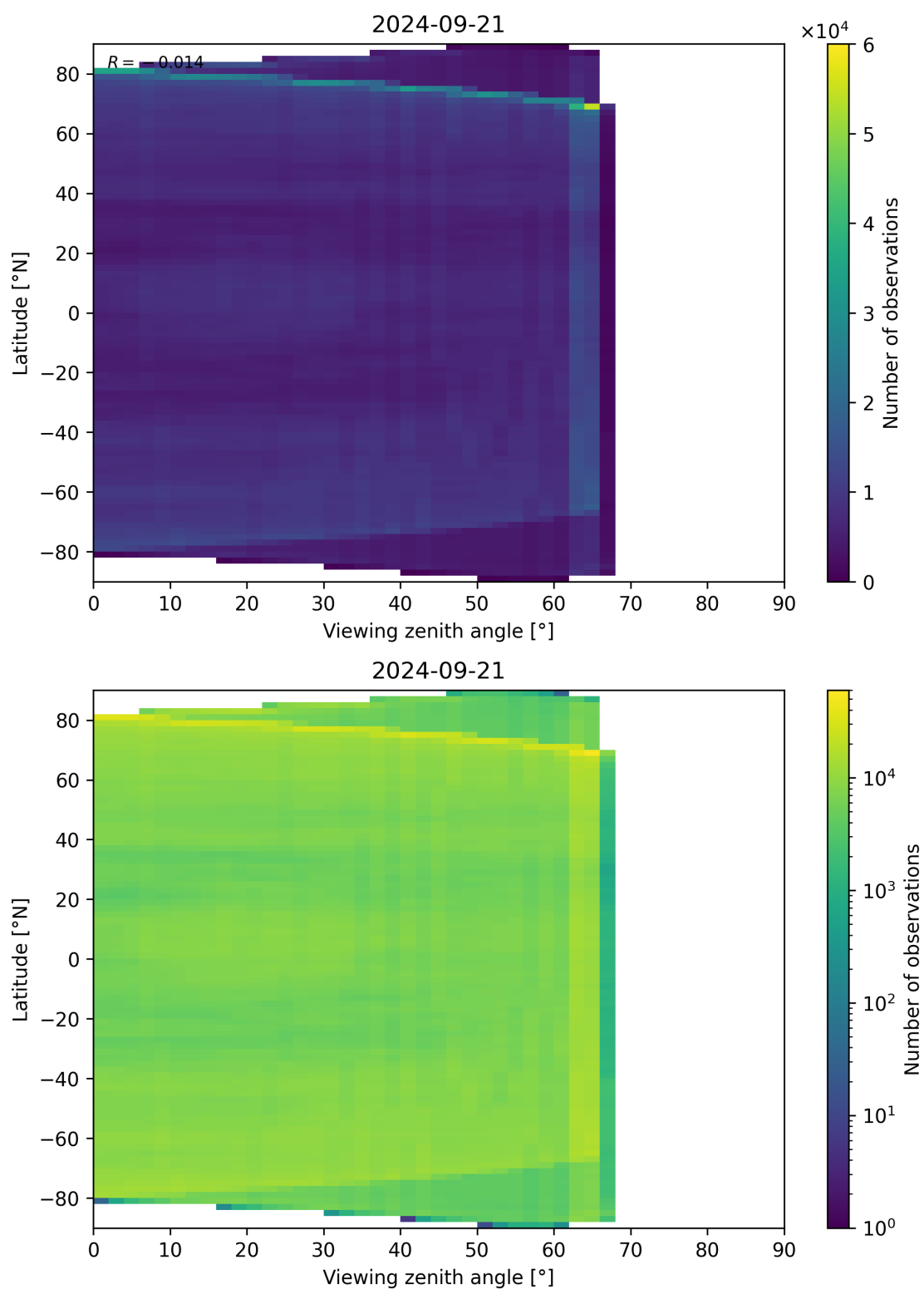
Figure 113: Scatter density plot of “Viewing zenith angle” against “Latitude” for 2024-09-20 to 2024-09-22.
