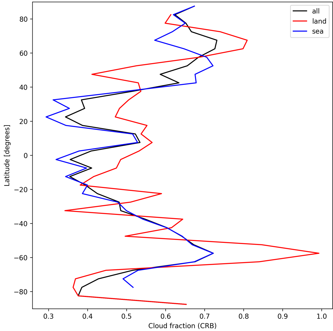
Figure 26: Zonal average of “Cloud fraction (CRB)” for 2024-09-20 to 2024-09-22.
