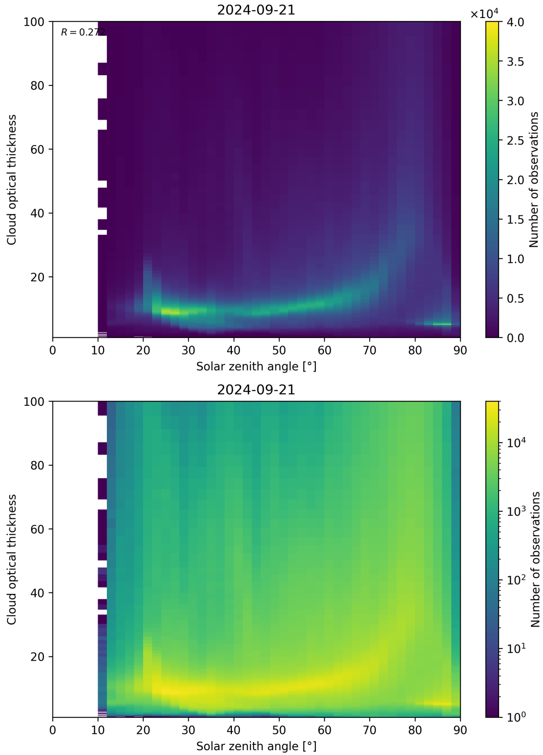
Figure 103: Scatter density plot of “Solar zenith angle” against “Cloud optical thickness” for 2024-09-20 to 2024-09-22.
