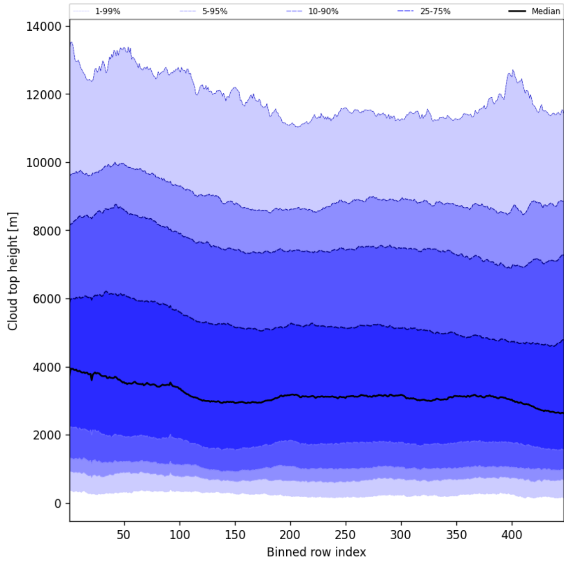
Figure 56: Along track statistics of “Cloud top height” for 2024-09-20 to 2024-09-22
