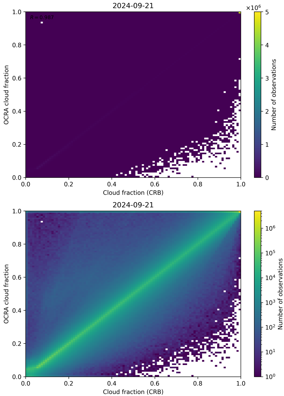
Figure 78: Scatter density plot of “Cloud fraction (CRB)” against “OCRA cloud fraction” for 2024-09-20 to 2024-09-22.
