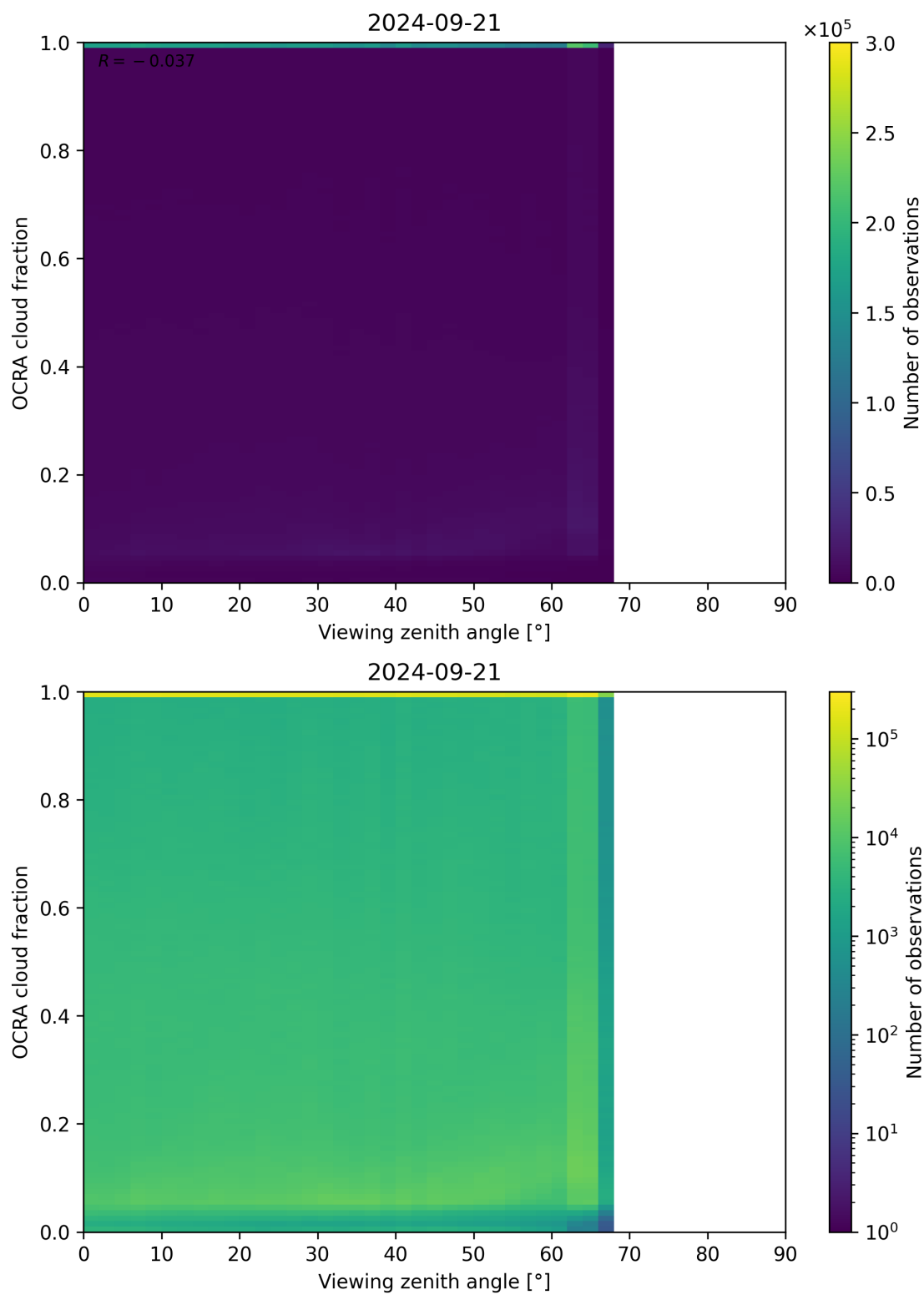
Figure 108: Scatter density plot of “Viewing zenith angle” against “OCRA cloud fraction” for 2024-09-20 to 2024-09-22.
