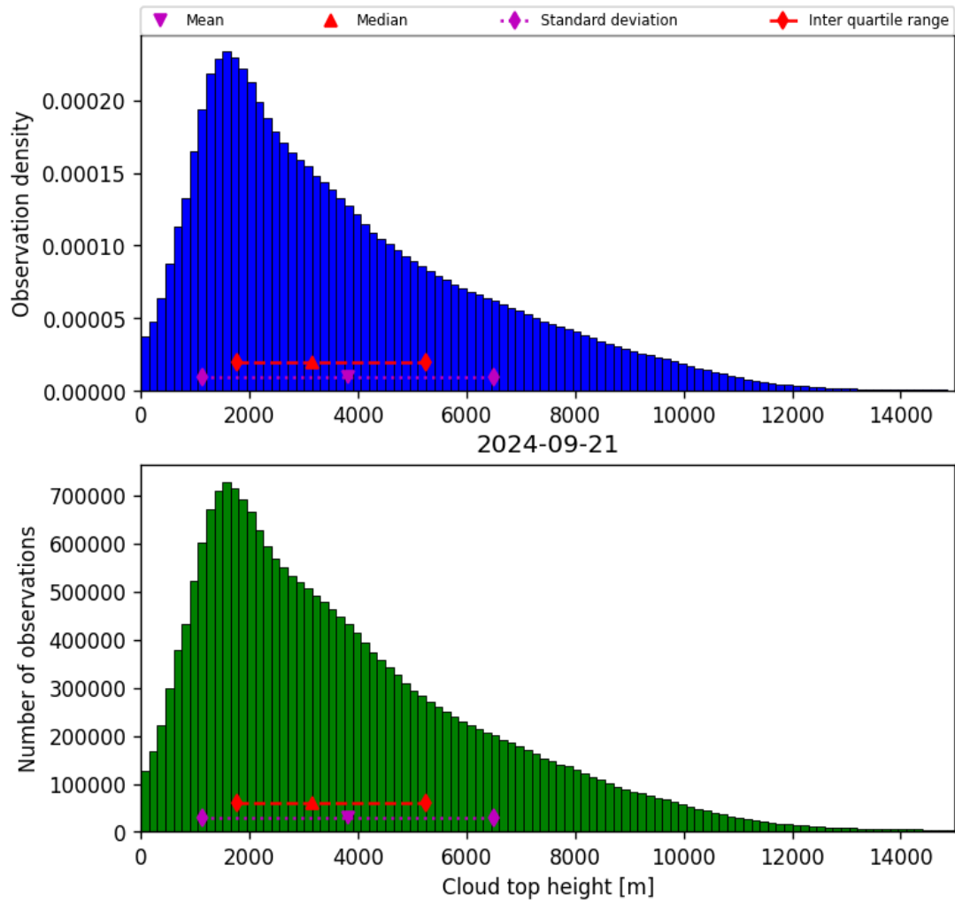
Figure 40: Histogram of “Cloud top height” for 2024-09-20 to 2024-09-22
