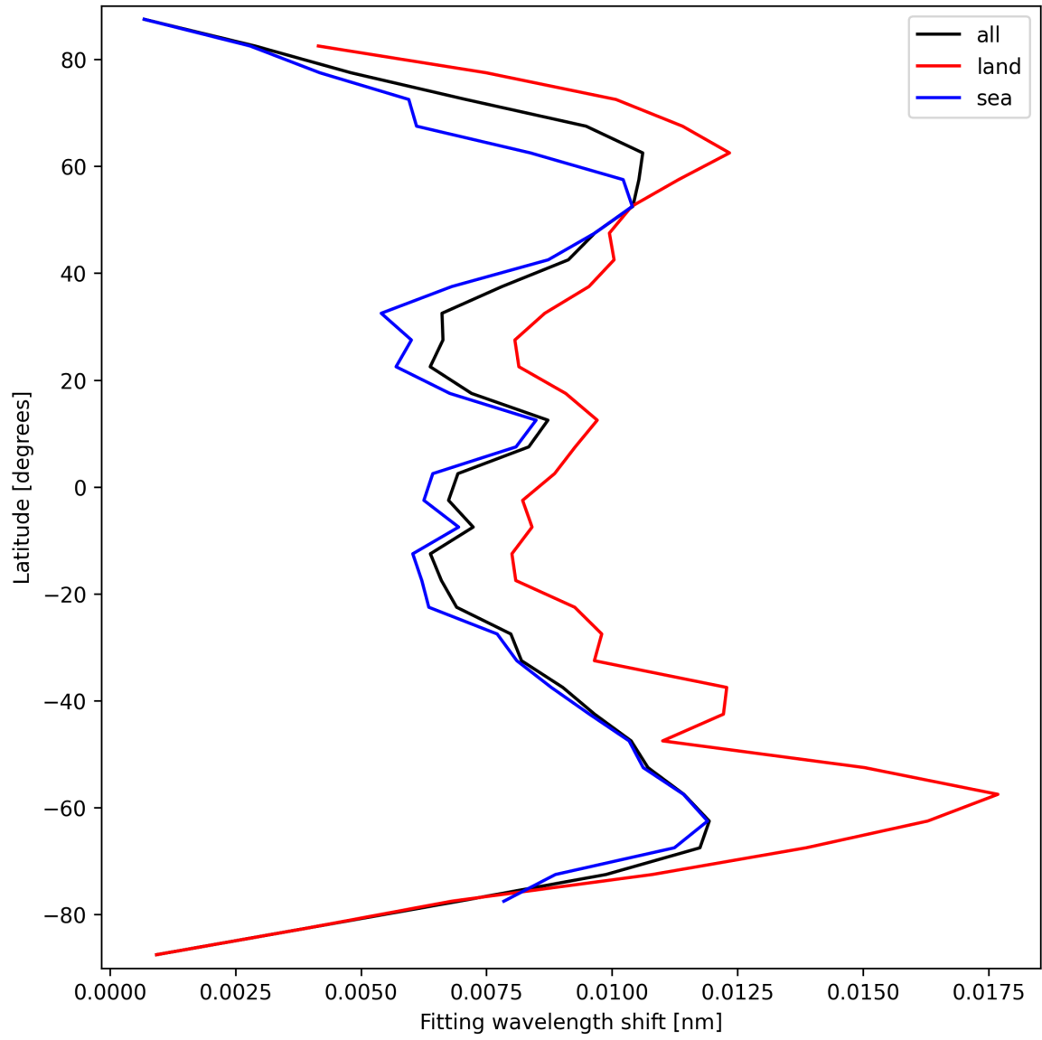
Figure 33: Zonal average of “Fitting wavelength shift” for 2024-09-20 to 2024-09-22.
