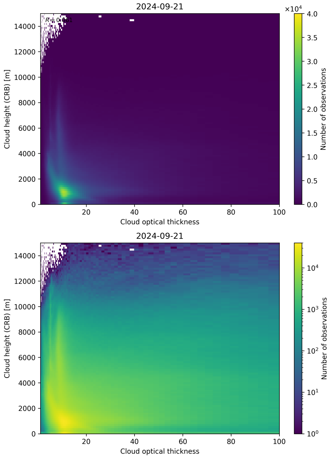
Figure 85: Scatter density plot of “Cloud optical thickness” against “Cloud height (CRB)” for 2024-09-20 to 2024-09-22.
