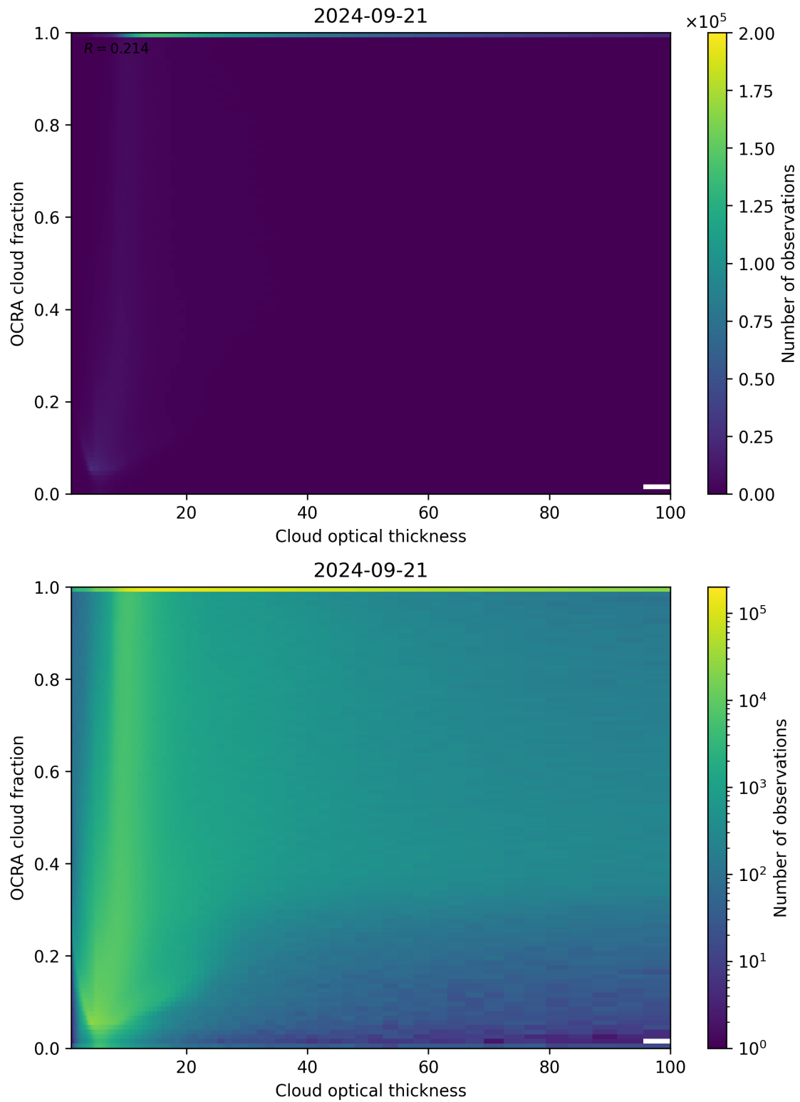
Figure 83: Scatter density plot of “Cloud optical thickness” against “OCRA cloud fraction” for 2024-09-20 to 2024-09-22.
