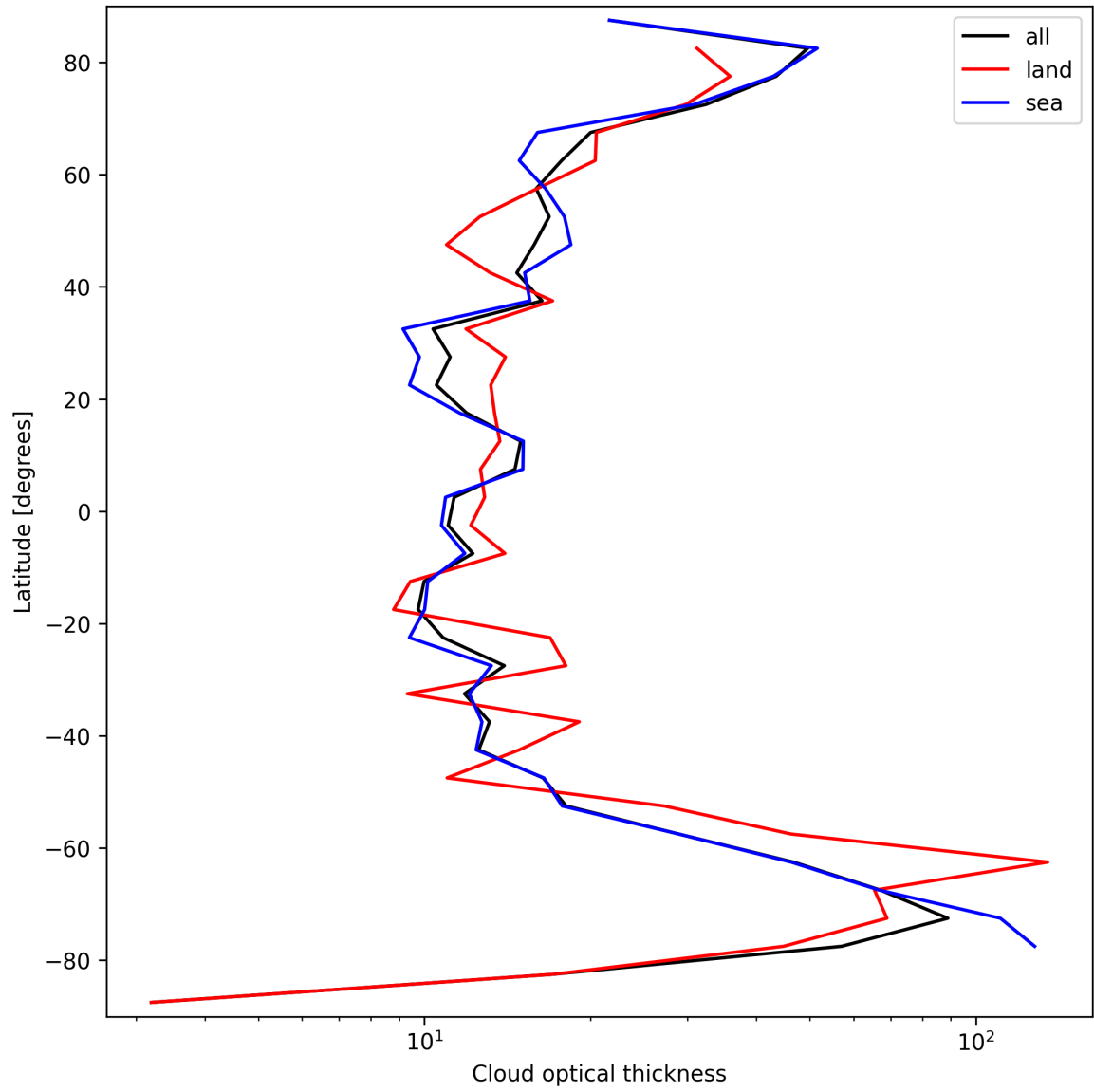
Figure 25: Zonal average of “Cloud optical thickness” for 2024-09-20 to 2024-09-22.
