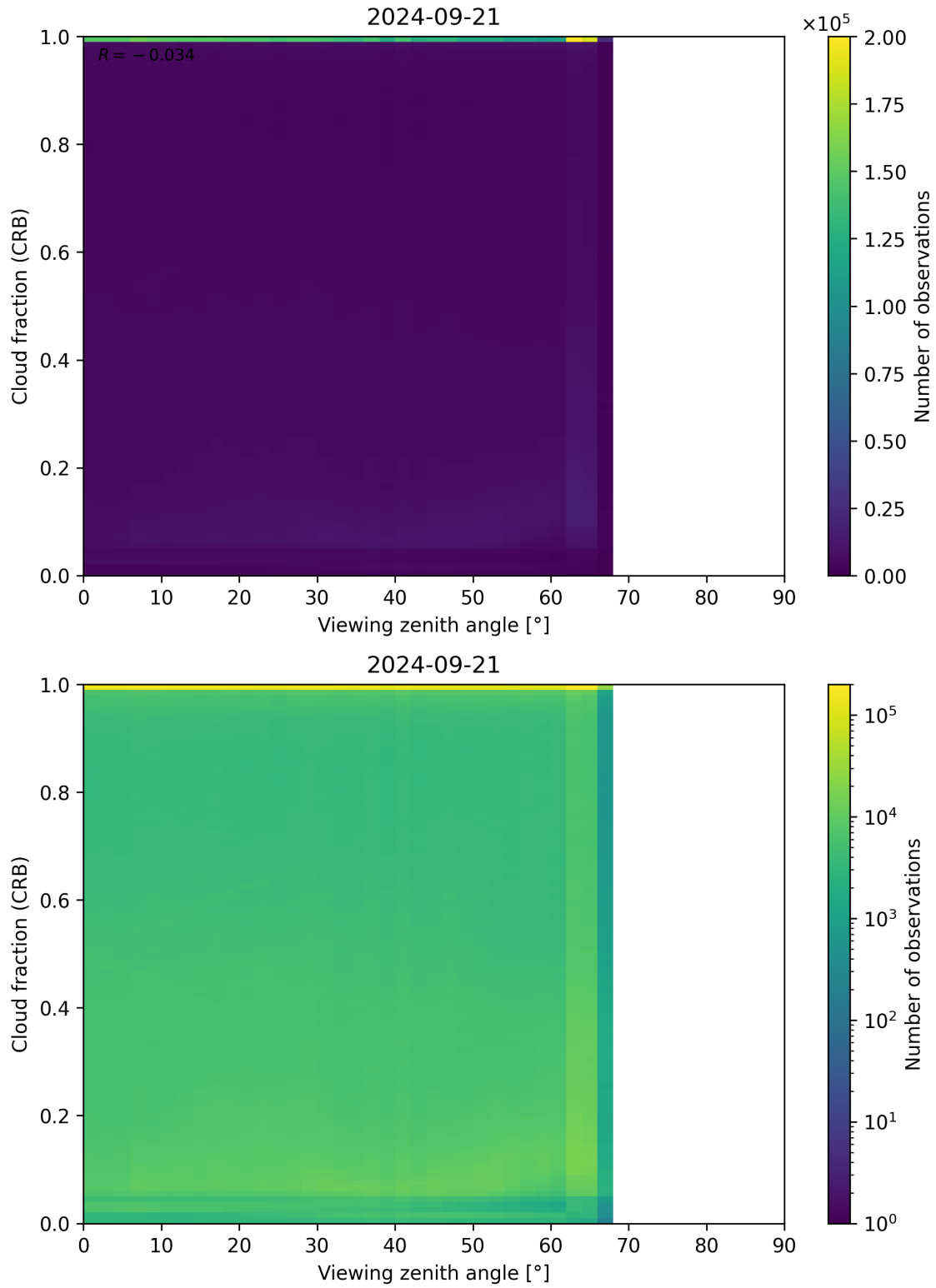
Figure 109: Scatter density plot of “Viewing zenith angle” against “Cloud fraction (CRB)” for 2024-09-20 to 2024-09-22.
