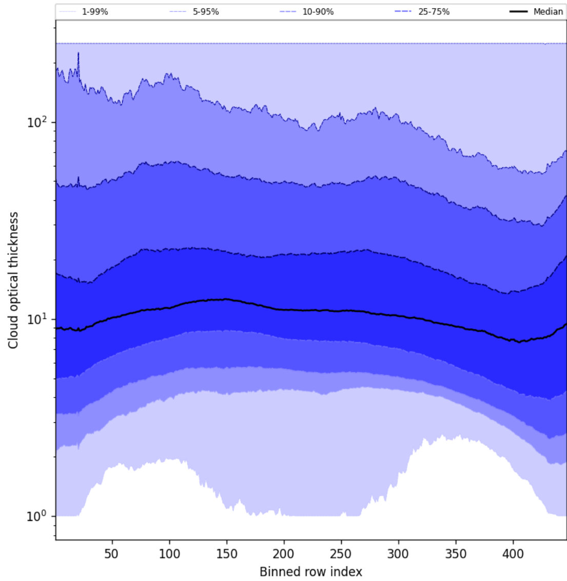
Figure 57: Along track statistics of “Cloud optical thickness” for 2024-09-20 to 2024-09-22
