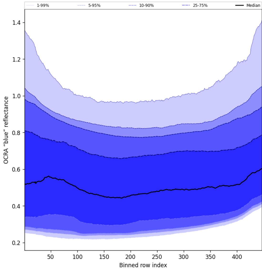
Figure 67: Along track statistics of “OCRA “blue” reflectance” for 2024-09-20 to 2024-09-22
