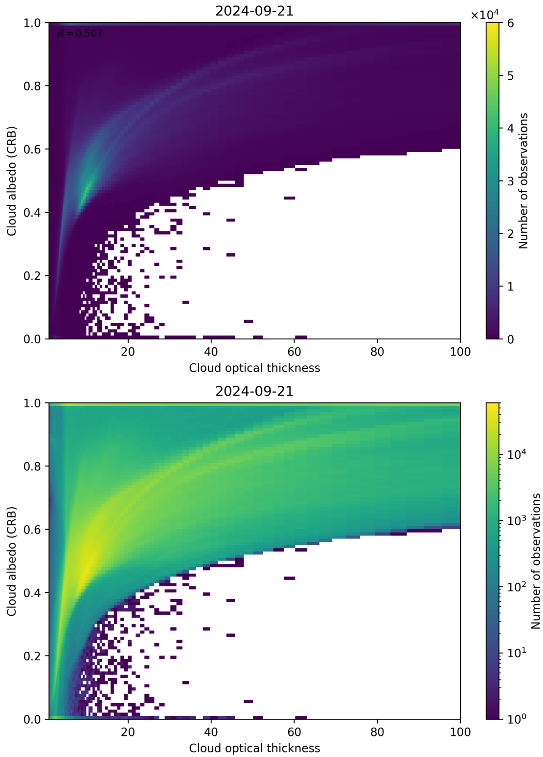
Figure 82: Scatter density plot of “Cloud optical thickness” against “Cloud albedo (CRB)” for 2024-09-20 to 2024-09-22.
