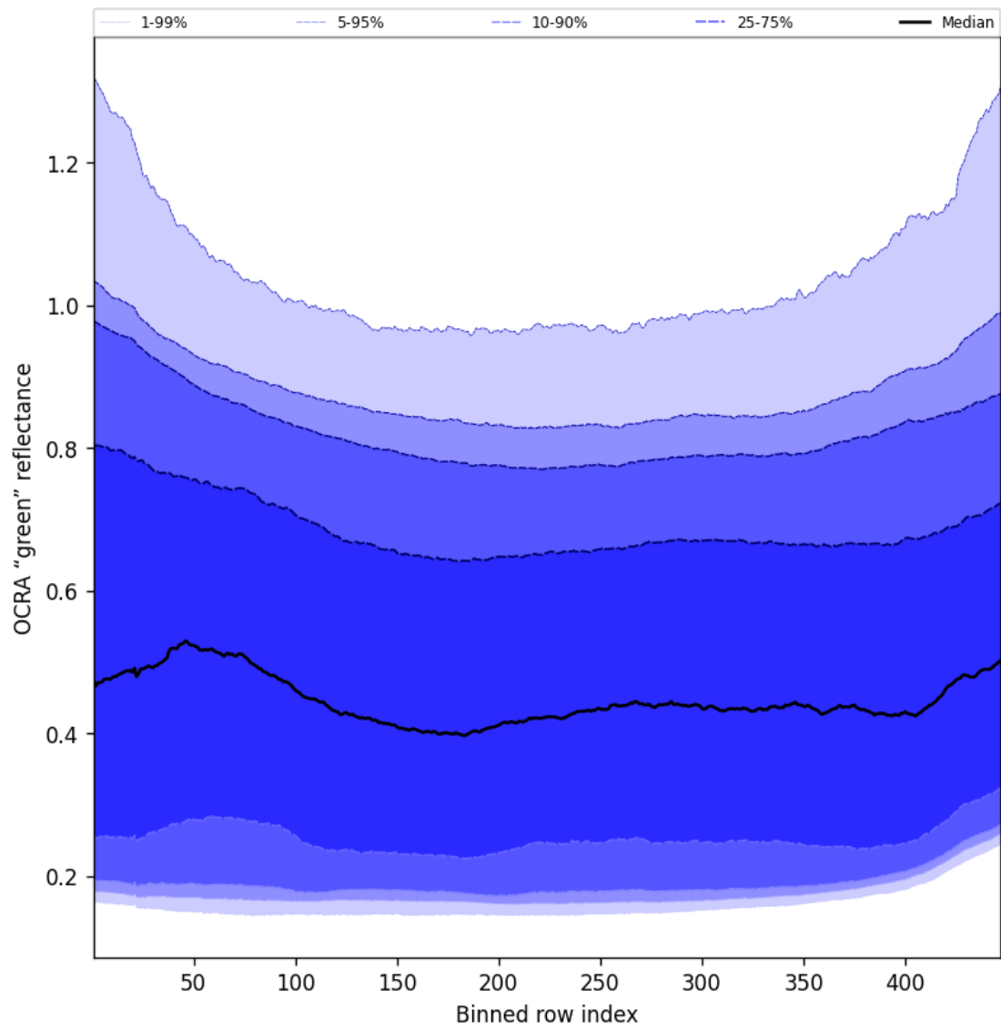
Figure 68: Along track statistics of “OCRA “green” reflectance” for 2024-09-20 to 2024-09-22
