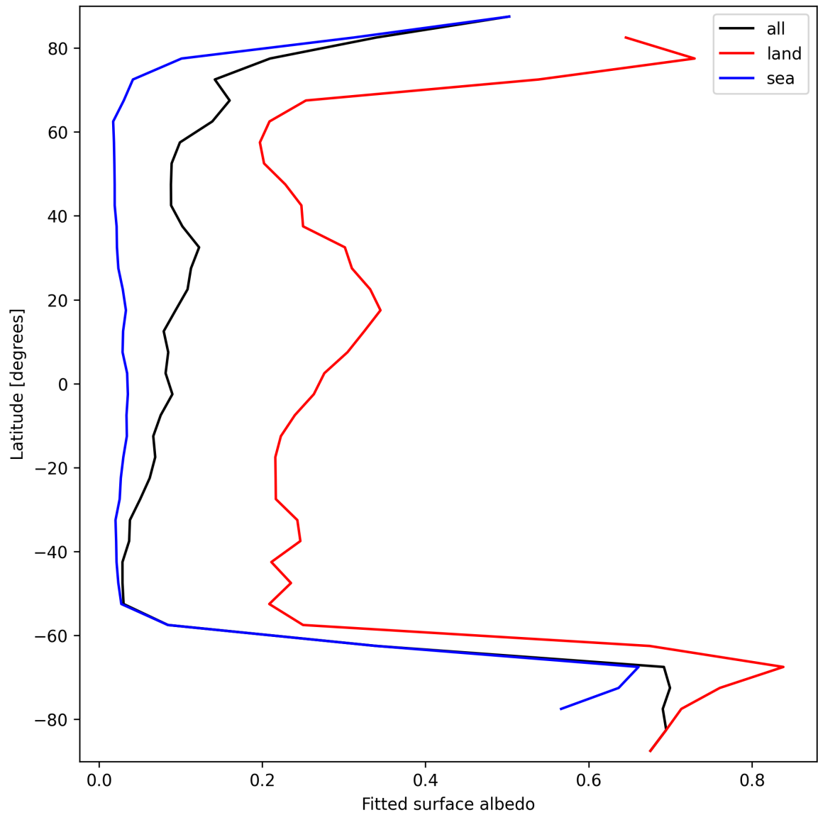
Figure 29: Zonal average of “Fitted surface albedo” for 2024-09-20 to 2024-09-22.
