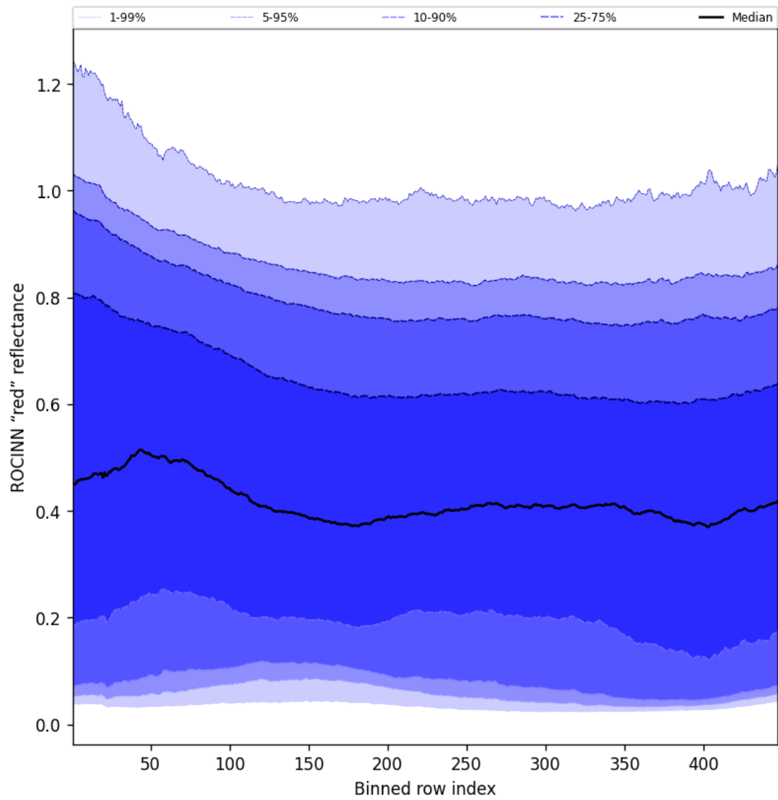
Figure 69: Along track statistics of “ROCINN “red” reflectance” for 2024-09-20 to 2024-09-22
