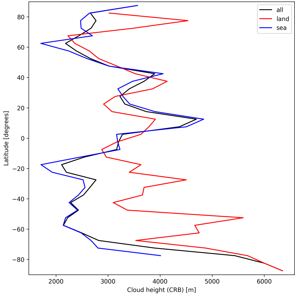
Figure 27: Zonal average of “Cloud height (CRB)” for 2024-09-20 to 2024-09-22.
