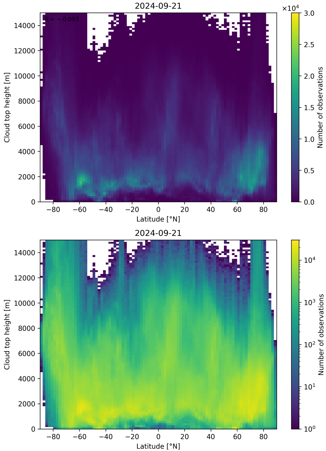
Figure 97: Scatter density plot of “Latitude” against “Cloud top height” for 2024-09-20 to 2024-09-22.
