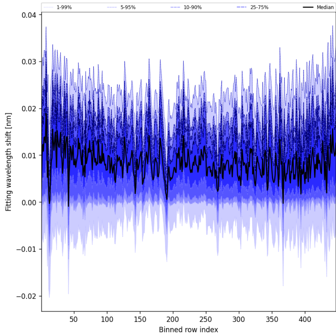
Figure 65: Along track statistics of “Fitting wavelength shift” for 2024-09-20 to 2024-09-22
