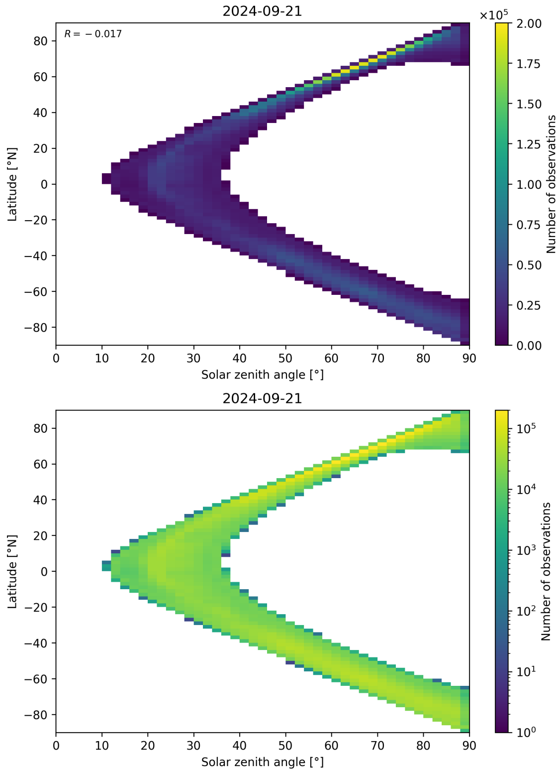
Figure 105: Scatter density plot of “Solar zenith angle” against “Latitude” for 2024-09-20 to 2024-09-22.
