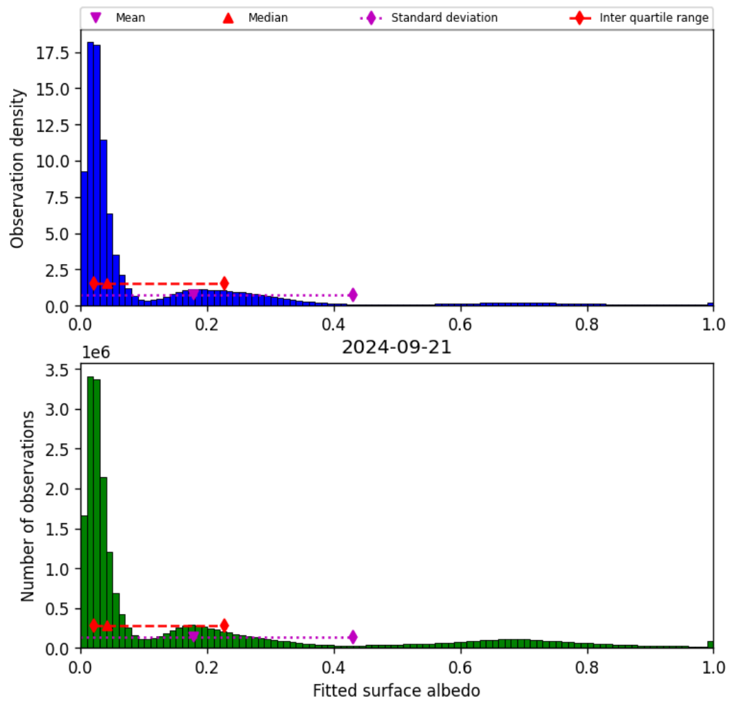
Figure 45: Histogram of “Fitted surface albedo” for 2024-09-20 to 2024-09-22
