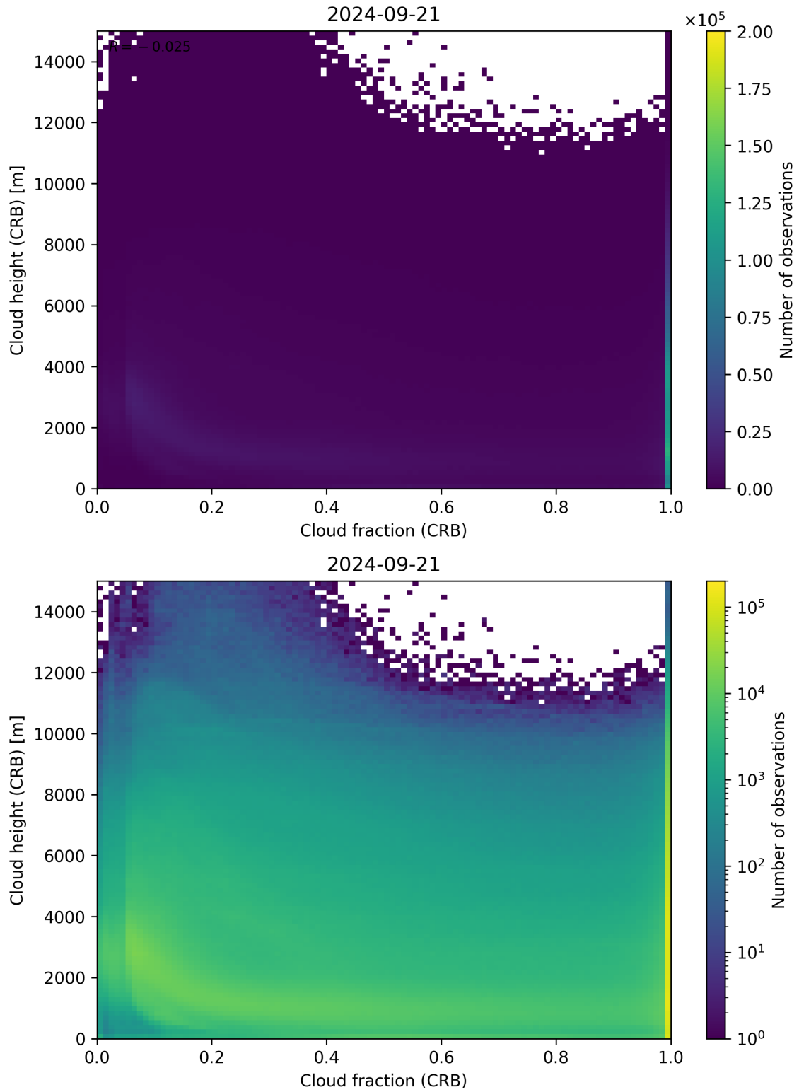
Figure 79: Scatter density plot of “Cloud fraction (CRB)” against “Cloud height (CRB)” for 2024-09-20 to 2024-09-22.
