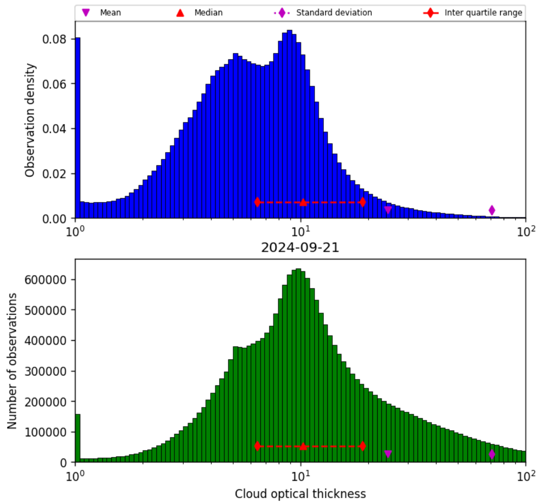
Figure 41: Histogram of “Cloud optical thickness” for 2024-09-20 to 2024-09-22
