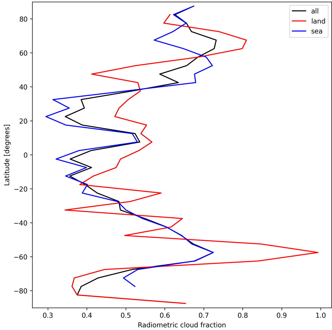
Figure 23: Zonal average of “Radiometric cloud fraction” for 2024-09-20 to 2024-09-22.
