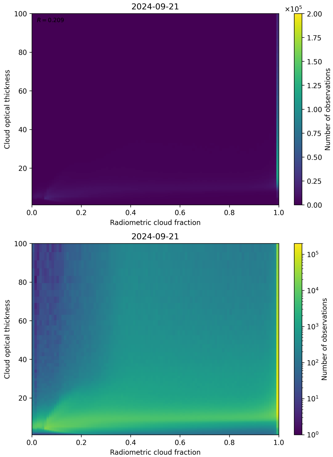
Figure 75: Scatter density plot of “Radiometric cloud fraction” against “Cloud optical thickness” for 2024-09-20 to 2024-09-22.
