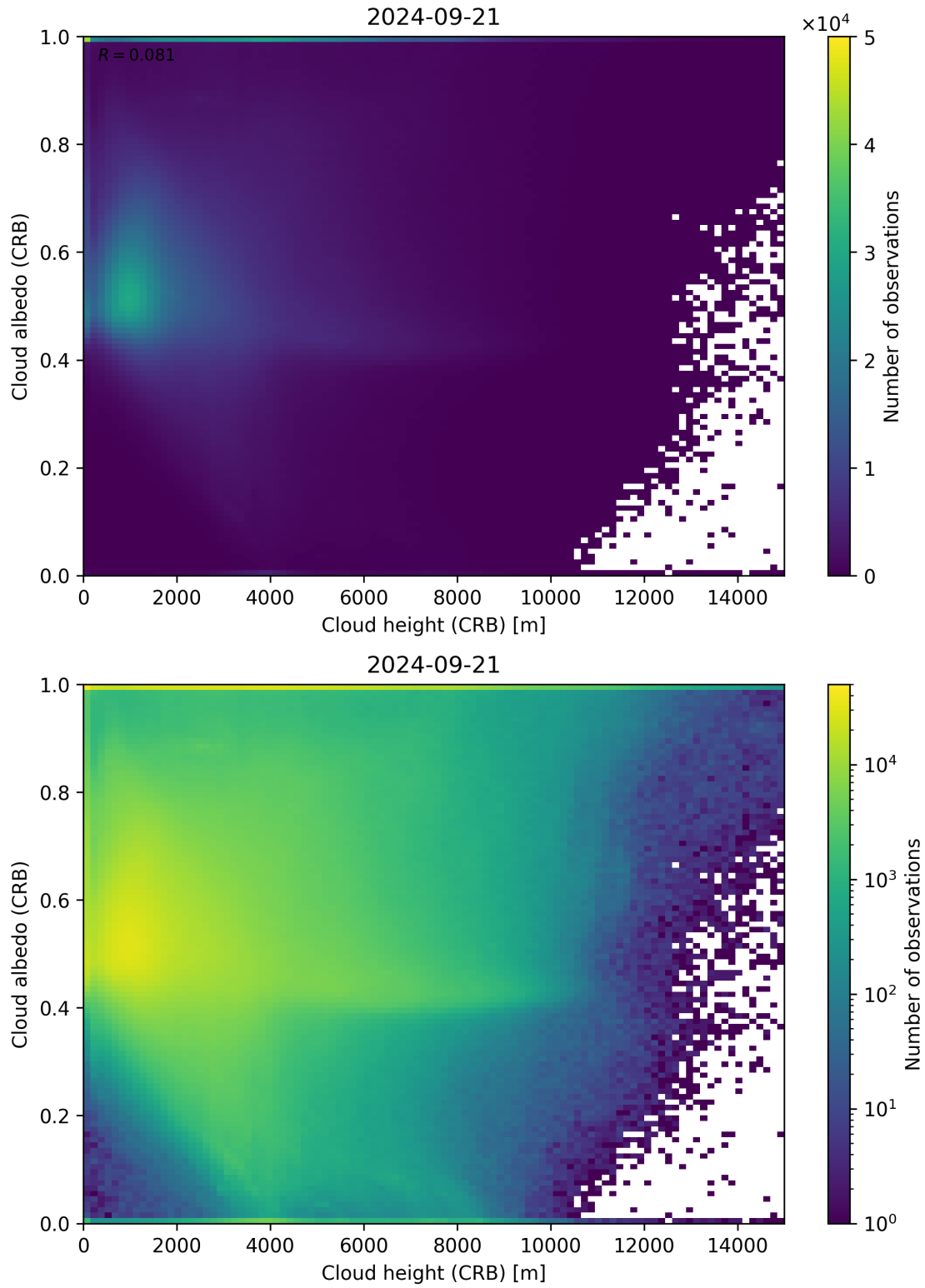
Figure 80: Scatter density plot of “Cloud height (CRB)” against “Cloud albedo (CRB)” for 2024-09-20 to 2024-09-22.
