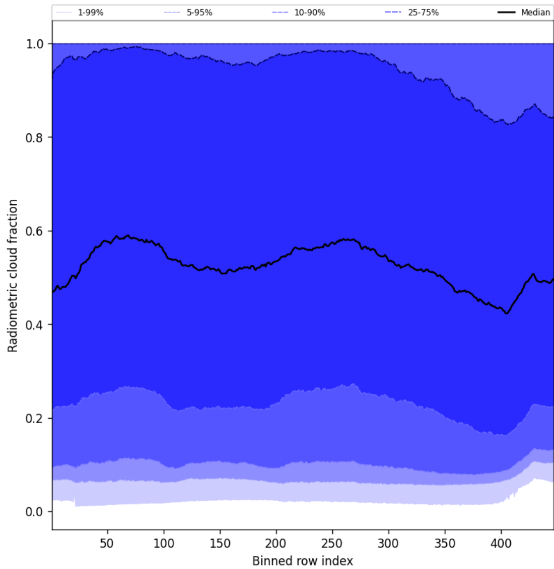
Figure 55: Along track statistics of “Radiometric cloud fraction” for 2024-09-20 to 2024-09-22
