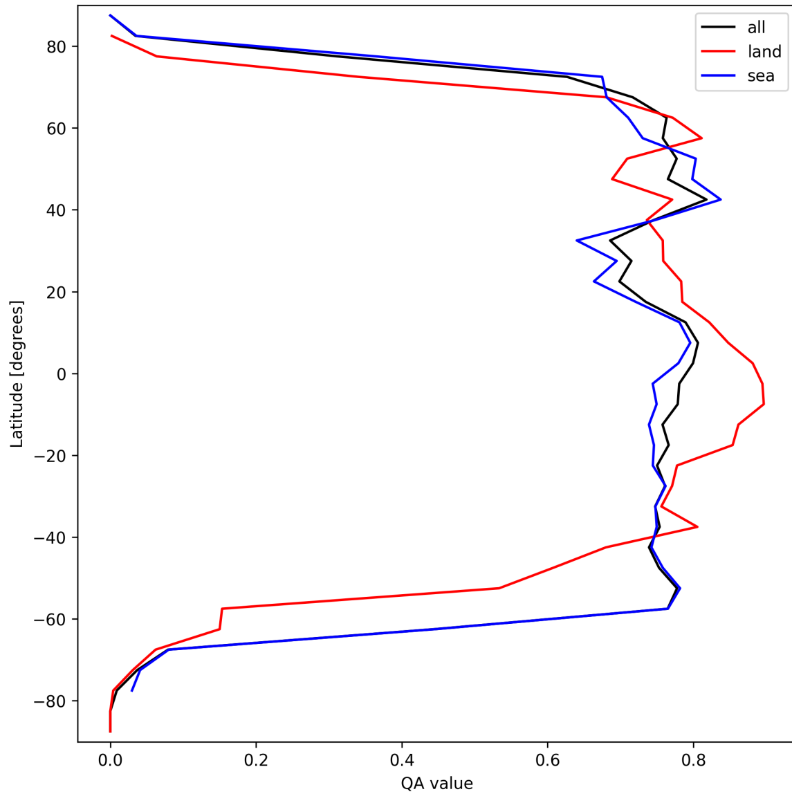
Figure 22: Zonal average of “QA value” for 2024-09-20 to 2024-09-22.
