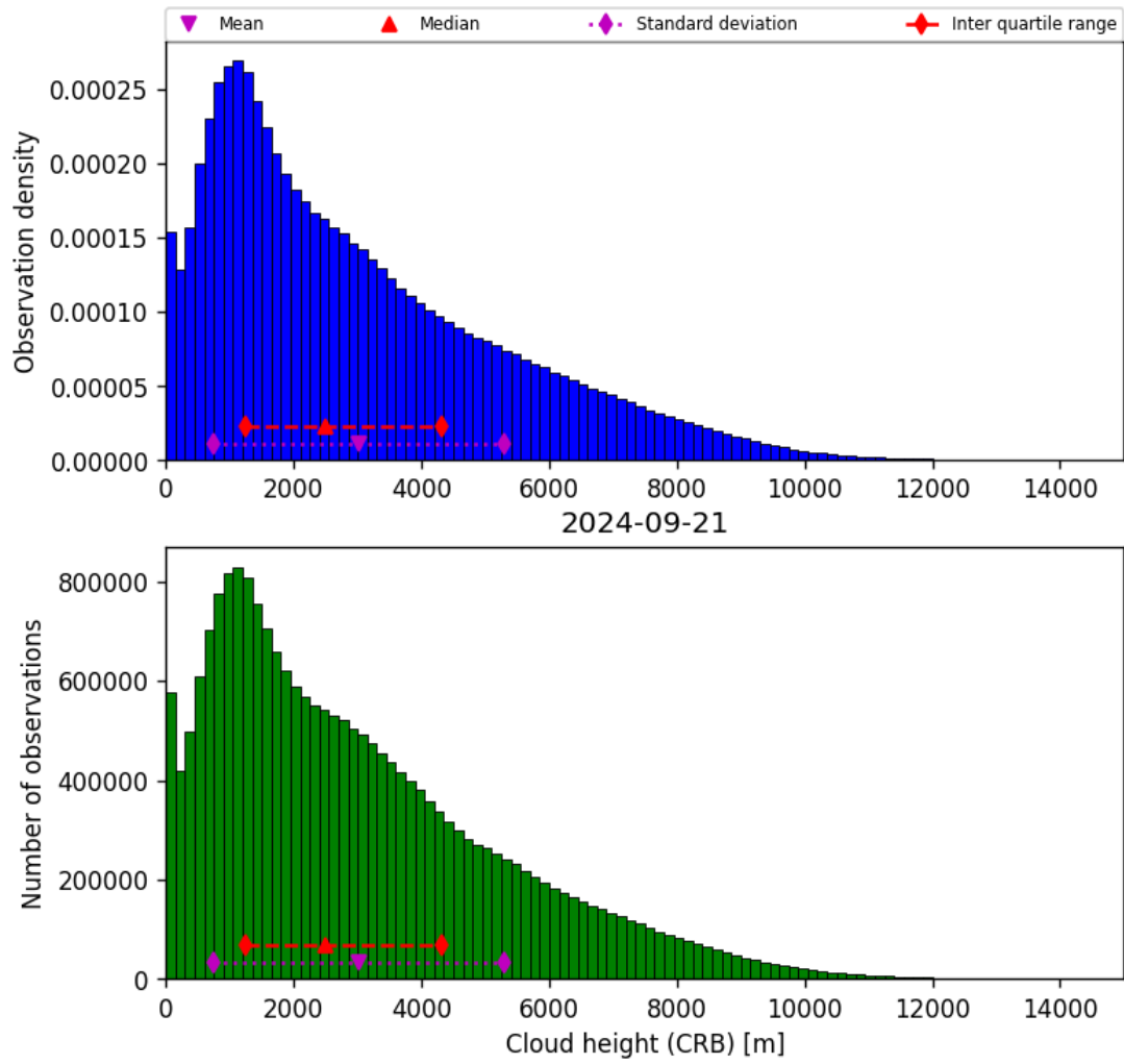
Figure 43: Histogram of “Cloud height (CRB)” for 2024-09-20 to 2024-09-22
