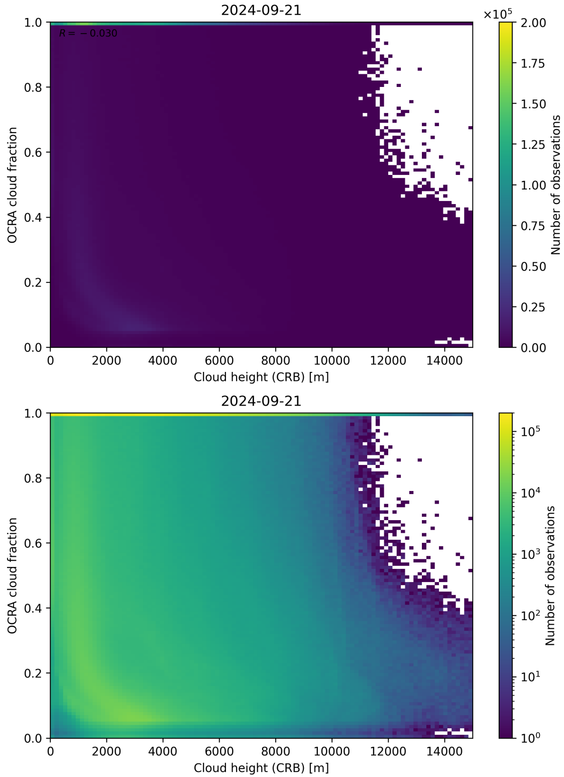
Figure 81: Scatter density plot of “Cloud height (CRB)” against “OCRA cloud fraction” for 2024-09-20 to 2024-09-22.
