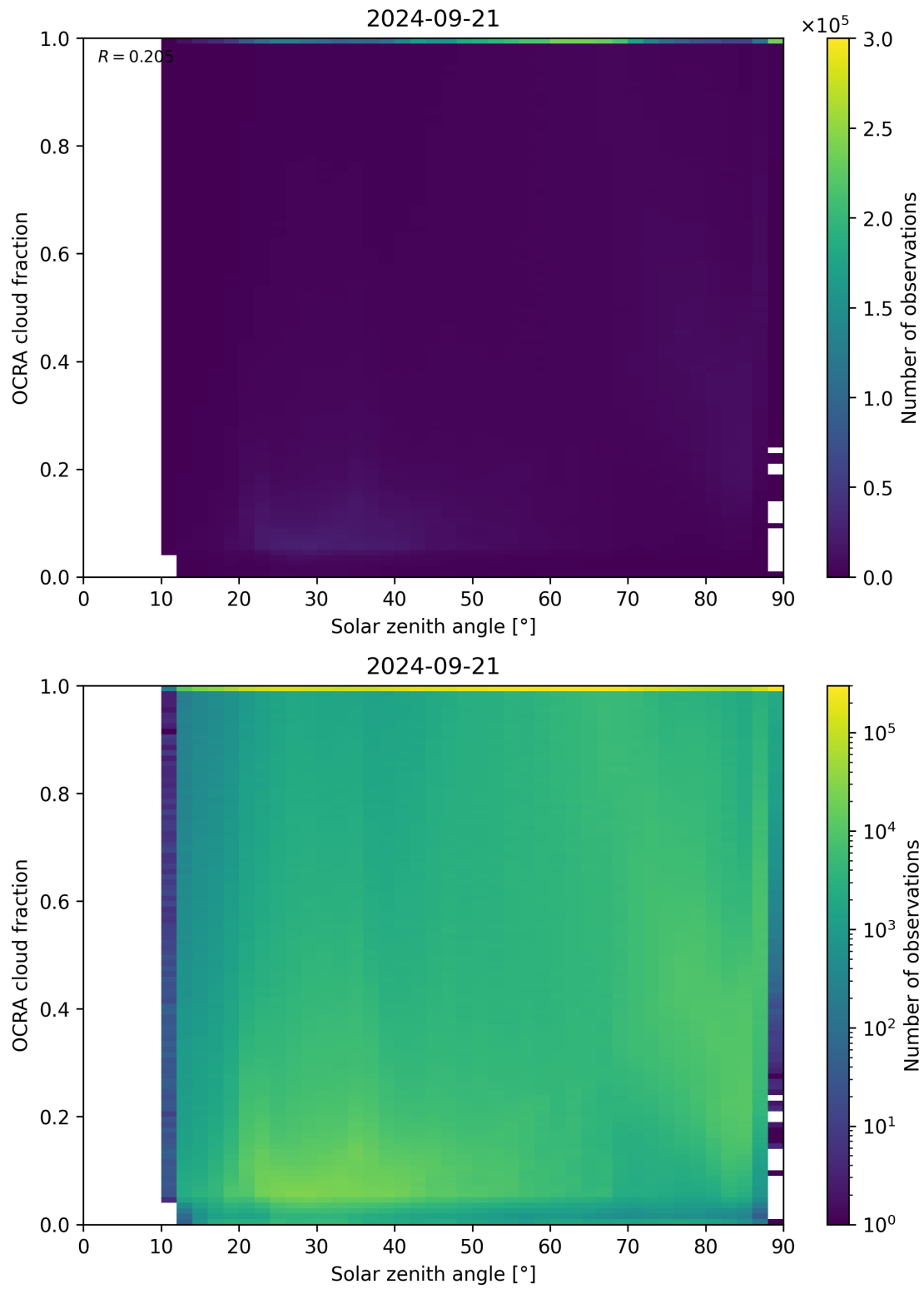
Figure 100: Scatter density plot of “Solar zenith angle” against “OCRA cloud fraction” for 2024-09-20 to 2024-09-22.
