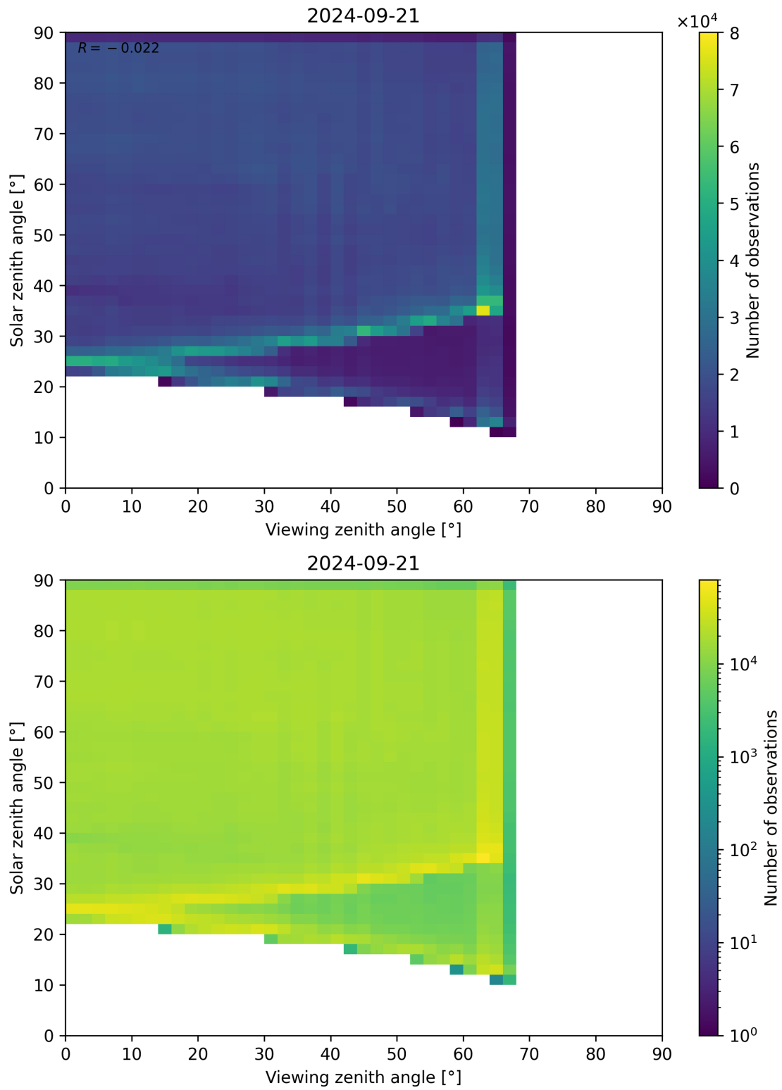
Figure 114: Scatter density plot of “Viewing zenith angle” against “Solar zenith angle” for 2024-09-20 to 2024-09-22.
