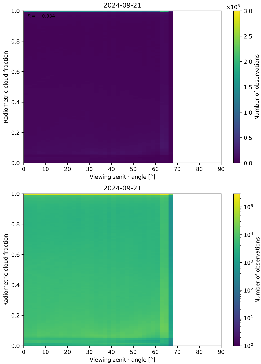
Figure 107: Scatter density plot of “Viewing zenith angle” against “Radiometric cloud fraction” for 2024-09-20 to 2024-09-22.
