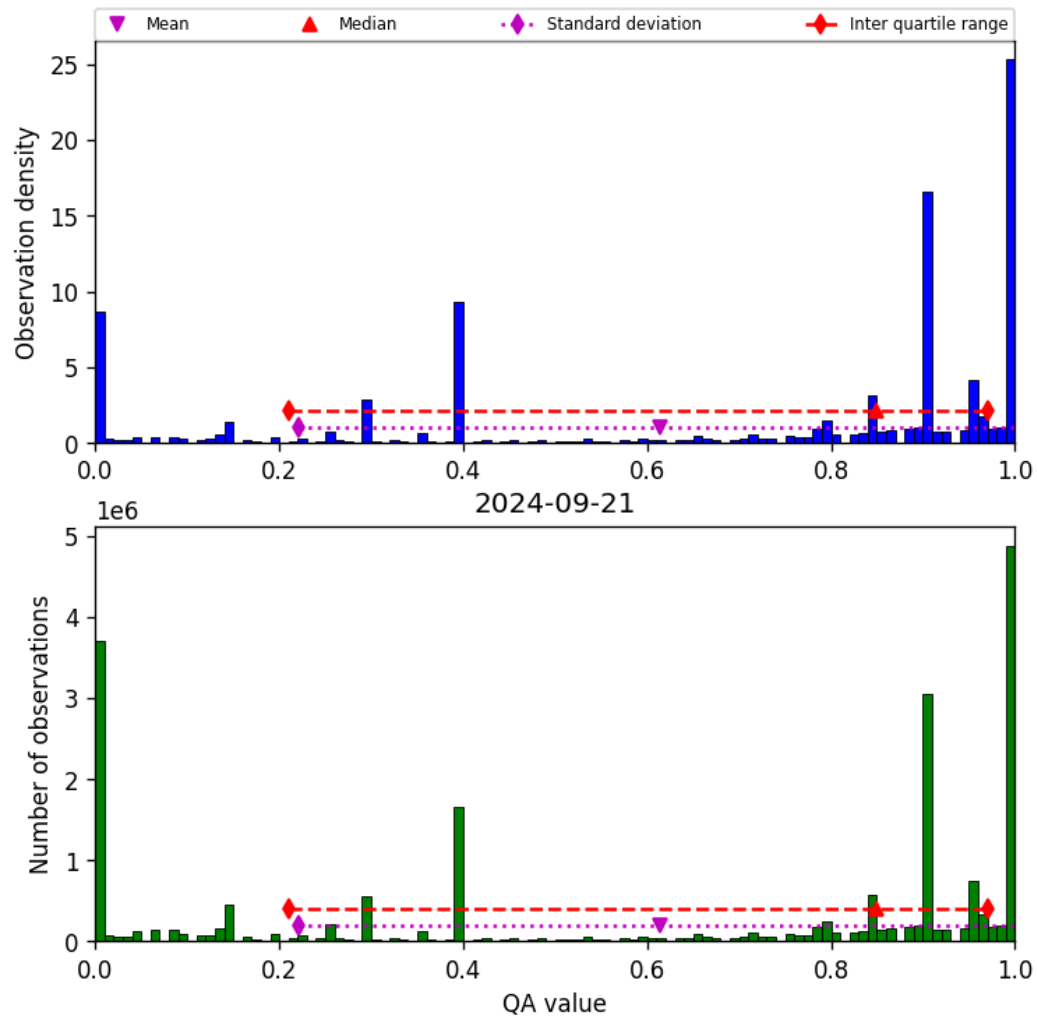
Figure 38: Histogram of “QA value” for 2024-09-20 to 2024-09-22
