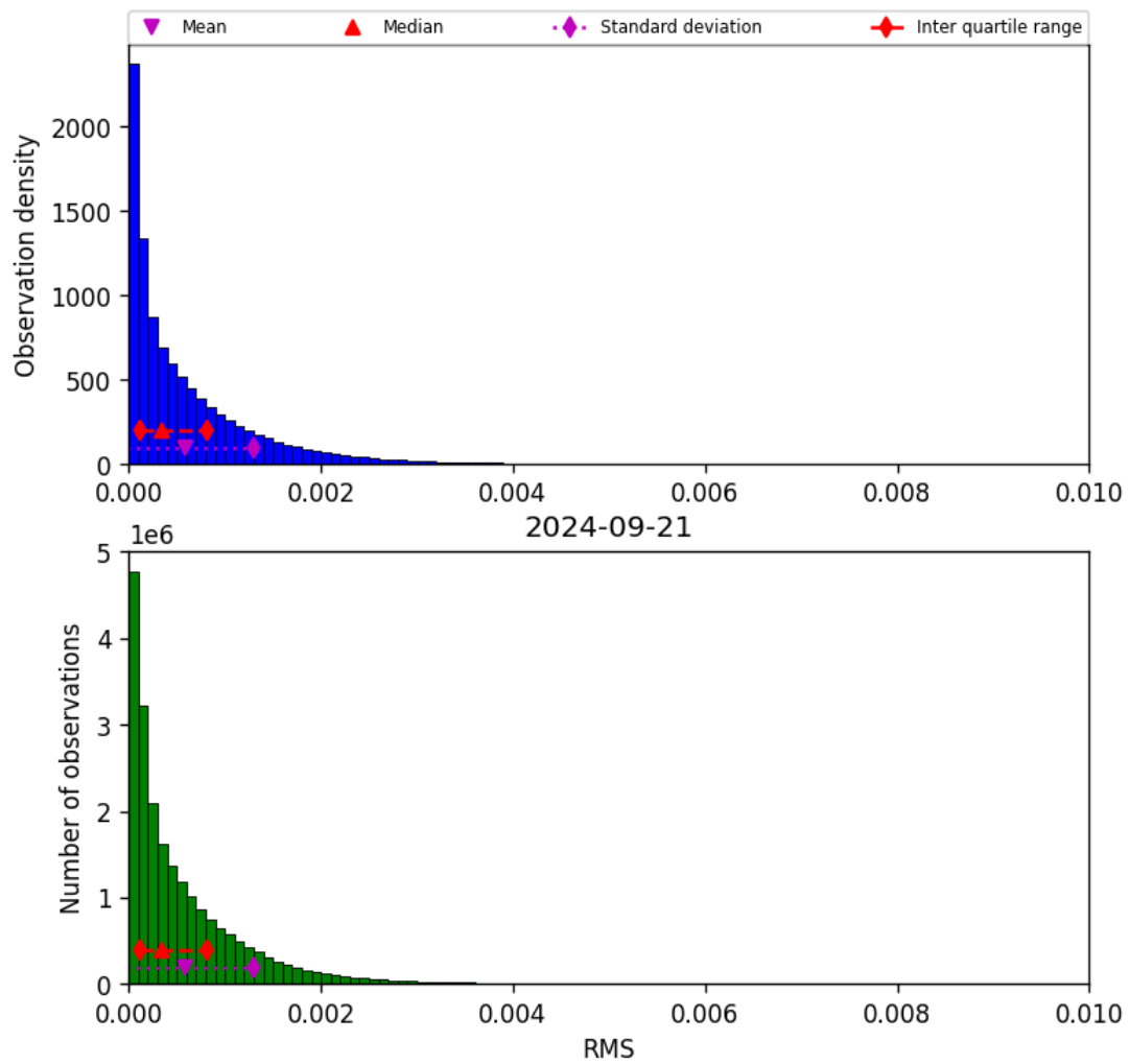
Figure 47: Histogram of “RMS” for 2024-09-20 to 2024-09-22
