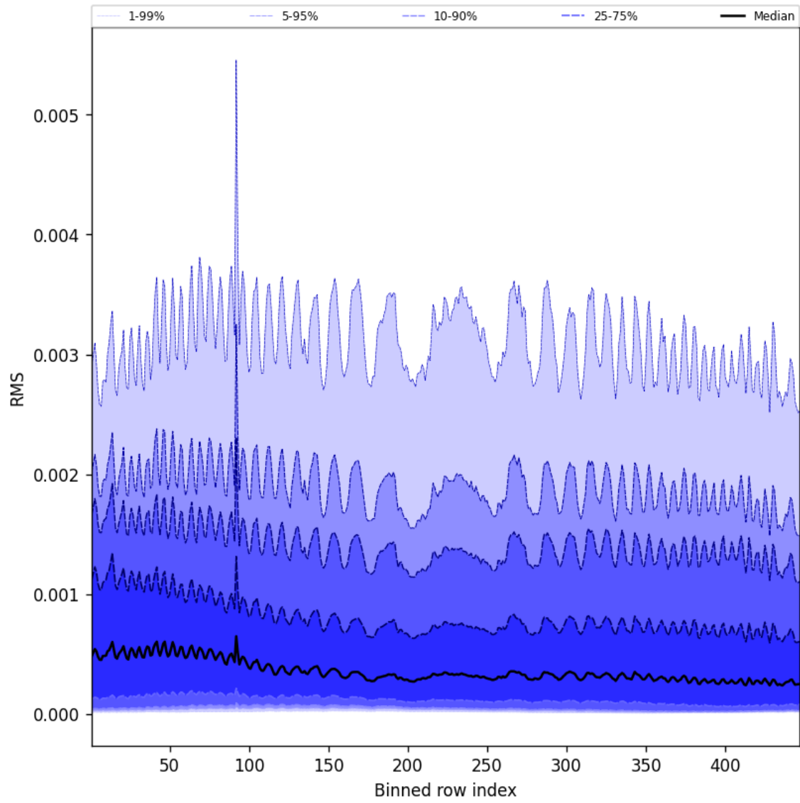
Figure 63: Along track statistics of "RMS" for 2024-09-20 to 2024-09-22
