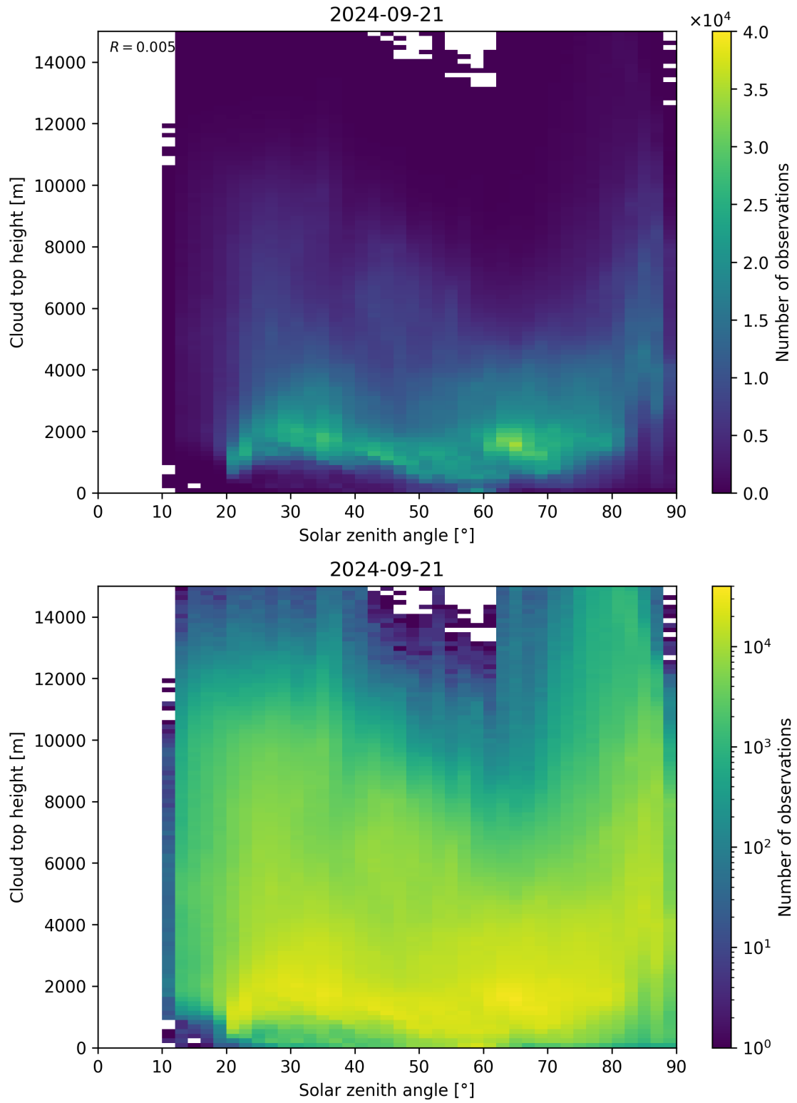
Figure 104: Scatter density plot of “Solar zenith angle” against “Cloud top height” for 2024-09-20 to 2024-09-22.
