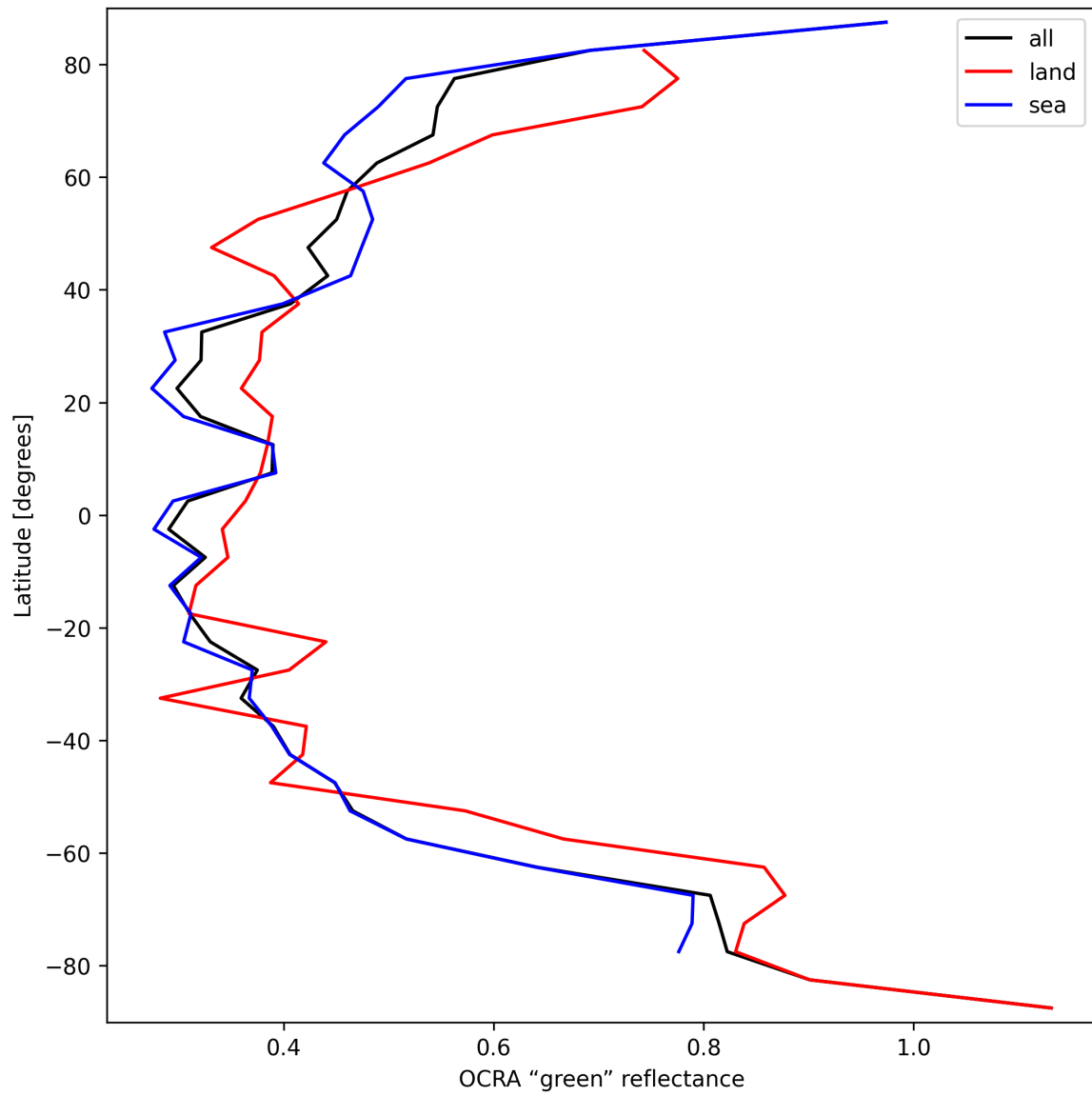
Figure 36: Zonal average of “OCRA “green” reflectance” for 2024-09-20 to 2024-09-22.
