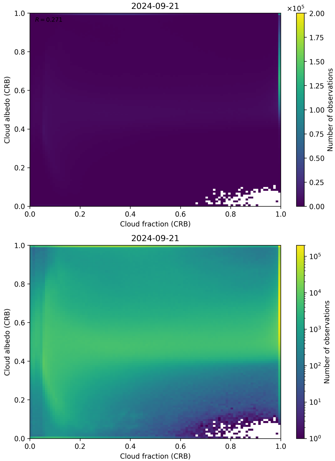
Figure 77: Scatter density plot of “Cloud fraction (CRB)” against “Cloud albedo (CRB)” for 2024-09-20 to 2024-09-22.
