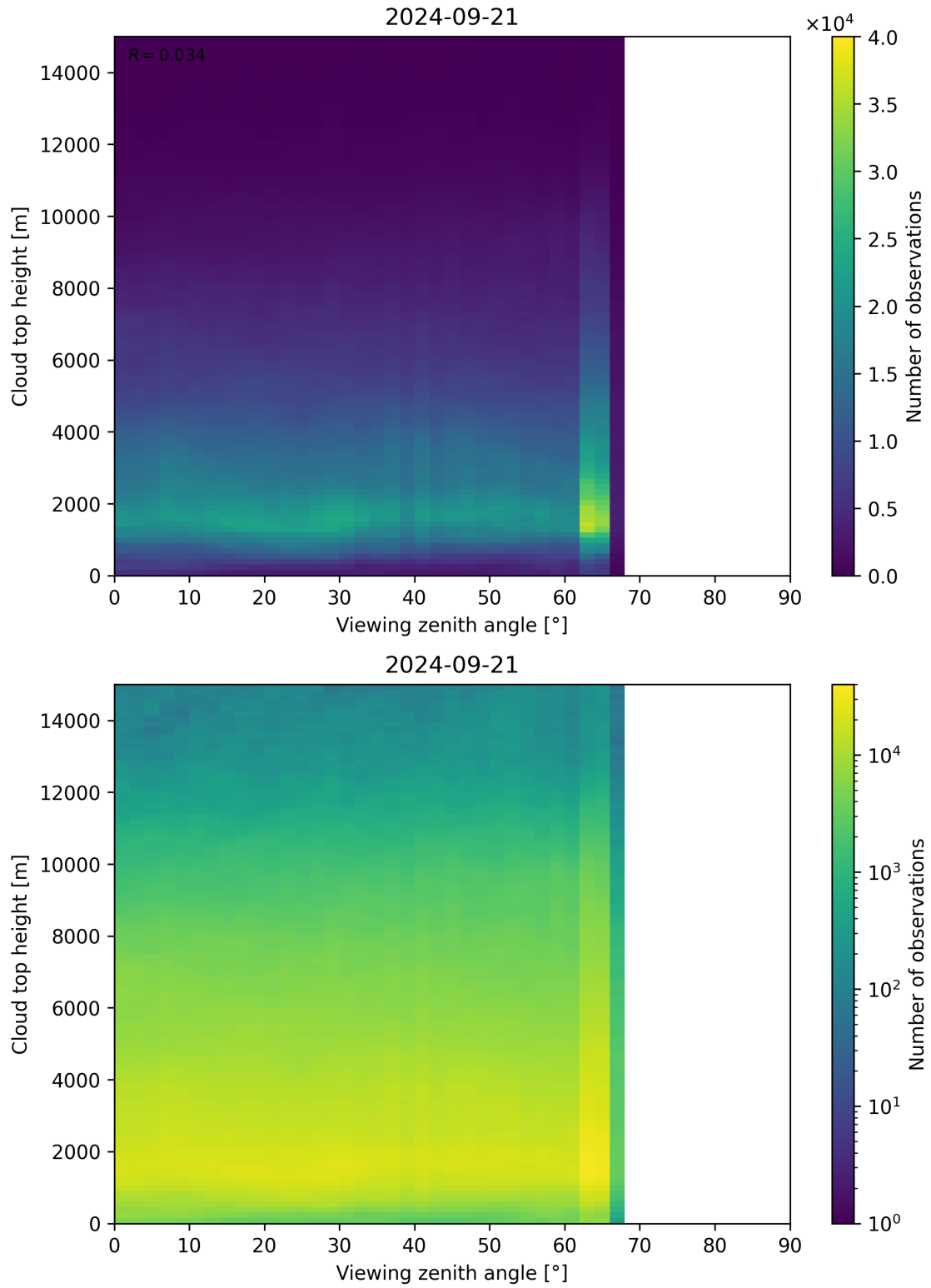
Figure 112: Scatter density plot of “Viewing zenith angle” against “Cloud top height” for 2024-09-20 to 2024-09-22.
