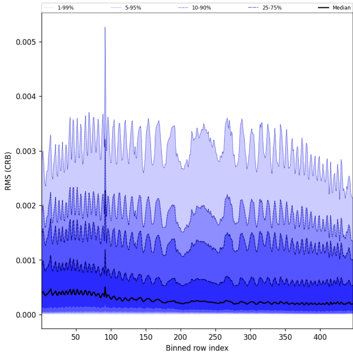
Figure 64: Along track statistics of “RMS (CRB)” for 2024-09-20 to 2024-09-22
