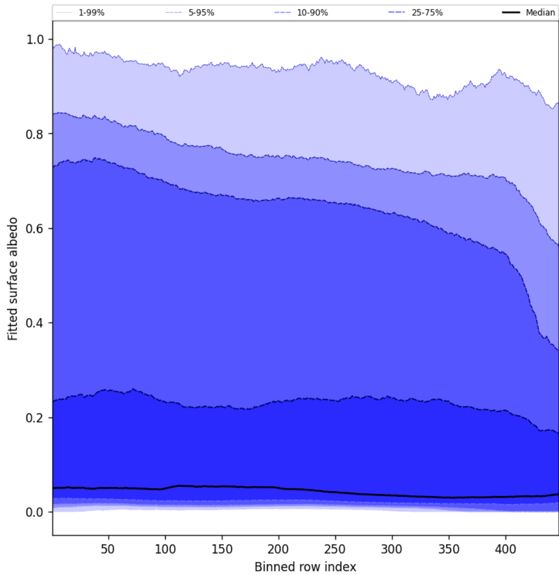
Figure 61: Along track statistics of “Fitted surface albedo” for 2024-09-20 to 2024-09-22
