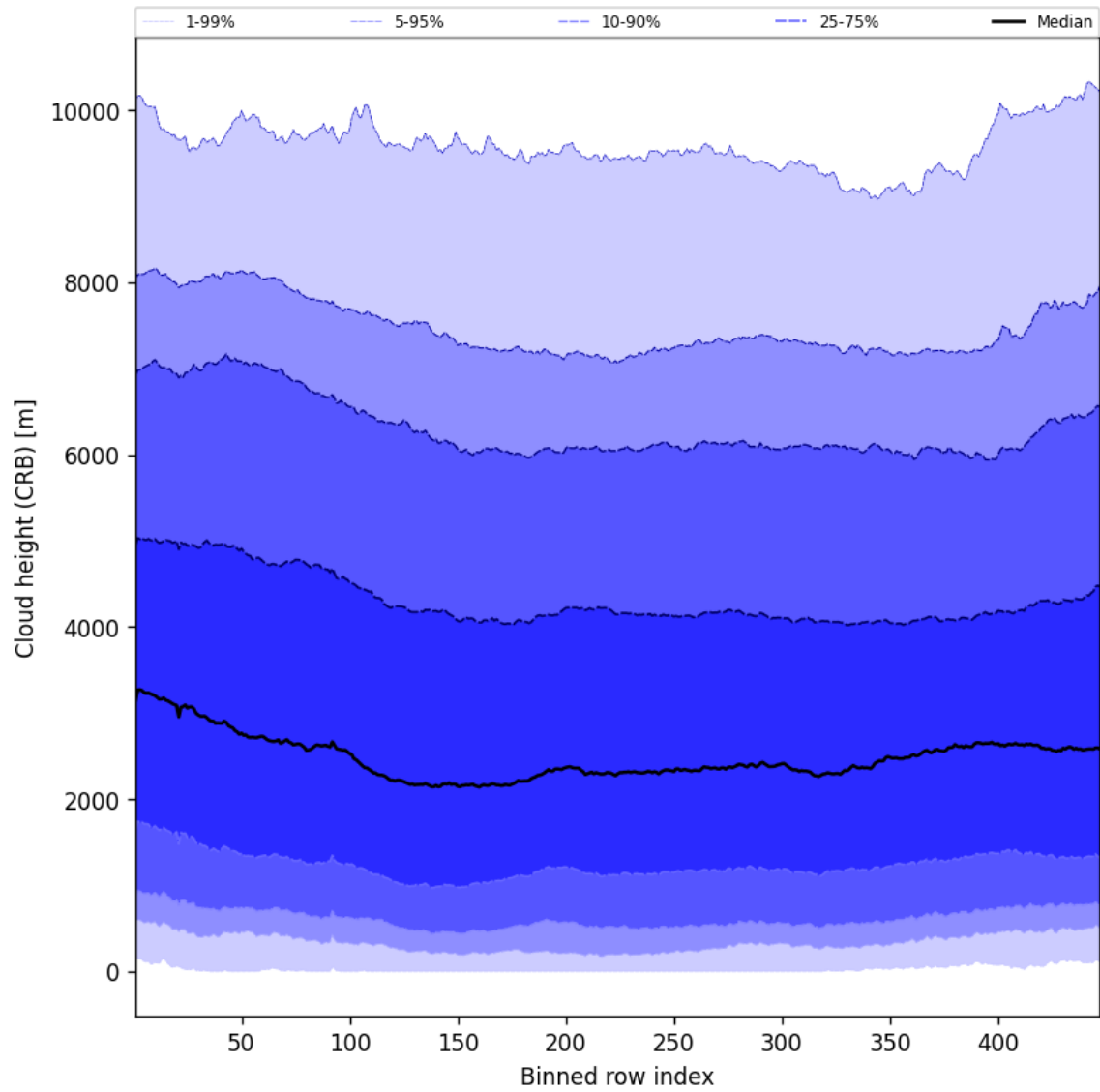
Figure 59: Along track statistics of “Cloud height (CRB)” for 2024-09-20 to 2024-09-22
