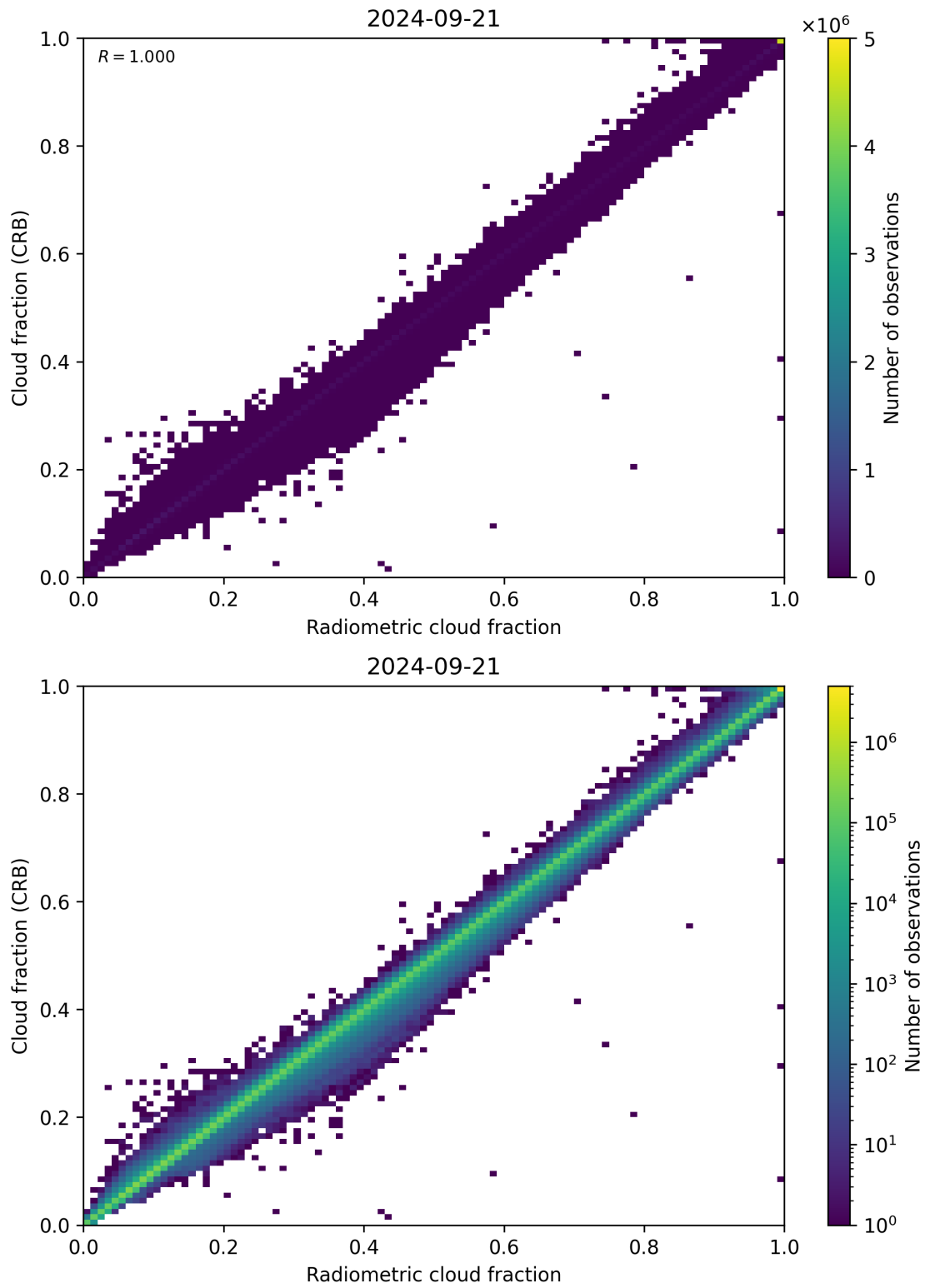
Figure 73: Scatter density plot of “Radiometric cloud fraction” against “Cloud fraction (CRB)” for 2024-09-20 to 2024-09-22.
