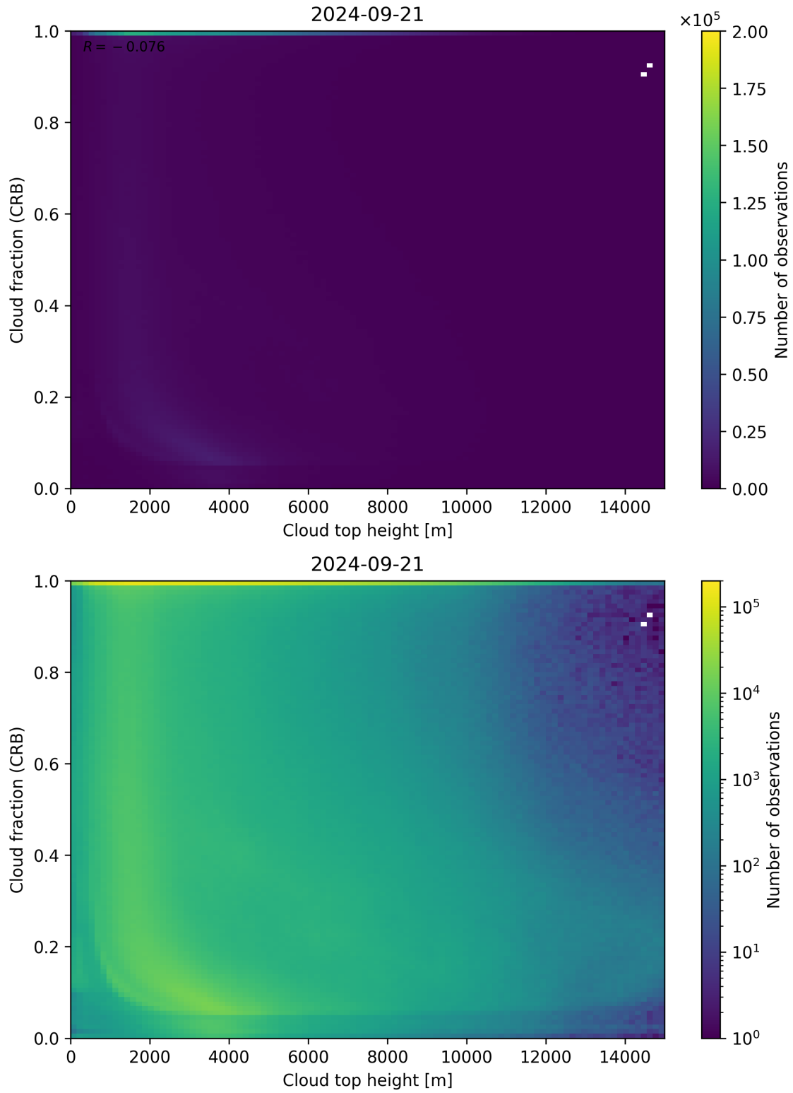
Figure 88: Scatter density plot of “Cloud top height” against “Cloud fraction (CRB)” for 2024-09-20 to 2024-09-22.
