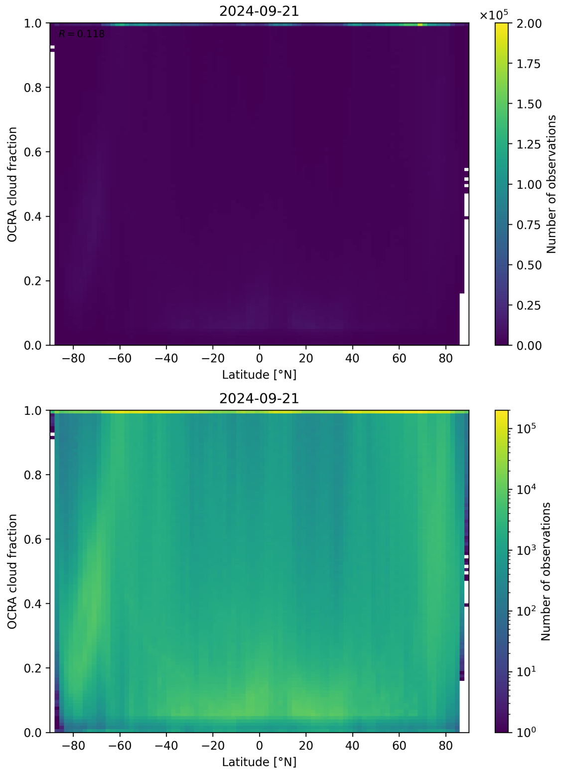
Figure 93: Scatter density plot of “Latitude” against “OCRA cloud fraction” for 2024-09-20 to 2024-09-22.
