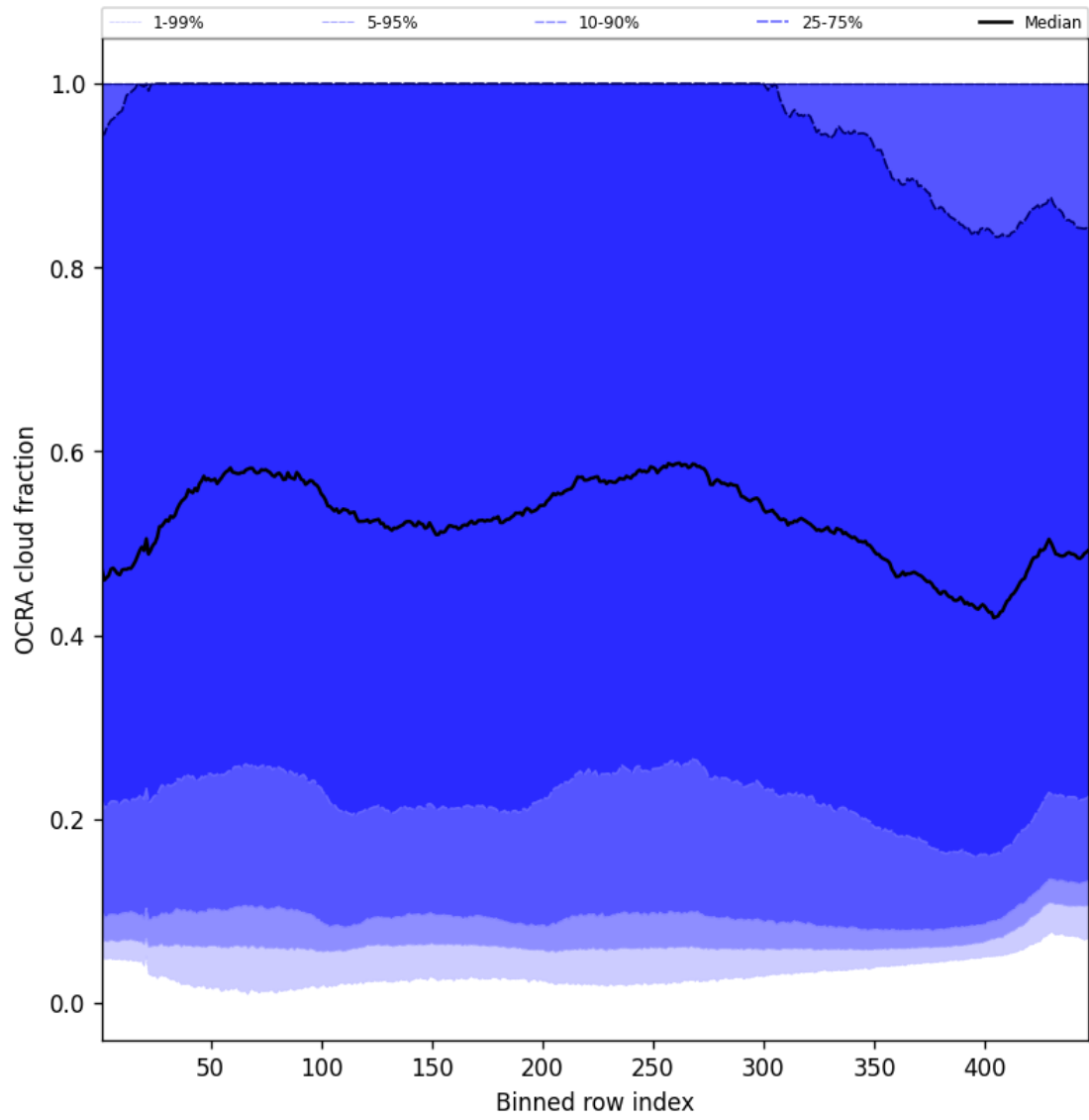
Figure 66: Along track statistics of “OCRA cloud fraction” for 2024-09-20 to 2024-09-22
