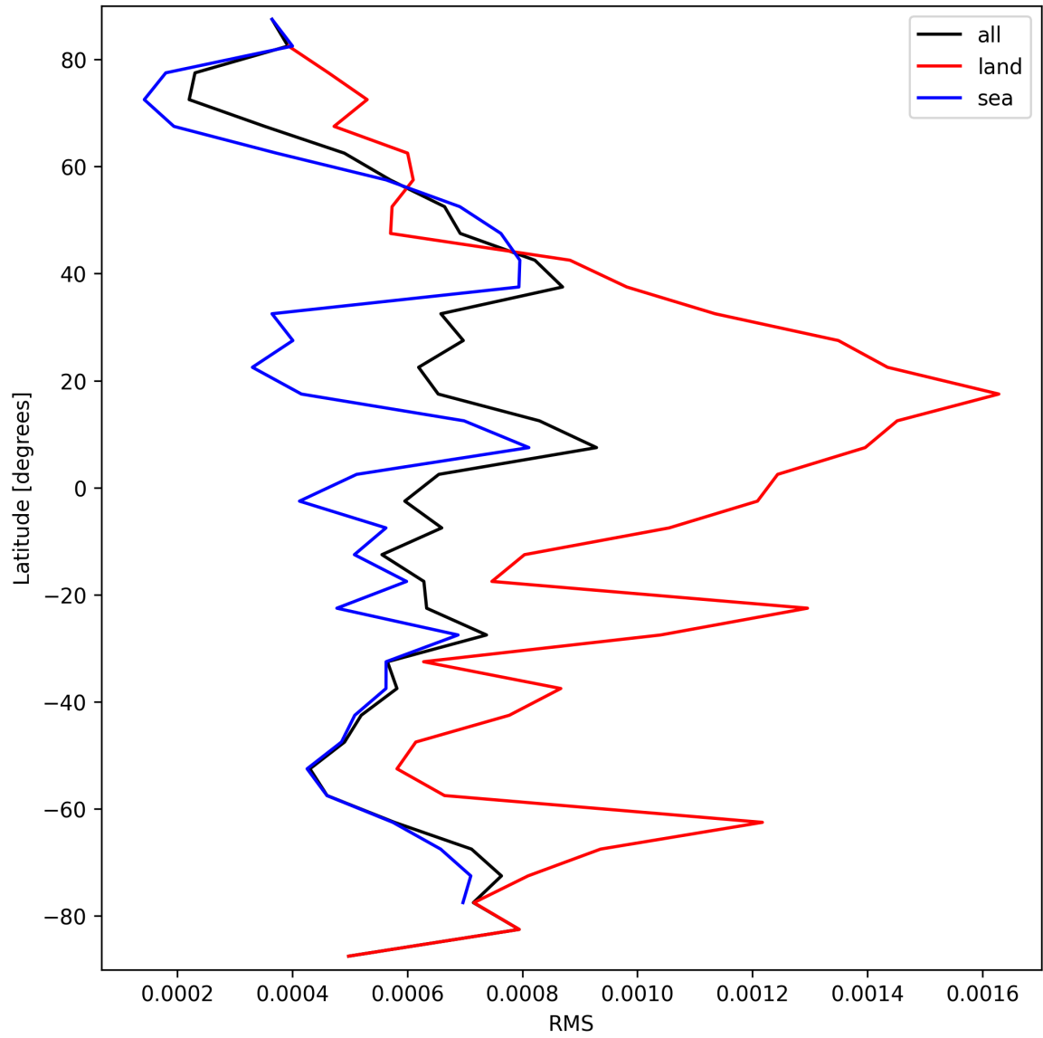
Figure 31: Zonal average of “RMS” for 2024-09-20 to 2024-09-22.
