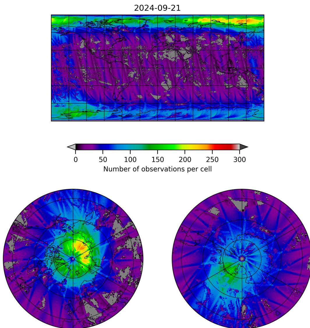
Figure 21: Map of the number of observations for 2024-09-20 to 2024-09-22
