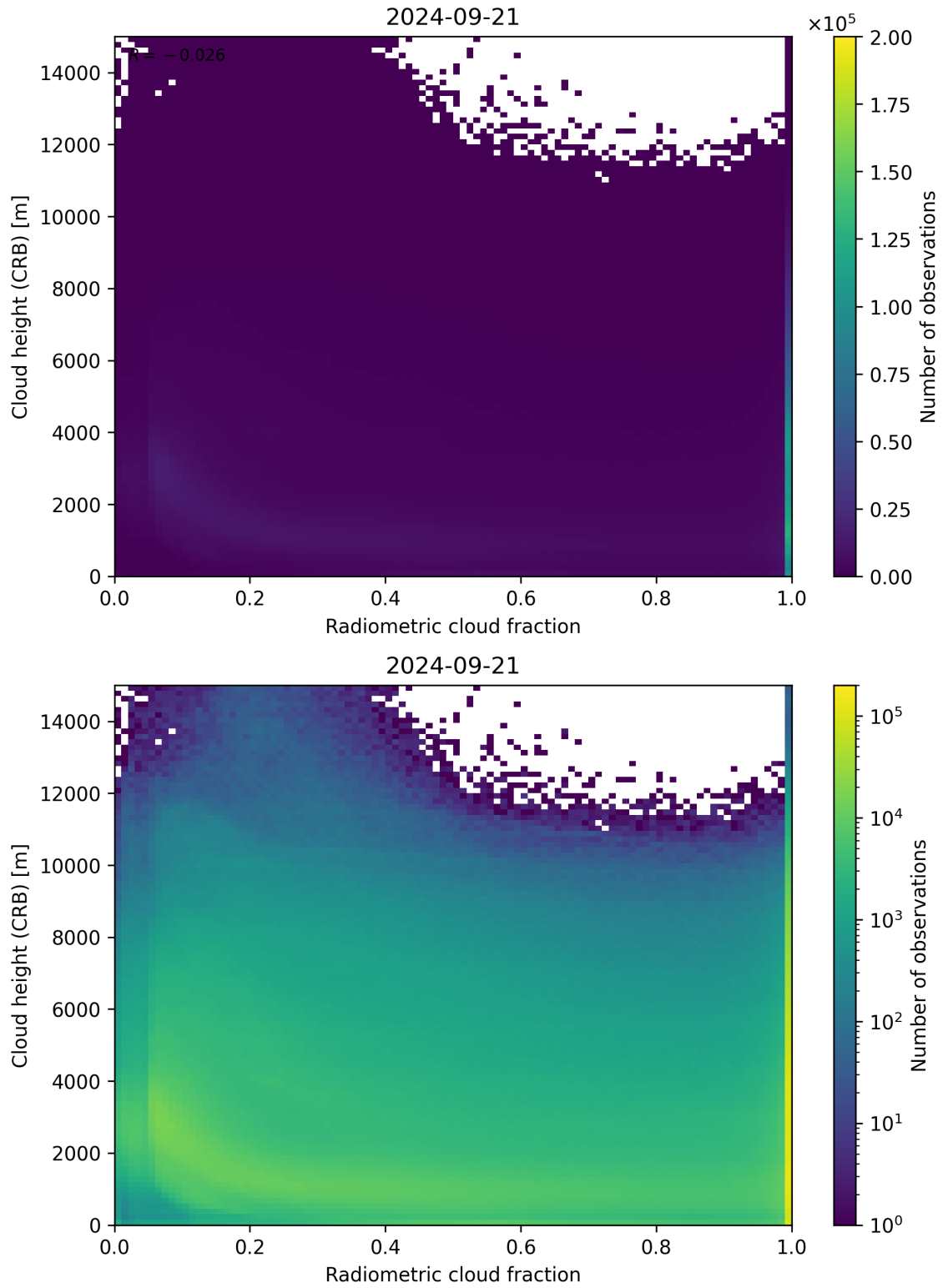
Figure 74: Scatter density plot of “Radiometric cloud fraction” against “Cloud height (CRB)” for 2024-09-20 to 2024-09-22.
