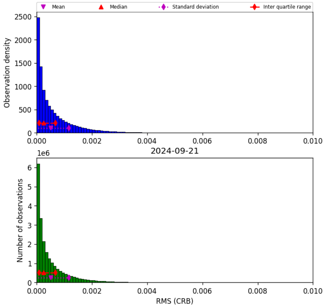
Figure 48: Histogram of “RMS (CRB)” for 2024-09-20 to 2024-09-22
