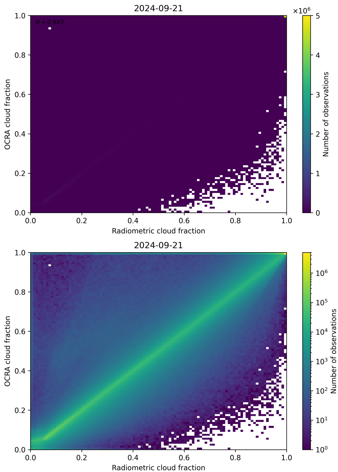
Figure 72: Scatter density plot of “Radiometric cloud fraction” against “OCRA cloud fraction” for 2024-09-20 to 2024-09-22.
