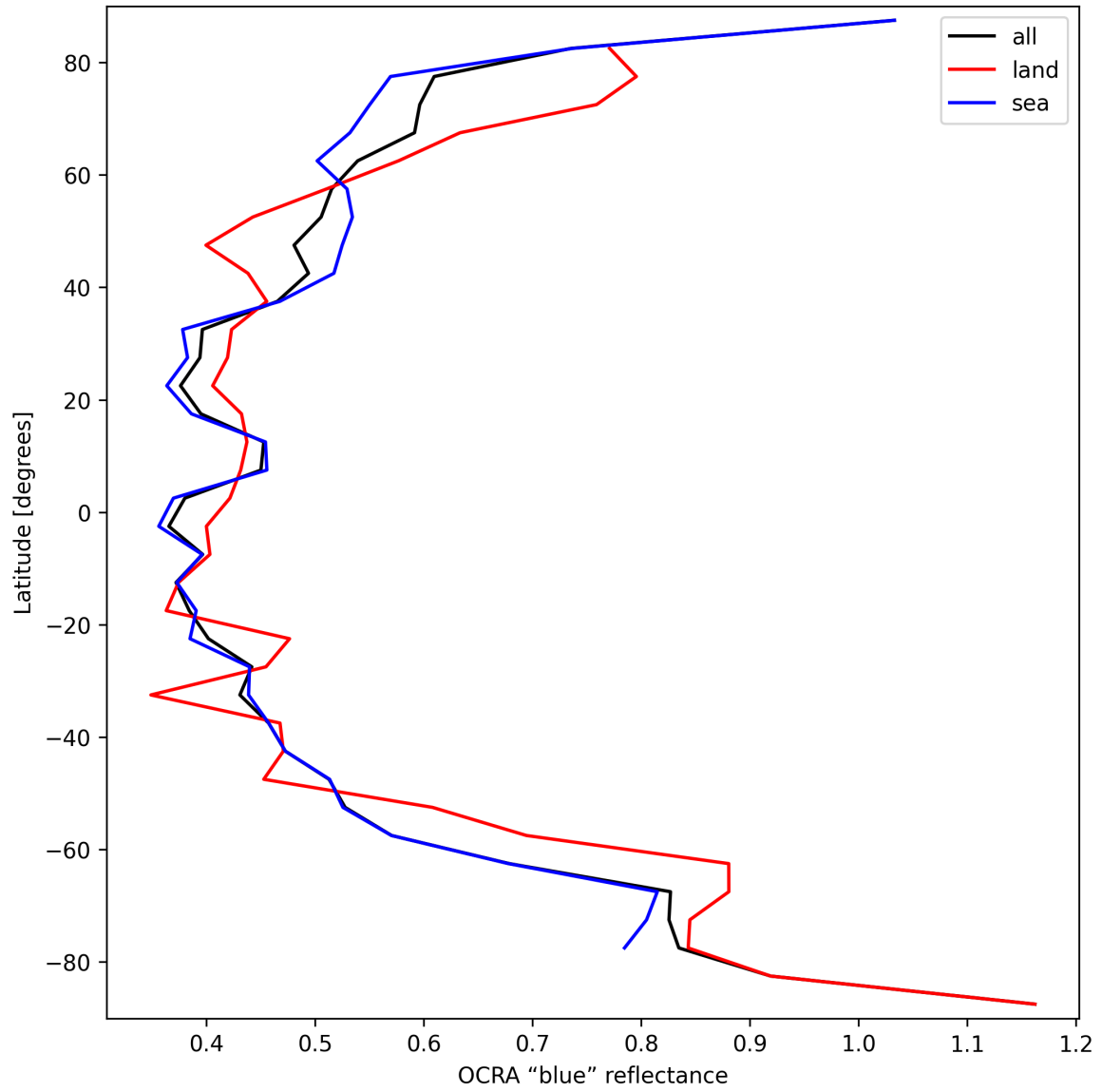
Figure 35: Zonal average of “OCRA “blue” reflectance” for 2024-09-20 to 2024-09-22.
