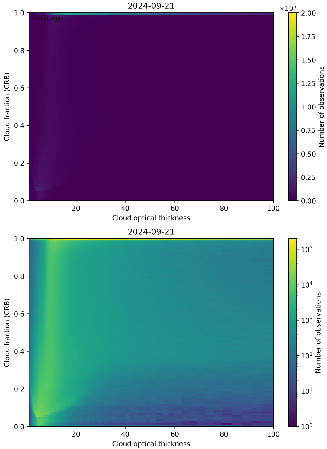
Figure 84: Scatter density plot of “Cloud optical thickness” against “Cloud fraction (CRB)” for 2024-09-20 to 2024-09-22.
