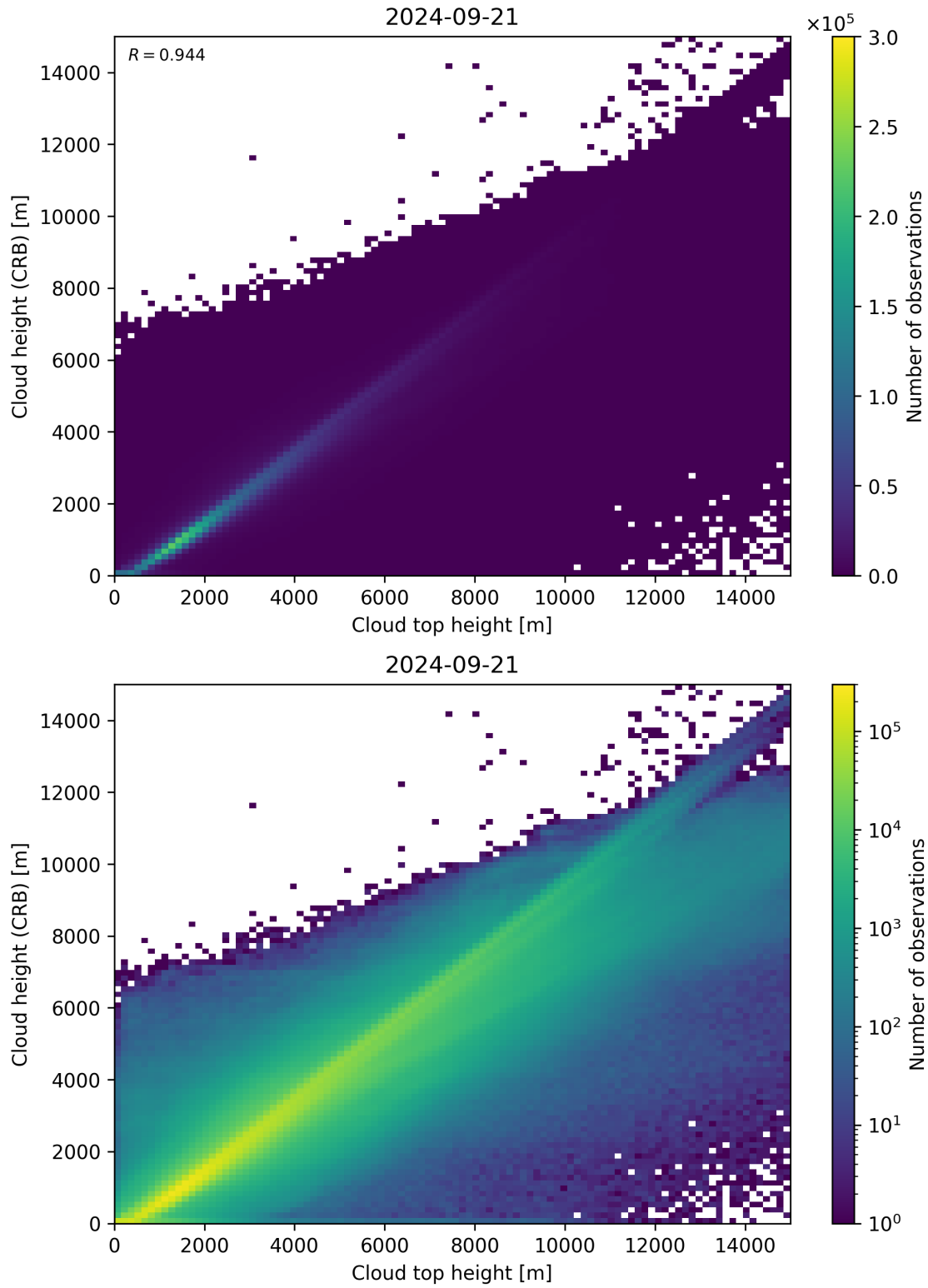
Figure 89: Scatter density plot of “Cloud top height” against “Cloud height (CRB)” for 2024-09-20 to 2024-09-22.
