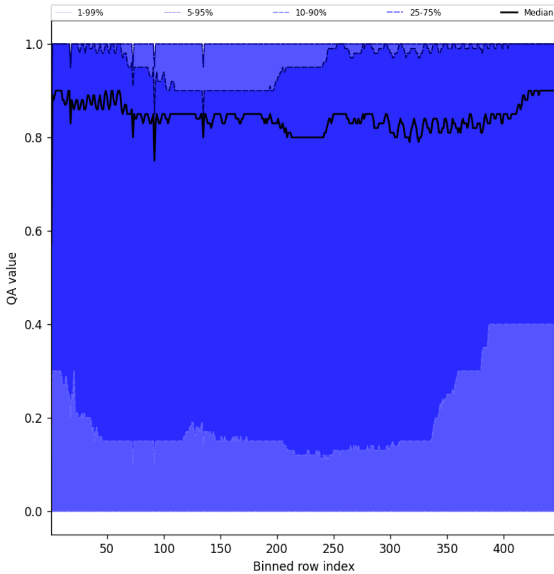
Figure 54: Along track statistics of “QA value” for 2024-09-20 to 2024-09-22
