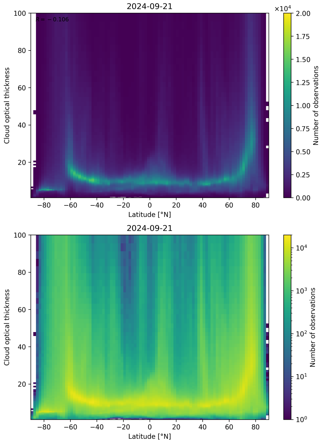
Figure 96: Scatter density plot of “Latitude” against “Cloud optical thickness” for 2024-09-20 to 2024-09-22.
