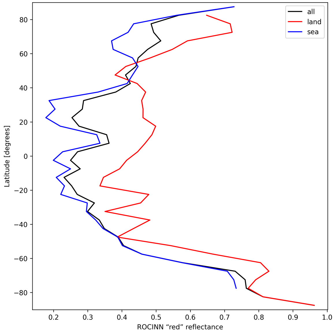
Figure 37: Zonal average of “ROCINN “red” reflectance” for 2024-09-20 to 2024-09-22.
