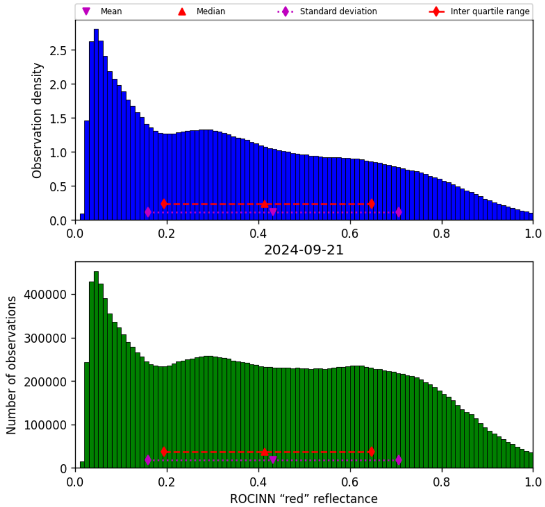
Figure 53: Histogram of “ROCINN “red” reflectance” for 2024-09-20 to 2024-09-22
