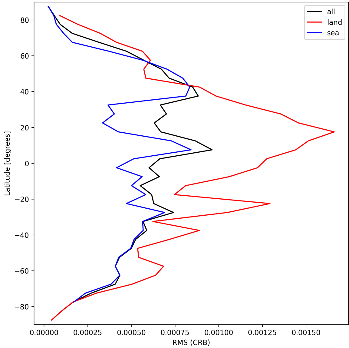
Figure 32: Zonal average of “RMS (CRB)” for 2024-09-20 to 2024-09-22.
