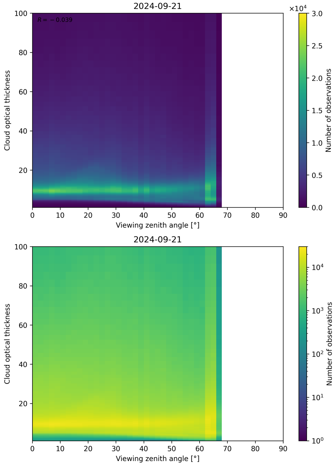
Figure 111: Scatter density plot of “Viewing zenith angle” against “Cloud optical thickness” for 2024-09-20 to 2024-09-22.
