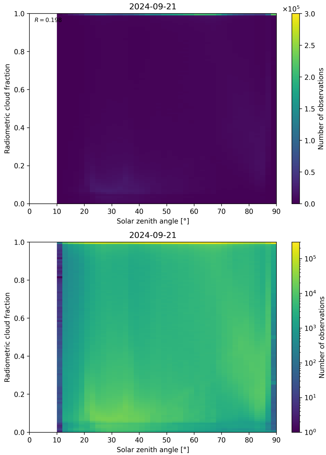
Figure 99: Scatter density plot of “Solar zenith angle” against “Radiometric cloud fraction” for 2024-09-20 to 2024-09-22.
