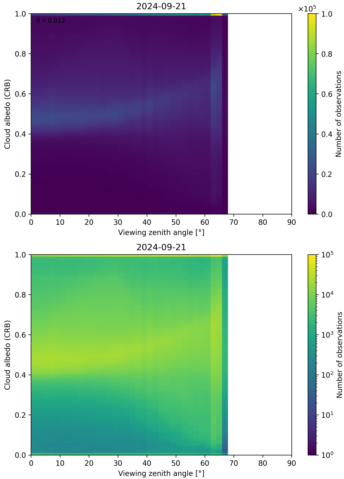
Figure 106: Scatter density plot of “Viewing zenith angle” against “Cloud albedo (CRB)” for 2024-09-20 to 2024-09-22.
