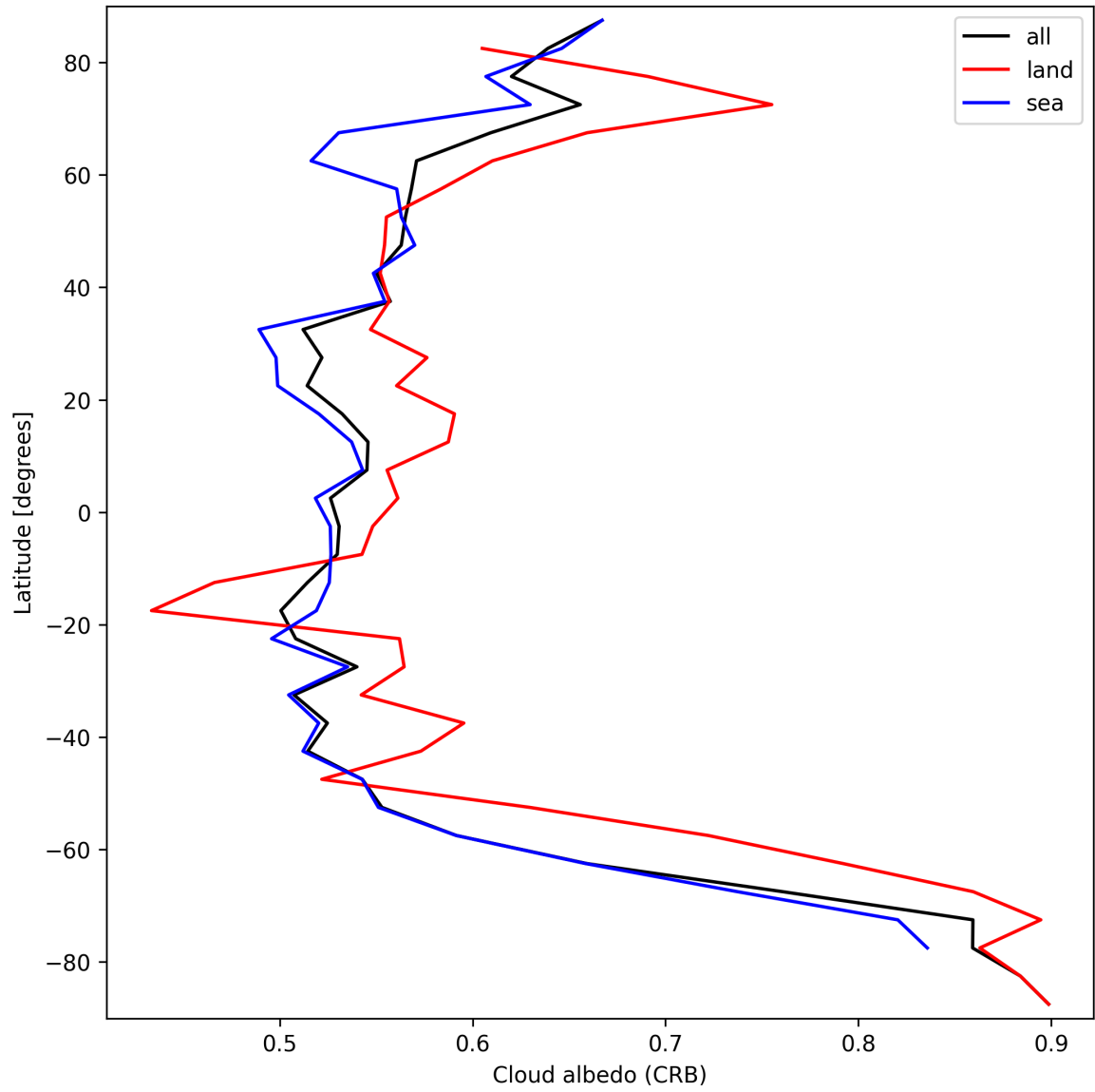
Figure 28: Zonal average of “Cloud albedo (CRB)” for 2024-09-20 to 2024-09-22.
