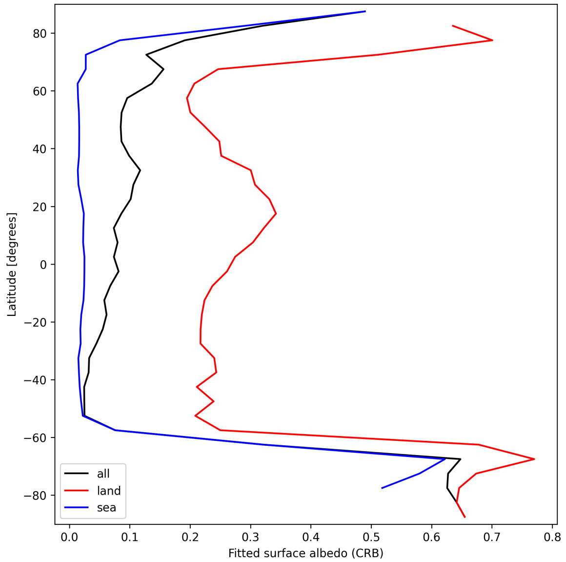
Figure 30: Zonal average of “Fitted surface albedo (CRB)” for 2024-09-20 to 2024-09-22.
