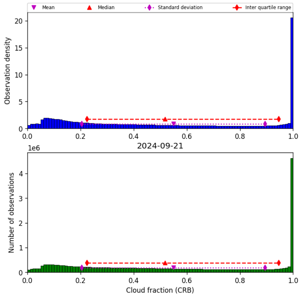
Figure 42: Histogram of “Cloud fraction (CRB)” for 2024-09-20 to 2024-09-22
