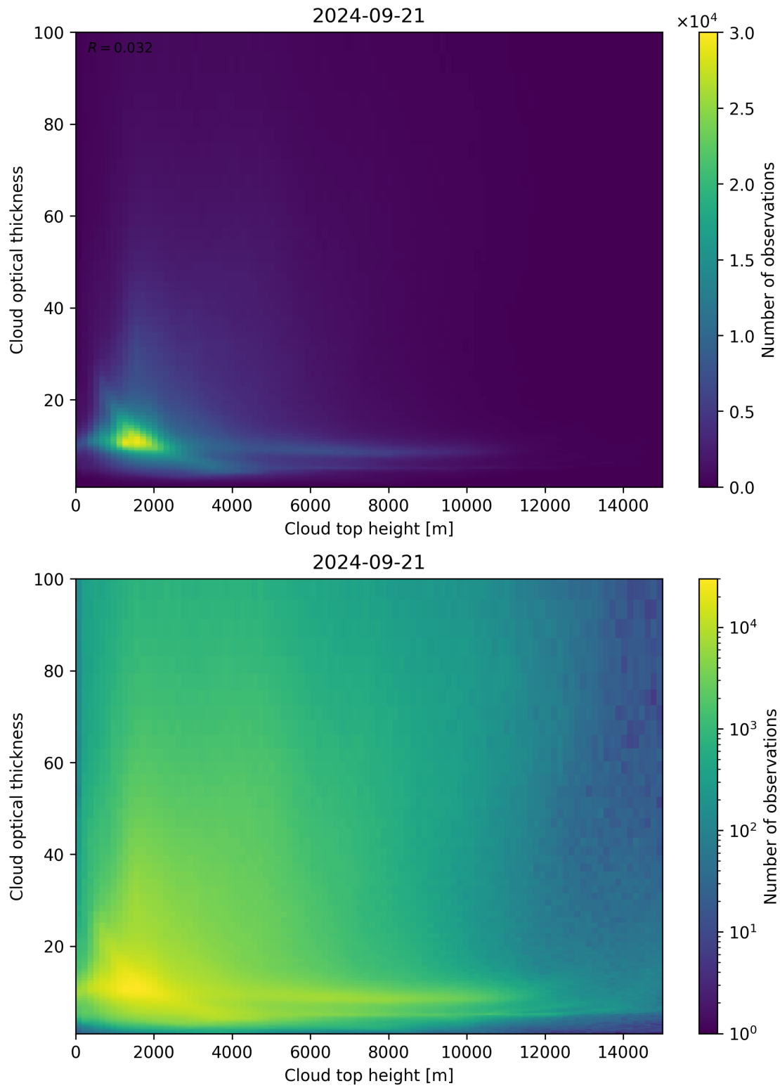
Figure 90: Scatter density plot of “Cloud top height” against “Cloud optical thickness” for 2024-09-20 to 2024-09-22.
