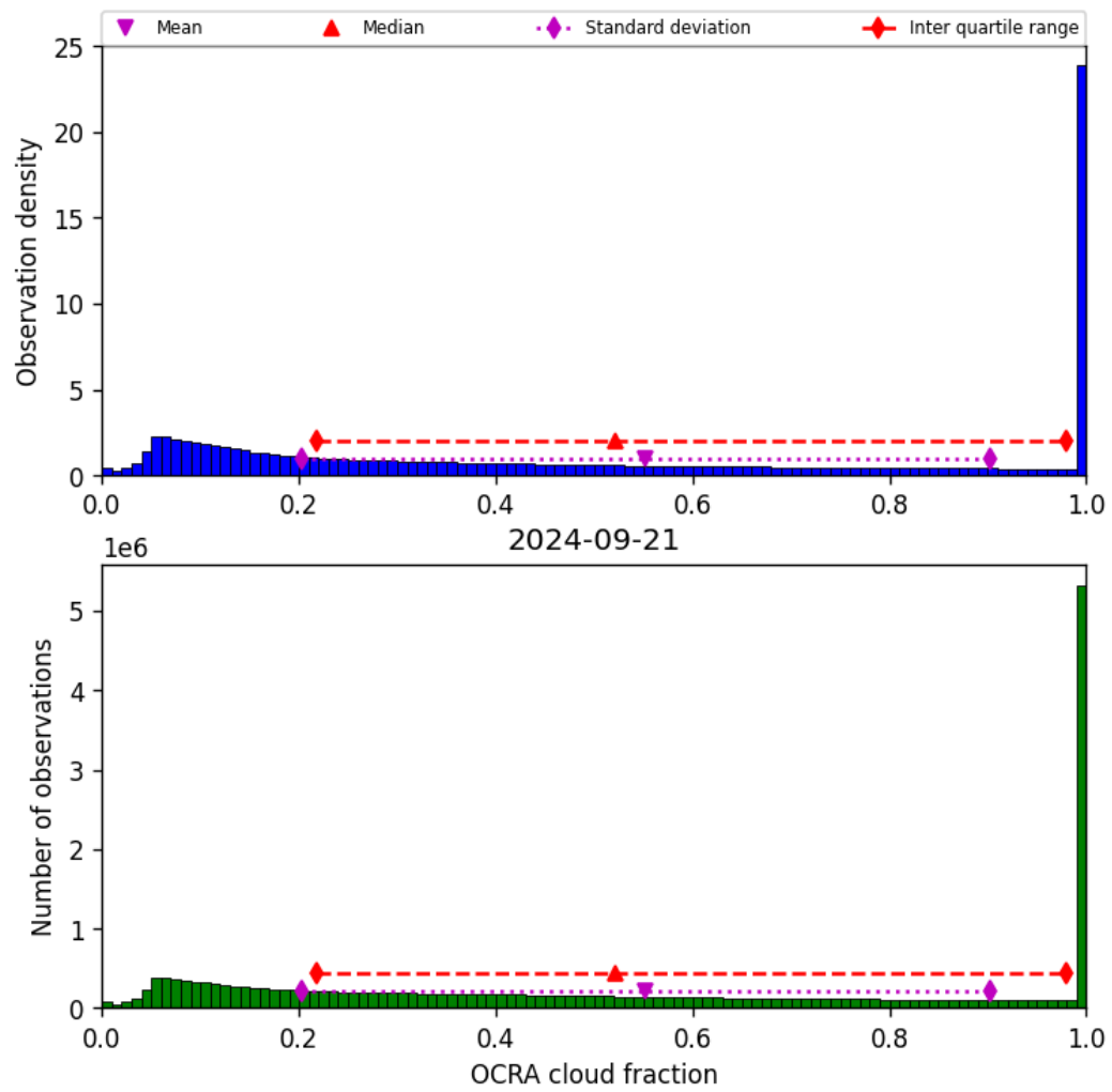
Figure 50: Histogram of “OCRA cloud fraction” for 2024-09-20 to 2024-09-22
