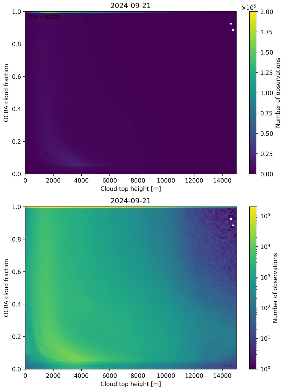
Figure 87: Scatter density plot of “Cloud top height” against “OCRA cloud fraction” for 2024-09-20 to 2024-09-22.
