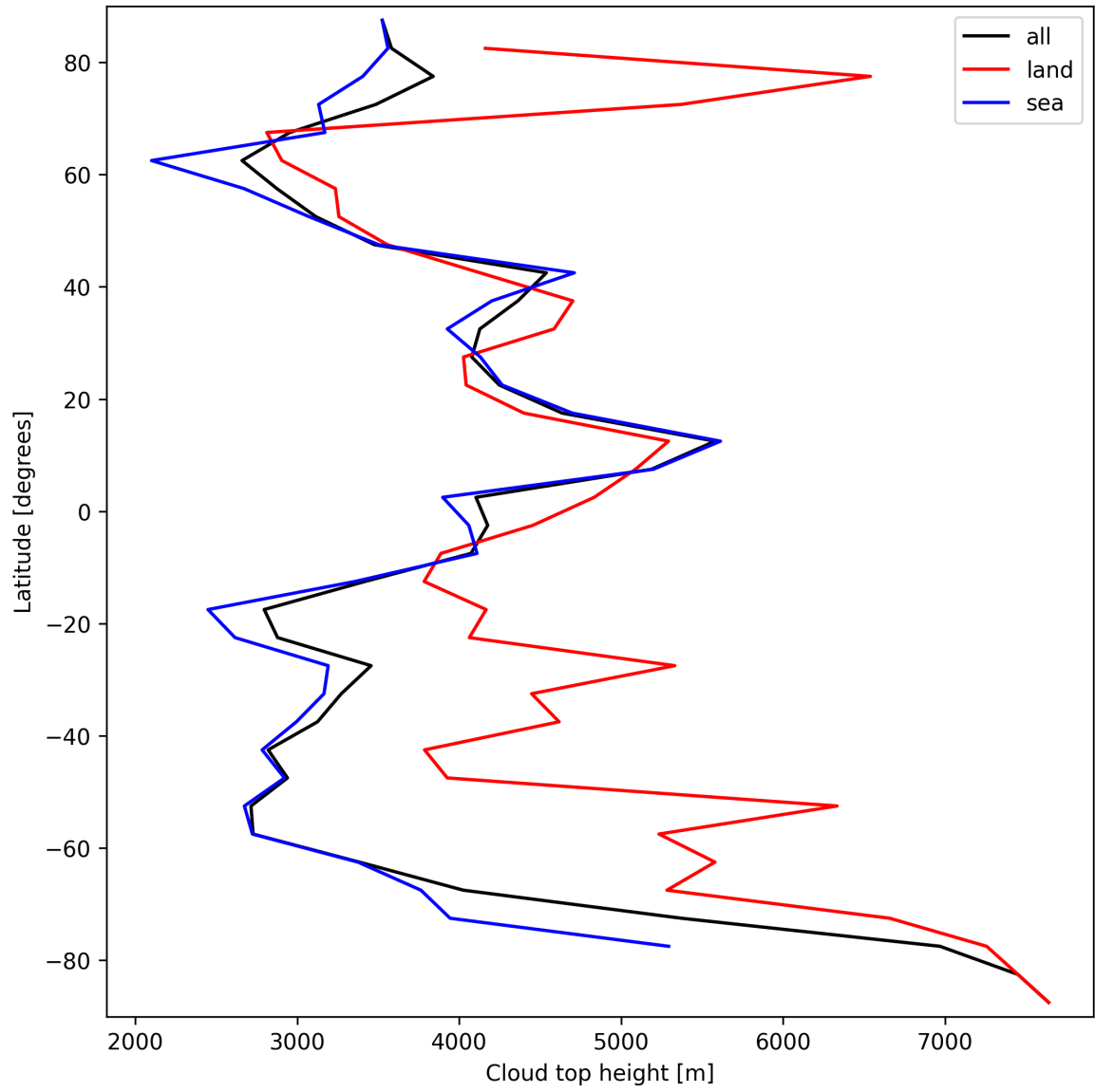
Figure 24: Zonal average of “Cloud top height” for 2024-09-20 to 2024-09-22.
