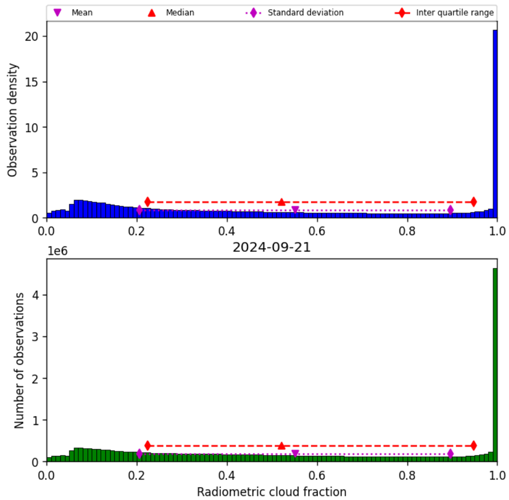
Figure 39: Histogram of “Radiometric cloud fraction” for 2024-09-20 to 2024-09-22
