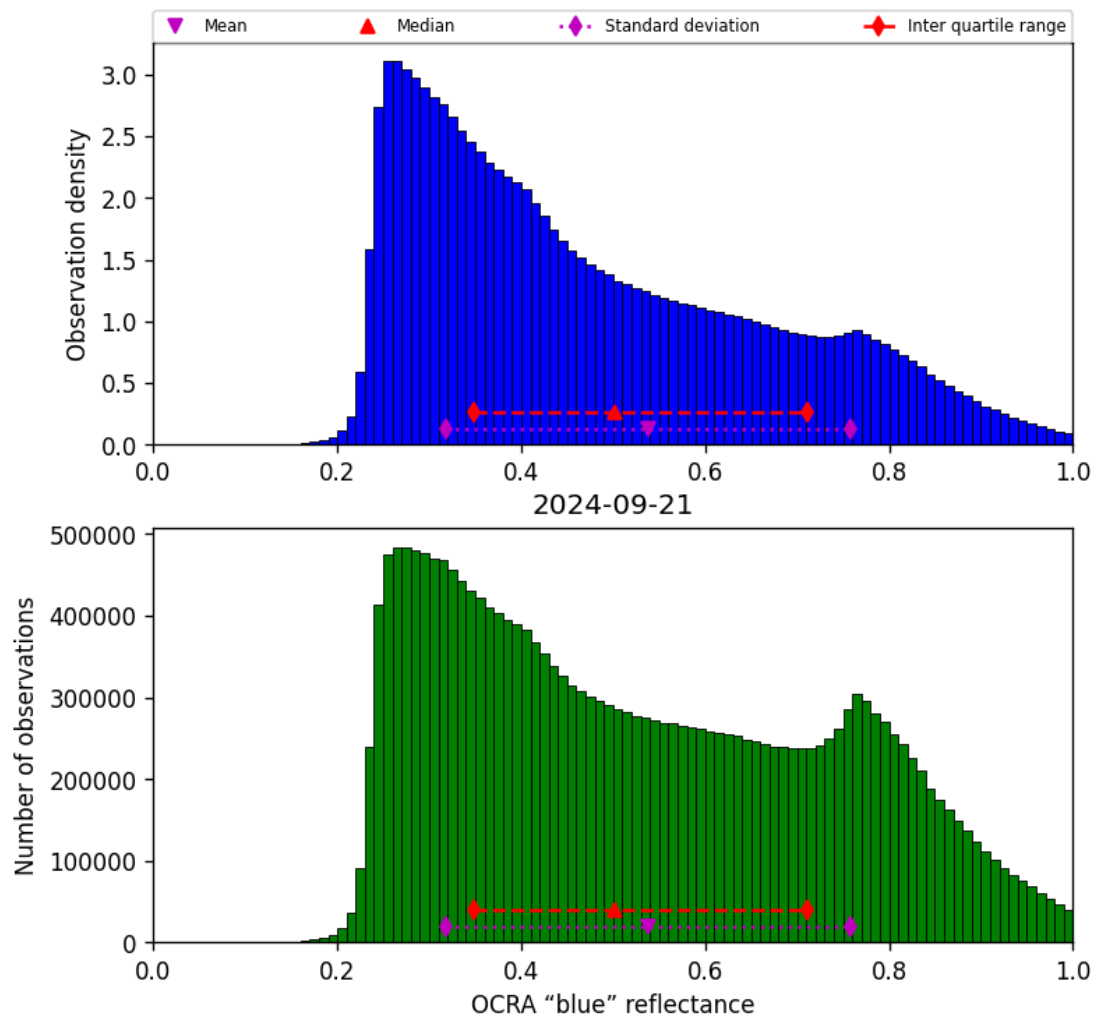
Figure 51: Histogram of “OCRA “blue” reflectance” for 2024-09-20 to 2024-09-22
