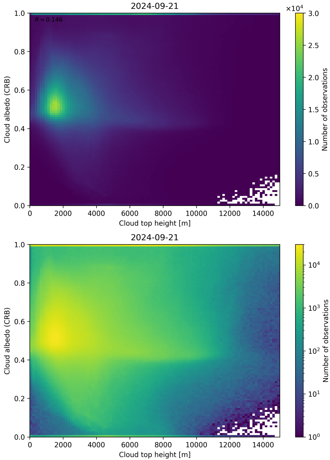
Figure 86: Scatter density plot of “Cloud top height” against “Cloud albedo (CRB)” for 2024-09-20 to 2024-09-22.
