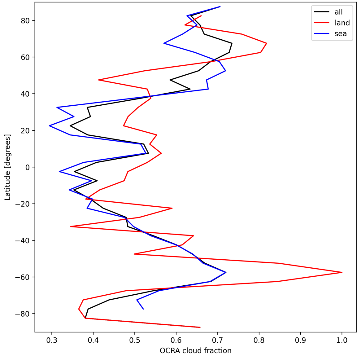
Figure 34: Zonal average of “OCRA cloud fraction” for 2024-09-20 to 2024-09-22.
