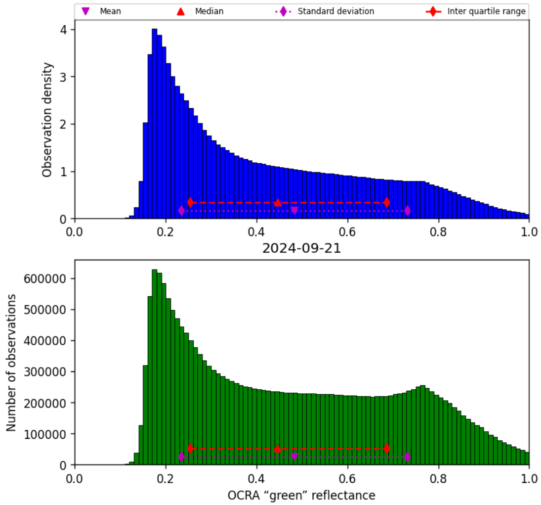
Figure 52: Histogram of “OCRA “green” reflectance” for 2024-09-20 to 2024-09-22
