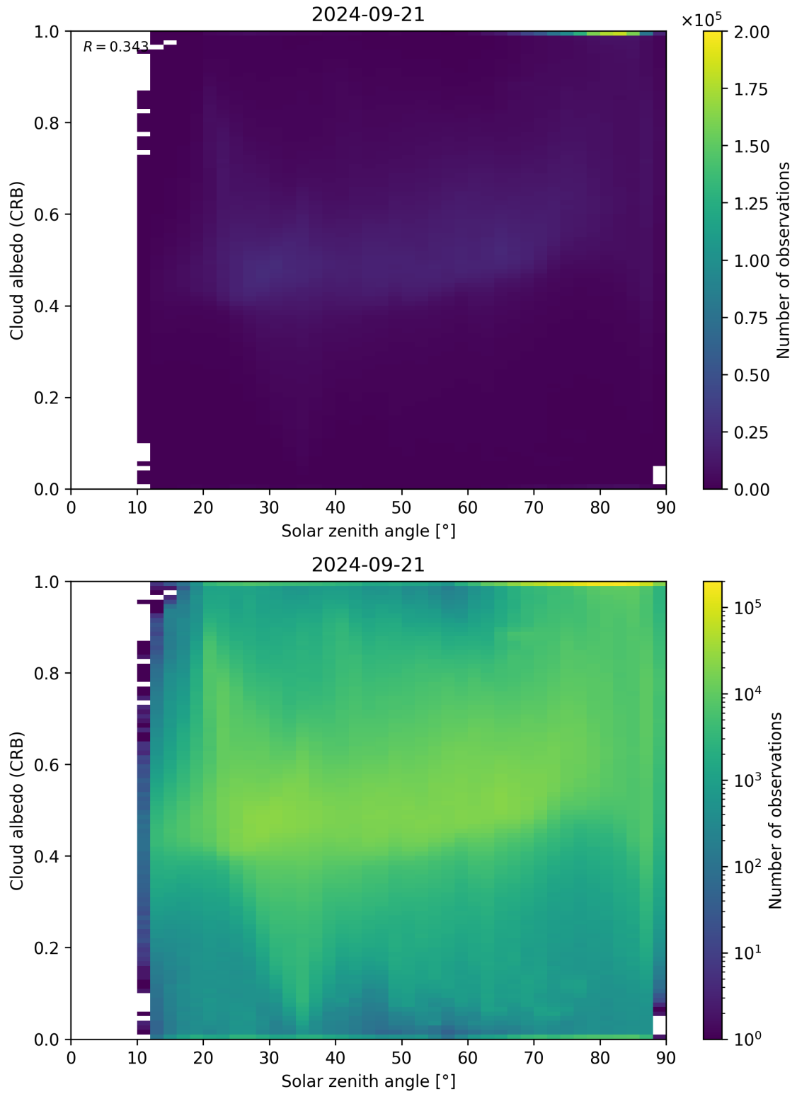
Figure 98: Scatter density plot of “Solar zenith angle” against “Cloud albedo (CRB)” for 2024-09-20 to 2024-09-22.
