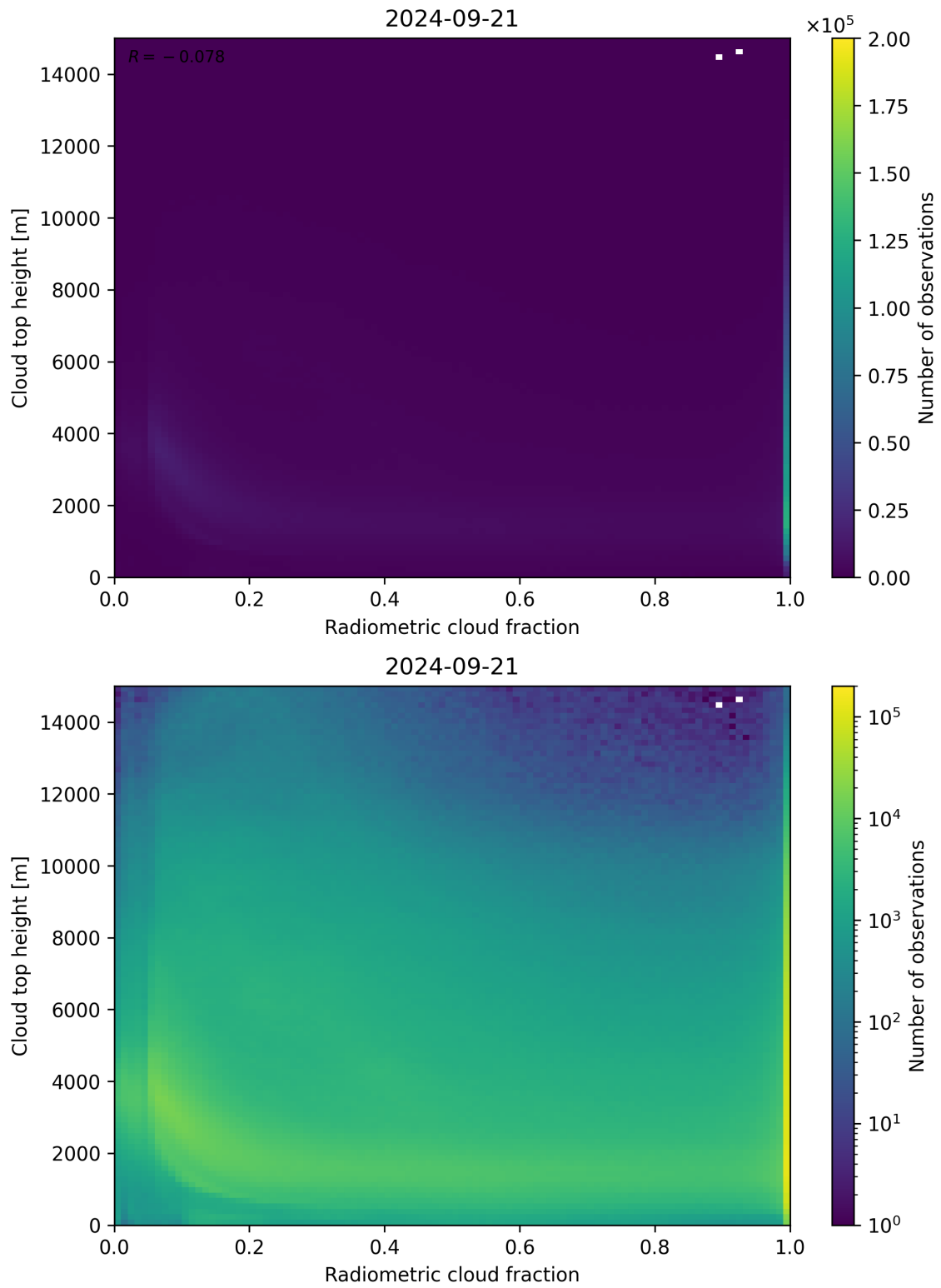
Figure 76: Scatter density plot of “Radiometric cloud fraction” against “Cloud top height” for 2024-09-20 to 2024-09-22.
