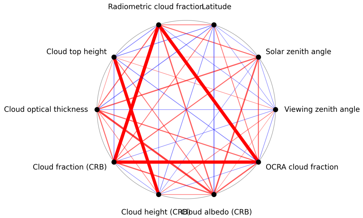
Figure 1: Map of correlation graph for 2024-09-20 to 2024-09-22.
