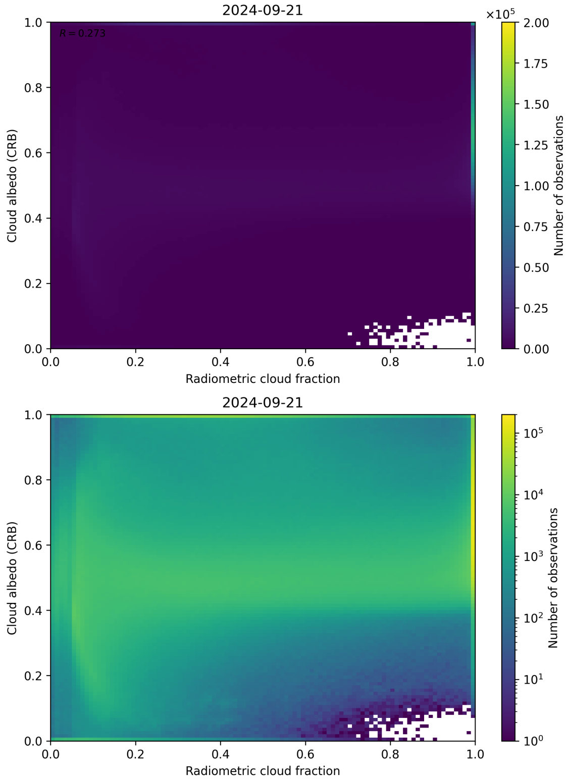
Figure 71: Scatter density plot of “Radiometric cloud fraction” against “Cloud albedo (CRB)” for 2024-09-20 to 2024-09-22.
