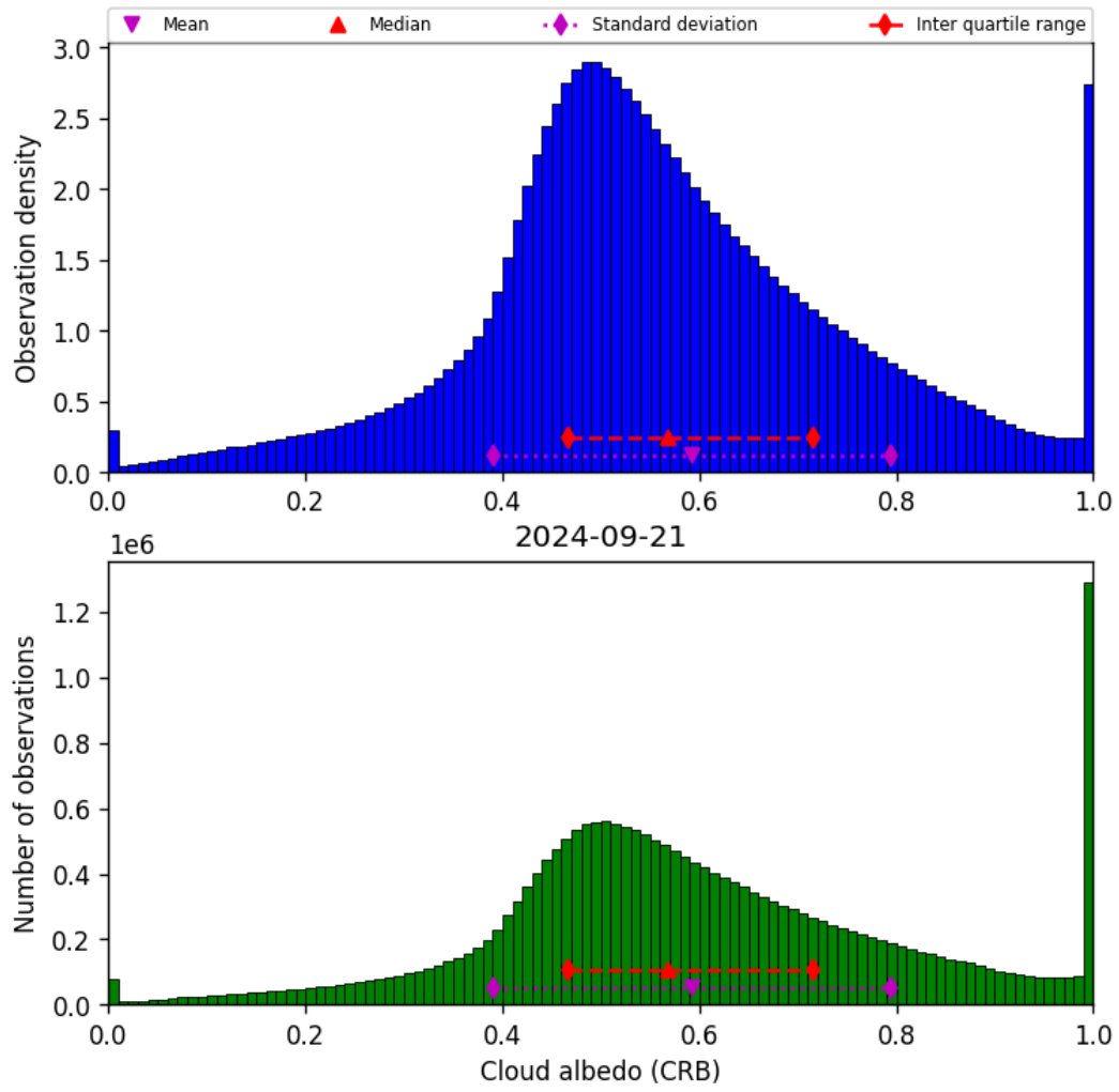
Figure 44: Histogram of “Cloud albedo (CRB)” for 2024-09-20 to 2024-09-22
