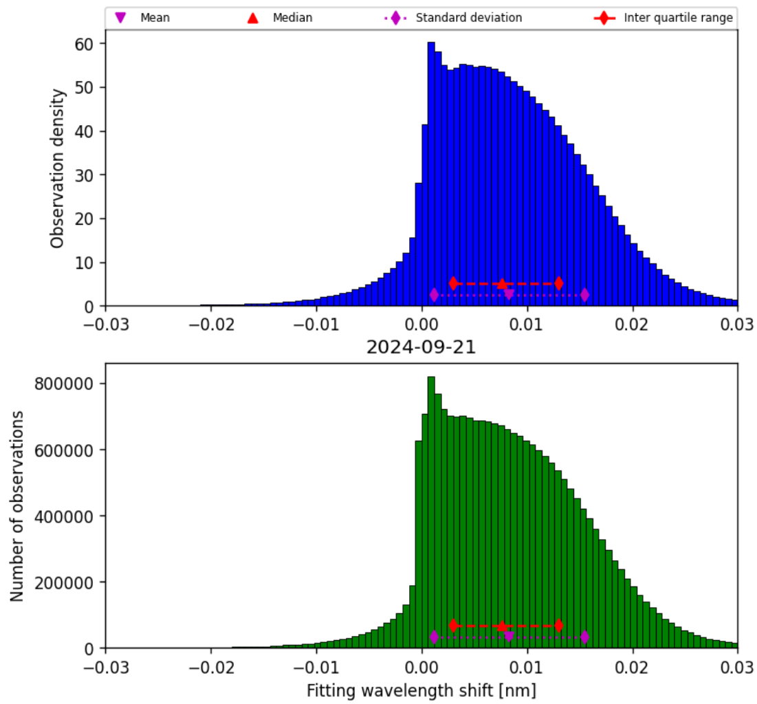
Figure 49: Histogram of “Fitting wavelength shift” for 2024-09-20 to 2024-09-22
