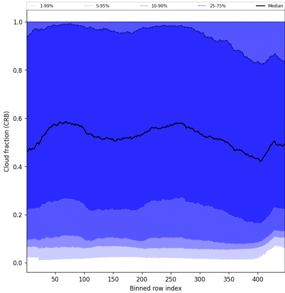
Figure 58: Along track statistics of “Cloud fraction (CRB)” for 2024-09-20 to 2024-09-22
