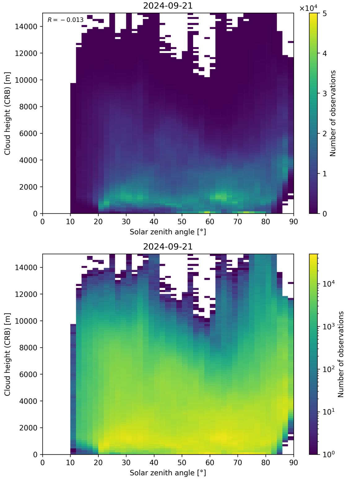
Figure 102: Scatter density plot of “Solar zenith angle” against “Cloud height (CRB)” for 2024-09-20 to 2024-09-22.
