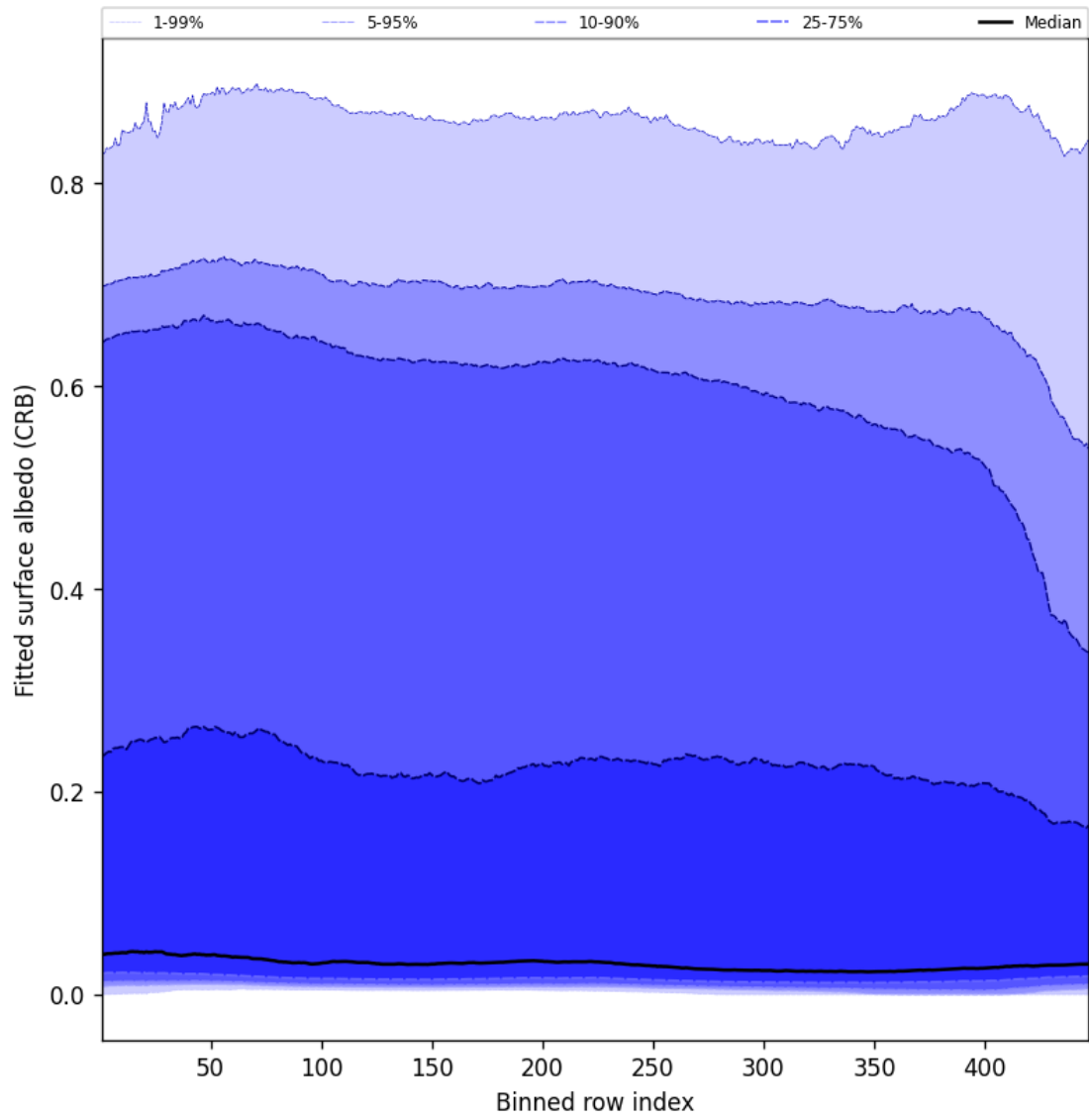
Figure 62: Along track statistics of “Fitted surface albedo (CRB)” for 2024-09-20 to 2024-09-22
