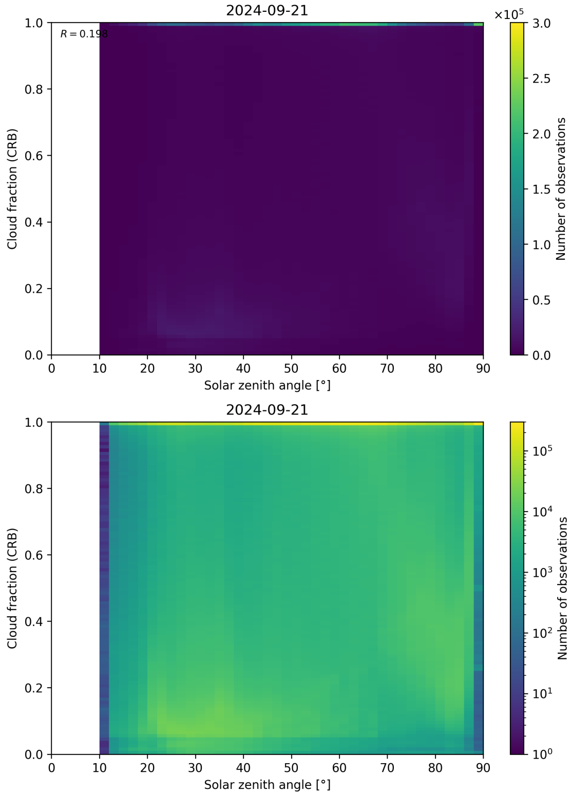
Figure 101: Scatter density plot of “Solar zenith angle” against “Cloud fraction (CRB)” for 2024-09-20 to 2024-09-22.
