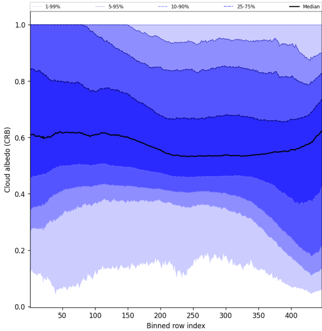
Figure 60: Along track statistics of “Cloud albedo (CRB)” for 2024-09-20 to 2024-09-22
