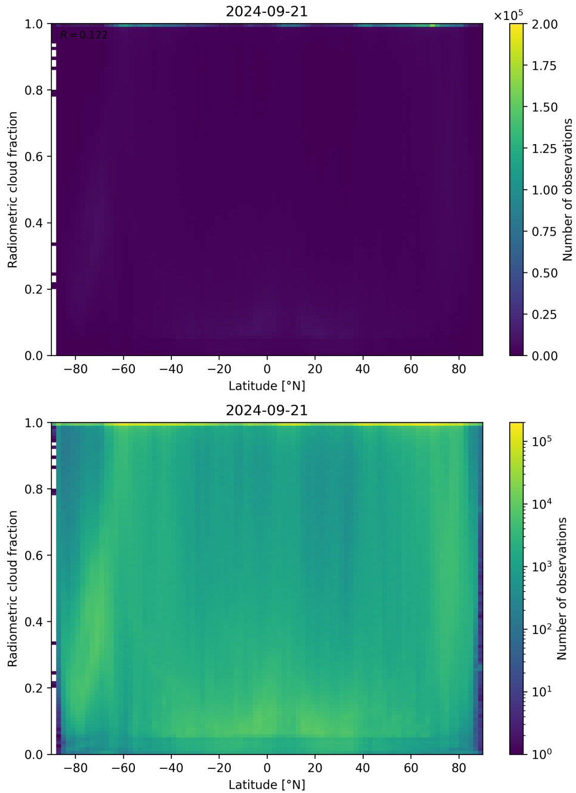
Figure 92: Scatter density plot of “Latitude” against “Radiometric cloud fraction” for 2024-09-20 to 2024-09-22.
