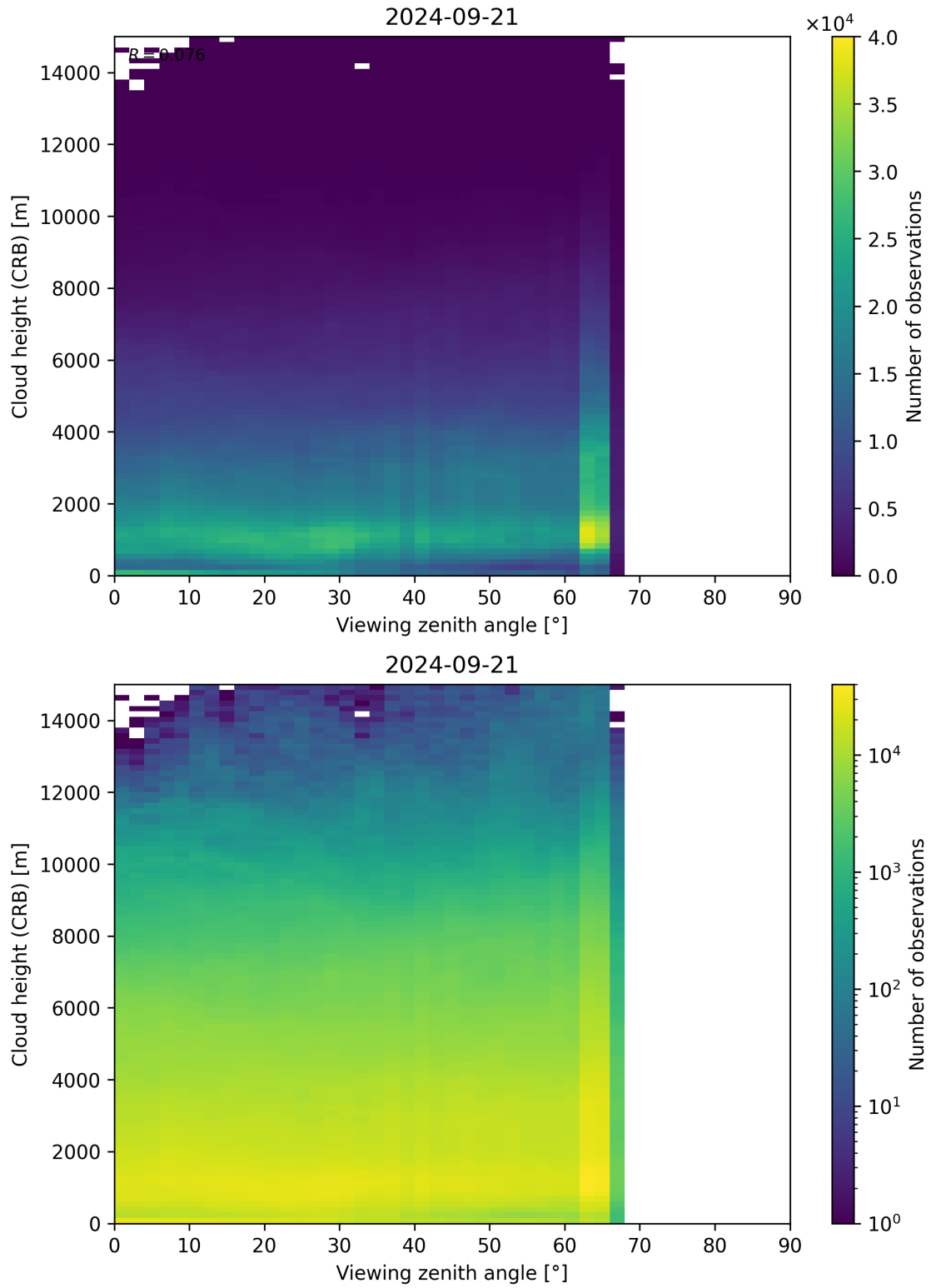
Figure 110: Scatter density plot of “Viewing zenith angle” against “Cloud height (CRB)” for 2024-09-20 to 2024-09-22.
