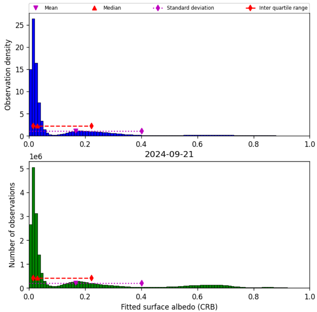
Figure 46: Histogram of “Fitted surface albedo (CRB)” for 2024-09-20 to 2024-09-22
