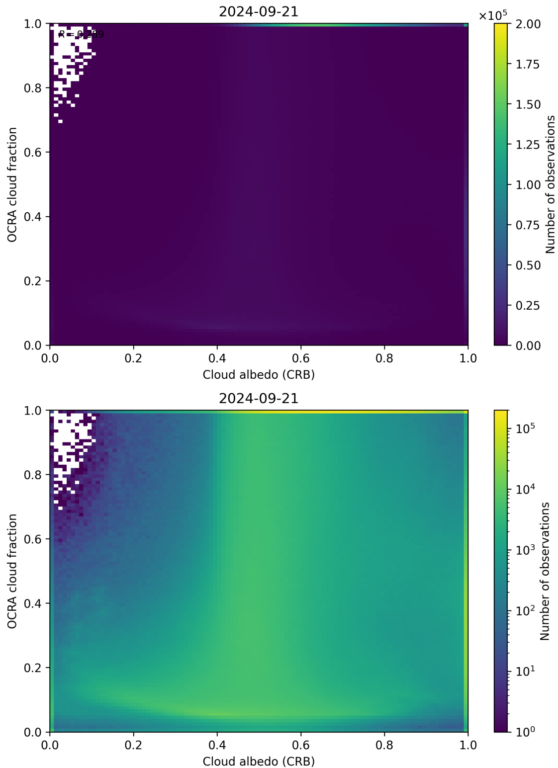
Figure 70: Scatter density plot of “Cloud albedo (CRB)” against “OCRA cloud fraction” for 2024-09-20 to 2024-09-22.
