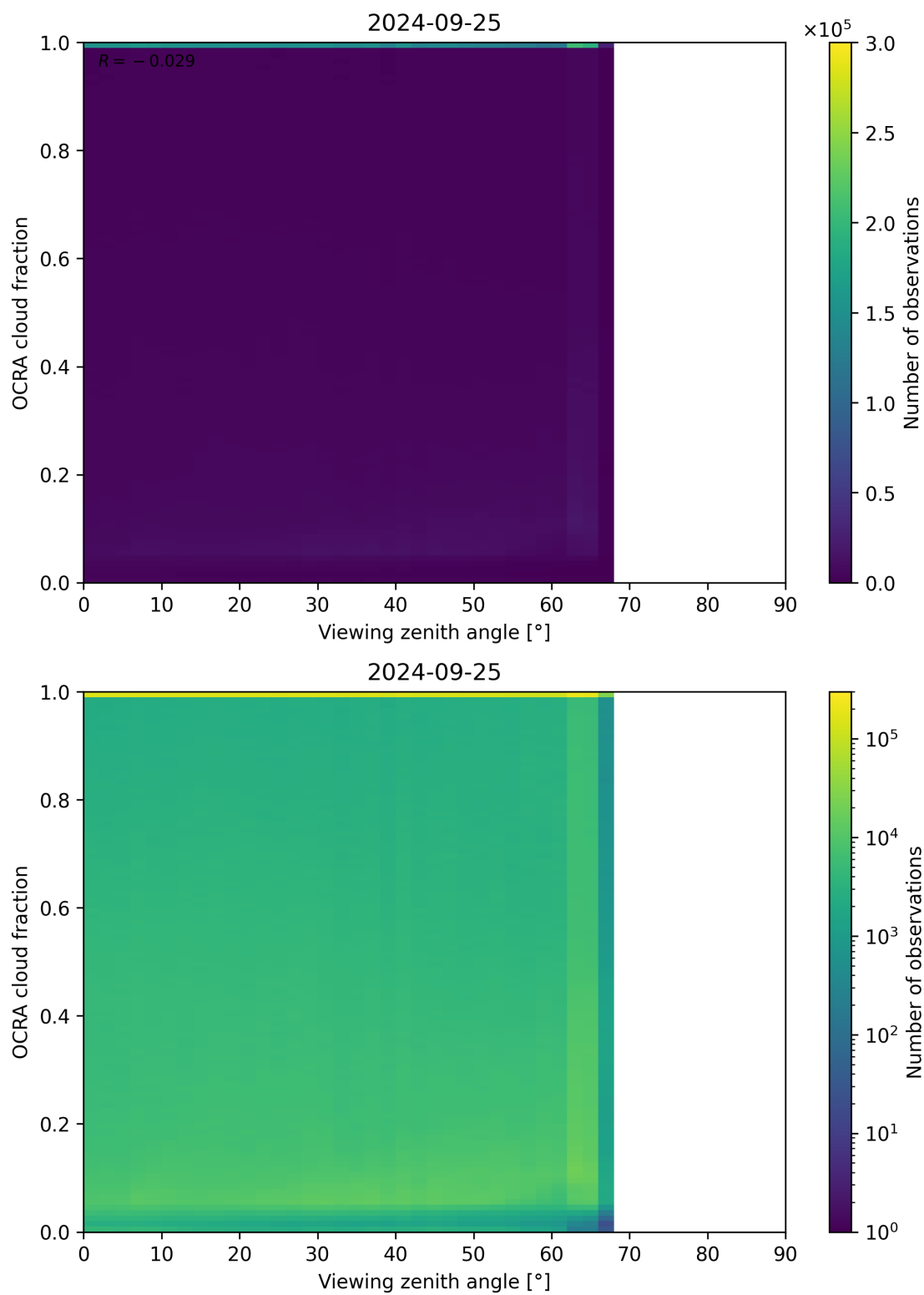
Figure 108: Scatter density plot of “Viewing zenith angle” against “OCRA cloud fraction” for 2024-09-24 to 2024-09-26.
