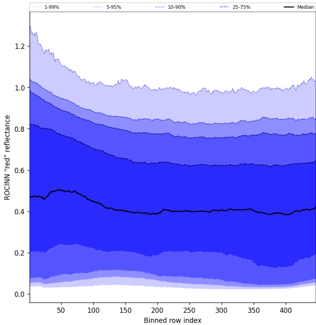
Figure 69: Along track statistics of "ROCINN "red" reflectance" for 2024-09-24 to 2024-09-26
