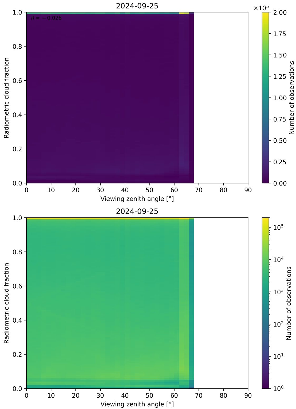
Figure 107: Scatter density plot of “Viewing zenith angle” against “Radiometric cloud fraction” for 2024-09-24 to 2024-09-26.
