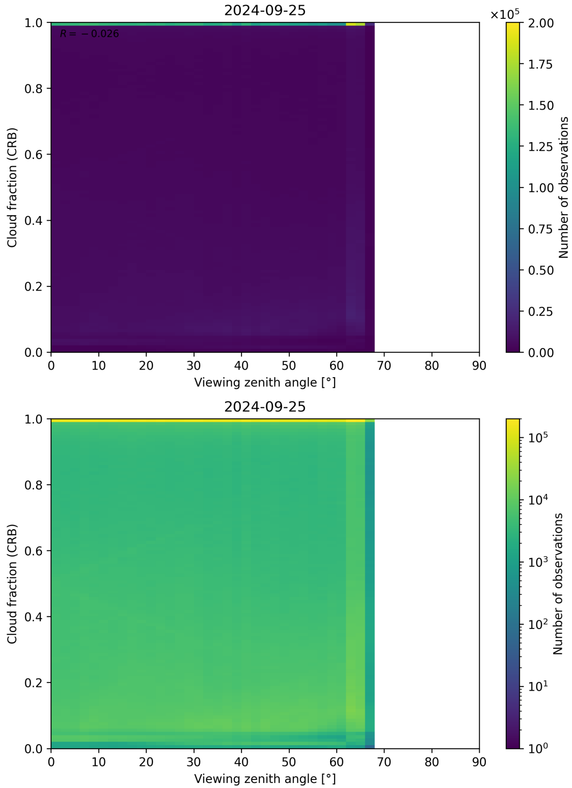
Figure 109: Scatter density plot of “Viewing zenith angle” against “Cloud fraction (CRB)” for 2024-09-24 to 2024-09-26.
