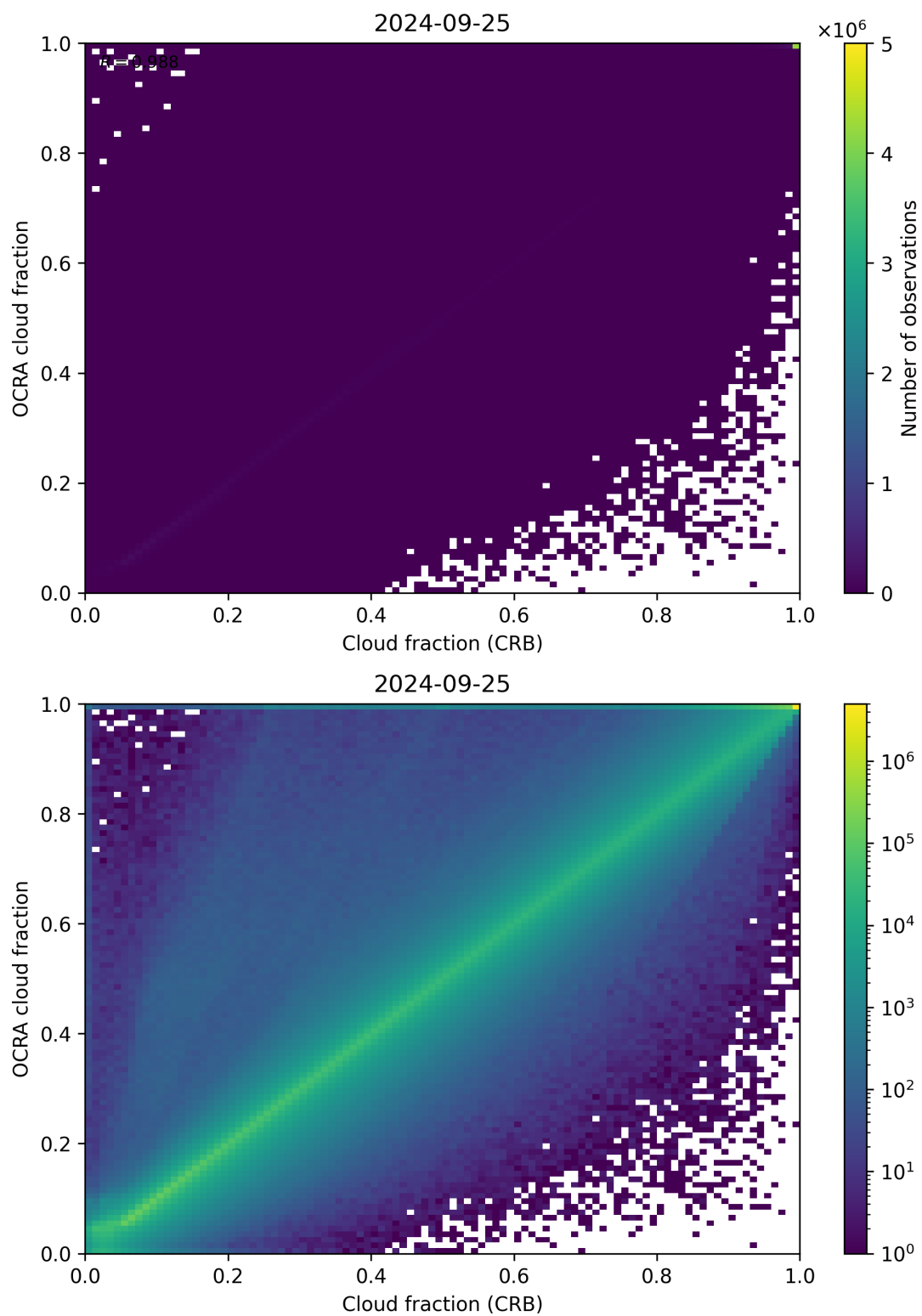
Figure 78: Scatter density plot of “Cloud fraction (CRB)” against “OCRA cloud fraction” for 2024-09-24 to 2024-09-26.
