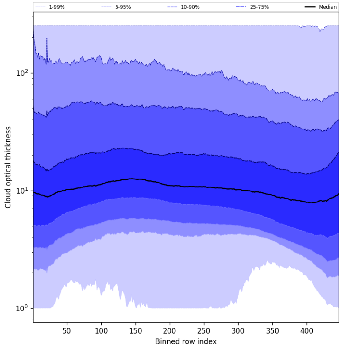
Figure 57: Along track statistics of “Cloud optical thickness” for 2024-09-24 to 2024-09-26
