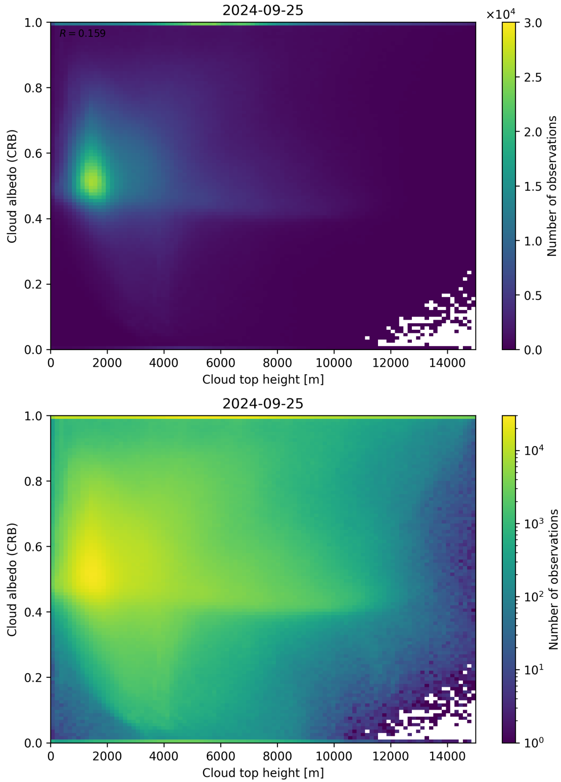
Figure 86: Scatter density plot of “Cloud top height” against “Cloud albedo (CRB)” for 2024-09-24 to 2024-09-26.
