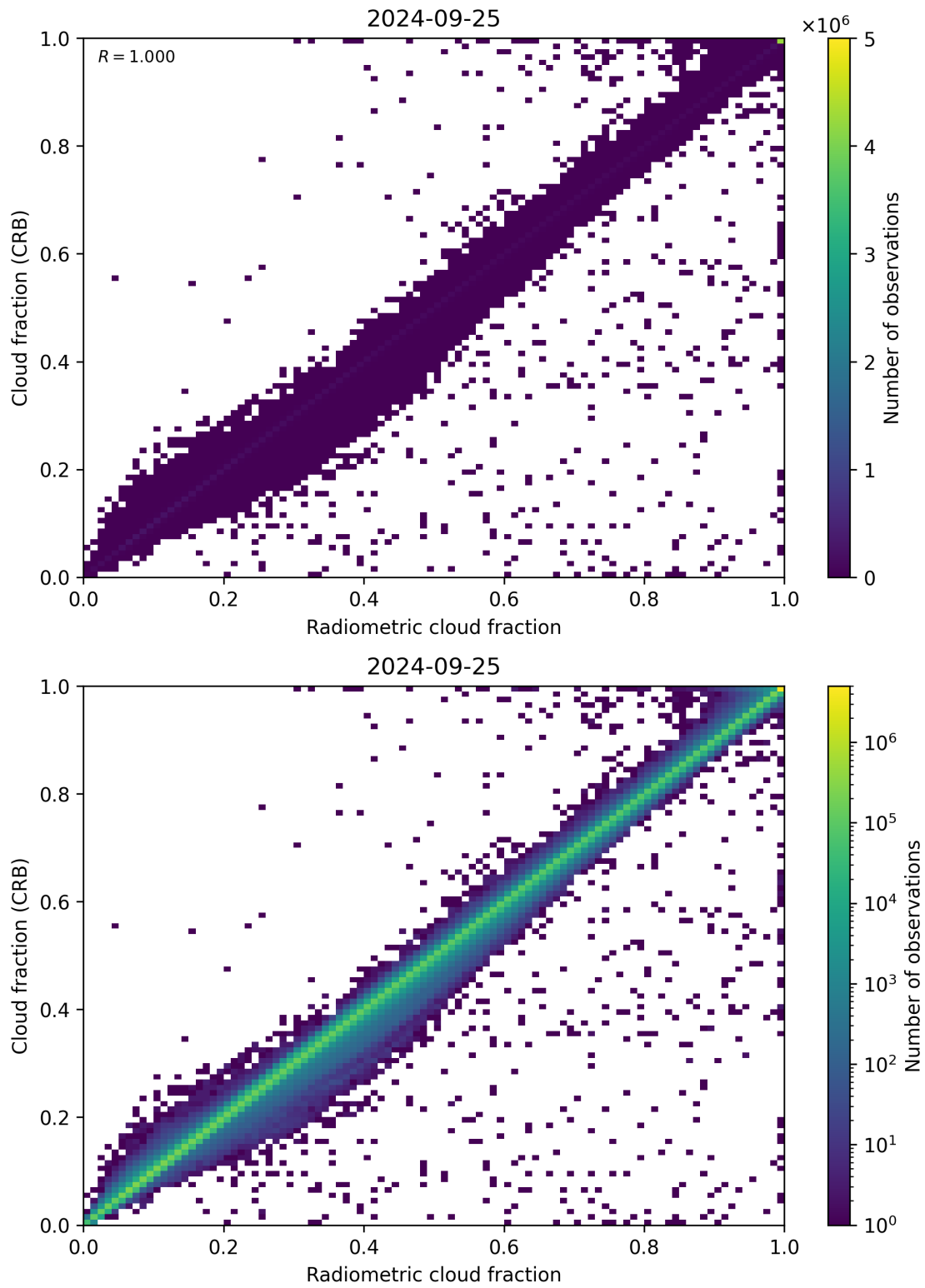
Figure 73: Scatter density plot of “Radiometric cloud fraction” against “Cloud fraction (CRB)” for 2024-09-24 to 2024-09-26.
