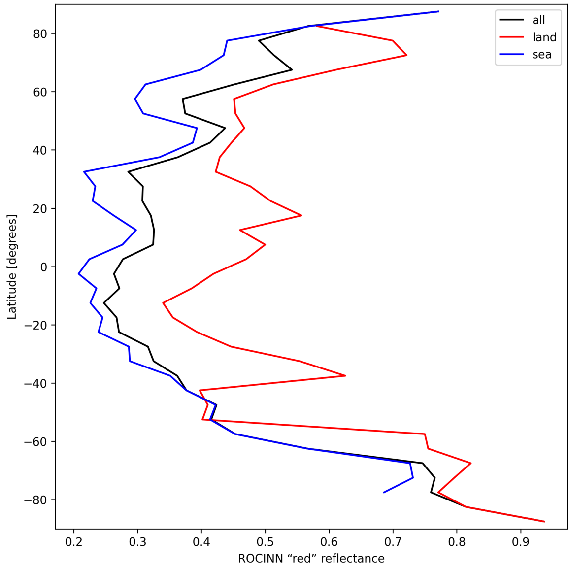
Figure 37: Zonal average of “ROCINN “red” reflectance” for 2024-09-24 to 2024-09-26.
