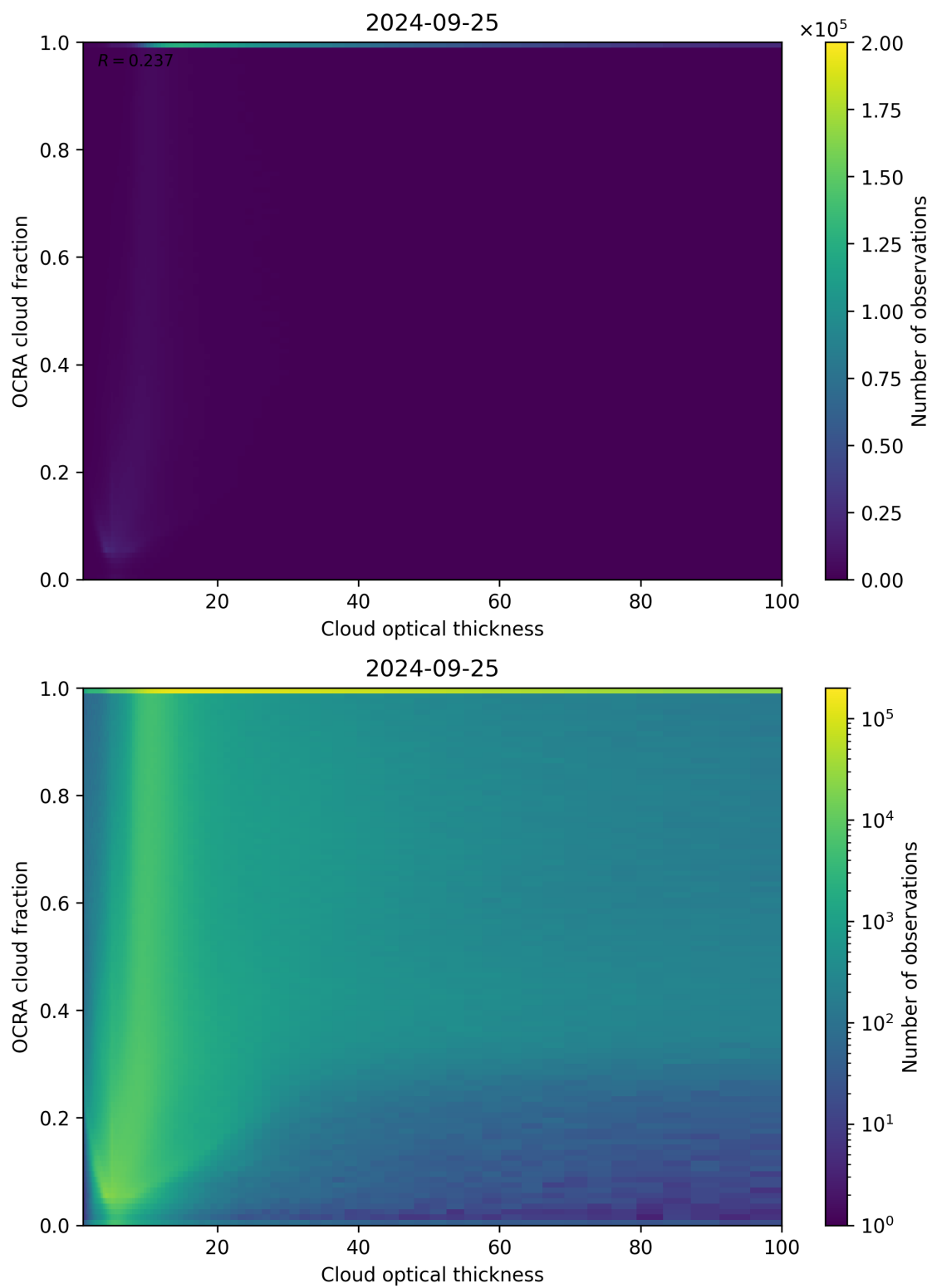
Figure 83: Scatter density plot of “Cloud optical thickness” against “OCRA cloud fraction” for 2024-09-24 to 2024-09-26.
