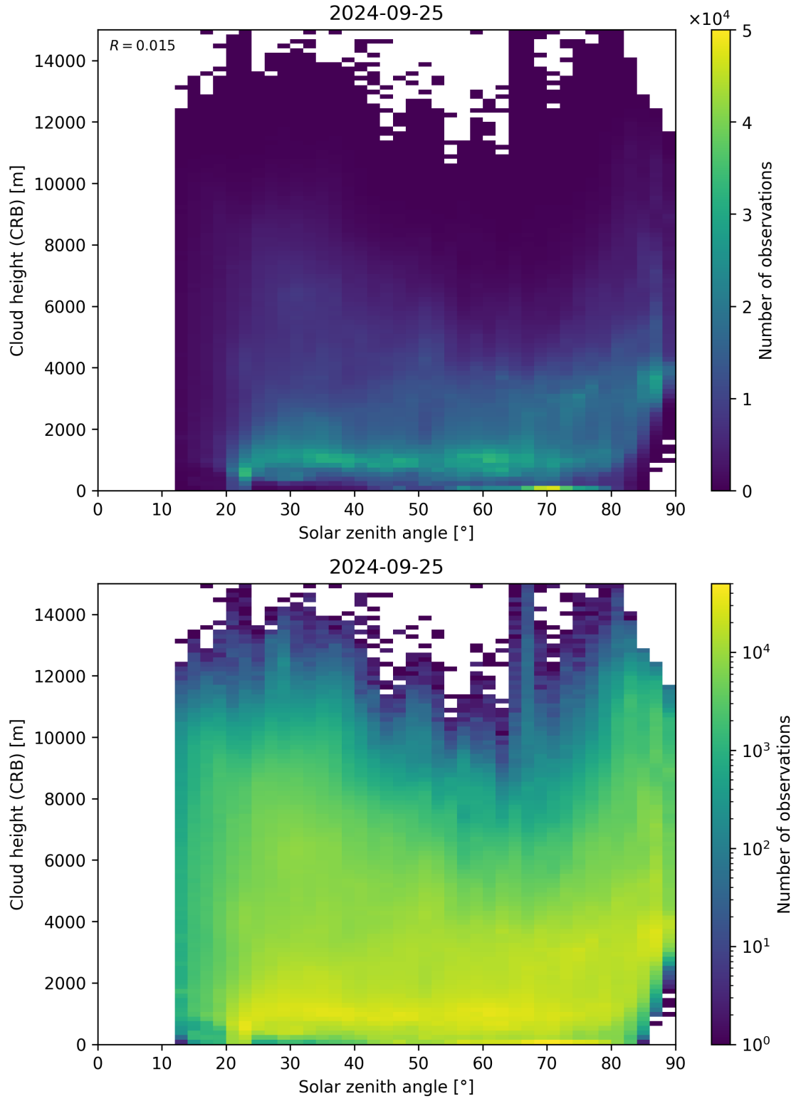
Figure 102: Scatter density plot of “Solar zenith angle” against “Cloud height (CRB)” for 2024-09-24 to 2024-09-26.
