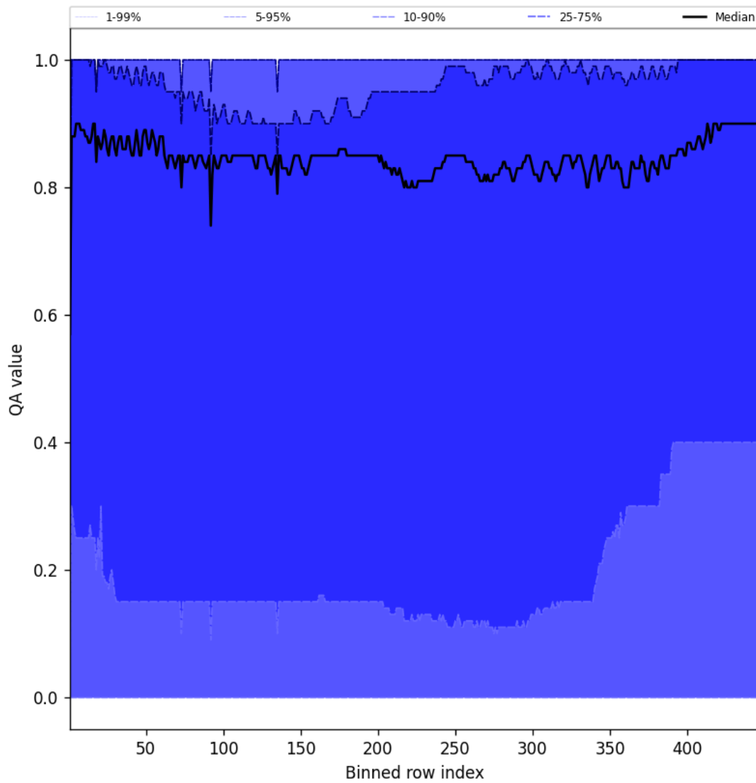
Figure 54: Along track statistics of “QA value” for 2024-09-24 to 2024-09-26
