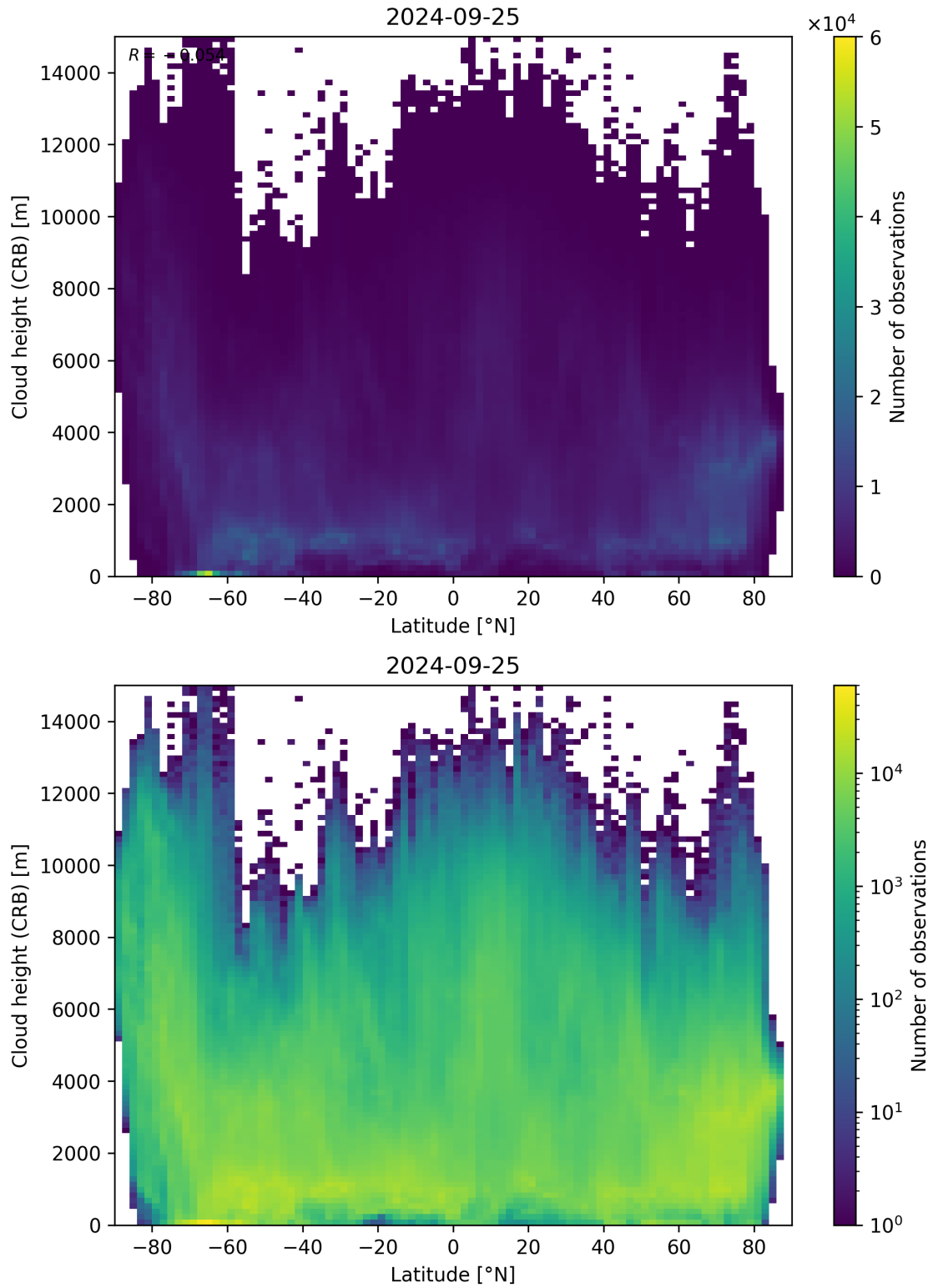
Figure 95: Scatter density plot of “Latitude” against “Cloud height (CRB)” for 2024-09-24 to 2024-09-26.
