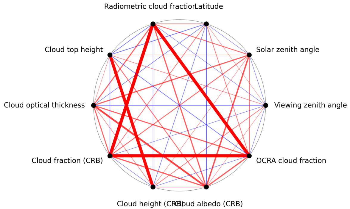
Figure 1: Map of correlation graph for 2024-09-24 to 2024-09-26.
