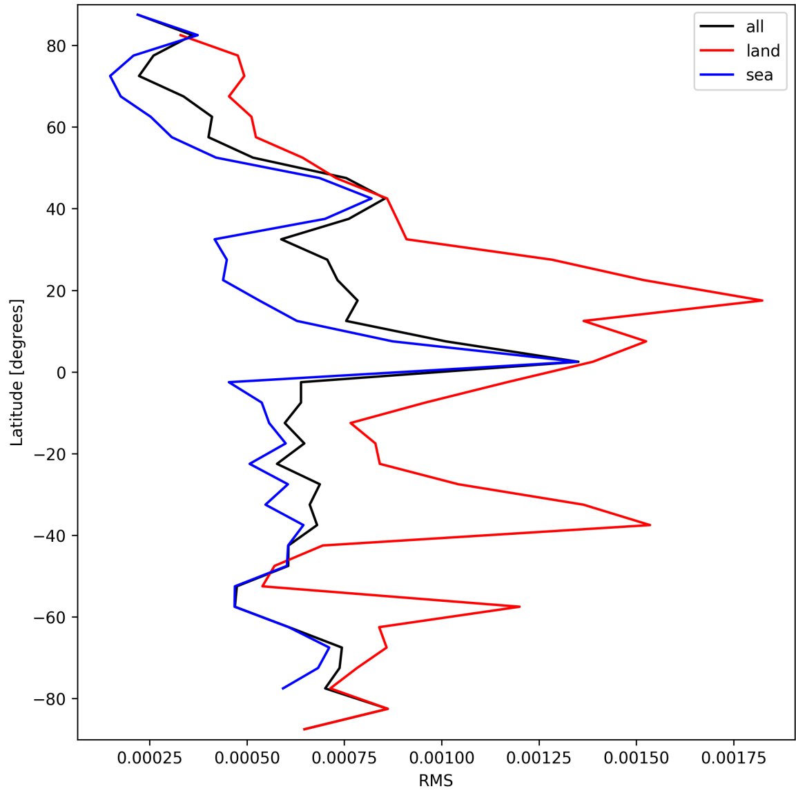
Figure 31: Zonal average of “RMS” for 2024-09-24 to 2024-09-26.
