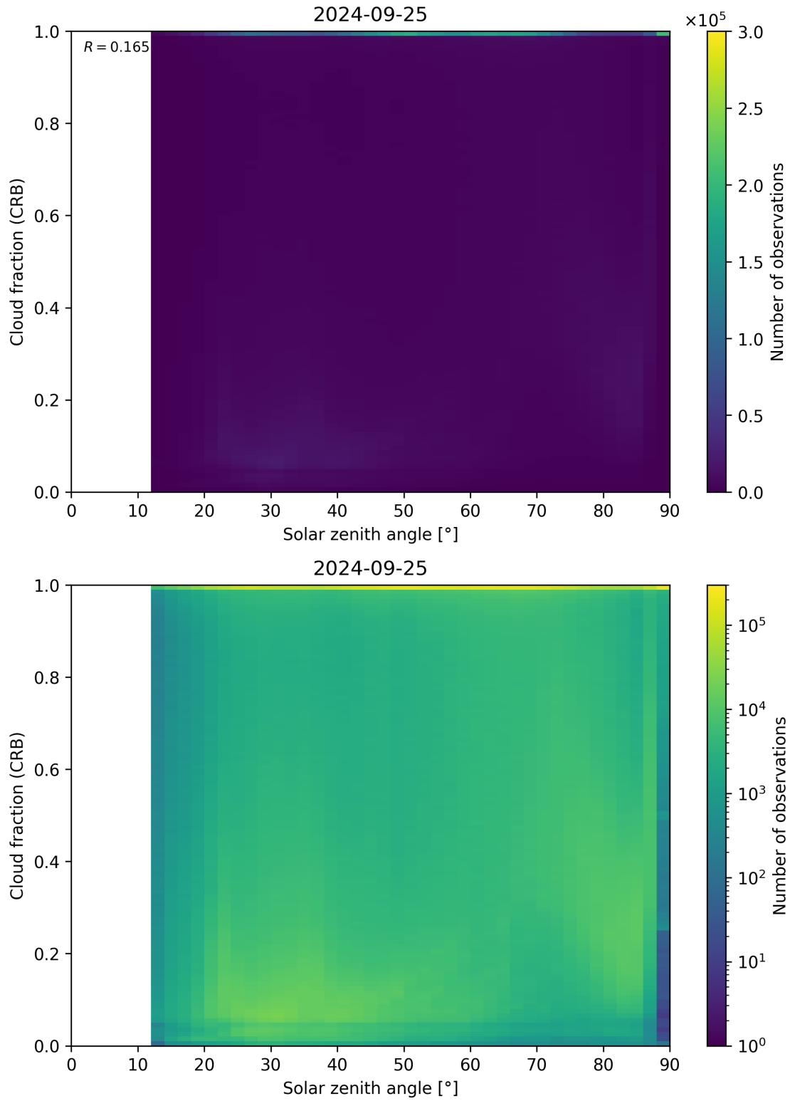
Figure 101: Scatter density plot of “Solar zenith angle” against “Cloud fraction (CRB)” for 2024-09-24 to 2024-09-26.
