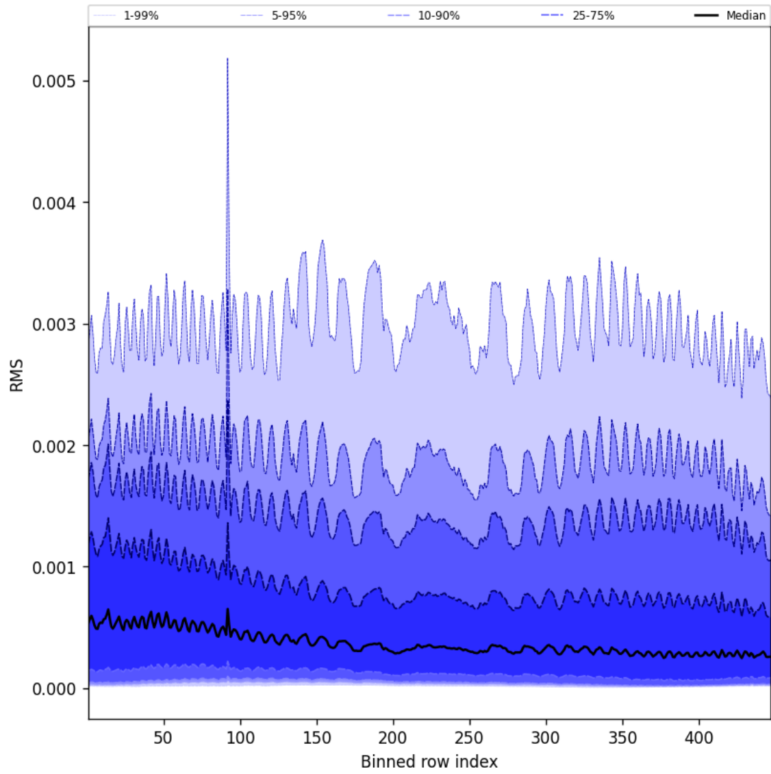
Figure 63: Along track statistics of “RMS” for 2024-09-24 to 2024-09-26
