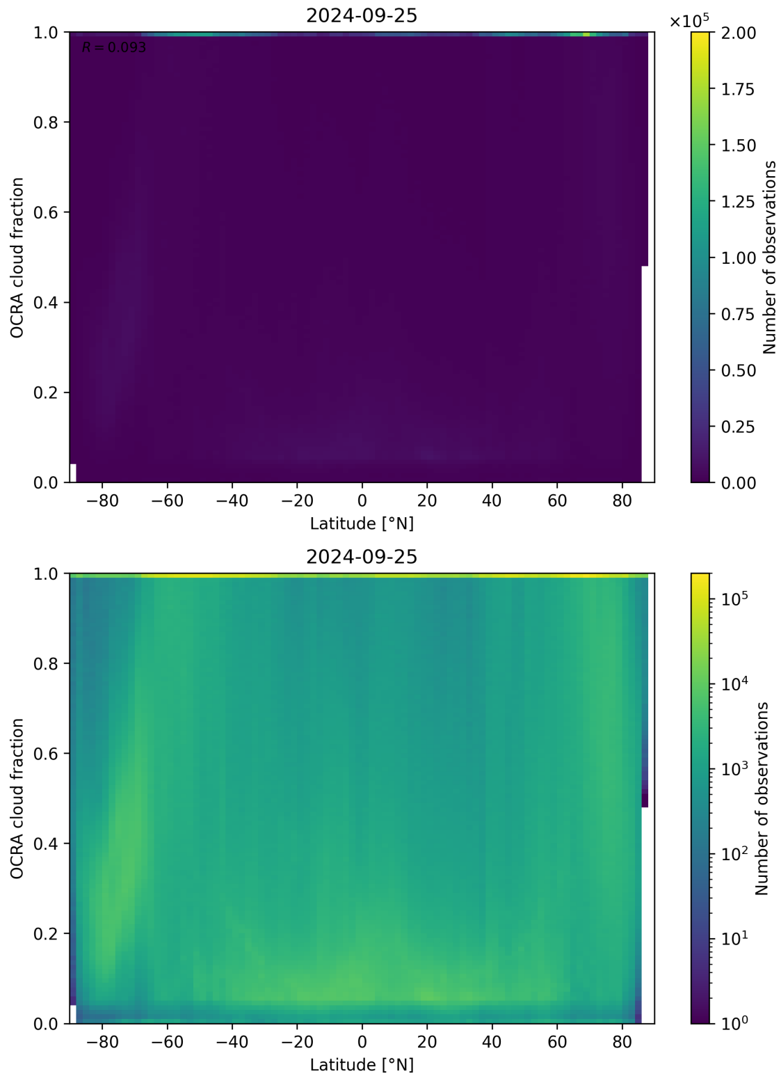
Figure 93: Scatter density plot of “Latitude” against “OCRA cloud fraction” for 2024-09-24 to 2024-09-26.
