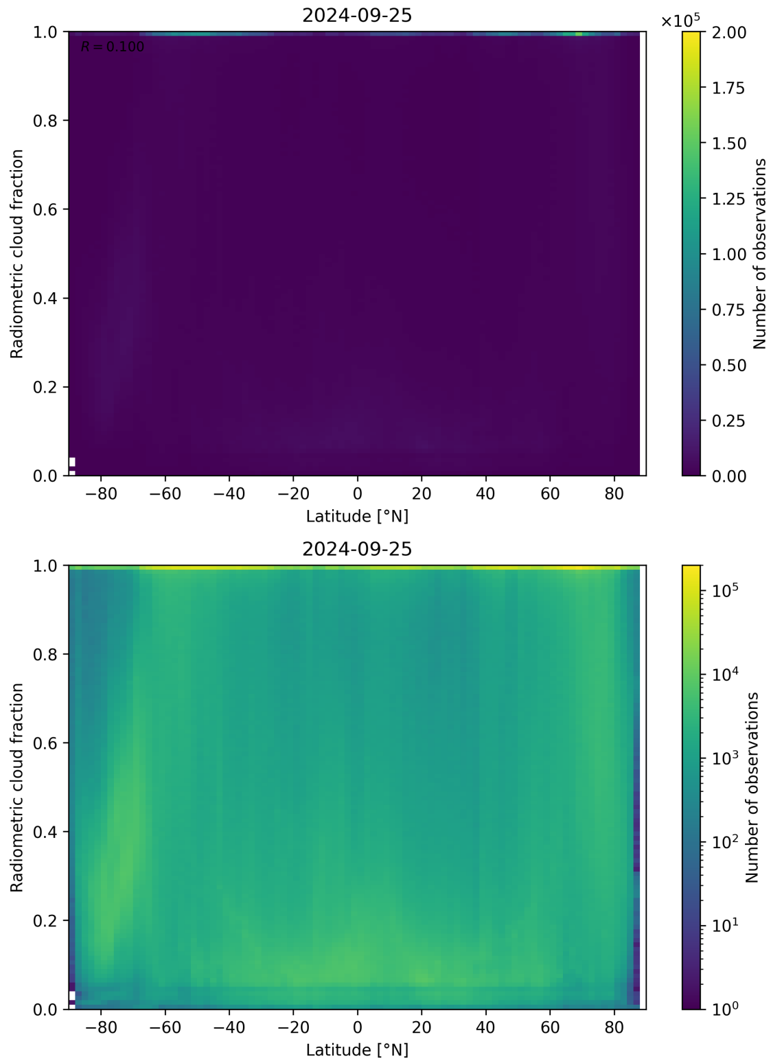
Figure 92: Scatter density plot of “Latitude” against “Radiometric cloud fraction” for 2024-09-24 to 2024-09-26.
