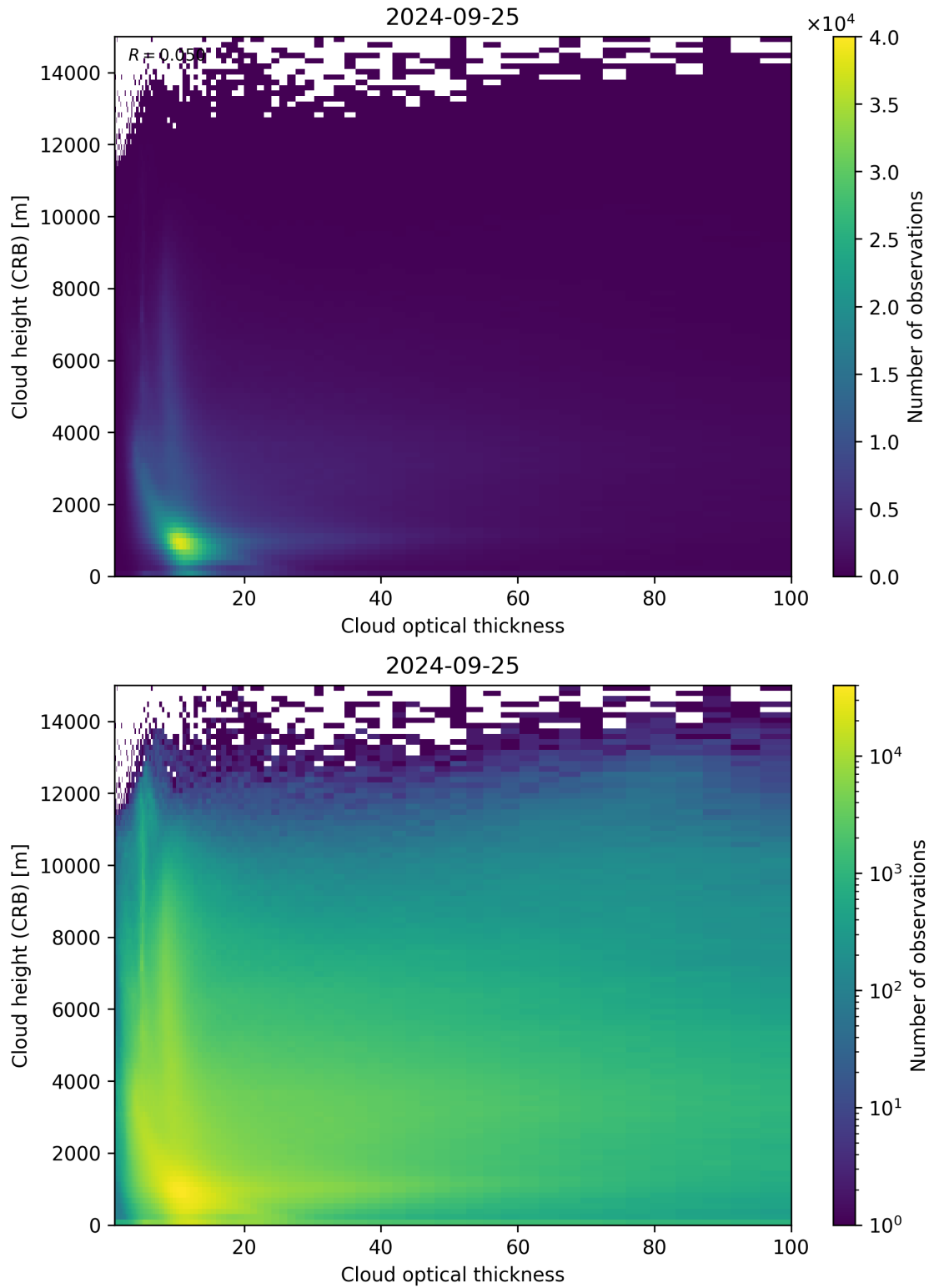
Figure 85: Scatter density plot of “Cloud optical thickness” against “Cloud height (CRB)” for 2024-09-24 to 2024-09-26.
