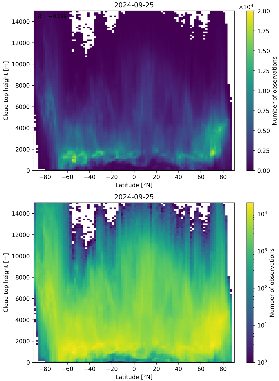
Figure 97: Scatter density plot of “Latitude” against “Cloud top height” for 2024-09-24 to 2024-09-26.
