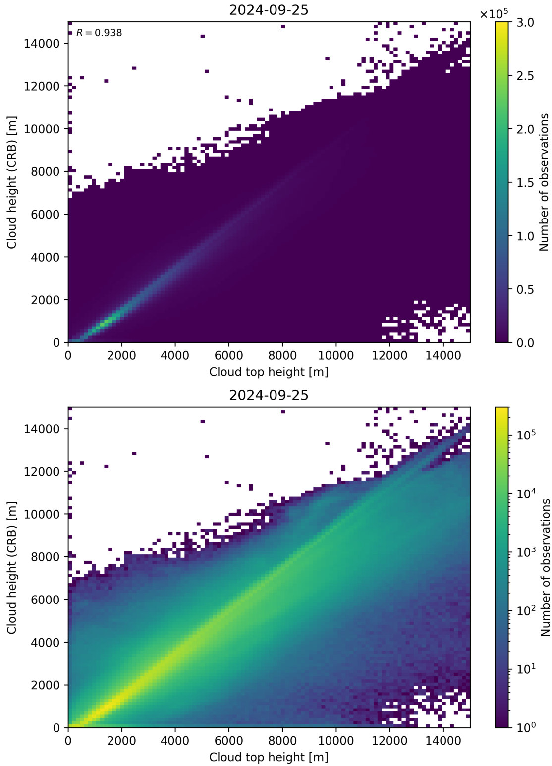
Figure 89: Scatter density plot of “Cloud top height” against “Cloud height (CRB)” for 2024-09-24 to 2024-09-26.
