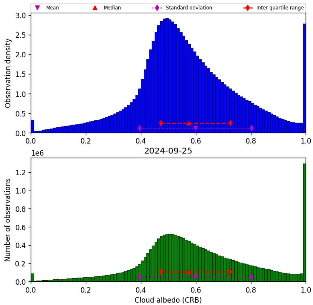
Figure 44: Histogram of “Cloud albedo (CRB)” for 2024-09-24 to 2024-09-26
