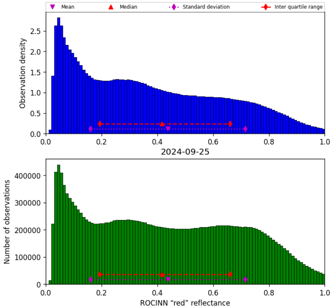
Figure 53: Histogram of “ROCINN “red” reflectance” for 2024-09-24 to 2024-09-26
