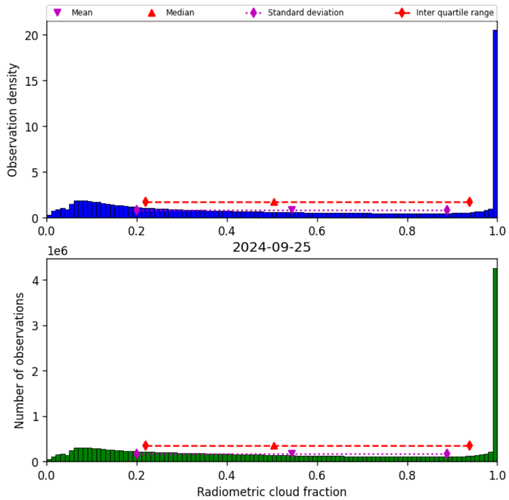
Figure 39: Histogram of “Radiometric cloud fraction” for 2024-09-24 to 2024-09-26
