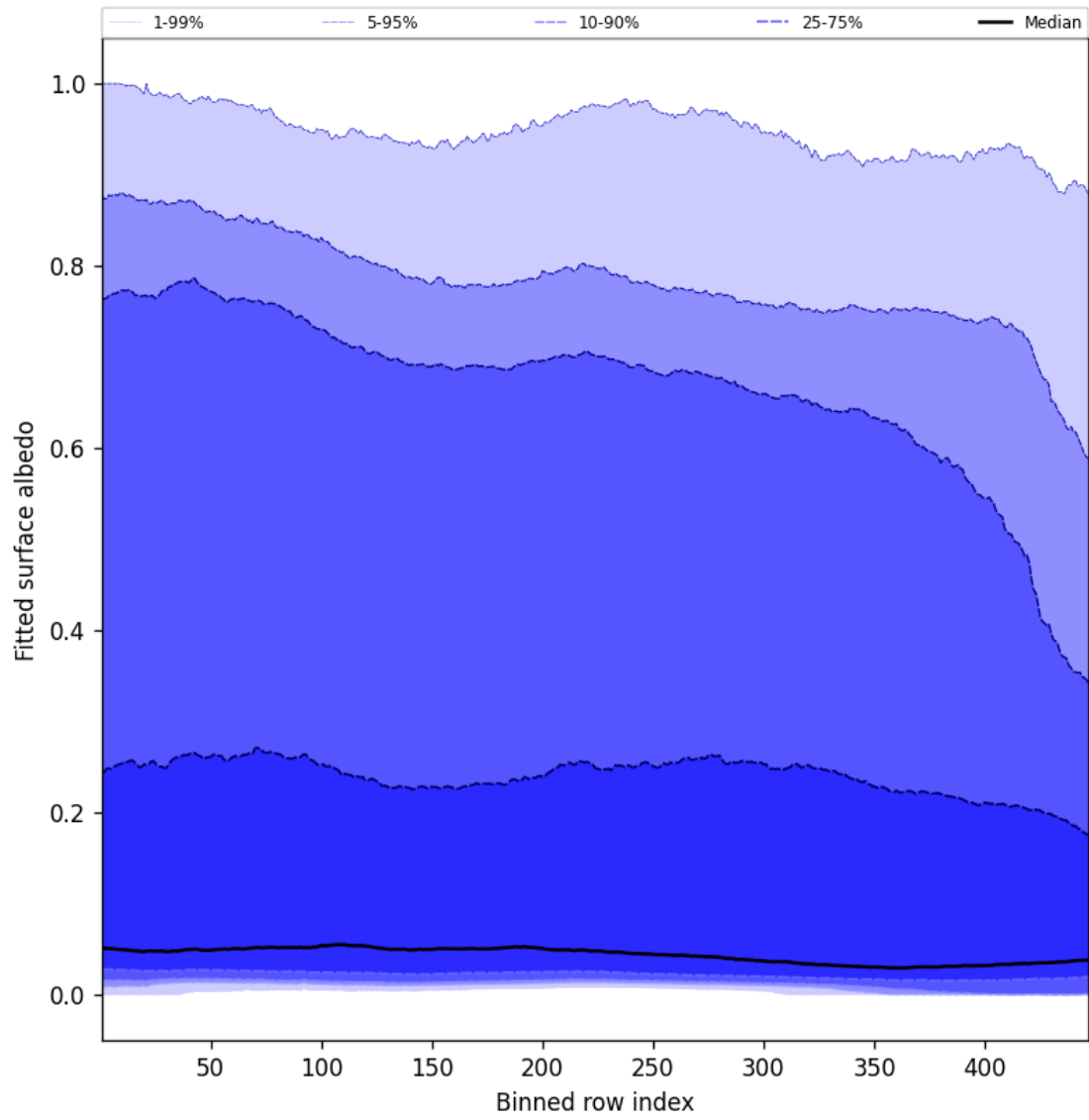
Figure 61: Along track statistics of “Fitted surface albedo” for 2024-09-24 to 2024-09-26
