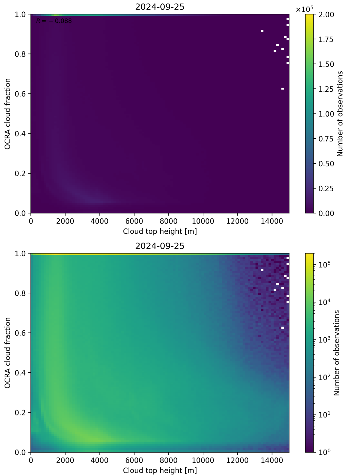
Figure 87: Scatter density plot of “Cloud top height” against “OCRA cloud fraction” for 2024-09-24 to 2024-09-26.
