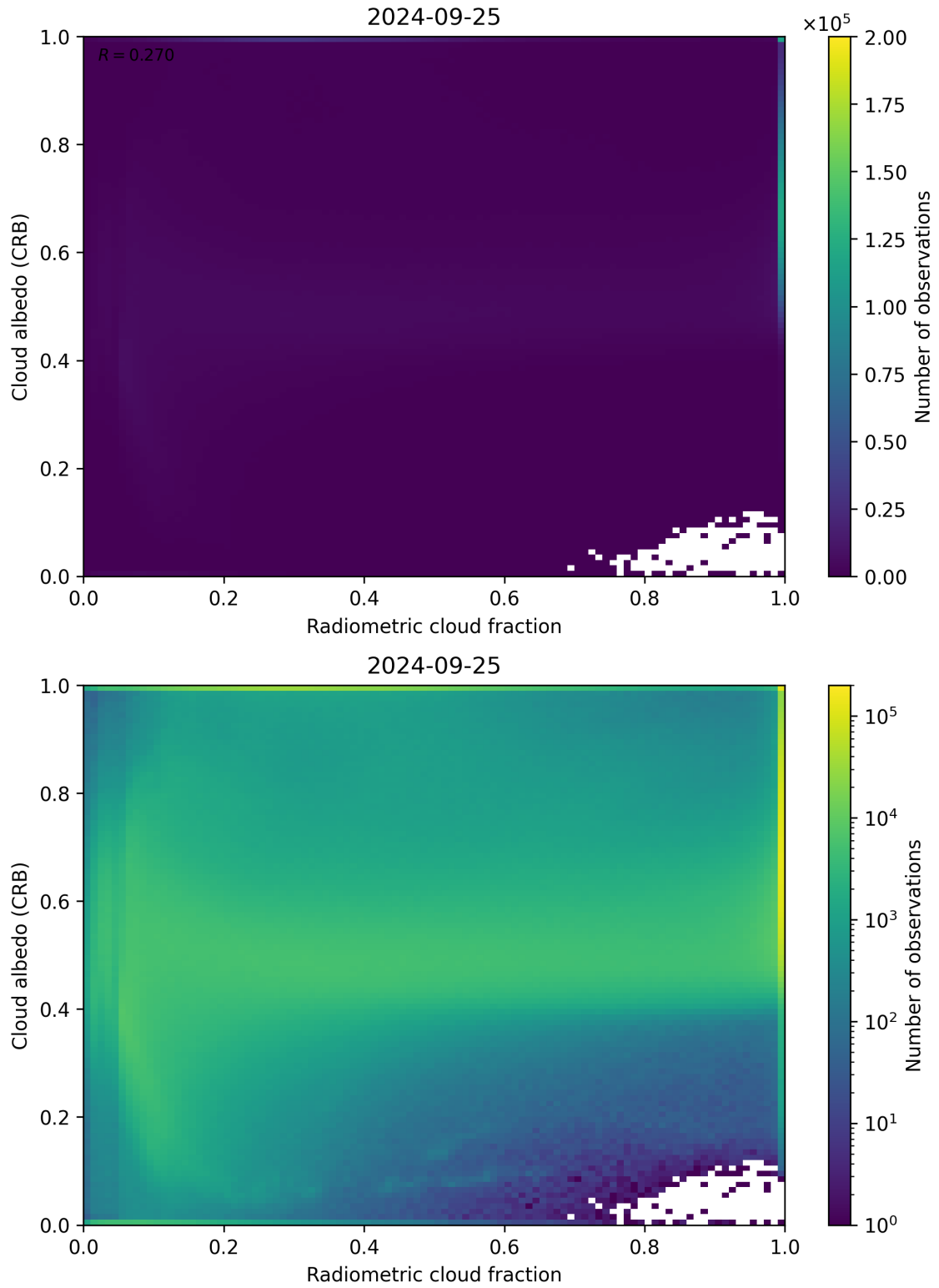
Figure 71: Scatter density plot of “Radiometric cloud fraction” against “Cloud albedo (CRB)” for 2024-09-24 to 2024-09-26.
