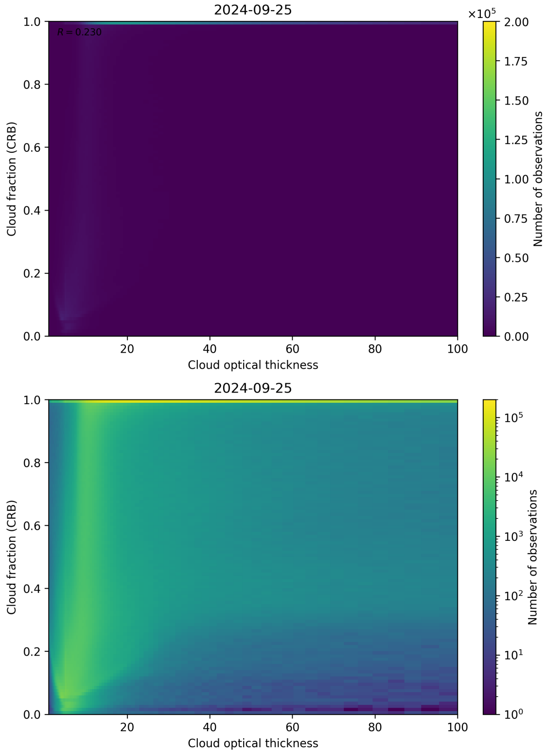
Figure 84: Scatter density plot of “Cloud optical thickness” against “Cloud fraction (CRB)” for 2024-09-24 to 2024-09-26.
