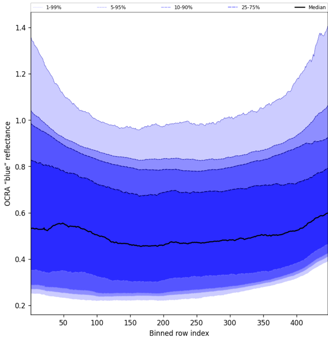
Figure 67: Along track statistics of “OCRA “blue” reflectance” for 2024-09-24 to 2024-09-26
