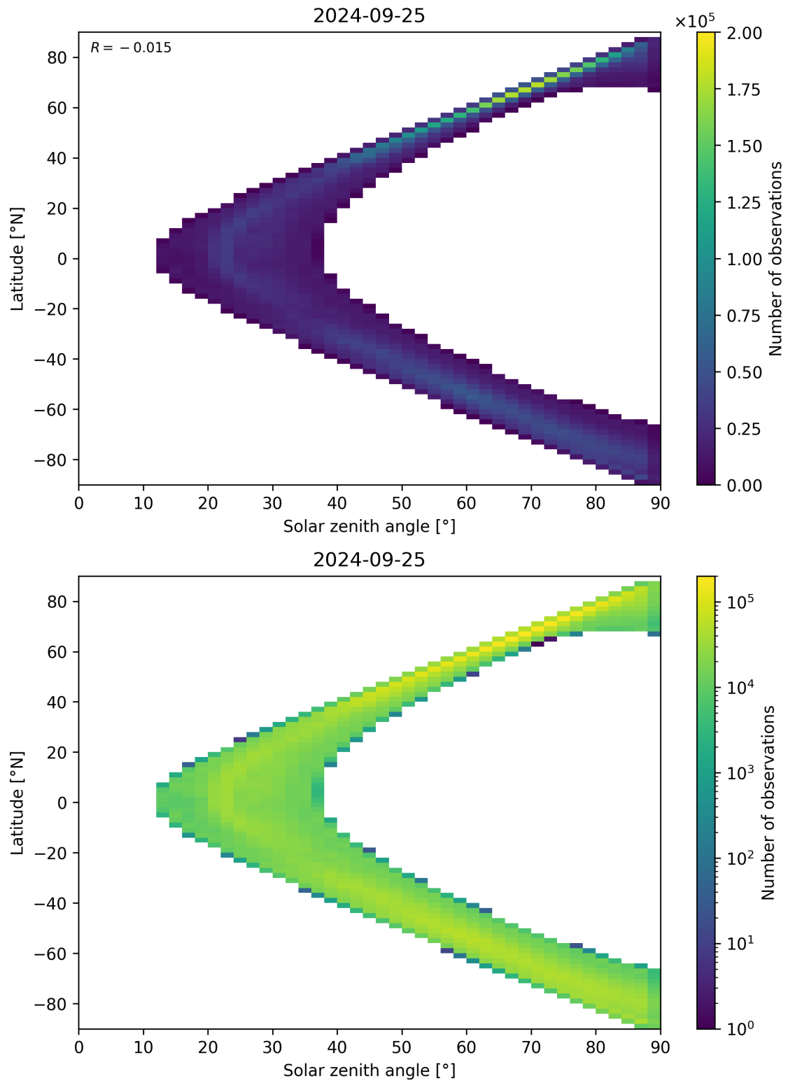
Figure 105: Scatter density plot of “Solar zenith angle” against “Latitude” for 2024-09-24 to 2024-09-26.
