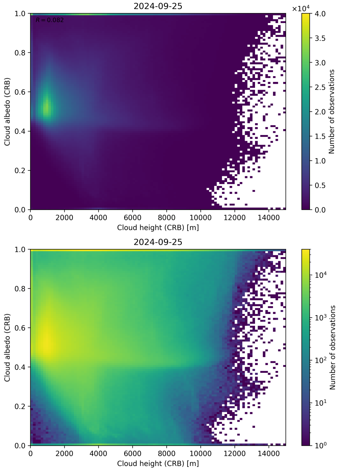
Figure 80: Scatter density plot of “Cloud height (CRB)” against “Cloud albedo (CRB)” for 2024-09-24 to 2024-09-26.
