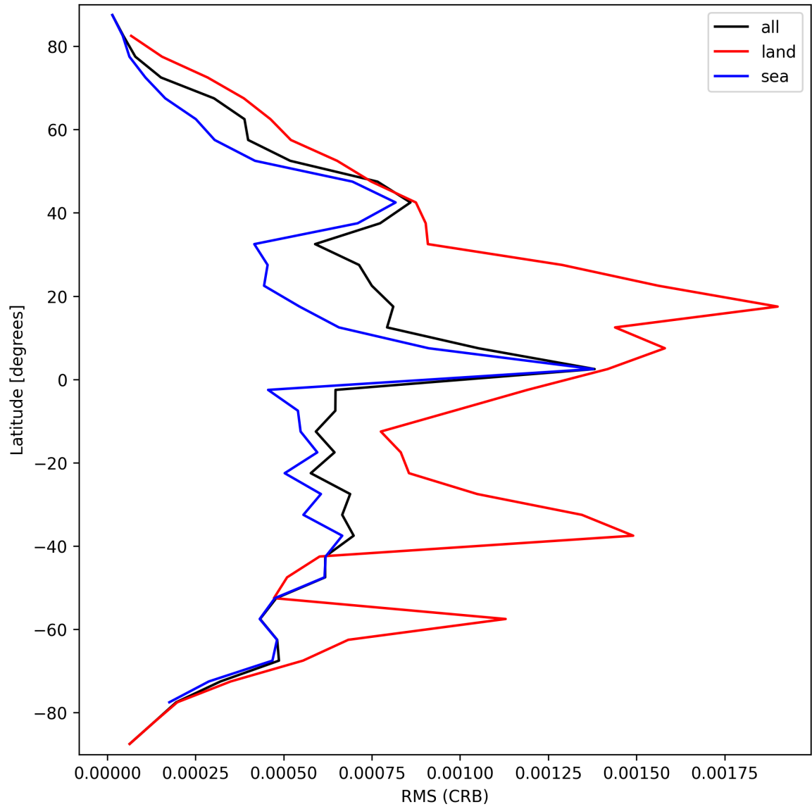
Figure 32: Zonal average of “RMS (CRB)” for 2024-09-24 to 2024-09-26.
