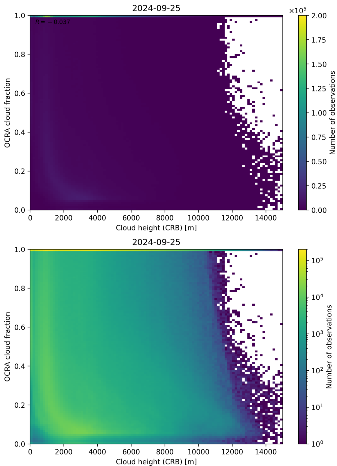
Figure 81: Scatter density plot of “Cloud height (CRB)” against “OCRA cloud fraction” for 2024-09-24 to 2024-09-26.
