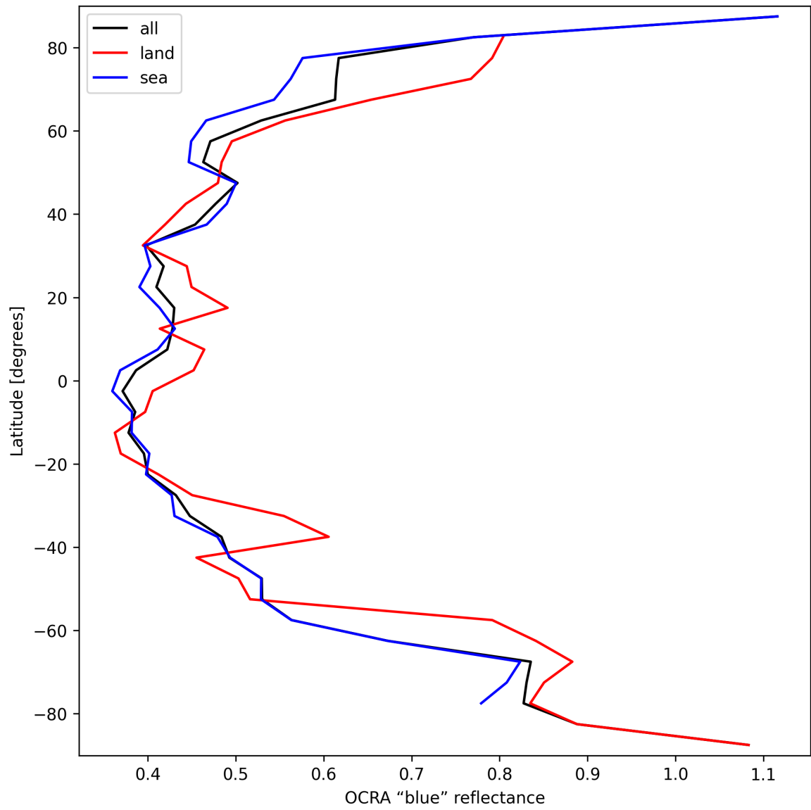
Figure 35: Zonal average of “OCRA “blue” reflectance” for 2024-09-24 to 2024-09-26.
