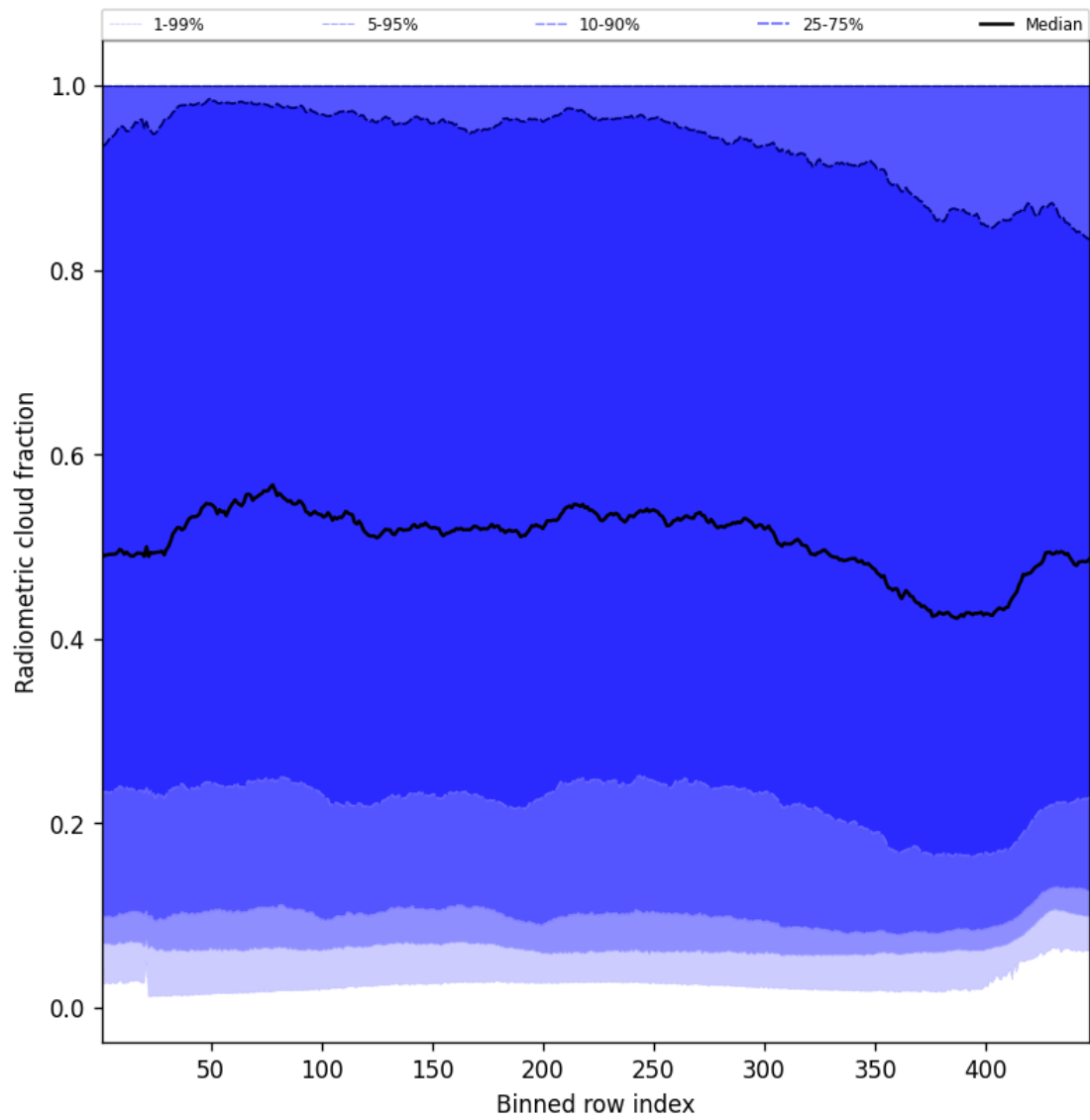
Figure 55: Along track statistics of “Radiometric cloud fraction” for 2024-09-24 to 2024-09-26
