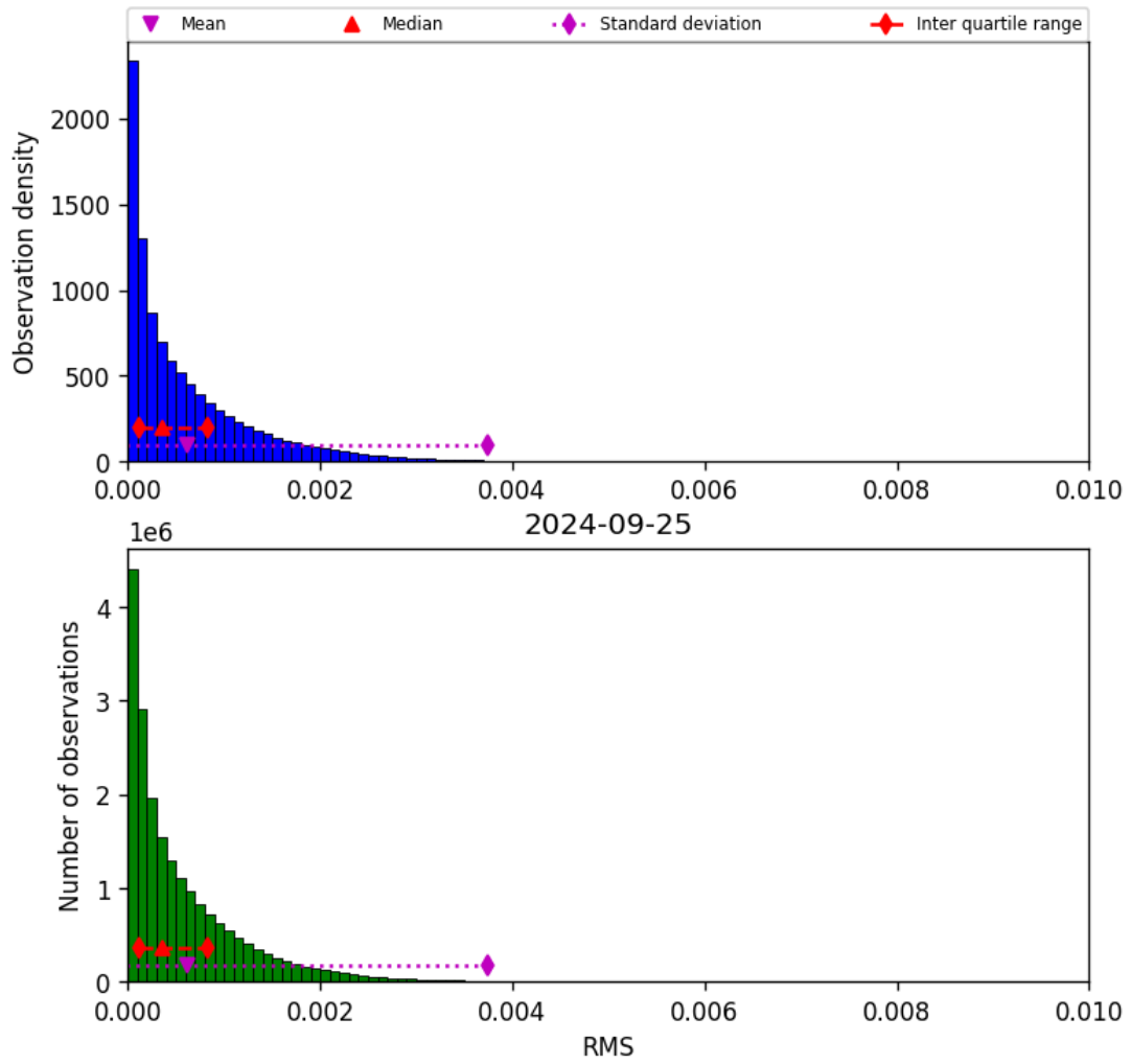
Figure 47: Histogram of “RMS” for 2024-09-24 to 2024-09-26
