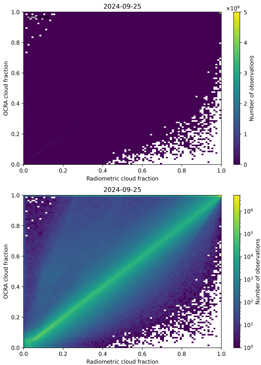
Figure 72: Scatter density plot of “Radiometric cloud fraction” against “OCRA cloud fraction” for 2024-09-24 to 2024-09-26.
