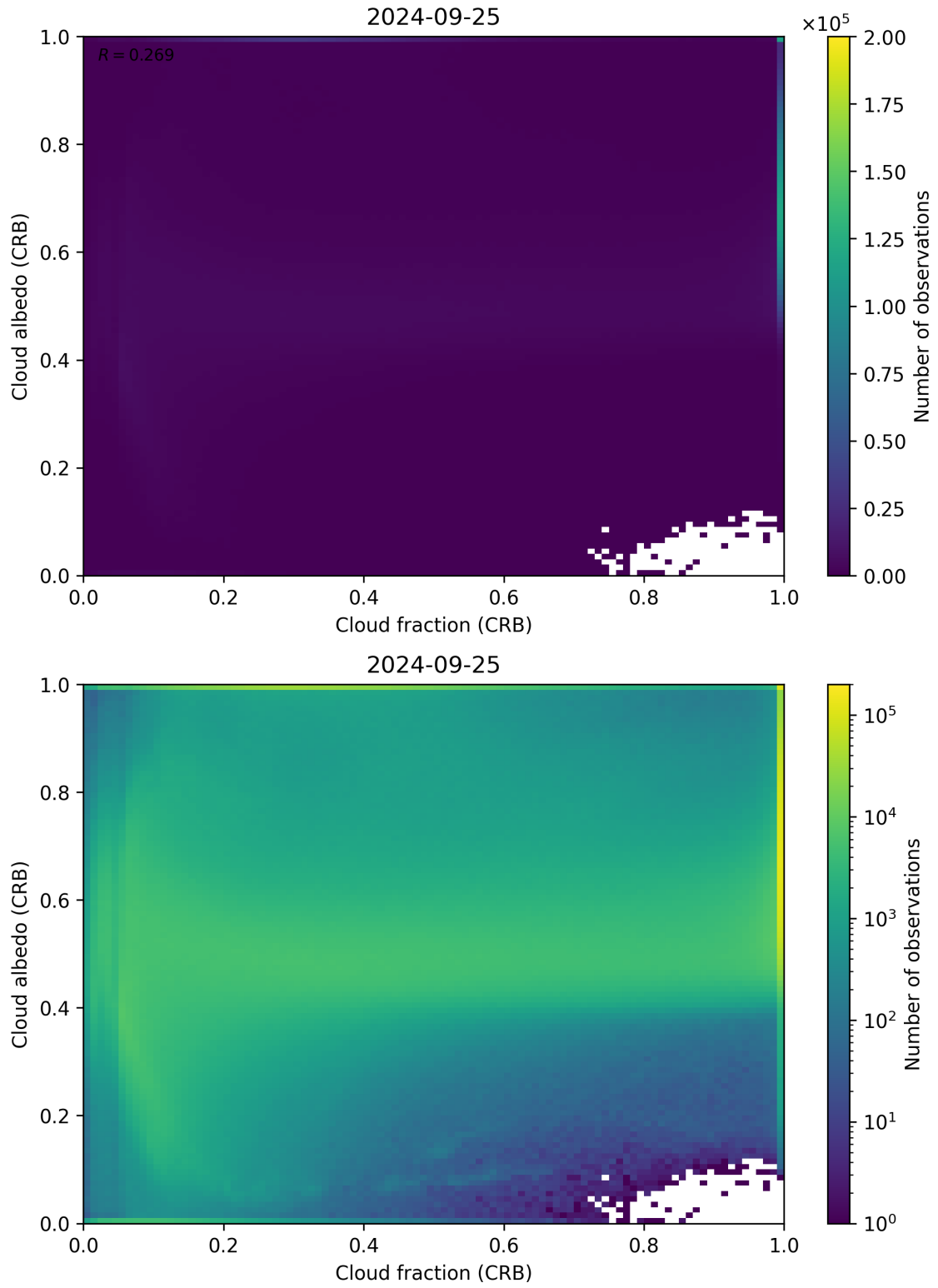
Figure 77: Scatter density plot of “Cloud fraction (CRB)” against “Cloud albedo (CRB)” for 2024-09-24 to 2024-09-26.
