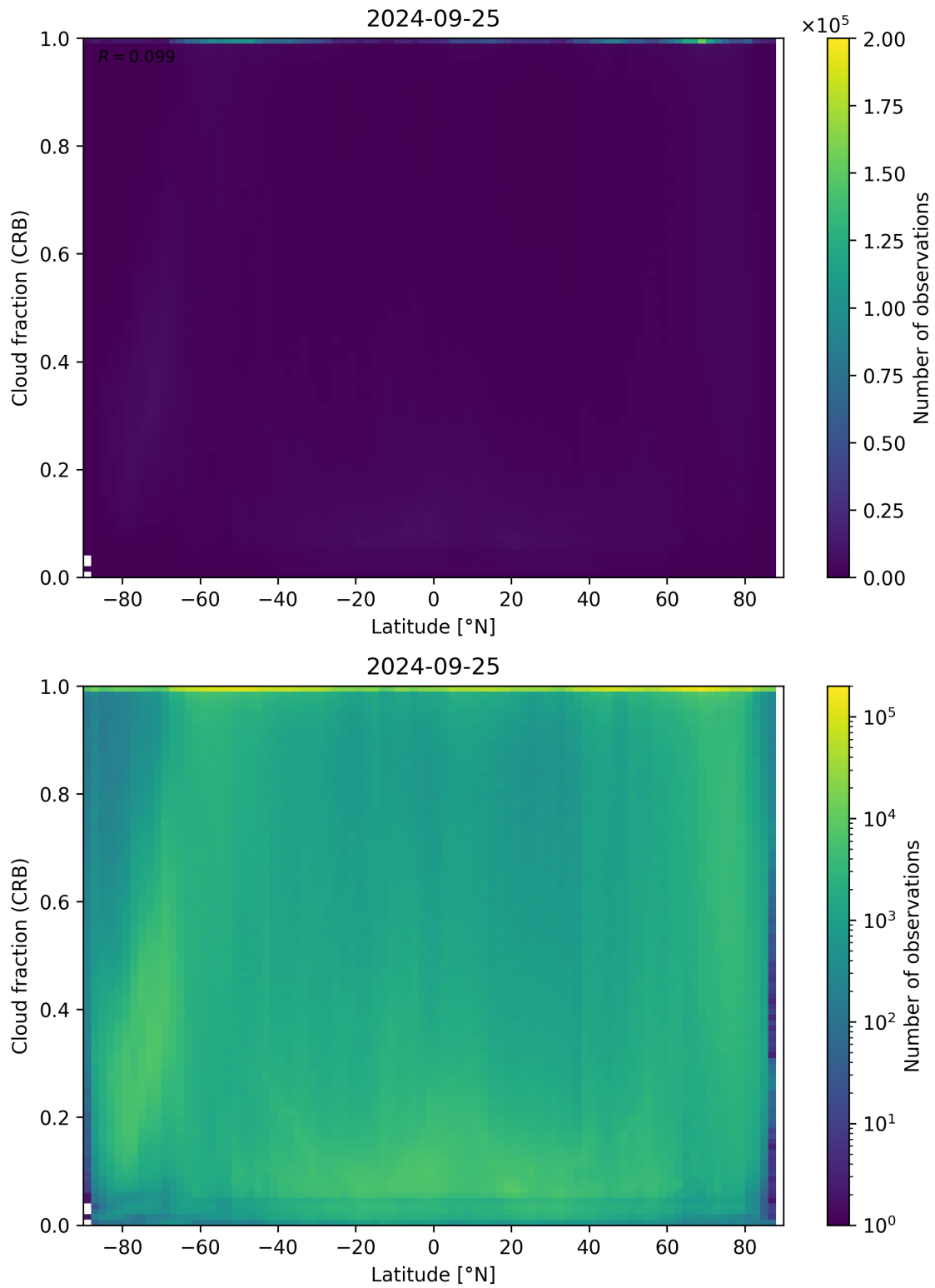
Figure 94: Scatter density plot of “Latitude” against “Cloud fraction (CRB)” for 2024-09-24 to 2024-09-26.
