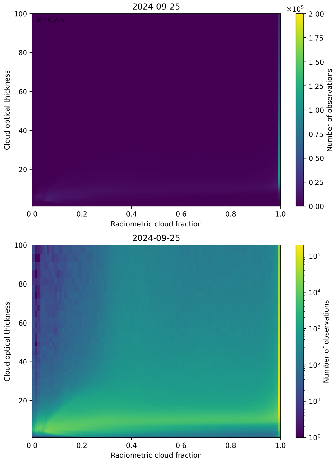
Figure 75: Scatter density plot of “Radiometric cloud fraction” against “Cloud optical thickness” for 2024-09-24 to 2024-09-26.
