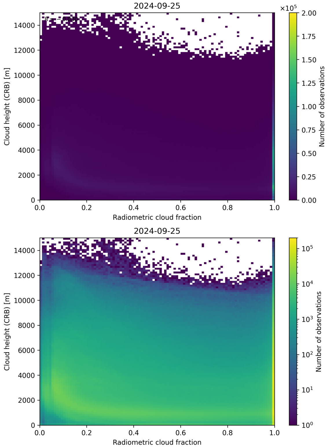
Figure 74: Scatter density plot of “Radiometric cloud fraction” against “Cloud height (CRB)” for 2024-09-24 to 2024-09-26.
