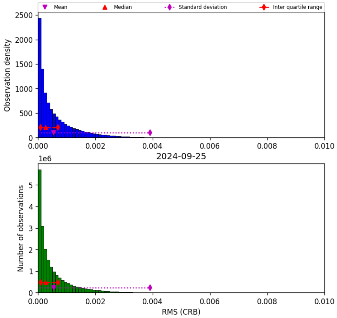
Figure 48: Histogram of “RMS (CRB)” for 2024-09-24 to 2024-09-26
