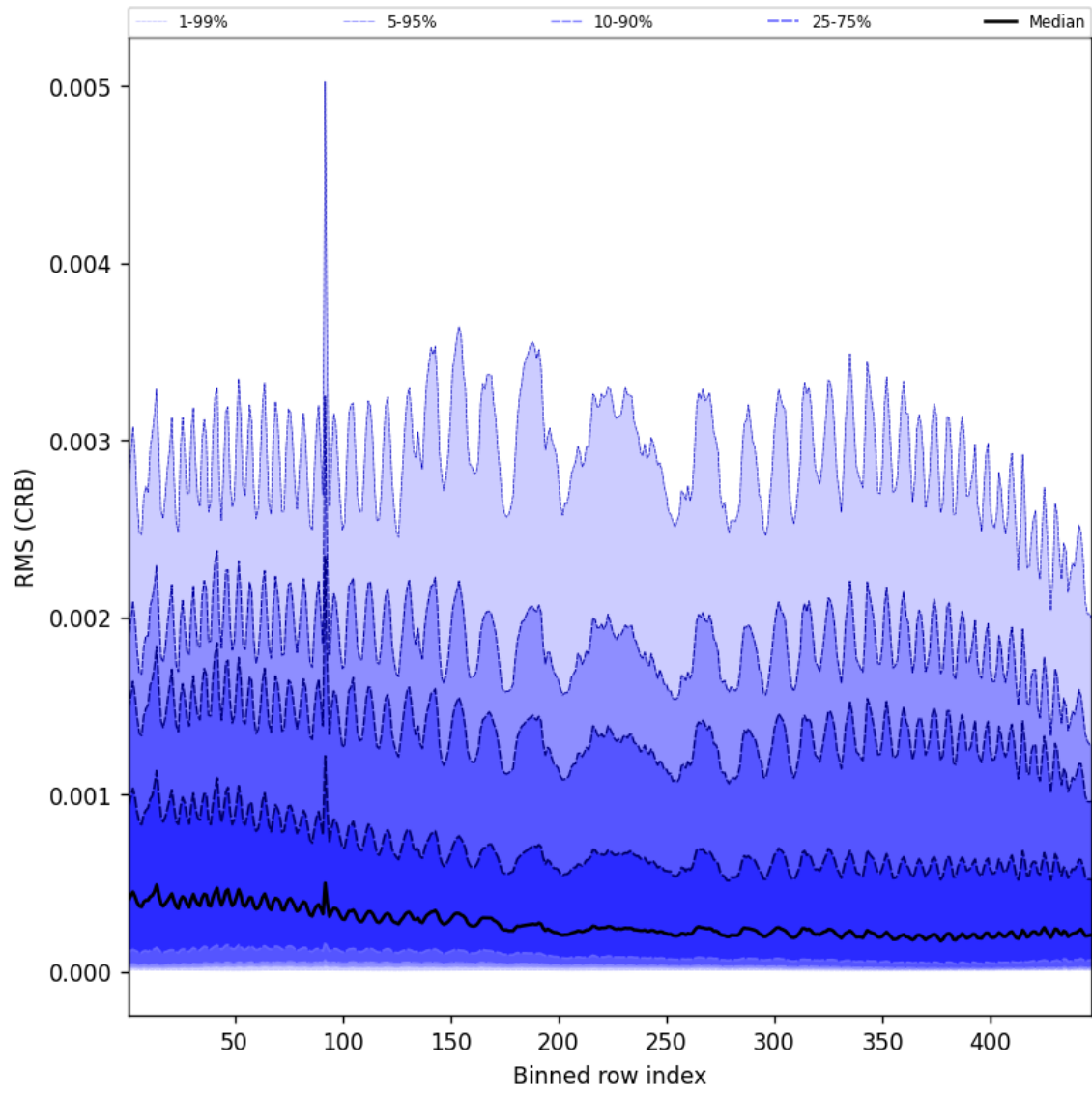
Figure 64: Along track statistics of “RMS (CRB)” for 2024-09-24 to 2024-09-26
