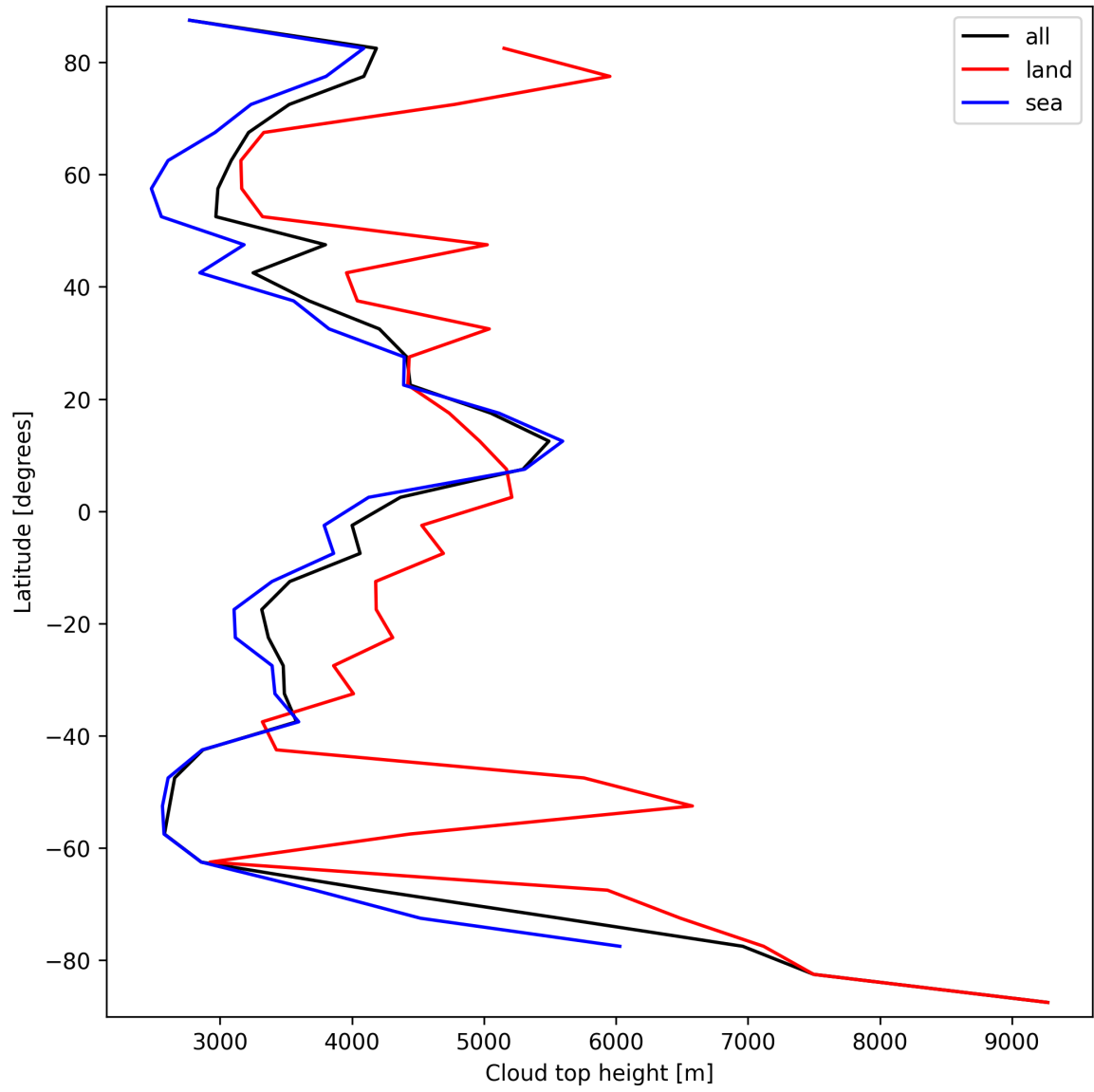
Figure 24: Zonal average of “Cloud top height” for 2024-09-24 to 2024-09-26.
