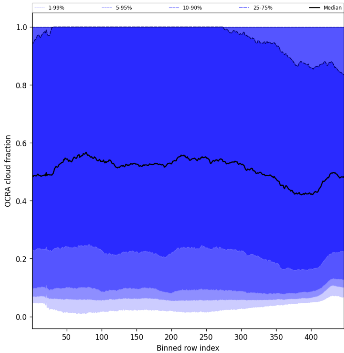
Figure 66: Along track statistics of “OCRA cloud fraction” for 2024-09-24 to 2024-09-26
