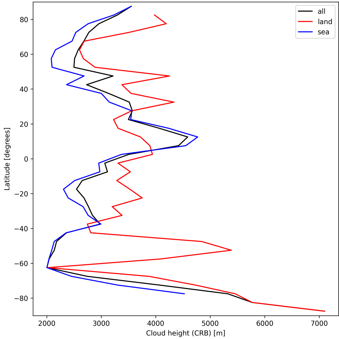
Figure 27: Zonal average of “Cloud height (CRB)” for 2024-09-24 to 2024-09-26.
