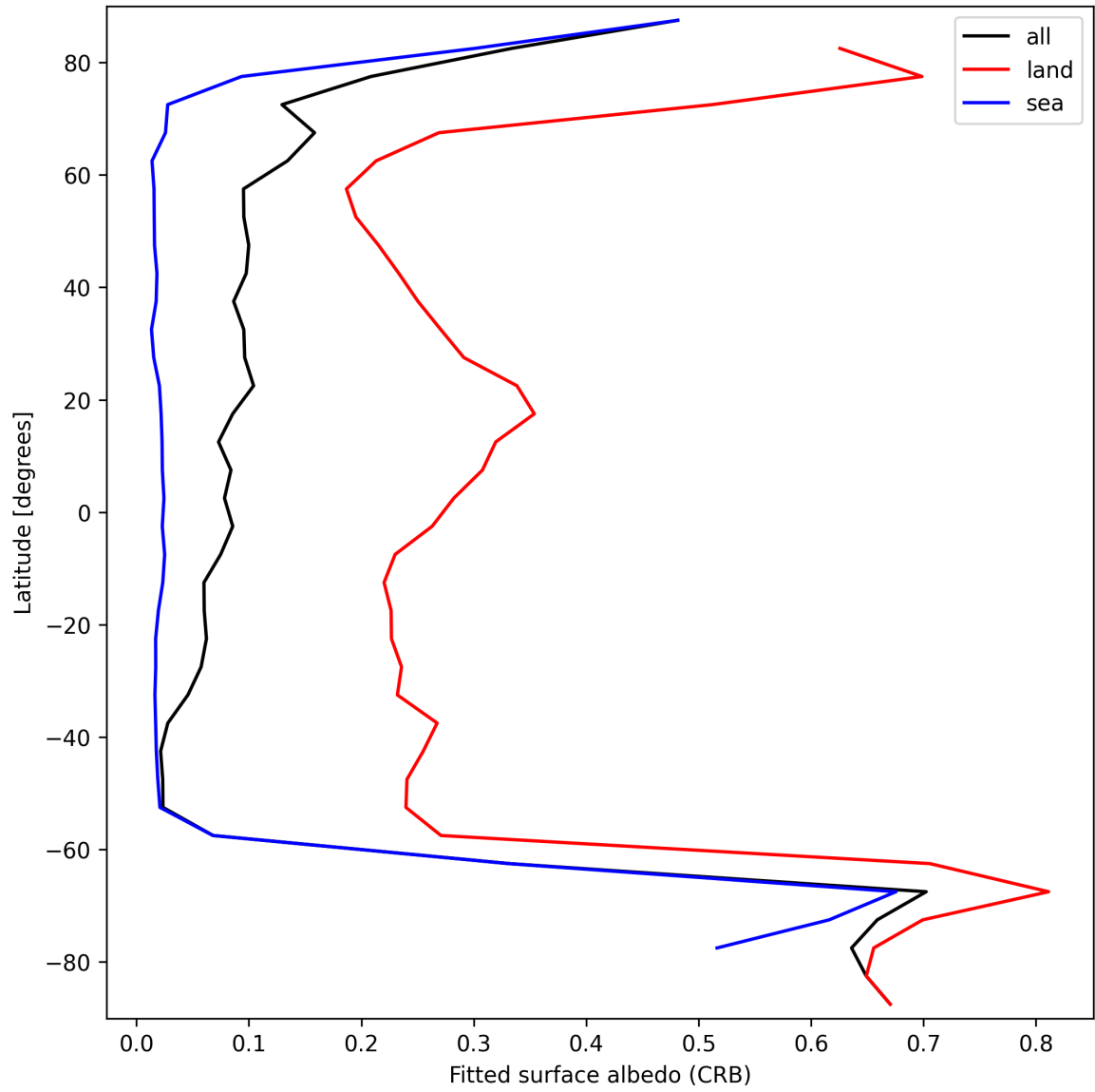
Figure 30: Zonal average of “Fitted surface albedo (CRB)” for 2024-09-24 to 2024-09-26.
