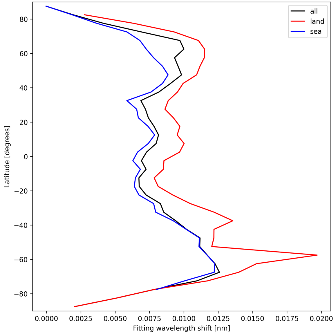
Figure 33: Zonal average of “Fitting wavelength shift” for 2024-09-24 to 2024-09-26.
