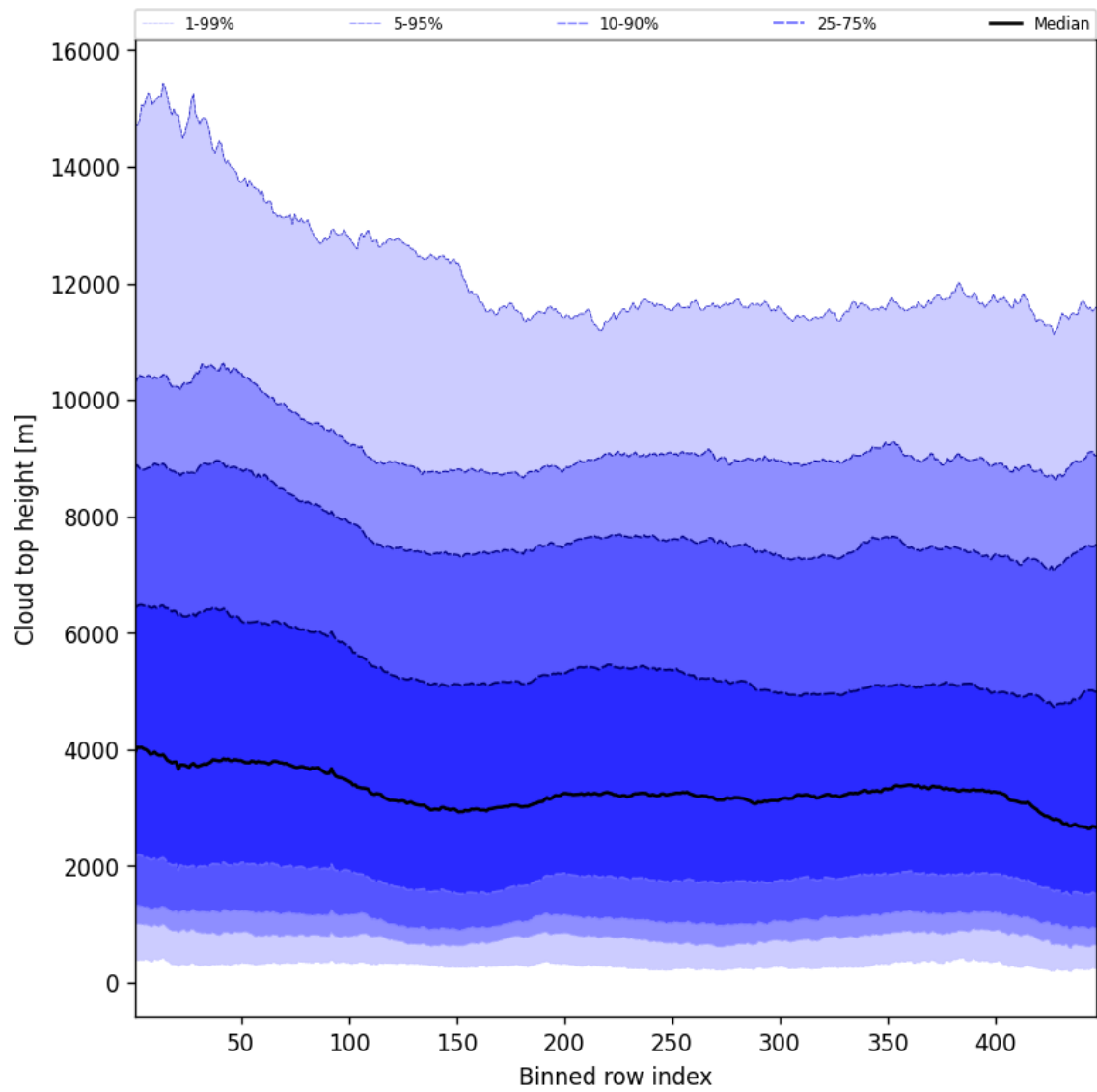
Figure 56: Along track statistics of “Cloud top height” for 2024-09-24 to 2024-09-26
