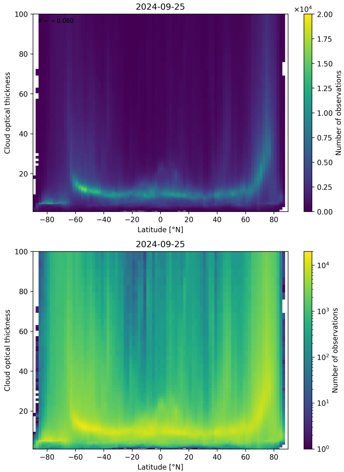
Figure 96: Scatter density plot of “Latitude” against “Cloud optical thickness” for 2024-09-24 to 2024-09-26.
