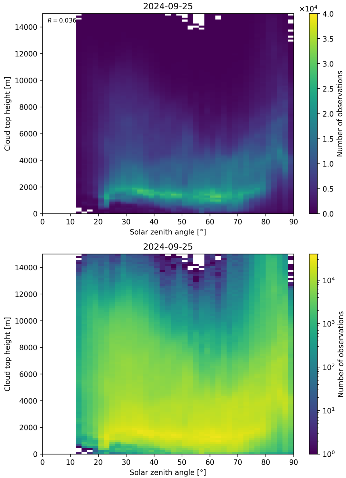
Figure 104: Scatter density plot of “Solar zenith angle” against “Cloud top height” for 2024-09-24 to 2024-09-26.
