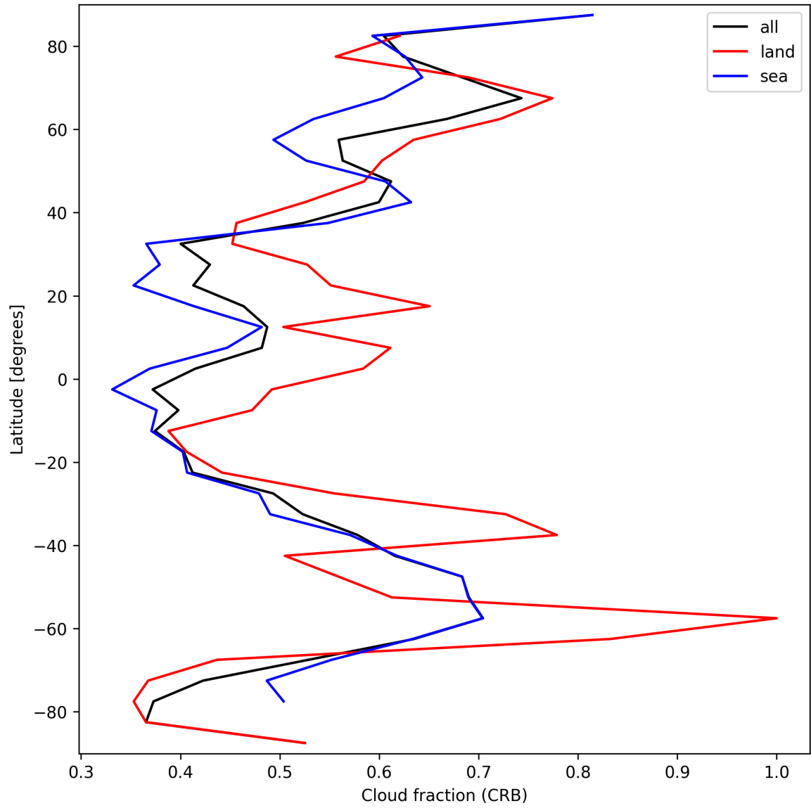
Figure 26: Zonal average of “Cloud fraction (CRB)” for 2024-09-24 to 2024-09-26.
