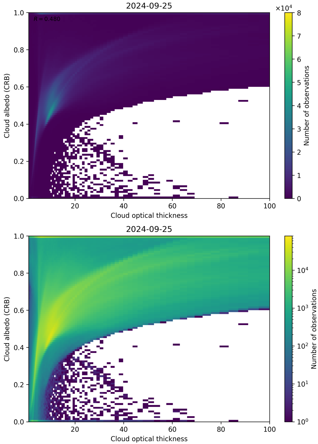
Figure 82: Scatter density plot of “Cloud optical thickness” against “Cloud albedo (CRB)” for 2024-09-24 to 2024-09-26.
