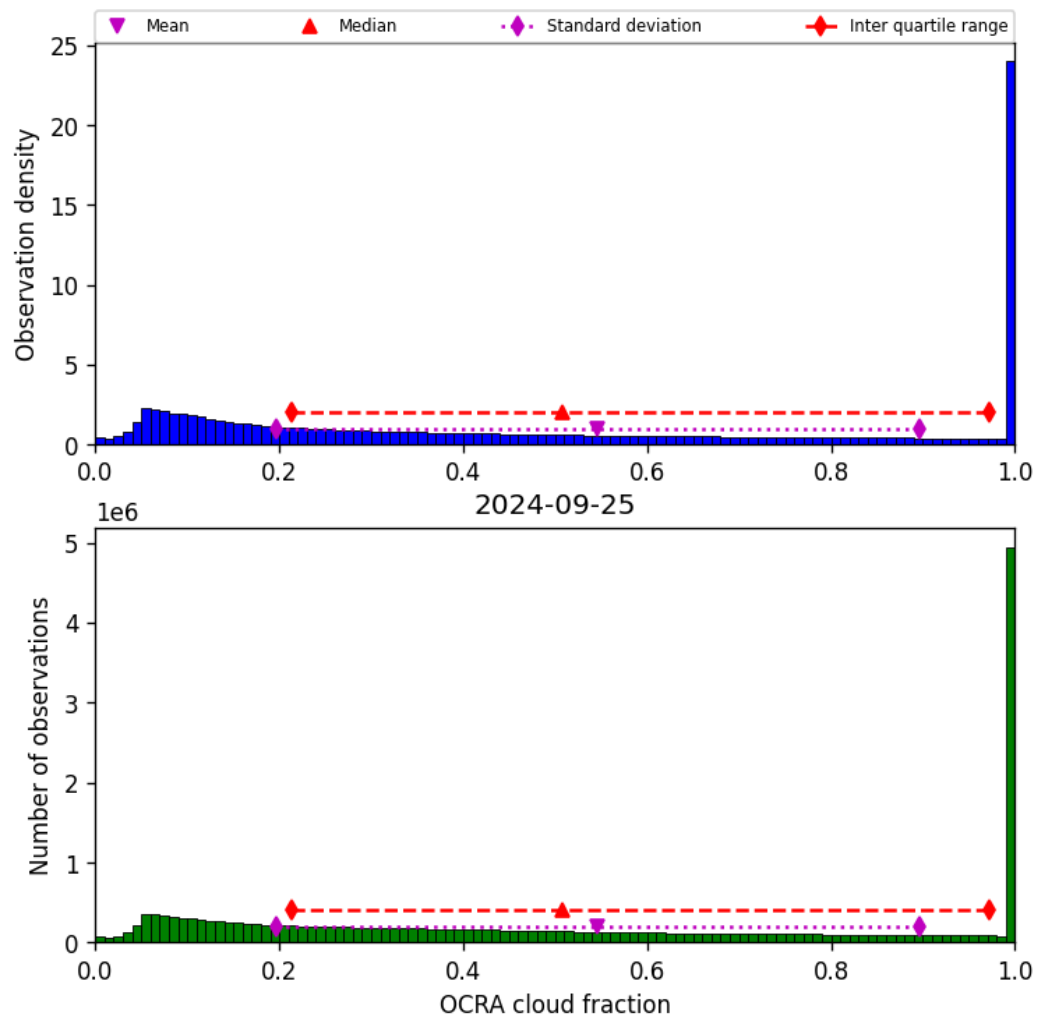
Figure 50: Histogram of “OCRA cloud fraction” for 2024-09-24 to 2024-09-26
