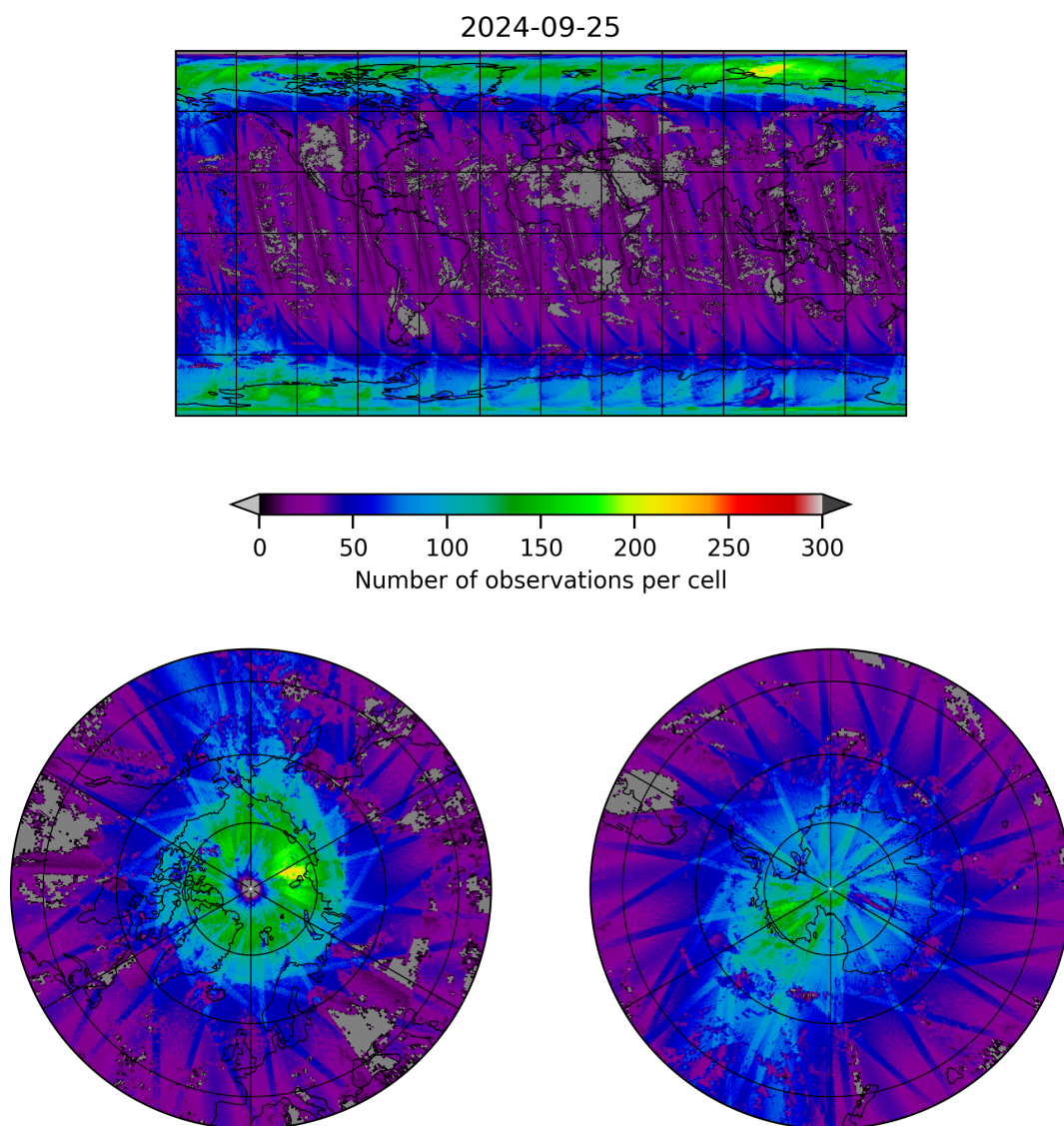
Figure 21: Map of the number of observations for 2024-09-24 to 2024-09-26
