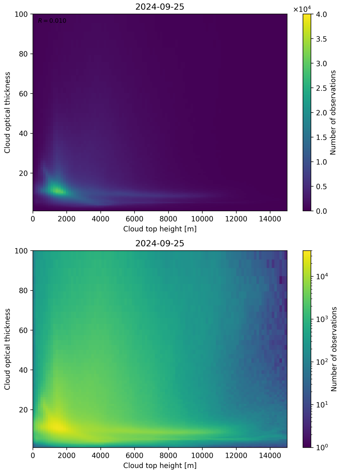
Figure 90: Scatter density plot of “Cloud top height” against “Cloud optical thickness” for 2024-09-24 to 2024-09-26.
