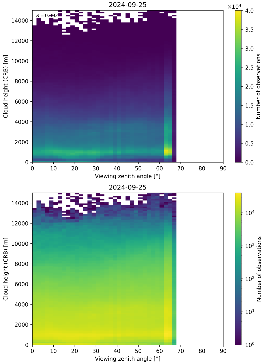
Figure 110: Scatter density plot of “Viewing zenith angle” against “Cloud height (CRB)” for 2024-09-24 to 2024-09-26.
