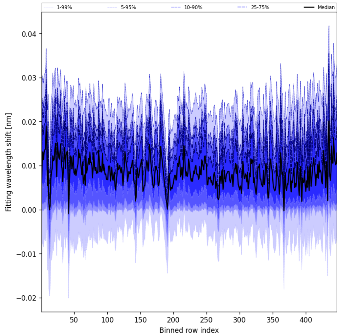
Figure 65: Along track statistics of “Fitting wavelength shift” for 2024-09-24 to 2024-09-26
