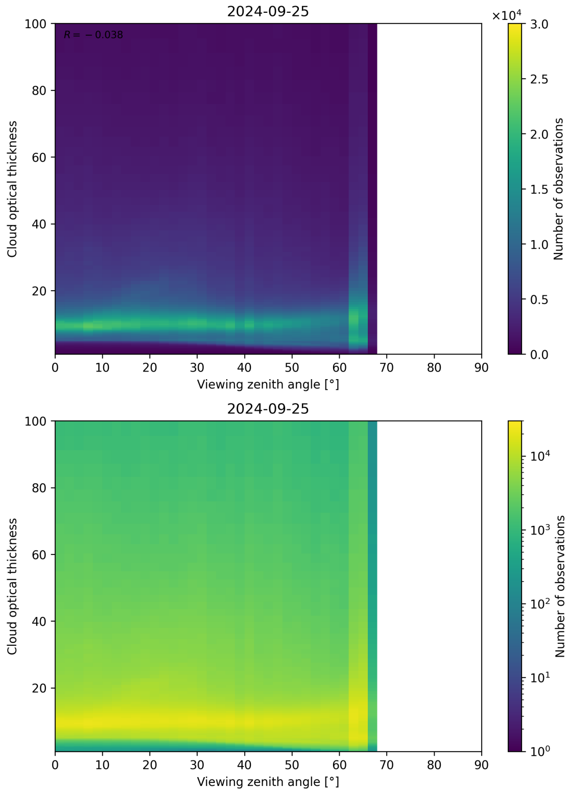
Figure 111: Scatter density plot of “Viewing zenith angle” against “Cloud optical thickness” for 2024-09-24 to 2024-09-26.
