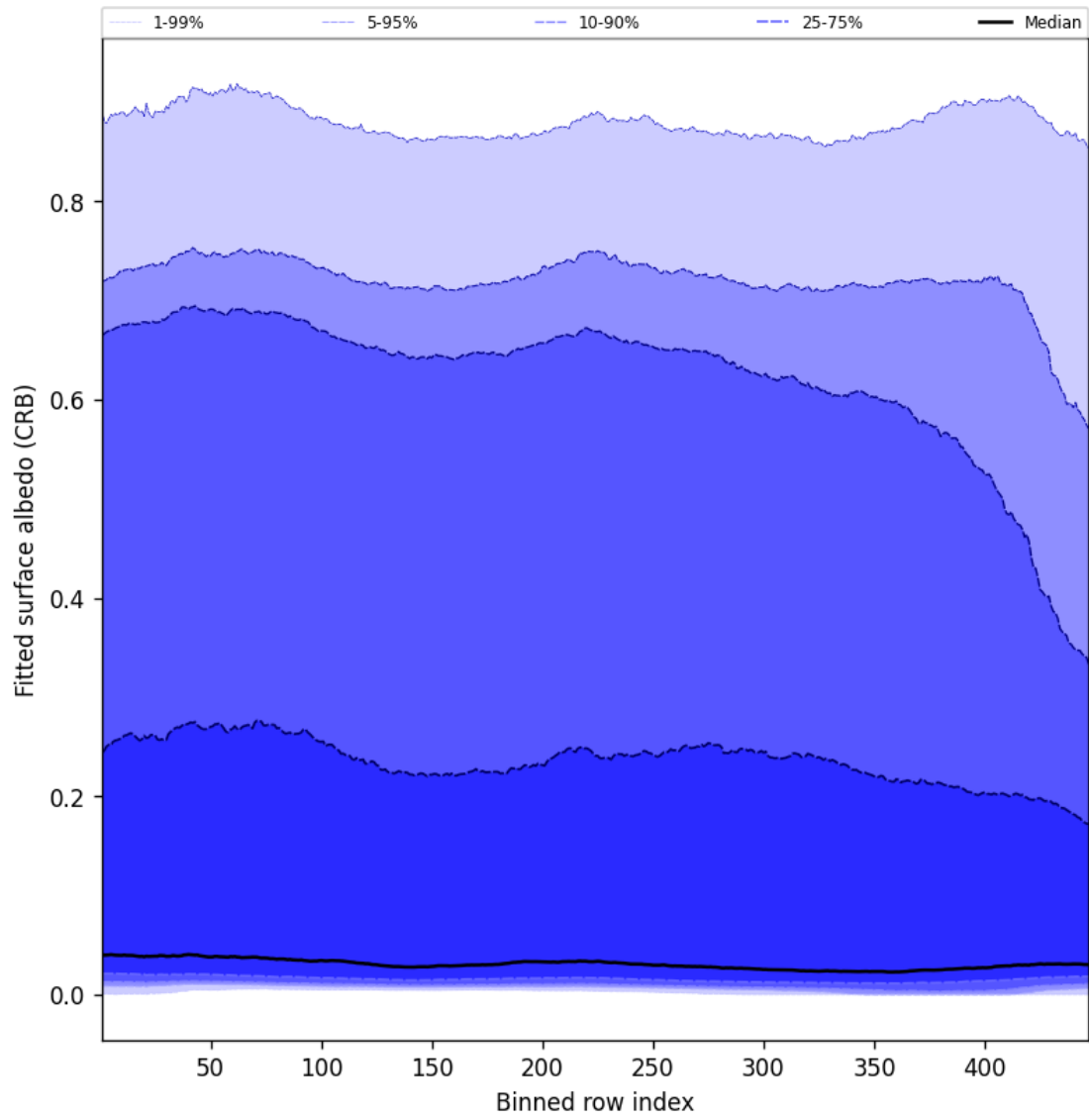
Figure 62: Along track statistics of “Fitted surface albedo (CRB)” for 2024-09-24 to 2024-09-26
