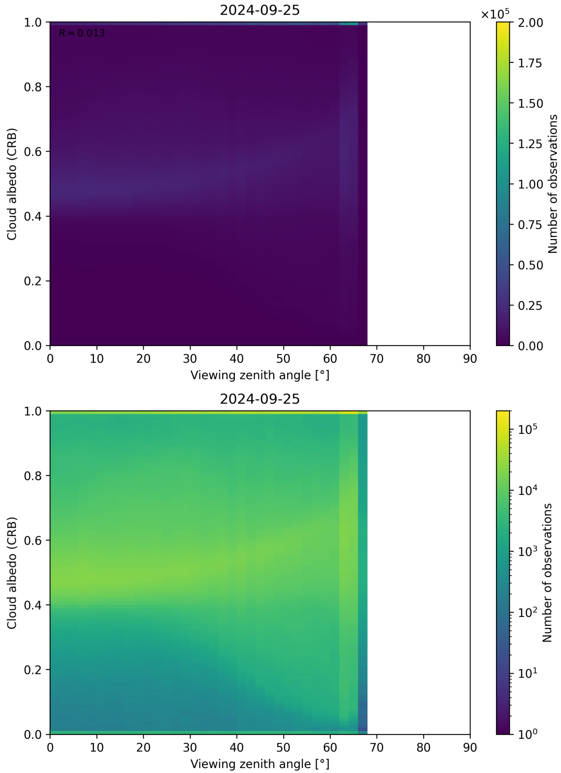
Figure 106: Scatter density plot of “Viewing zenith angle” against “Cloud albedo (CRB)” for 2024-09-24 to 2024-09-26.
