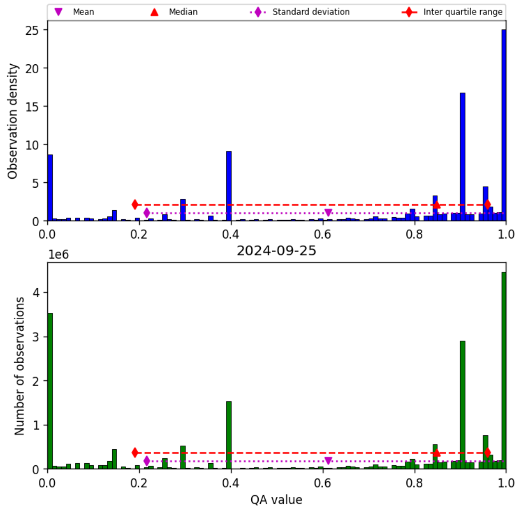
Figure 38: Histogram of “QA value” for 2024-09-24 to 2024-09-26
