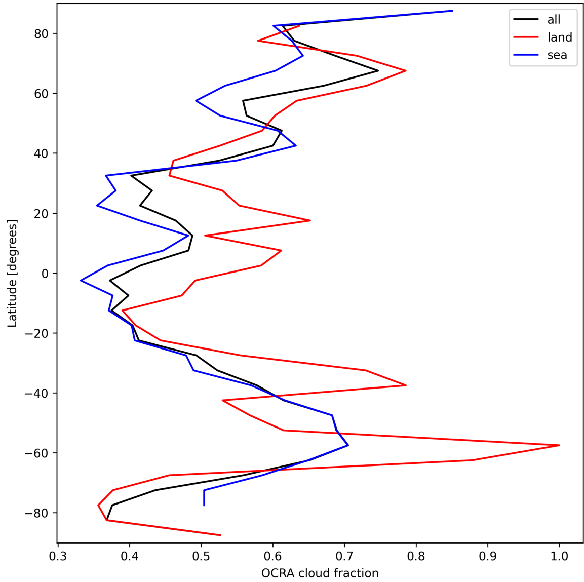
Figure 34: Zonal average of “OCRA cloud fraction” for 2024-09-24 to 2024-09-26.
