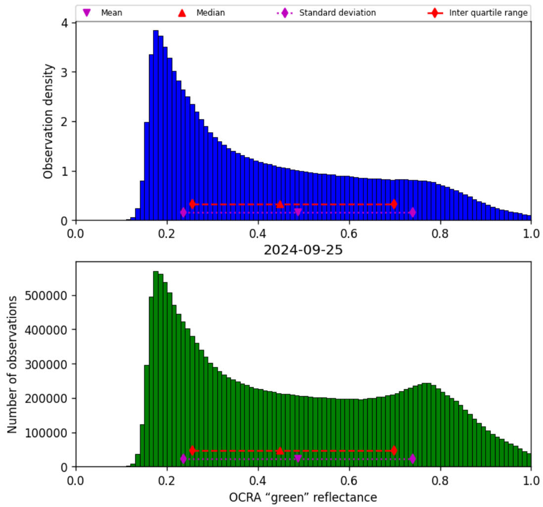
Figure 52: Histogram of “OCRA “green” reflectance” for 2024-09-24 to 2024-09-26
