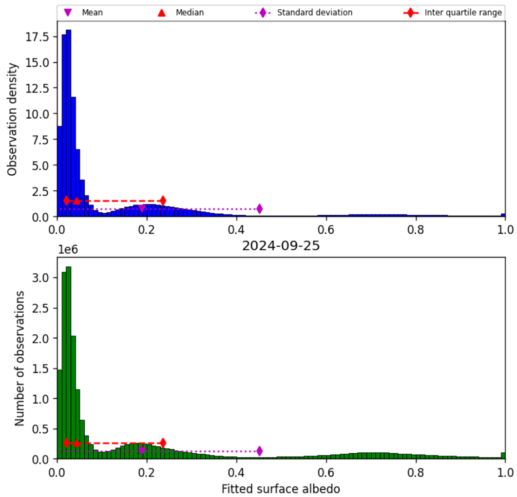
Figure 45: Histogram of “Fitted surface albedo” for 2024-09-24 to 2024-09-26
