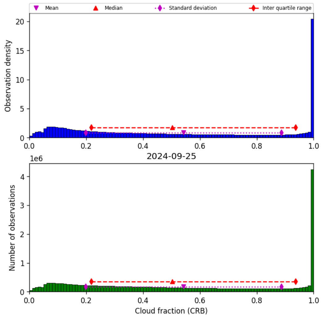
Figure 42: Histogram of “Cloud fraction (CRB)” for 2024-09-24 to 2024-09-26
