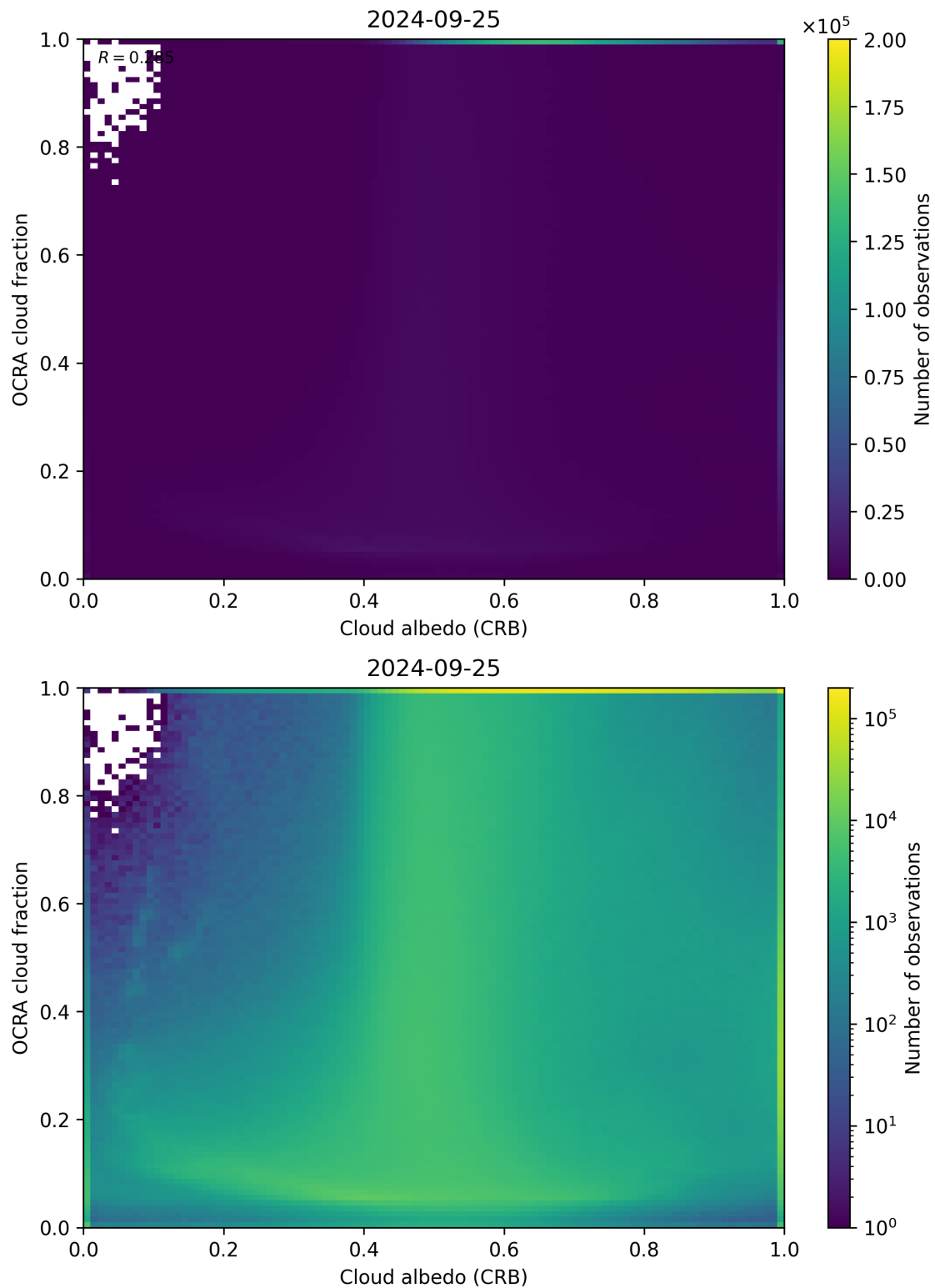
Figure 70: Scatter density plot of “Cloud albedo (CRB)” against “OCRA cloud fraction” for 2024-09-24 to 2024-09-26.
