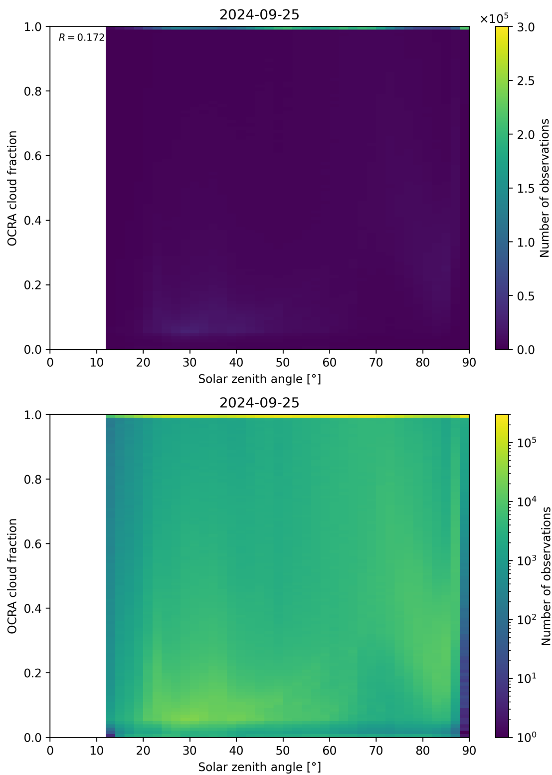
Figure 100: Scatter density plot of “Solar zenith angle” against “OCRA cloud fraction” for 2024-09-24 to 2024-09-26.
