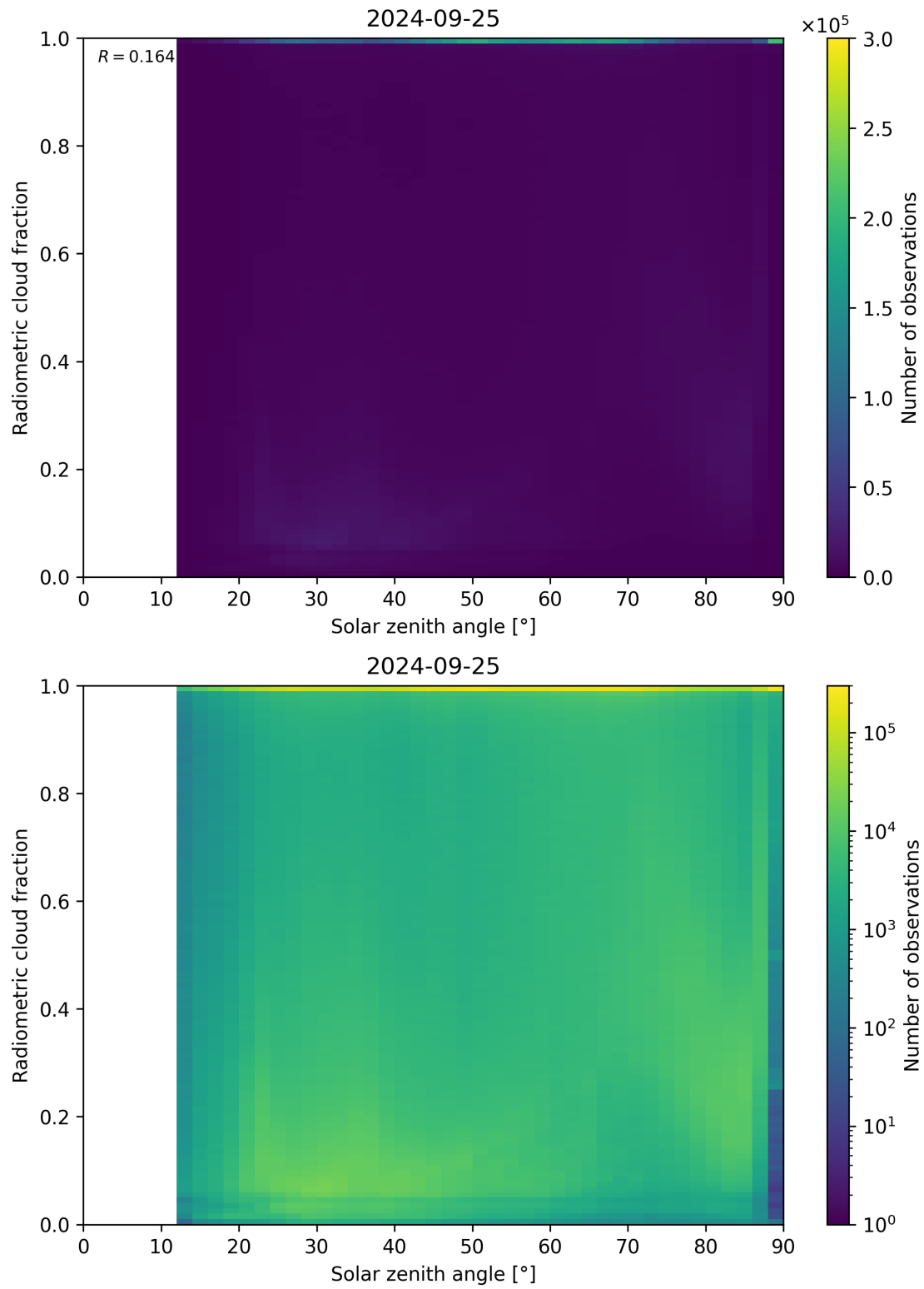
Figure 99: Scatter density plot of “Solar zenith angle” against “Radiometric cloud fraction” for 2024-09-24 to 2024-09-26.
