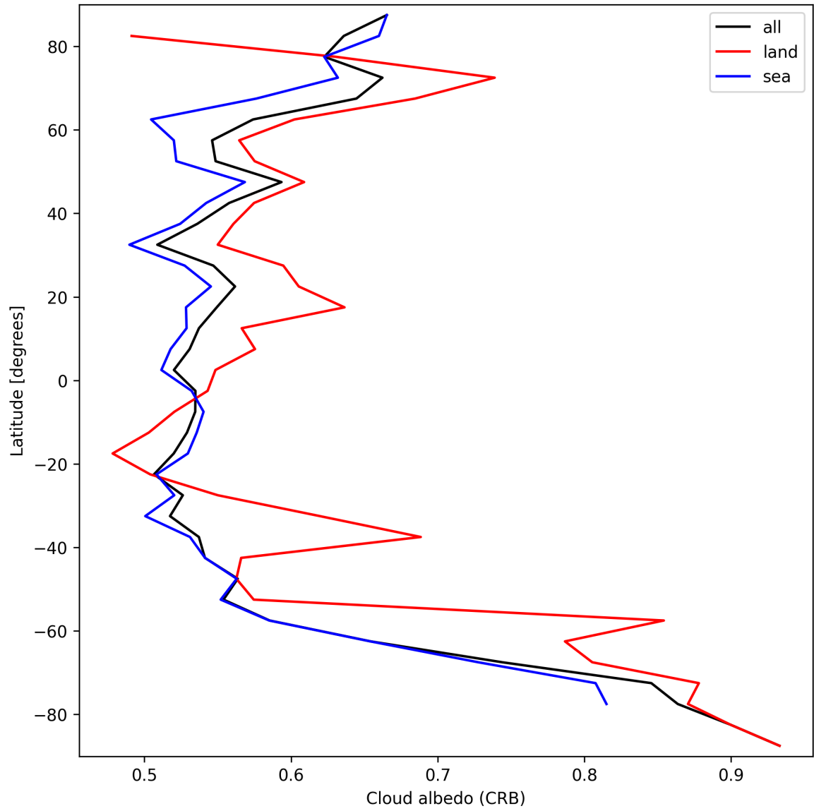
Figure 28: Zonal average of “Cloud albedo (CRB)” for 2024-09-24 to 2024-09-26.
