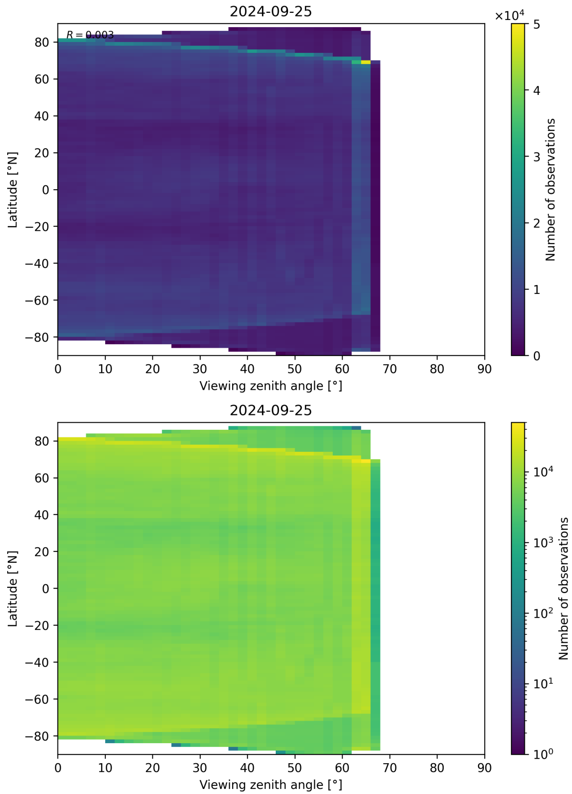
Figure 113: Scatter density plot of “Viewing zenith angle” against “Latitude” for 2024-09-24 to 2024-09-26.
