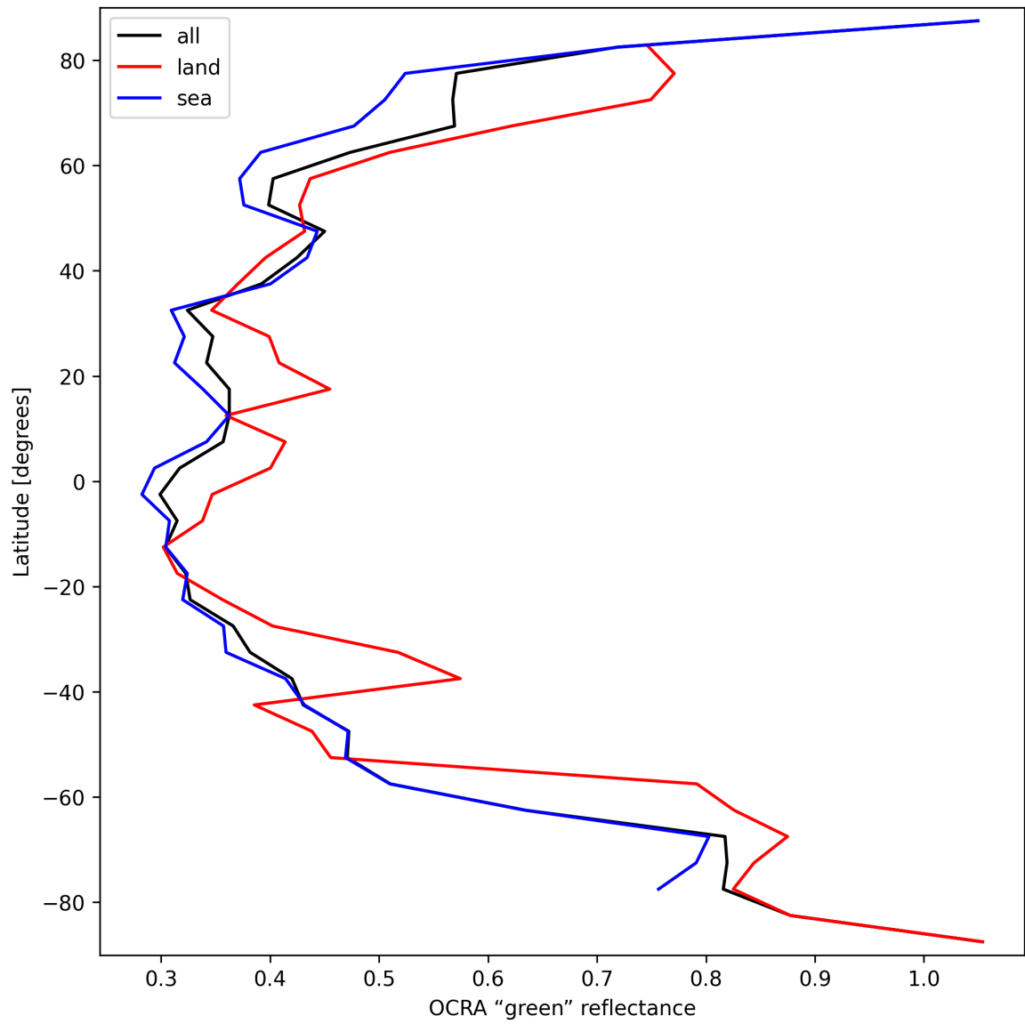
Figure 36: Zonal average of “OCRA “green” reflectance” for 2024-09-24 to 2024-09-26.
