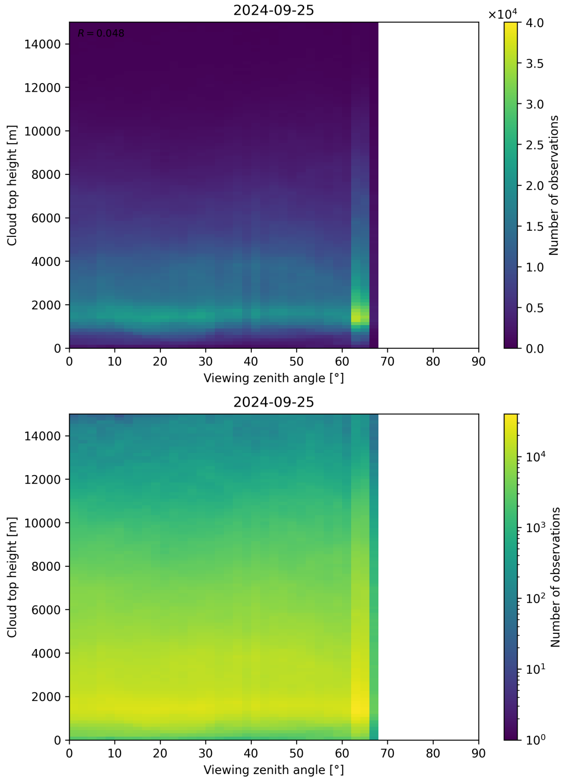
Figure 112: Scatter density plot of “Viewing zenith angle” against “Cloud top height” for 2024-09-24 to 2024-09-26.
