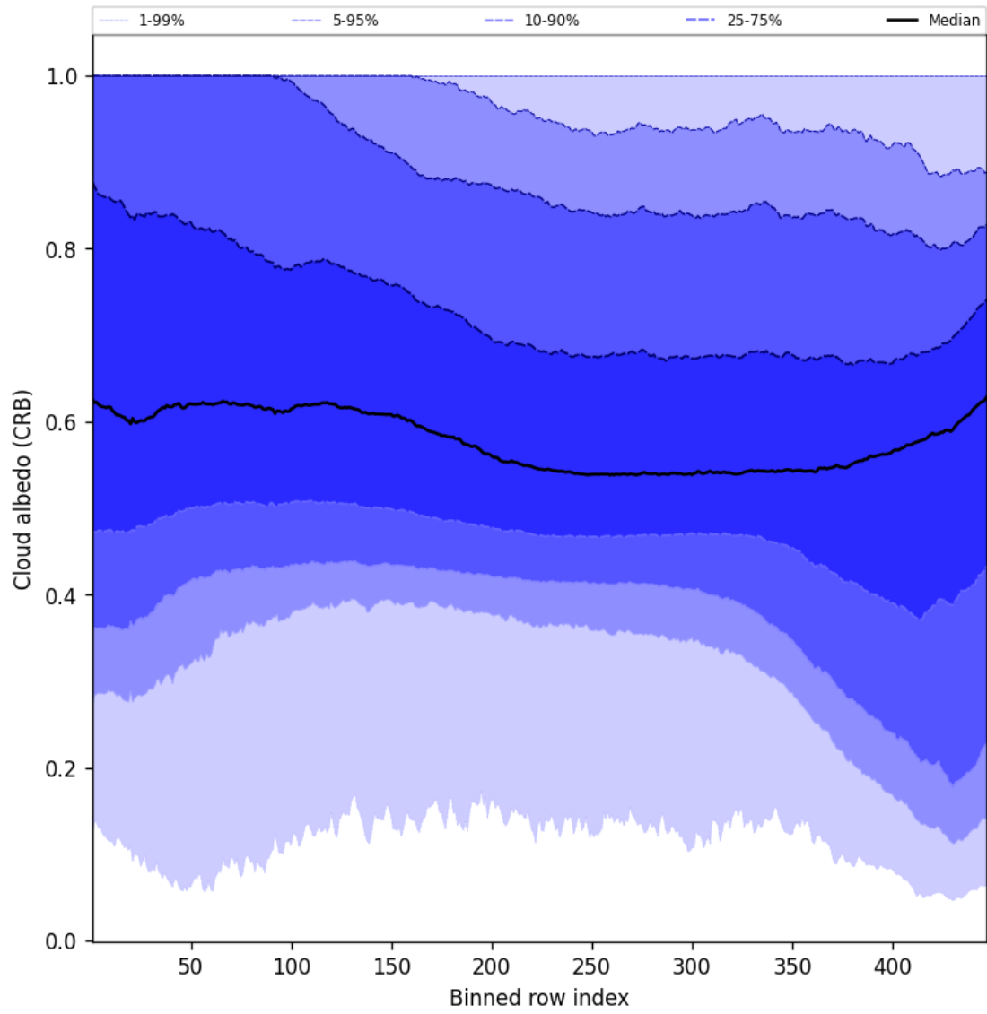
Figure 60: Along track statistics of “Cloud albedo (CRB)” for 2024-09-24 to 2024-09-26
