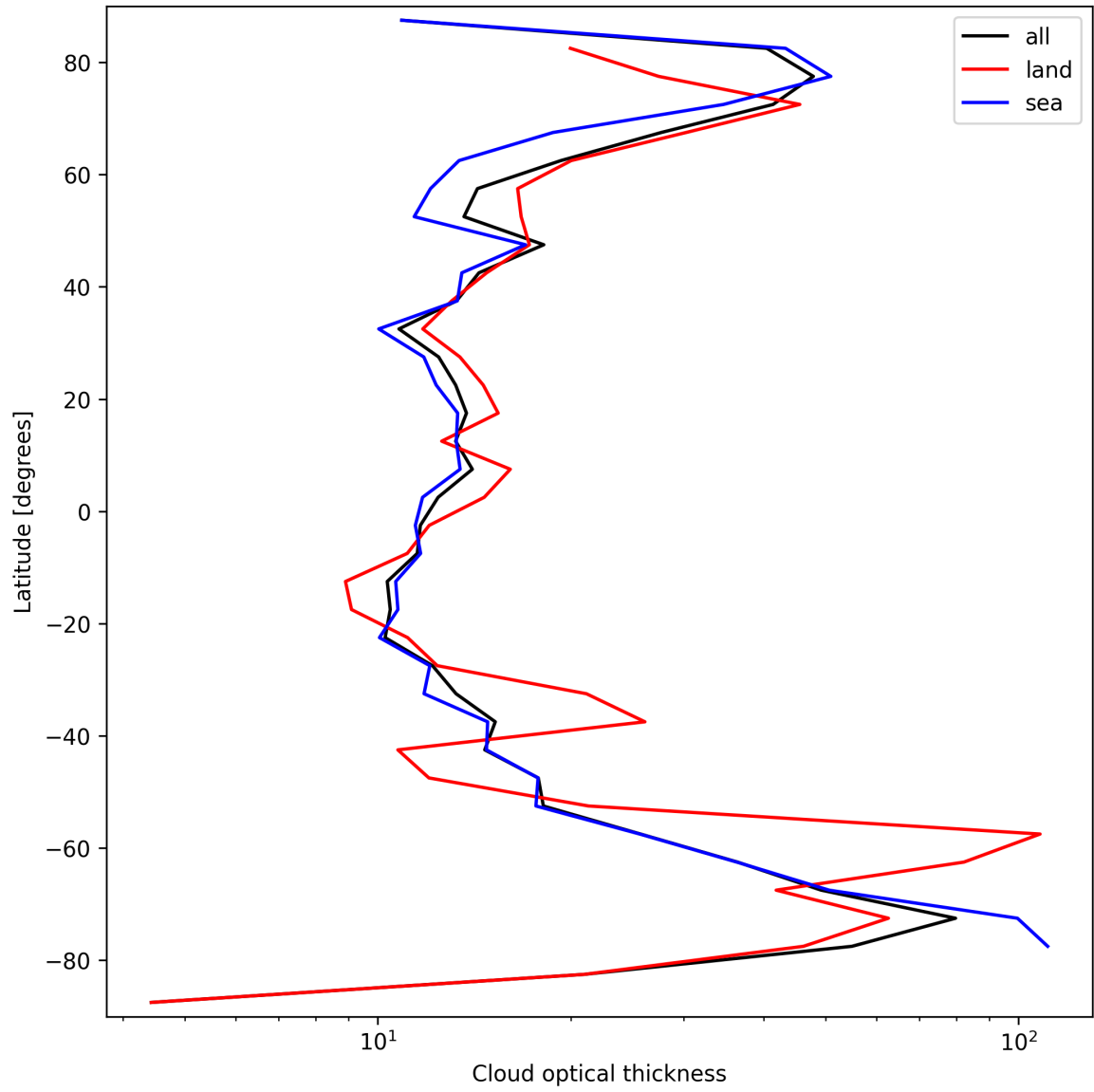
Figure 25: Zonal average of “Cloud optical thickness” for 2024-09-24 to 2024-09-26.
