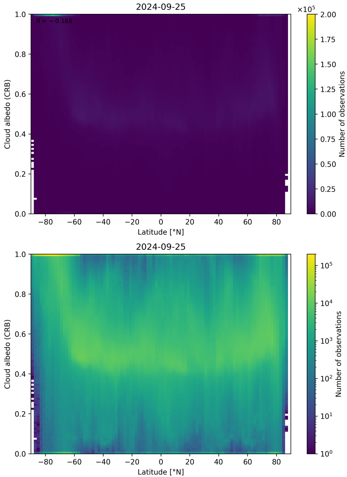
Figure 91: Scatter density plot of “Latitude” against “Cloud albedo (CRB)” for 2024-09-24 to 2024-09-26.
