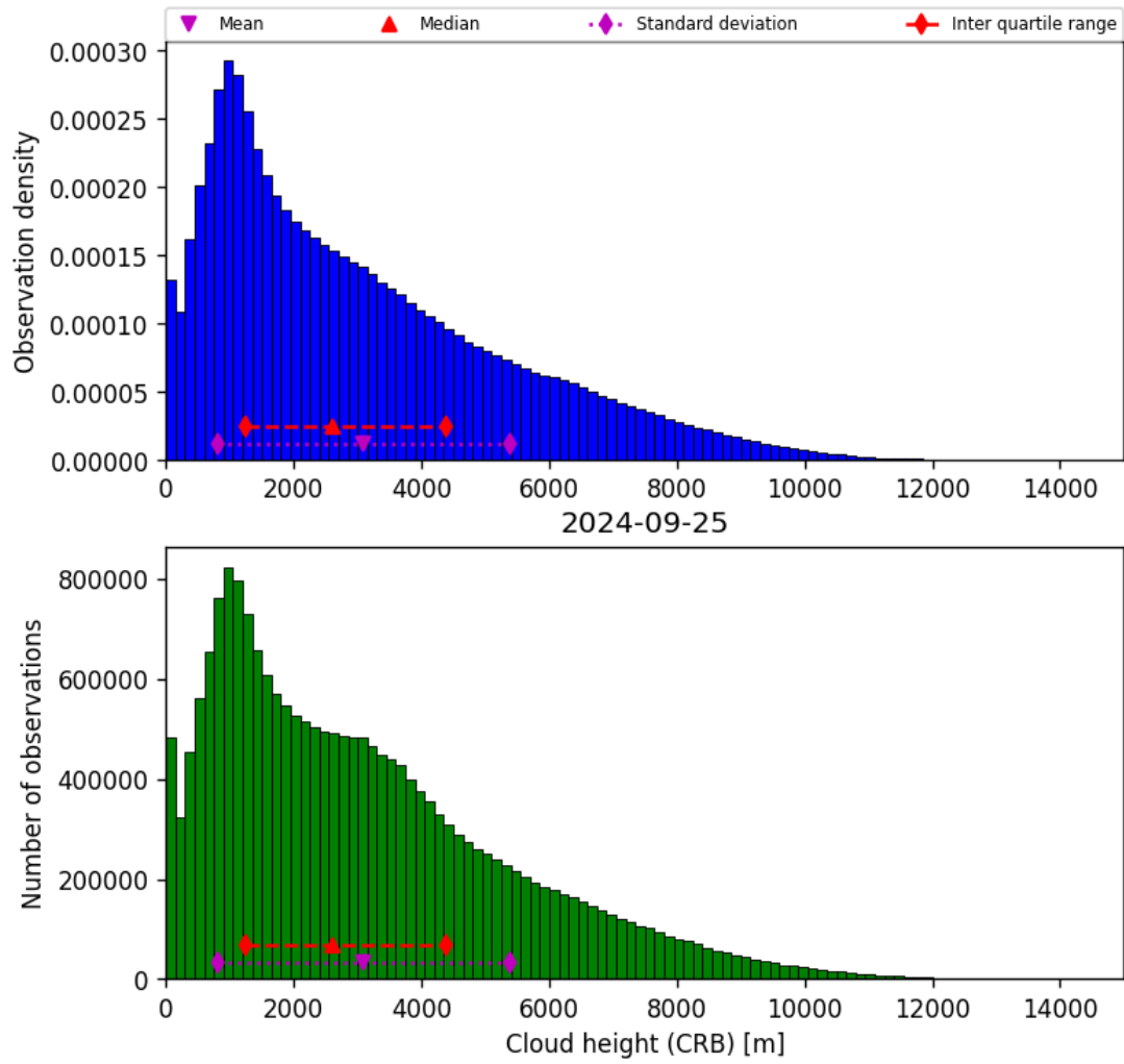
Figure 43: Histogram of “Cloud height (CRB)” for 2024-09-24 to 2024-09-26
