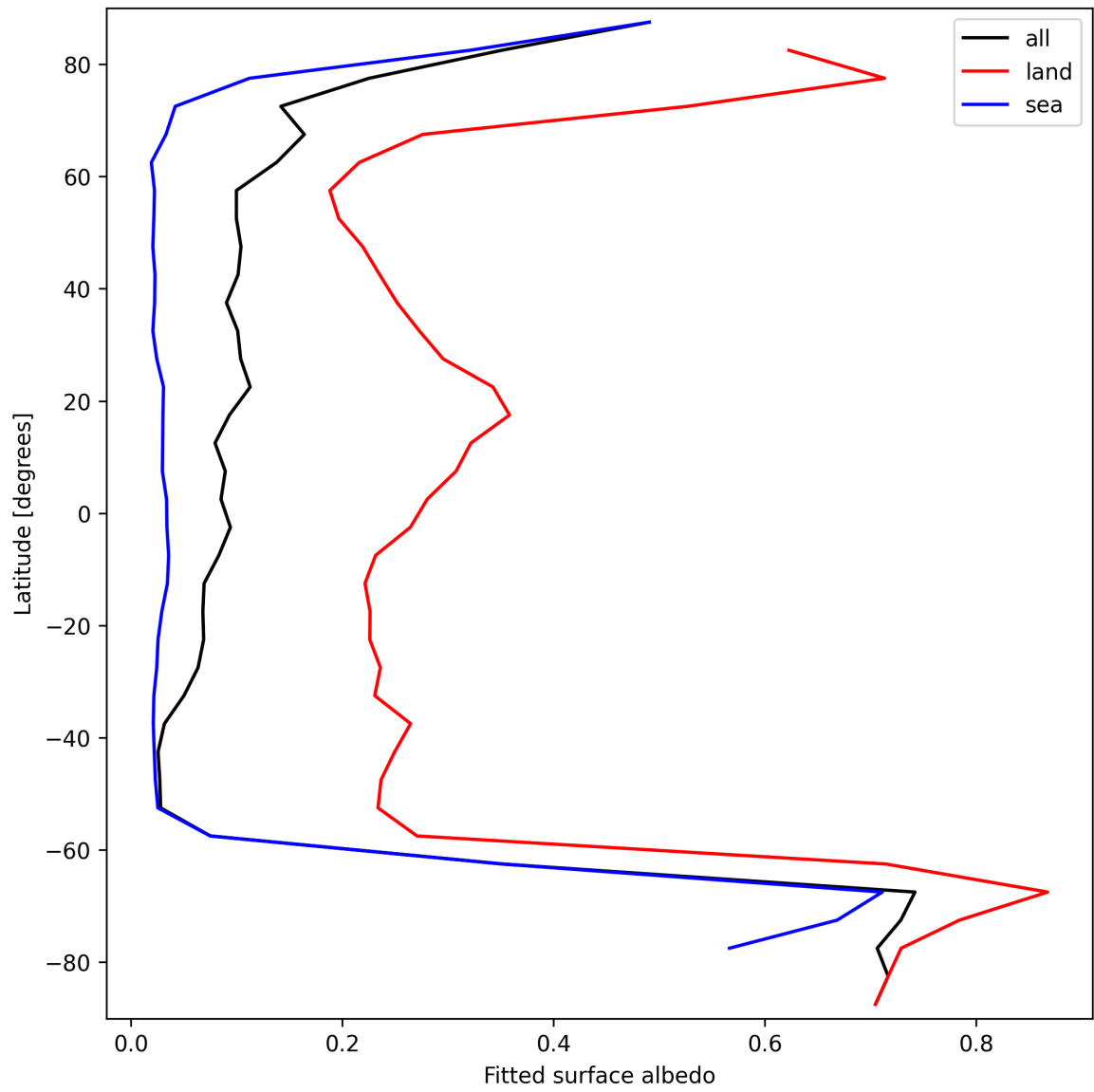
Figure 29: Zonal average of “Fitted surface albedo” for 2024-09-24 to 2024-09-26.
