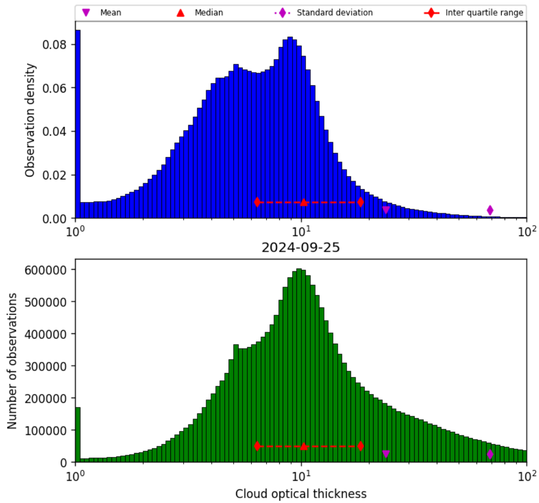
Figure 41: Histogram of “Cloud optical thickness” for 2024-09-24 to 2024-09-26
