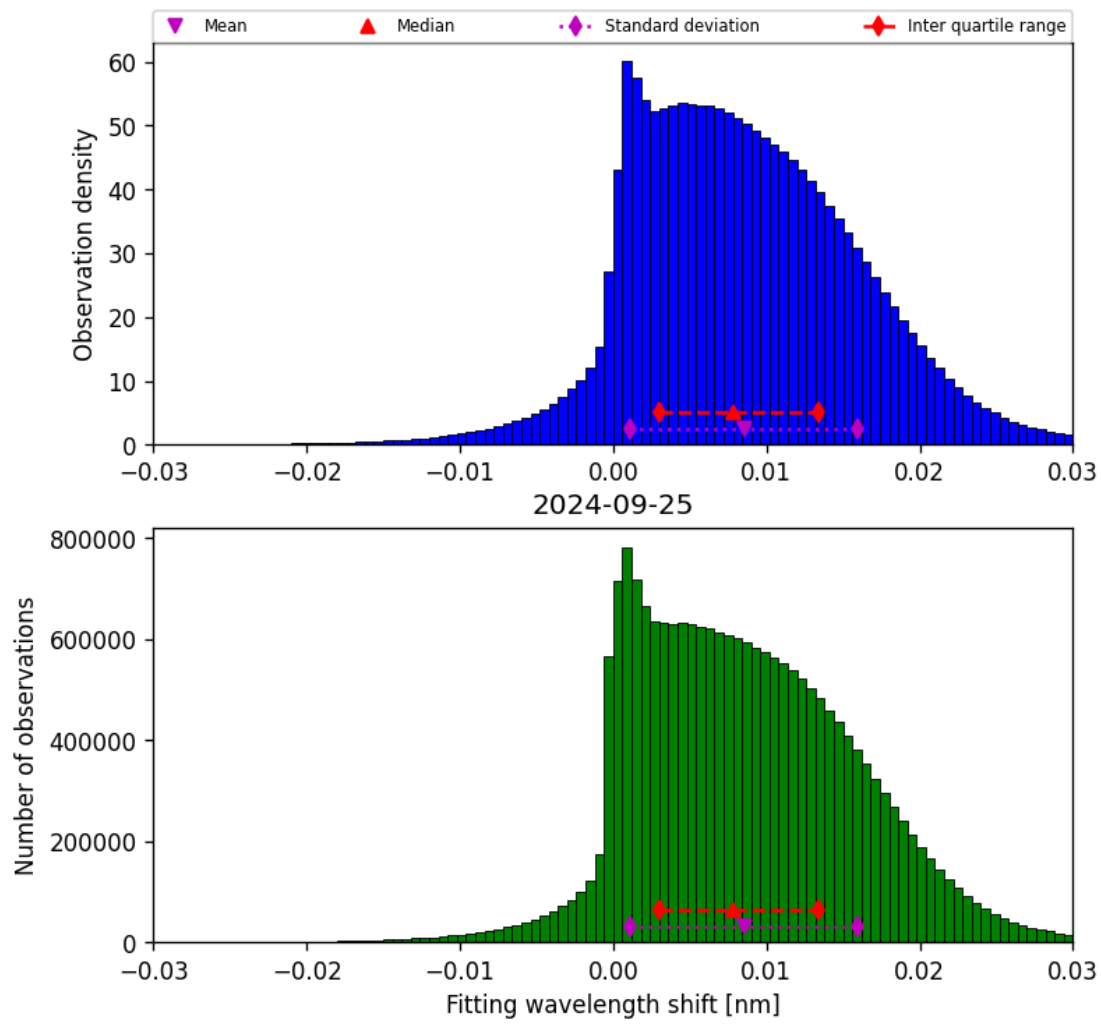
Figure 49: Histogram of “Fitting wavelength shift” for 2024-09-24 to 2024-09-26
