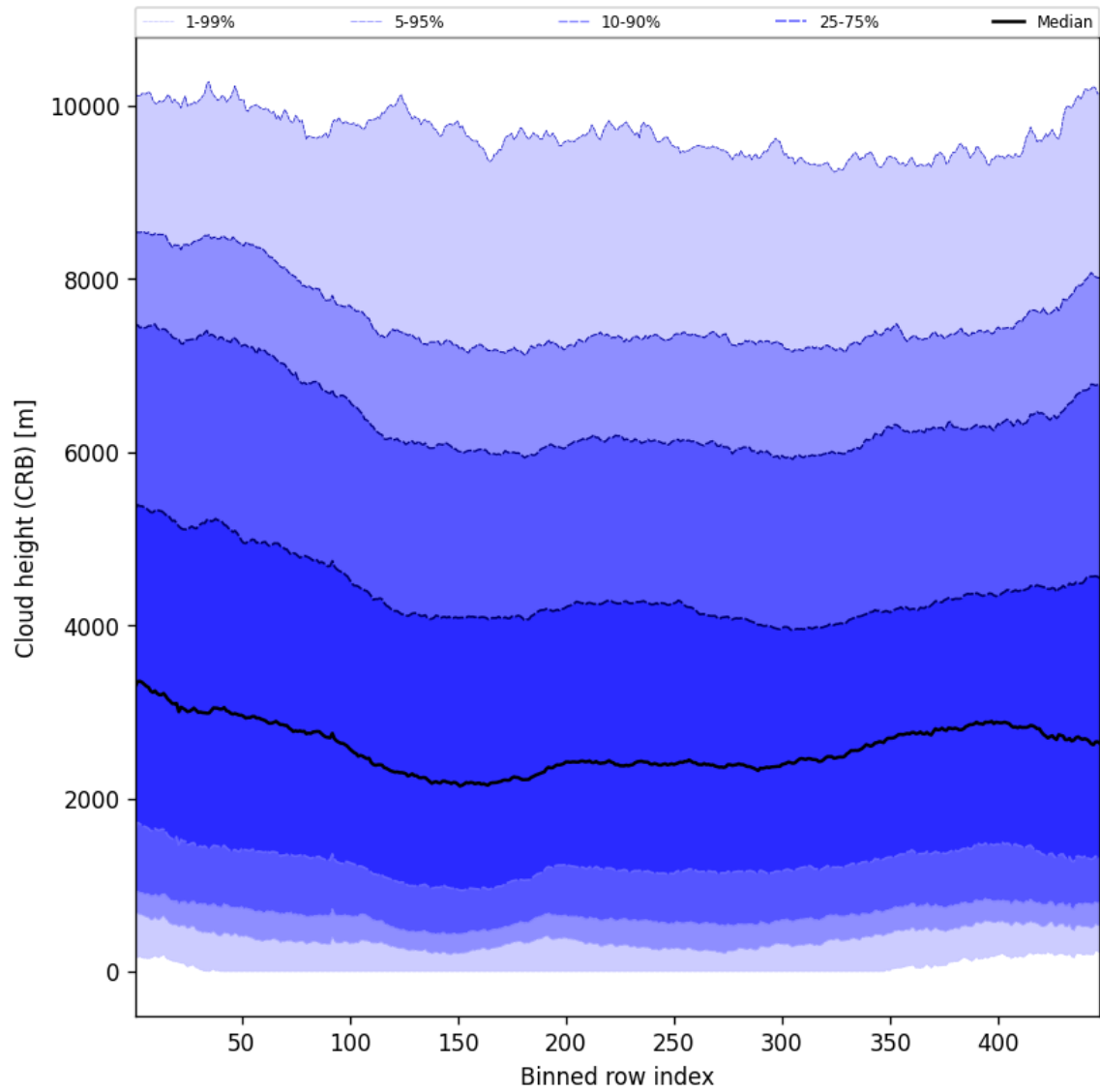
Figure 59: Along track statistics of “Cloud height (CRB)” for 2024-09-24 to 2024-09-26
