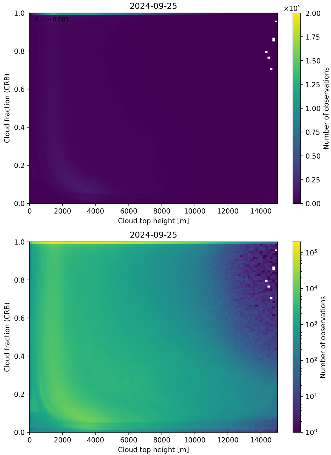
Figure 88: Scatter density plot of “Cloud top height” against “Cloud fraction (CRB)” for 2024-09-24 to 2024-09-26.
