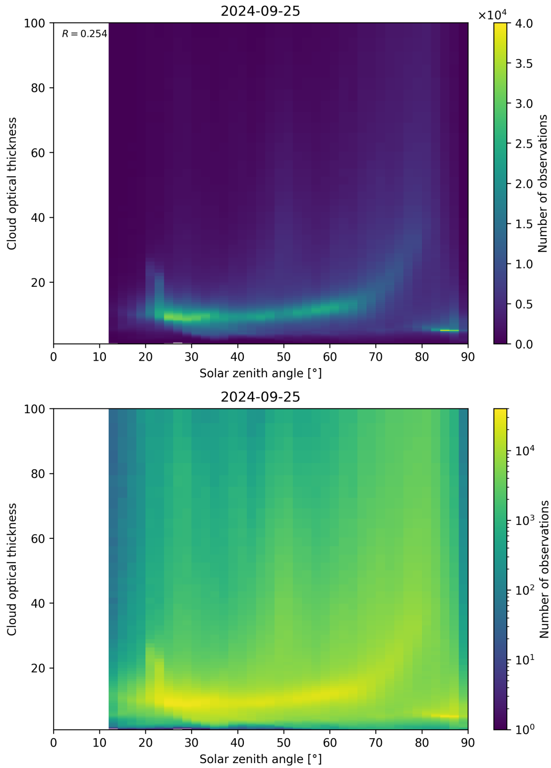
Figure 103: Scatter density plot of “Solar zenith angle” against “Cloud optical thickness” for 2024-09-24 to 2024-09-26.
