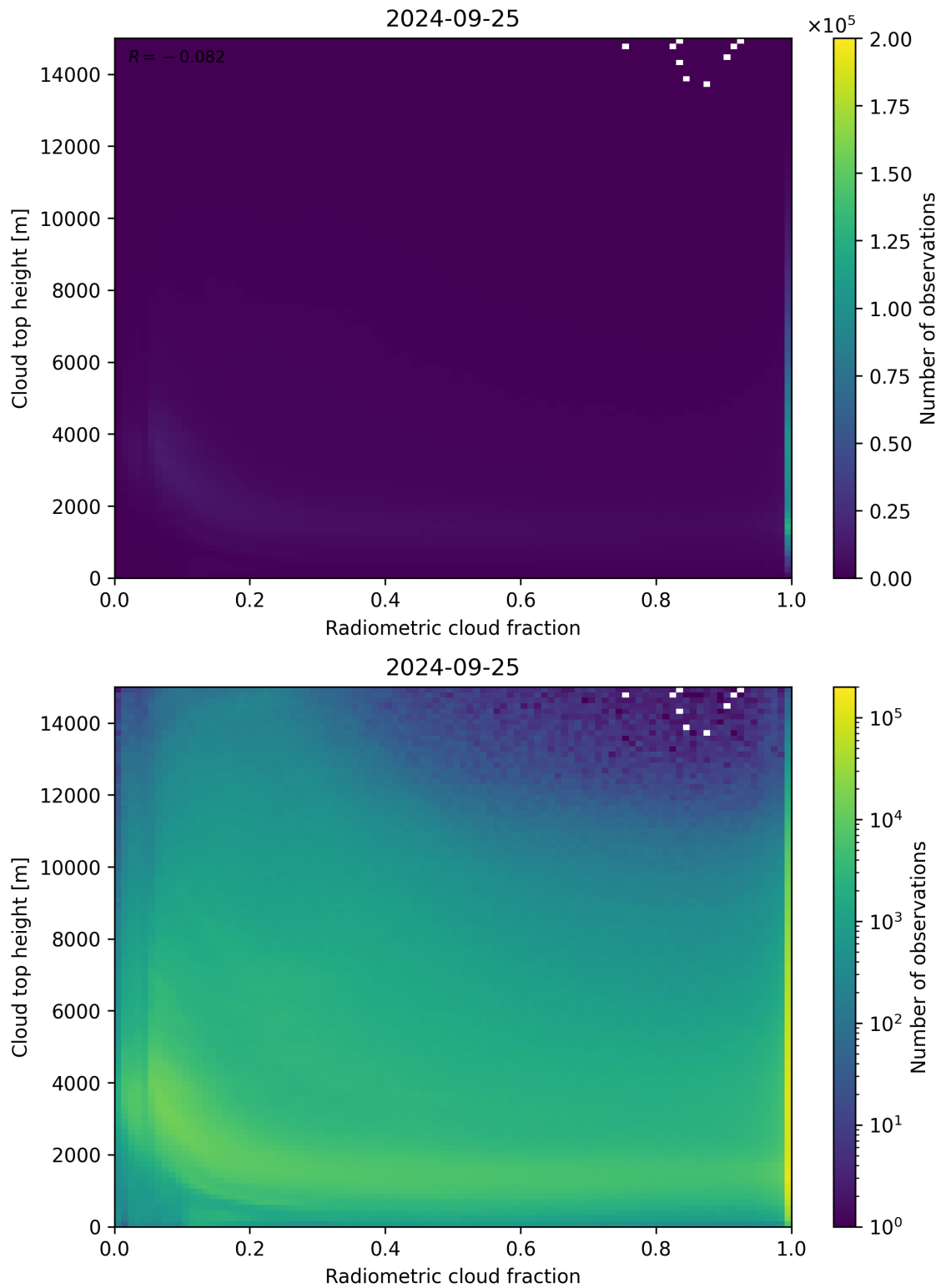
Figure 76: Scatter density plot of “Radiometric cloud fraction” against “Cloud top height” for 2024-09-24 to 2024-09-26.
