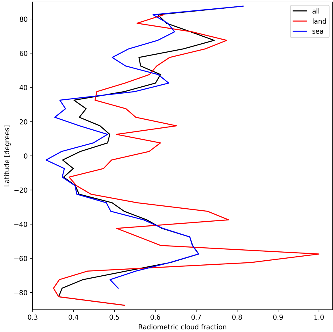
Figure 23: Zonal average of “Radiometric cloud fraction” for 2024-09-24 to 2024-09-26.
