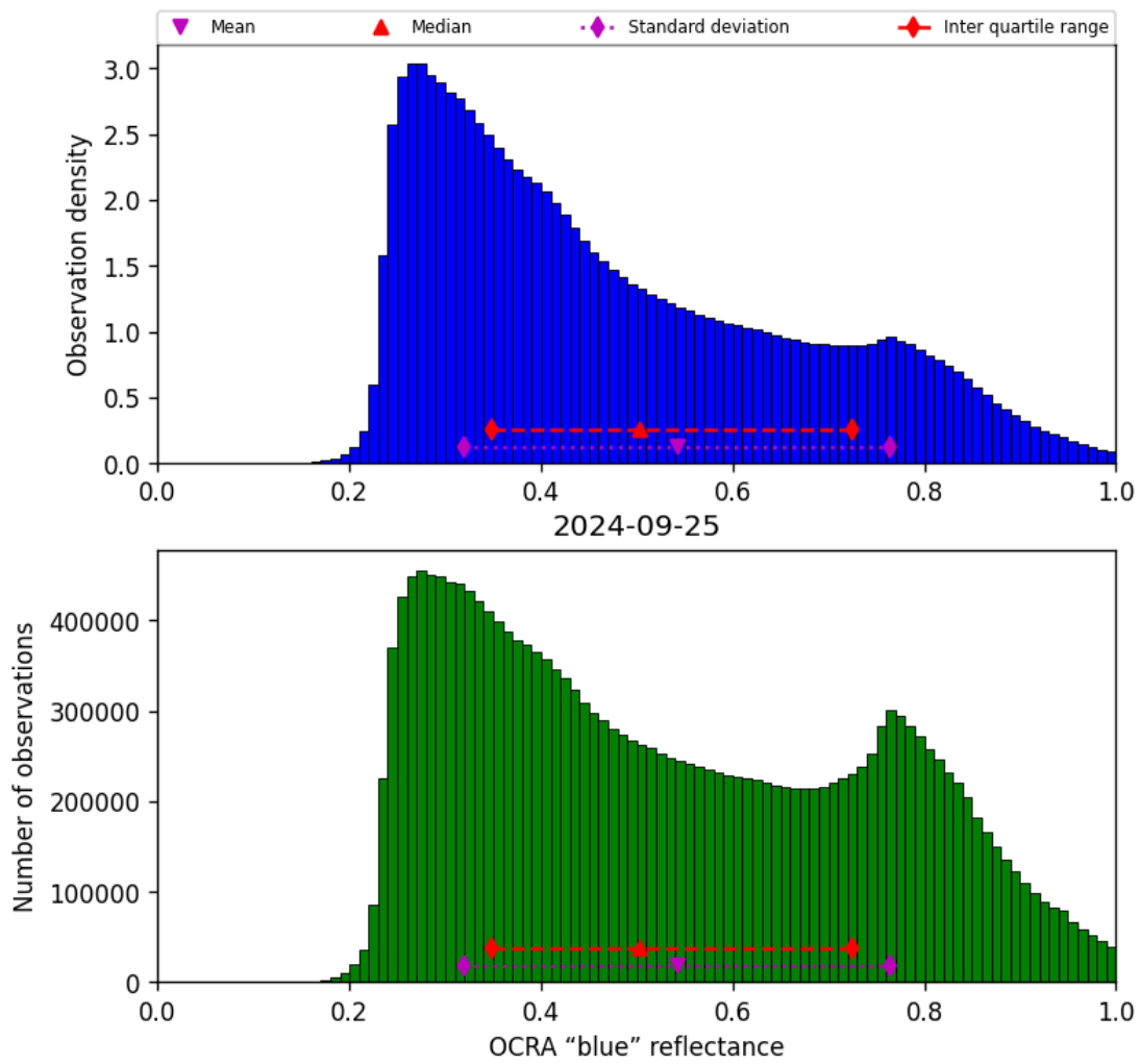
Figure 51: Histogram of “OCRA “blue” reflectance” for 2024-09-24 to 2024-09-26
