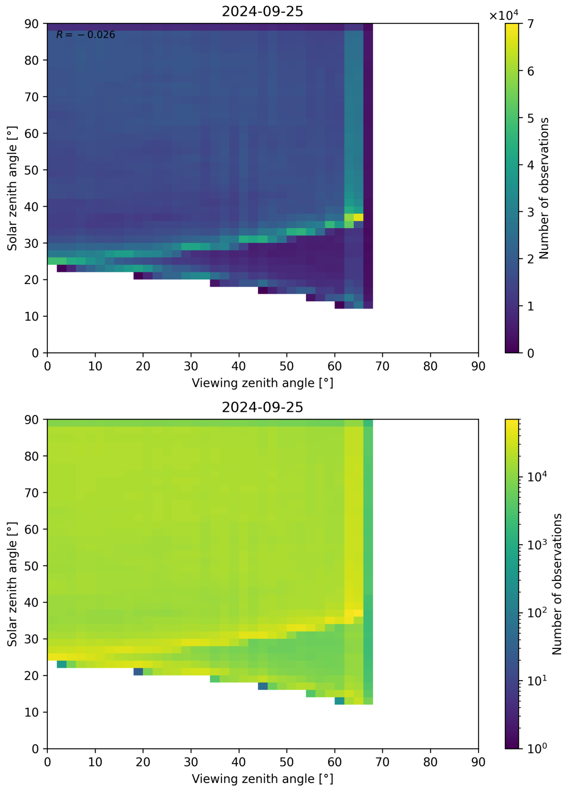
Figure 114: Scatter density plot of “Viewing zenith angle” against “Solar zenith angle” for 2024-09-24 to 2024-09-26.
