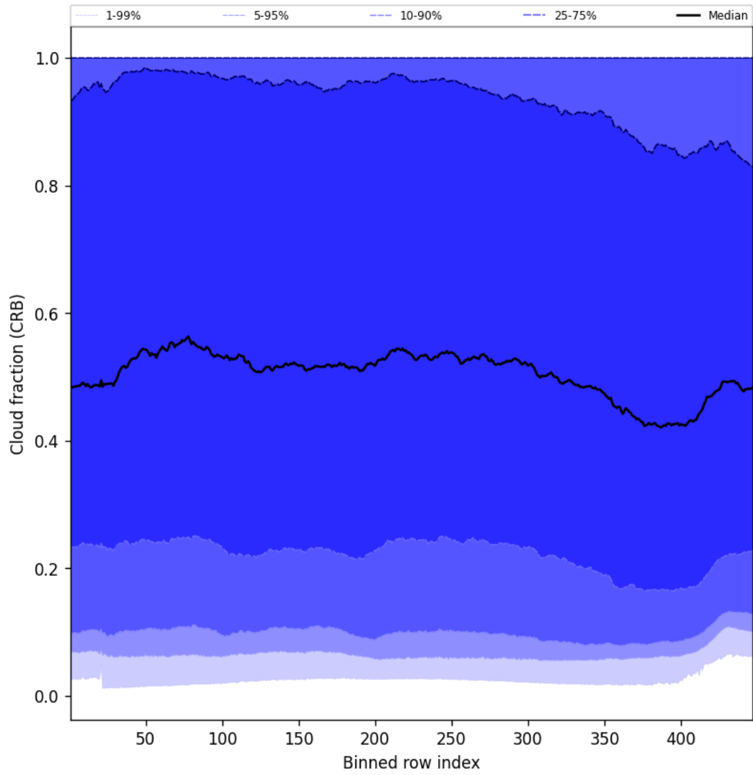
Figure 58: Along track statistics of “Cloud fraction (CRB)” for 2024-09-24 to 2024-09-26
