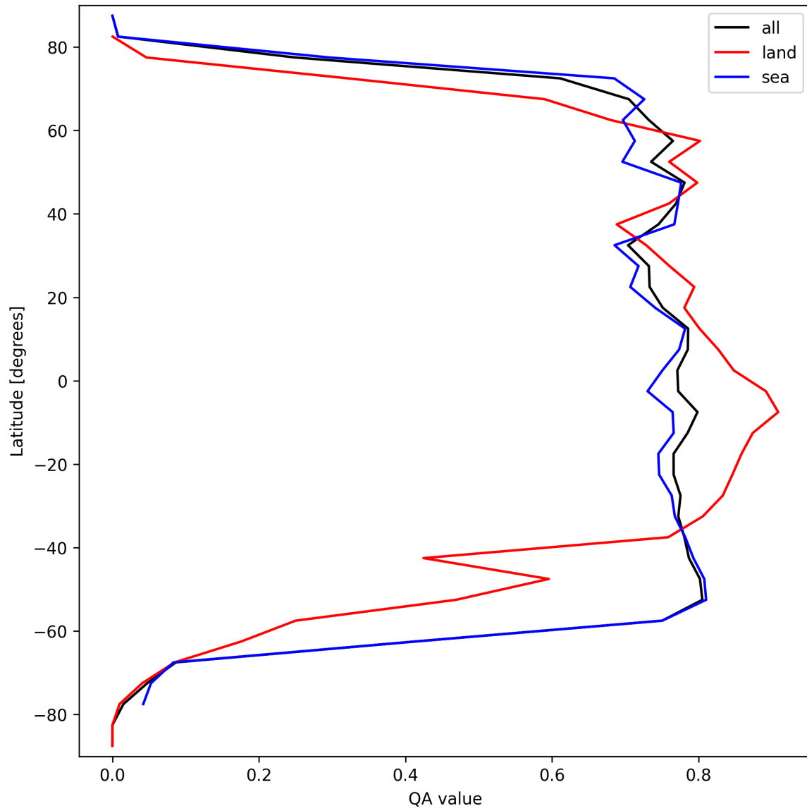
Figure 22: Zonal average of “QA value” for 2024-09-24 to 2024-09-26.
