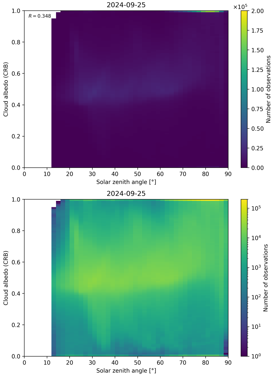
Figure 98: Scatter density plot of “Solar zenith angle” against “Cloud albedo (CRB)” for 2024-09-24 to 2024-09-26.
