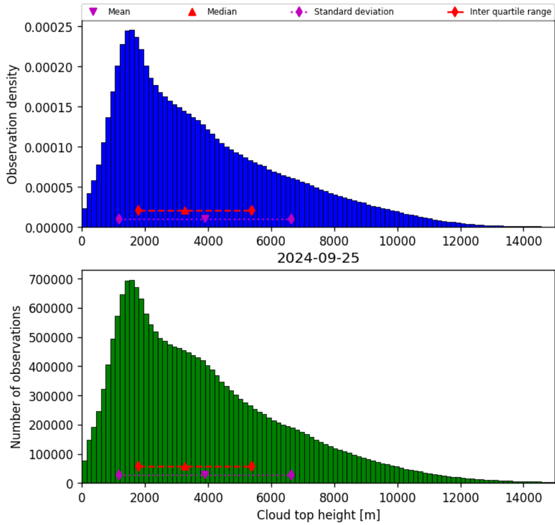
Figure 40: Histogram of “Cloud top height” for 2024-09-24 to 2024-09-26
