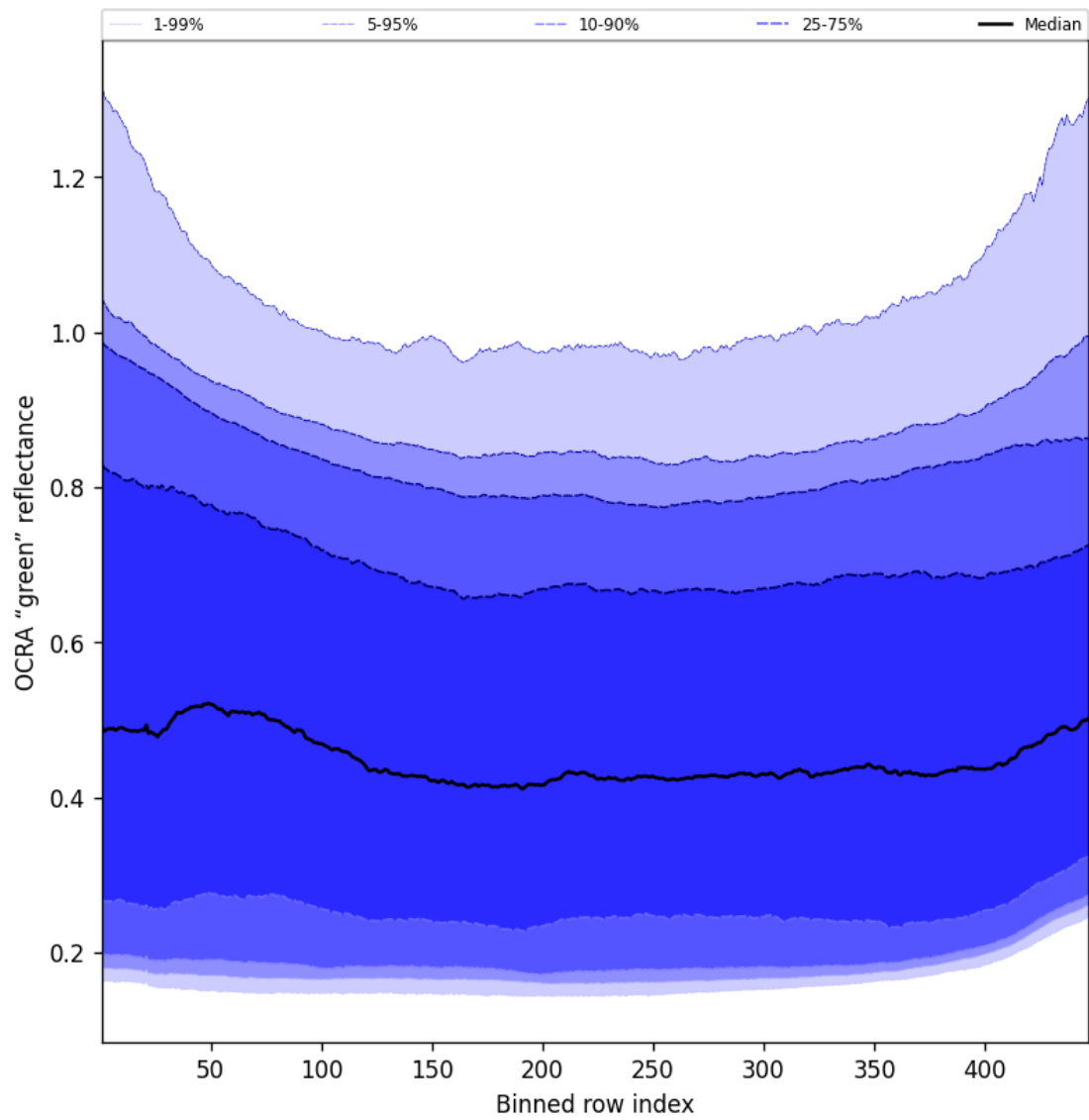
Figure 68: Along track statistics of "OCRA "green" reflectance" for 2024-09-24 to 2024-09-26
