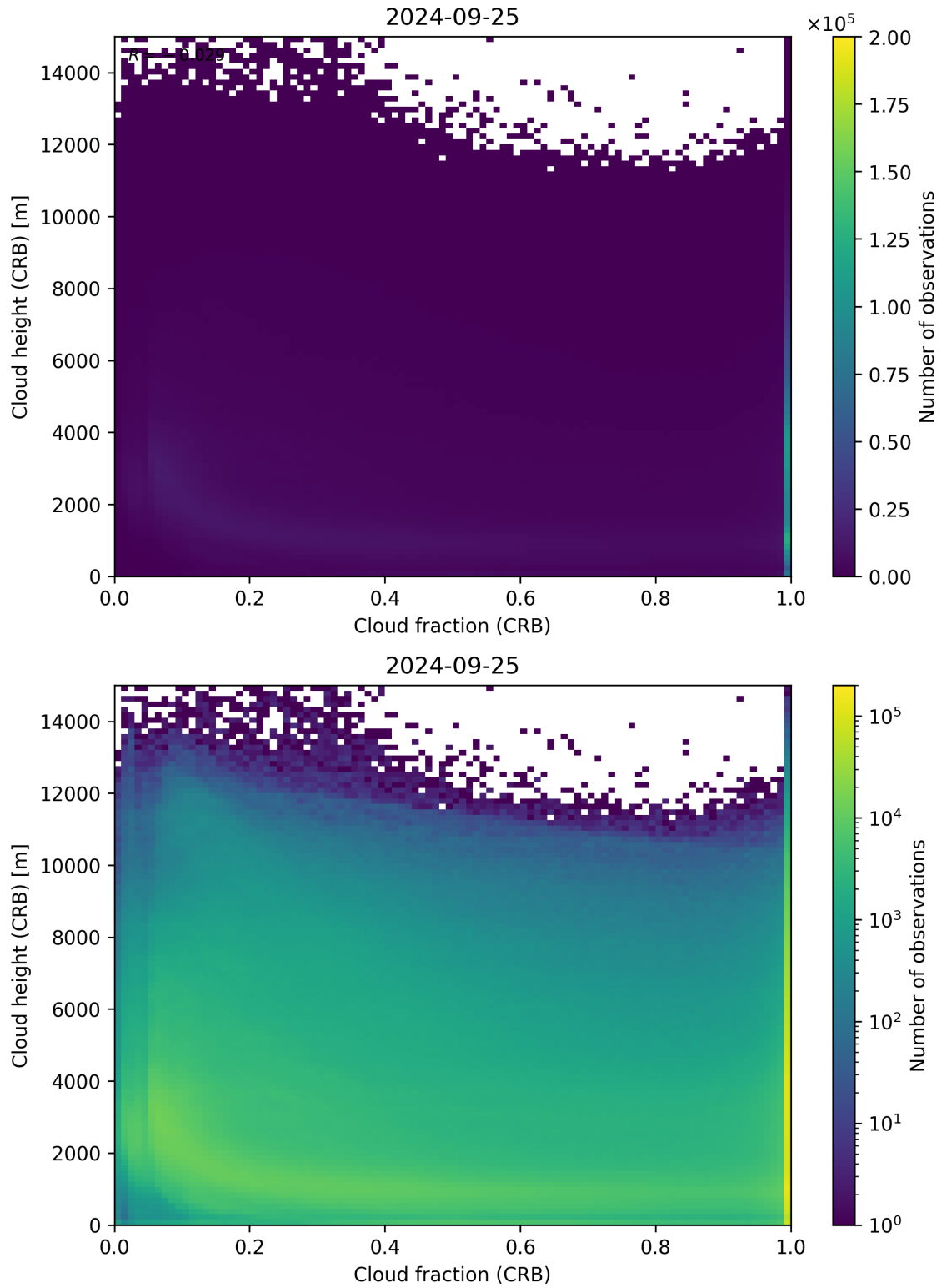
Figure 79: Scatter density plot of “Cloud fraction (CRB)” against “Cloud height (CRB)” for 2024-09-24 to 2024-09-26.
