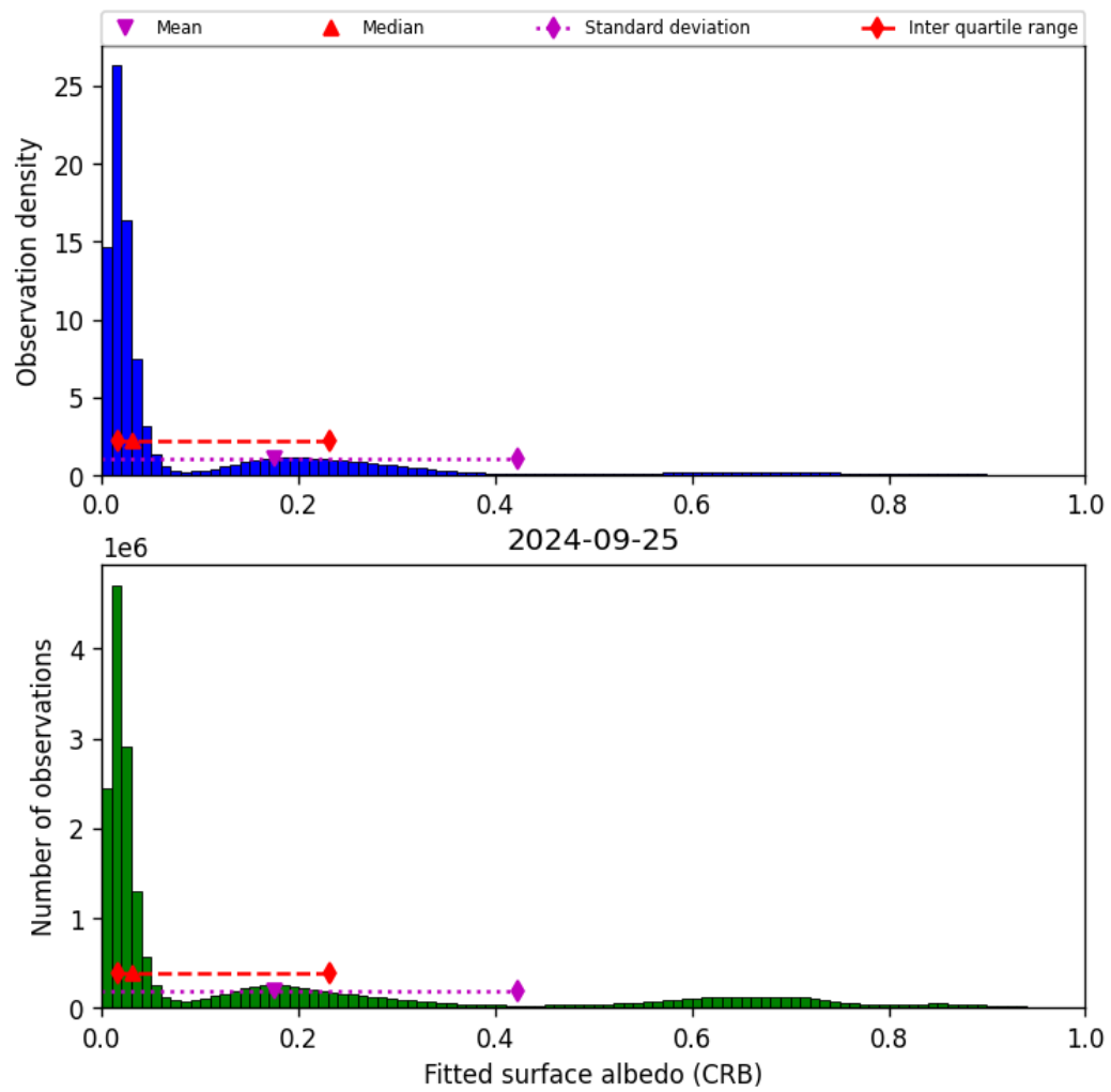
Figure 46: Histogram of “Fitted surface albedo (CRB)” for 2024-09-24 to 2024-09-26
