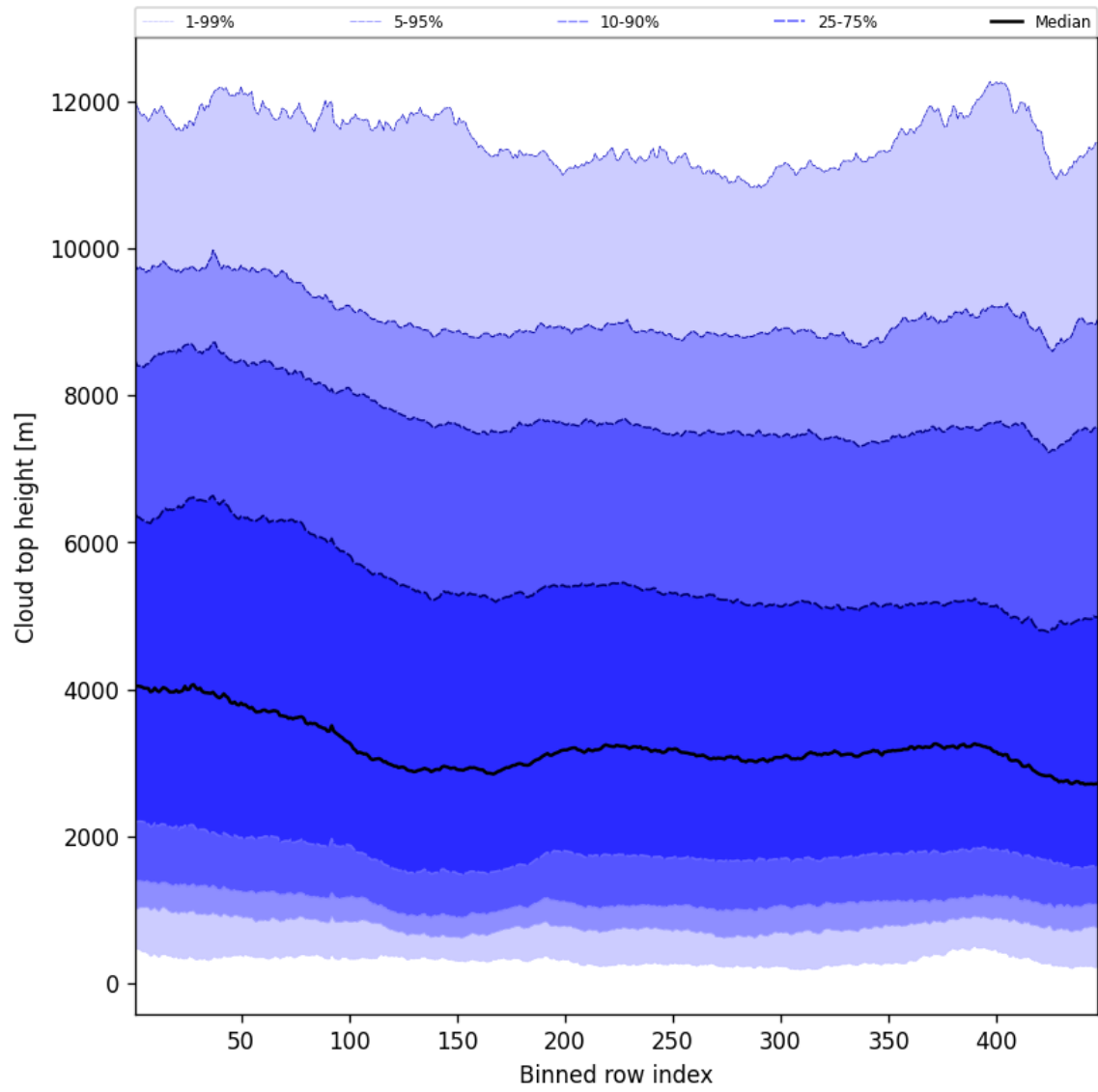
Figure 56: Along track statistics of “Cloud top height” for 2024-09-25 to 2024-09-27
