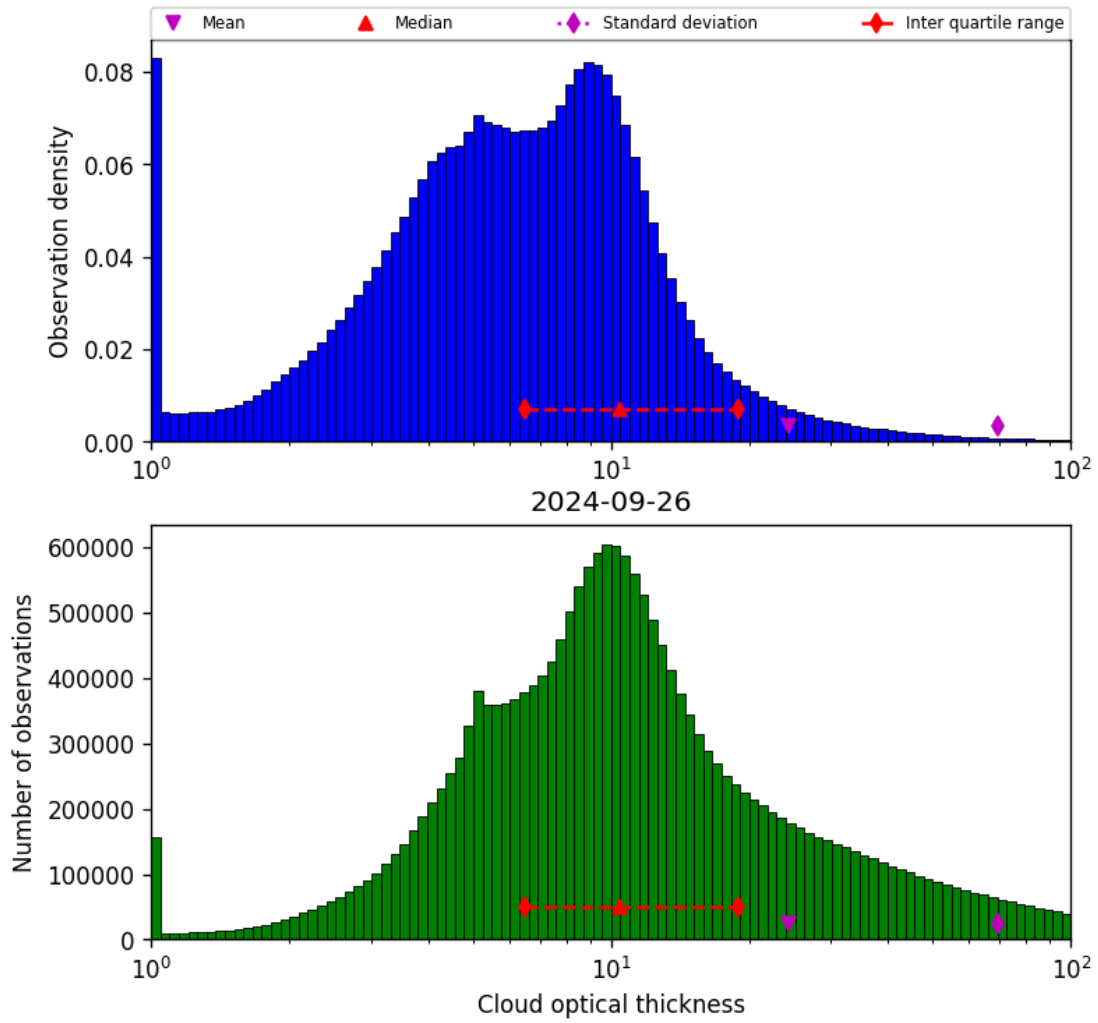
Figure 41: Histogram of “Cloud optical thickness” for 2024-09-25 to 2024-09-27
