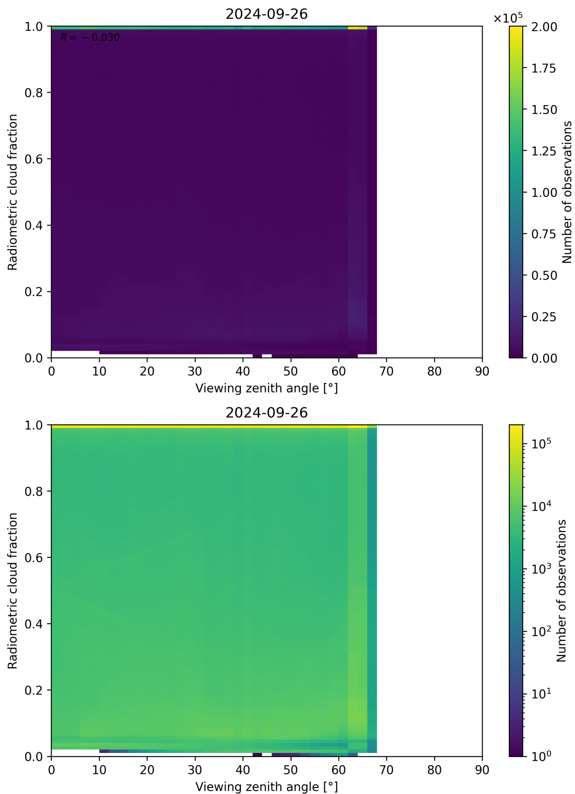
Figure 107: Scatter density plot of “Viewing zenith angle” against “Radiometric cloud fraction” for 2024-09-25 to 2024-09-27.
