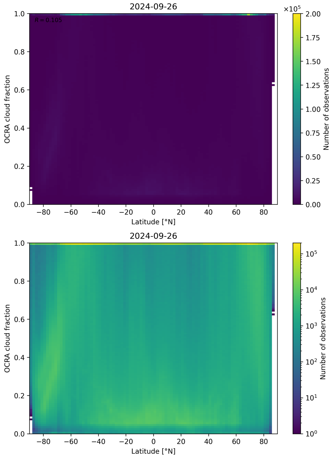
Figure 93: Scatter density plot of “Latitude” against “OCRA cloud fraction” for 2024-09-25 to 2024-09-27.
