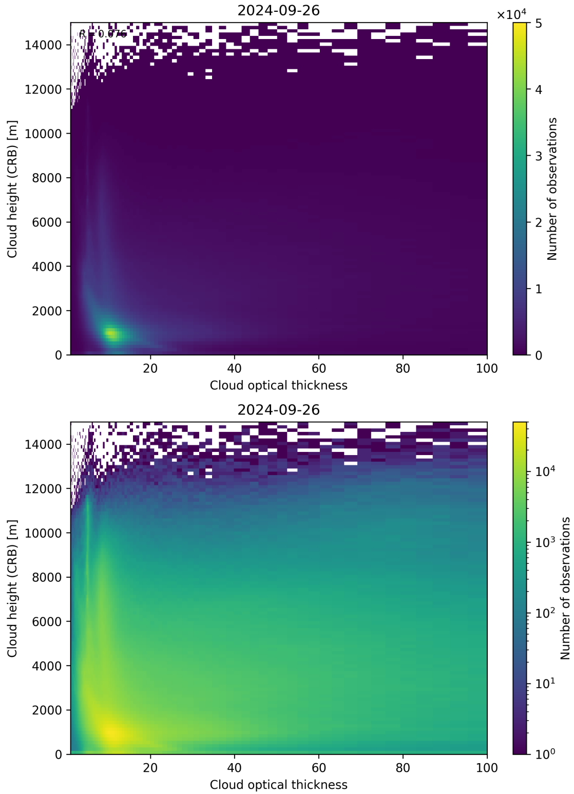
Figure 85: Scatter density plot of “Cloud optical thickness” against “Cloud height (CRB)” for 2024-09-25 to 2024-09-27.
