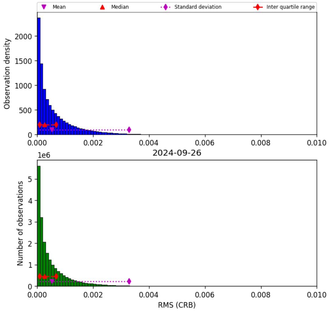
Figure 48: Histogram of “RMS (CRB)” for 2024-09-25 to 2024-09-27
