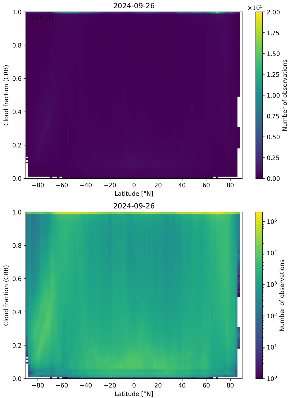
Figure 94: Scatter density plot of “Latitude” against “Cloud fraction (CRB)” for 2024-09-25 to 2024-09-27.
