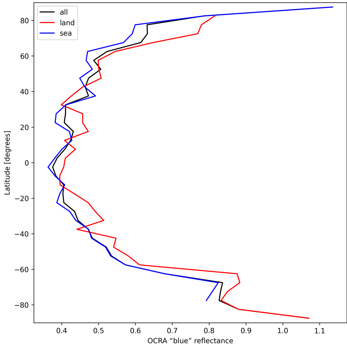
Figure 35: Zonal average of “OCRA “blue” reflectance” for 2024-09-25 to 2024-09-27.
