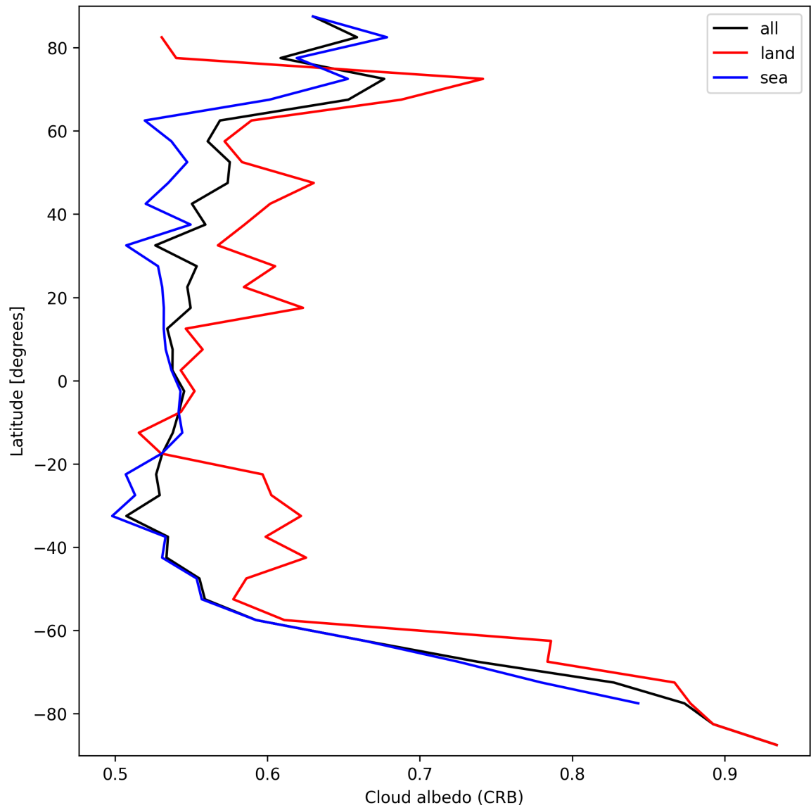
Figure 28: Zonal average of “Cloud albedo (CRB)” for 2024-09-25 to 2024-09-27.
