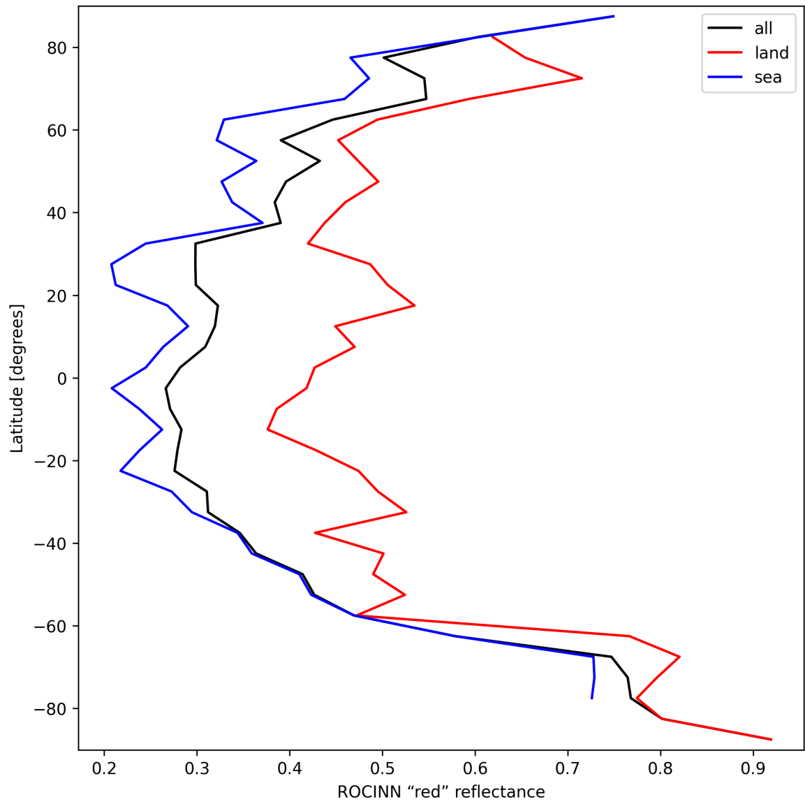
Figure 37: Zonal average of “ROCINN “red” reflectance” for 2024-09-25 to 2024-09-27.
