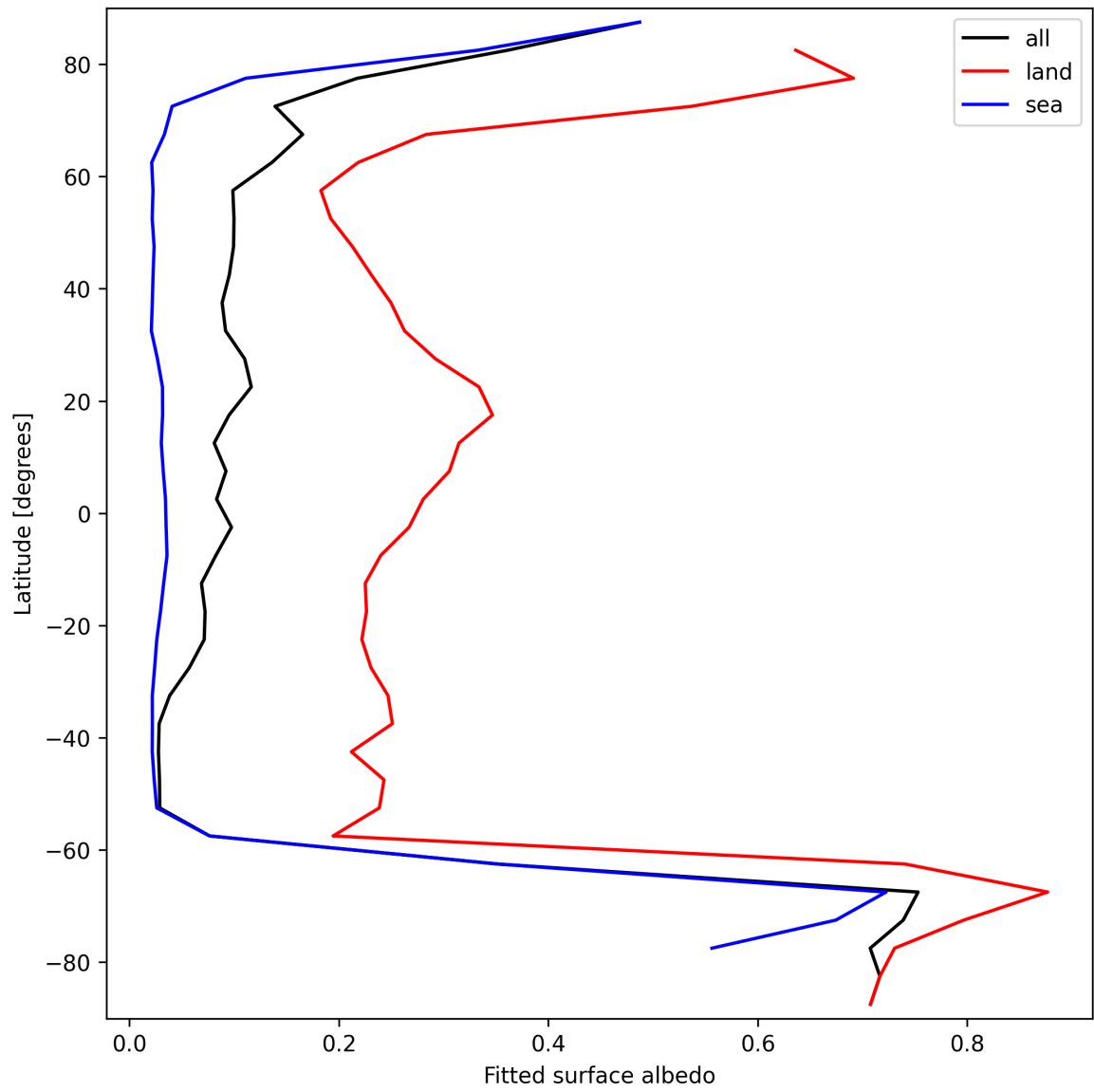
Figure 29: Zonal average of “Fitted surface albedo” for 2024-09-25 to 2024-09-27.
