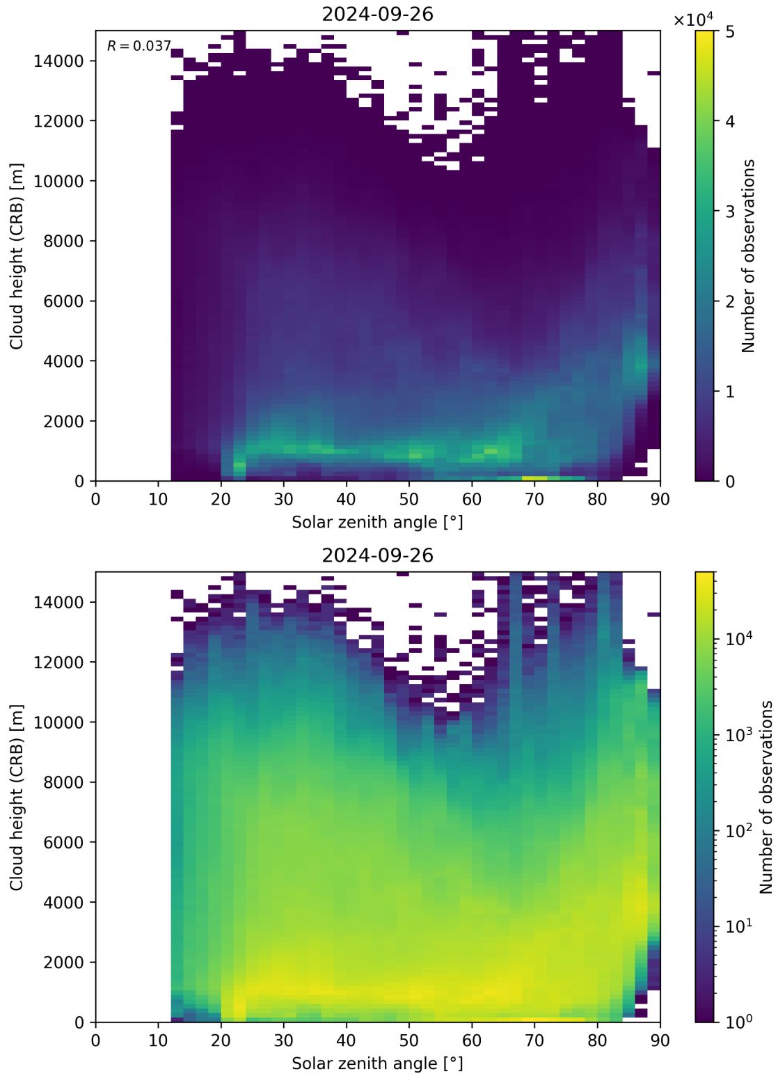
Figure 102: Scatter density plot of “Solar zenith angle” against “Cloud height (CRB)” for 2024-09-25 to 2024-09-27.
