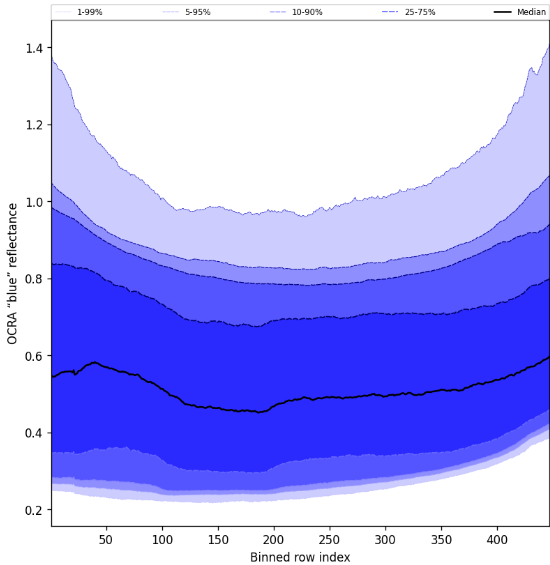
Figure 67: Along track statistics of “OCRA “blue” reflectance” for 2024-09-25 to 2024-09-27
