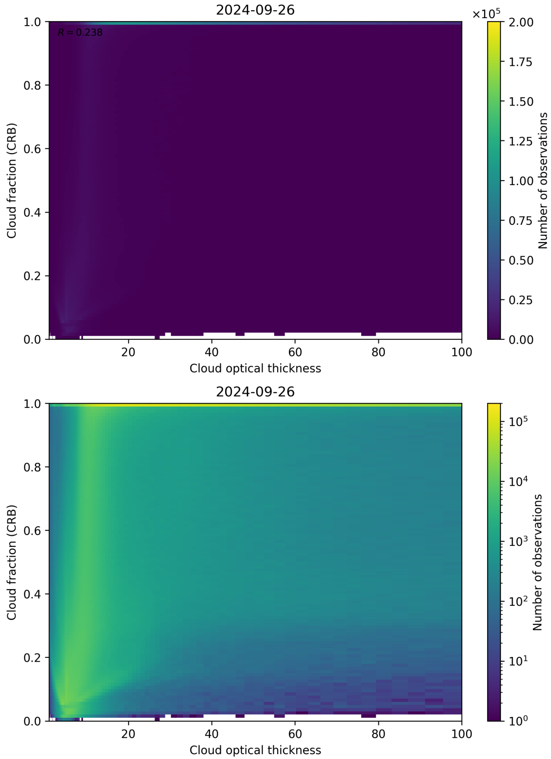
Figure 84: Scatter density plot of “Cloud optical thickness” against “Cloud fraction (CRB)” for 2024-09-25 to 2024-09-27.
