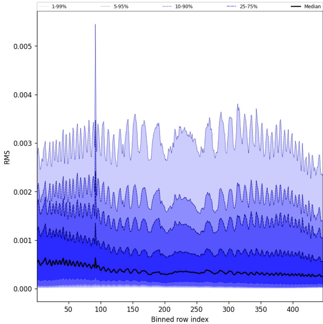
Figure 63: Along track statistics of “RMS” for 2024-09-25 to 2024-09-27
