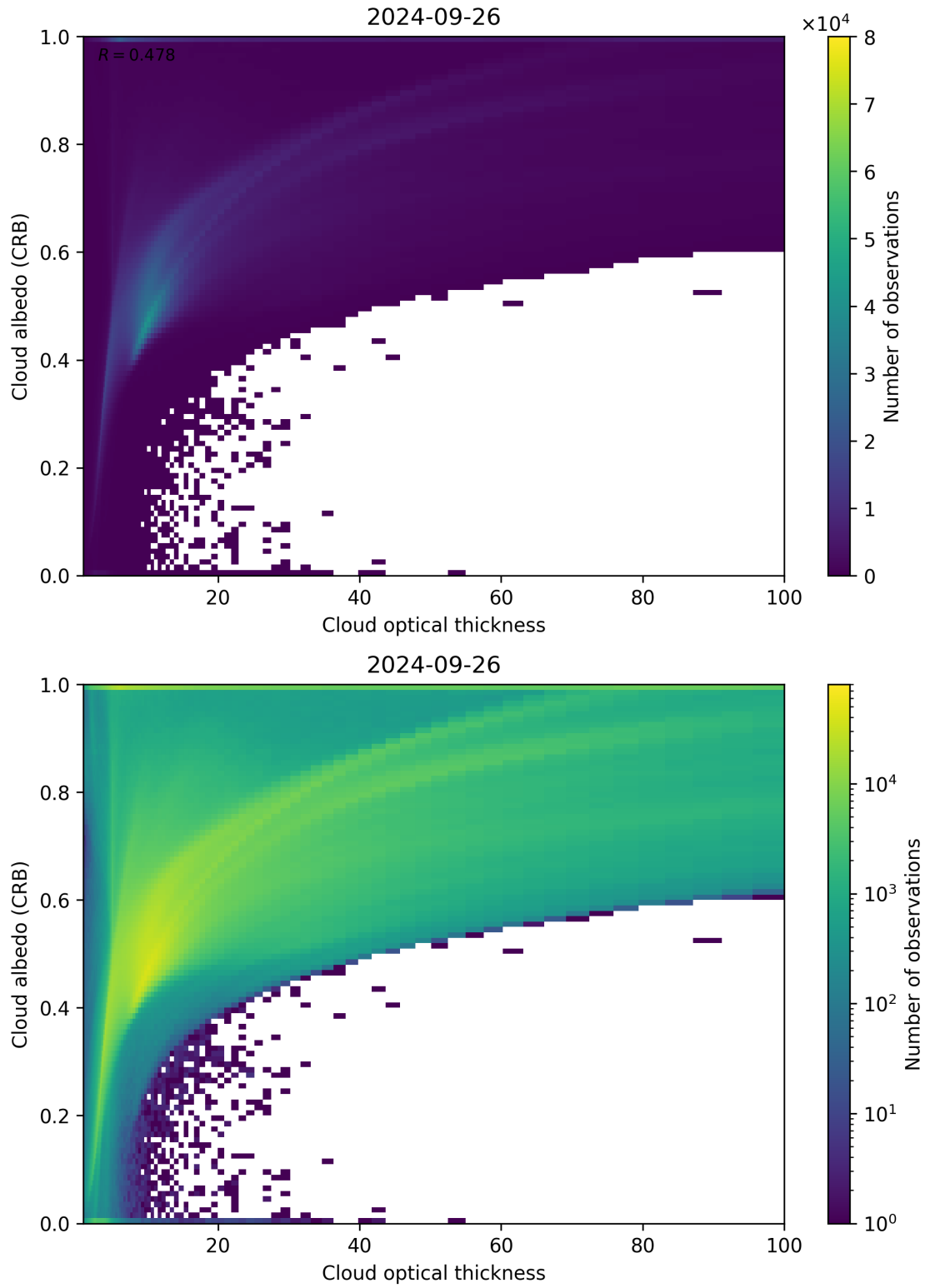
Figure 82: Scatter density plot of “Cloud optical thickness” against “Cloud albedo (CRB)” for 2024-09-25 to 2024-09-27.
