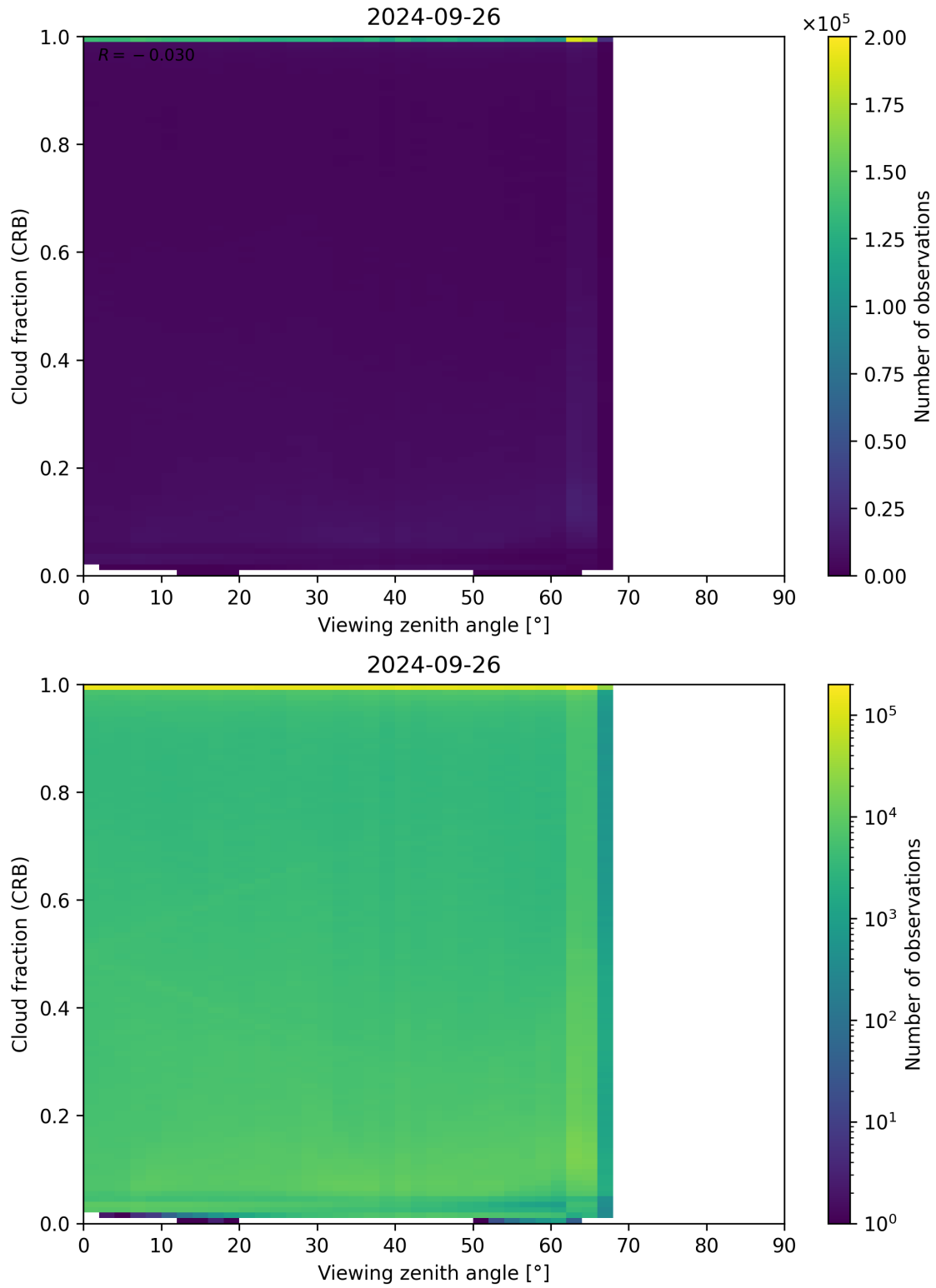
Figure 109: Scatter density plot of “Viewing zenith angle” against “Cloud fraction (CRB)” for 2024-09-25 to 2024-09-27.
