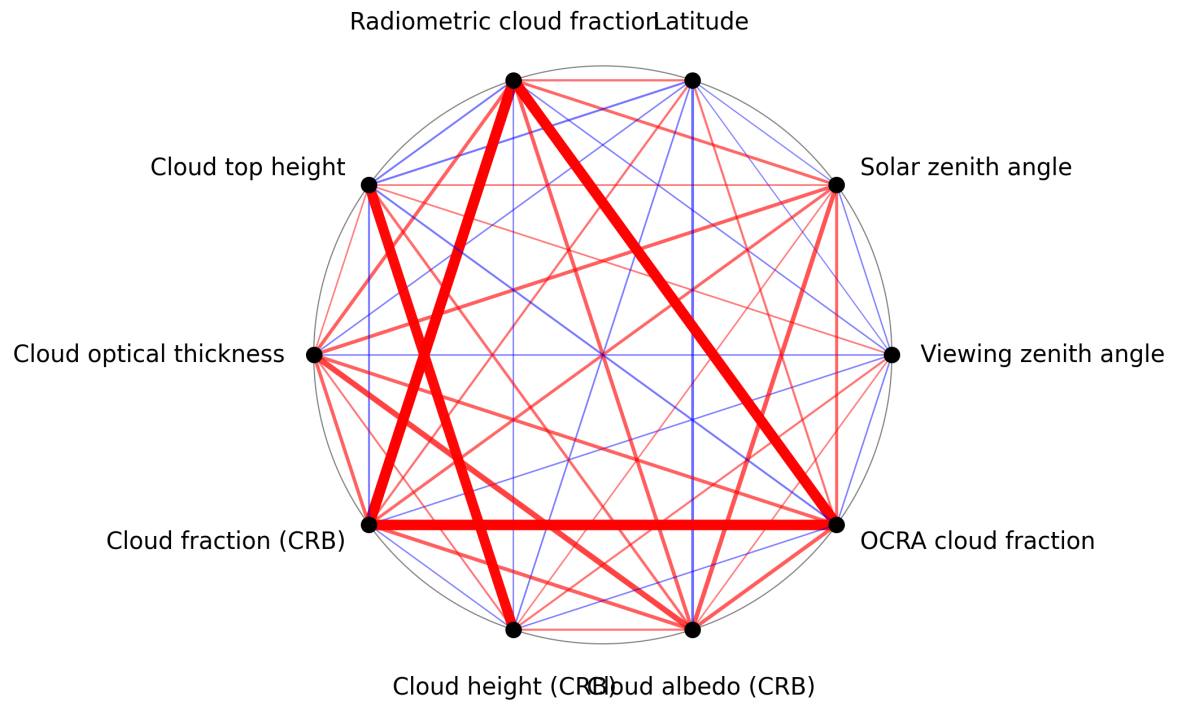
Figure 1: Map of correlation graph for 2024-09-25 to 2024-09-27.
