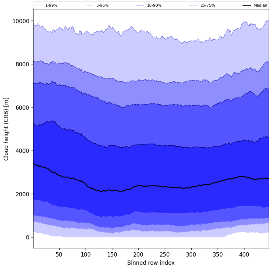
Figure 59: Along track statistics of “Cloud height (CRB)” for 2024-09-25 to 2024-09-27
