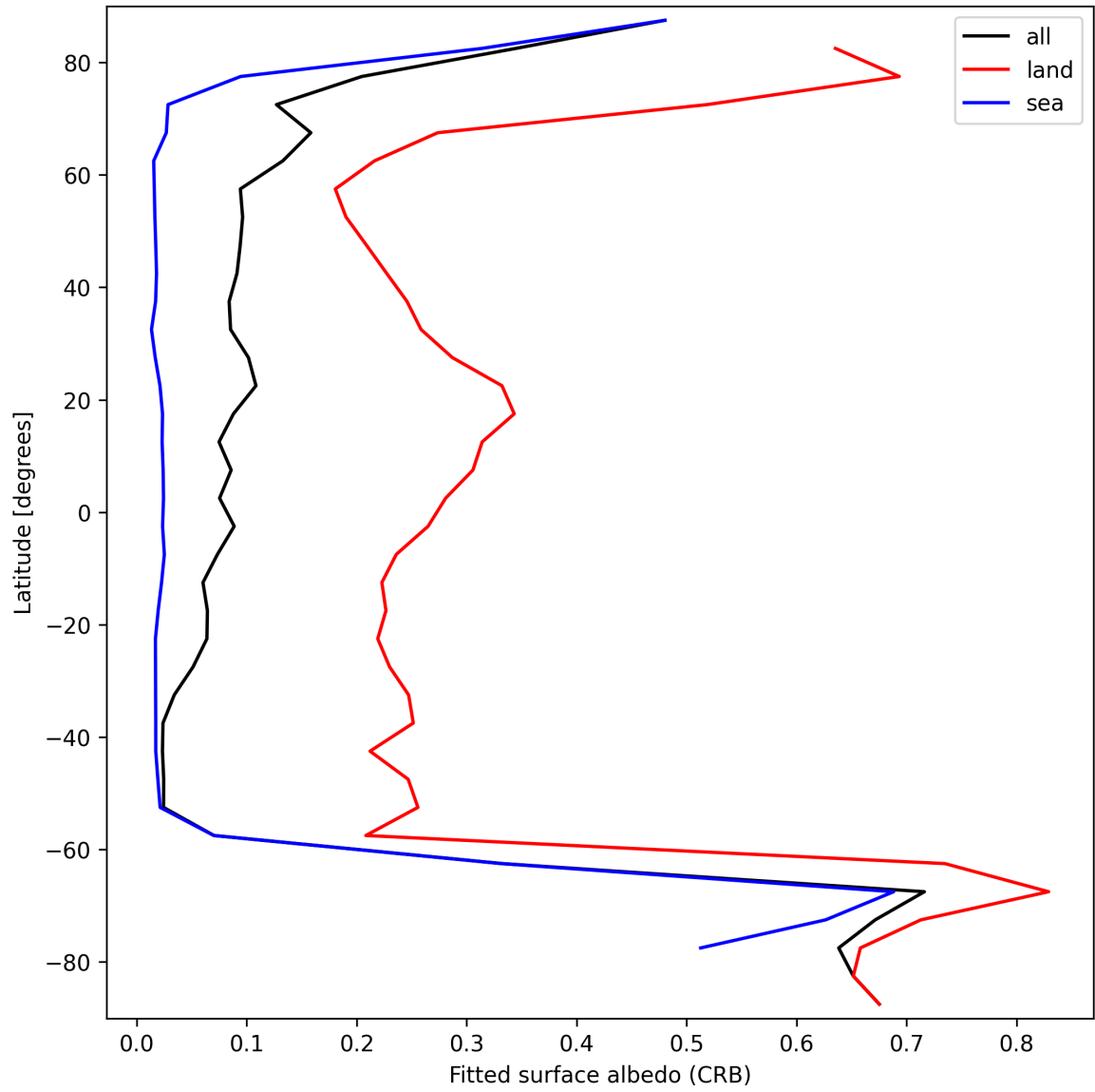
Figure 30: Zonal average of “Fitted surface albedo (CRB)” for 2024-09-25 to 2024-09-27.
