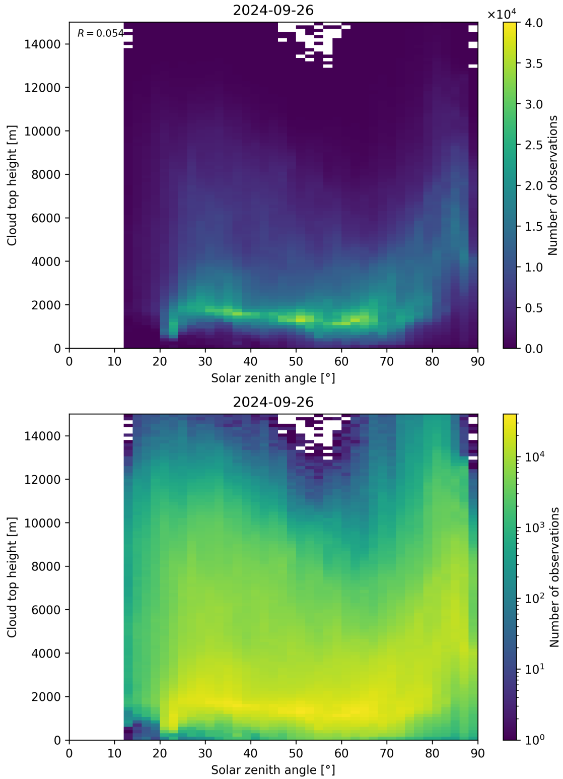
Figure 104: Scatter density plot of “Solar zenith angle” against “Cloud top height” for 2024-09-25 to 2024-09-27.
