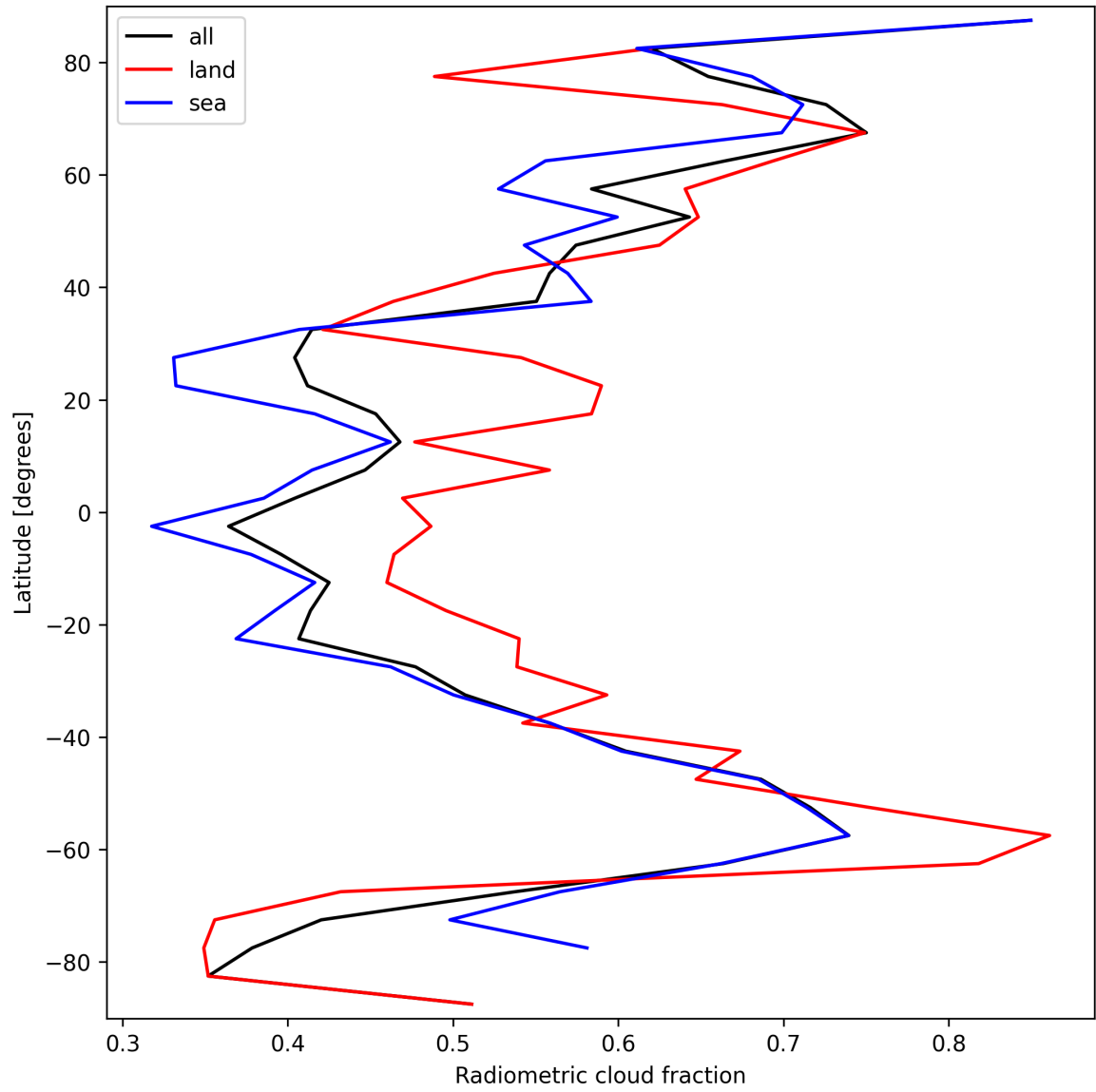
Figure 23: Zonal average of “Radiometric cloud fraction” for 2024-09-25 to 2024-09-27.
