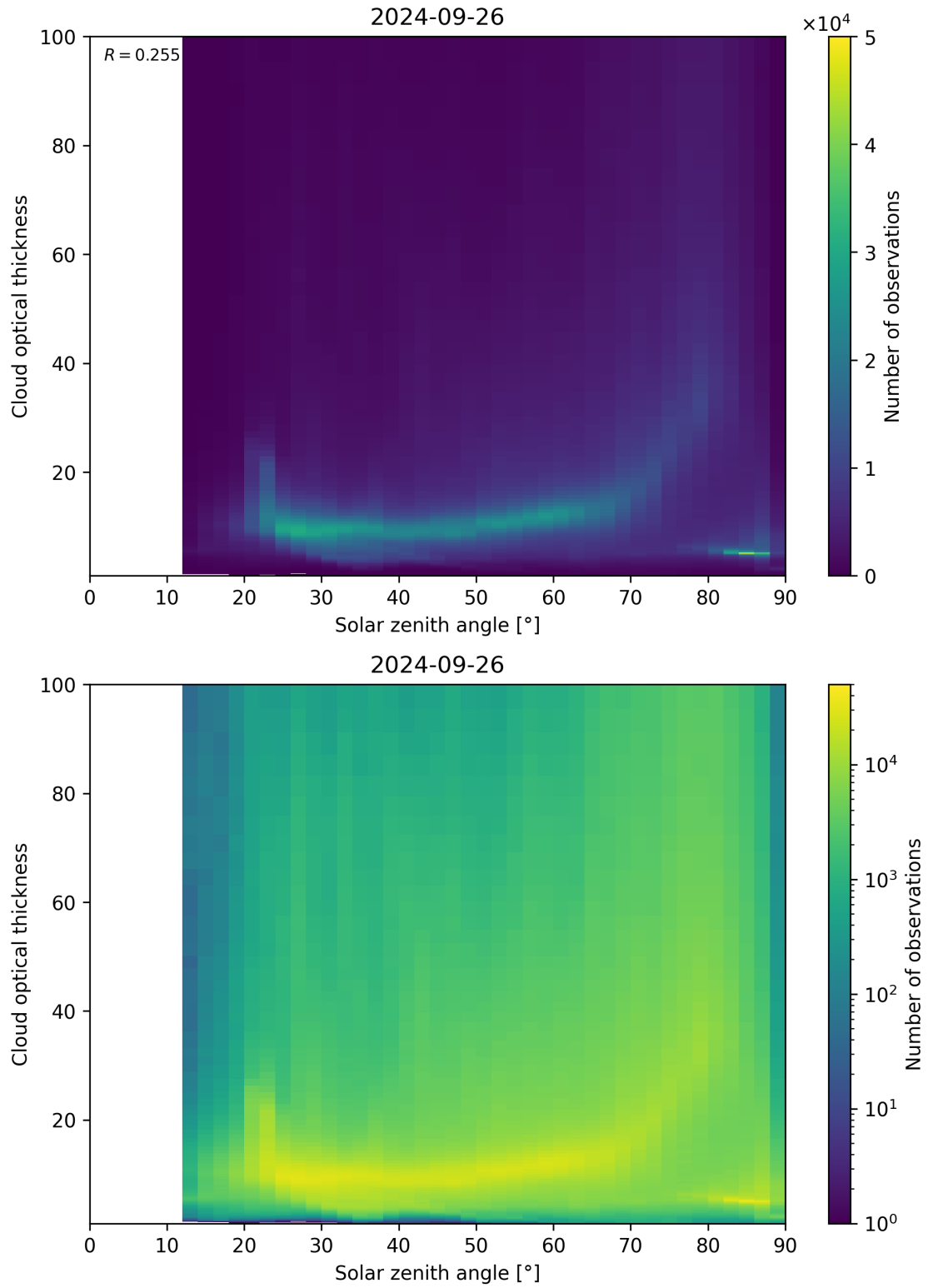
Figure 103: Scatter density plot of “Solar zenith angle” against “Cloud optical thickness” for 2024-09-25 to 2024-09-27.
