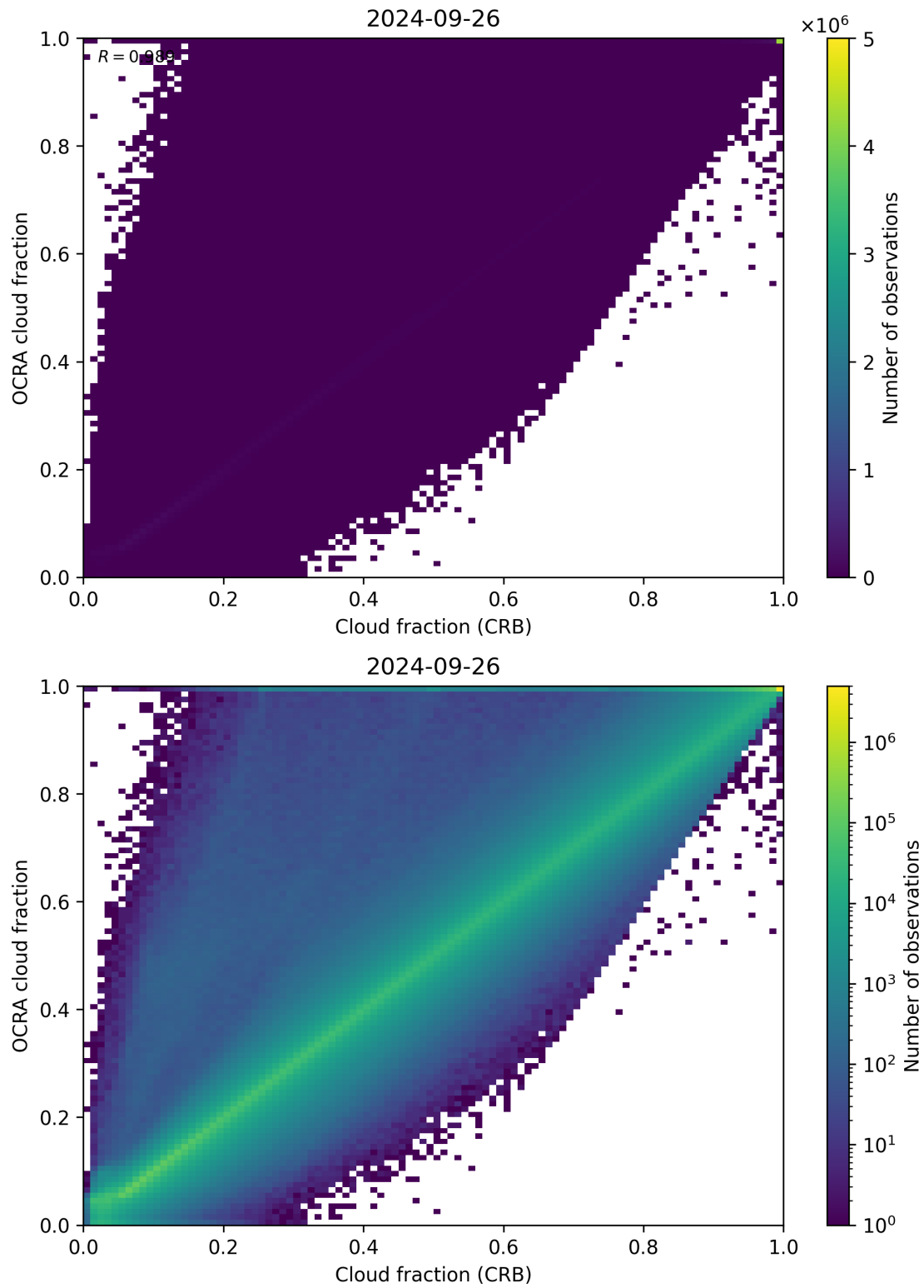
Figure 78: Scatter density plot of “Cloud fraction (CRB)” against “OCRA cloud fraction” for 2024-09-25 to 2024-09-27.
