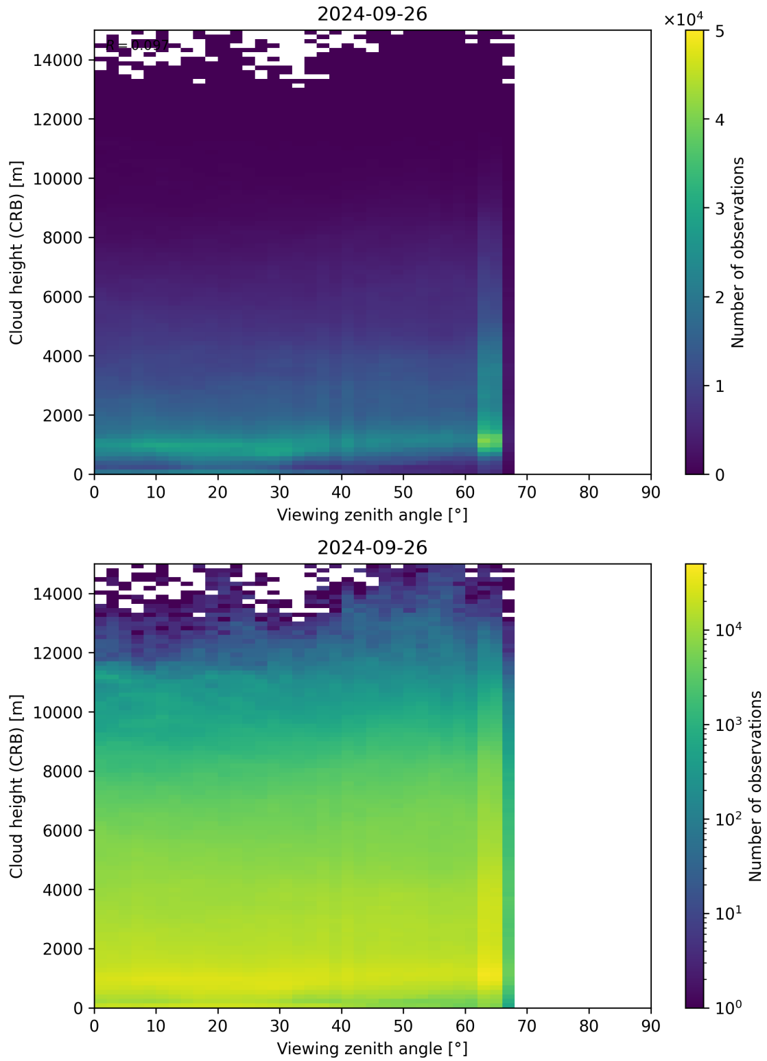
Figure 110: Scatter density plot of “Viewing zenith angle” against “Cloud height (CRB)” for 2024-09-25 to 2024-09-27.
