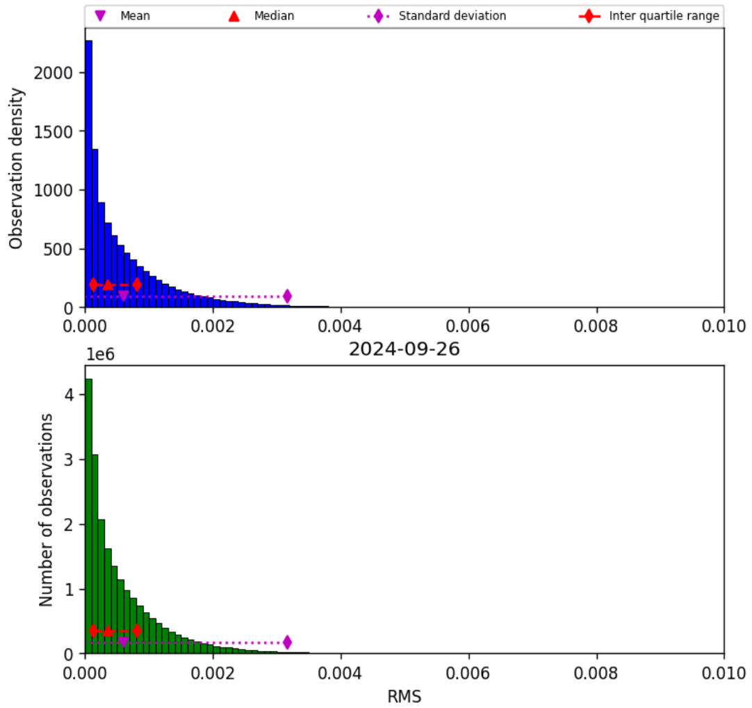
Figure 47: Histogram of “RMS” for 2024-09-25 to 2024-09-27
