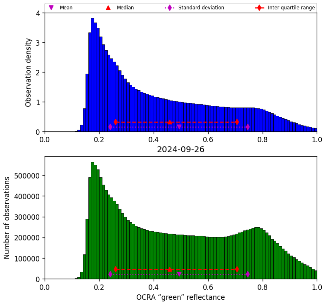
Figure 52: Histogram of “OCRA “green” reflectance” for 2024-09-25 to 2024-09-27
