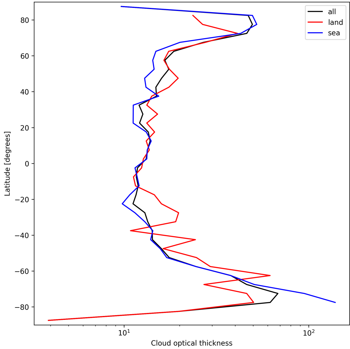
Figure 25: Zonal average of “Cloud optical thickness” for 2024-09-25 to 2024-09-27.
