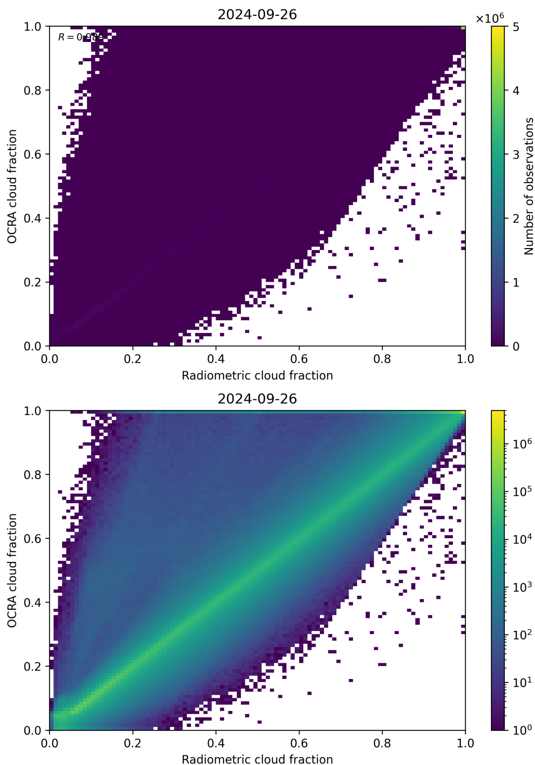
Figure 72: Scatter density plot of “Radiometric cloud fraction” against “OCRA cloud fraction” for 2024-09-25 to 2024-09-27.
