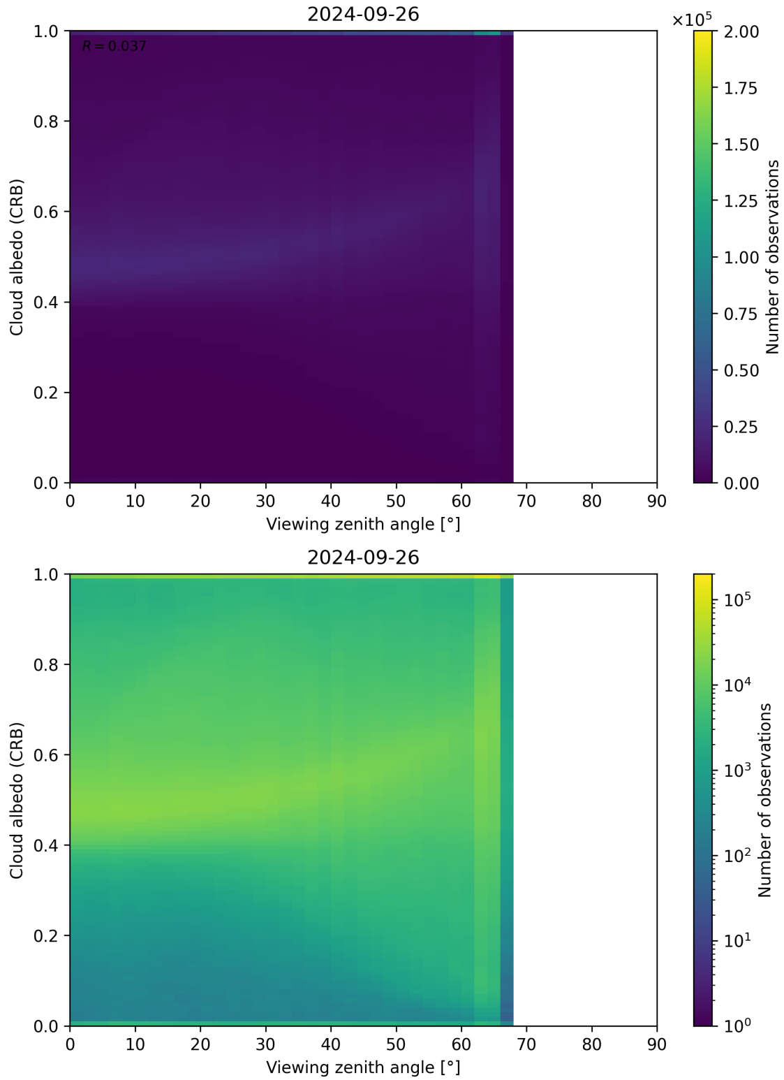
Figure 106: Scatter density plot of “Viewing zenith angle” against “Cloud albedo (CRB)” for 2024-09-25 to 2024-09-27.
