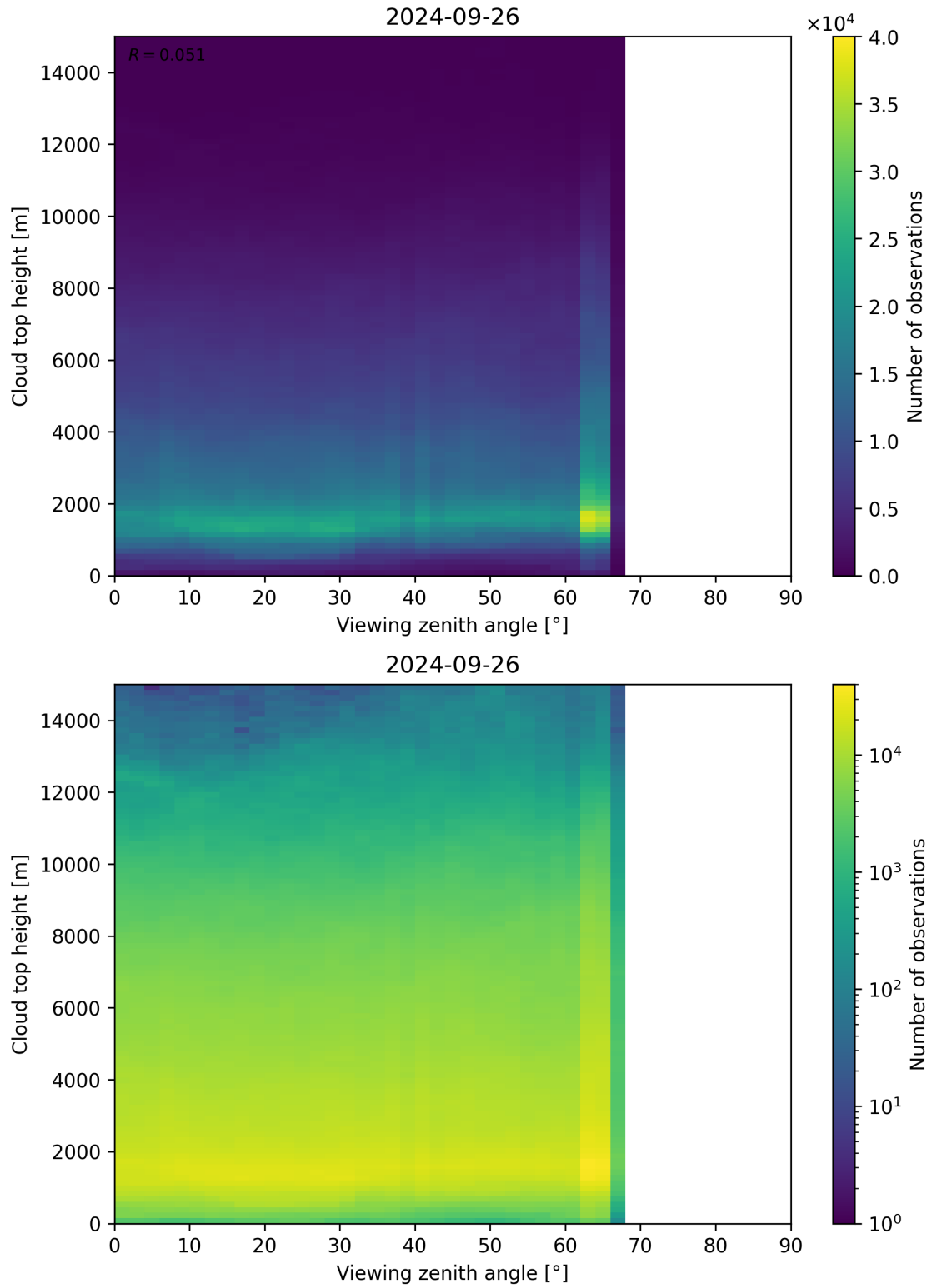
Figure 112: Scatter density plot of “Viewing zenith angle” against “Cloud top height” for 2024-09-25 to 2024-09-27.
