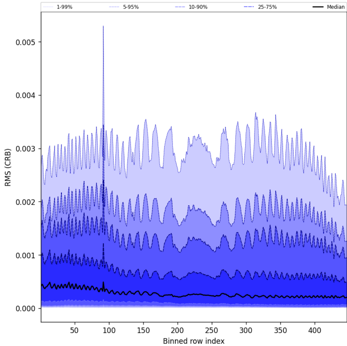
Figure 64: Along track statistics of “RMS (CRB)” for 2024-09-25 to 2024-09-27
