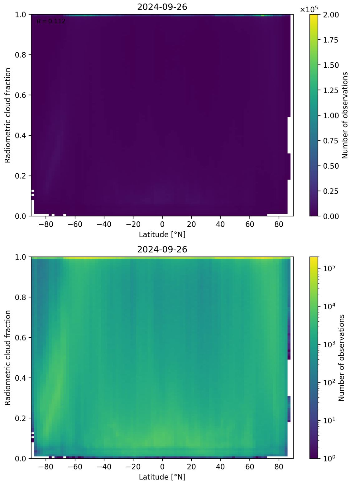
Figure 92: Scatter density plot of “Latitude” against “Radiometric cloud fraction” for 2024-09-25 to 2024-09-27.
