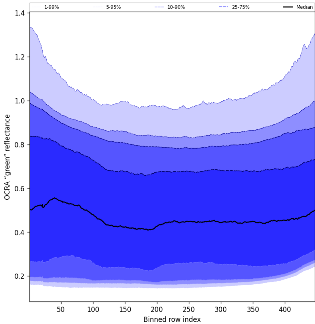
Figure 68: Along track statistics of “OCRA “green” reflectance” for 2024-09-25 to 2024-09-27
