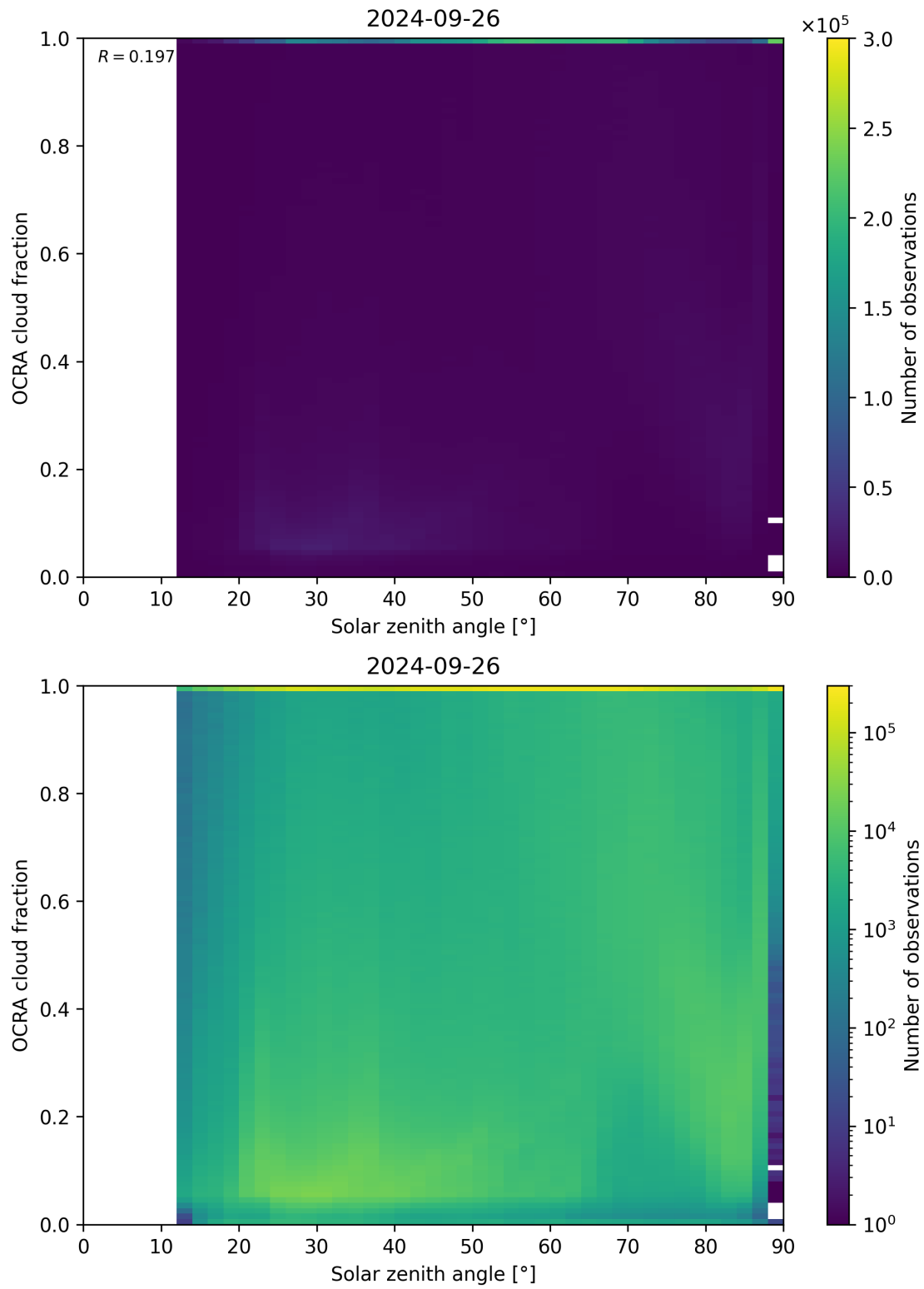
Figure 100: Scatter density plot of “Solar zenith angle” against “OCRA cloud fraction” for 2024-09-25 to 2024-09-27.
