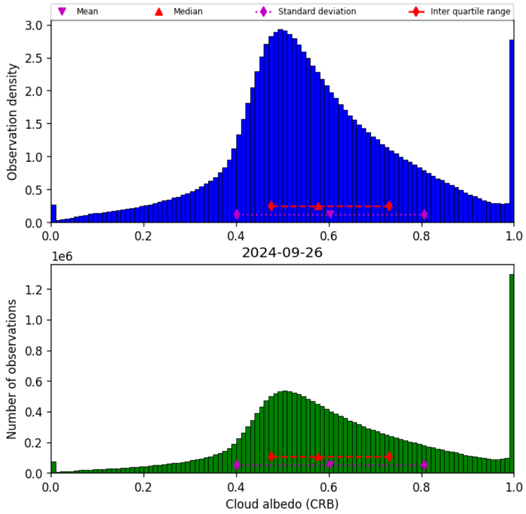
Figure 44: Histogram of “Cloud albedo (CRB)” for 2024-09-25 to 2024-09-27
