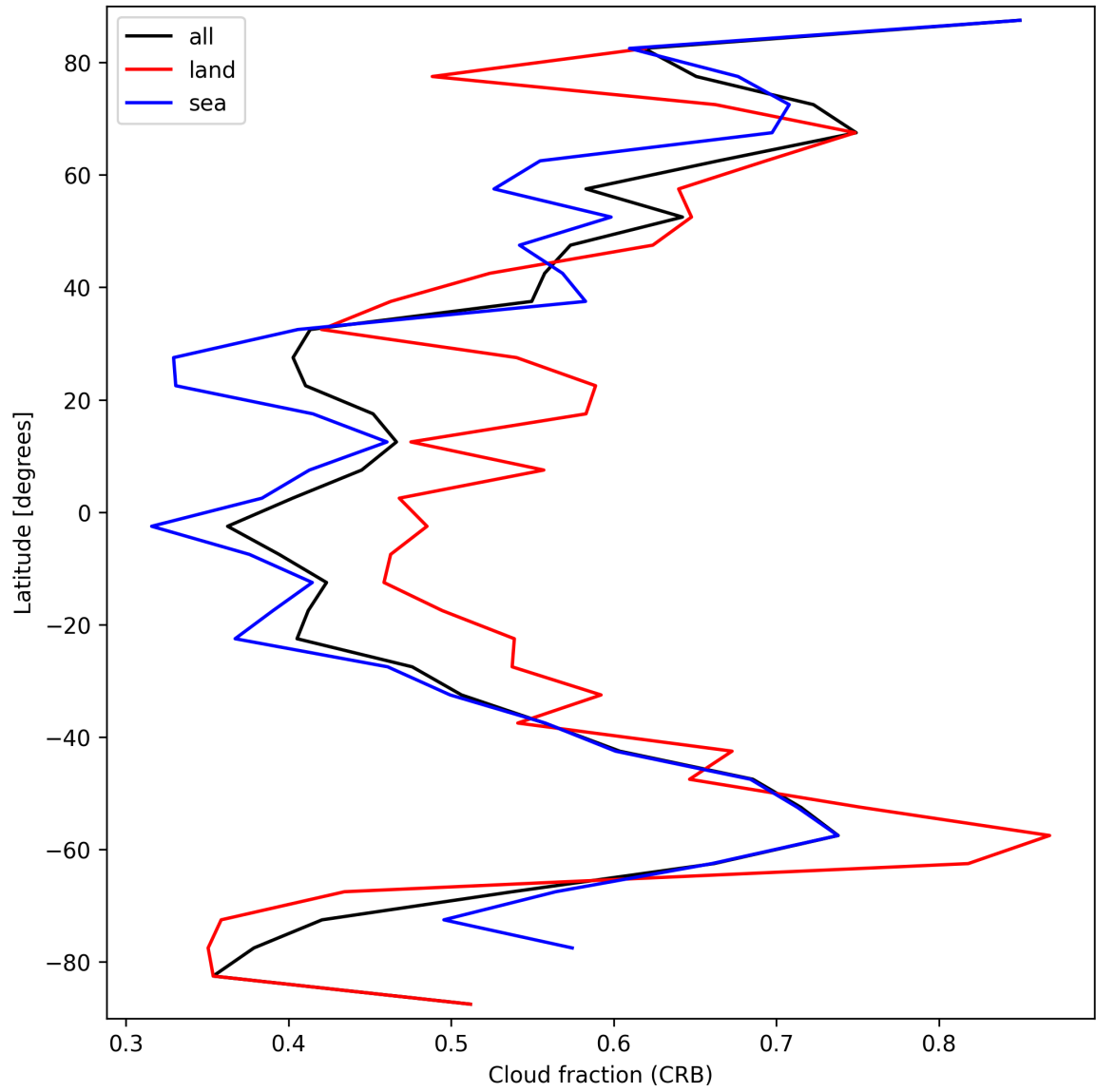
Figure 26: Zonal average of “Cloud fraction (CRB)” for 2024-09-25 to 2024-09-27.
