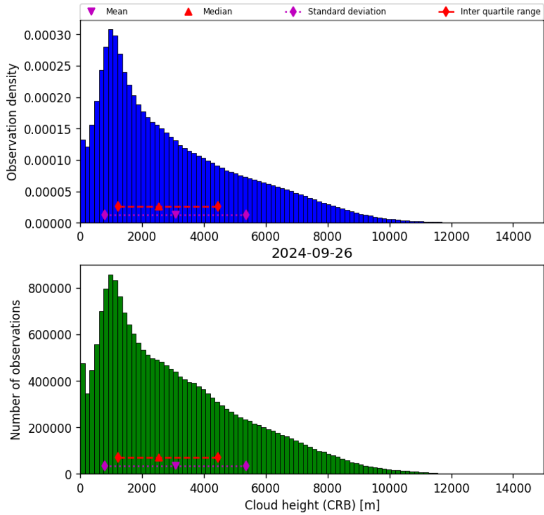
Figure 43: Histogram of “Cloud height (CRB)” for 2024-09-25 to 2024-09-27
