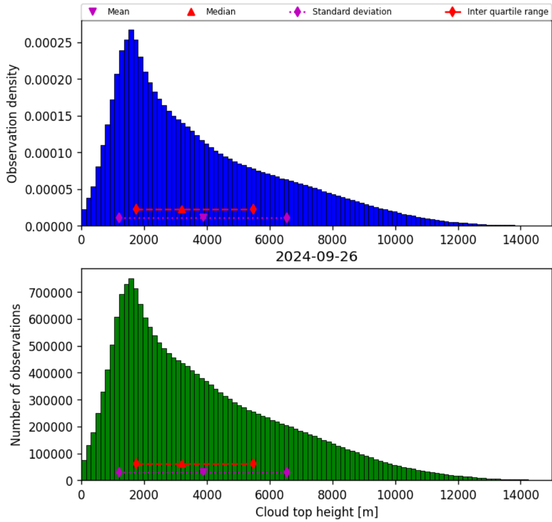
Figure 40: Histogram of “Cloud top height” for 2024-09-25 to 2024-09-27
