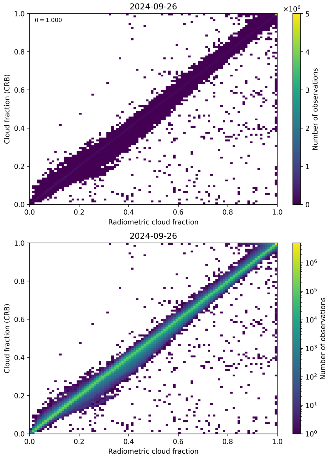
Figure 73: Scatter density plot of “Radiometric cloud fraction” against “Cloud fraction (CRB)” for 2024-09-25 to 2024-09-27.
