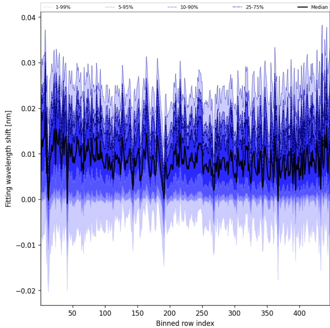
Figure 65: Along track statistics of “Fitting wavelength shift” for 2024-09-25 to 2024-09-27
