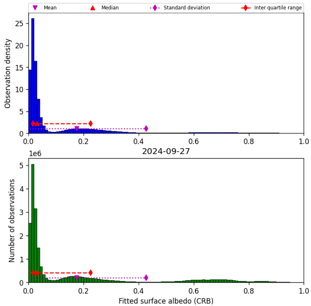
Figure 46: Histogram of “Fitted surface albedo (CRB)” for 2024-09-26 to 2024-09-28
