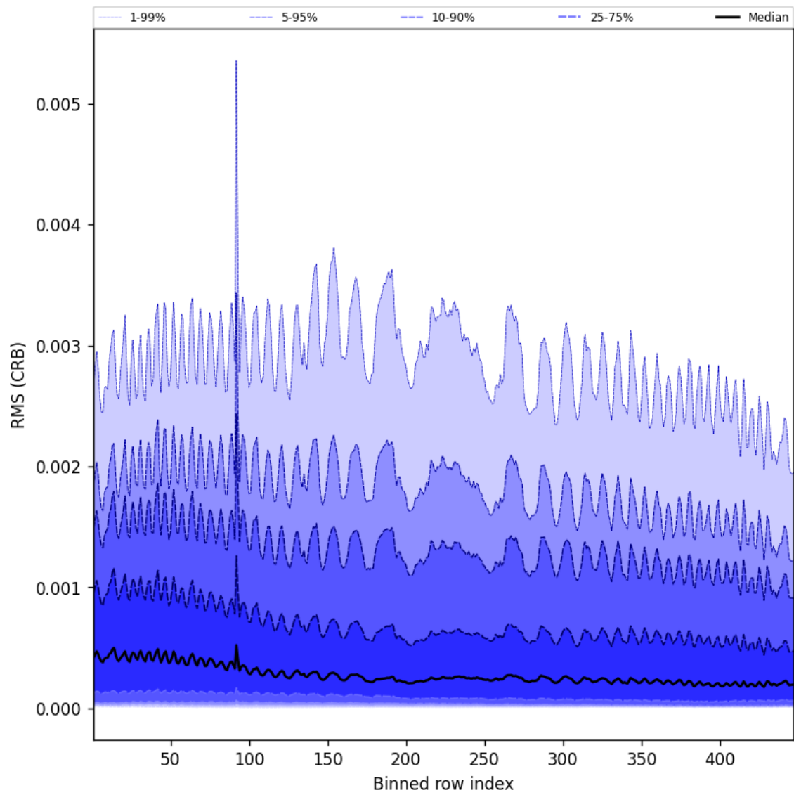
Figure 64: Along track statistics of “RMS (CRB)” for 2024-09-26 to 2024-09-28
