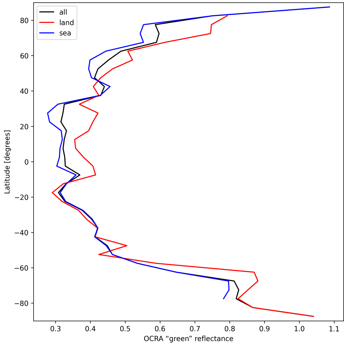
Figure 36: Zonal average of “OCRA “green” reflectance” for 2024-09-26 to 2024-09-28.
