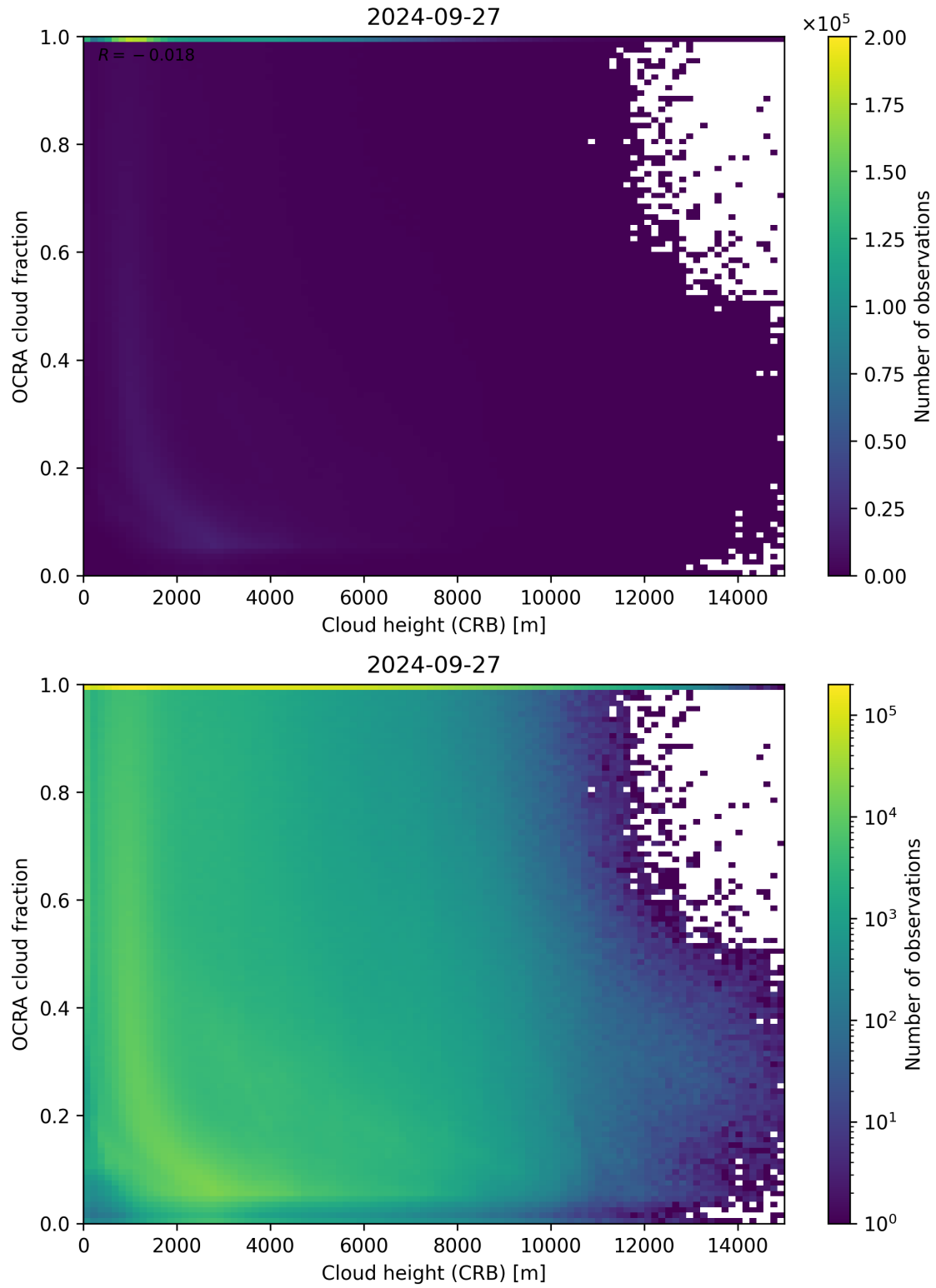
Figure 81: Scatter density plot of “Cloud height (CRB)” against “OCRA cloud fraction” for 2024-09-26 to 2024-09-28.
