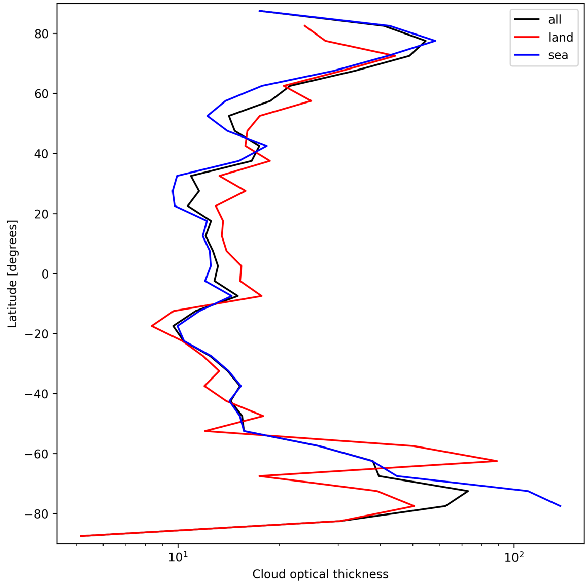
Figure 25: Zonal average of “Cloud optical thickness” for 2024-09-26 to 2024-09-28.
