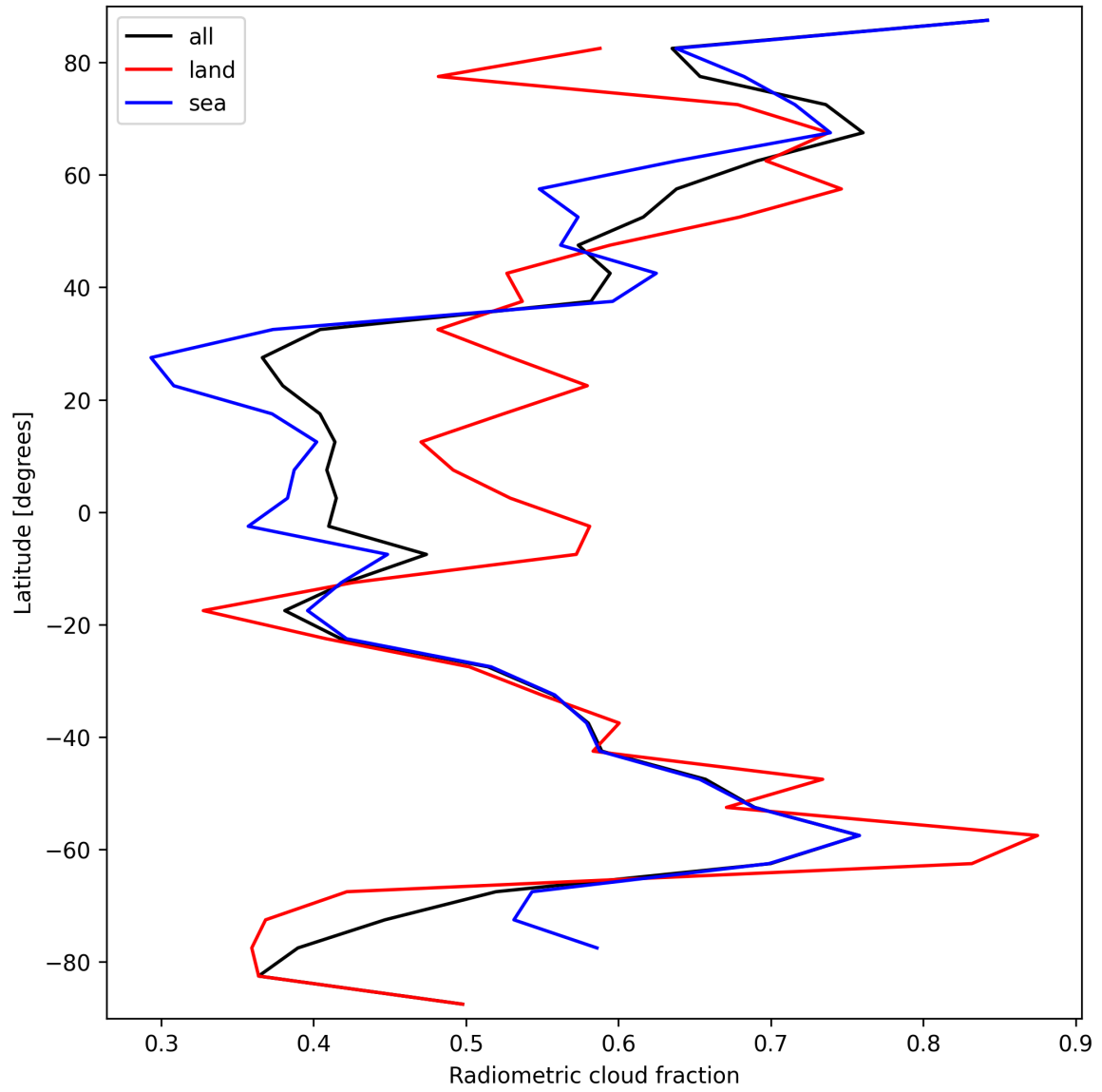
Figure 23: Zonal average of “Radiometric cloud fraction” for 2024-09-26 to 2024-09-28.
