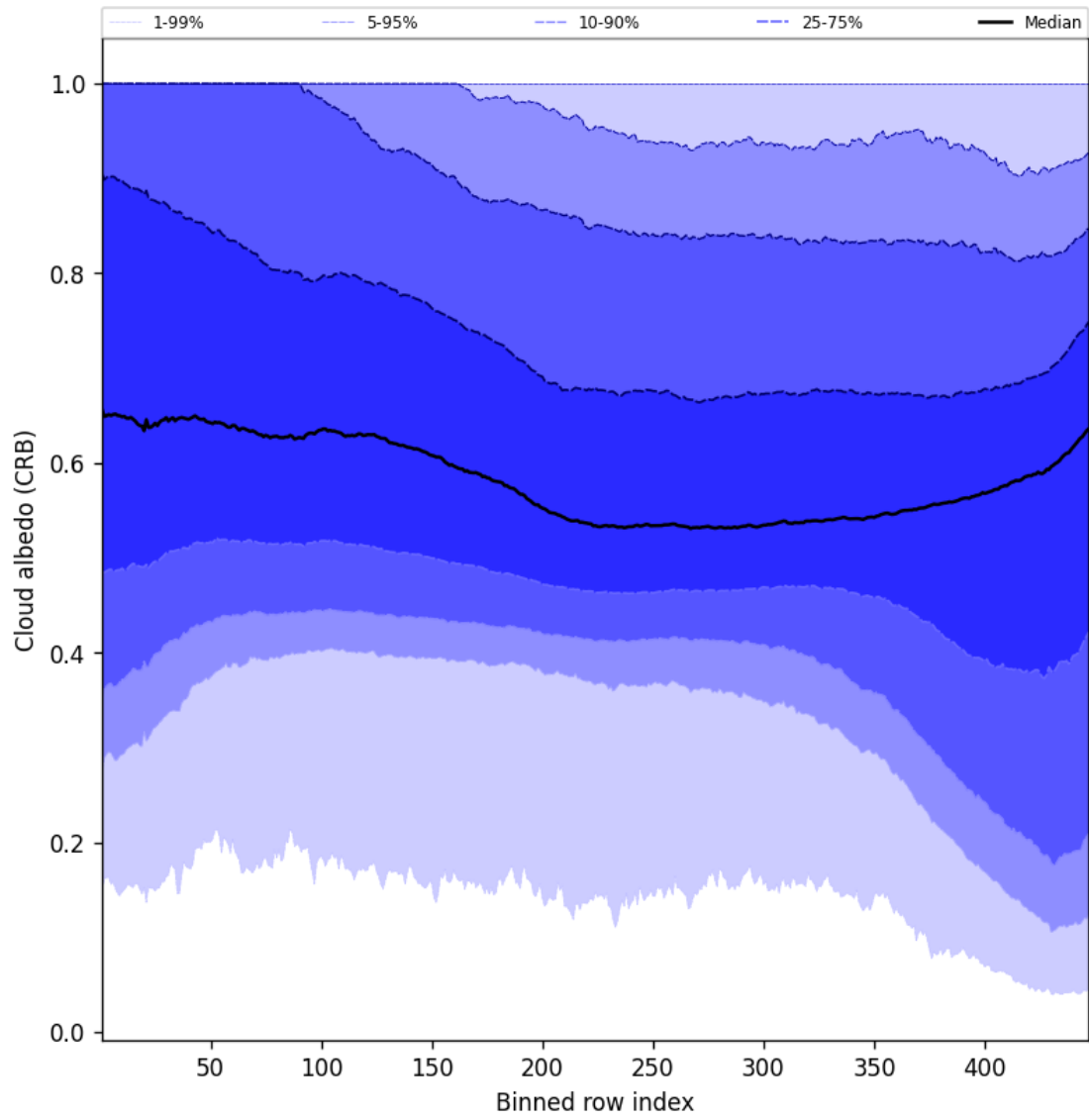
Figure 60: Along track statistics of “Cloud albedo (CRB)” for 2024-09-26 to 2024-09-28
