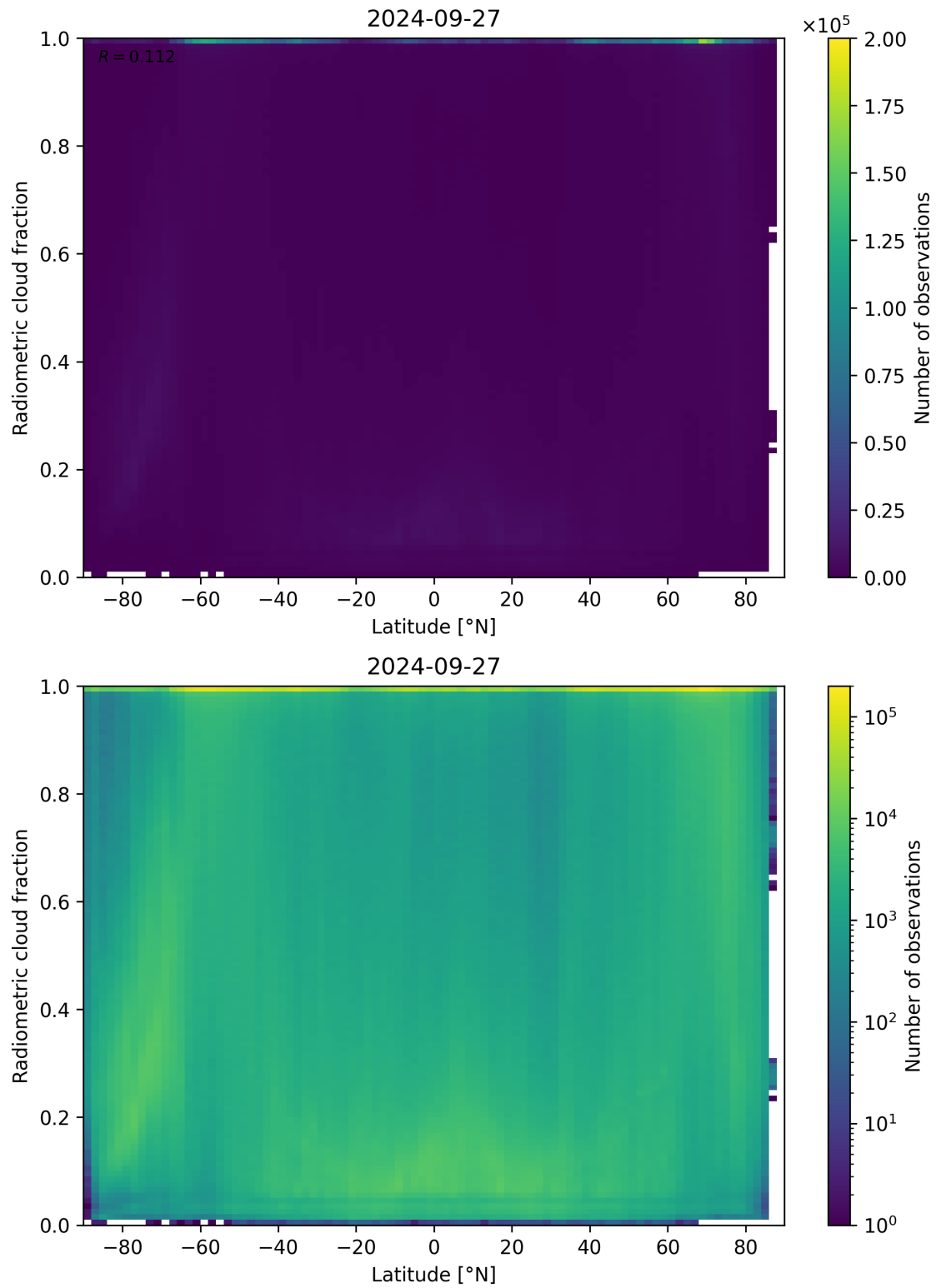
Figure 92: Scatter density plot of “Latitude” against “Radiometric cloud fraction” for 2024-09-26 to 2024-09-28.
