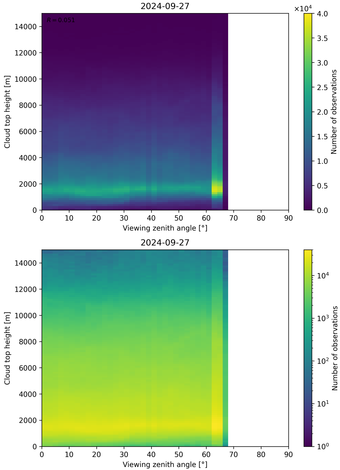
Figure 112: Scatter density plot of “Viewing zenith angle” against “Cloud top height” for 2024-09-26 to 2024-09-28.
