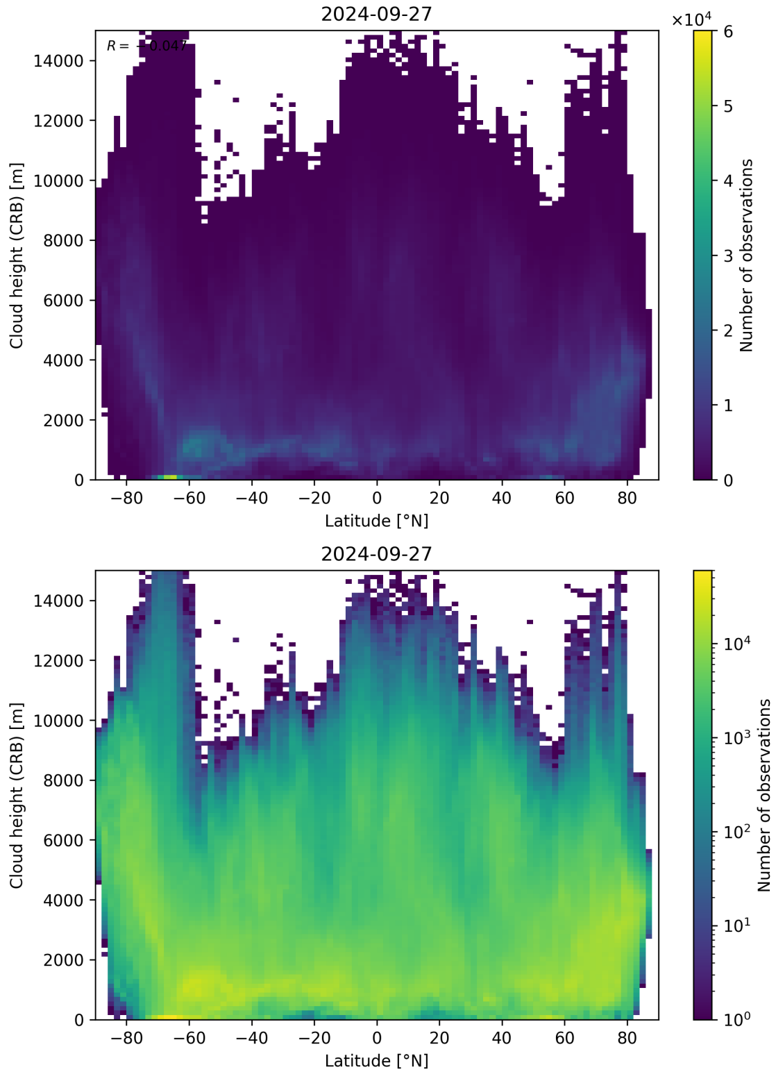
Figure 95: Scatter density plot of “Latitude” against “Cloud height (CRB)” for 2024-09-26 to 2024-09-28.
