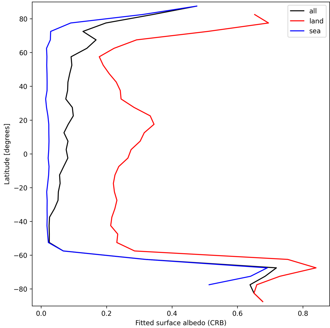
Figure 30: Zonal average of “Fitted surface albedo (CRB)” for 2024-09-26 to 2024-09-28.
