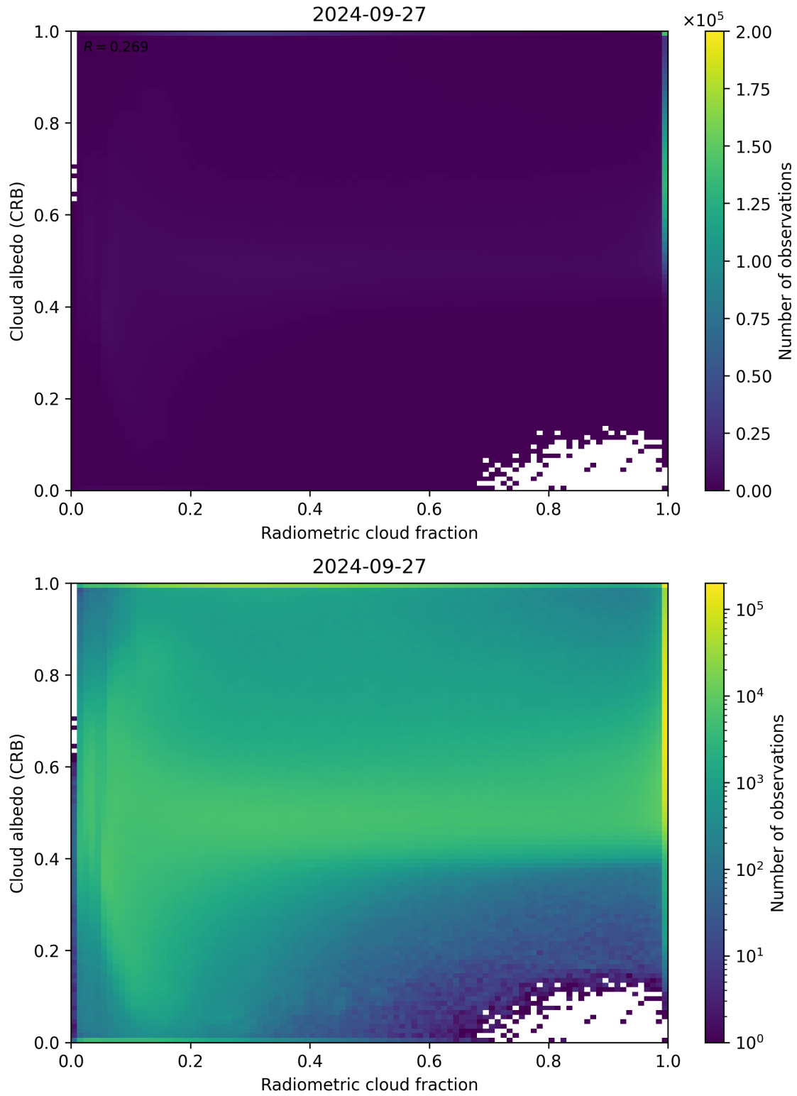
Figure 71: Scatter density plot of “Radiometric cloud fraction” against “Cloud albedo (CRB)” for 2024-09-26 to 2024-09-28.
