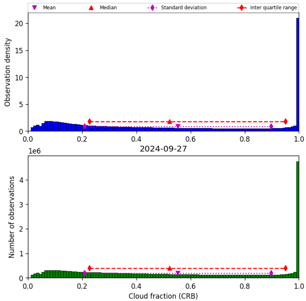
Figure 42: Histogram of “Cloud fraction (CRB)” for 2024-09-26 to 2024-09-28
