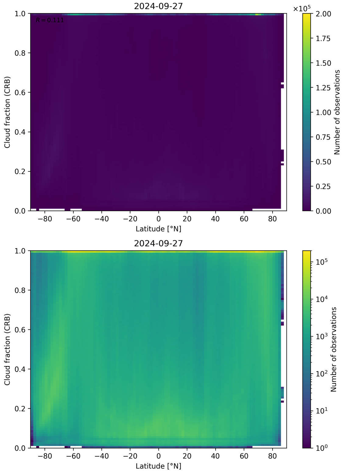
Figure 94: Scatter density plot of “Latitude” against “Cloud fraction (CRB)” for 2024-09-26 to 2024-09-28.
