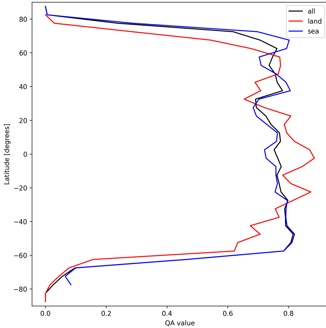
Figure 22: Zonal average of “QA value” for 2024-09-26 to 2024-09-28.
