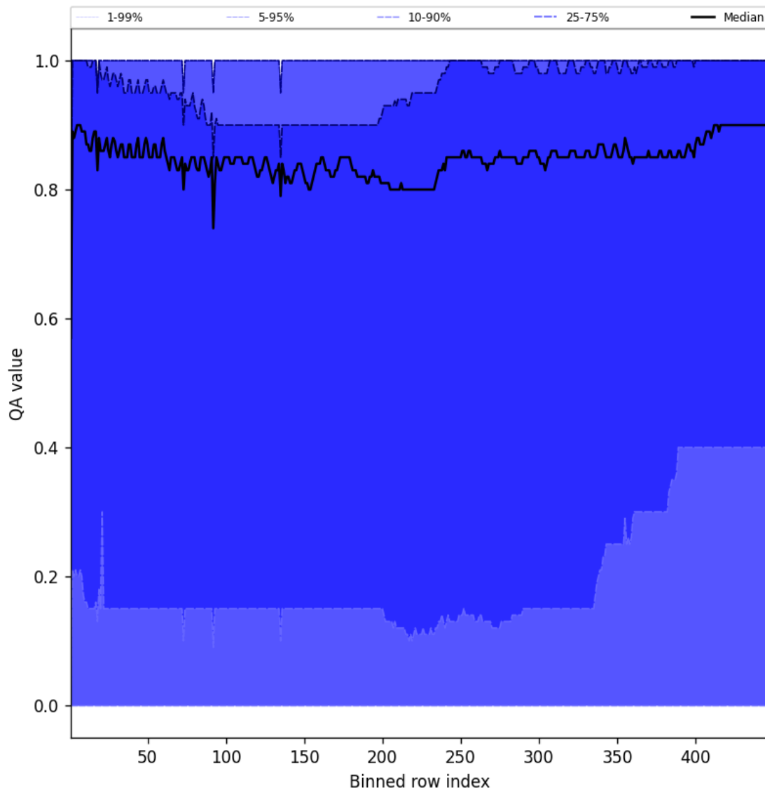
Figure 54: Along track statistics of “QA value” for 2024-09-26 to 2024-09-28
