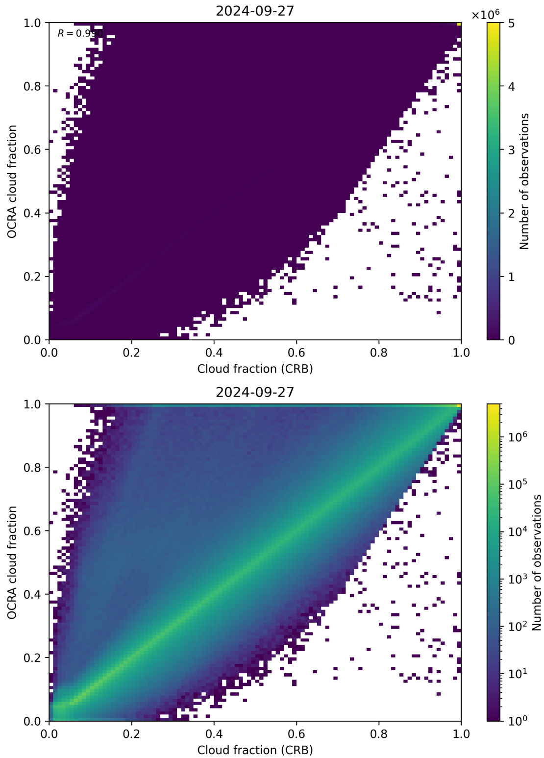
Figure 78: Scatter density plot of “Cloud fraction (CRB)” against “OCRA cloud fraction” for 2024-09-26 to 2024-09-28.
