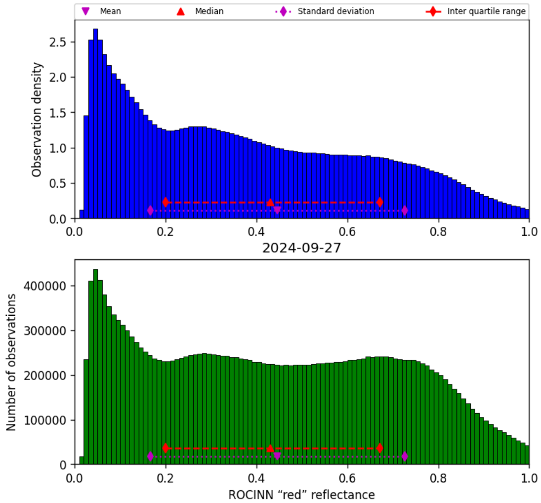
Figure 53: Histogram of “ROCINN “red” reflectance” for 2024-09-26 to 2024-09-28
