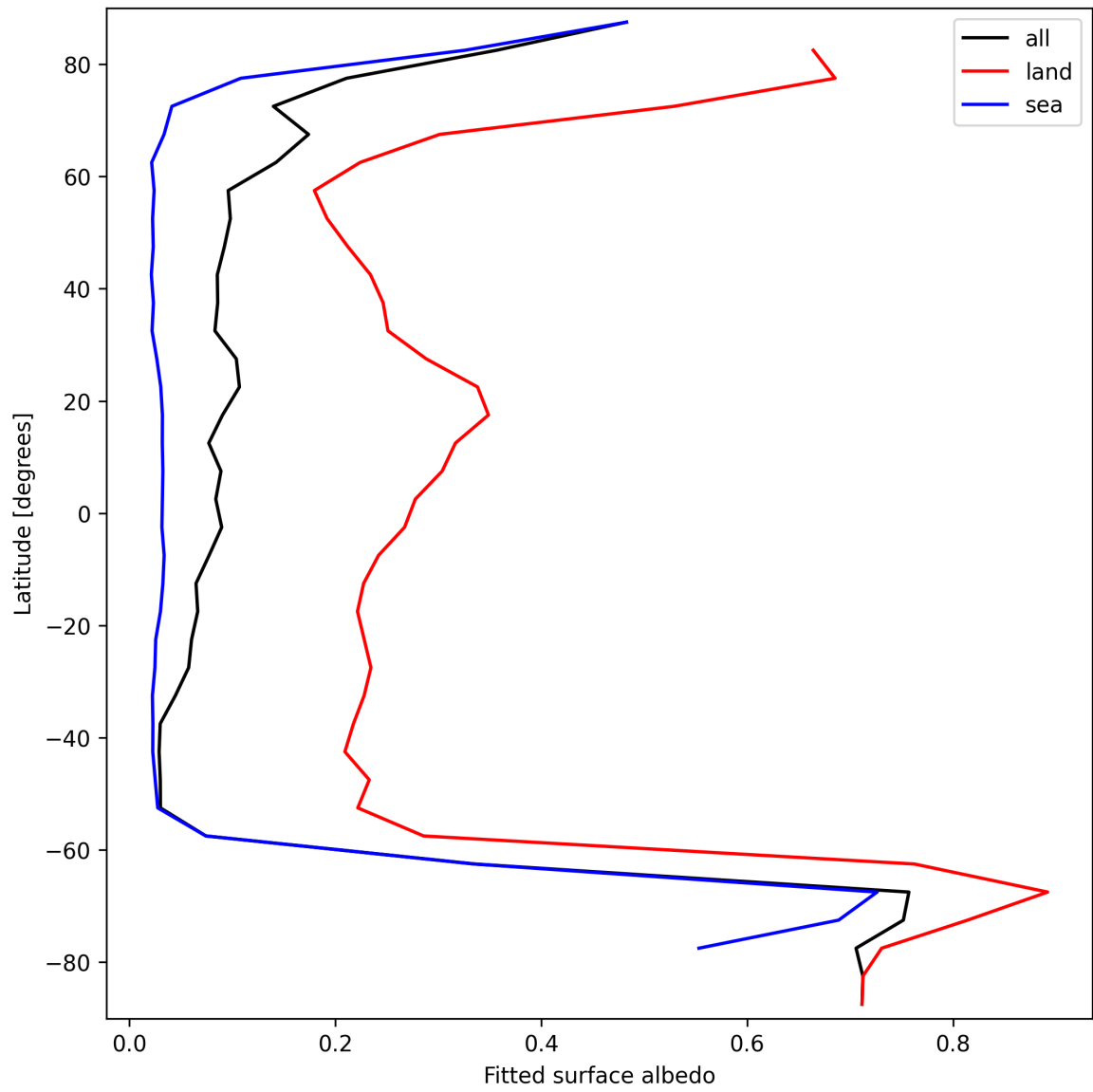
Figure 29: Zonal average of “Fitted surface albedo” for 2024-09-26 to 2024-09-28.
