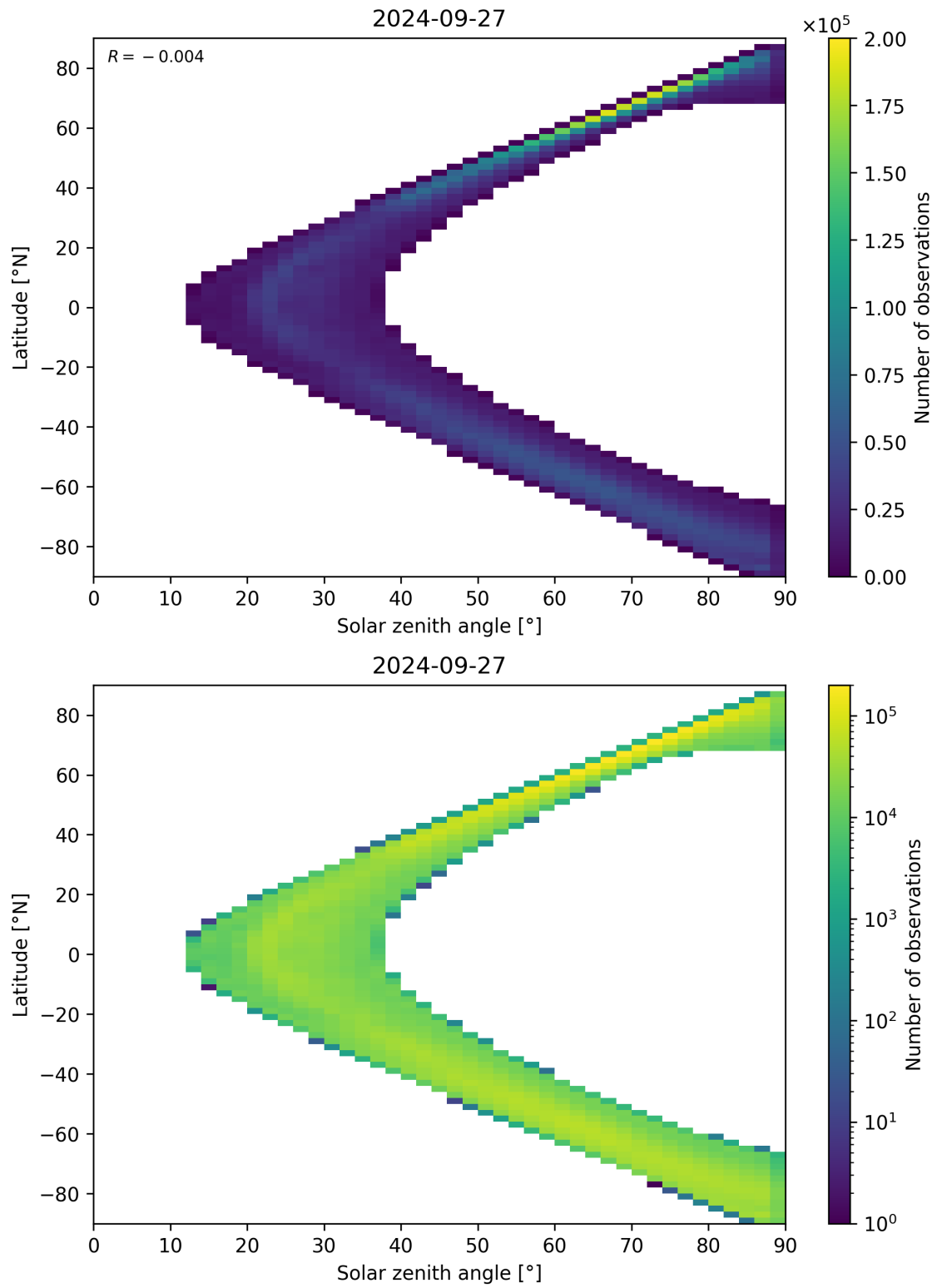
Figure 105: Scatter density plot of “Solar zenith angle” against “Latitude” for 2024-09-26 to 2024-09-28.
