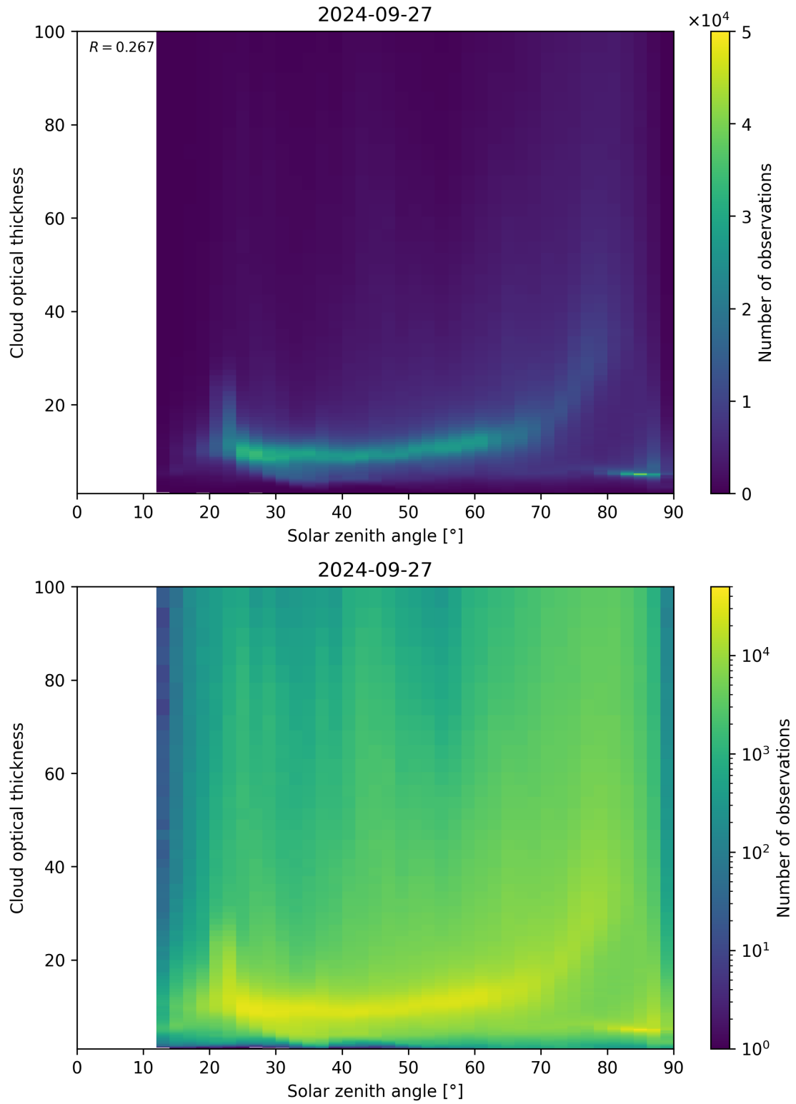
Figure 103: Scatter density plot of “Solar zenith angle” against “Cloud optical thickness” for 2024-09-26 to 2024-09-28.
