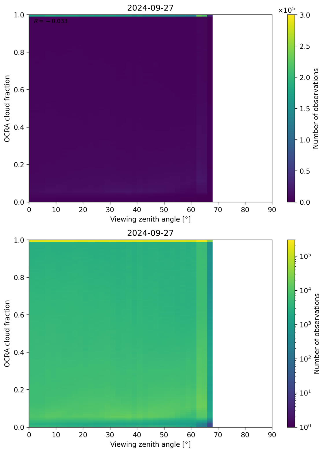
Figure 108: Scatter density plot of “Viewing zenith angle” against “OCRA cloud fraction” for 2024-09-26 to 2024-09-28.
