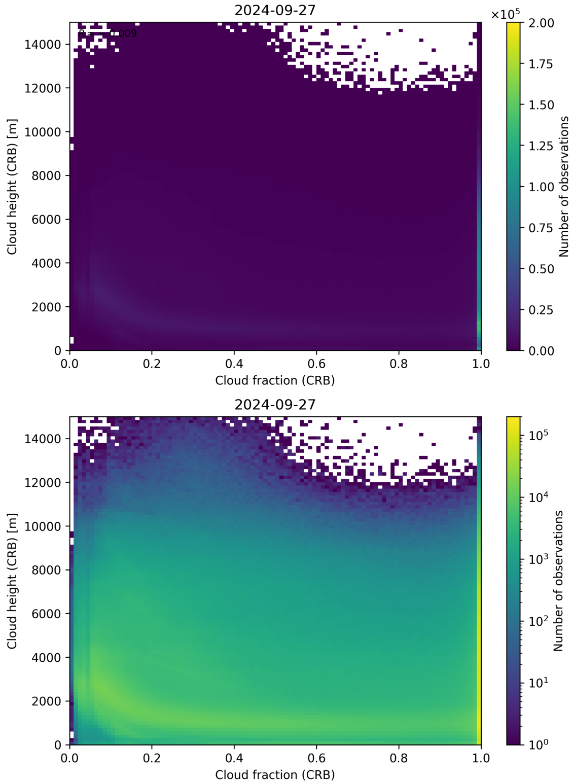
Figure 79: Scatter density plot of “Cloud fraction (CRB)” against “Cloud height (CRB)” for 2024-09-26 to 2024-09-28.
