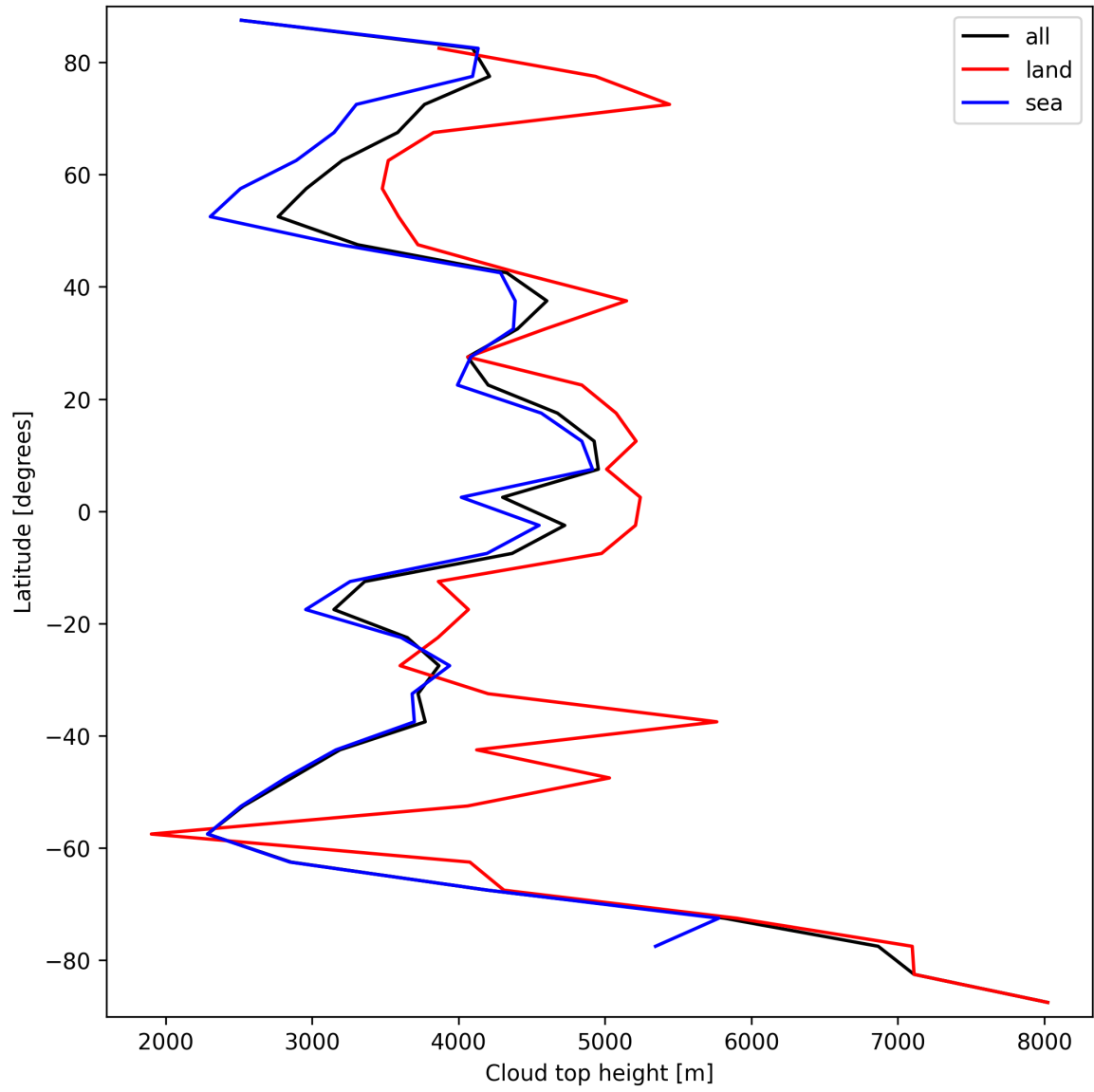
Figure 24: Zonal average of “Cloud top height” for 2024-09-26 to 2024-09-28.
