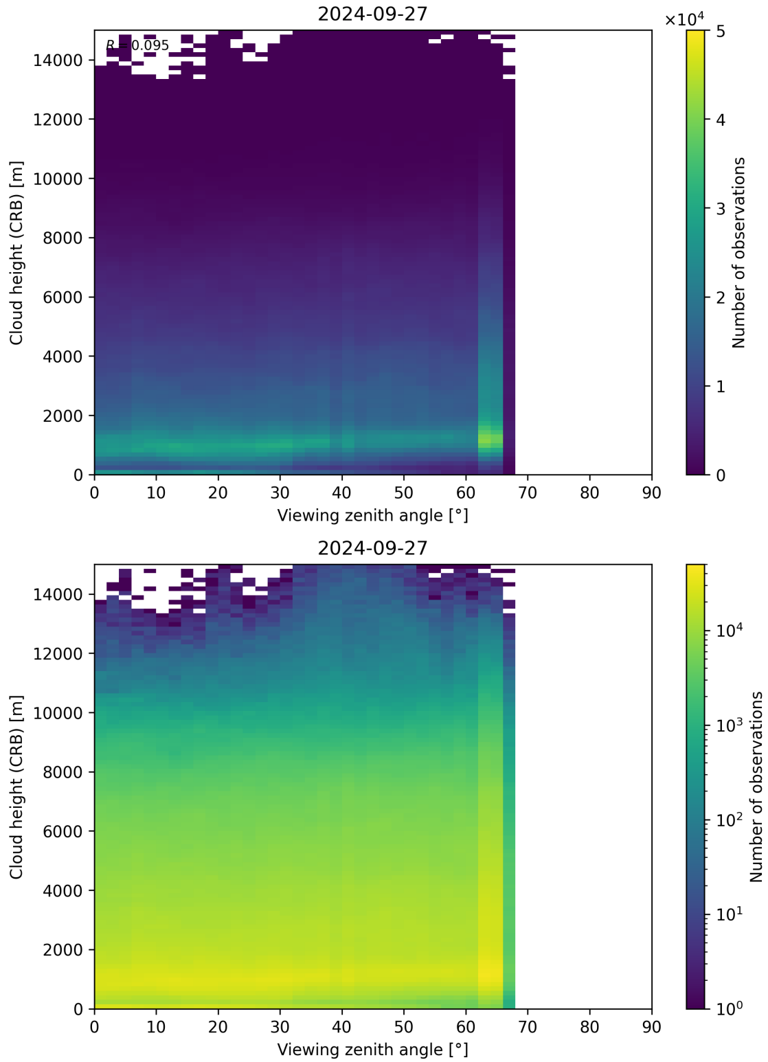
Figure 110: Scatter density plot of “Viewing zenith angle” against “Cloud height (CRB)” for 2024-09-26 to 2024-09-28.
