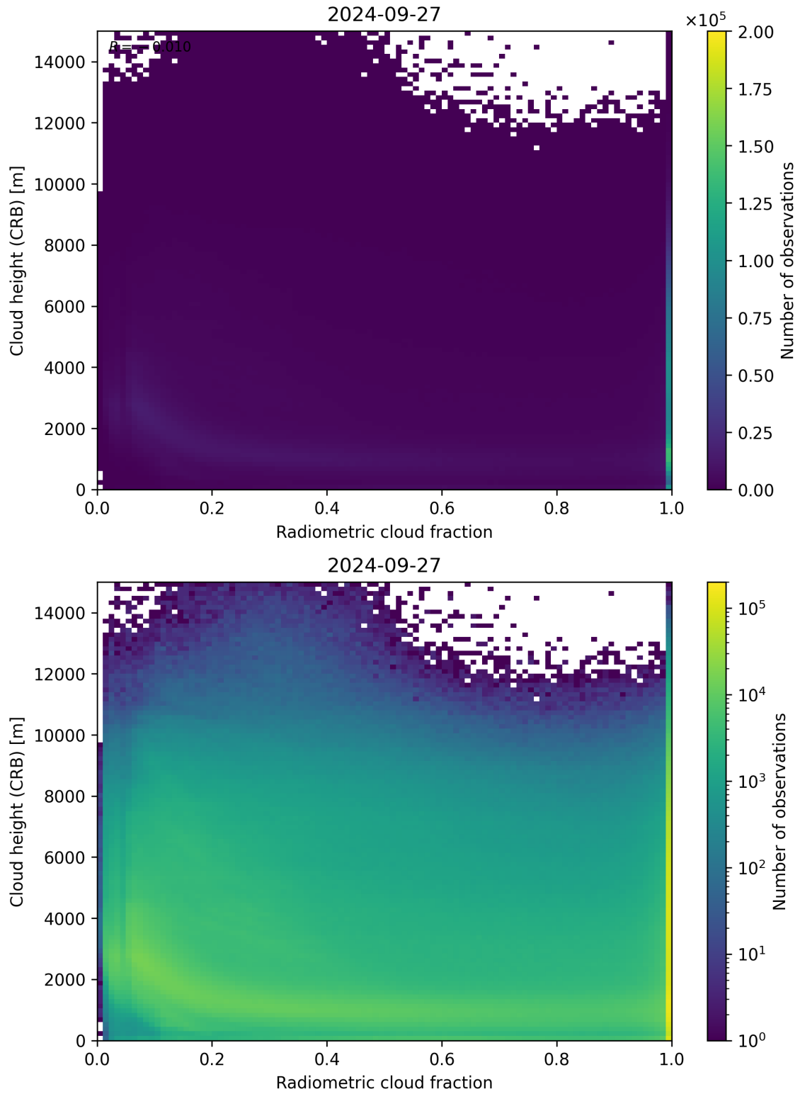
Figure 74: Scatter density plot of “Radiometric cloud fraction” against “Cloud height (CRB)” for 2024-09-26 to 2024-09-28.
