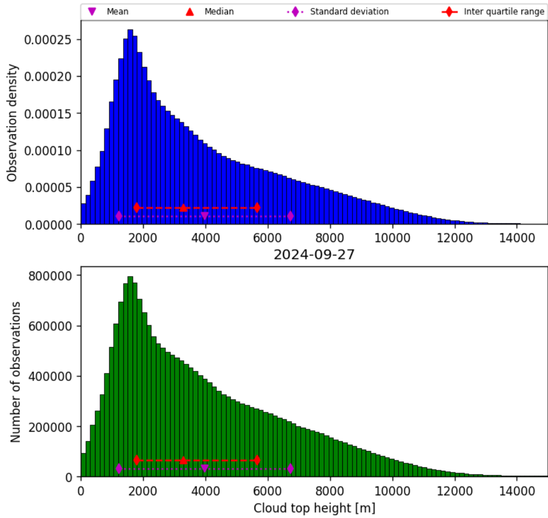
Figure 40: Histogram of “Cloud top height” for 2024-09-26 to 2024-09-28
