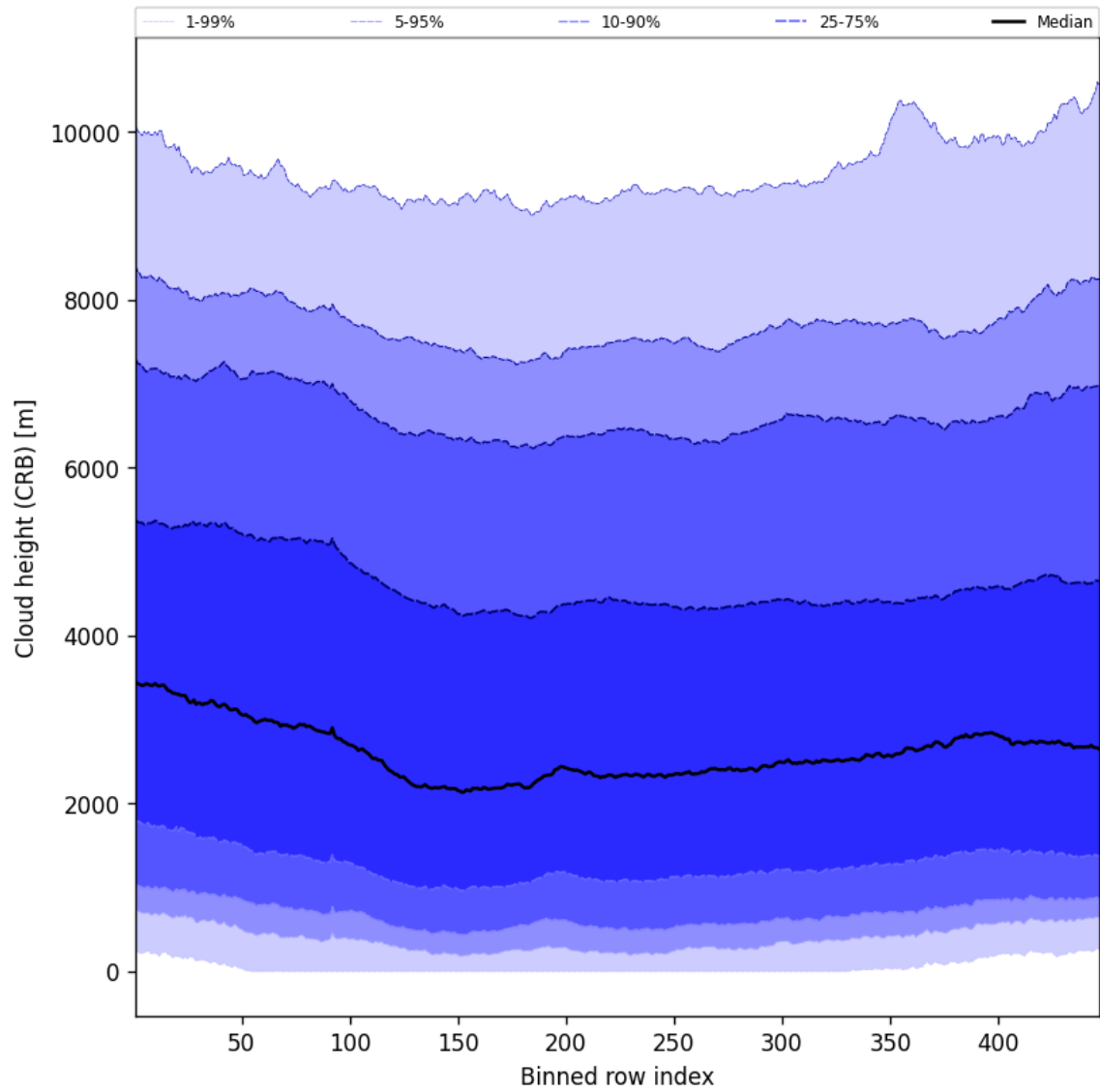
Figure 59: Along track statistics of “Cloud height (CRB)” for 2024-09-26 to 2024-09-28
