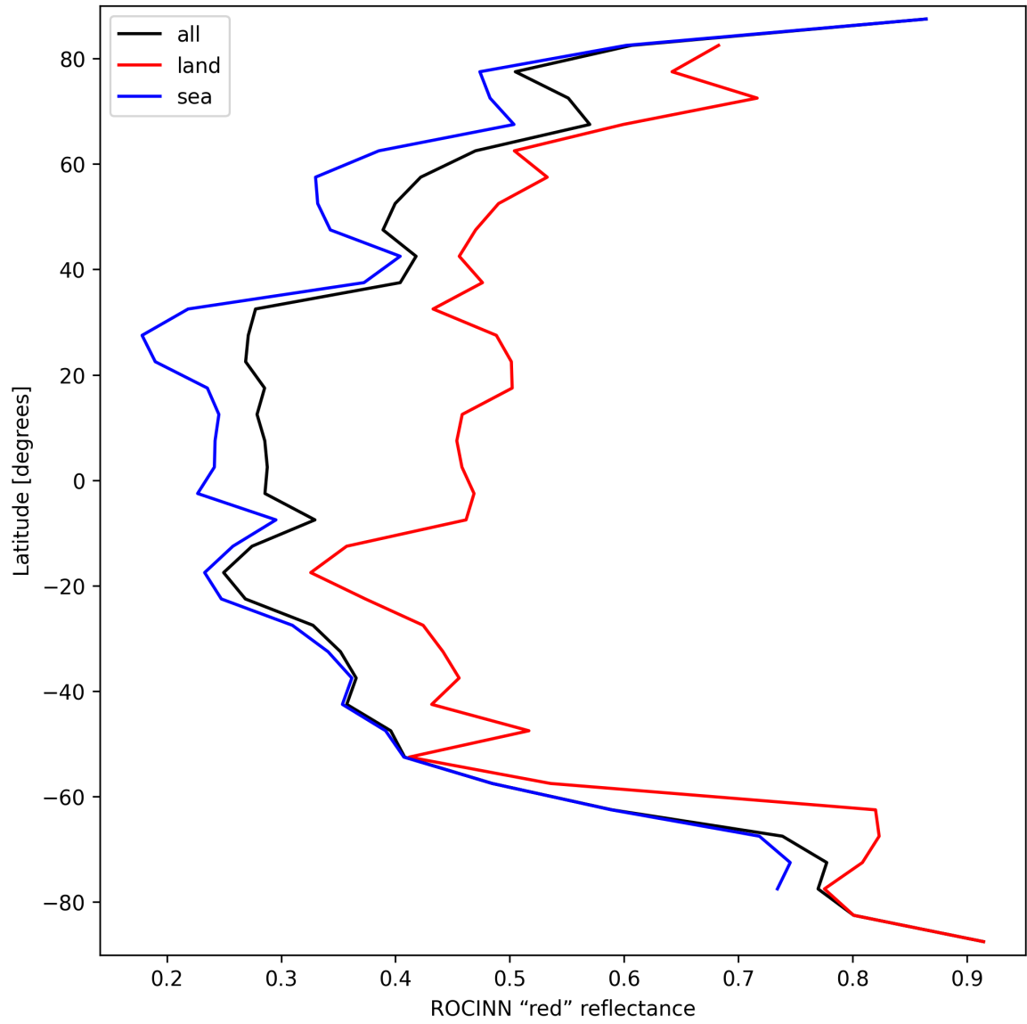
Figure 37: Zonal average of “ROCINN “red” reflectance” for 2024-09-26 to 2024-09-28.
