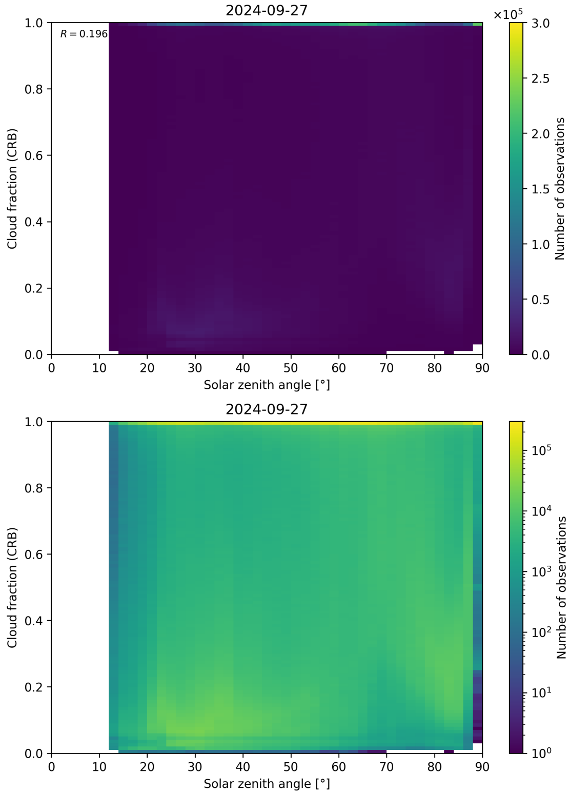
Figure 101: Scatter density plot of “Solar zenith angle” against “Cloud fraction (CRB)” for 2024-09-26 to 2024-09-28.
