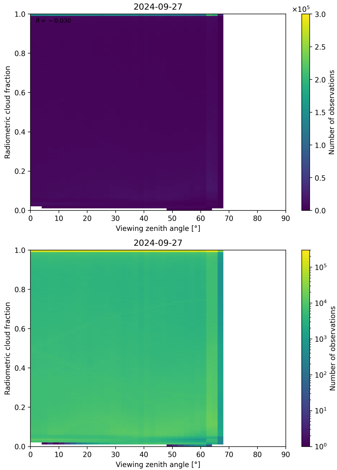
Figure 107: Scatter density plot of “Viewing zenith angle” against “Radiometric cloud fraction” for 2024-09-26 to 2024-09-28.
