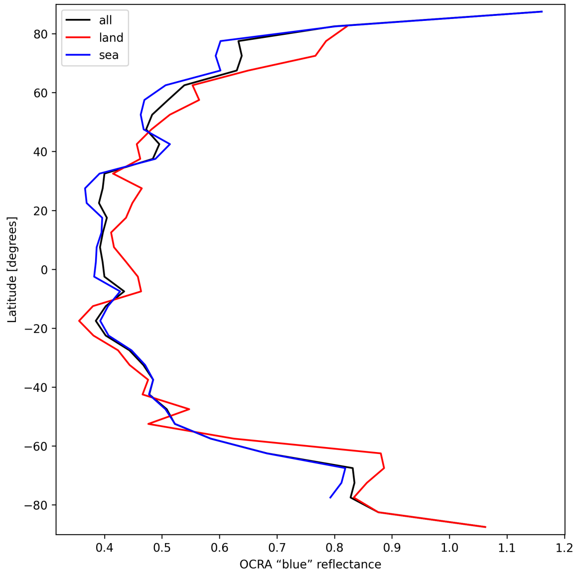
Figure 35: Zonal average of “OCRA “blue” reflectance” for 2024-09-26 to 2024-09-28.
