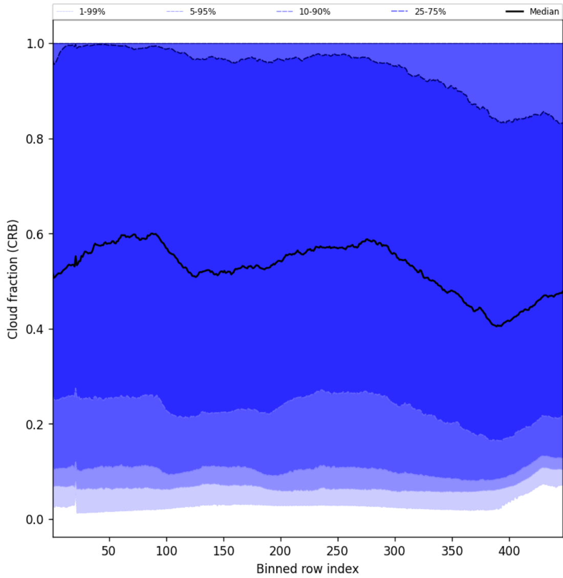
Figure 58: Along track statistics of “Cloud fraction (CRB)” for 2024-09-26 to 2024-09-28
