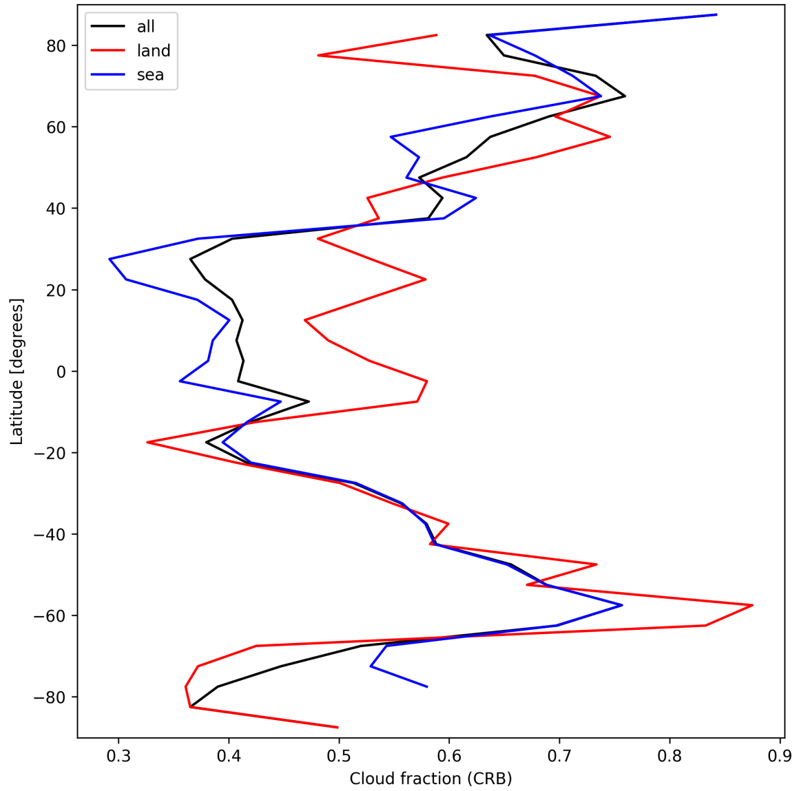
Figure 26: Zonal average of “Cloud fraction (CRB)” for 2024-09-26 to 2024-09-28.
