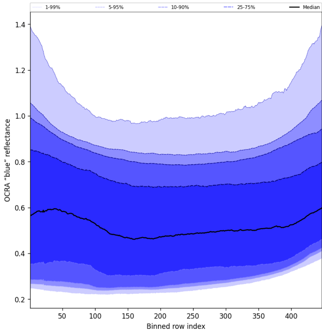
Figure 67: Along track statistics of “OCRA “blue” reflectance” for 2024-09-26 to 2024-09-28
