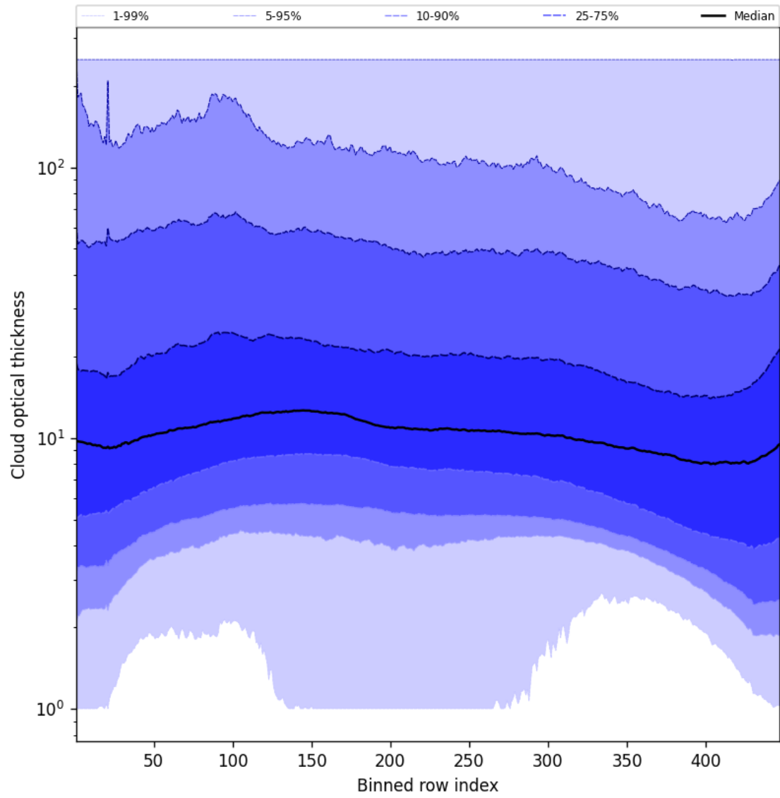
Figure 57: Along track statistics of “Cloud optical thickness” for 2024-09-26 to 2024-09-28
