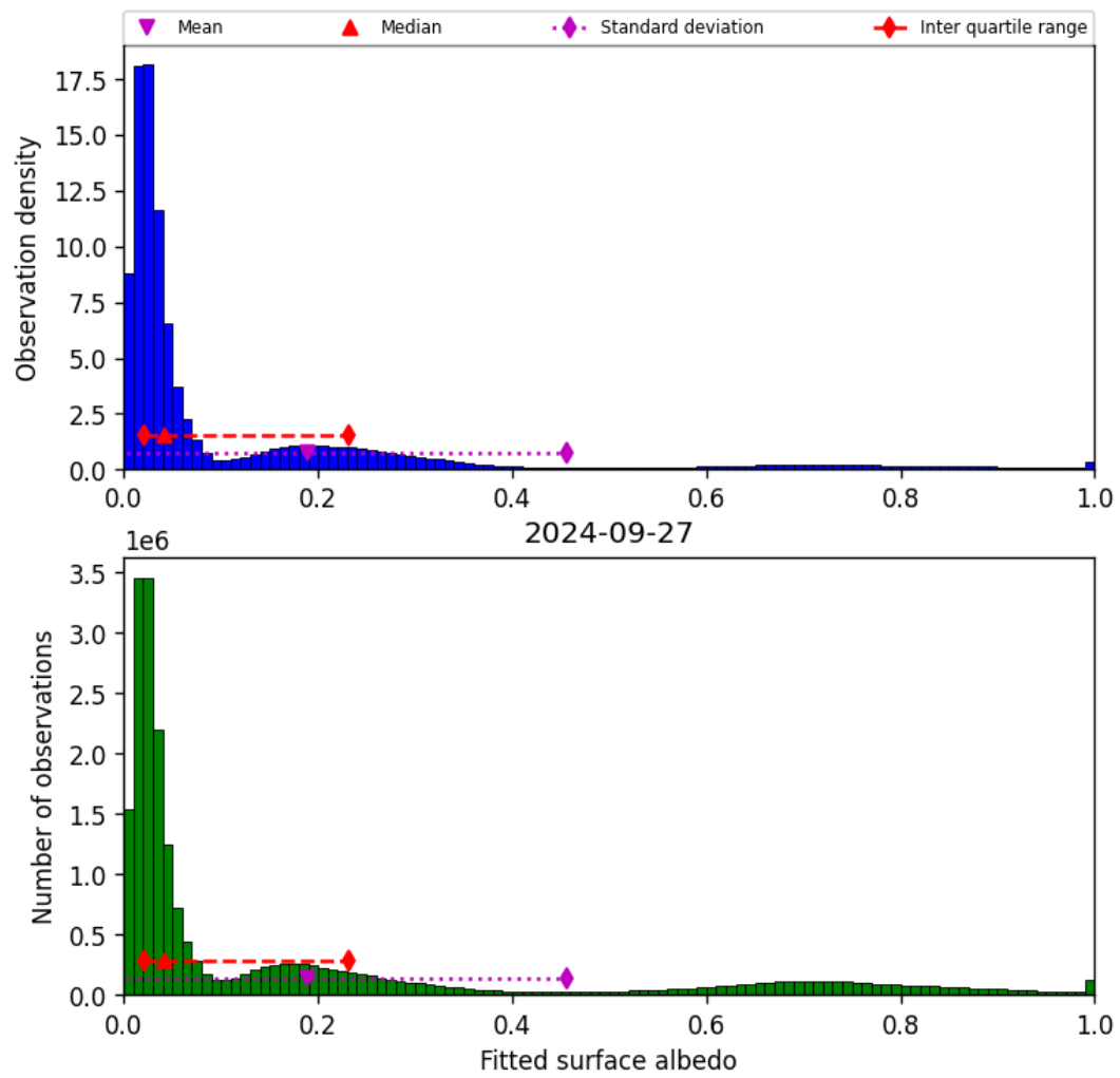
Figure 45: Histogram of “Fitted surface albedo” for 2024-09-26 to 2024-09-28
