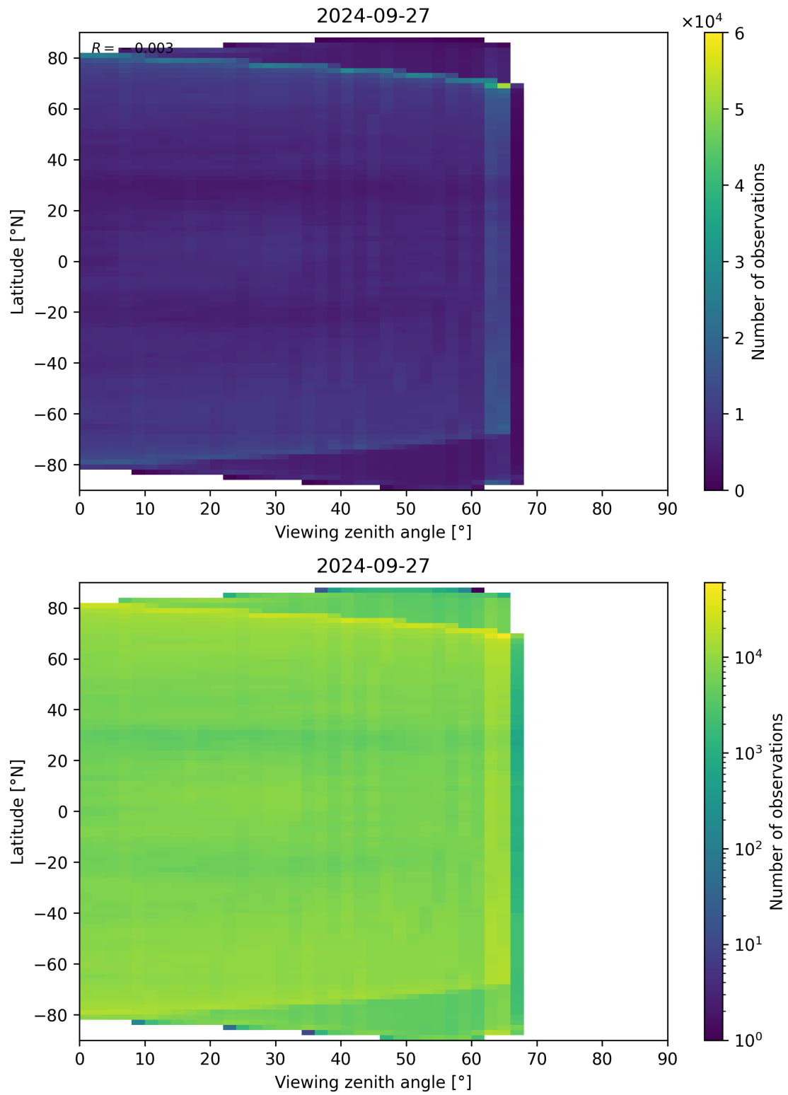
Figure 113: Scatter density plot of “Viewing zenith angle” against “Latitude” for 2024-09-26 to 2024-09-28.
