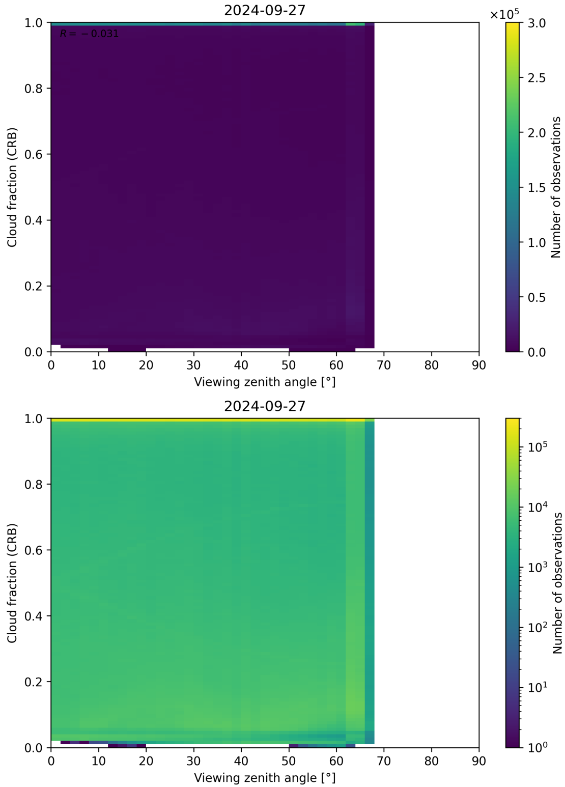
Figure 109: Scatter density plot of “Viewing zenith angle” against “Cloud fraction (CRB)” for 2024-09-26 to 2024-09-28.
