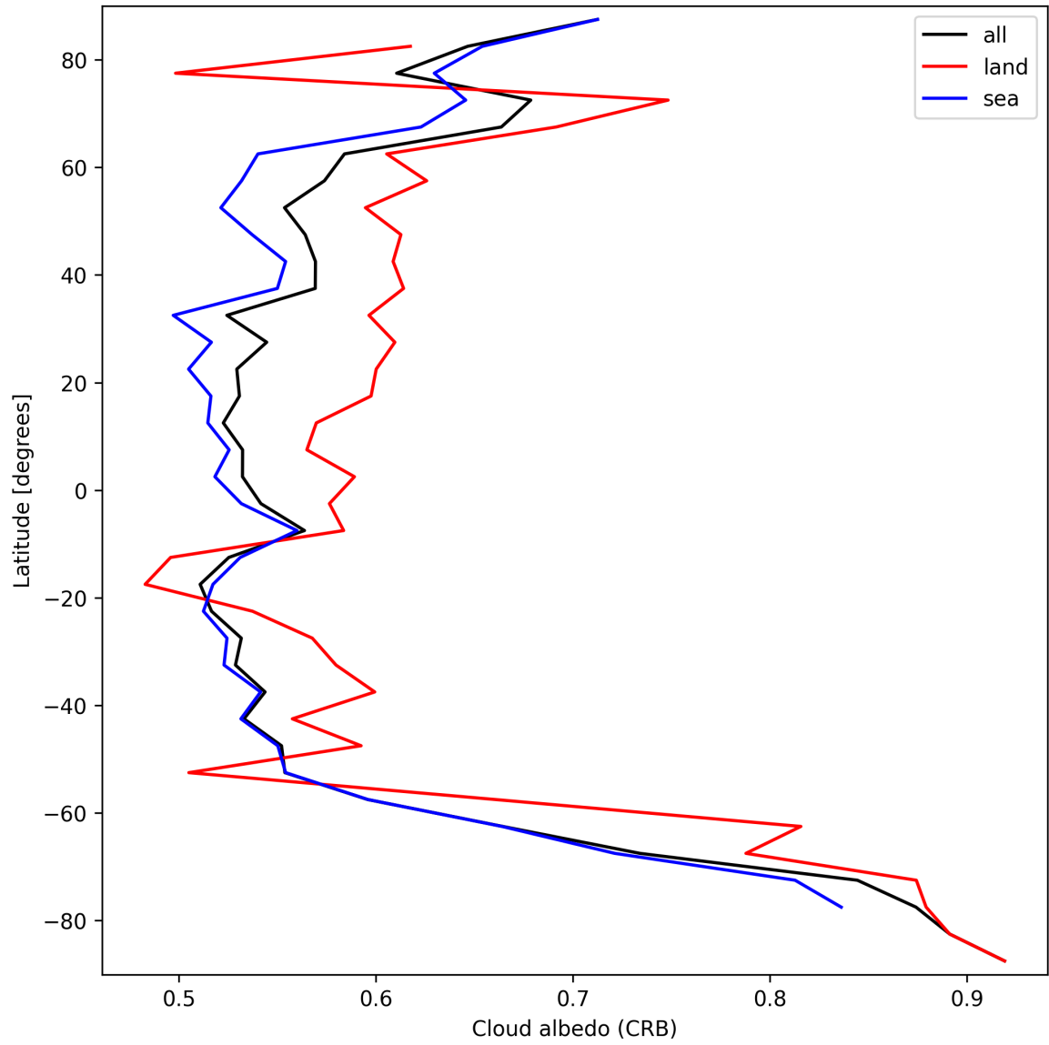
Figure 28: Zonal average of “Cloud albedo (CRB)” for 2024-09-26 to 2024-09-28.
