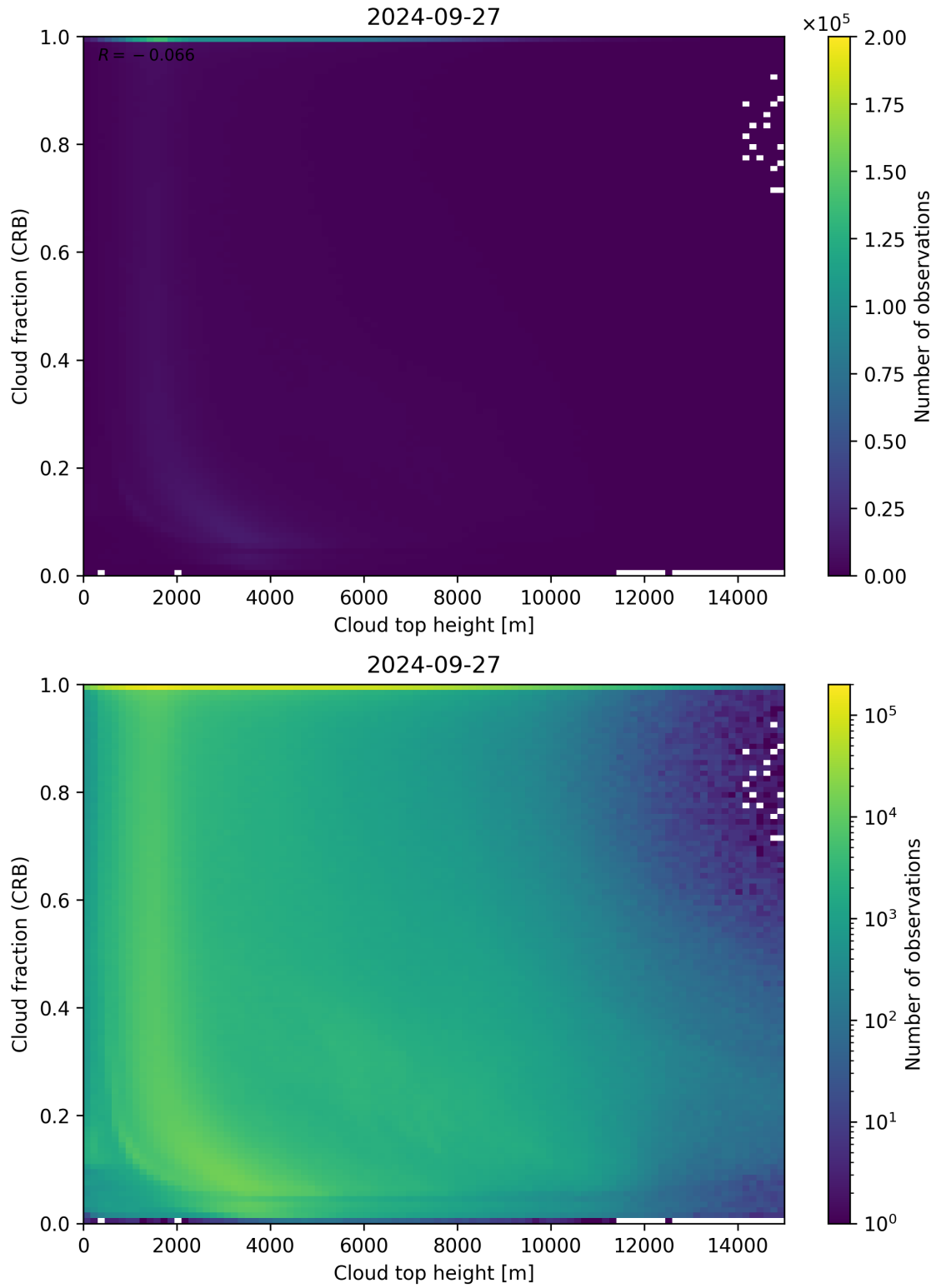
Figure 88: Scatter density plot of “Cloud top height” against “Cloud fraction (CRB)” for 2024-09-26 to 2024-09-28.
