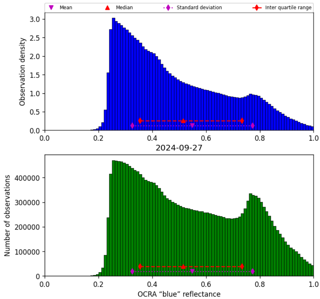
Figure 51: Histogram of “OCRA “blue” reflectance” for 2024-09-26 to 2024-09-28
