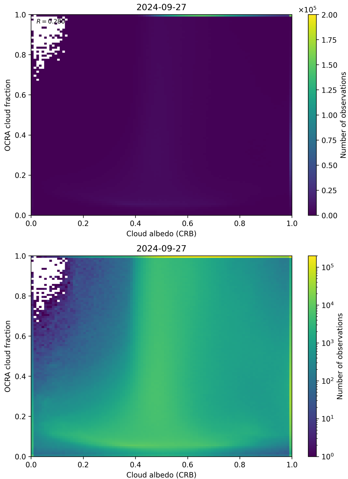
Figure 70: Scatter density plot of “Cloud albedo (CRB)” against “OCRA cloud fraction” for 2024-09-26 to 2024-09-28.
