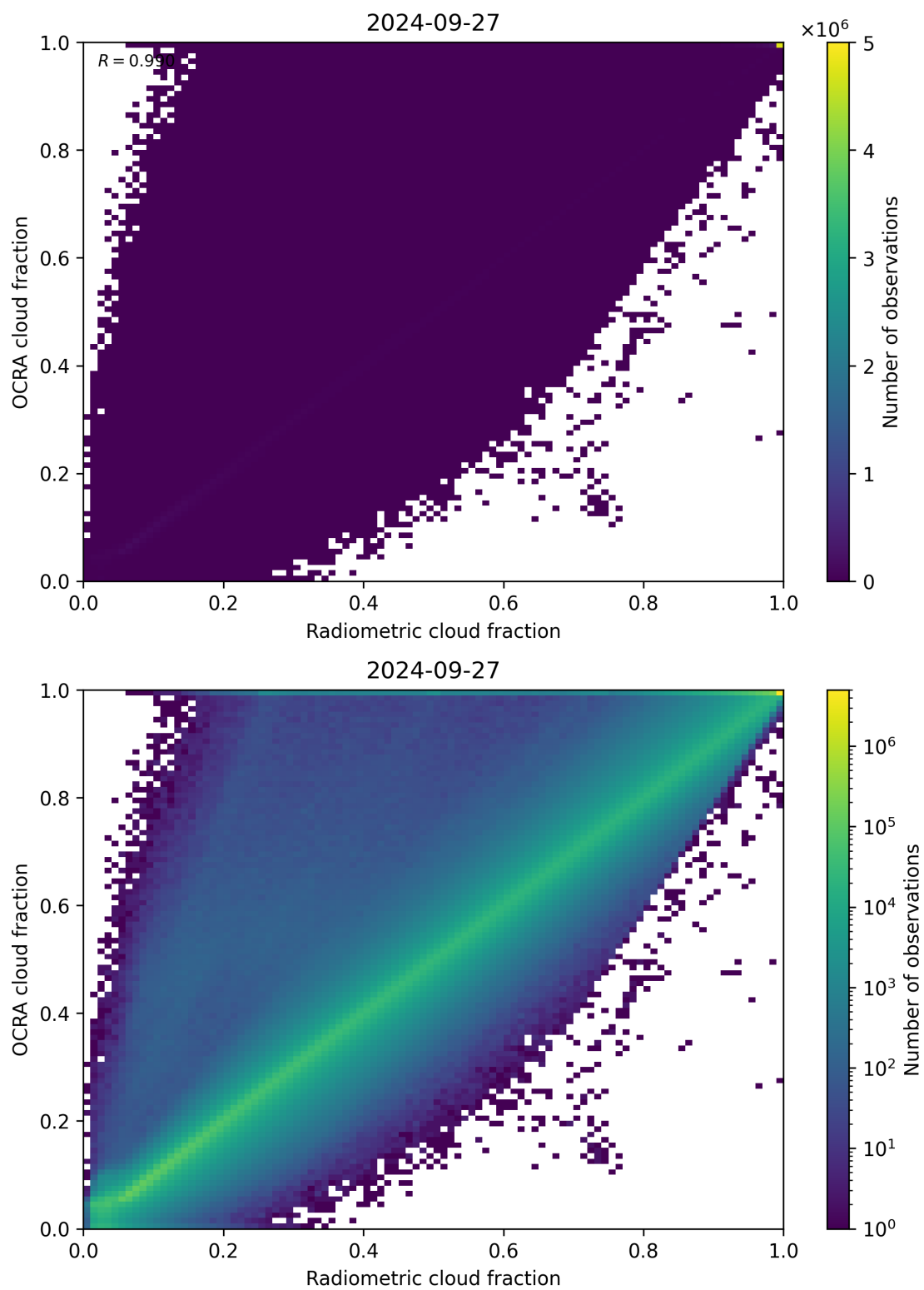
Figure 72: Scatter density plot of “Radiometric cloud fraction” against “OCRA cloud fraction” for 2024-09-26 to 2024-09-28.
