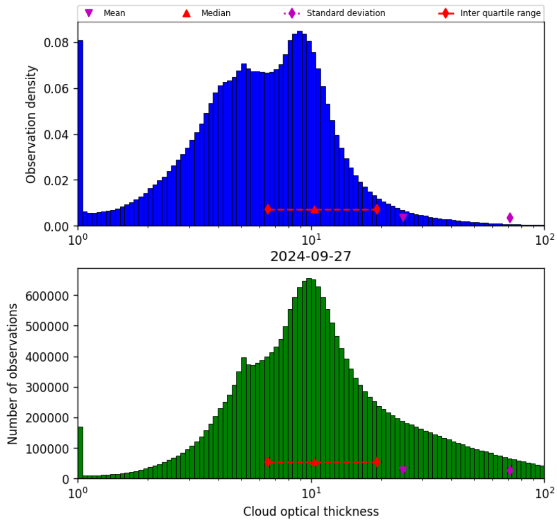
Figure 41: Histogram of “Cloud optical thickness” for 2024-09-26 to 2024-09-28
