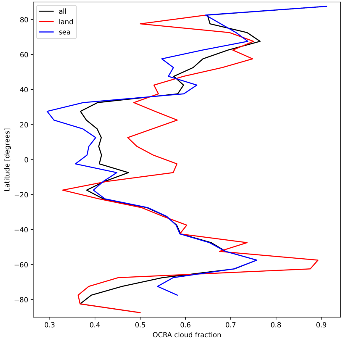
Figure 34: Zonal average of “OCRA cloud fraction” for 2024-09-26 to 2024-09-28.
