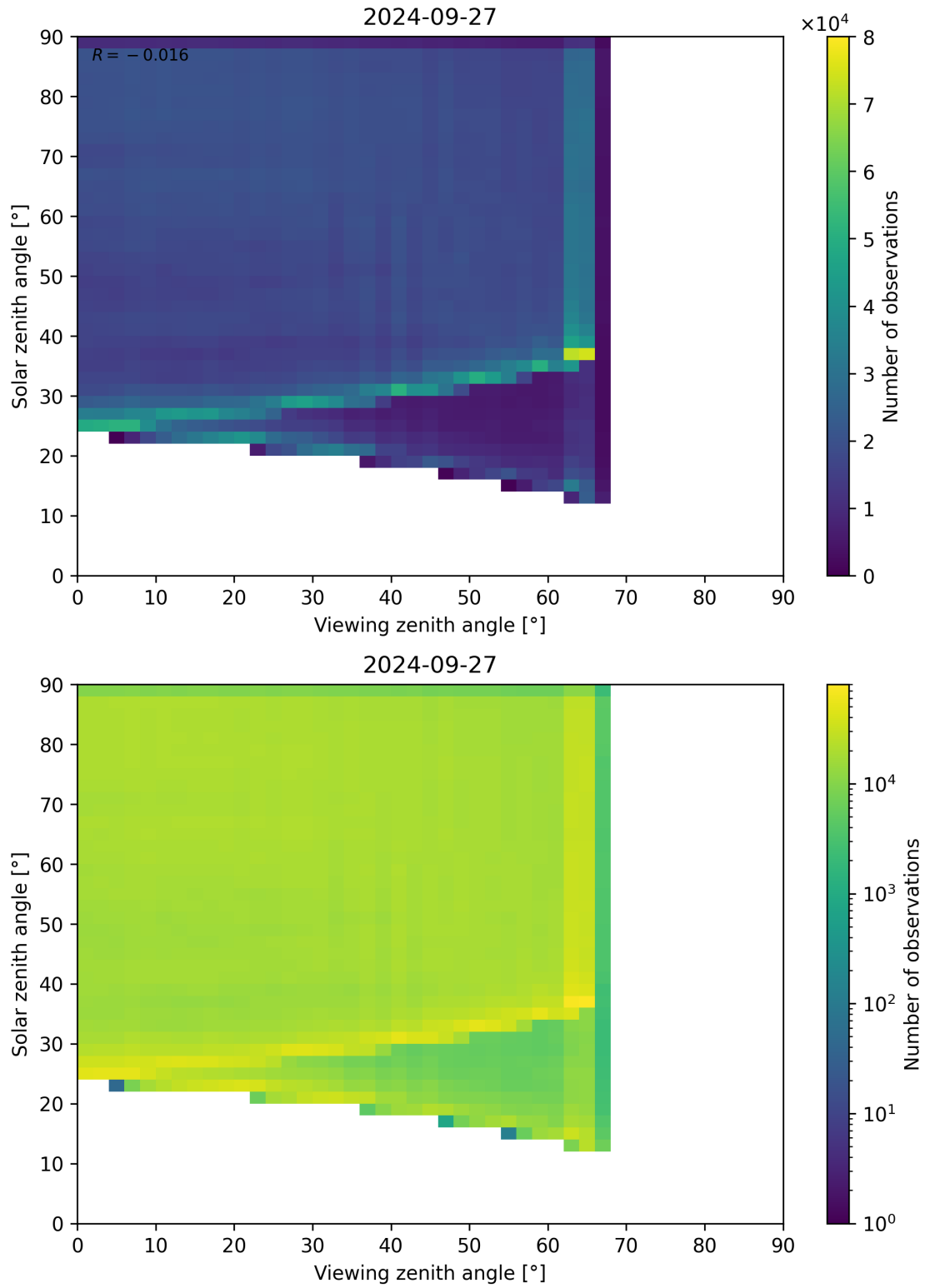
Figure 114: Scatter density plot of “Viewing zenith angle” against “Solar zenith angle” for 2024-09-26 to 2024-09-28.
