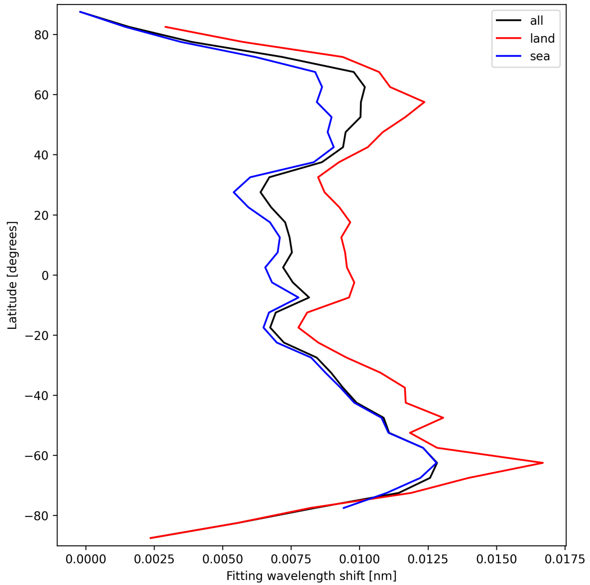
Figure 33: Zonal average of “Fitting wavelength shift” for 2024-09-26 to 2024-09-28.
