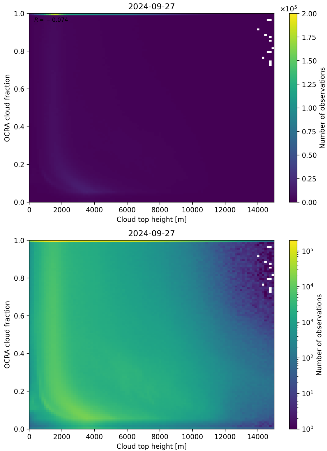
Figure 87: Scatter density plot of “Cloud top height” against “OCRA cloud fraction” for 2024-09-26 to 2024-09-28.
