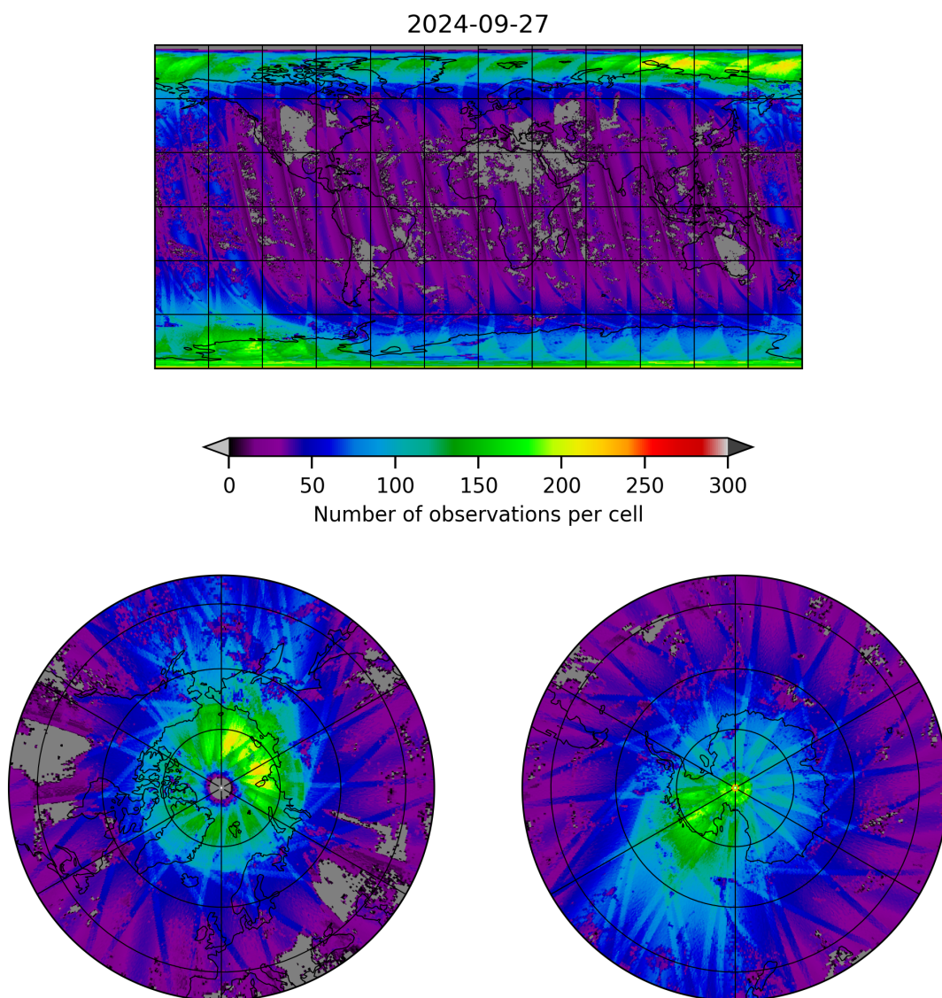
Figure 21: Map of the number of observations for 2024-09-26 to 2024-09-28
