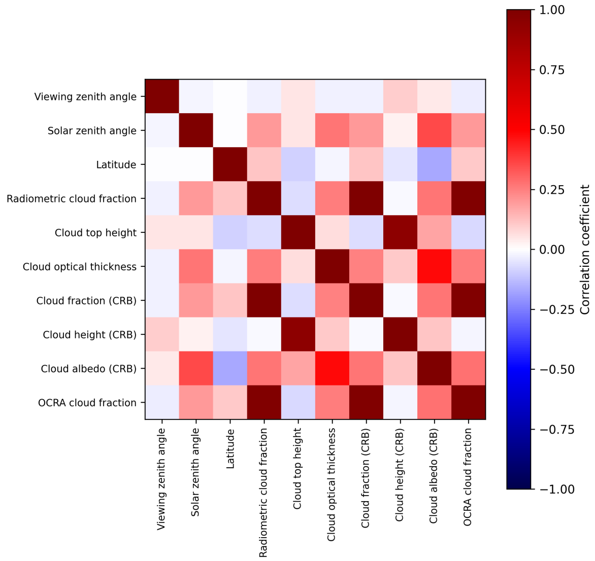
Figure 2: Map of correlation matrix for 2024-09-26 to 2024-09-28.
