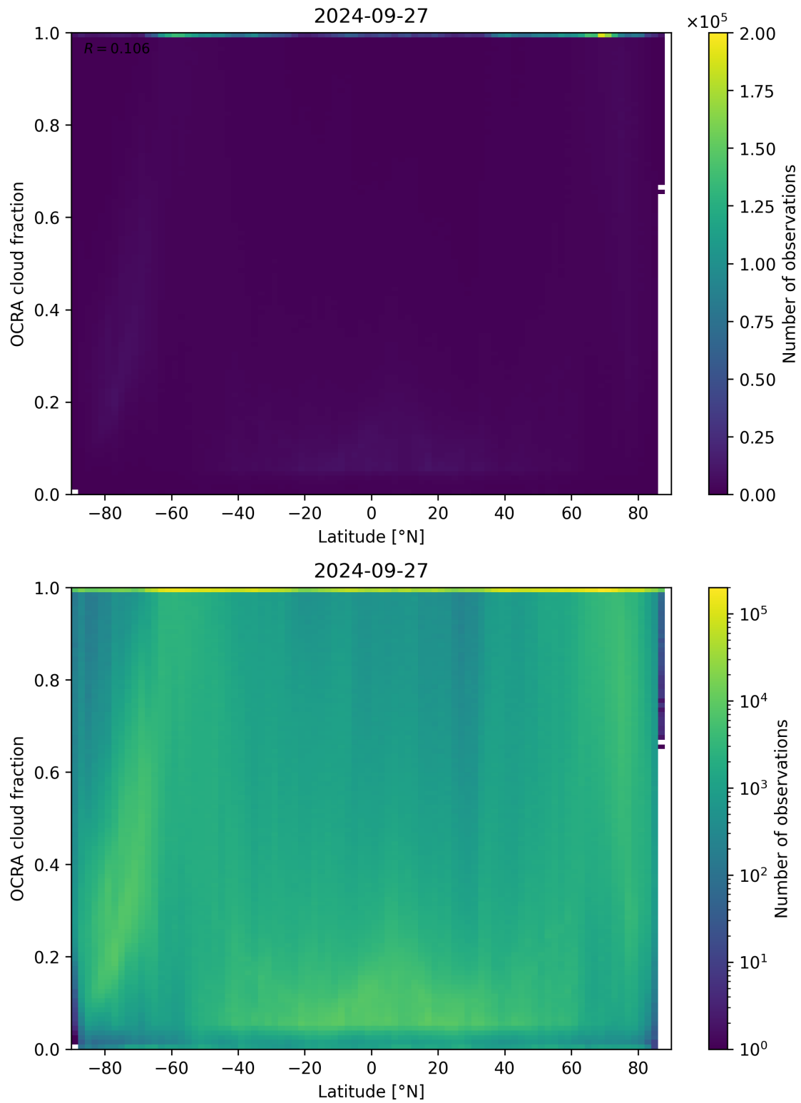
Figure 93: Scatter density plot of “Latitude” against “OCRA cloud fraction” for 2024-09-26 to 2024-09-28.
