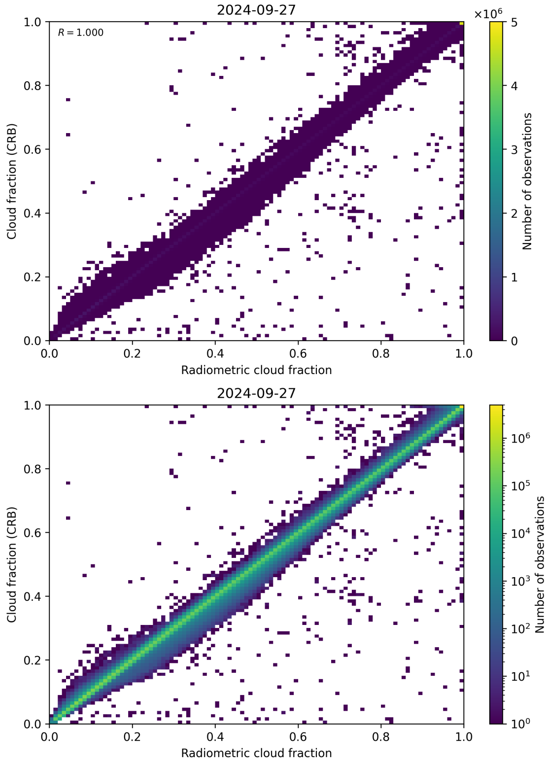
Figure 73: Scatter density plot of “Radiometric cloud fraction” against “Cloud fraction (CRB)” for 2024-09-26 to 2024-09-28.
