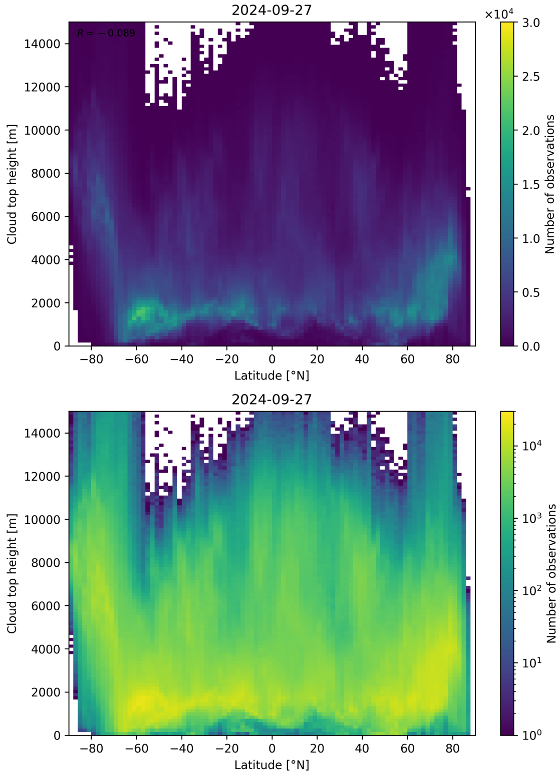
Figure 97: Scatter density plot of “Latitude” against “Cloud top height” for 2024-09-26 to 2024-09-28.
