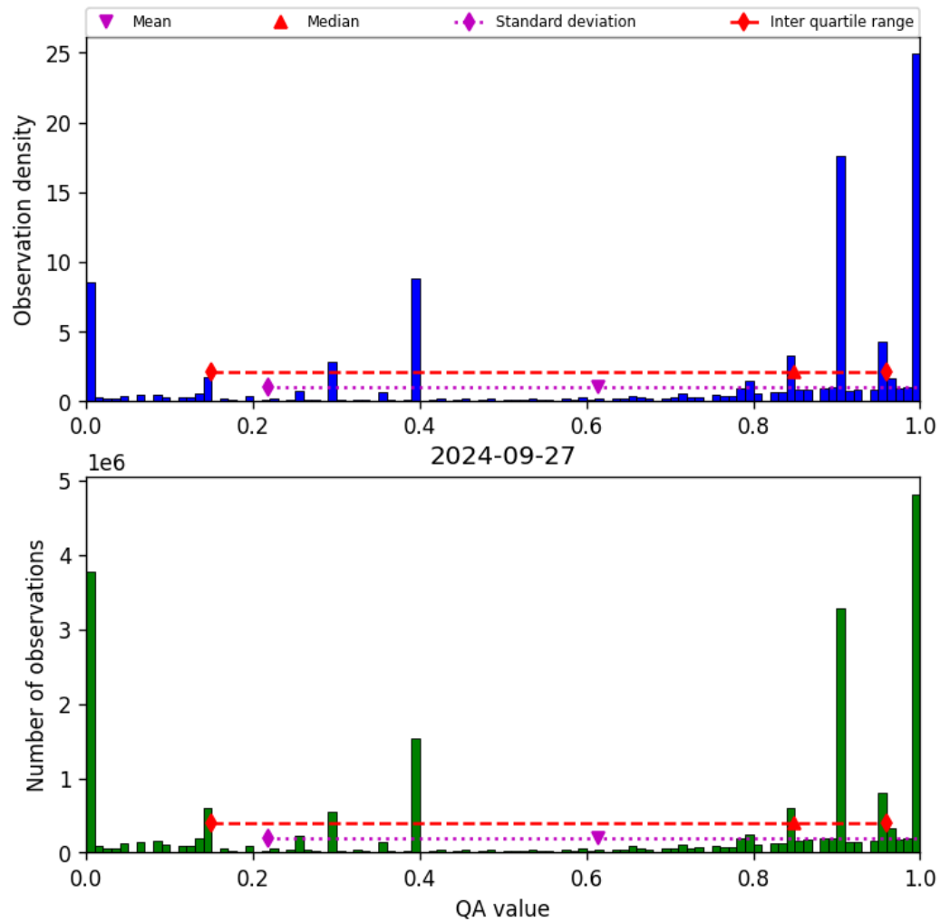
Figure 38: Histogram of “QA value” for 2024-09-26 to 2024-09-28
