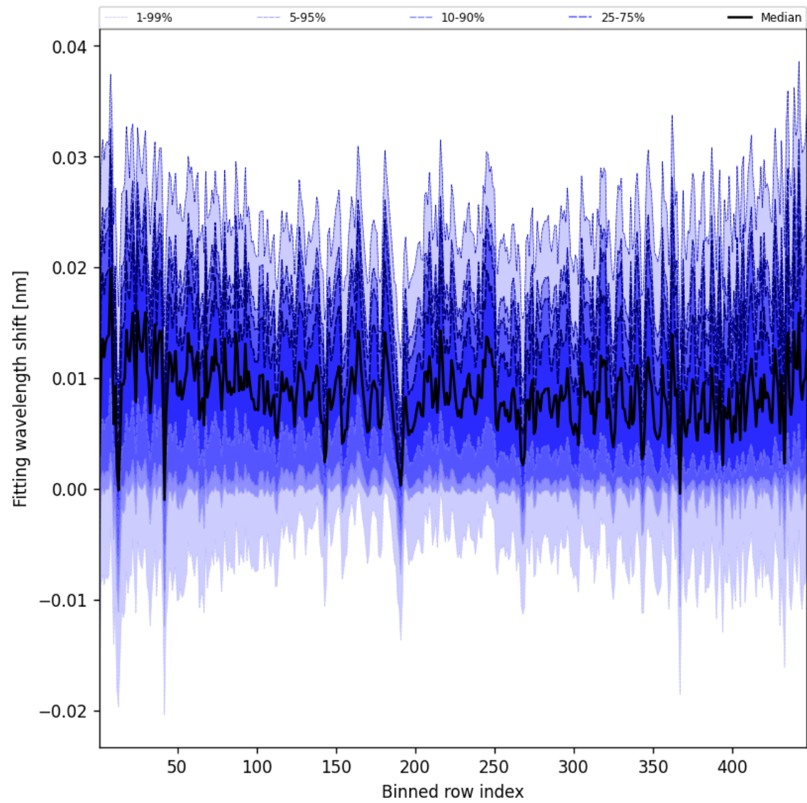
Figure 65: Along track statistics of “Fitting wavelength shift” for 2024-09-26 to 2024-09-28
