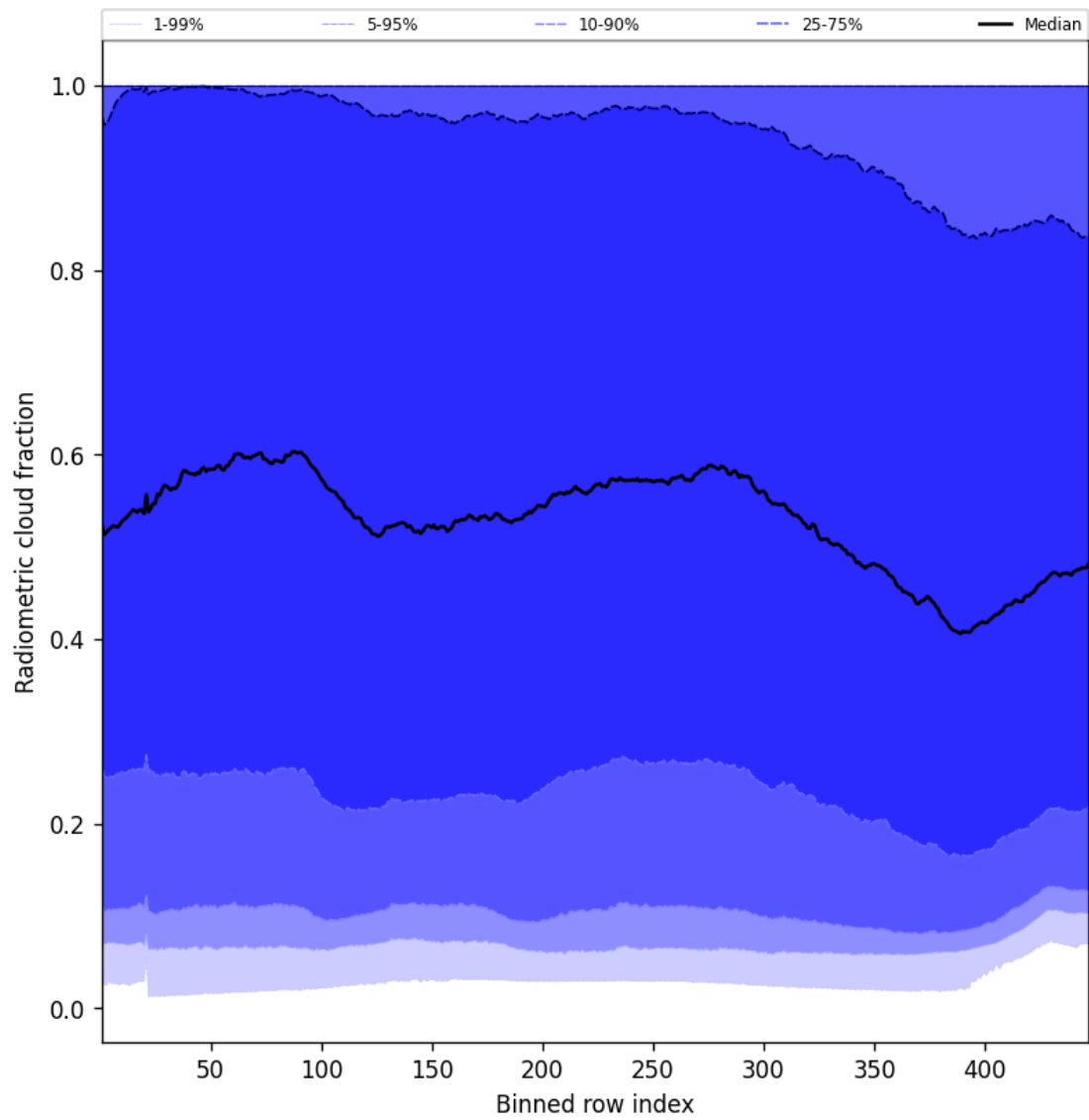
Figure 55: Along track statistics of “Radiometric cloud fraction” for 2024-09-26 to 2024-09-28
