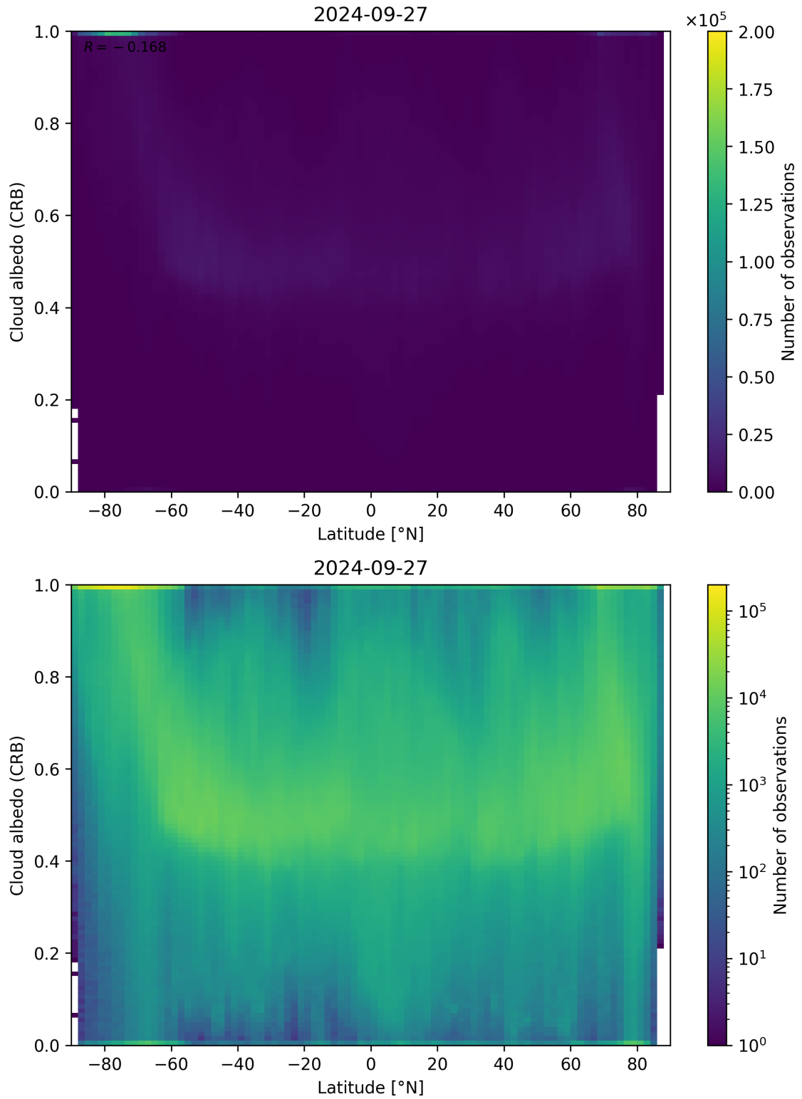
Figure 91: Scatter density plot of “Latitude” against “Cloud albedo (CRB)” for 2024-09-26 to 2024-09-28.
