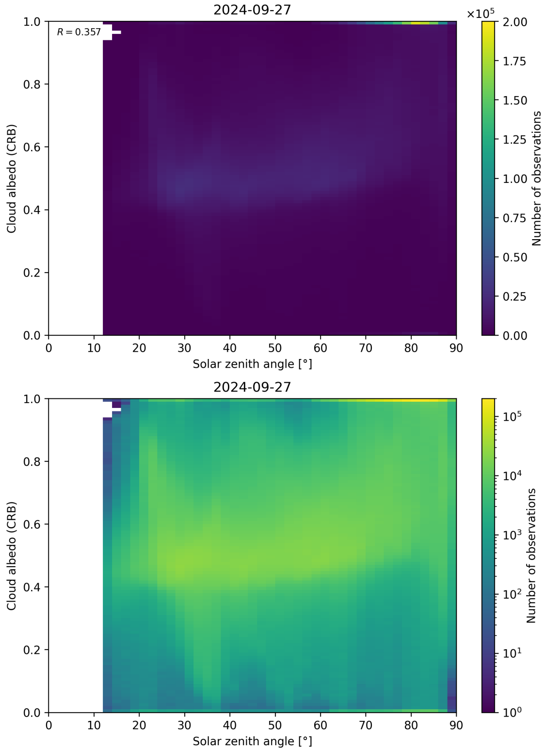
Figure 98: Scatter density plot of “Solar zenith angle” against “Cloud albedo (CRB)” for 2024-09-26 to 2024-09-28.
