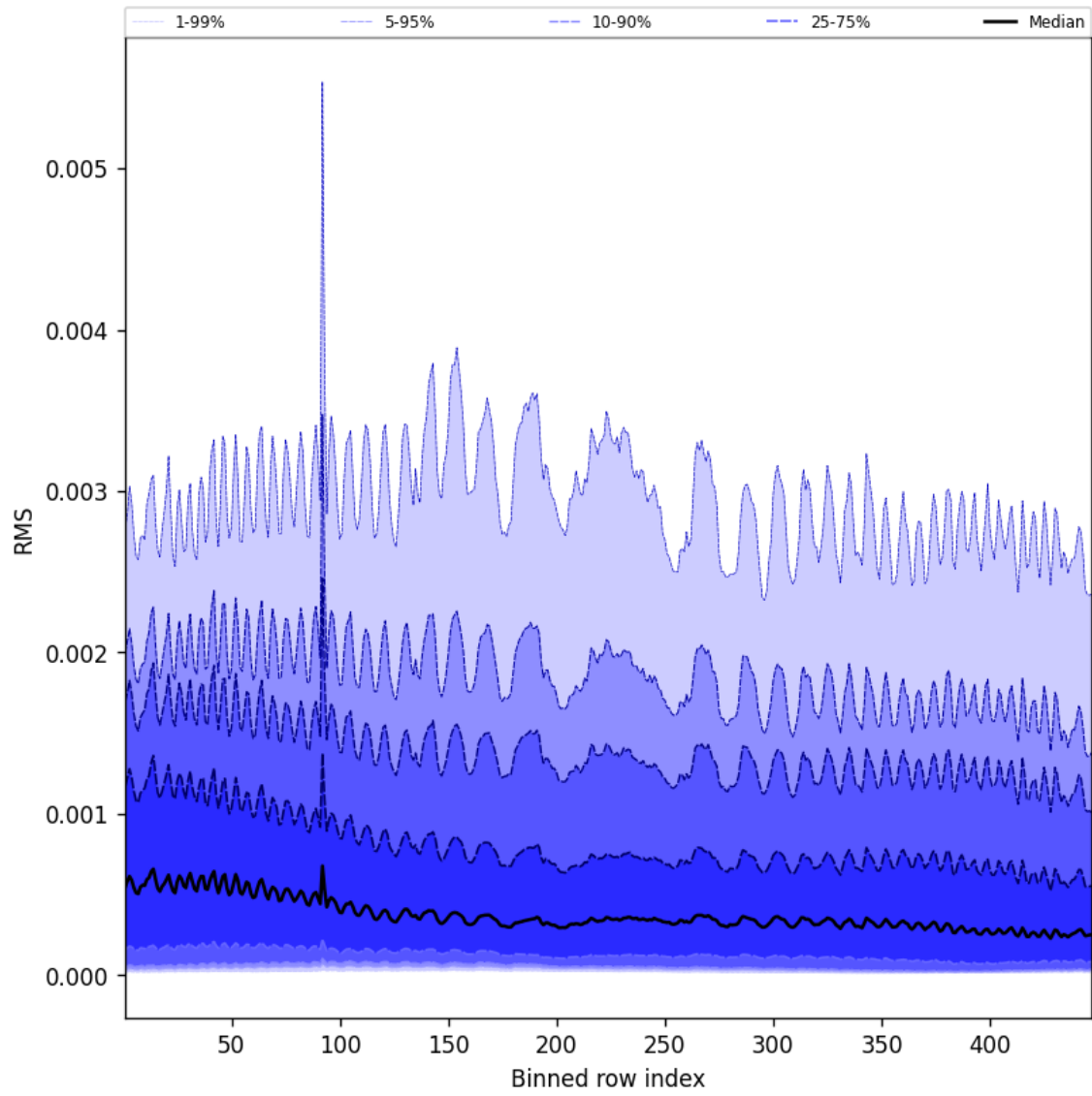
Figure 63: Along track statistics of “RMS” for 2024-09-26 to 2024-09-28
