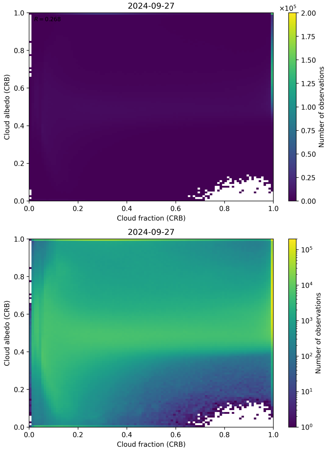
Figure 77: Scatter density plot of “Cloud fraction (CRB)” against “Cloud albedo (CRB)” for 2024-09-26 to 2024-09-28.
