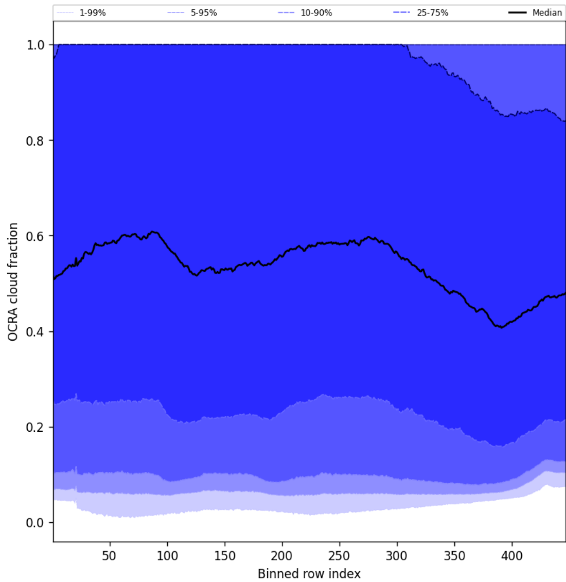
Figure 66: Along track statistics of “OCRA cloud fraction” for 2024-09-26 to 2024-09-28
