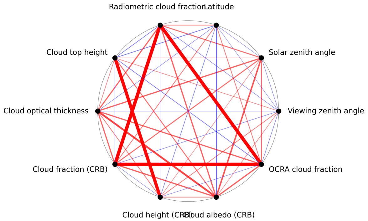
Figure 1: Map of correlation graph for 2024-09-26 to 2024-09-28.
