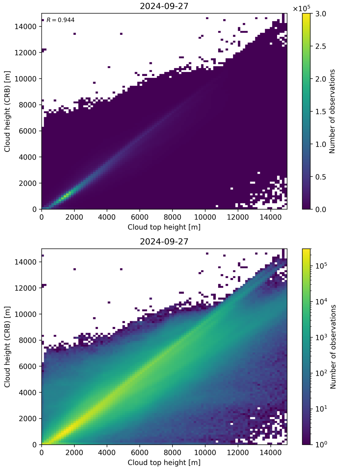
Figure 89: Scatter density plot of “Cloud top height” against “Cloud height (CRB)” for 2024-09-26 to 2024-09-28.
