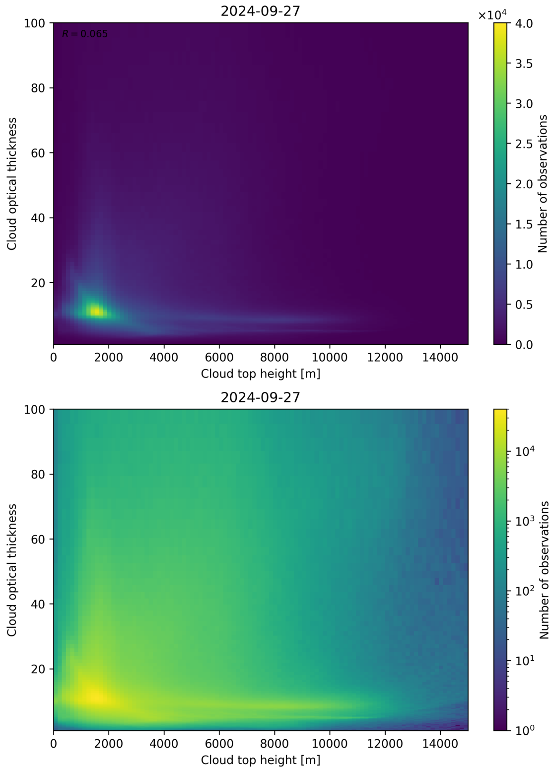
Figure 90: Scatter density plot of “Cloud top height” against “Cloud optical thickness” for 2024-09-26 to 2024-09-28.
