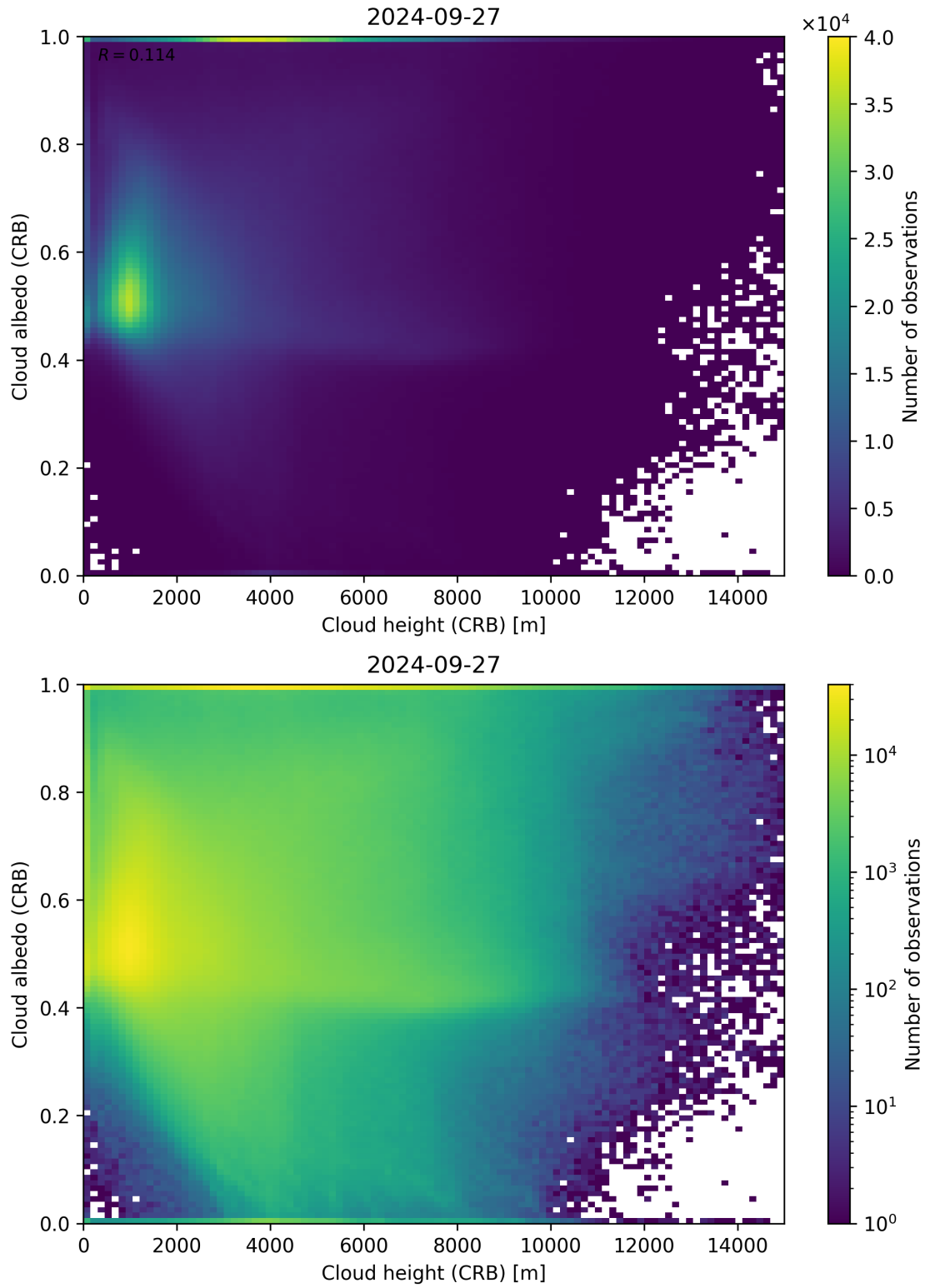
Figure 80: Scatter density plot of “Cloud height (CRB)” against “Cloud albedo (CRB)” for 2024-09-26 to 2024-09-28.
