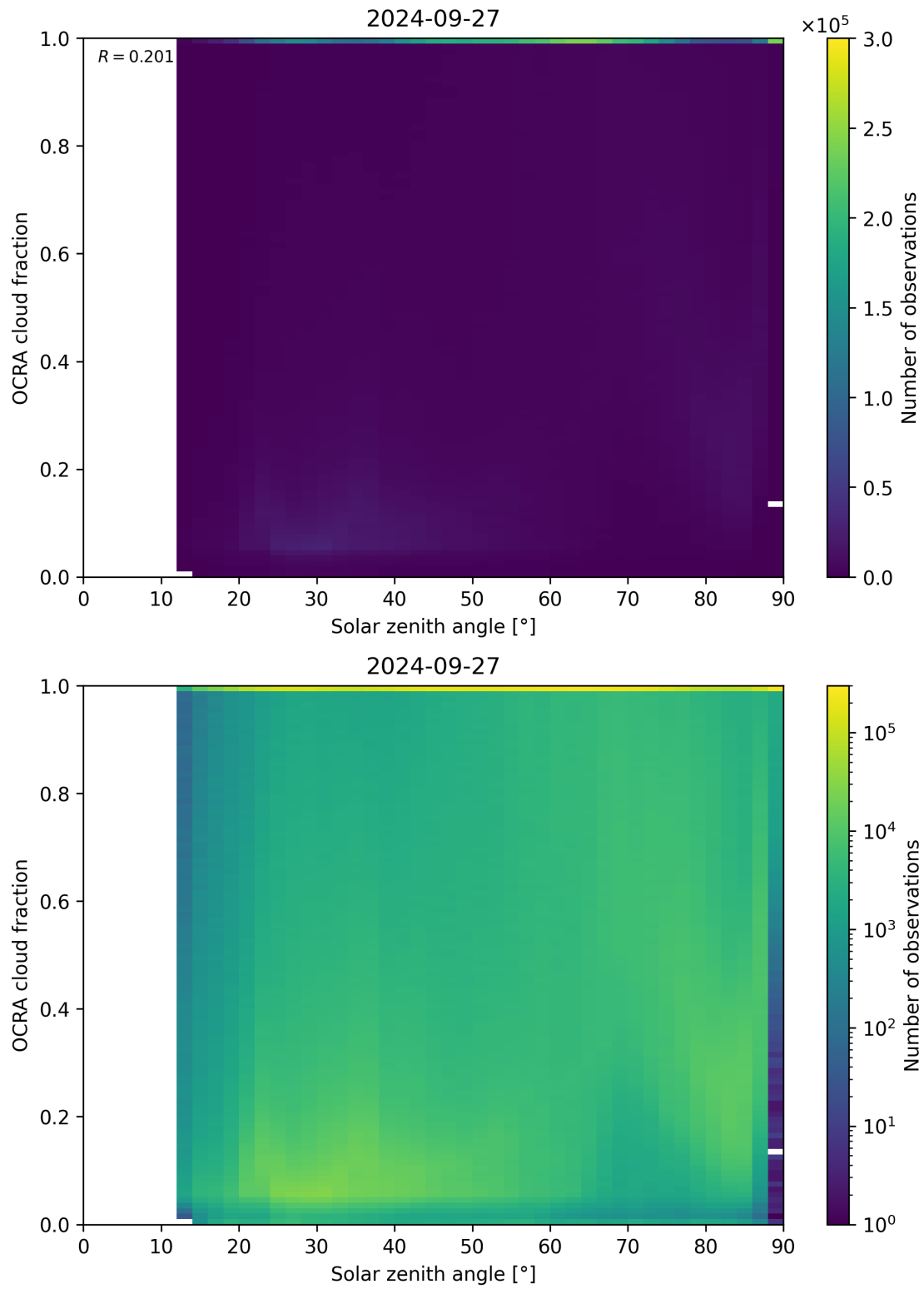
Figure 100: Scatter density plot of “Solar zenith angle” against “OCRA cloud fraction” for 2024-09-26 to 2024-09-28.
