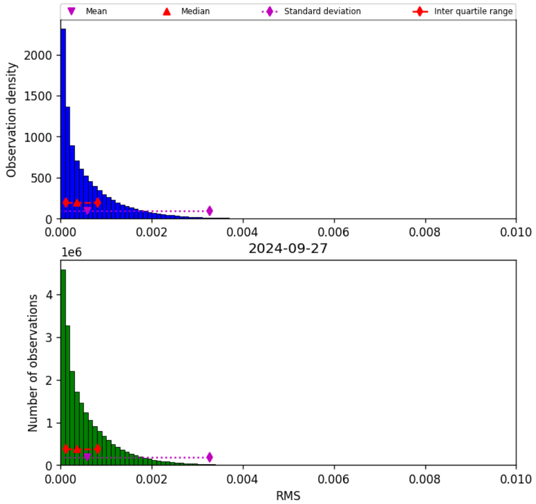
Figure 47: Histogram of “RMS” for 2024-09-26 to 2024-09-28
