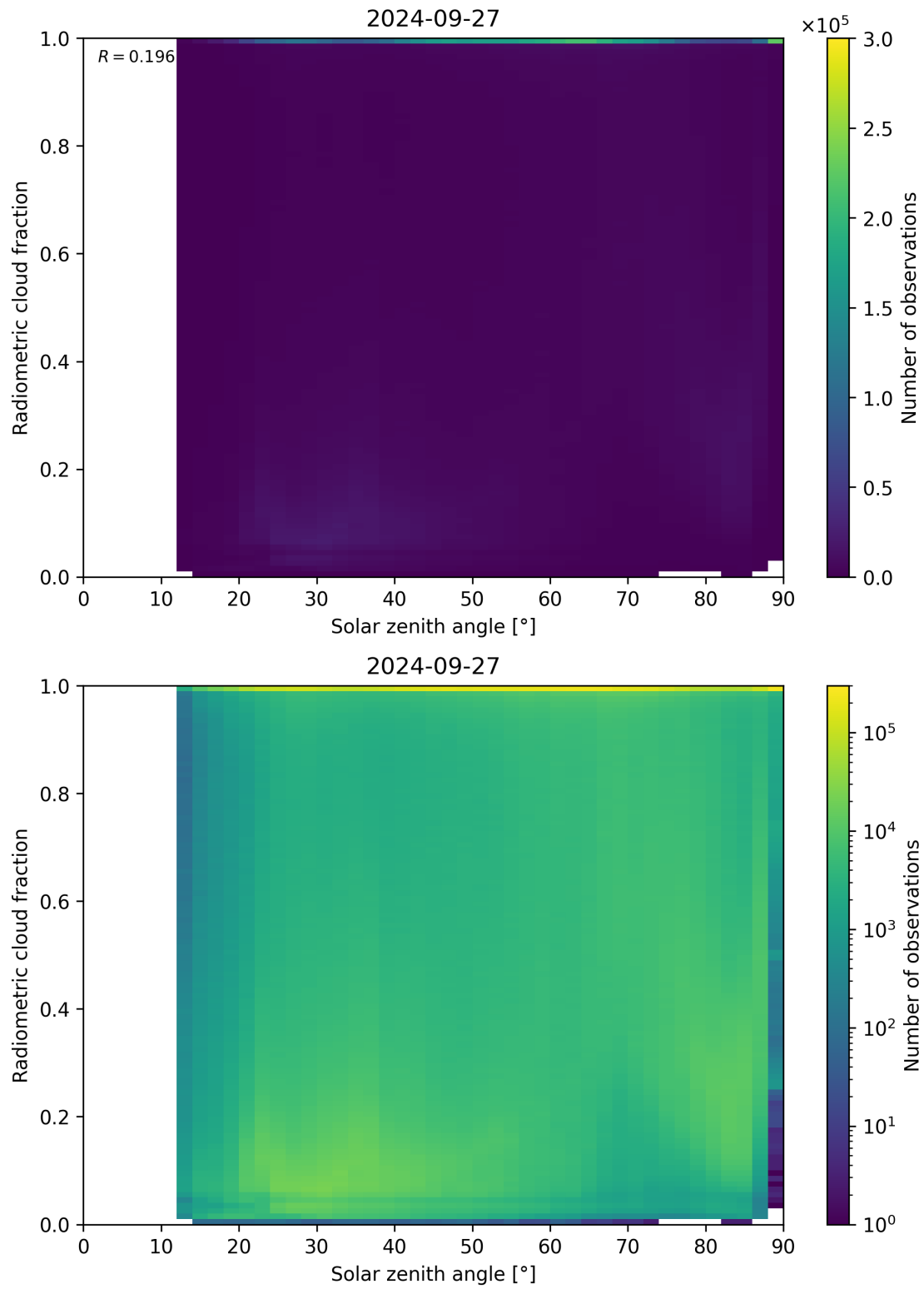
Figure 99: Scatter density plot of “Solar zenith angle” against “Radiometric cloud fraction” for 2024-09-26 to 2024-09-28.
