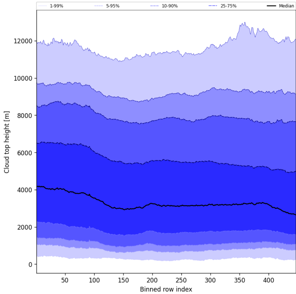
Figure 56: Along track statistics of “Cloud top height” for 2024-09-26 to 2024-09-28
