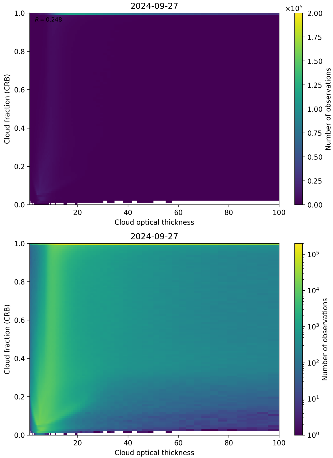
Figure 84: Scatter density plot of “Cloud optical thickness” against “Cloud fraction (CRB)” for 2024-09-26 to 2024-09-28.
