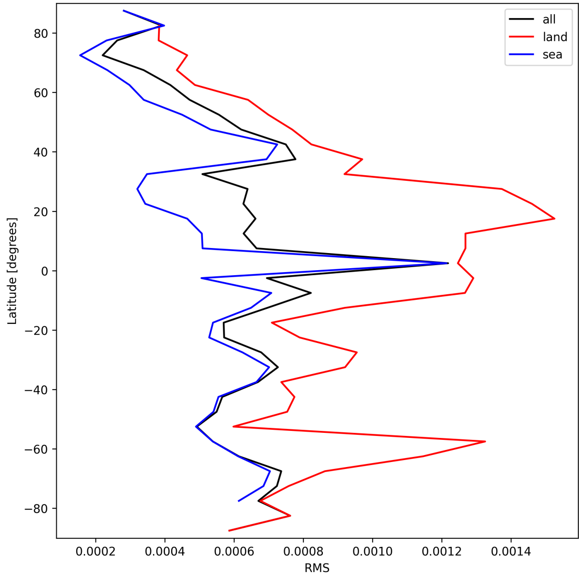
Figure 31: Zonal average of “RMS” for 2024-09-26 to 2024-09-28.
