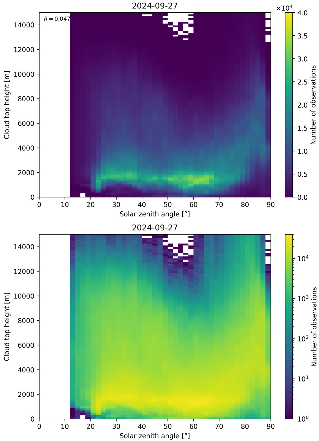
Figure 104: Scatter density plot of “Solar zenith angle” against “Cloud top height” for 2024-09-26 to 2024-09-28.
