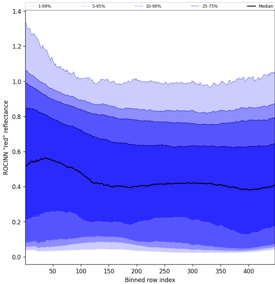
Figure 69: Along track statistics of “ROCINN “red” reflectance” for 2024-09-26 to 2024-09-28
