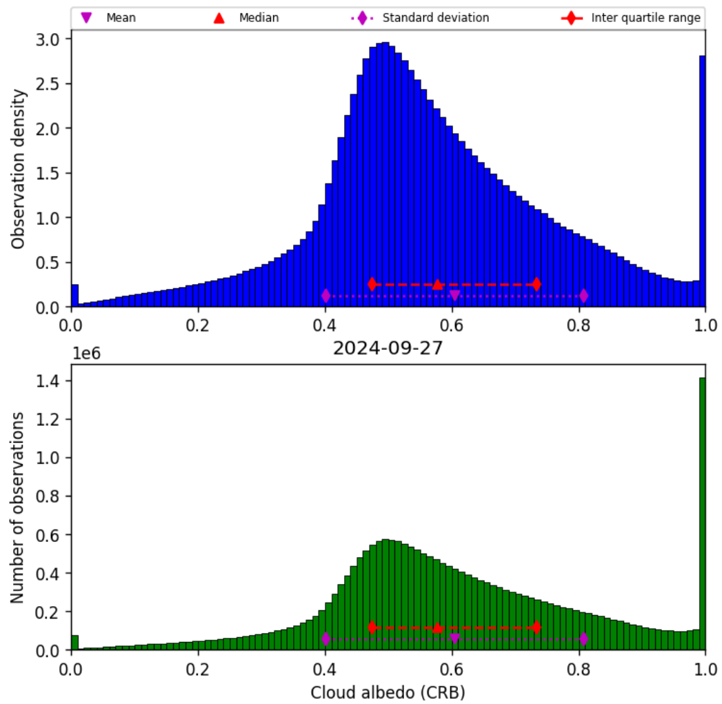
Figure 44: Histogram of “Cloud albedo (CRB)” for 2024-09-26 to 2024-09-28
