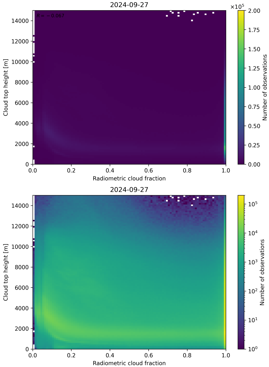
Figure 76: Scatter density plot of “Radiometric cloud fraction” against “Cloud top height” for 2024-09-26 to 2024-09-28.
