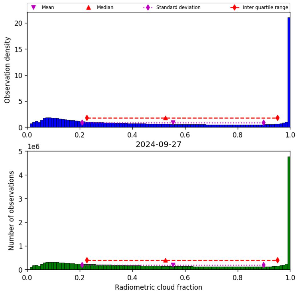
Figure 39: Histogram of “Radiometric cloud fraction” for 2024-09-26 to 2024-09-28
