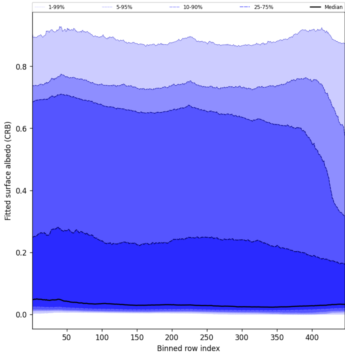
Figure 62: Along track statistics of “Fitted surface albedo (CRB)” for 2024-09-26 to 2024-09-28
