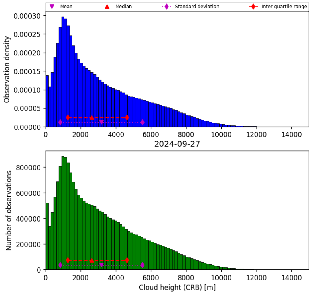
Figure 43: Histogram of “Cloud height (CRB)” for 2024-09-26 to 2024-09-28
