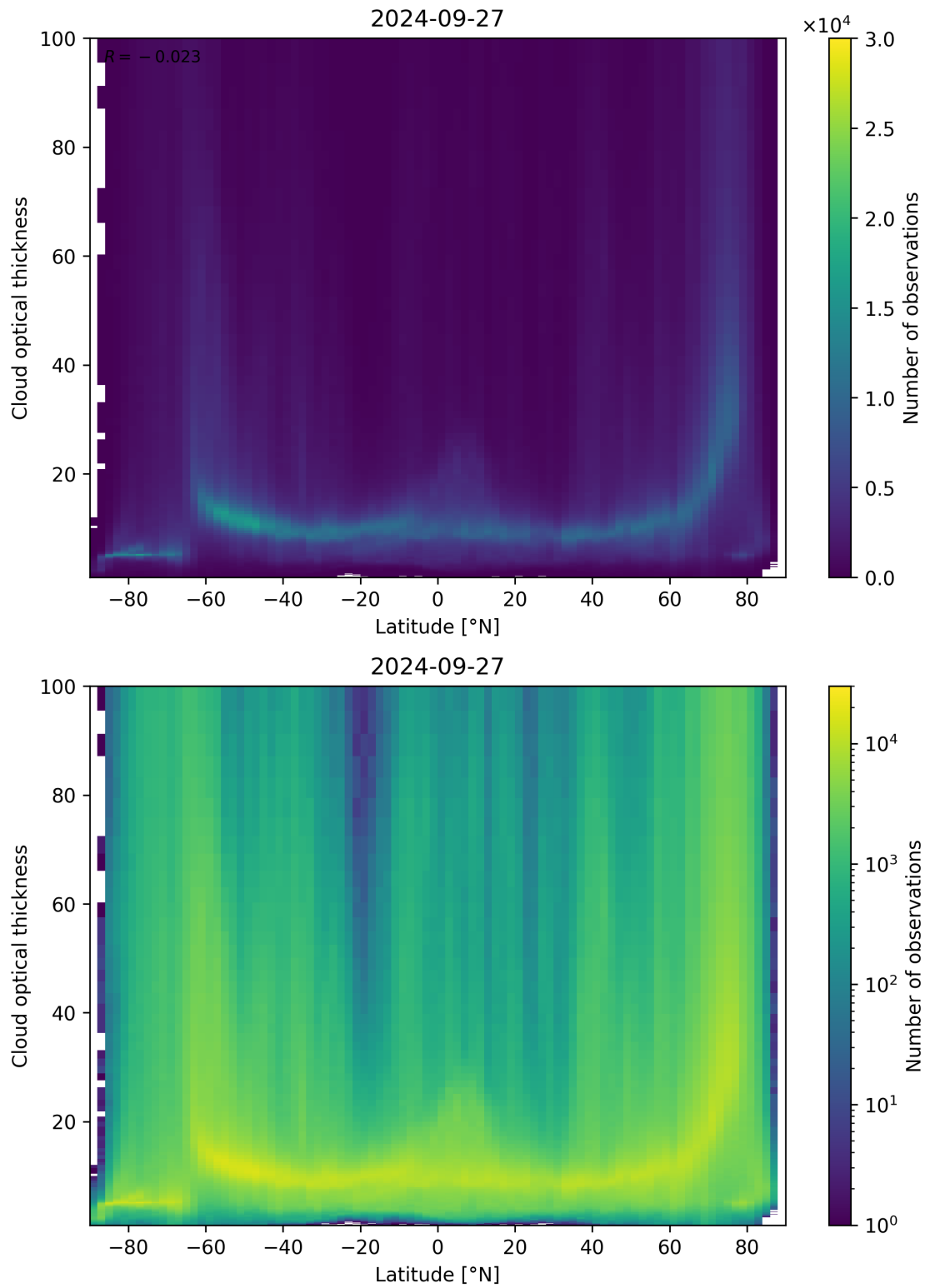
Figure 96: Scatter density plot of “Latitude” against “Cloud optical thickness” for 2024-09-26 to 2024-09-28.
