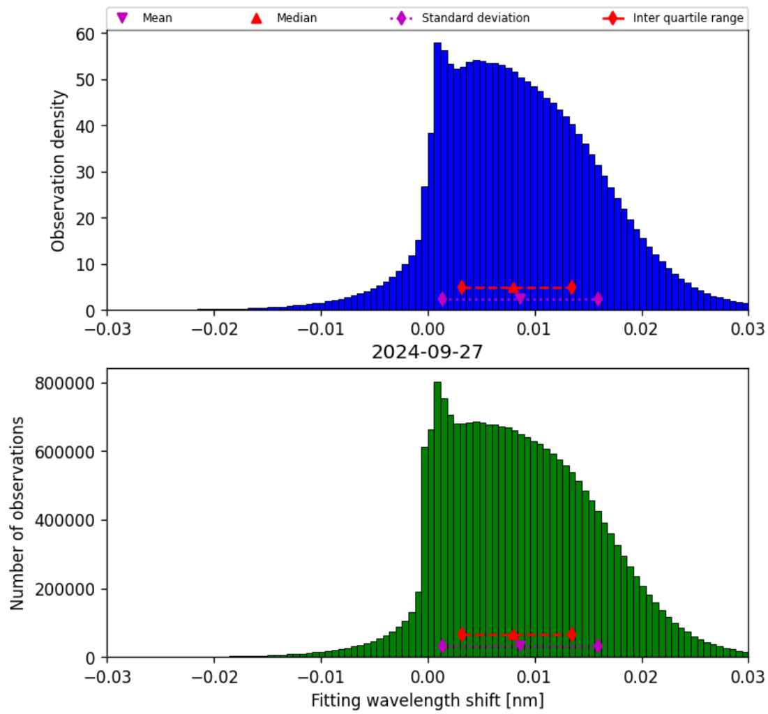
Figure 49: Histogram of “Fitting wavelength shift” for 2024-09-26 to 2024-09-28
