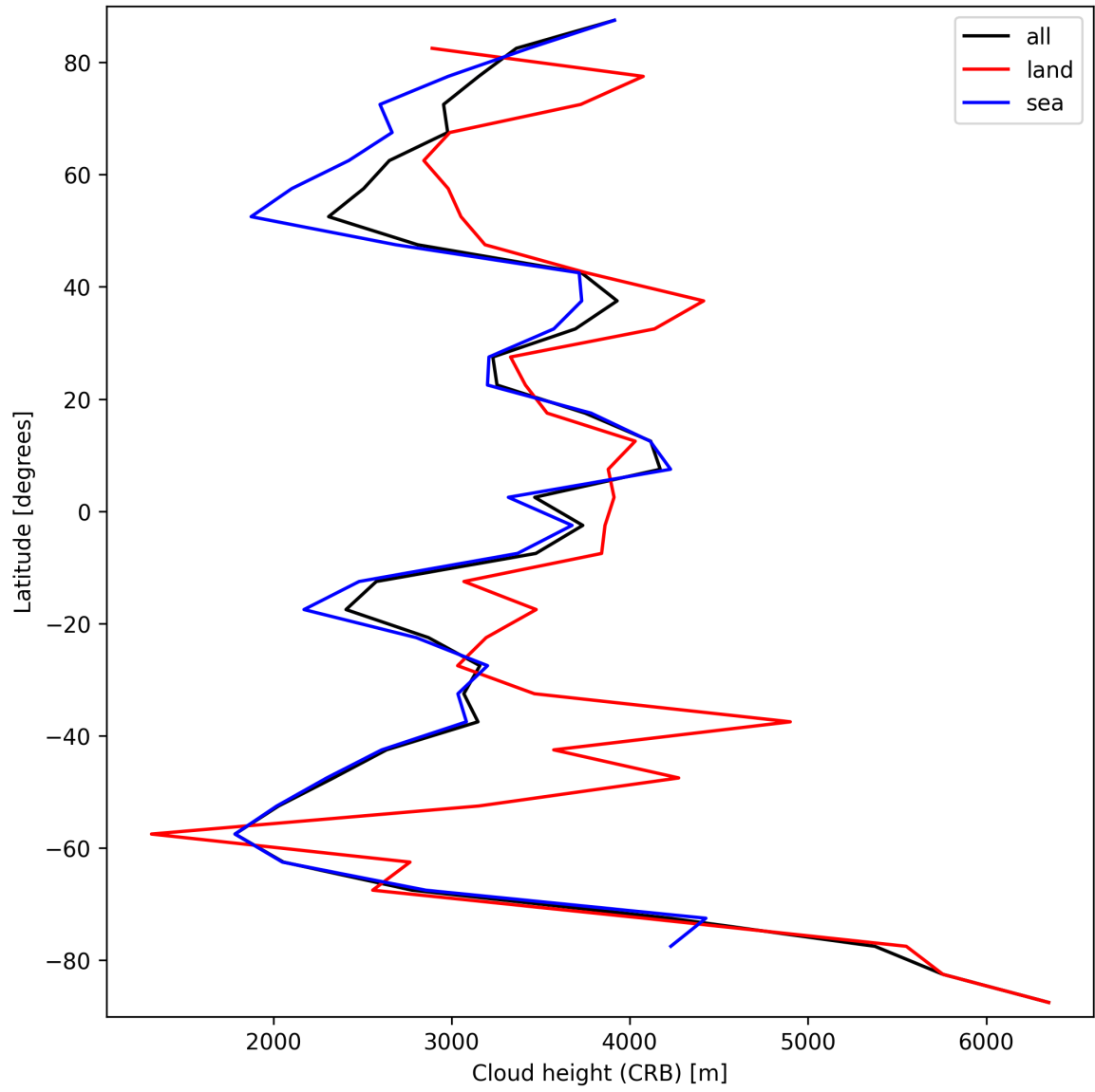
Figure 27: Zonal average of “Cloud height (CRB)” for 2024-09-26 to 2024-09-28.
