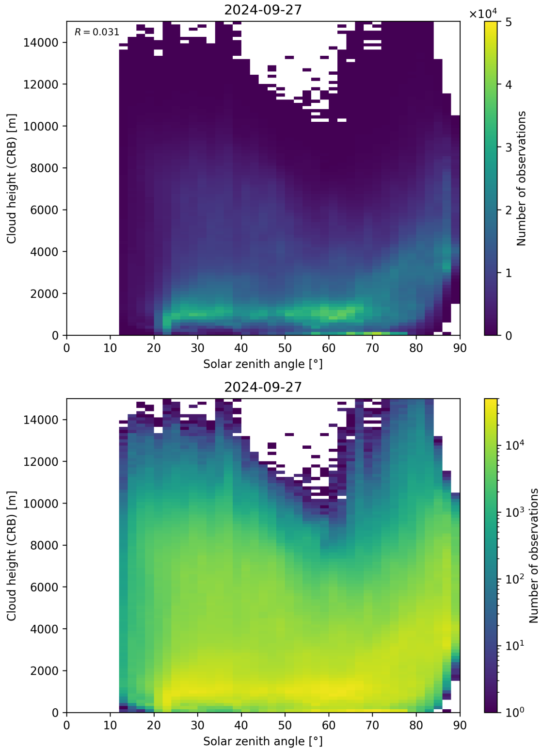
Figure 102: Scatter density plot of “Solar zenith angle” against “Cloud height (CRB)” for 2024-09-26 to 2024-09-28.
