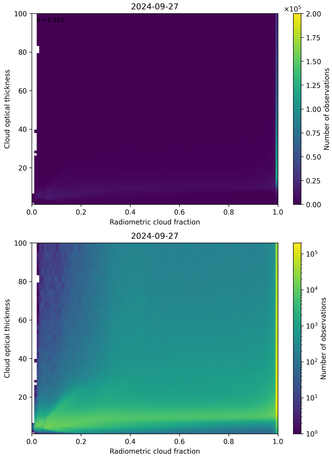
Figure 75: Scatter density plot of “Radiometric cloud fraction” against “Cloud optical thickness” for 2024-09-26 to 2024-09-28.
