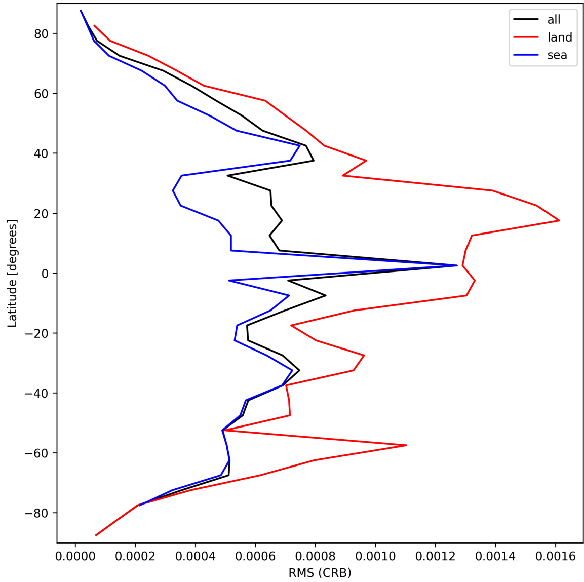
Figure 32: Zonal average of “RMS (CRB)” for 2024-09-26 to 2024-09-28.
