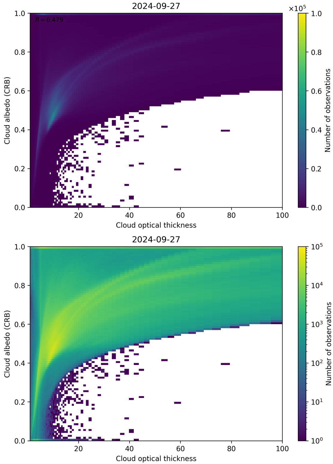
Figure 82: Scatter density plot of “Cloud optical thickness” against “Cloud albedo (CRB)” for 2024-09-26 to 2024-09-28.
