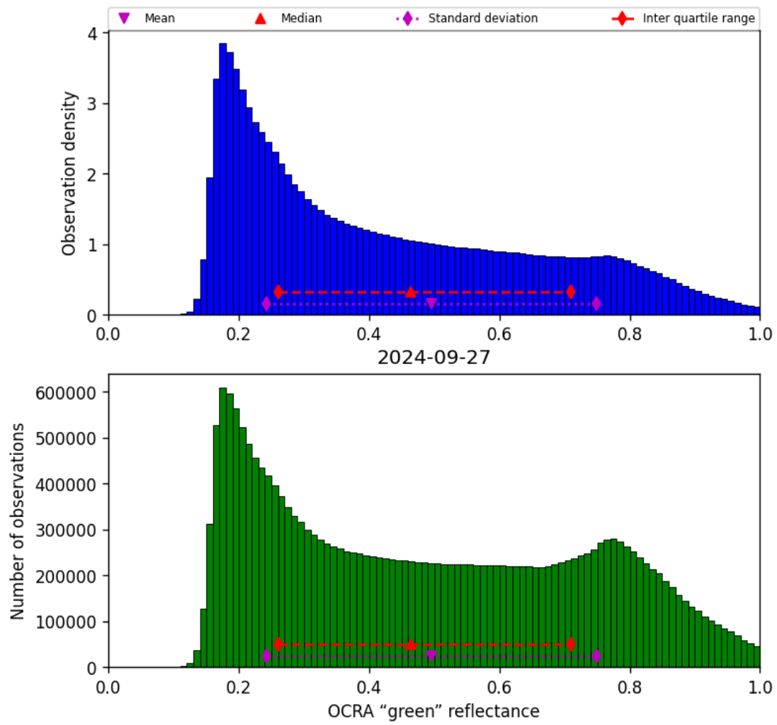
Figure 52: Histogram of “OCRA “green” reflectance” for 2024-09-26 to 2024-09-28
