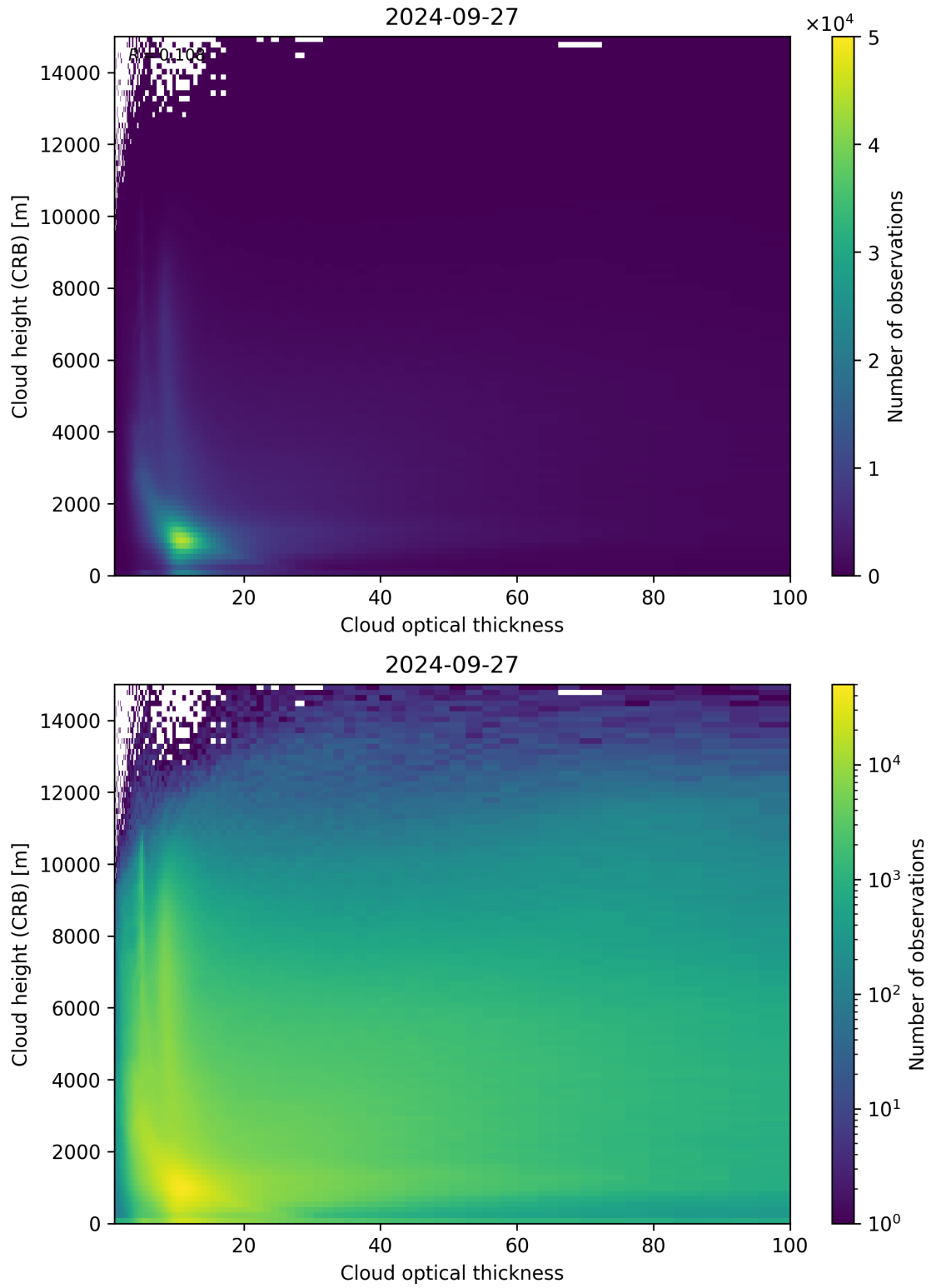
Figure 85: Scatter density plot of “Cloud optical thickness” against “Cloud height (CRB)” for 2024-09-26 to 2024-09-28.
