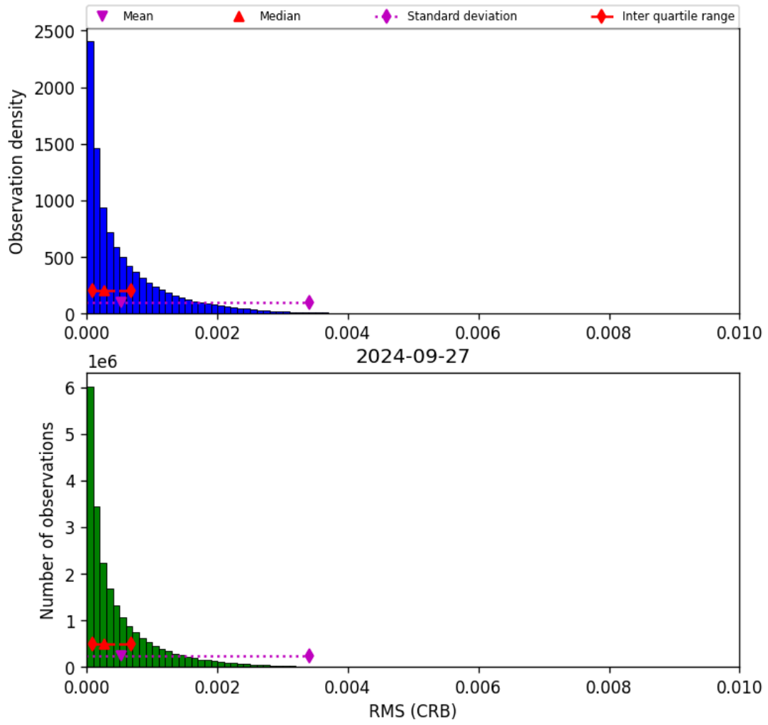
Figure 48: Histogram of “RMS (CRB)” for 2024-09-26 to 2024-09-28
