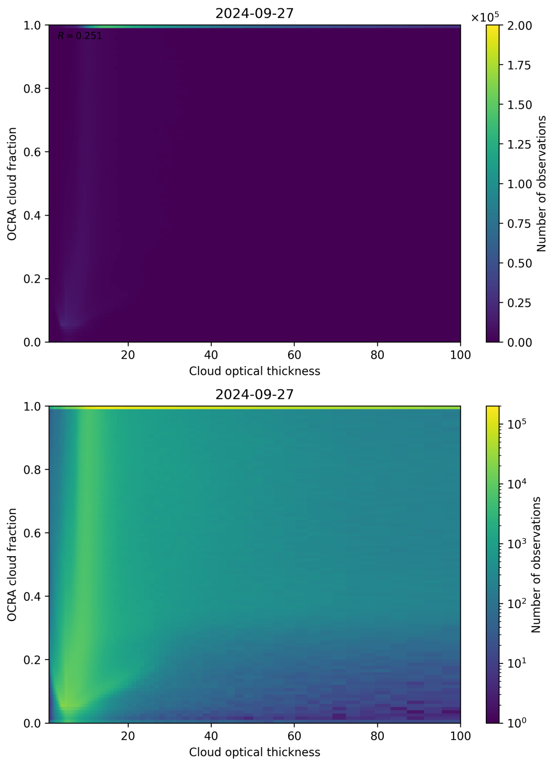
Figure 83: Scatter density plot of “Cloud optical thickness” against “OCRA cloud fraction” for 2024-09-26 to 2024-09-28.
