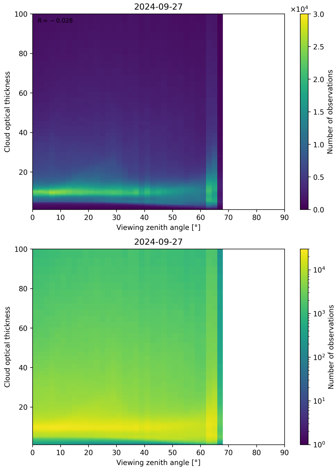
Figure 111: Scatter density plot of “Viewing zenith angle” against “Cloud optical thickness” for 2024-09-26 to 2024-09-28.
