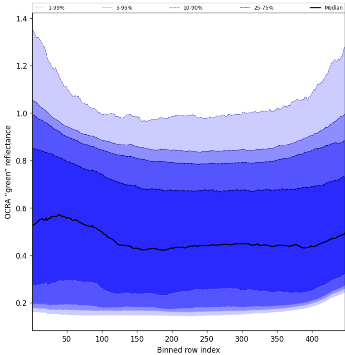
Figure 68: Along track statistics of “OCRA “green” reflectance” for 2024-09-26 to 2024-09-28
