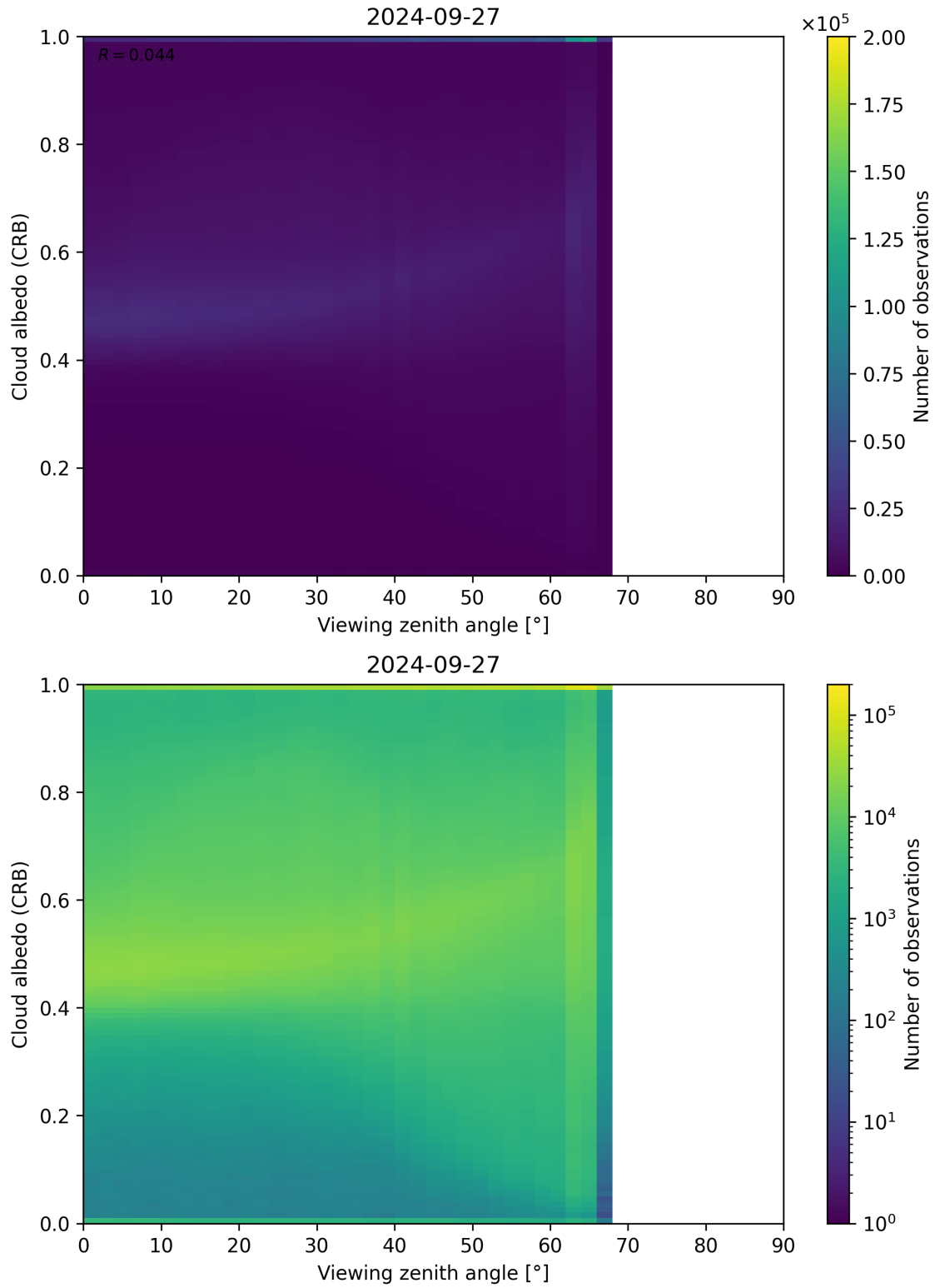
Figure 106: Scatter density plot of “Viewing zenith angle” against “Cloud albedo (CRB)” for 2024-09-26 to 2024-09-28.
