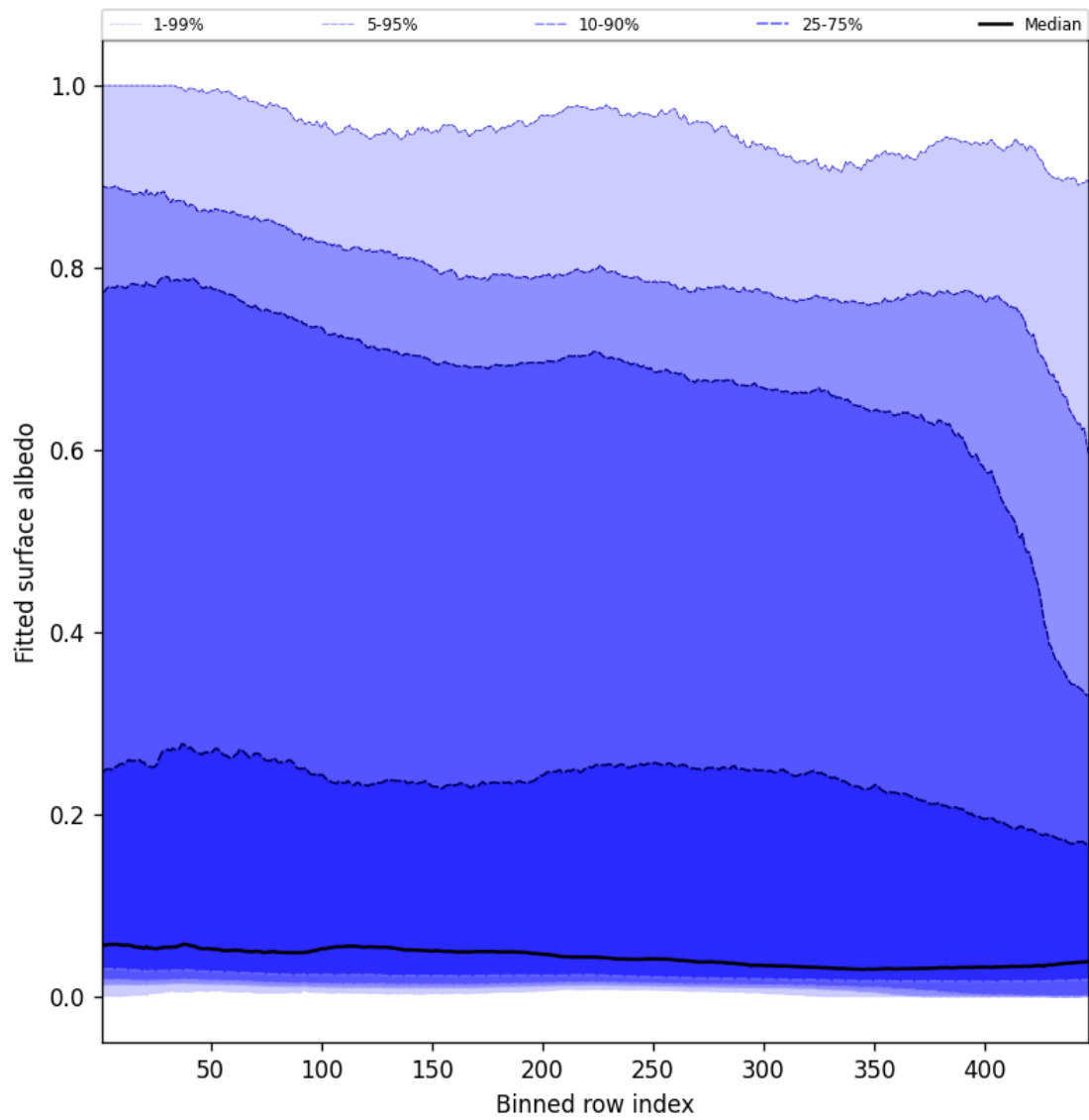
Figure 61: Along track statistics of “Fitted surface albedo” for 2024-09-26 to 2024-09-28
