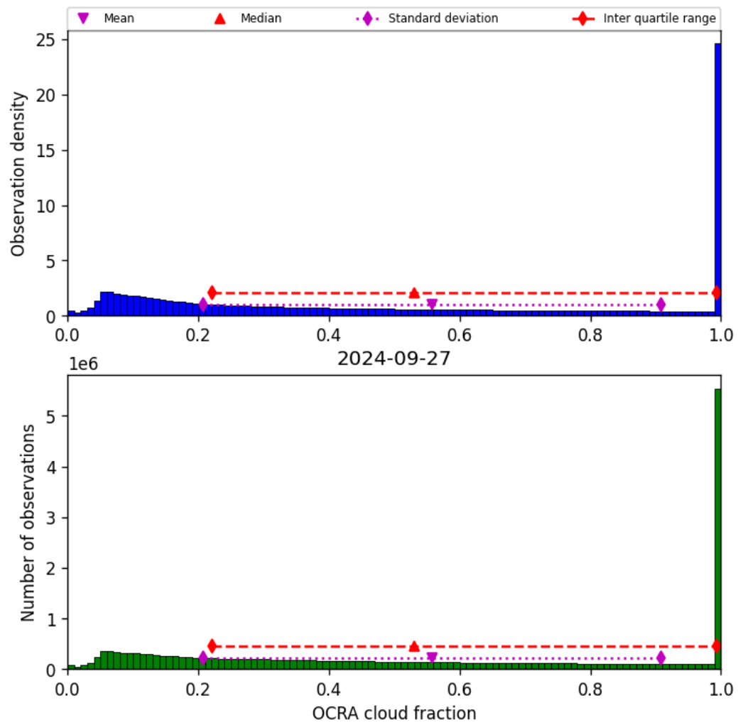
Figure 50: Histogram of “OCRA cloud fraction” for 2024-09-26 to 2024-09-28
