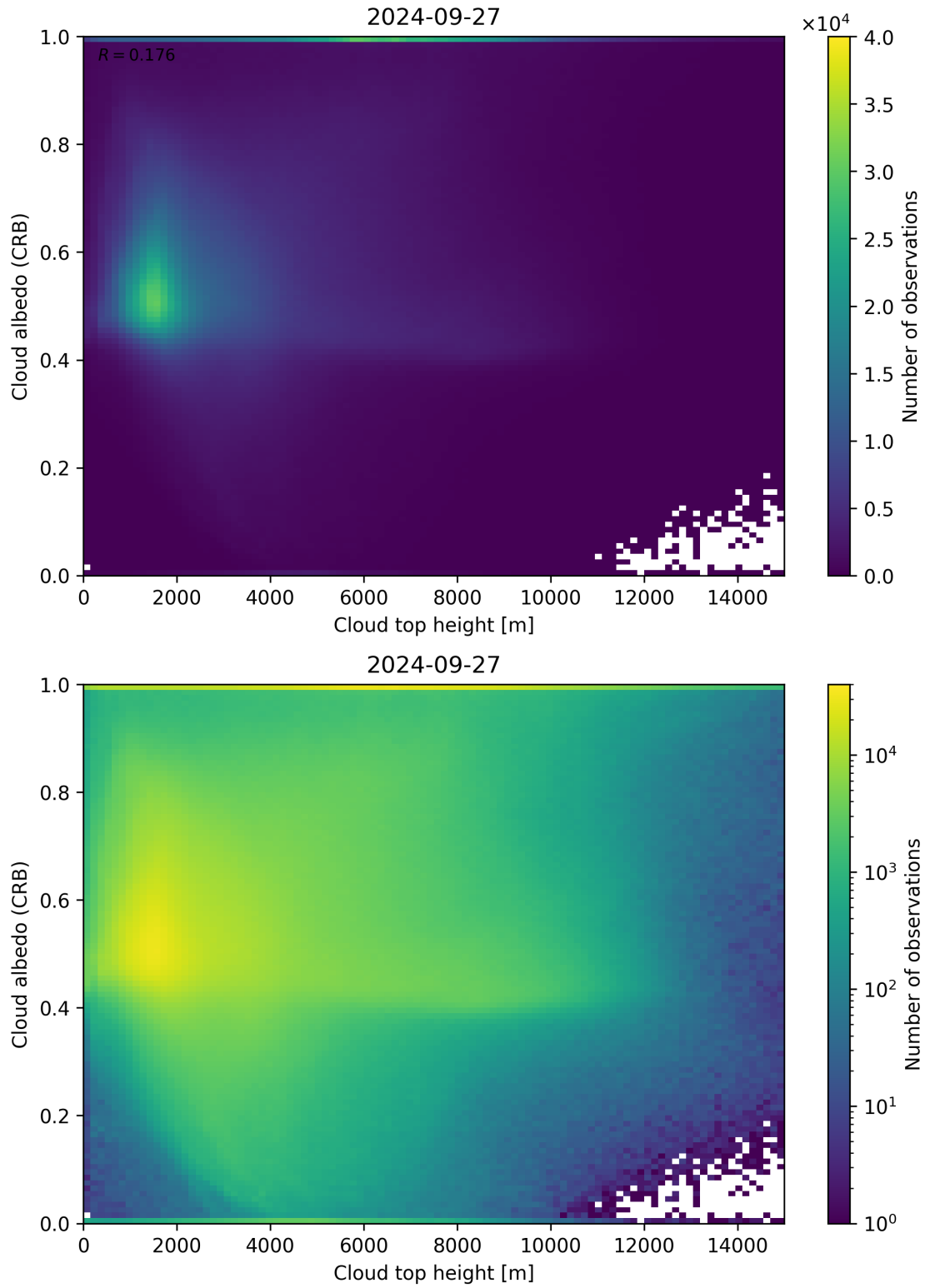
Figure 86: Scatter density plot of “Cloud top height” against “Cloud albedo (CRB)” for 2024-09-26 to 2024-09-28.
