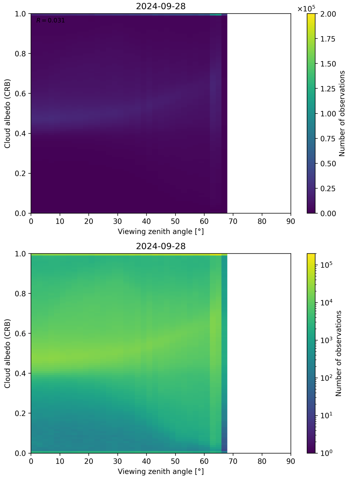
Figure 106: Scatter density plot of “Viewing zenith angle” against “Cloud albedo (CRB)” for 2024-09-28 to 2024-09-29.
