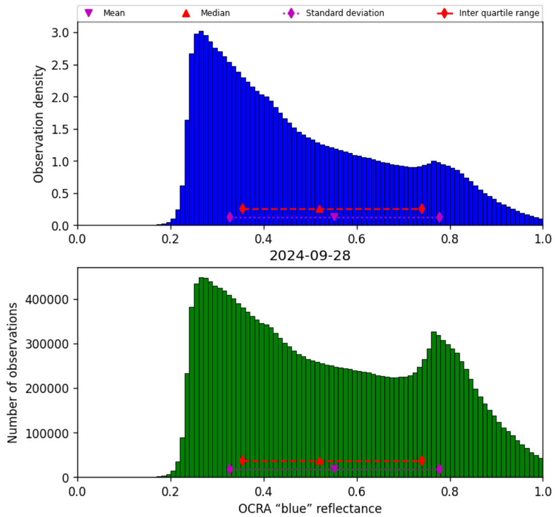
Figure 51: Histogram of “OCRA “blue” reflectance” for 2024-09-28 to 2024-09-29
