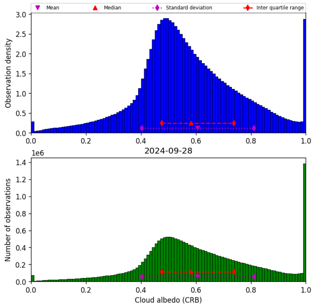
Figure 44: Histogram of “Cloud albedo (CRB)” for 2024-09-28 to 2024-09-29
