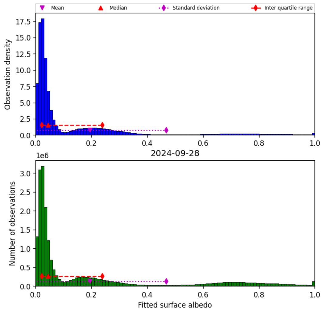
Figure 45: Histogram of “Fitted surface albedo” for 2024-09-28 to 2024-09-29
