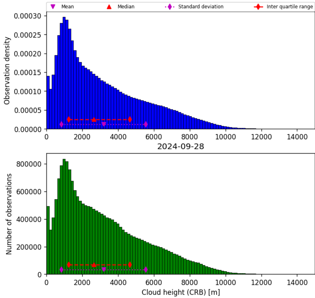
Figure 43: Histogram of “Cloud height (CRB)” for 2024-09-28 to 2024-09-29
