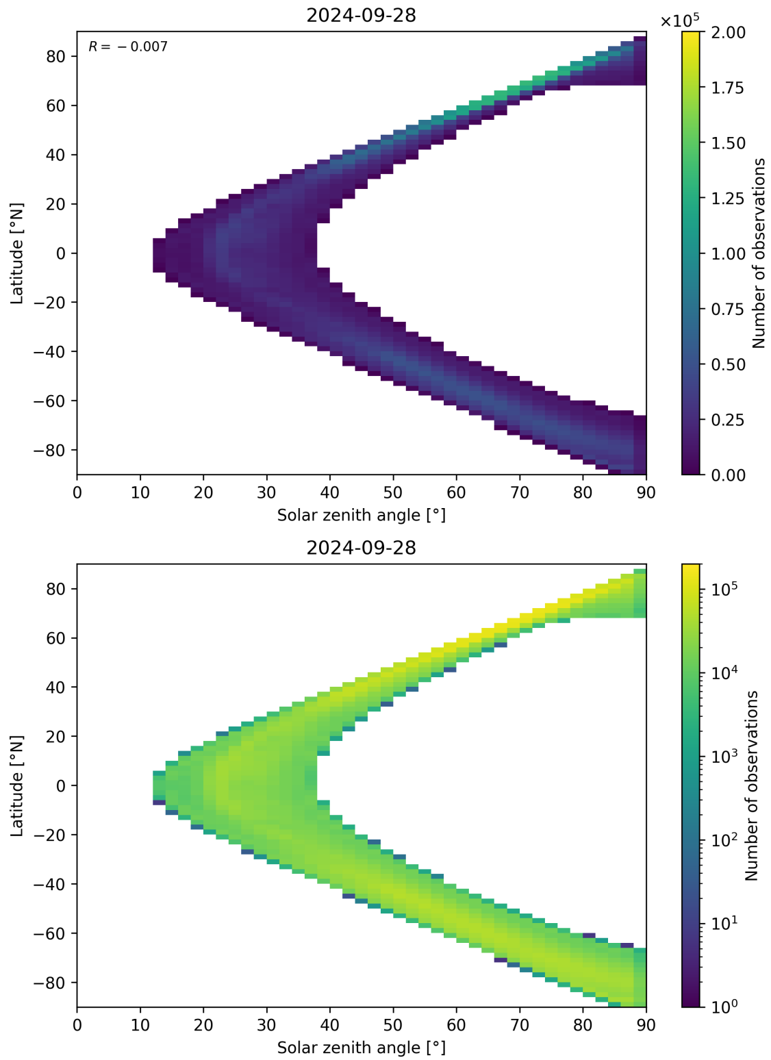
Figure 105: Scatter density plot of “Solar zenith angle” against “Latitude” for 2024-09-28 to 2024-09-29.
