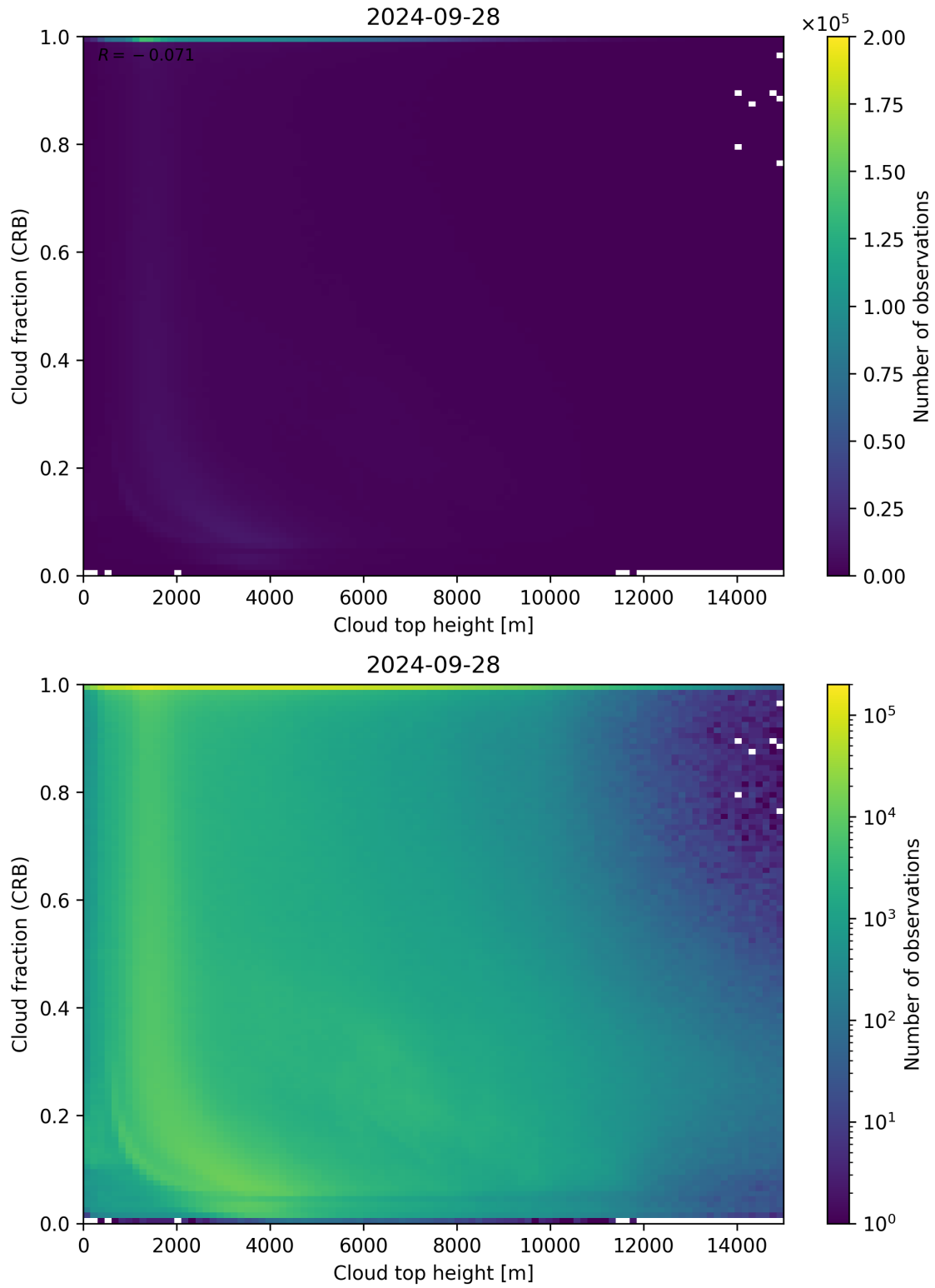
Figure 88: Scatter density plot of “Cloud top height” against “Cloud fraction (CRB)” for 2024-09-28 to 2024-09-29.
