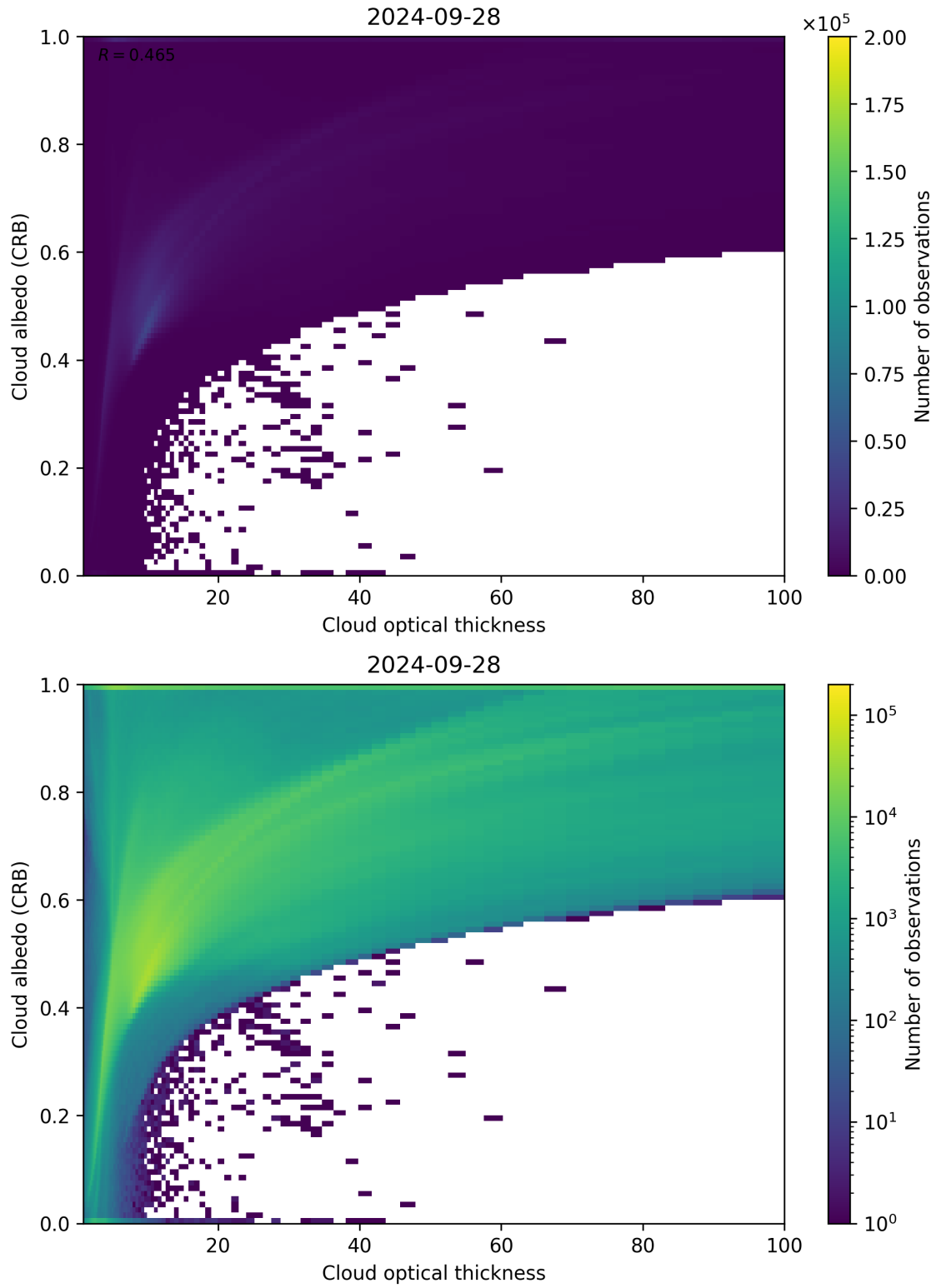
Figure 82: Scatter density plot of “Cloud optical thickness” against “Cloud albedo (CRB)” for 2024-09-28 to 2024-09-29.
