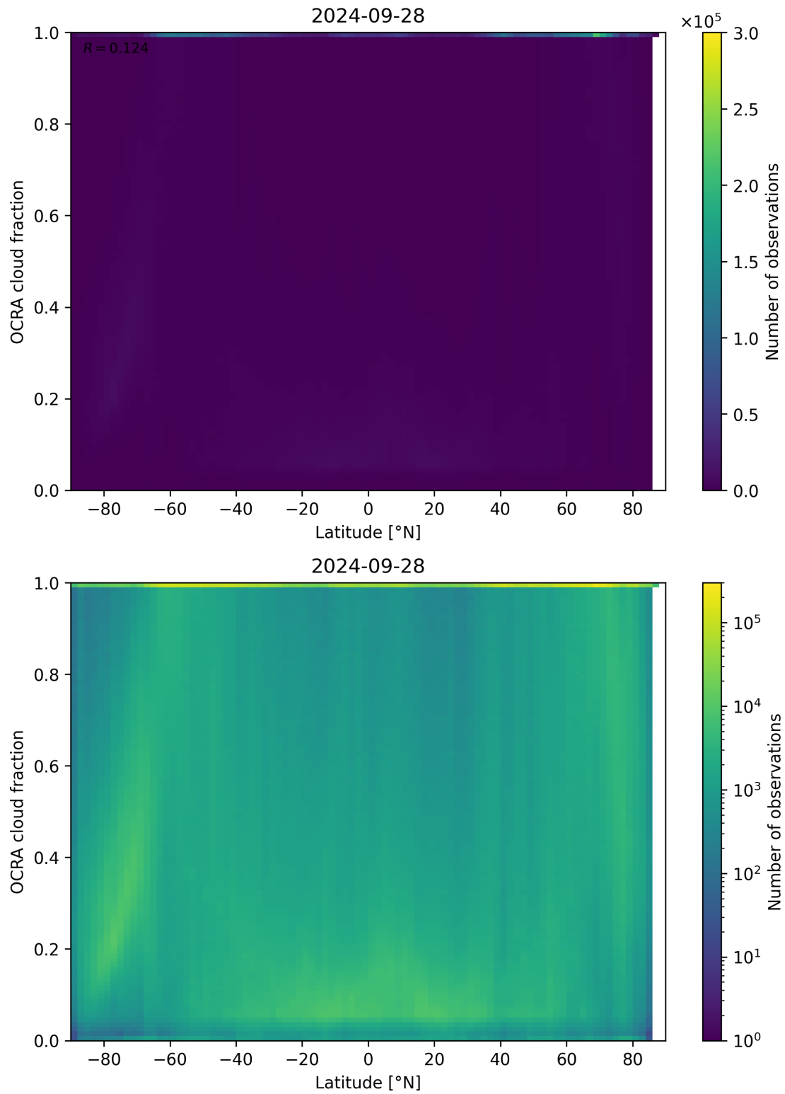
Figure 93: Scatter density plot of “Latitude” against “OCRA cloud fraction” for 2024-09-28 to 2024-09-29.
