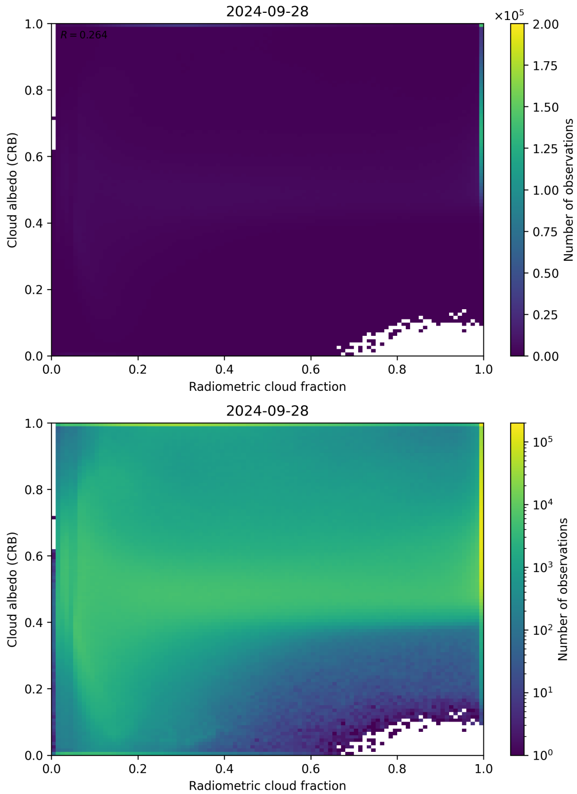
Figure 71: Scatter density plot of “Radiometric cloud fraction” against “Cloud albedo (CRB)” for 2024-09-28 to 2024-09-29.
