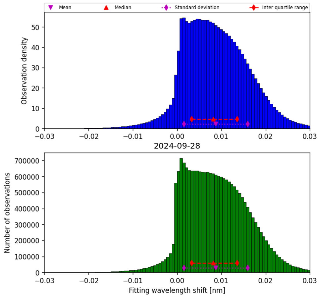
Figure 49: Histogram of “Fitting wavelength shift” for 2024-09-28 to 2024-09-29
