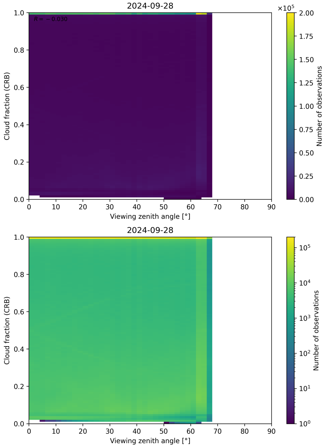
Figure 109: Scatter density plot of “Viewing zenith angle” against “Cloud fraction (CRB)” for 2024-09-28 to 2024-09-29.
