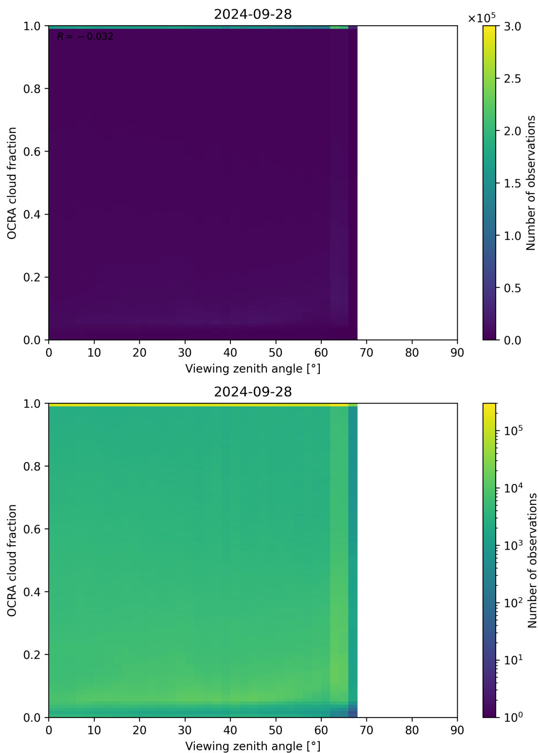
Figure 108: Scatter density plot of “Viewing zenith angle” against “OCRA cloud fraction” for 2024-09-28 to 2024-09-29.
