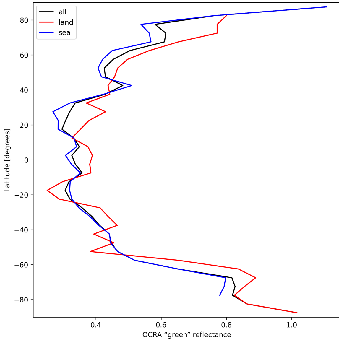
Figure 36: Zonal average of “OCRA “green” reflectance” for 2024-09-28 to 2024-09-29.
