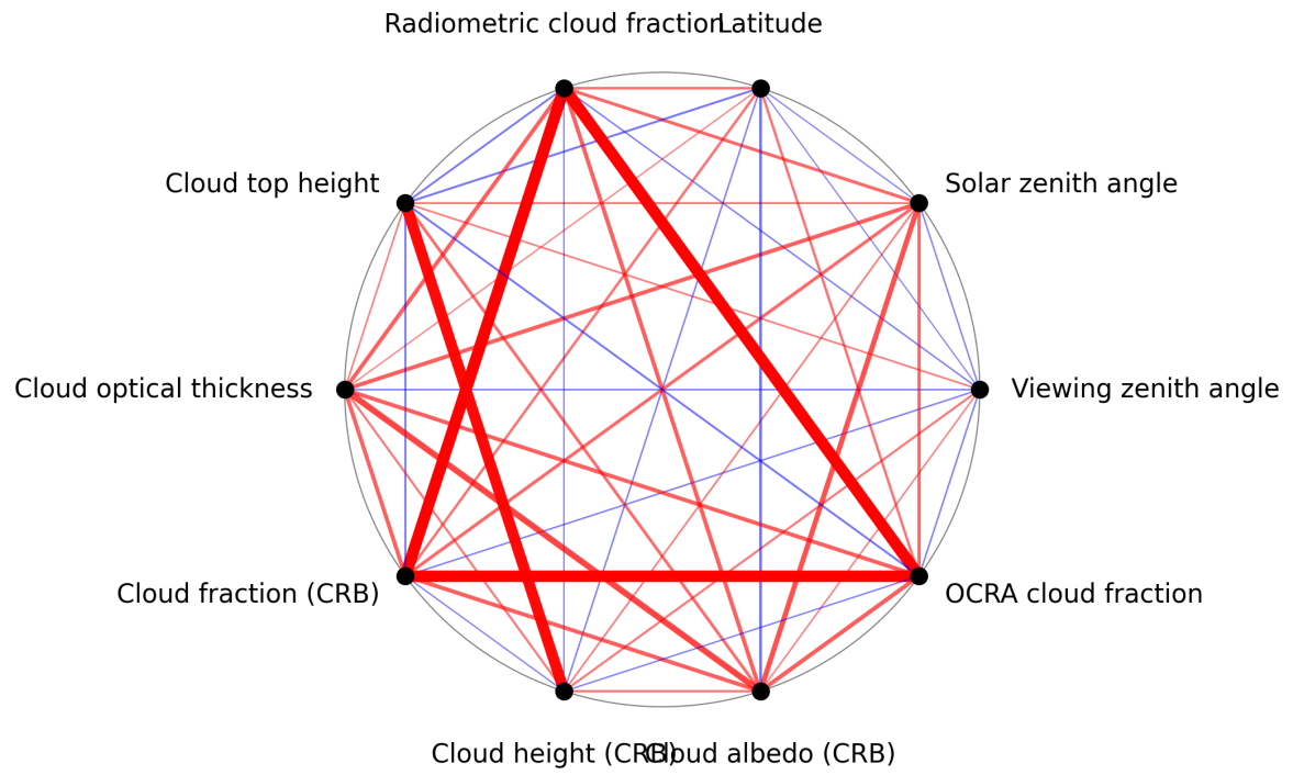
Figure 1: Map of correlation graph for 2024-09-28 to 2024-09-29.
