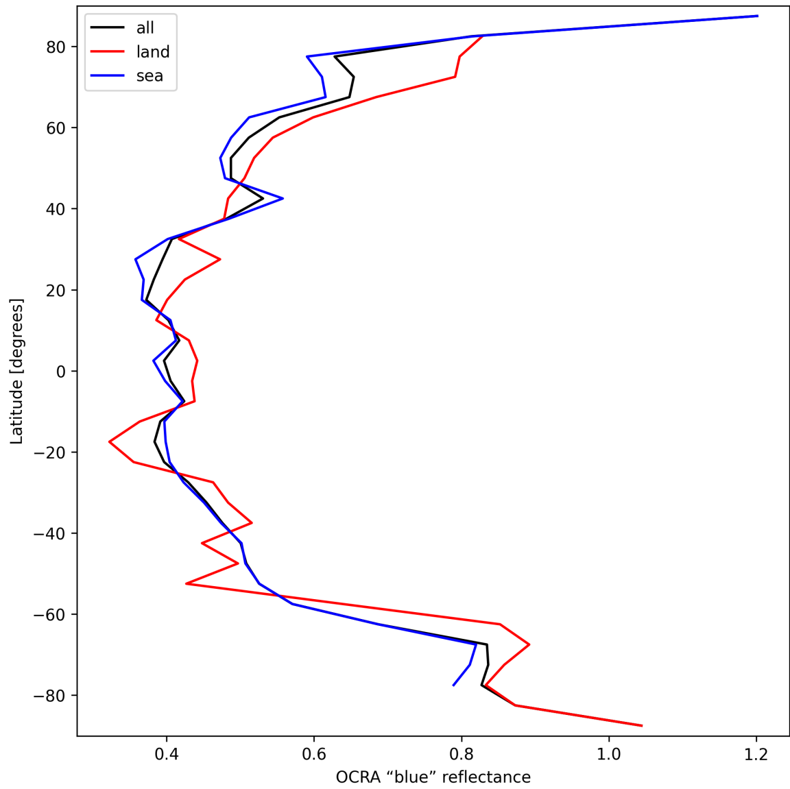
Figure 35: Zonal average of “OCRA “blue” reflectance” for 2024-09-28 to 2024-09-29.
