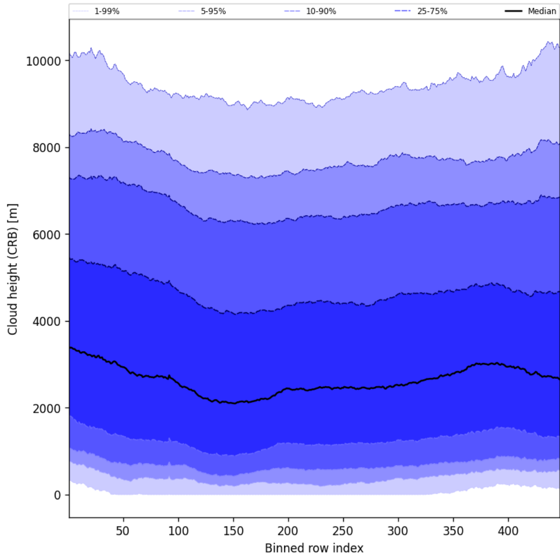
Figure 59: Along track statistics of “Cloud height (CRB)” for 2024-09-28 to 2024-09-29
