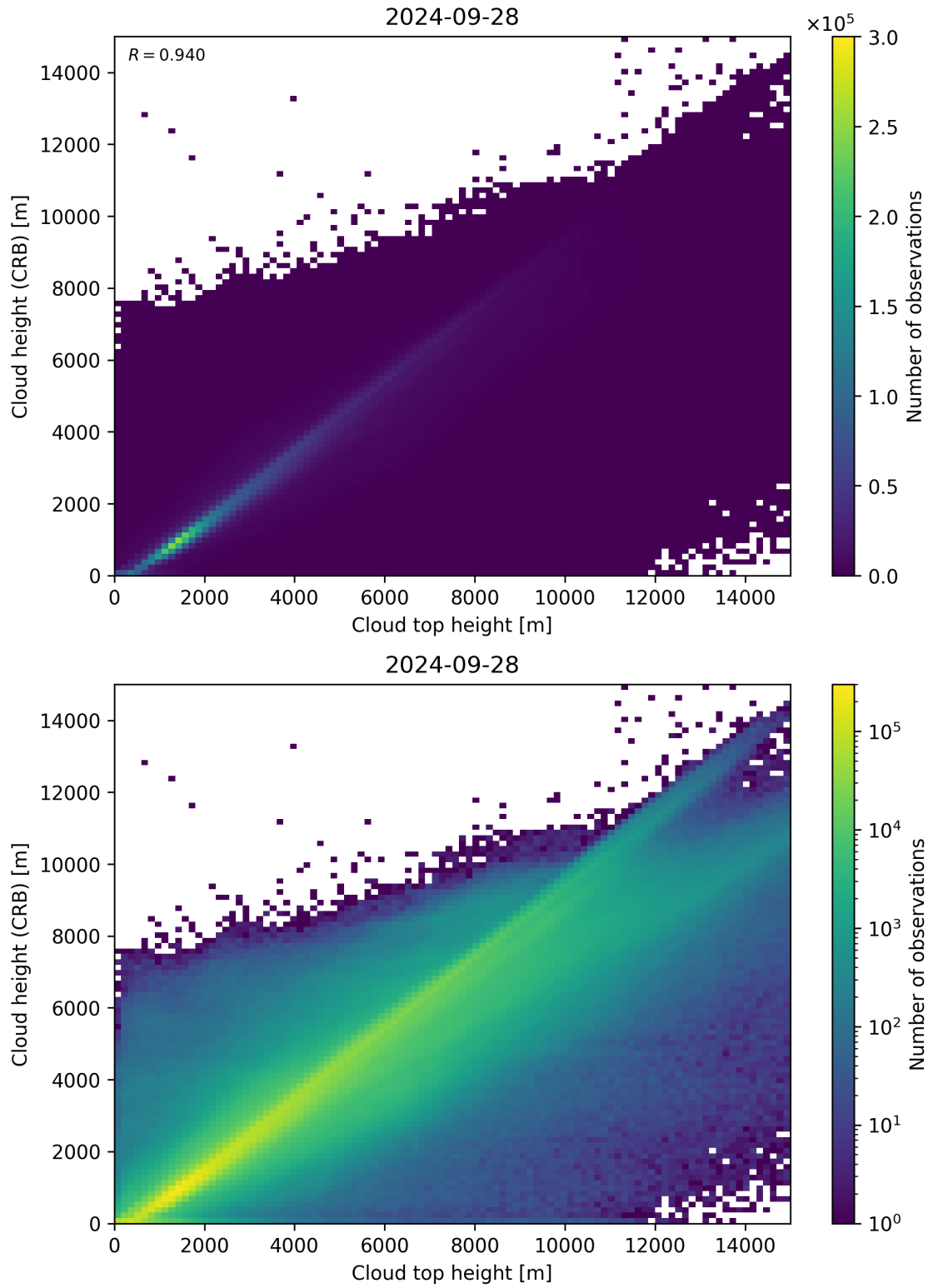
Figure 89: Scatter density plot of “Cloud top height” against “Cloud height (CRB)” for 2024-09-28 to 2024-09-29.
