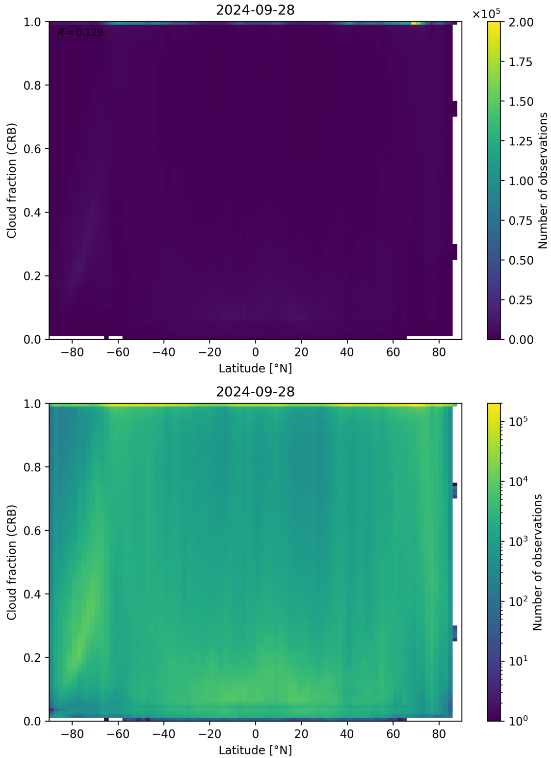
Figure 94: Scatter density plot of “Latitude” against “Cloud fraction (CRB)” for 2024-09-28 to 2024-09-29.
