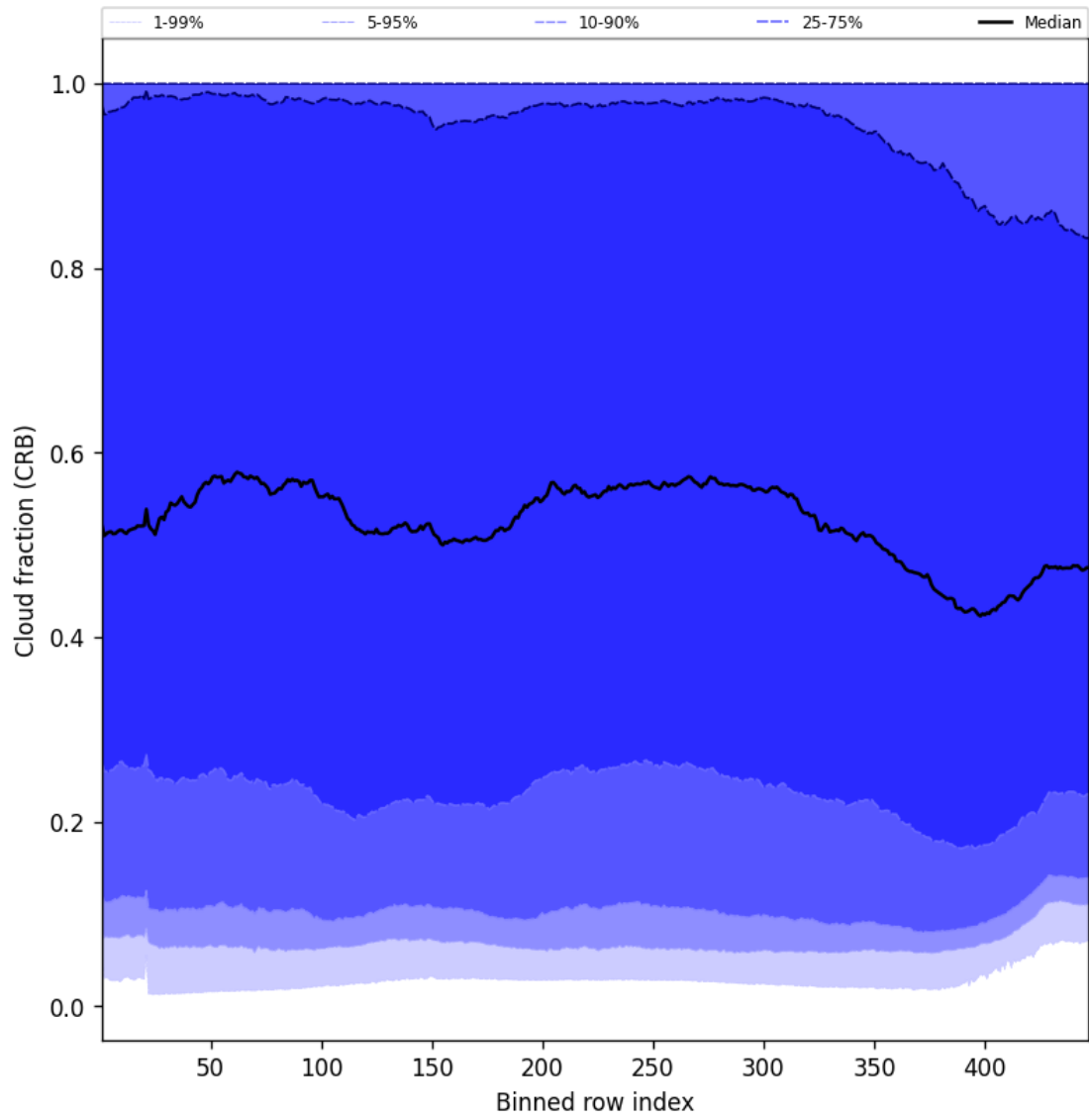
Figure 58: Along track statistics of “Cloud fraction (CRB)” for 2024-09-28 to 2024-09-29
