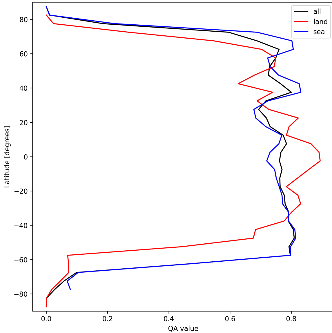
Figure 22: Zonal average of “QA value” for 2024-09-28 to 2024-09-29.
