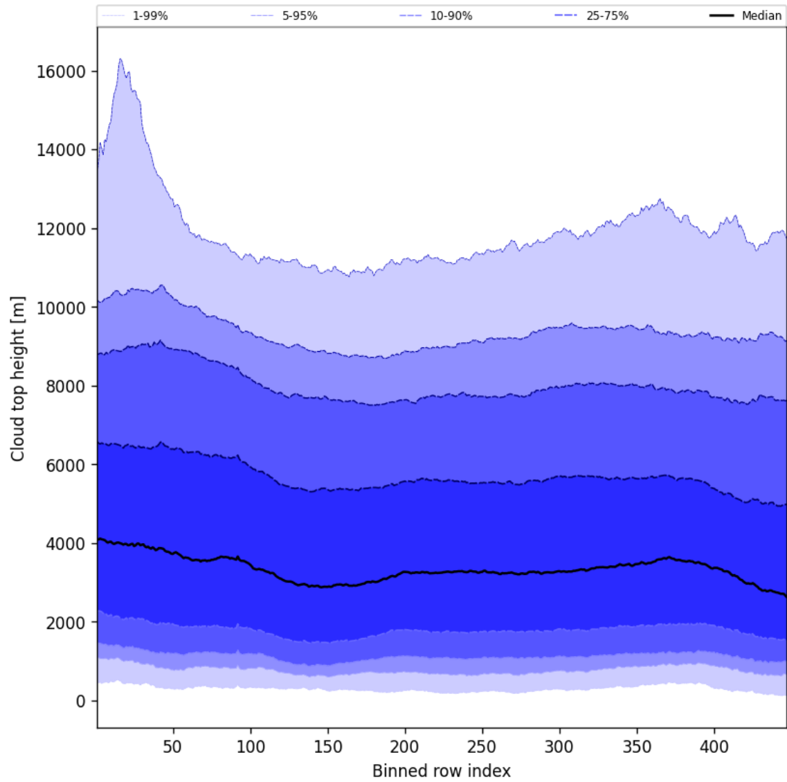
Figure 56: Along track statistics of “Cloud top height” for 2024-09-28 to 2024-09-29
