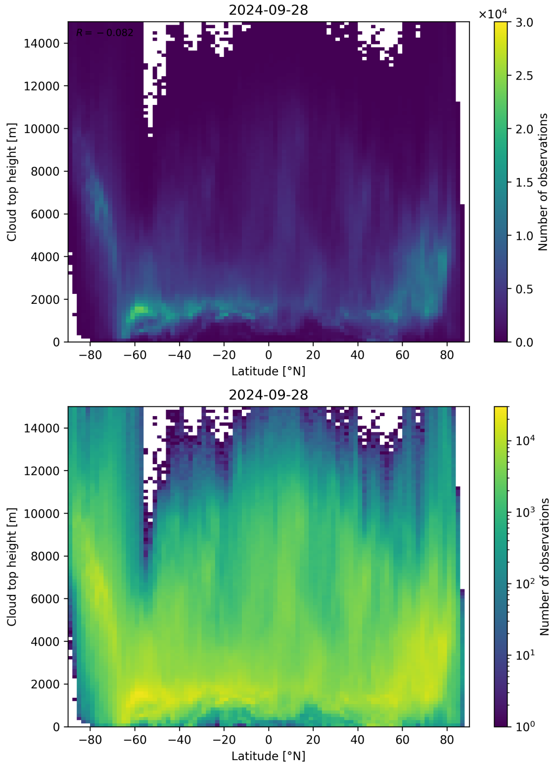
Figure 97: Scatter density plot of “Latitude” against “Cloud top height” for 2024-09-28 to 2024-09-29.
