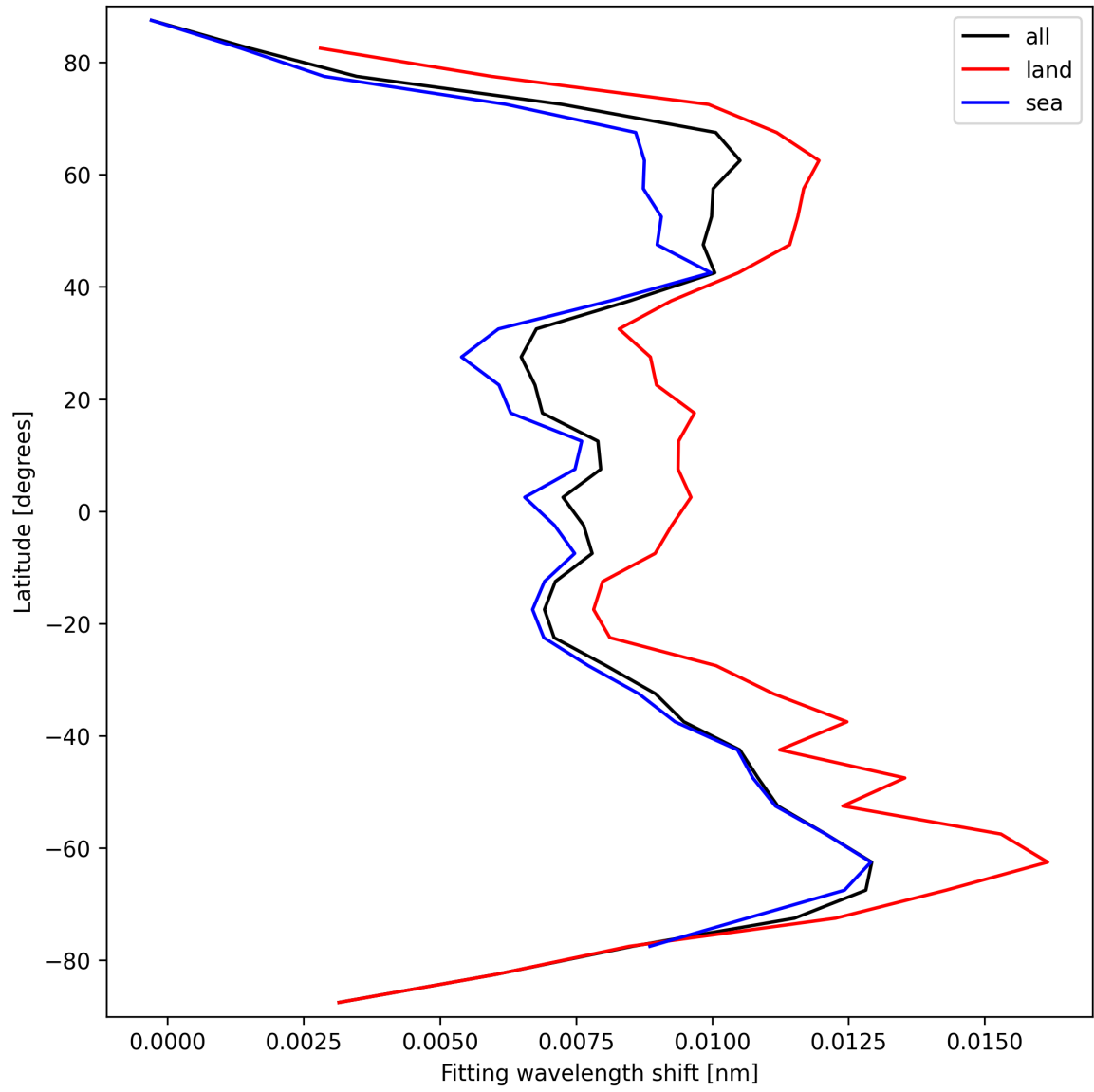
Figure 33: Zonal average of “Fitting wavelength shift” for 2024-09-28 to 2024-09-29.
