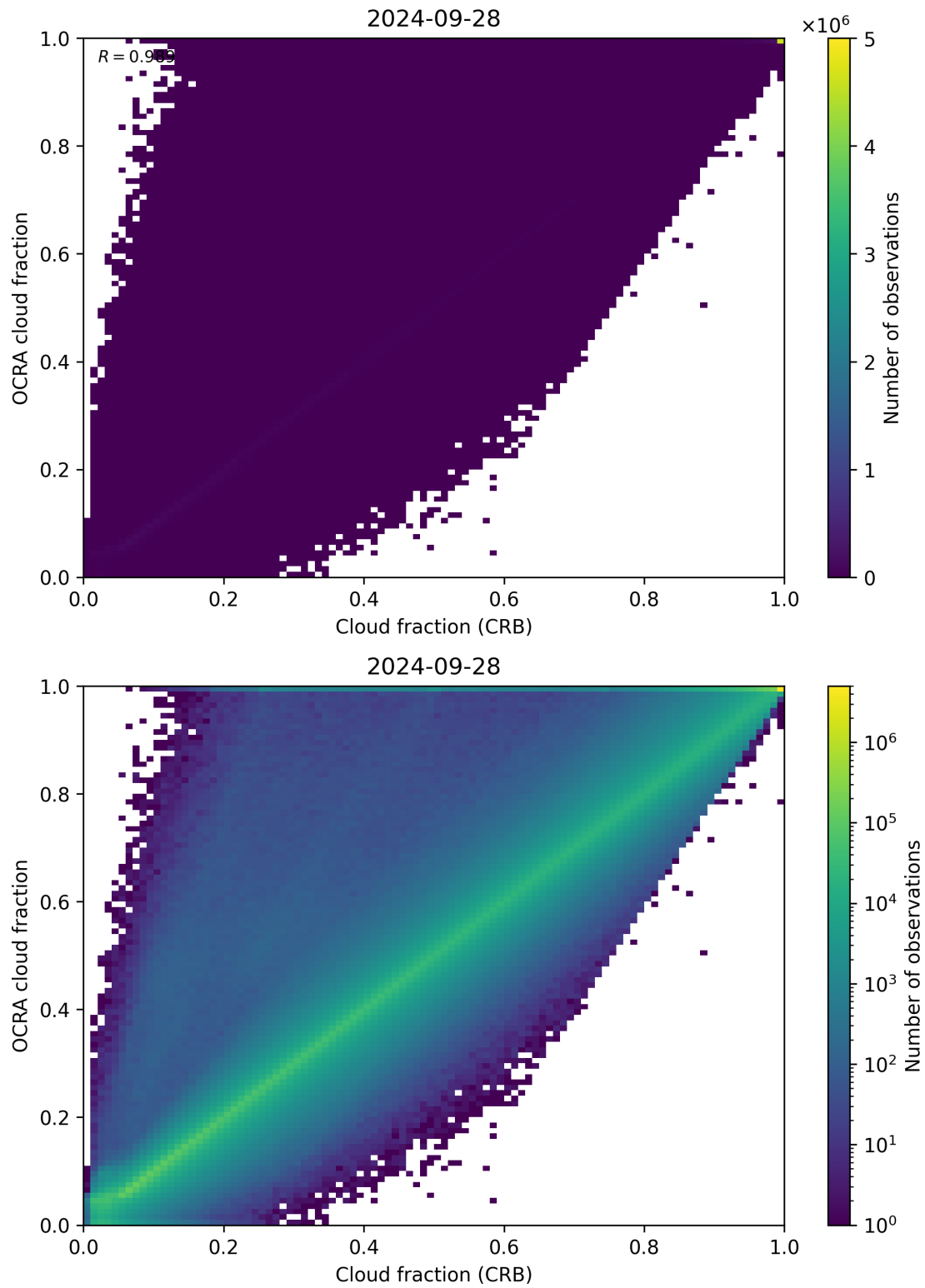
Figure 78: Scatter density plot of “Cloud fraction (CRB)” against “OCRA cloud fraction” for 2024-09-28 to 2024-09-29.
