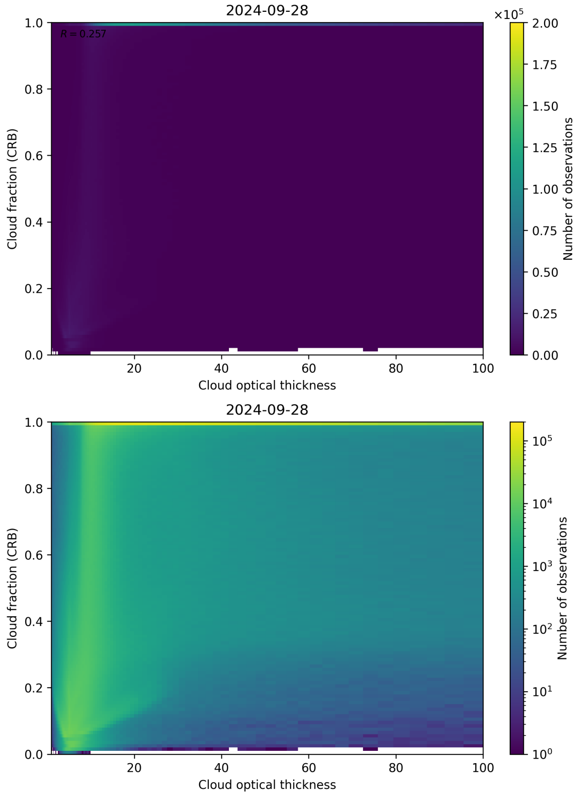
Figure 84: Scatter density plot of “Cloud optical thickness” against “Cloud fraction (CRB)” for 2024-09-28 to 2024-09-29.
