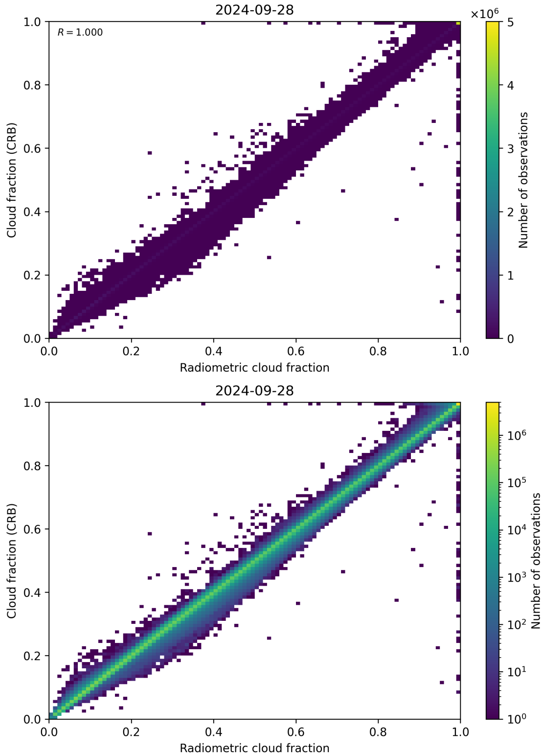
Figure 73: Scatter density plot of “Radiometric cloud fraction” against “Cloud fraction (CRB)” for 2024-09-28 to 2024-09-29.
