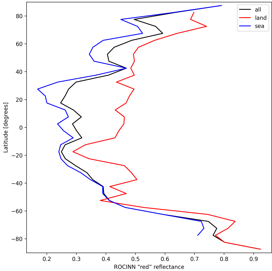
Figure 37: Zonal average of “ROCINN “red” reflectance” for 2024-09-28 to 2024-09-29.
