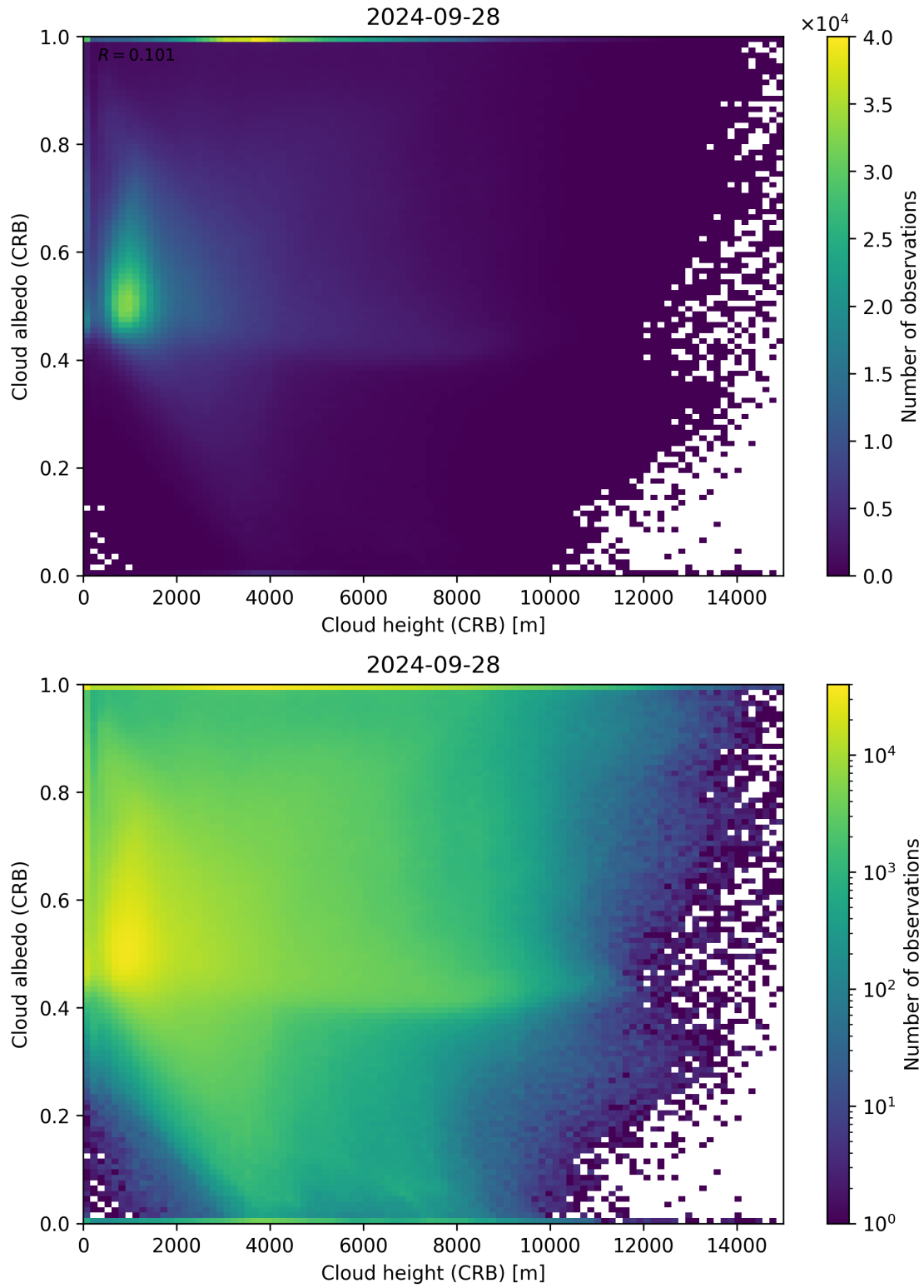
Figure 80: Scatter density plot of “Cloud height (CRB)” against “Cloud albedo (CRB)” for 2024-09-28 to 2024-09-29.
