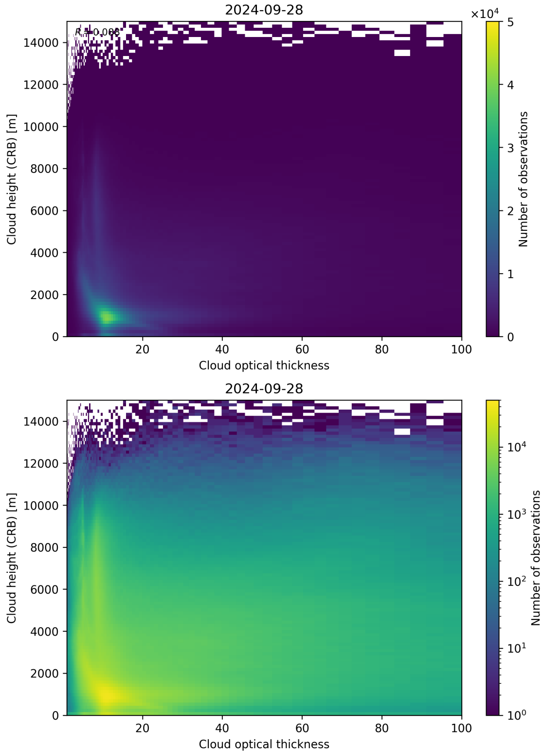
Figure 85: Scatter density plot of “Cloud optical thickness” against “Cloud height (CRB)” for 2024-09-28 to 2024-09-29.
