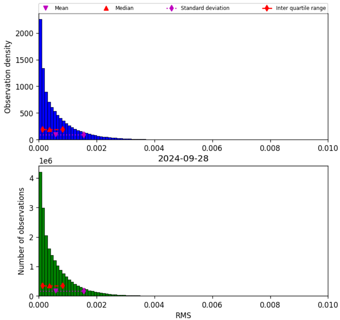
Figure 47: Histogram of “RMS” for 2024-09-28 to 2024-09-29
