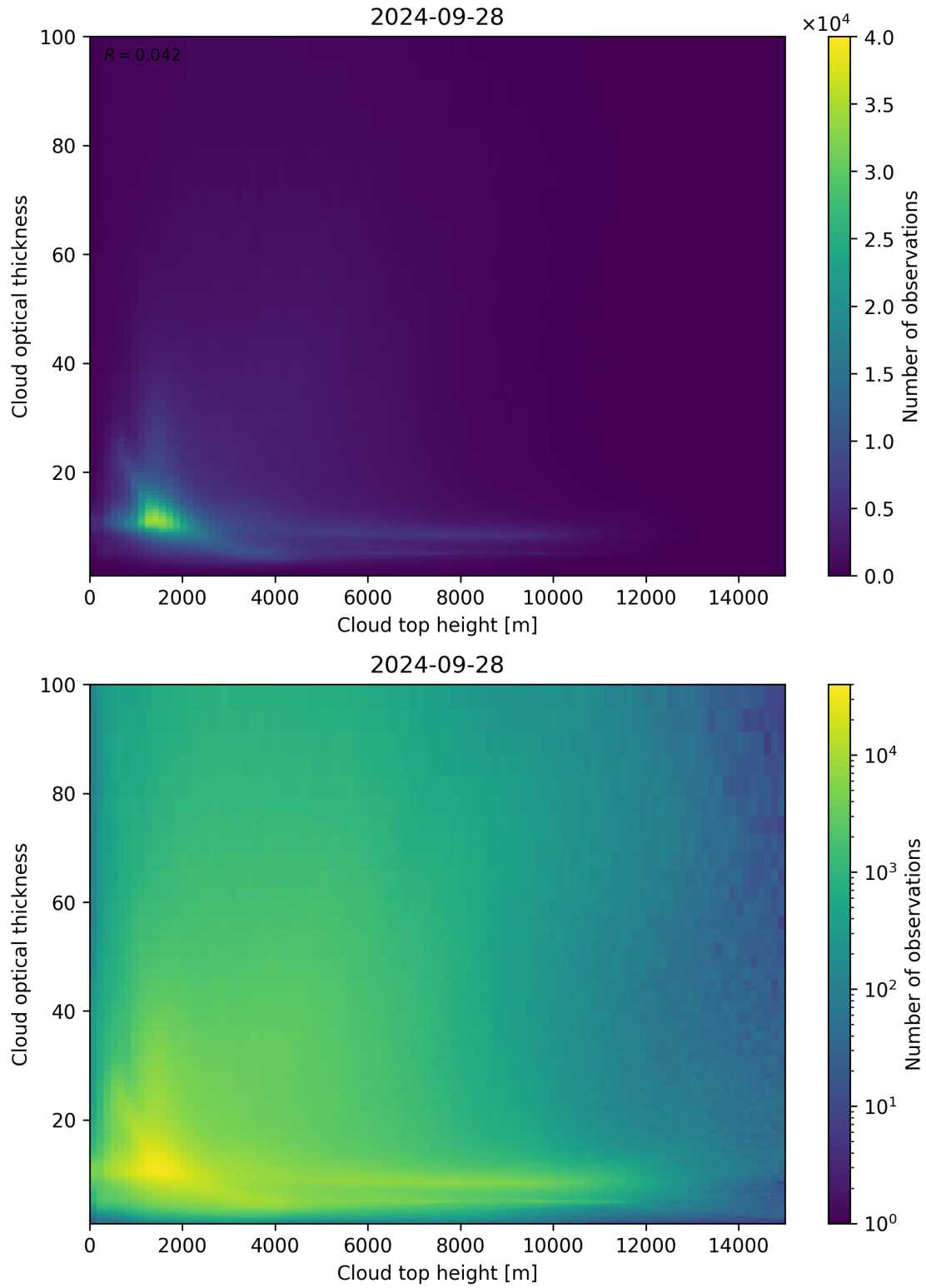
Figure 90: Scatter density plot of “Cloud top height” against “Cloud optical thickness” for 2024-09-28 to 2024-09-29.
