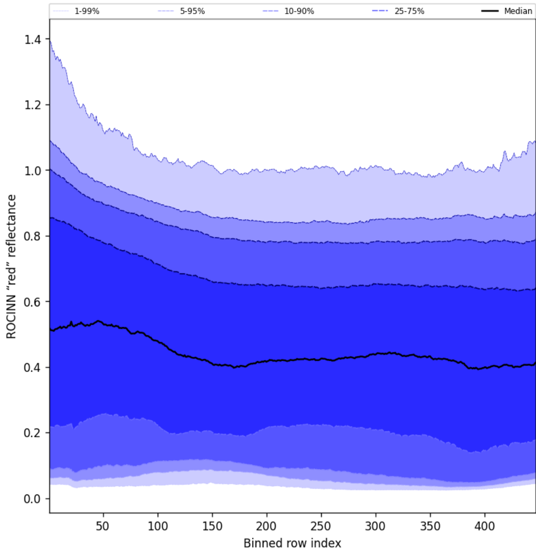
Figure 69: Along track statistics of "ROCINN "red" reflectance" for 2024-09-28 to 2024-09-29
