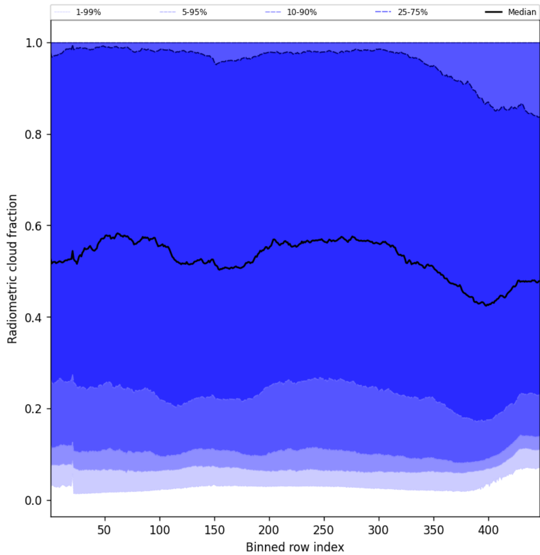
Figure 55: Along track statistics of “Radiometric cloud fraction” for 2024-09-28 to 2024-09-29
