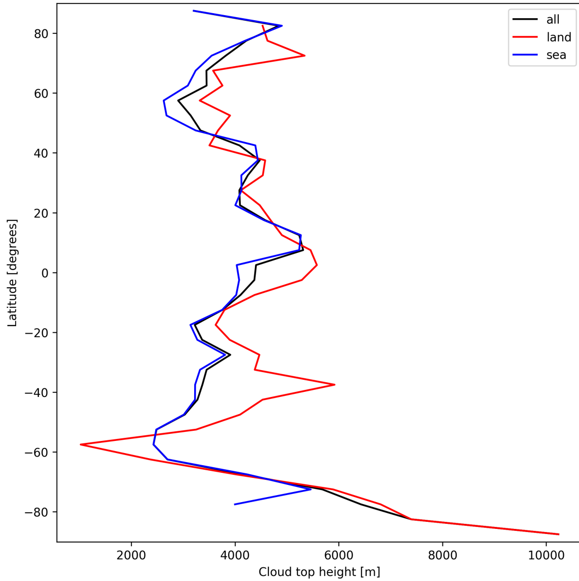
Figure 24: Zonal average of “Cloud top height” for 2024-09-28 to 2024-09-29.
