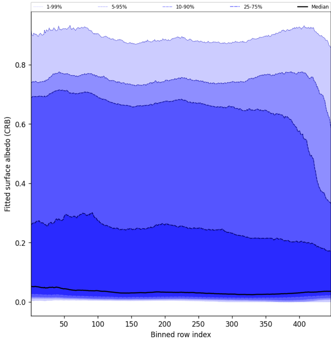
Figure 62: Along track statistics of “Fitted surface albedo (CRB)” for 2024-09-28 to 2024-09-29
