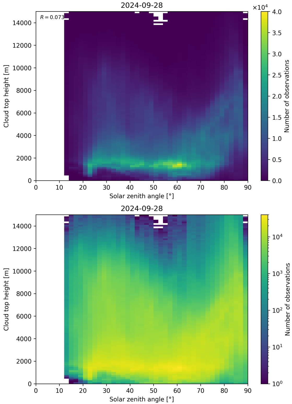
Figure 104: Scatter density plot of “Solar zenith angle” against “Cloud top height” for 2024-09-28 to 2024-09-29.
