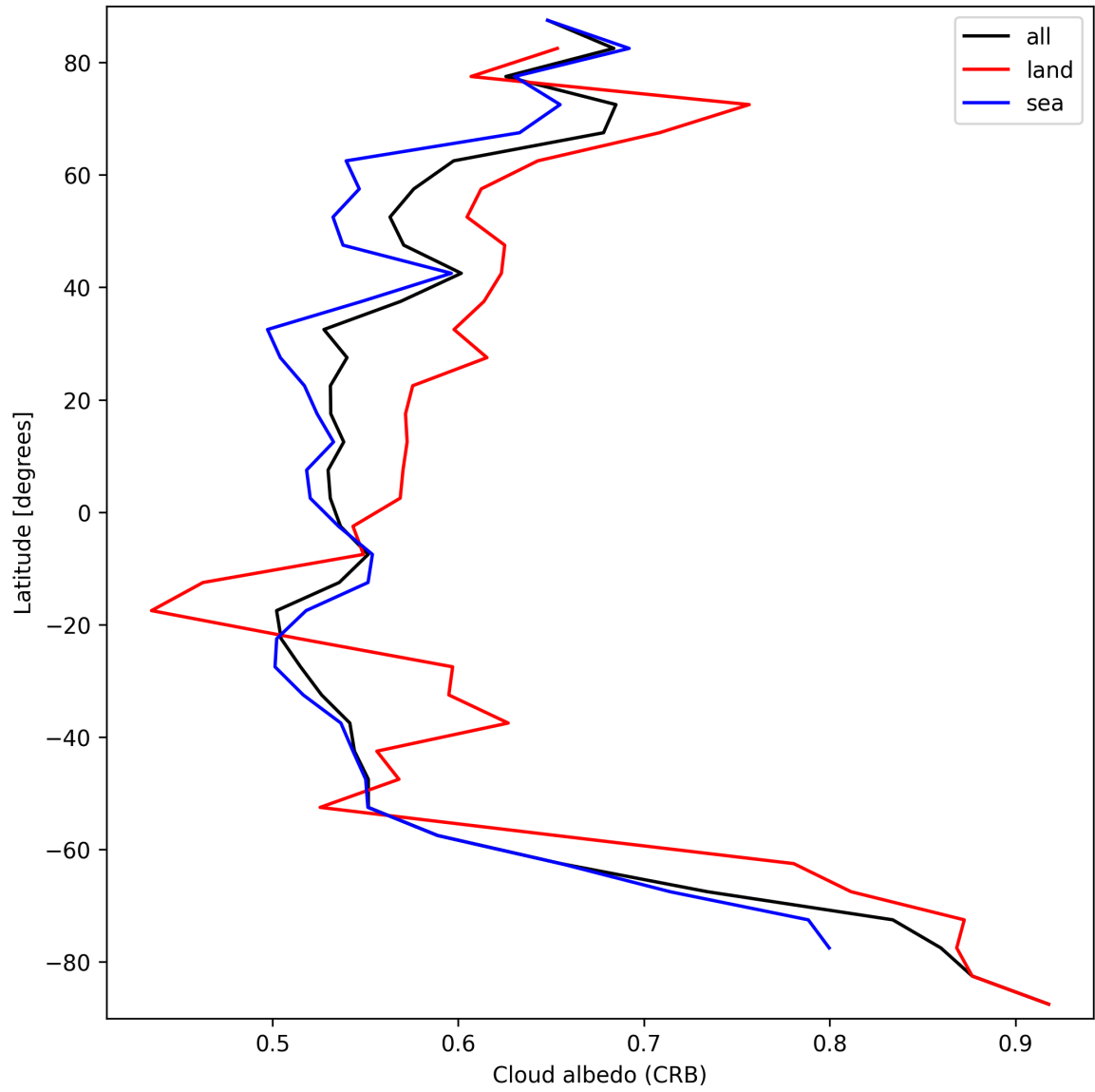
Figure 28: Zonal average of “Cloud albedo (CRB)” for 2024-09-28 to 2024-09-29.
