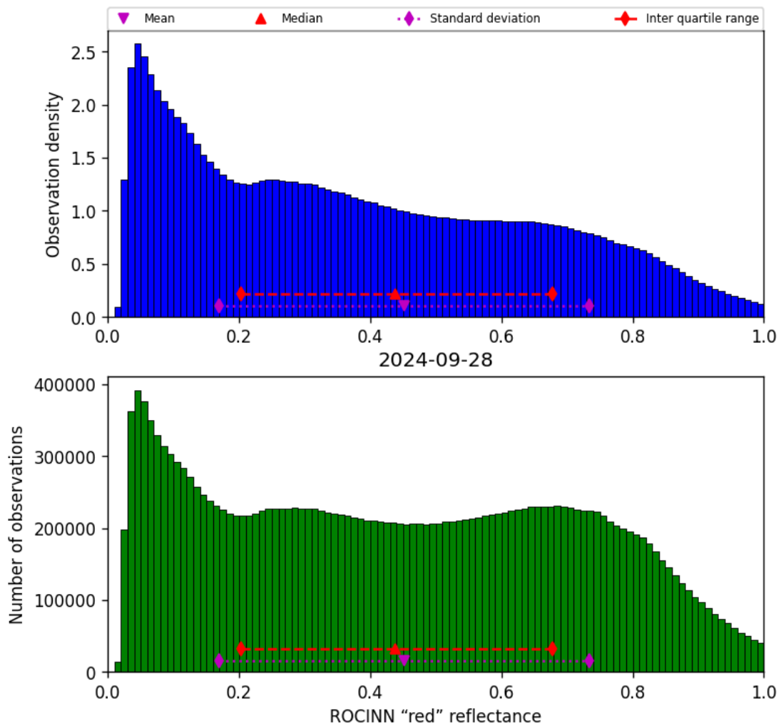
Figure 53: Histogram of “ROCINN “red” reflectance” for 2024-09-28 to 2024-09-29
