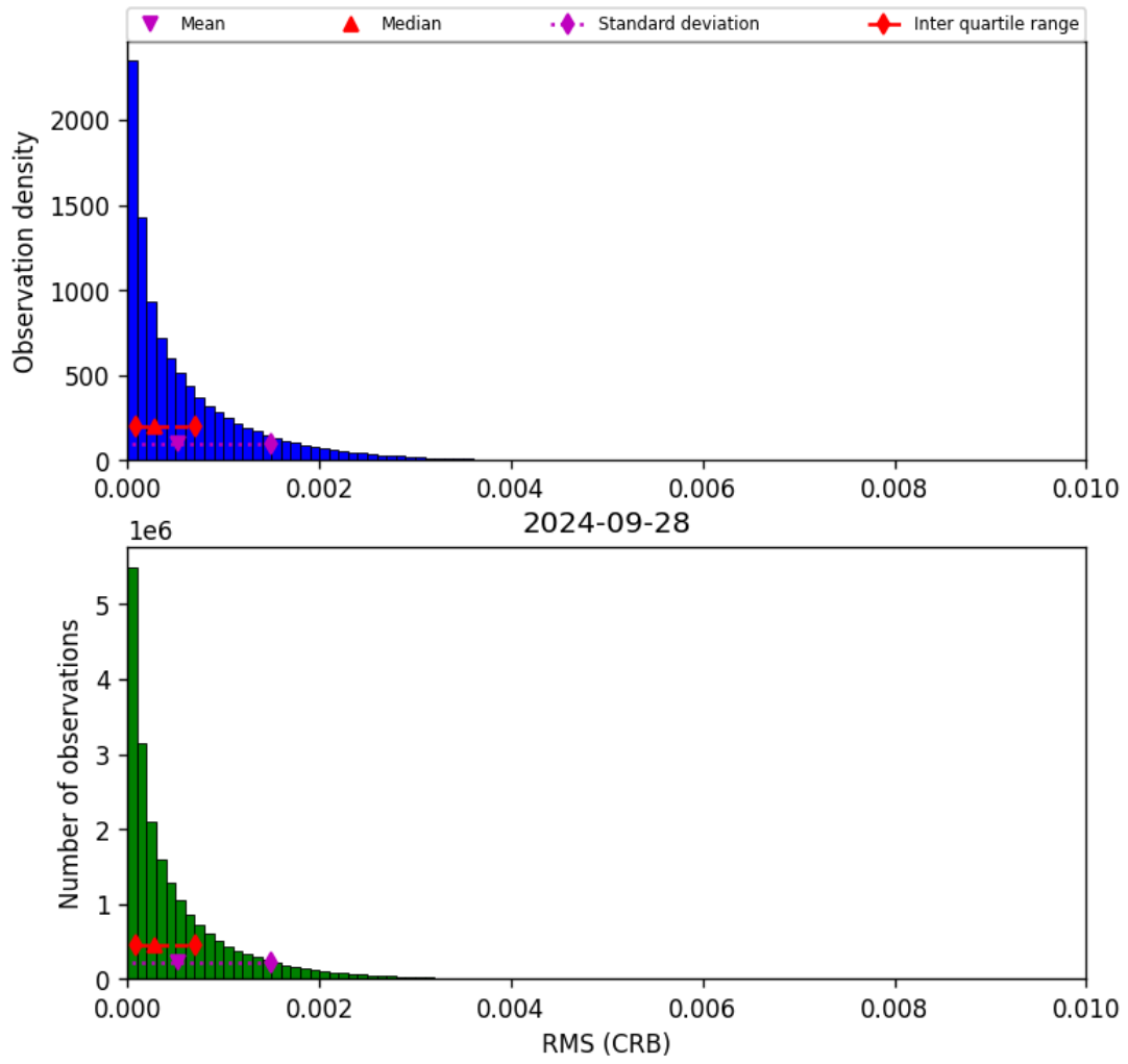
Figure 48: Histogram of "RMS (CRB)" for 2024-09-28 to 2024-09-29
