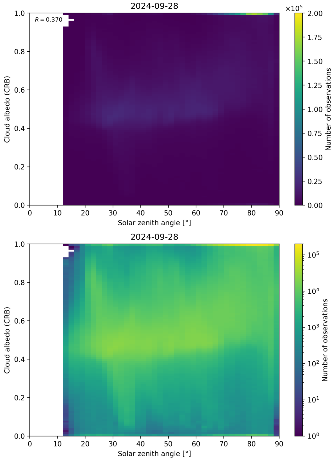
Figure 98: Scatter density plot of “Solar zenith angle” against “Cloud albedo (CRB)” for 2024-09-28 to 2024-09-29.
