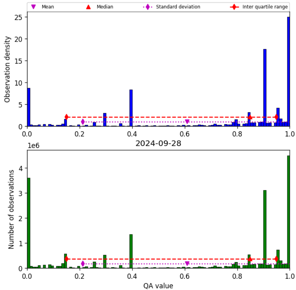
Figure 38: Histogram of “QA value” for 2024-09-28 to 2024-09-29
