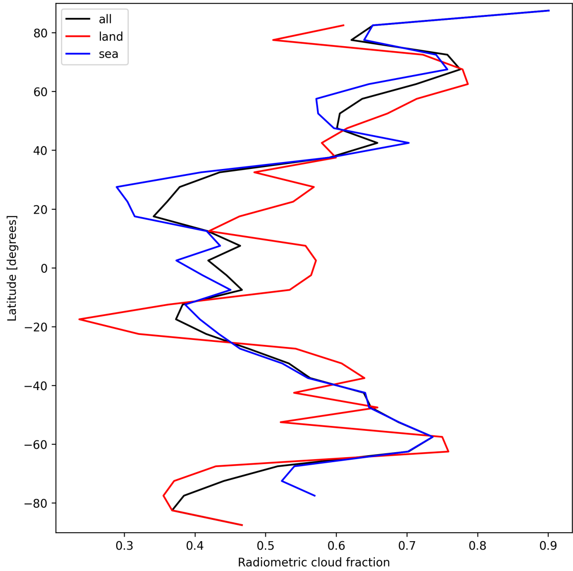
Figure 23: Zonal average of “Radiometric cloud fraction” for 2024-09-28 to 2024-09-29.
