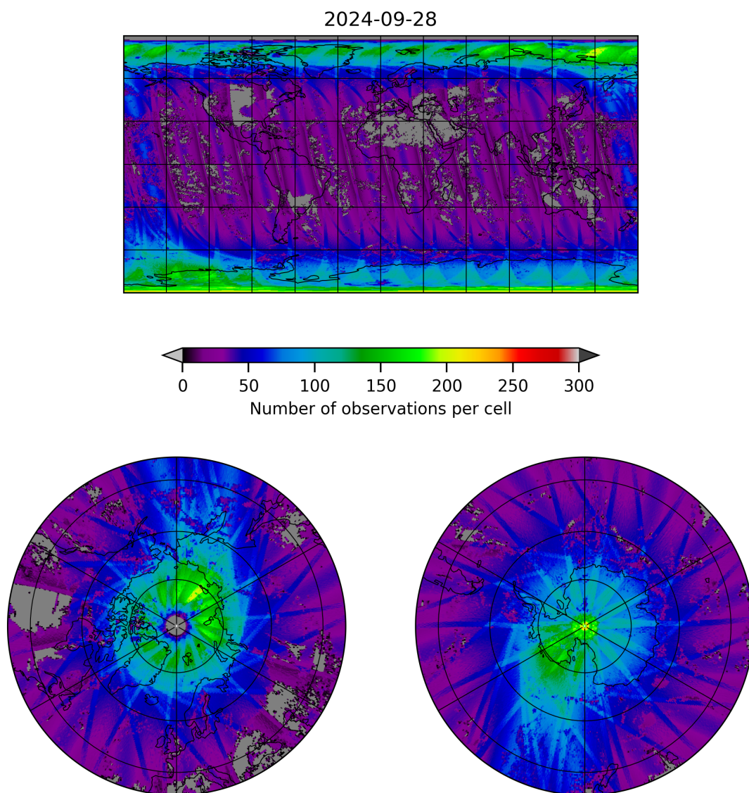
Figure 21: Map of the number of observations for 2024-09-28 to 2024-09-29
