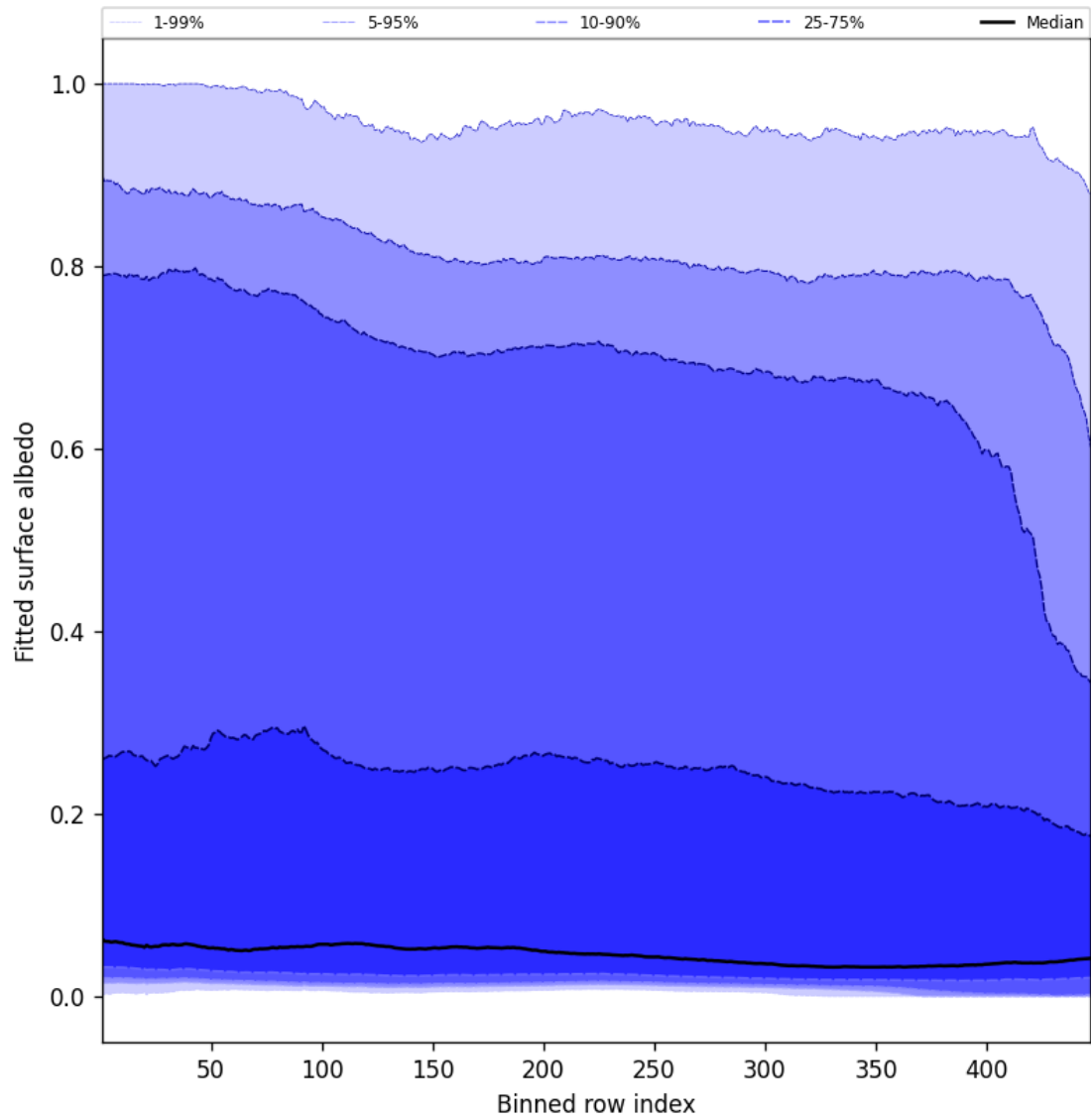
Figure 61: Along track statistics of “Fitted surface albedo” for 2024-09-28 to 2024-09-29
