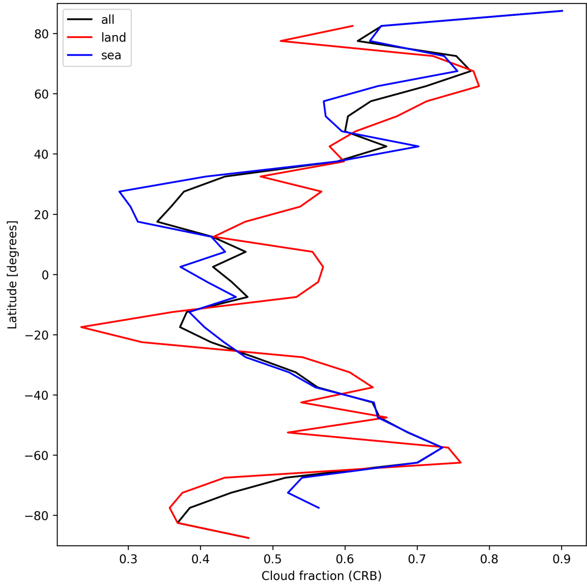
Figure 26: Zonal average of “Cloud fraction (CRB)” for 2024-09-28 to 2024-09-29.
