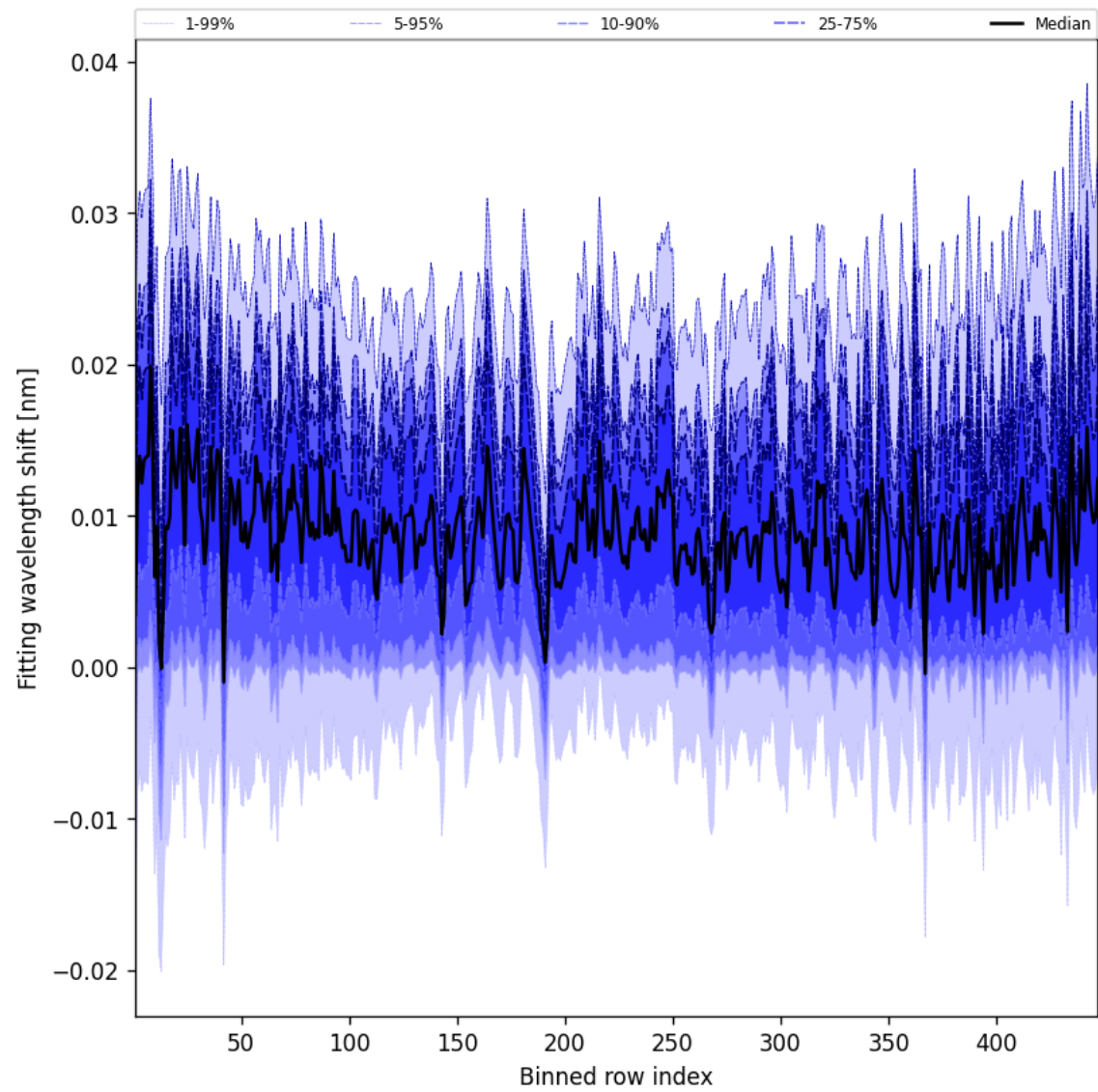
Figure 65: Along track statistics of “Fitting wavelength shift” for 2024-09-28 to 2024-09-29
