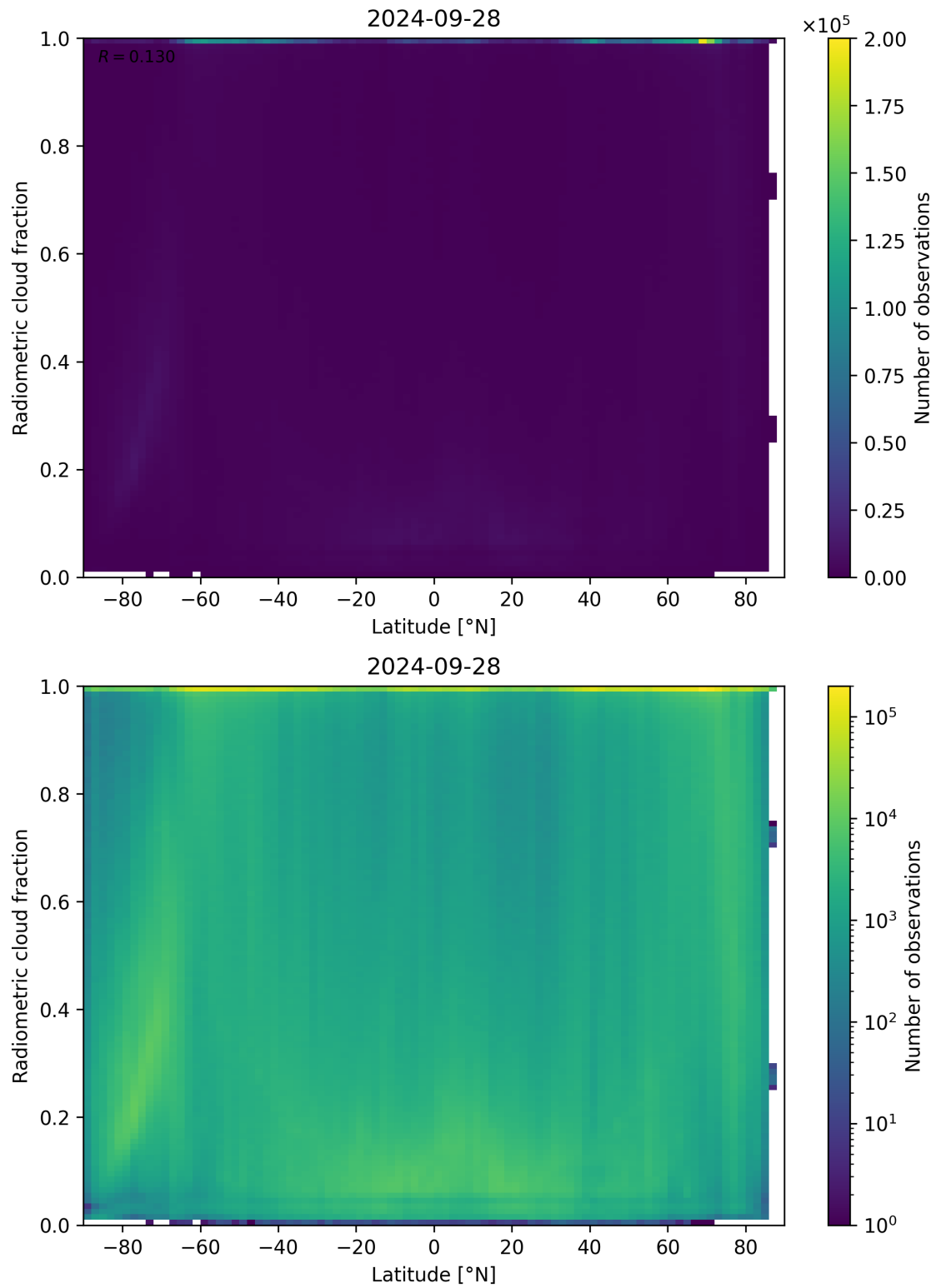
Figure 92: Scatter density plot of “Latitude” against “Radiometric cloud fraction” for 2024-09-28 to 2024-09-29.
