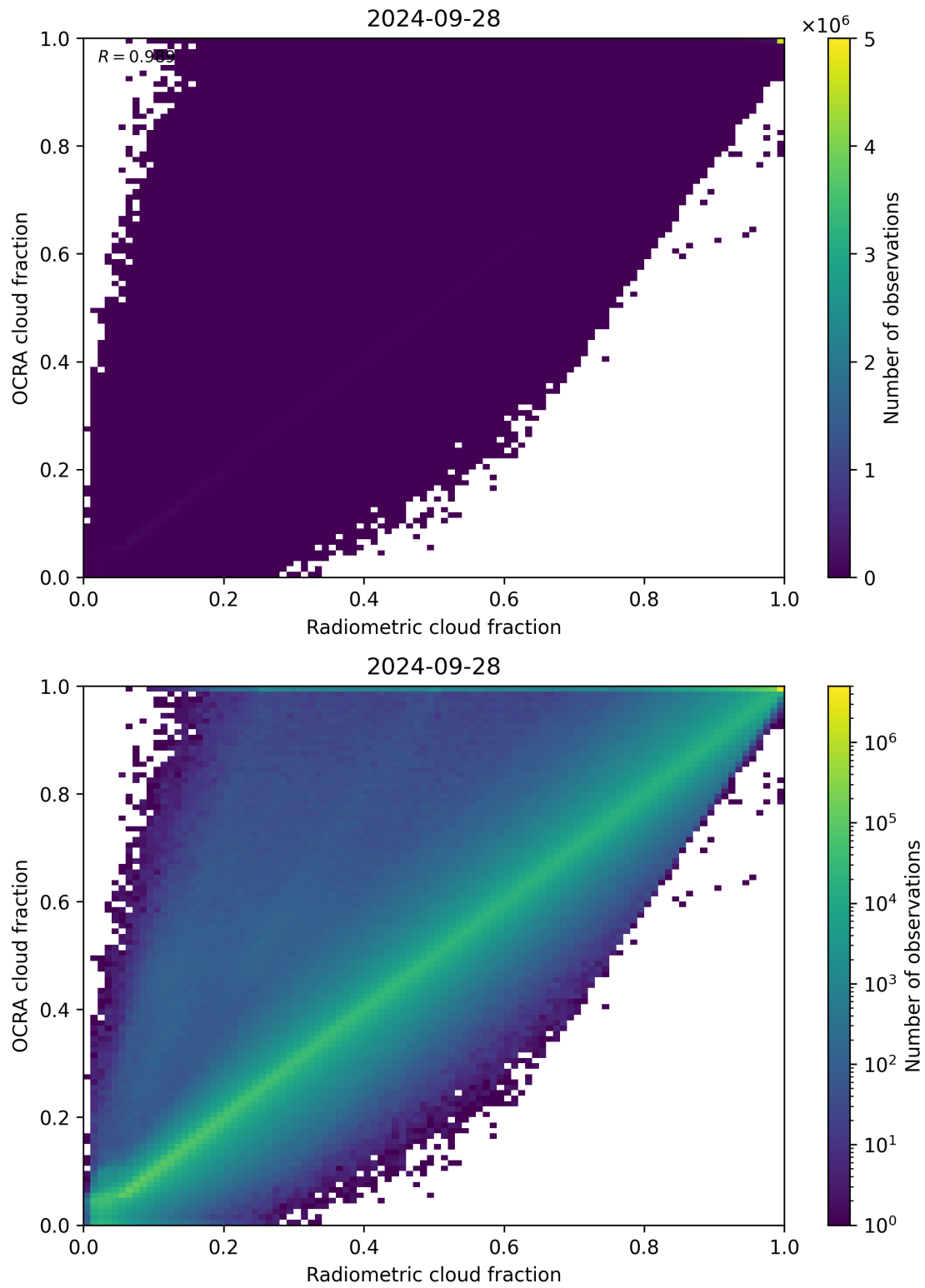
Figure 72: Scatter density plot of “Radiometric cloud fraction” against “OCRA cloud fraction” for 2024-09-28 to 2024-09-29.
