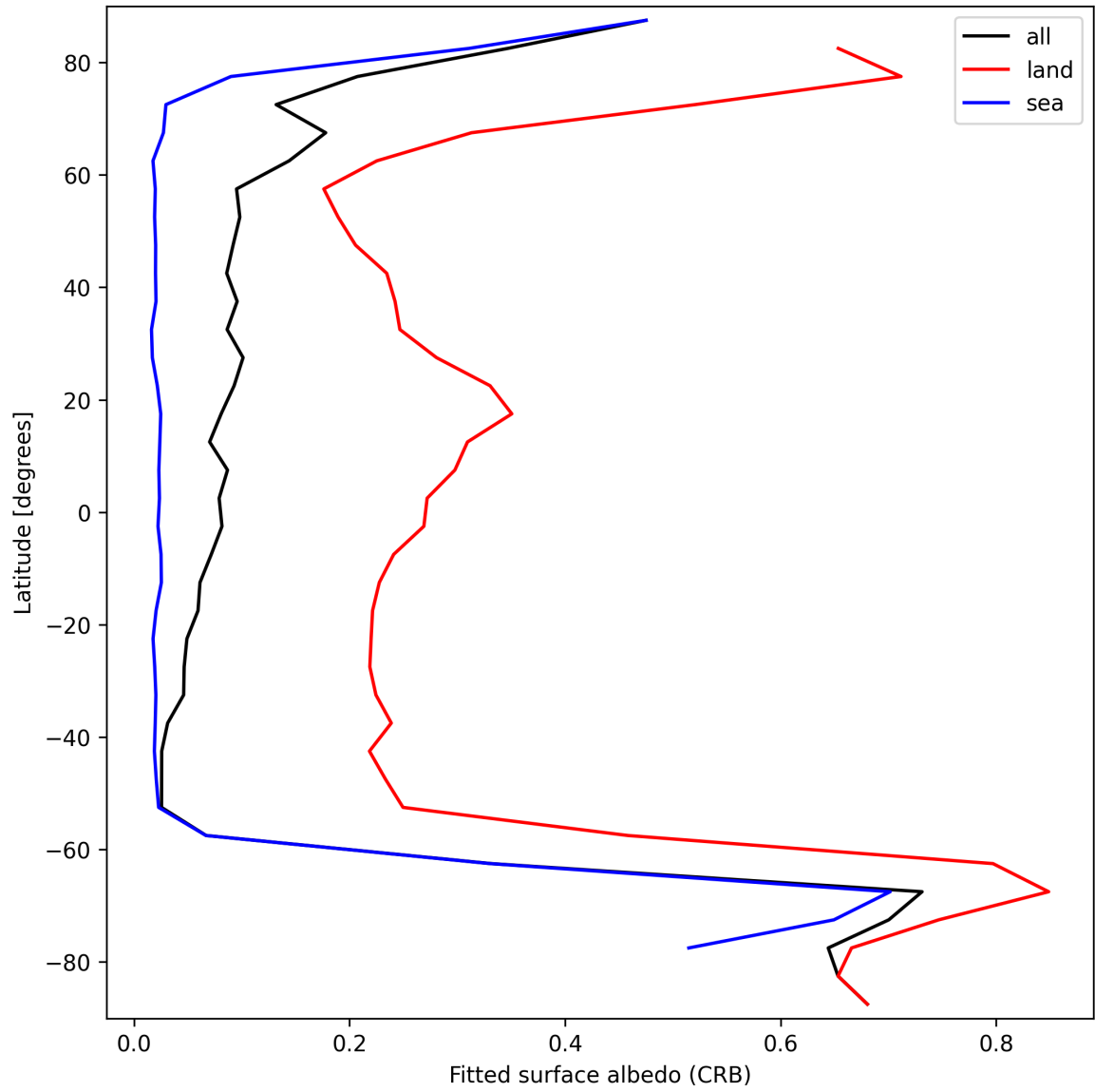
Figure 30: Zonal average of “Fitted surface albedo (CRB)” for 2024-09-28 to 2024-09-29.
