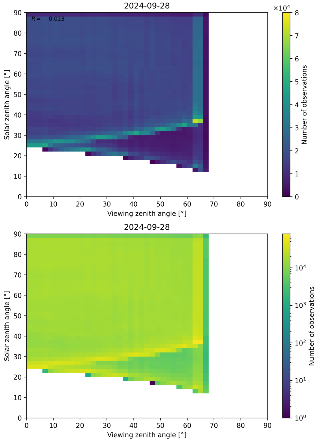
Figure 114: Scatter density plot of “Viewing zenith angle” against “Solar zenith angle” for 2024-09-28 to 2024-09-29.
