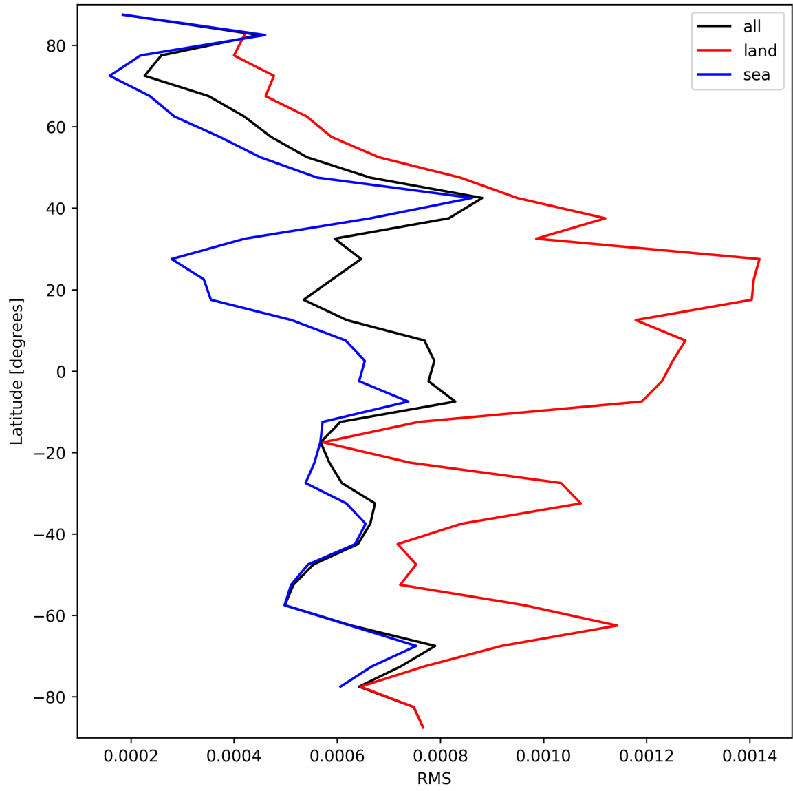
Figure 31: Zonal average of “RMS” for 2024-09-28 to 2024-09-29.
