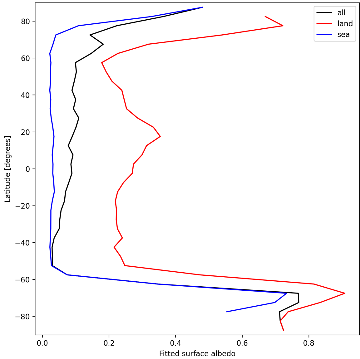
Figure 29: Zonal average of “Fitted surface albedo” for 2024-09-28 to 2024-09-29.
