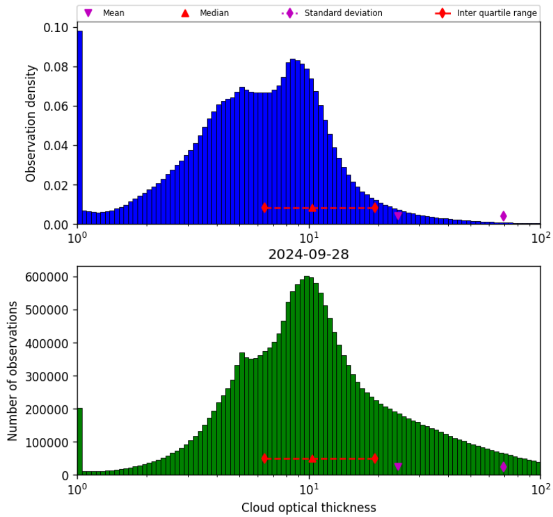
Figure 41: Histogram of “Cloud optical thickness” for 2024-09-28 to 2024-09-29
