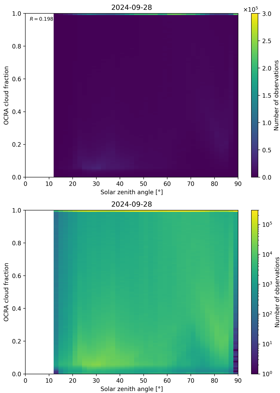
Figure 100: Scatter density plot of “Solar zenith angle” against “OCRA cloud fraction” for 2024-09-28 to 2024-09-29.
