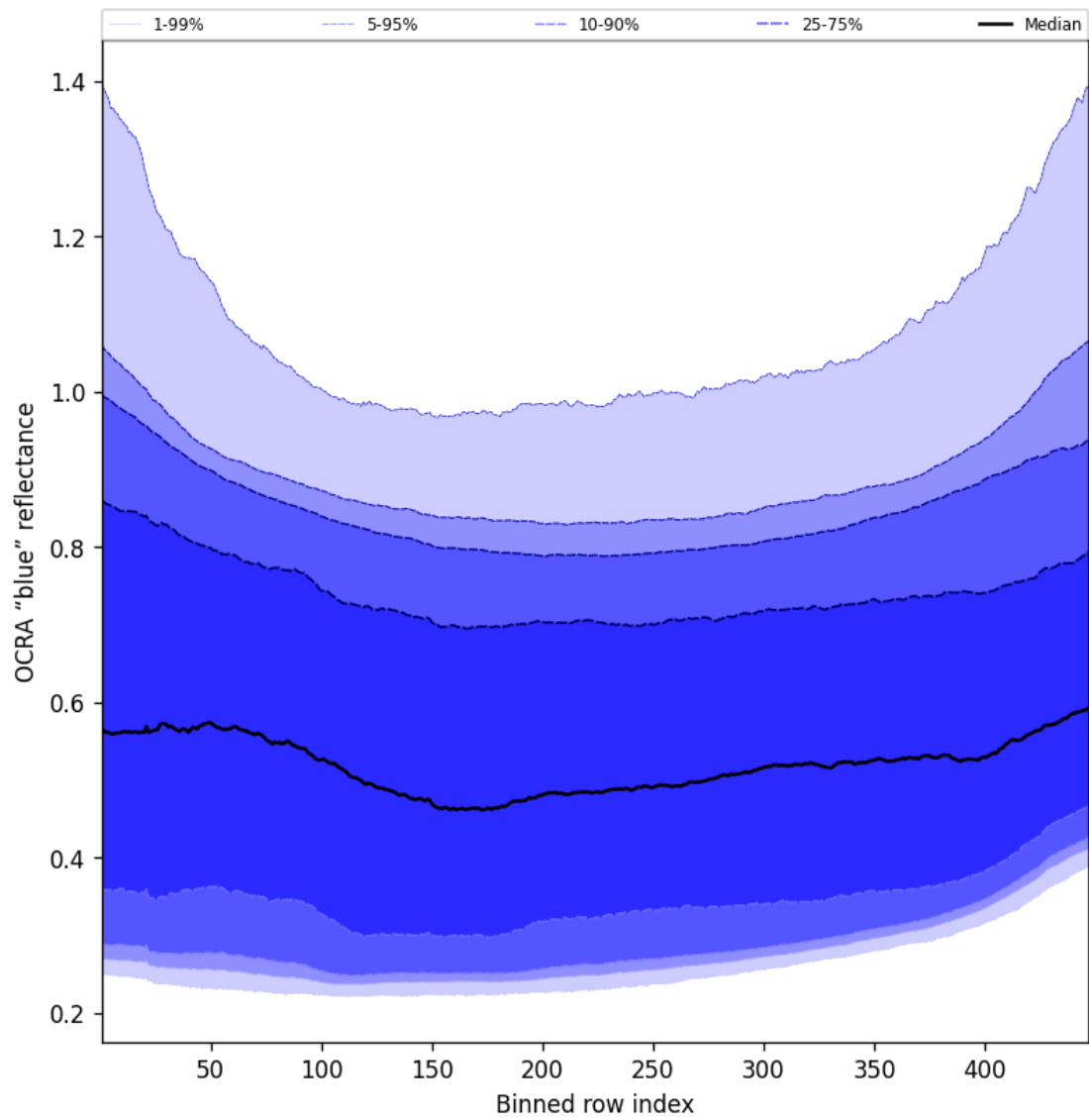
Figure 67: Along track statistics of “OCRA “blue” reflectance” for 2024-09-28 to 2024-09-29
