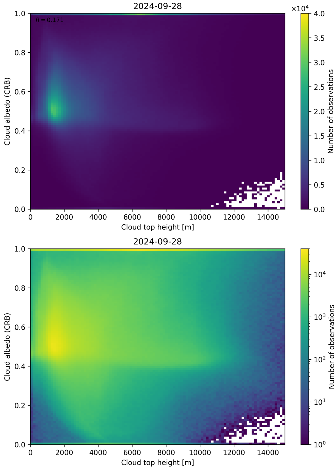
Figure 86: Scatter density plot of “Cloud top height” against “Cloud albedo (CRB)” for 2024-09-28 to 2024-09-29.
