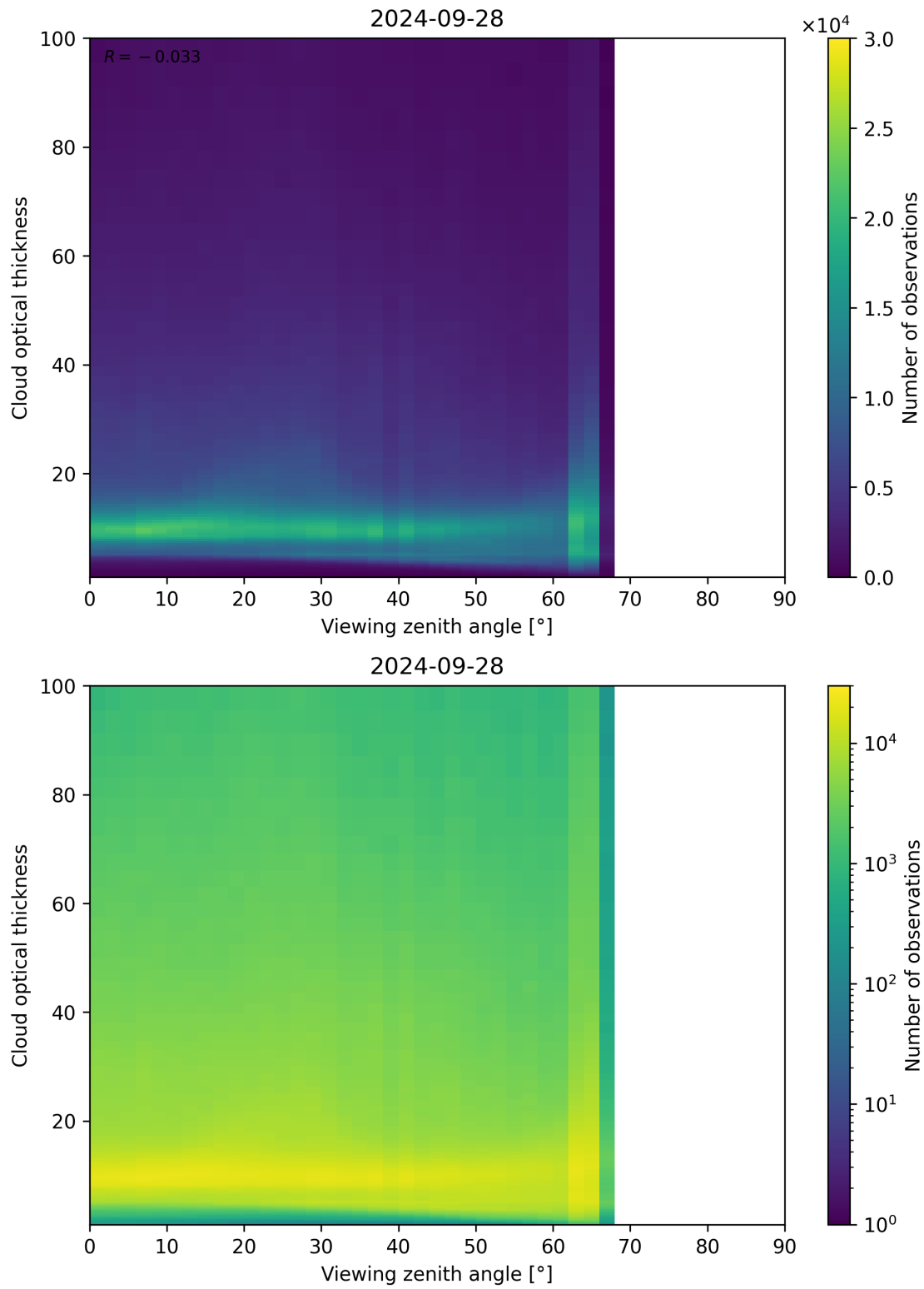
Figure 111: Scatter density plot of “Viewing zenith angle” against “Cloud optical thickness” for 2024-09-28 to 2024-09-29.
