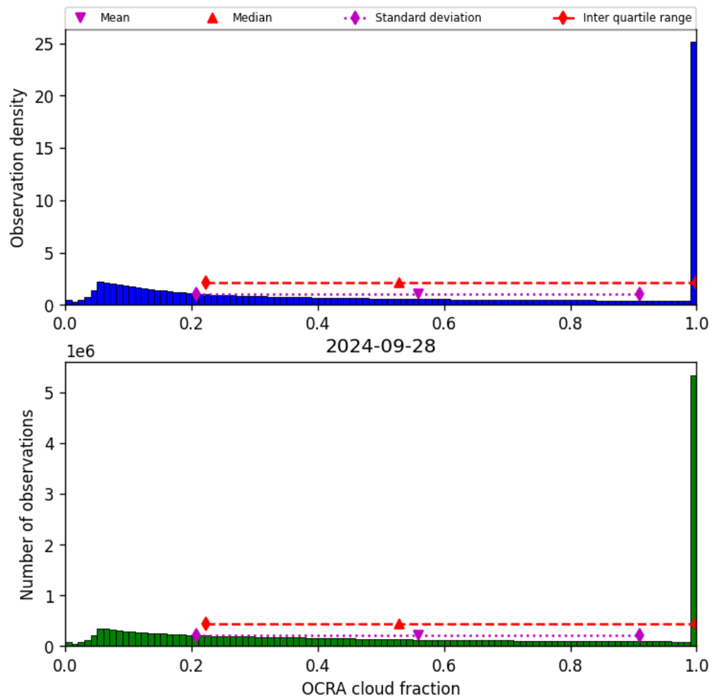
Figure 50: Histogram of “OCRA cloud fraction” for 2024-09-28 to 2024-09-29
