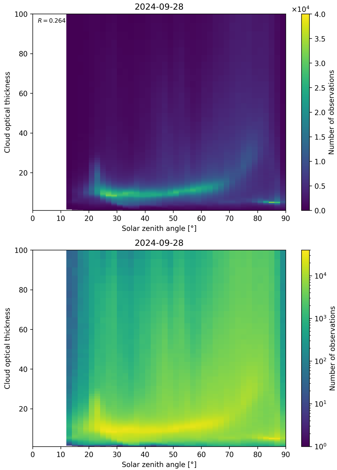
Figure 103: Scatter density plot of “Solar zenith angle” against “Cloud optical thickness” for 2024-09-28 to 2024-09-29.
