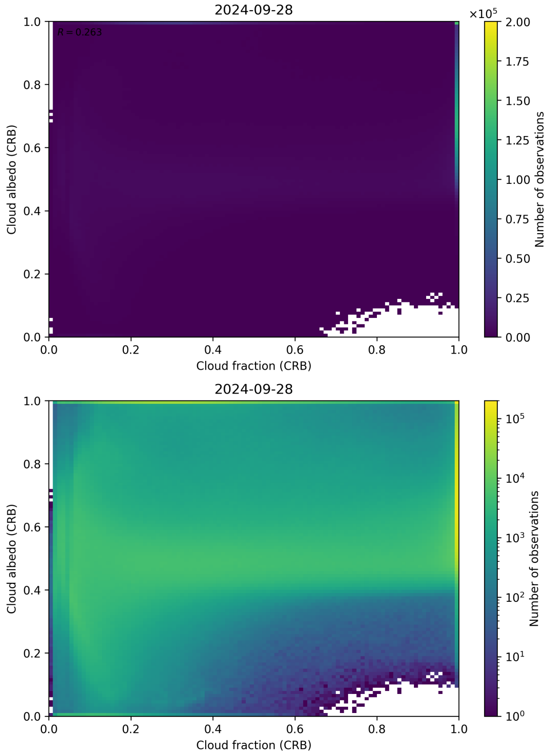
Figure 77: Scatter density plot of “Cloud fraction (CRB)” against “Cloud albedo (CRB)” for 2024-09-28 to 2024-09-29.
