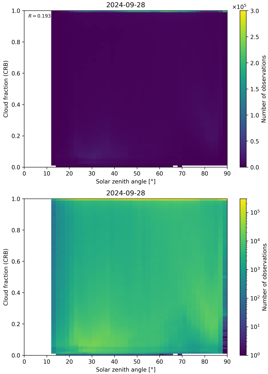
Figure 101: Scatter density plot of “Solar zenith angle” against “Cloud fraction (CRB)” for 2024-09-28 to 2024-09-29.
