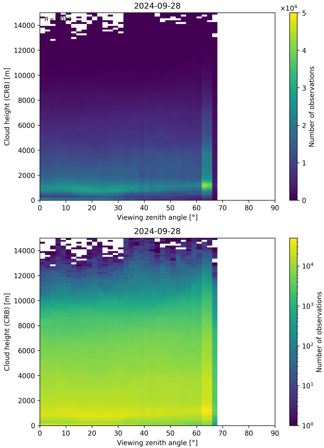
Figure 110: Scatter density plot of “Viewing zenith angle” against “Cloud height (CRB)” for 2024-09-28 to 2024-09-29.
