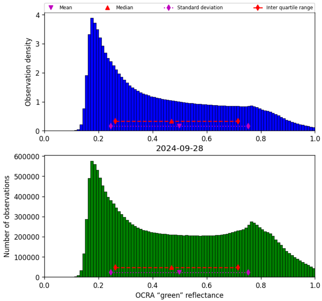
Figure 52: Histogram of “OCRA “green” reflectance” for 2024-09-28 to 2024-09-29
