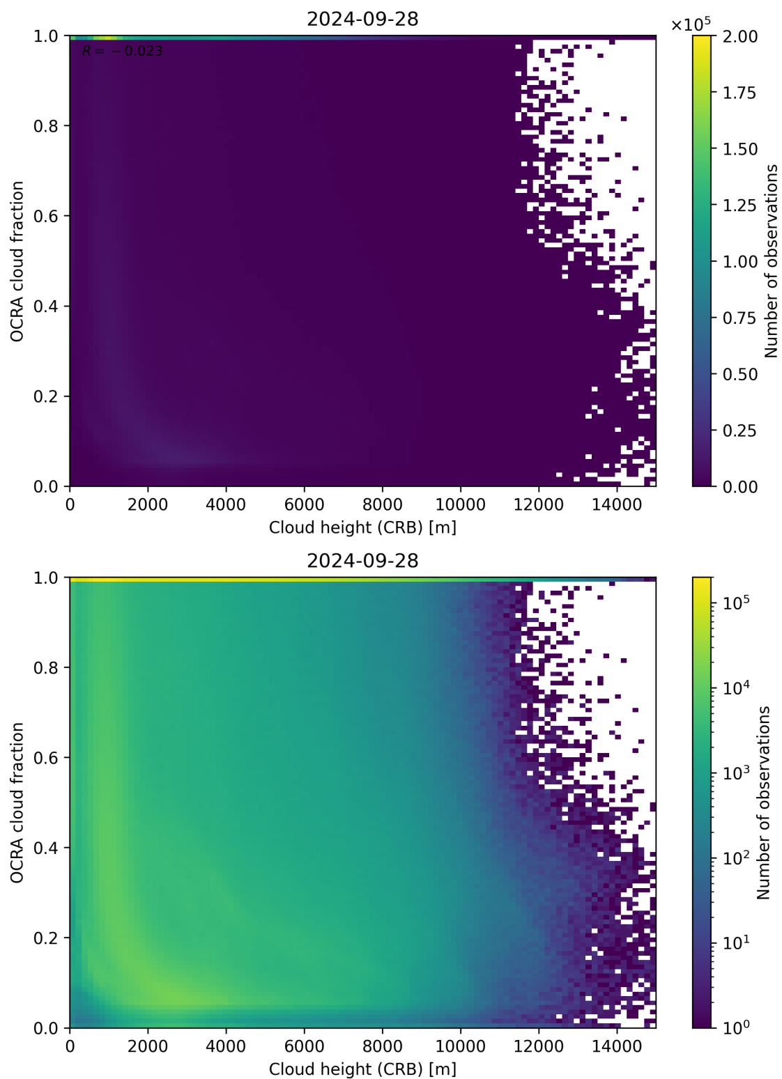
Figure 81: Scatter density plot of “Cloud height (CRB)” against “OCRA cloud fraction” for 2024-09-28 to 2024-09-29.
