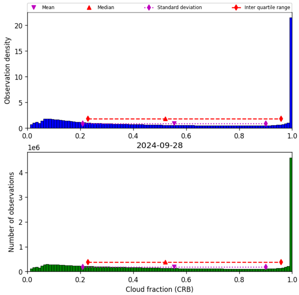
Figure 42: Histogram of “Cloud fraction (CRB)” for 2024-09-28 to 2024-09-29
