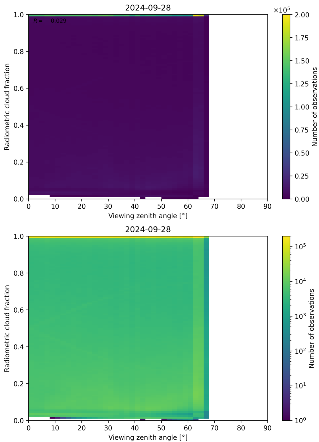
Figure 107: Scatter density plot of “Viewing zenith angle” against “Radiometric cloud fraction” for 2024-09-28 to 2024-09-29.
