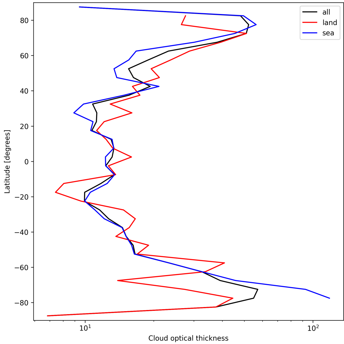
Figure 25: Zonal average of “Cloud optical thickness” for 2024-09-28 to 2024-09-29.
