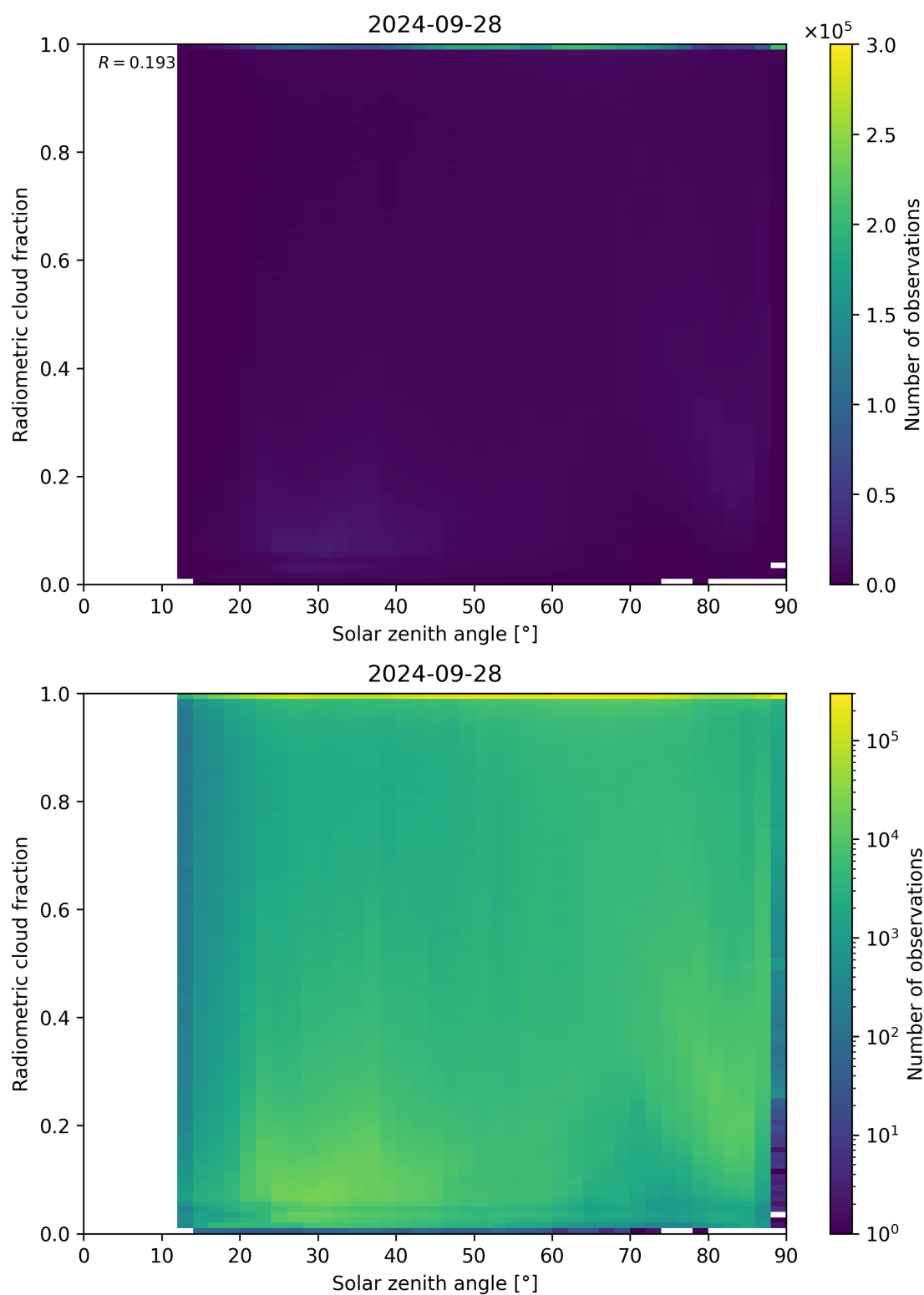
Figure 99: Scatter density plot of “Solar zenith angle” against “Radiometric cloud fraction” for 2024-09-28 to 2024-09-29.
