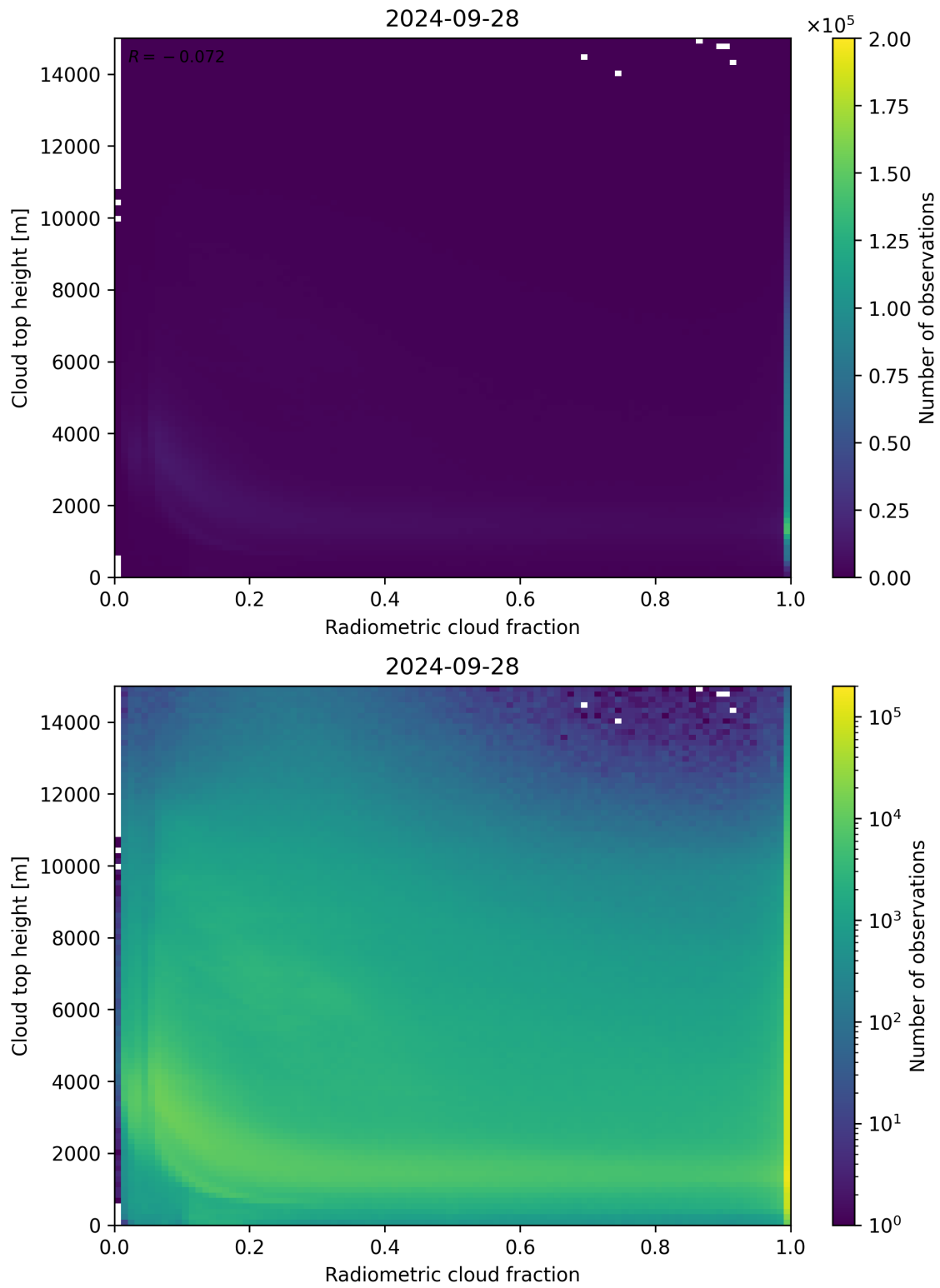
Figure 76: Scatter density plot of “Radiometric cloud fraction” against “Cloud top height” for 2024-09-28 to 2024-09-29.
