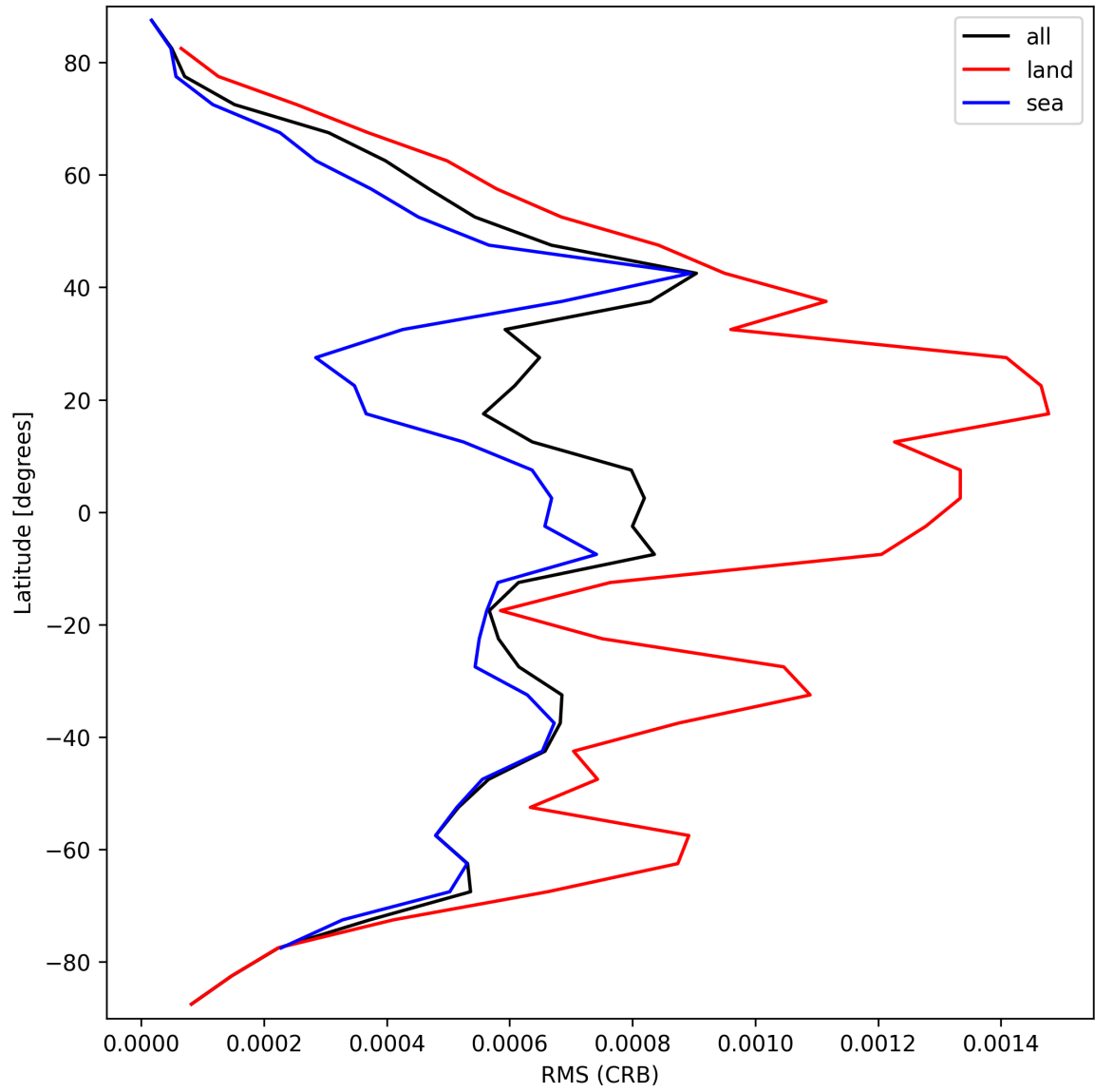
Figure 32: Zonal average of “RMS (CRB)” for 2024-09-28 to 2024-09-29.
