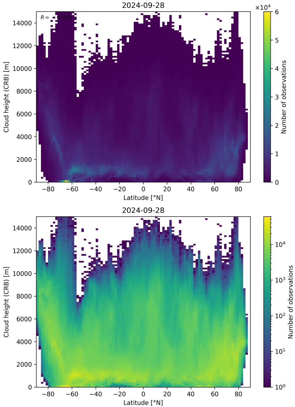
Figure 95: Scatter density plot of “Latitude” against “Cloud height (CRB)” for 2024-09-28 to 2024-09-29.
