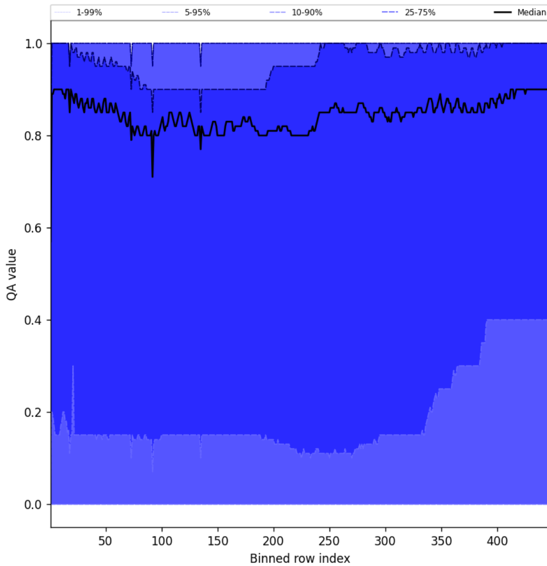
Figure 54: Along track statistics of “QA value” for 2024-09-28 to 2024-09-29
