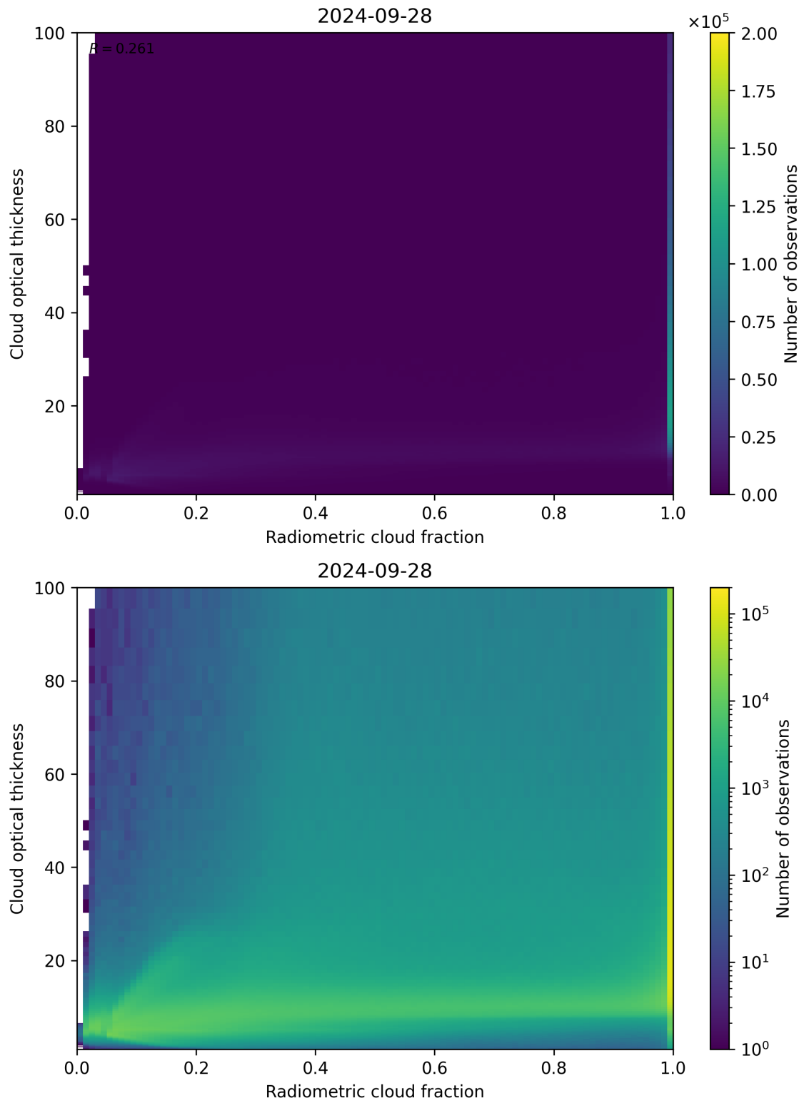
Figure 75: Scatter density plot of “Radiometric cloud fraction” against “Cloud optical thickness” for 2024-09-28 to 2024-09-29.
