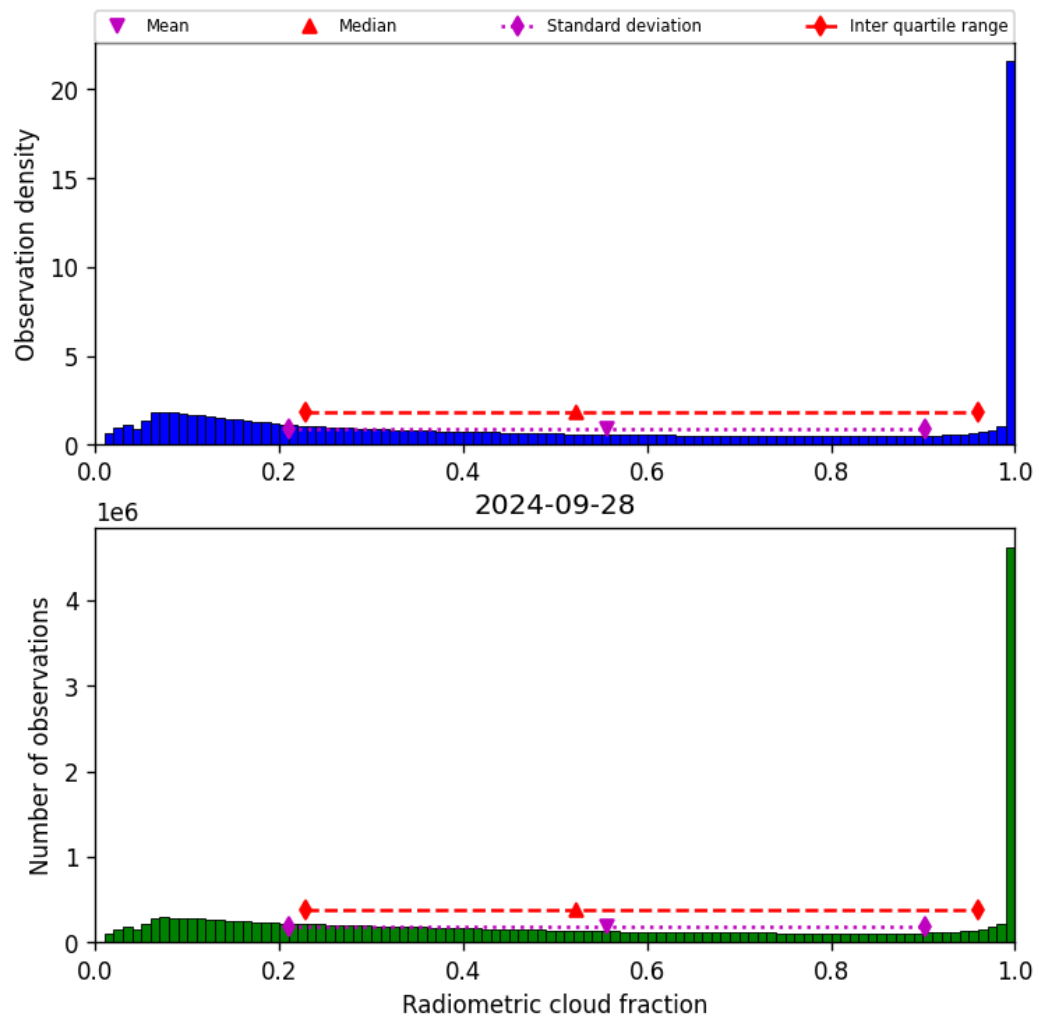
Figure 39: Histogram of “Radiometric cloud fraction” for 2024-09-28 to 2024-09-29
