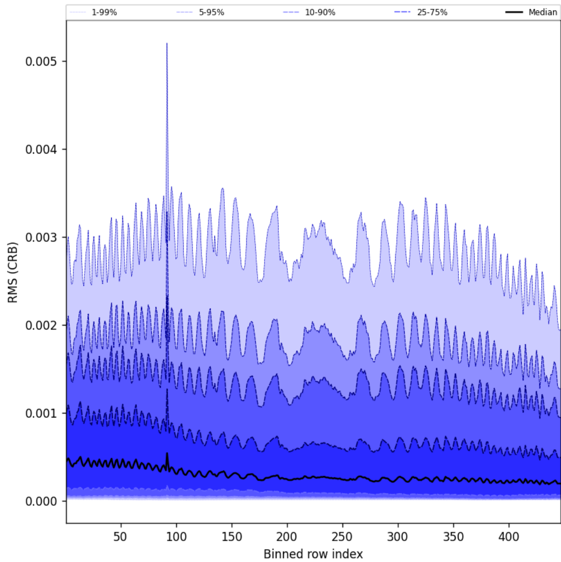
Figure 64: Along track statistics of “RMS (CRB)” for 2024-09-28 to 2024-09-29
