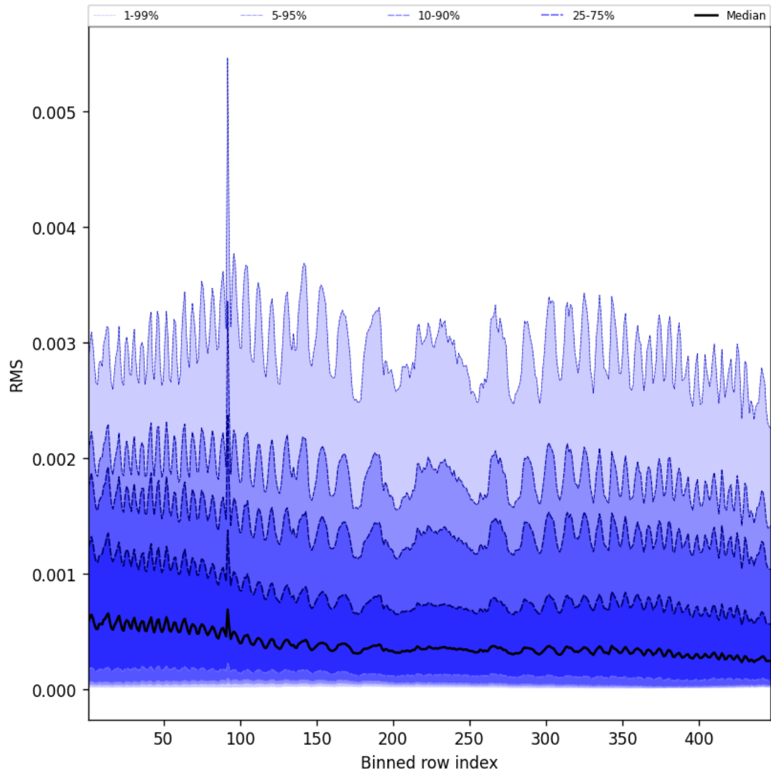
Figure 63: Along track statistics of “RMS” for 2024-09-28 to 2024-09-29
