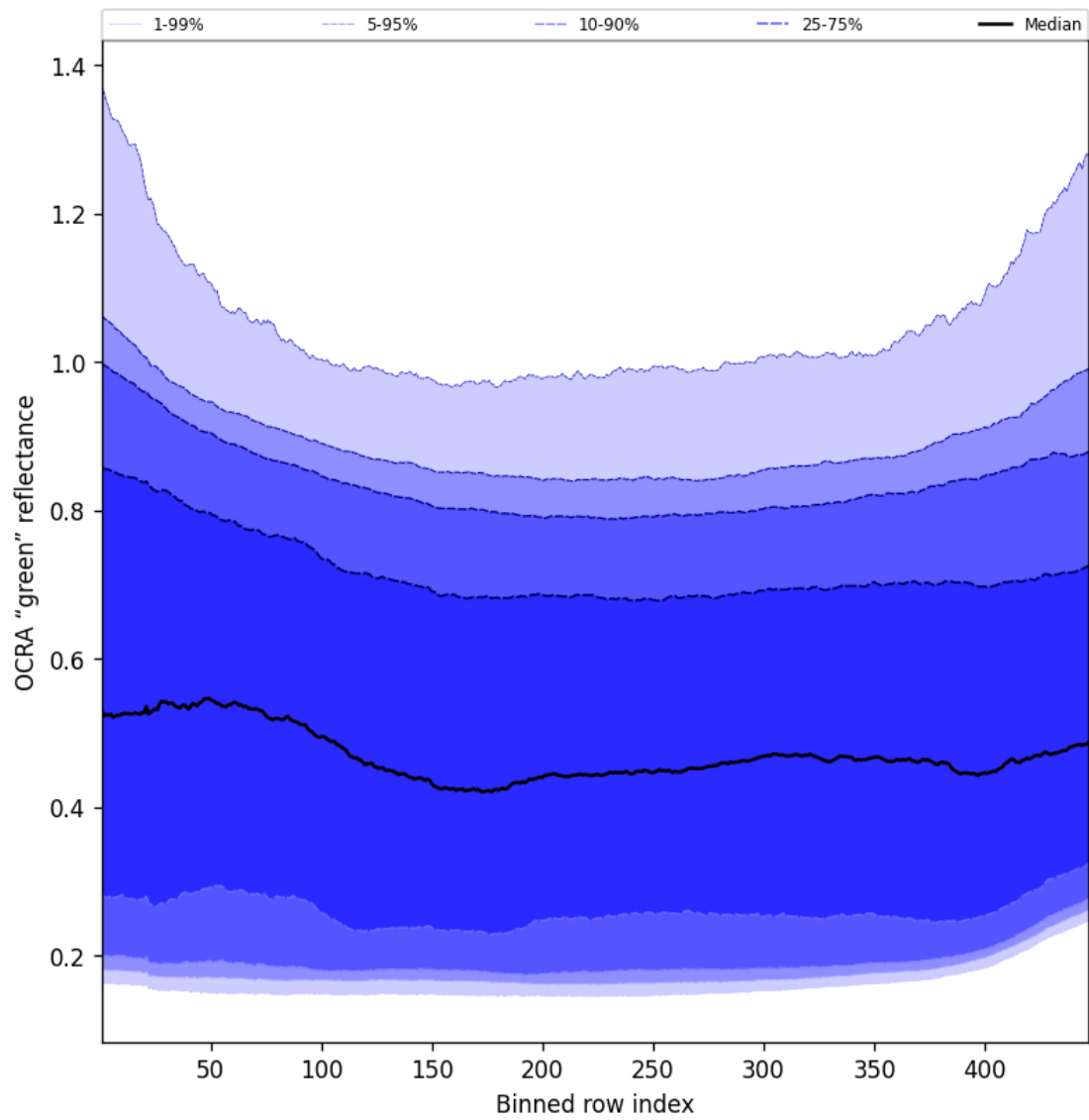
Figure 68: Along track statistics of “OCRA “green” reflectance” for 2024-09-28 to 2024-09-29
