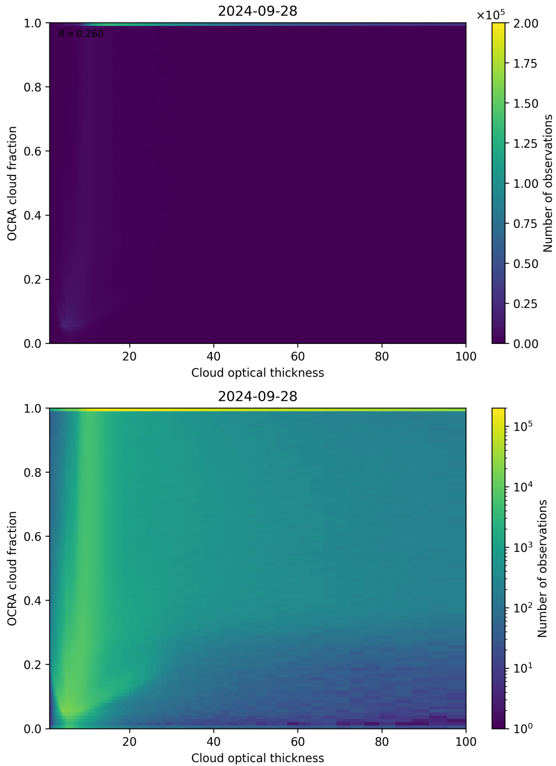
Figure 83: Scatter density plot of “Cloud optical thickness” against “OCRA cloud fraction” for 2024-09-28 to 2024-09-29.
