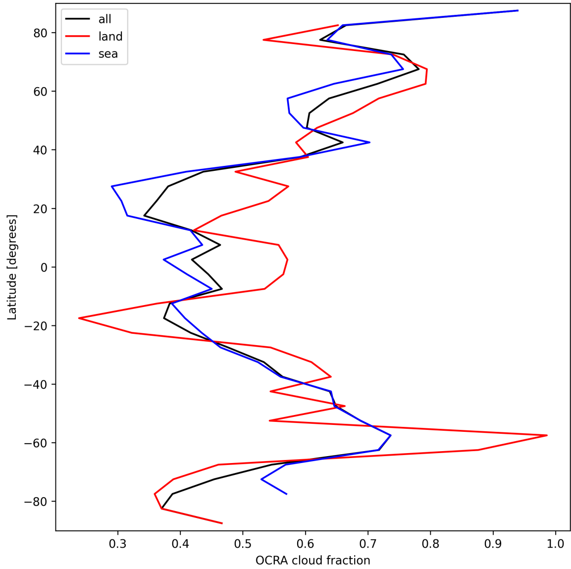
Figure 34: Zonal average of “OCRA cloud fraction” for 2024-09-28 to 2024-09-29.
