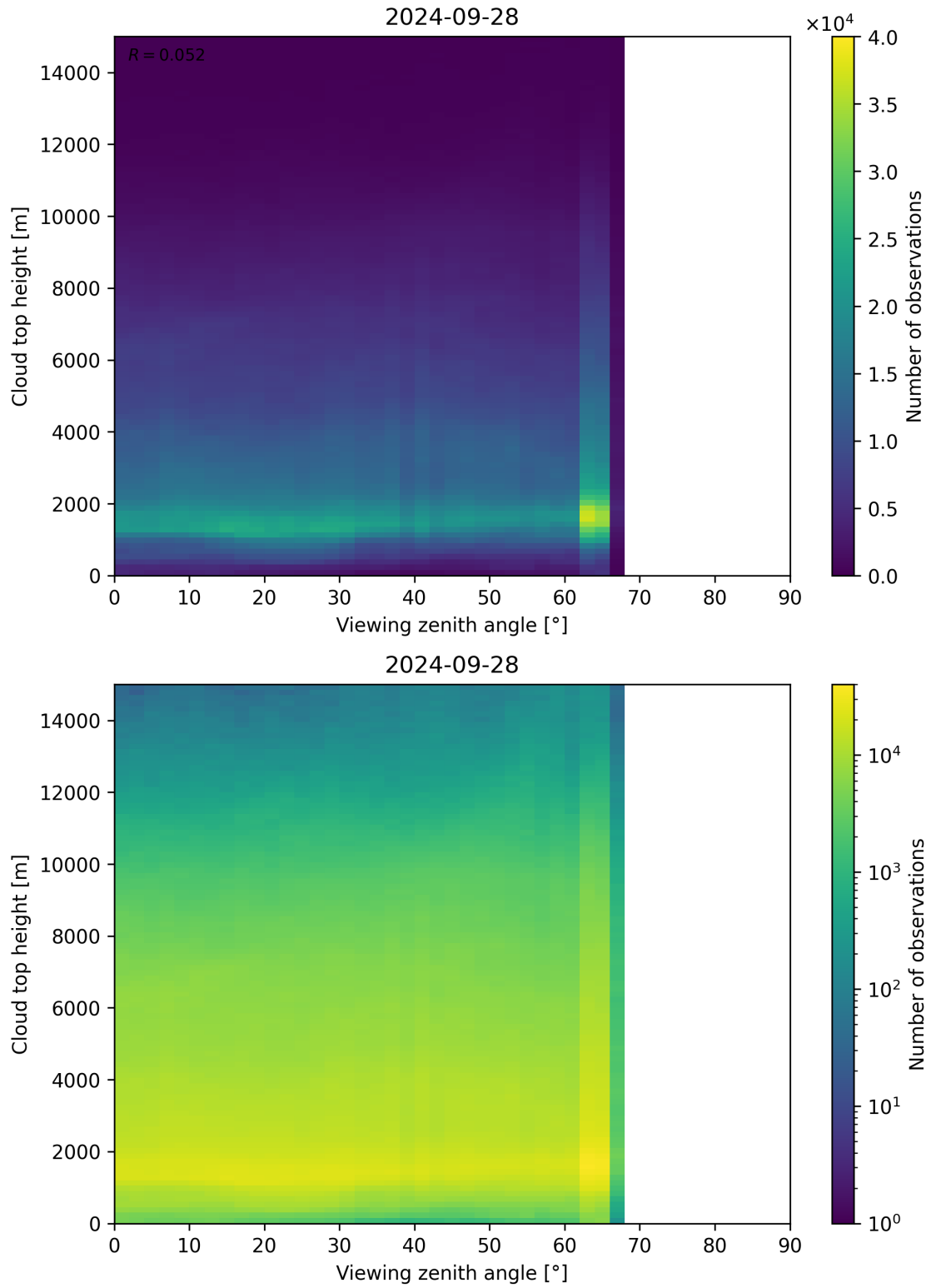
Figure 112: Scatter density plot of “Viewing zenith angle” against “Cloud top height” for 2024-09-28 to 2024-09-29.
