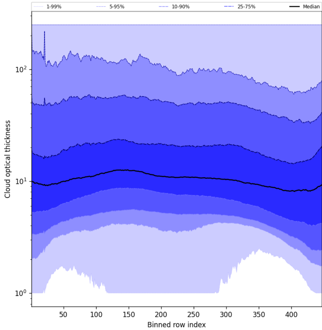
Figure 57: Along track statistics of “Cloud optical thickness” for 2024-09-28 to 2024-09-29
