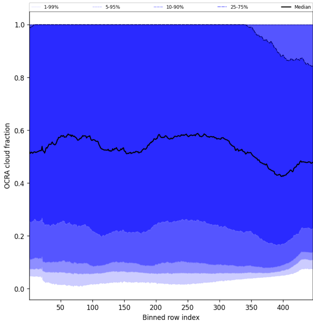
Figure 66: Along track statistics of “OCRA cloud fraction” for 2024-09-28 to 2024-09-29
