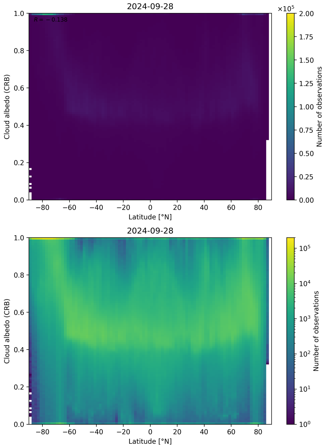
Figure 91: Scatter density plot of “Latitude” against “Cloud albedo (CRB)” for 2024-09-28 to 2024-09-29.
