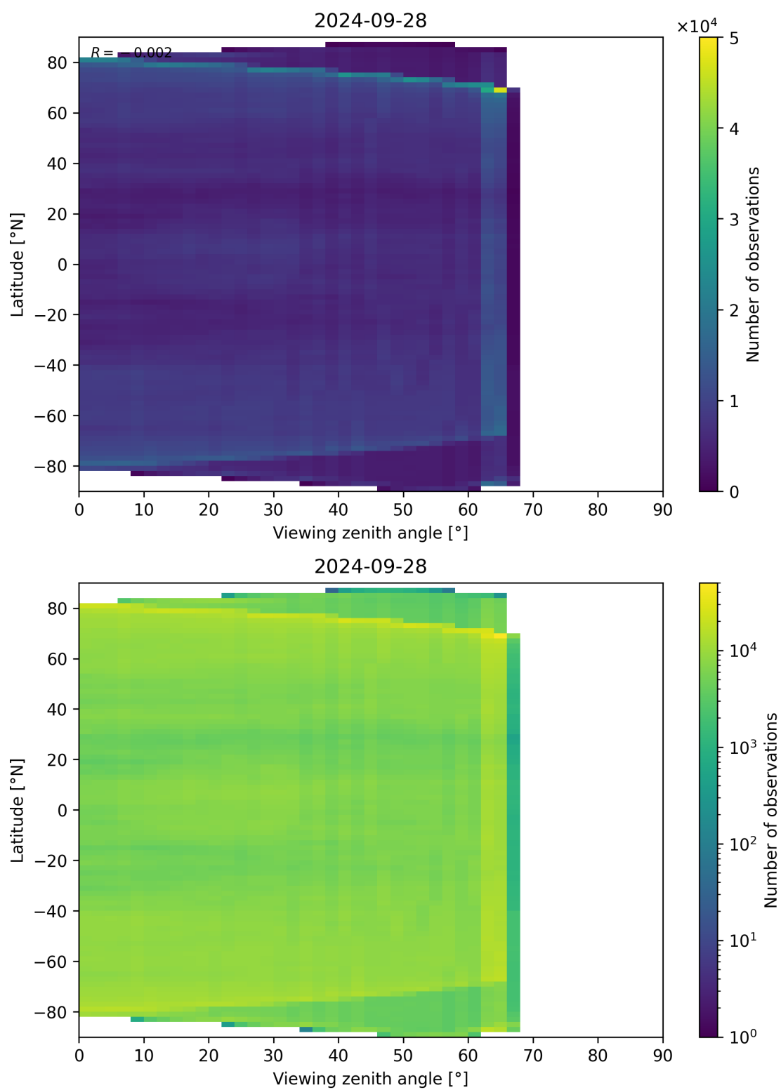
Figure 113: Scatter density plot of “Viewing zenith angle” against “Latitude” for 2024-09-28 to 2024-09-29.
