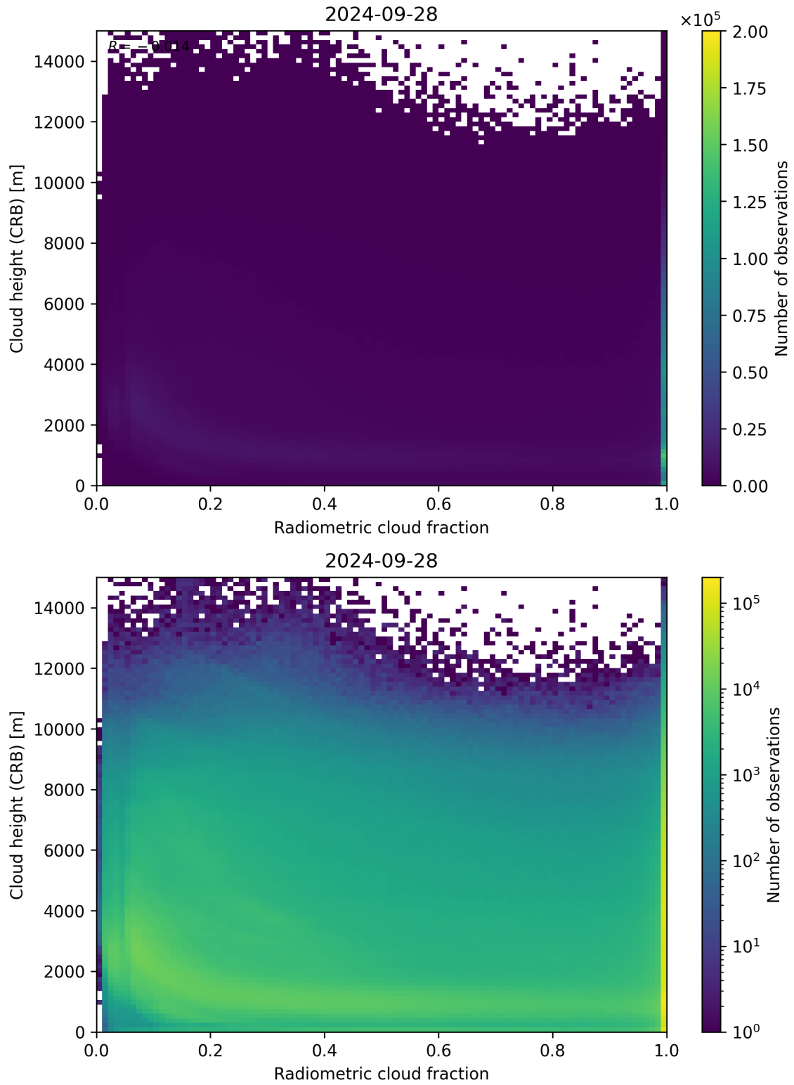
Figure 74: Scatter density plot of “Radiometric cloud fraction” against “Cloud height (CRB)” for 2024-09-28 to 2024-09-29.
