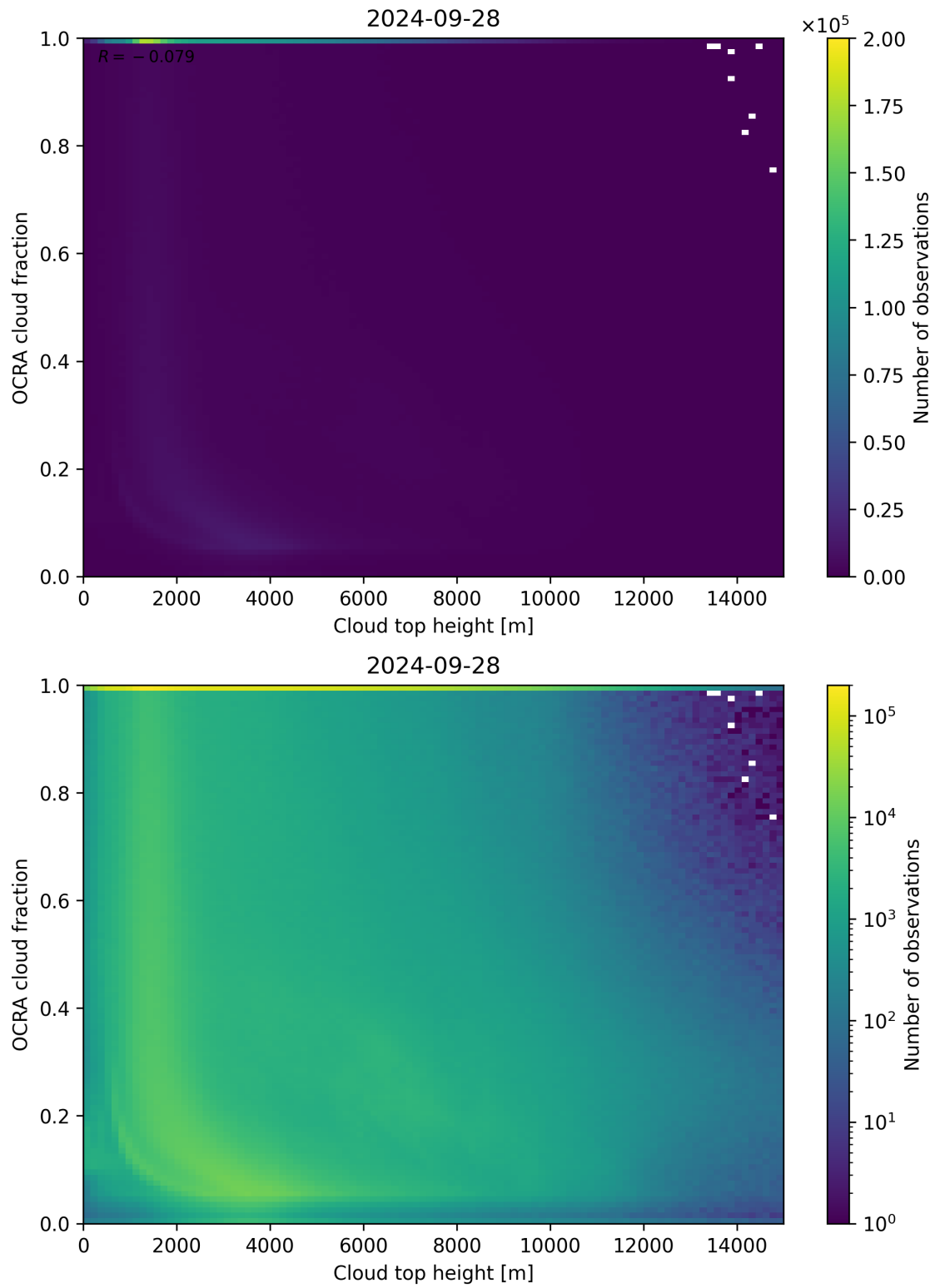
Figure 87: Scatter density plot of “Cloud top height” against “OCRA cloud fraction” for 2024-09-28 to 2024-09-29.
