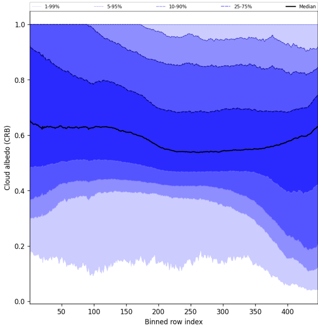
Figure 60: Along track statistics of “Cloud albedo (CRB)” for 2024-09-28 to 2024-09-29
