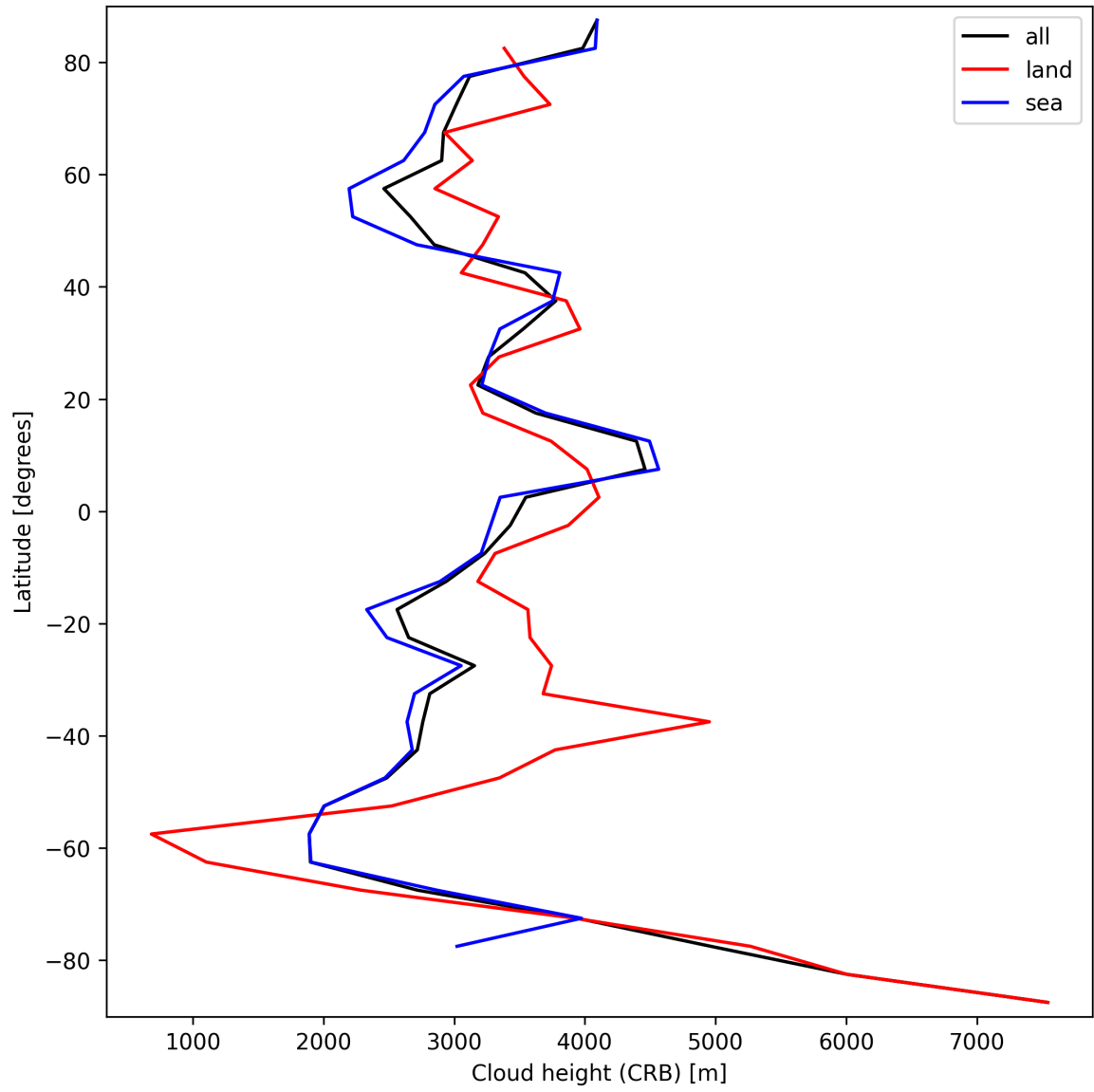
Figure 27: Zonal average of “Cloud height (CRB)” for 2024-09-28 to 2024-09-29.
