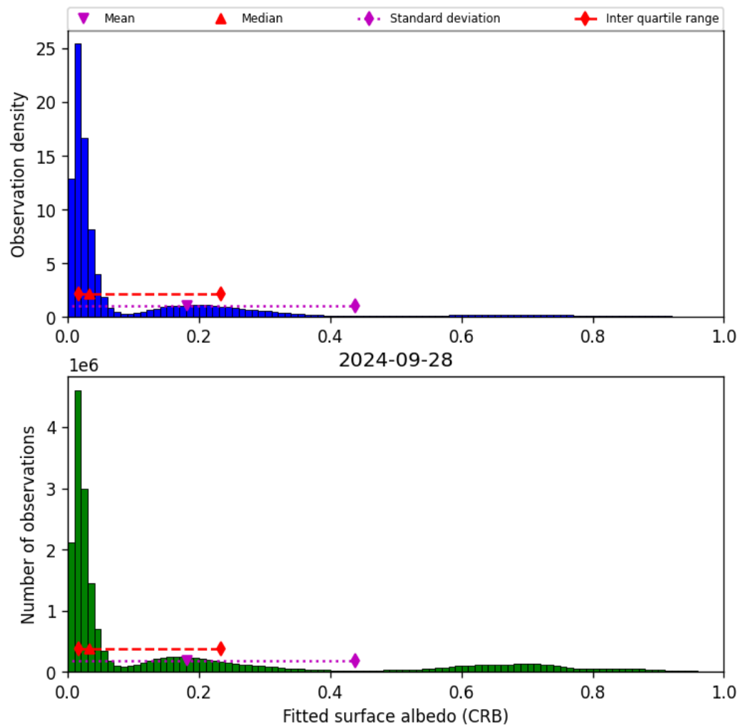
Figure 46: Histogram of “Fitted surface albedo (CRB)” for 2024-09-28 to 2024-09-29
