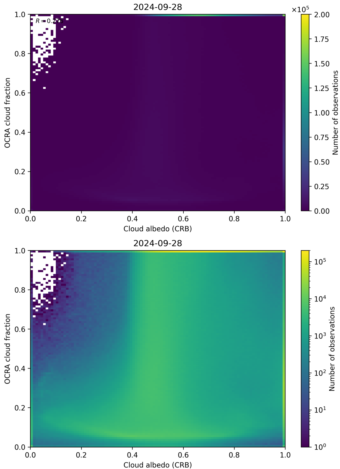
Figure 70: Scatter density plot of “Cloud albedo (CRB)” against “OCRA cloud fraction” for 2024-09-28 to 2024-09-29.
