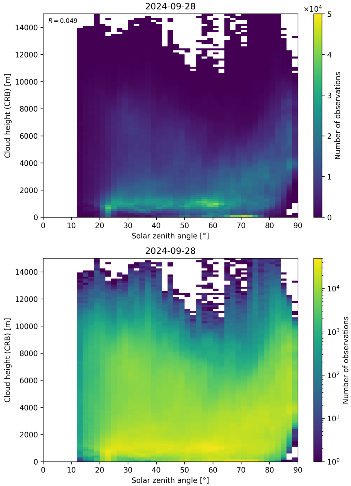
Figure 102: Scatter density plot of “Solar zenith angle” against “Cloud height (CRB)” for 2024-09-28 to 2024-09-29.
