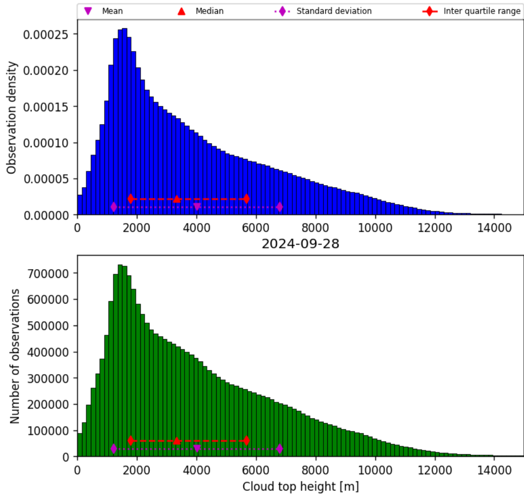
Figure 40: Histogram of “Cloud top height” for 2024-09-28 to 2024-09-29
