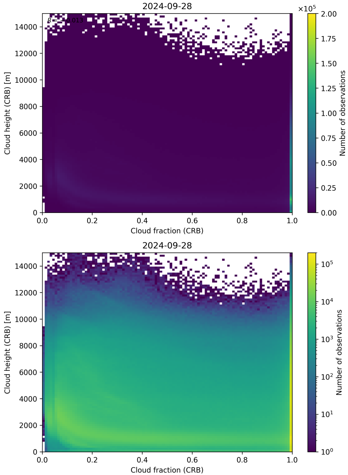
Figure 79: Scatter density plot of “Cloud fraction (CRB)” against “Cloud height (CRB)” for 2024-09-28 to 2024-09-29.
