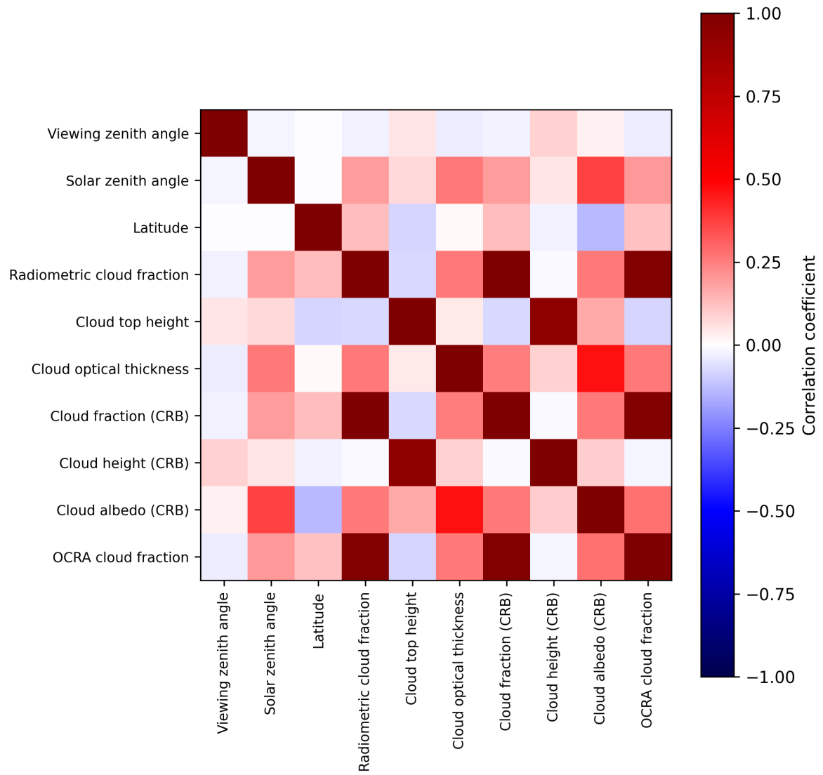
Figure 2: Map of correlation matrix for 2024-09-28 to 2024-09-29.
