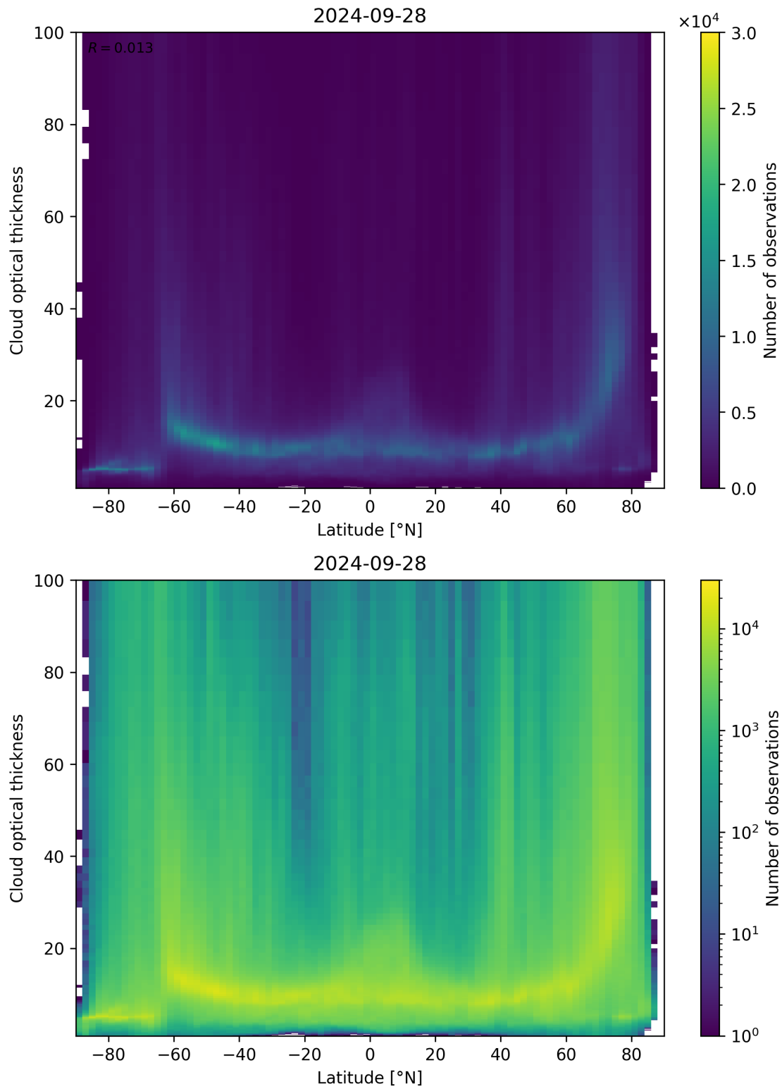
Figure 96: Scatter density plot of “Latitude” against “Cloud optical thickness” for 2024-09-28 to 2024-09-29.
