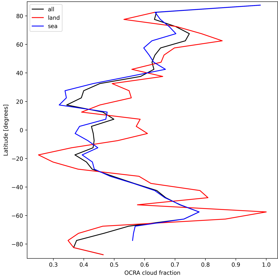
Figure 34: Zonal average of “OCRA cloud fraction” for 2024-09-28 to 2024-09-30.
