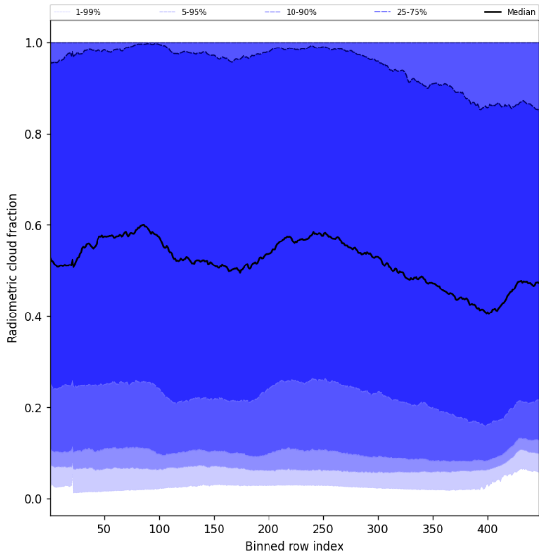
Figure 55: Along track statistics of “Radiometric cloud fraction” for 2024-09-29 to 2024-10-01
