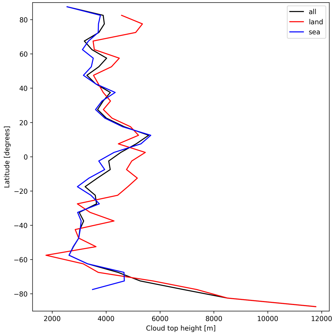
Figure 24: Zonal average of “Cloud top height” for 2024-09-29 to 2024-10-01.
