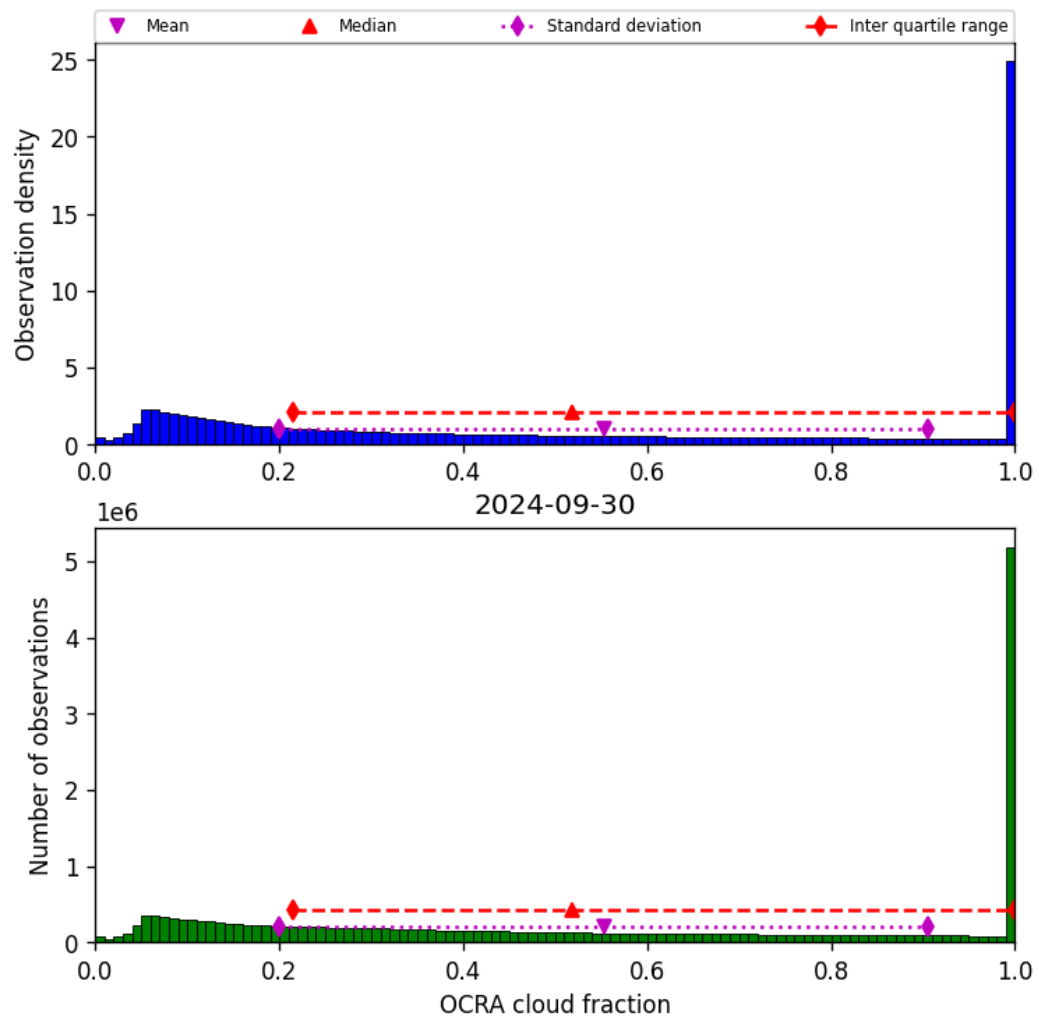
Figure 50: Histogram of “OCRA cloud fraction” for 2024-09-29 to 2024-10-01
