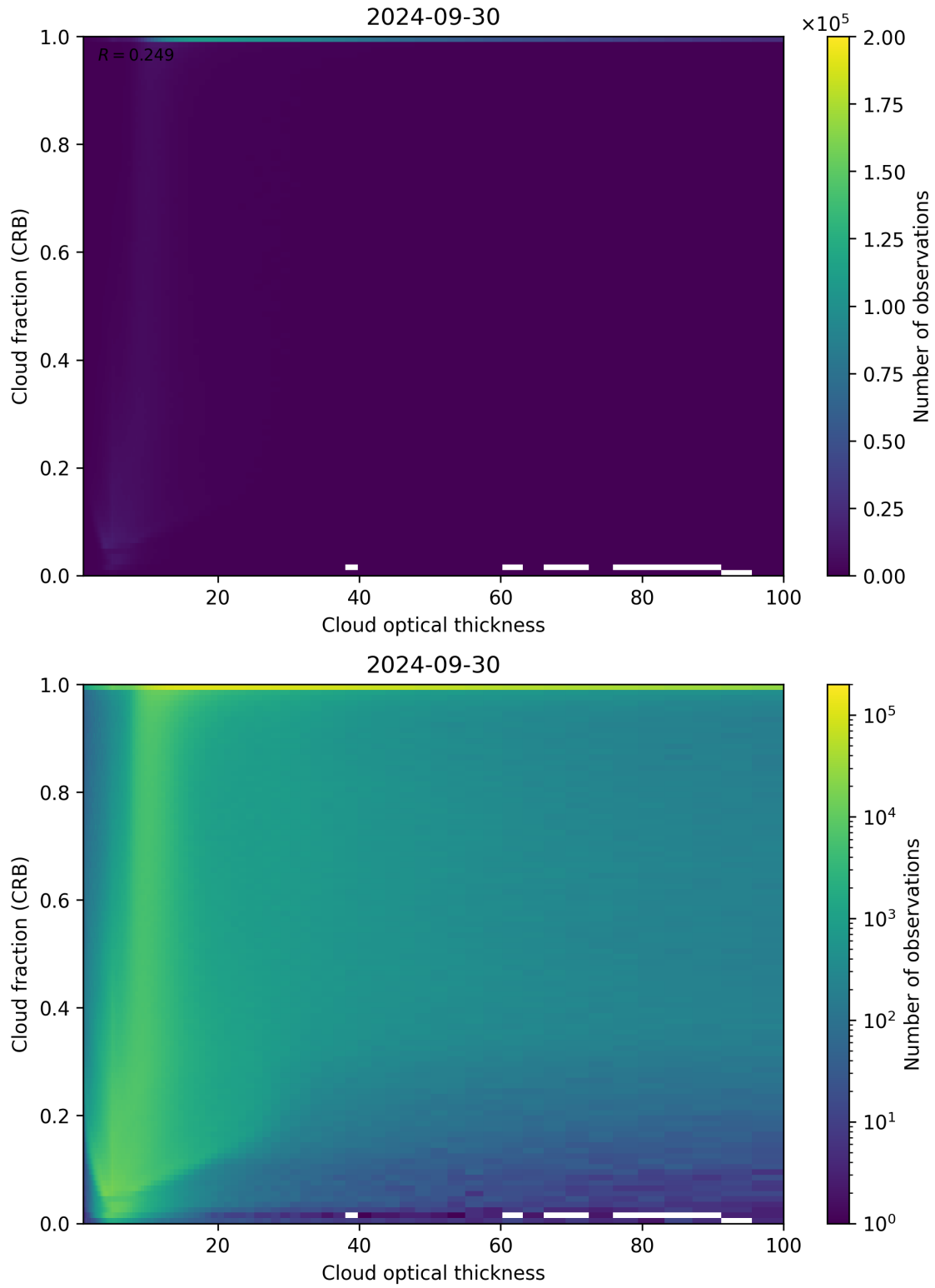
Figure 84: Scatter density plot of “Cloud optical thickness” against “Cloud fraction (CRB)” for 2024-09-29 to 2024-10-01.
