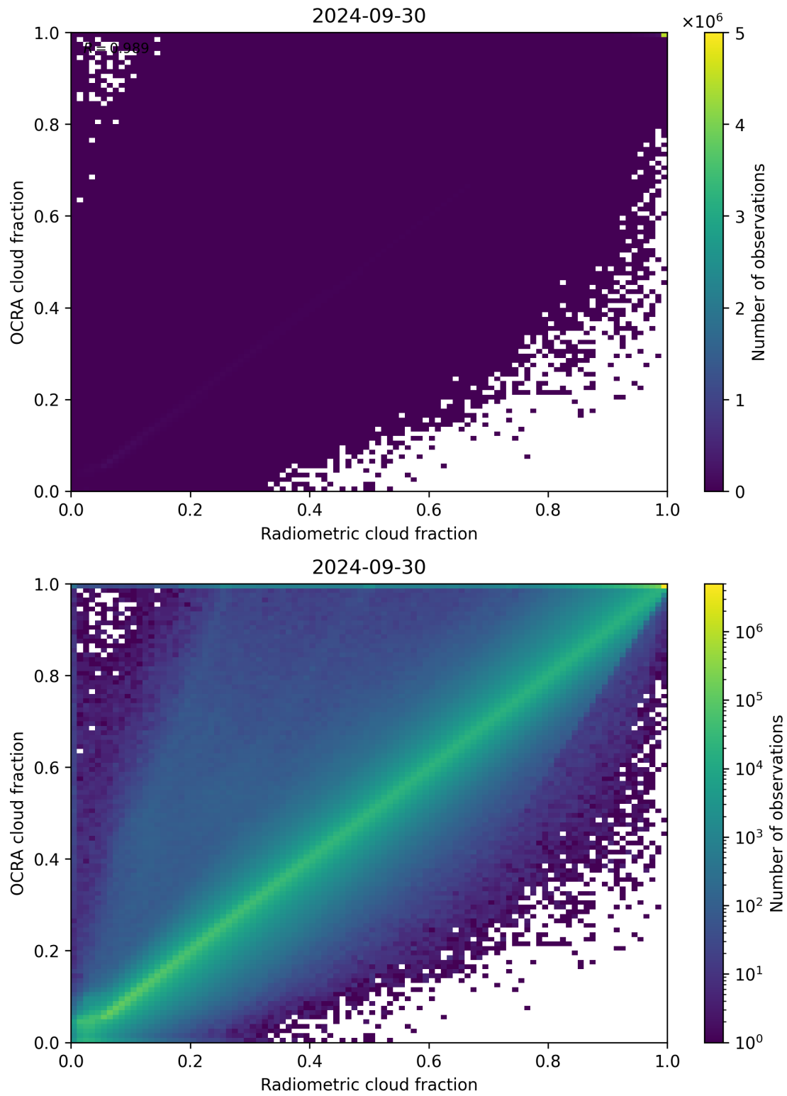
Figure 72: Scatter density plot of “Radiometric cloud fraction” against “OCRA cloud fraction” for 2024-09-29 to 2024-10-01.
