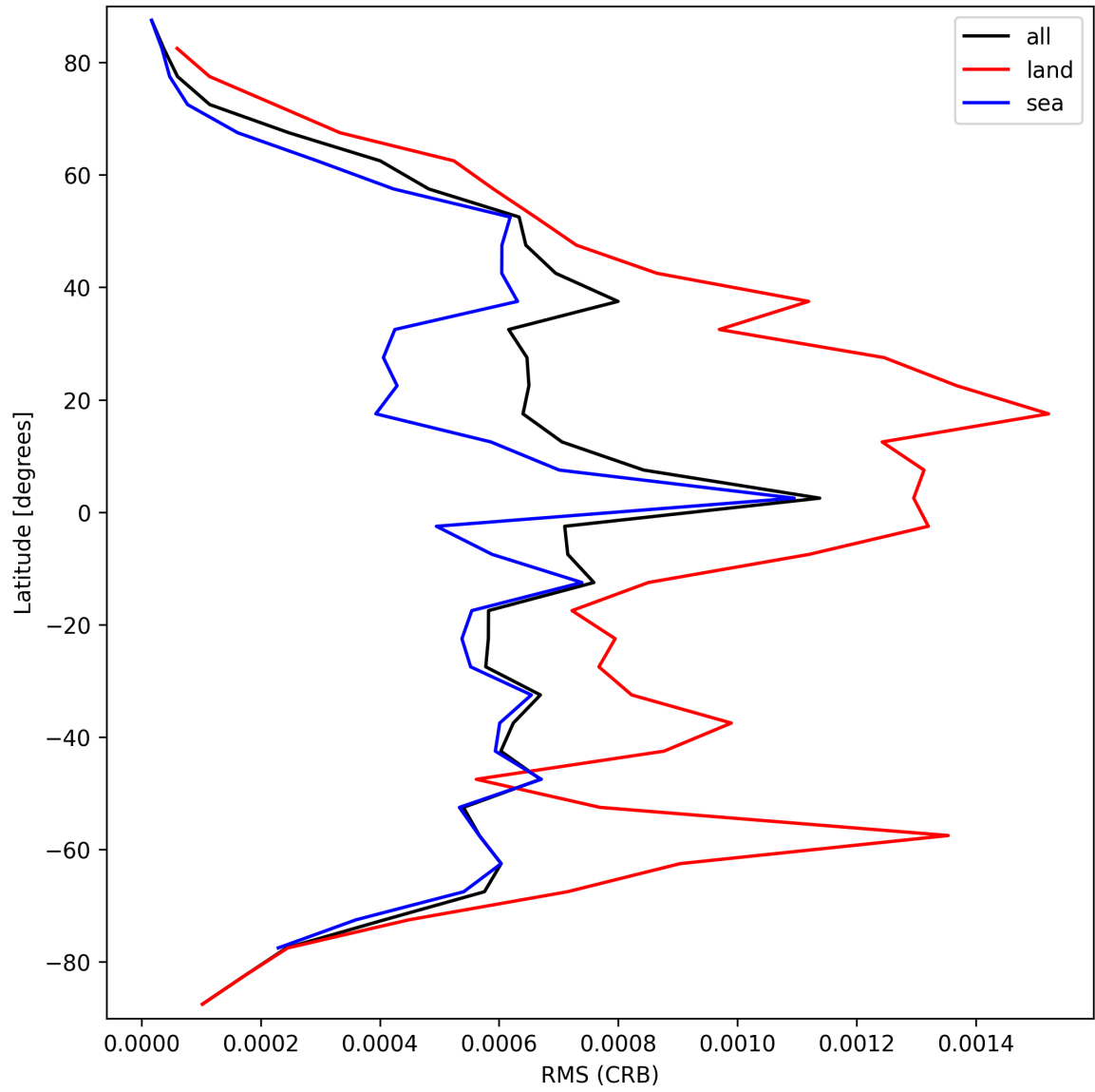
Figure 32: Zonal average of “RMS (CRB)” for 2024-09-29 to 2024-10-01.
