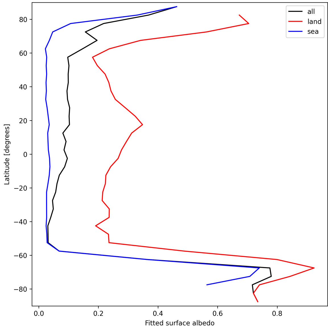
Figure 29: Zonal average of “Fitted surface albedo” for 2024-09-29 to 2024-10-01.
