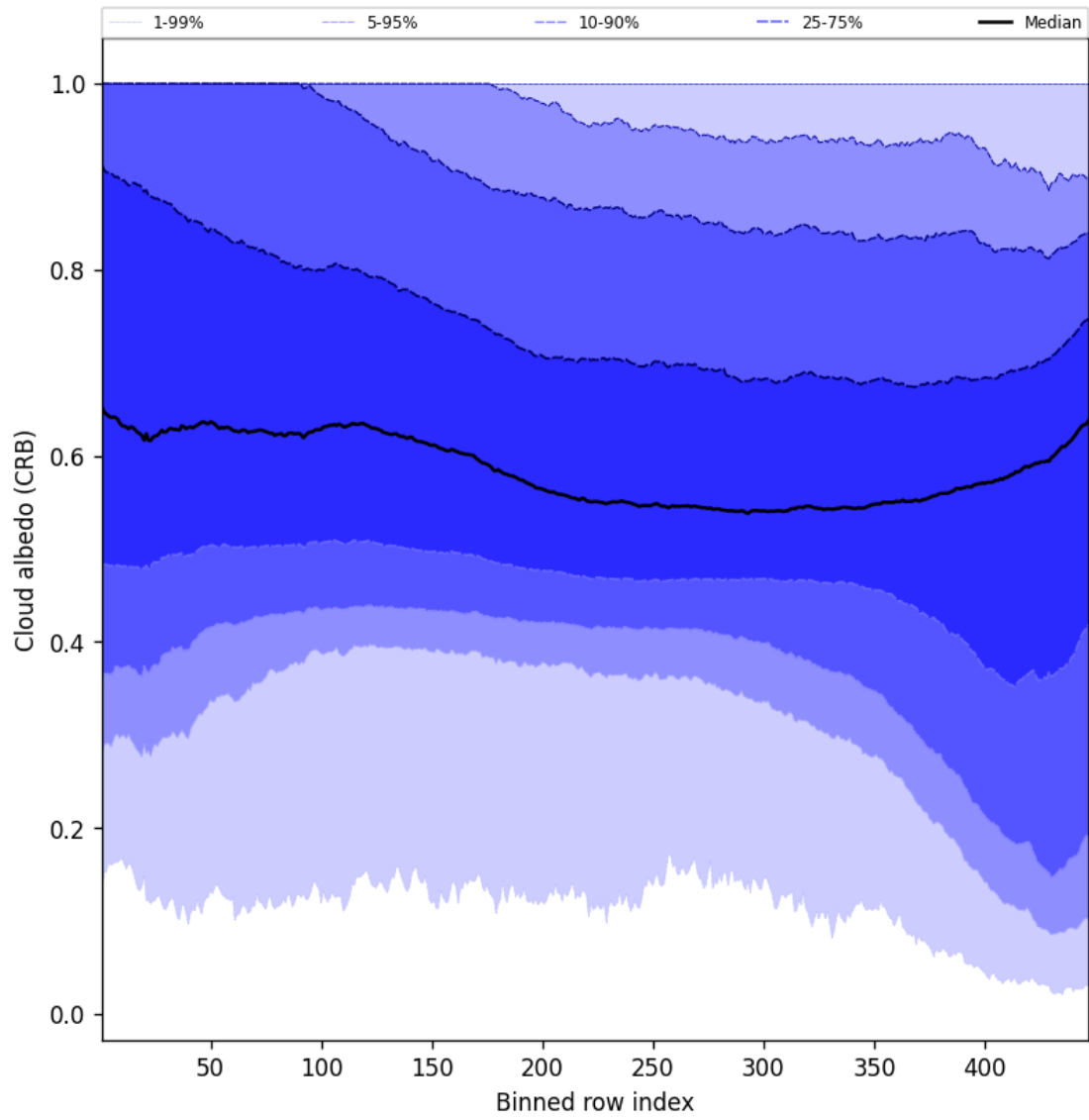
Figure 60: Along track statistics of “Cloud albedo (CRB)” for 2024-09-29 to 2024-10-01
