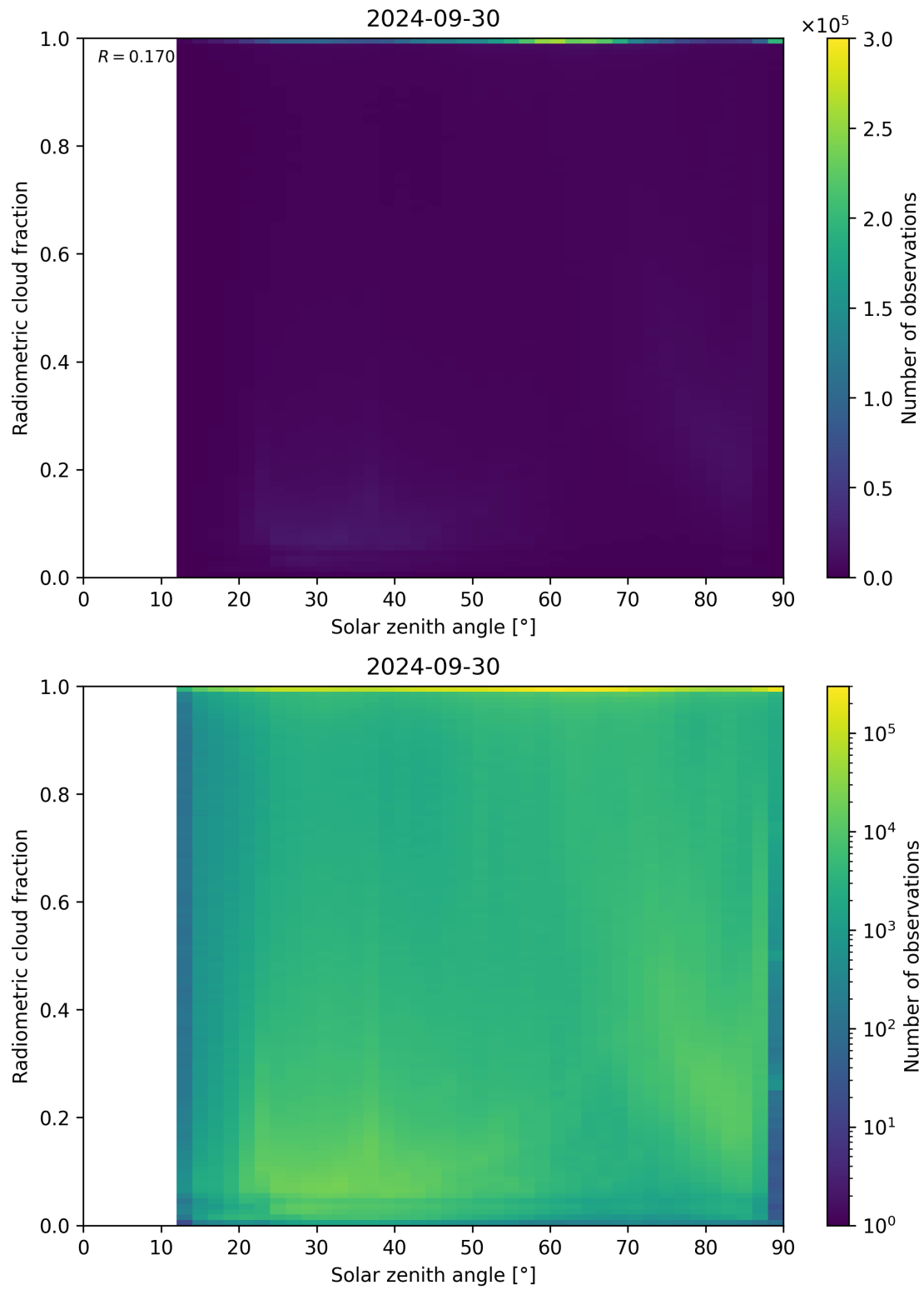
Figure 99: Scatter density plot of “Solar zenith angle” against “Radiometric cloud fraction” for 2024-09-29 to 2024-10-01.
