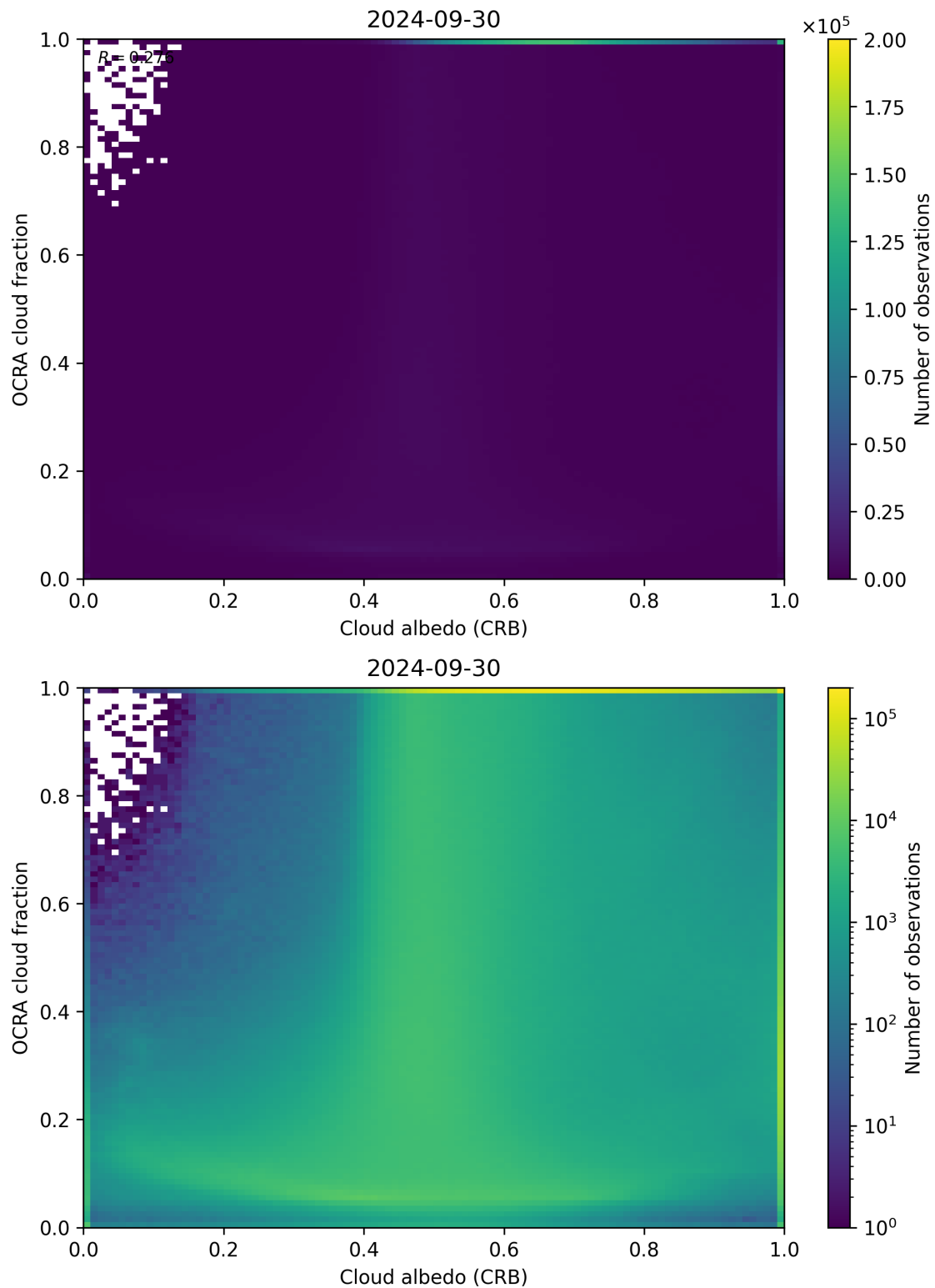
Figure 70: Scatter density plot of “Cloud albedo (CRB)” against “OCRA cloud fraction” for 2024-09-29 to 2024-10-01.
