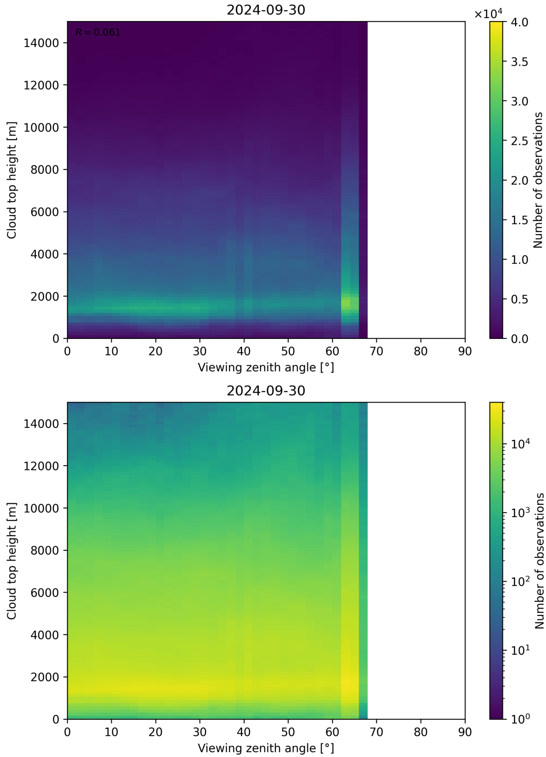
Figure 112: Scatter density plot of “Viewing zenith angle” against “Cloud top height” for 2024-09-29 to 2024-10-01.
