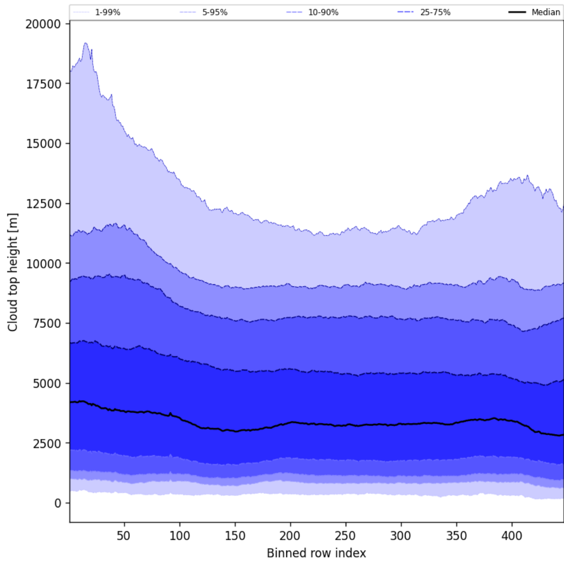
Figure 56: Along track statistics of “Cloud top height” for 2024-09-29 to 2024-10-01
