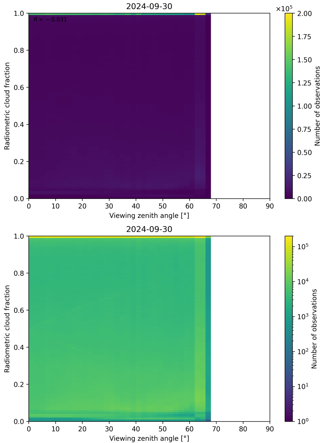
Figure 107: Scatter density plot of “Viewing zenith angle” against “Radiometric cloud fraction” for 2024-09-29 to 2024-10-01.
