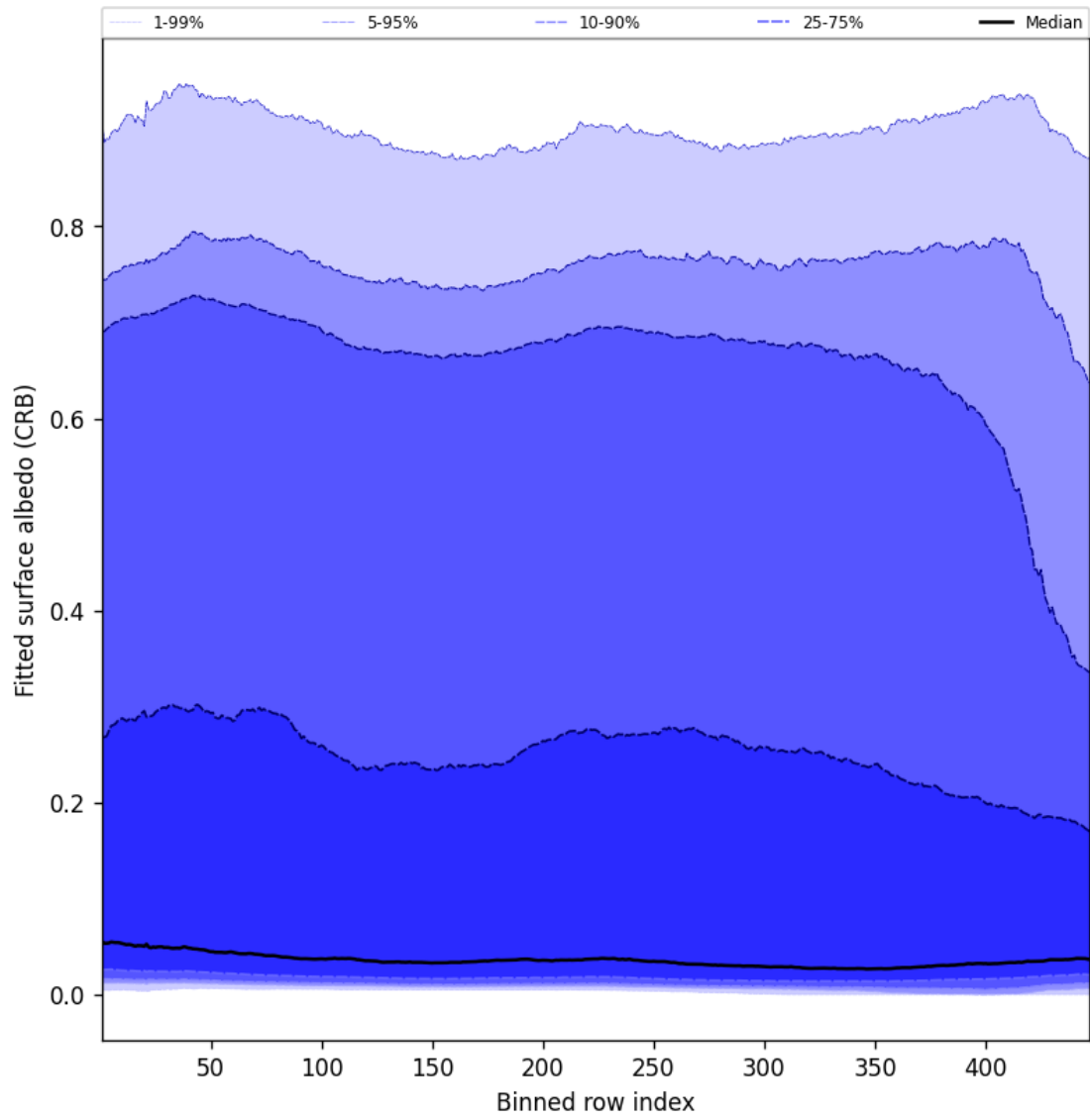
Figure 62: Along track statistics of “Fitted surface albedo (CRB)” for 2024-09-29 to 2024-10-01
