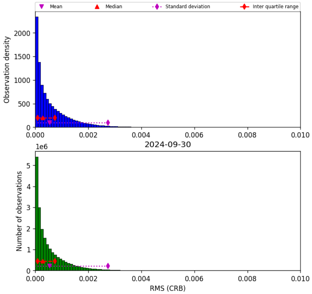
Figure 48: Histogram of “RMS (CRB)” for 2024-09-29 to 2024-10-01
