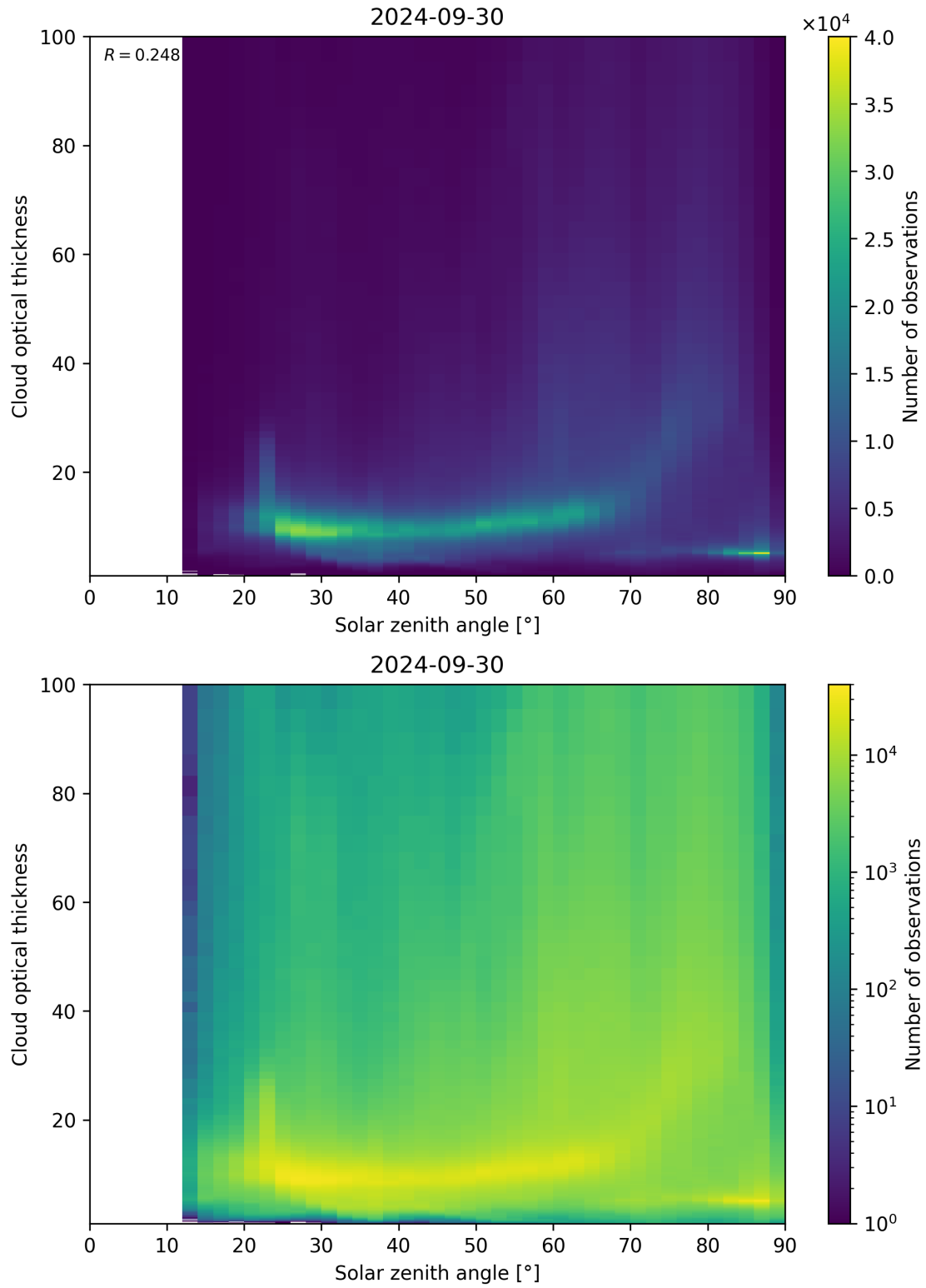
Figure 103: Scatter density plot of “Solar zenith angle” against “Cloud optical thickness” for 2024-09-29 to 2024-10-01.
