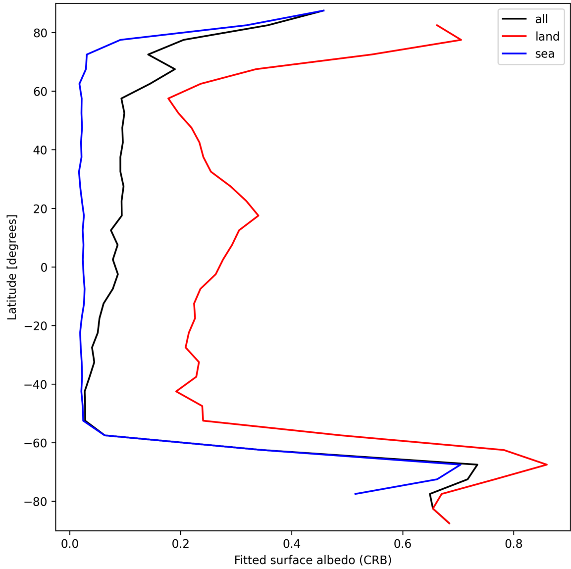
Figure 30: Zonal average of “Fitted surface albedo (CRB)” for 2024-09-29 to 2024-10-01.
