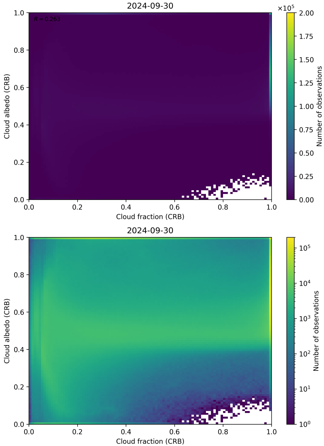
Figure 77: Scatter density plot of “Cloud fraction (CRB)” against “Cloud albedo (CRB)” for 2024-09-29 to 2024-10-01.
