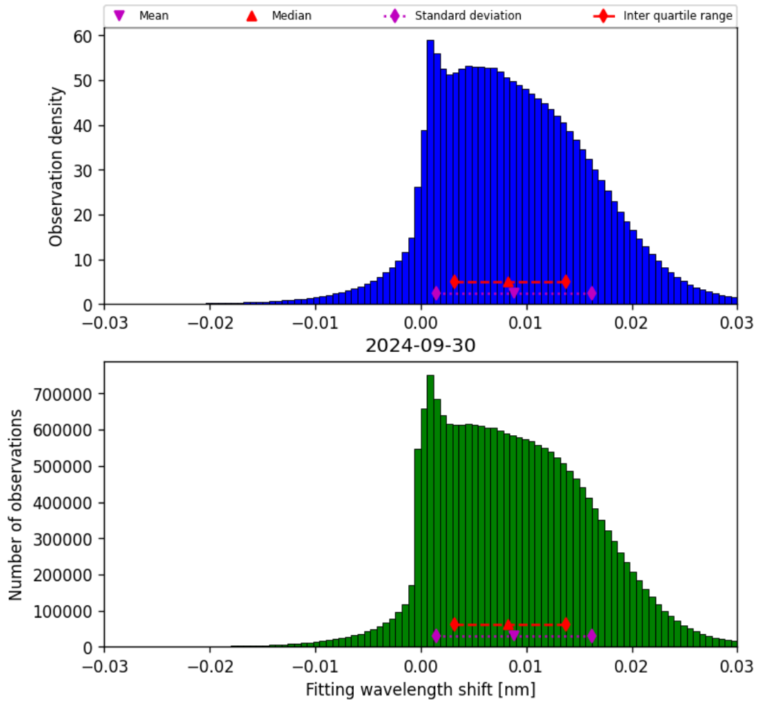
Figure 49: Histogram of “Fitting wavelength shift” for 2024-09-29 to 2024-10-01
