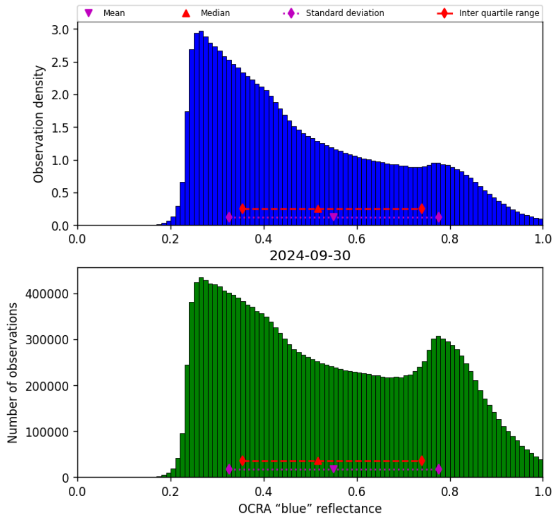
Figure 51: Histogram of “OCRA “blue” reflectance” for 2024-09-29 to 2024-10-01
