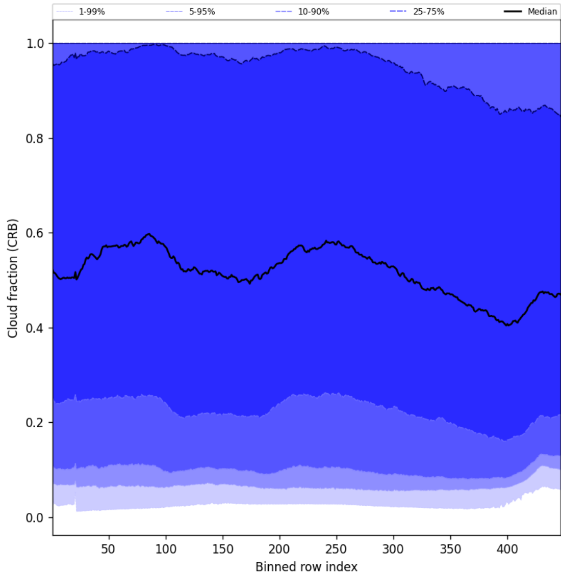
Figure 58: Along track statistics of “Cloud fraction (CRB)” for 2024-09-29 to 2024-10-01
