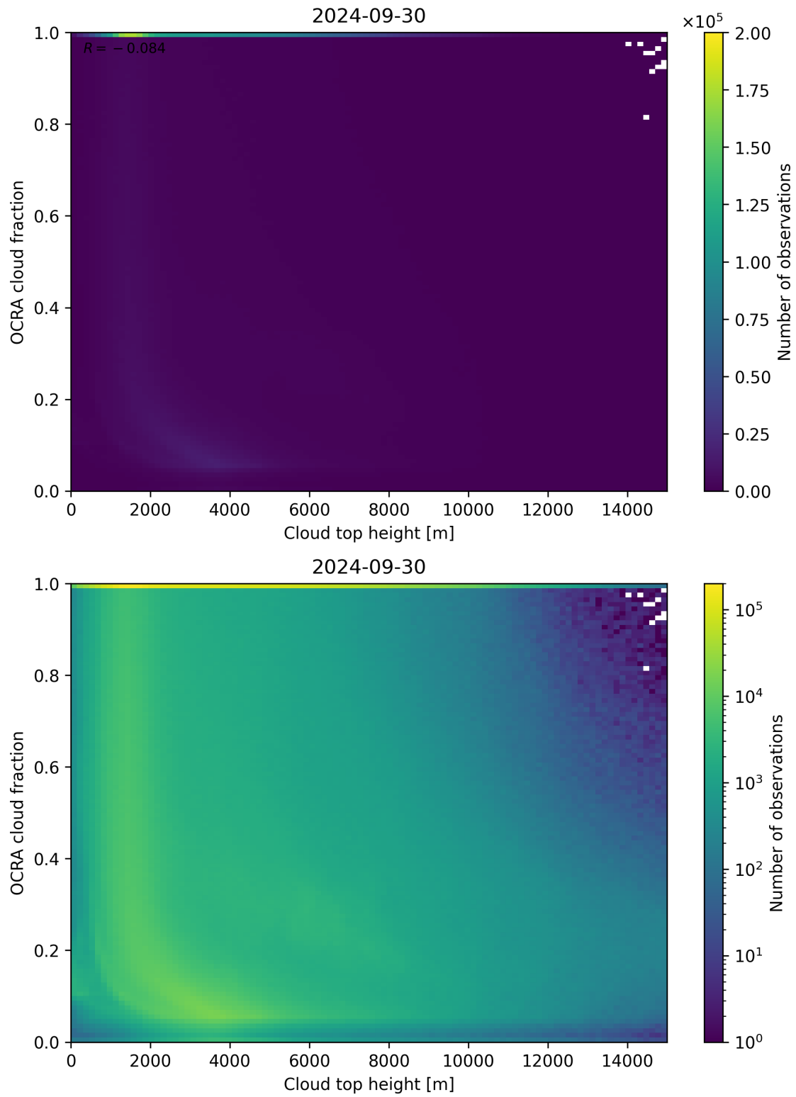
Figure 87: Scatter density plot of “Cloud top height” against “OCRA cloud fraction” for 2024-09-29 to 2024-10-01.
