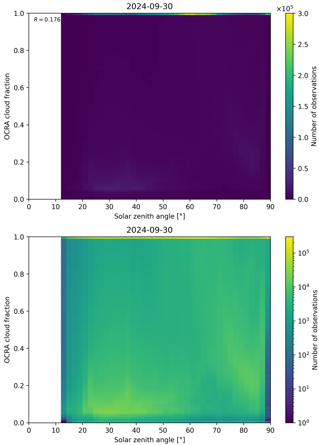
Figure 100: Scatter density plot of “Solar zenith angle” against “OCRA cloud fraction” for 2024-09-29 to 2024-10-01.
