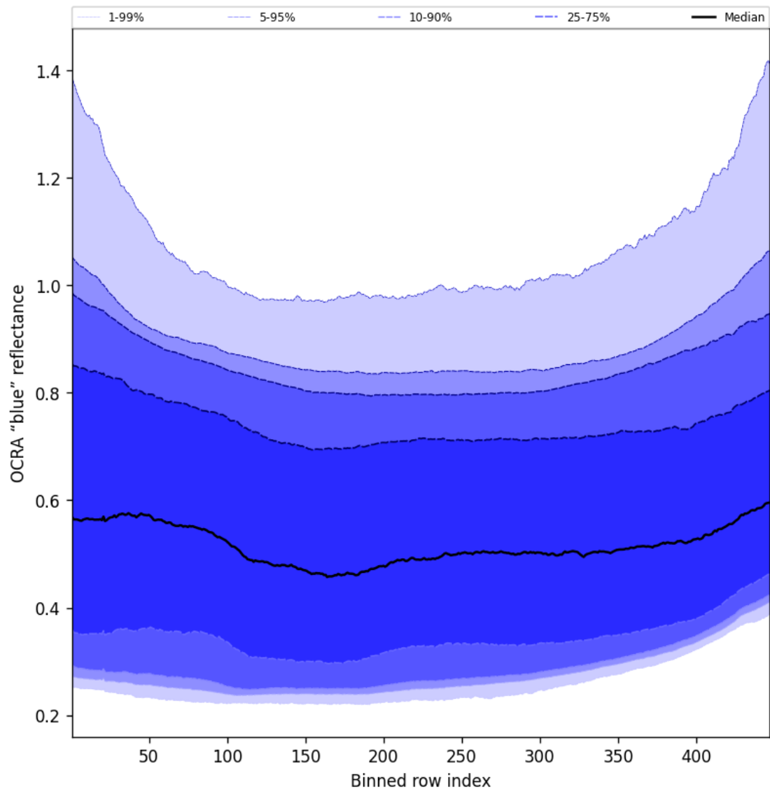
Figure 67: Along track statistics of “OCRA “blue” reflectance” for 2024-09-29 to 2024-10-01
