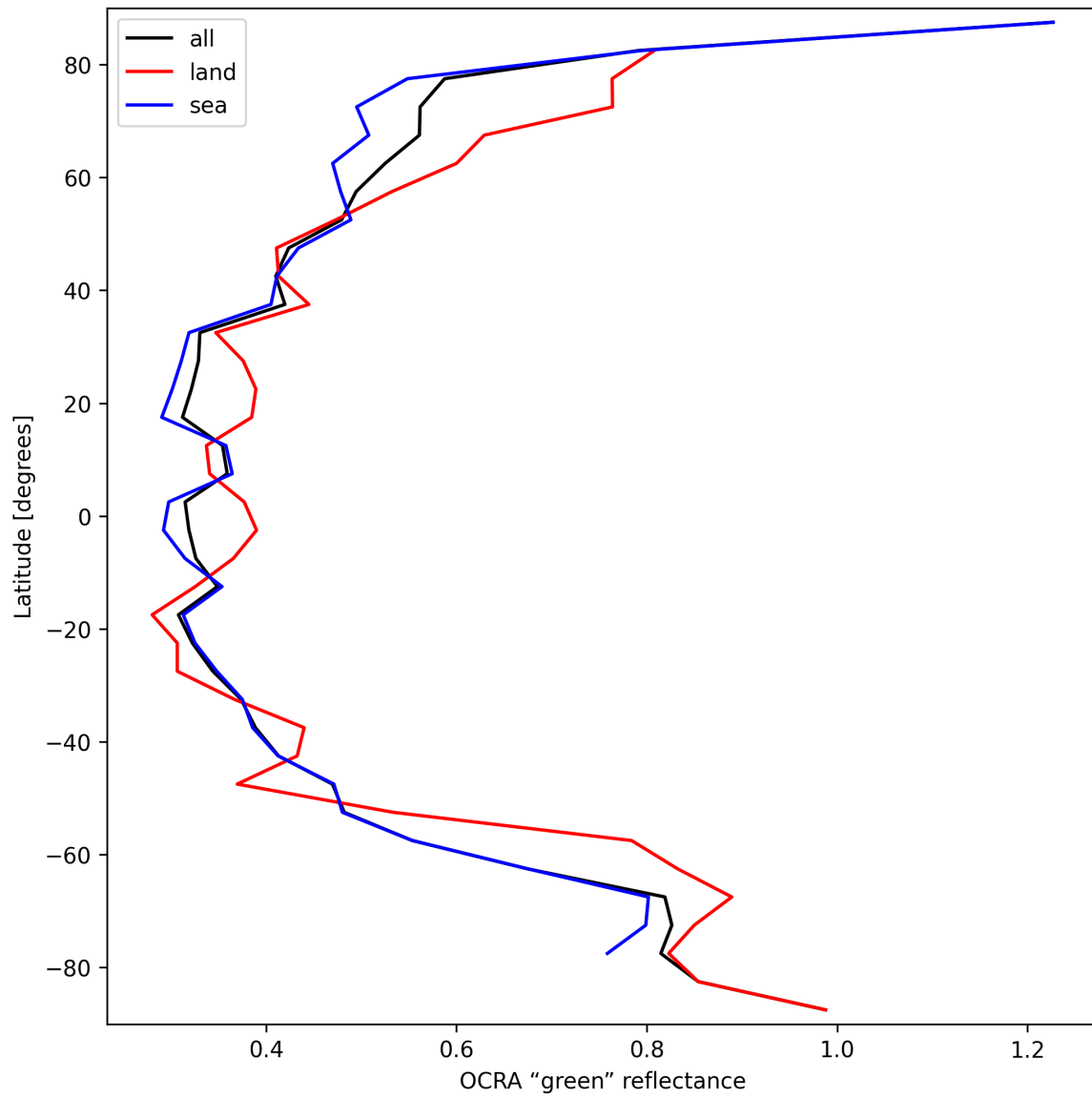
Figure 36: Zonal average of “OCRA “green” reflectance” for 2024-09-29 to 2024-10-01.
