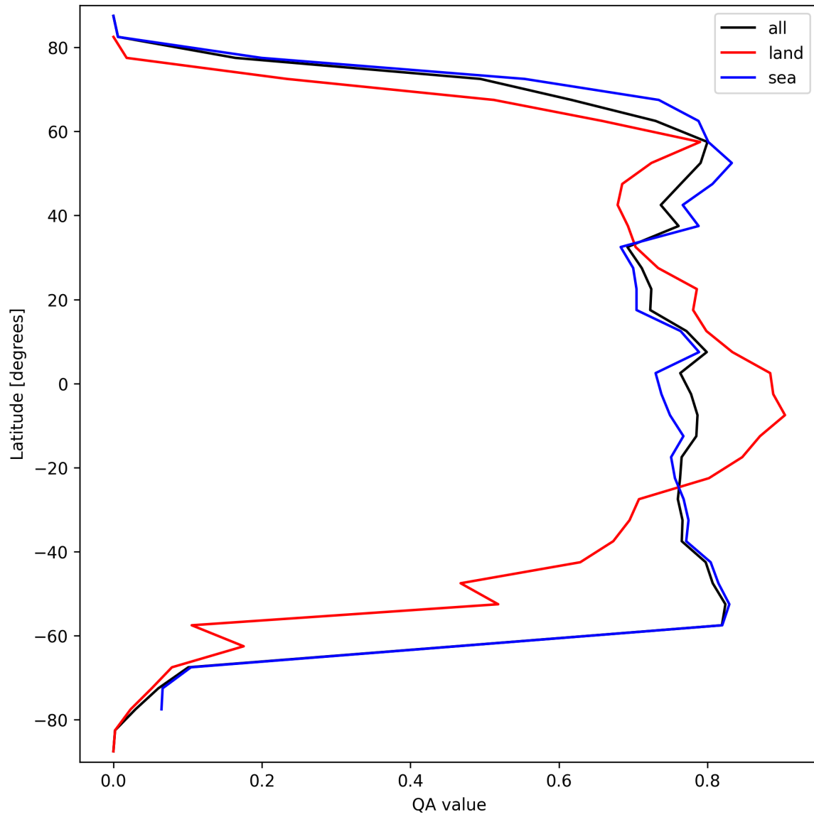
Figure 22: Zonal average of “QA value” for 2024-09-29 to 2024-10-01.
