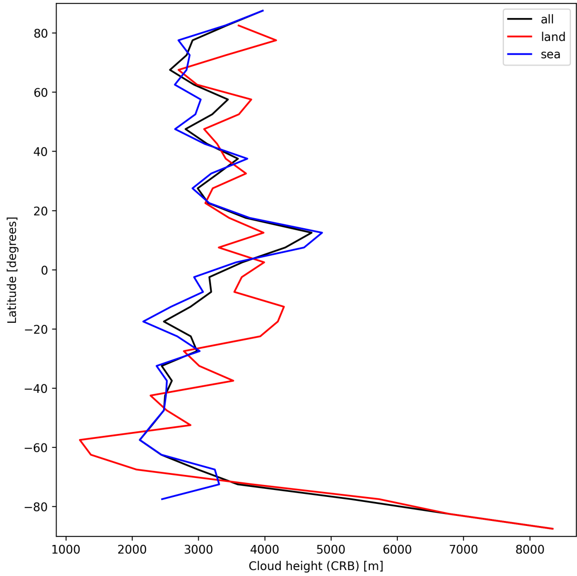
Figure 27: Zonal average of “Cloud height (CRB)” for 2024-09-29 to 2024-10-01.
