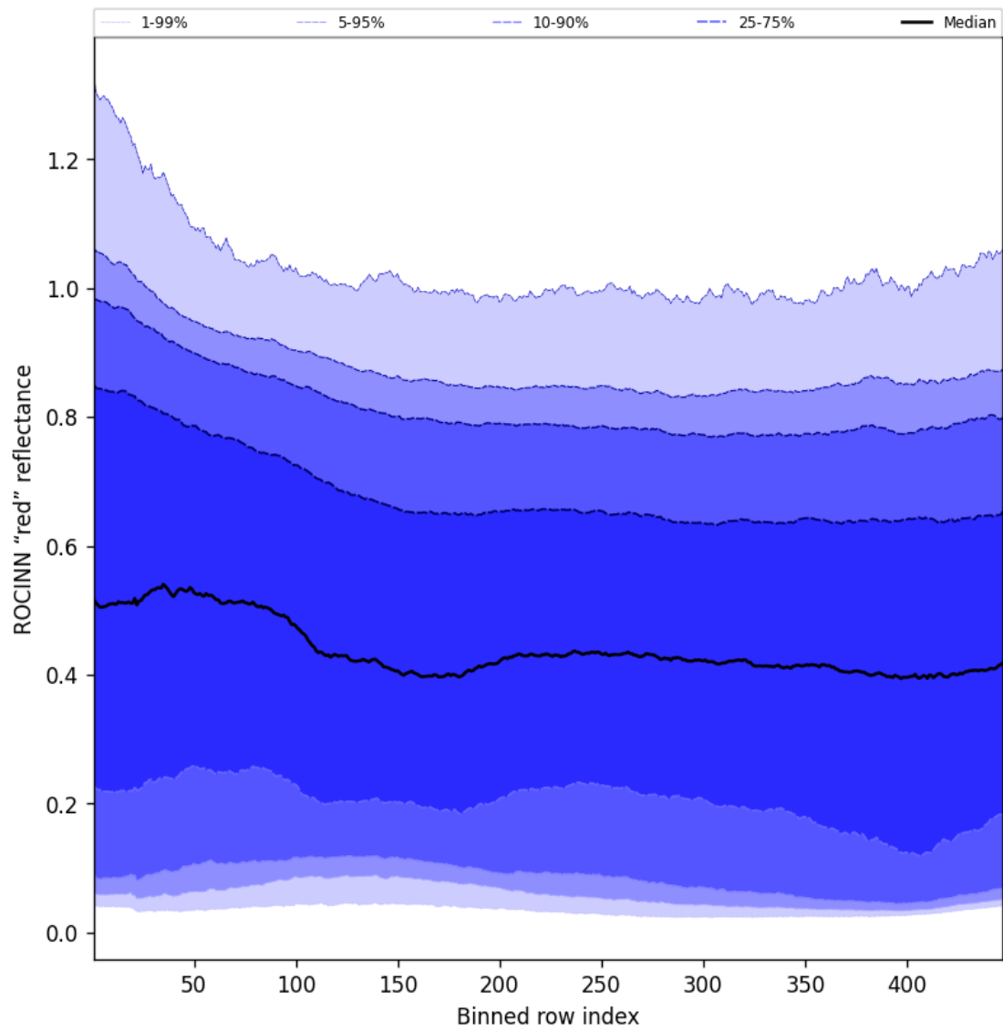
Figure 69: Along track statistics of "ROCINN "red" reflectance" for 2024-09-29 to 2024-10-01
