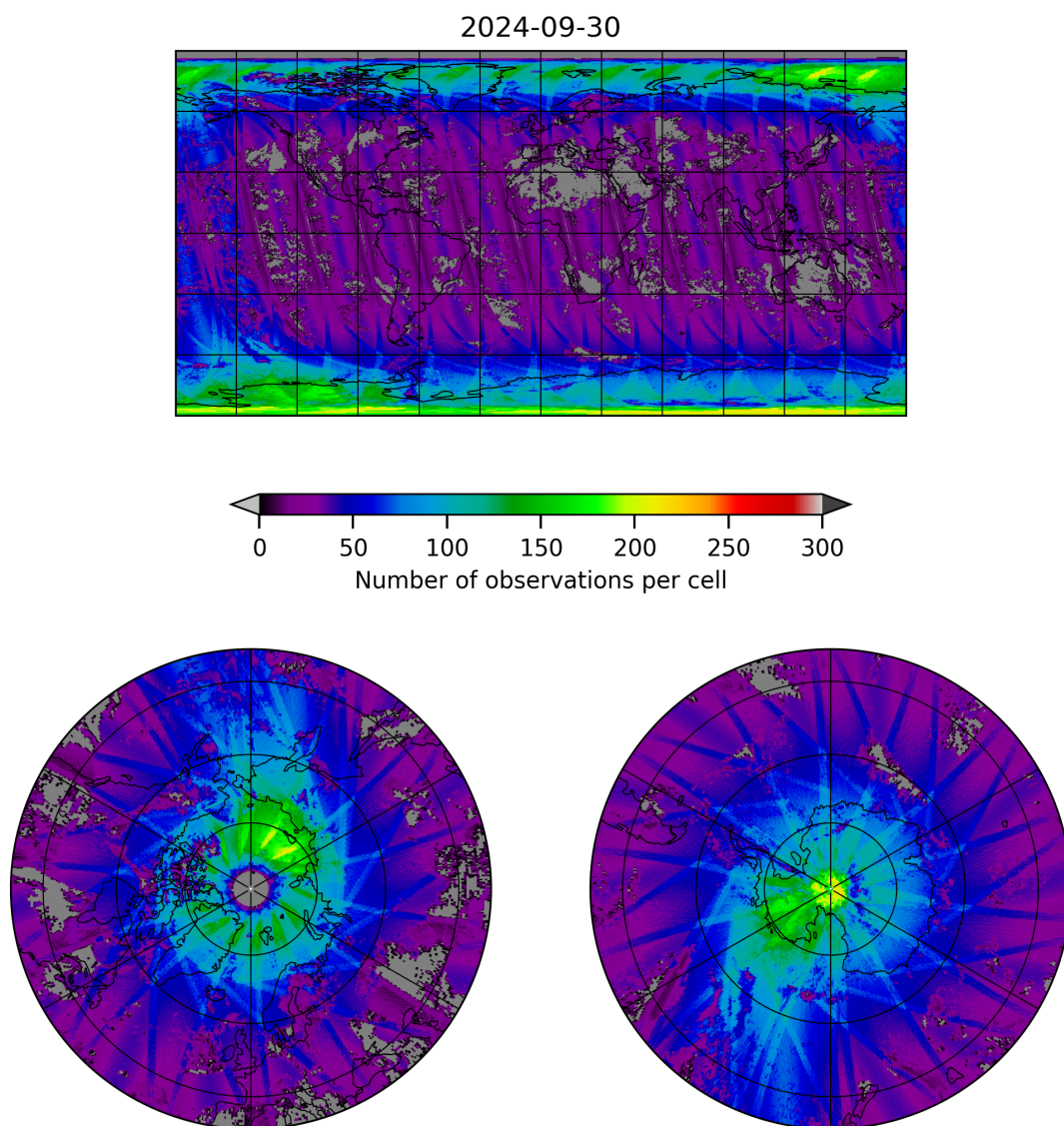
Figure 21: Map of the number of observations for 2024-09-29 to 2024-10-01
