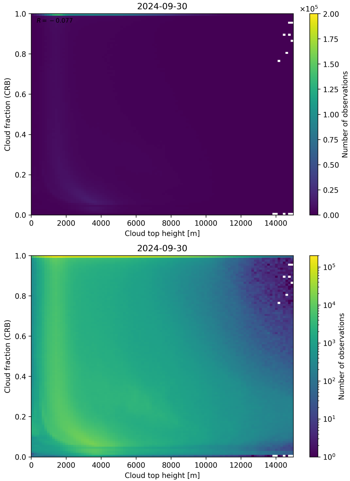
Figure 88: Scatter density plot of “Cloud top height” against “Cloud fraction (CRB)” for 2024-09-29 to 2024-10-01.
