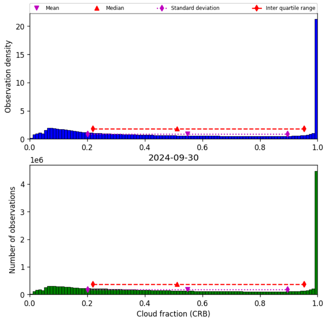
Figure 42: Histogram of “Cloud fraction (CRB)” for 2024-09-29 to 2024-10-01
