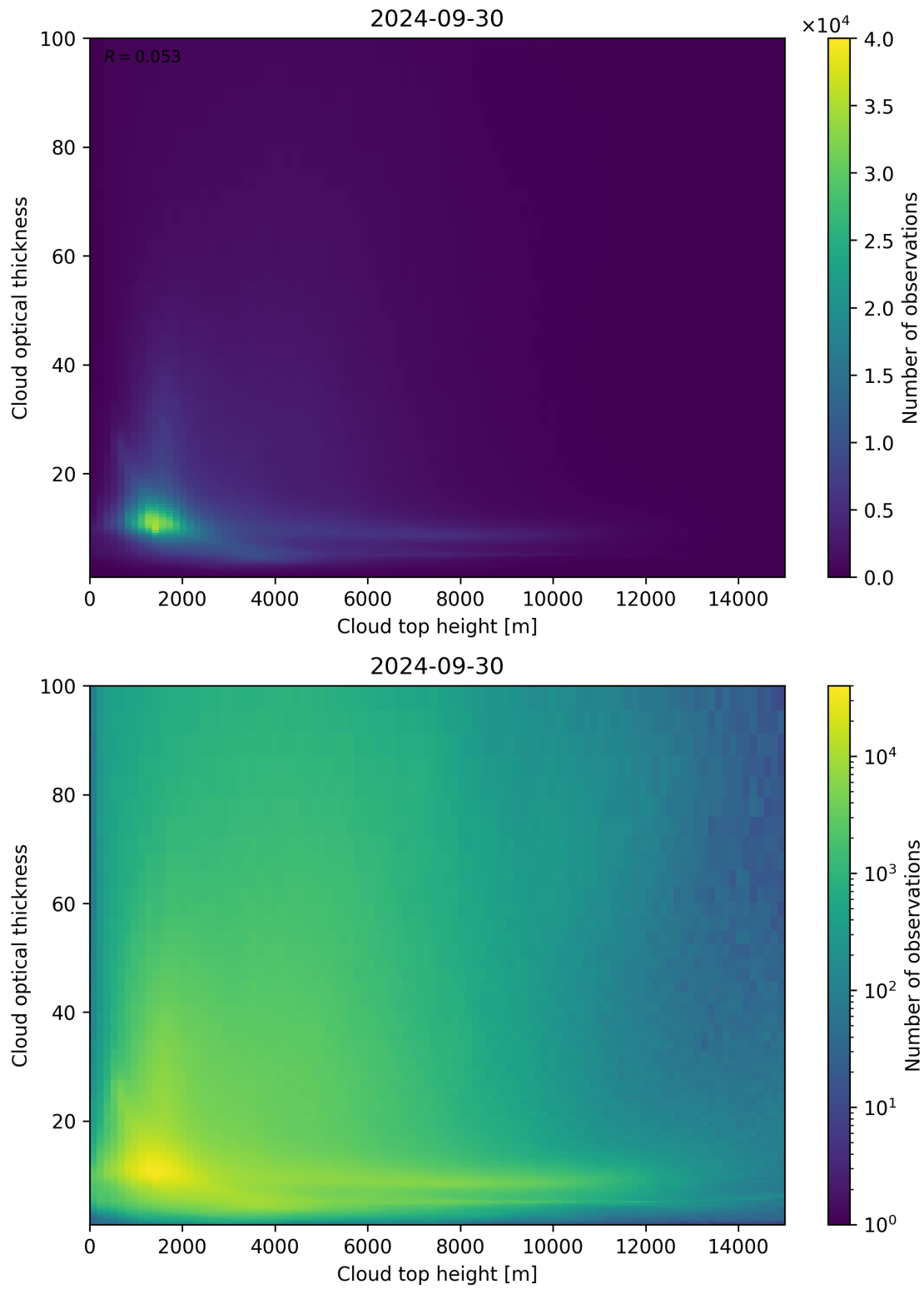
Figure 90: Scatter density plot of “Cloud top height” against “Cloud optical thickness” for 2024-09-29 to 2024-10-01.
