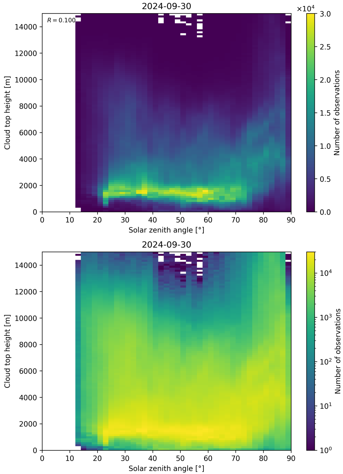
Figure 104: Scatter density plot of “Solar zenith angle” against “Cloud top height” for 2024-09-29 to 2024-10-01.
