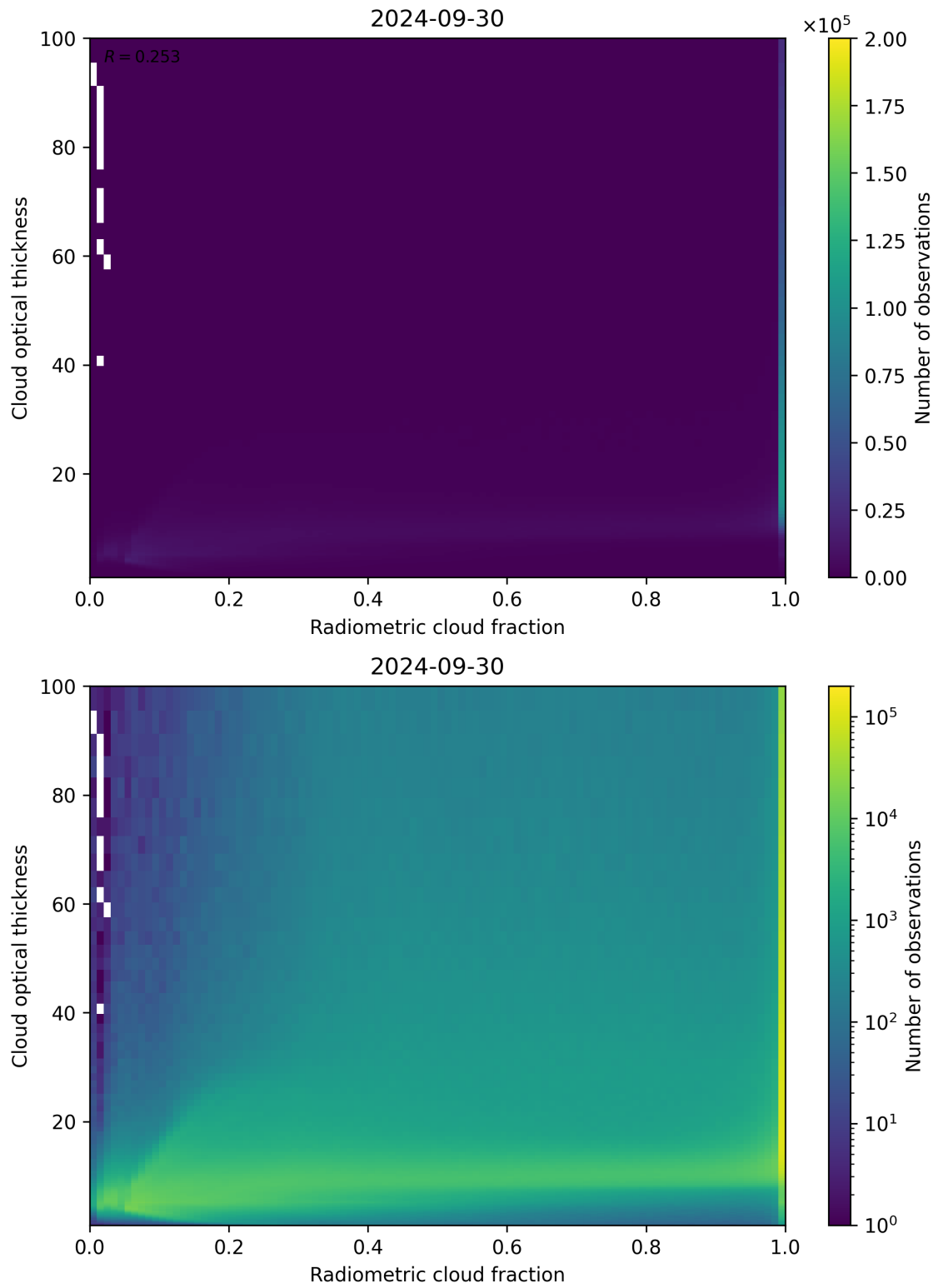
Figure 75: Scatter density plot of “Radiometric cloud fraction” against “Cloud optical thickness” for 2024-09-29 to 2024-10-01.
