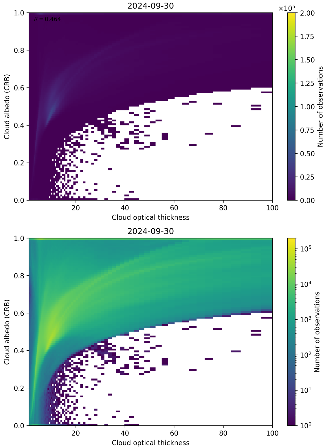
Figure 82: Scatter density plot of “Cloud optical thickness” against “Cloud albedo (CRB)” for 2024-09-29 to 2024-10-01.
