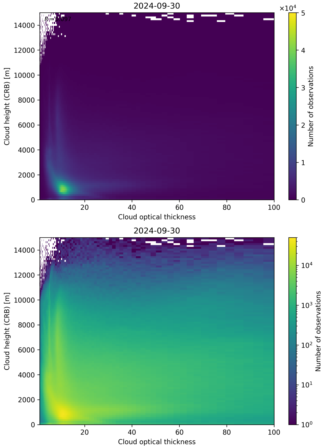
Figure 85: Scatter density plot of “Cloud optical thickness” against “Cloud height (CRB)” for 2024-09-29 to 2024-10-01.
