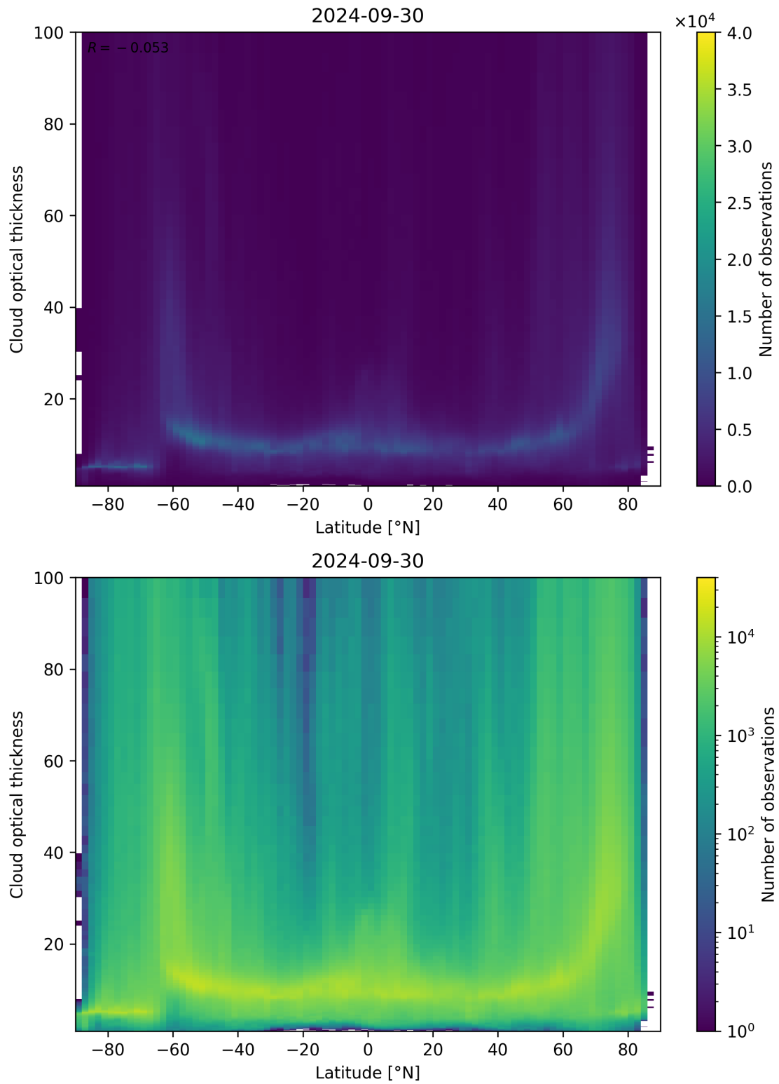
Figure 96: Scatter density plot of “Latitude” against “Cloud optical thickness” for 2024-09-29 to 2024-10-01.
