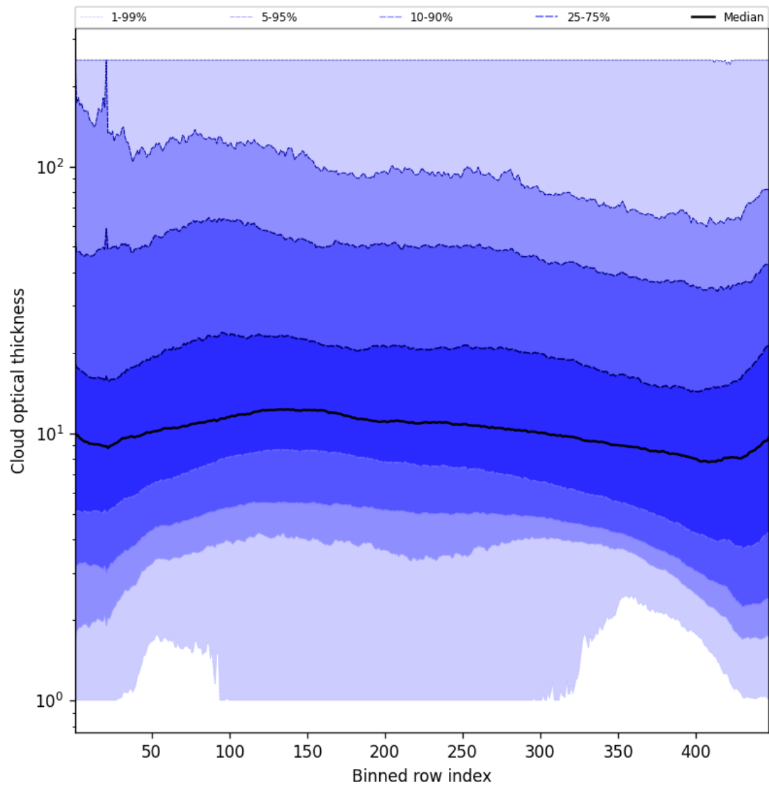
Figure 57: Along track statistics of “Cloud optical thickness” for 2024-09-29 to 2024-10-01
