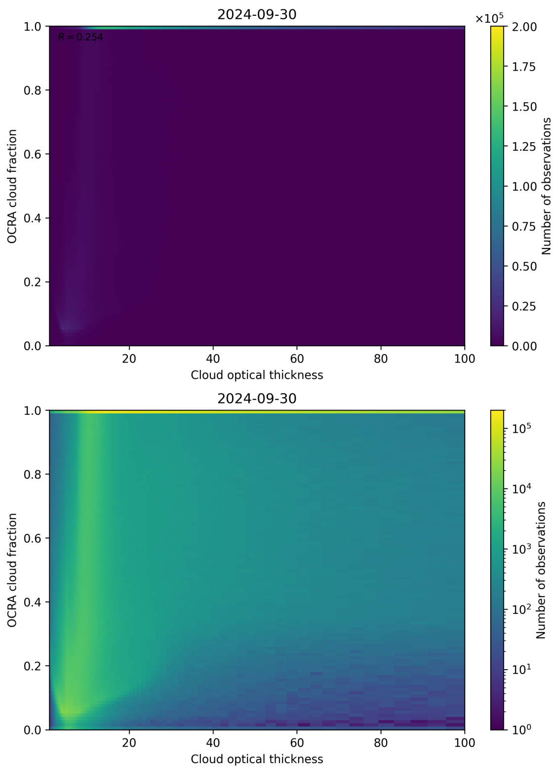
Figure 83: Scatter density plot of “Cloud optical thickness” against “OCRA cloud fraction” for 2024-09-29 to 2024-10-01.
