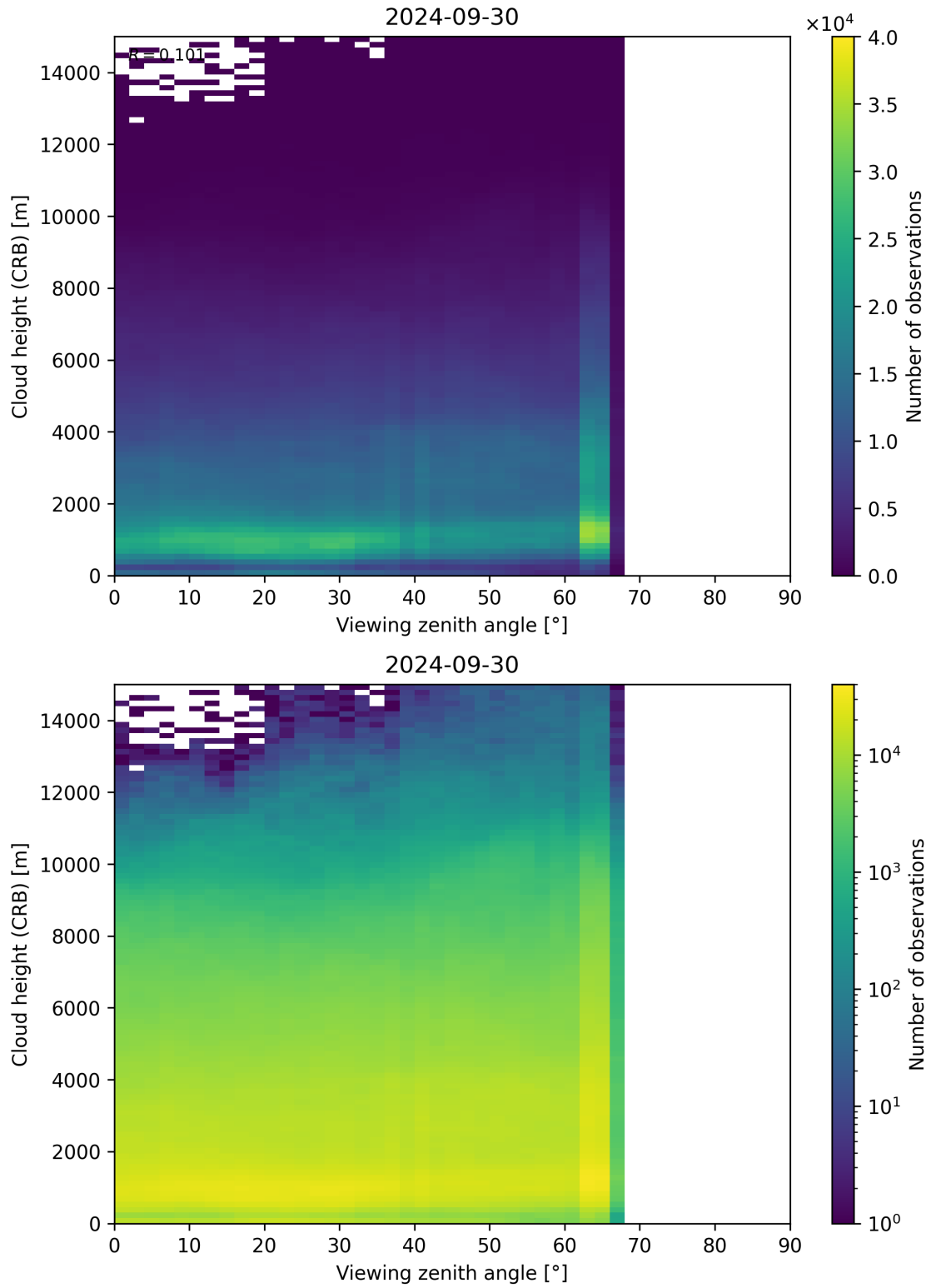
Figure 110: Scatter density plot of “Viewing zenith angle” against “Cloud height (CRB)” for 2024-09-29 to 2024-10-01.
