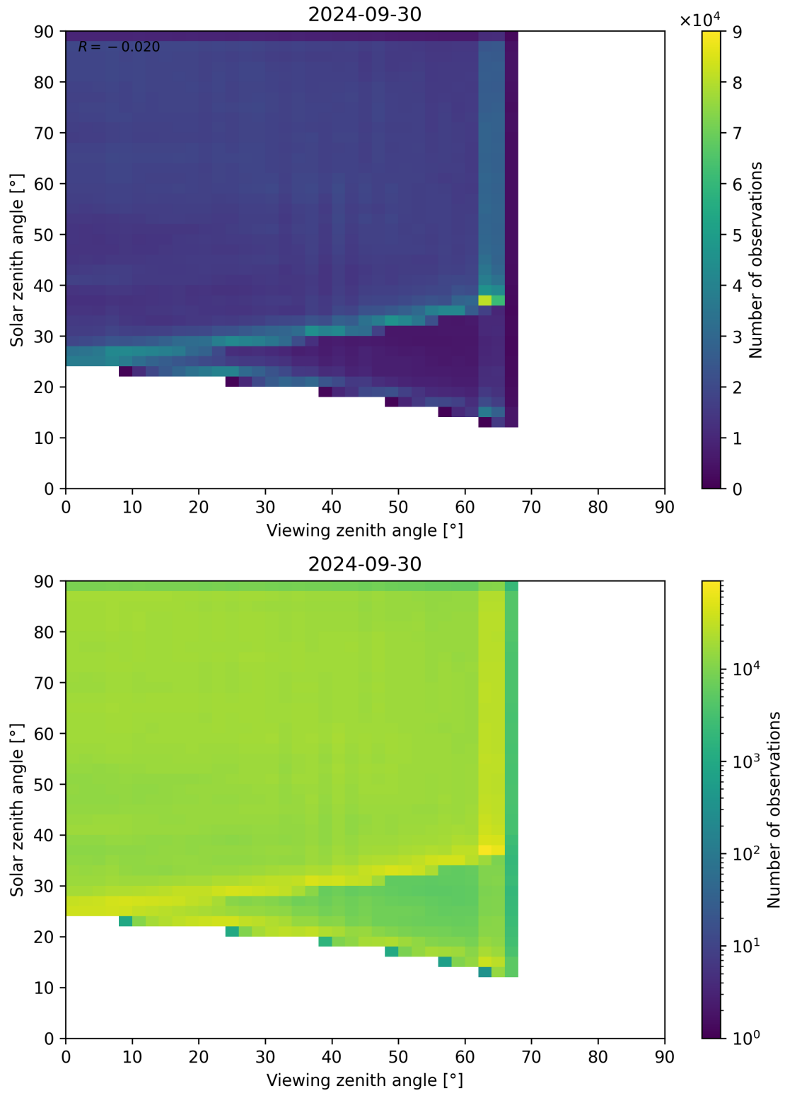
Figure 114: Scatter density plot of “Viewing zenith angle” against “Solar zenith angle” for 2024-09-29 to 2024-10-01.
