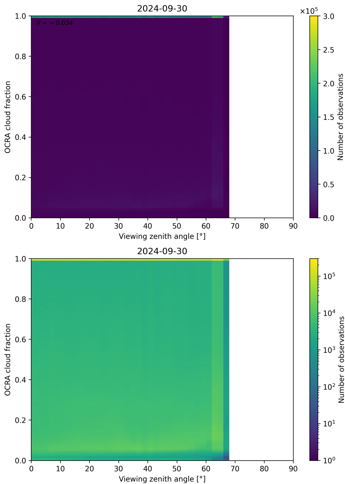
Figure 108: Scatter density plot of “Viewing zenith angle” against “OCRA cloud fraction” for 2024-09-29 to 2024-10-01.
