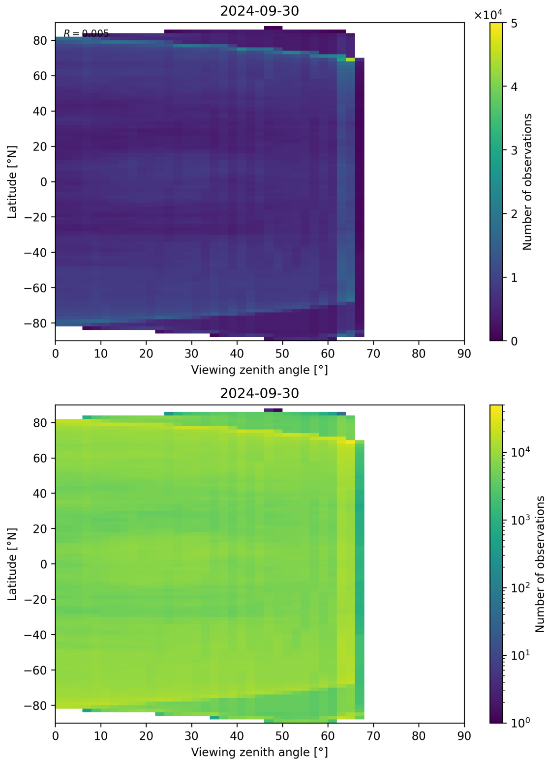
Figure 113: Scatter density plot of “Viewing zenith angle” against “Latitude” for 2024-09-29 to 2024-10-01.
