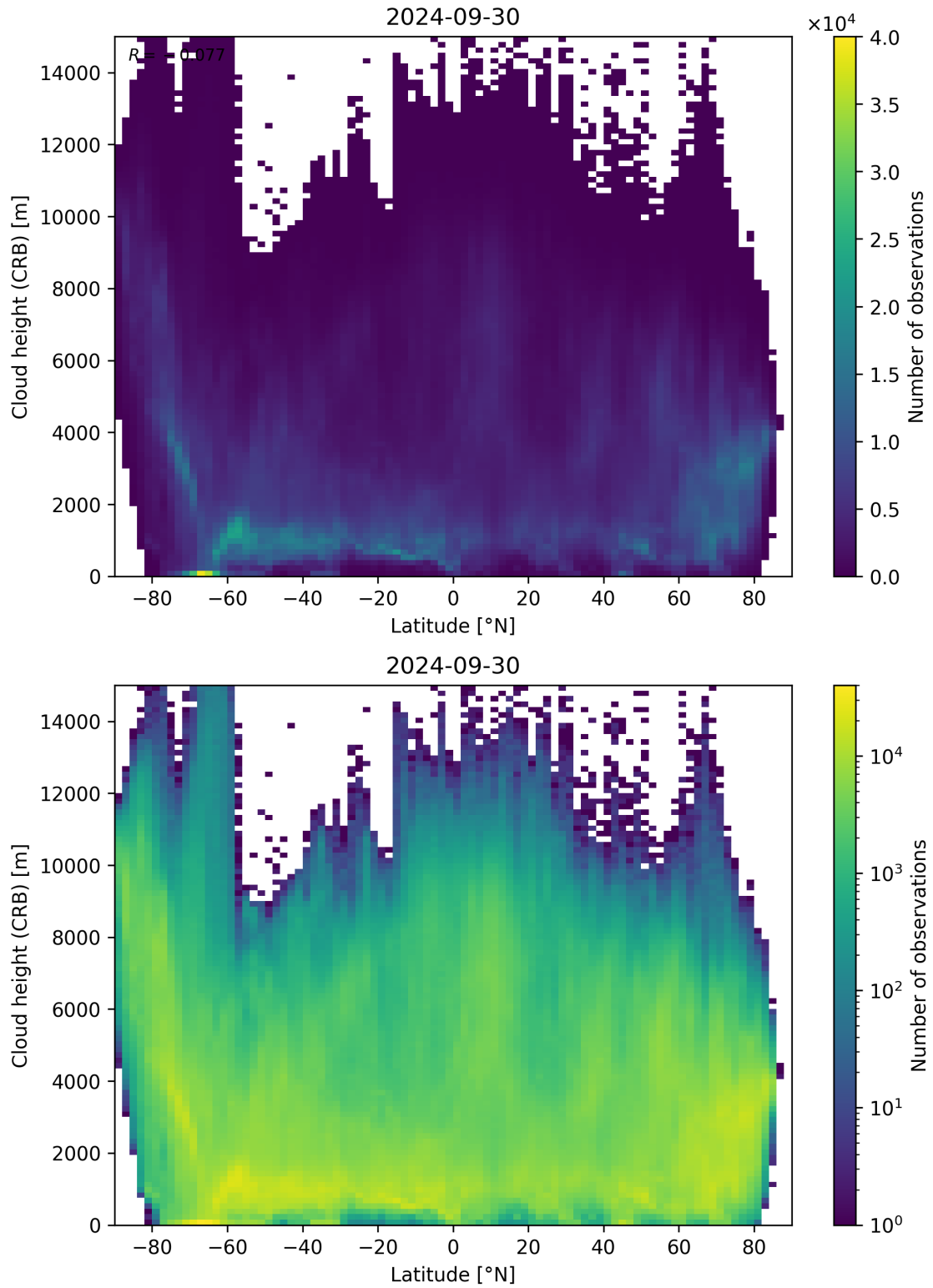
Figure 95: Scatter density plot of “Latitude” against “Cloud height (CRB)” for 2024-09-29 to 2024-10-01.
