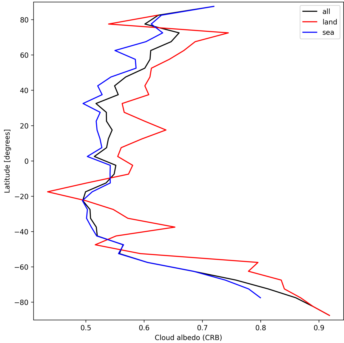
Figure 28: Zonal average of “Cloud albedo (CRB)” for 2024-09-29 to 2024-10-01.
