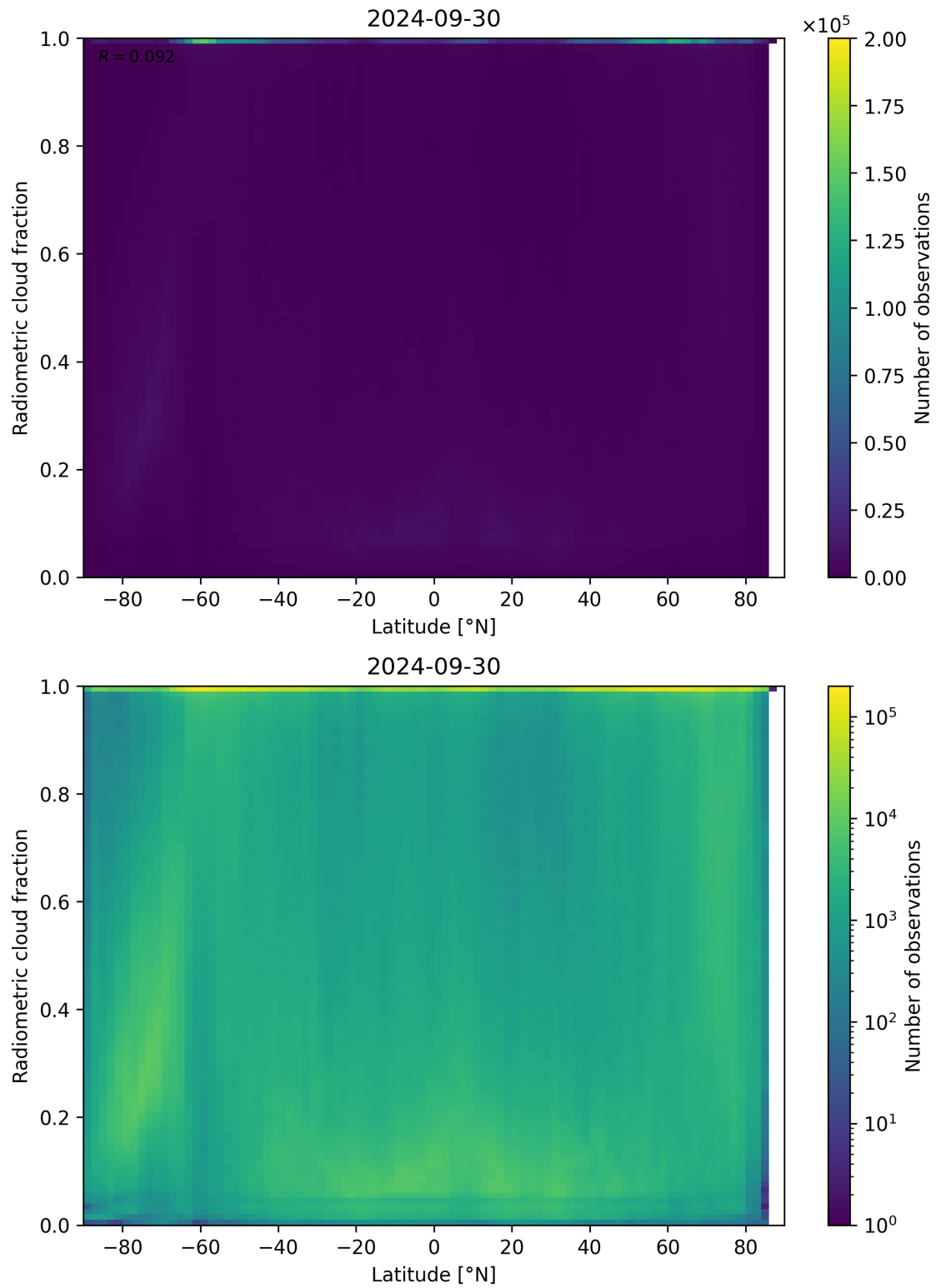
Figure 92: Scatter density plot of “Latitude” against “Radiometric cloud fraction” for 2024-09-29 to 2024-10-01.
