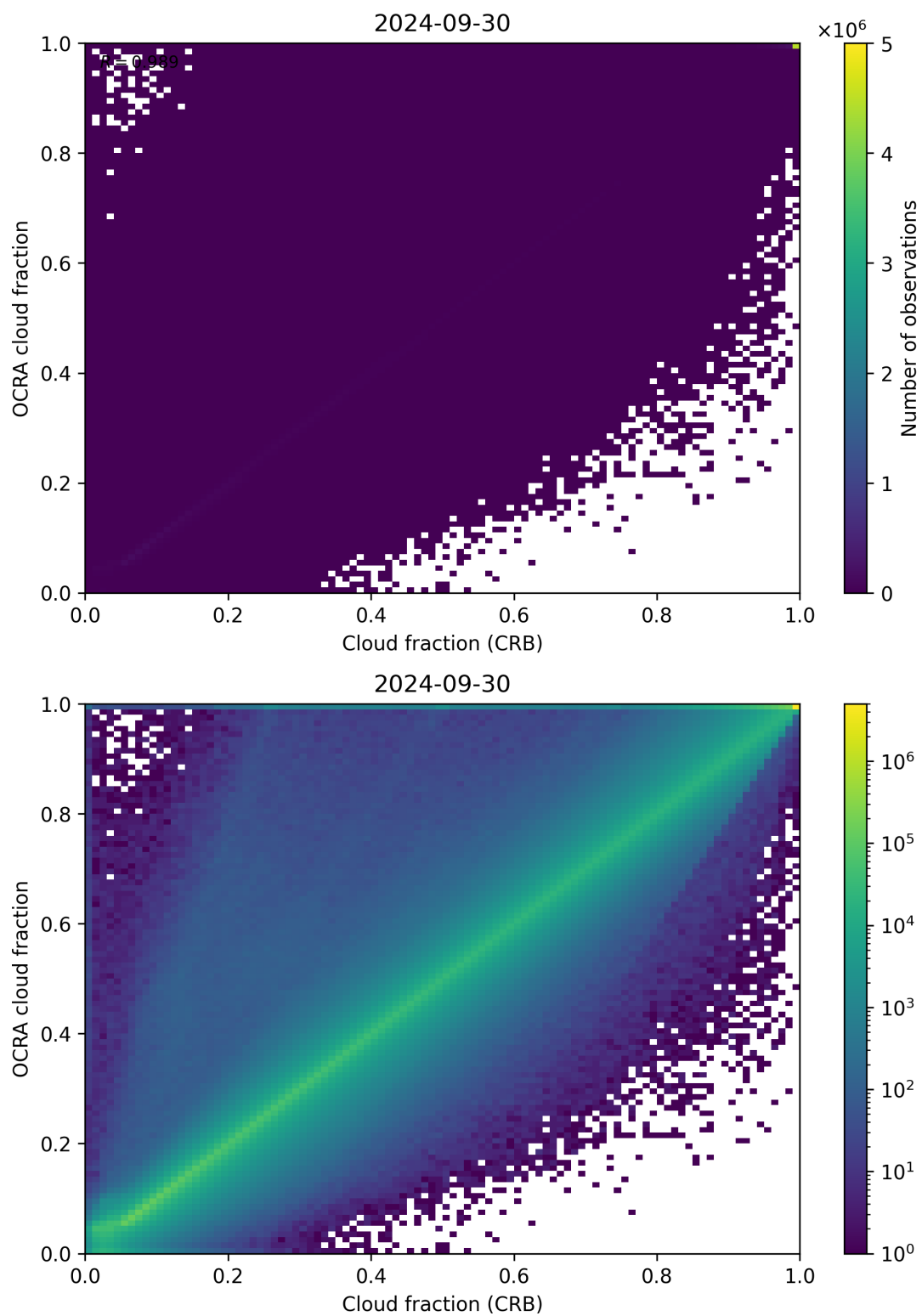
Figure 78: Scatter density plot of “Cloud fraction (CRB)” against “OCRA cloud fraction” for 2024-09-29 to 2024-10-01.
