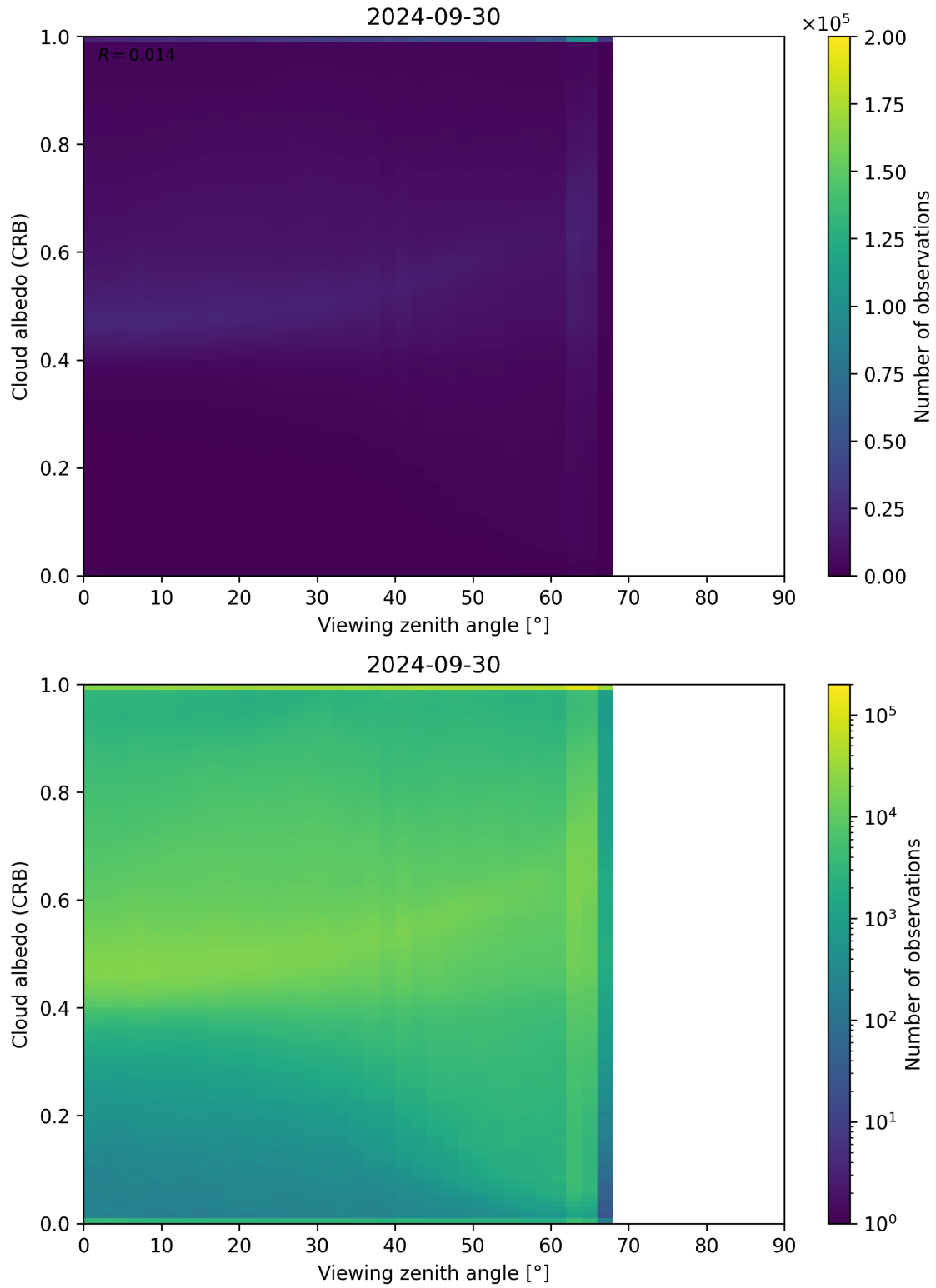
Figure 106: Scatter density plot of “Viewing zenith angle” against “Cloud albedo (CRB)” for 2024-09-29 to 2024-10-01.
