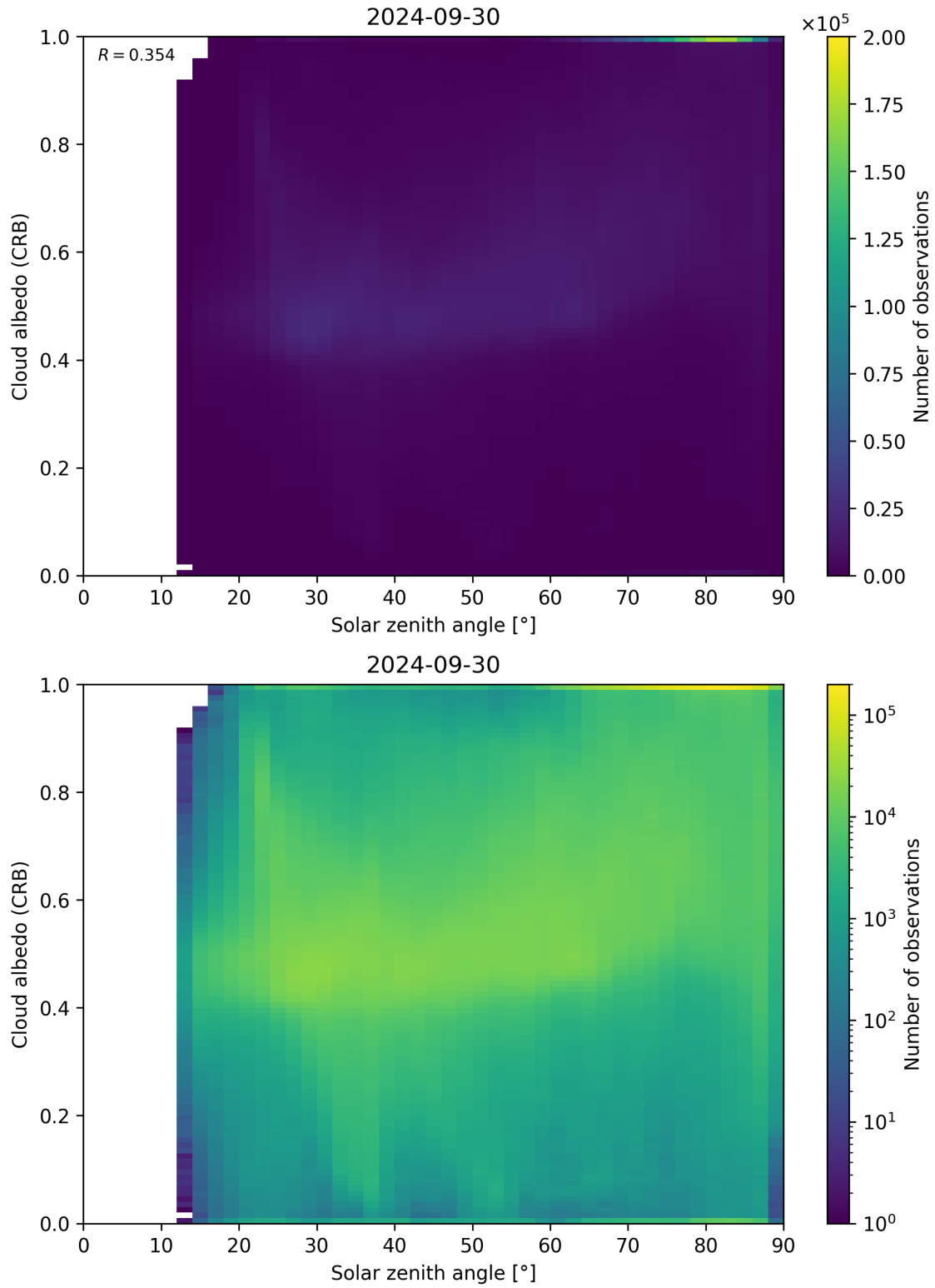
Figure 98: Scatter density plot of “Solar zenith angle” against “Cloud albedo (CRB)” for 2024-09-29 to 2024-10-01.
