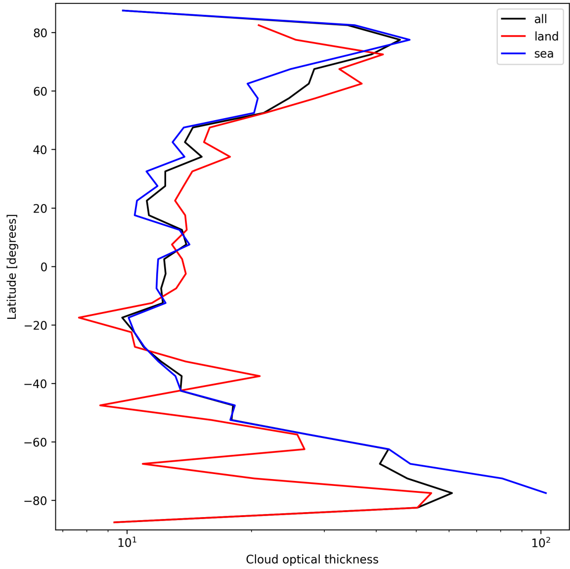
Figure 25: Zonal average of “Cloud optical thickness” for 2024-09-29 to 2024-10-01.
