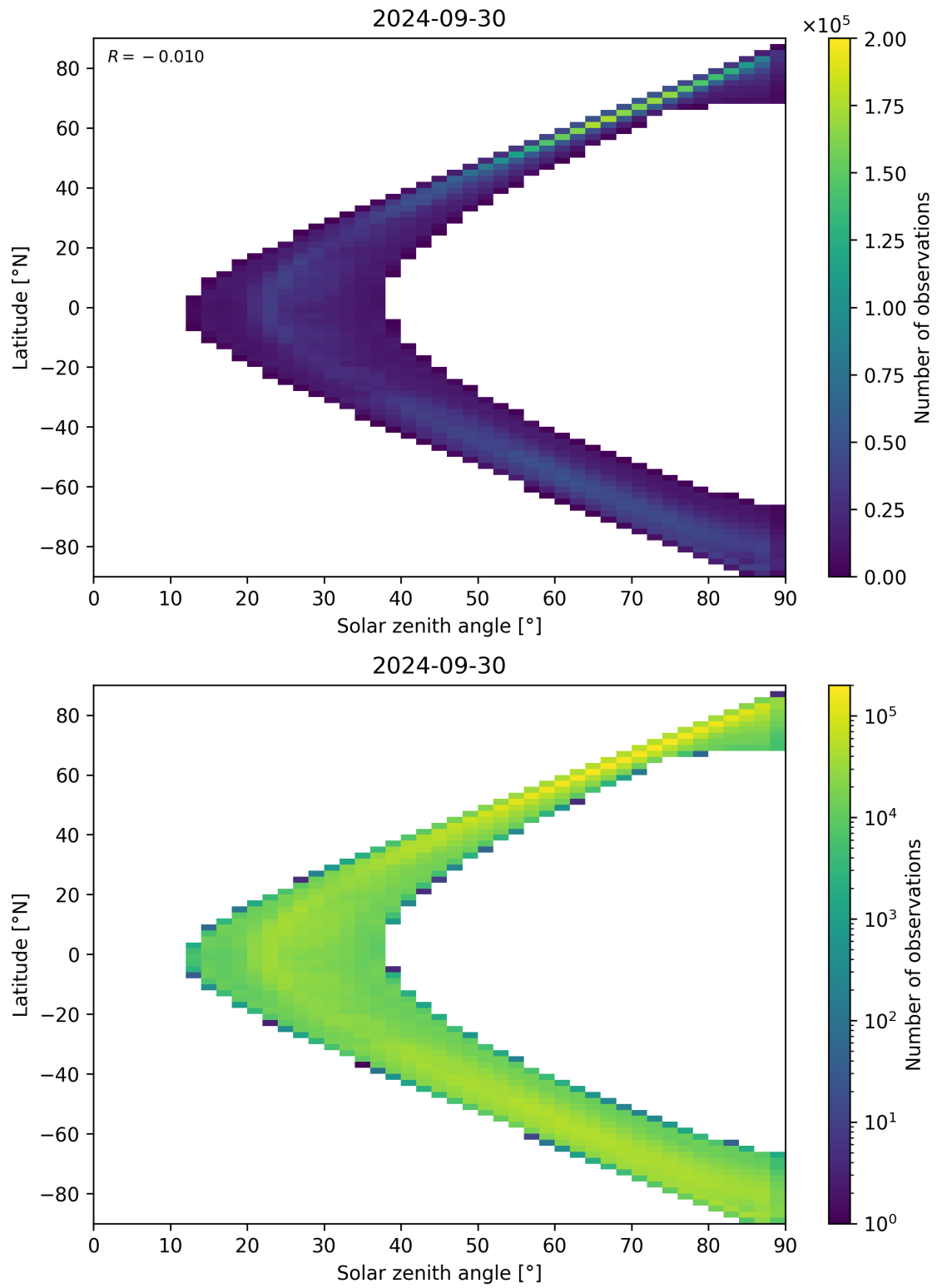
Figure 105: Scatter density plot of “Solar zenith angle” against “Latitude” for 2024-09-29 to 2024-10-01.
