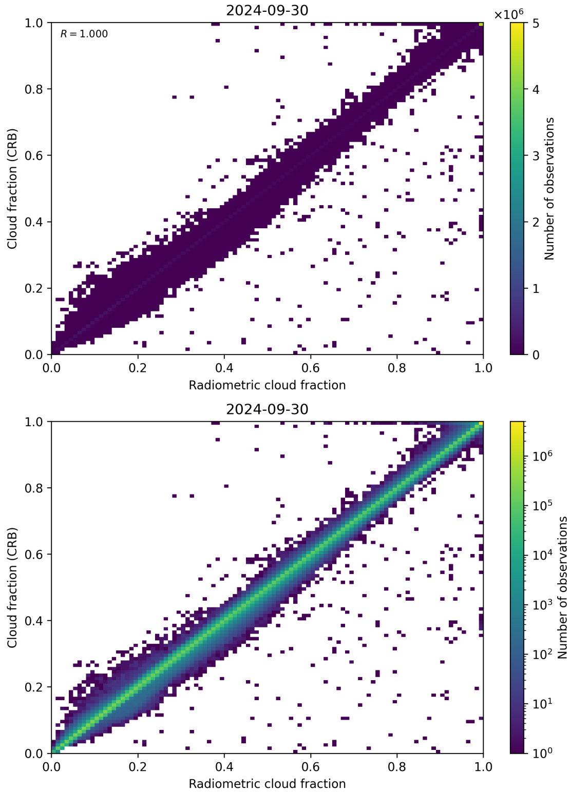
Figure 73: Scatter density plot of “Radiometric cloud fraction” against “Cloud fraction (CRB)” for 2024-09-29 to 2024-10-01.
