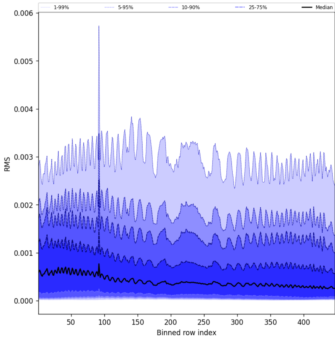
Figure 63: Along track statistics of “RMS” for 2024-09-29 to 2024-10-01
