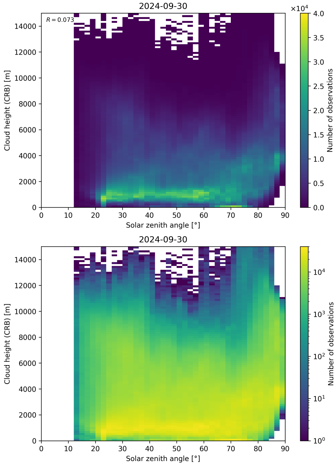
Figure 102: Scatter density plot of “Solar zenith angle” against “Cloud height (CRB)” for 2024-09-29 to 2024-10-01.
