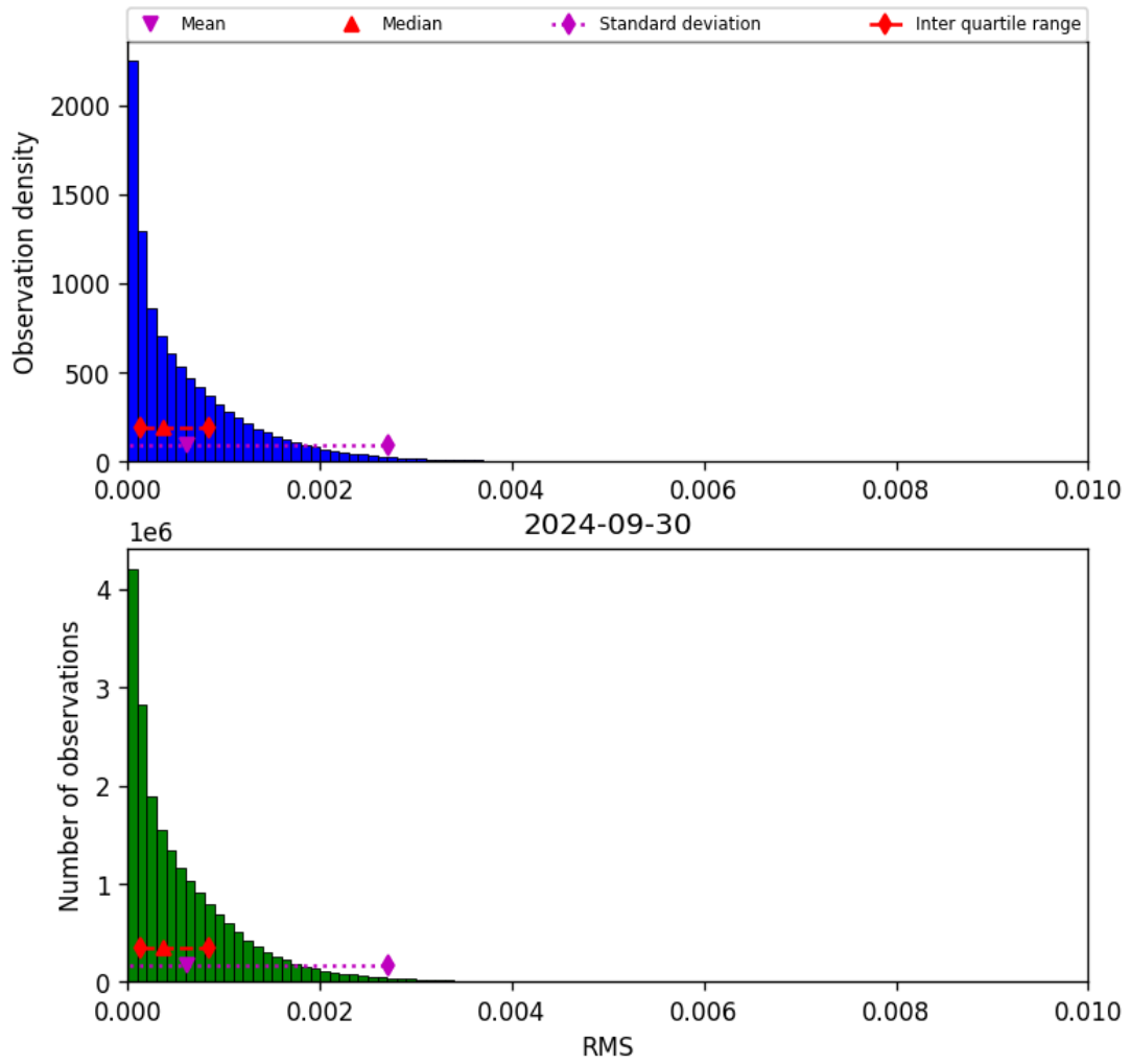
Figure 47: Histogram of “RMS” for 2024-09-29 to 2024-10-01
