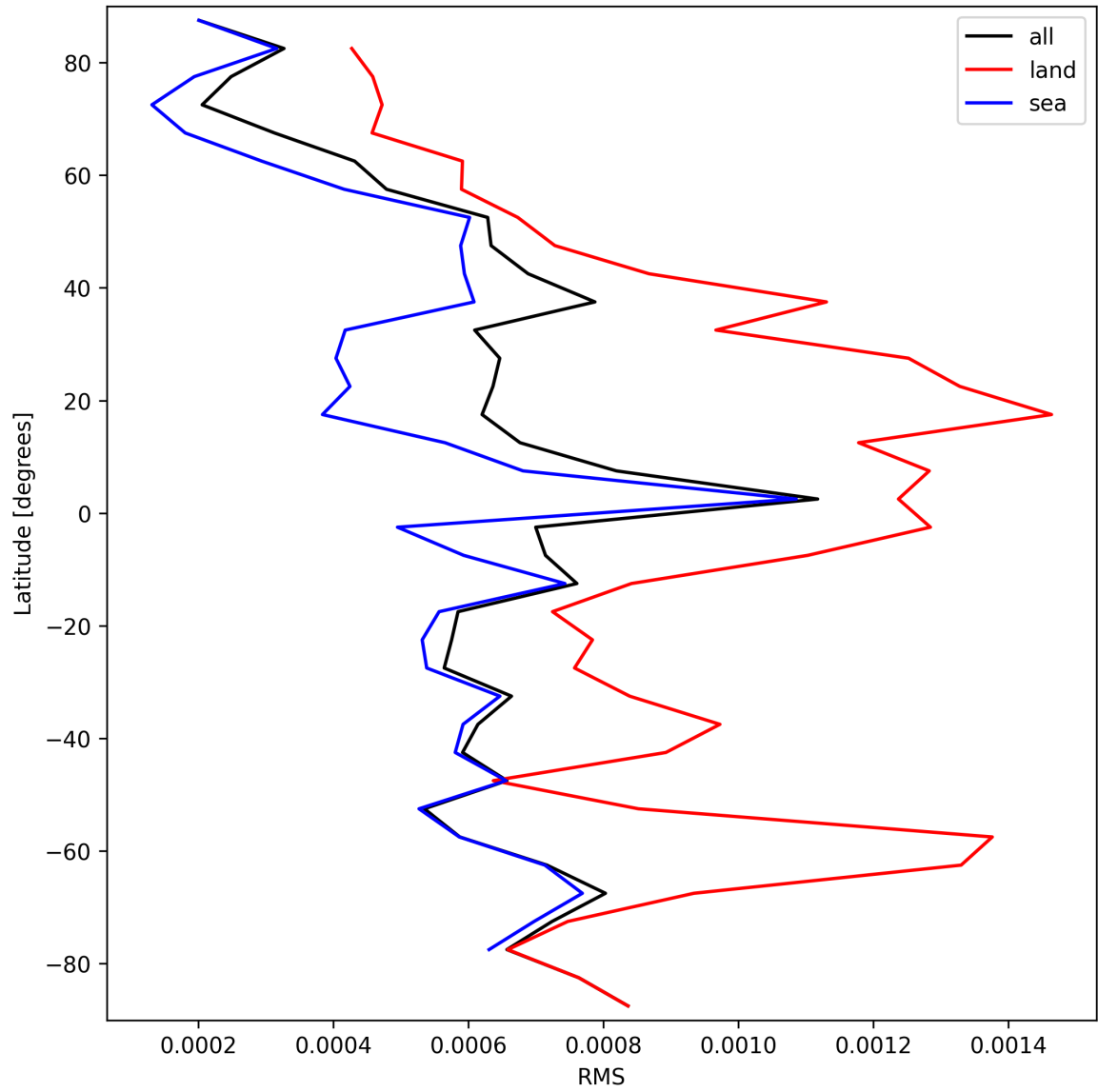
Figure 31: Zonal average of “RMS” for 2024-09-29 to 2024-10-01.
