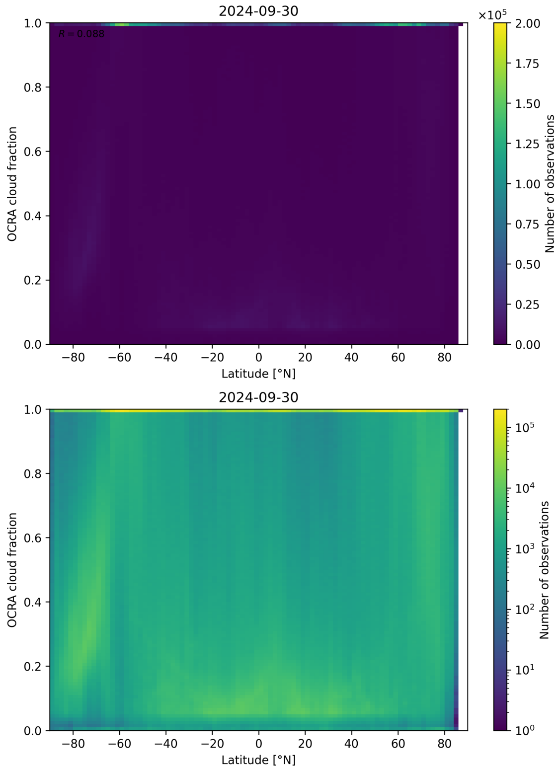
Figure 93: Scatter density plot of “Latitude” against “OCRA cloud fraction” for 2024-09-29 to 2024-10-01.
