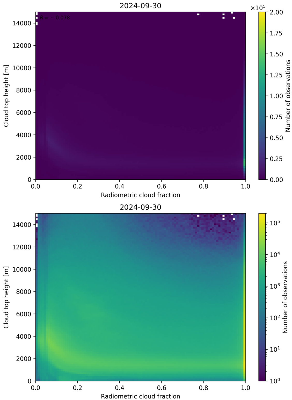
Figure 76: Scatter density plot of “Radiometric cloud fraction” against “Cloud top height” for 2024-09-29 to 2024-10-01.
