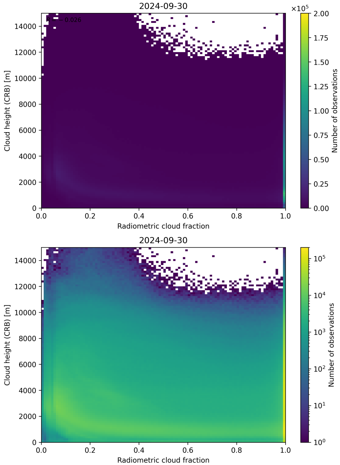
Figure 74: Scatter density plot of “Radiometric cloud fraction” against “Cloud height (CRB)” for 2024-09-29 to 2024-10-01.
