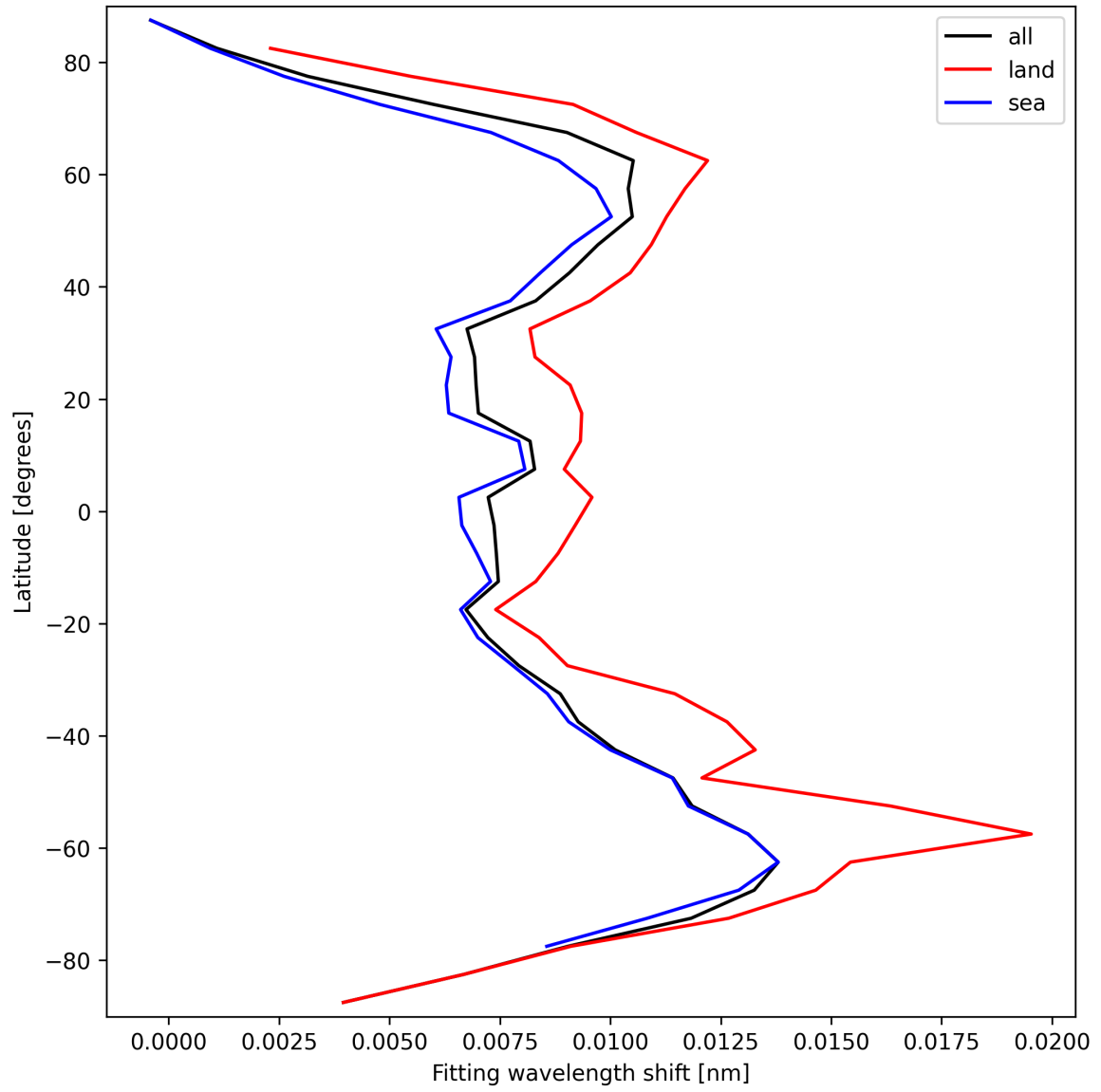
Figure 33: Zonal average of “Fitting wavelength shift” for 2024-09-29 to 2024-10-01.
