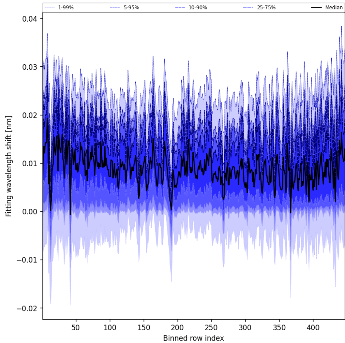
Figure 65: Along track statistics of “Fitting wavelength shift” for 2024-09-29 to 2024-10-01
