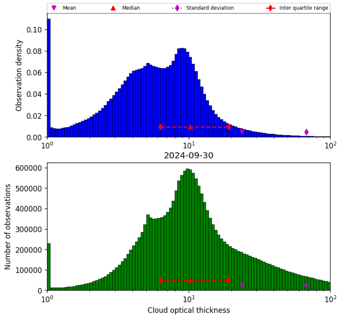
Figure 41: Histogram of “Cloud optical thickness” for 2024-09-29 to 2024-10-01
