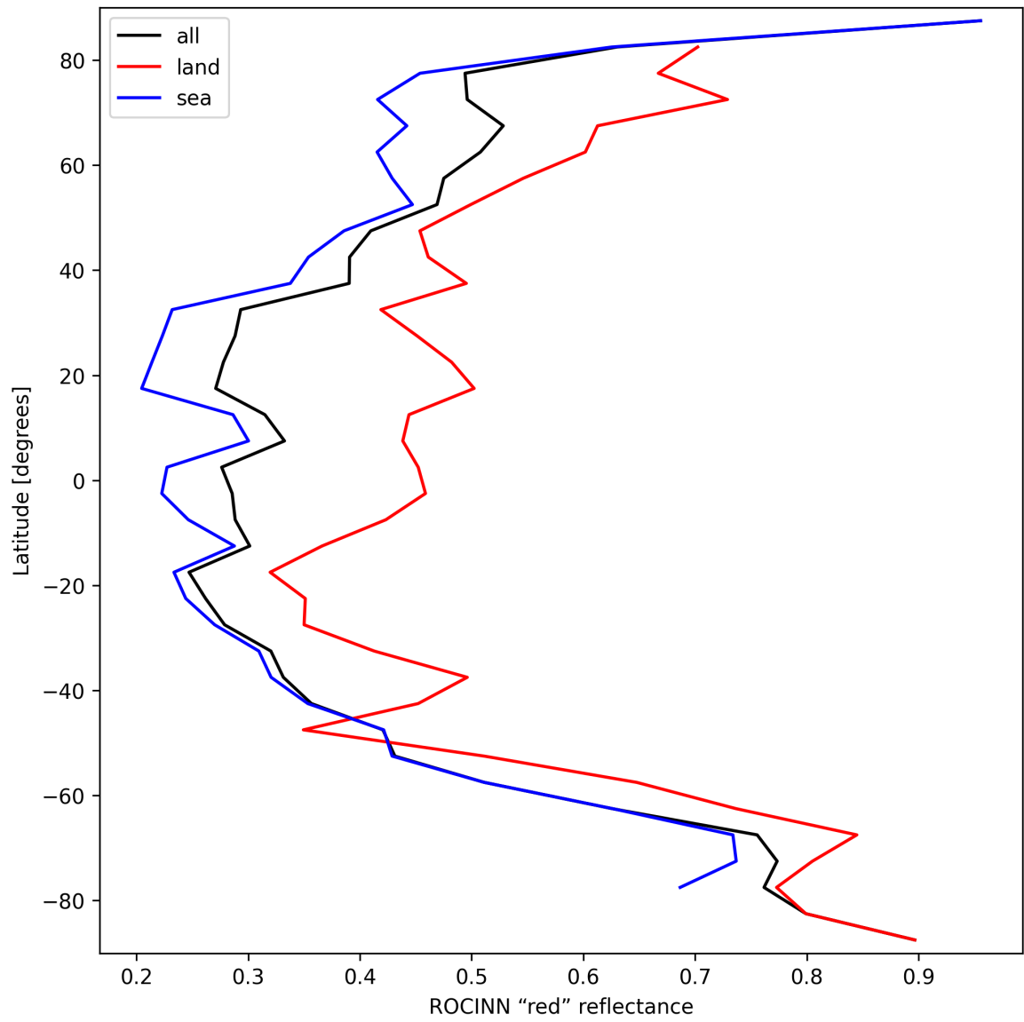
Figure 37: Zonal average of “ROCINN “red” reflectance” for 2024-09-29 to 2024-10-01.
