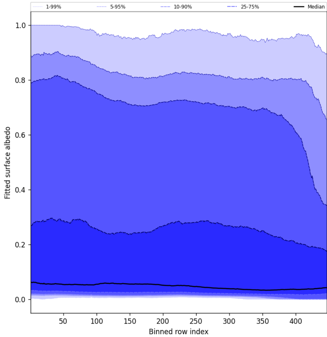
Figure 61: Along track statistics of “Fitted surface albedo” for 2024-09-29 to 2024-10-01
