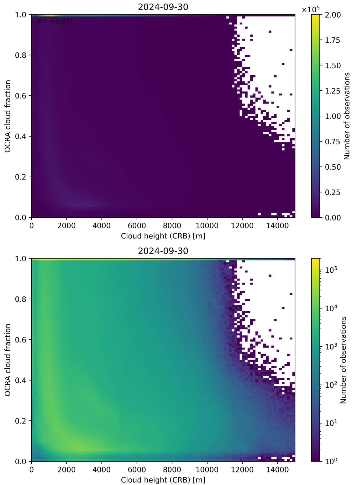
Figure 81: Scatter density plot of “Cloud height (CRB)” against “OCRA cloud fraction” for 2024-09-29 to 2024-10-01.
