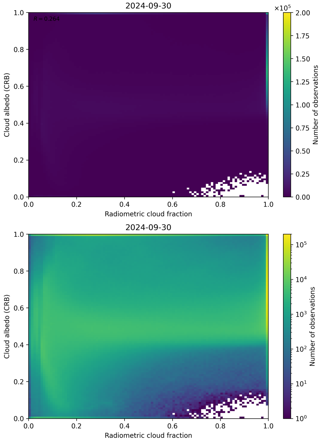
Figure 71: Scatter density plot of “Radiometric cloud fraction” against “Cloud albedo (CRB)” for 2024-09-29 to 2024-10-01.
