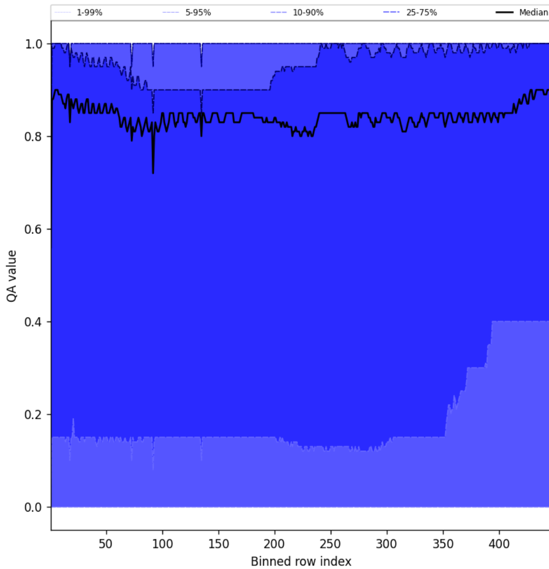
Figure 54: Along track statistics of “QA value” for 2024-09-29 to 2024-10-01
