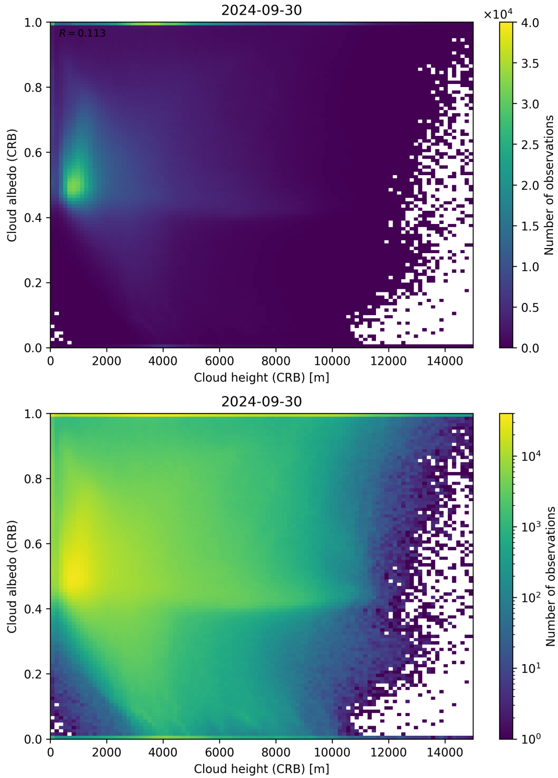
Figure 80: Scatter density plot of “Cloud height (CRB)” against “Cloud albedo (CRB)” for 2024-09-29 to 2024-10-01.
