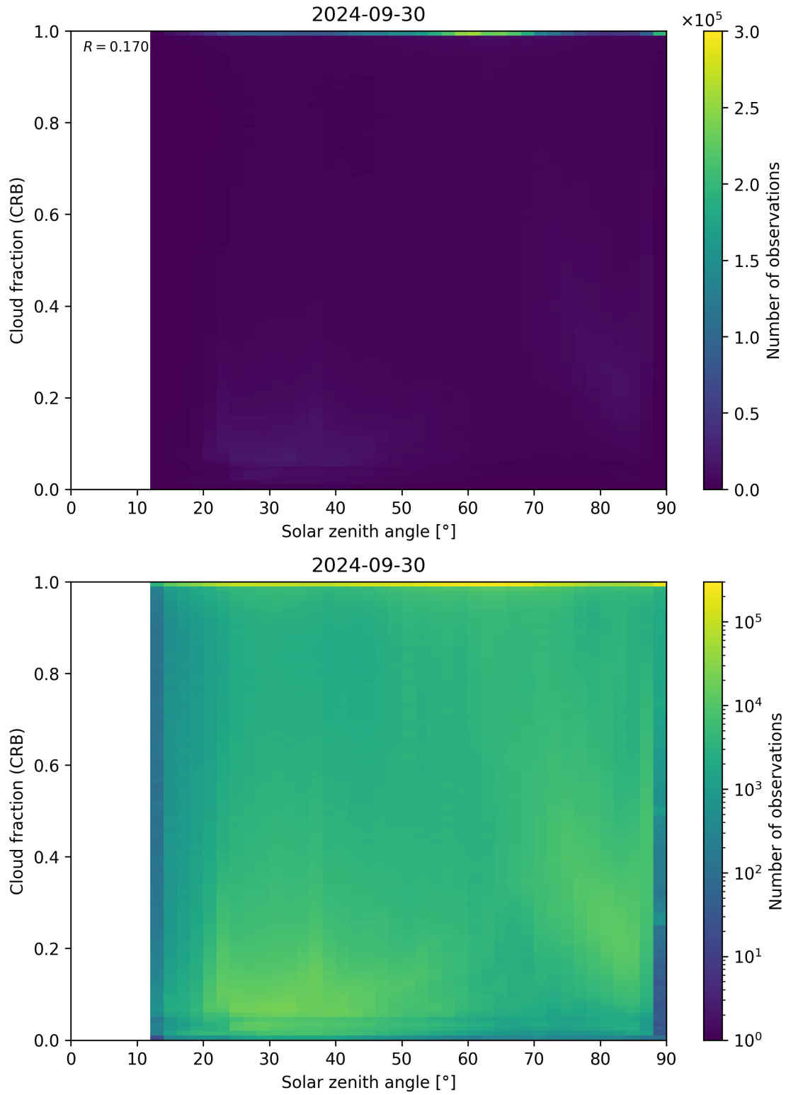
Figure 101: Scatter density plot of “Solar zenith angle” against “Cloud fraction (CRB)” for 2024-09-29 to 2024-10-01.
