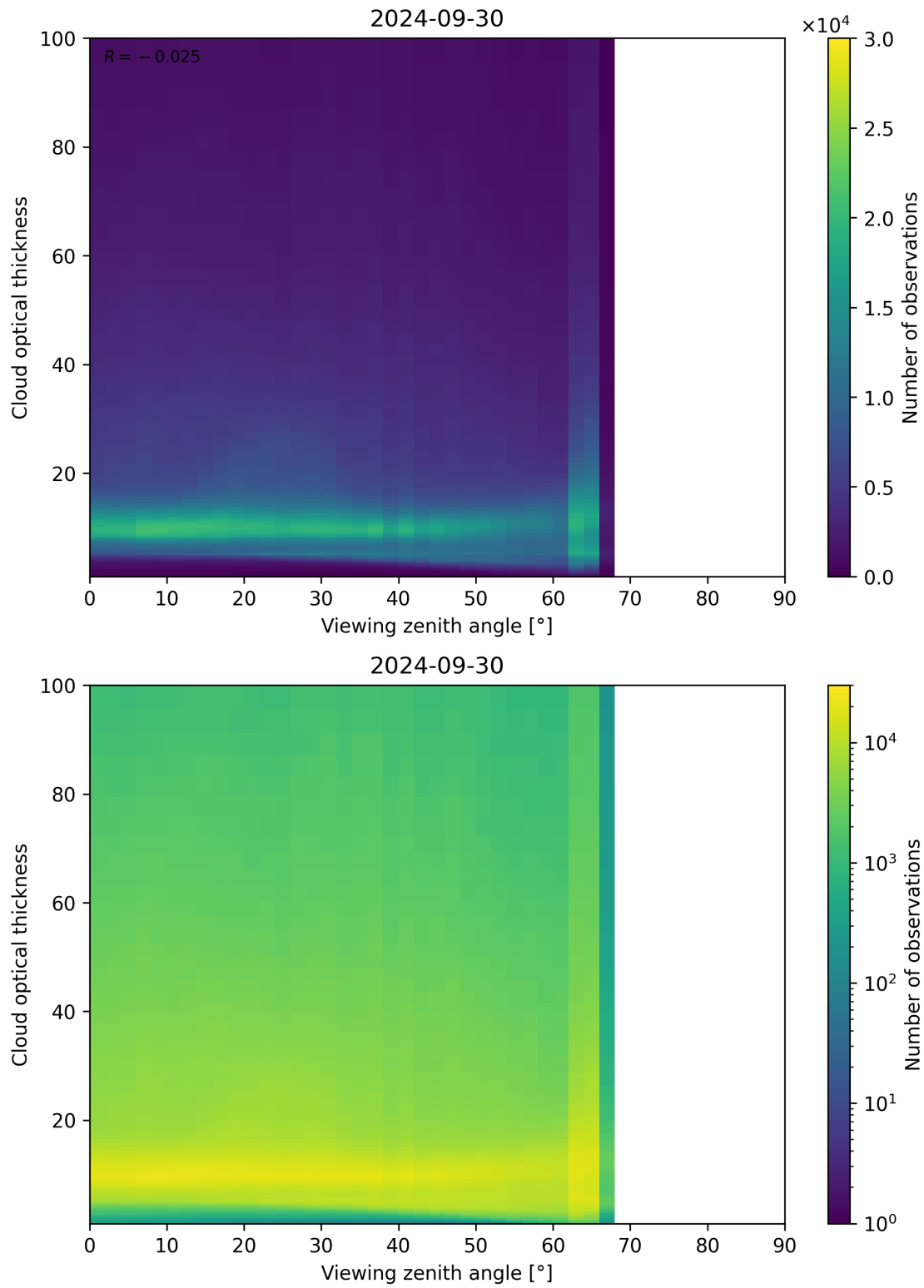
Figure 111: Scatter density plot of “Viewing zenith angle” against “Cloud optical thickness” for 2024-09-29 to 2024-10-01.
