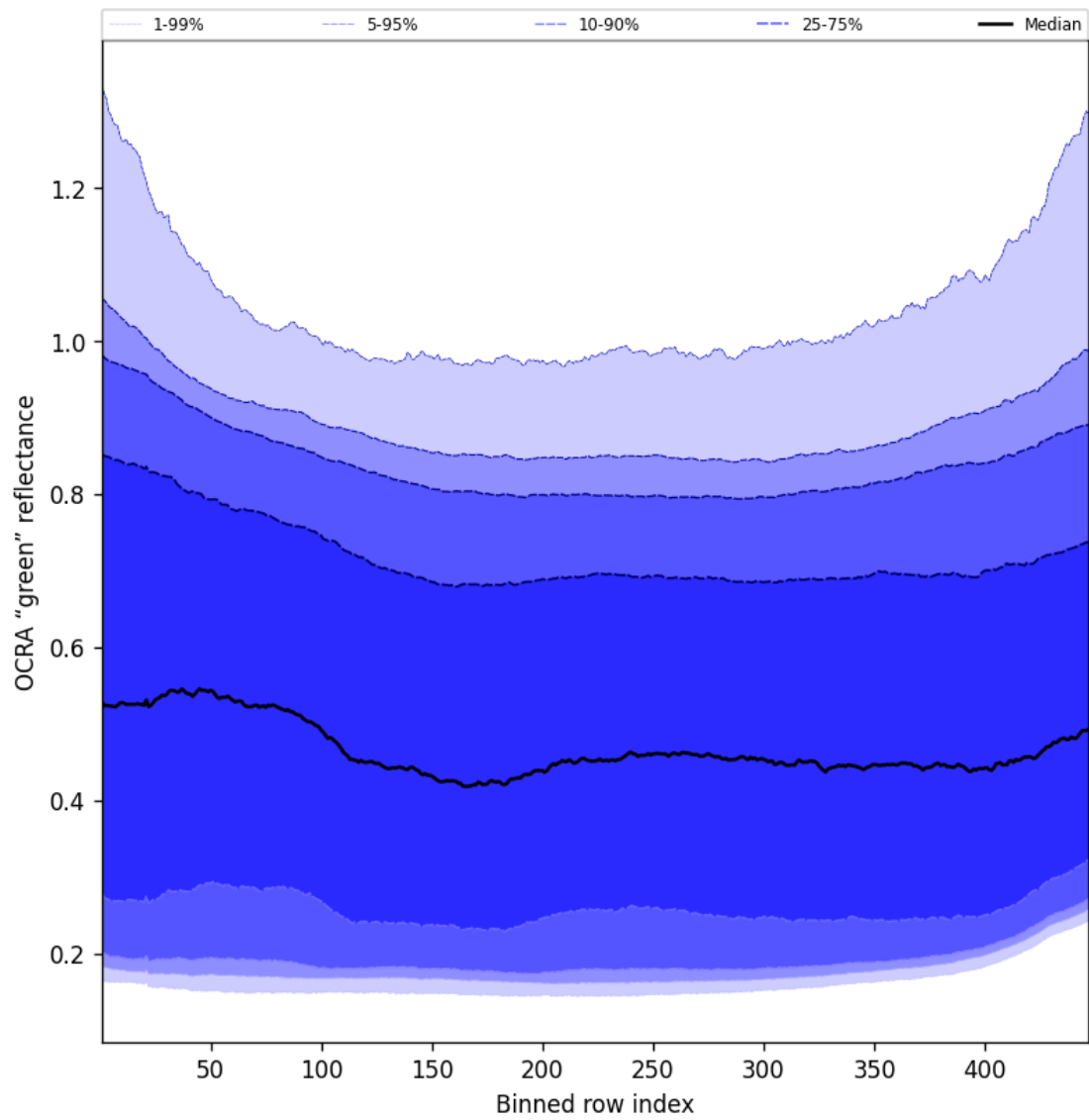
Figure 68: Along track statistics of “OCRA “green” reflectance” for 2024-09-29 to 2024-10-01
