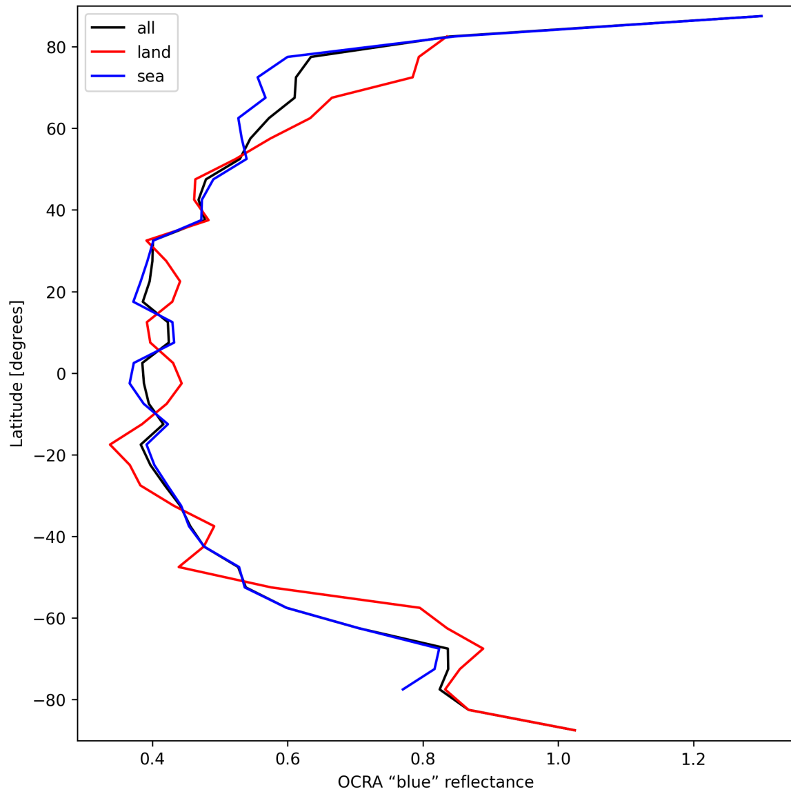
Figure 35: Zonal average of “OCRA “blue” reflectance” for 2024-09-29 to 2024-10-01.
