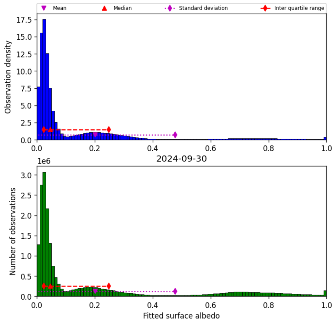
Figure 45: Histogram of “Fitted surface albedo” for 2024-09-29 to 2024-10-01
