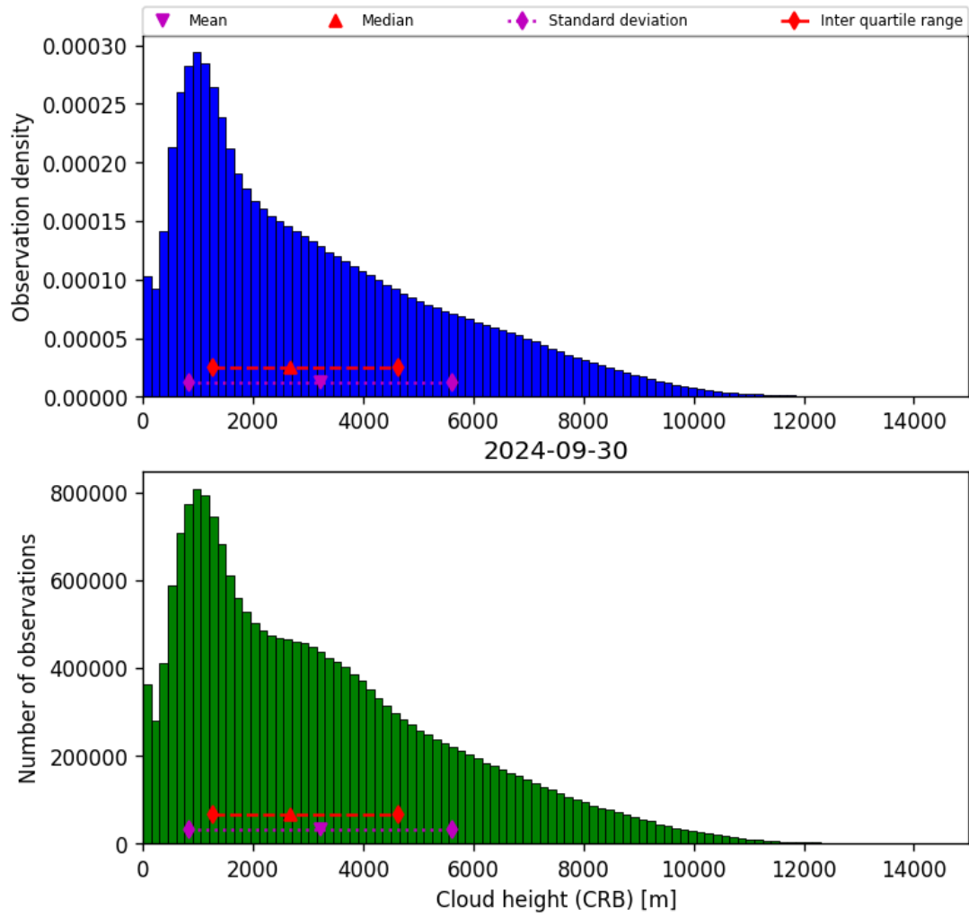
Figure 43: Histogram of “Cloud height (CRB)” for 2024-09-29 to 2024-10-01
