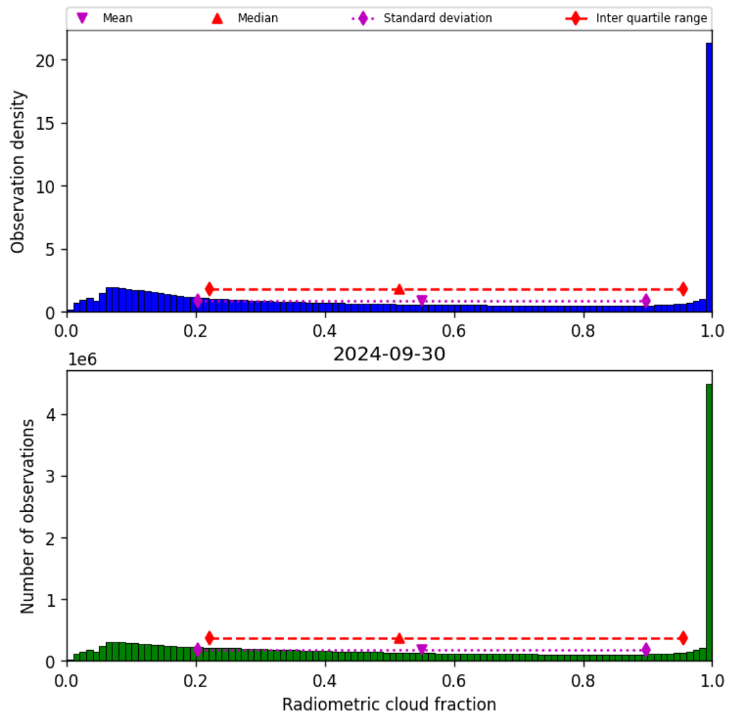
Figure 39: Histogram of “Radiometric cloud fraction” for 2024-09-29 to 2024-10-01
