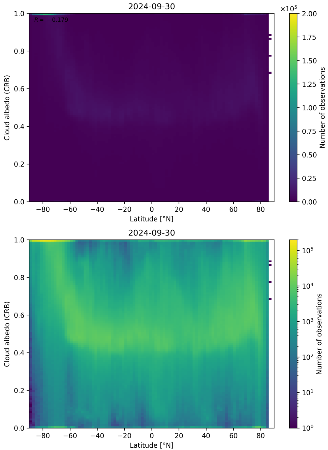
Figure 91: Scatter density plot of “Latitude” against “Cloud albedo (CRB)” for 2024-09-29 to 2024-10-01.
