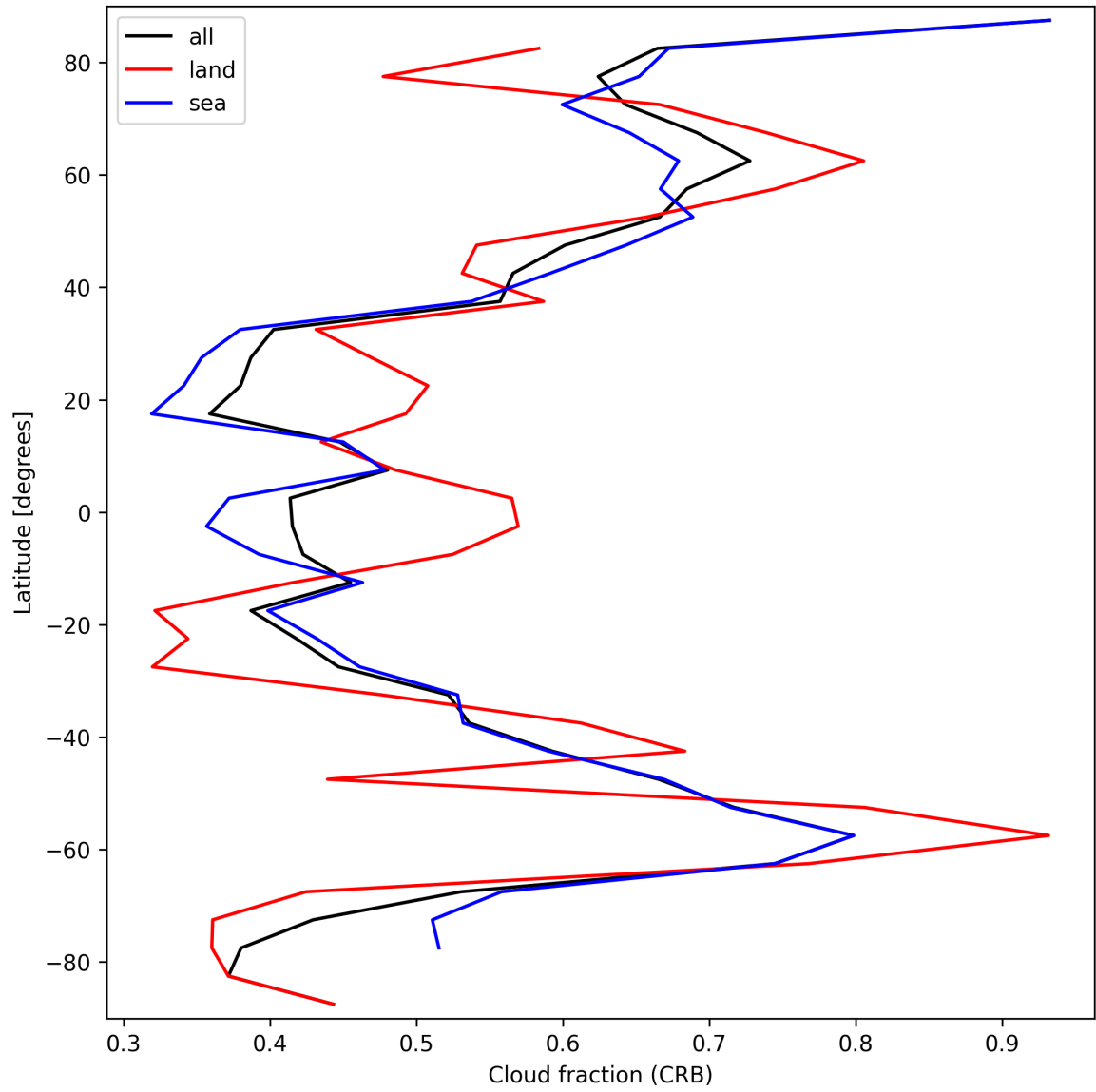
Figure 26: Zonal average of “Cloud fraction (CRB)” for 2024-09-29 to 2024-10-01.
