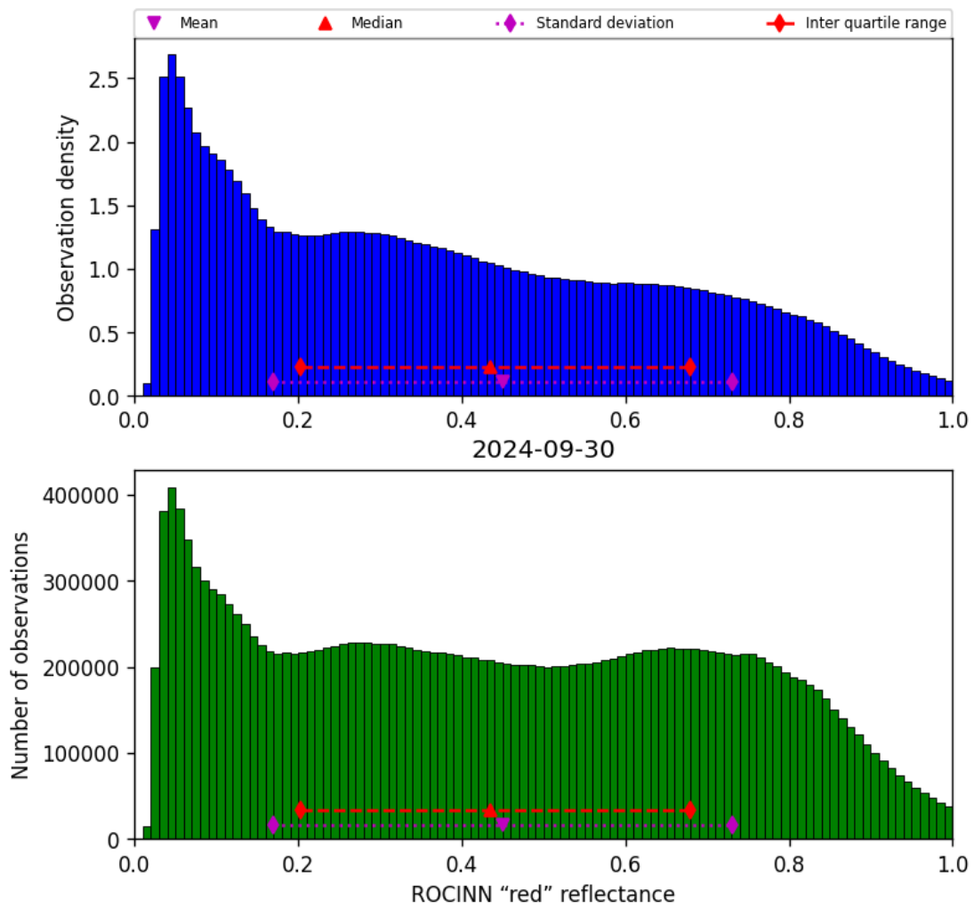
Figure 53: Histogram of “ROCINN “red” reflectance” for 2024-09-29 to 2024-10-01
