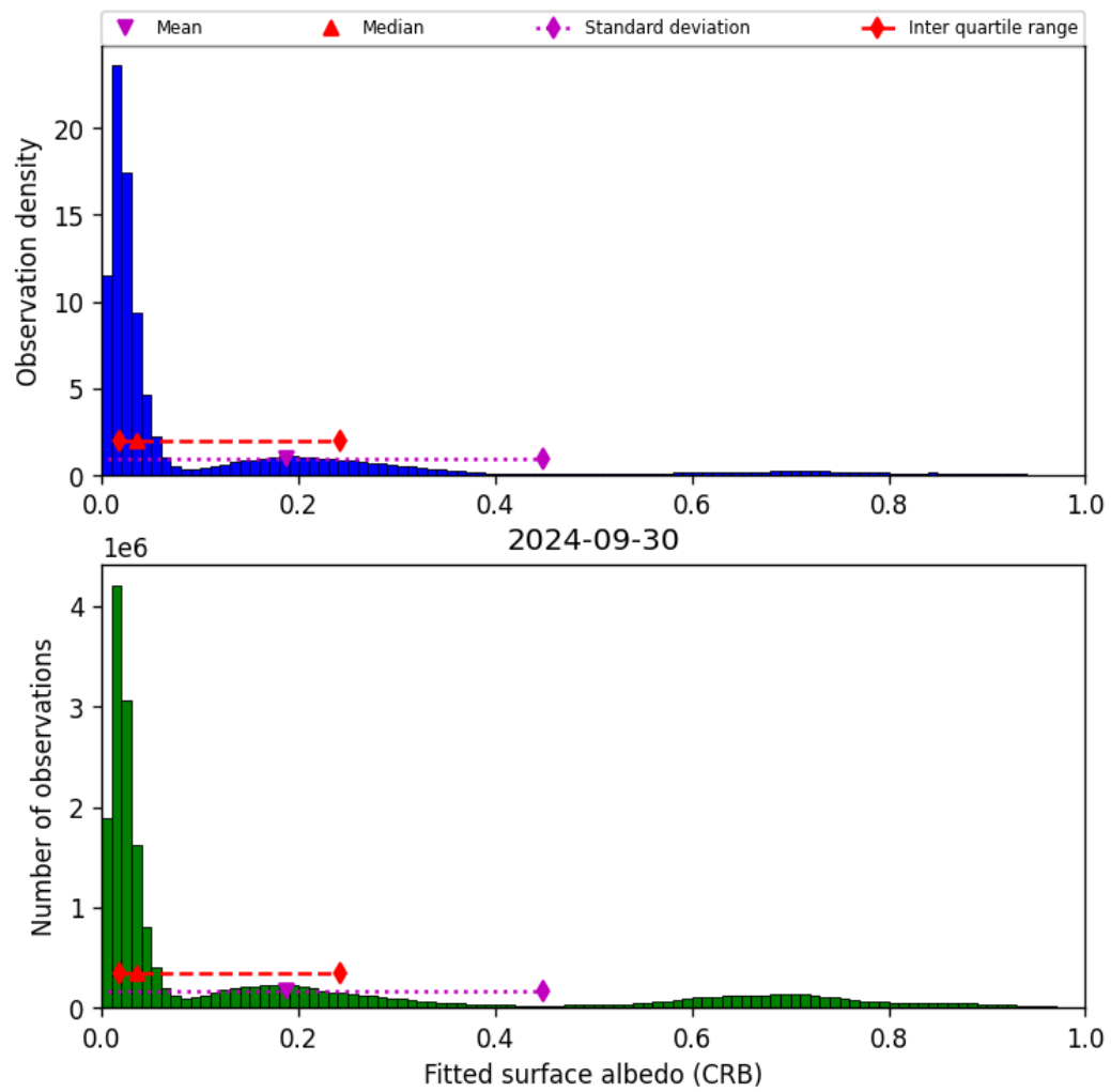
Figure 46: Histogram of “Fitted surface albedo (CRB)” for 2024-09-29 to 2024-10-01
