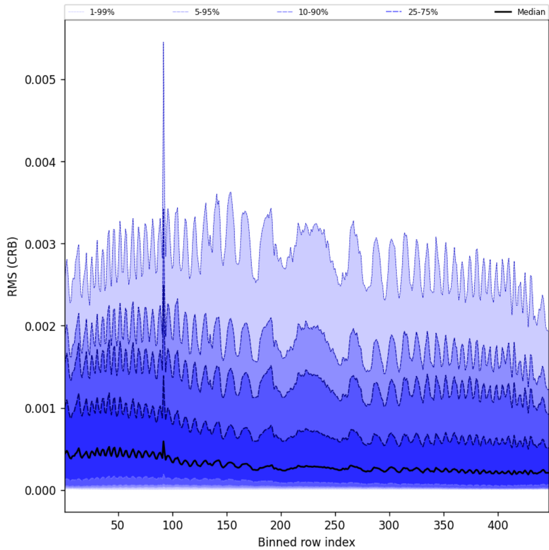
Figure 64: Along track statistics of “RMS (CRB)” for 2024-09-29 to 2024-10-01
