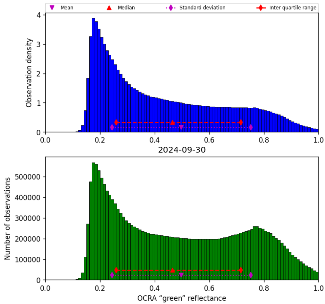
Figure 52: Histogram of “OCRA “green” reflectance” for 2024-09-29 to 2024-10-01
