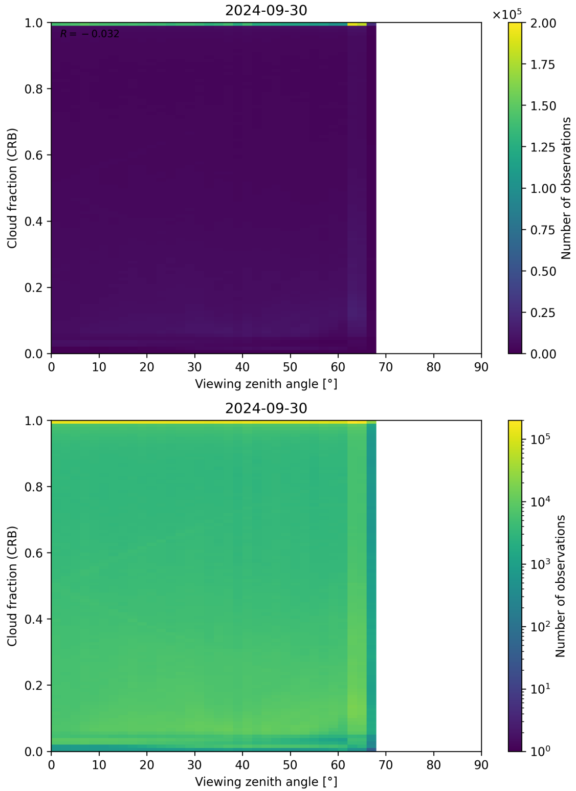
Figure 109: Scatter density plot of “Viewing zenith angle” against “Cloud fraction (CRB)” for 2024-09-29 to 2024-10-01.
