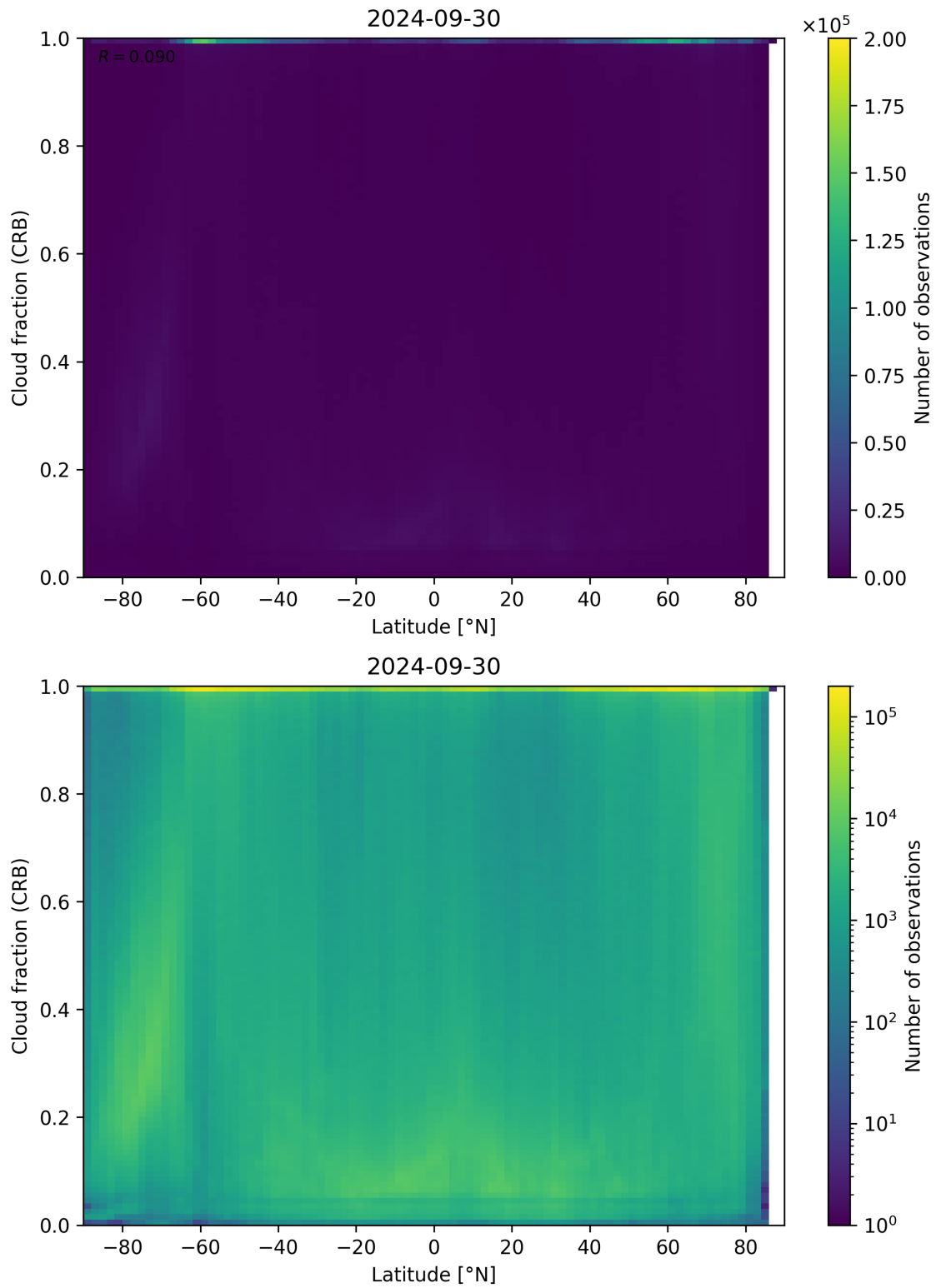
Figure 94: Scatter density plot of “Latitude” against “Cloud fraction (CRB)” for 2024-09-29 to 2024-10-01.
