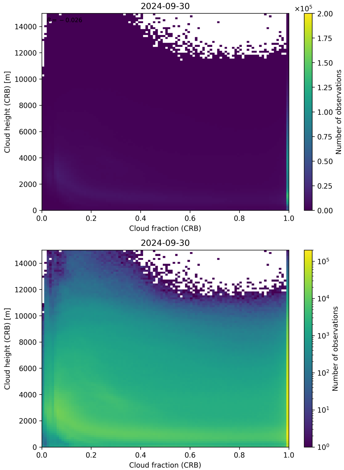
Figure 79: Scatter density plot of “Cloud fraction (CRB)” against “Cloud height (CRB)” for 2024-09-29 to 2024-10-01.
