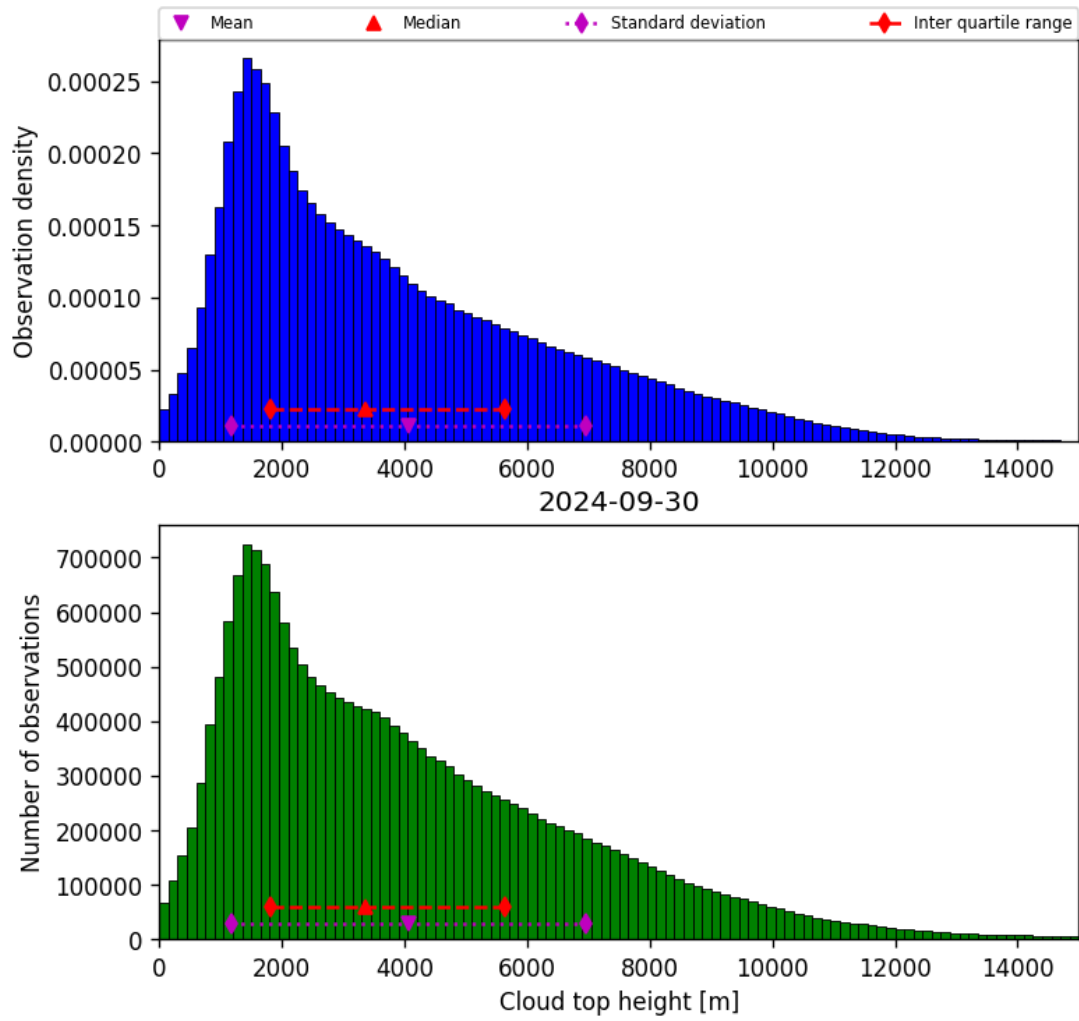
Figure 40: Histogram of “Cloud top height” for 2024-09-29 to 2024-10-01
