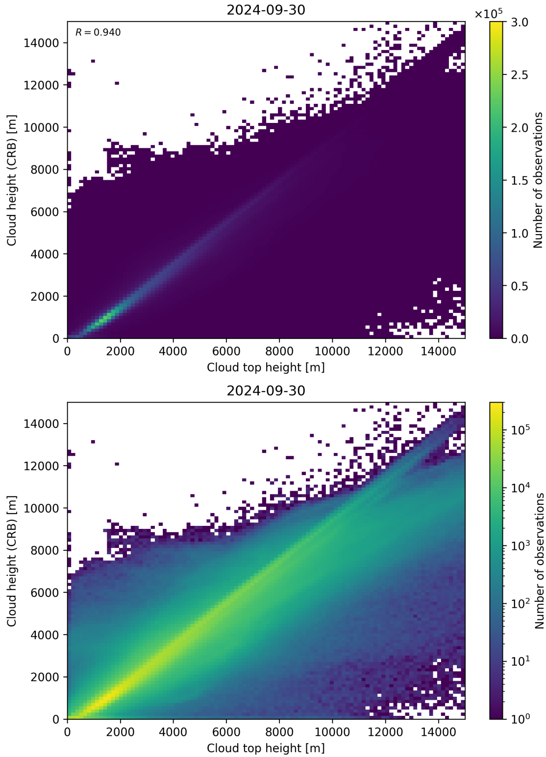
Figure 89: Scatter density plot of “Cloud top height” against “Cloud height (CRB)” for 2024-09-29 to 2024-10-01.
