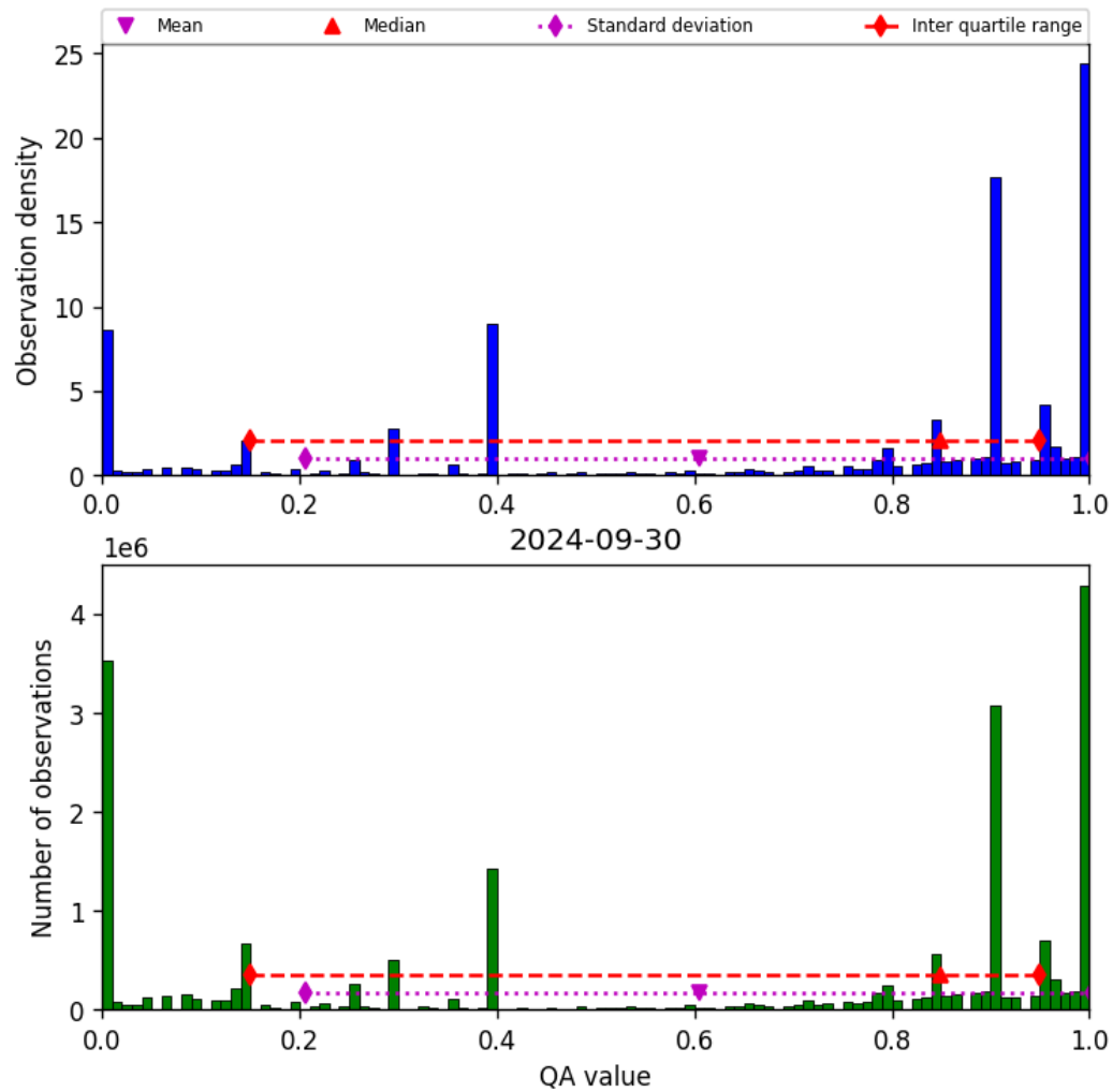
Figure 38: Histogram of “QA value” for 2024-09-29 to 2024-10-01
