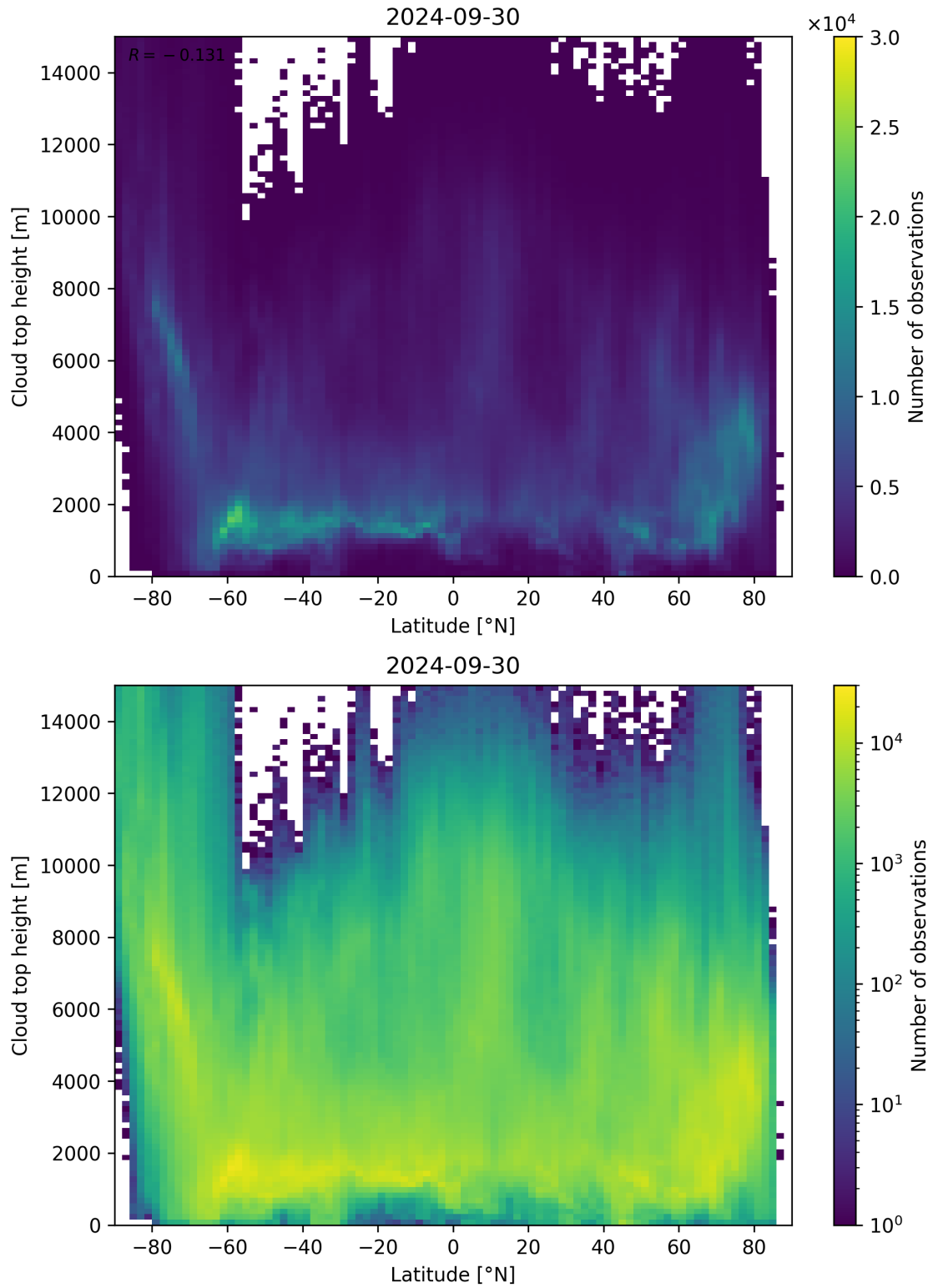
Figure 97: Scatter density plot of “Latitude” against “Cloud top height” for 2024-09-29 to 2024-10-01.
