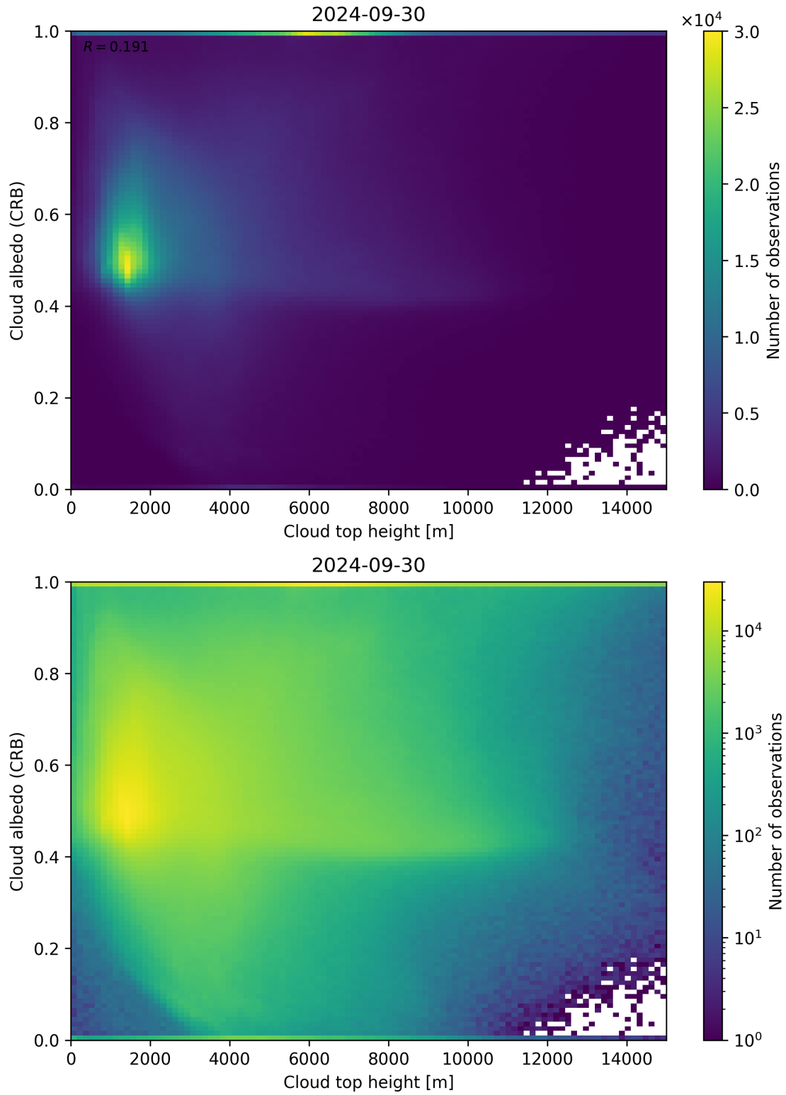
Figure 86: Scatter density plot of “Cloud top height” against “Cloud albedo (CRB)” for 2024-09-29 to 2024-10-01.
