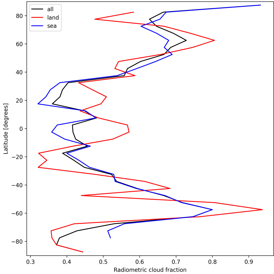
Figure 23: Zonal average of “Radiometric cloud fraction” for 2024-09-29 to 2024-10-01.
