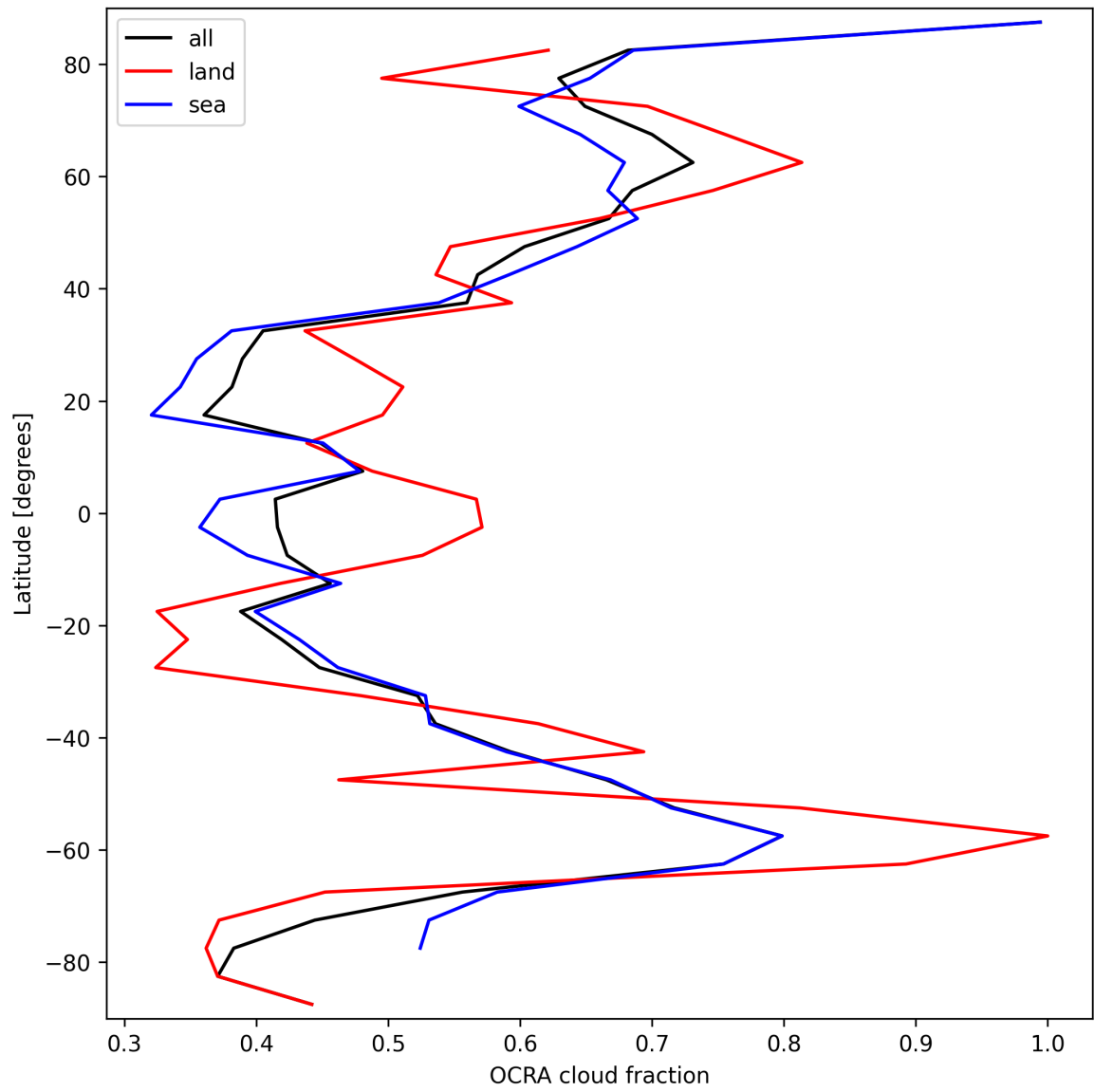
Figure 34: Zonal average of “OCRA cloud fraction” for 2024-09-29 to 2024-10-01.
