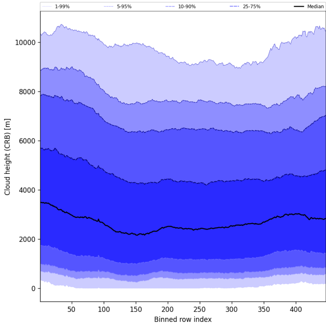
Figure 59: Along track statistics of “Cloud height (CRB)” for 2024-09-29 to 2024-10-01
