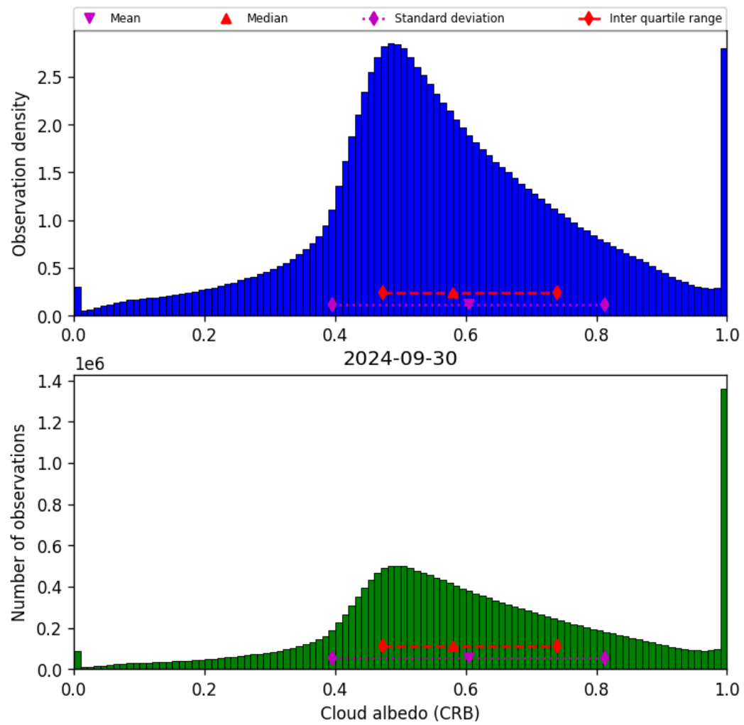
Figure 44: Histogram of “Cloud albedo (CRB)” for 2024-09-29 to 2024-10-01
