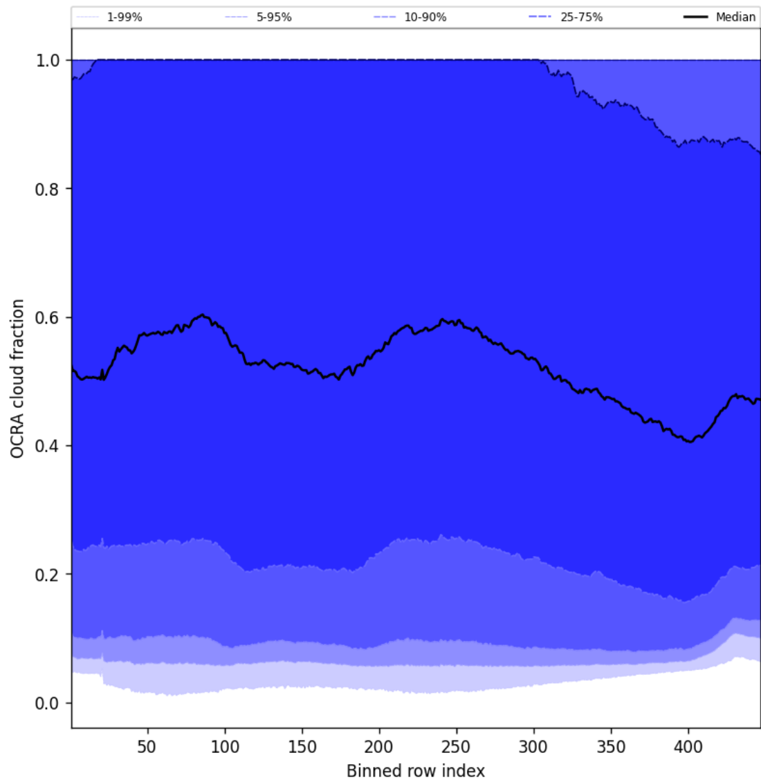
Figure 66: Along track statistics of “OCRA cloud fraction” for 2024-09-29 to 2024-10-01
