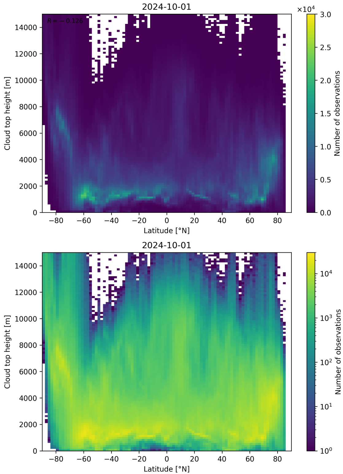
Figure 97: Scatter density plot of “Latitude” against “Cloud top height” for 2024-09-30 to 2024-10-02.
