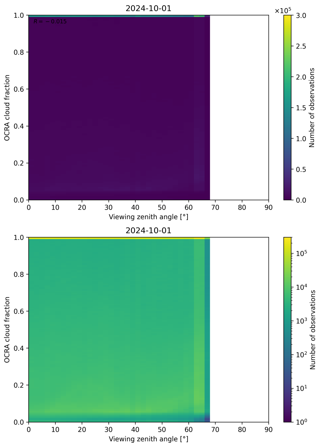
Figure 108: Scatter density plot of “Viewing zenith angle” against “OCRA cloud fraction” for 2024-09-30 to 2024-10-02.
