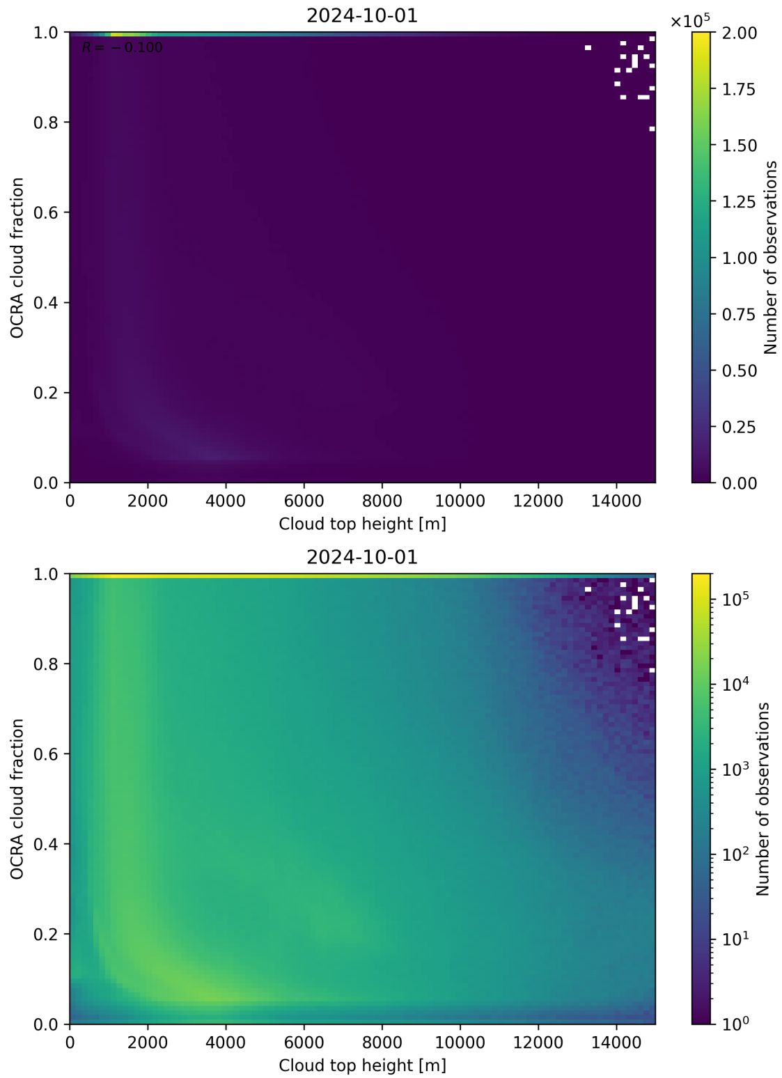
Figure 87: Scatter density plot of “Cloud top height” against “OCRA cloud fraction” for 2024-09-30 to 2024-10-02.
