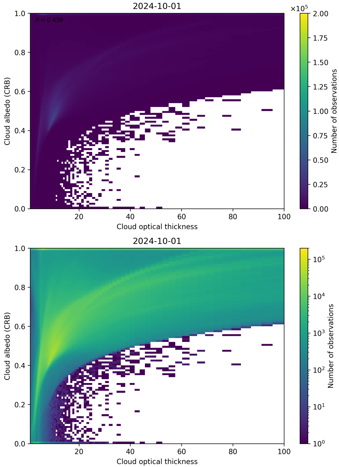
Figure 82: Scatter density plot of “Cloud optical thickness” against “Cloud albedo (CRB)” for 2024-09-30 to 2024-10-02.
