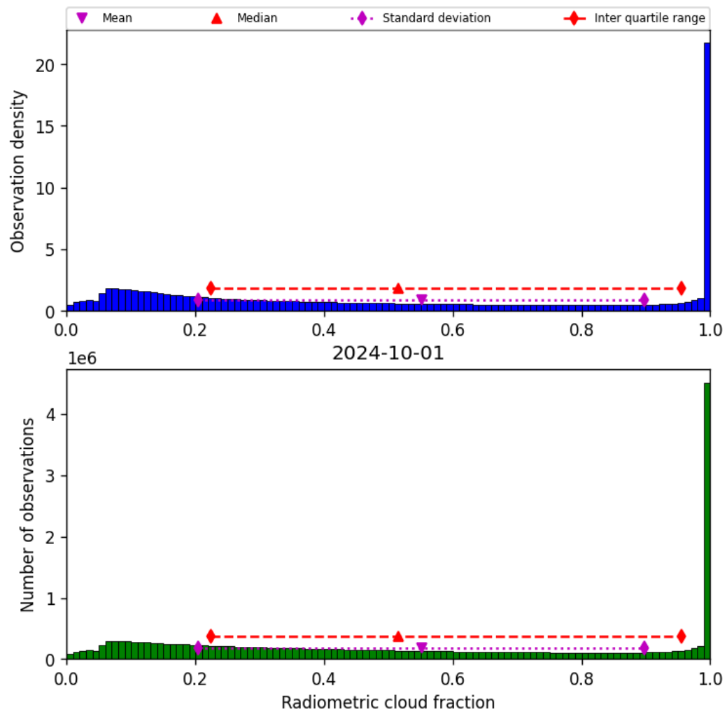
Figure 39: Histogram of “Radiometric cloud fraction” for 2024-09-30 to 2024-10-02
