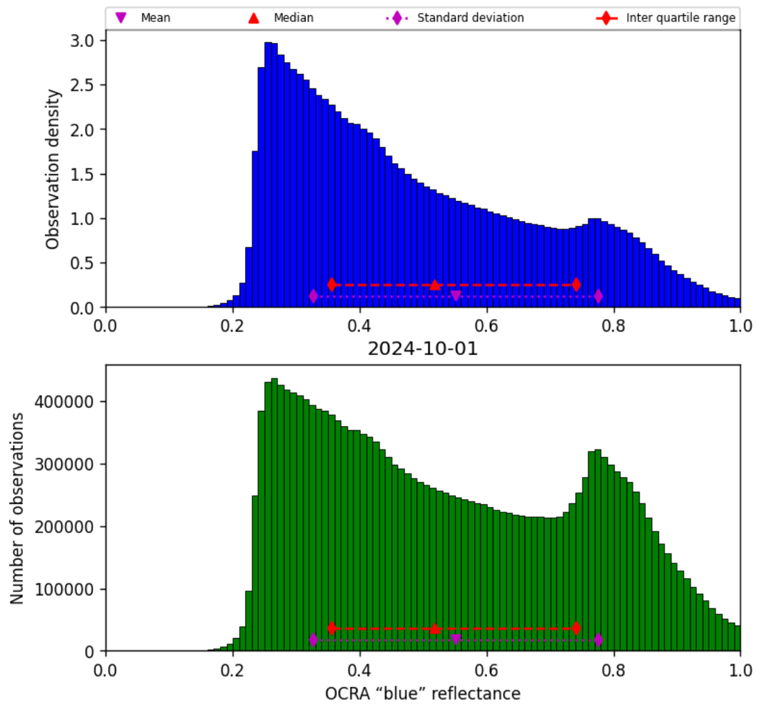
Figure 51: Histogram of “OCRA “blue” reflectance” for 2024-09-30 to 2024-10-02
