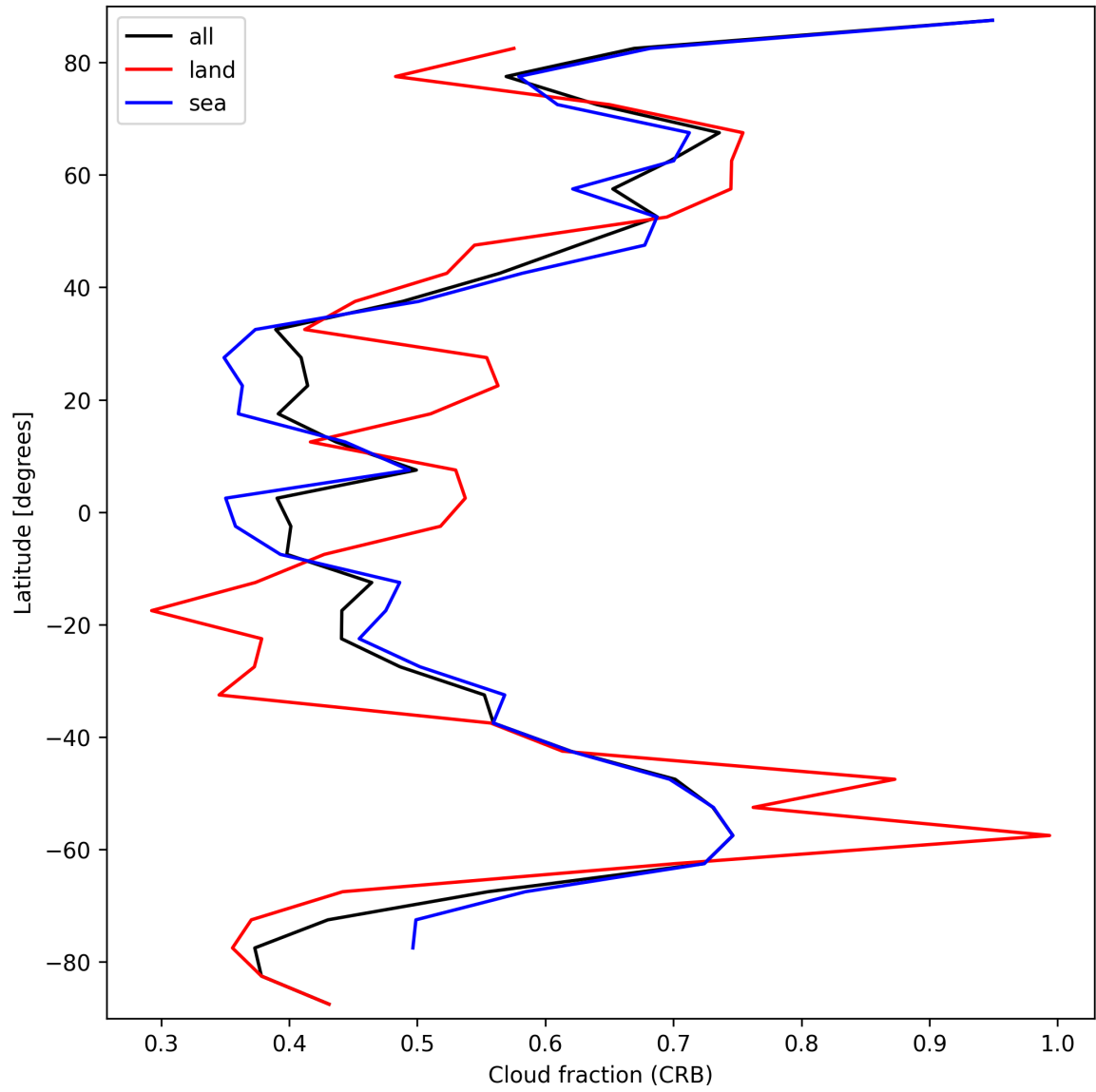
Figure 26: Zonal average of “Cloud fraction (CRB)” for 2024-09-30 to 2024-10-02.
