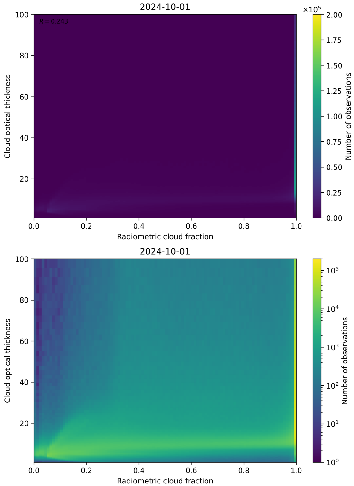
Figure 75: Scatter density plot of “Radiometric cloud fraction” against “Cloud optical thickness” for 2024-09-30 to 2024-10-02.
