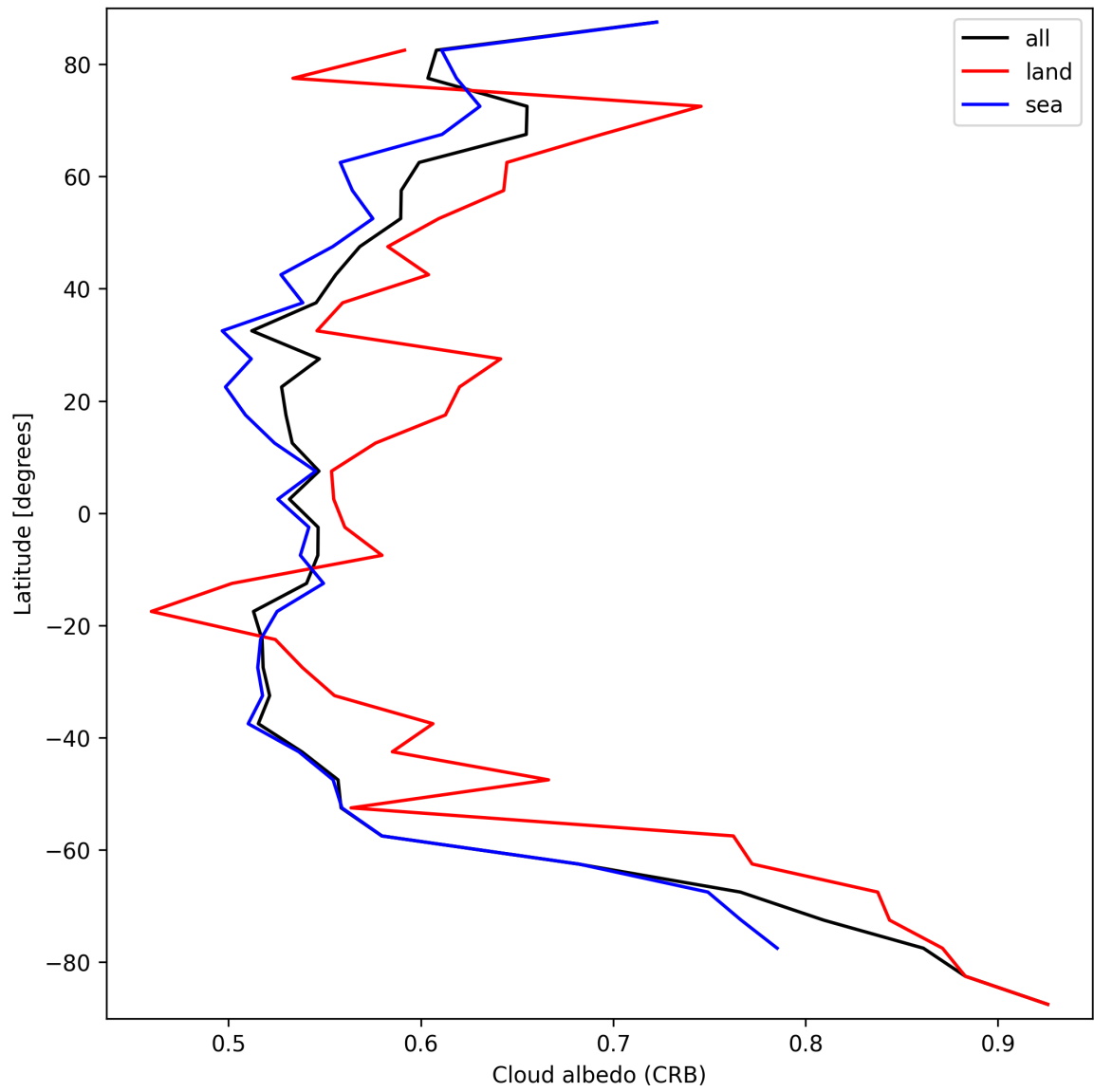
Figure 28: Zonal average of “Cloud albedo (CRB)” for 2024-09-30 to 2024-10-02.
