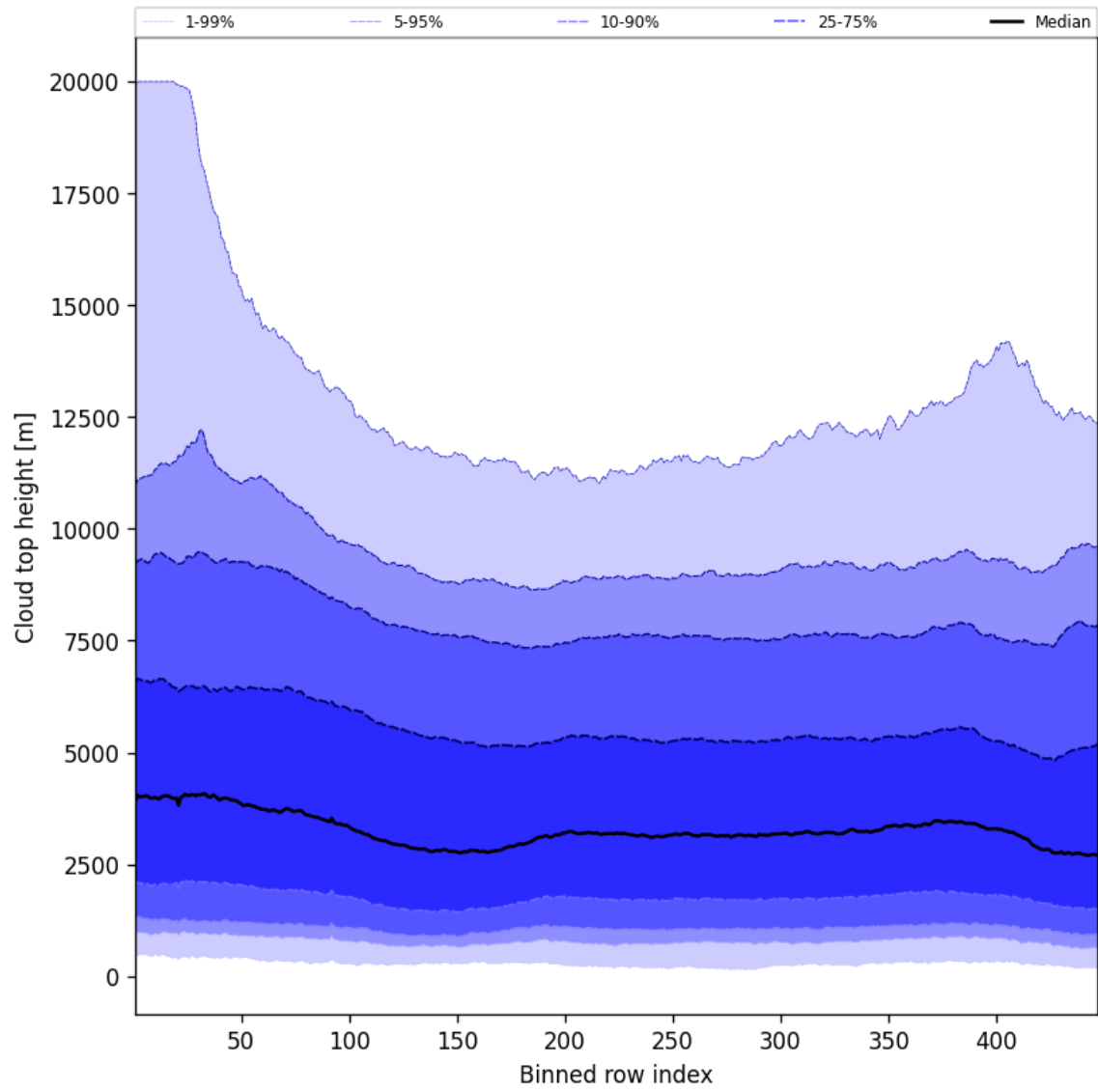
Figure 56: Along track statistics of “Cloud top height” for 2024-09-30 to 2024-10-02
