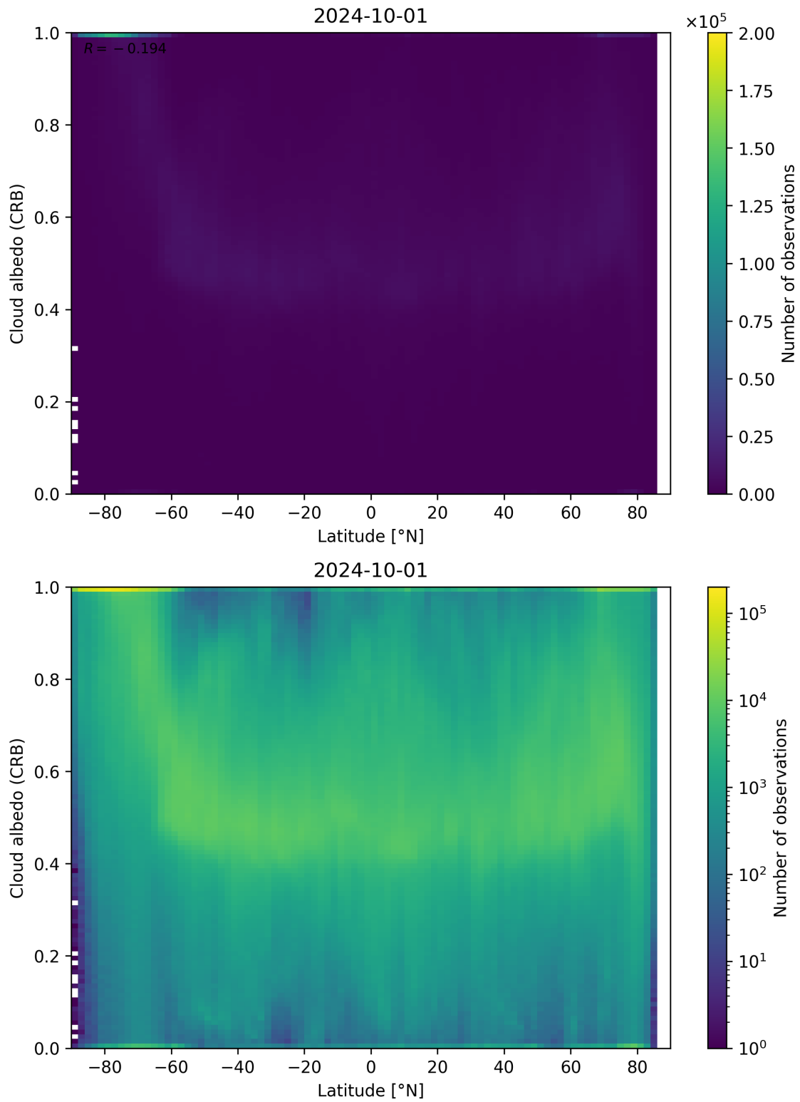
Figure 91: Scatter density plot of “Latitude” against “Cloud albedo (CRB)” for 2024-09-30 to 2024-10-02.
