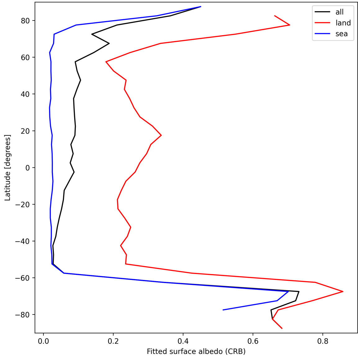
Figure 30: Zonal average of “Fitted surface albedo (CRB)” for 2024-09-30 to 2024-10-02.
