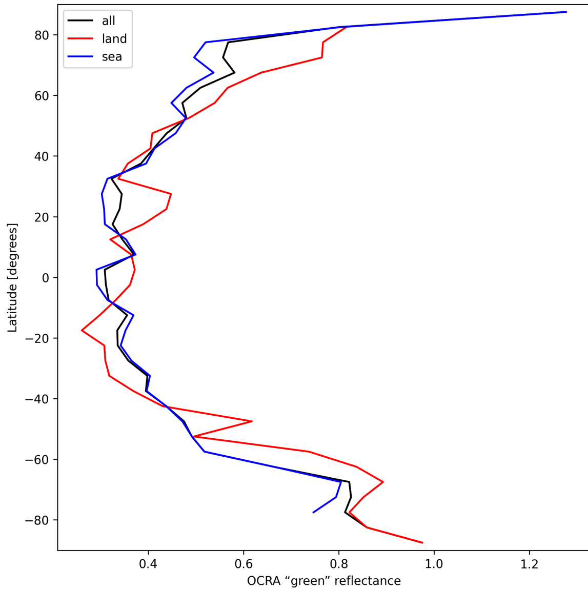
Figure 36: Zonal average of “OCRA “green” reflectance” for 2024-09-30 to 2024-10-02.
