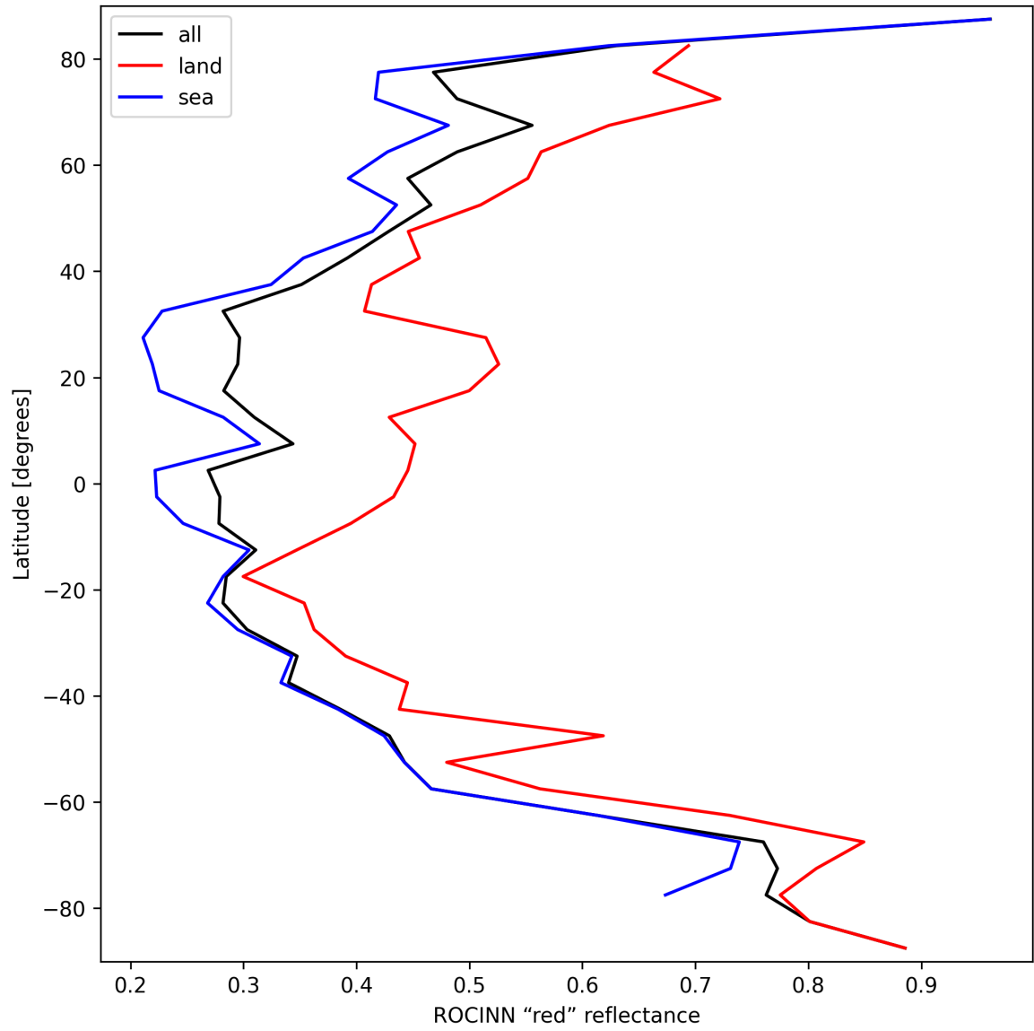
Figure 37: Zonal average of “ROCINN “red” reflectance” for 2024-09-30 to 2024-10-02.
