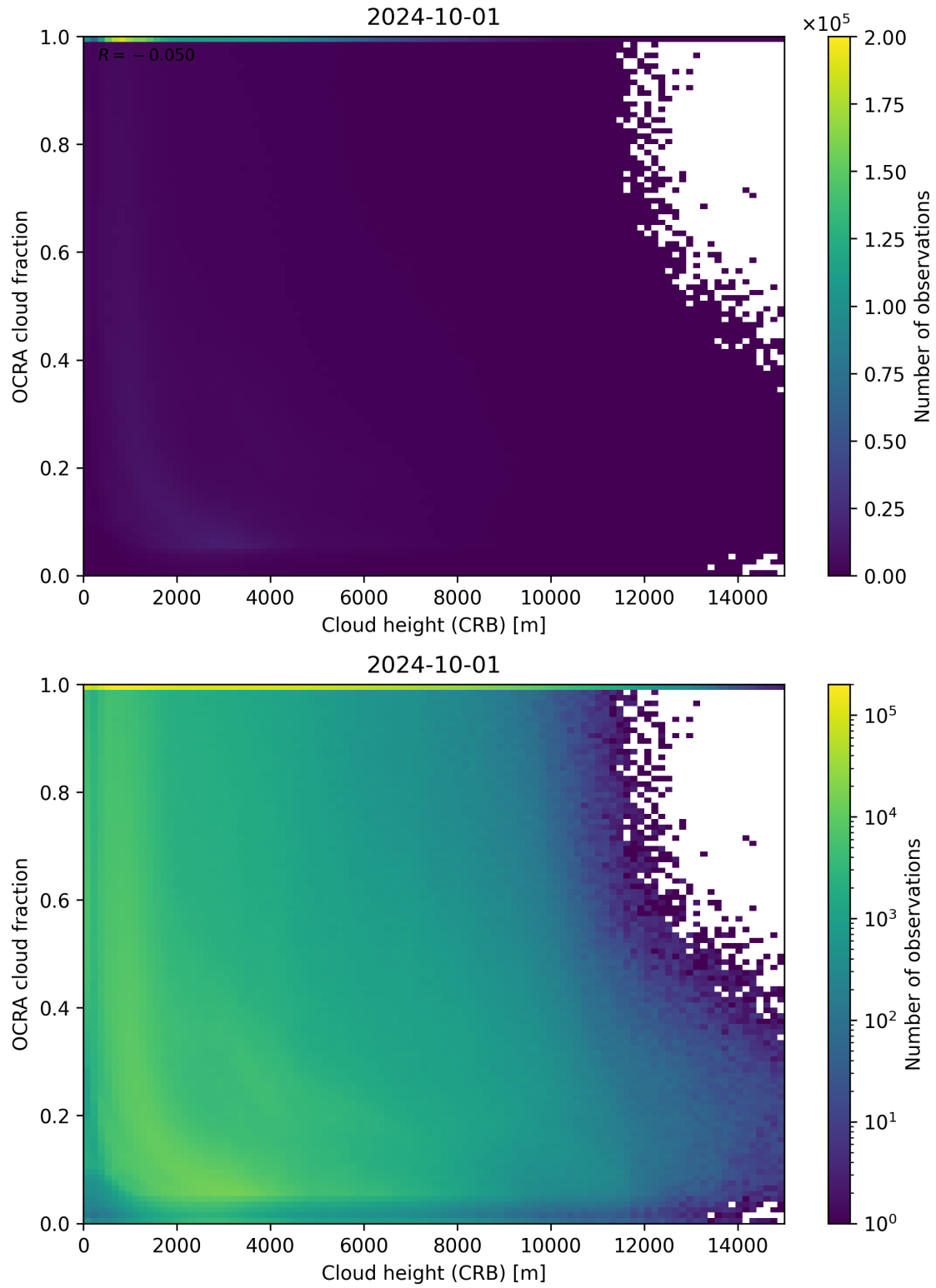
Figure 81: Scatter density plot of “Cloud height (CRB)” against “OCRA cloud fraction” for 2024-09-30 to 2024-10-02.
