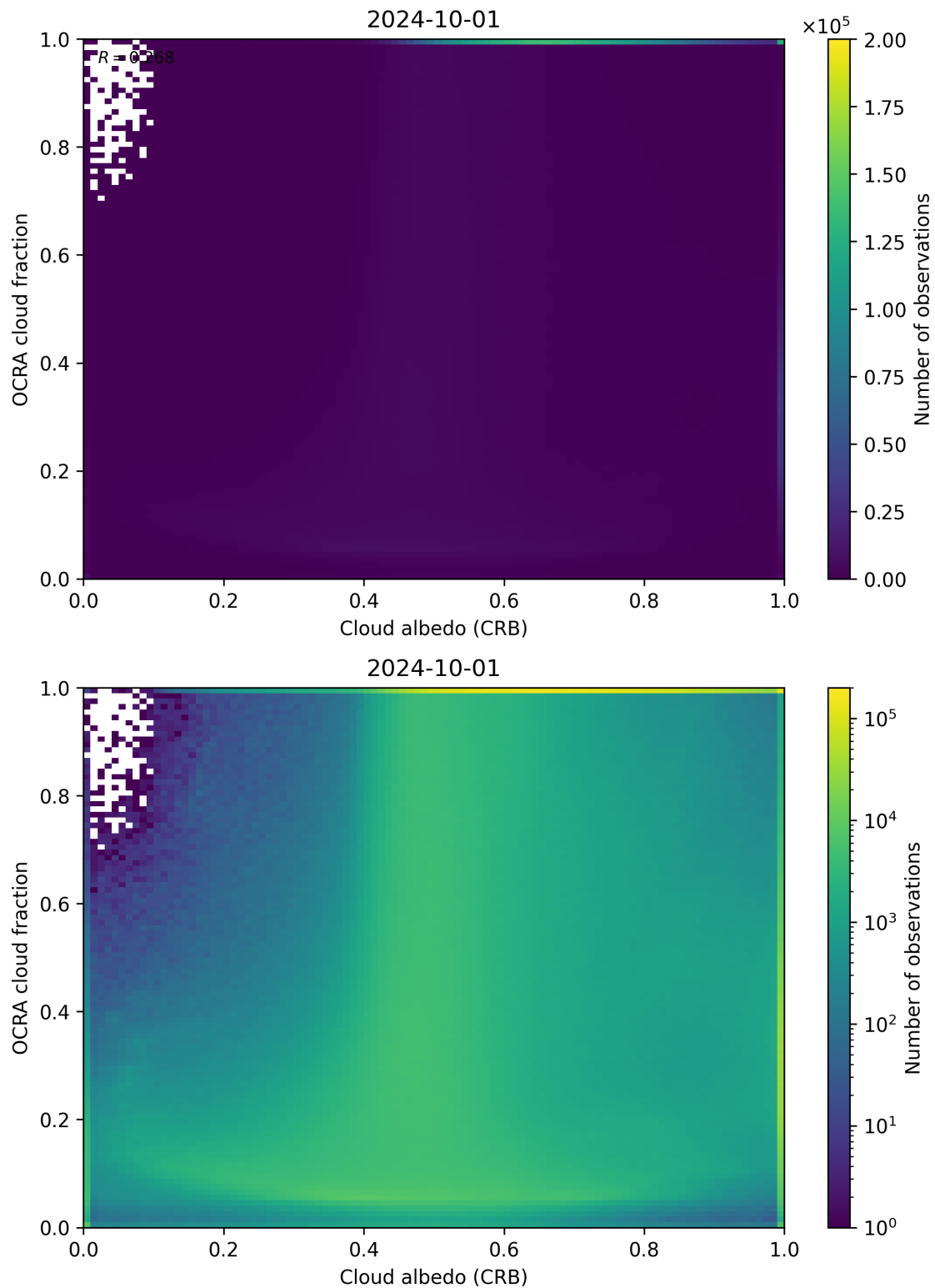
Figure 70: Scatter density plot of “Cloud albedo (CRB)” against “OCRA cloud fraction” for 2024-09-30 to 2024-10-02.
