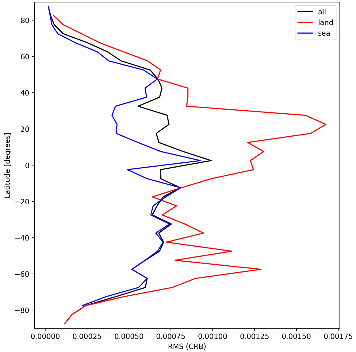
Figure 32: Zonal average of “RMS (CRB)” for 2024-09-30 to 2024-10-02.
