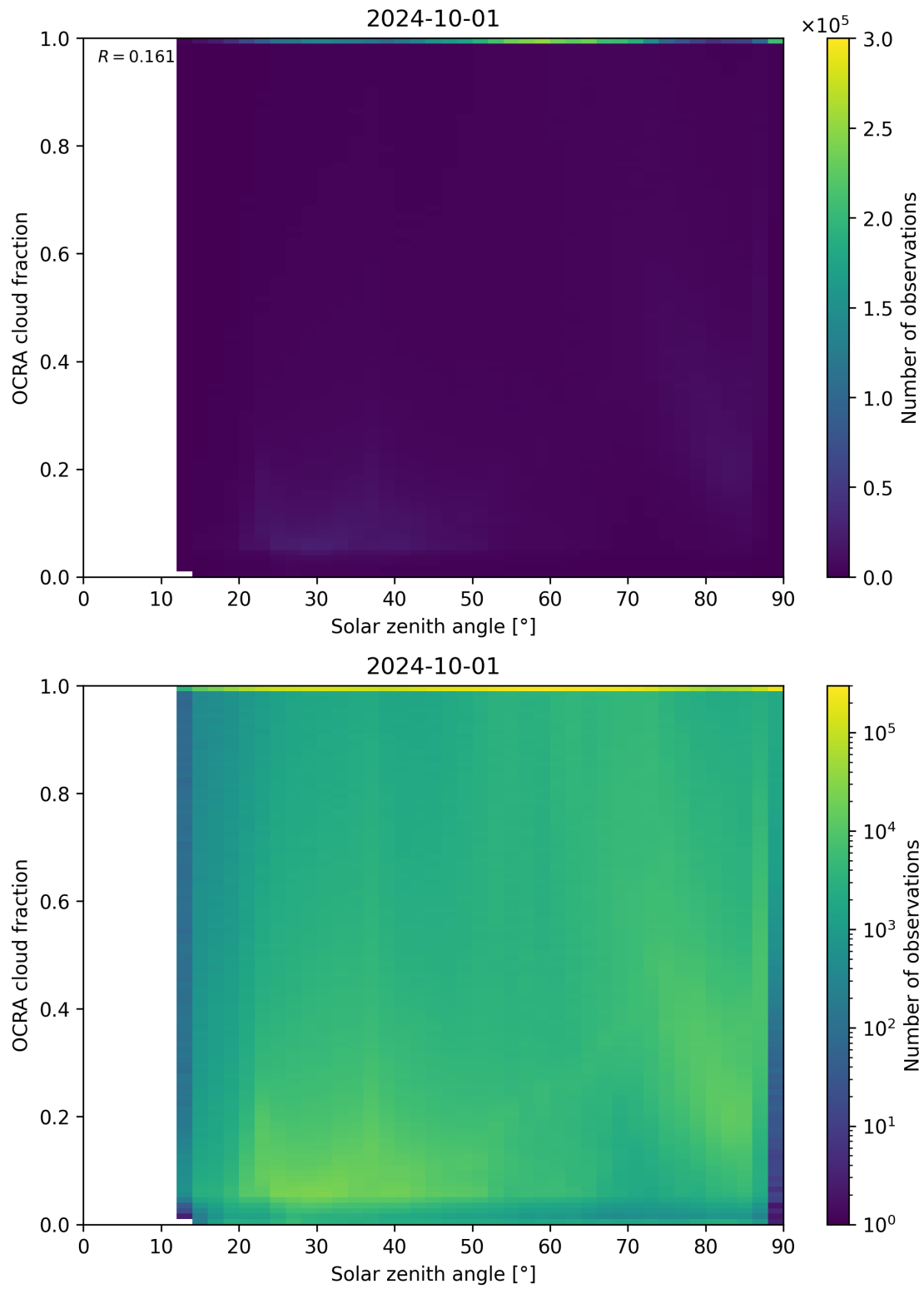
Figure 100: Scatter density plot of “Solar zenith angle” against “OCRA cloud fraction” for 2024-09-30 to 2024-10-02.
