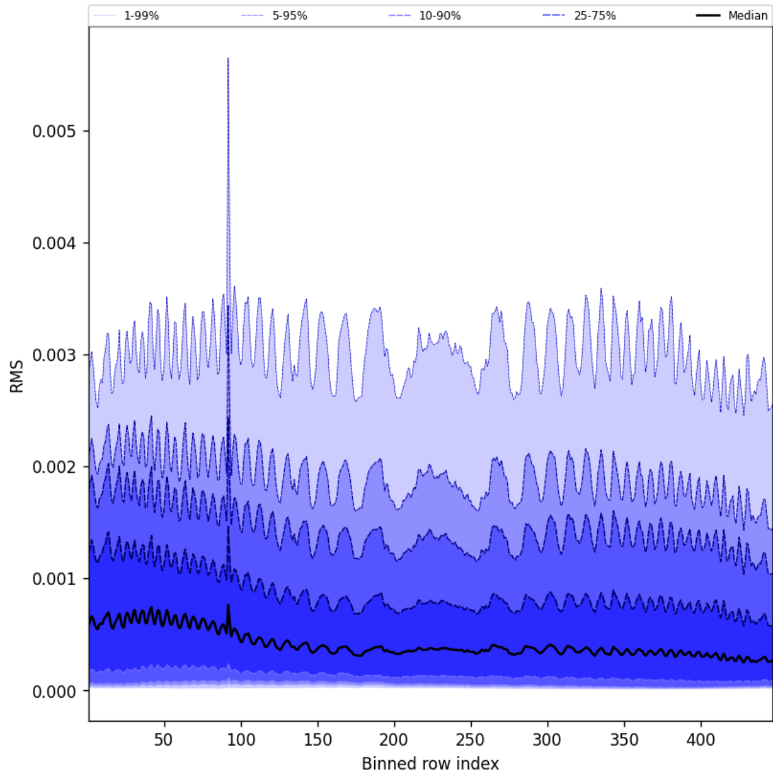
Figure 63: Along track statistics of “RMS” for 2024-09-30 to 2024-10-02
