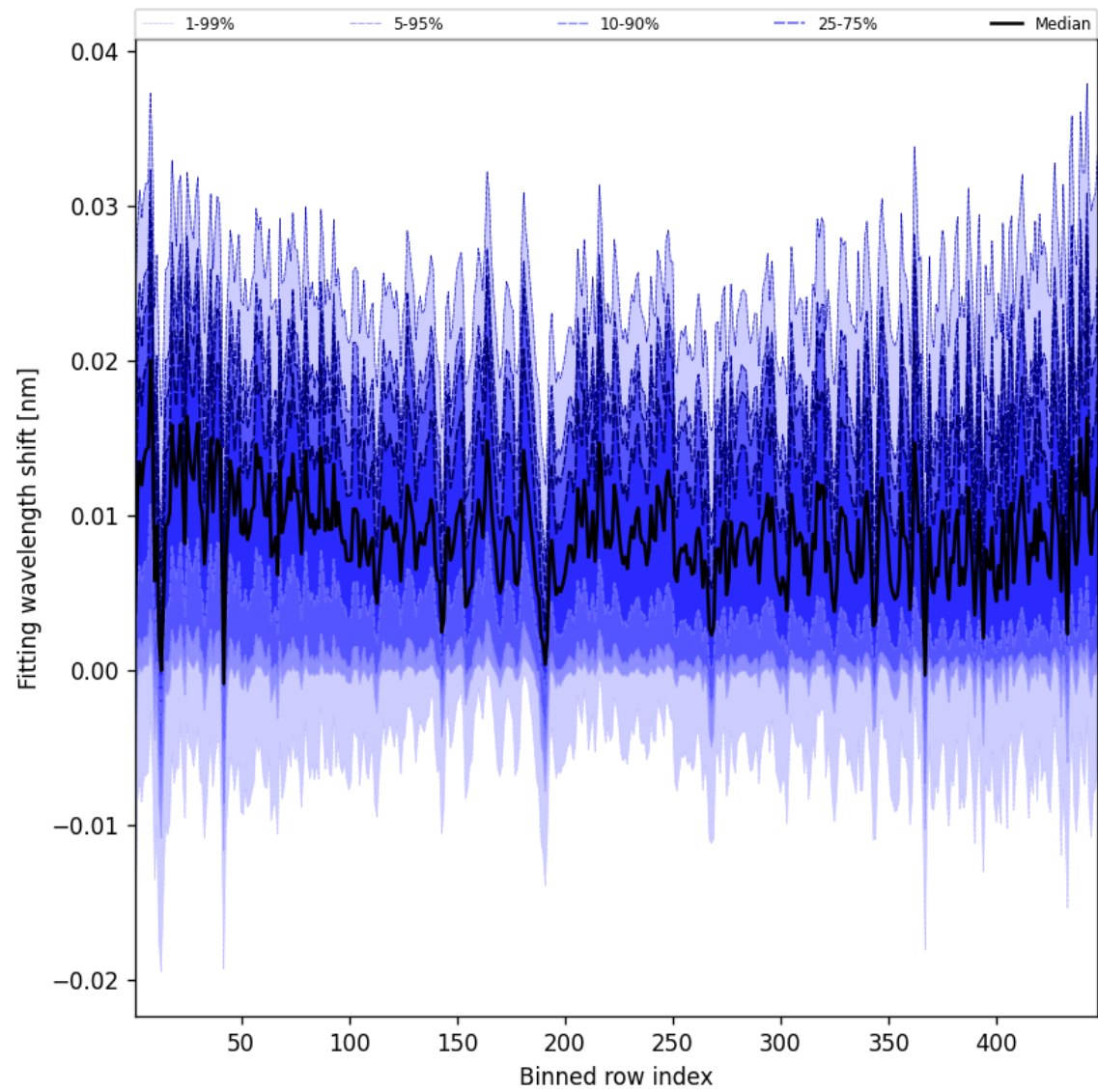
Figure 65: Along track statistics of “Fitting wavelength shift” for 2024-09-30 to 2024-10-02
