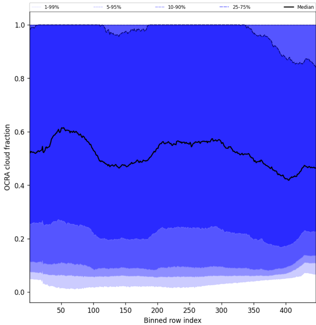
Figure 66: Along track statistics of “OCRA cloud fraction” for 2024-09-30 to 2024-10-02
