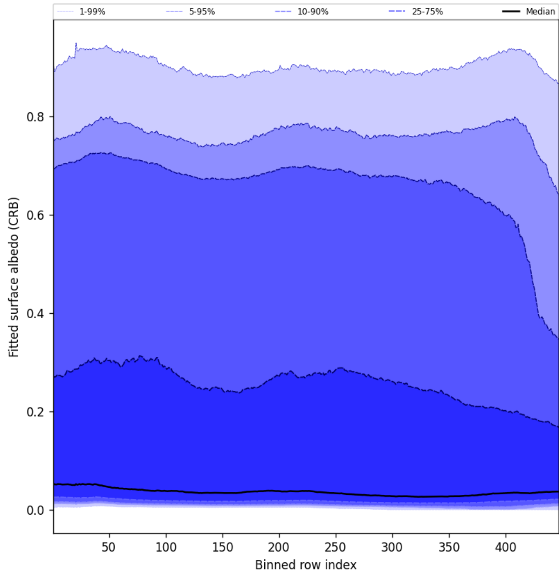
Figure 62: Along track statistics of “Fitted surface albedo (CRB)” for 2024-09-30 to 2024-10-02
