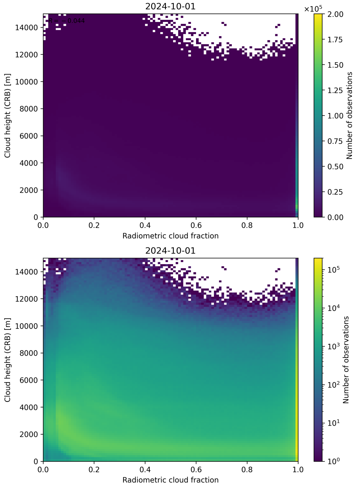
Figure 74: Scatter density plot of “Radiometric cloud fraction” against “Cloud height (CRB)” for 2024-09-30 to 2024-10-02.
