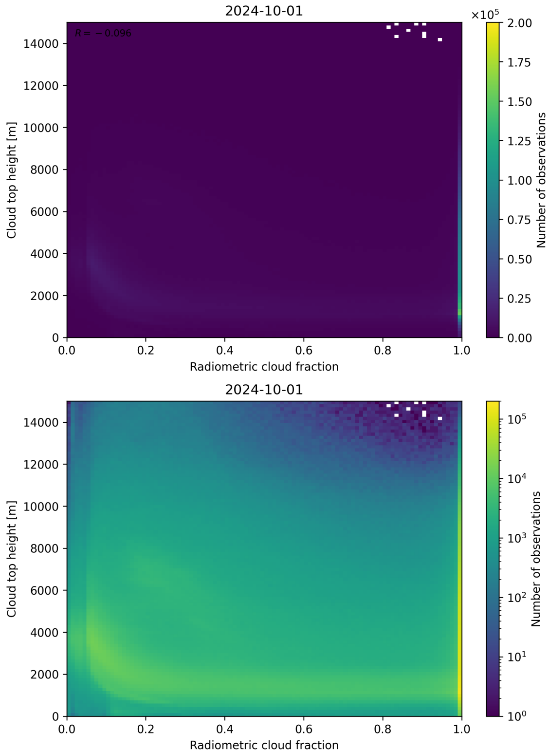
Figure 76: Scatter density plot of “Radiometric cloud fraction” against “Cloud top height” for 2024-09-30 to 2024-10-02.
