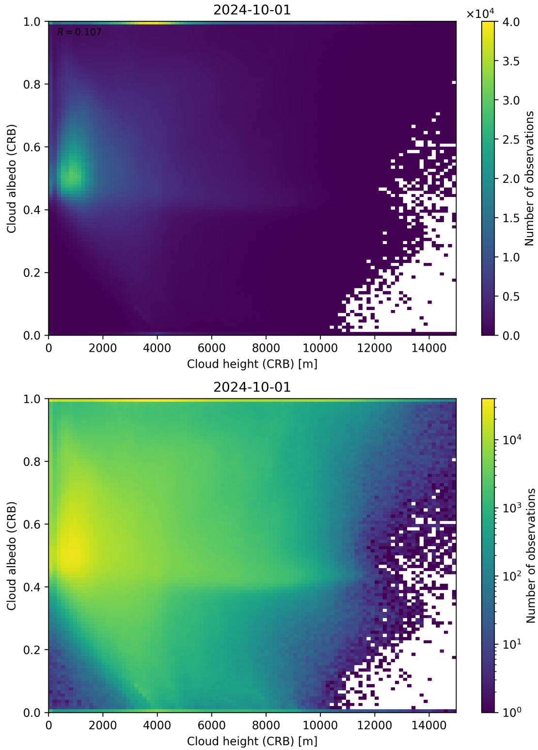
Figure 80: Scatter density plot of “Cloud height (CRB)” against “Cloud albedo (CRB)” for 2024-09-30 to 2024-10-02.
