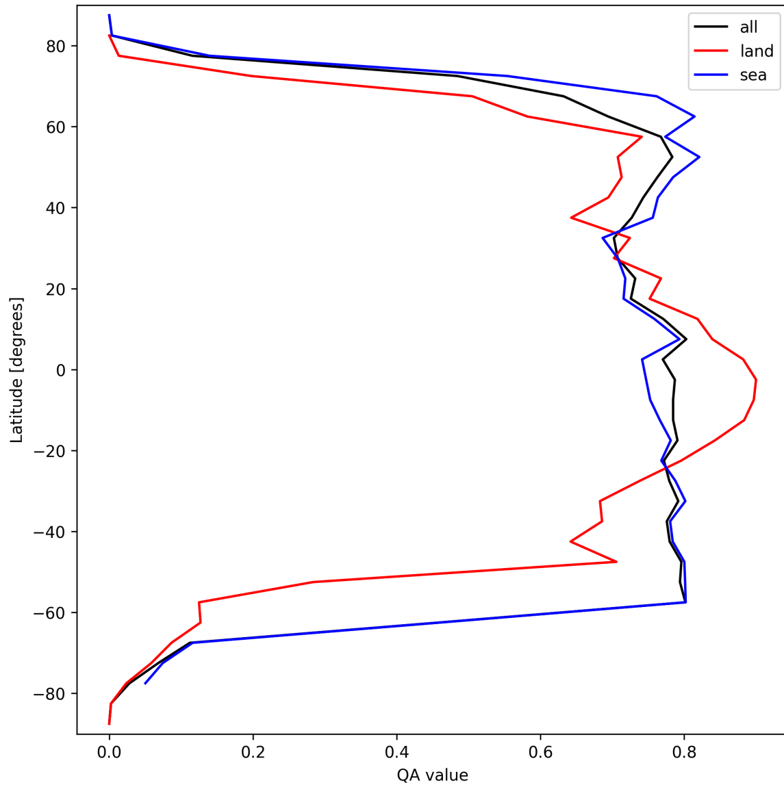
Figure 22: Zonal average of “QA value” for 2024-09-30 to 2024-10-02.
