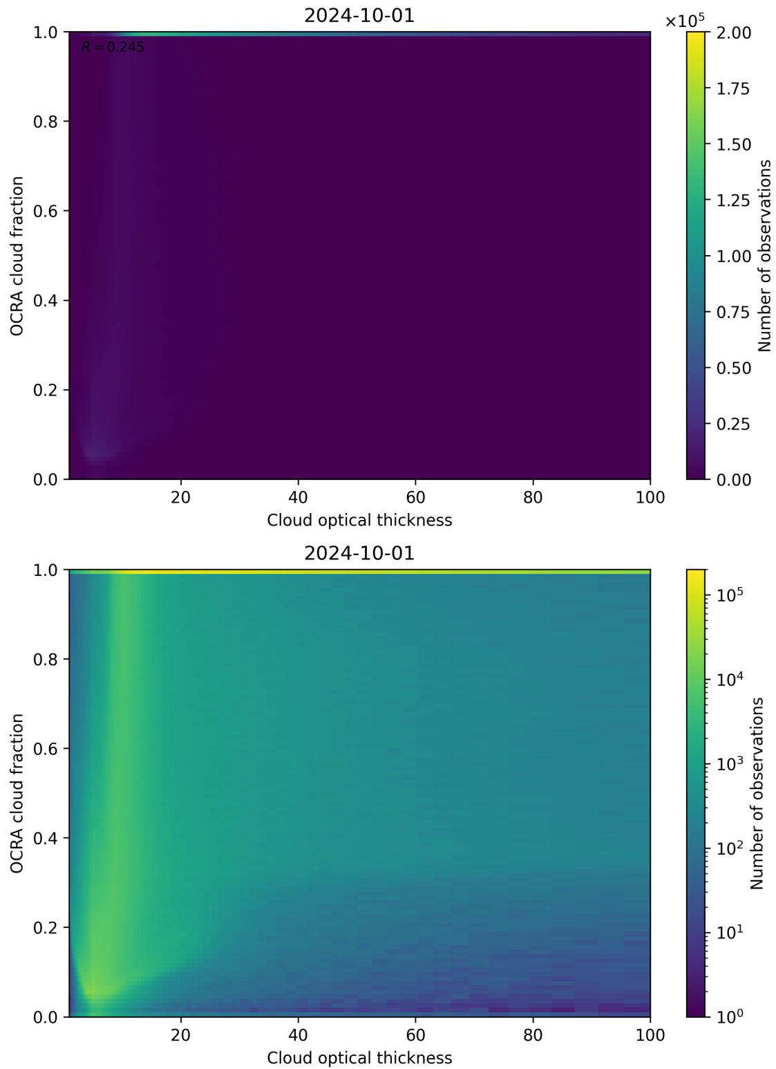
Figure 83: Scatter density plot of “Cloud optical thickness” against “OCRA cloud fraction” for 2024-09-30 to 2024-10-02.
