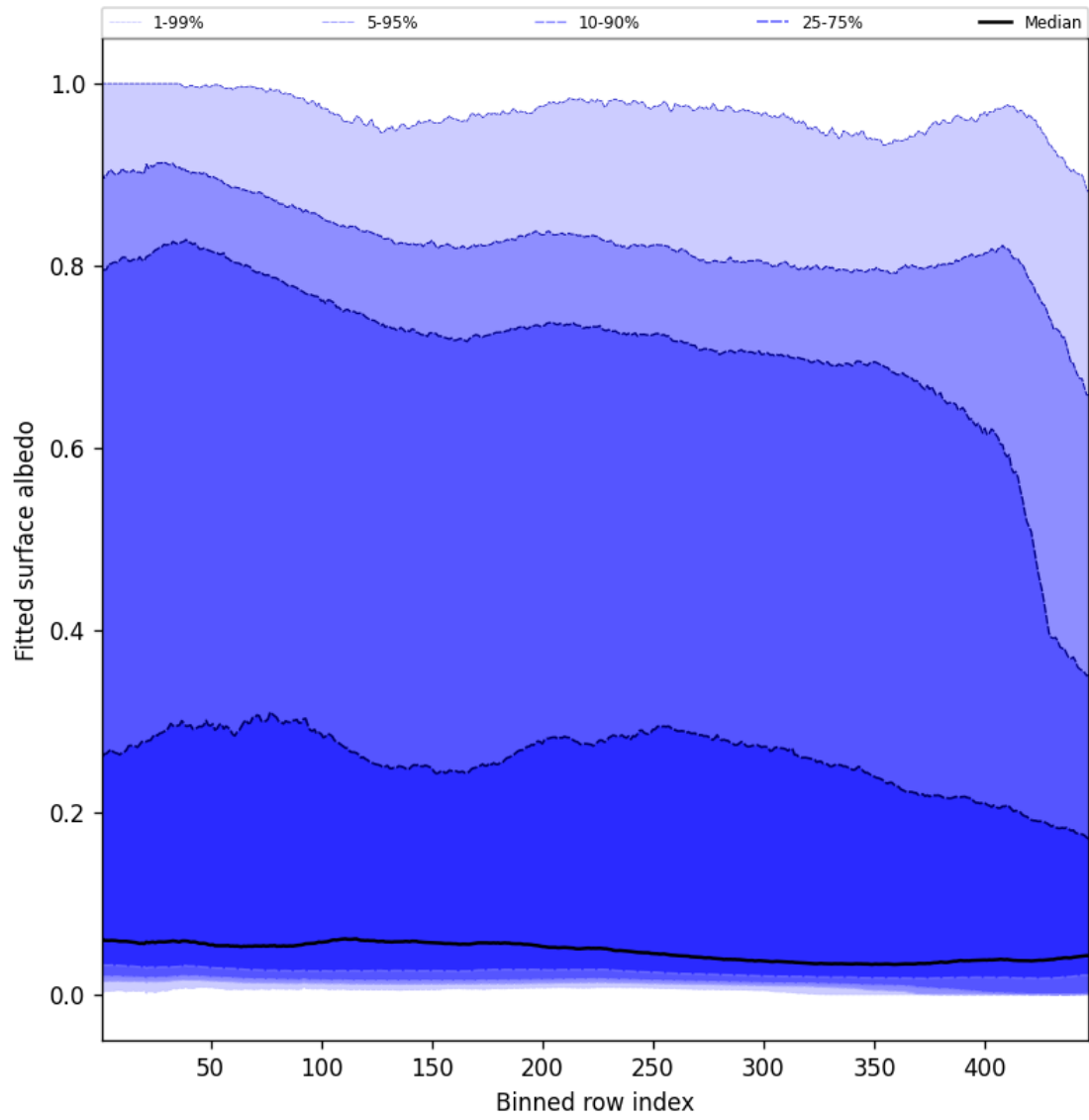
Figure 61: Along track statistics of “Fitted surface albedo” for 2024-09-30 to 2024-10-02
