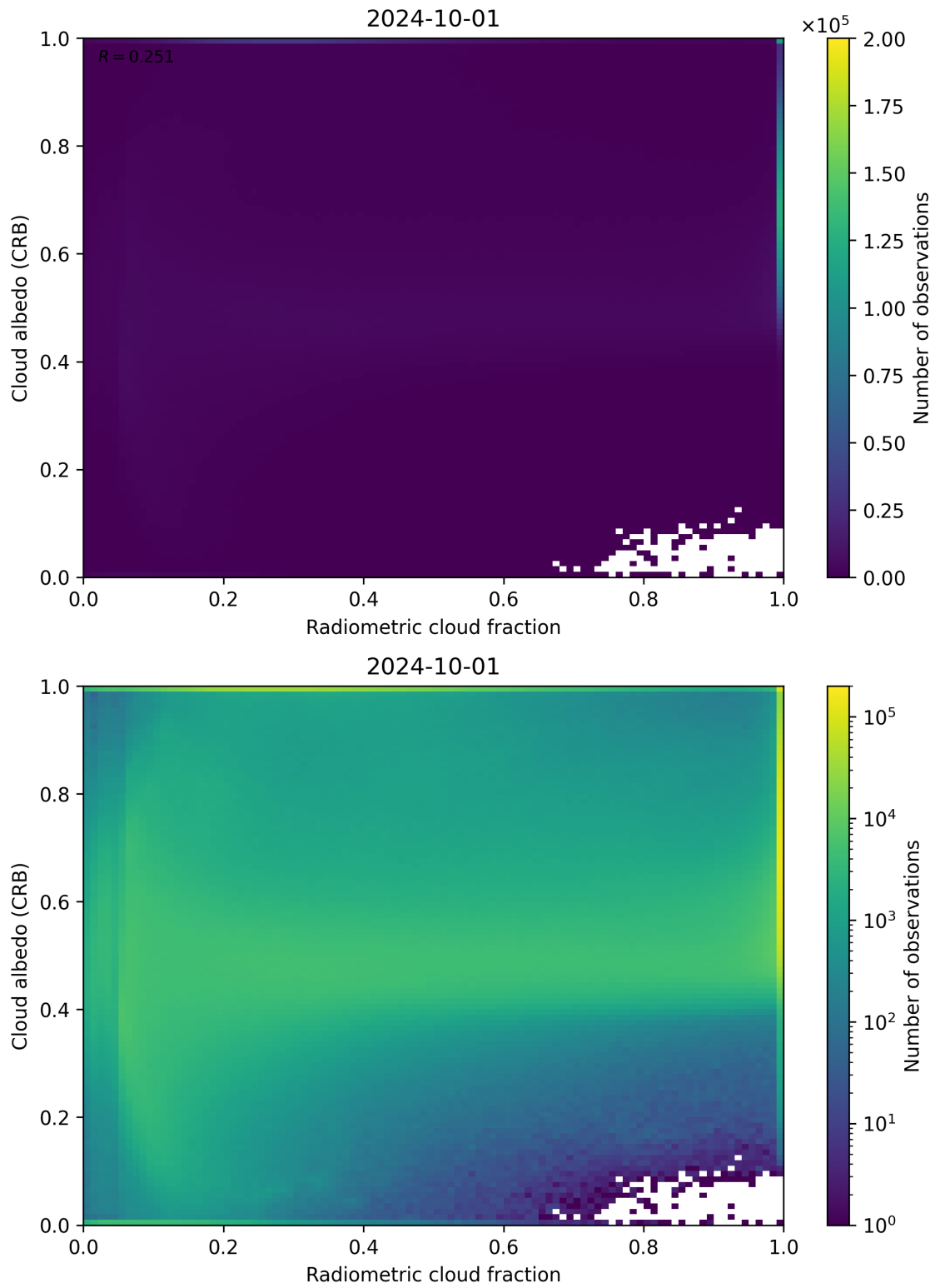
Figure 71: Scatter density plot of “Radiometric cloud fraction” against “Cloud albedo (CRB)” for 2024-09-30 to 2024-10-02.
