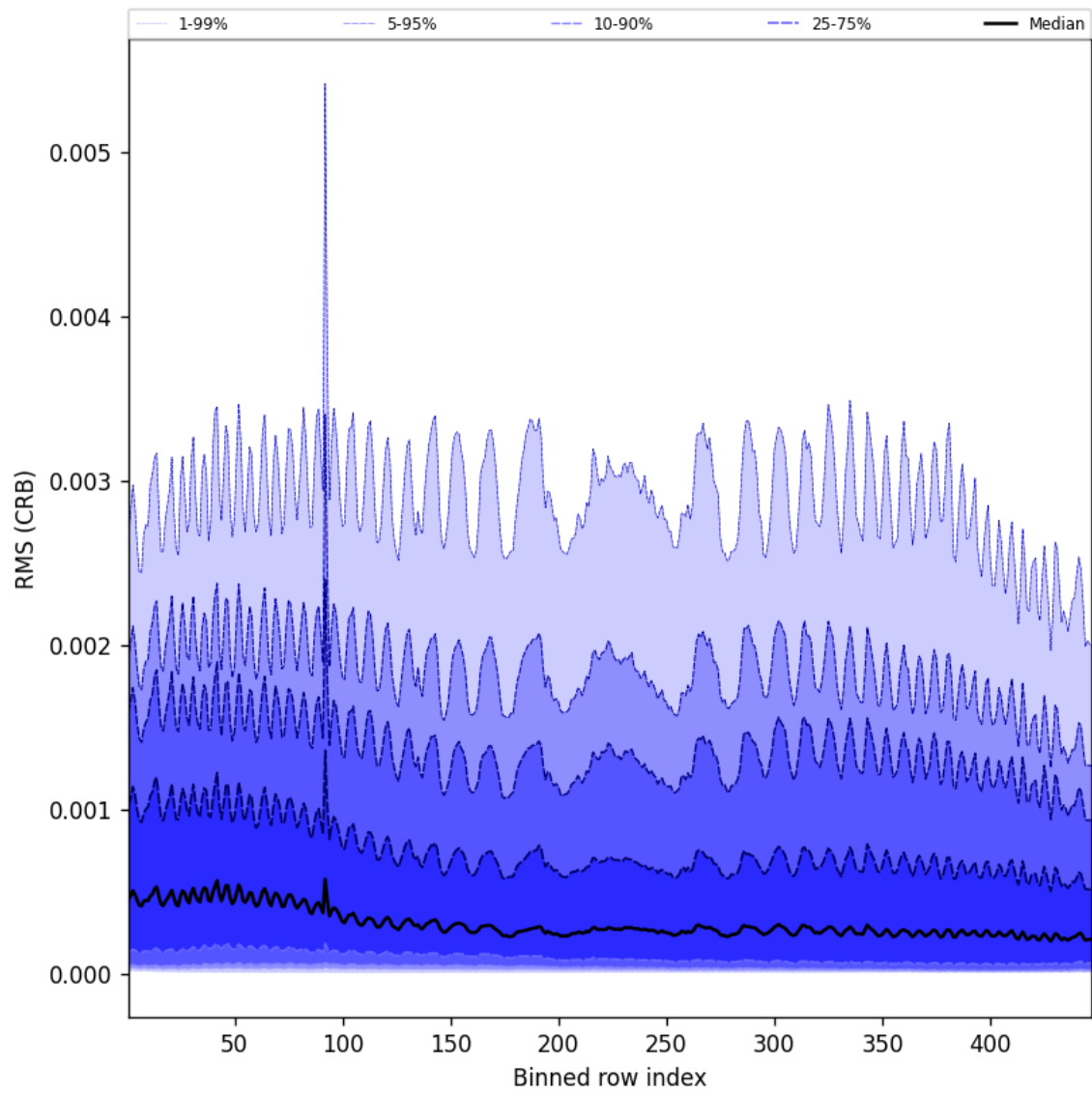
Figure 64: Along track statistics of “RMS (CRB)” for 2024-09-30 to 2024-10-02
