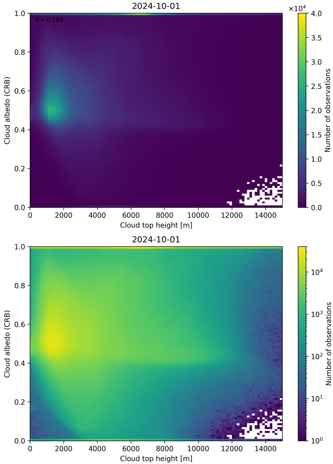
Figure 86: Scatter density plot of “Cloud top height” against “Cloud albedo (CRB)” for 2024-09-30 to 2024-10-02.
