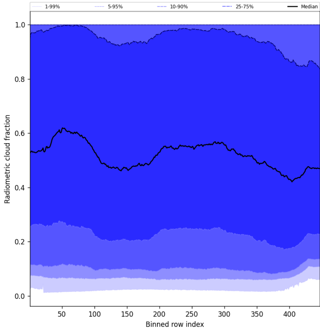
Figure 55: Along track statistics of “Radiometric cloud fraction” for 2024-09-30 to 2024-10-02
