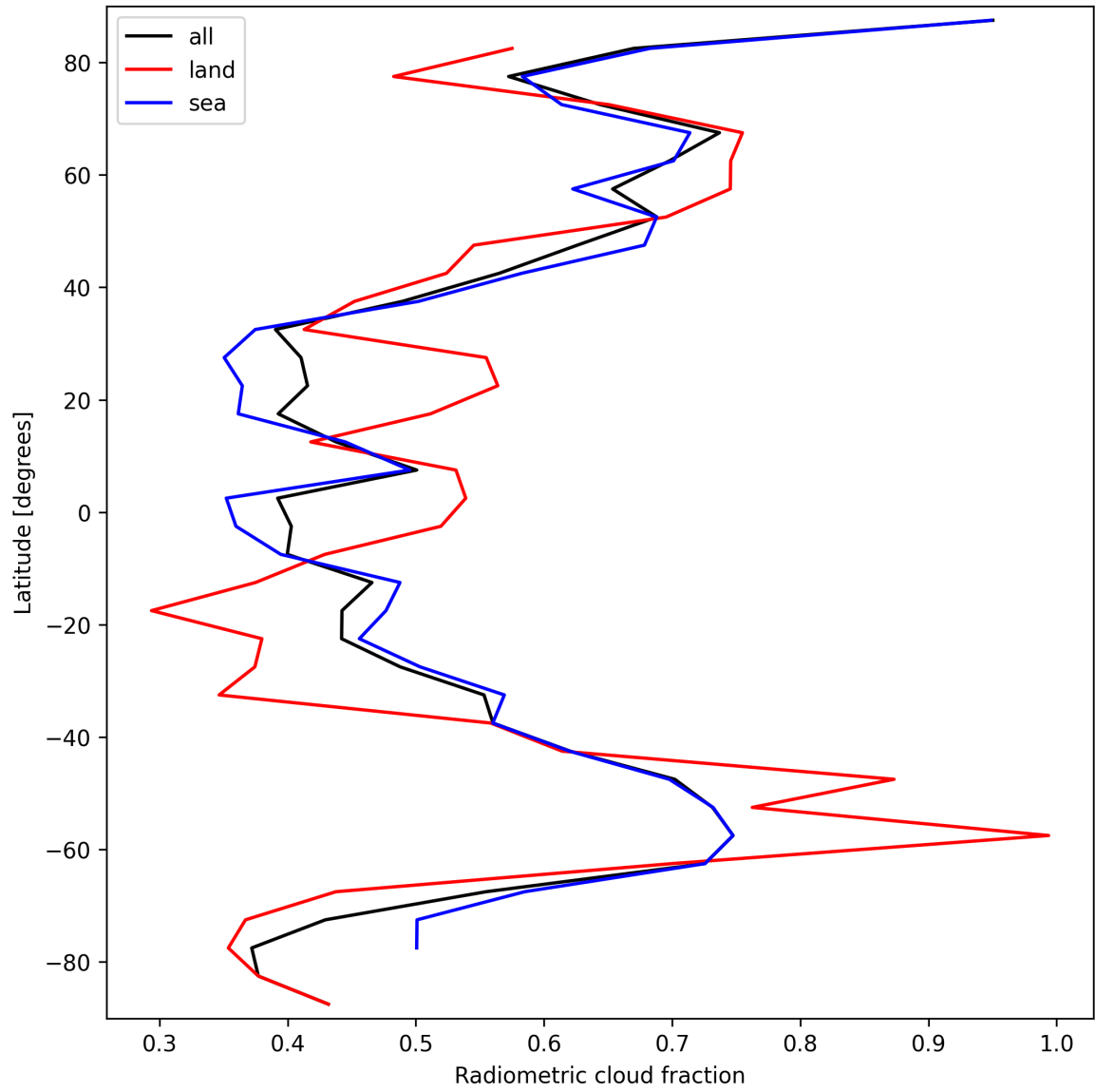
Figure 23: Zonal average of “Radiometric cloud fraction” for 2024-09-30 to 2024-10-02.
