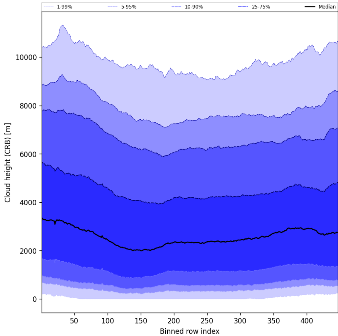
Figure 59: Along track statistics of “Cloud height (CRB)” for 2024-09-30 to 2024-10-02
