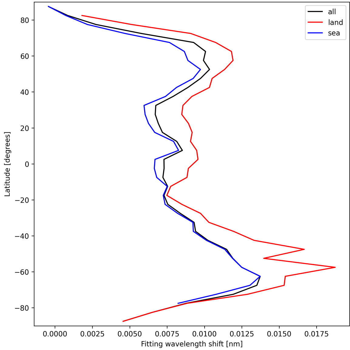
Figure 33: Zonal average of “Fitting wavelength shift” for 2024-09-30 to 2024-10-02.
