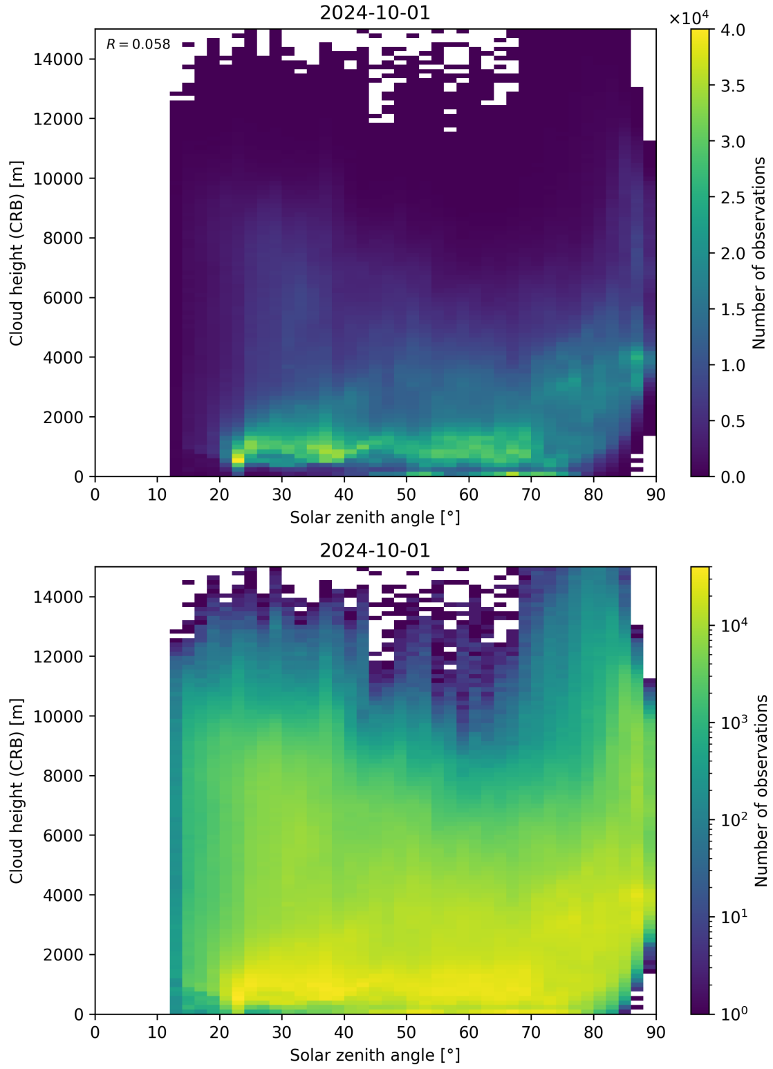
Figure 102: Scatter density plot of “Solar zenith angle” against “Cloud height (CRB)” for 2024-09-30 to 2024-10-02.
