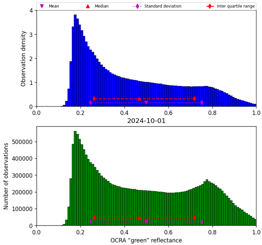
Figure 52: Histogram of “OCRA “green” reflectance” for 2024-09-30 to 2024-10-02
