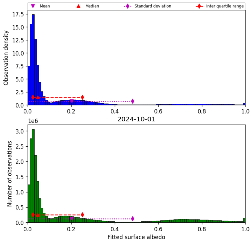
Figure 45: Histogram of “Fitted surface albedo” for 2024-09-30 to 2024-10-02
