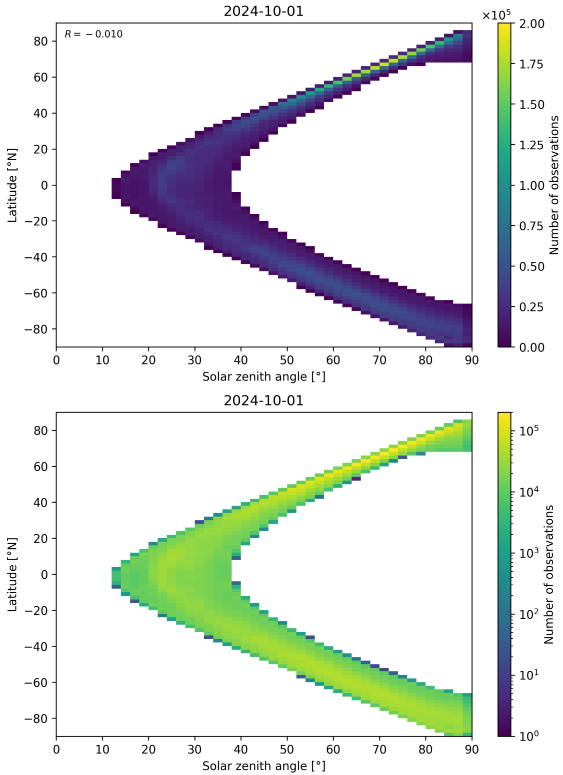
Figure 105: Scatter density plot of “Solar zenith angle” against “Latitude” for 2024-09-30 to 2024-10-02.
