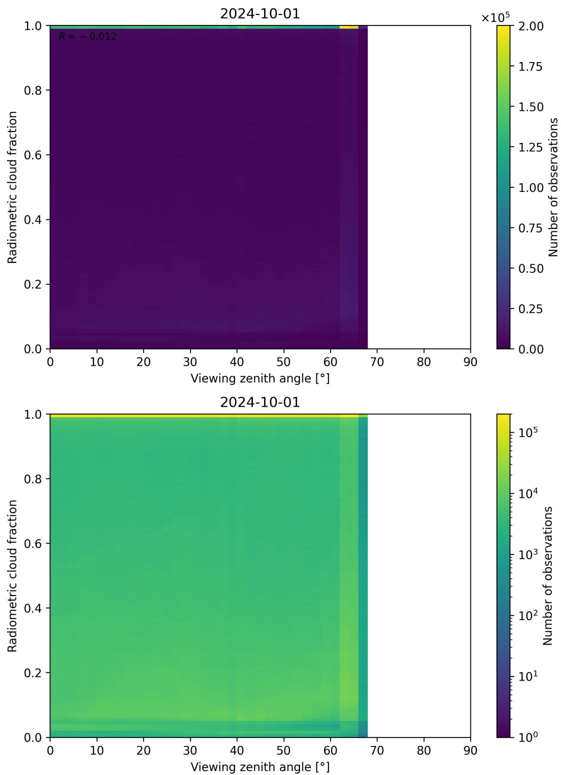
Figure 107: Scatter density plot of “Viewing zenith angle” against “Radiometric cloud fraction” for 2024-09-30 to 2024-10-02.
