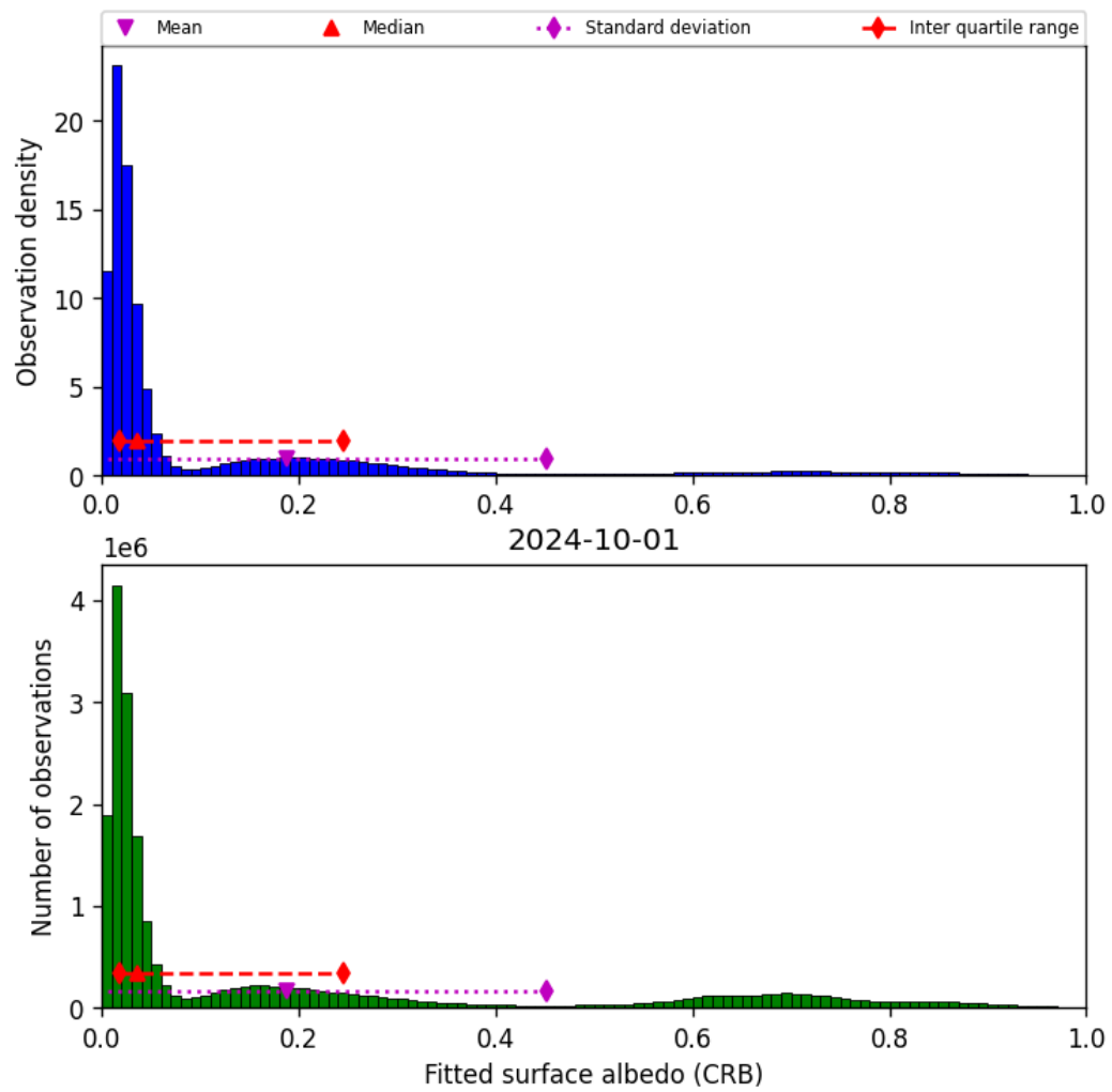
Figure 46: Histogram of “Fitted surface albedo (CRB)” for 2024-09-30 to 2024-10-02
