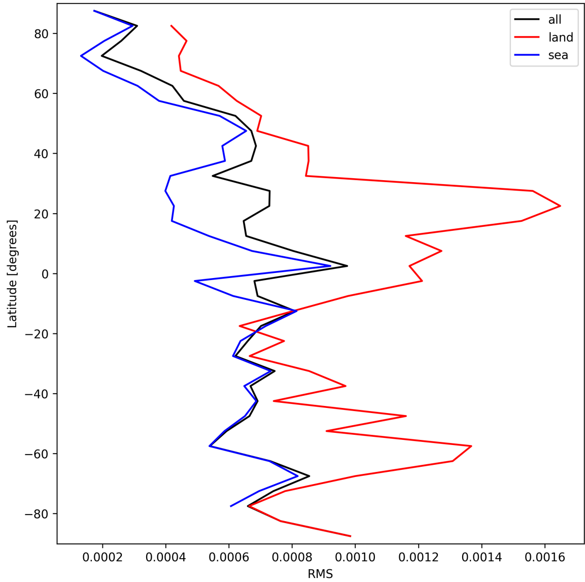
Figure 31: Zonal average of “RMS” for 2024-09-30 to 2024-10-02.
