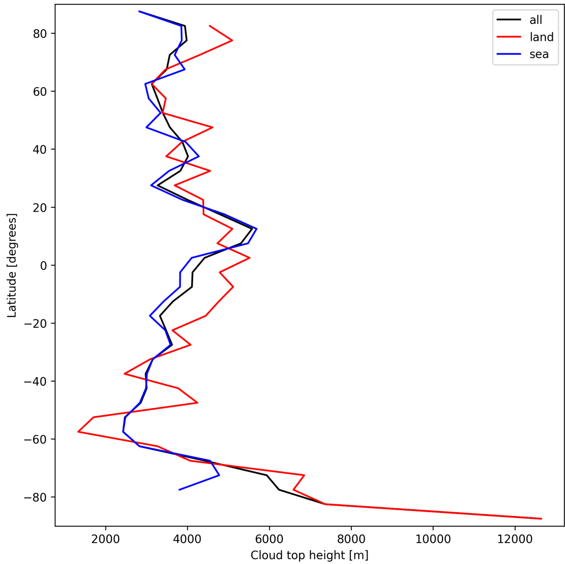
Figure 24: Zonal average of “Cloud top height” for 2024-09-30 to 2024-10-02.
