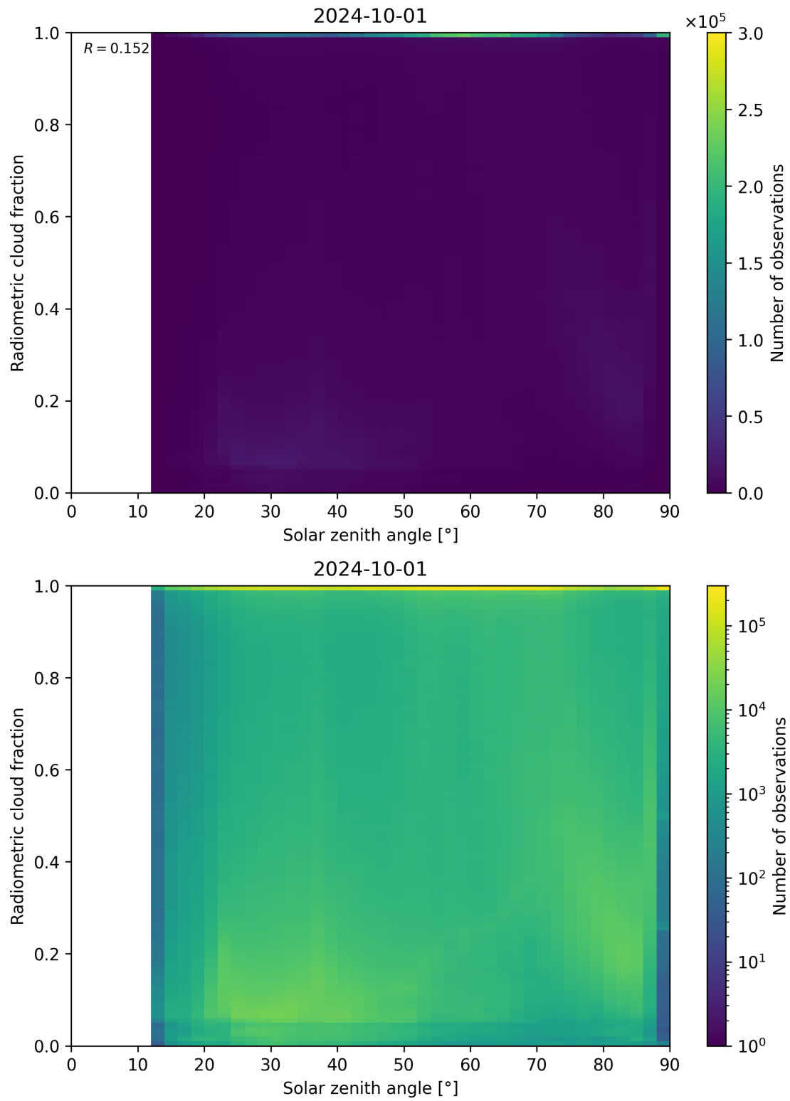
Figure 99: Scatter density plot of “Solar zenith angle” against “Radiometric cloud fraction” for 2024-09-30 to 2024-10-02.
