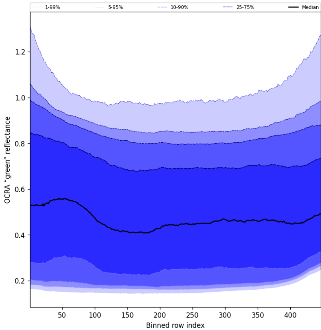
Figure 68: Along track statistics of "OCRA "green" reflectance" for 2024-09-30 to 2024-10-02
