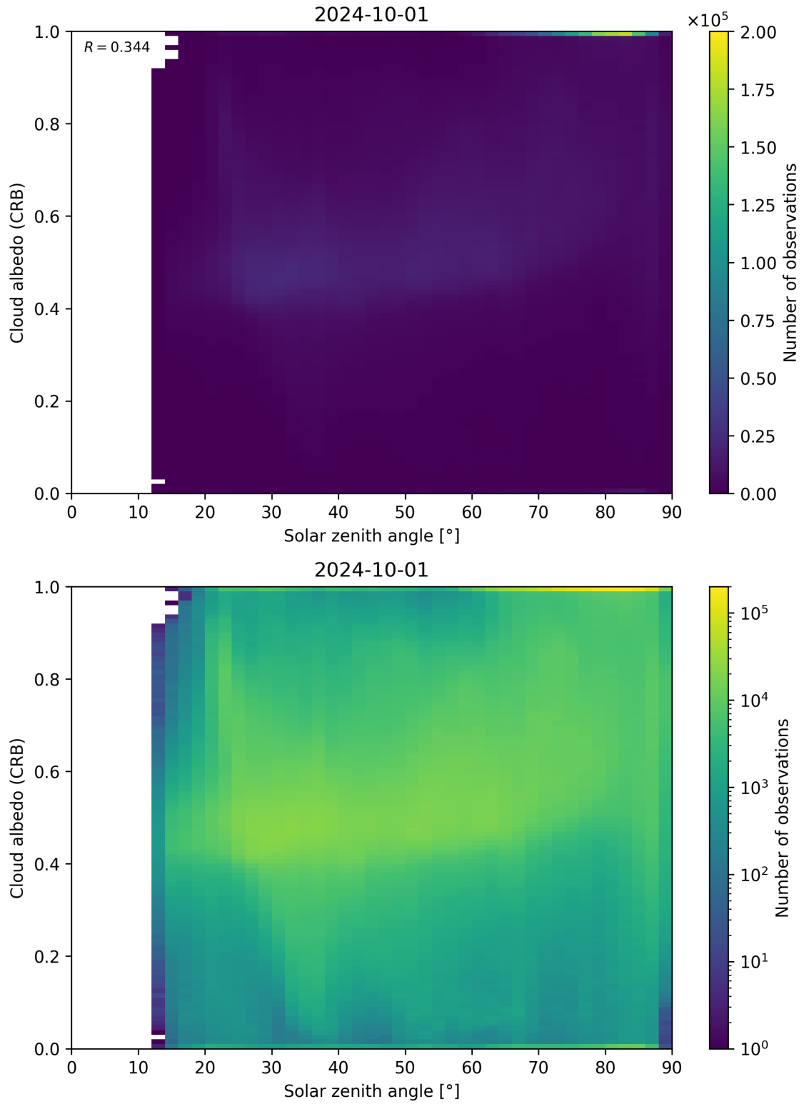
Figure 98: Scatter density plot of “Solar zenith angle” against “Cloud albedo (CRB)” for 2024-09-30 to 2024-10-02.
