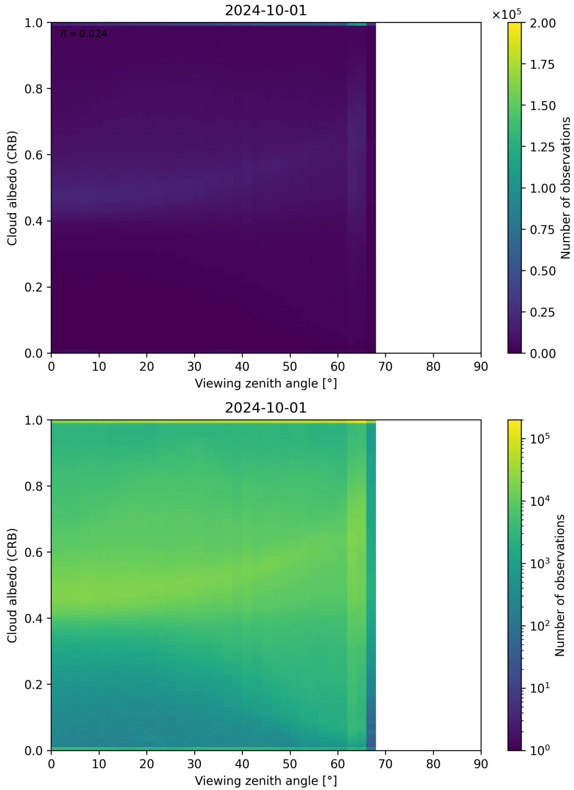
Figure 106: Scatter density plot of “Viewing zenith angle” against “Cloud albedo (CRB)” for 2024-09-30 to 2024-10-02.
