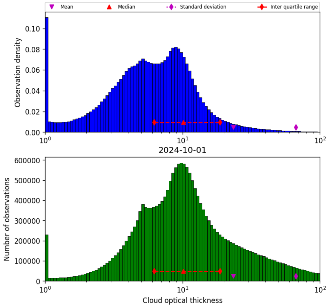
Figure 41: Histogram of “Cloud optical thickness” for 2024-09-30 to 2024-10-02
