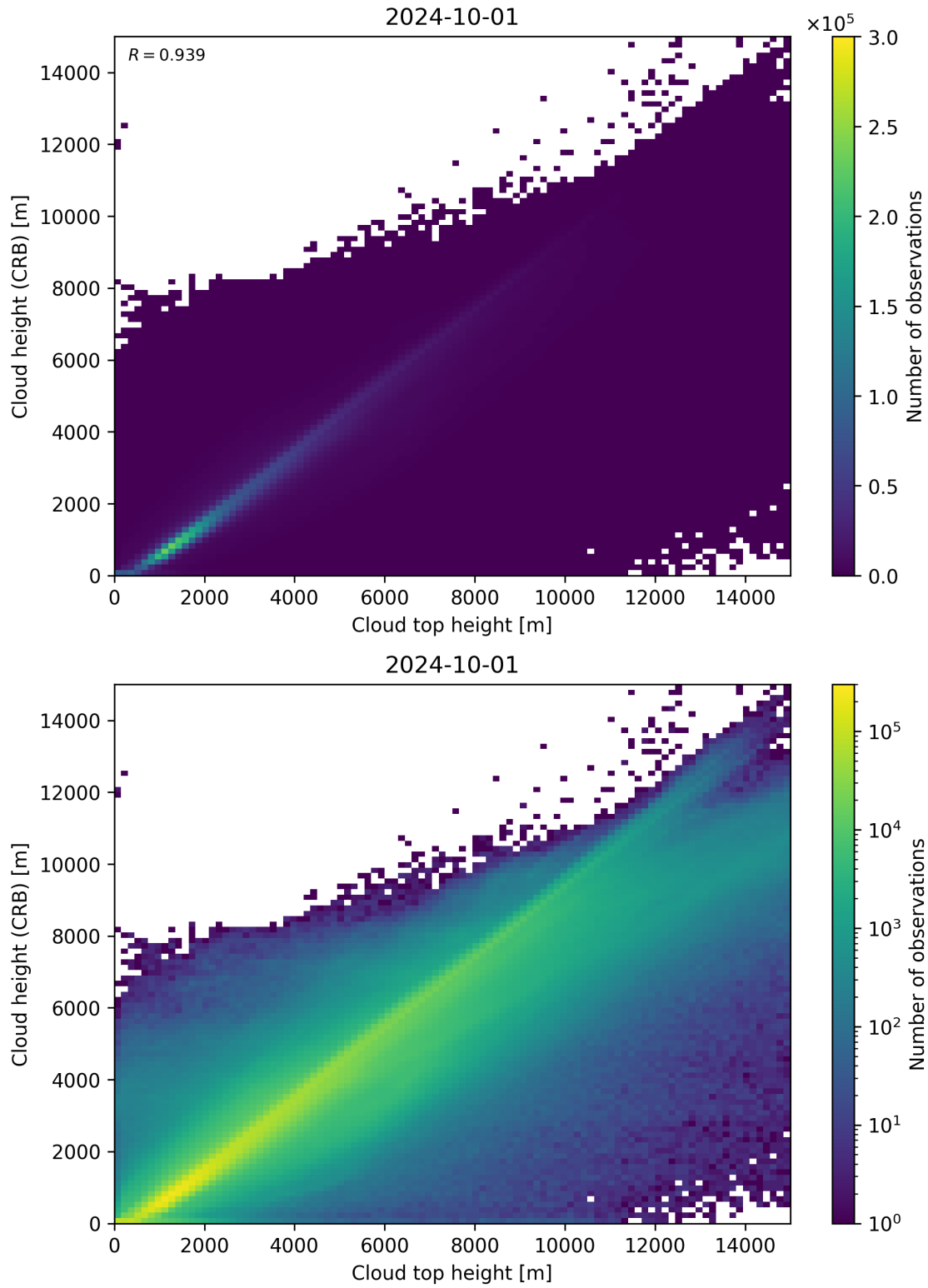
Figure 89: Scatter density plot of “Cloud top height” against “Cloud height (CRB)” for 2024-09-30 to 2024-10-02.
