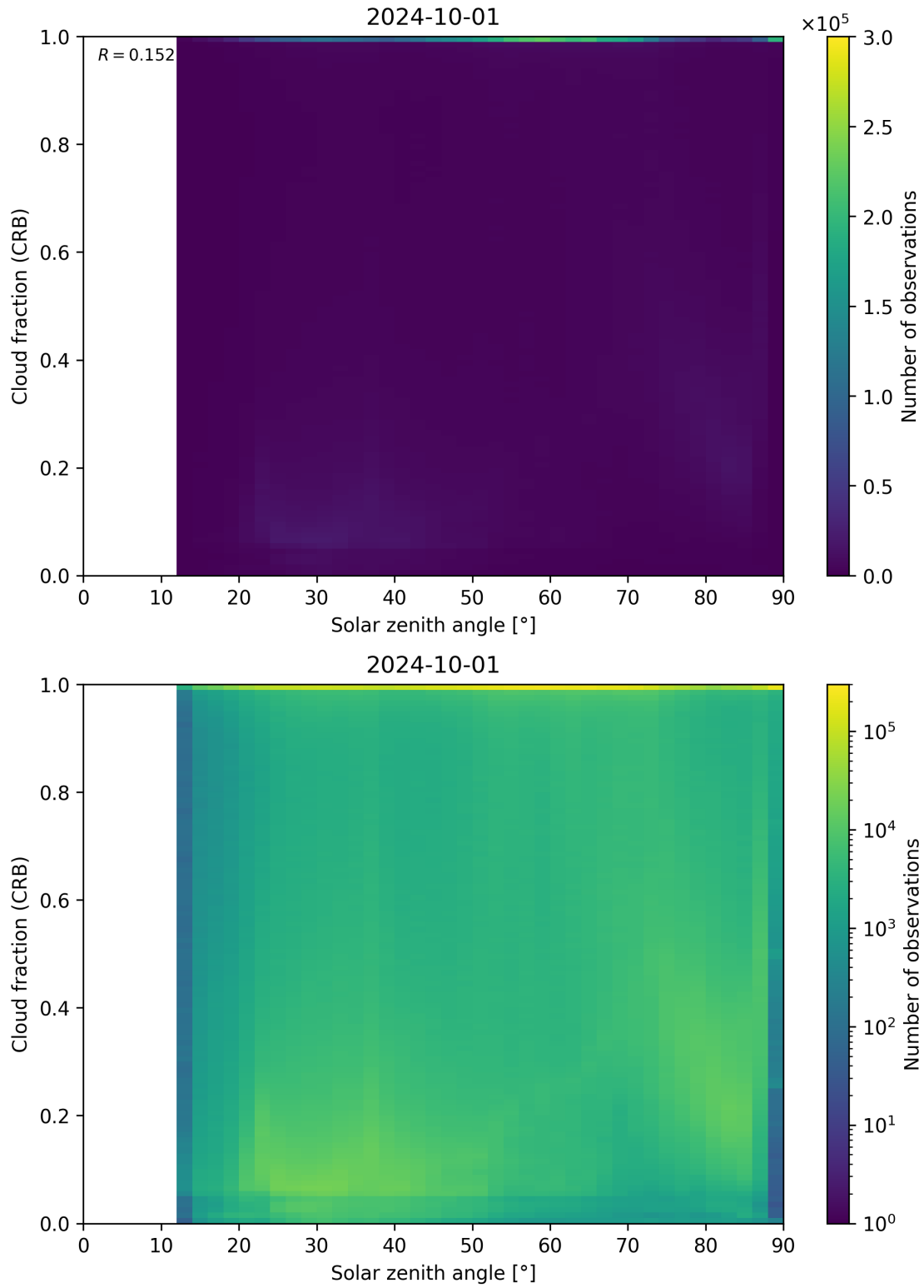
Figure 101: Scatter density plot of “Solar zenith angle” against “Cloud fraction (CRB)” for 2024-09-30 to 2024-10-02.
