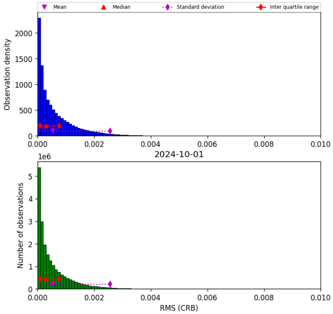
Figure 48: Histogram of “RMS (CRB)” for 2024-09-30 to 2024-10-02
