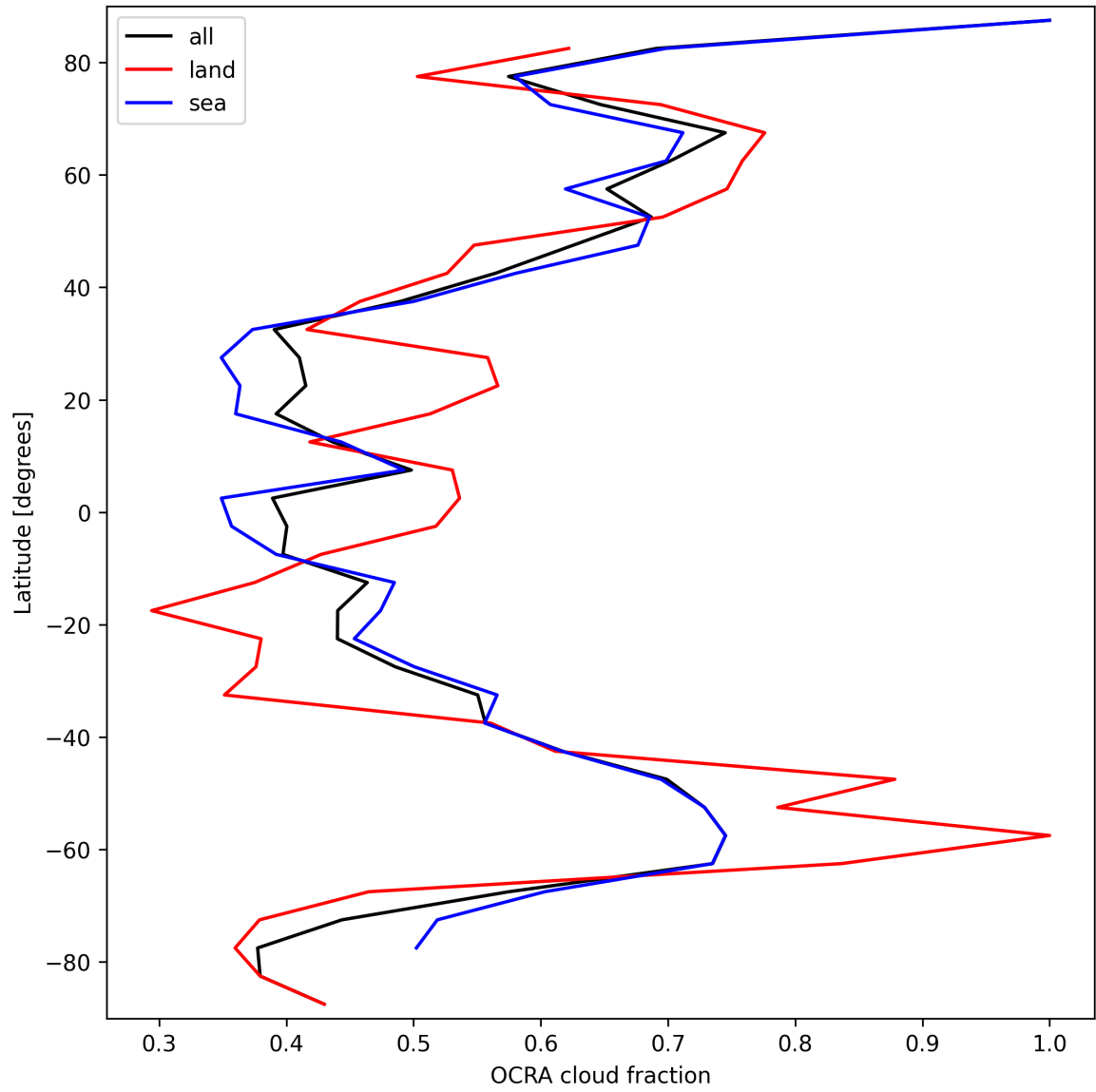
Figure 34: Zonal average of “OCRA cloud fraction” for 2024-09-30 to 2024-10-02.
