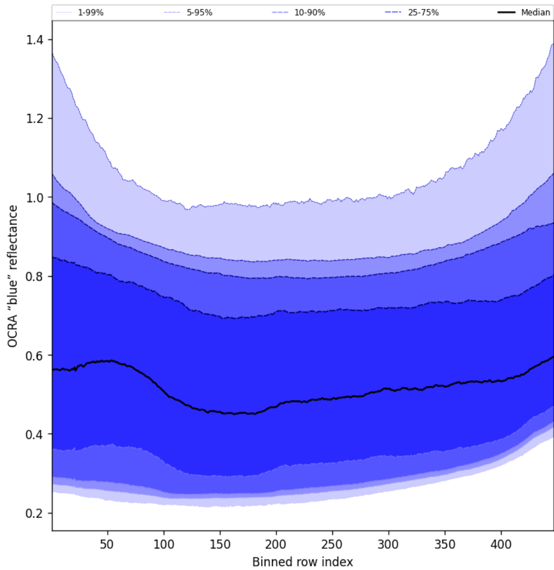
Figure 67: Along track statistics of "OCRA "blue" reflectance" for 2024-09-30 to 2024-10-02
