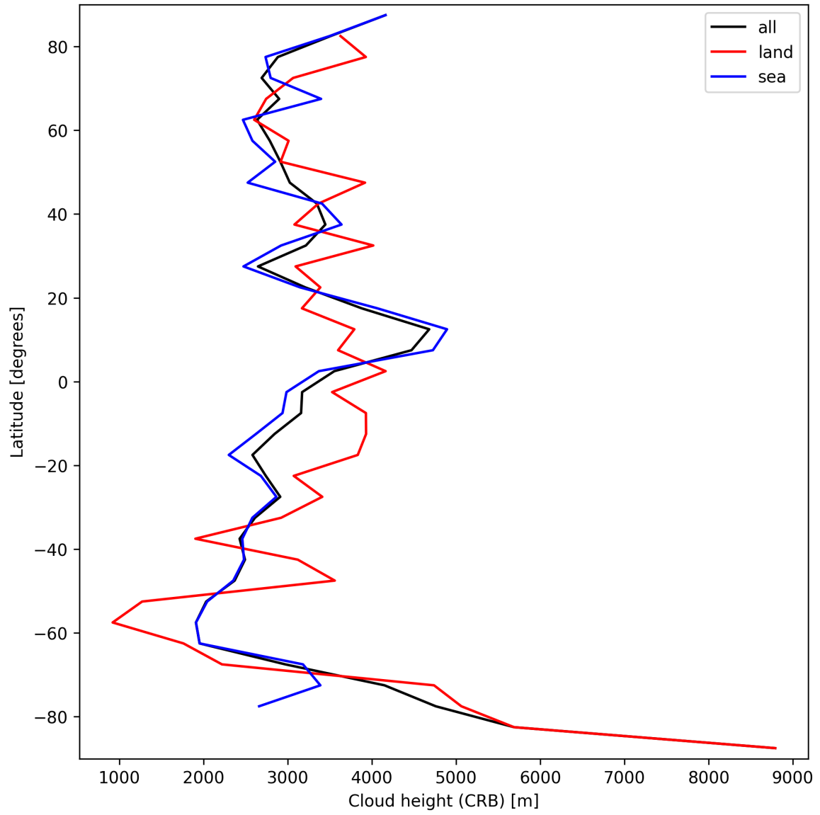
Figure 27: Zonal average of “Cloud height (CRB)” for 2024-09-30 to 2024-10-02.
