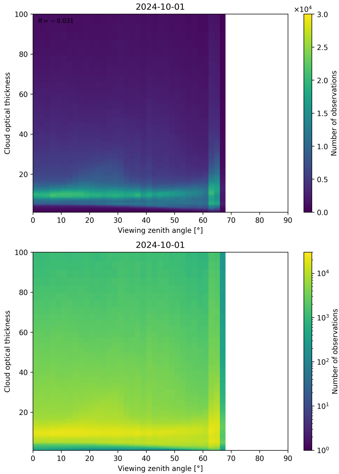
Figure 111: Scatter density plot of “Viewing zenith angle” against “Cloud optical thickness” for 2024-09-30 to 2024-10-02.
