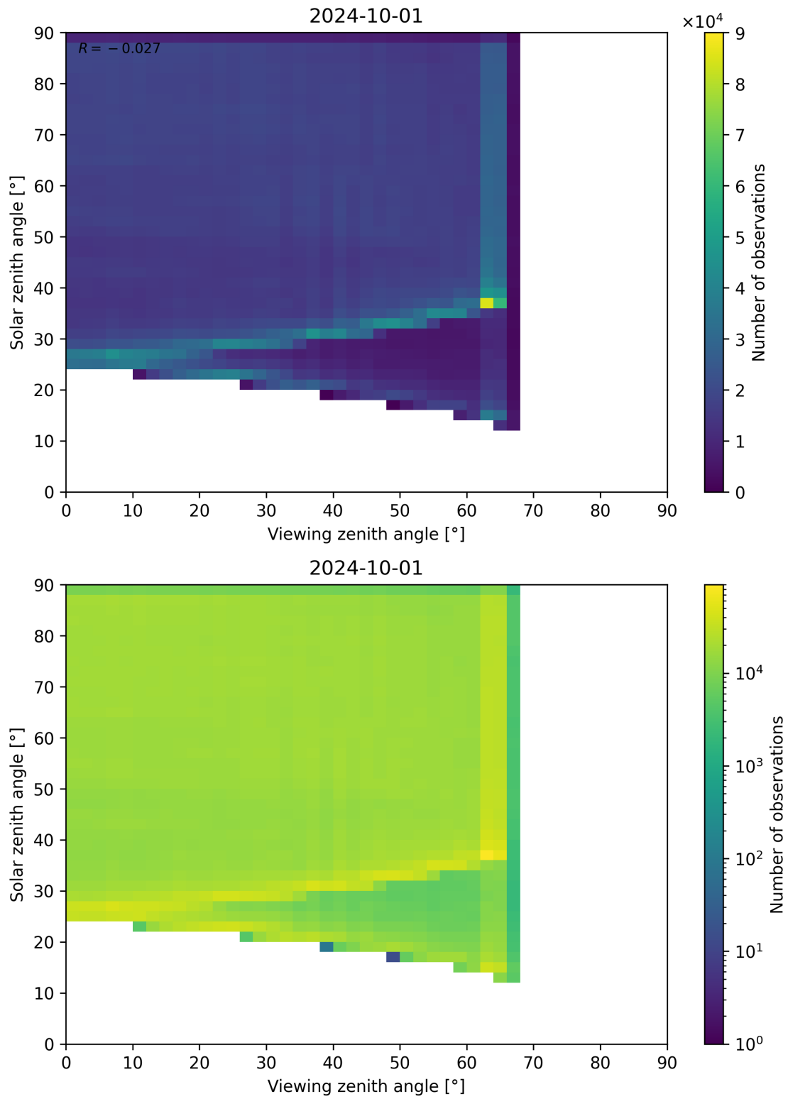
Figure 114: Scatter density plot of “Viewing zenith angle” against “Solar zenith angle” for 2024-09-30 to 2024-10-02.
