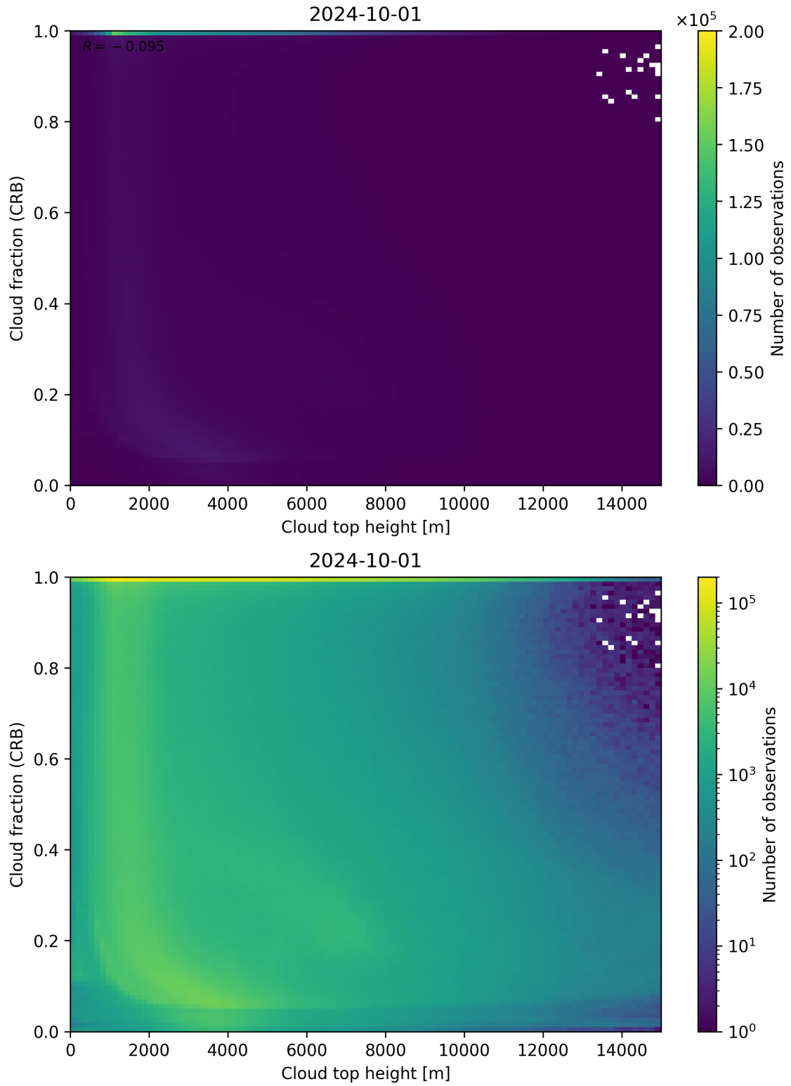
Figure 88: Scatter density plot of “Cloud top height” against “Cloud fraction (CRB)” for 2024-09-30 to 2024-10-02.
