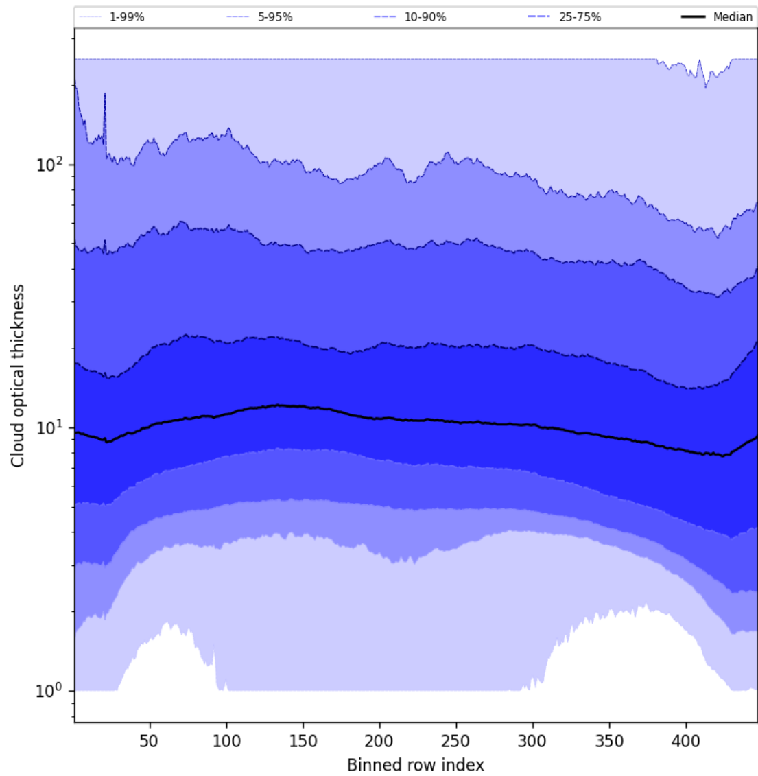
Figure 57: Along track statistics of “Cloud optical thickness” for 2024-09-30 to 2024-10-02
