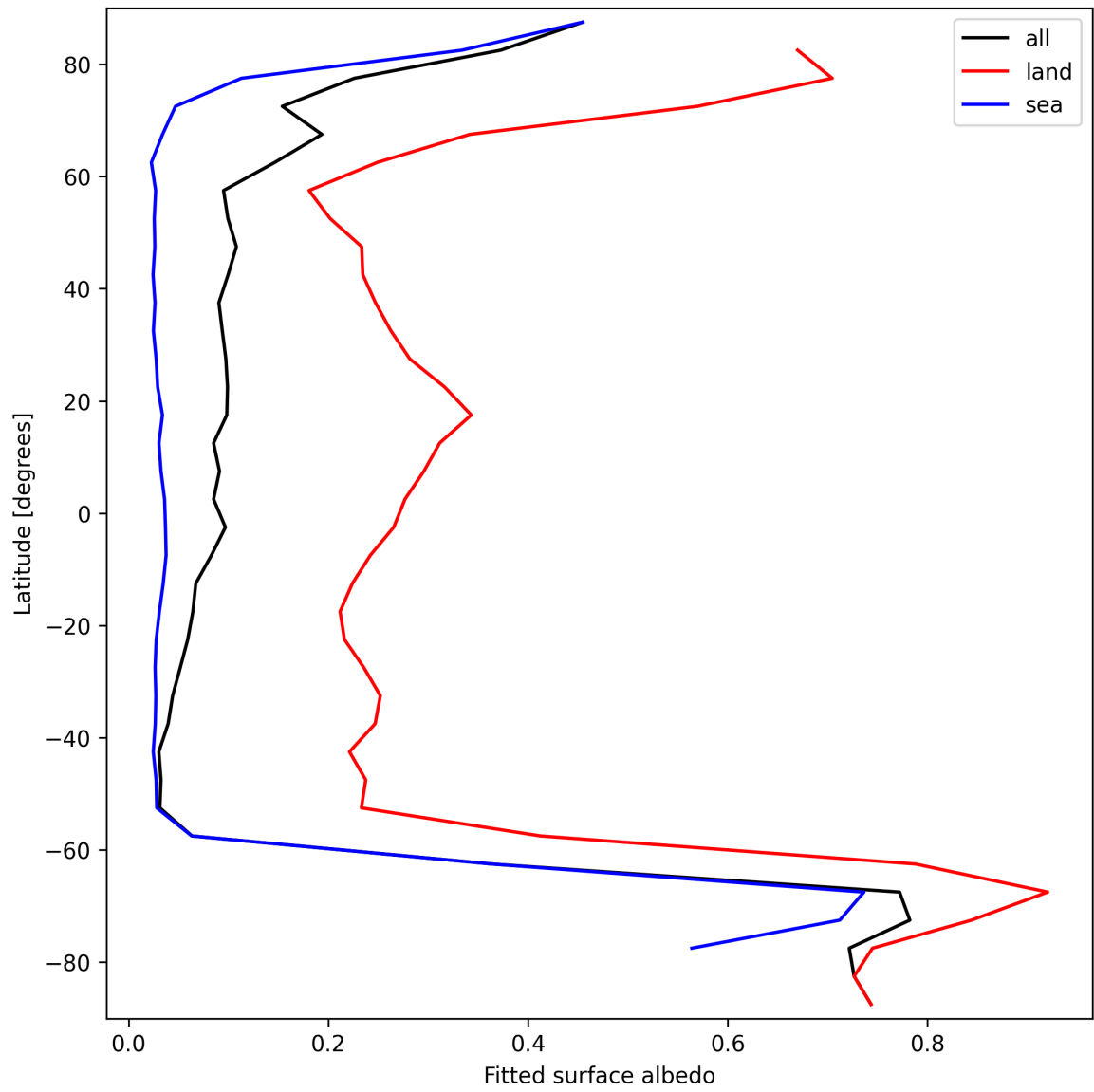
Figure 29: Zonal average of “Fitted surface albedo” for 2024-09-30 to 2024-10-02.
