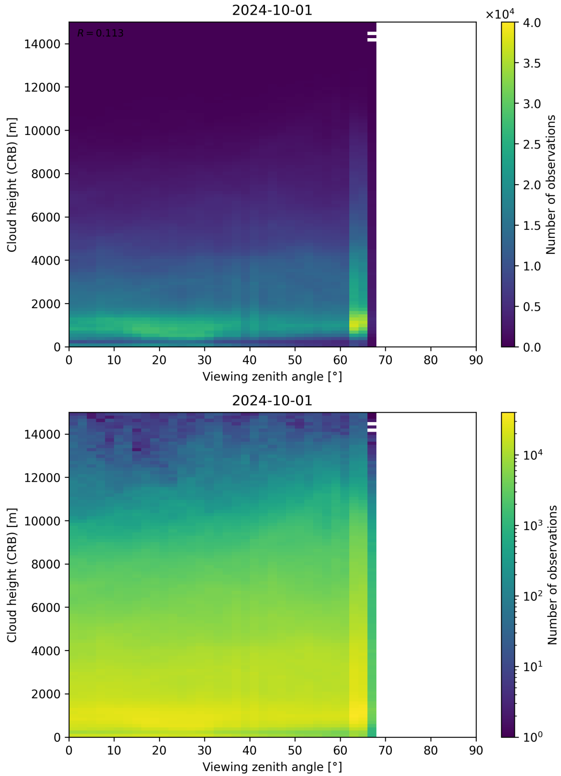
Figure 110: Scatter density plot of “Viewing zenith angle” against “Cloud height (CRB)” for 2024-09-30 to 2024-10-02.
