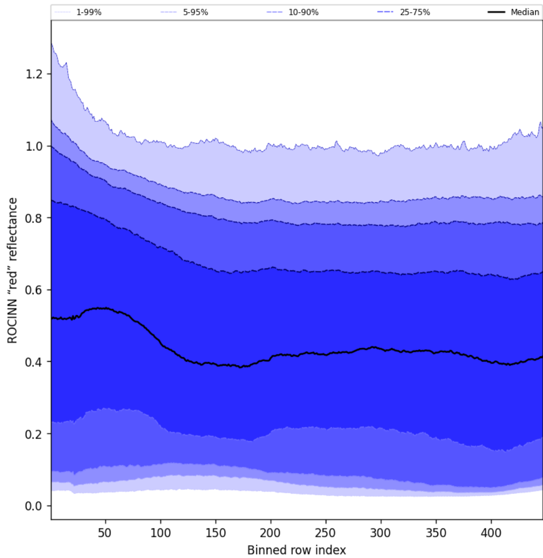
Figure 69: Along track statistics of “ROCINN “red” reflectance” for 2024-09-30 to 2024-10-02
