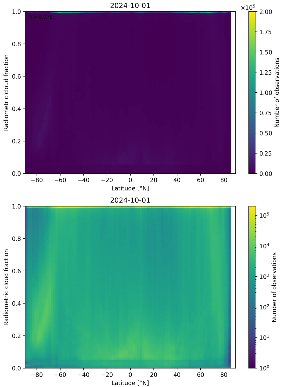
Figure 92: Scatter density plot of “Latitude” against “Radiometric cloud fraction” for 2024-09-30 to 2024-10-02.
