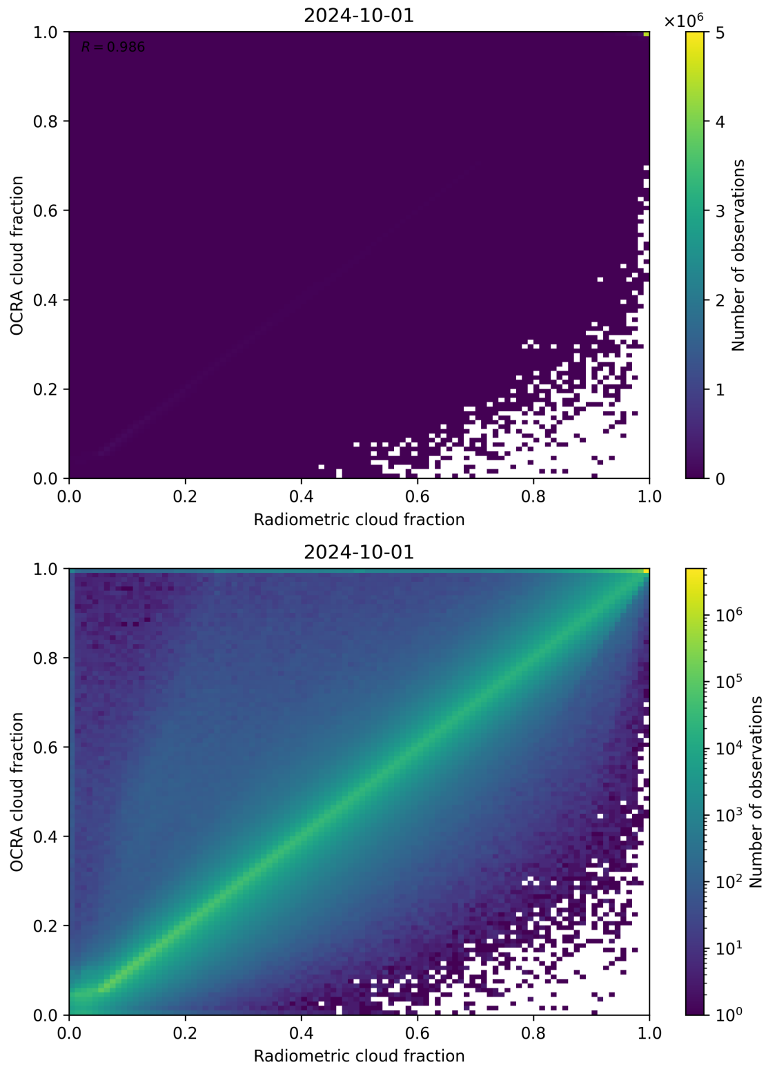
Figure 72: Scatter density plot of “Radiometric cloud fraction” against “OCRA cloud fraction” for 2024-09-30 to 2024-10-02.
