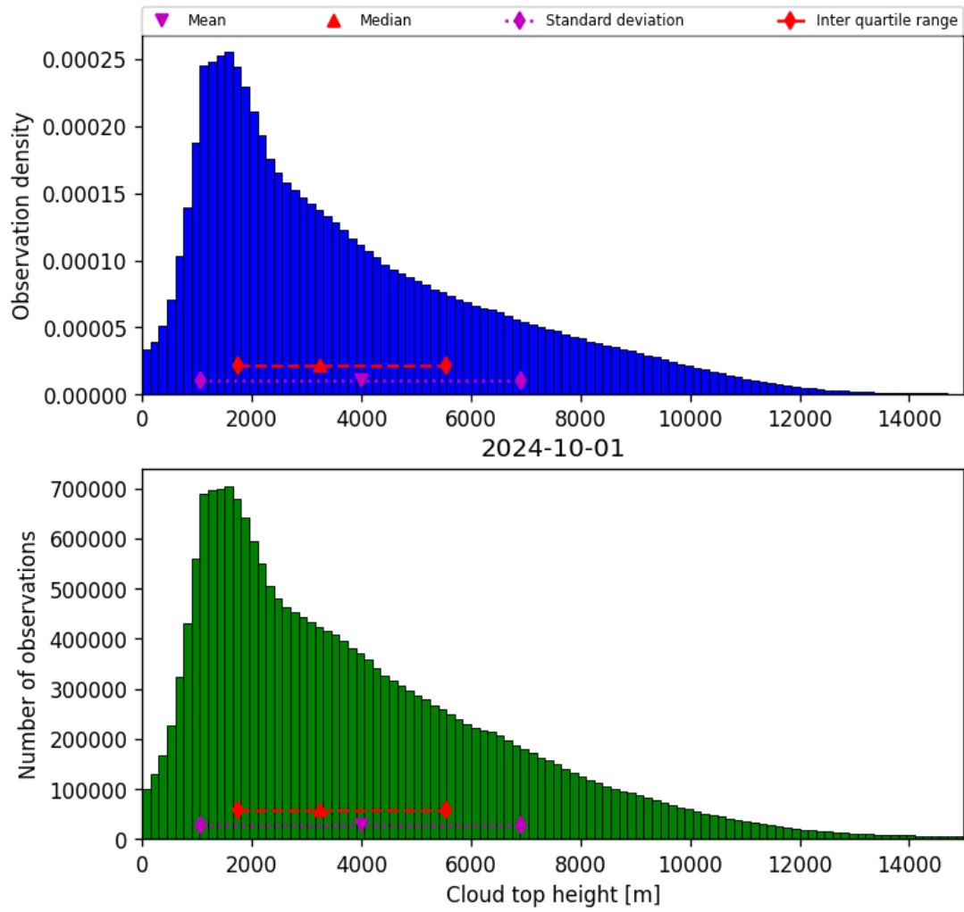
Figure 40: Histogram of “Cloud top height” for 2024-09-30 to 2024-10-02
