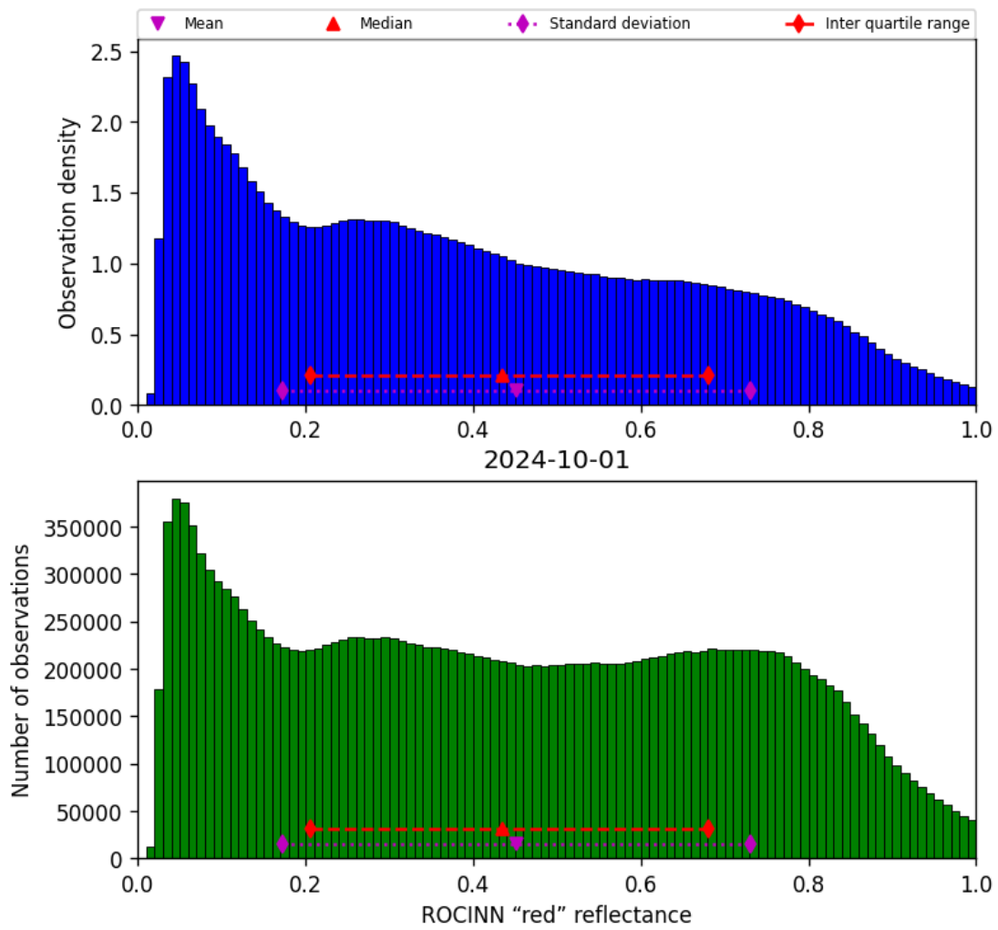
Figure 53: Histogram of “ROCINN “red” reflectance” for 2024-09-30 to 2024-10-02
