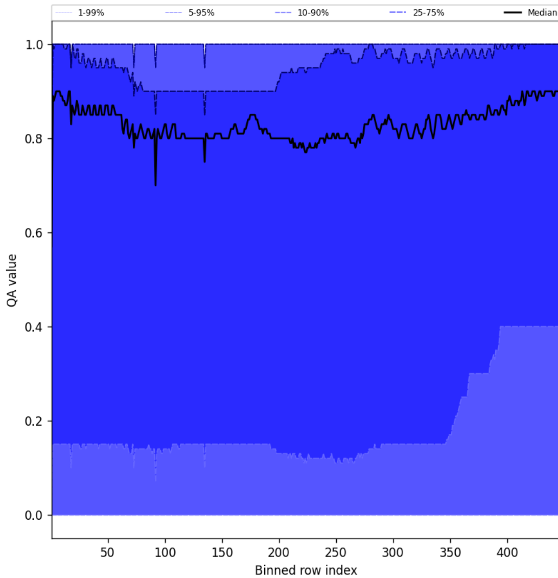
Figure 54: Along track statistics of “QA value” for 2024-09-30 to 2024-10-02
