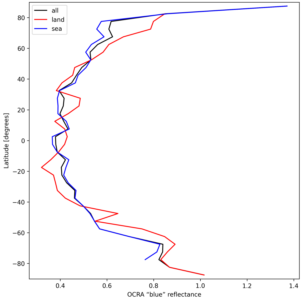
Figure 35: Zonal average of "OCRA "blue" reflectance" for 2024-09-30 to 2024-10-02.
