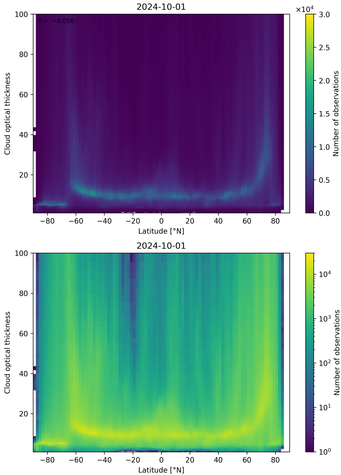
Figure 96: Scatter density plot of “Latitude” against “Cloud optical thickness” for 2024-09-30 to 2024-10-02.
