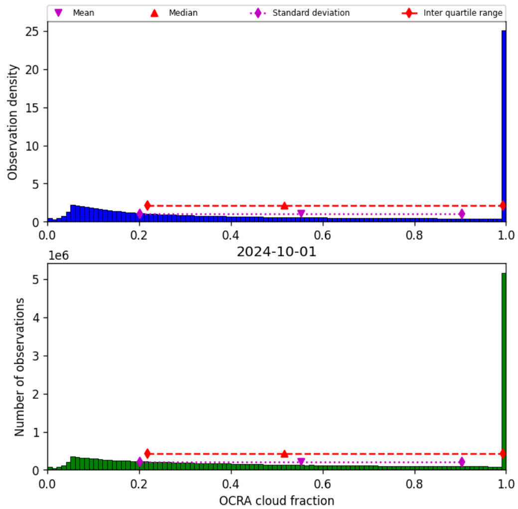
Figure 50: Histogram of “OCRA cloud fraction” for 2024-09-30 to 2024-10-02
