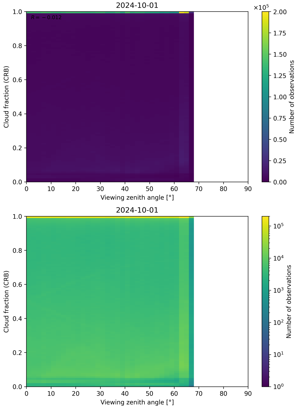
Figure 109: Scatter density plot of “Viewing zenith angle” against “Cloud fraction (CRB)” for 2024-09-30 to 2024-10-02.
