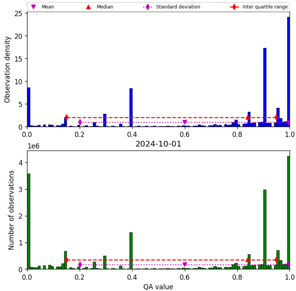
Figure 38: Histogram of “QA value” for 2024-09-30 to 2024-10-02
