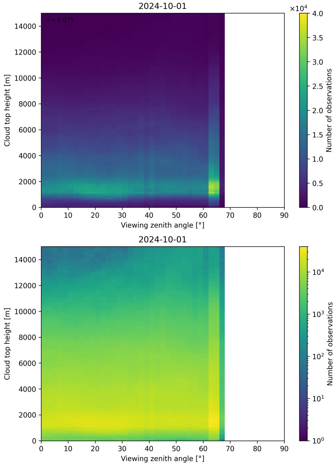
Figure 112: Scatter density plot of “Viewing zenith angle” against “Cloud top height” for 2024-09-30 to 2024-10-02.
