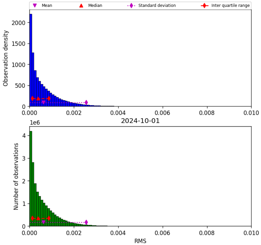
Figure 47: Histogram of “RMS” for 2024-09-30 to 2024-10-02
