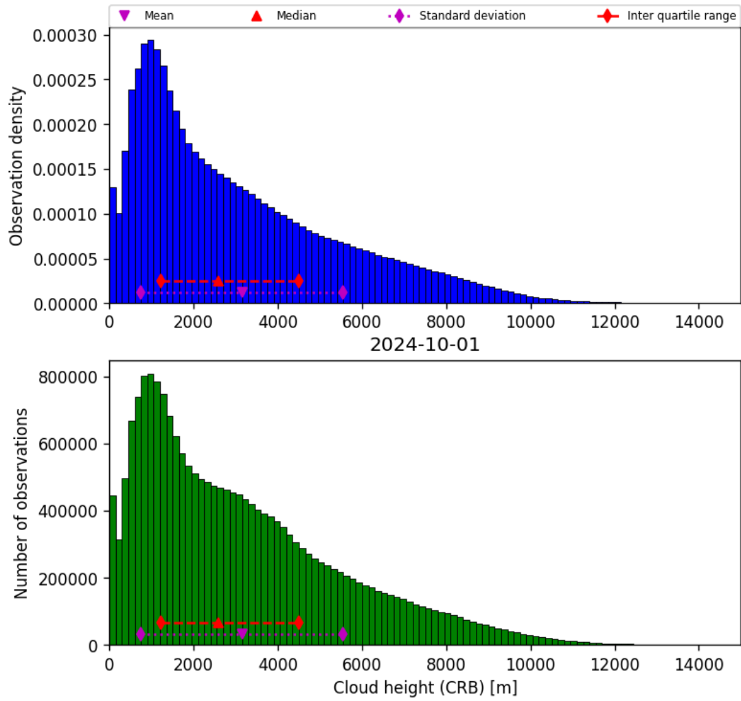
Figure 43: Histogram of “Cloud height (CRB)” for 2024-09-30 to 2024-10-02
