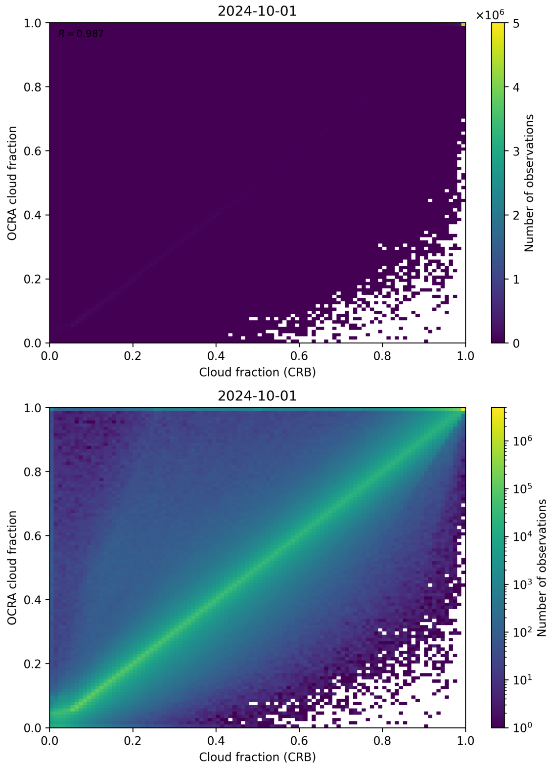
Figure 78: Scatter density plot of “Cloud fraction (CRB)” against “OCRA cloud fraction” for 2024-09-30 to 2024-10-02.
