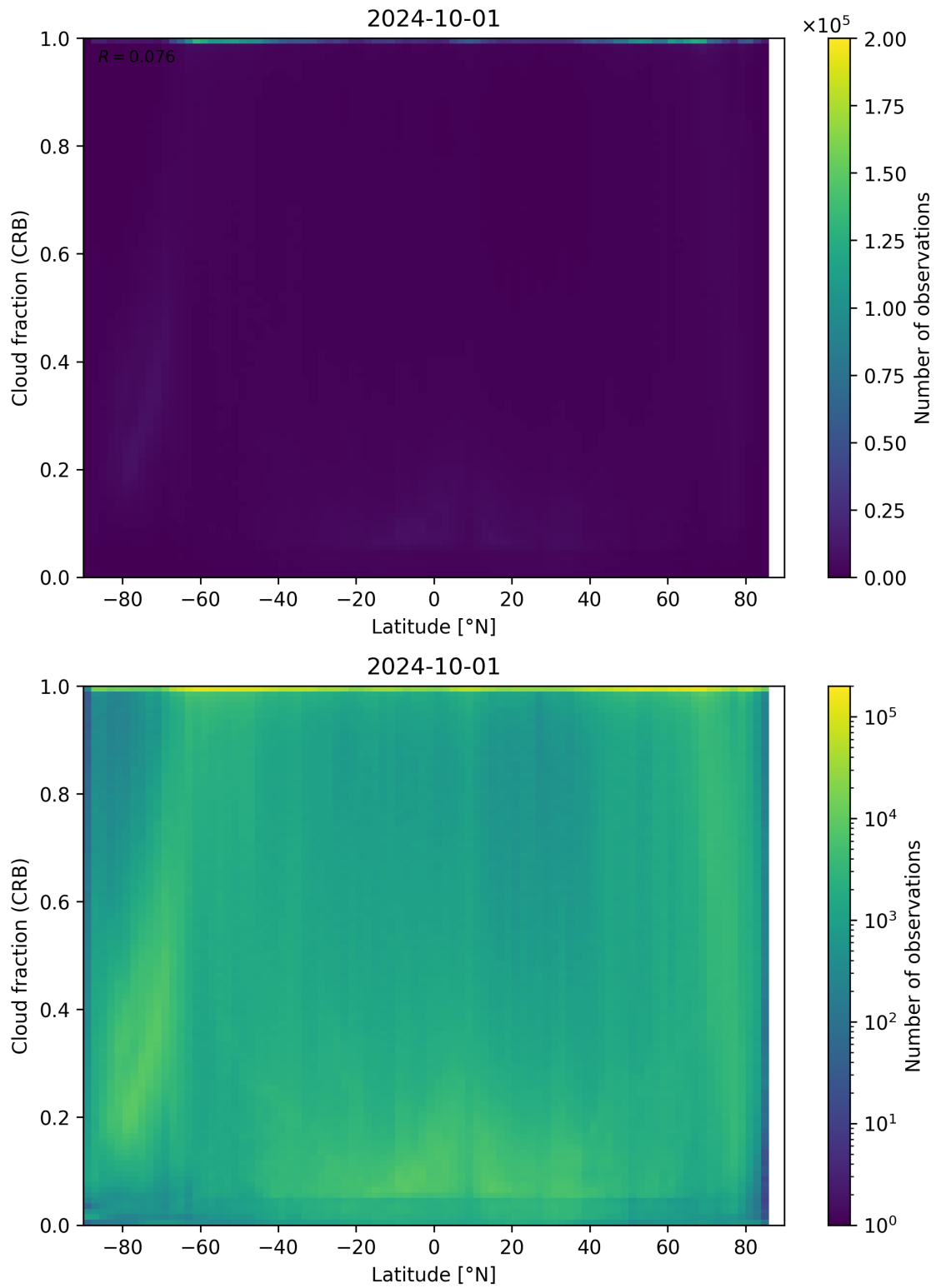
Figure 94: Scatter density plot of “Latitude” against “Cloud fraction (CRB)” for 2024-09-30 to 2024-10-02.
