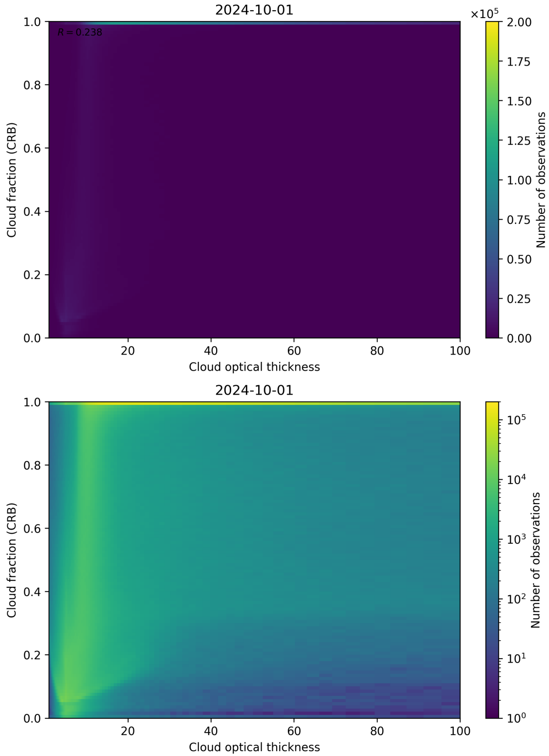
Figure 84: Scatter density plot of “Cloud optical thickness” against “Cloud fraction (CRB)” for 2024-09-30 to 2024-10-02.
