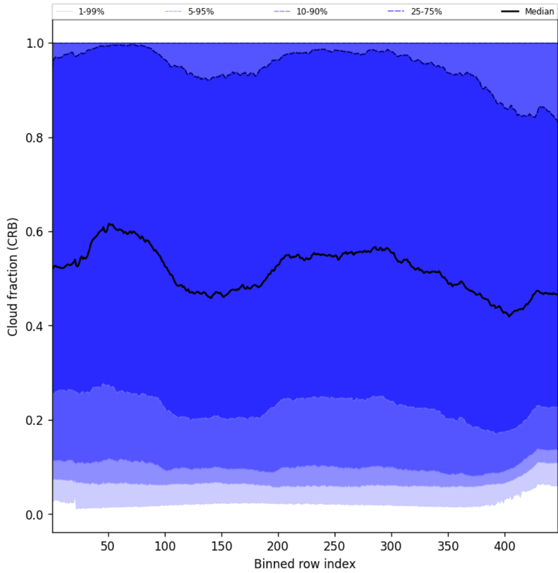
Figure 58: Along track statistics of “Cloud fraction (CRB)” for 2024-09-30 to 2024-10-02
