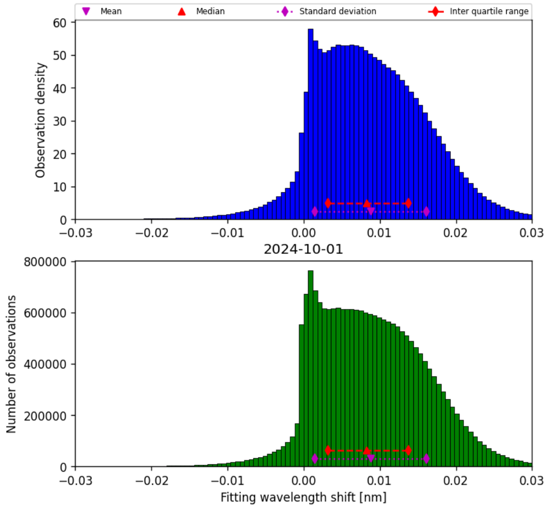
Figure 49: Histogram of “Fitting wavelength shift” for 2024-09-30 to 2024-10-02
