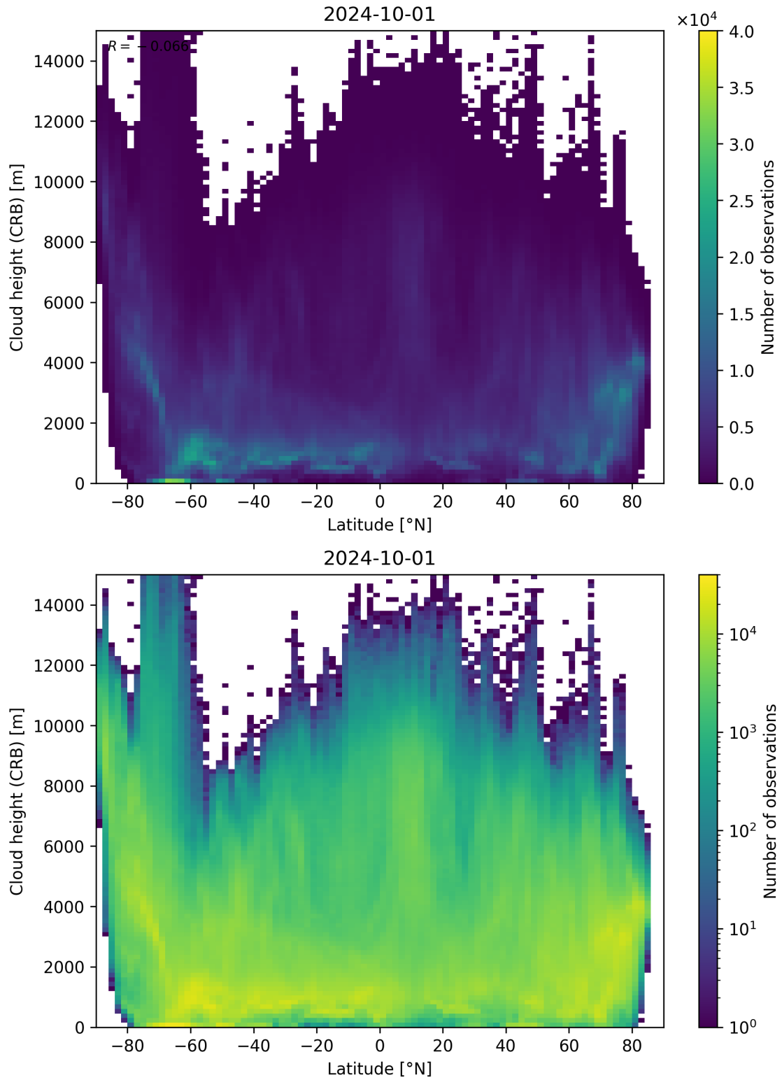
Figure 95: Scatter density plot of “Latitude” against “Cloud height (CRB)” for 2024-09-30 to 2024-10-02.
