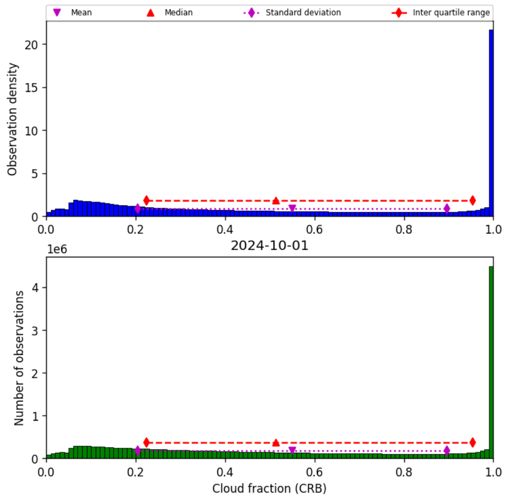
Figure 42: Histogram of “Cloud fraction (CRB)” for 2024-09-30 to 2024-10-02
