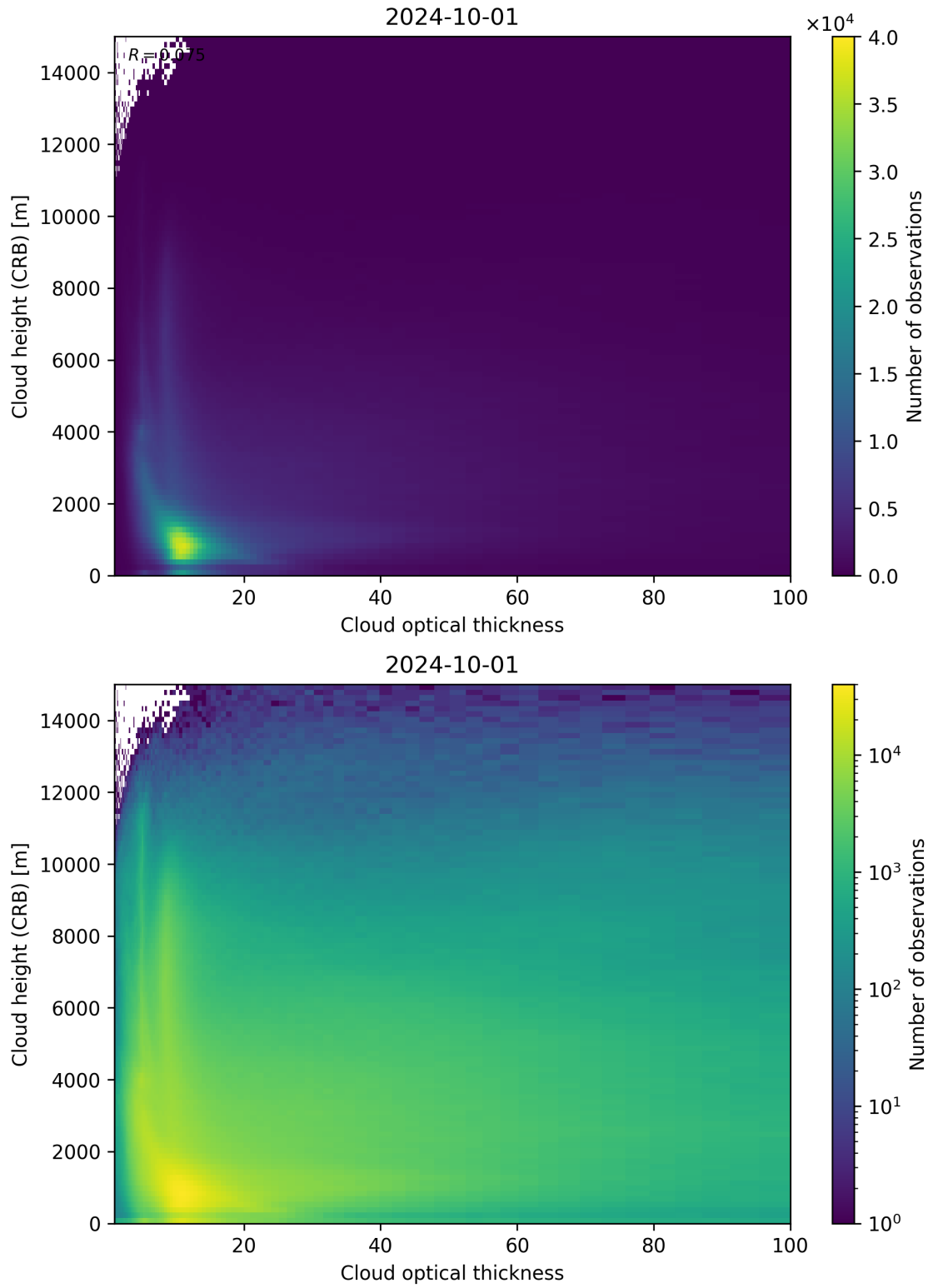
Figure 85: Scatter density plot of “Cloud optical thickness” against “Cloud height (CRB)” for 2024-09-30 to 2024-10-02.
