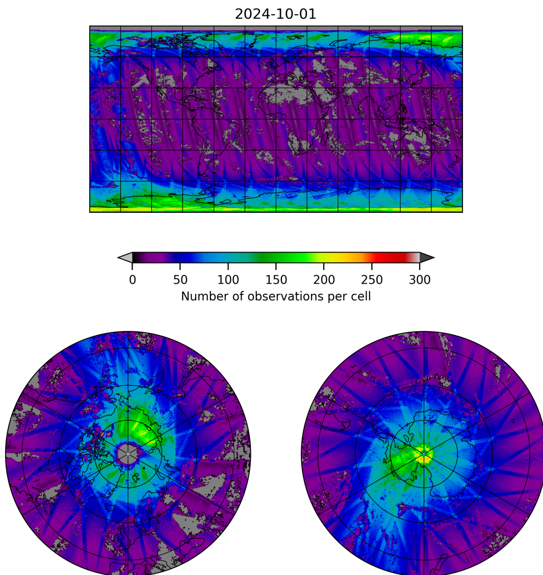
Figure 21: Map of the number of observations for 2024-09-30 to 2024-10-02
