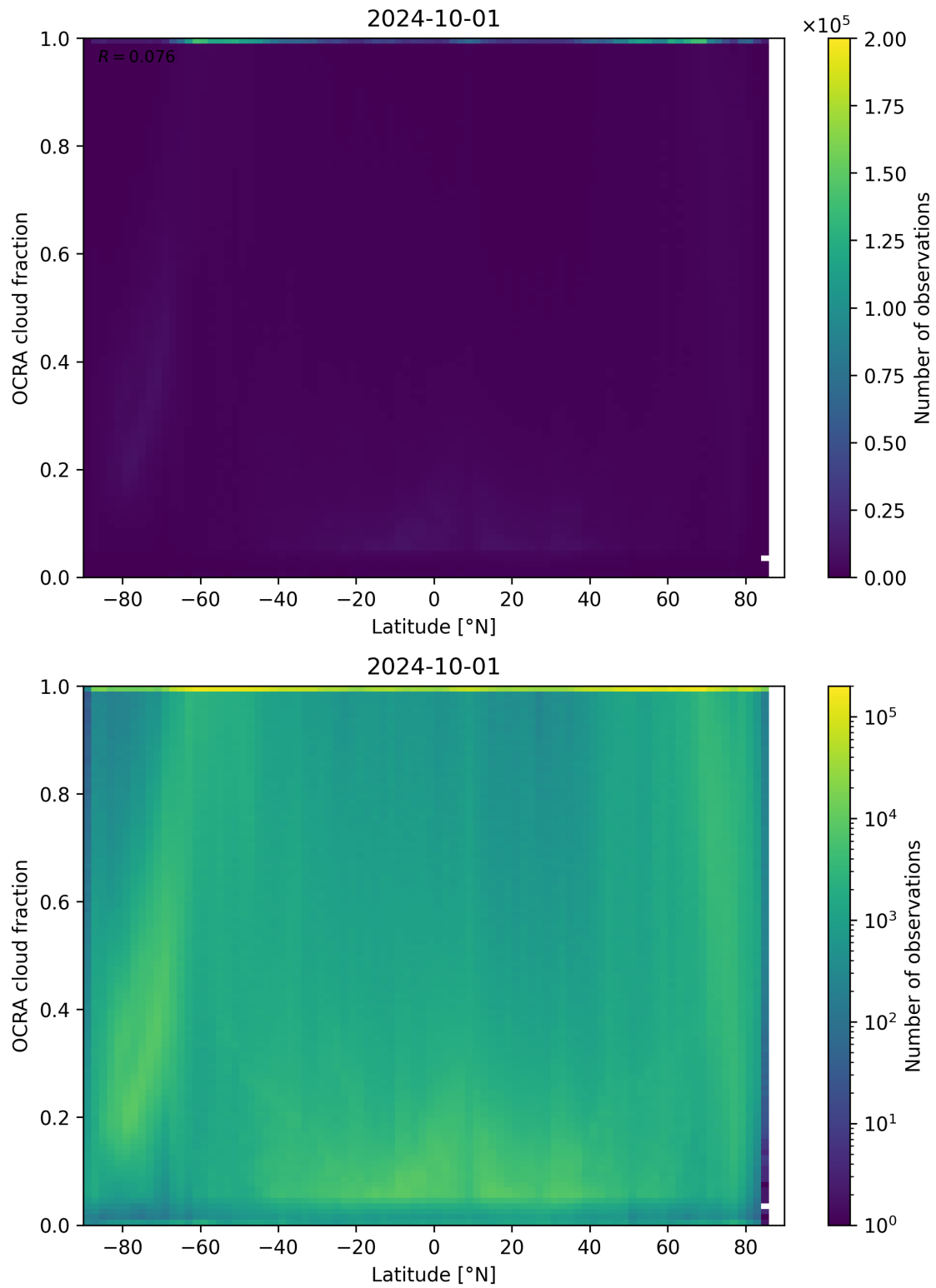
Figure 93: Scatter density plot of “Latitude” against “OCRA cloud fraction” for 2024-09-30 to 2024-10-02.
