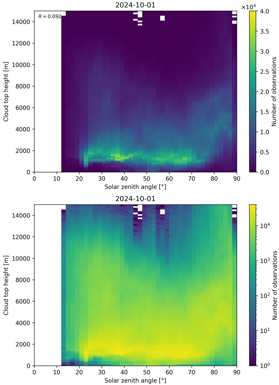
Figure 104: Scatter density plot of “Solar zenith angle” against “Cloud top height” for 2024-09-30 to 2024-10-02.
