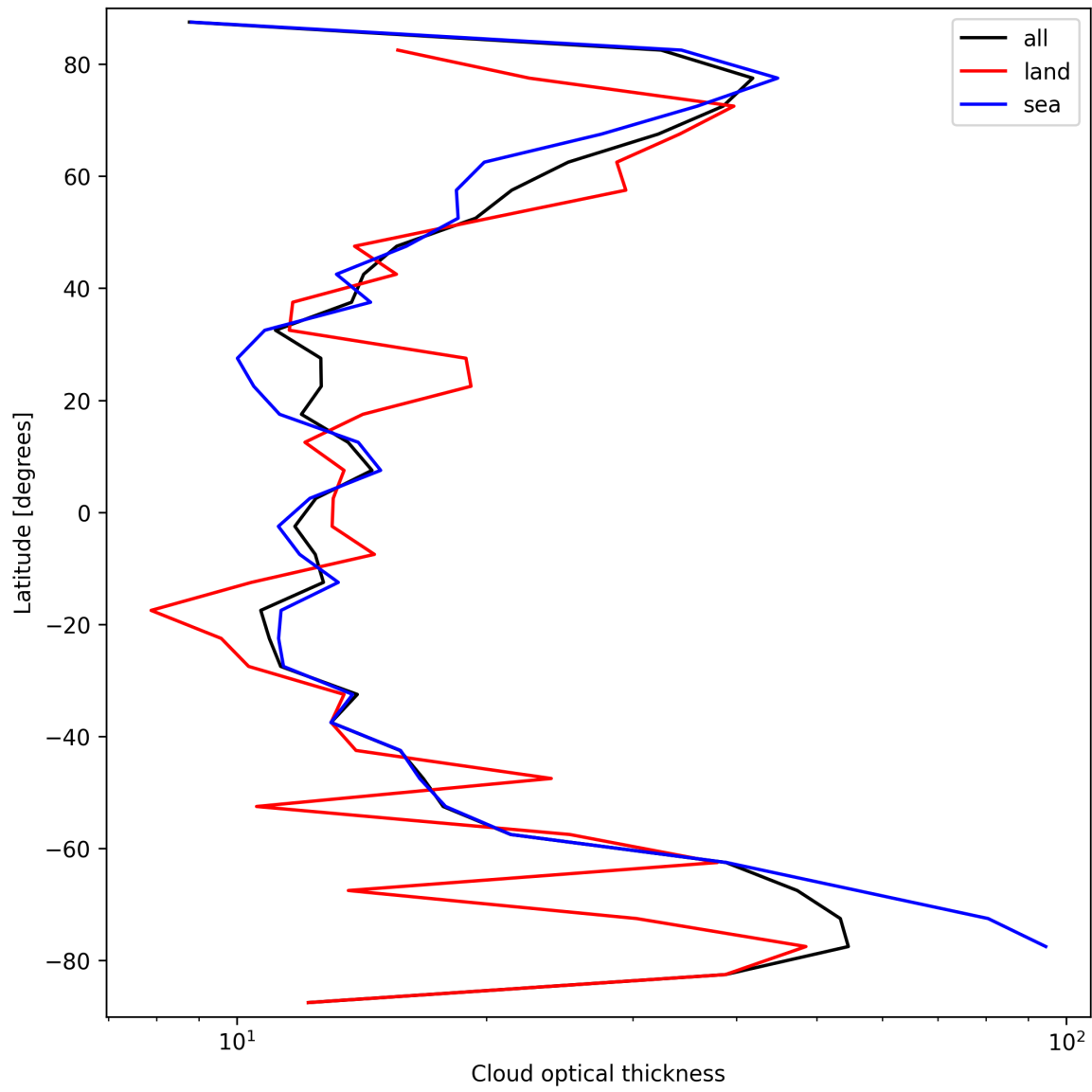
Figure 25: Zonal average of “Cloud optical thickness” for 2024-09-30 to 2024-10-02.
