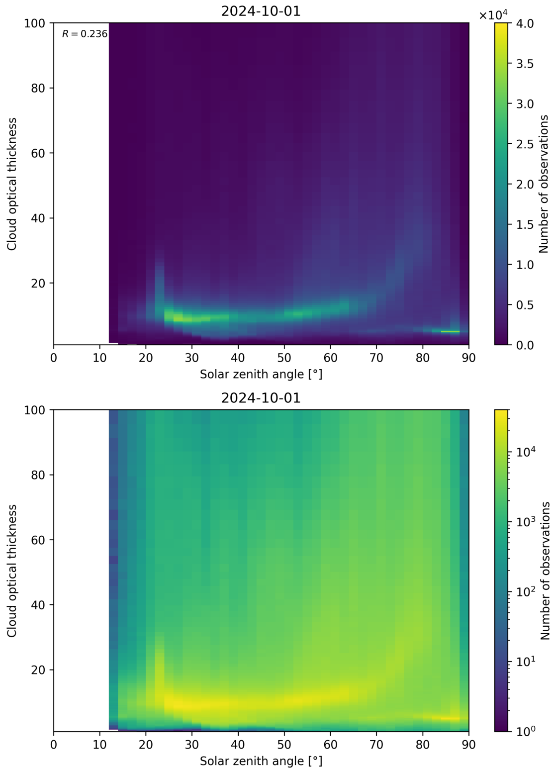
Figure 103: Scatter density plot of “Solar zenith angle” against “Cloud optical thickness” for 2024-09-30 to 2024-10-02.
