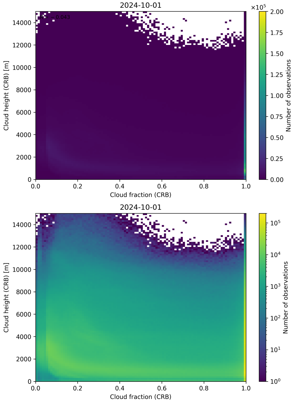
Figure 79: Scatter density plot of “Cloud fraction (CRB)” against “Cloud height (CRB)” for 2024-09-30 to 2024-10-02.
