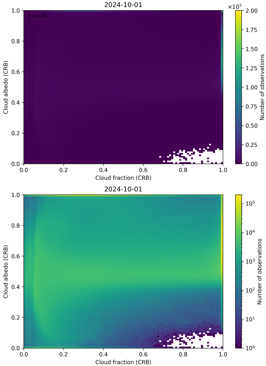
Figure 77: Scatter density plot of “Cloud fraction (CRB)” against “Cloud albedo (CRB)” for 2024-09-30 to 2024-10-02.
