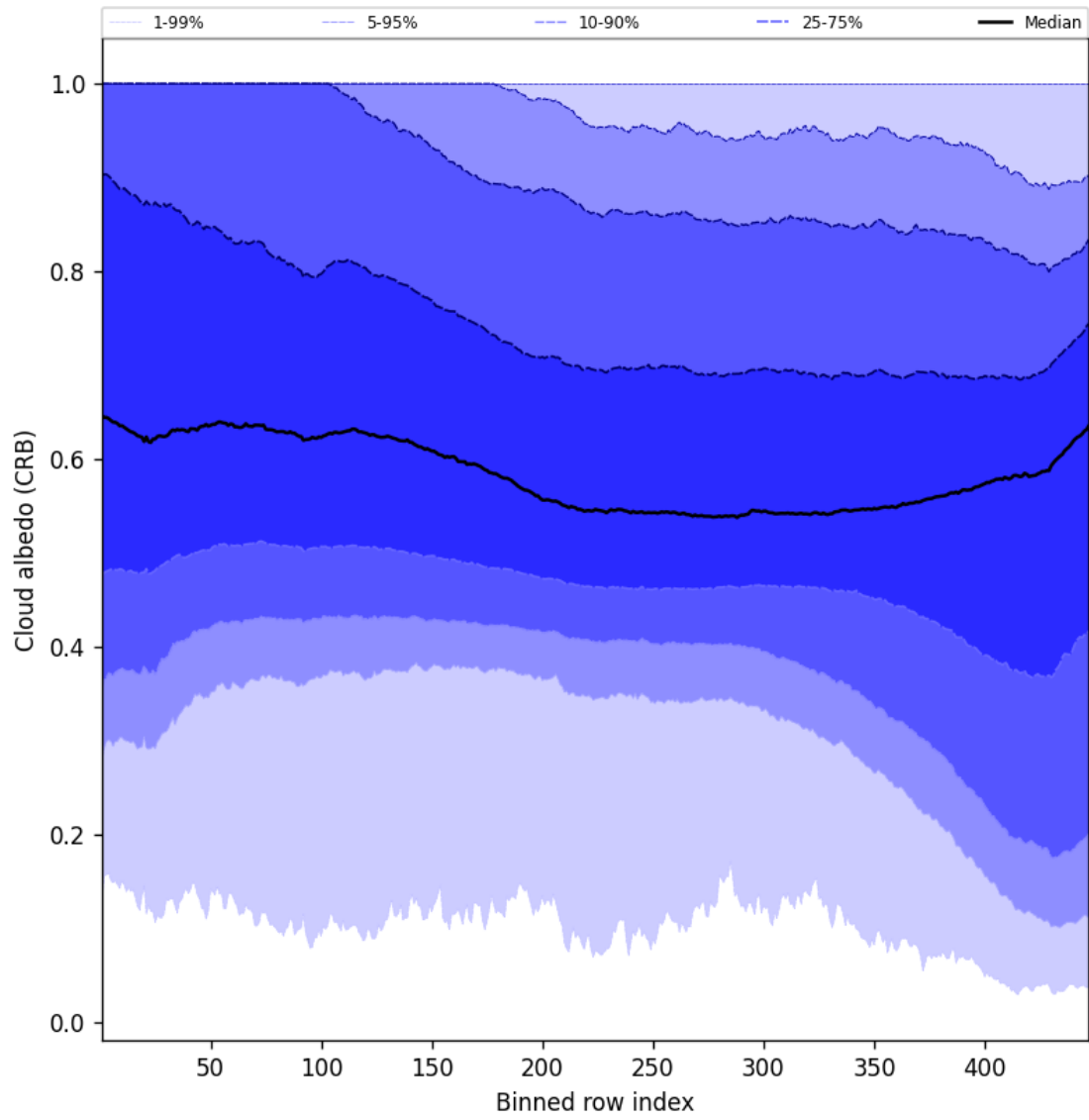
Figure 60: Along track statistics of “Cloud albedo (CRB)” for 2024-09-30 to 2024-10-02
