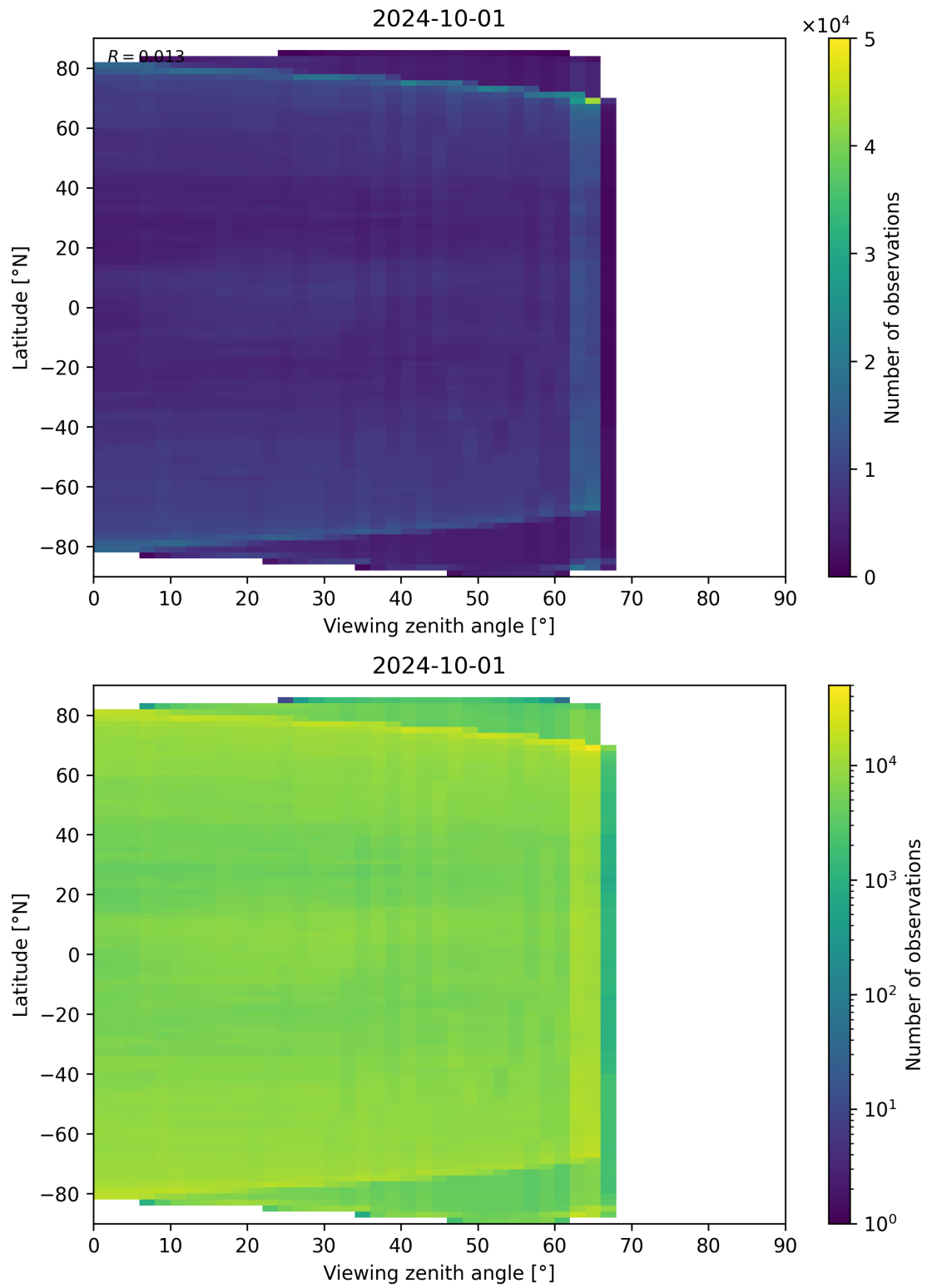
Figure 113: Scatter density plot of “Viewing zenith angle” against “Latitude” for 2024-09-30 to 2024-10-02.
