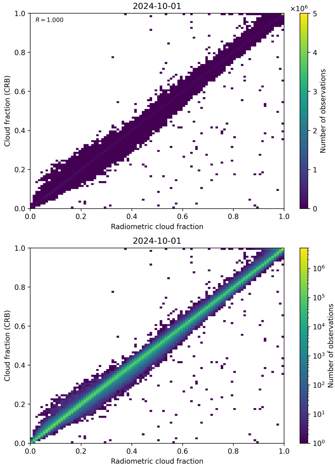
Figure 73: Scatter density plot of “Radiometric cloud fraction” against “Cloud fraction (CRB)” for 2024-09-30 to 2024-10-02.
