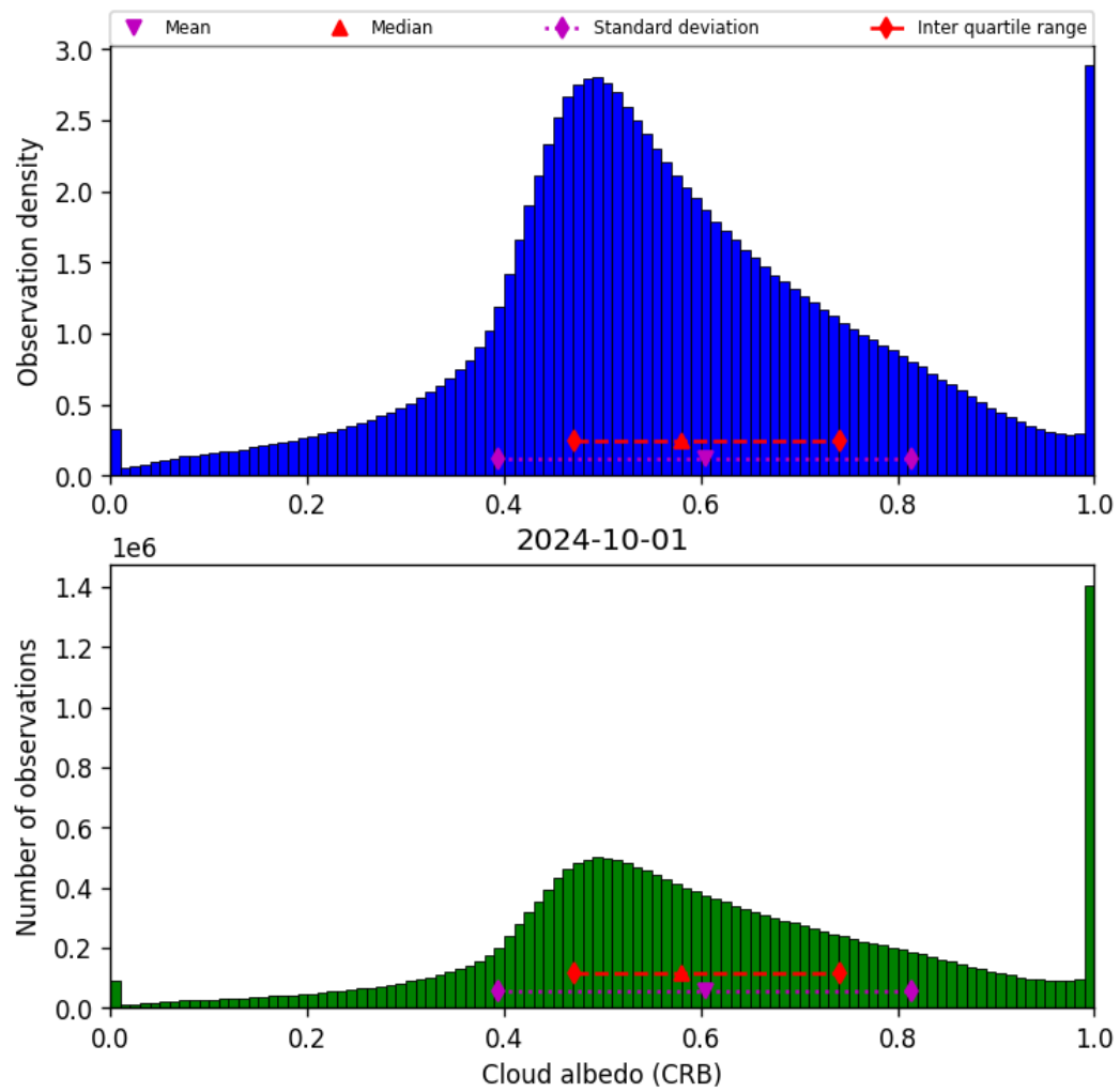
Figure 44: Histogram of “Cloud albedo (CRB)” for 2024-09-30 to 2024-10-02
