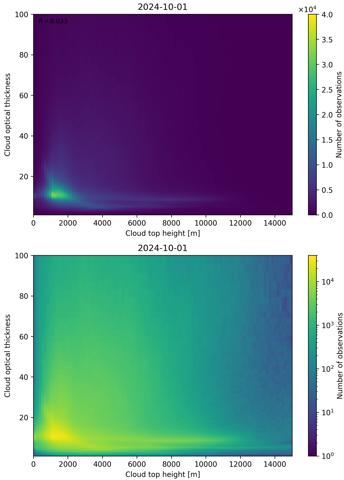
Figure 90: Scatter density plot of “Cloud top height” against “Cloud optical thickness” for 2024-09-30 to 2024-10-02.
