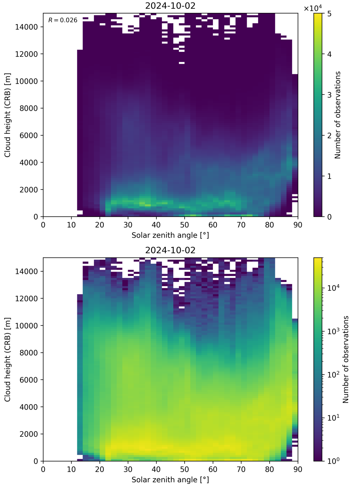
Figure 102: Scatter density plot of “Solar zenith angle” against “Cloud height (CRB)” for 2024-10-01 to 2024-10-03.
