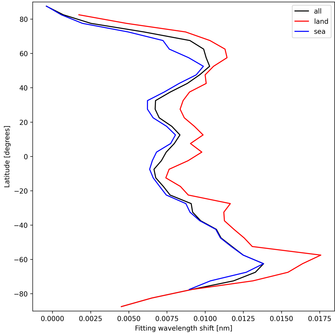
Figure 33: Zonal average of “Fitting wavelength shift” for 2024-10-01 to 2024-10-03.
