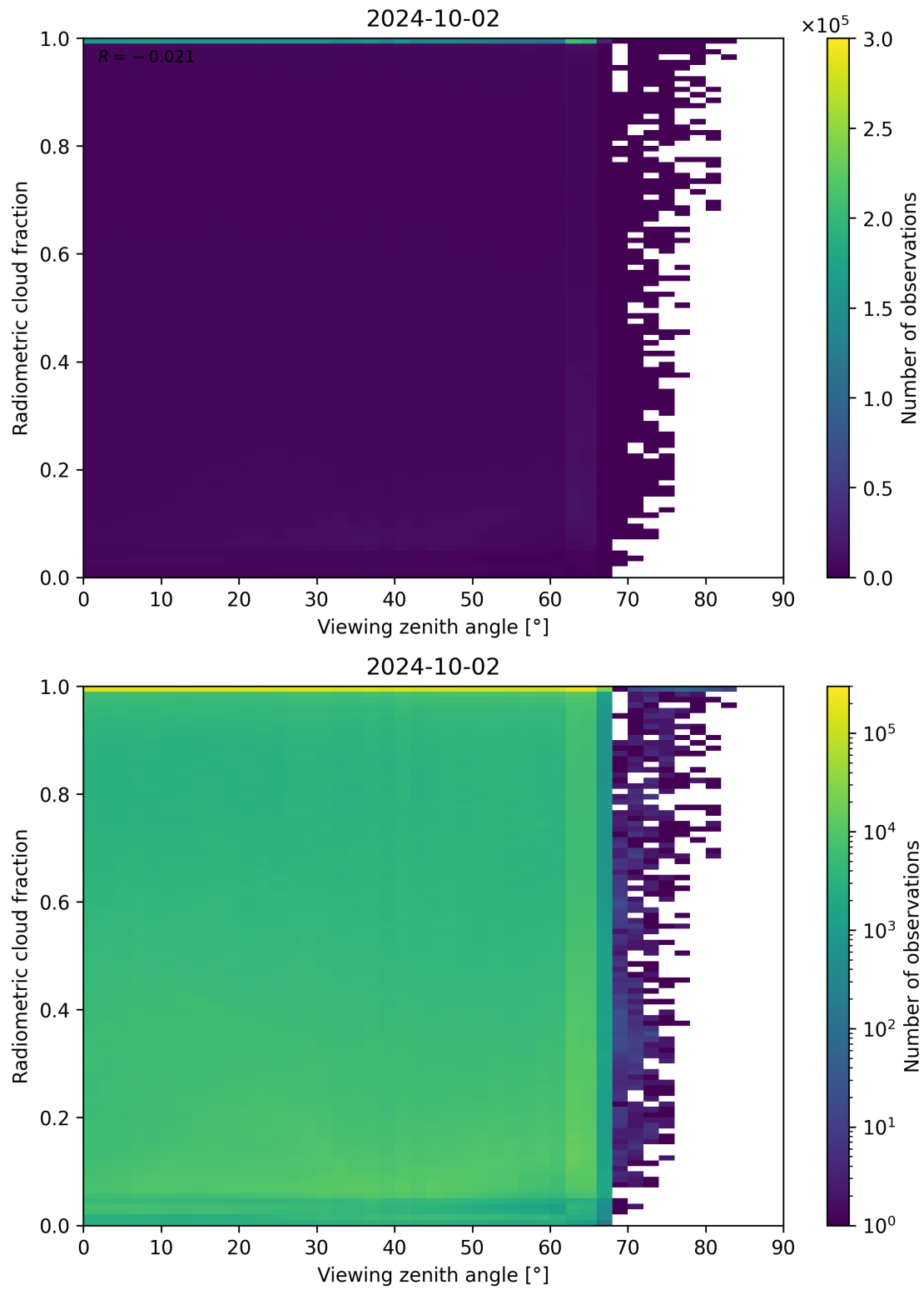
Figure 107: Scatter density plot of “Viewing zenith angle” against “Radiometric cloud fraction” for 2024-10-01 to 2024-10-03.
