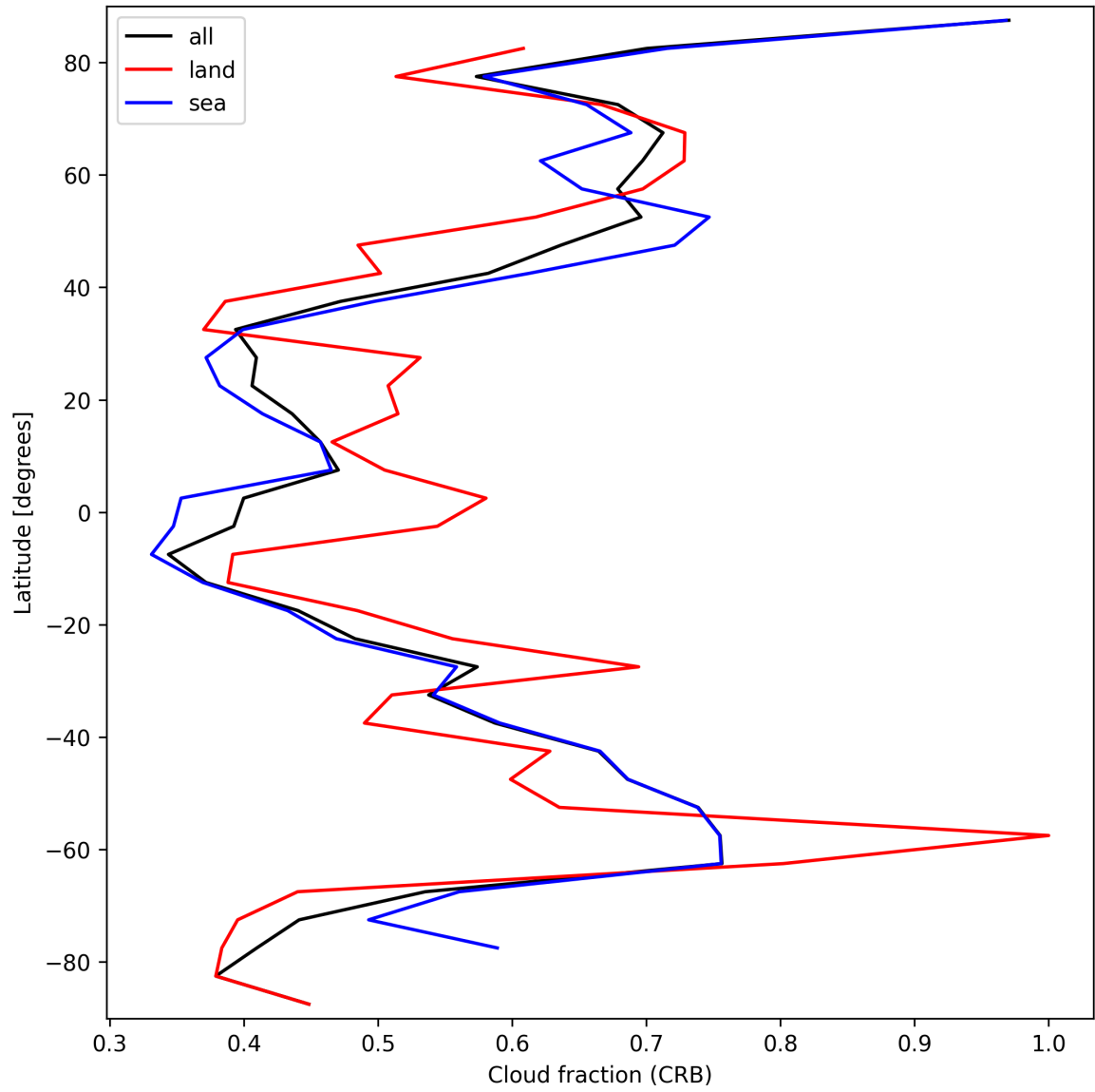
Figure 26: Zonal average of “Cloud fraction (CRB)” for 2024-10-01 to 2024-10-03.
