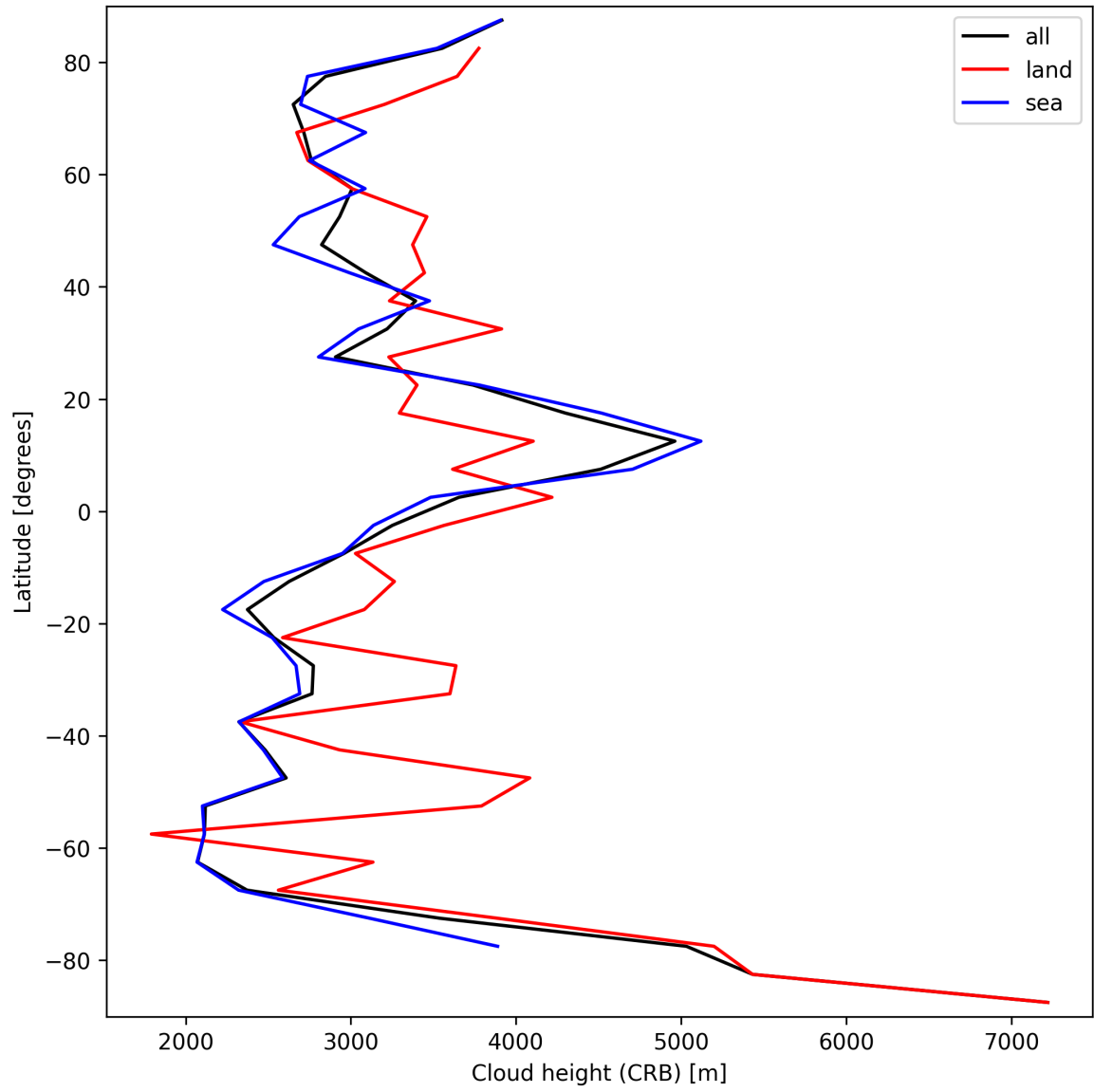
Figure 27: Zonal average of “Cloud height (CRB)” for 2024-10-01 to 2024-10-03.
