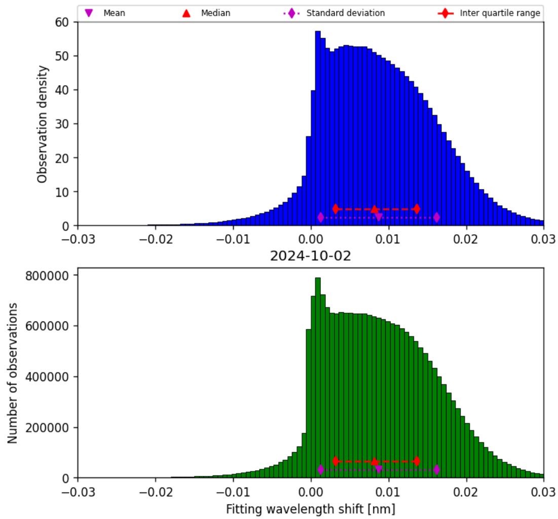
Figure 49: Histogram of “Fitting wavelength shift” for 2024-10-01 to 2024-10-03
