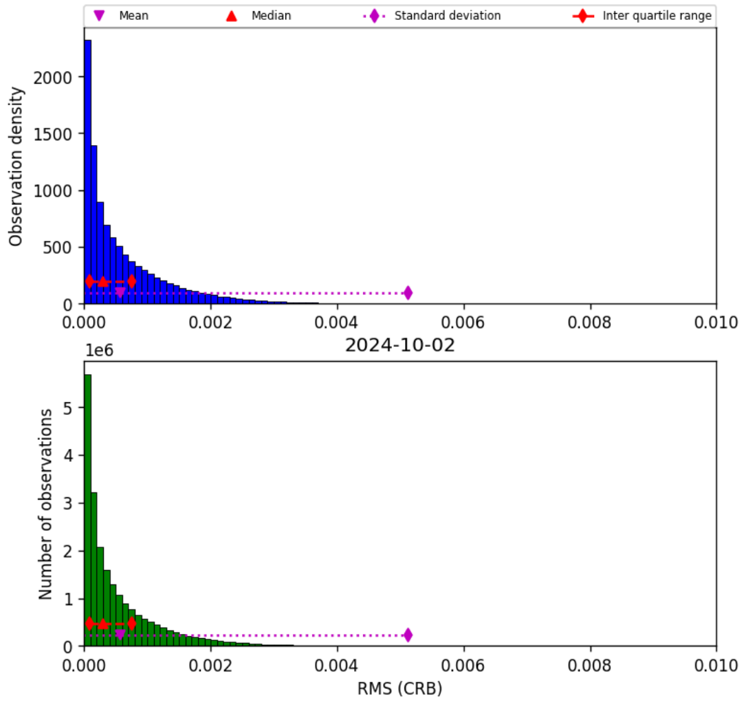
Figure 48: Histogram of “RMS (CRB)” for 2024-10-01 to 2024-10-03
