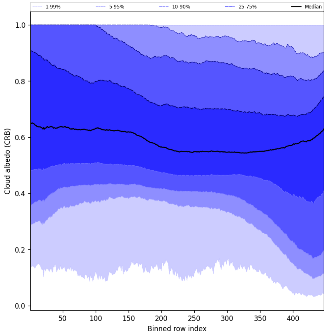
Figure 60: Along track statistics of “Cloud albedo (CRB)” for 2024-10-01 to 2024-10-03
