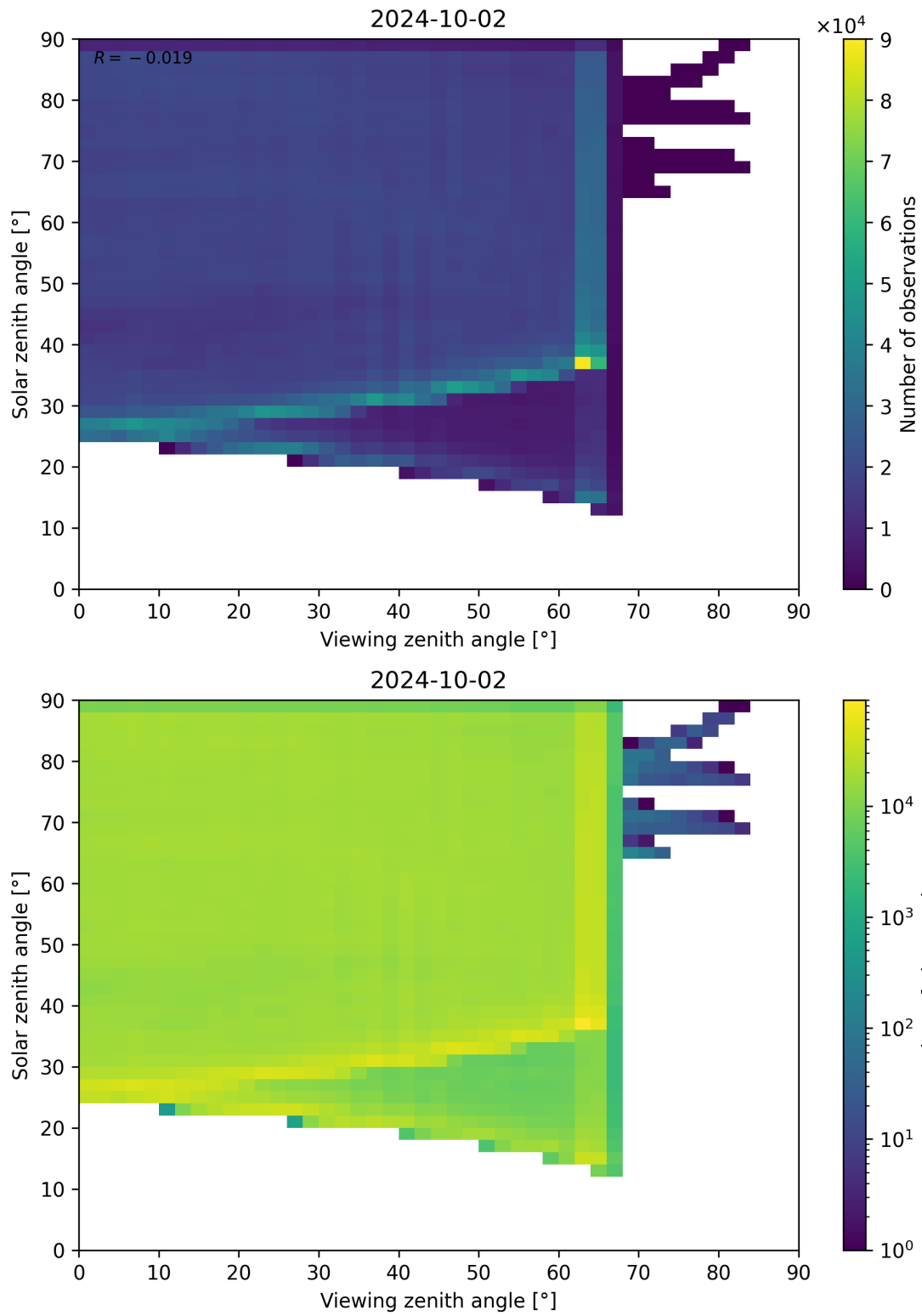
Figure 114: Scatter density plot of “Viewing zenith angle” against “Solar zenith angle” for 2024-10-01 to 2024-10-03.
