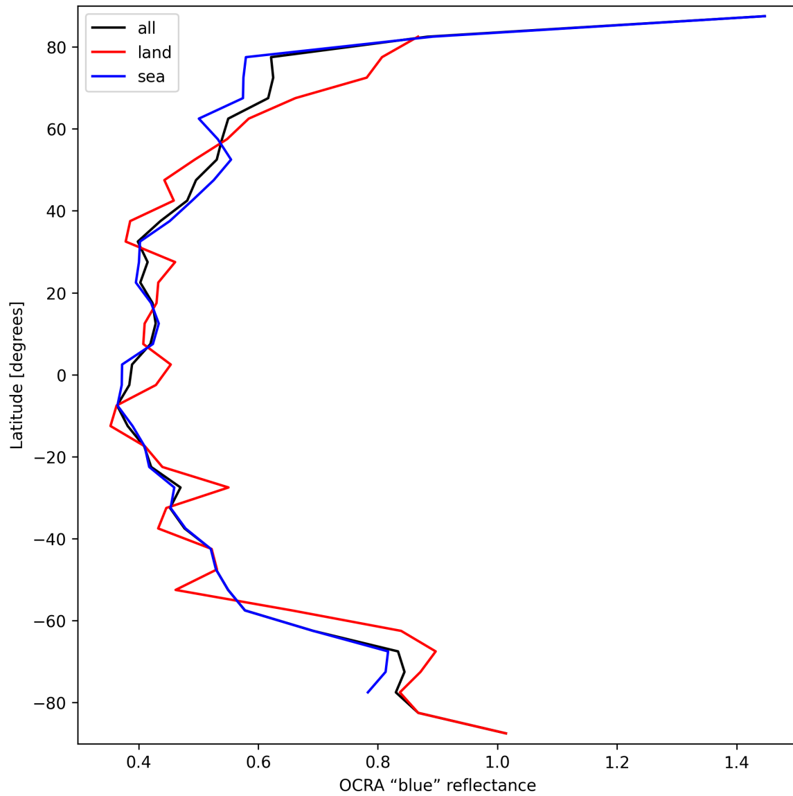
Figure 35: Zonal average of “OCRA “blue” reflectance” for 2024-10-01 to 2024-10-03.
