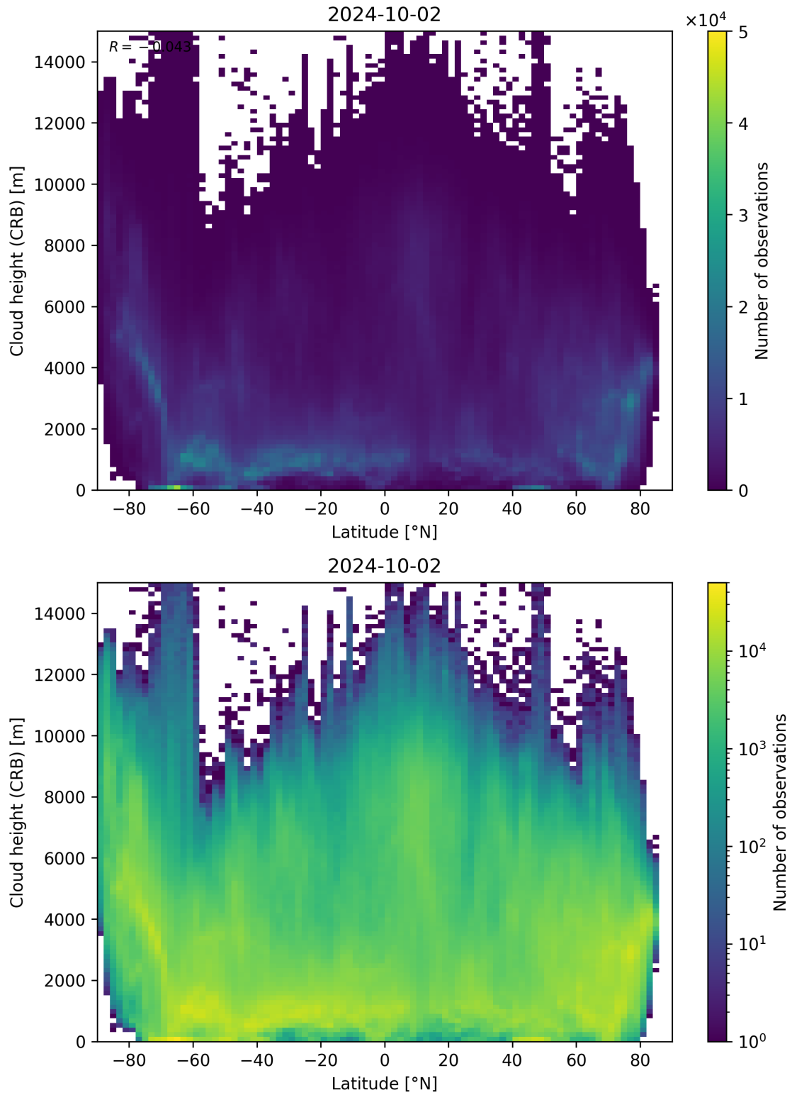
Figure 95: Scatter density plot of “Latitude” against “Cloud height (CRB)” for 2024-10-01 to 2024-10-03.
