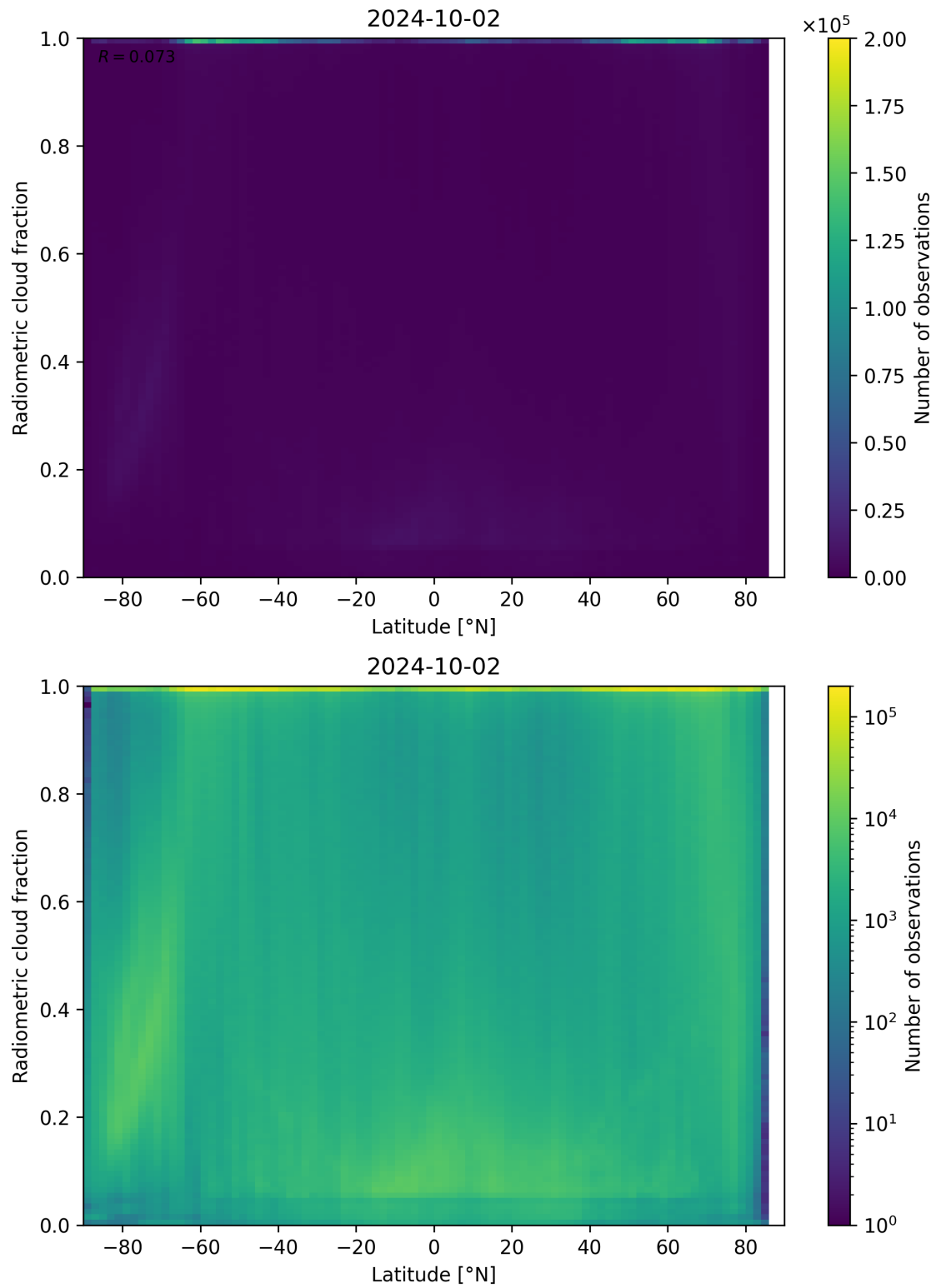
Figure 92: Scatter density plot of “Latitude” against “Radiometric cloud fraction” for 2024-10-01 to 2024-10-03.
