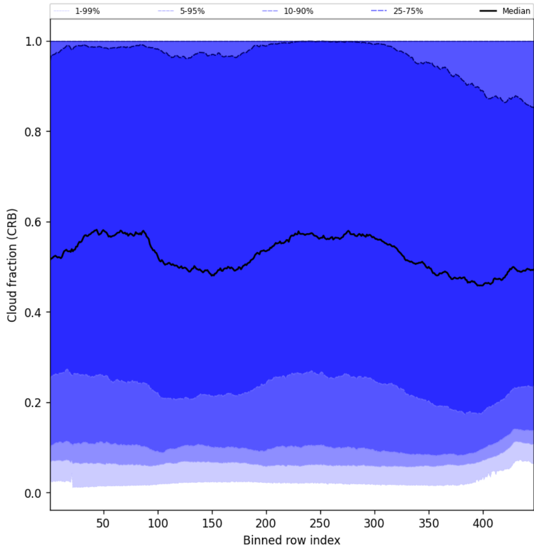
Figure 58: Along track statistics of “Cloud fraction (CRB)” for 2024-10-01 to 2024-10-03
