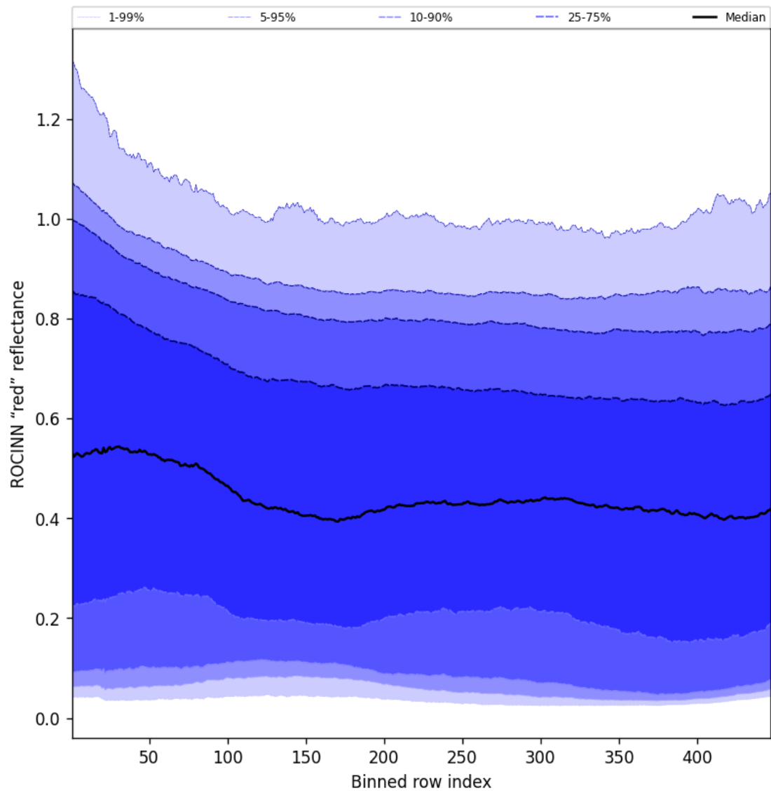
Figure 69: Along track statistics of “ROCINN “red” reflectance” for 2024-10-01 to 2024-10-03
