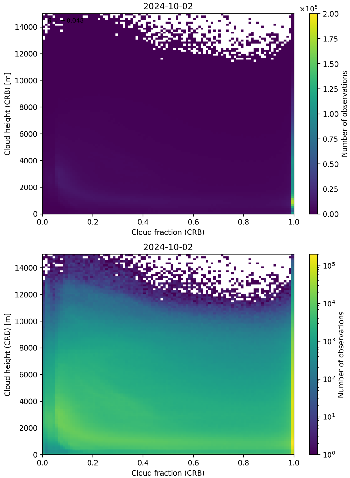
Figure 79: Scatter density plot of “Cloud fraction (CRB)” against “Cloud height (CRB)” for 2024-10-01 to 2024-10-03.
