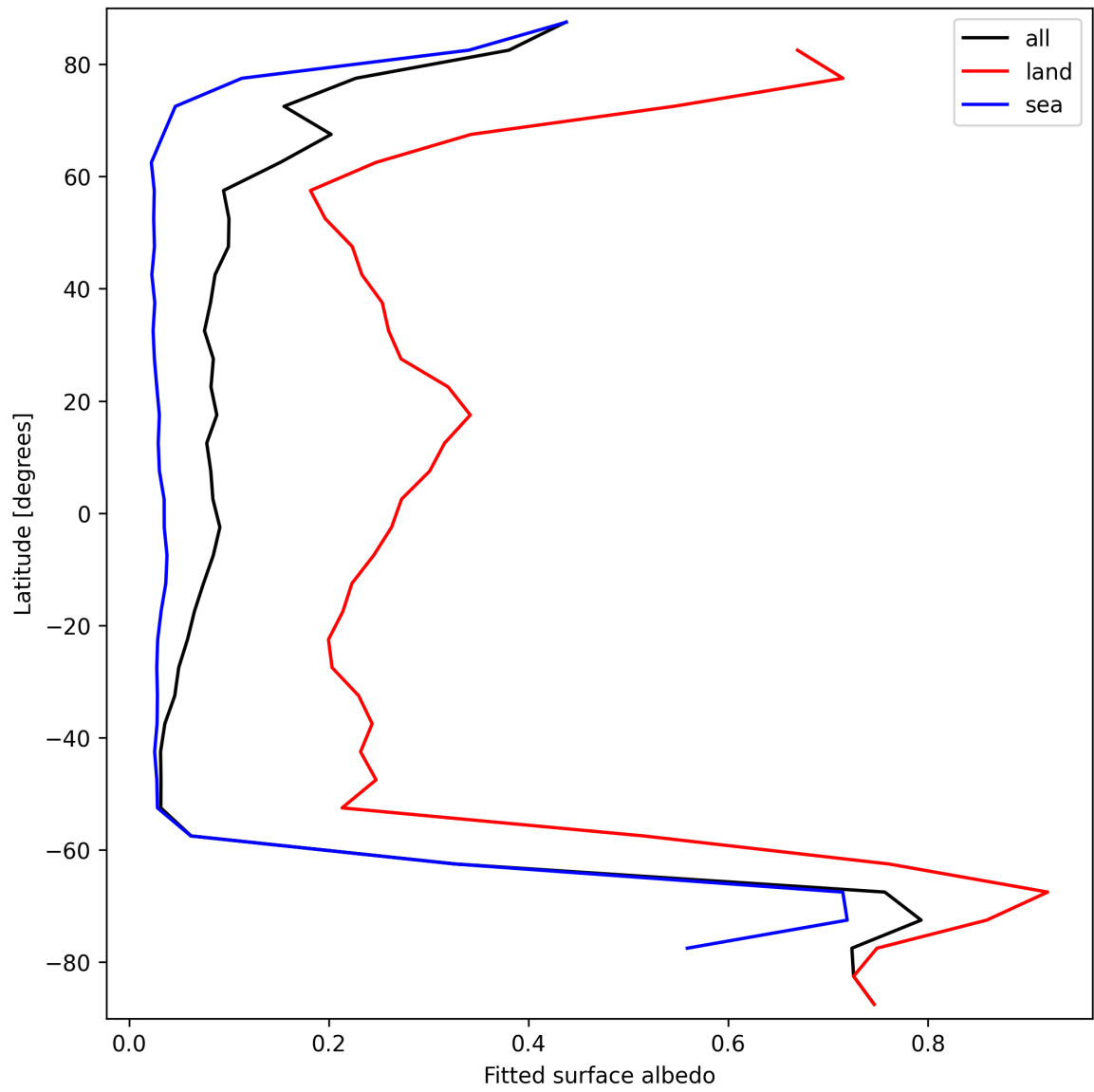
Figure 29: Zonal average of “Fitted surface albedo” for 2024-10-01 to 2024-10-03.
