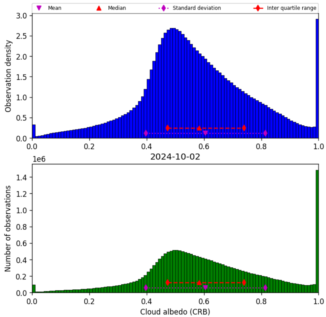
Figure 44: Histogram of “Cloud albedo (CRB)” for 2024-10-01 to 2024-10-03
