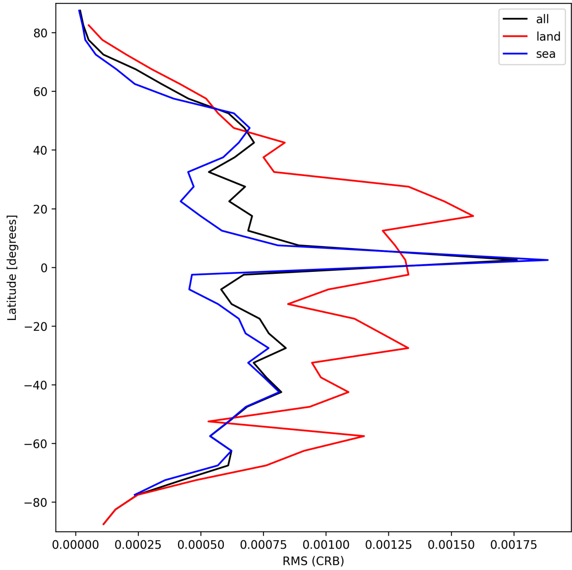
Figure 32: Zonal average of “RMS (CRB)” for 2024-10-01 to 2024-10-03.
