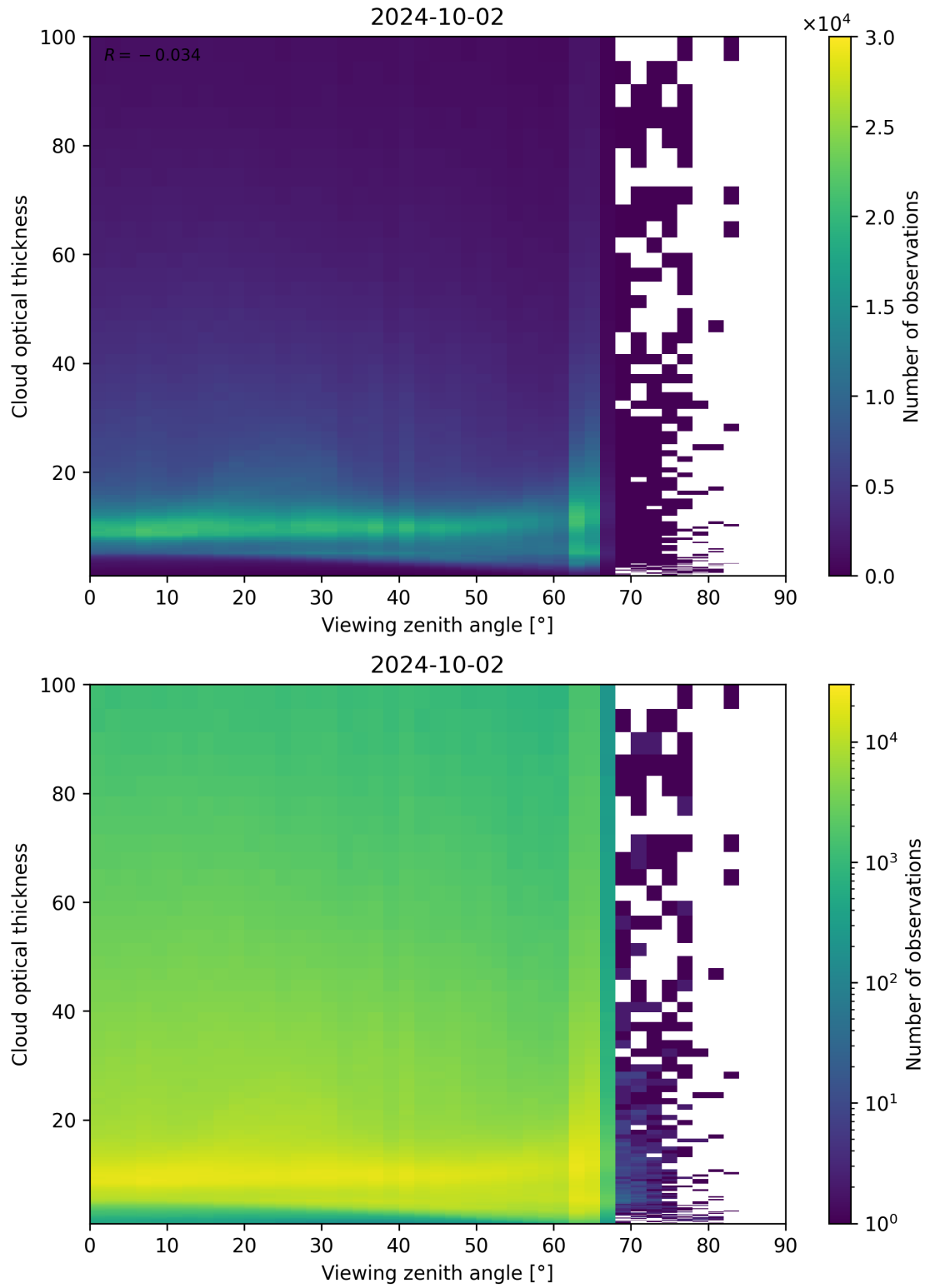
Figure 111: Scatter density plot of “Viewing zenith angle” against “Cloud optical thickness” for 2024-10-01 to 2024-10-03.
