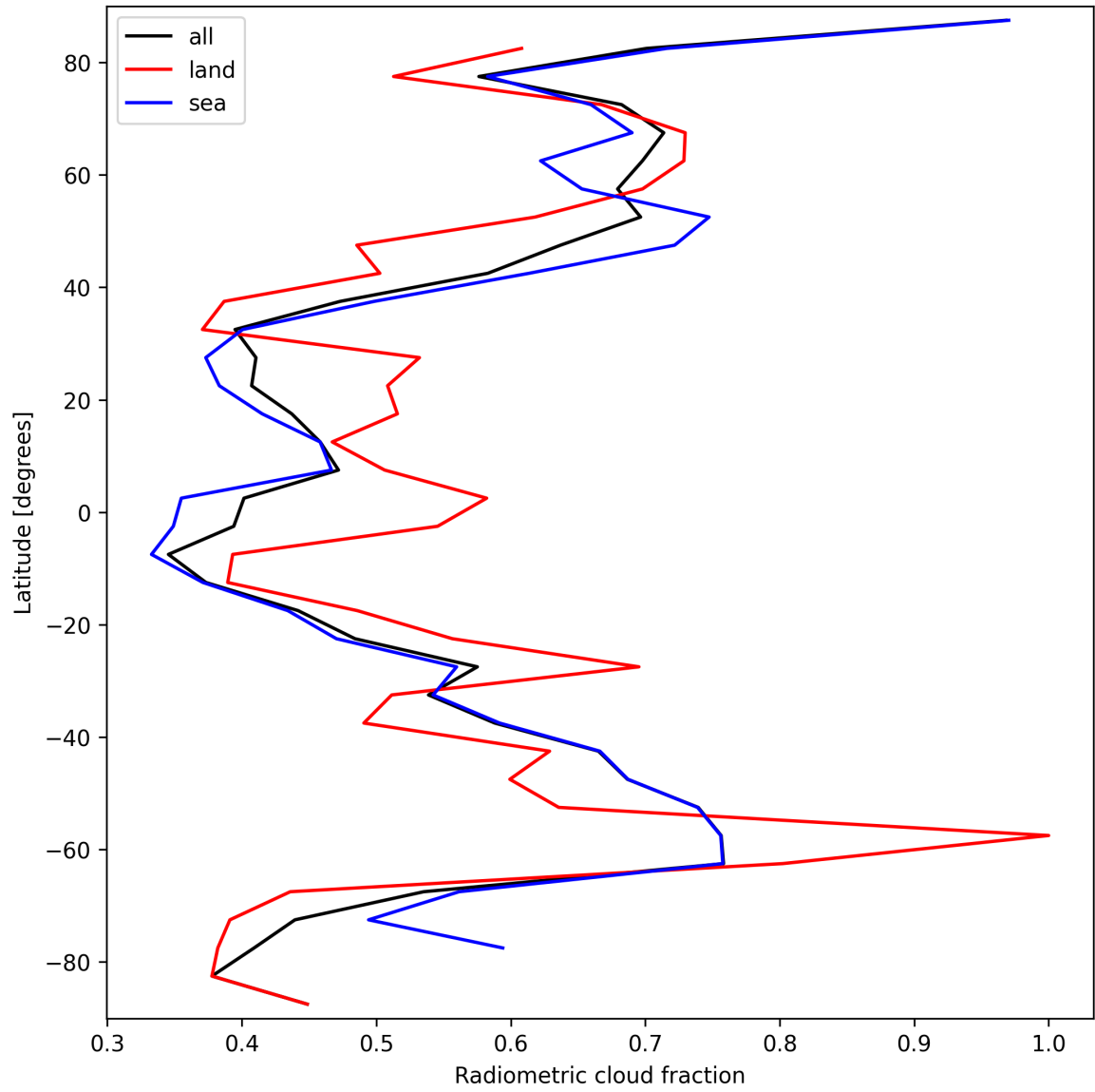
Figure 23: Zonal average of “Radiometric cloud fraction” for 2024-10-01 to 2024-10-03.
