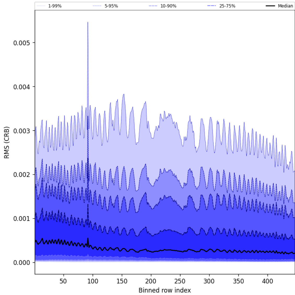
Figure 64: Along track statistics of “RMS (CRB)” for 2024-10-01 to 2024-10-03
