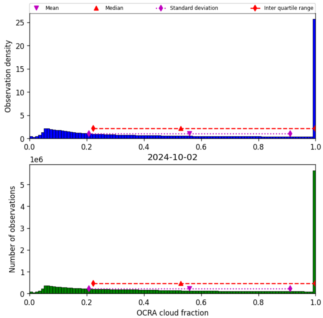
Figure 50: Histogram of “OCRA cloud fraction” for 2024-10-01 to 2024-10-03
