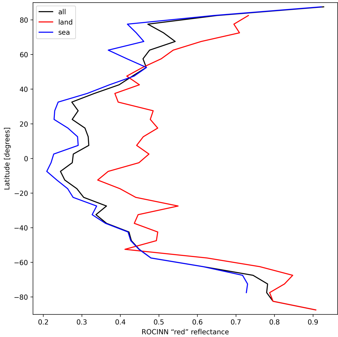
Figure 37: Zonal average of “ROCINN “red” reflectance” for 2024-10-01 to 2024-10-03.
