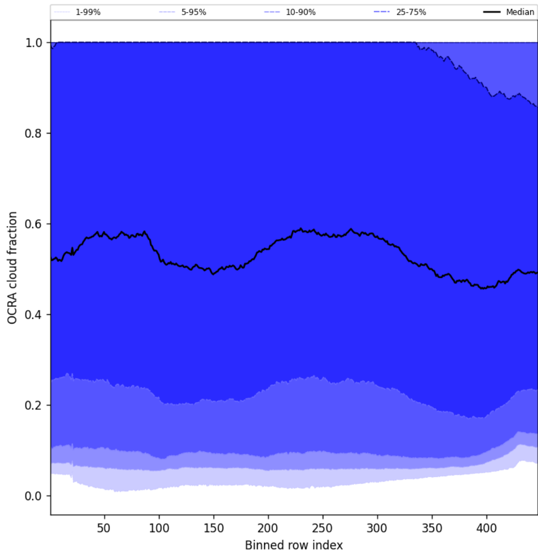
Figure 66: Along track statistics of “OCRA cloud fraction” for 2024-10-01 to 2024-10-03
