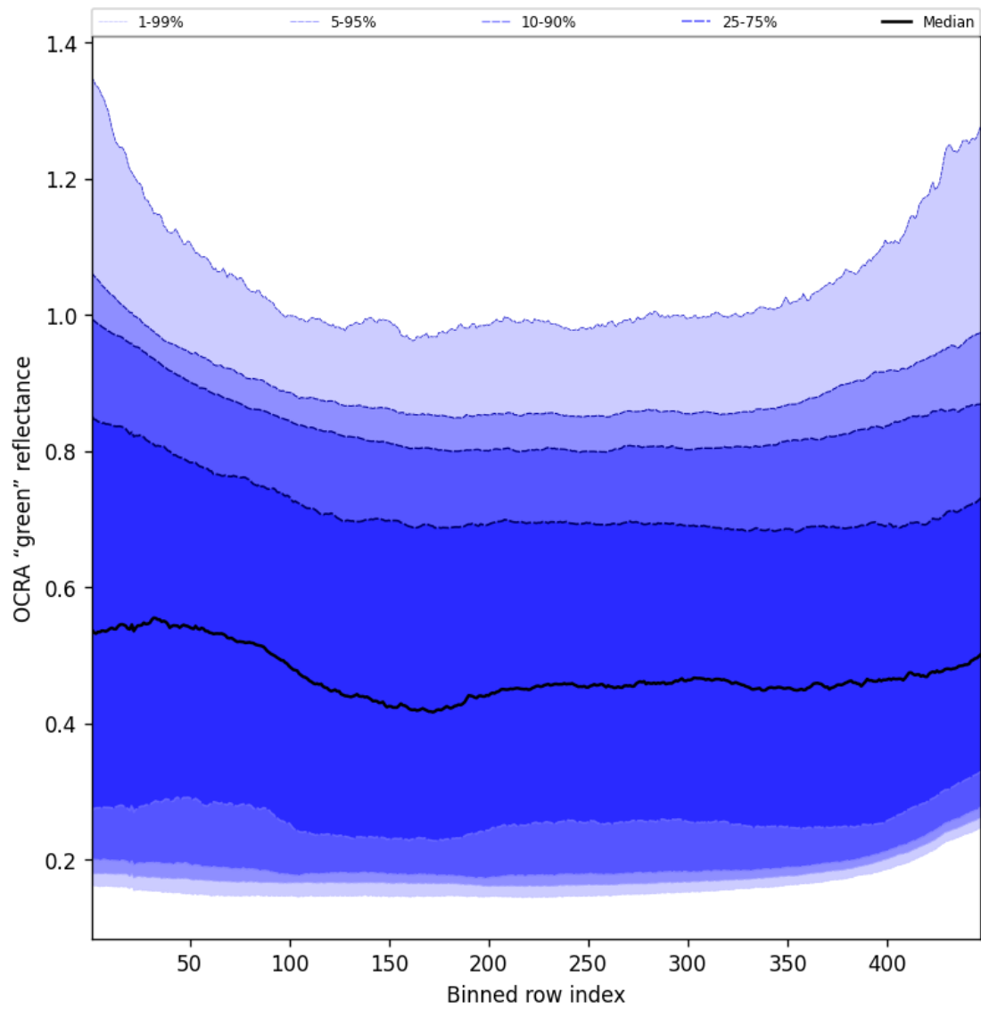
Figure 68: Along track statistics of “OCRA “green” reflectance” for 2024-10-01 to 2024-10-03
