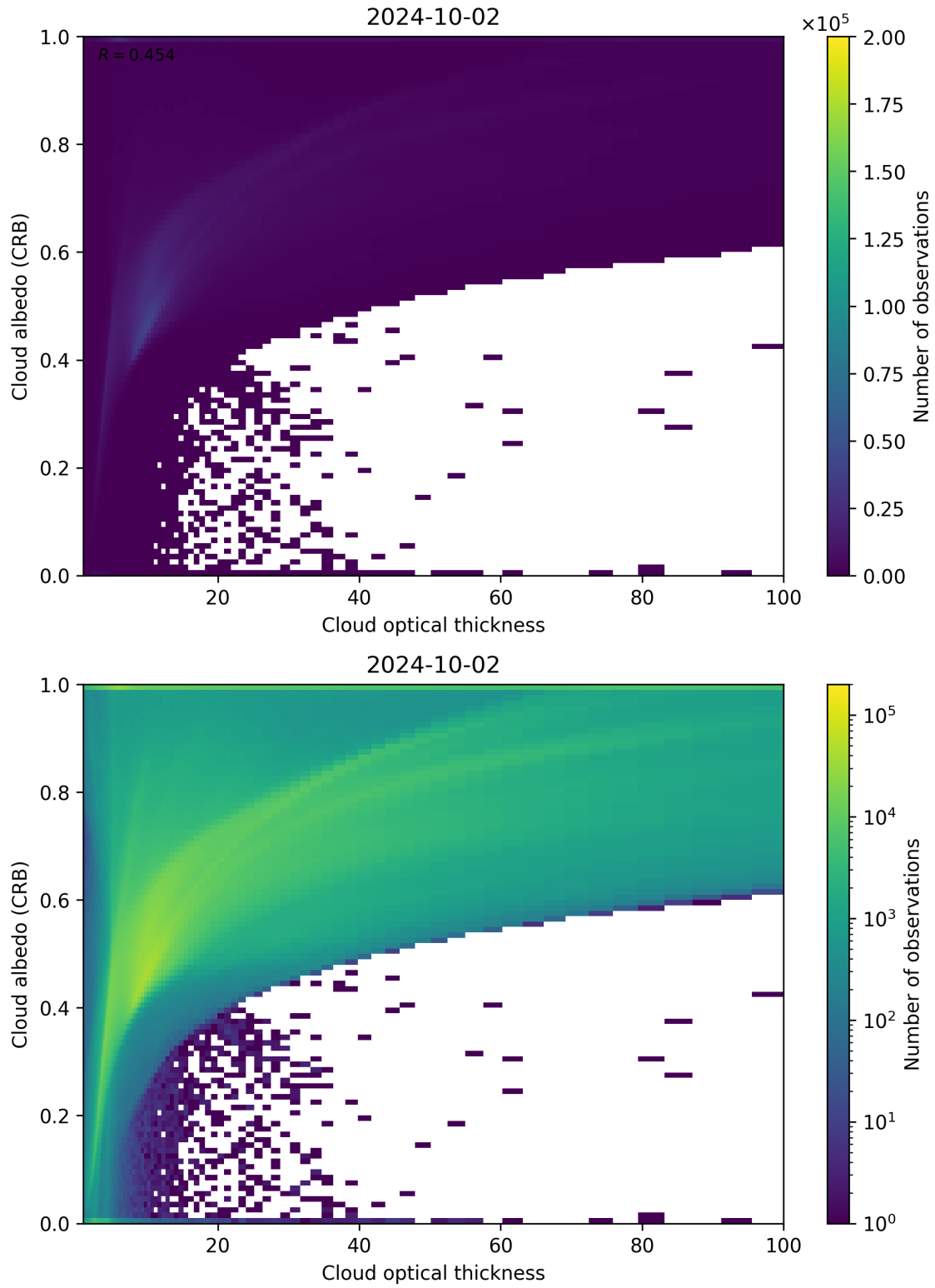
Figure 82: Scatter density plot of “Cloud optical thickness” against “Cloud albedo (CRB)” for 2024-10-01 to 2024-10-03.
