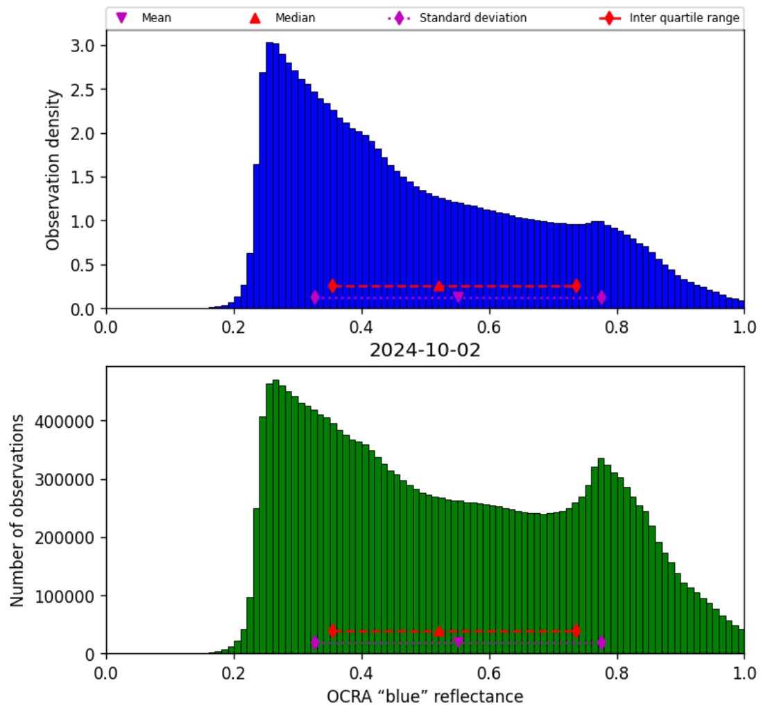
Figure 51: Histogram of "OCRA "blue" reflectance" for 2024-10-01 to 2024-10-03
