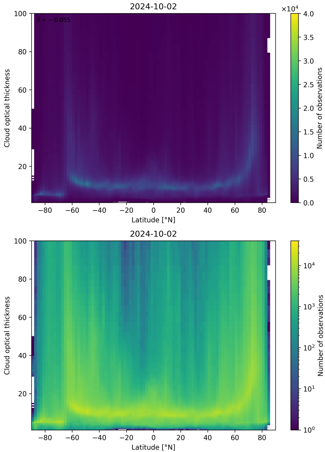
Figure 96: Scatter density plot of “Latitude” against “Cloud optical thickness” for 2024-10-01 to 2024-10-03.
