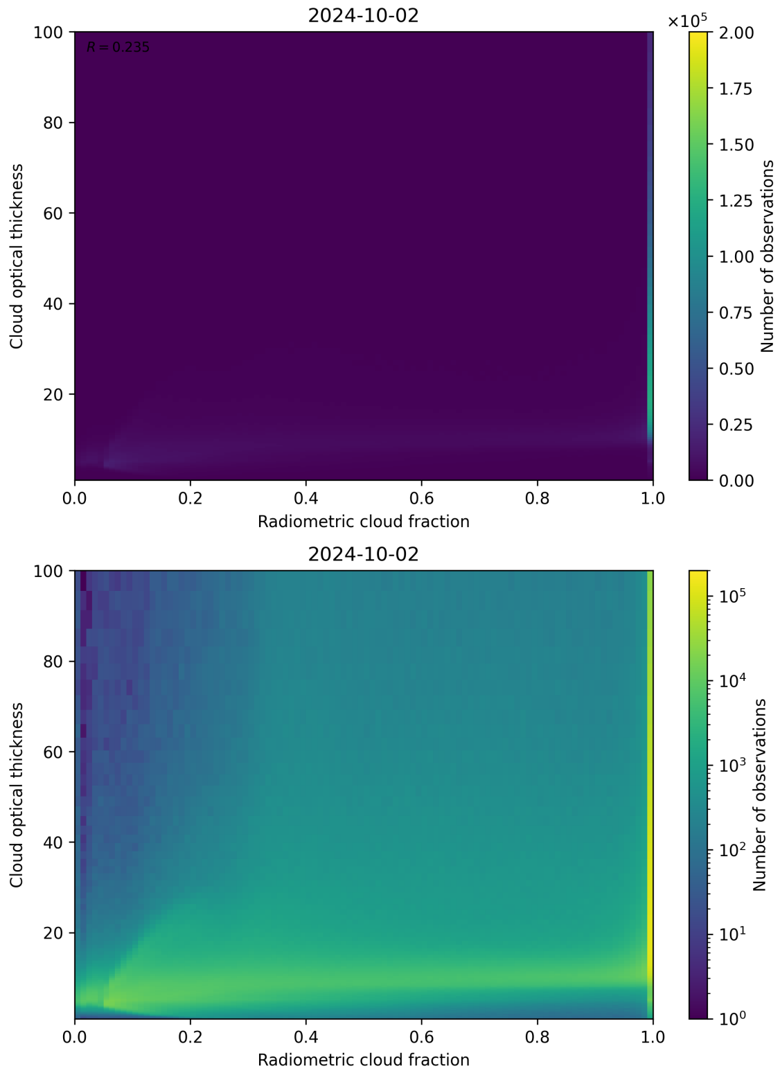
Figure 75: Scatter density plot of “Radiometric cloud fraction” against “Cloud optical thickness” for 2024-10-01 to 2024-10-03.
