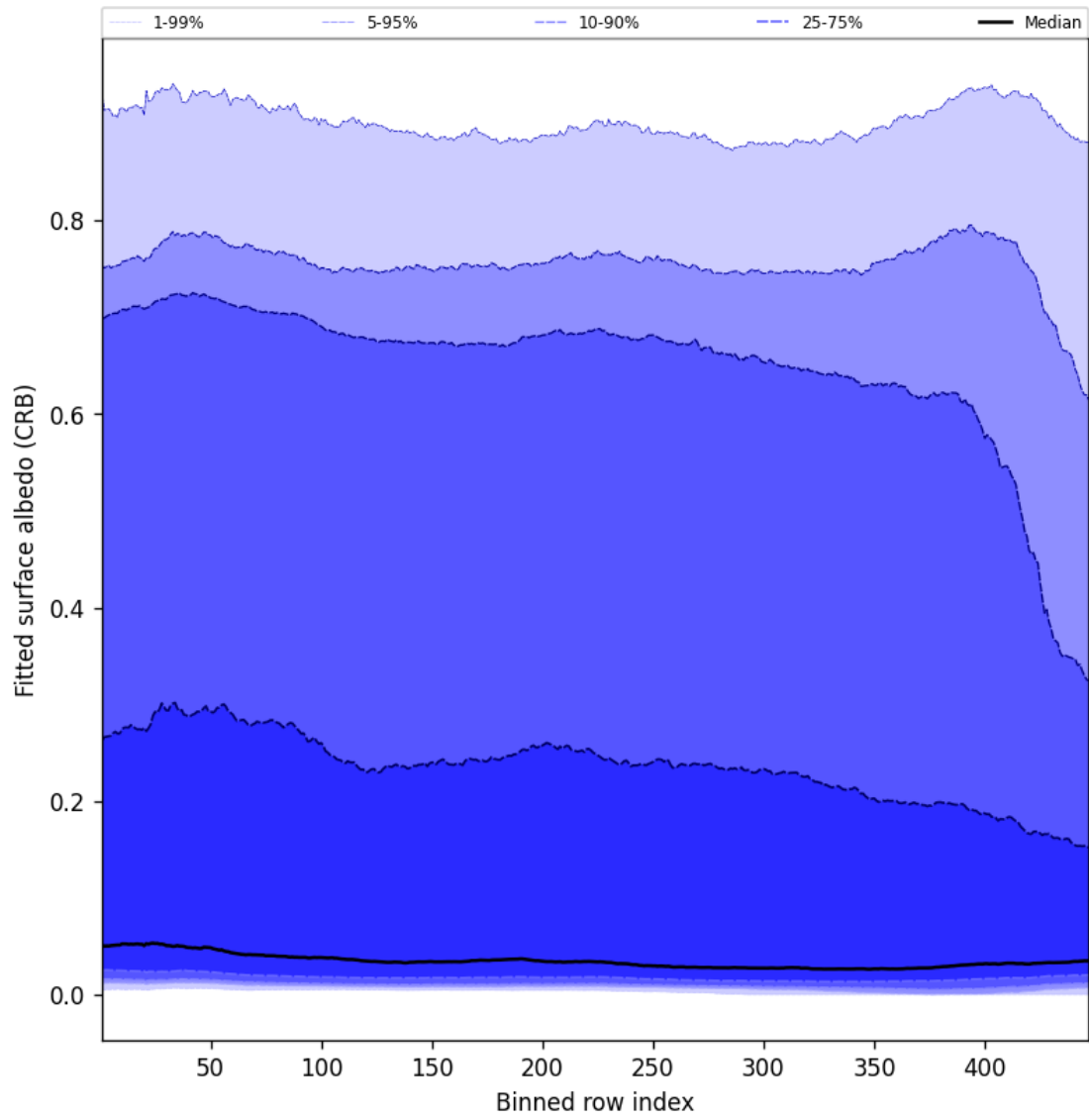
Figure 62: Along track statistics of “Fitted surface albedo (CRB)” for 2024-10-01 to 2024-10-03
