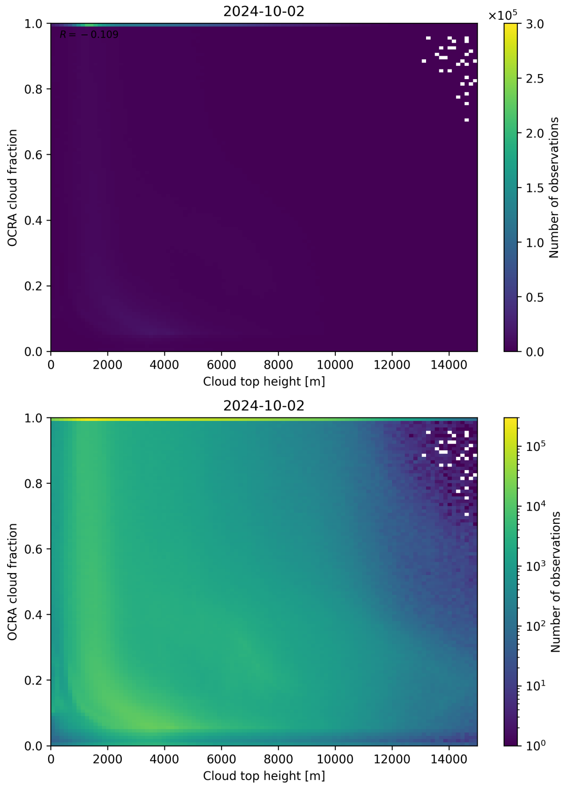
Figure 87: Scatter density plot of “Cloud top height” against “OCRA cloud fraction” for 2024-10-01 to 2024-10-03.
