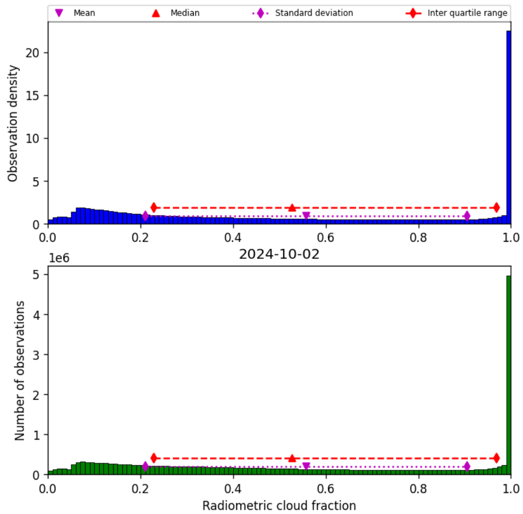
Figure 39: Histogram of “Radiometric cloud fraction” for 2024-10-01 to 2024-10-03
