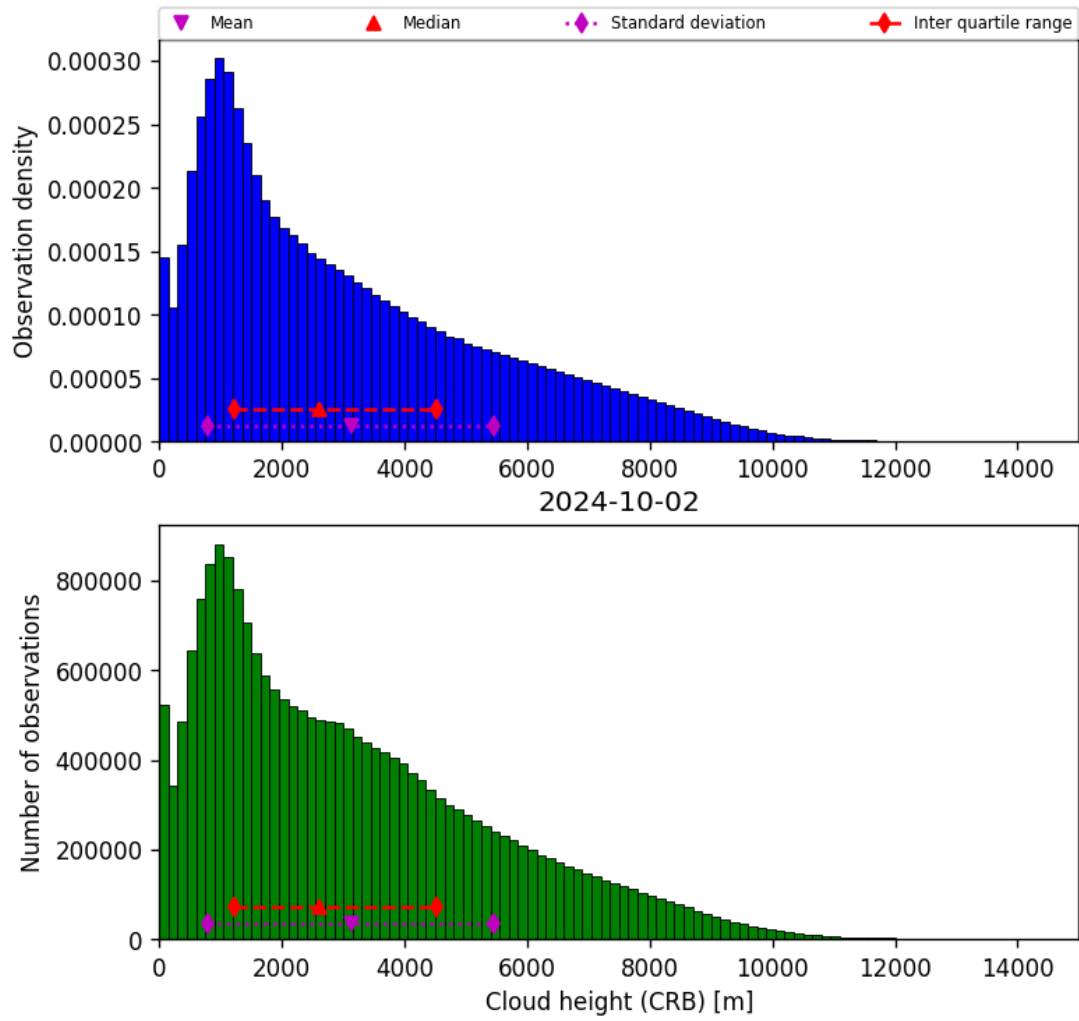
Figure 43: Histogram of “Cloud height (CRB)” for 2024-10-01 to 2024-10-03
