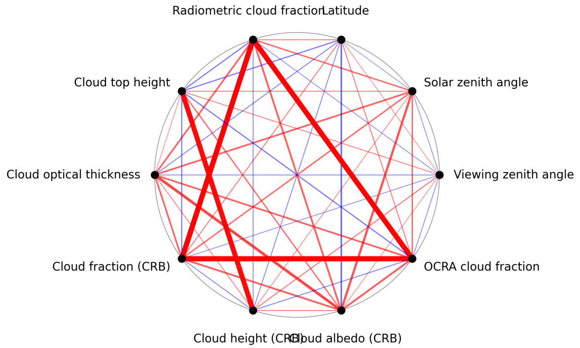
Figure 1: Map of correlation graph for 2024-10-01 to 2024-10-03.
