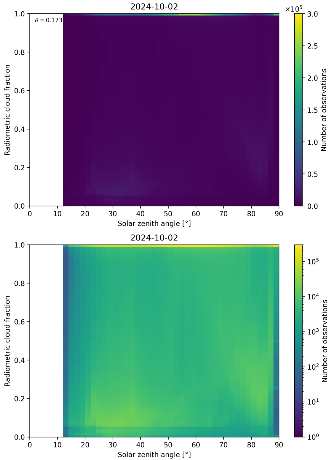
Figure 99: Scatter density plot of “Solar zenith angle” against “Radiometric cloud fraction” for 2024-10-01 to 2024-10-03.
