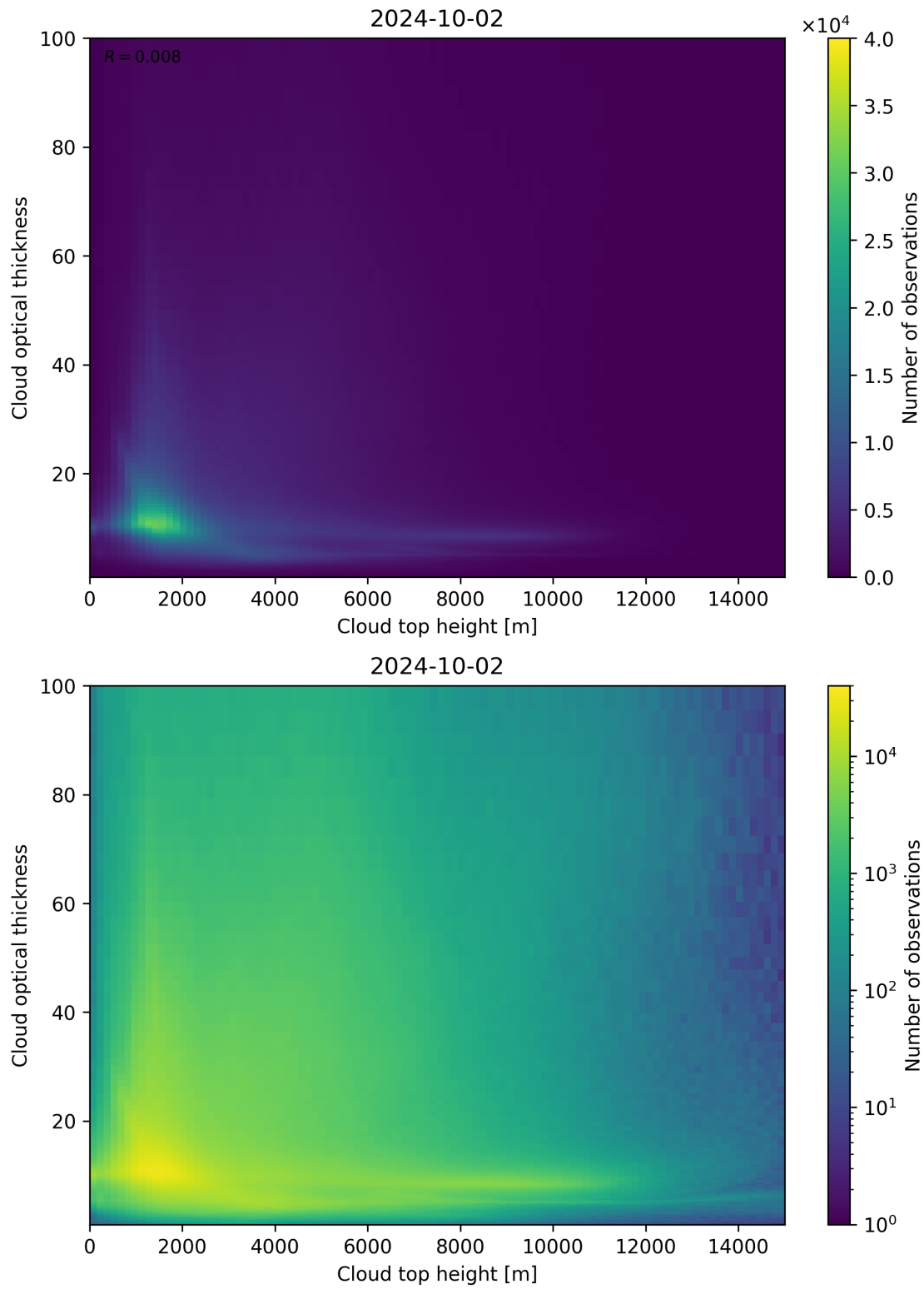
Figure 90: Scatter density plot of “Cloud top height” against “Cloud optical thickness” for 2024-10-01 to 2024-10-03.
