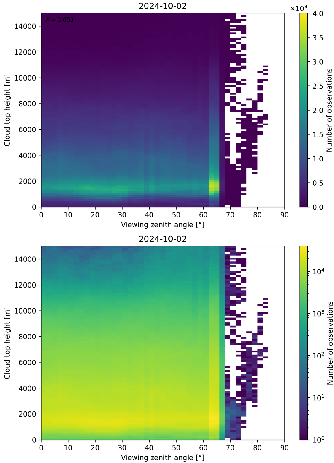
Figure 112: Scatter density plot of “Viewing zenith angle” against “Cloud top height” for 2024-10-01 to 2024-10-03.
