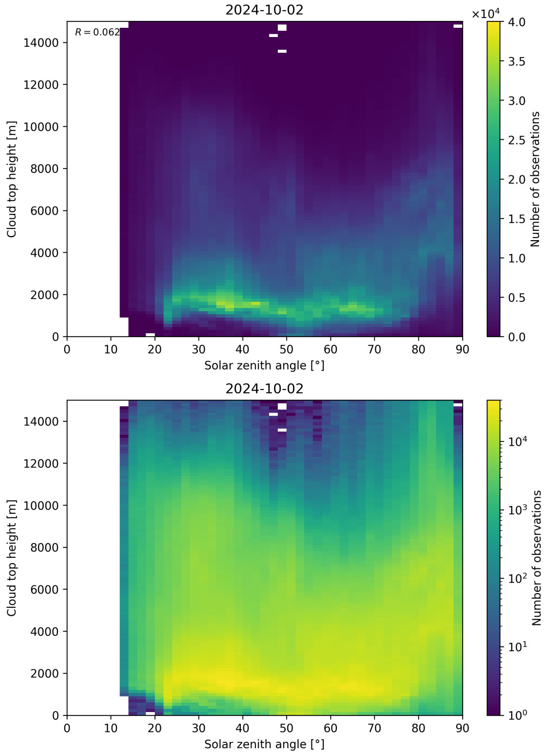
Figure 104: Scatter density plot of “Solar zenith angle” against “Cloud top height” for 2024-10-01 to 2024-10-03.
