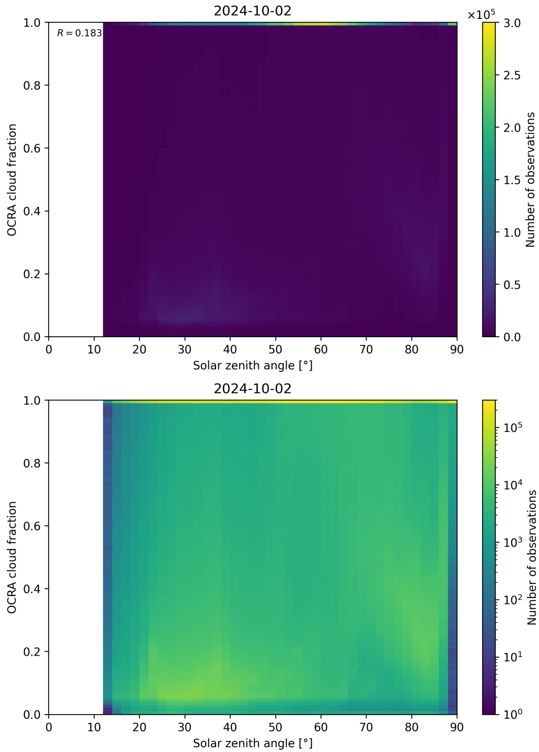
Figure 100: Scatter density plot of “Solar zenith angle” against “OCRA cloud fraction” for 2024-10-01 to 2024-10-03.
