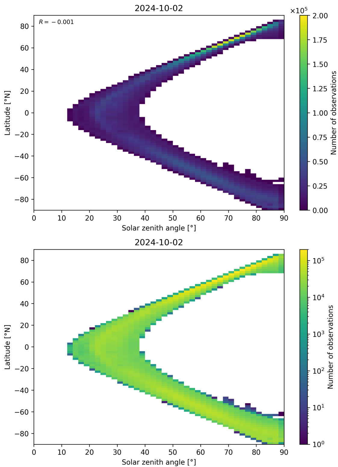
Figure 105: Scatter density plot of “Solar zenith angle” against “Latitude” for 2024-10-01 to 2024-10-03.
