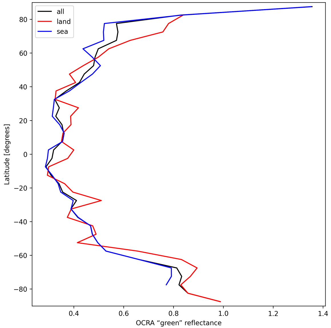
Figure 36: Zonal average of “OCRA “green” reflectance” for 2024-10-01 to 2024-10-03.
