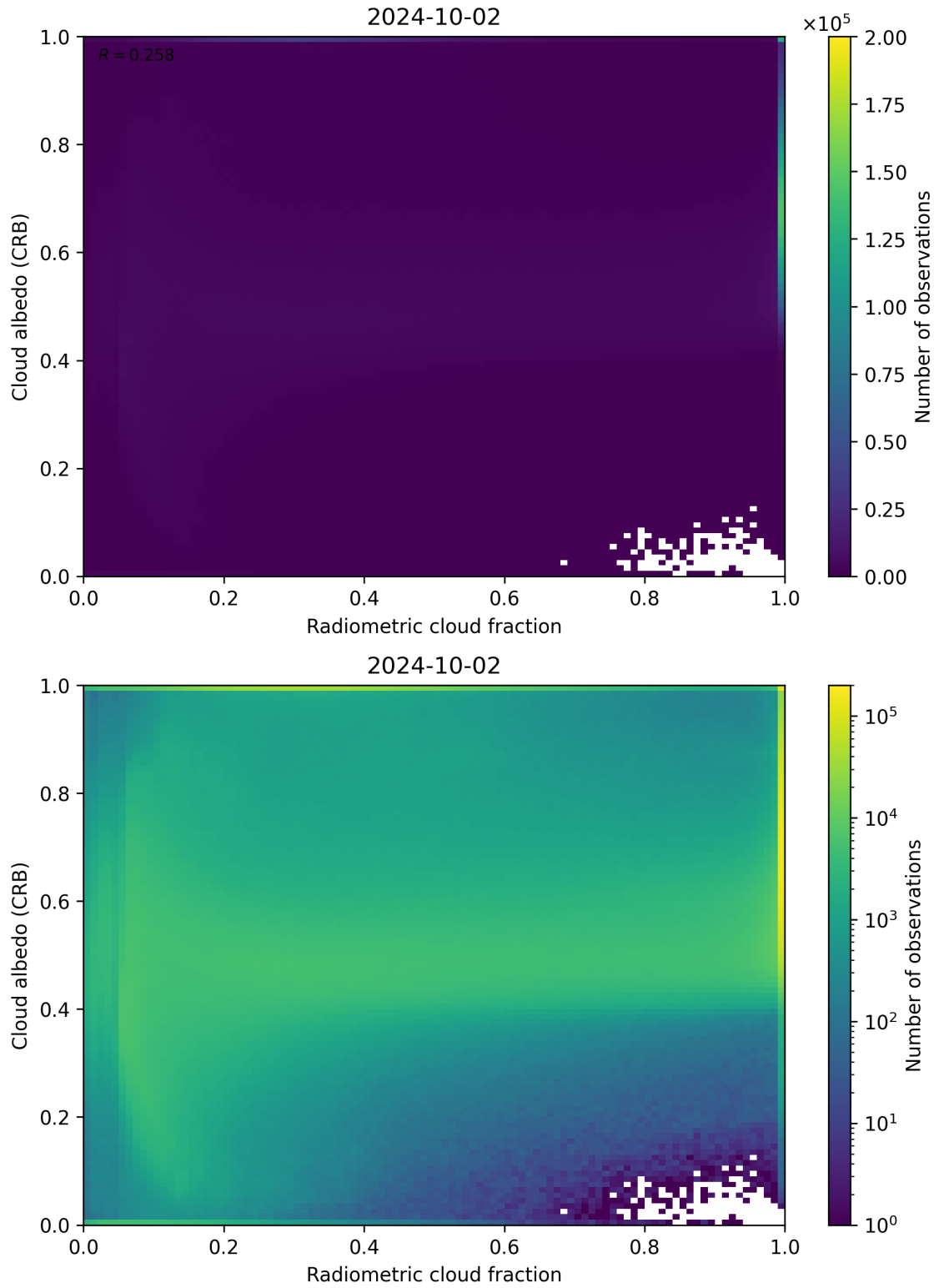
Figure 71: Scatter density plot of “Radiometric cloud fraction” against “Cloud albedo (CRB)” for 2024-10-01 to 2024-10-03.
