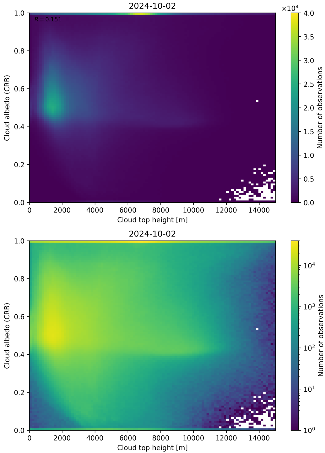
Figure 86: Scatter density plot of “Cloud top height” against “Cloud albedo (CRB)” for 2024-10-01 to 2024-10-03.
