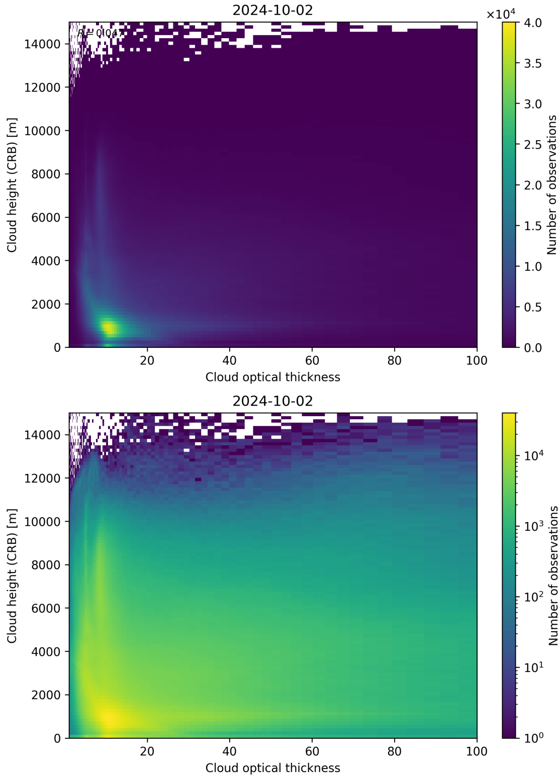
Figure 85: Scatter density plot of “Cloud optical thickness” against “Cloud height (CRB)” for 2024-10-01 to 2024-10-03.
