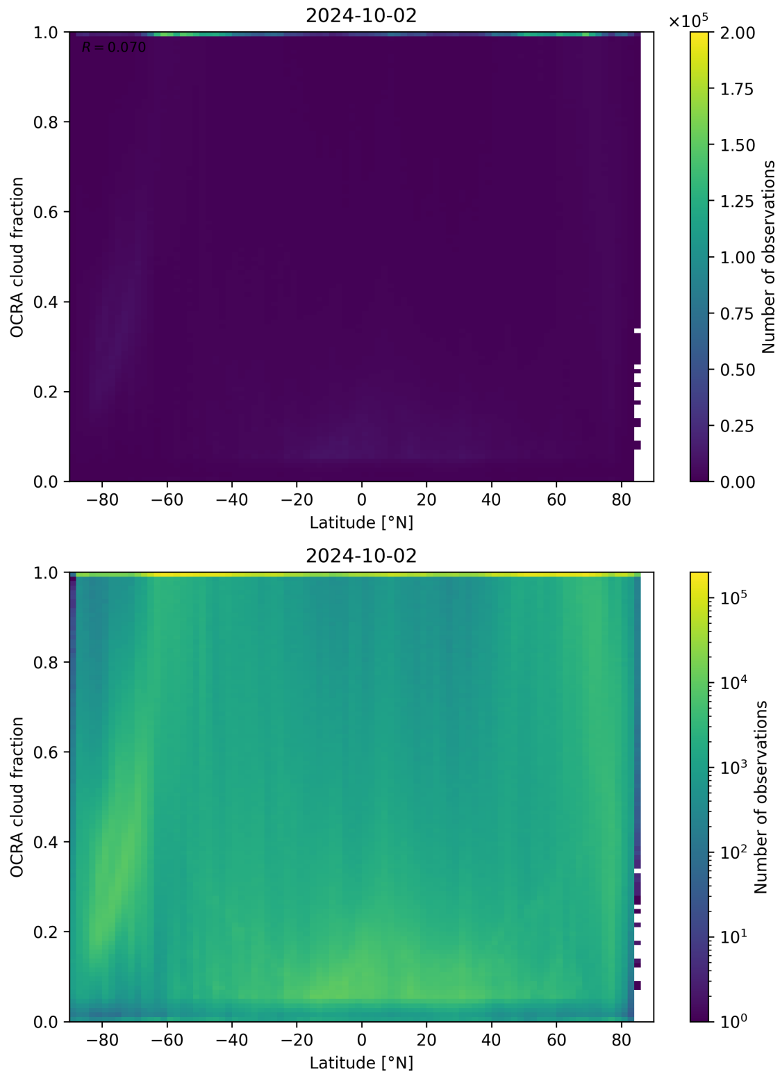
Figure 93: Scatter density plot of “Latitude” against “OCRA cloud fraction” for 2024-10-01 to 2024-10-03.
