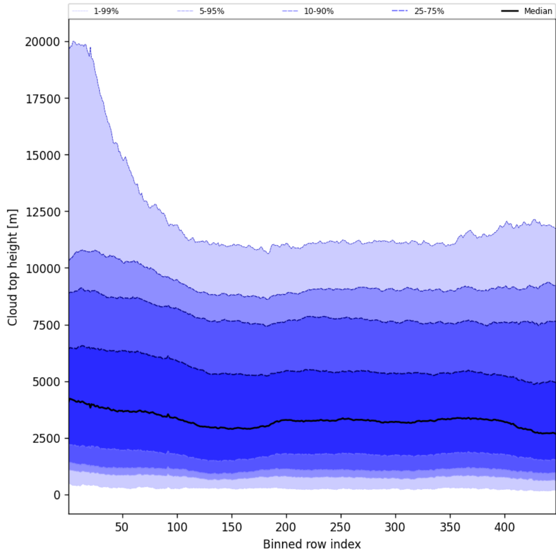
Figure 56: Along track statistics of “Cloud top height” for 2024-10-01 to 2024-10-03
