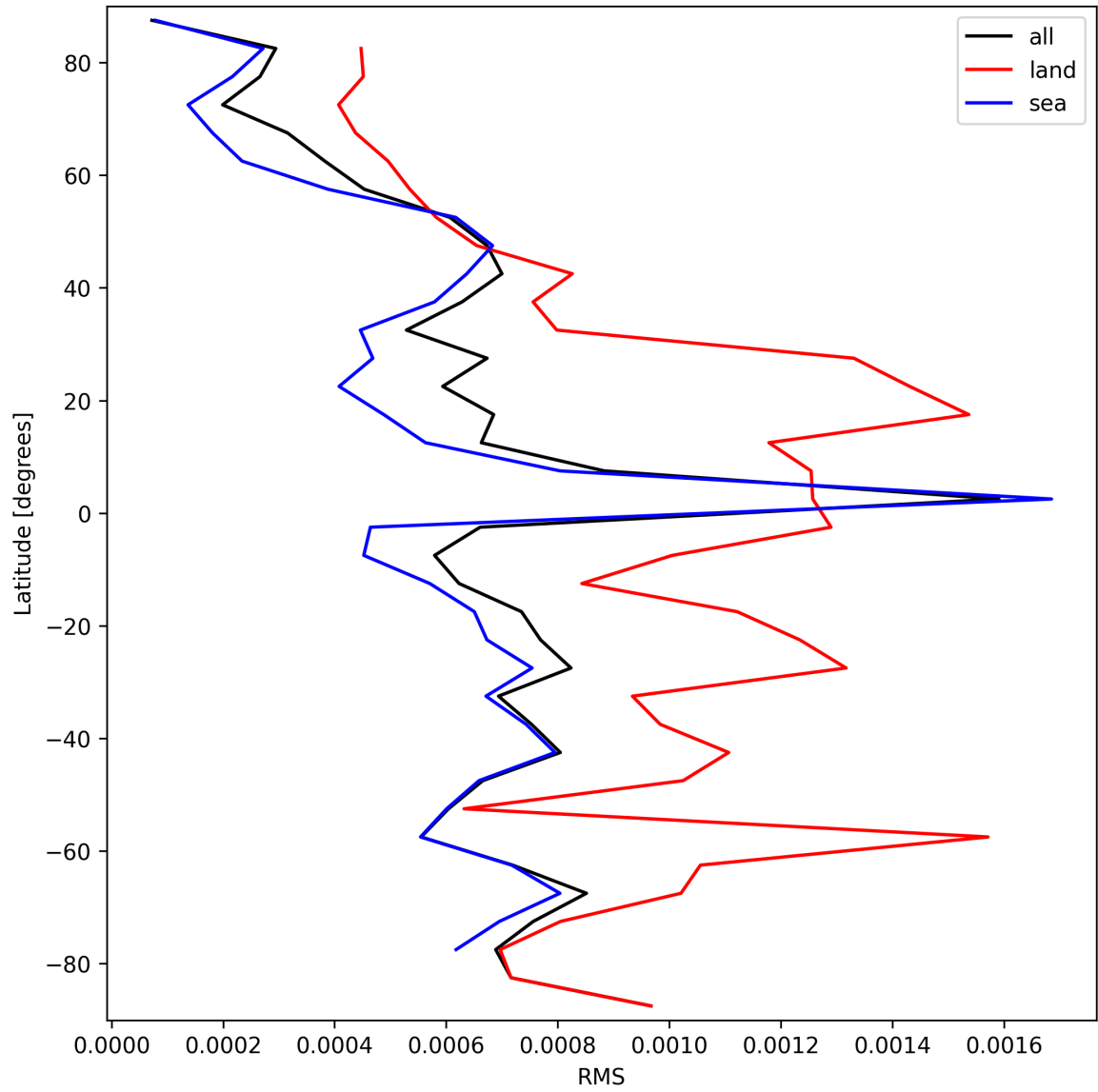
Figure 31: Zonal average of “RMS” for 2024-10-01 to 2024-10-03.
