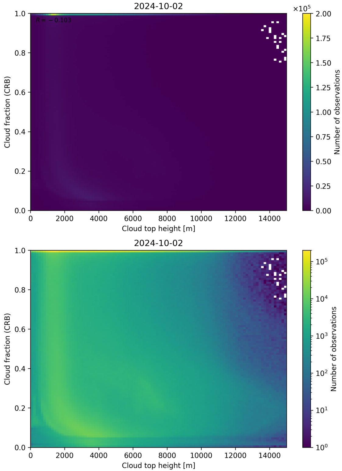
Figure 88: Scatter density plot of “Cloud top height” against “Cloud fraction (CRB)” for 2024-10-01 to 2024-10-03.
