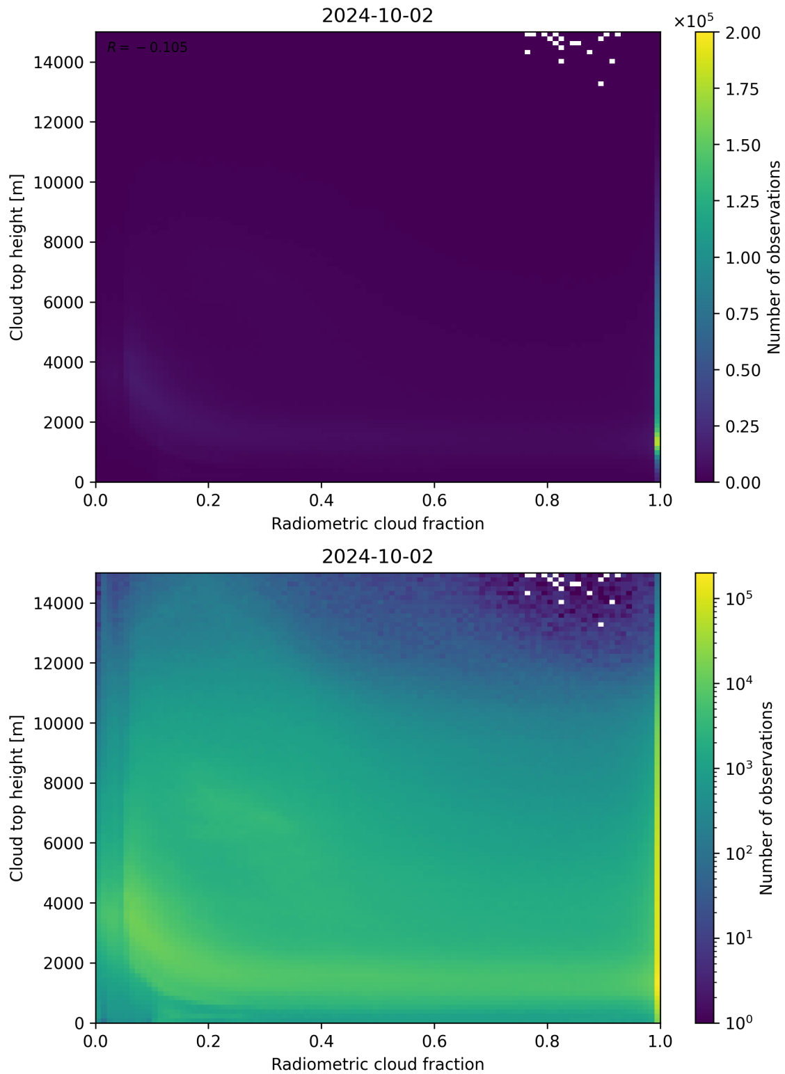
Figure 76: Scatter density plot of “Radiometric cloud fraction” against “Cloud top height” for 2024-10-01 to 2024-10-03.
