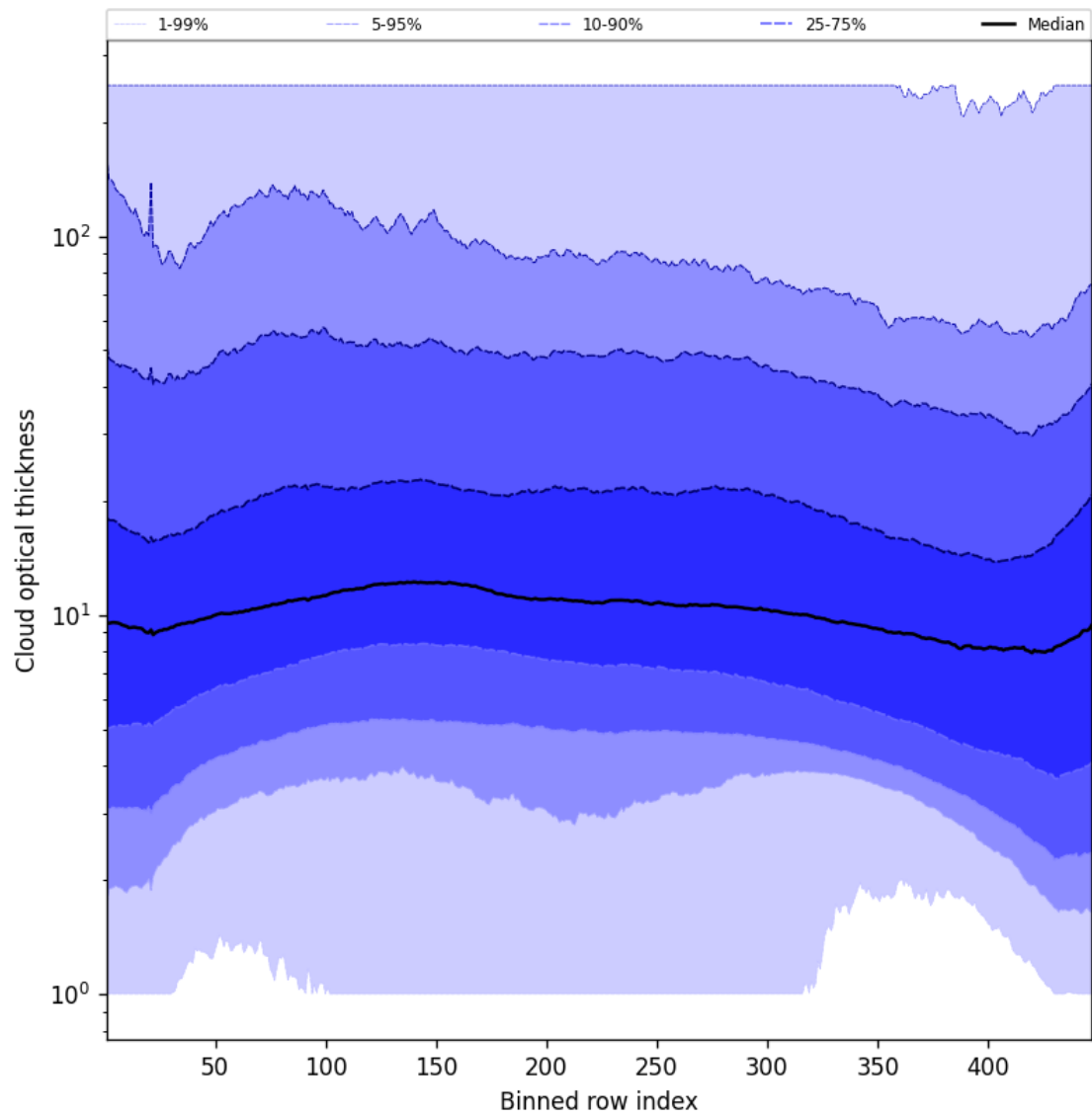
Figure 57: Along track statistics of “Cloud optical thickness” for 2024-10-01 to 2024-10-03
