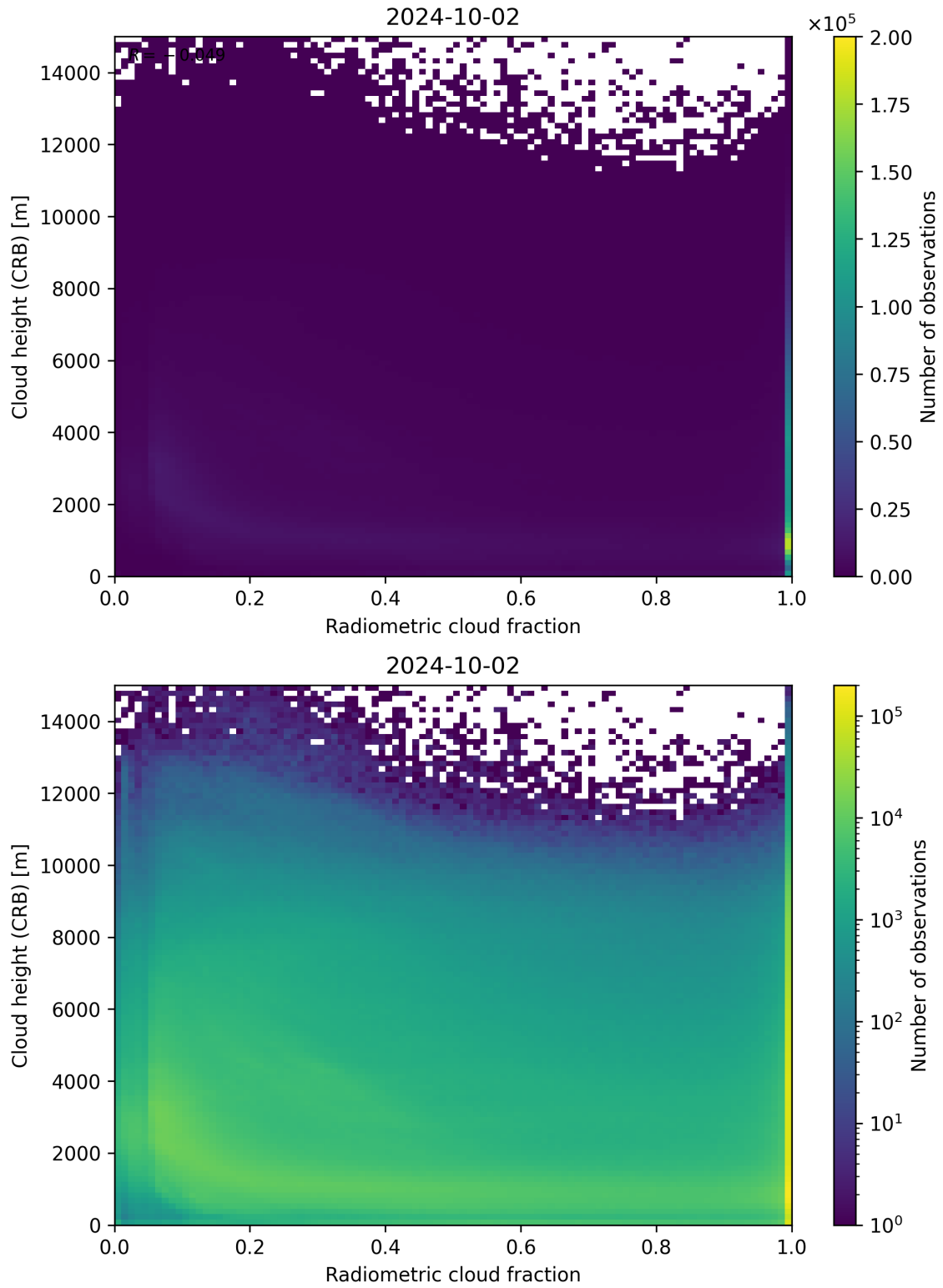
Figure 74: Scatter density plot of “Radiometric cloud fraction” against “Cloud height (CRB)” for 2024-10-01 to 2024-10-03.
