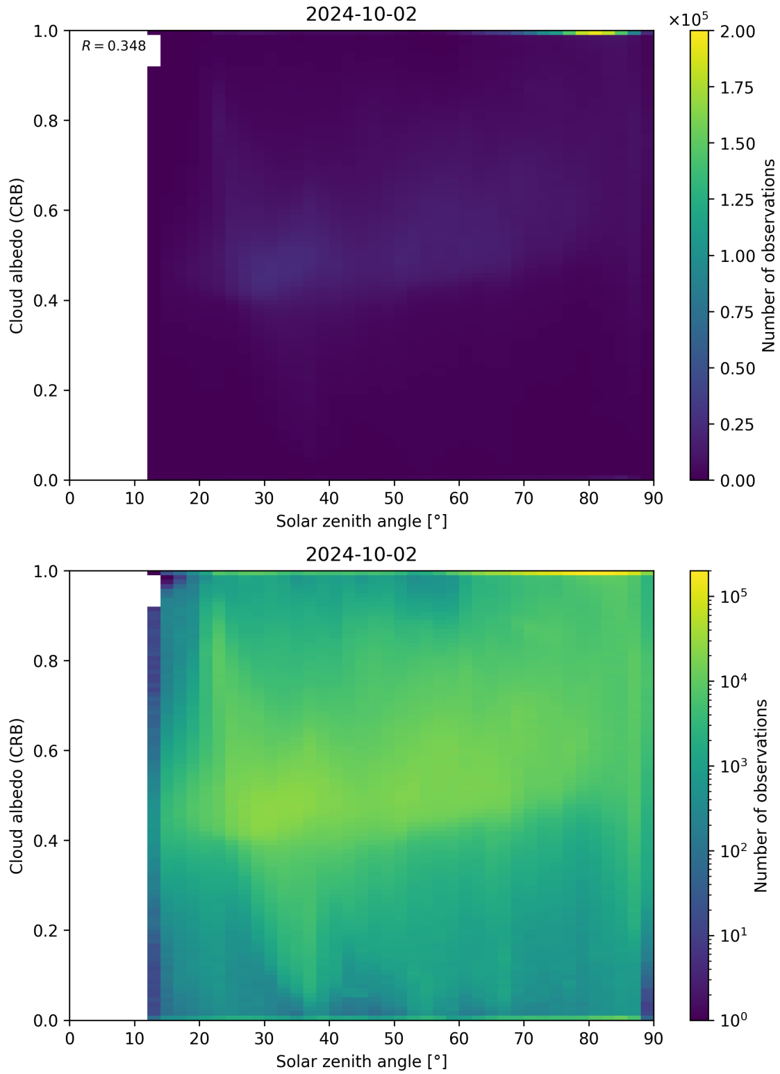
Figure 98: Scatter density plot of “Solar zenith angle” against “Cloud albedo (CRB)” for 2024-10-01 to 2024-10-03.
