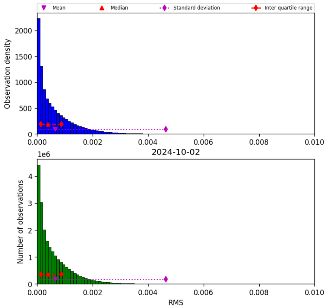
Figure 47: Histogram of “RMS” for 2024-10-01 to 2024-10-03
