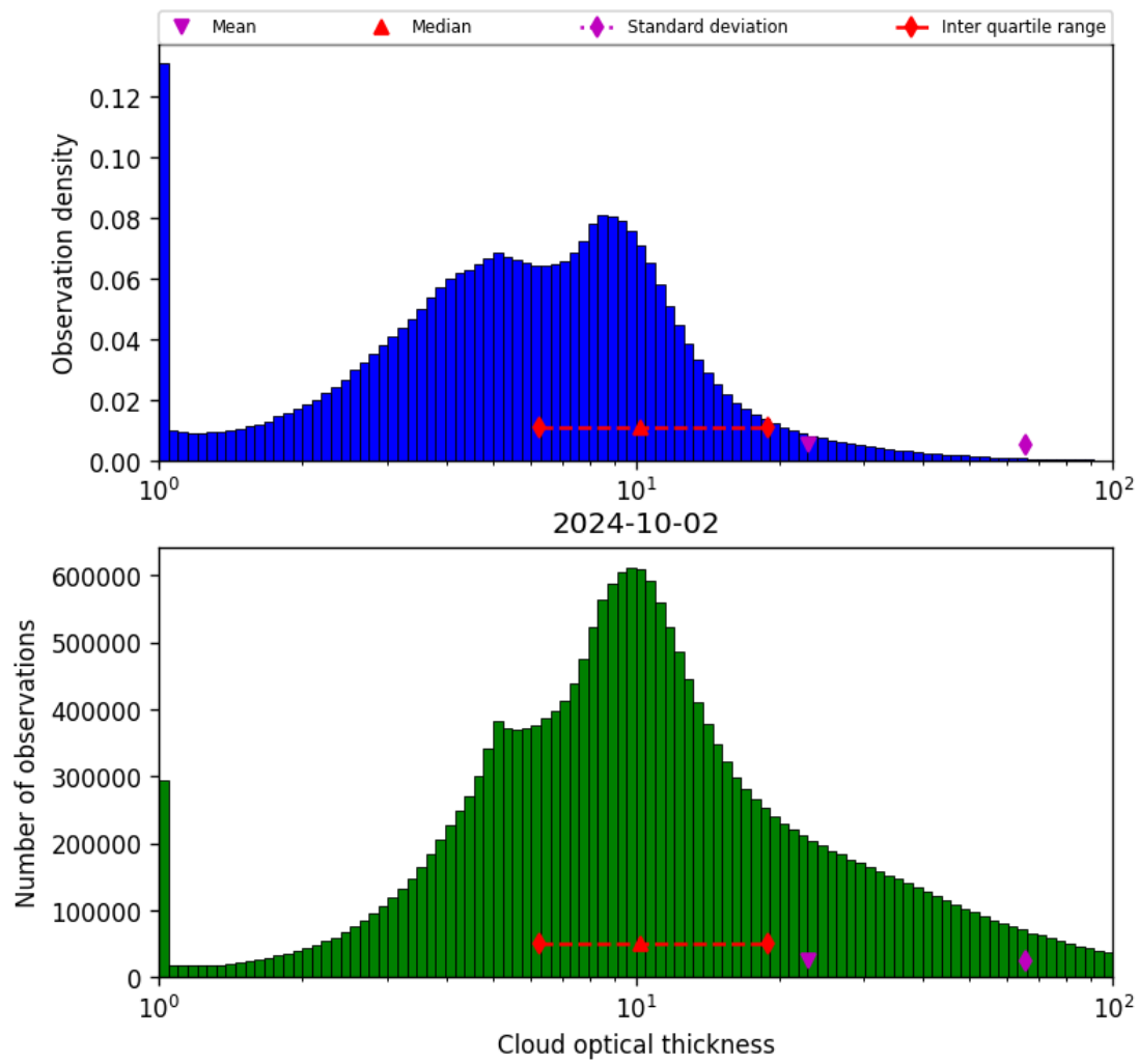
Figure 41: Histogram of “Cloud optical thickness” for 2024-10-01 to 2024-10-03
