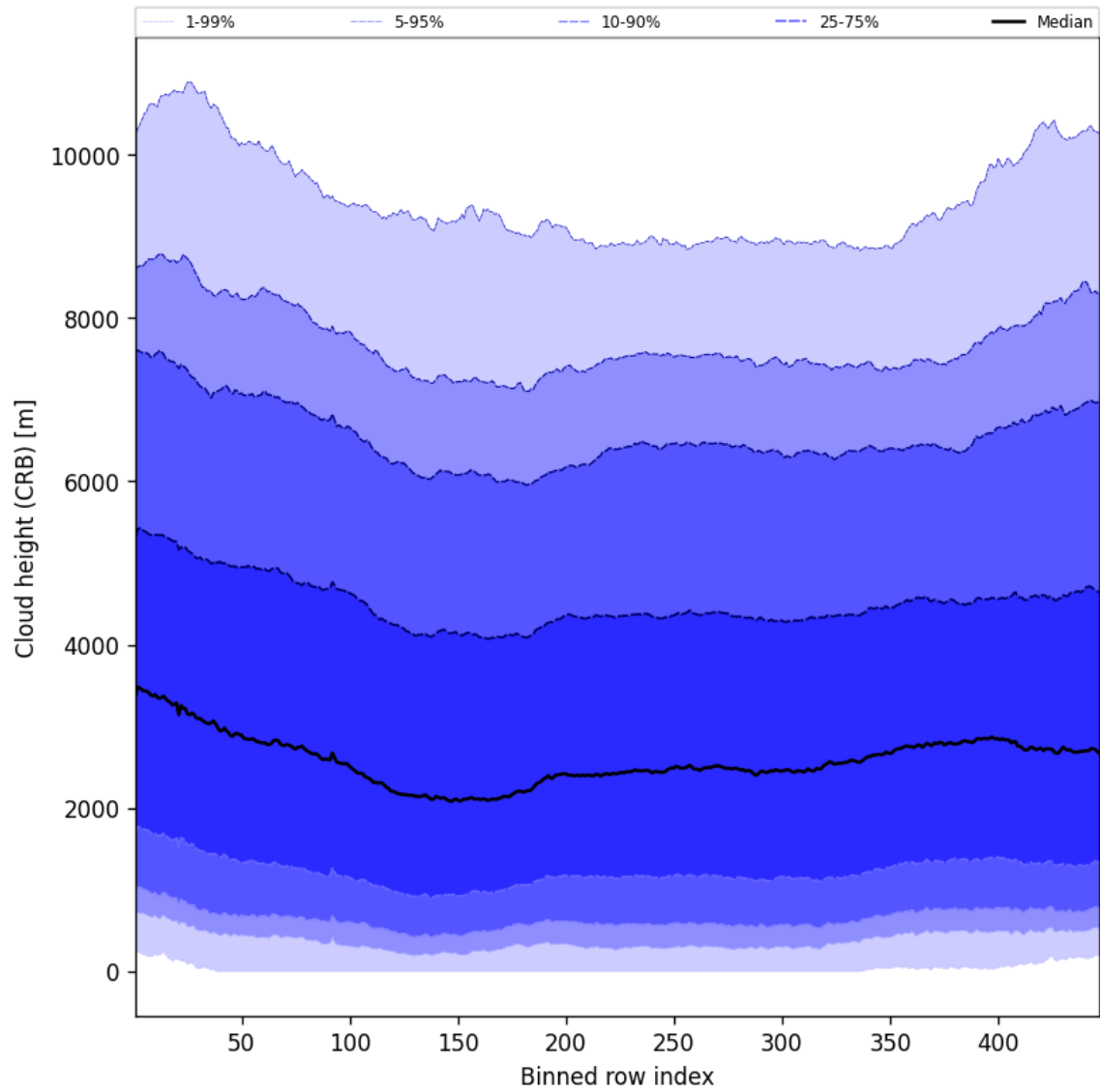
Figure 59: Along track statistics of “Cloud height (CRB)” for 2024-10-01 to 2024-10-03
