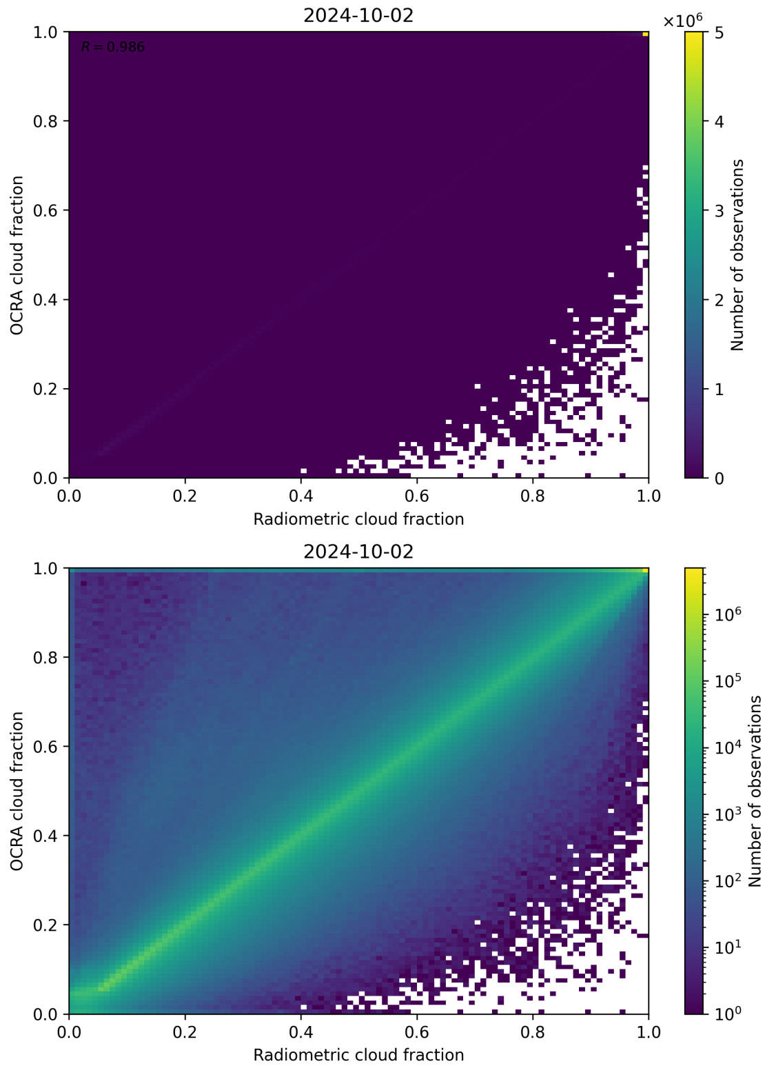
Figure 72: Scatter density plot of “Radiometric cloud fraction” against “OCRA cloud fraction” for 2024-10-01 to 2024-10-03.
