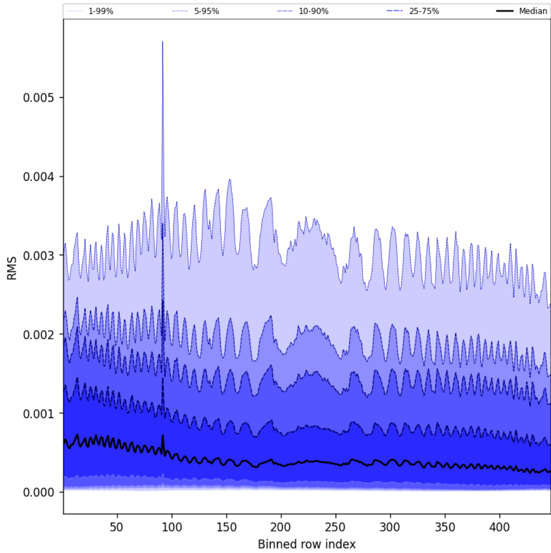
Figure 63: Along track statistics of “RMS” for 2024-10-01 to 2024-10-03
