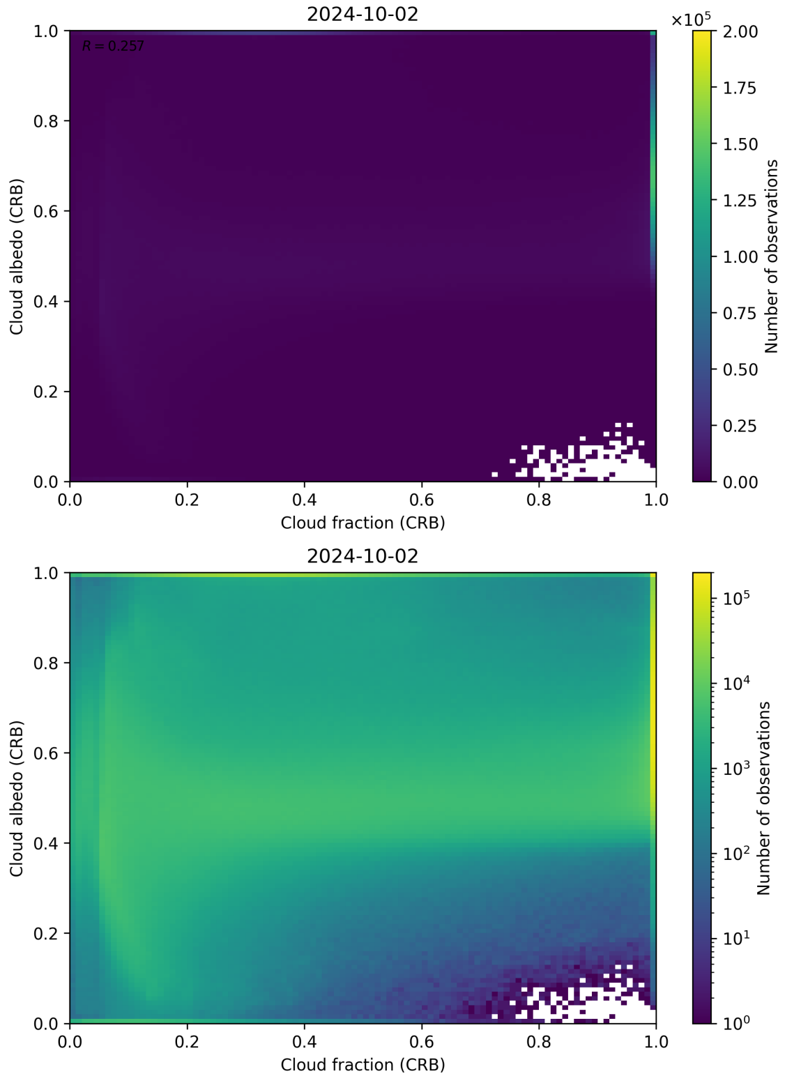
Figure 77: Scatter density plot of “Cloud fraction (CRB)” against “Cloud albedo (CRB)” for 2024-10-01 to 2024-10-03.
