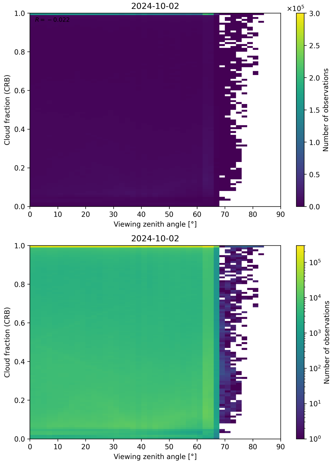
Figure 109: Scatter density plot of “Viewing zenith angle” against “Cloud fraction (CRB)” for 2024-10-01 to 2024-10-03.
