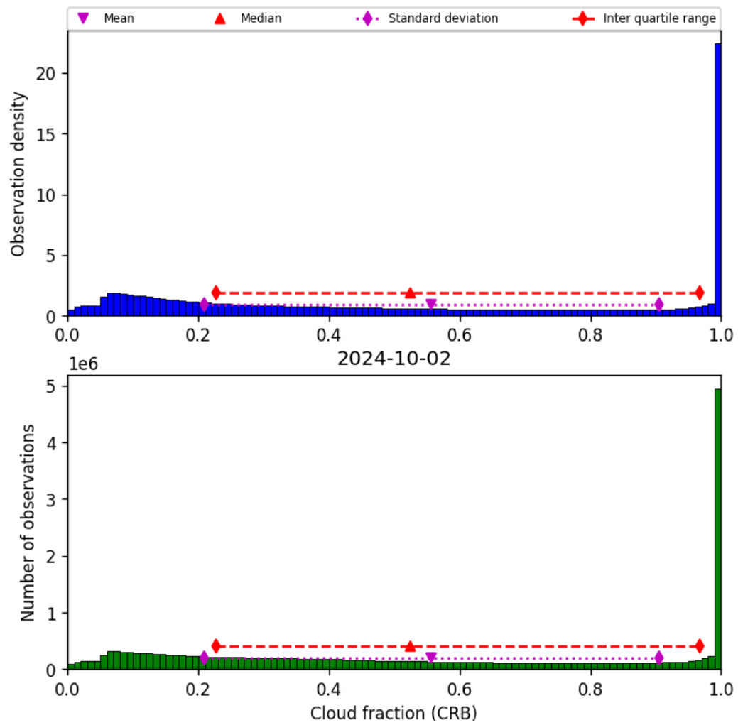
Figure 42: Histogram of “Cloud fraction (CRB)” for 2024-10-01 to 2024-10-03
