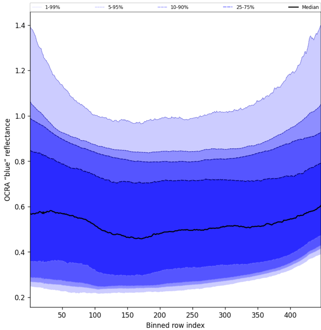
Figure 67: Along track statistics of “OCRA “blue” reflectance” for 2024-10-01 to 2024-10-03
