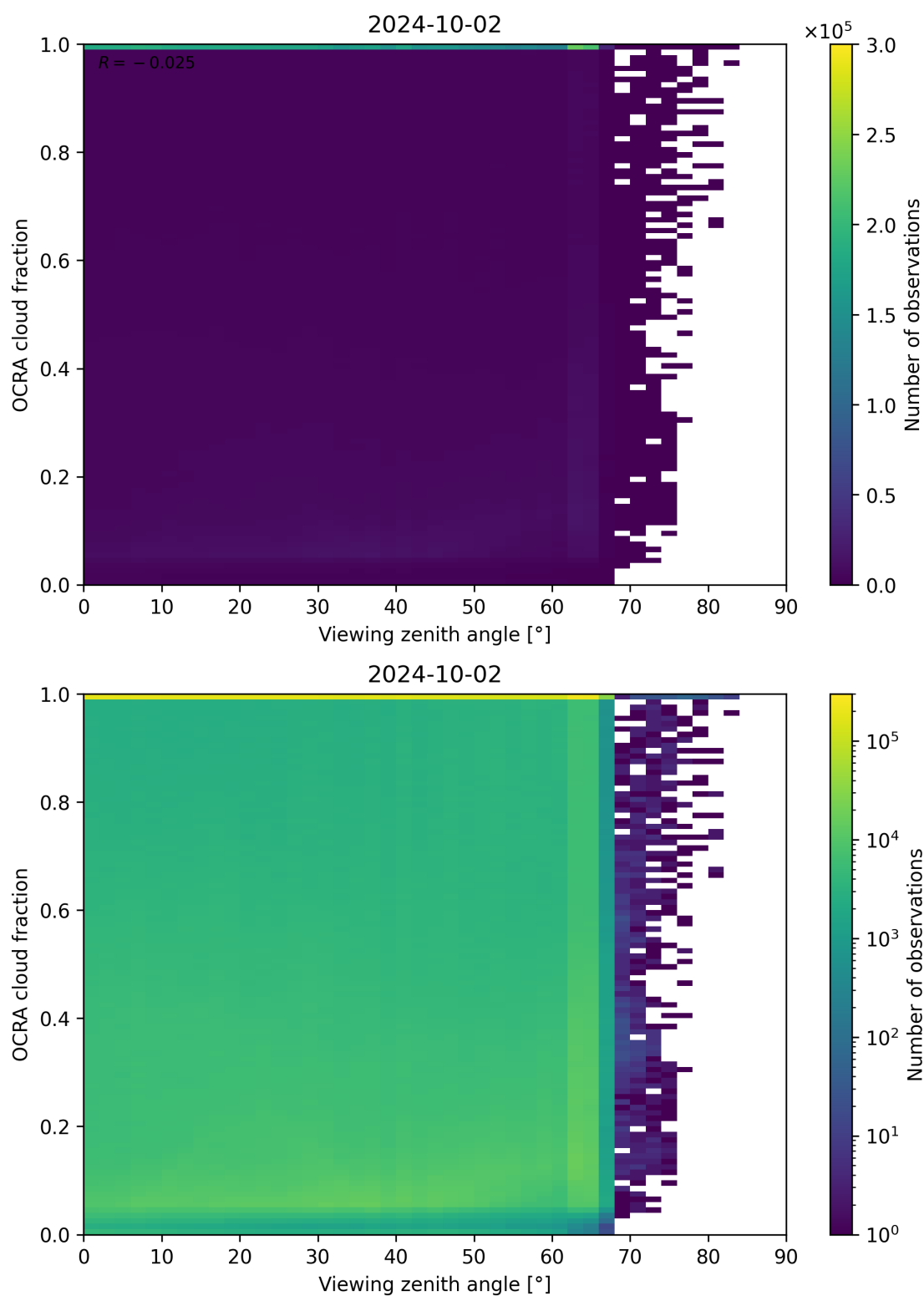
Figure 108: Scatter density plot of “Viewing zenith angle” against “OCRA cloud fraction” for 2024-10-01 to 2024-10-03.
