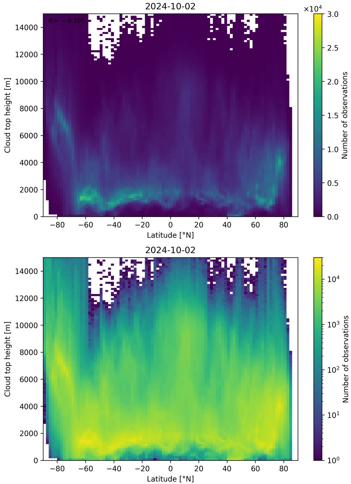
Figure 97: Scatter density plot of “Latitude” against “Cloud top height” for 2024-10-01 to 2024-10-03.
