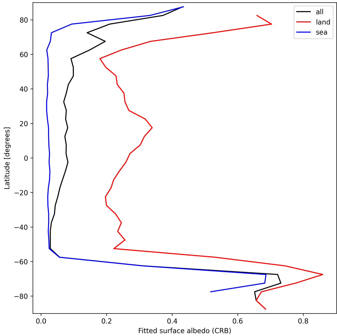
Figure 30: Zonal average of “Fitted surface albedo (CRB)” for 2024-10-01 to 2024-10-03.
