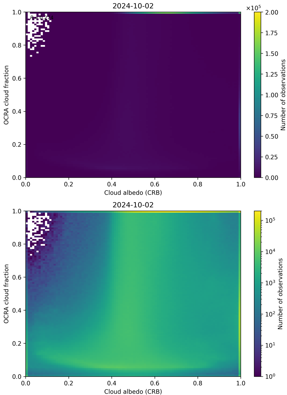
Figure 70: Scatter density plot of “Cloud albedo (CRB)” against “OCRA cloud fraction” for 2024-10-01 to 2024-10-03.
