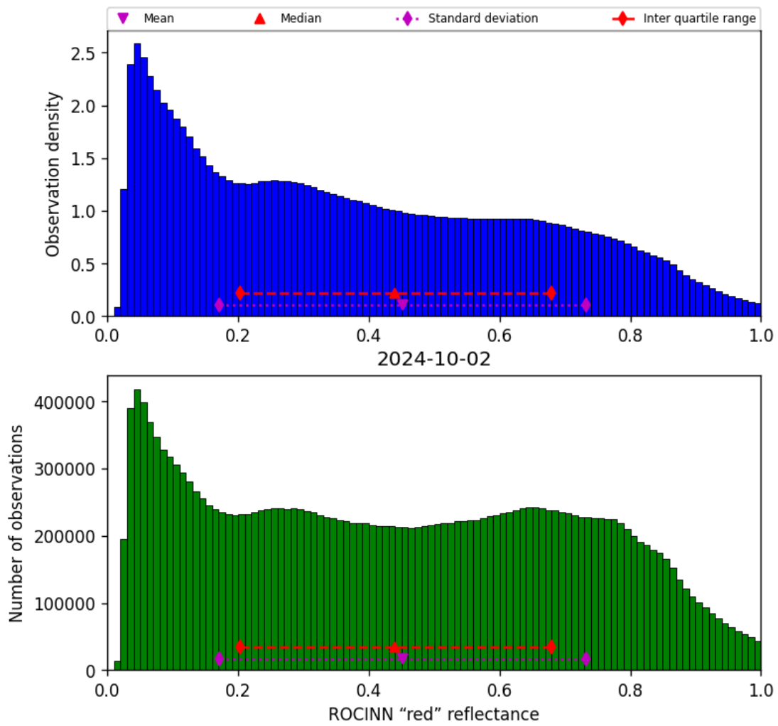
Figure 53: Histogram of “ROCINN “red” reflectance” for 2024-10-01 to 2024-10-03
