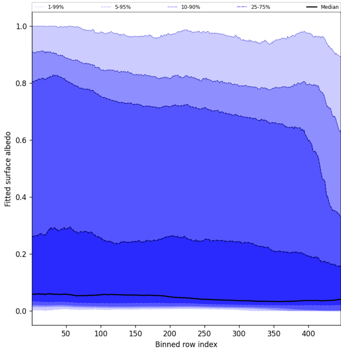
Figure 61: Along track statistics of “Fitted surface albedo” for 2024-10-01 to 2024-10-03
