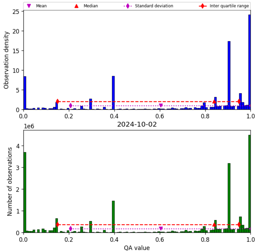
Figure 38: Histogram of “QA value” for 2024-10-01 to 2024-10-03
