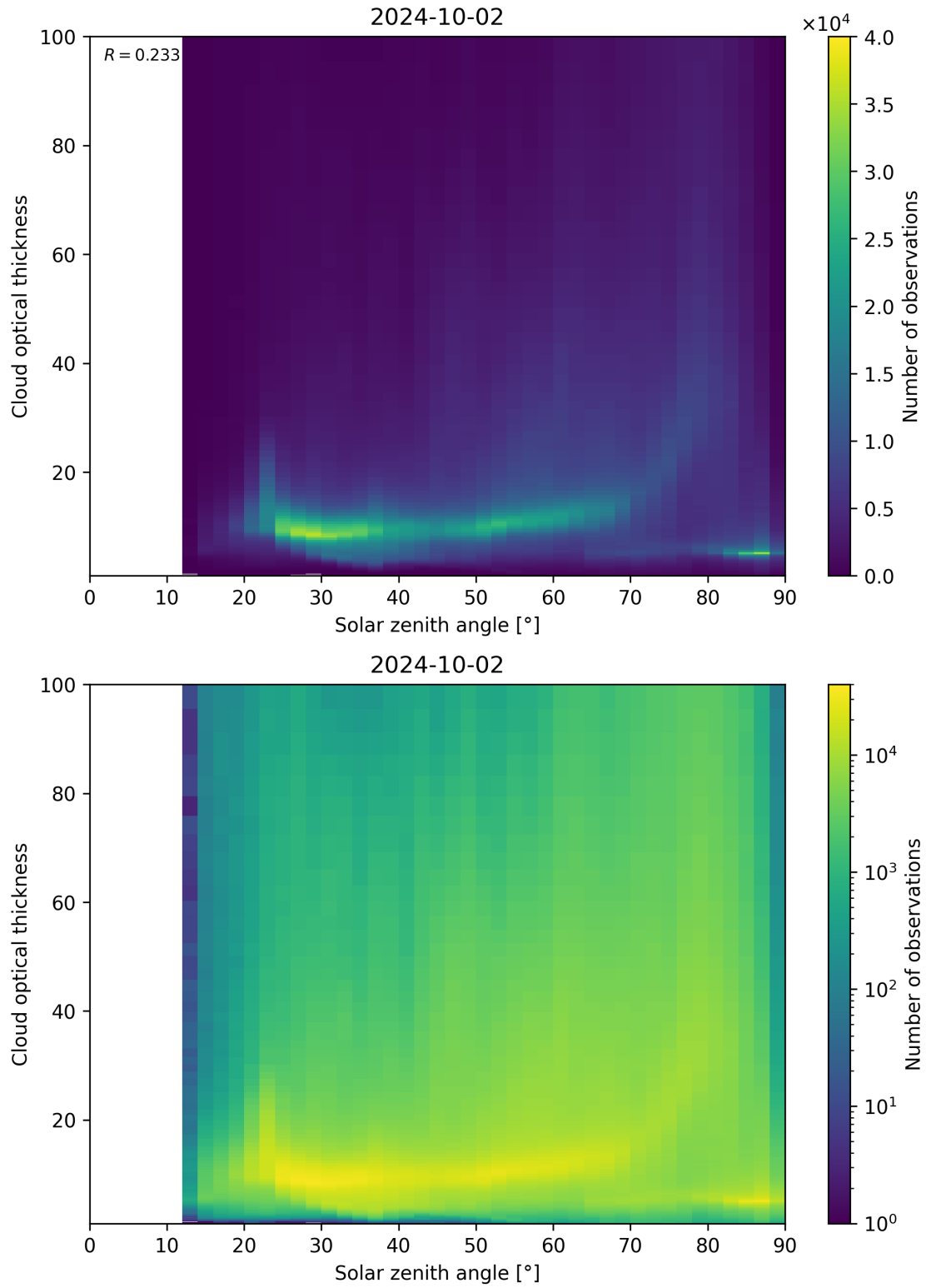
Figure 103: Scatter density plot of “Solar zenith angle” against “Cloud optical thickness” for 2024-10-01 to 2024-10-03.
