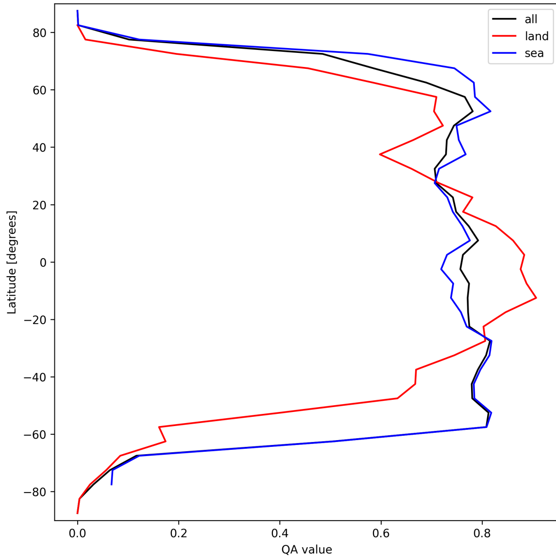
Figure 22: Zonal average of “QA value” for 2024-10-01 to 2024-10-03.
