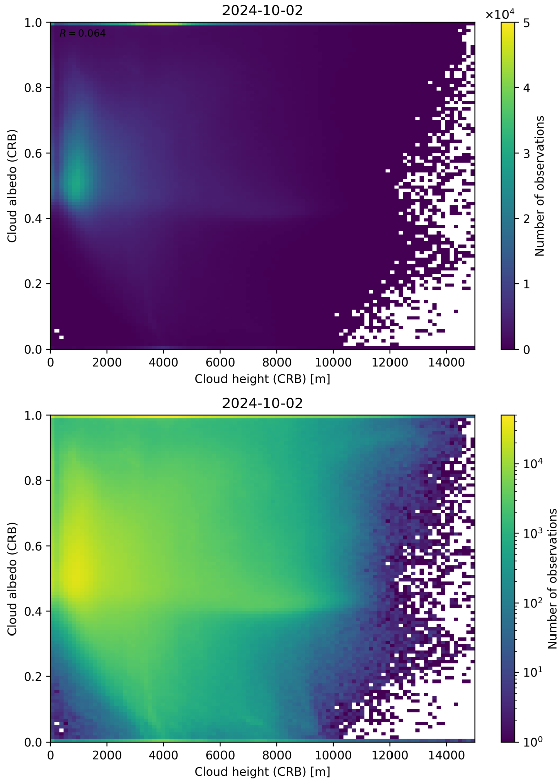
Figure 80: Scatter density plot of “Cloud height (CRB)” against “Cloud albedo (CRB)” for 2024-10-01 to 2024-10-03.
