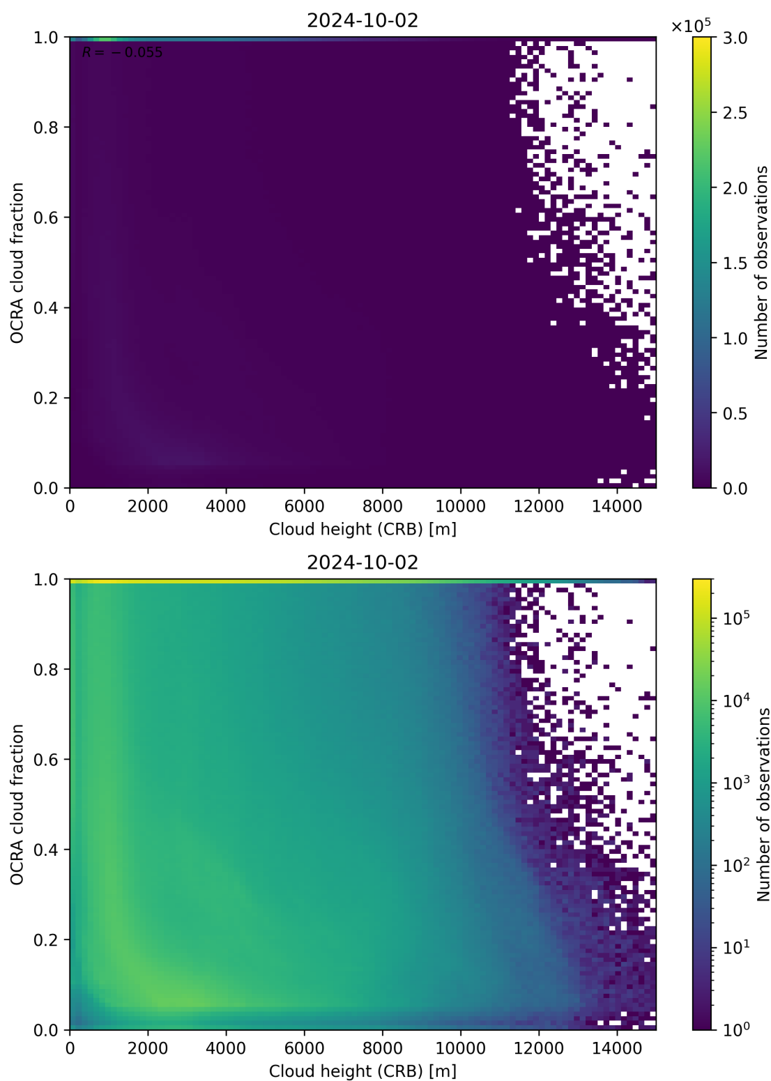
Figure 81: Scatter density plot of “Cloud height (CRB)” against “OCRA cloud fraction” for 2024-10-01 to 2024-10-03.
