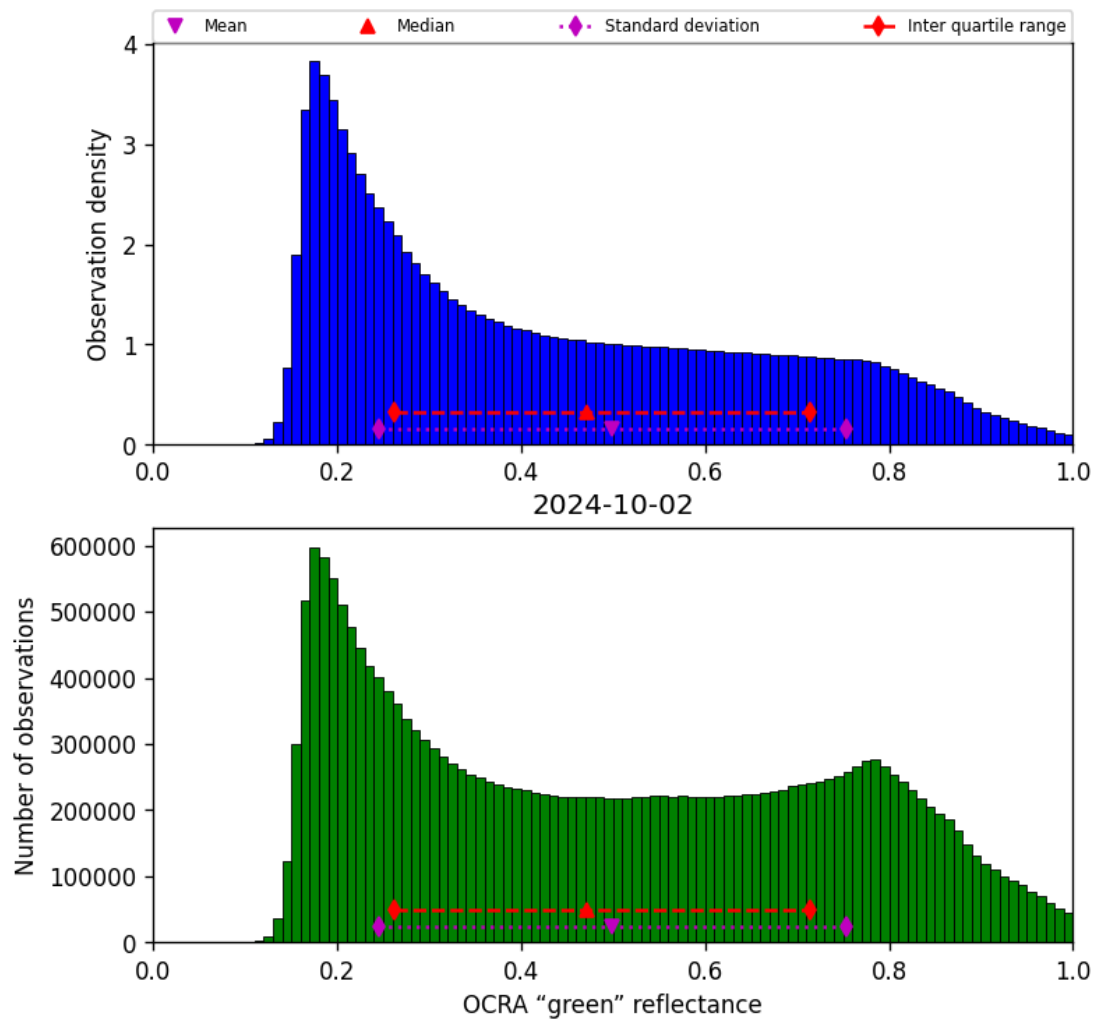
Figure 52: Histogram of “OCRA “green” reflectance” for 2024-10-01 to 2024-10-03
