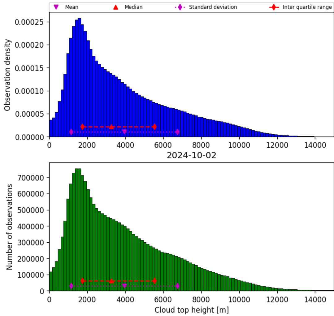
Figure 40: Histogram of “Cloud top height” for 2024-10-01 to 2024-10-03
