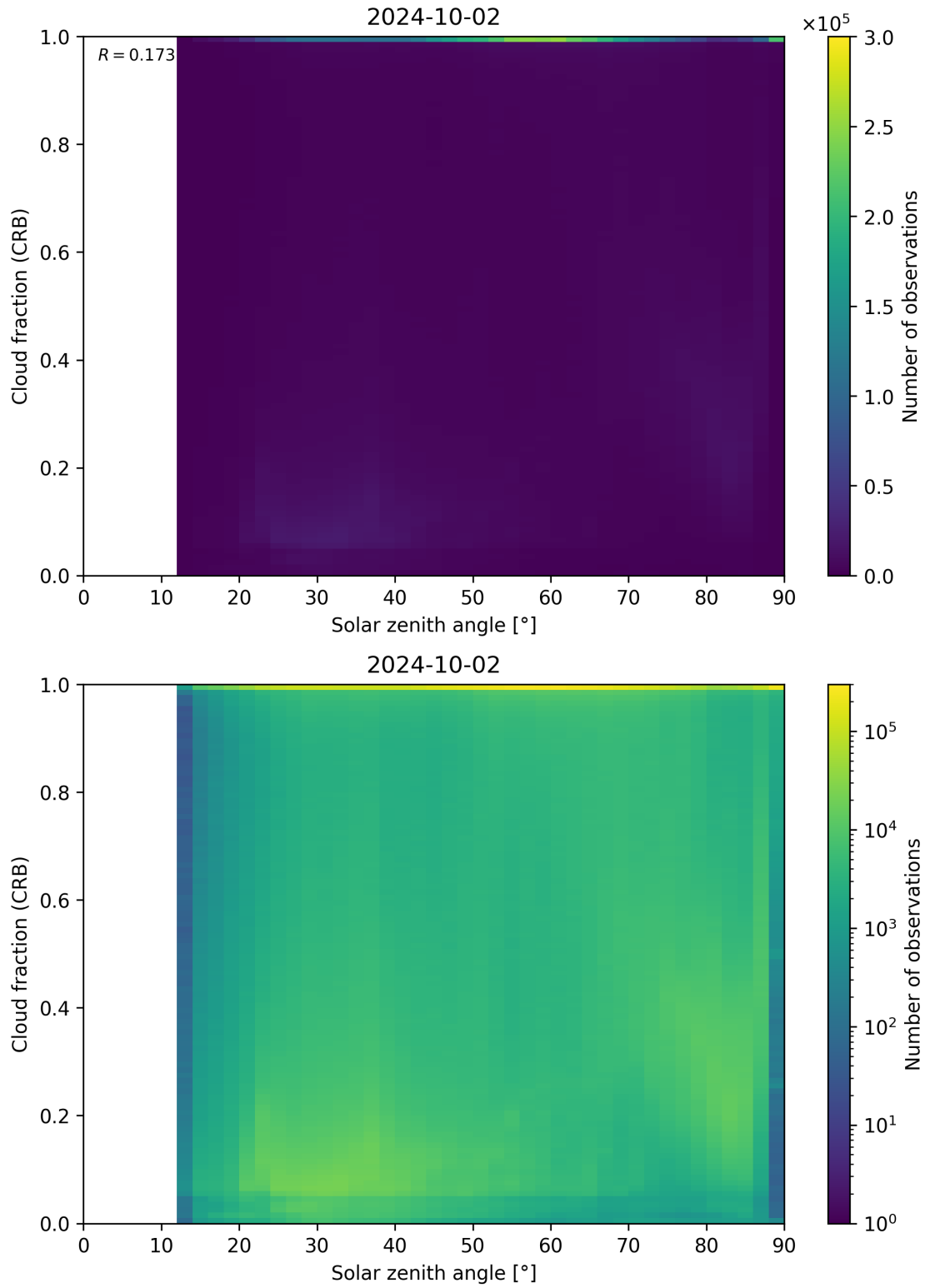
Figure 101: Scatter density plot of “Solar zenith angle” against “Cloud fraction (CRB)” for 2024-10-01 to 2024-10-03.
