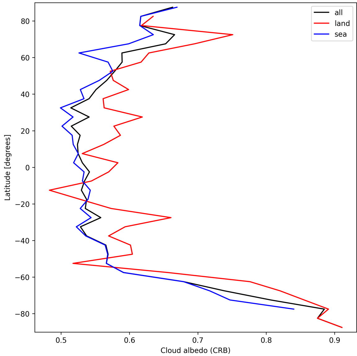
Figure 28: Zonal average of “Cloud albedo (CRB)” for 2024-10-01 to 2024-10-03.
