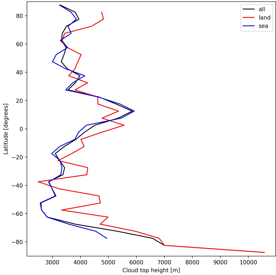
Figure 24: Zonal average of “Cloud top height” for 2024-10-01 to 2024-10-03.
