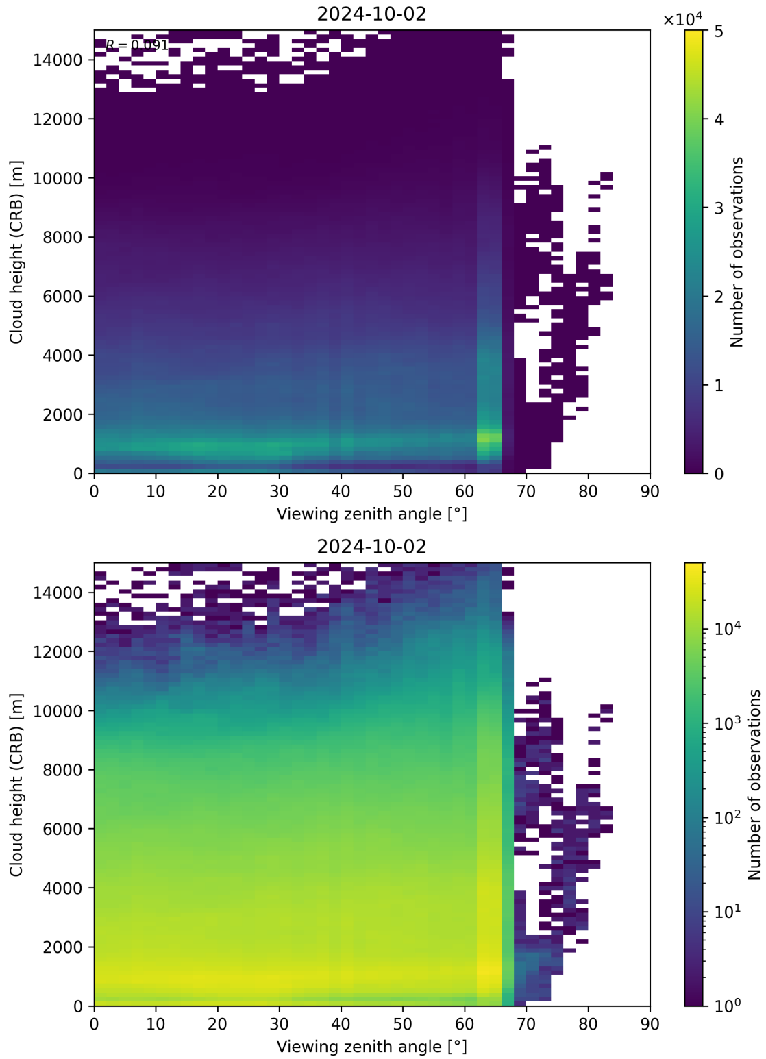
Figure 110: Scatter density plot of “Viewing zenith angle” against “Cloud height (CRB)” for 2024-10-01 to 2024-10-03.
