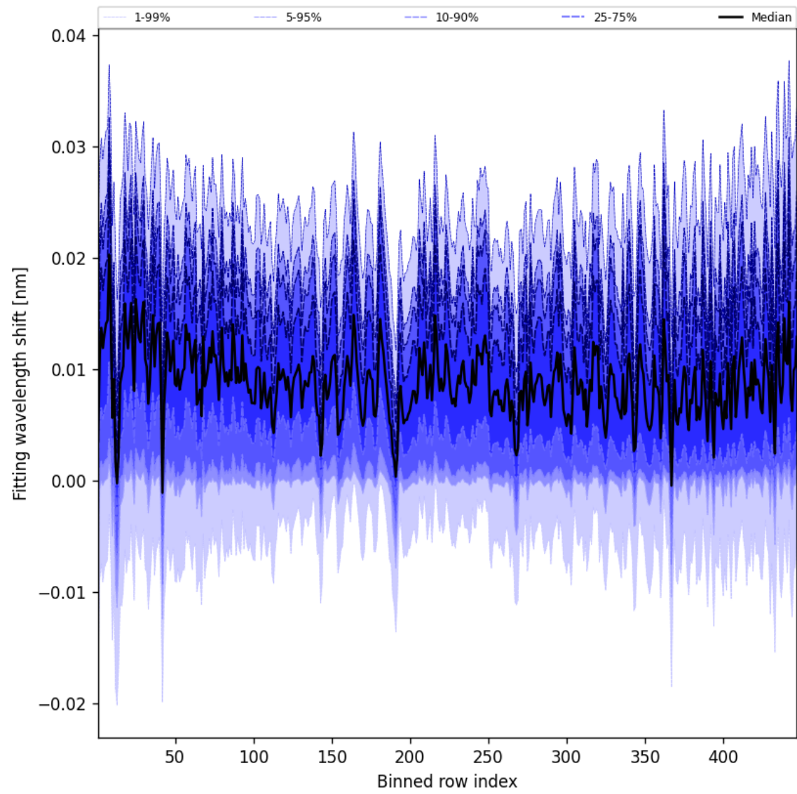
Figure 65: Along track statistics of “Fitting wavelength shift” for 2024-10-01 to 2024-10-03
