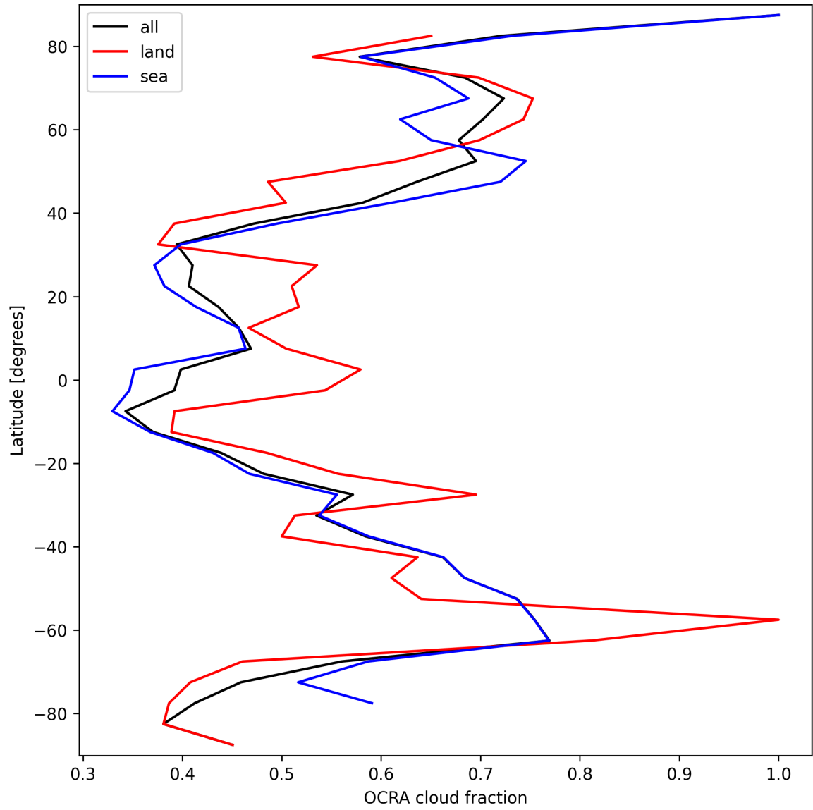
Figure 34: Zonal average of “OCRA cloud fraction” for 2024-10-01 to 2024-10-03.
