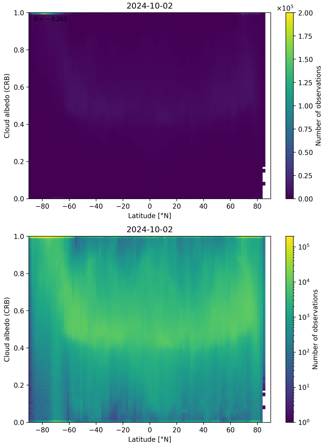
Figure 91: Scatter density plot of “Latitude” against “Cloud albedo (CRB)” for 2024-10-01 to 2024-10-03.
