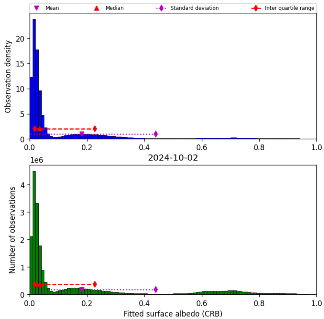
Figure 46: Histogram of “Fitted surface albedo (CRB)” for 2024-10-01 to 2024-10-03
