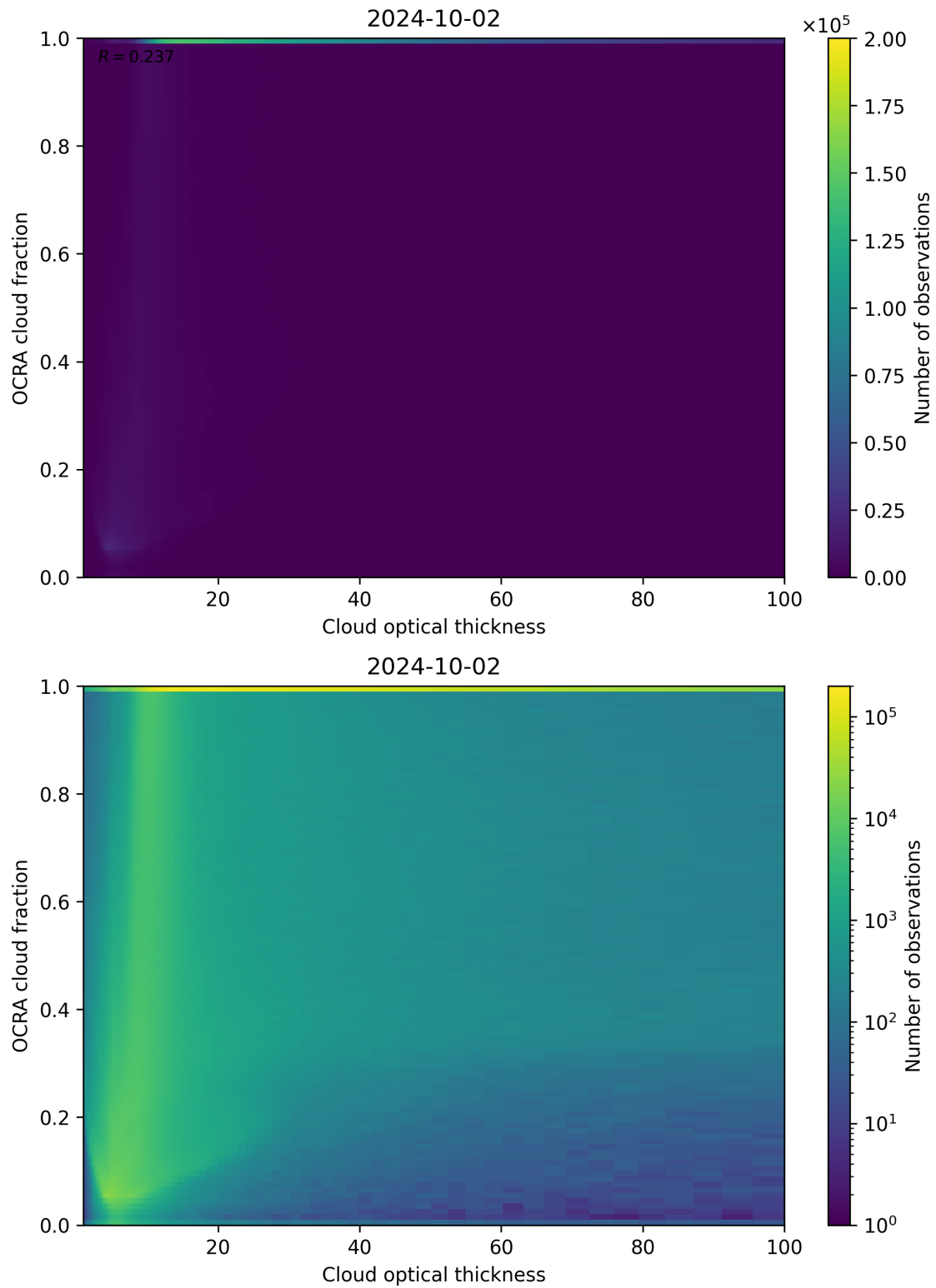
Figure 83: Scatter density plot of “Cloud optical thickness” against “OCRA cloud fraction” for 2024-10-01 to 2024-10-03.
