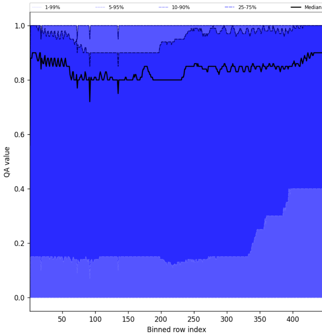
Figure 54: Along track statistics of “QA value” for 2024-10-01 to 2024-10-03
