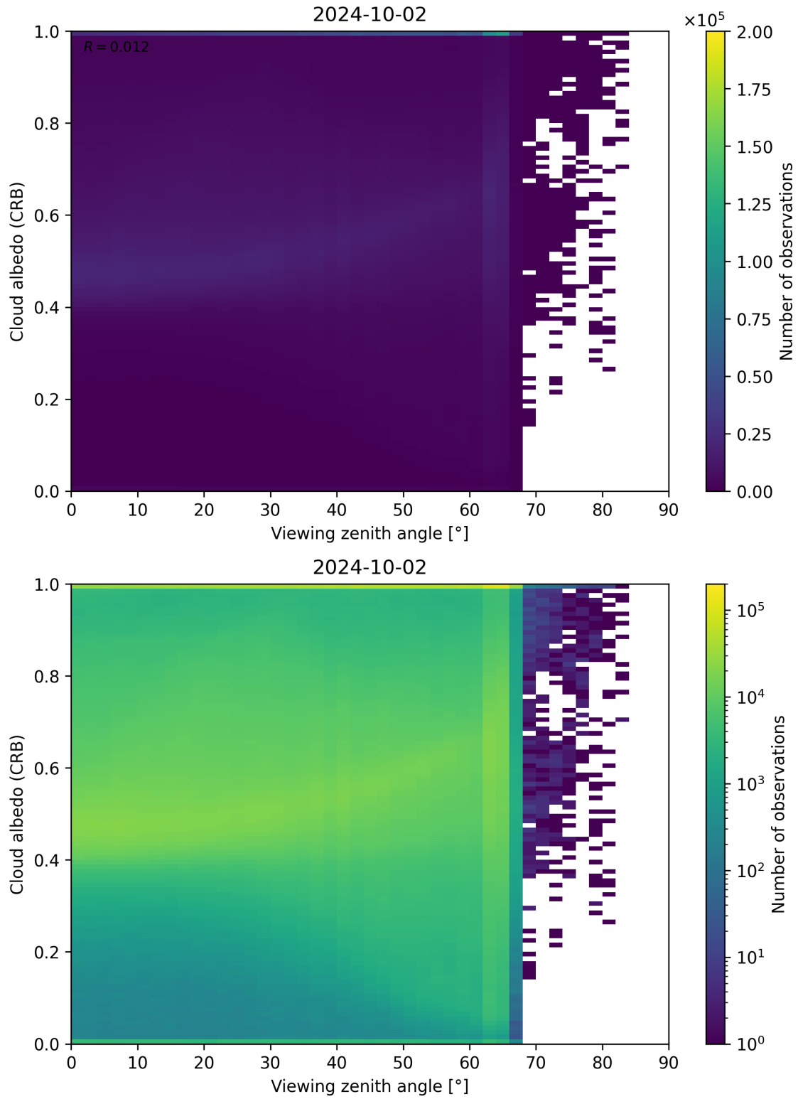
Figure 106: Scatter density plot of “Viewing zenith angle” against “Cloud albedo (CRB)” for 2024-10-01 to 2024-10-03.
