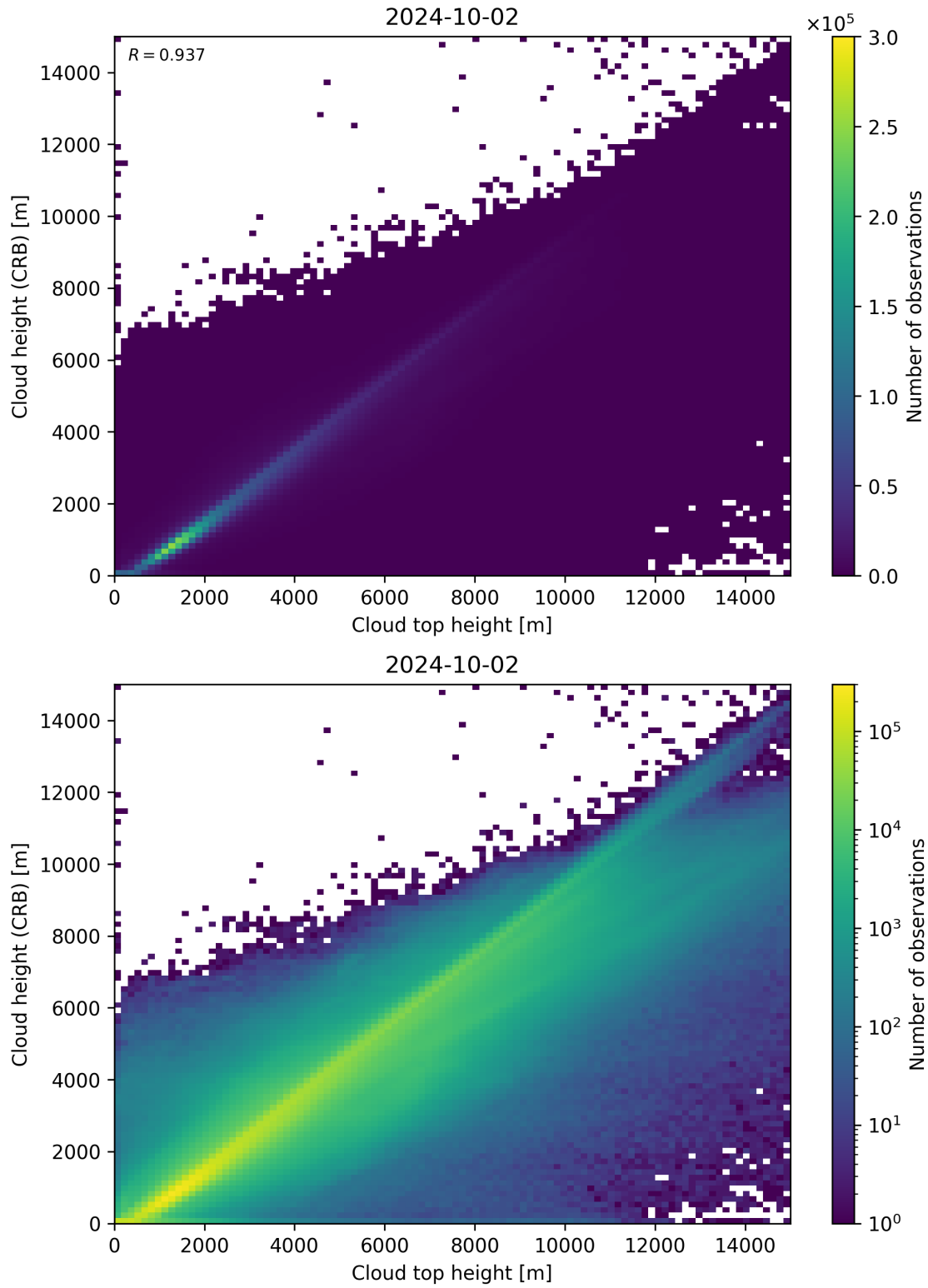
Figure 89: Scatter density plot of “Cloud top height” against “Cloud height (CRB)” for 2024-10-01 to 2024-10-03.
