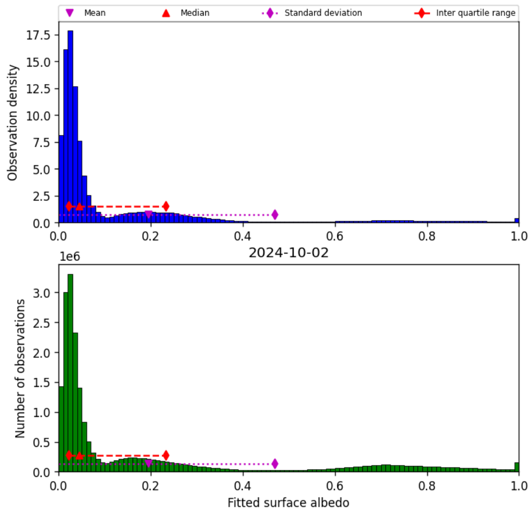
Figure 45: Histogram of “Fitted surface albedo” for 2024-10-01 to 2024-10-03
