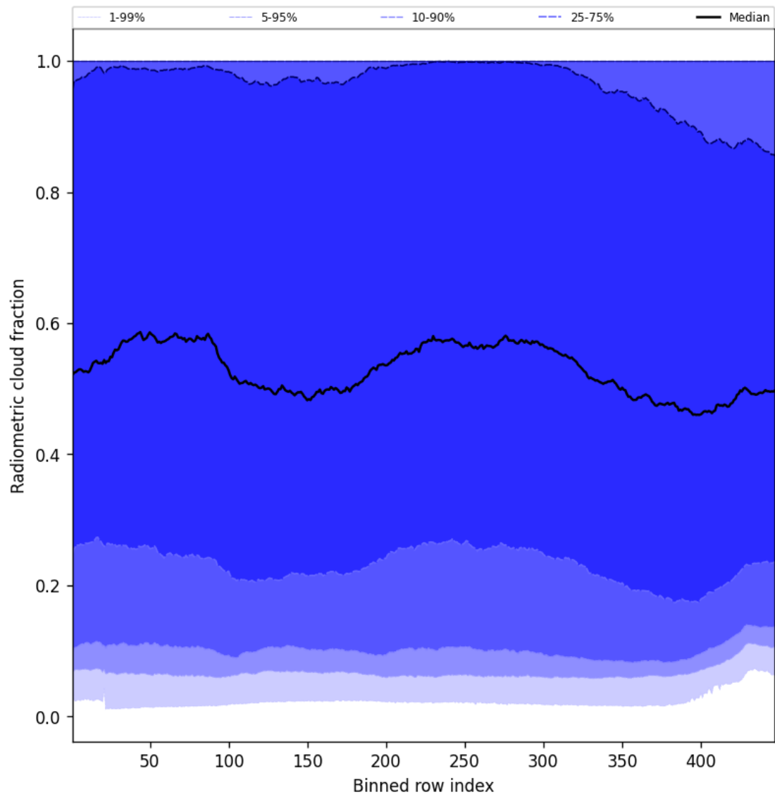
Figure 55: Along track statistics of “Radiometric cloud fraction” for 2024-10-01 to 2024-10-03
