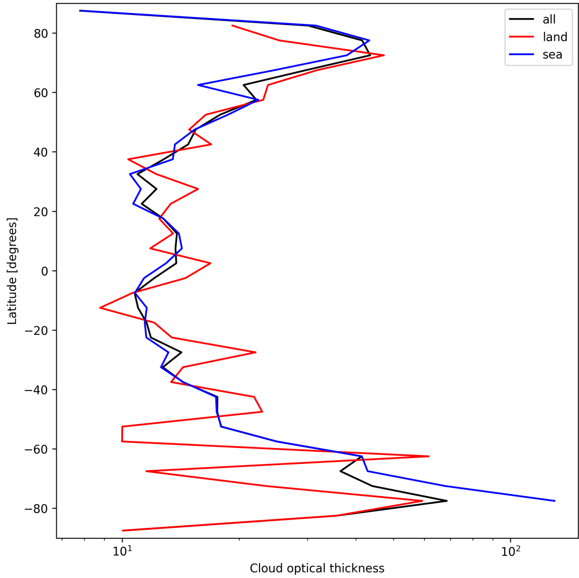
Figure 25: Zonal average of “Cloud optical thickness” for 2024-10-01 to 2024-10-03.
