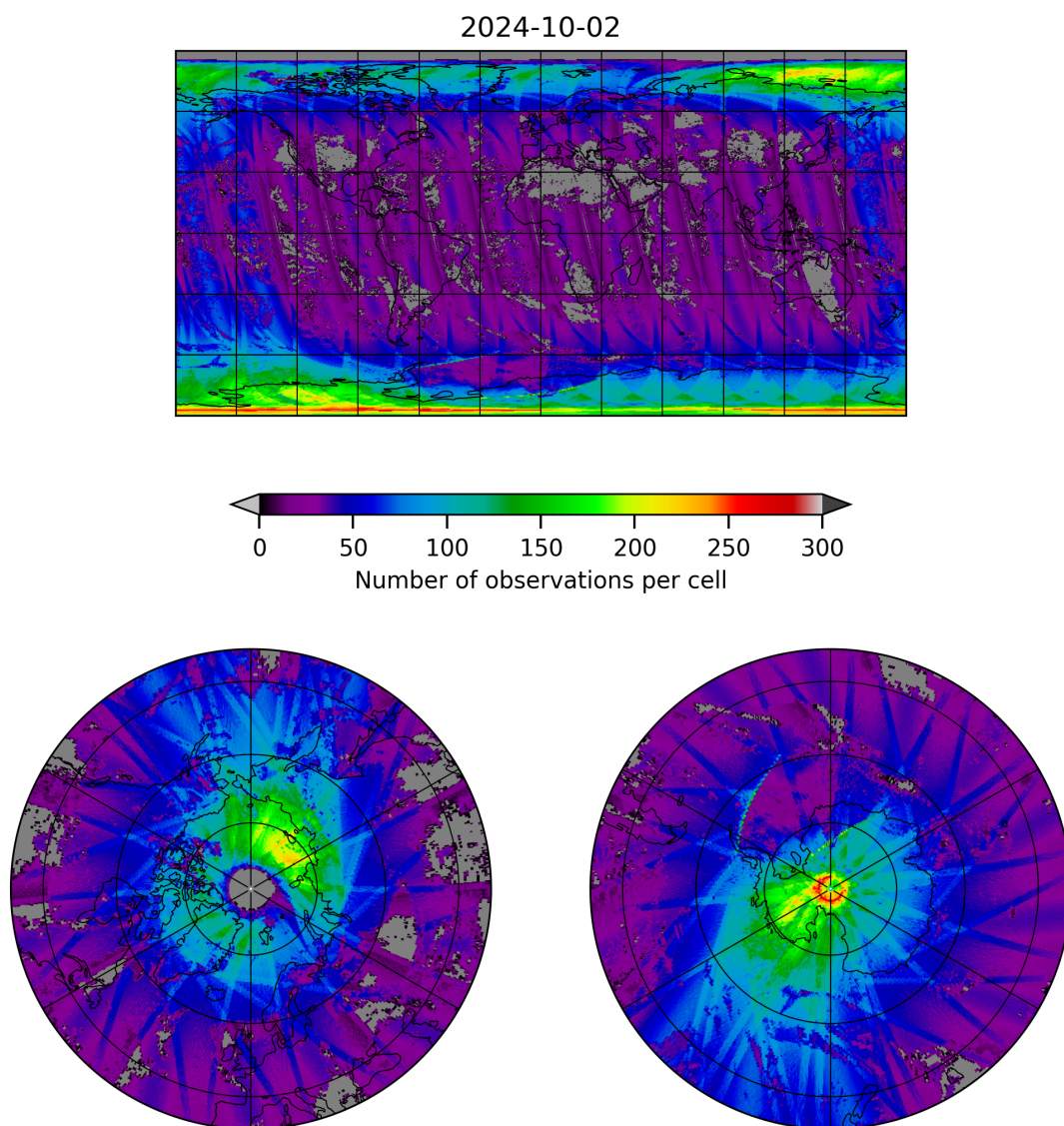
Figure 21: Map of the number of observations for 2024-10-01 to 2024-10-03
