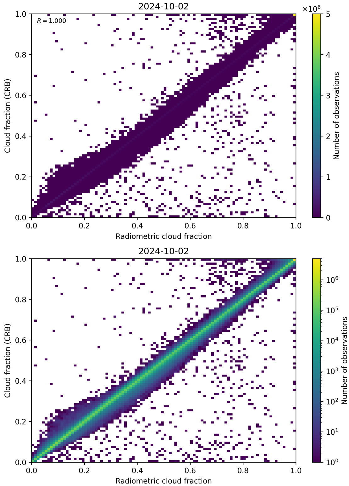
Figure 73: Scatter density plot of “Radiometric cloud fraction” against “Cloud fraction (CRB)” for 2024-10-01 to 2024-10-03.
