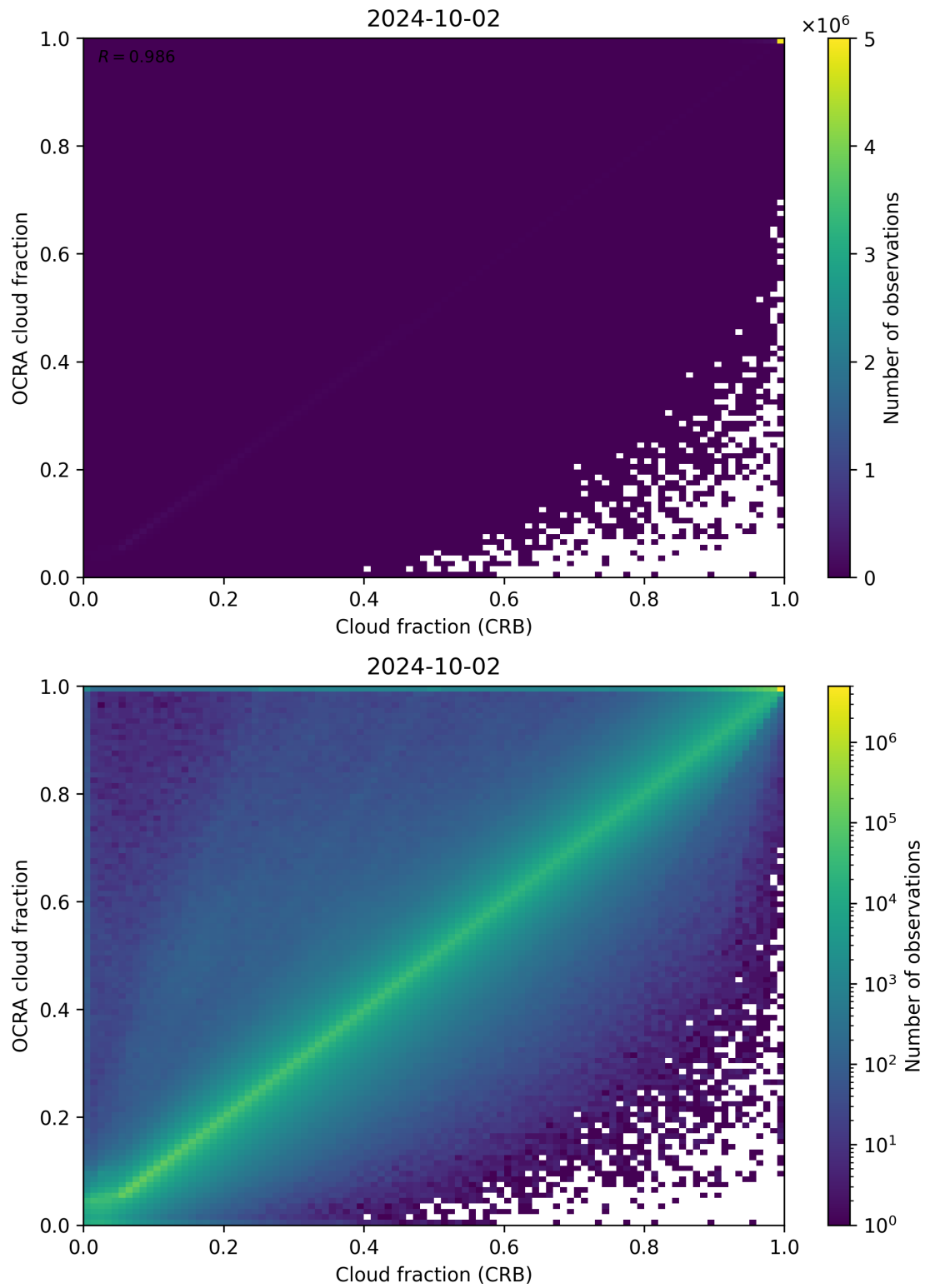
Figure 78: Scatter density plot of “Cloud fraction (CRB)” against “OCRA cloud fraction” for 2024-10-01 to 2024-10-03.
