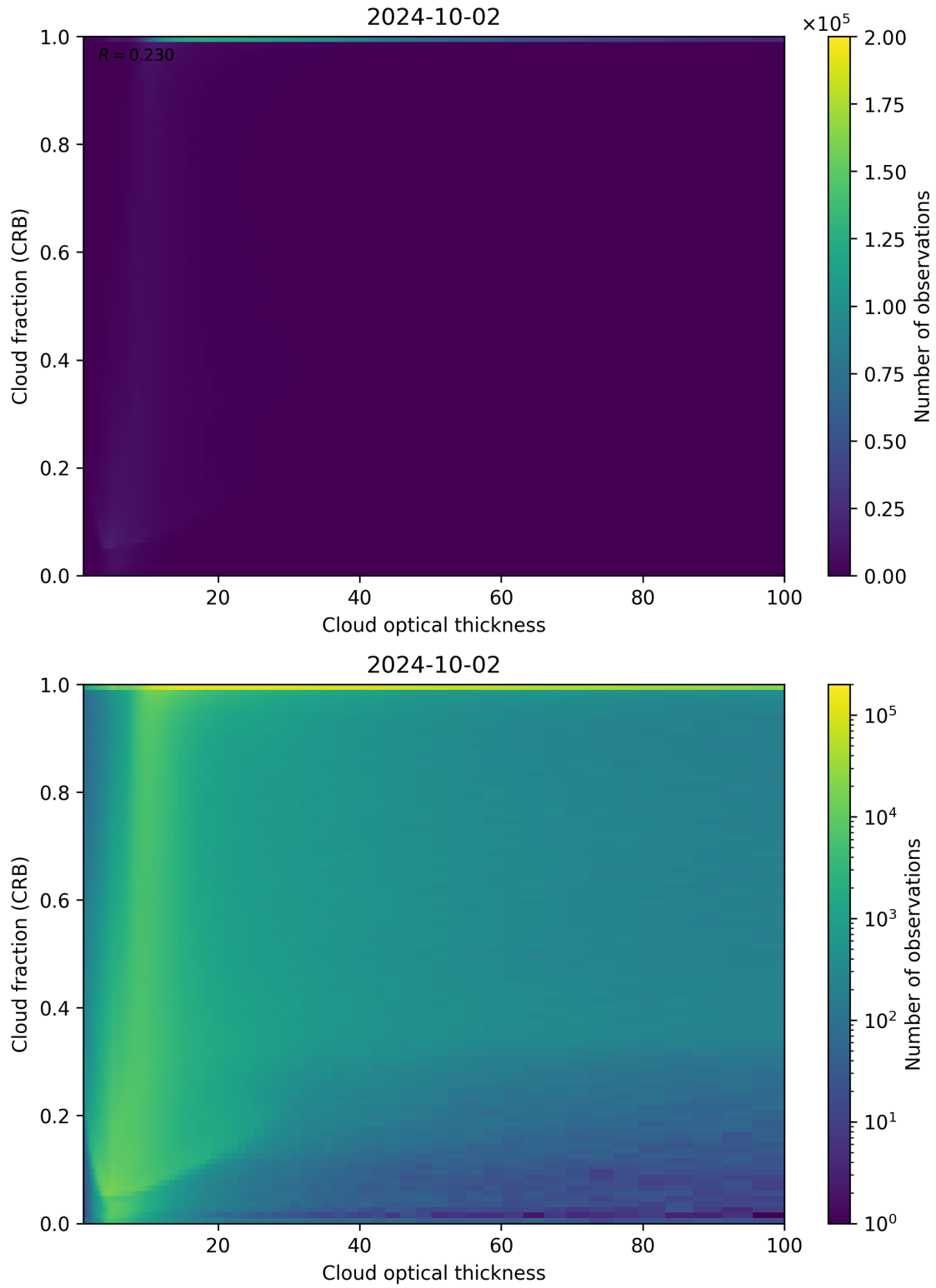
Figure 84: Scatter density plot of “Cloud optical thickness” against “Cloud fraction (CRB)” for 2024-10-01 to 2024-10-03.
