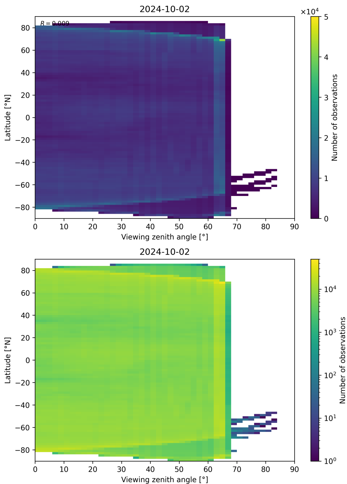
Figure 113: Scatter density plot of “Viewing zenith angle” against “Latitude” for 2024-10-01 to 2024-10-03.
