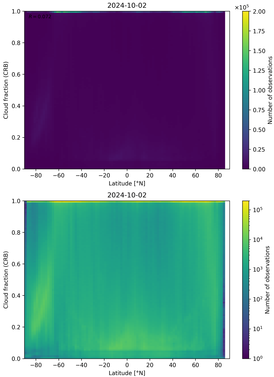
Figure 94: Scatter density plot of “Latitude” against “Cloud fraction (CRB)” for 2024-10-01 to 2024-10-03.
