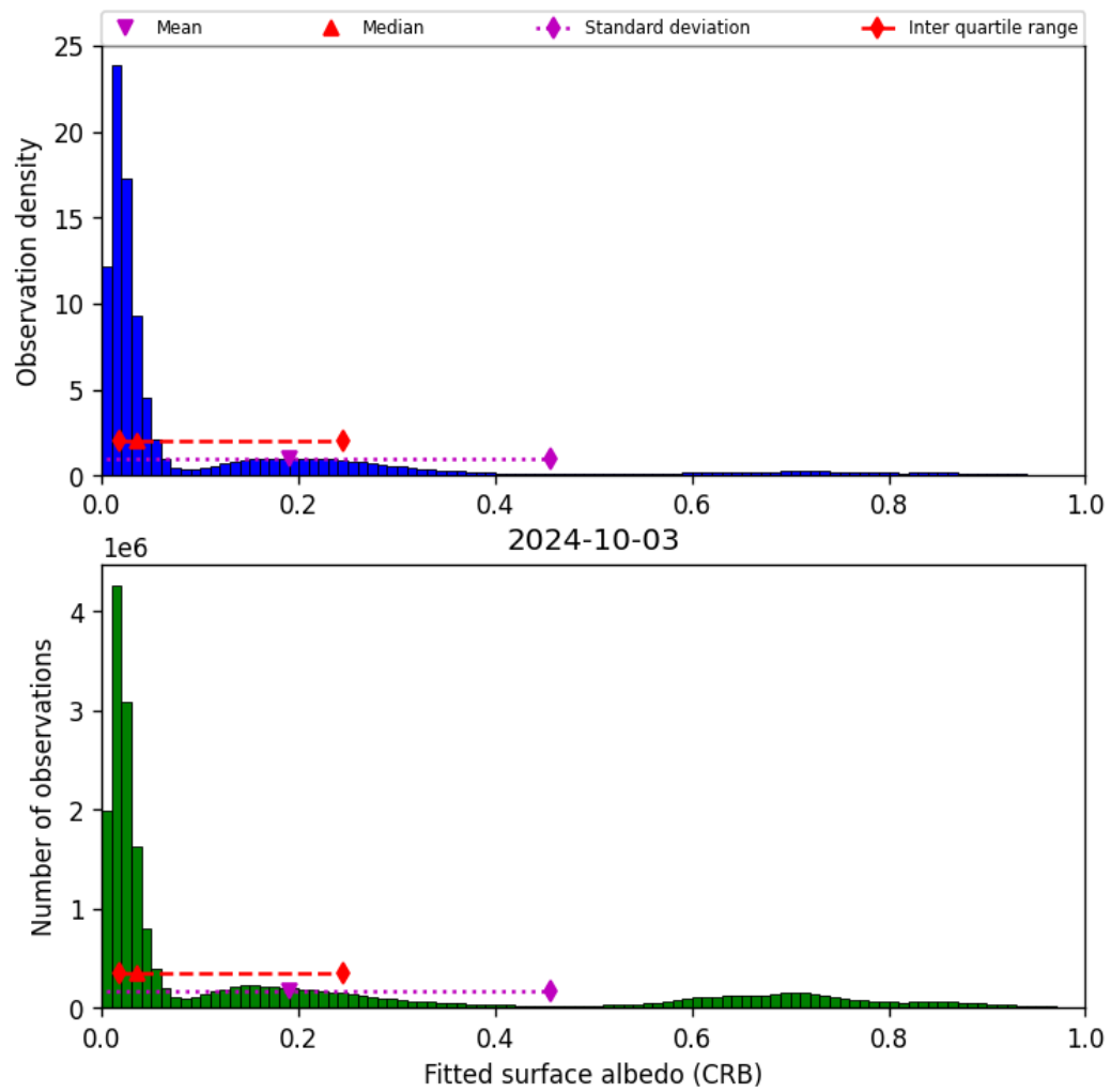
Figure 46: Histogram of “Fitted surface albedo (CRB)” for 2024-10-03 to 2024-10-04
