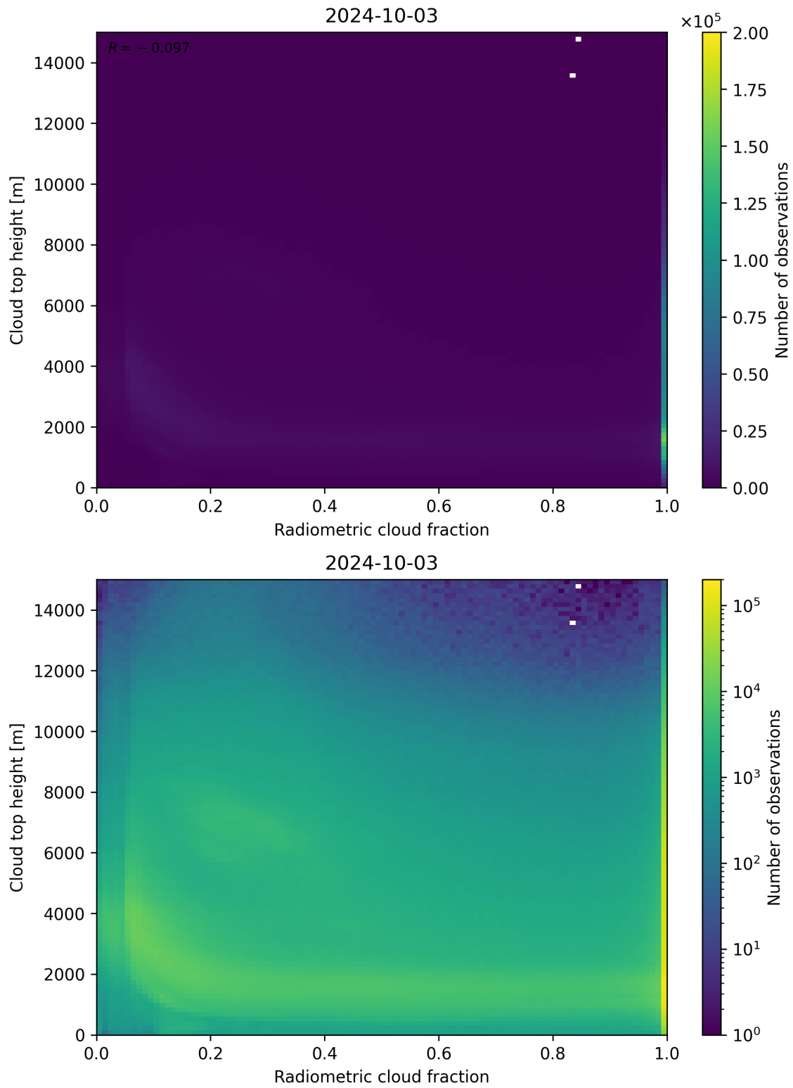
Figure 76: Scatter density plot of “Radiometric cloud fraction” against “Cloud top height” for 2024-10-03 to 2024-10-04.
