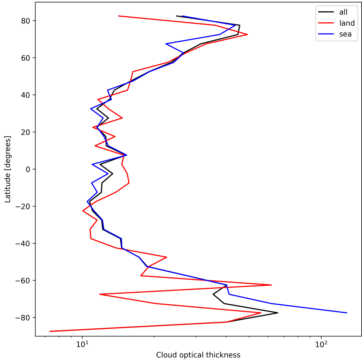
Figure 25: Zonal average of “Cloud optical thickness” for 2024-10-03 to 2024-10-04.
