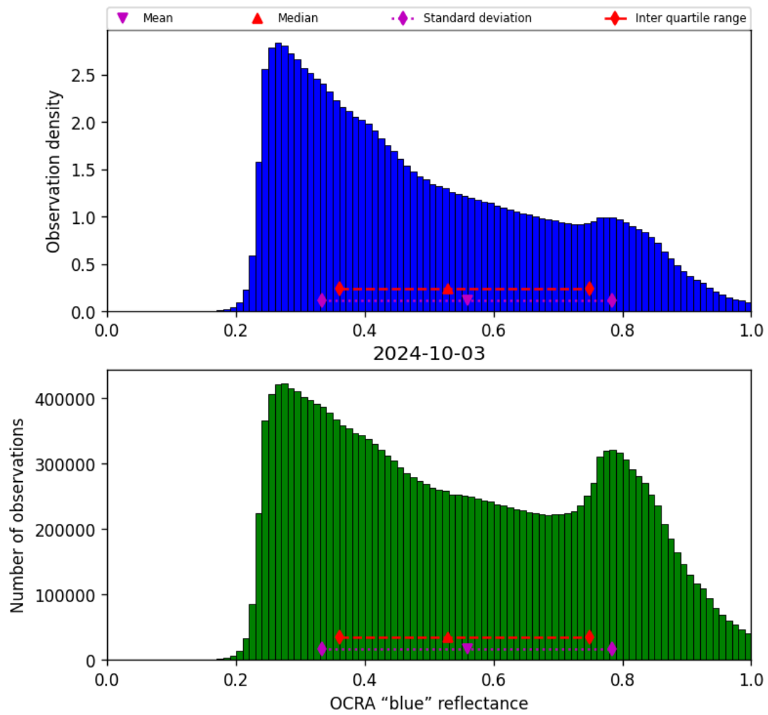
Figure 51: Histogram of “OCRA “blue” reflectance” for 2024-10-03 to 2024-10-04
