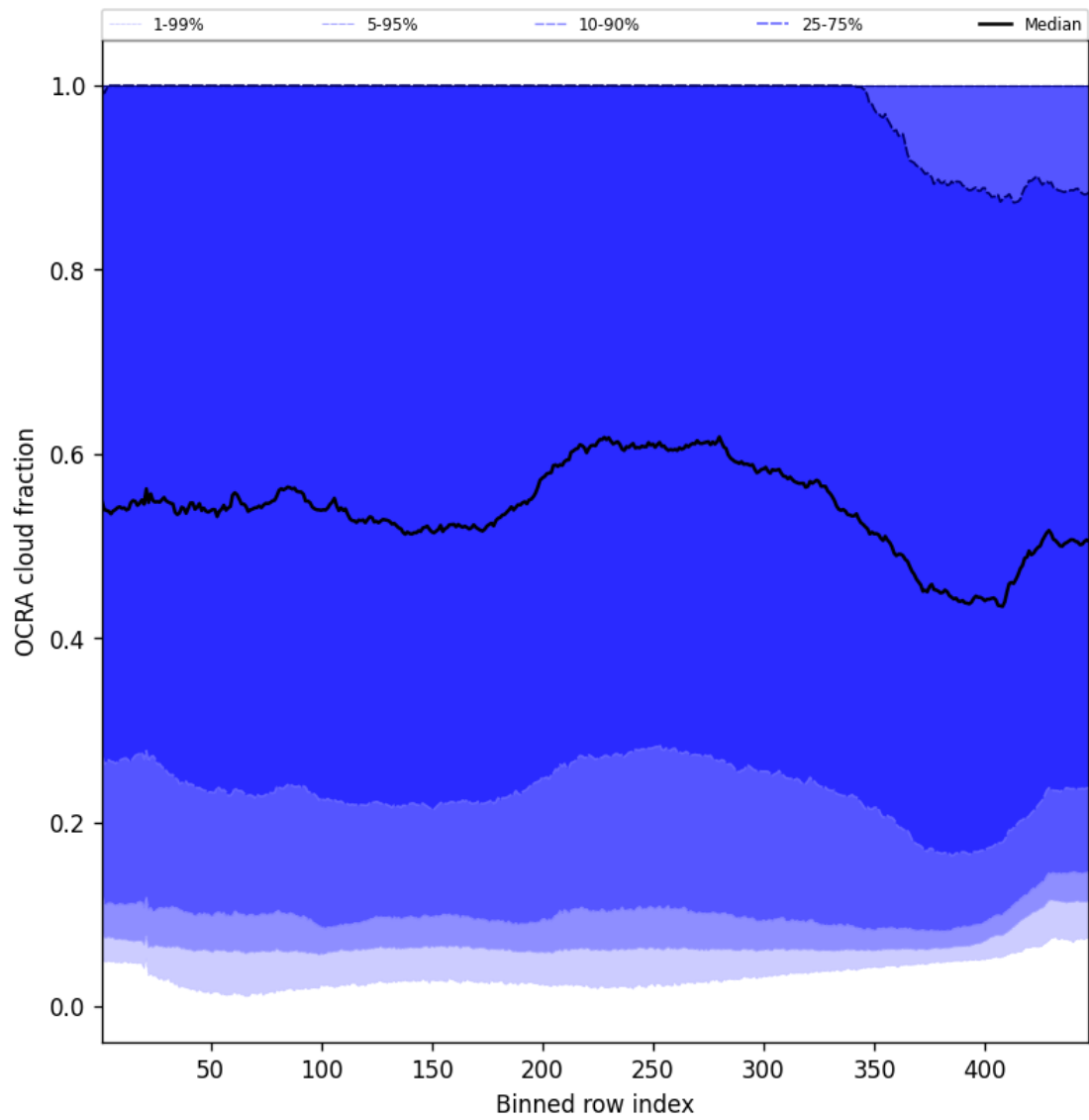
Figure 66: Along track statistics of “OCRA cloud fraction” for 2024-10-03 to 2024-10-04
