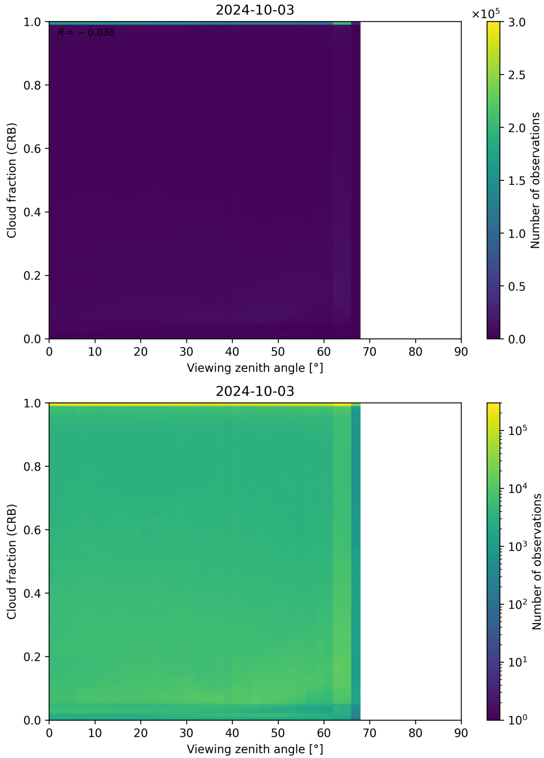
Figure 109: Scatter density plot of “Viewing zenith angle” against “Cloud fraction (CRB)” for 2024-10-03 to 2024-10-04.
