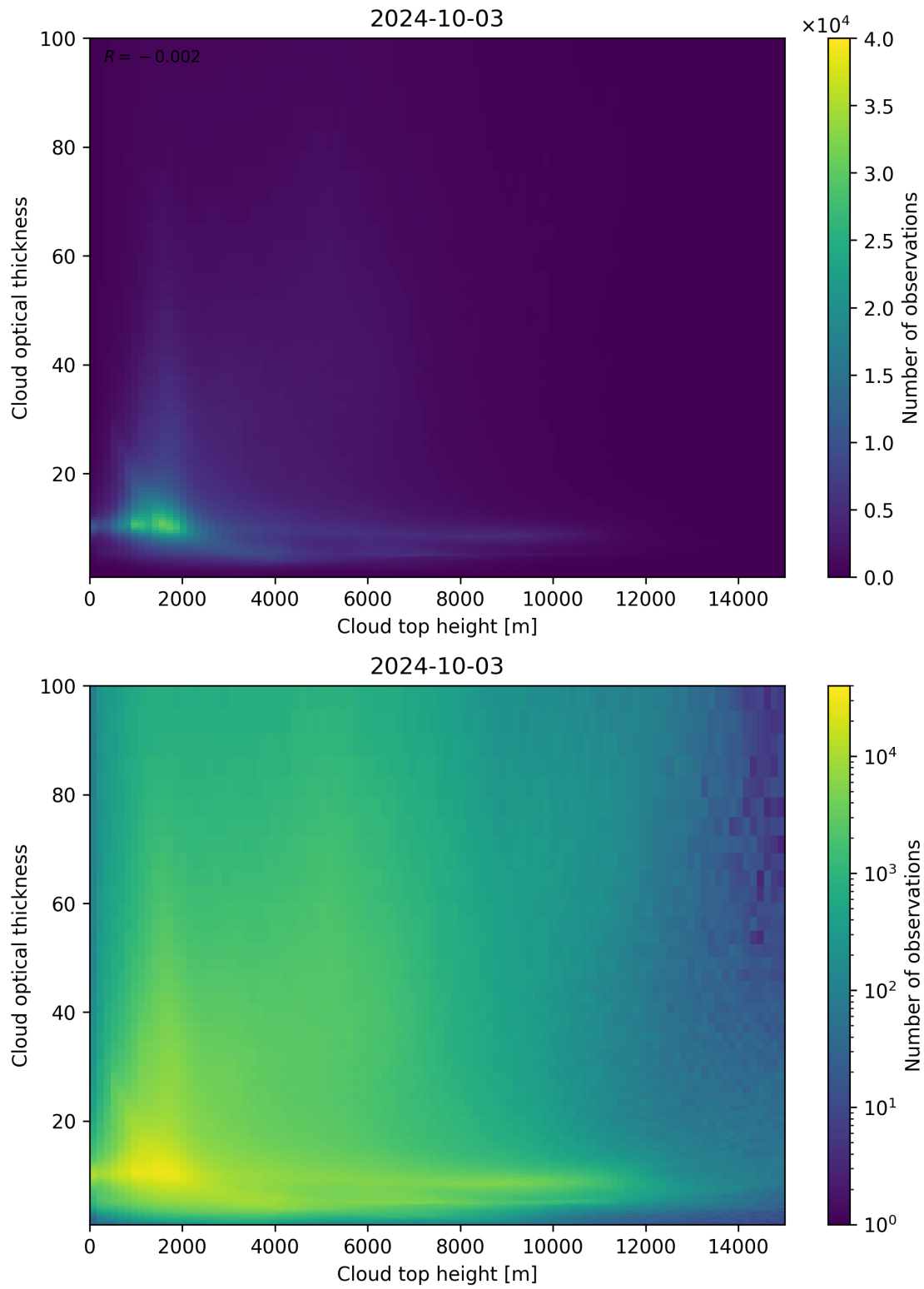
Figure 90: Scatter density plot of “Cloud top height” against “Cloud optical thickness” for 2024-10-03 to 2024-10-04.
