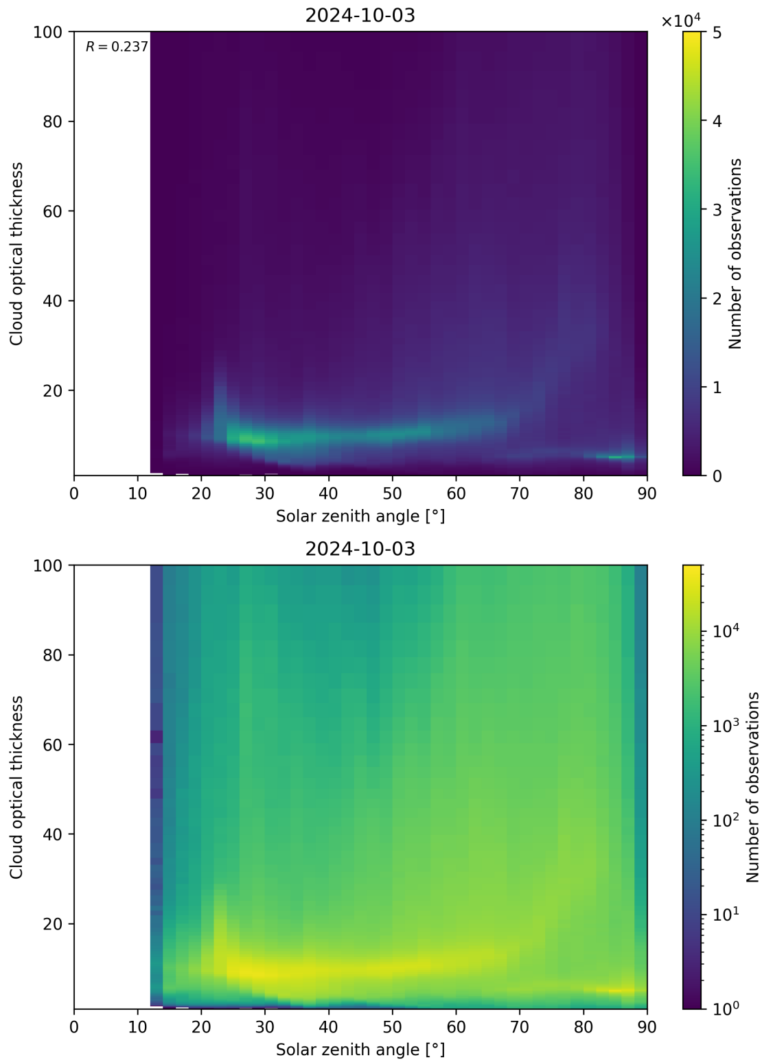
Figure 103: Scatter density plot of “Solar zenith angle” against “Cloud optical thickness” for 2024-10-03 to 2024-10-04.
