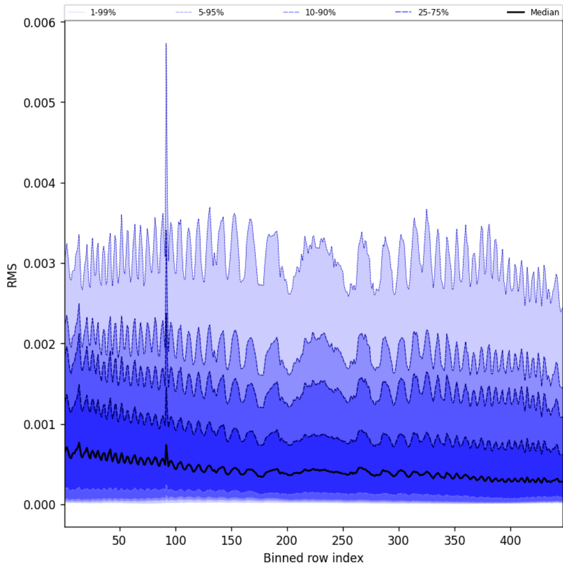
Figure 63: Along track statistics of “RMS” for 2024-10-03 to 2024-10-04
