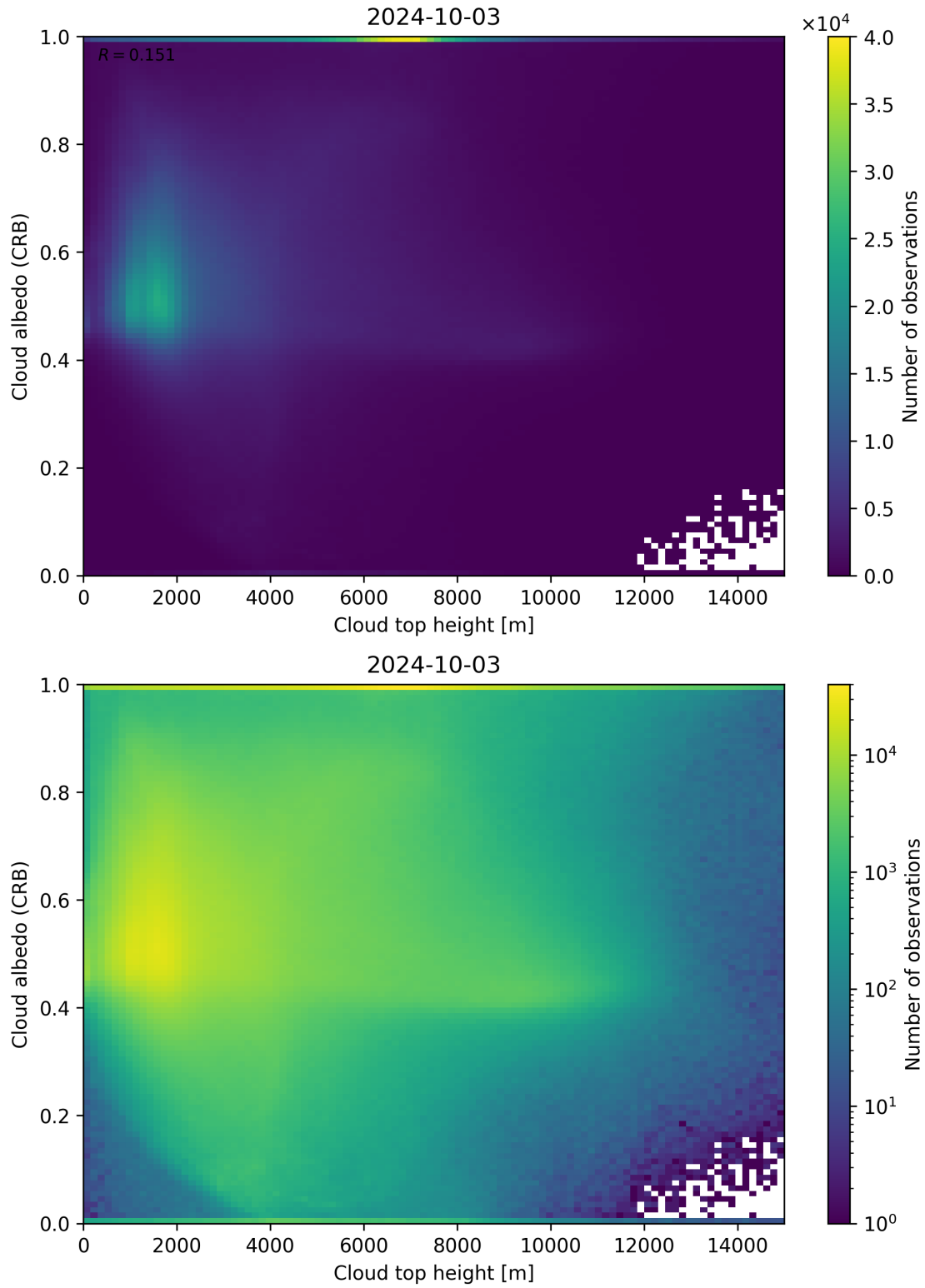
Figure 86: Scatter density plot of “Cloud top height” against “Cloud albedo (CRB)” for 2024-10-03 to 2024-10-04.
