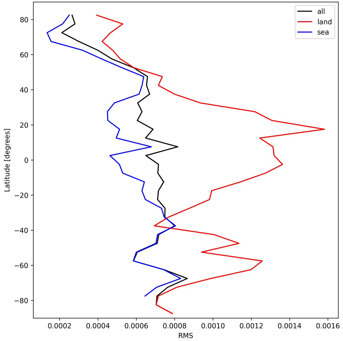
Figure 31: Zonal average of “RMS” for 2024-10-03 to 2024-10-04.
