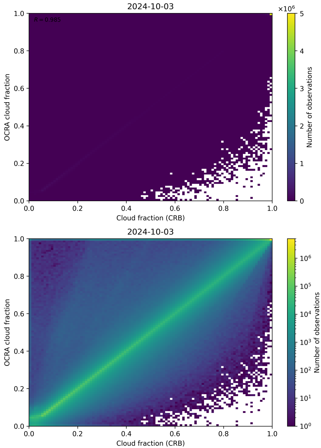
Figure 78: Scatter density plot of “Cloud fraction (CRB)” against “OCRA cloud fraction” for 2024-10-03 to 2024-10-04.
