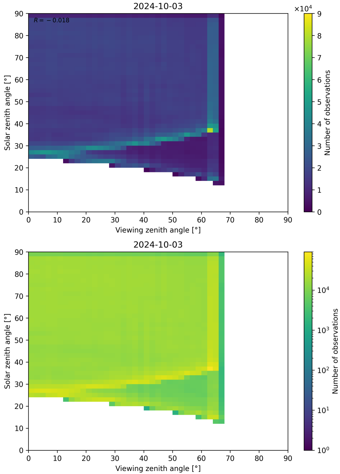
Figure 114: Scatter density plot of “Viewing zenith angle” against “Solar zenith angle” for 2024-10-03 to 2024-10-04.
