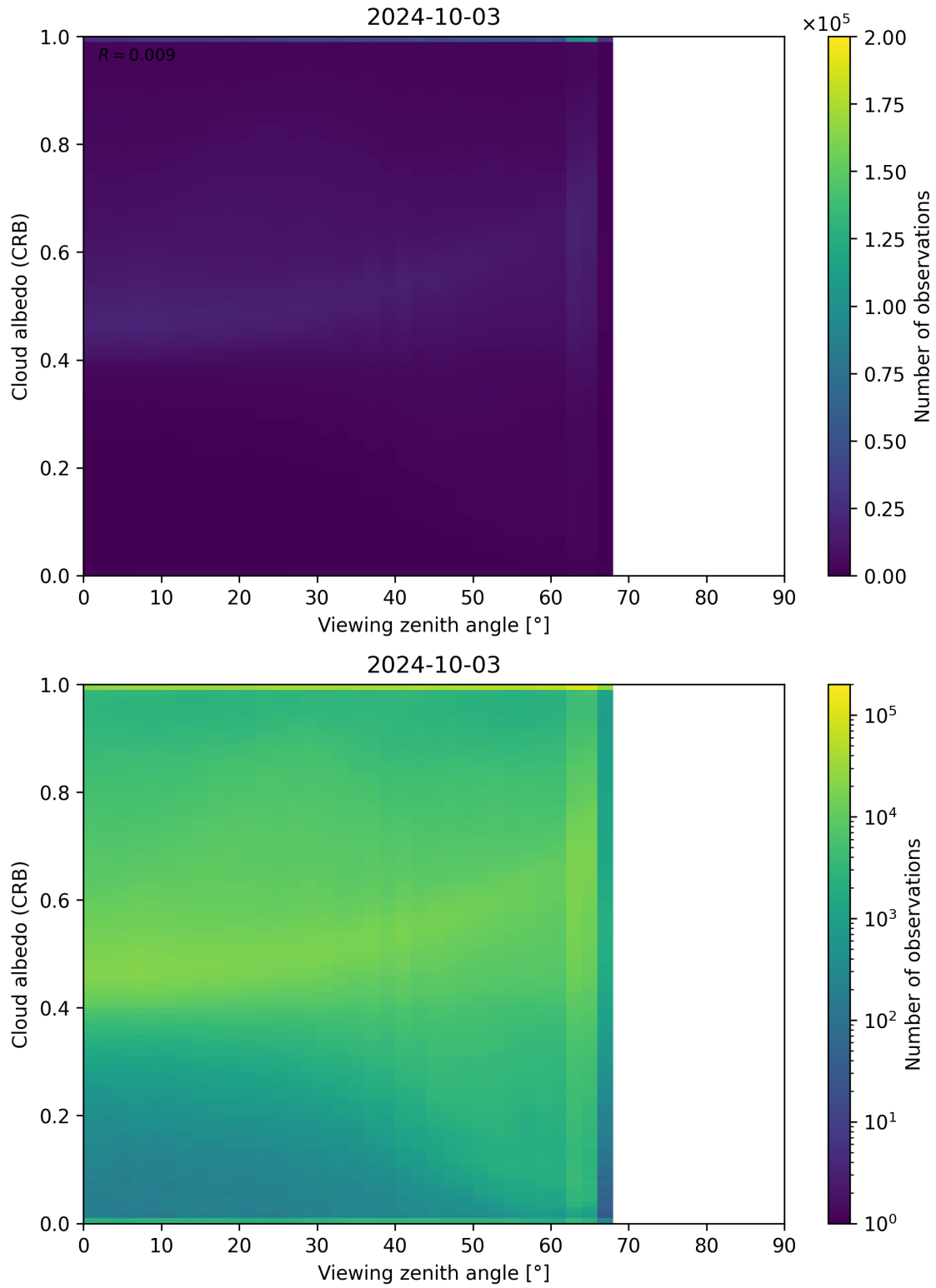
Figure 106: Scatter density plot of “Viewing zenith angle” against “Cloud albedo (CRB)” for 2024-10-03 to 2024-10-04.
