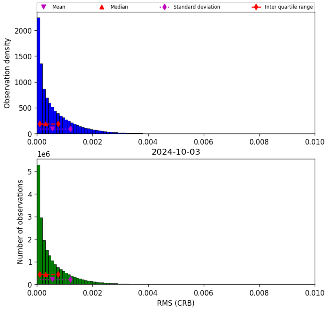
Figure 48: Histogram of “RMS (CRB)” for 2024-10-03 to 2024-10-04
