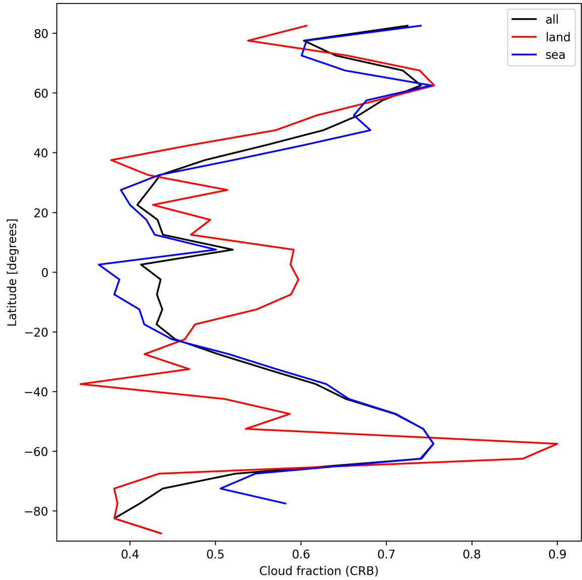
Figure 26: Zonal average of “Cloud fraction (CRB)” for 2024-10-03 to 2024-10-04.
