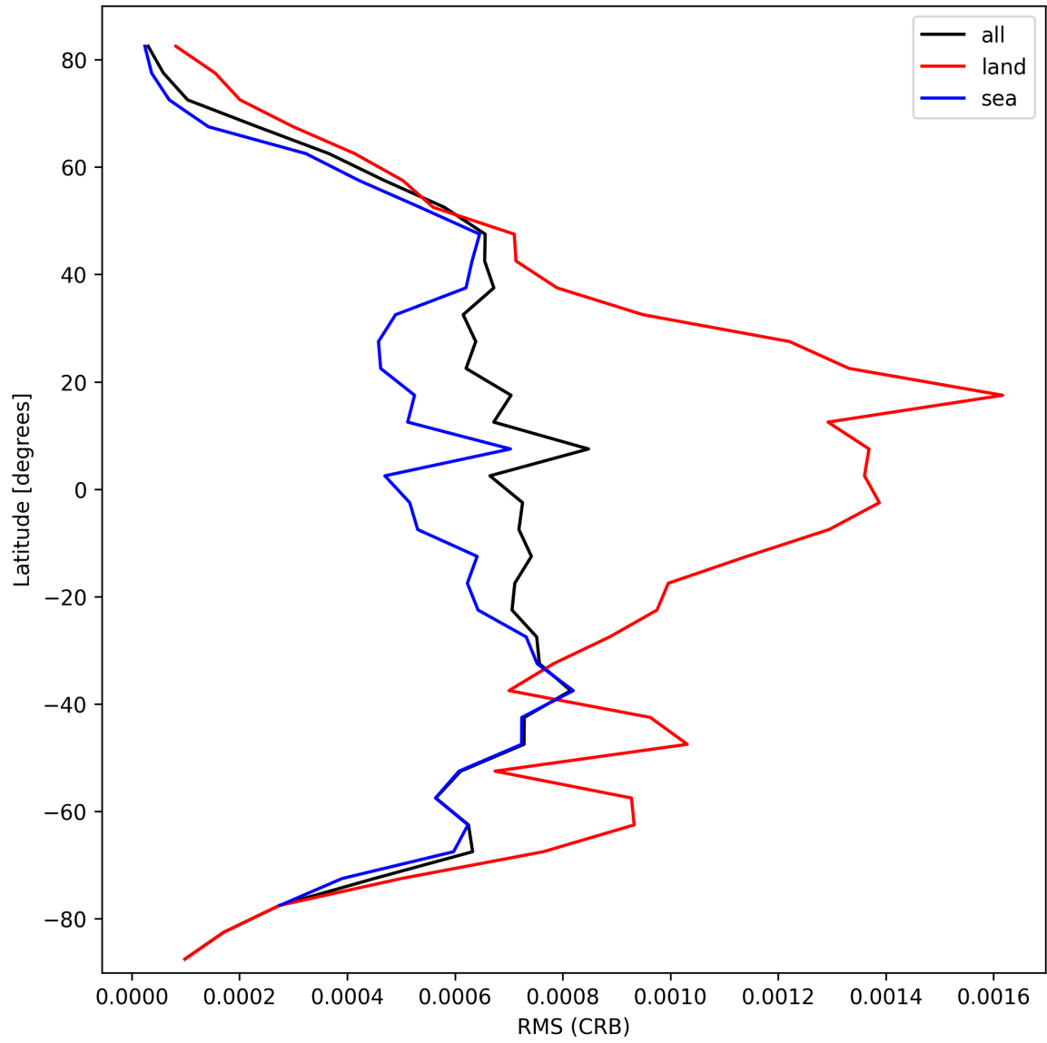
Figure 32: Zonal average of “RMS (CRB)” for 2024-10-03 to 2024-10-04.
