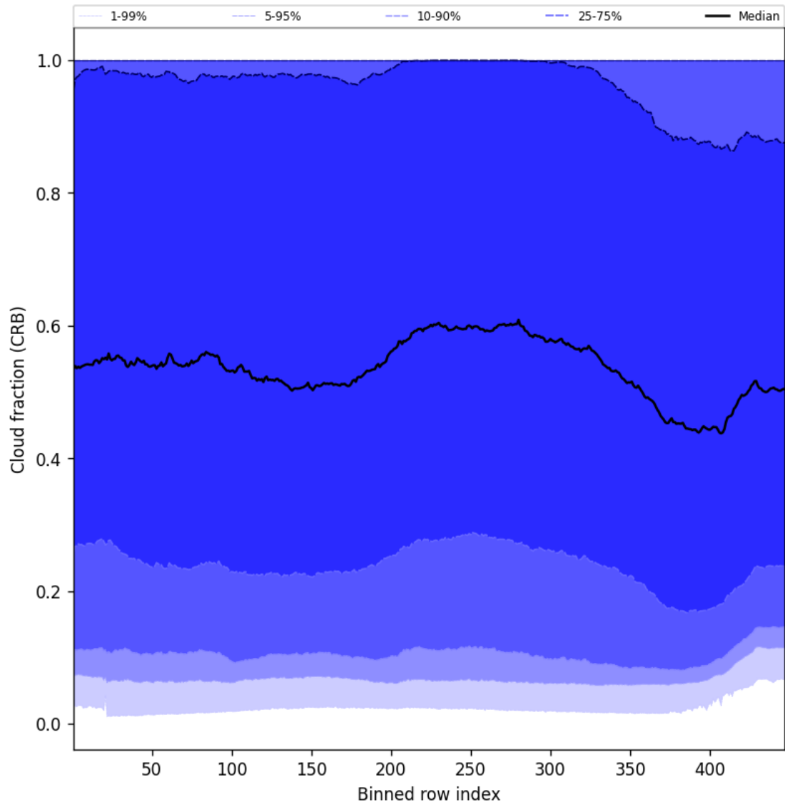
Figure 58: Along track statistics of “Cloud fraction (CRB)” for 2024-10-03 to 2024-10-04
