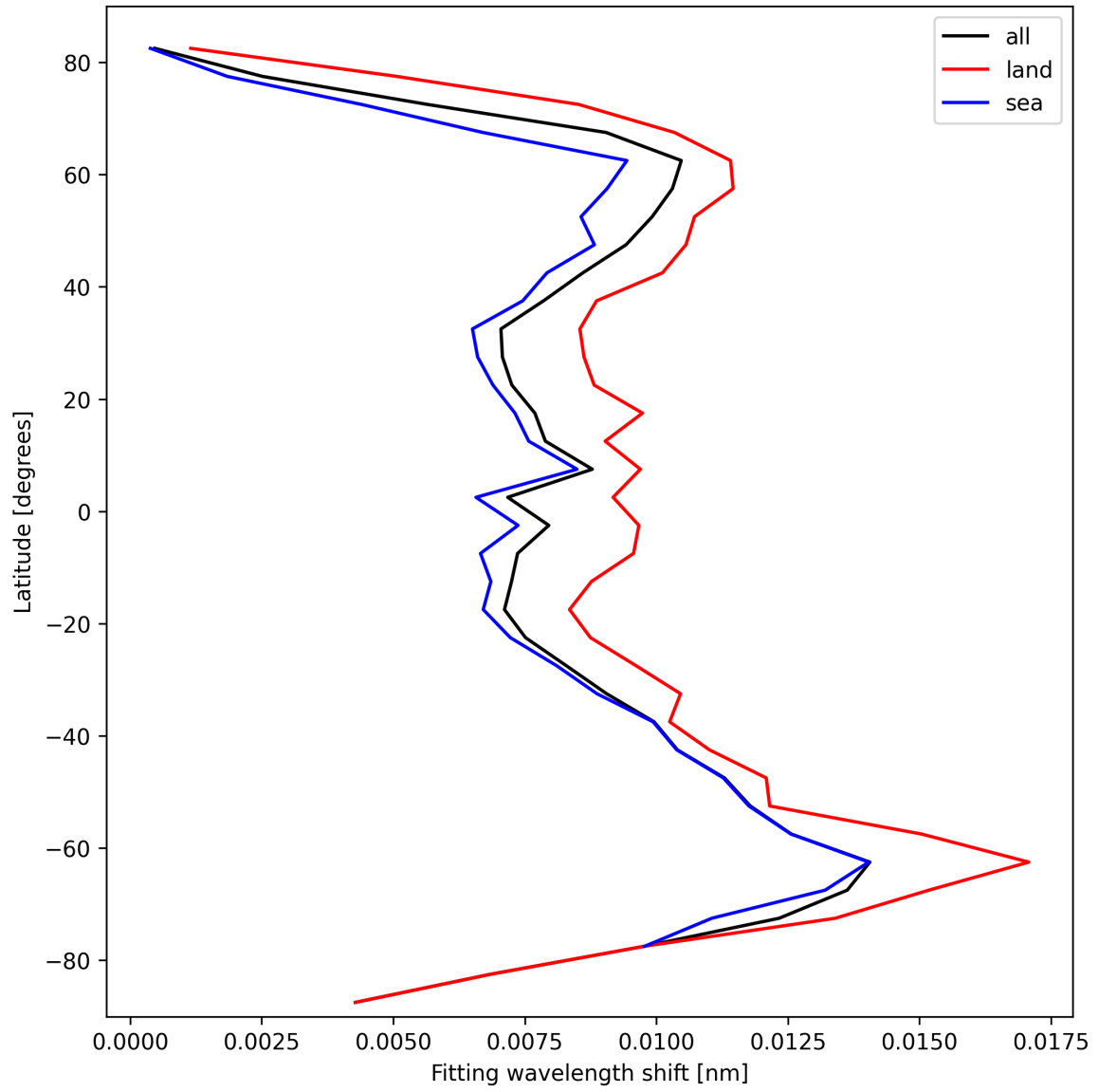
Figure 33: Zonal average of “Fitting wavelength shift” for 2024-10-03 to 2024-10-04.
