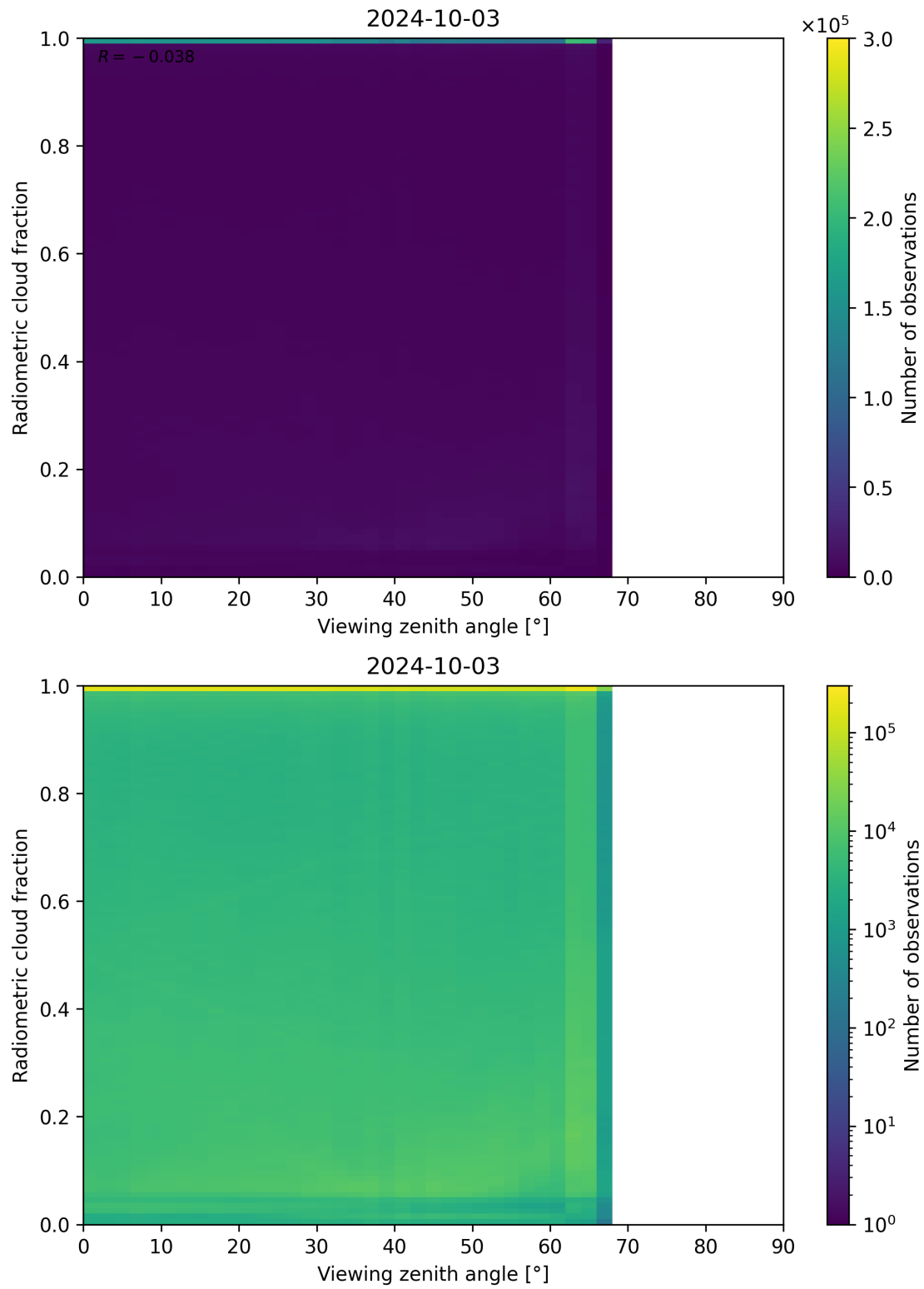
Figure 107: Scatter density plot of “Viewing zenith angle” against “Radiometric cloud fraction” for 2024-10-03 to 2024-10-04.
