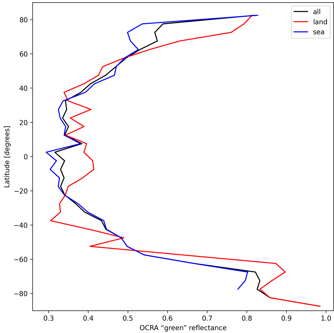
Figure 36: Zonal average of “OCRA “green” reflectance” for 2024-10-03 to 2024-10-04.
