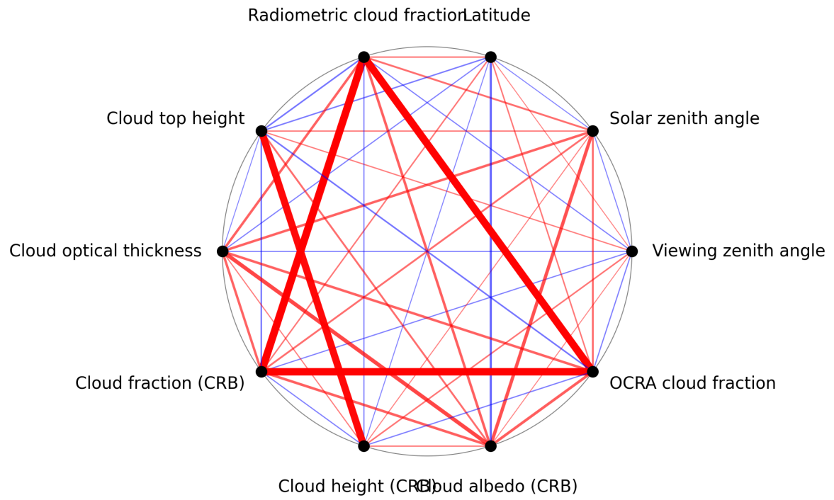
Figure 1: Map of correlation graph for 2024-10-03 to 2024-10-04.
