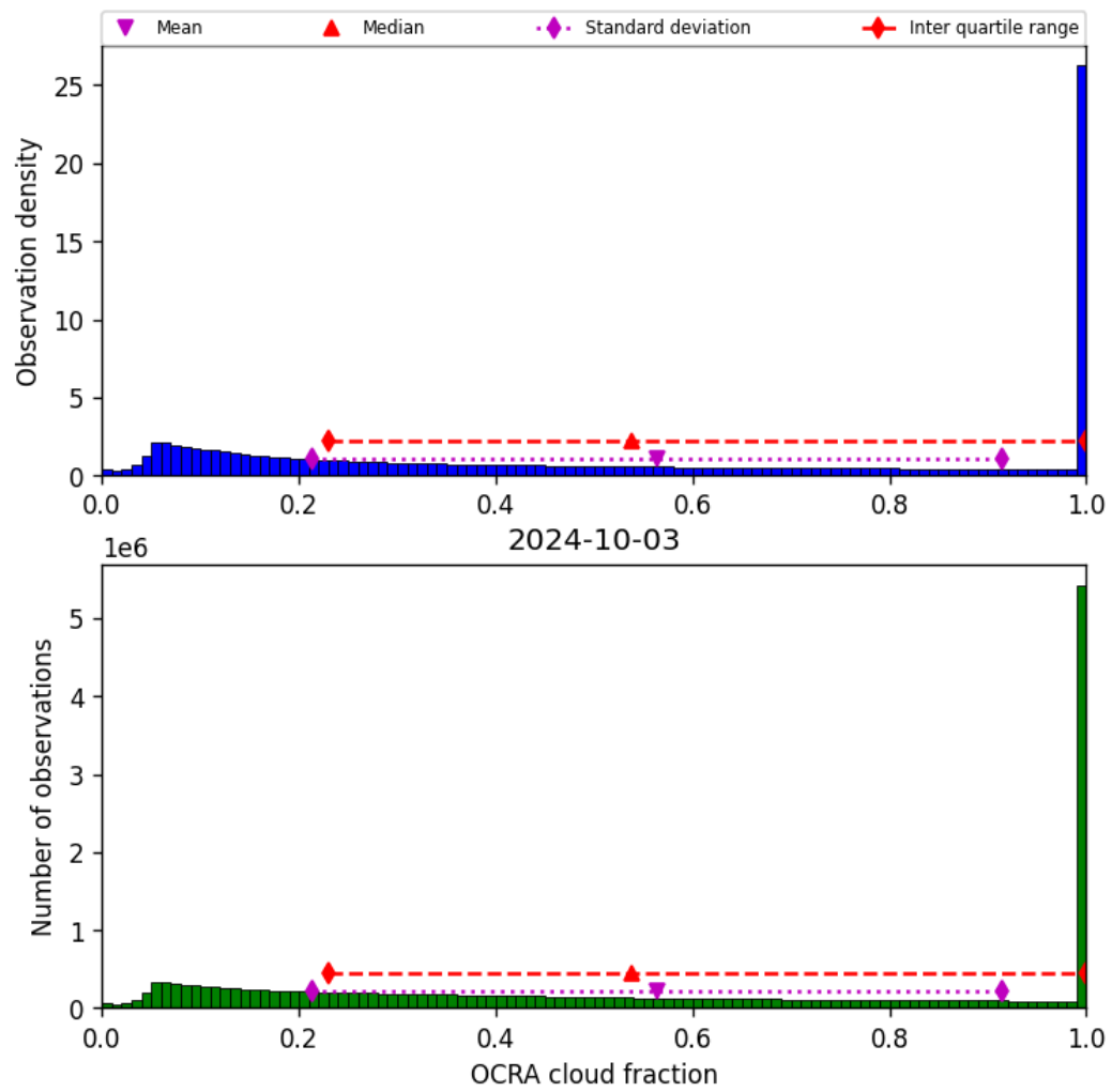
Figure 50: Histogram of “OCRA cloud fraction” for 2024-10-03 to 2024-10-04
