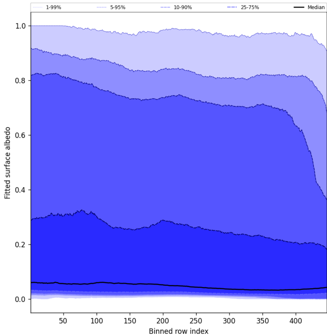
Figure 61: Along track statistics of “Fitted surface albedo” for 2024-10-03 to 2024-10-04
