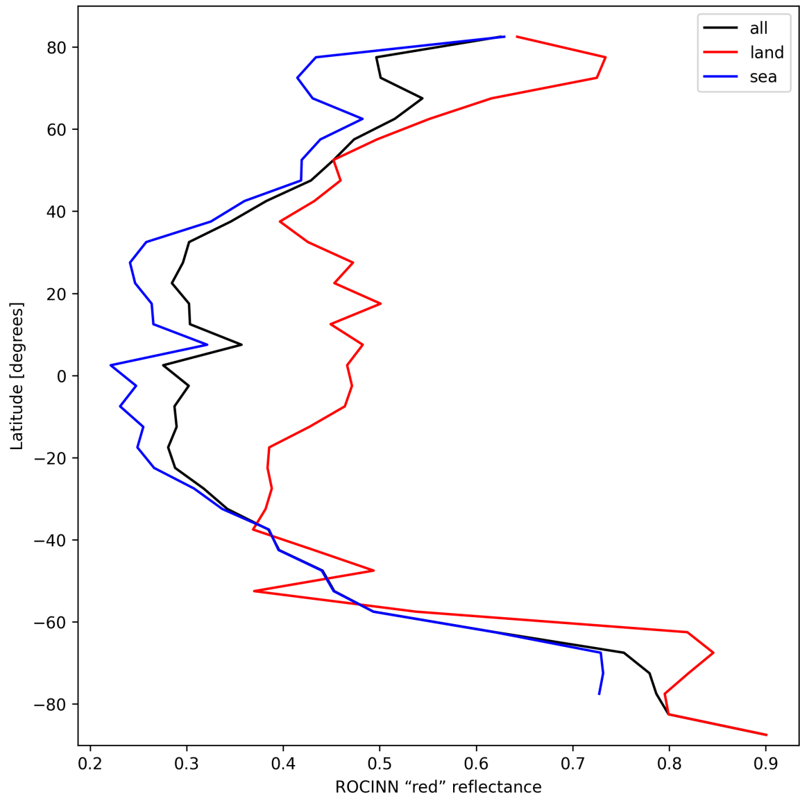
Figure 37: Zonal average of “ROCINN “red” reflectance” for 2024-10-03 to 2024-10-04.
