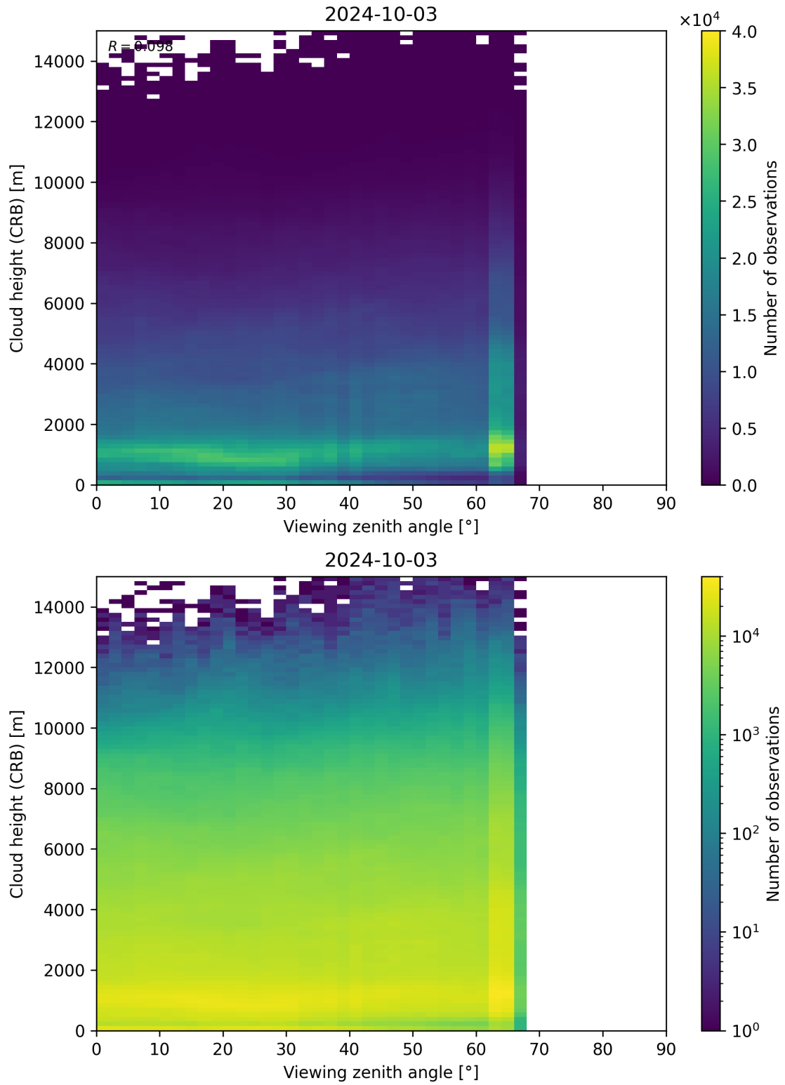
Figure 110: Scatter density plot of “Viewing zenith angle” against “Cloud height (CRB)” for 2024-10-03 to 2024-10-04.
