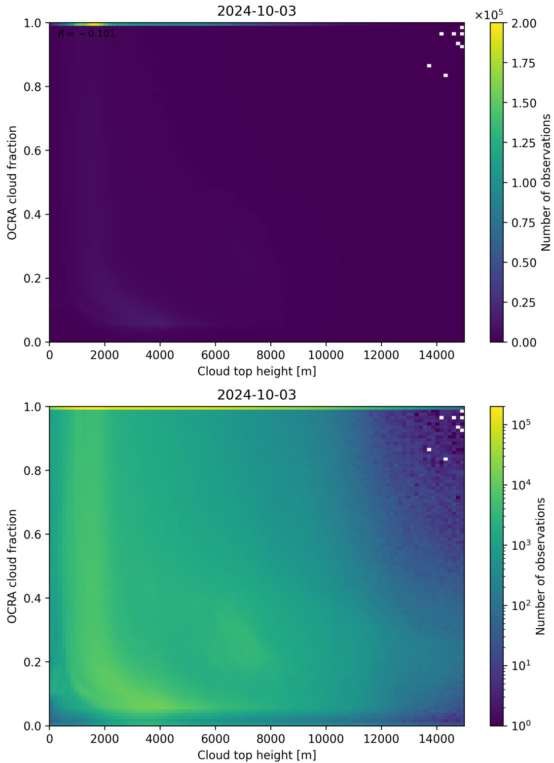
Figure 87: Scatter density plot of “Cloud top height” against “OCRA cloud fraction” for 2024-10-03 to 2024-10-04.
