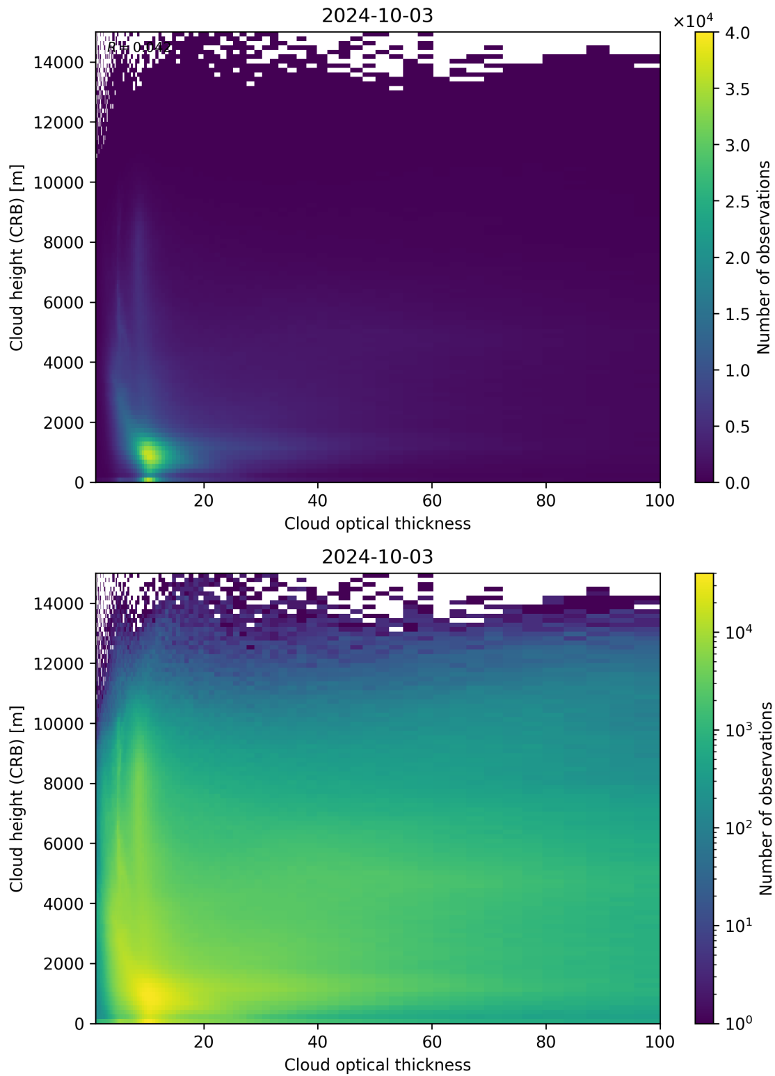
Figure 85: Scatter density plot of “Cloud optical thickness” against “Cloud height (CRB)” for 2024-10-03 to 2024-10-04.
