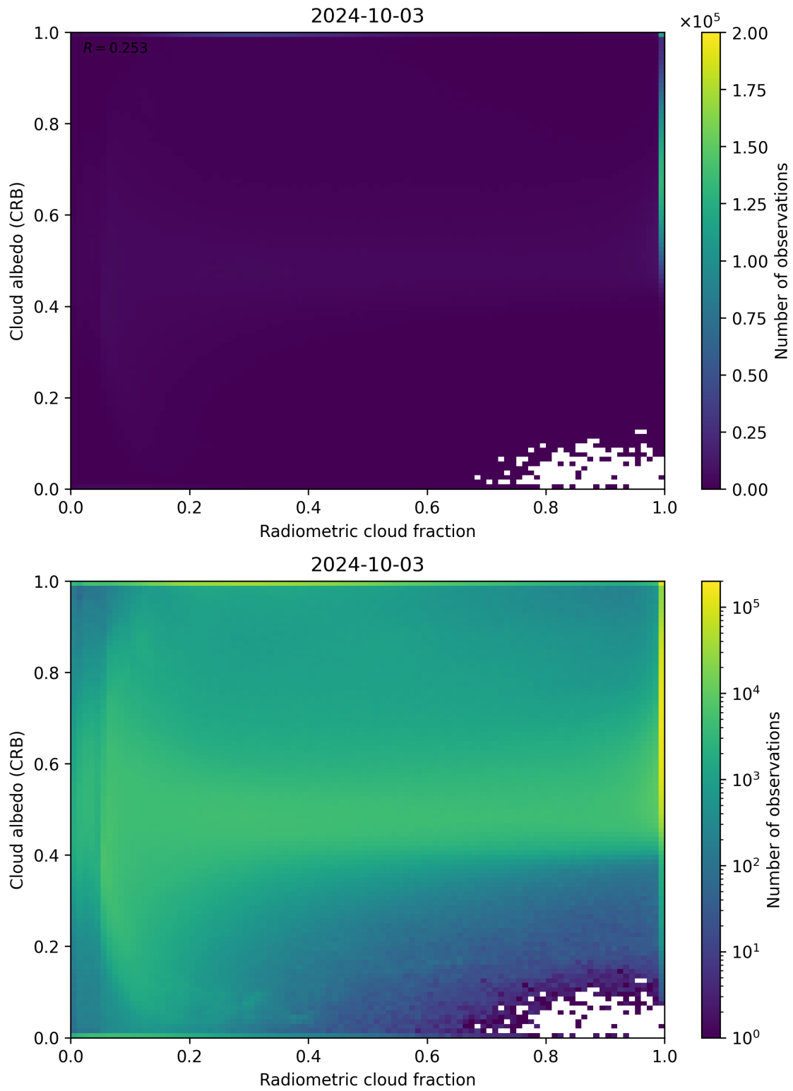
Figure 71: Scatter density plot of “Radiometric cloud fraction” against “Cloud albedo (CRB)” for 2024-10-03 to 2024-10-04.
