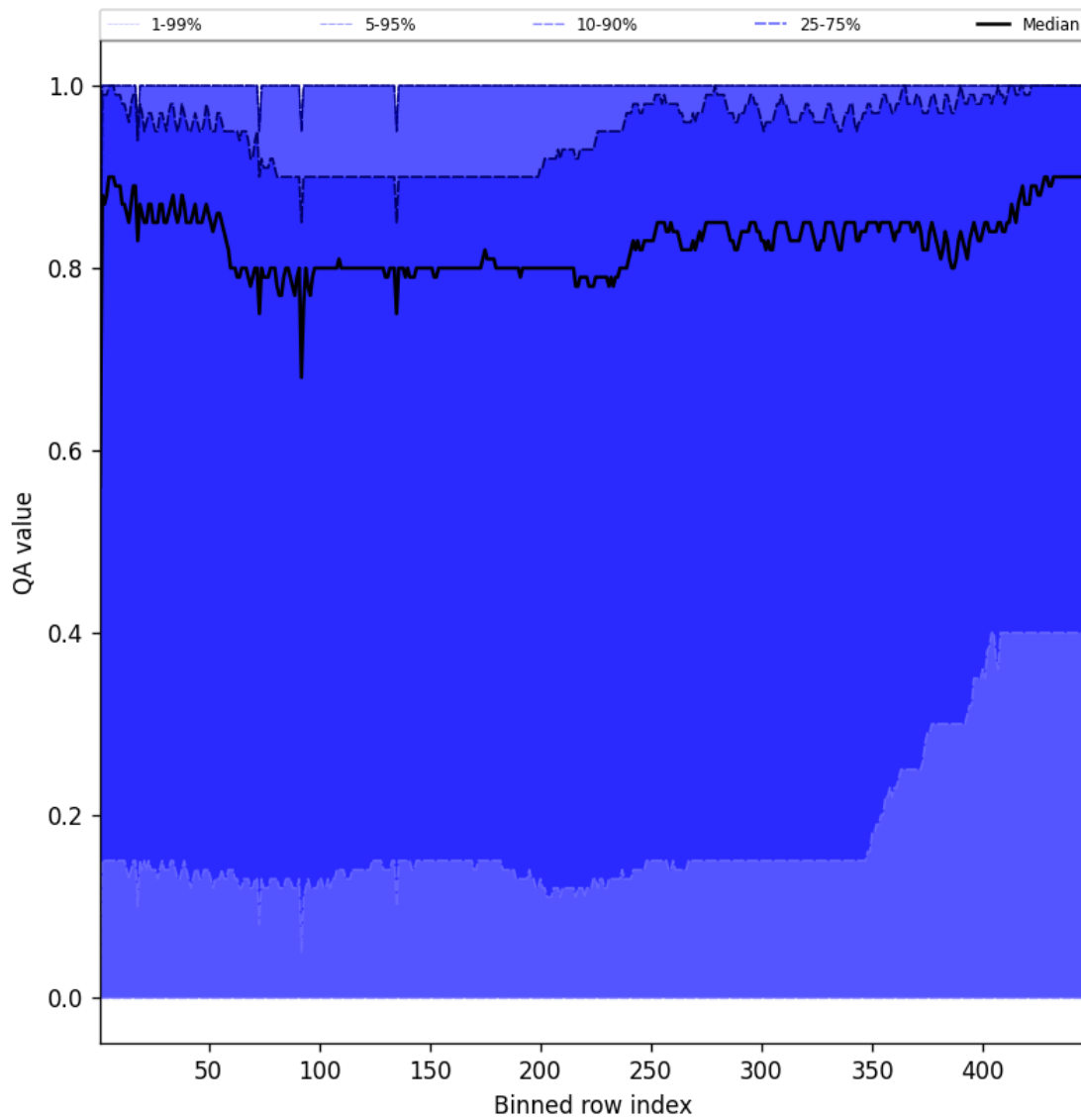
Figure 54: Along track statistics of “QA value” for 2024-10-03 to 2024-10-04
