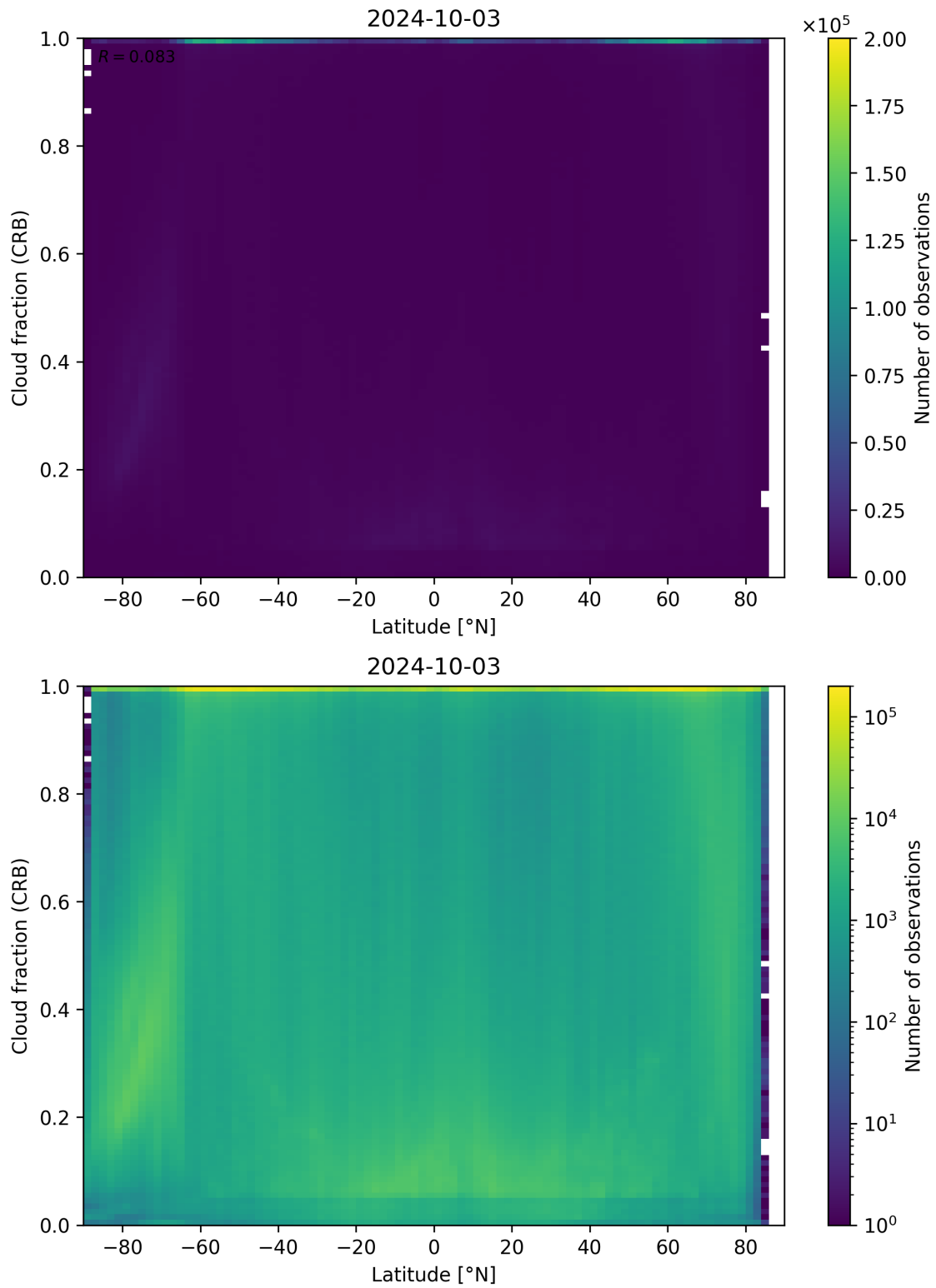
Figure 94: Scatter density plot of “Latitude” against “Cloud fraction (CRB)” for 2024-10-03 to 2024-10-04.
