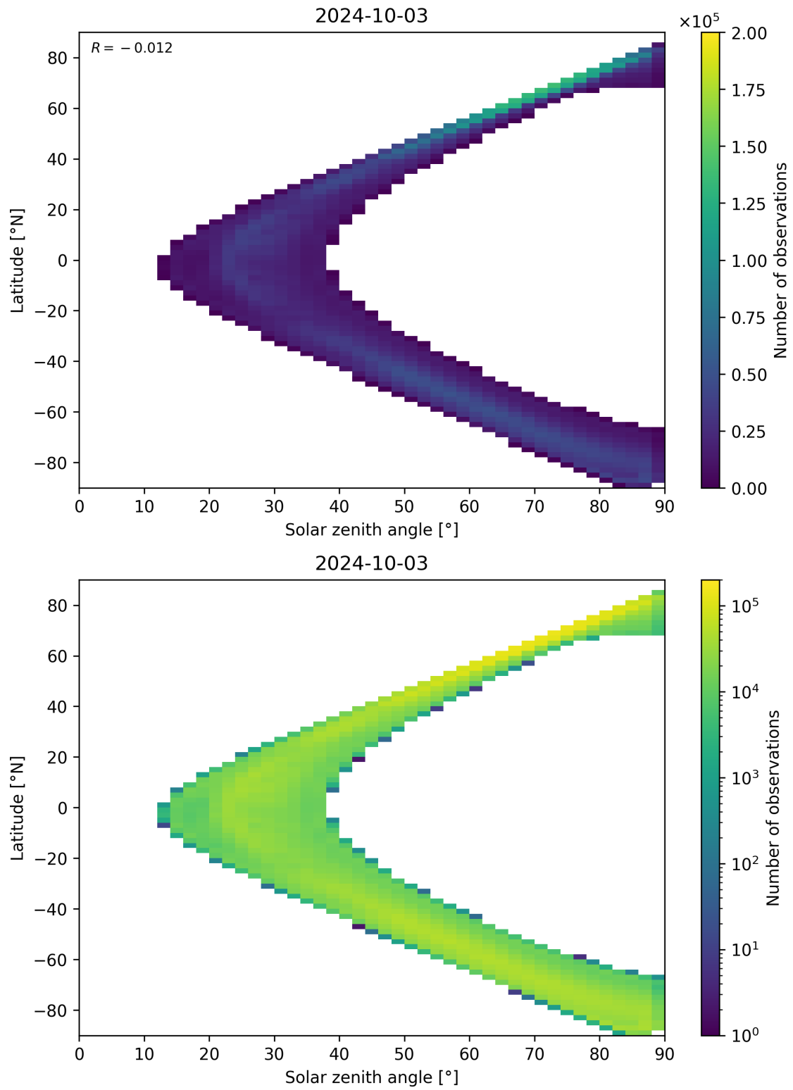
Figure 105: Scatter density plot of “Solar zenith angle” against “Latitude” for 2024-10-03 to 2024-10-04.
