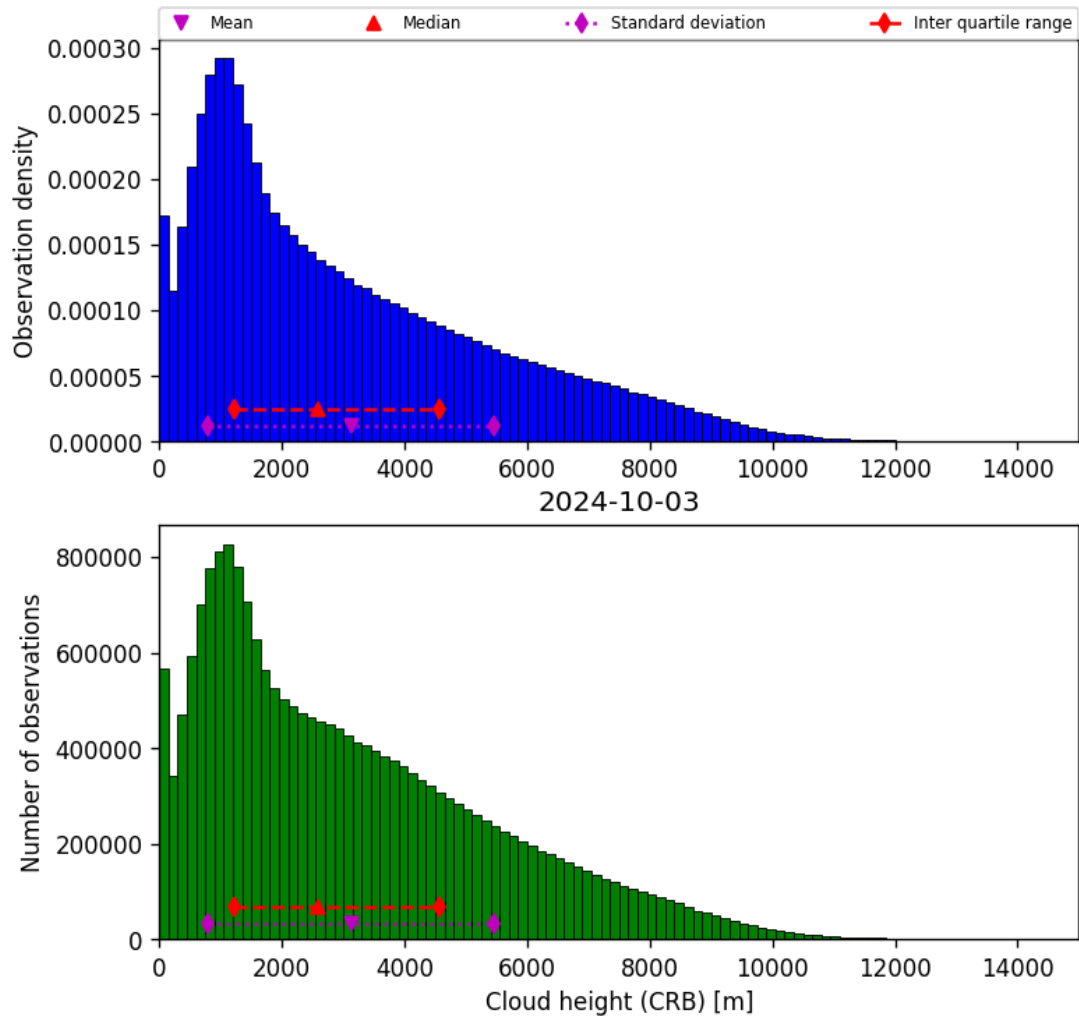
Figure 43: Histogram of “Cloud height (CRB)” for 2024-10-03 to 2024-10-04
