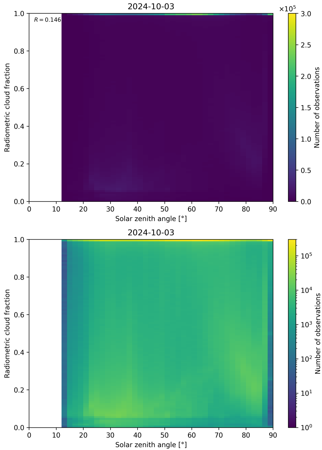
Figure 99: Scatter density plot of “Solar zenith angle” against “Radiometric cloud fraction” for 2024-10-03 to 2024-10-04.
