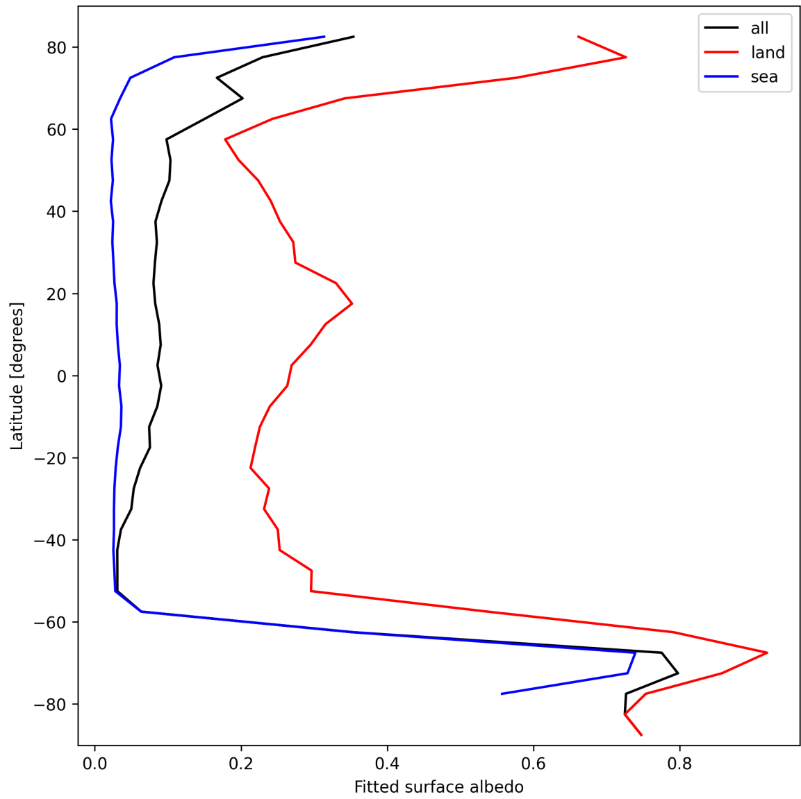
Figure 29: Zonal average of “Fitted surface albedo” for 2024-10-03 to 2024-10-04.
