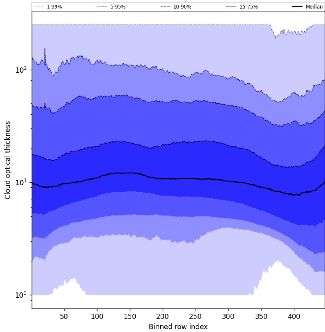
Figure 57: Along track statistics of “Cloud optical thickness” for 2024-10-03 to 2024-10-04
