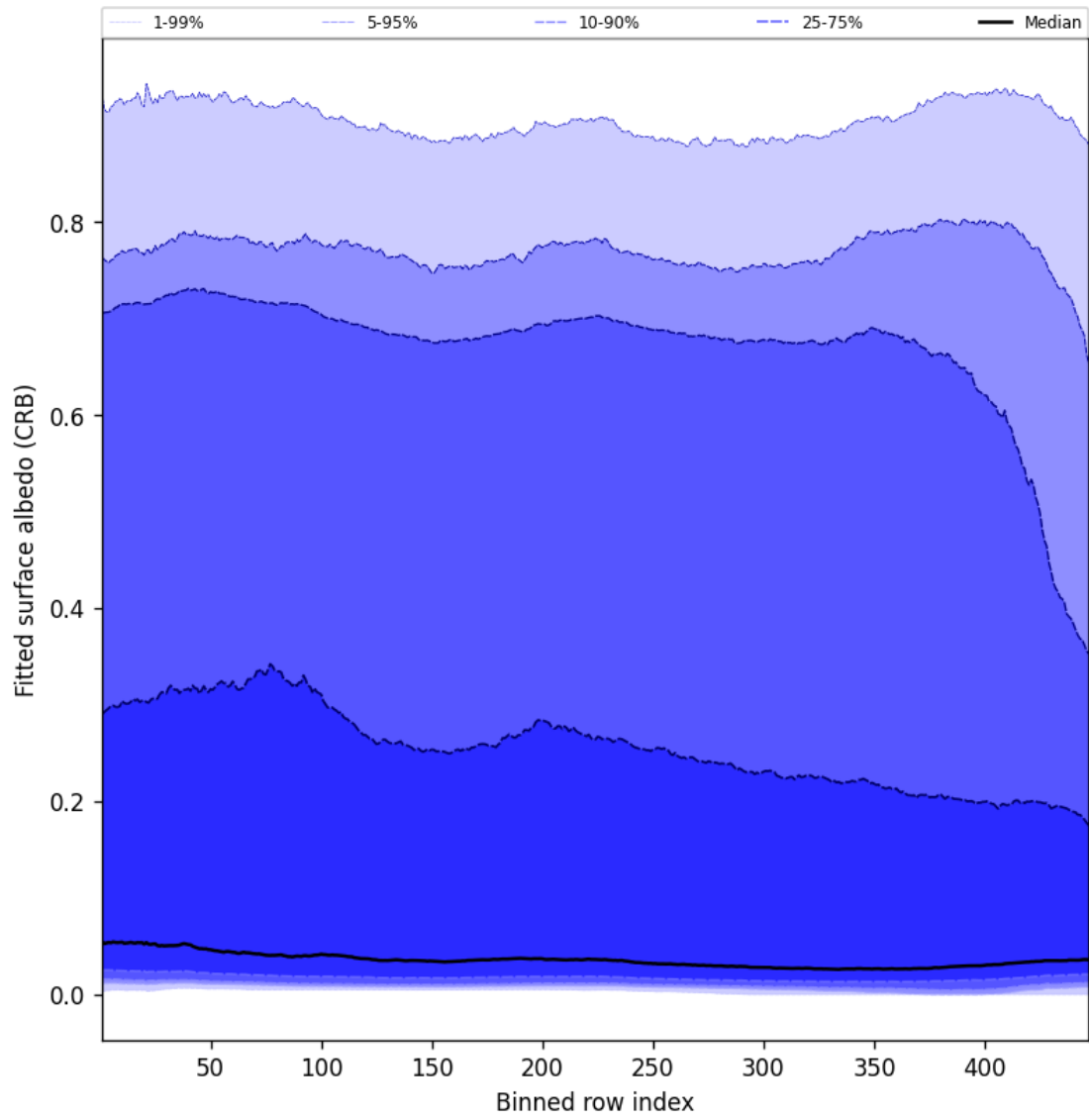
Figure 62: Along track statistics of “Fitted surface albedo (CRB)” for 2024-10-03 to 2024-10-04
