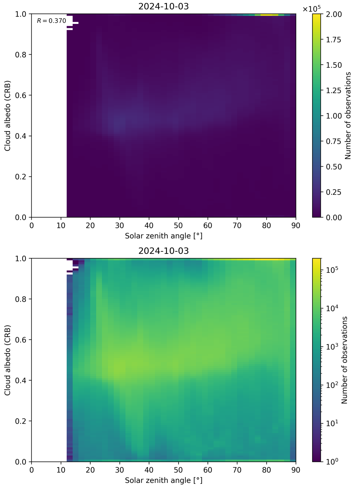
Figure 98: Scatter density plot of “Solar zenith angle” against “Cloud albedo (CRB)” for 2024-10-03 to 2024-10-04.
