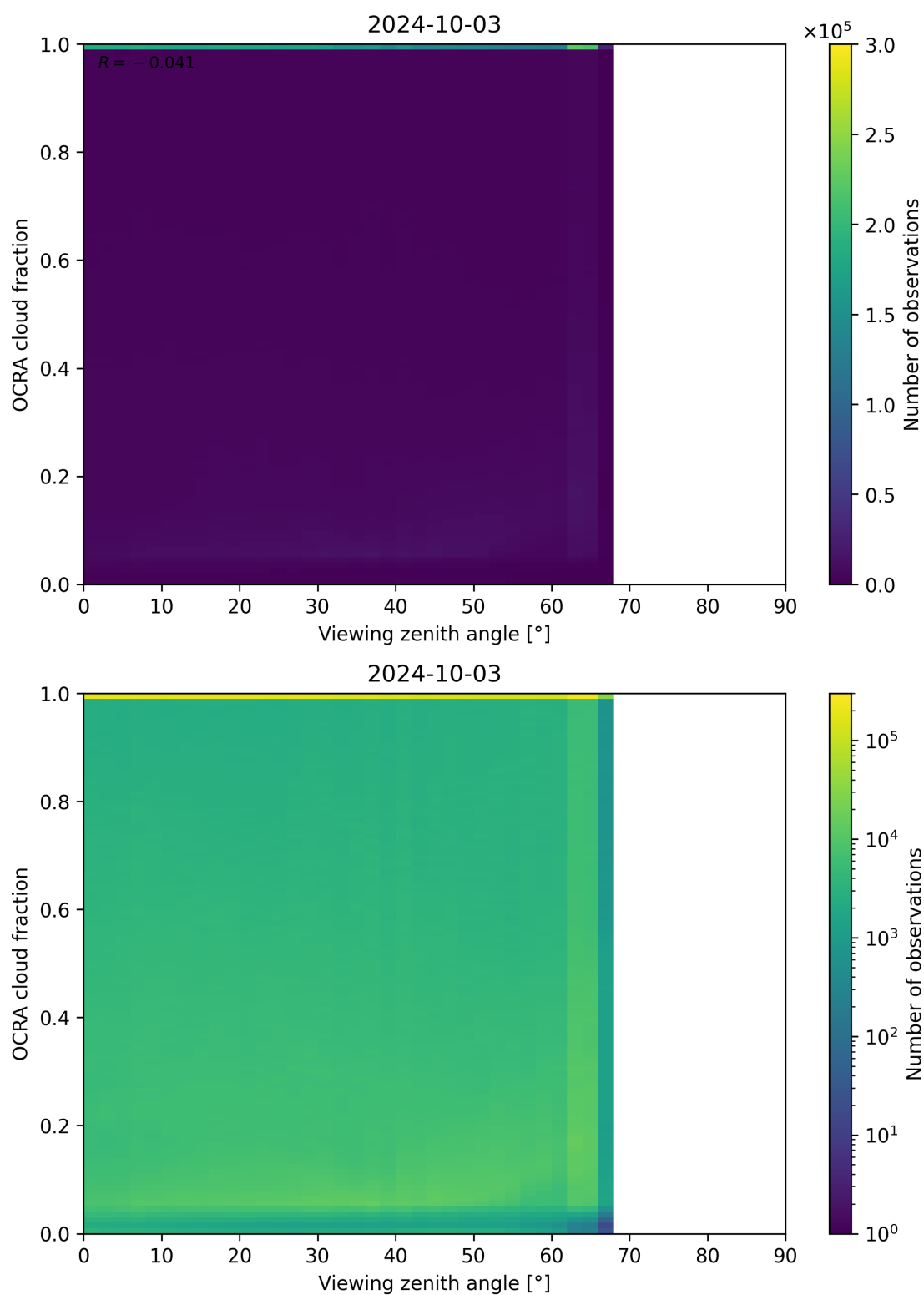
Figure 108: Scatter density plot of “Viewing zenith angle” against “OCRA cloud fraction” for 2024-10-03 to 2024-10-04.
