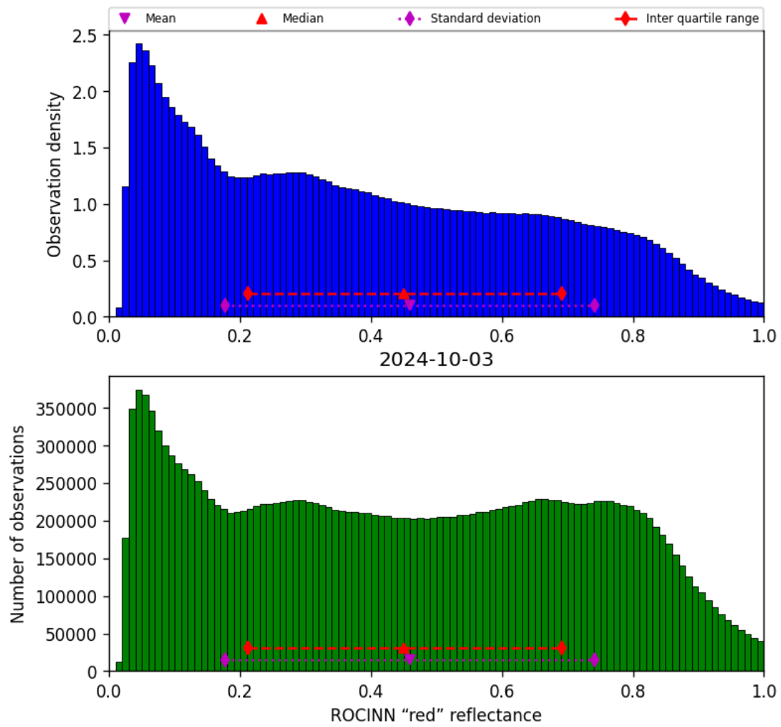
Figure 53: Histogram of “ROCINN “red” reflectance” for 2024-10-03 to 2024-10-04
