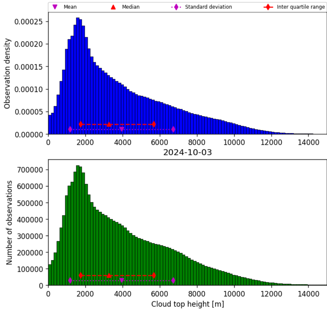
Figure 40: Histogram of “Cloud top height” for 2024-10-03 to 2024-10-04
