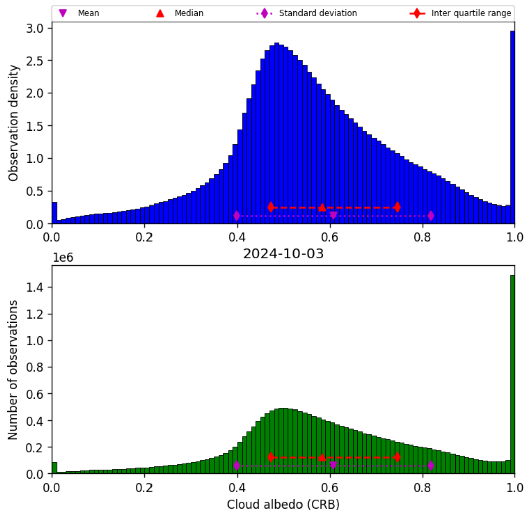
Figure 44: Histogram of “Cloud albedo (CRB)” for 2024-10-03 to 2024-10-04
