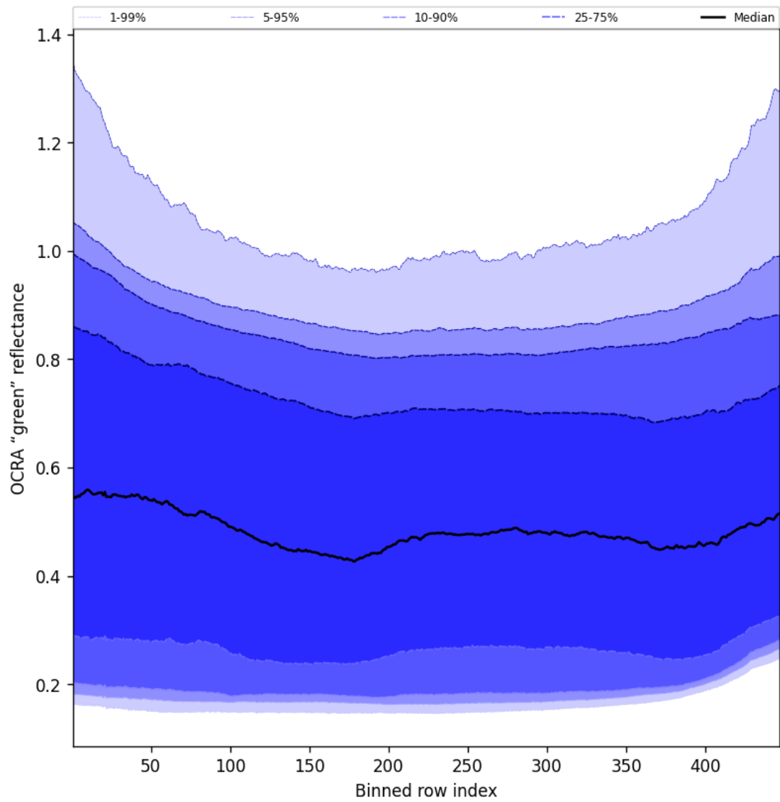
Figure 68: Along track statistics of “OCRA “green” reflectance” for 2024-10-03 to 2024-10-04
