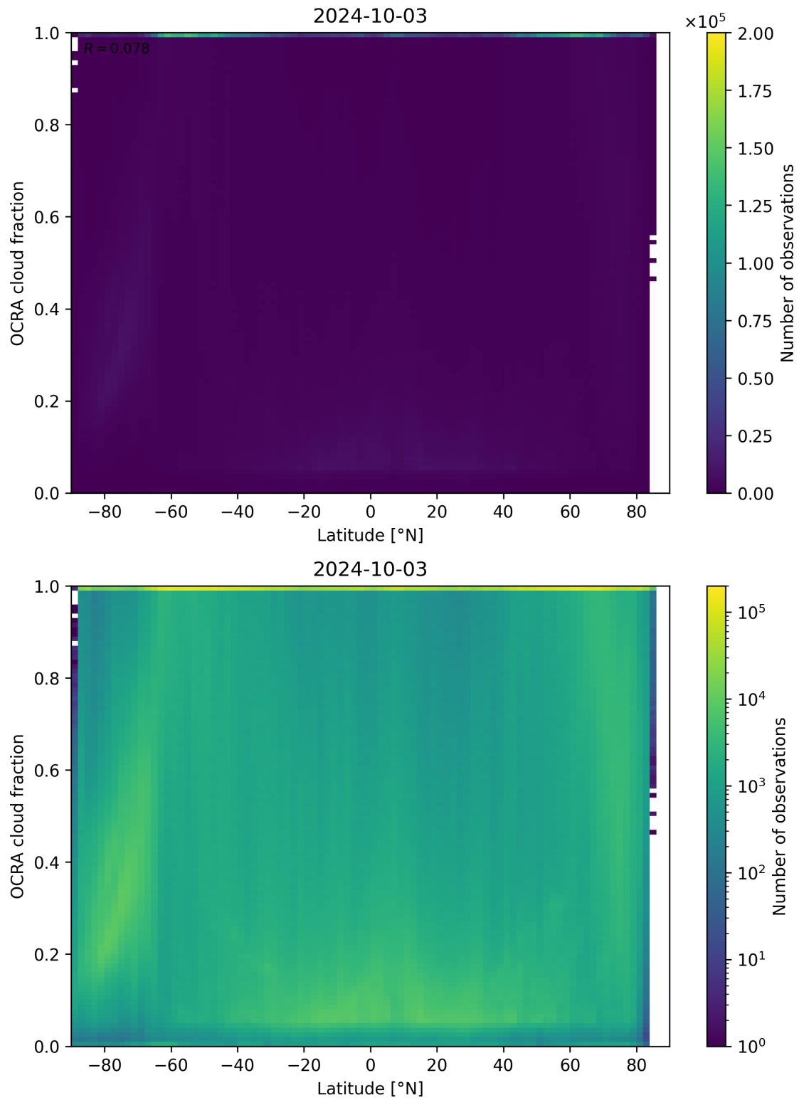
Figure 93: Scatter density plot of “Latitude” against “OCRA cloud fraction” for 2024-10-03 to 2024-10-04.
