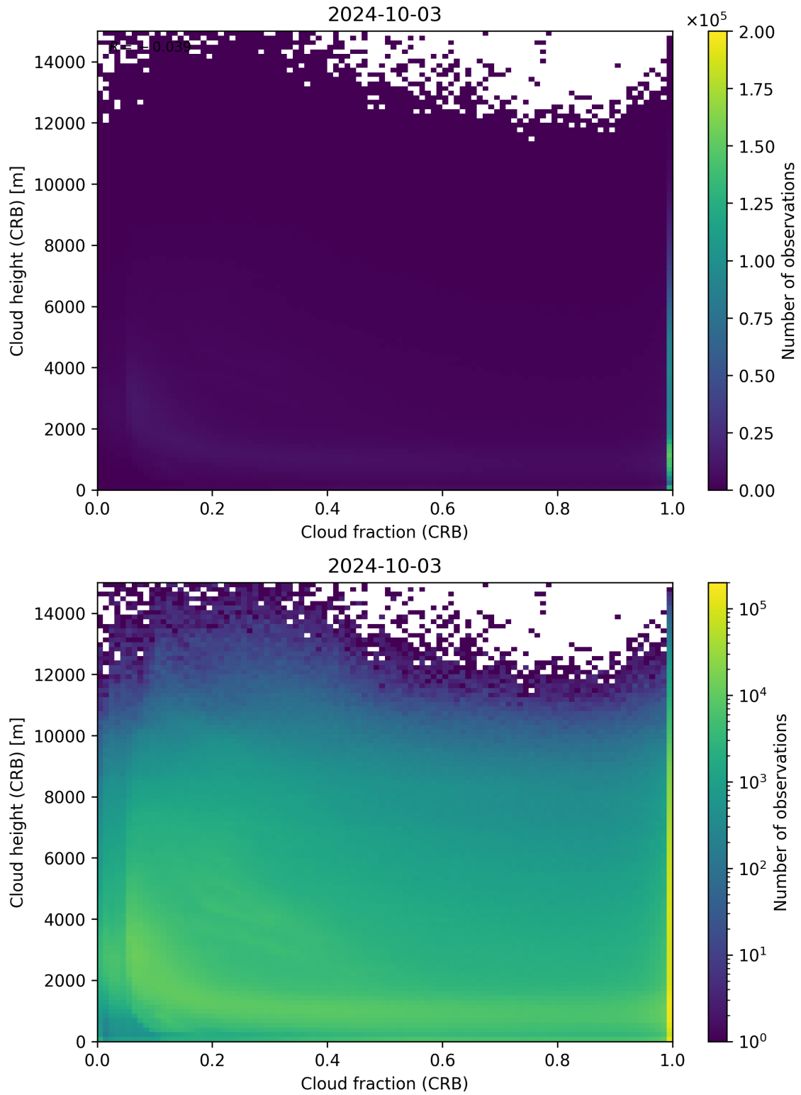
Figure 79: Scatter density plot of “Cloud fraction (CRB)” against “Cloud height (CRB)” for 2024-10-03 to 2024-10-04.
