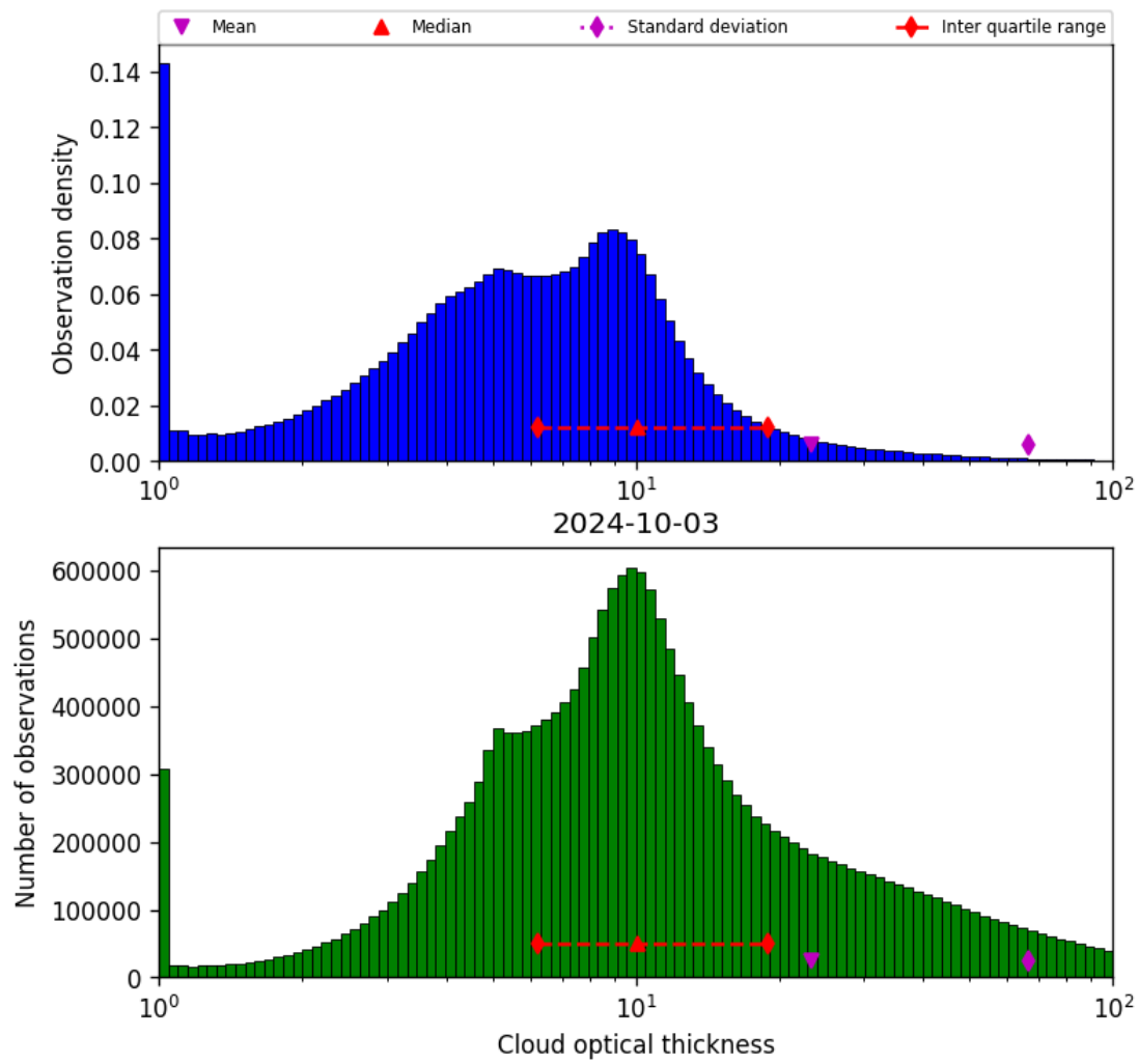
Figure 41: Histogram of “Cloud optical thickness” for 2024-10-03 to 2024-10-04
