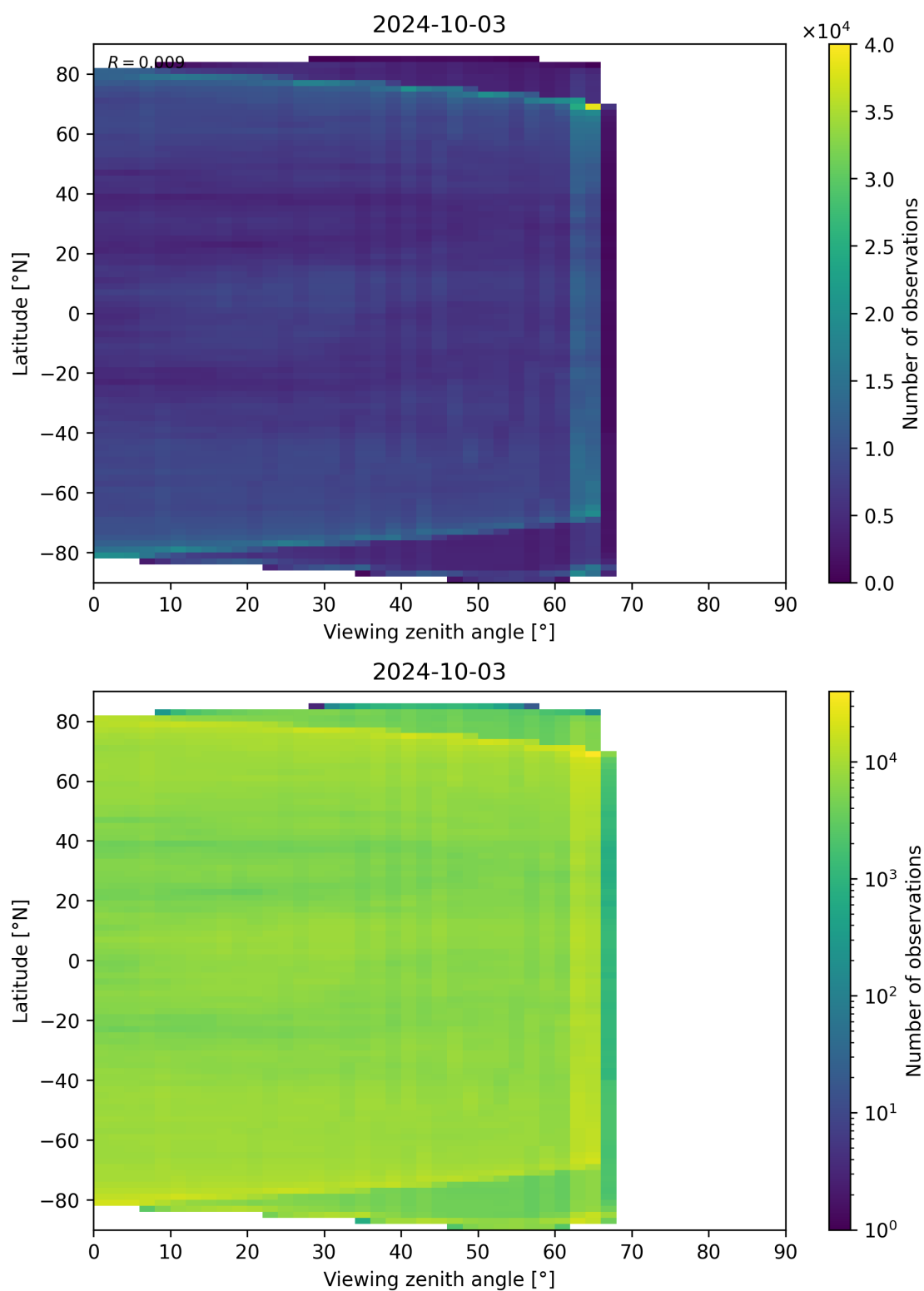
Figure 113: Scatter density plot of “Viewing zenith angle” against “Latitude” for 2024-10-03 to 2024-10-04.
