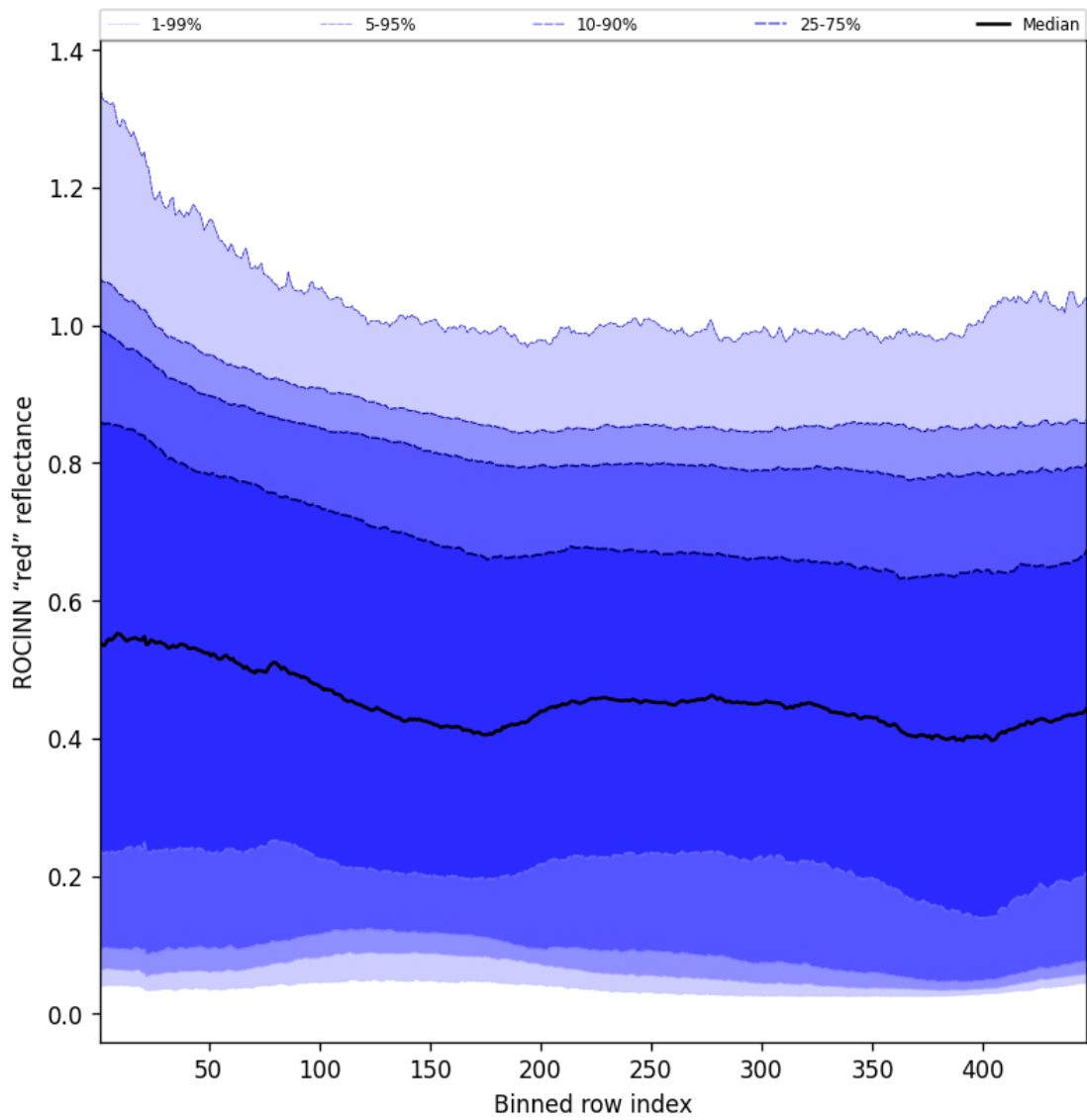
Figure 69: Along track statistics of "ROCINN "red" reflectance" for 2024-10-03 to 2024-10-04
