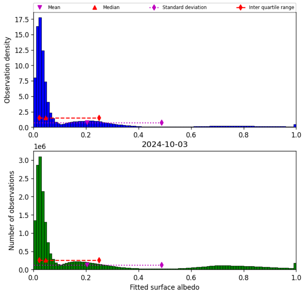
Figure 45: Histogram of “Fitted surface albedo” for 2024-10-03 to 2024-10-04
