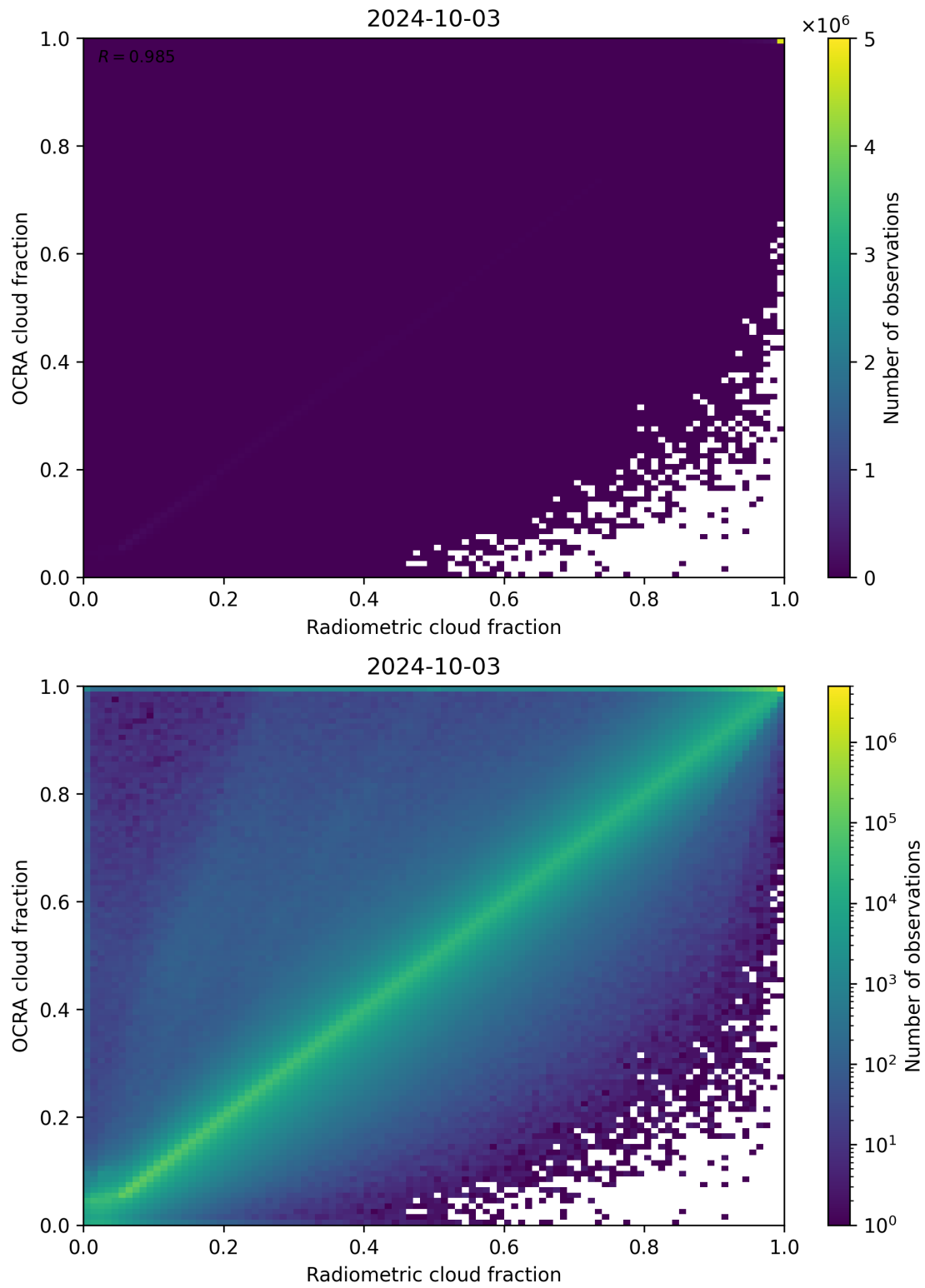
Figure 72: Scatter density plot of “Radiometric cloud fraction” against “OCRA cloud fraction” for 2024-10-03 to 2024-10-04.
