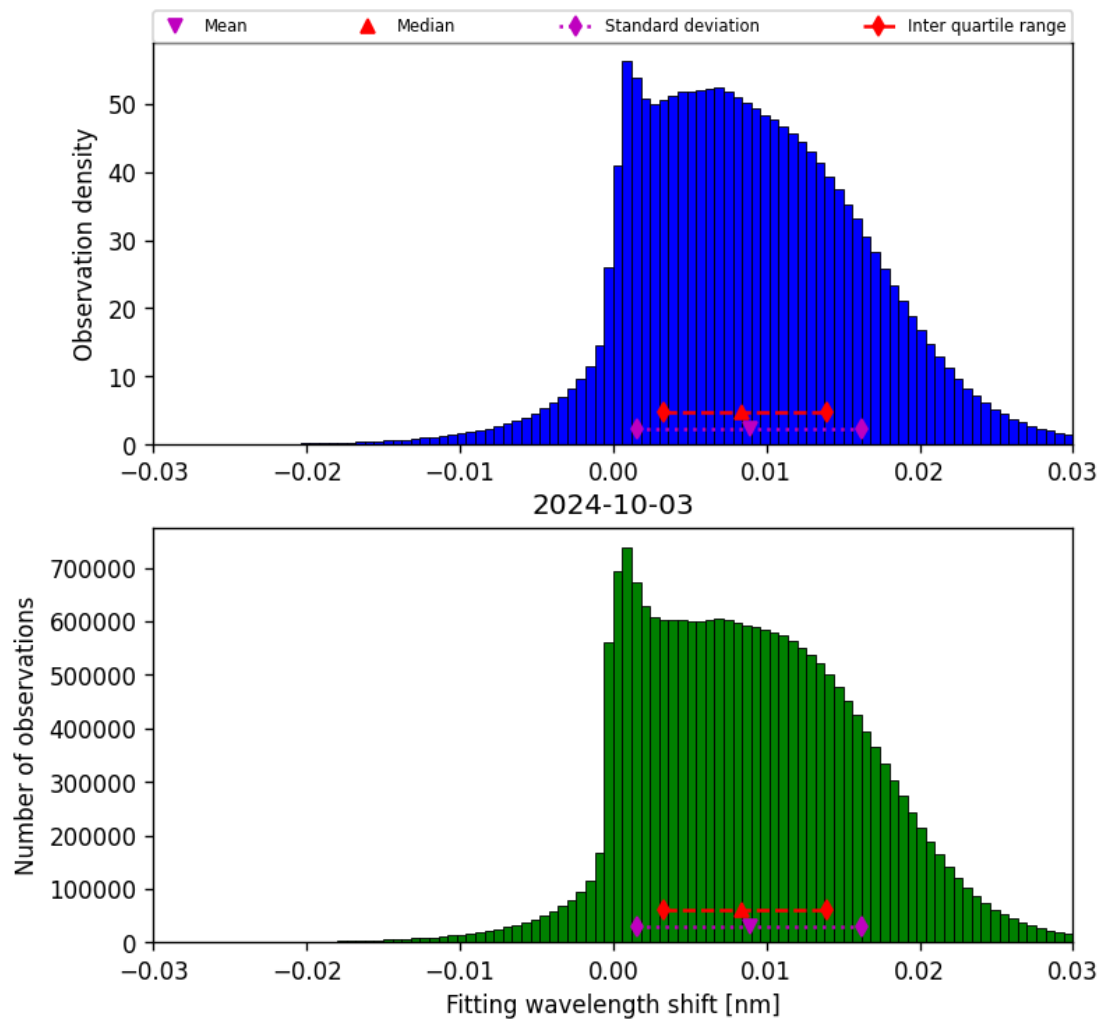
Figure 49: Histogram of “Fitting wavelength shift” for 2024-10-03 to 2024-10-04
