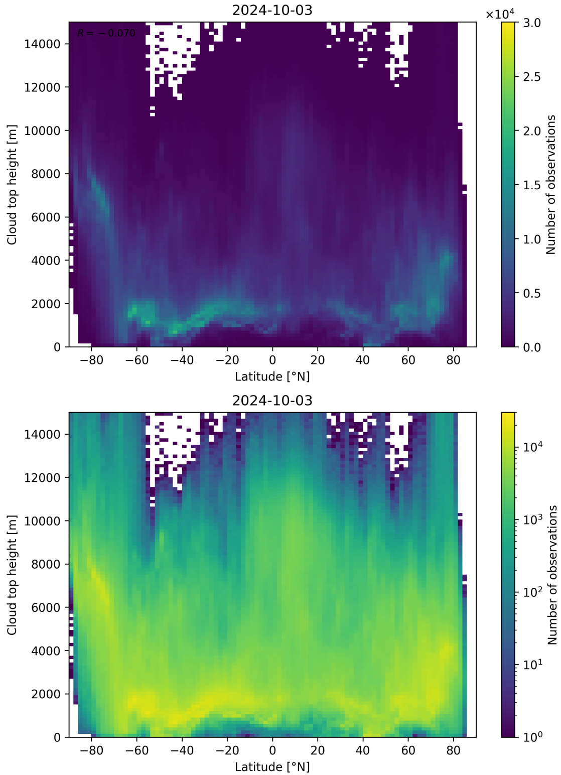
Figure 97: Scatter density plot of “Latitude” against “Cloud top height” for 2024-10-03 to 2024-10-04.
