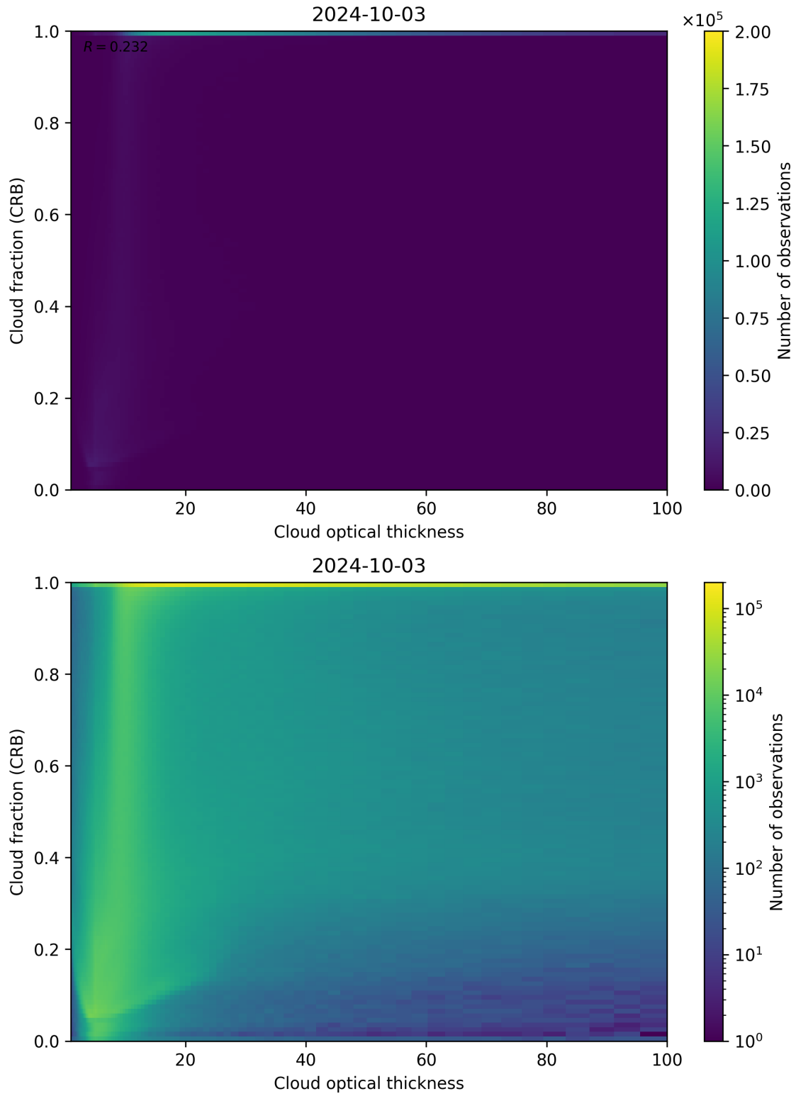
Figure 84: Scatter density plot of “Cloud optical thickness” against “Cloud fraction (CRB)” for 2024-10-03 to 2024-10-04.
