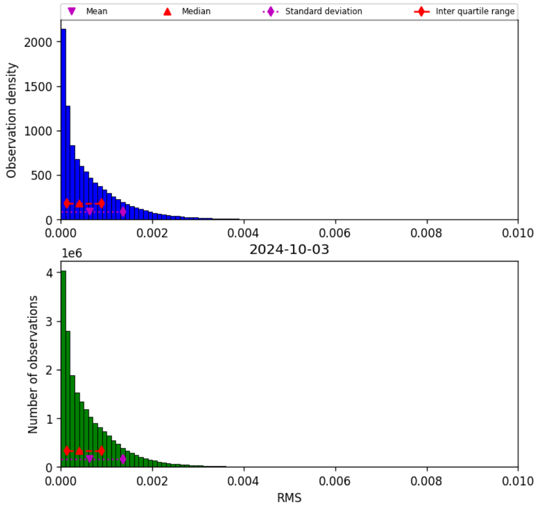
Figure 47: Histogram of “RMS” for 2024-10-03 to 2024-10-04
