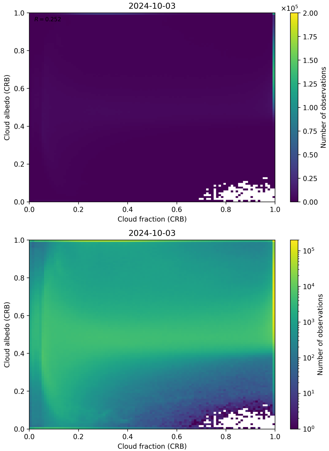
Figure 77: Scatter density plot of “Cloud fraction (CRB)” against “Cloud albedo (CRB)” for 2024-10-03 to 2024-10-04.
