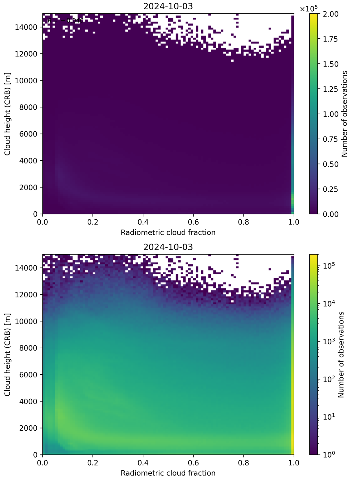
Figure 74: Scatter density plot of “Radiometric cloud fraction” against “Cloud height (CRB)” for 2024-10-03 to 2024-10-04.
