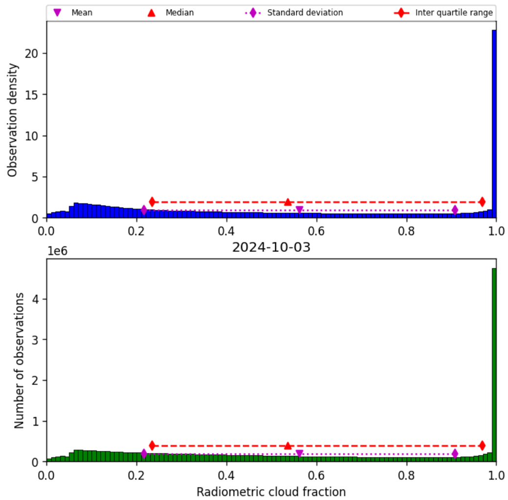
Figure 39: Histogram of “Radiometric cloud fraction” for 2024-10-03 to 2024-10-04
