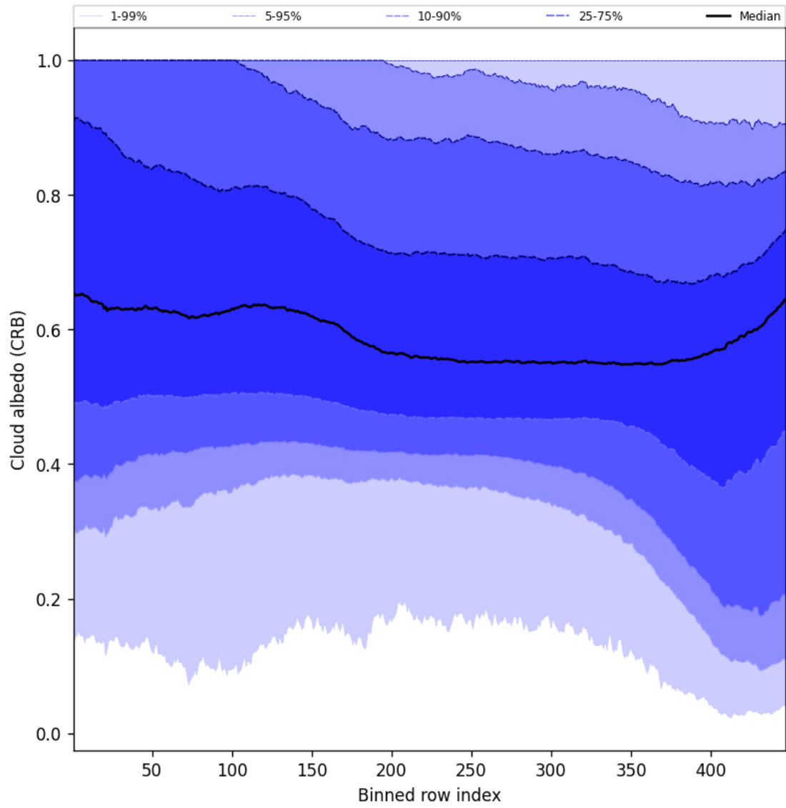
Figure 60: Along track statistics of “Cloud albedo (CRB)” for 2024-10-03 to 2024-10-04
