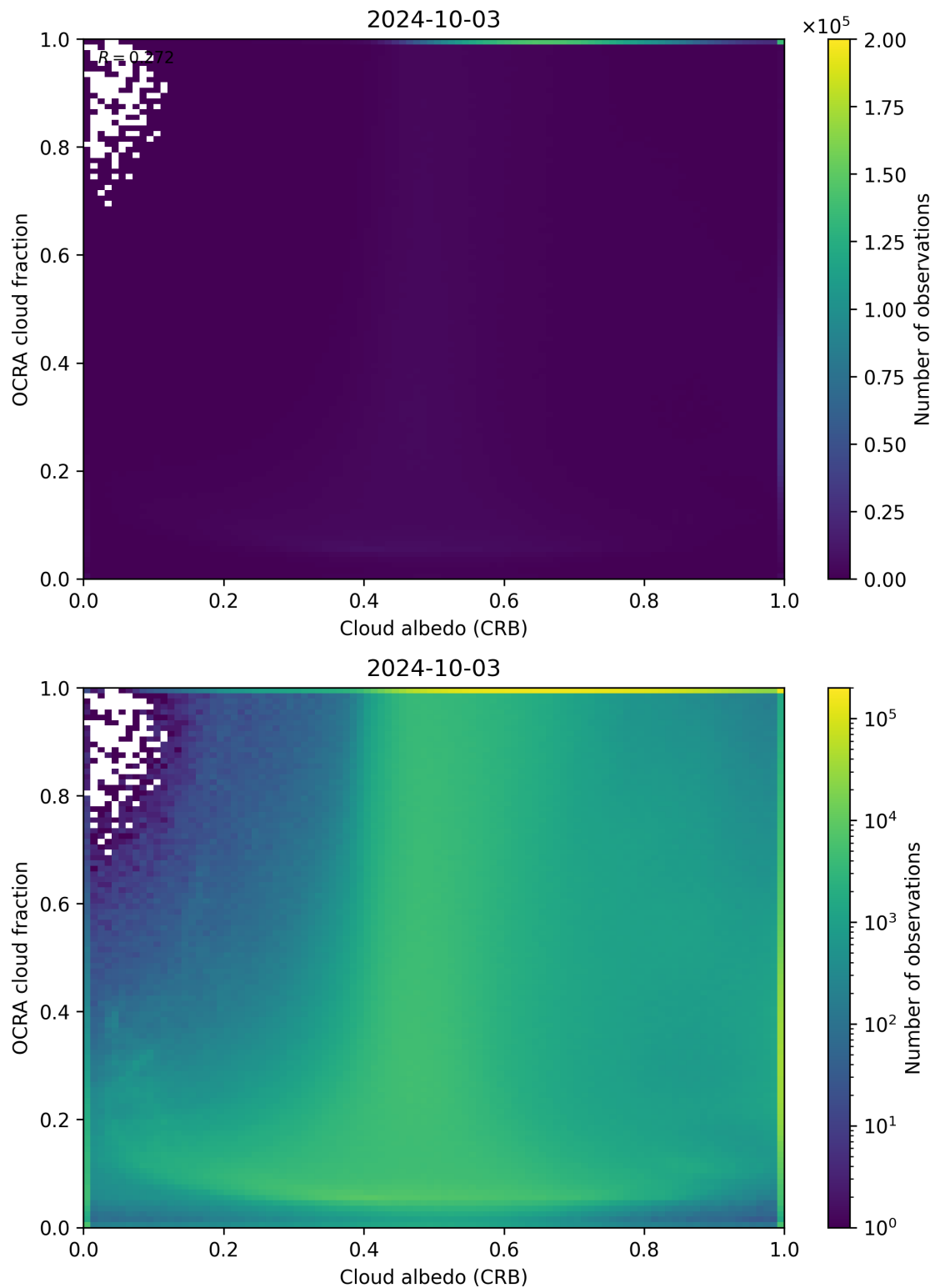
Figure 70: Scatter density plot of “Cloud albedo (CRB)” against “OCRA cloud fraction” for 2024-10-03 to 2024-10-04.
