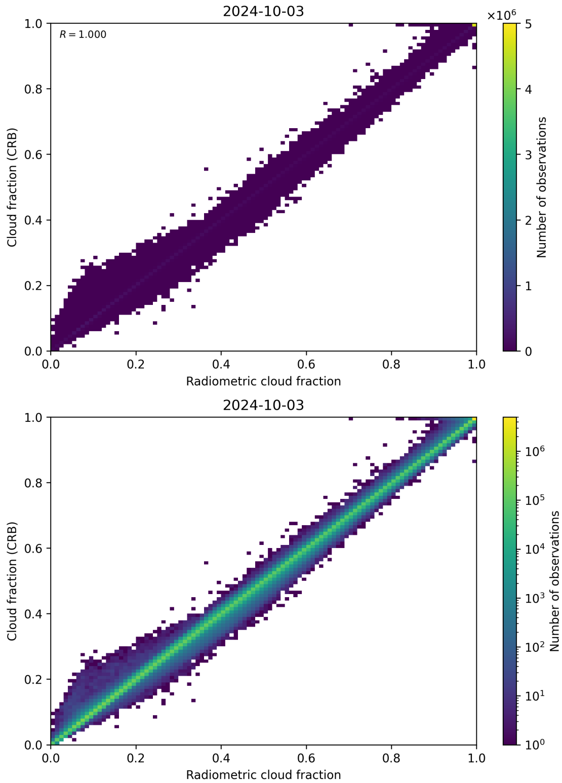
Figure 73: Scatter density plot of “Radiometric cloud fraction” against “Cloud fraction (CRB)” for 2024-10-03 to 2024-10-04.
