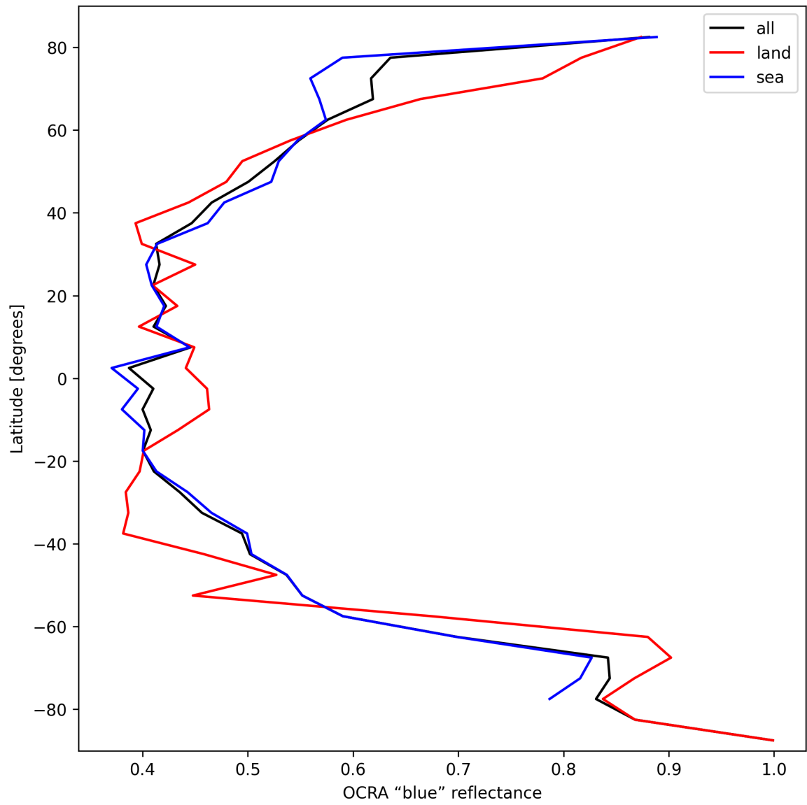
Figure 35: Zonal average of “OCRA “blue” reflectance” for 2024-10-03 to 2024-10-04.
