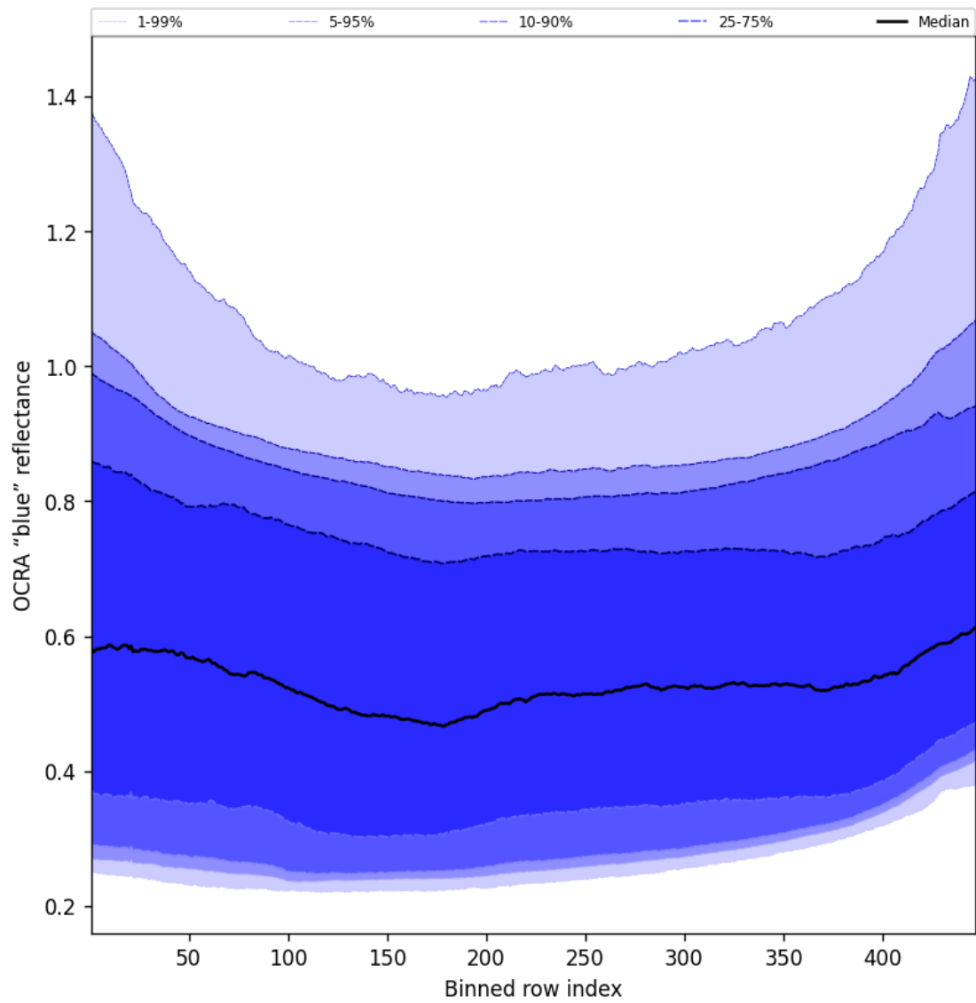
Figure 67: Along track statistics of "OCRA "blue" reflectance" for 2024-10-03 to 2024-10-04
