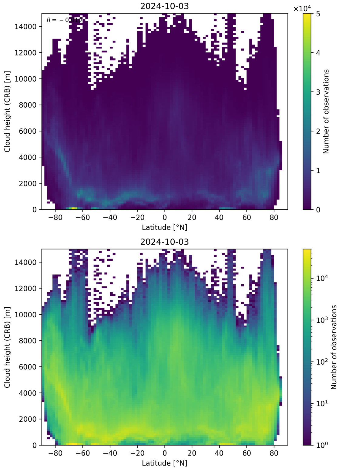
Figure 95: Scatter density plot of “Latitude” against “Cloud height (CRB)” for 2024-10-03 to 2024-10-04.
