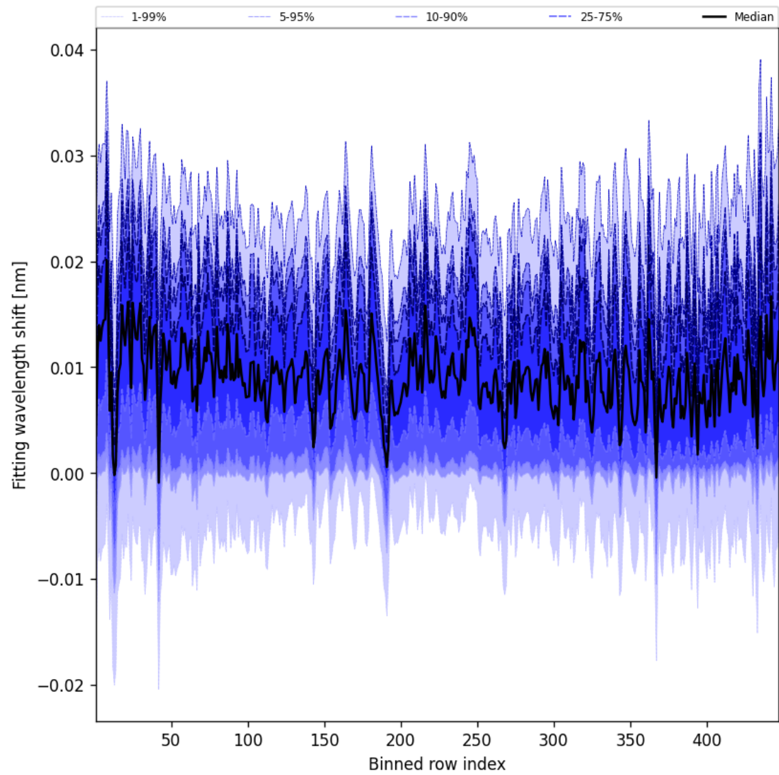
Figure 65: Along track statistics of “Fitting wavelength shift” for 2024-10-03 to 2024-10-04
