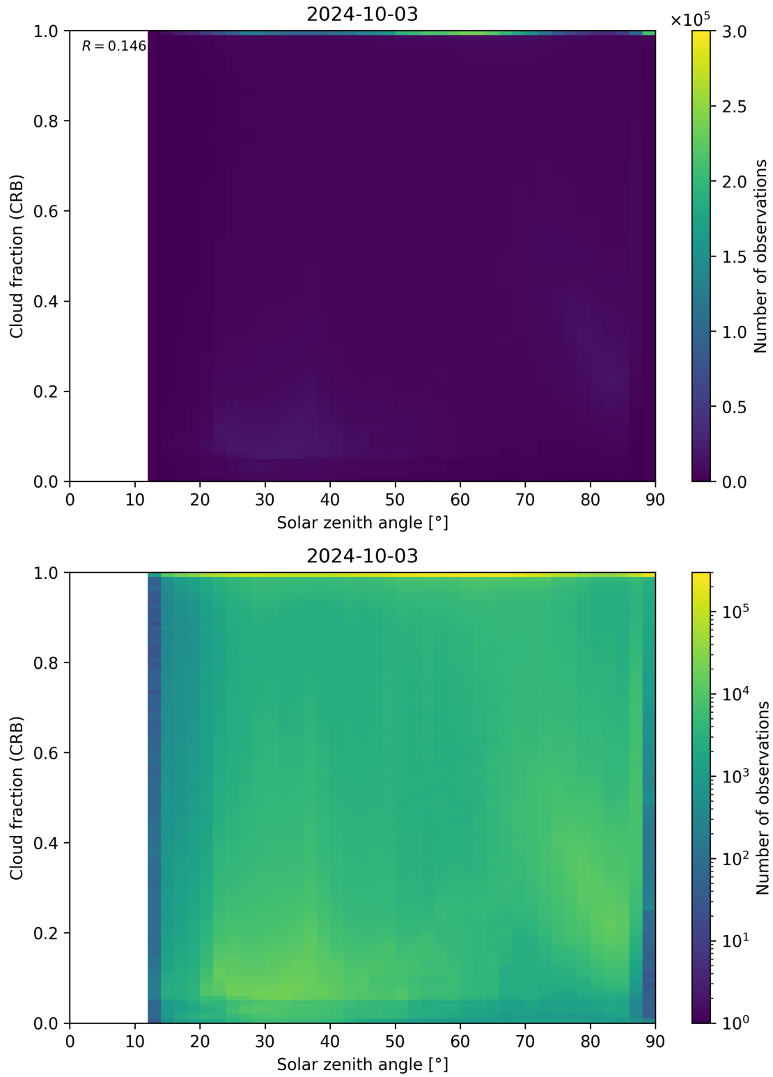
Figure 101: Scatter density plot of “Solar zenith angle” against “Cloud fraction (CRB)” for 2024-10-03 to 2024-10-04.
