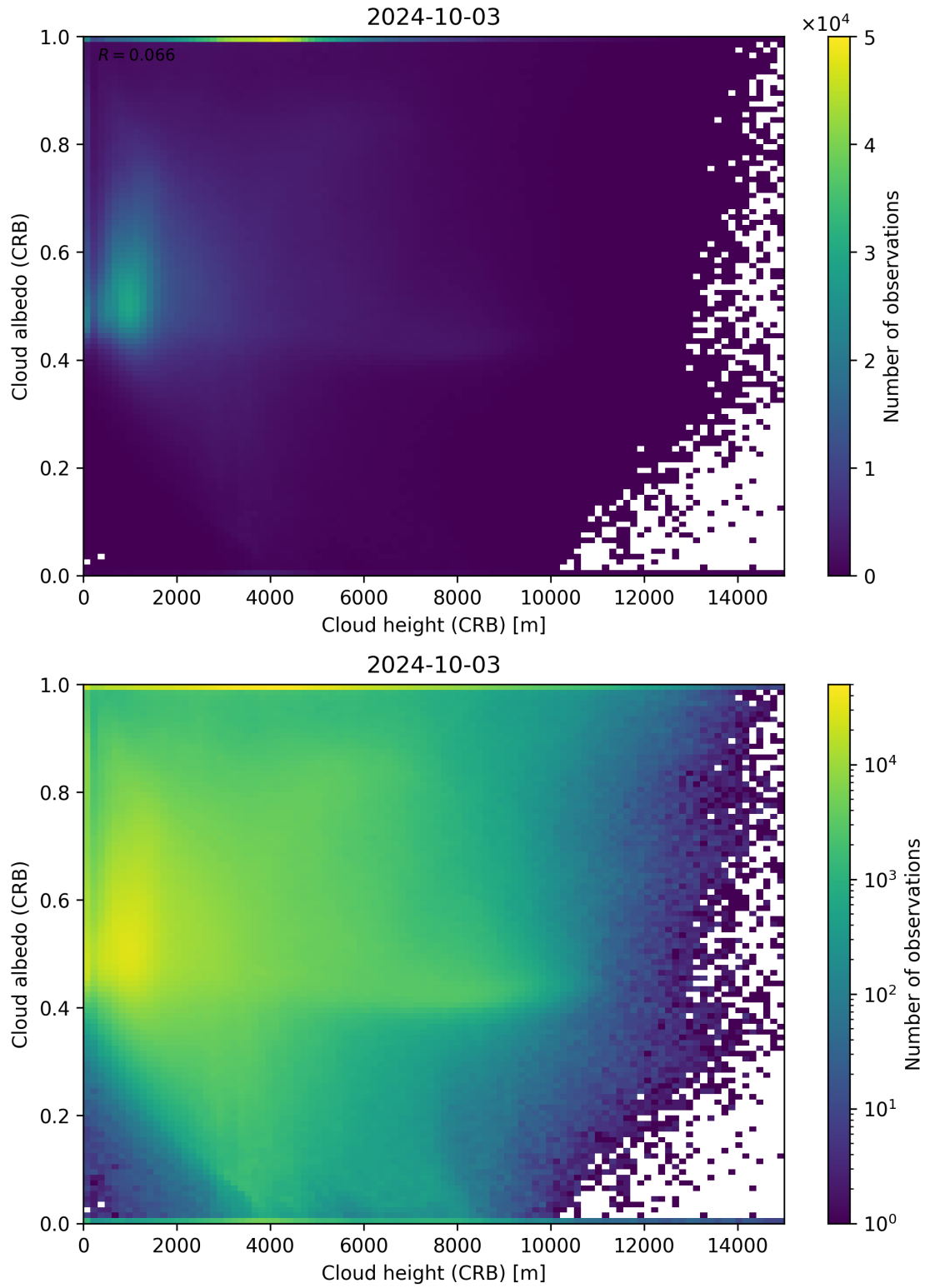
Figure 80: Scatter density plot of “Cloud height (CRB)” against “Cloud albedo (CRB)” for 2024-10-03 to 2024-10-04.
