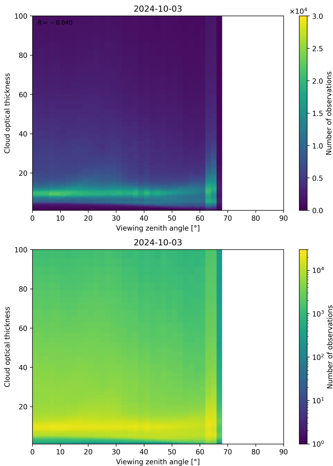
Figure 111: Scatter density plot of “Viewing zenith angle” against “Cloud optical thickness” for 2024-10-03 to 2024-10-04.
