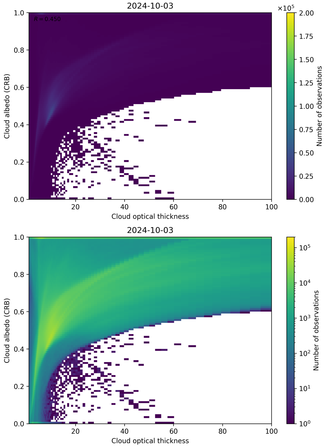
Figure 82: Scatter density plot of “Cloud optical thickness” against “Cloud albedo (CRB)” for 2024-10-03 to 2024-10-04.
