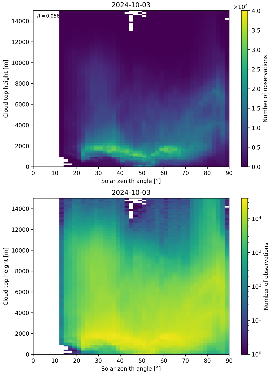
Figure 104: Scatter density plot of “Solar zenith angle” against “Cloud top height” for 2024-10-03 to 2024-10-04.
