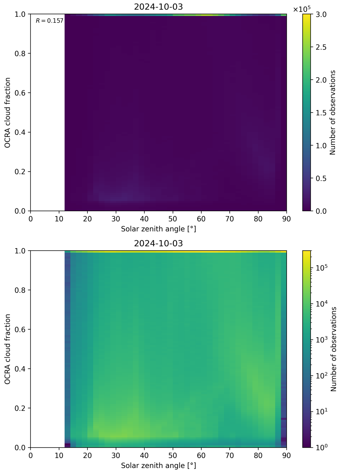
Figure 100: Scatter density plot of “Solar zenith angle” against “OCRA cloud fraction” for 2024-10-03 to 2024-10-04.
