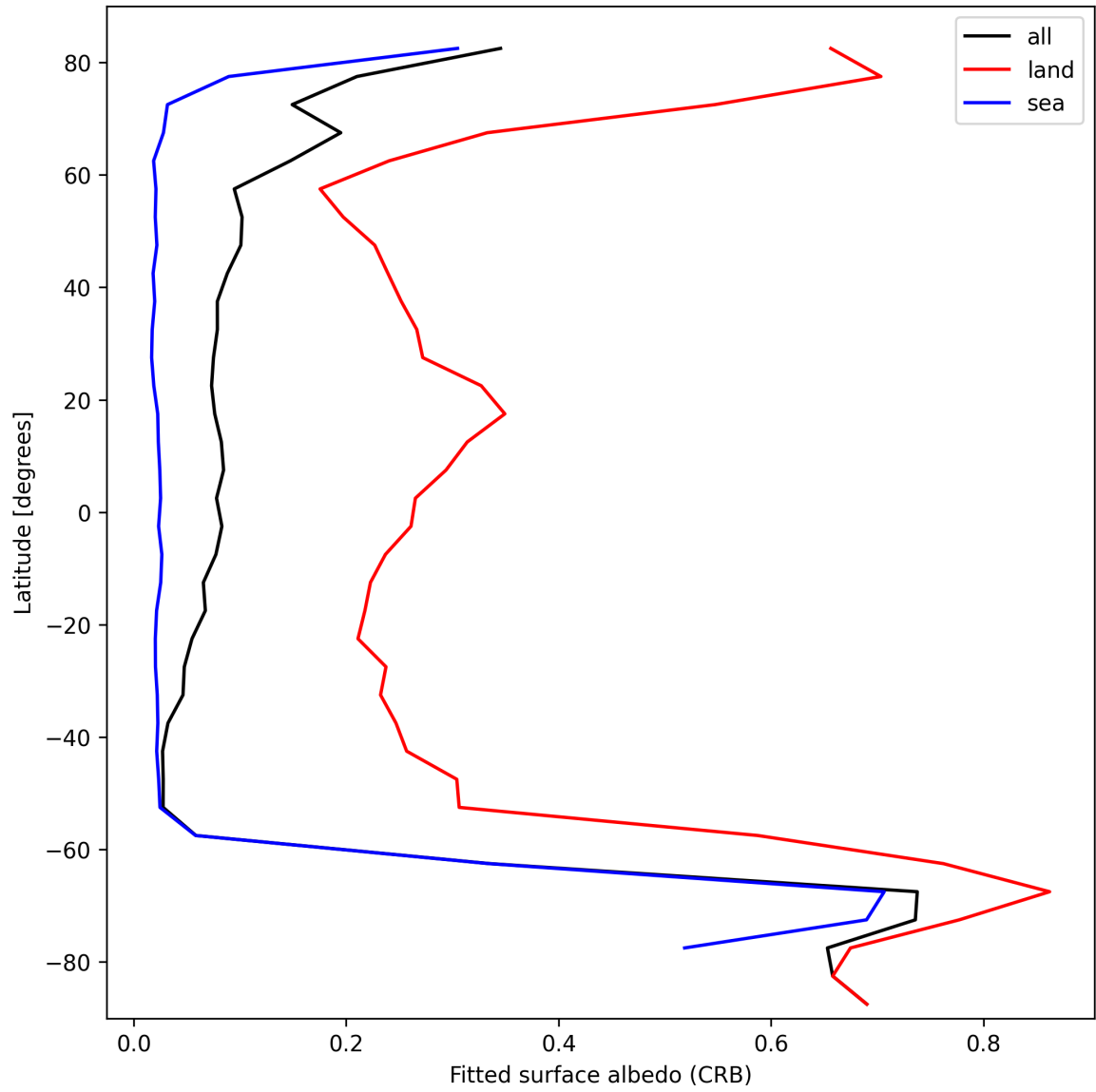
Figure 30: Zonal average of “Fitted surface albedo (CRB)” for 2024-10-03 to 2024-10-04.
