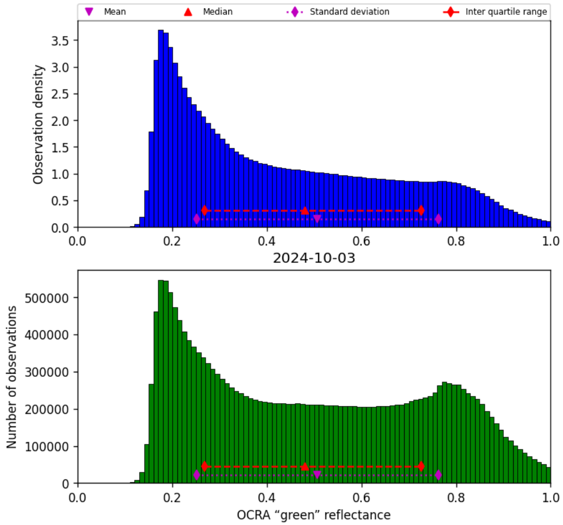
Figure 52: Histogram of “OCRA “green” reflectance” for 2024-10-03 to 2024-10-04
