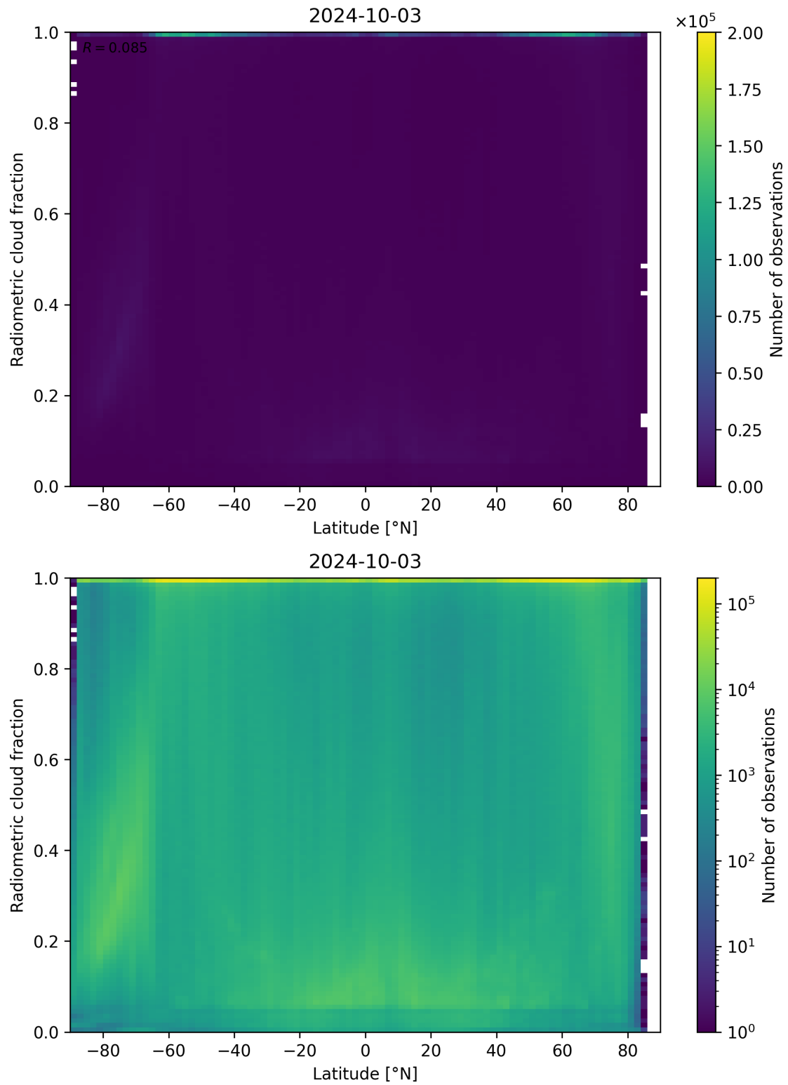
Figure 92: Scatter density plot of “Latitude” against “Radiometric cloud fraction” for 2024-10-03 to 2024-10-04.
