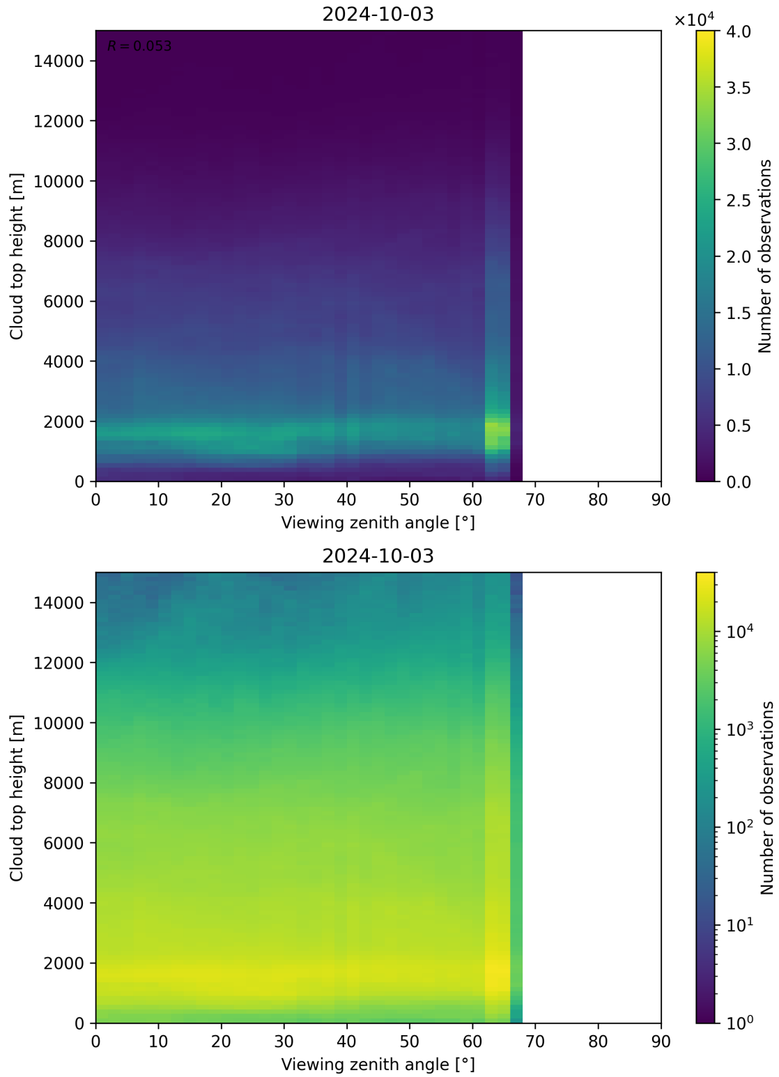
Figure 112: Scatter density plot of “Viewing zenith angle” against “Cloud top height” for 2024-10-03 to 2024-10-04.
