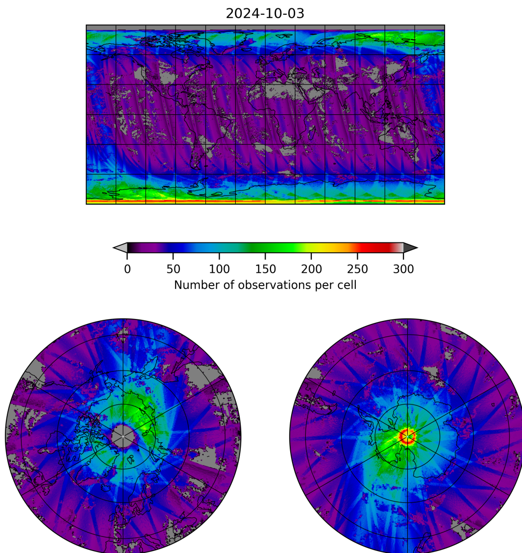
Figure 21: Map of the number of observations for 2024-10-03 to 2024-10-04
