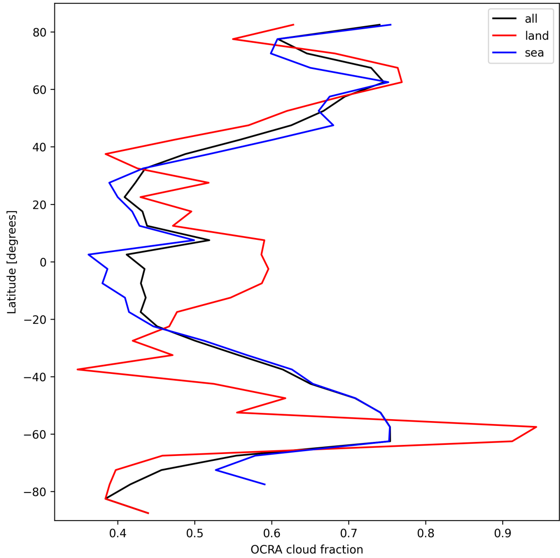
Figure 34: Zonal average of “OCRA cloud fraction” for 2024-10-03 to 2024-10-04.
