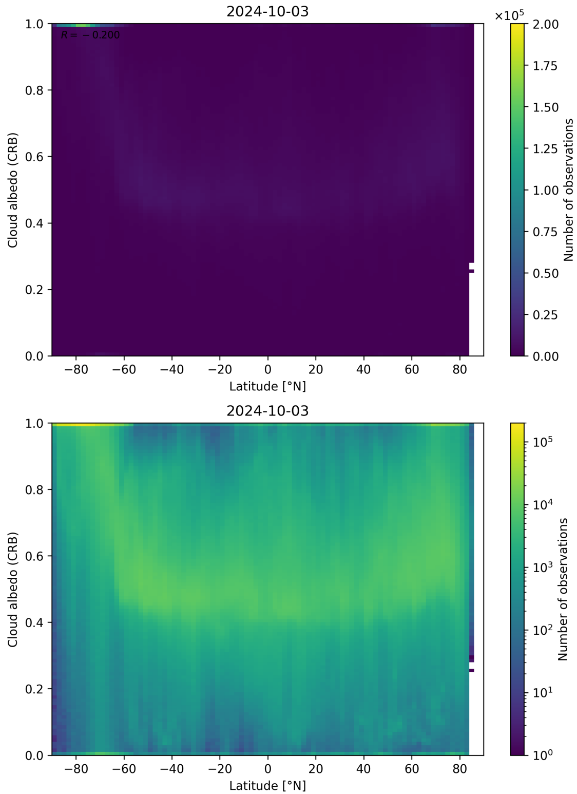
Figure 91: Scatter density plot of “Latitude” against “Cloud albedo (CRB)” for 2024-10-03 to 2024-10-04.
