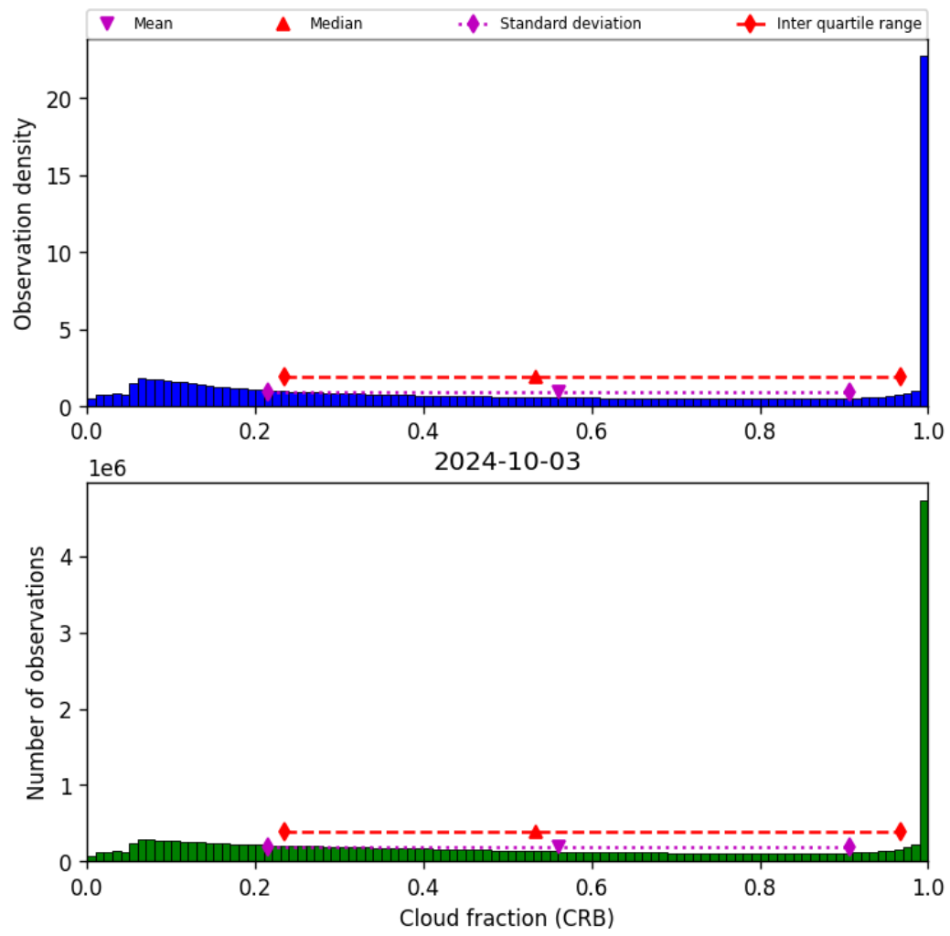
Figure 42: Histogram of “Cloud fraction (CRB)” for 2024-10-03 to 2024-10-04
