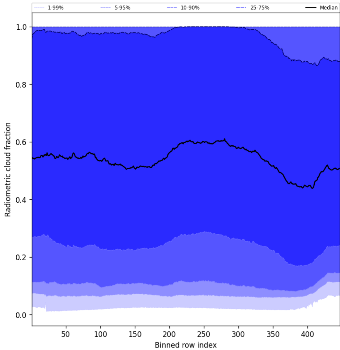
Figure 55: Along track statistics of “Radiometric cloud fraction” for 2024-10-03 to 2024-10-04
