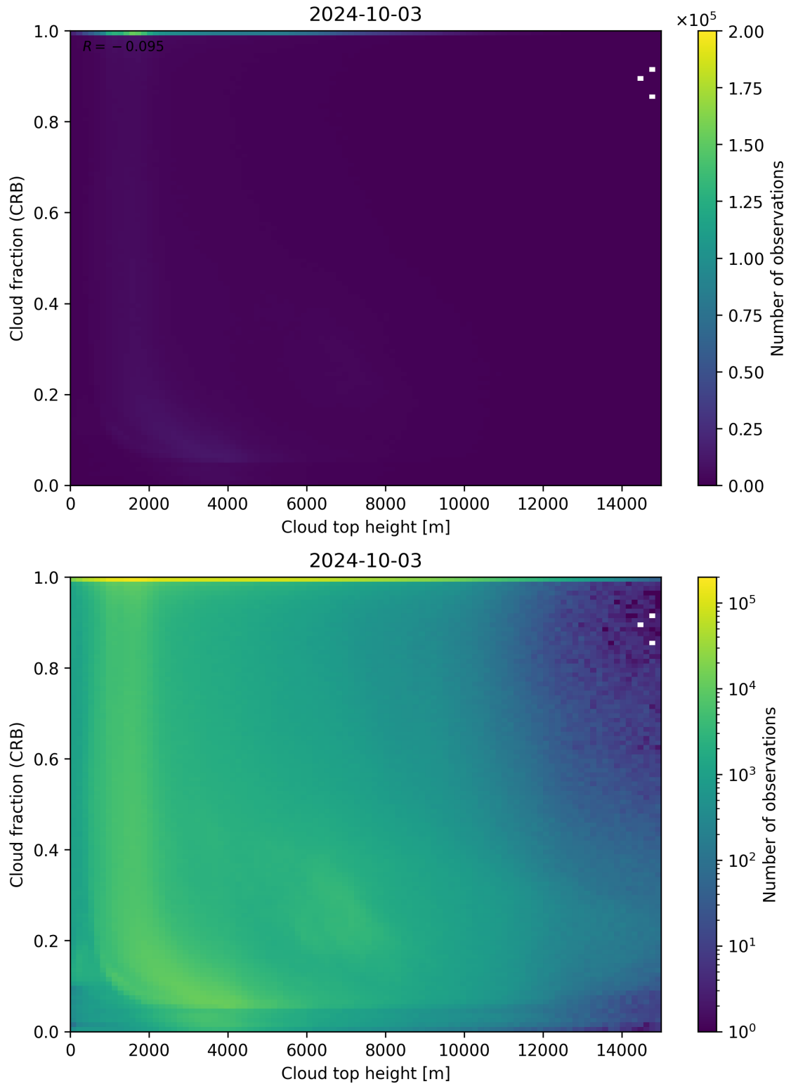
Figure 88: Scatter density plot of “Cloud top height” against “Cloud fraction (CRB)” for 2024-10-03 to 2024-10-04.
