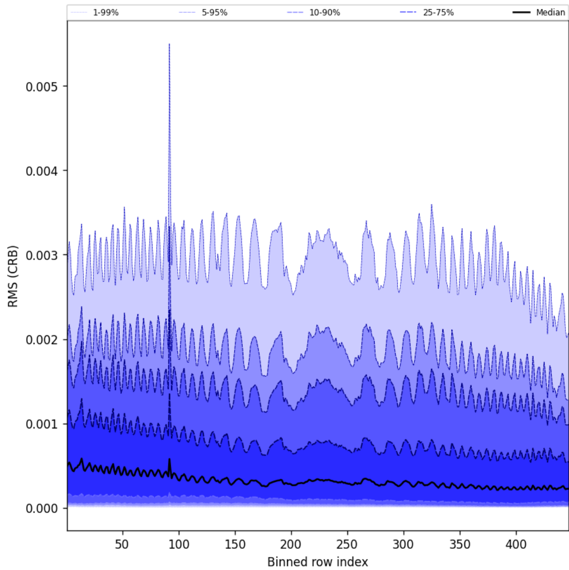
Figure 64: Along track statistics of “RMS (CRB)” for 2024-10-03 to 2024-10-04
