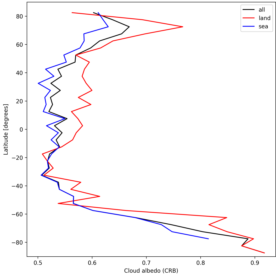
Figure 28: Zonal average of “Cloud albedo (CRB)” for 2024-10-03 to 2024-10-04.
