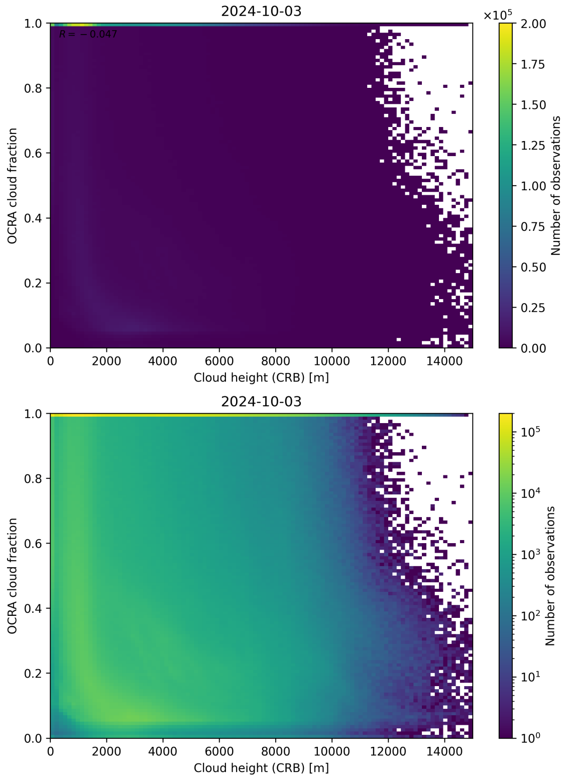
Figure 81: Scatter density plot of “Cloud height (CRB)” against “OCRA cloud fraction” for 2024-10-03 to 2024-10-04.
