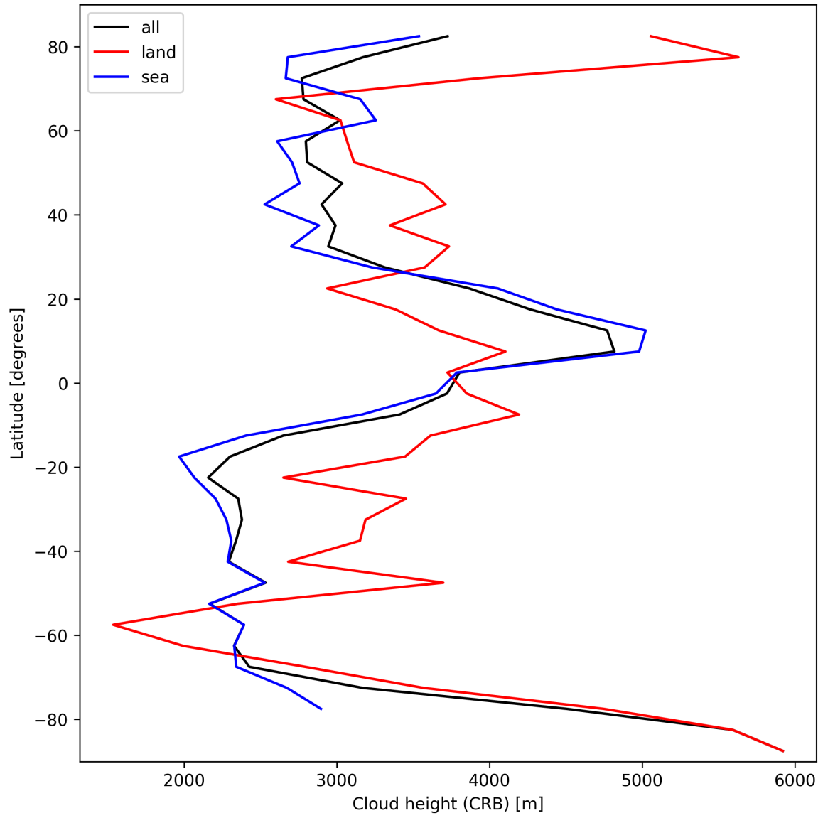
Figure 27: Zonal average of “Cloud height (CRB)” for 2024-10-03 to 2024-10-04.
