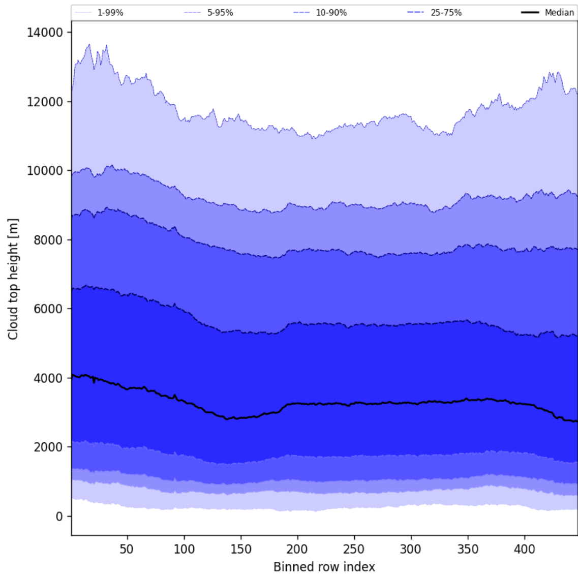
Figure 56: Along track statistics of “Cloud top height” for 2024-10-03 to 2024-10-04
