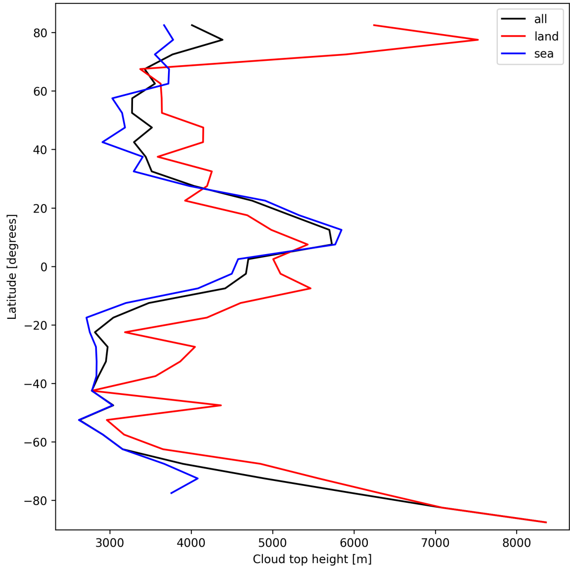
Figure 24: Zonal average of “Cloud top height” for 2024-10-03 to 2024-10-04.
