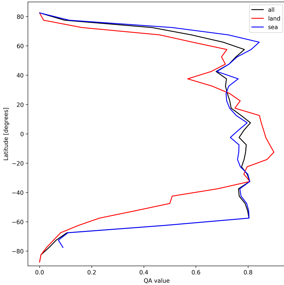
Figure 22: Zonal average of “QA value” for 2024-10-03 to 2024-10-04.
