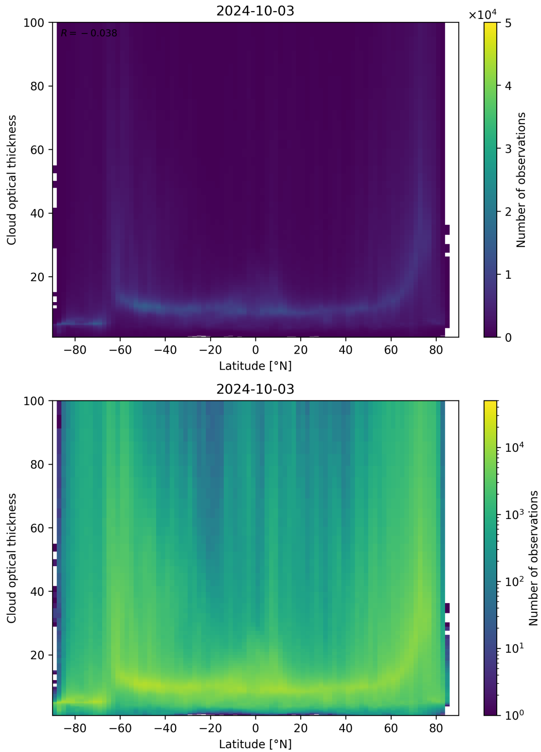
Figure 96: Scatter density plot of “Latitude” against “Cloud optical thickness” for 2024-10-03 to 2024-10-04.
