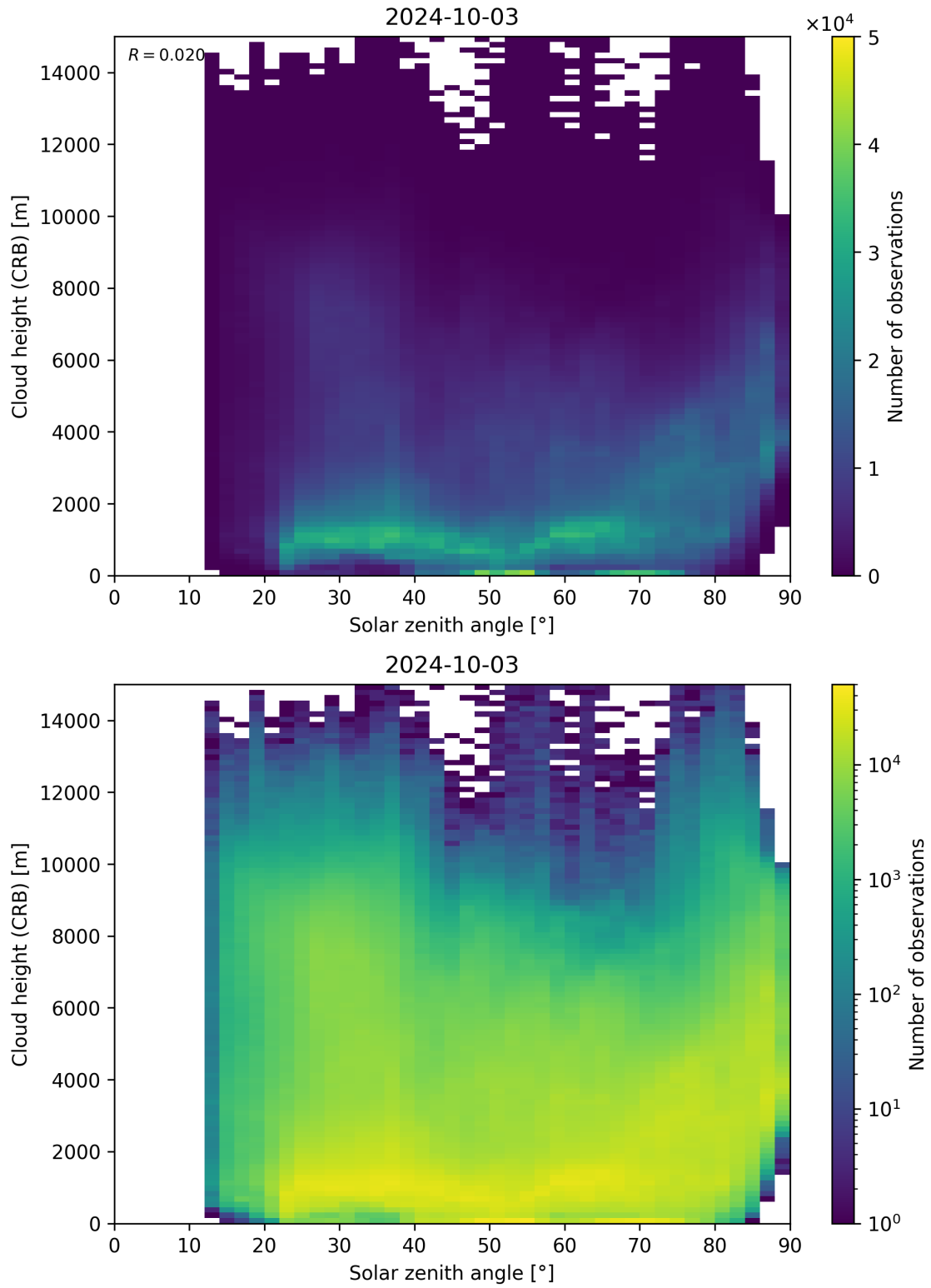
Figure 102: Scatter density plot of “Solar zenith angle” against “Cloud height (CRB)” for 2024-10-03 to 2024-10-04.
