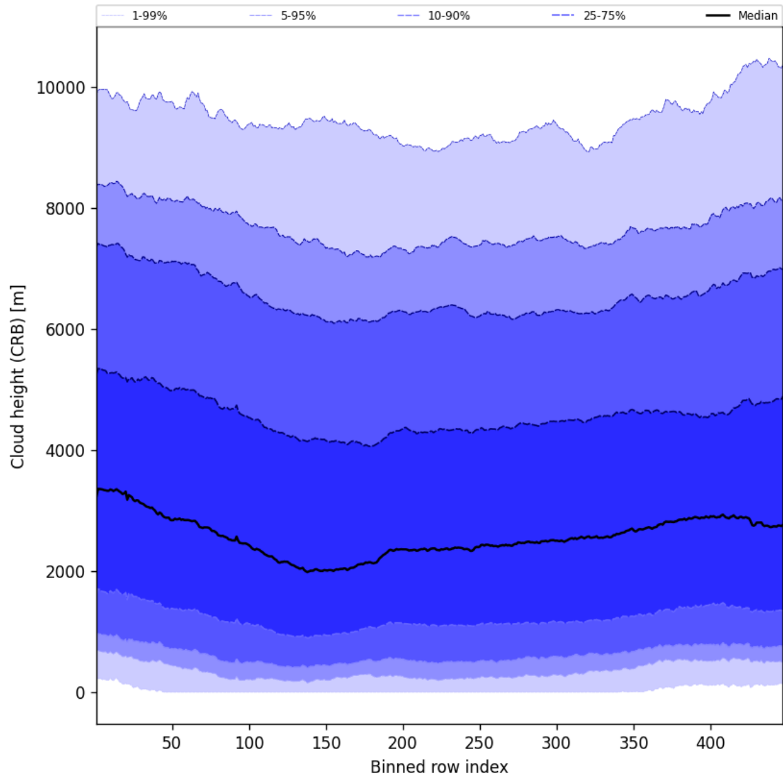
Figure 59: Along track statistics of “Cloud height (CRB)” for 2024-10-03 to 2024-10-04
