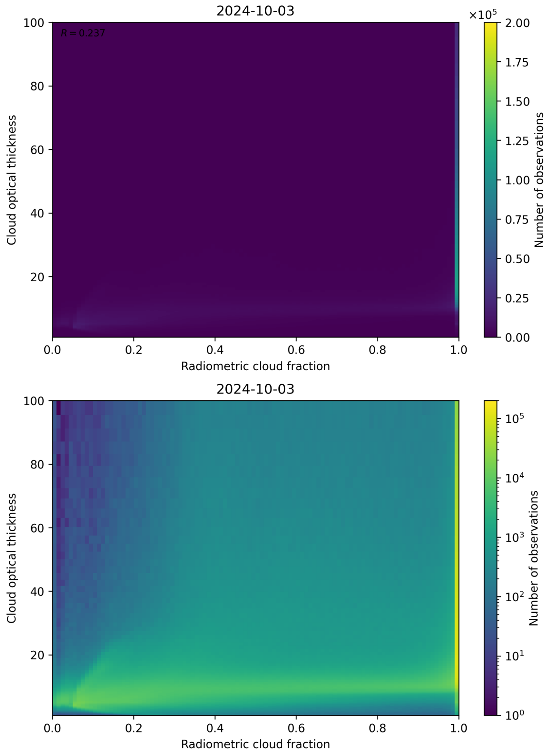
Figure 75: Scatter density plot of “Radiometric cloud fraction” against “Cloud optical thickness” for 2024-10-03 to 2024-10-04.
