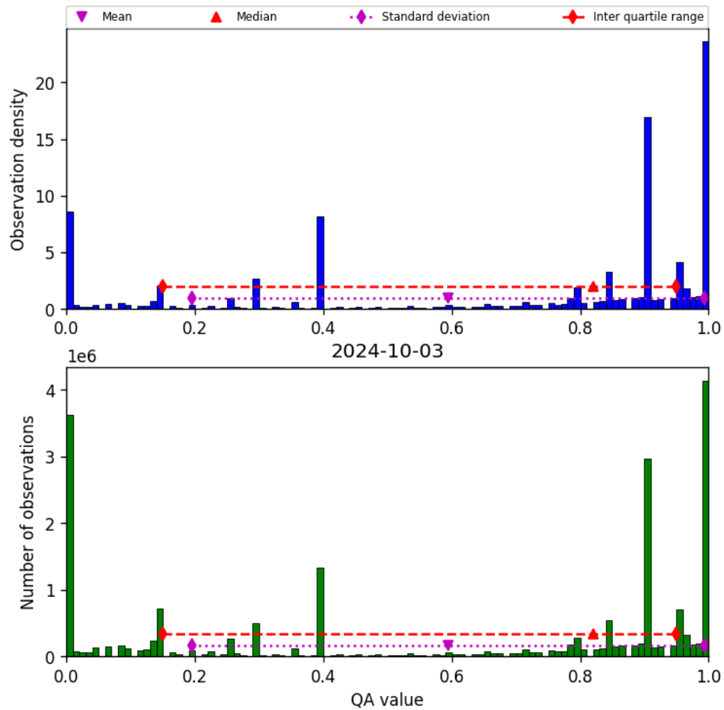
Figure 38: Histogram of “QA value” for 2024-10-03 to 2024-10-04
