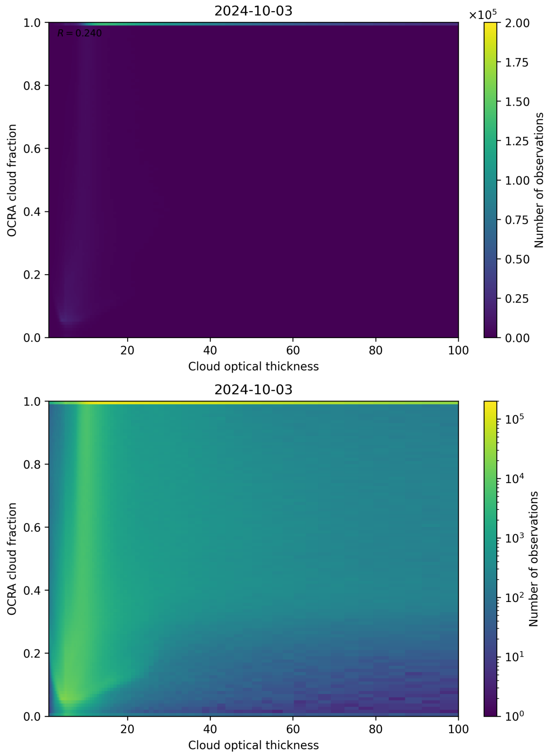
Figure 83: Scatter density plot of “Cloud optical thickness” against “OCRA cloud fraction” for 2024-10-03 to 2024-10-04.
