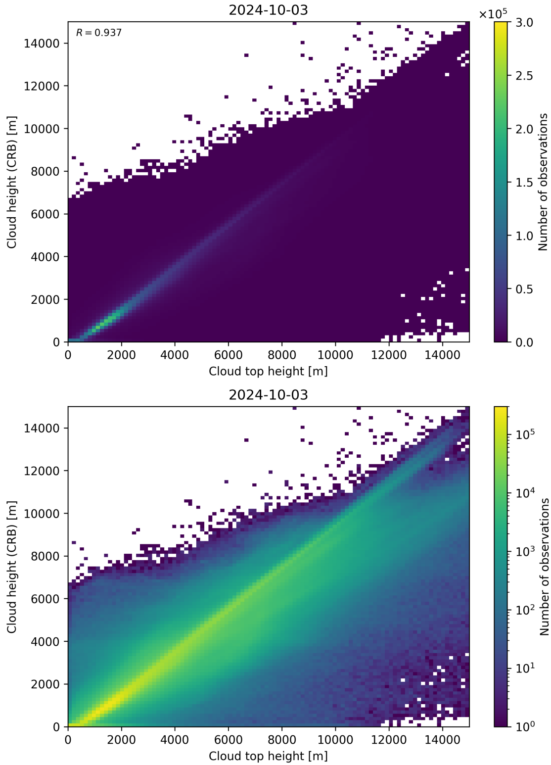
Figure 89: Scatter density plot of “Cloud top height” against “Cloud height (CRB)” for 2024-10-03 to 2024-10-04.
