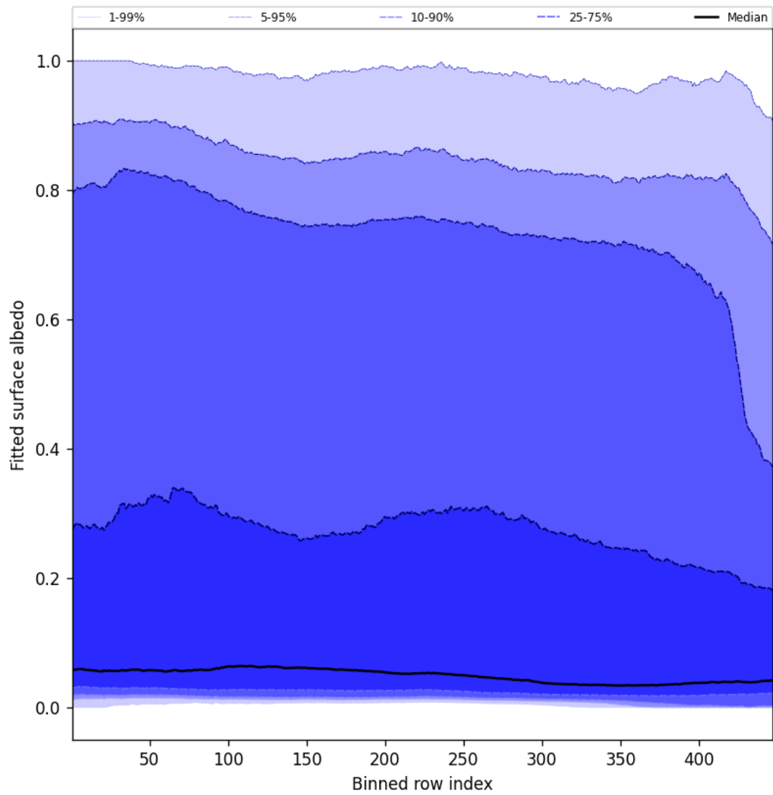
Figure 61: Along track statistics of “Fitted surface albedo” for 2024-10-05 to 2024-10-07
