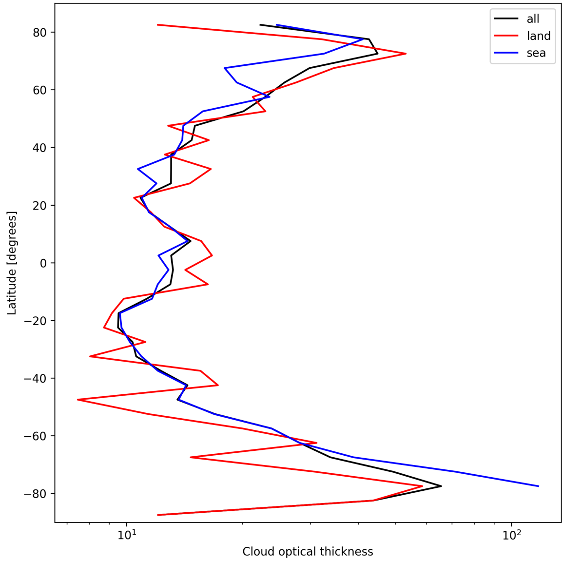
Figure 25: Zonal average of “Cloud optical thickness” for 2024-10-05 to 2024-10-07.
