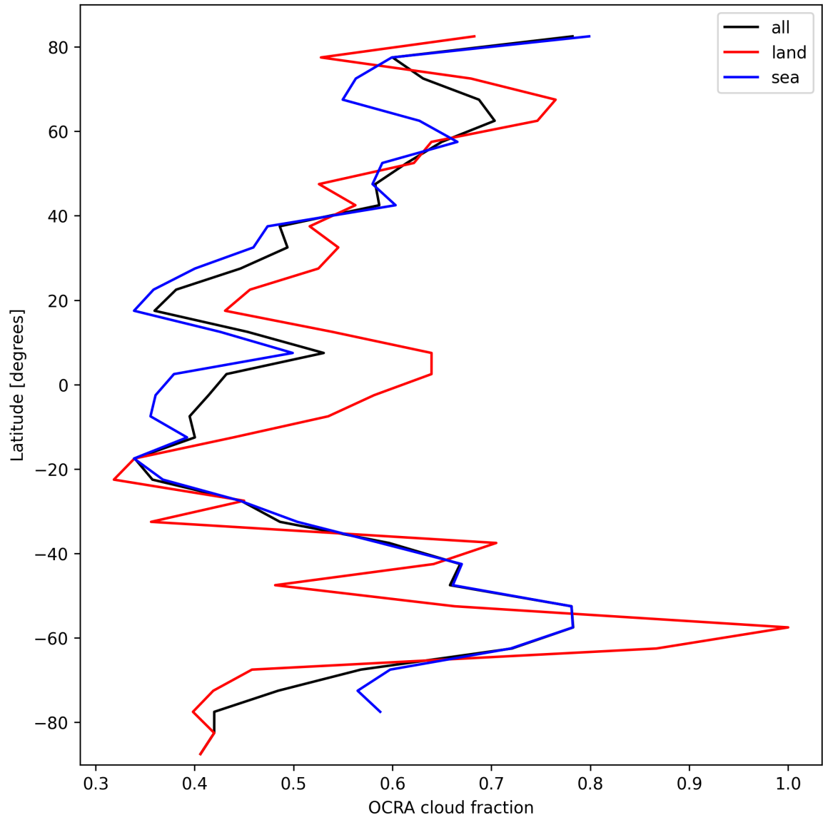
Figure 34: Zonal average of “OCRA cloud fraction” for 2024-10-05 to 2024-10-07.
