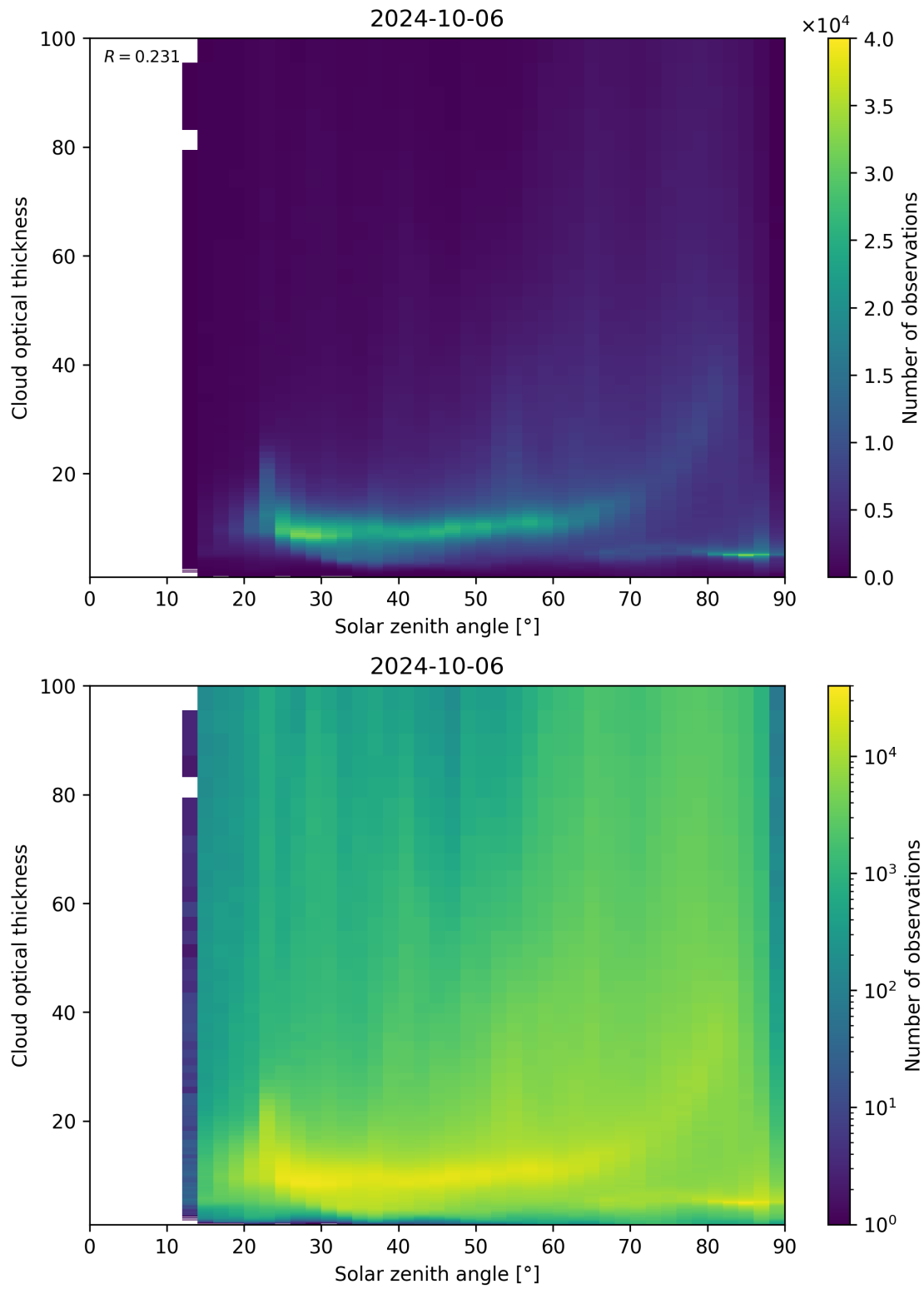
Figure 103: Scatter density plot of “Solar zenith angle” against “Cloud optical thickness” for 2024-10-05 to 2024-10-07.
