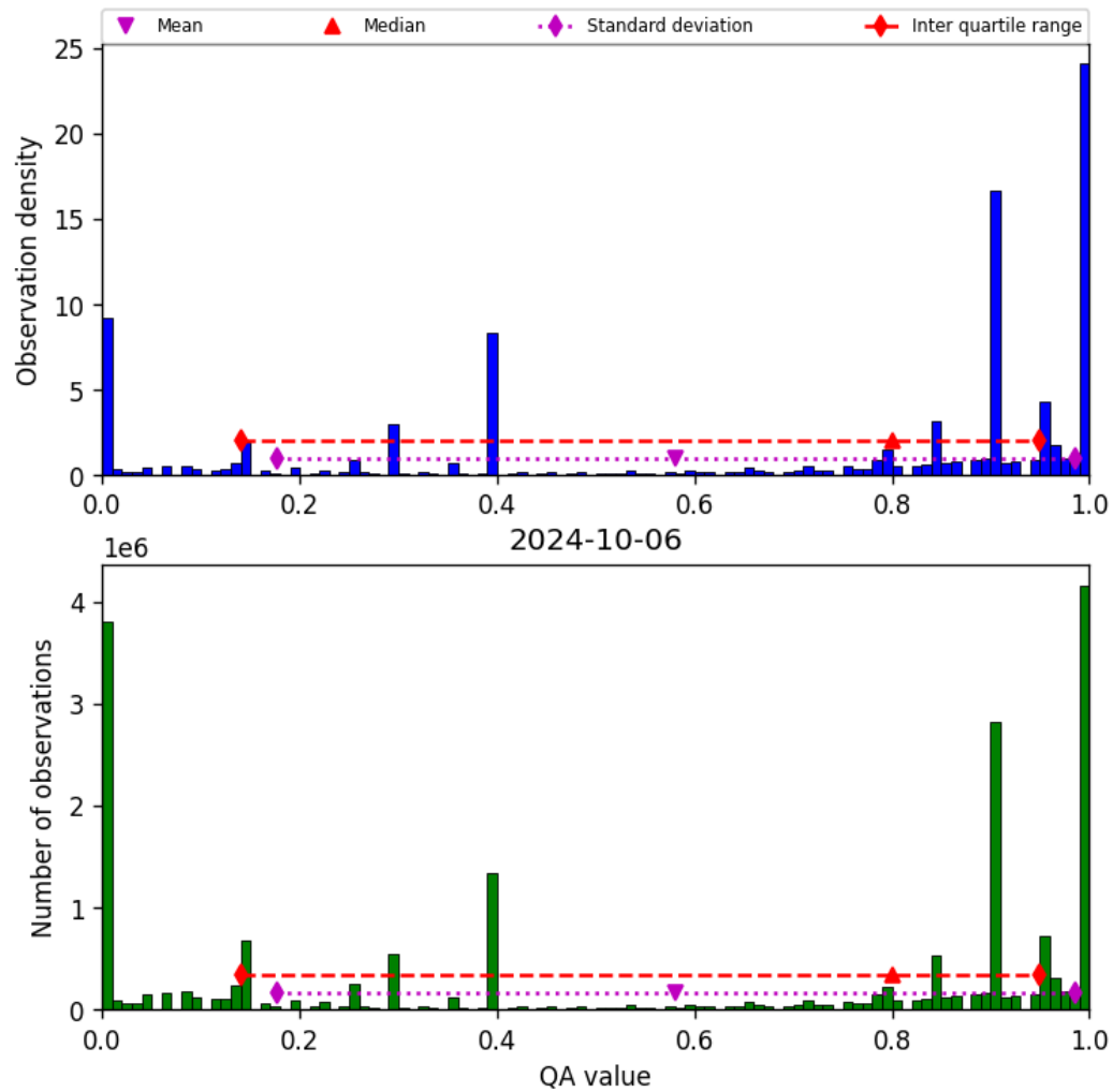
Figure 38: Histogram of “QA value” for 2024-10-05 to 2024-10-07
