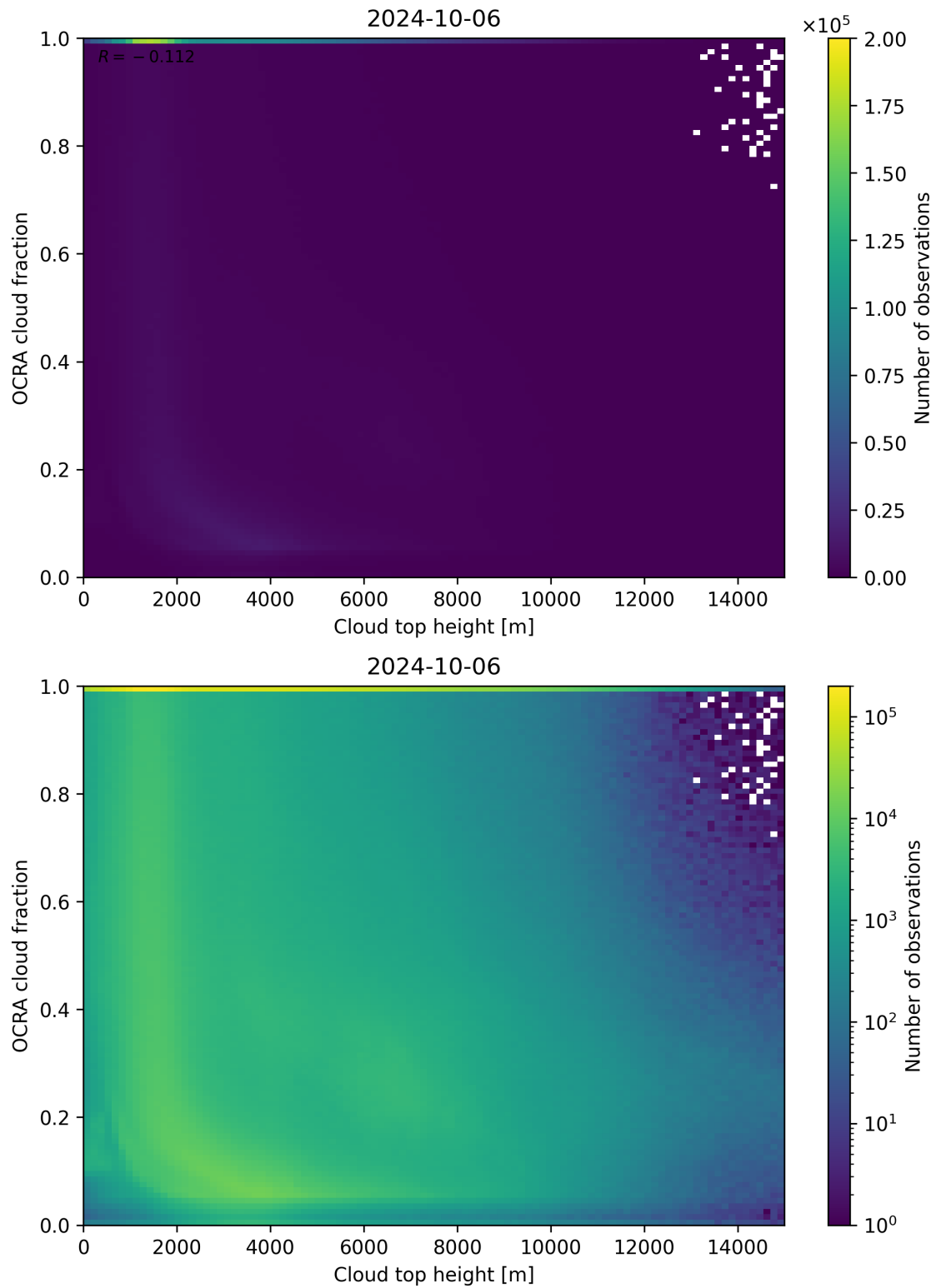
Figure 87: Scatter density plot of “Cloud top height” against “OCRA cloud fraction” for 2024-10-05 to 2024-10-07.
