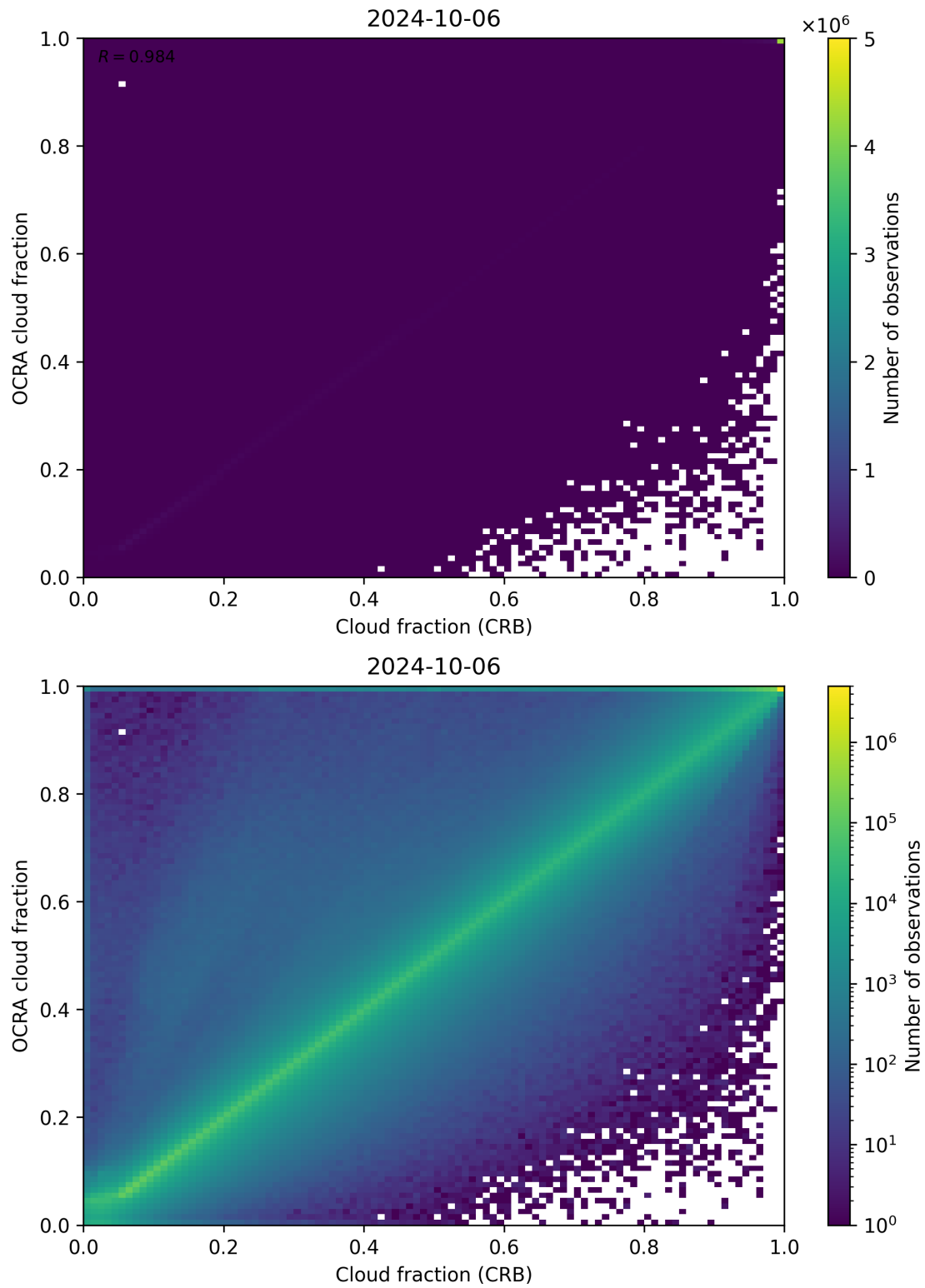
Figure 78: Scatter density plot of “Cloud fraction (CRB)” against “OCRA cloud fraction” for 2024-10-05 to 2024-10-07.
