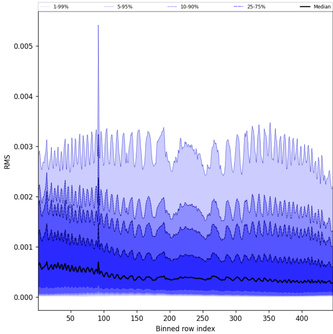
Figure 63: Along track statistics of “RMS” for 2024-10-05 to 2024-10-07
