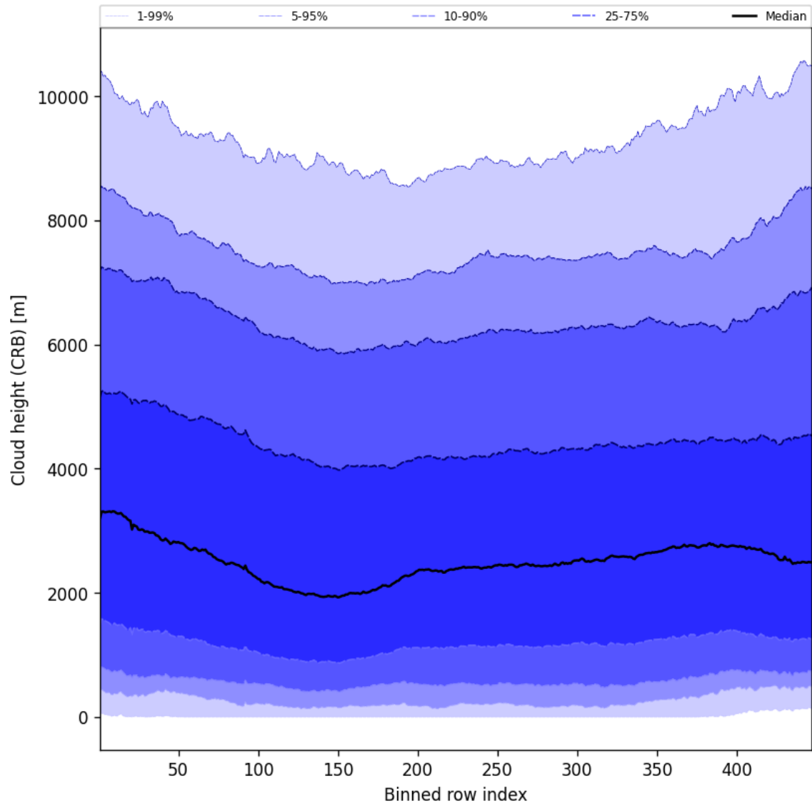
Figure 59: Along track statistics of “Cloud height (CRB)” for 2024-10-05 to 2024-10-07
