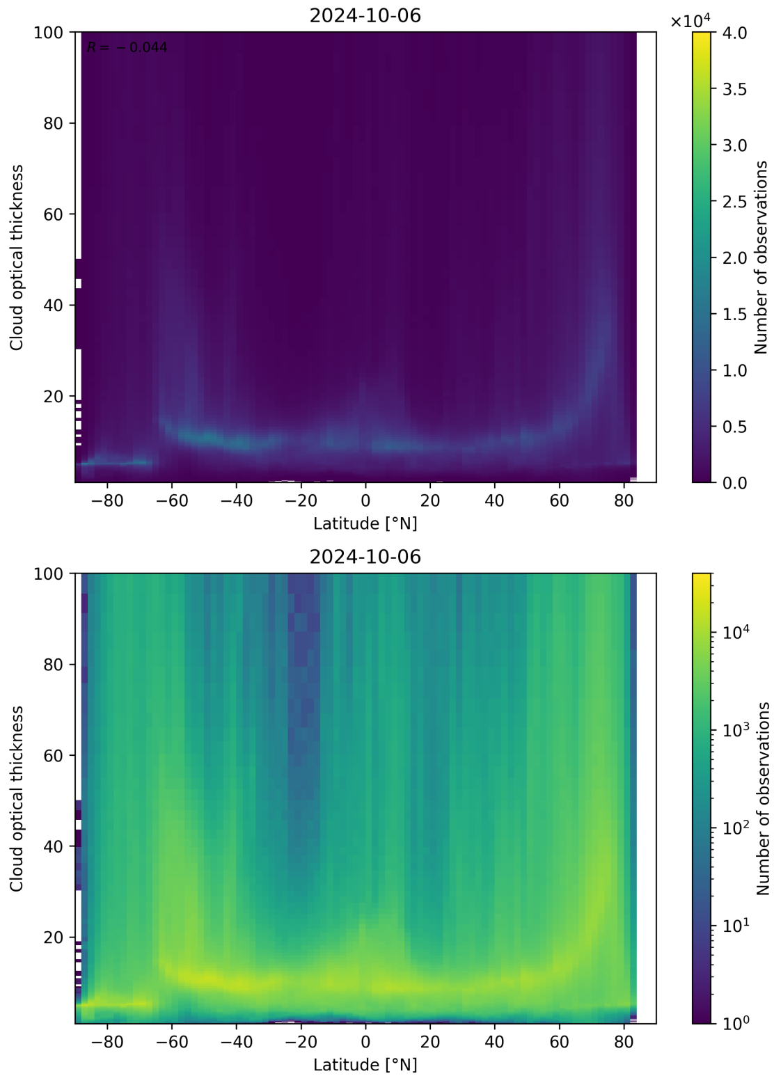
Figure 96: Scatter density plot of “Latitude” against “Cloud optical thickness” for 2024-10-05 to 2024-10-07.
