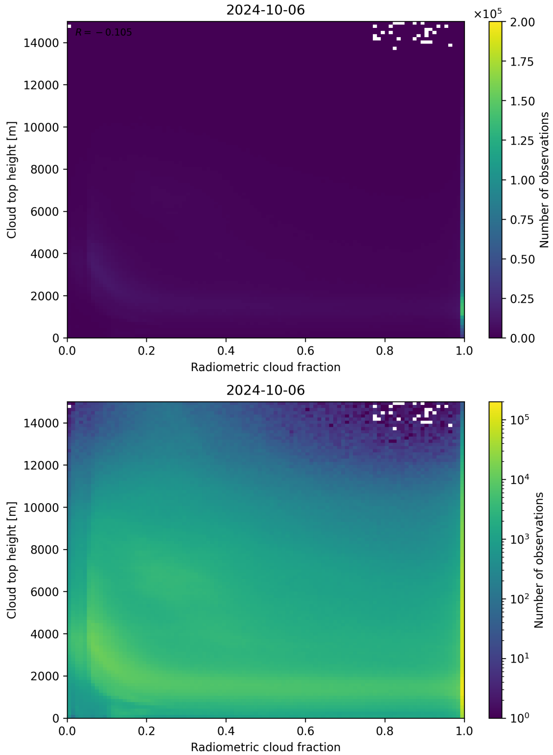
Figure 76: Scatter density plot of “Radiometric cloud fraction” against “Cloud top height” for 2024-10-05 to 2024-10-07.
