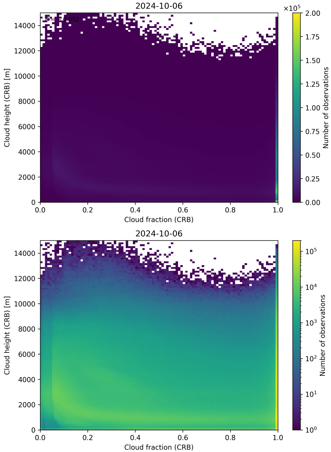
Figure 79: Scatter density plot of “Cloud fraction (CRB)” against “Cloud height (CRB)” for 2024-10-05 to 2024-10-07.
