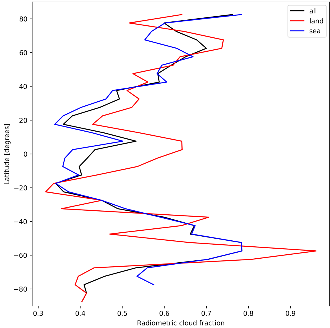
Figure 23: Zonal average of “Radiometric cloud fraction” for 2024-10-05 to 2024-10-07.
