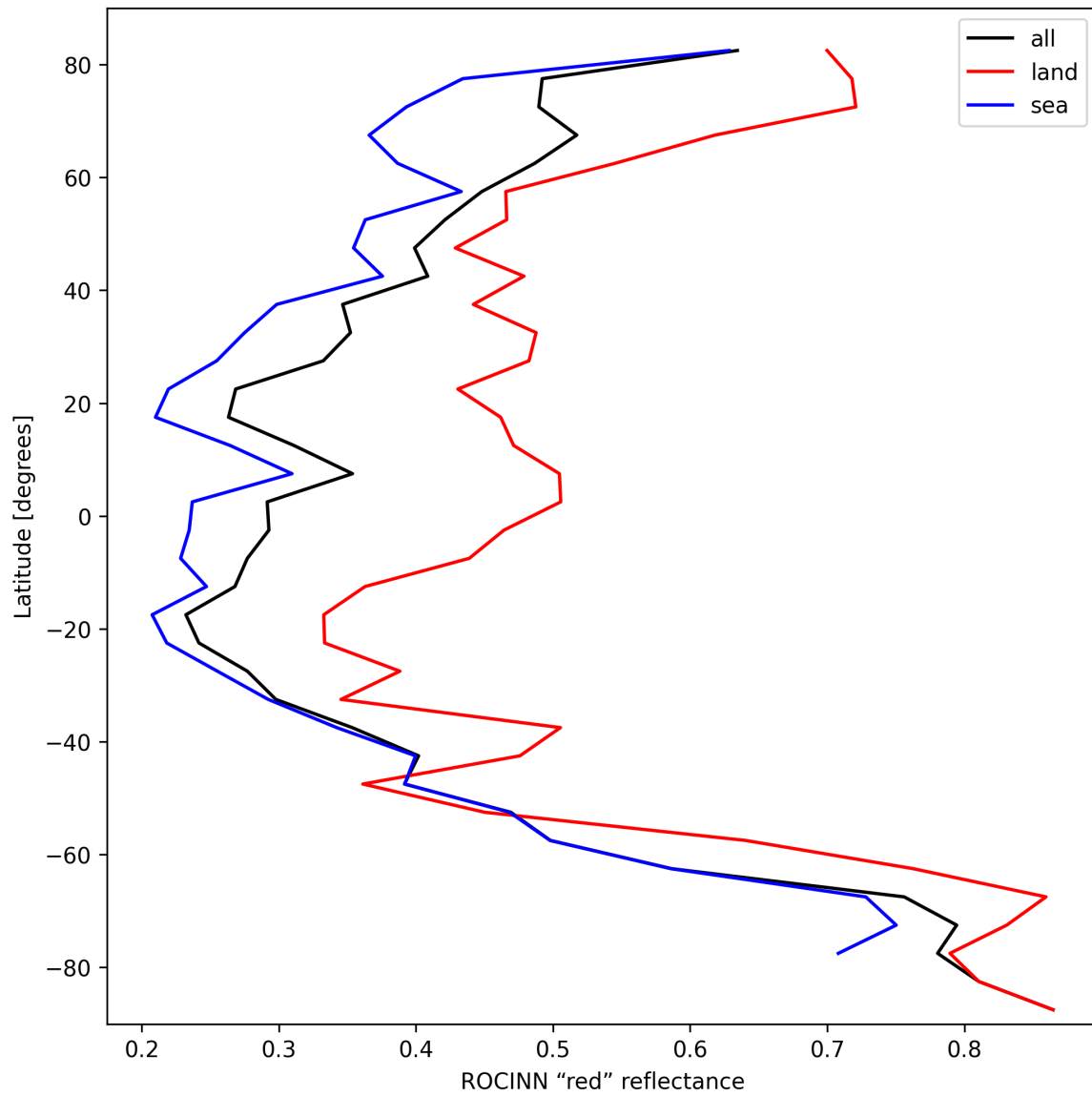
Figure 37: Zonal average of “ROCINN “red” reflectance” for 2024-10-05 to 2024-10-07.
