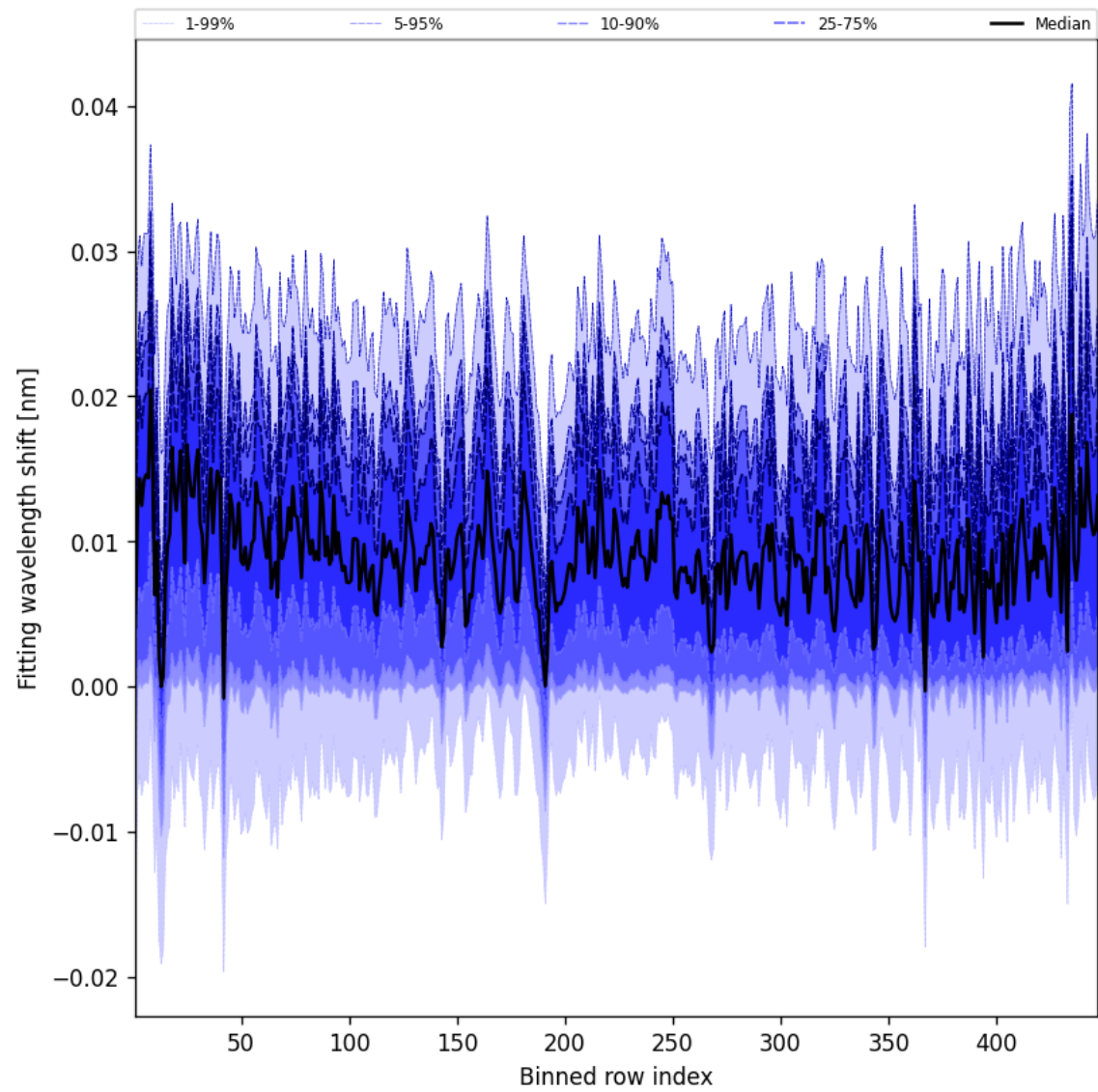
Figure 65: Along track statistics of “Fitting wavelength shift” for 2024-10-05 to 2024-10-07
