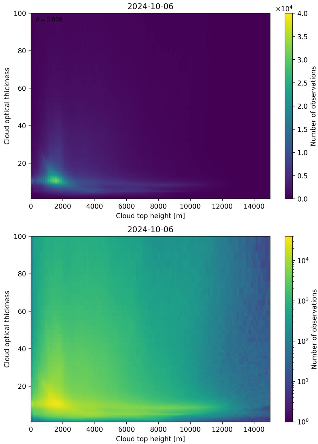
Figure 90: Scatter density plot of “Cloud top height” against “Cloud optical thickness” for 2024-10-05 to 2024-10-07.
