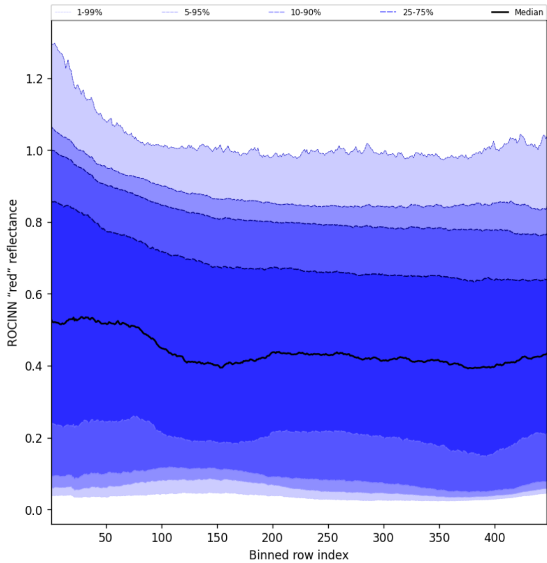
Figure 69: Along track statistics of “ROCINN “red” reflectance” for 2024-10-05 to 2024-10-07
