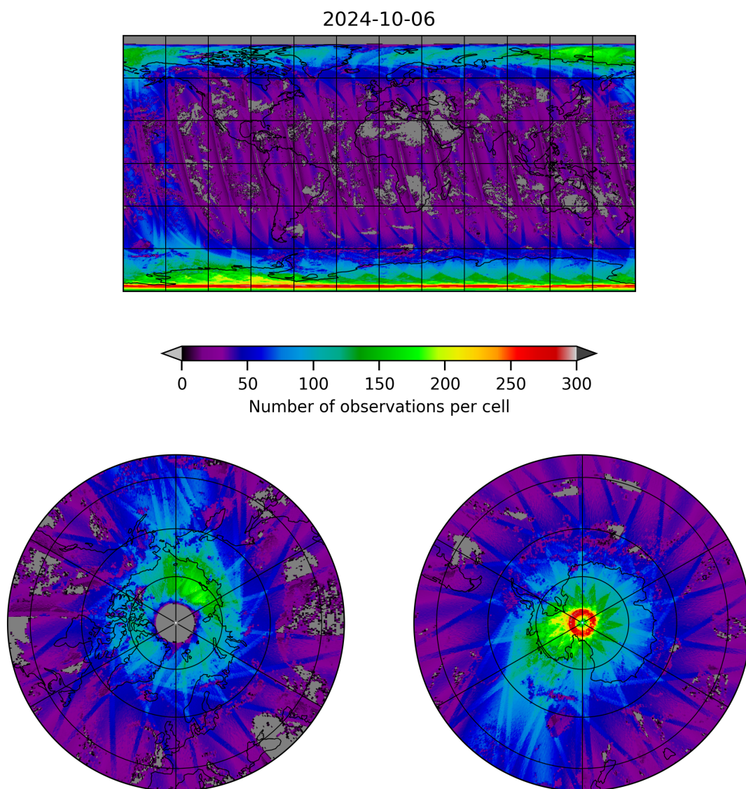
Figure 21: Map of the number of observations for 2024-10-05 to 2024-10-07
