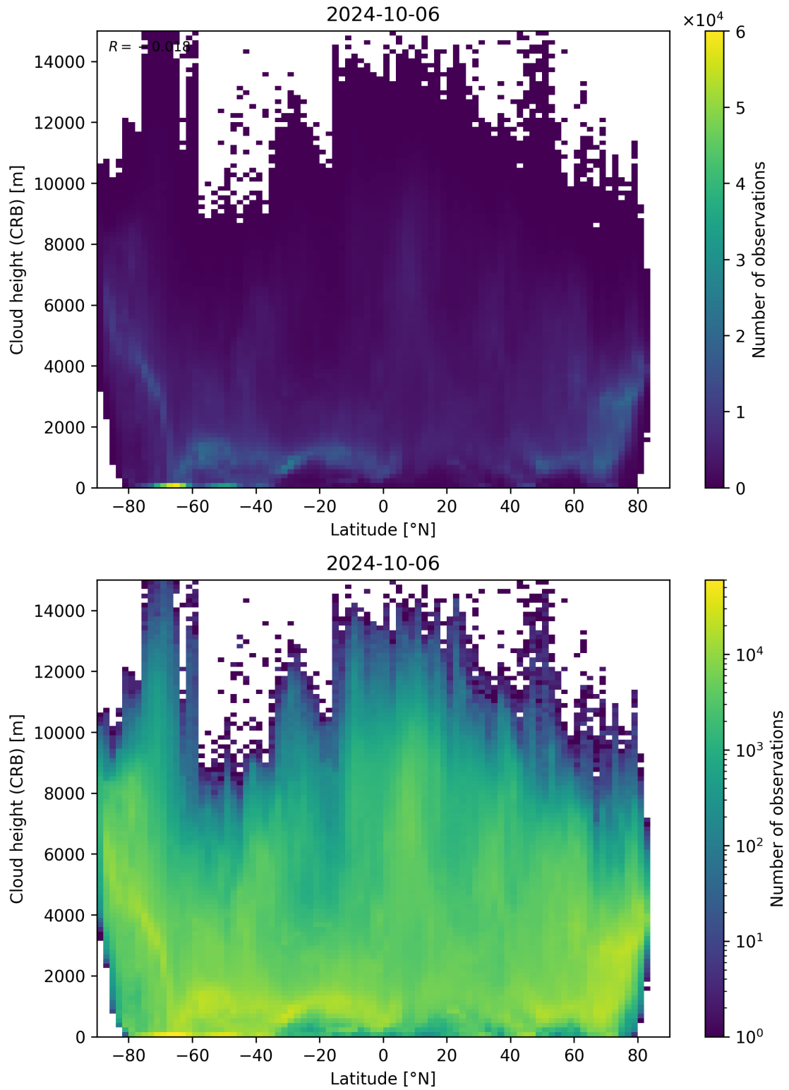
Figure 95: Scatter density plot of “Latitude” against “Cloud height (CRB)” for 2024-10-05 to 2024-10-07.
