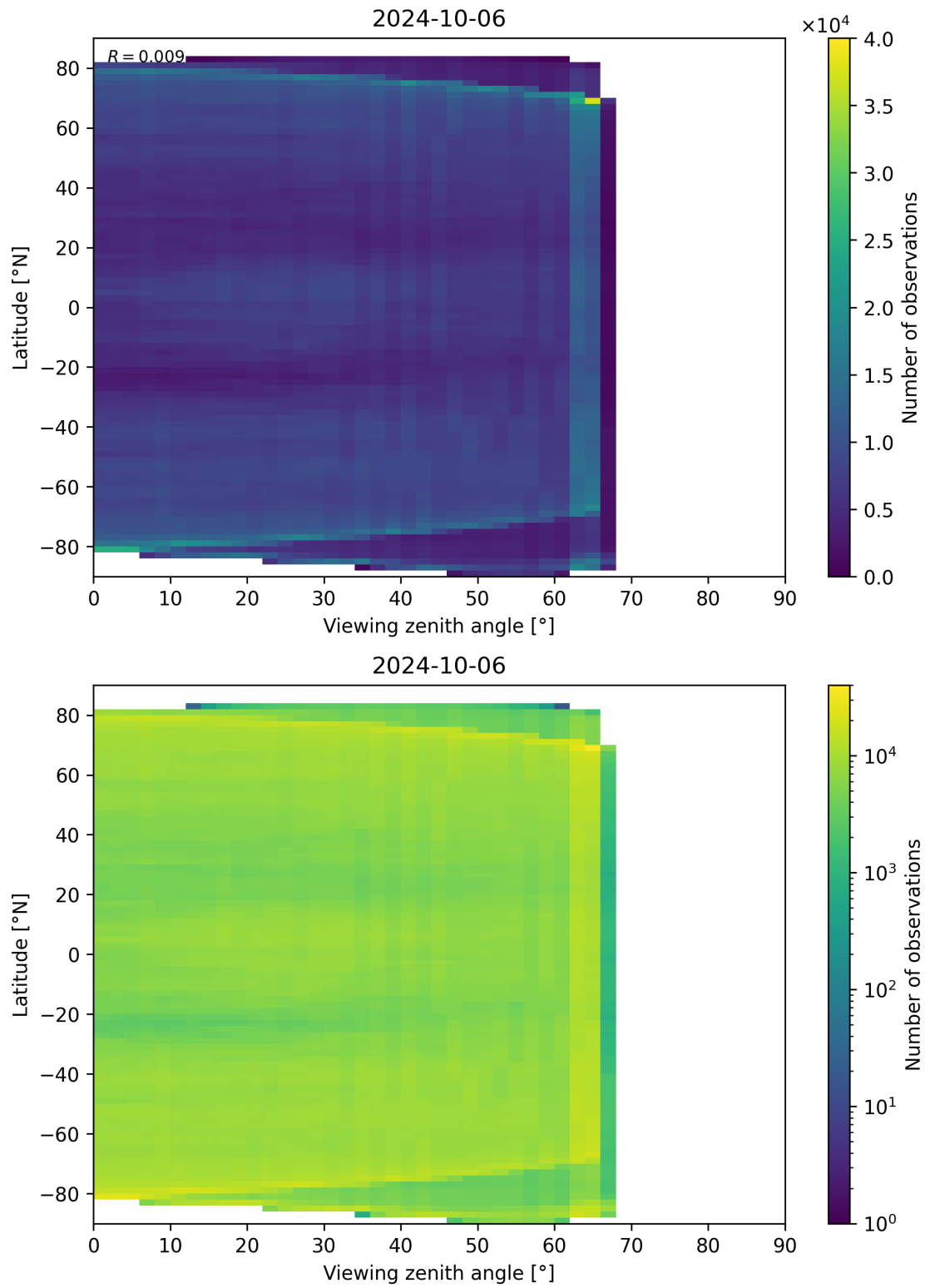
Figure 113: Scatter density plot of “Viewing zenith angle” against “Latitude” for 2024-10-05 to 2024-10-07.
