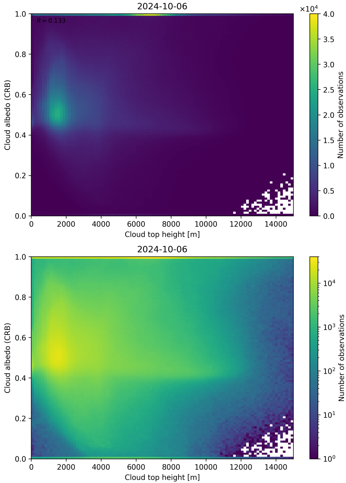
Figure 86: Scatter density plot of “Cloud top height” against “Cloud albedo (CRB)” for 2024-10-05 to 2024-10-07.
