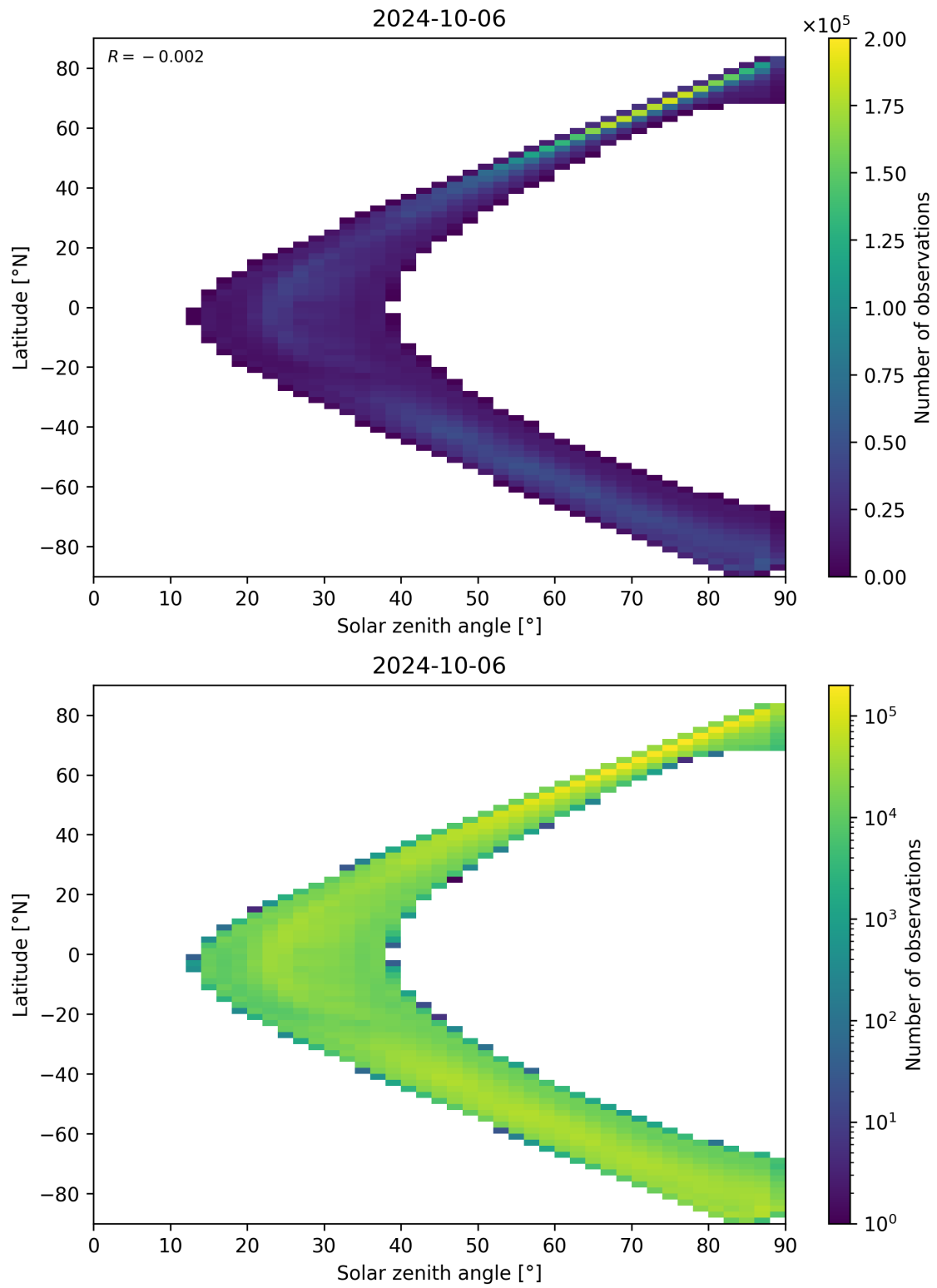
Figure 105: Scatter density plot of “Solar zenith angle” against “Latitude” for 2024-10-05 to 2024-10-07.
