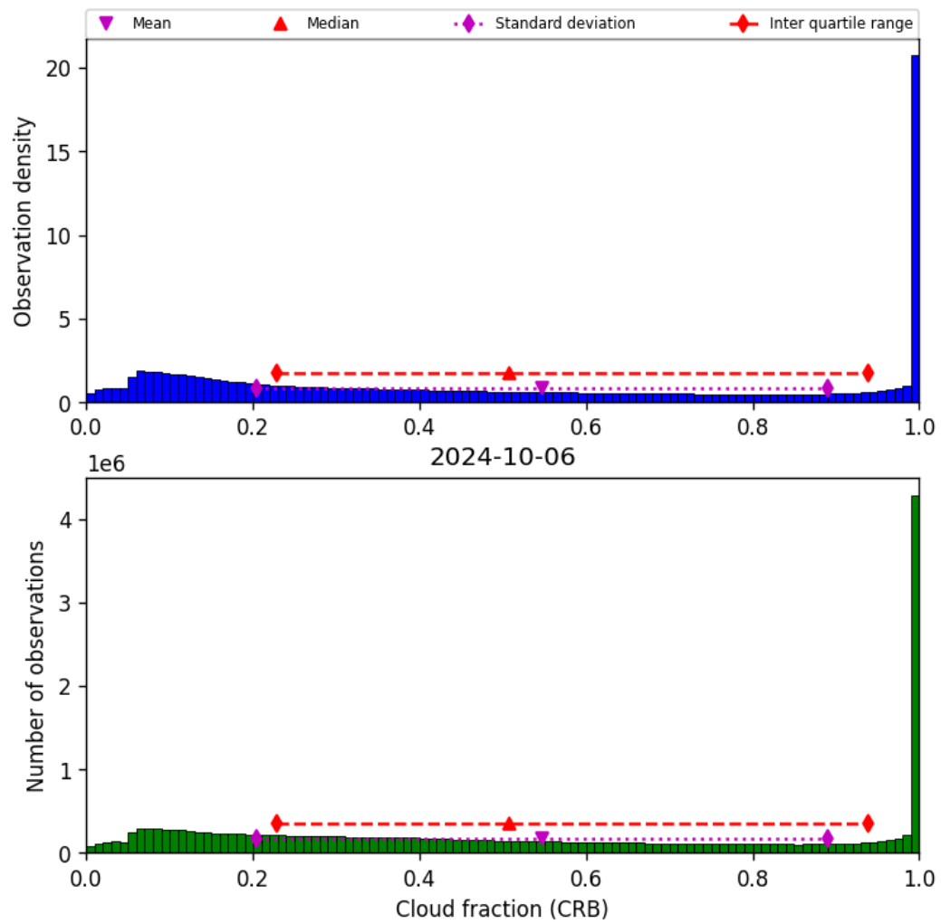
Figure 42: Histogram of “Cloud fraction (CRB)” for 2024-10-05 to 2024-10-07
