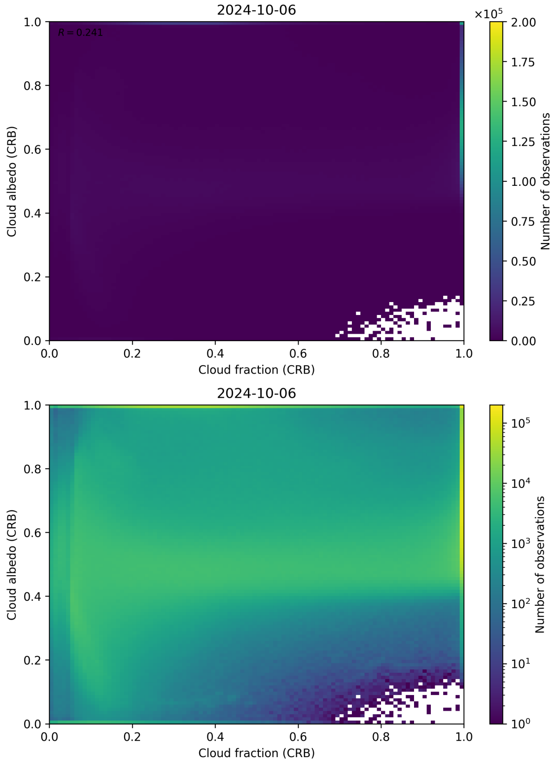
Figure 77: Scatter density plot of “Cloud fraction (CRB)” against “Cloud albedo (CRB)” for 2024-10-05 to 2024-10-07.
