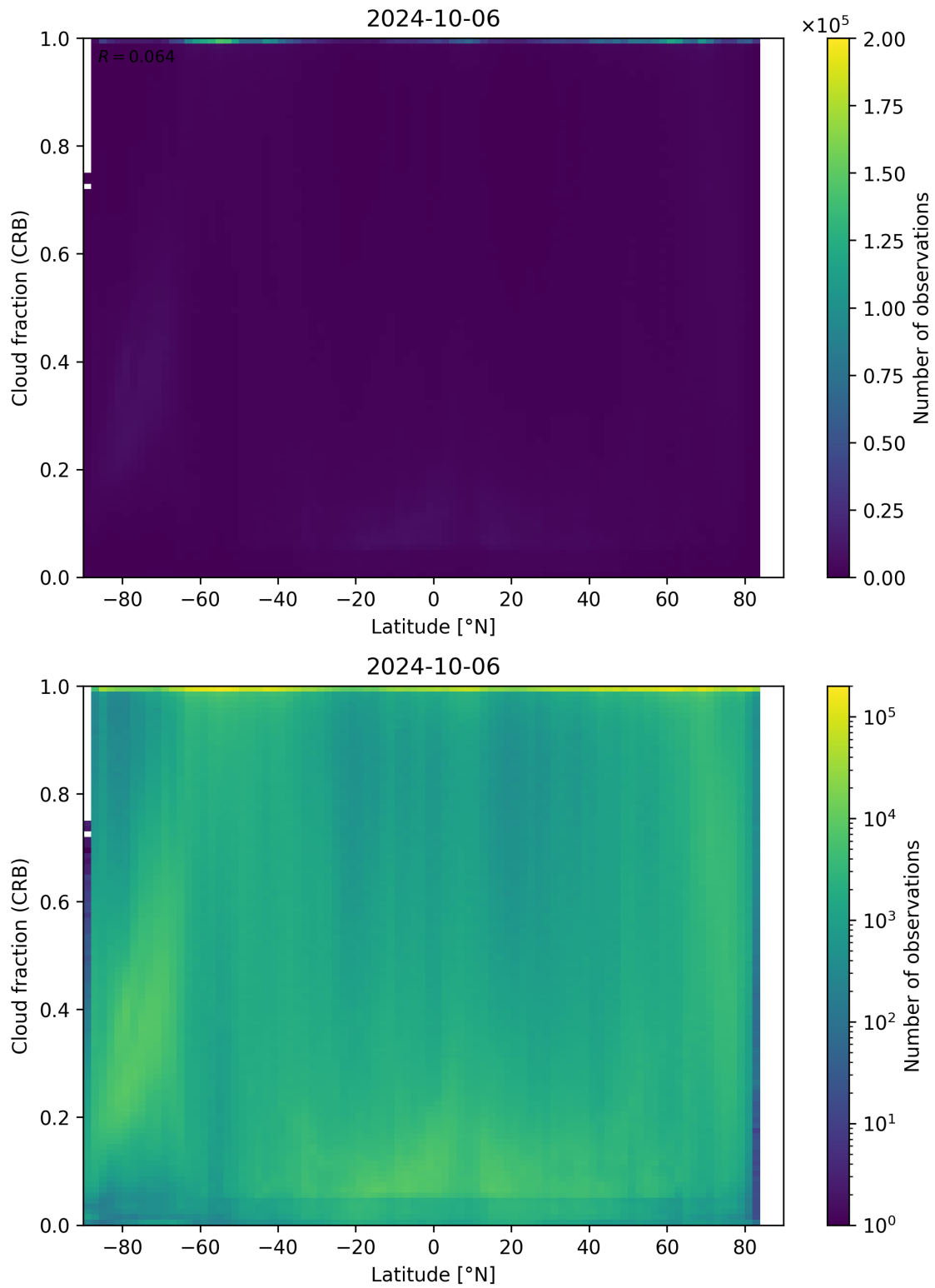
Figure 94: Scatter density plot of “Latitude” against “Cloud fraction (CRB)” for 2024-10-05 to 2024-10-07.
