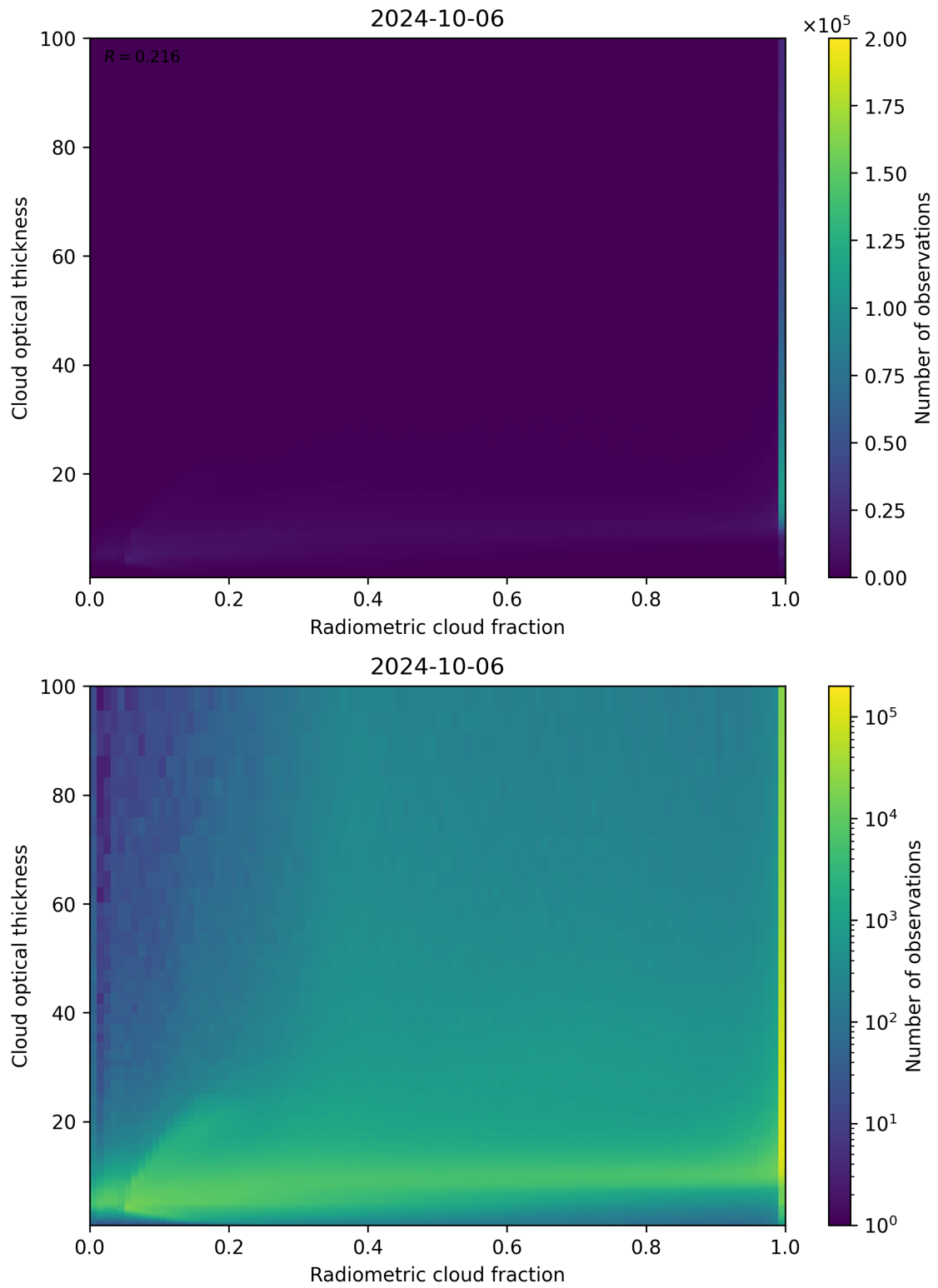
Figure 75: Scatter density plot of “Radiometric cloud fraction” against “Cloud optical thickness” for 2024-10-05 to 2024-10-07.
