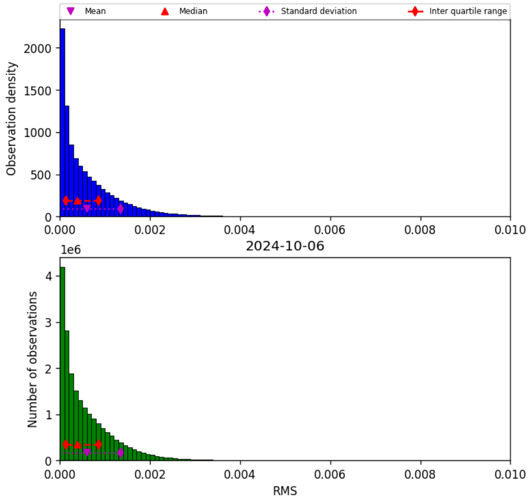
Figure 47: Histogram of “RMS” for 2024-10-05 to 2024-10-07
