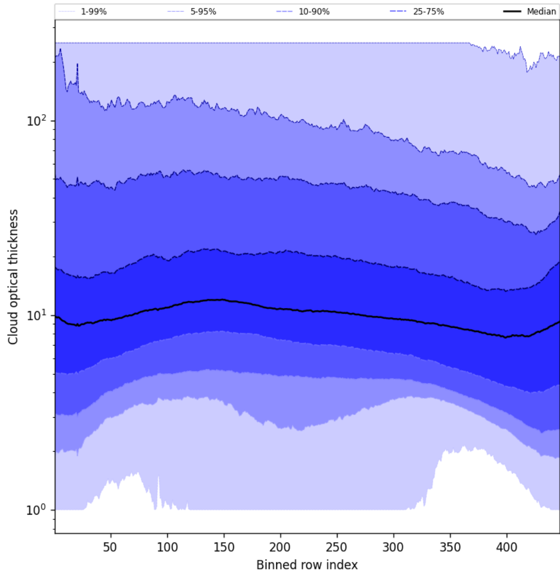
Figure 57: Along track statistics of “Cloud optical thickness” for 2024-10-05 to 2024-10-07
