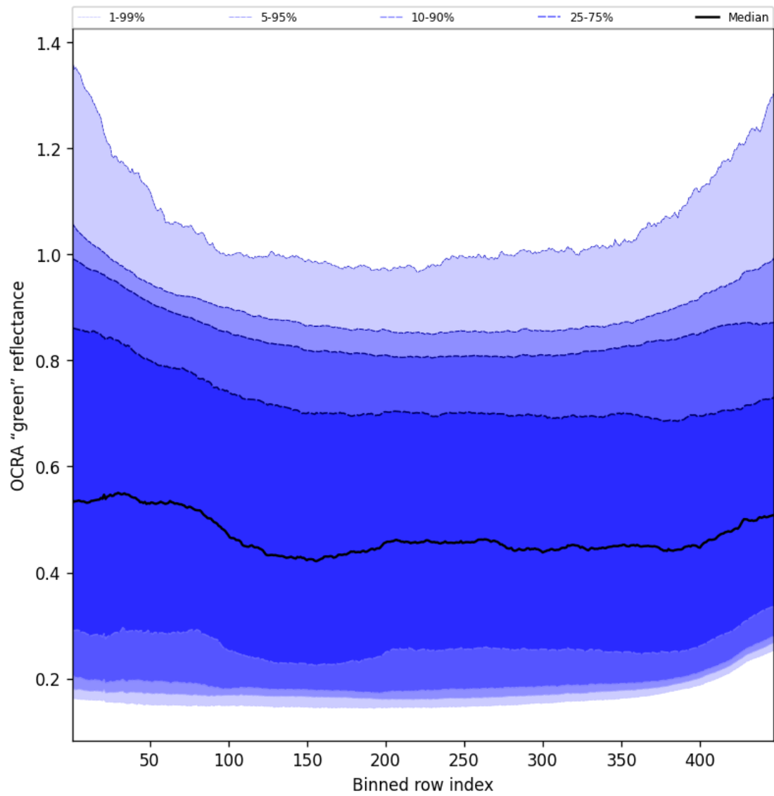
Figure 68: Along track statistics of "OCRA "green" reflectance" for 2024-10-05 to 2024-10-07
