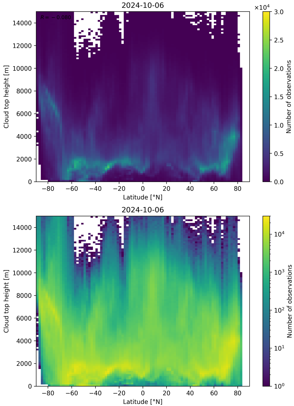
Figure 97: Scatter density plot of “Latitude” against “Cloud top height” for 2024-10-05 to 2024-10-07.
