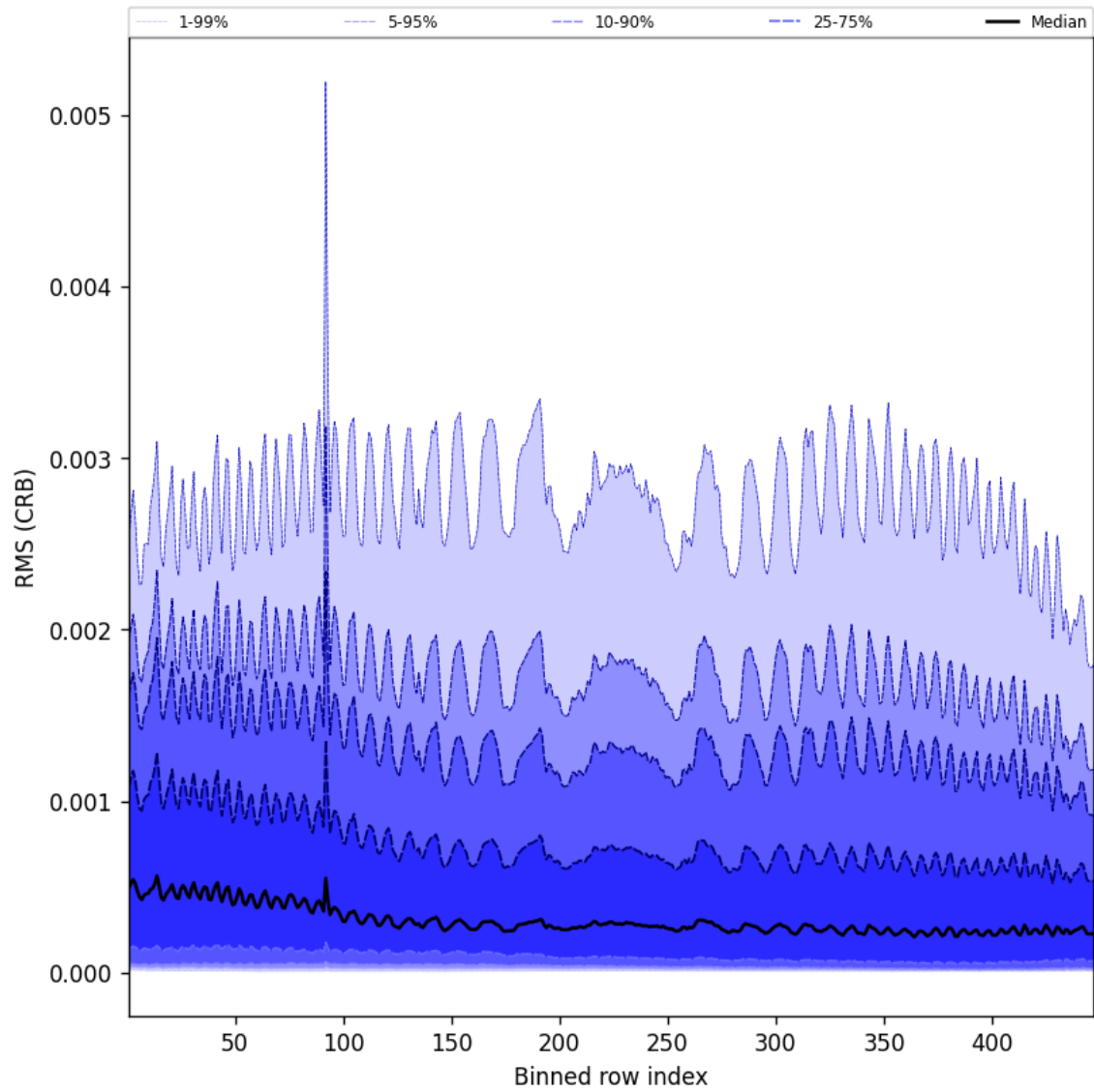
Figure 64: Along track statistics of “RMS (CRB)” for 2024-10-05 to 2024-10-07
