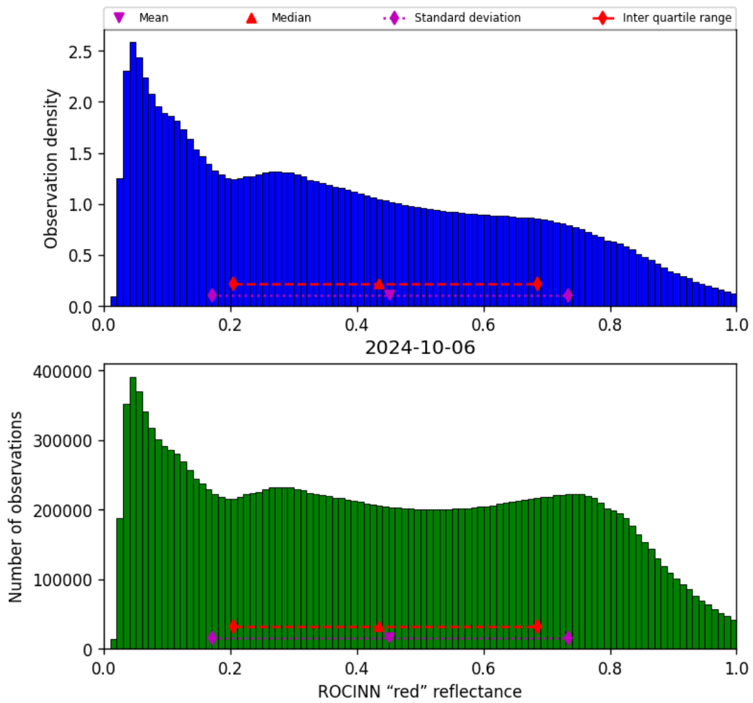
Figure 53: Histogram of “ROCINN “red” reflectance” for 2024-10-05 to 2024-10-07
