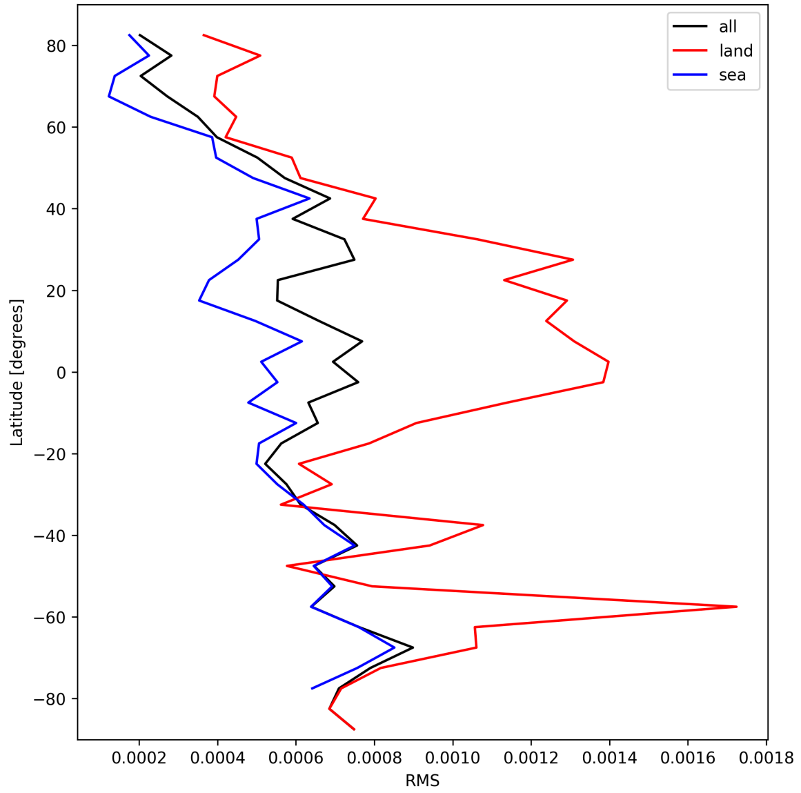
Figure 31: Zonal average of “RMS” for 2024-10-05 to 2024-10-07.
