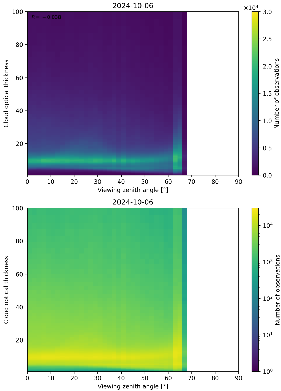
Figure 111: Scatter density plot of “Viewing zenith angle” against “Cloud optical thickness” for 2024-10-05 to 2024-10-07.
