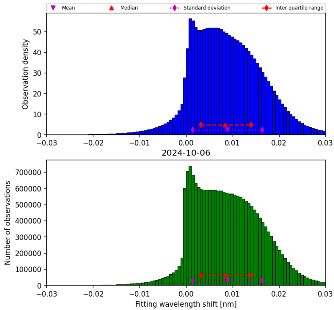
Figure 49: Histogram of “Fitting wavelength shift” for 2024-10-05 to 2024-10-07
