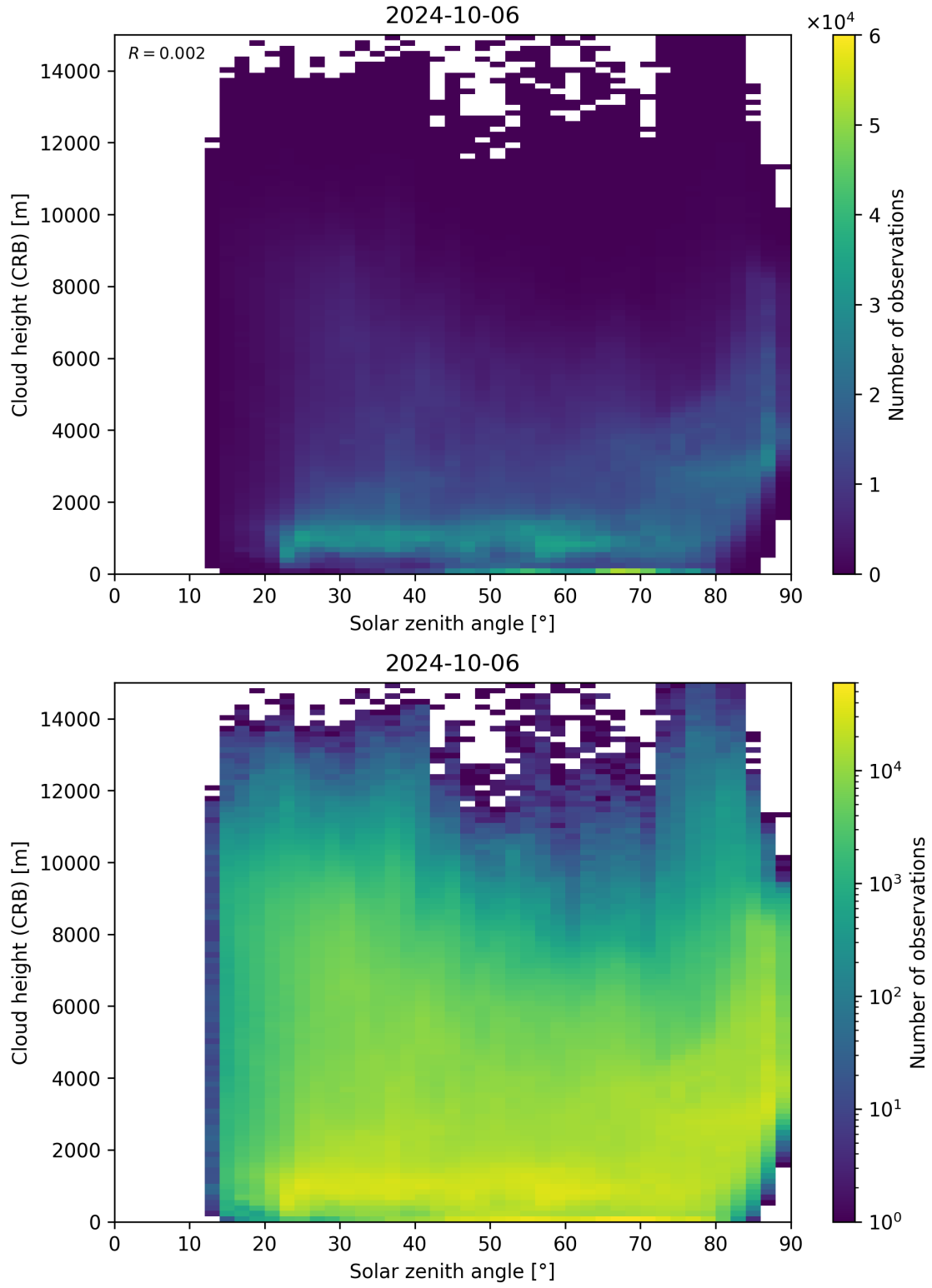
Figure 102: Scatter density plot of “Solar zenith angle” against “Cloud height (CRB)” for 2024-10-05 to 2024-10-07.
