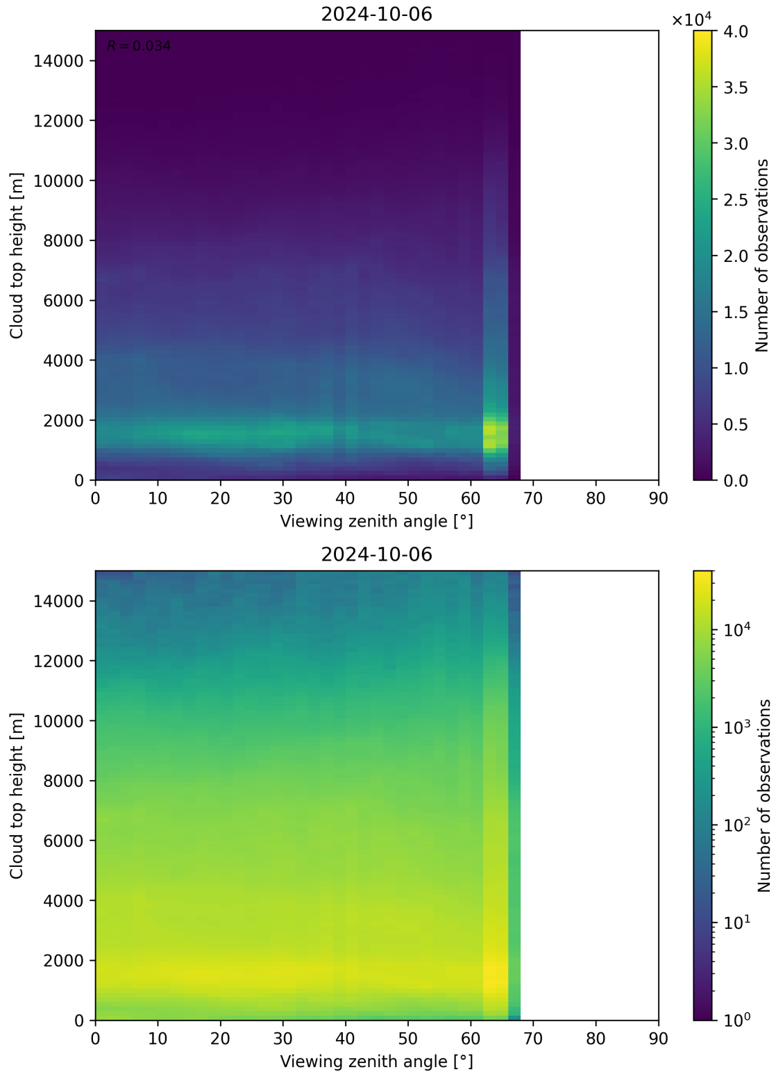
Figure 112: Scatter density plot of “Viewing zenith angle” against “Cloud top height” for 2024-10-05 to 2024-10-07.
