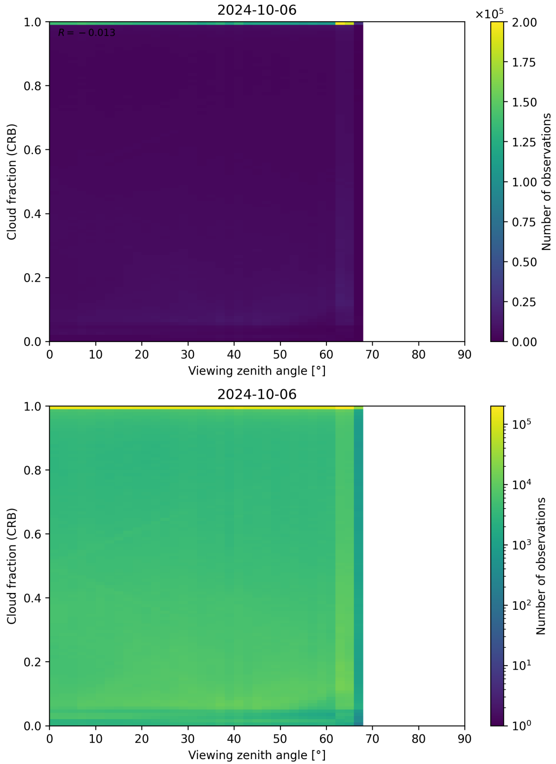
Figure 109: Scatter density plot of “Viewing zenith angle” against “Cloud fraction (CRB)” for 2024-10-05 to 2024-10-07.
