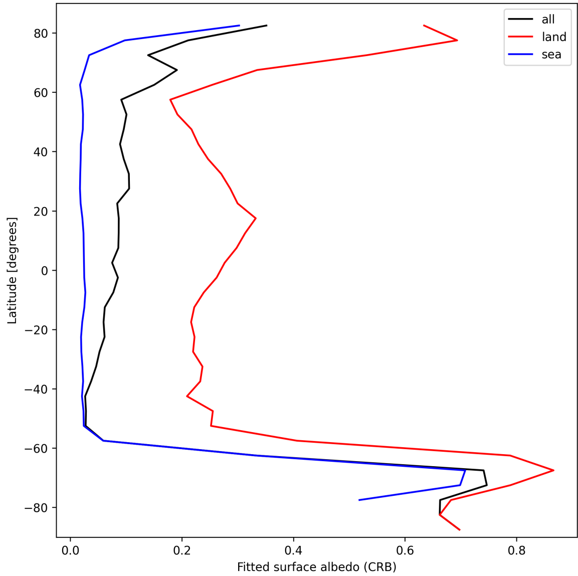
Figure 30: Zonal average of “Fitted surface albedo (CRB)” for 2024-10-05 to 2024-10-07.
