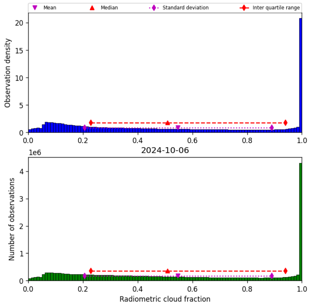
Figure 39: Histogram of “Radiometric cloud fraction” for 2024-10-05 to 2024-10-07
