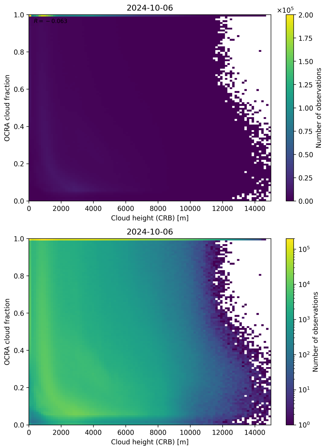
Figure 81: Scatter density plot of “Cloud height (CRB)” against “OCRA cloud fraction” for 2024-10-05 to 2024-10-07.
