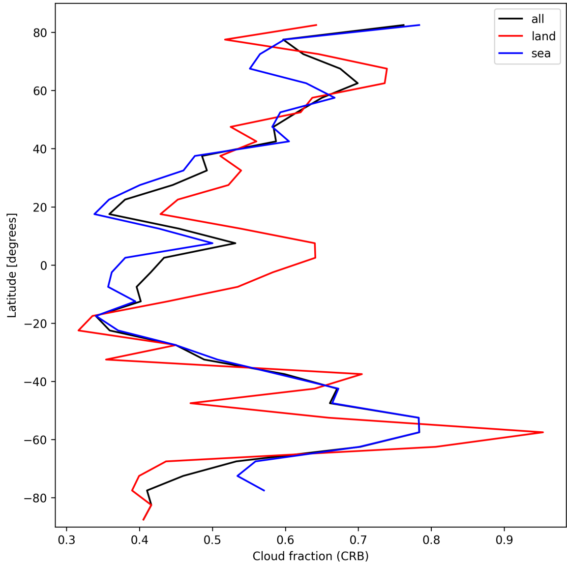
Figure 26: Zonal average of “Cloud fraction (CRB)” for 2024-10-05 to 2024-10-07.
