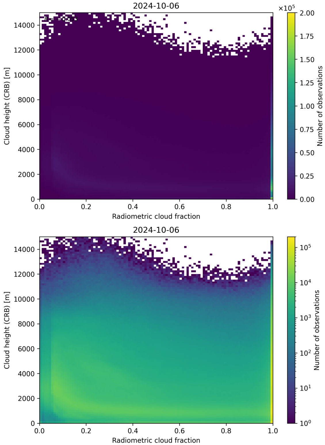
Figure 74: Scatter density plot of “Radiometric cloud fraction” against “Cloud height (CRB)” for 2024-10-05 to 2024-10-07.
