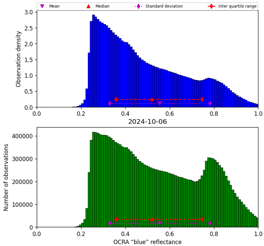
Figure 51: Histogram of “OCRA “blue” reflectance” for 2024-10-05 to 2024-10-07
