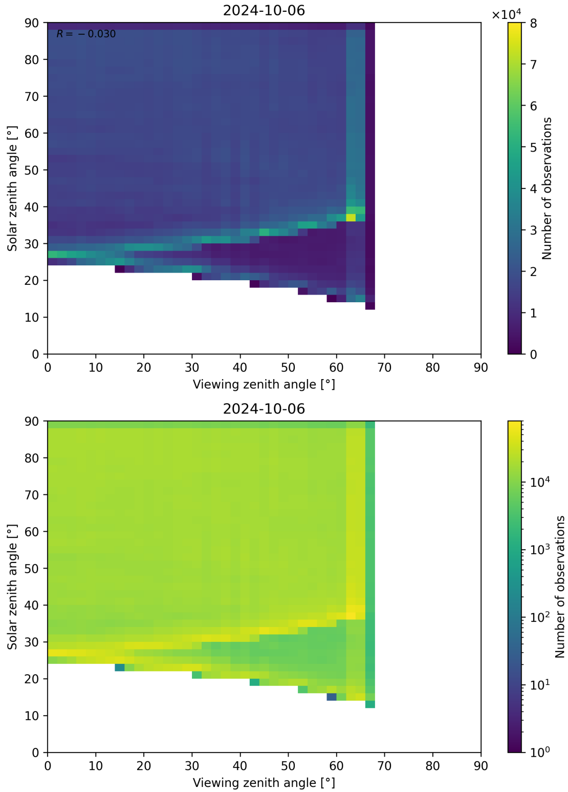
Figure 114: Scatter density plot of “Viewing zenith angle” against “Solar zenith angle” for 2024-10-05 to 2024-10-07.
