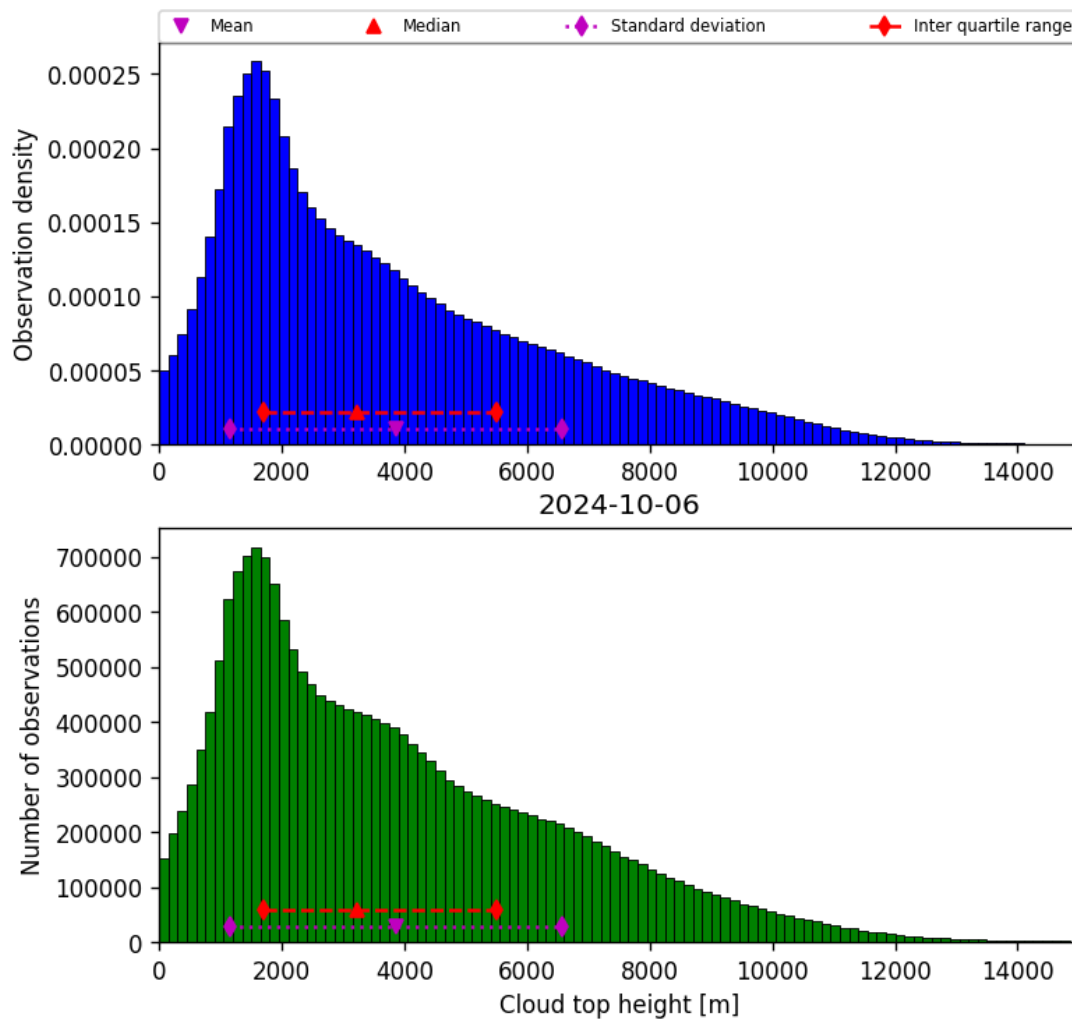
Figure 40: Histogram of “Cloud top height” for 2024-10-05 to 2024-10-07
