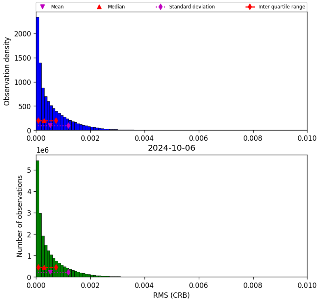
Figure 48: Histogram of “RMS (CRB)” for 2024-10-05 to 2024-10-07
