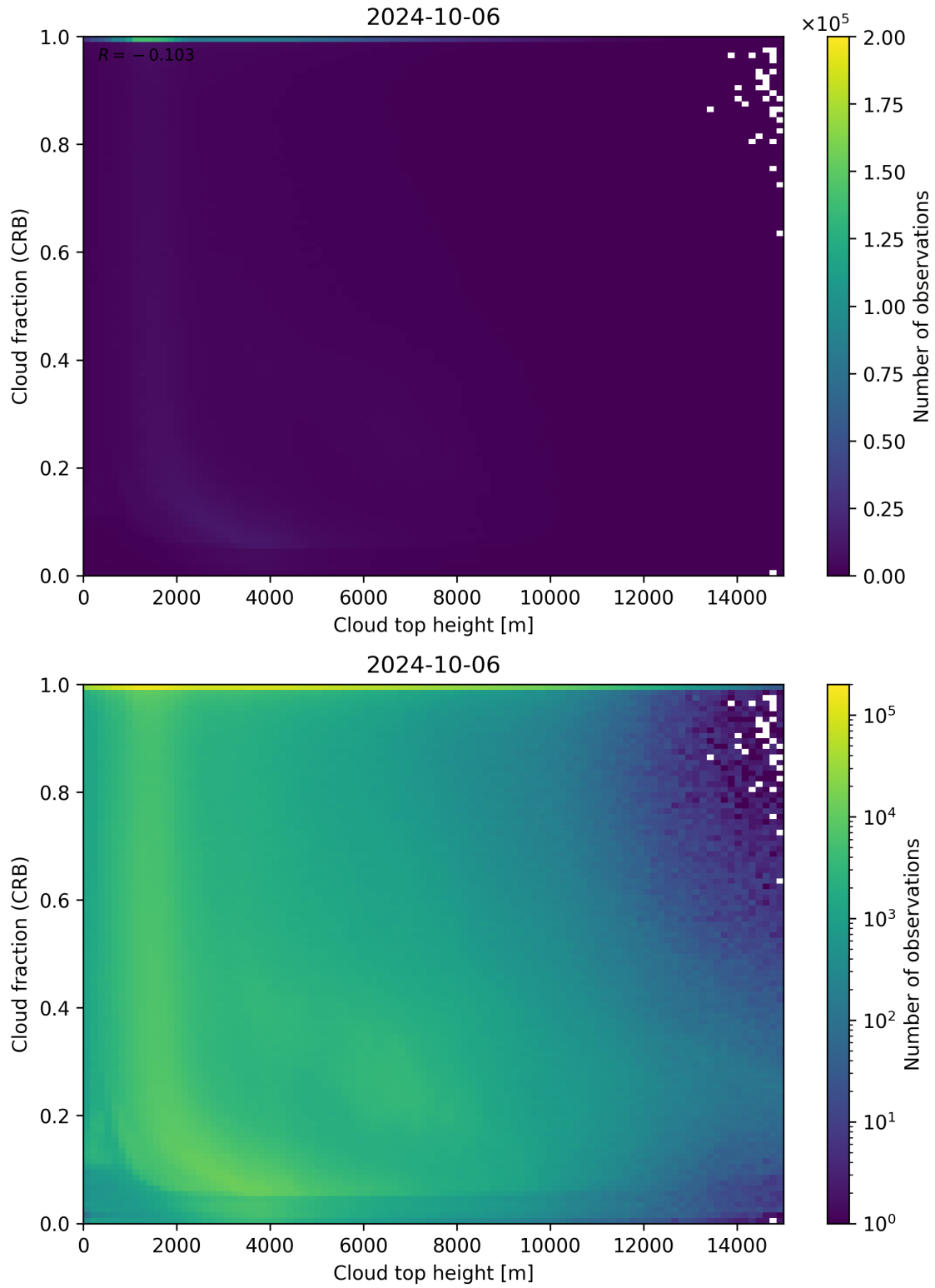
Figure 88: Scatter density plot of “Cloud top height” against “Cloud fraction (CRB)” for 2024-10-05 to 2024-10-07.
