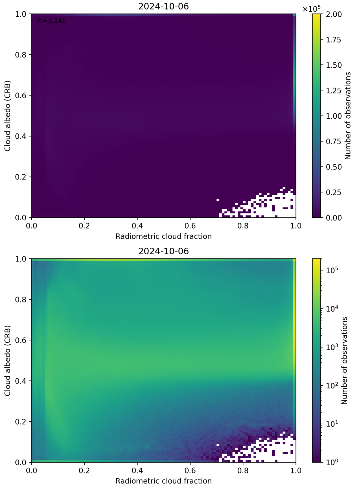
Figure 71: Scatter density plot of “Radiometric cloud fraction” against “Cloud albedo (CRB)” for 2024-10-05 to 2024-10-07.
