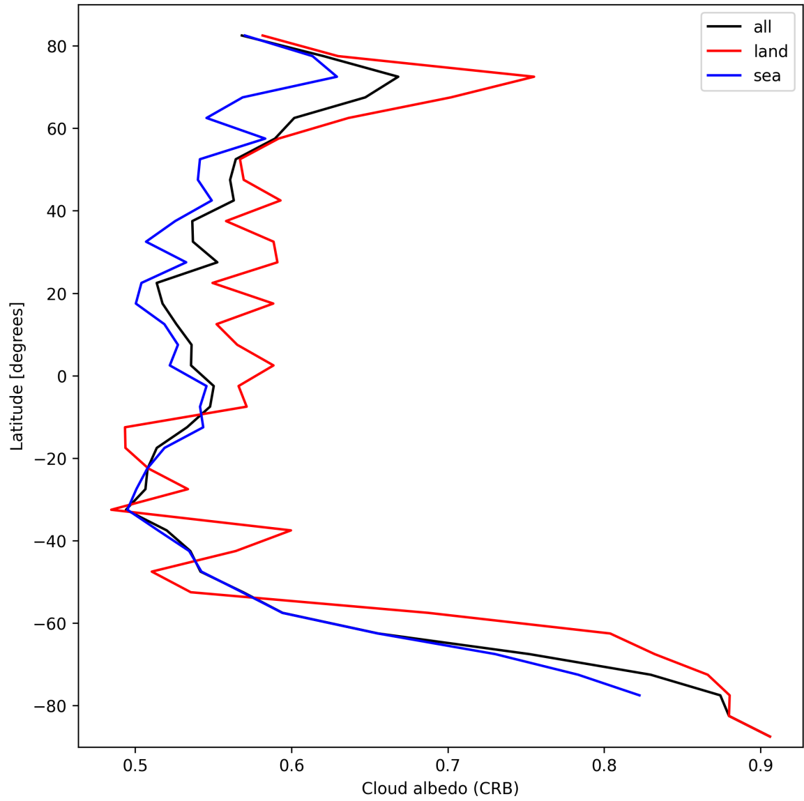
Figure 28: Zonal average of “Cloud albedo (CRB)” for 2024-10-05 to 2024-10-07.
