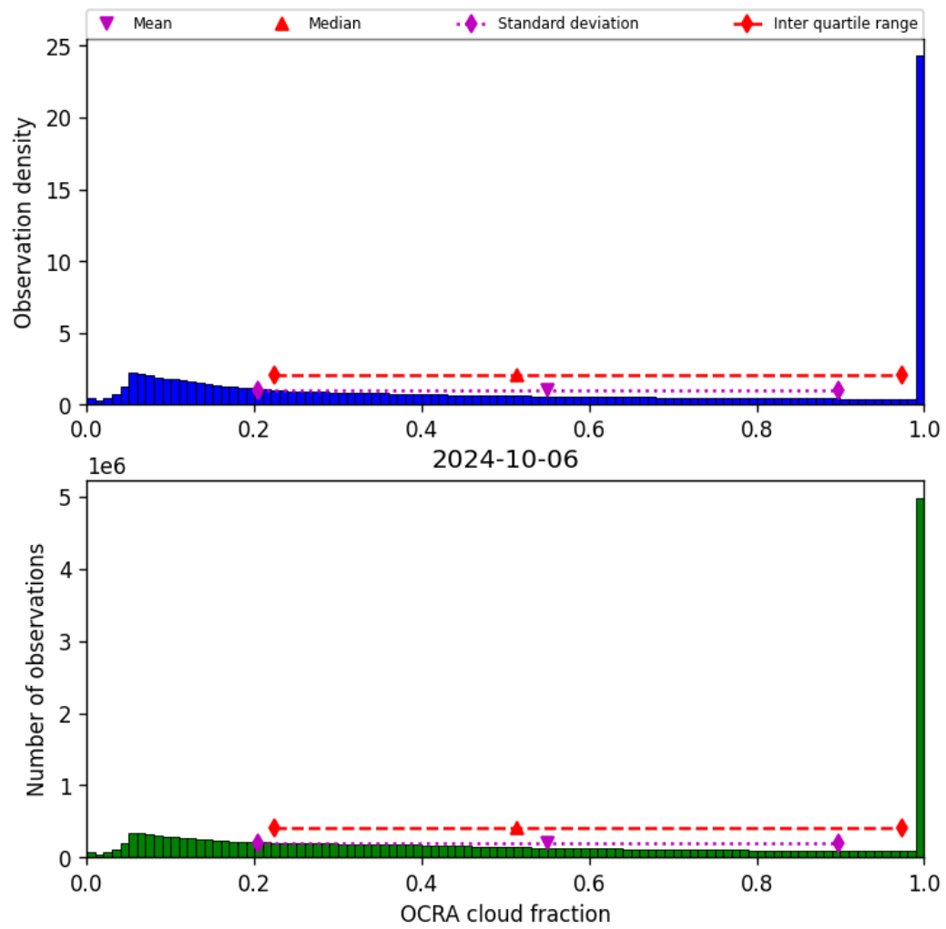
Figure 50: Histogram of “OCRA cloud fraction” for 2024-10-05 to 2024-10-07
