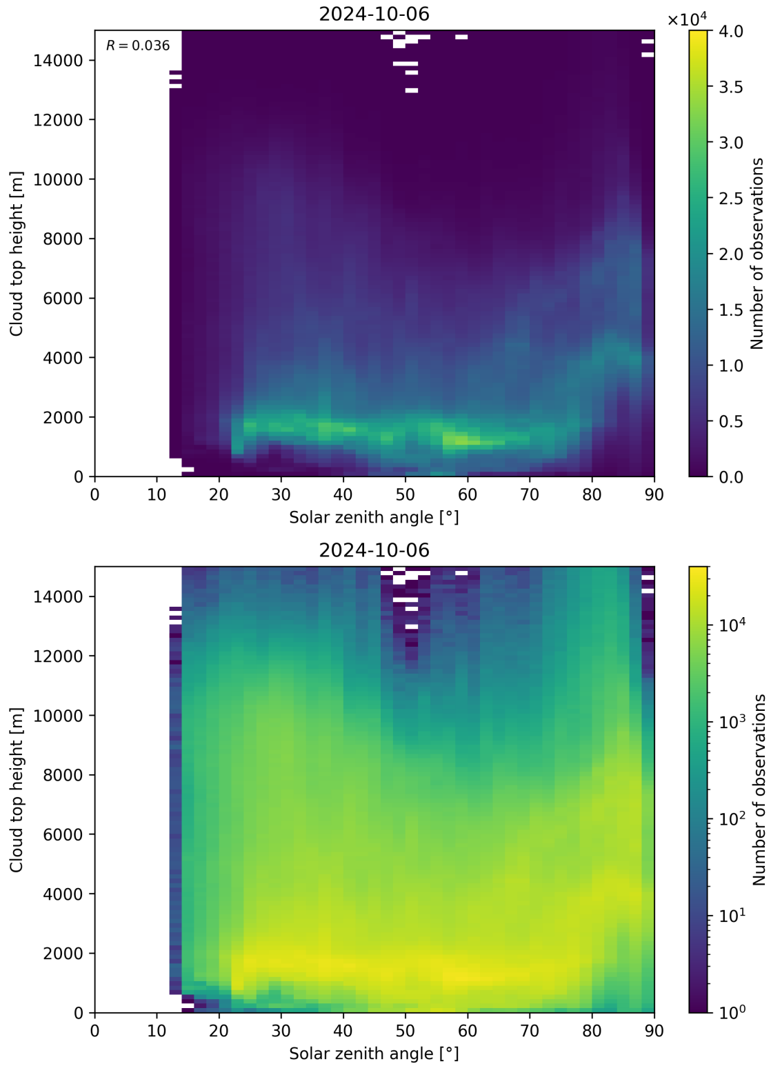
Figure 104: Scatter density plot of “Solar zenith angle” against “Cloud top height” for 2024-10-05 to 2024-10-07.
