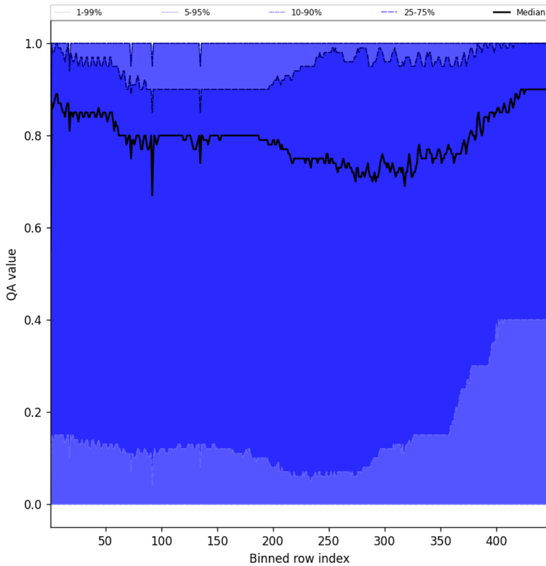
Figure 54: Along track statistics of “QA value” for 2024-10-05 to 2024-10-07
