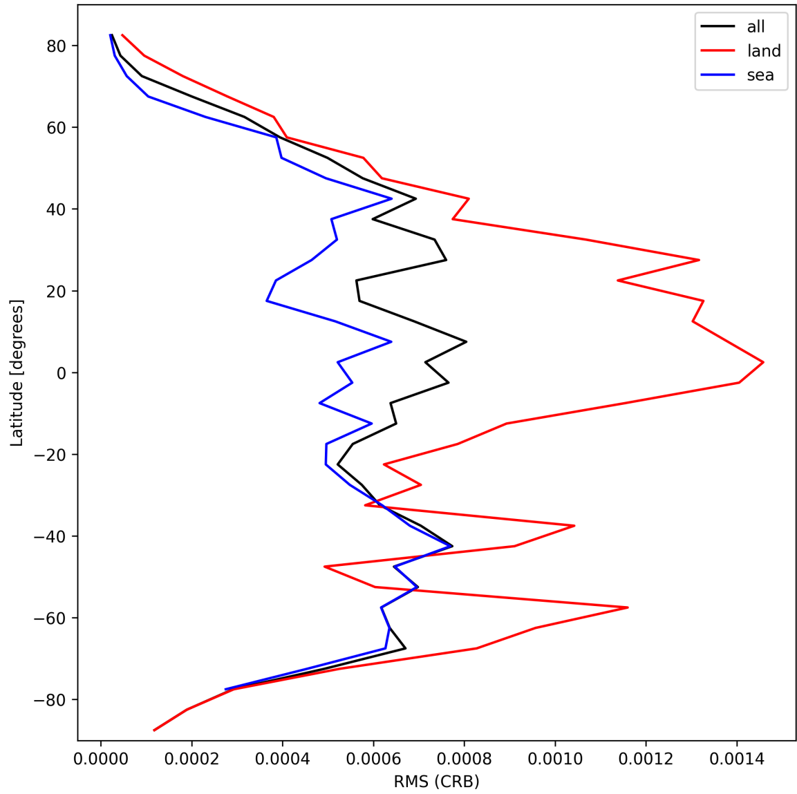
Figure 32: Zonal average of “RMS (CRB)” for 2024-10-05 to 2024-10-07.
