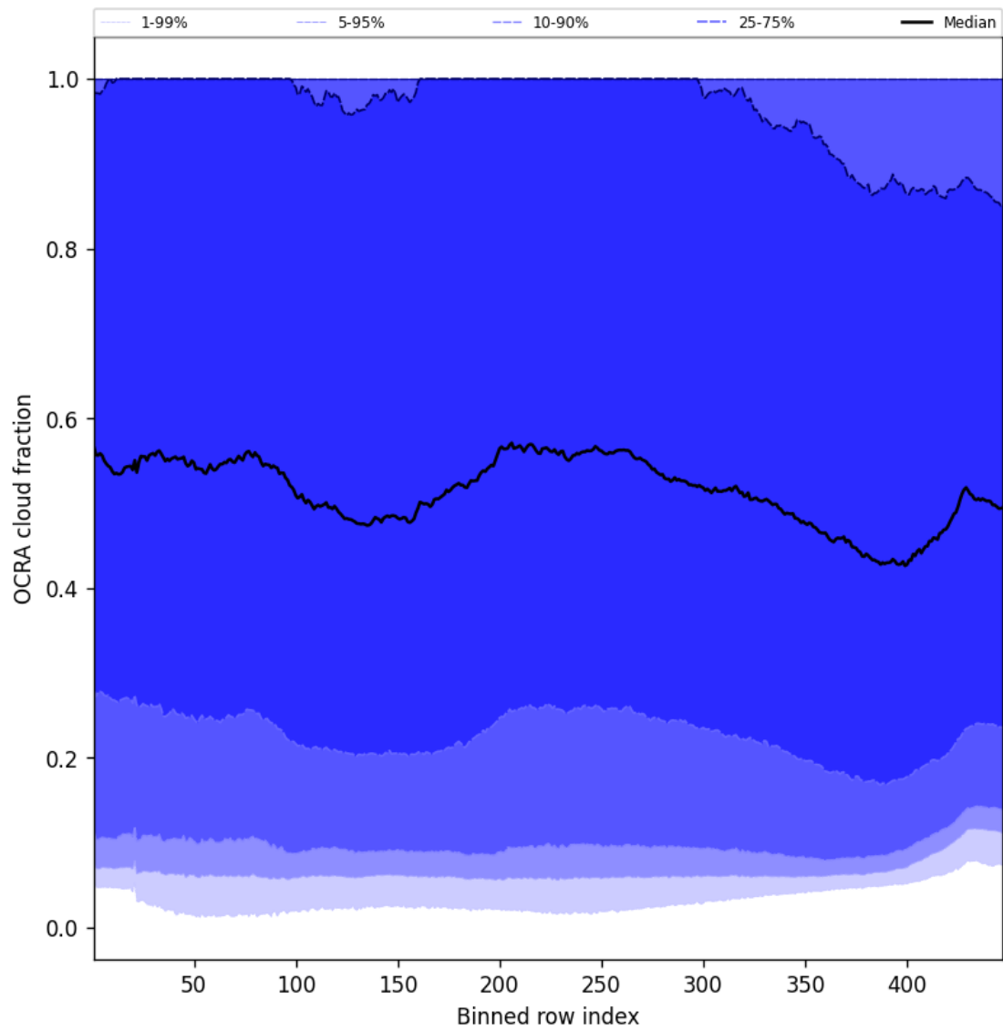
Figure 66: Along track statistics of “OCRA cloud fraction” for 2024-10-05 to 2024-10-07
