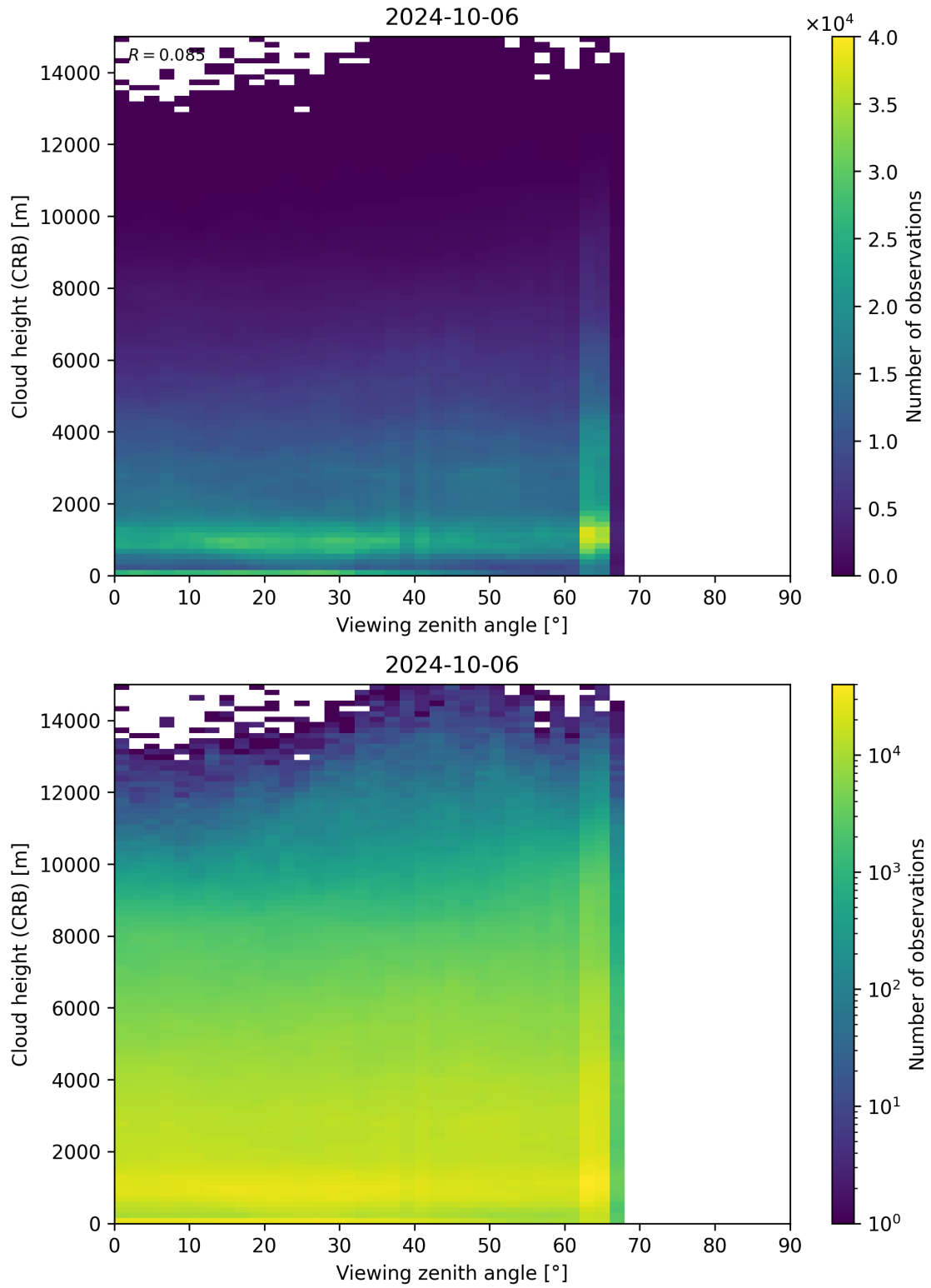
Figure 110: Scatter density plot of “Viewing zenith angle” against “Cloud height (CRB)” for 2024-10-05 to 2024-10-07.
