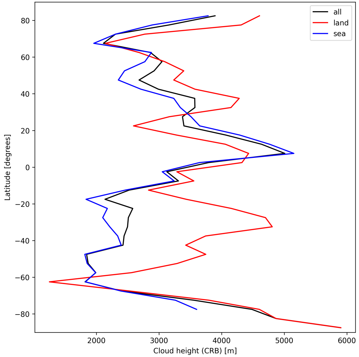
Figure 27: Zonal average of “Cloud height (CRB)” for 2024-10-05 to 2024-10-07.
