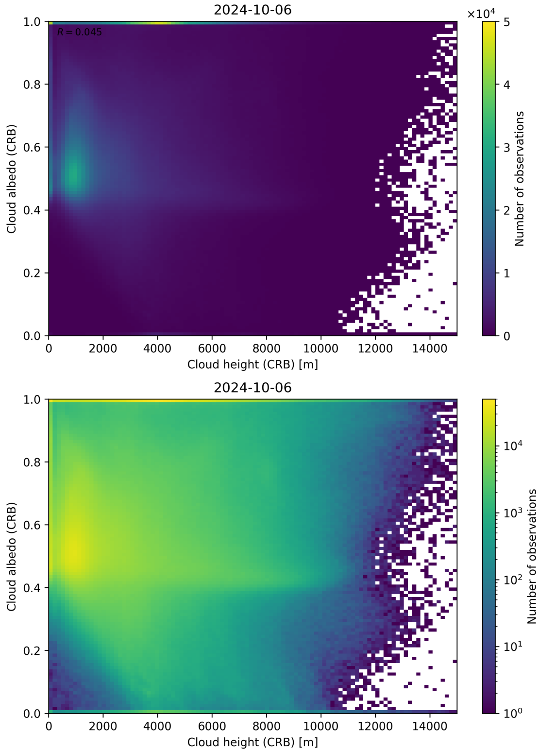
Figure 80: Scatter density plot of “Cloud height (CRB)” against “Cloud albedo (CRB)” for 2024-10-05 to 2024-10-07.
