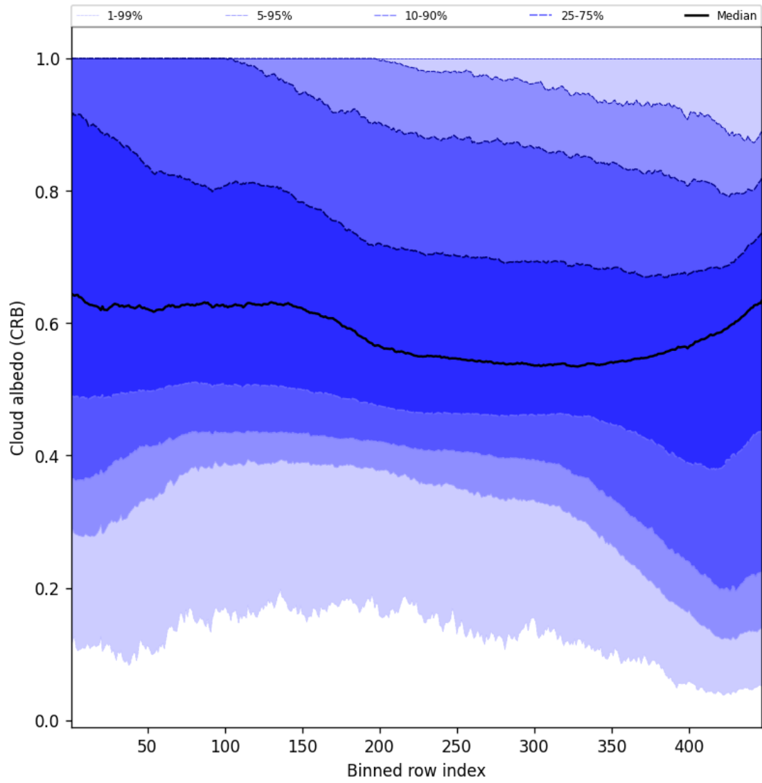
Figure 60: Along track statistics of “Cloud albedo (CRB)” for 2024-10-05 to 2024-10-07
