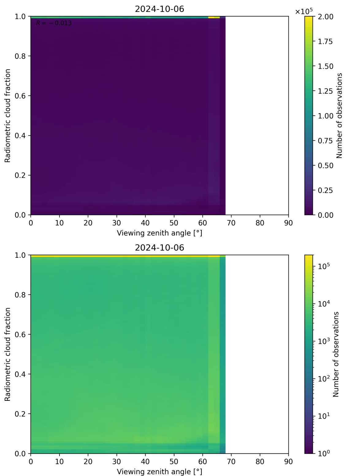
Figure 107: Scatter density plot of “Viewing zenith angle” against “Radiometric cloud fraction” for 2024-10-05 to 2024-10-07.
