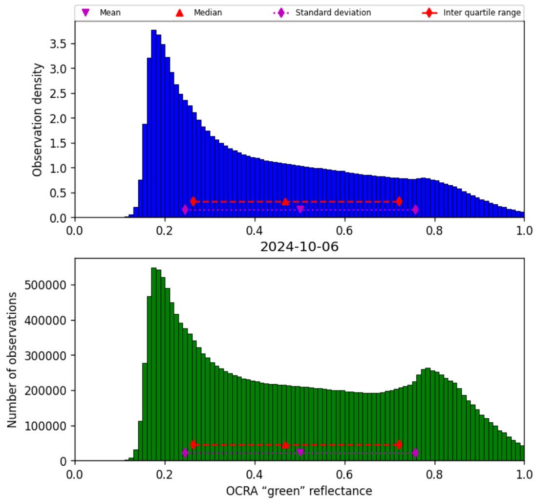
Figure 52: Histogram of “OCRA “green” reflectance” for 2024-10-05 to 2024-10-07
