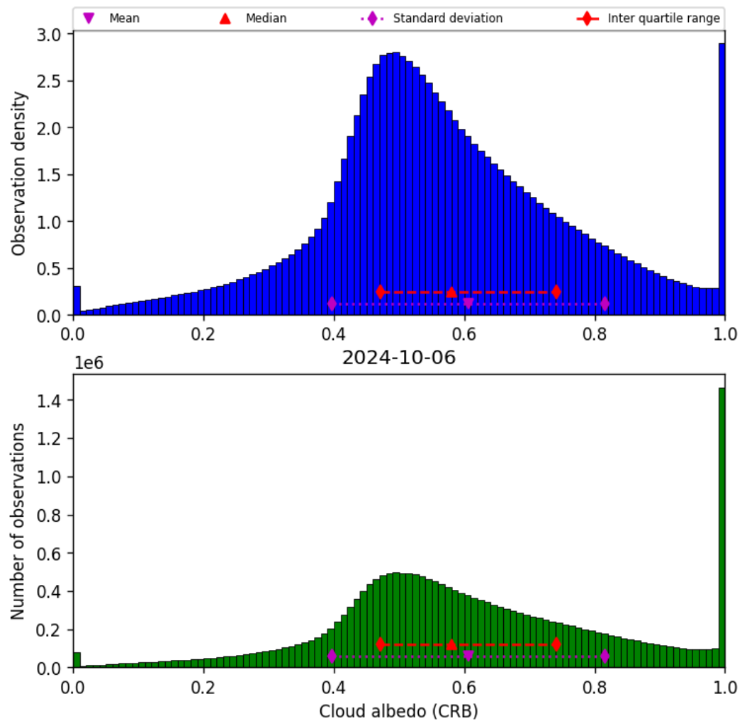
Figure 44: Histogram of “Cloud albedo (CRB)” for 2024-10-05 to 2024-10-07
