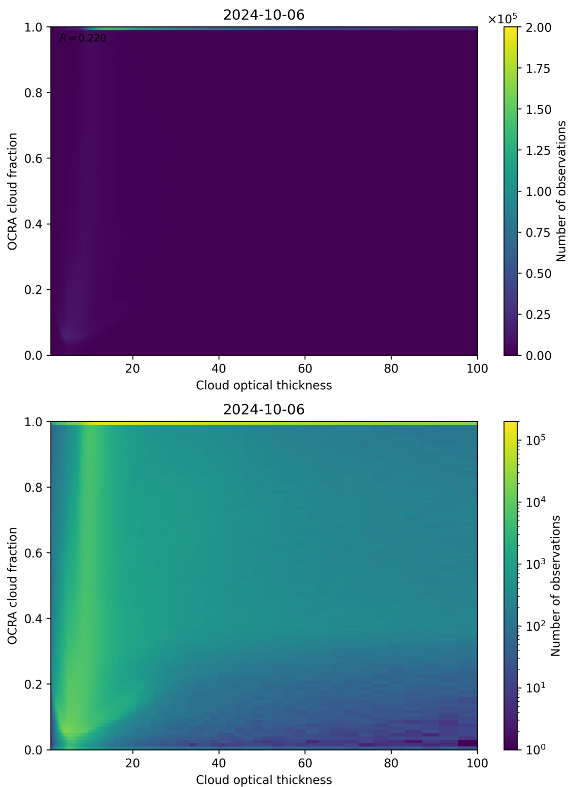
Figure 83: Scatter density plot of “Cloud optical thickness” against “OCRA cloud fraction” for 2024-10-05 to 2024-10-07.
