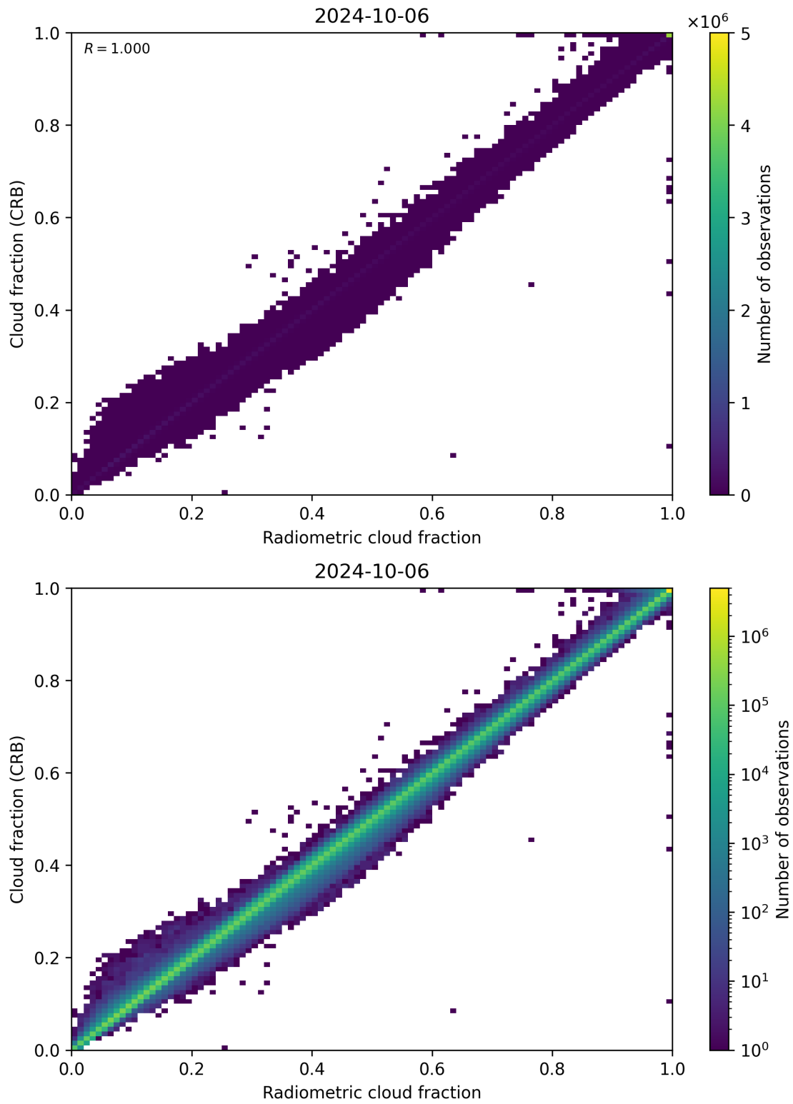
Figure 73: Scatter density plot of “Radiometric cloud fraction” against “Cloud fraction (CRB)” for 2024-10-05 to 2024-10-07.
