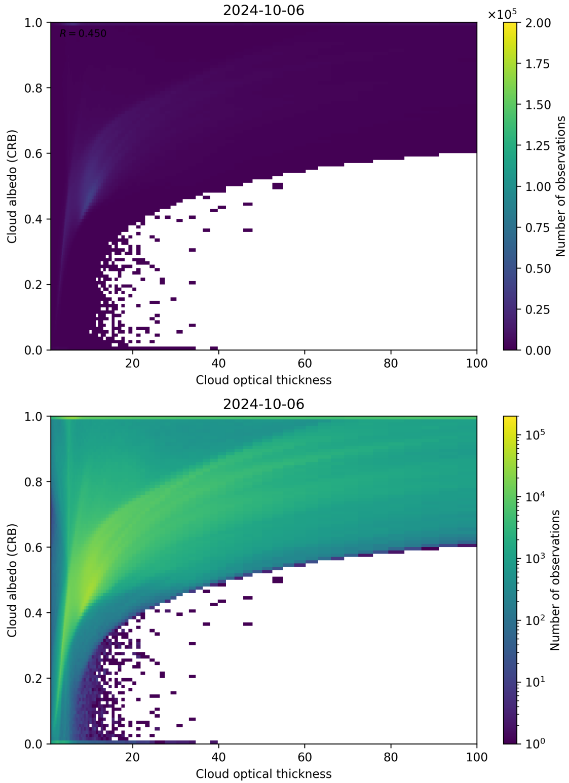
Figure 82: Scatter density plot of “Cloud optical thickness” against “Cloud albedo (CRB)” for 2024-10-05 to 2024-10-07.
