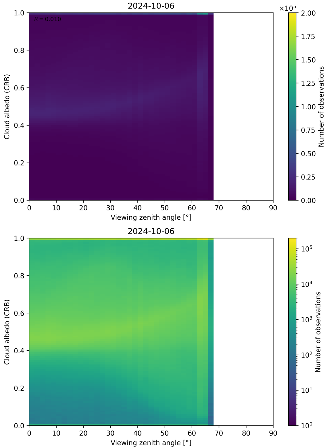
Figure 106: Scatter density plot of “Viewing zenith angle” against “Cloud albedo (CRB)” for 2024-10-05 to 2024-10-07.
