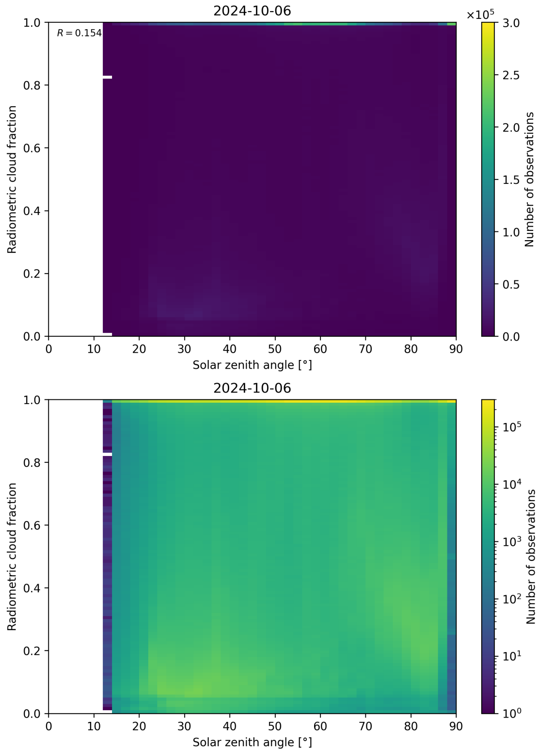
Figure 99: Scatter density plot of “Solar zenith angle” against “Radiometric cloud fraction” for 2024-10-05 to 2024-10-07.
