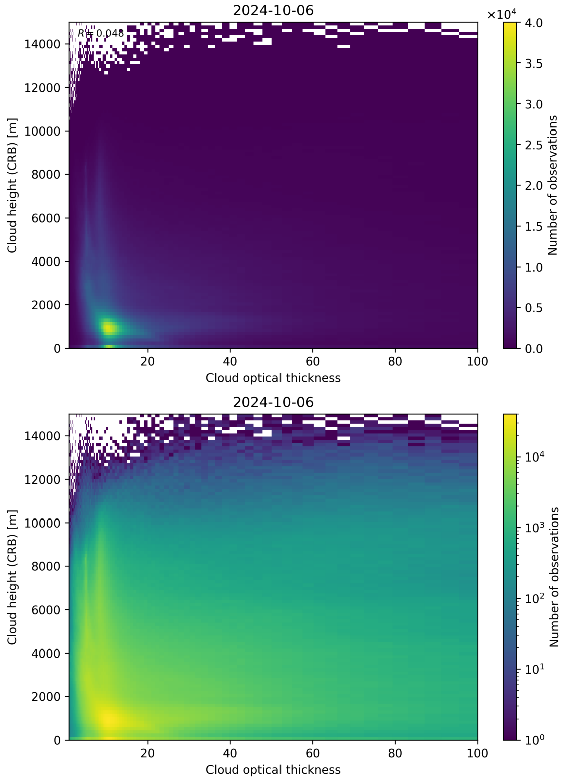
Figure 85: Scatter density plot of “Cloud optical thickness” against “Cloud height (CRB)” for 2024-10-05 to 2024-10-07.
