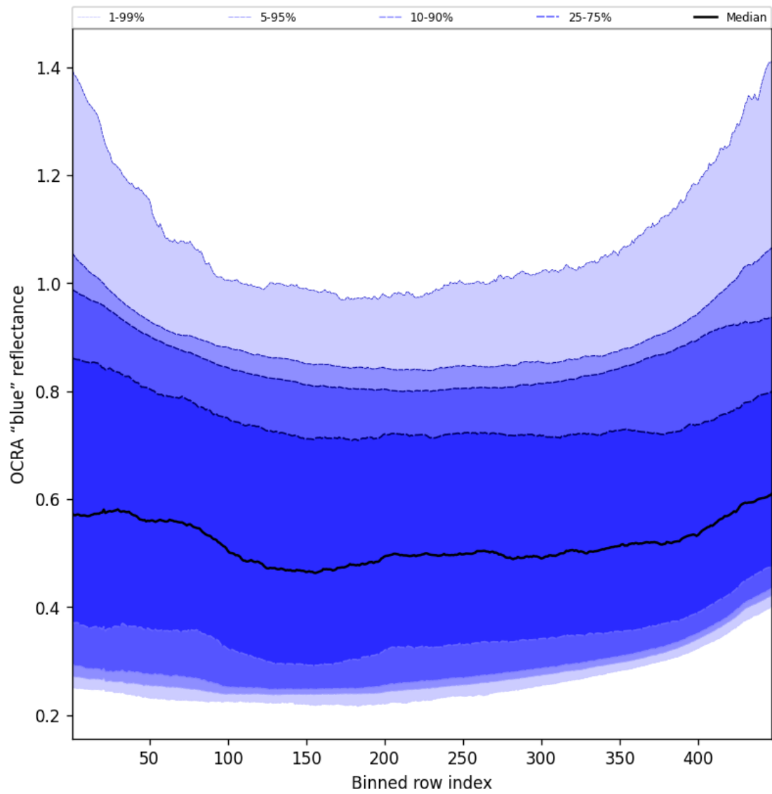
Figure 67: Along track statistics of “OCRA “blue” reflectance” for 2024-10-05 to 2024-10-07
