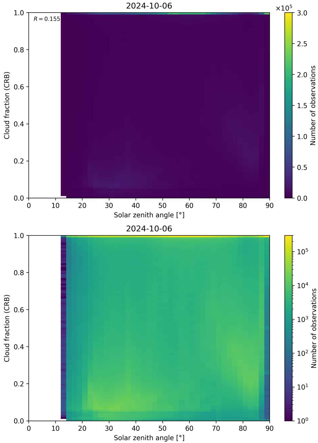
Figure 101: Scatter density plot of “Solar zenith angle” against “Cloud fraction (CRB)” for 2024-10-05 to 2024-10-07.
