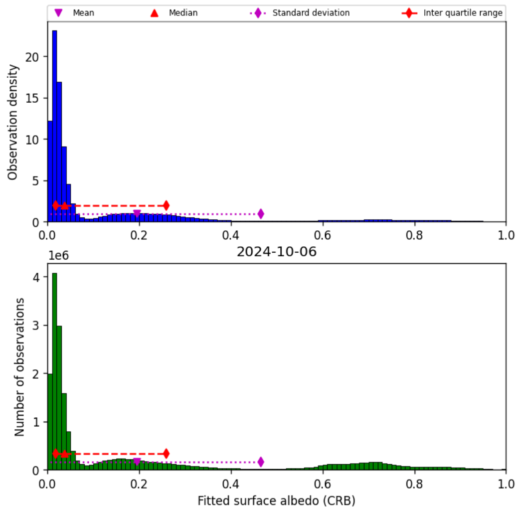
Figure 46: Histogram of “Fitted surface albedo (CRB)” for 2024-10-05 to 2024-10-07
