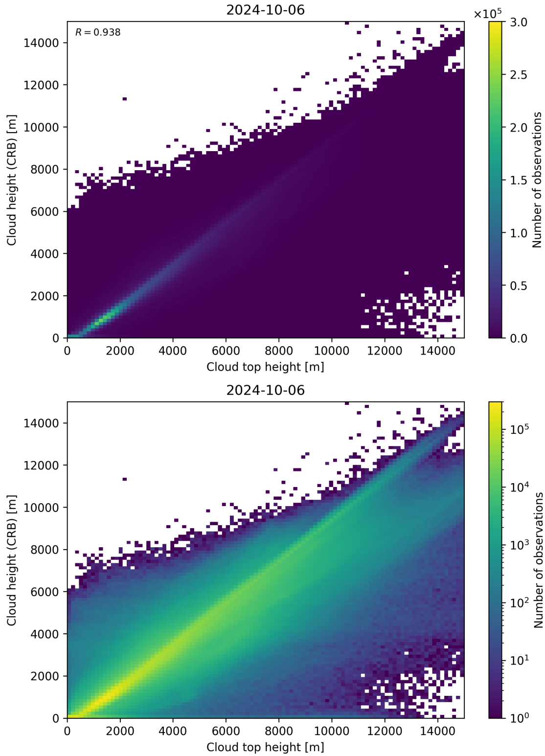
Figure 89: Scatter density plot of “Cloud top height” against “Cloud height (CRB)” for 2024-10-05 to 2024-10-07.
