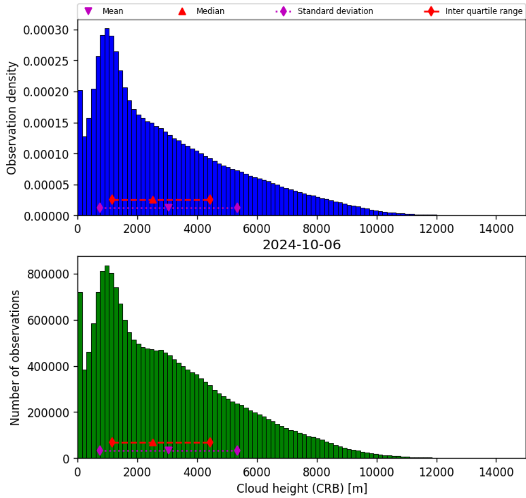
Figure 43: Histogram of “Cloud height (CRB)” for 2024-10-05 to 2024-10-07
