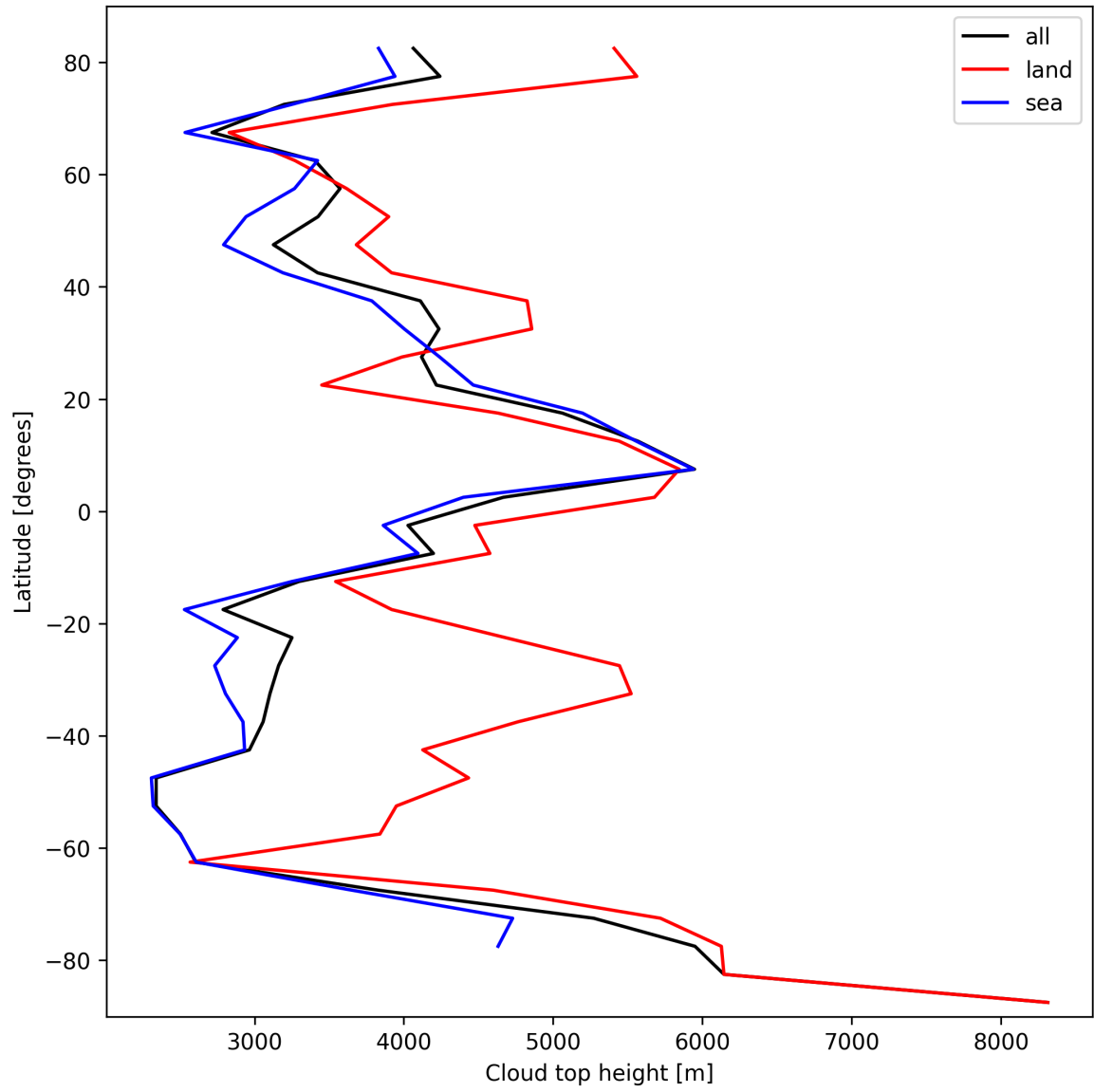
Figure 24: Zonal average of “Cloud top height” for 2024-10-05 to 2024-10-07.
