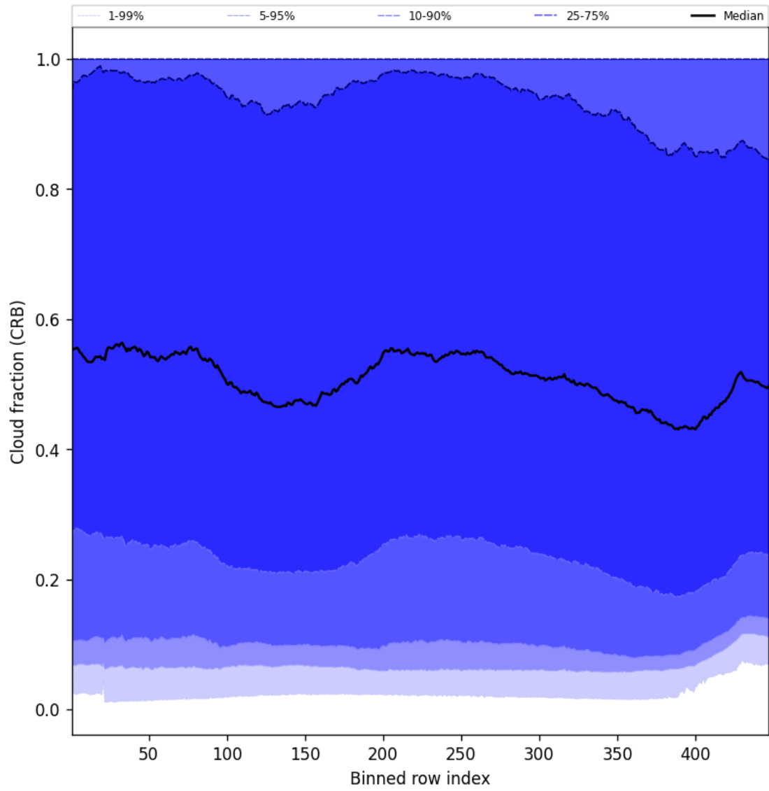
Figure 58: Along track statistics of “Cloud fraction (CRB)” for 2024-10-05 to 2024-10-07
