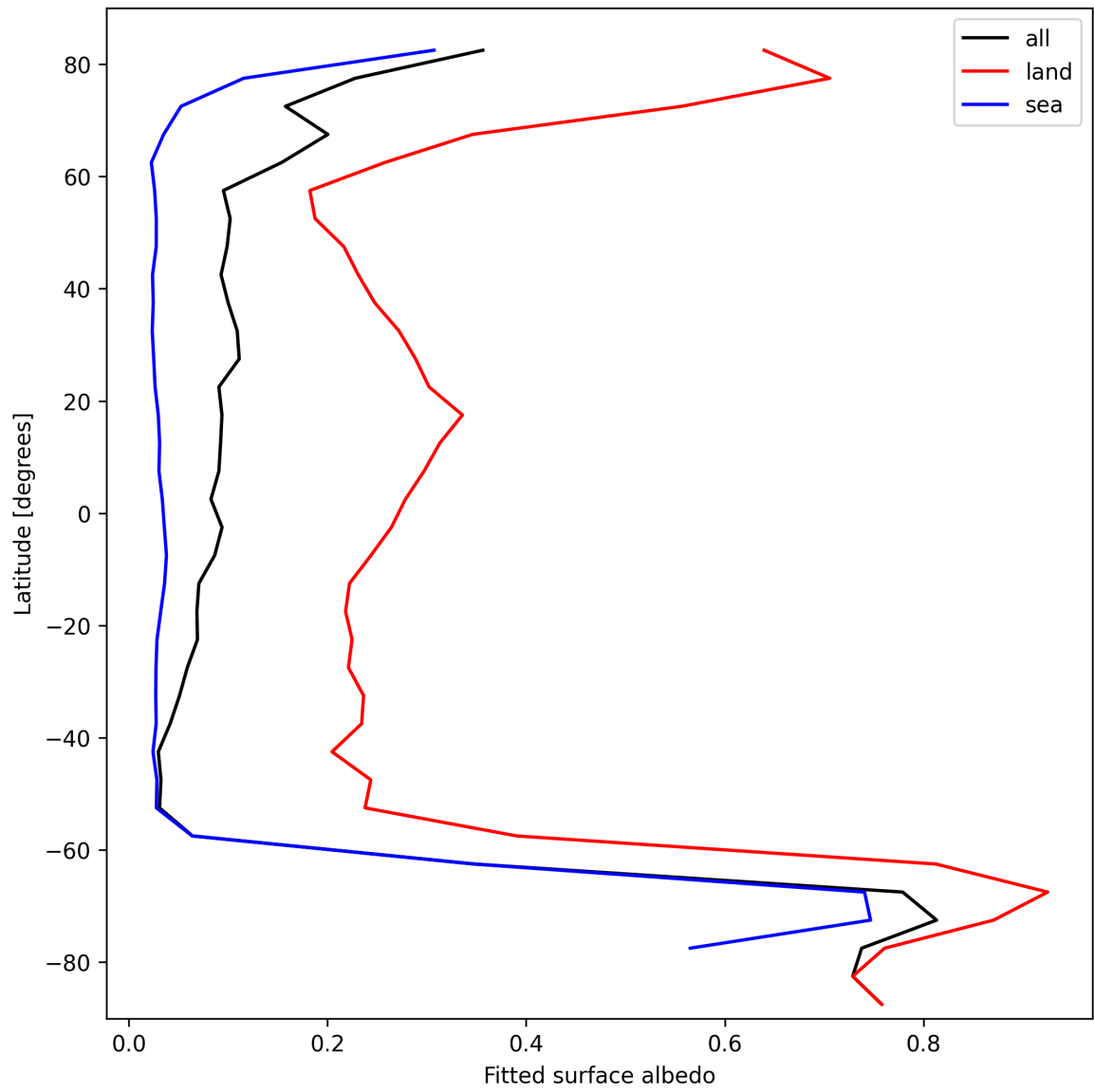
Figure 29: Zonal average of “Fitted surface albedo” for 2024-10-05 to 2024-10-07.
