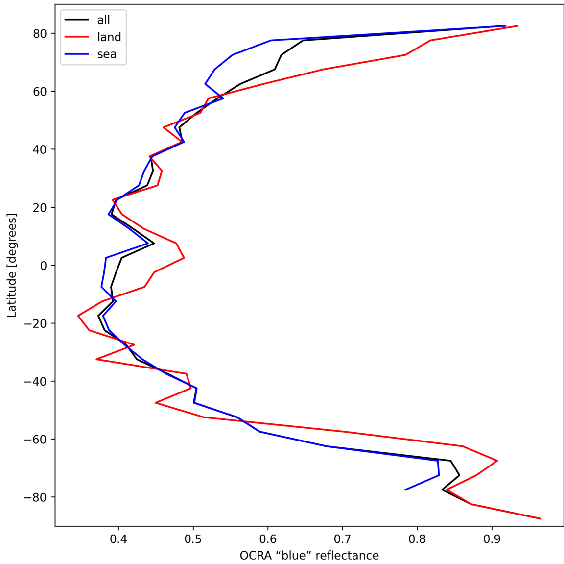
Figure 35: Zonal average of “OCRA “blue” reflectance” for 2024-10-05 to 2024-10-07.
