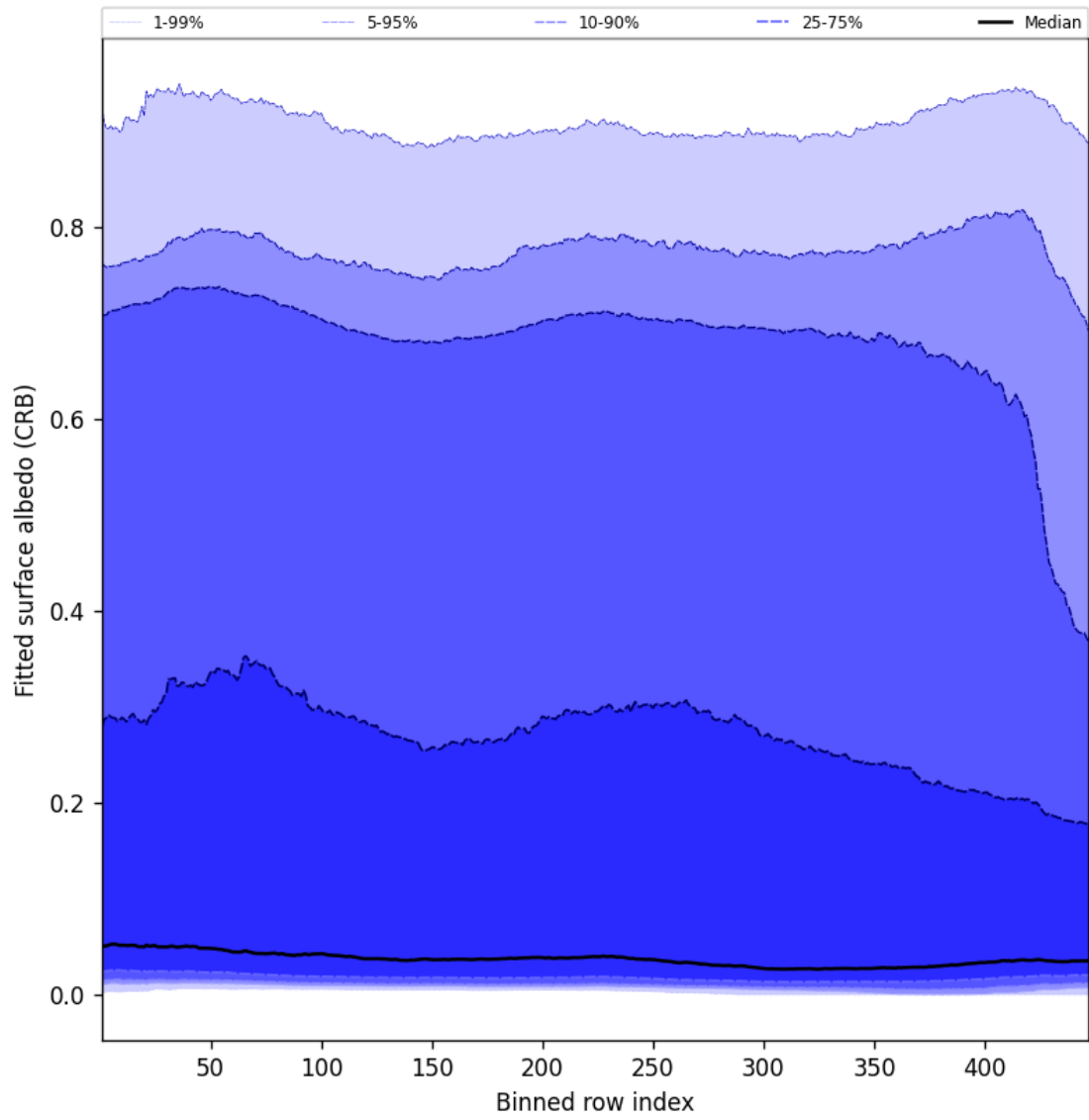
Figure 62: Along track statistics of “Fitted surface albedo (CRB)” for 2024-10-05 to 2024-10-07
