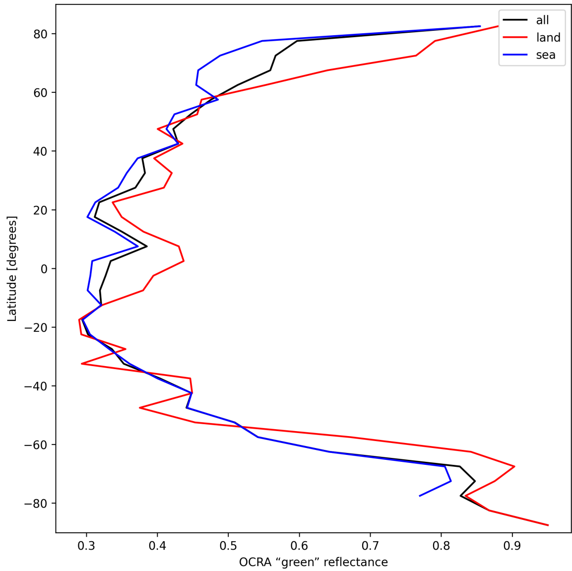
Figure 36: Zonal average of “OCRA “green” reflectance” for 2024-10-05 to 2024-10-07.
