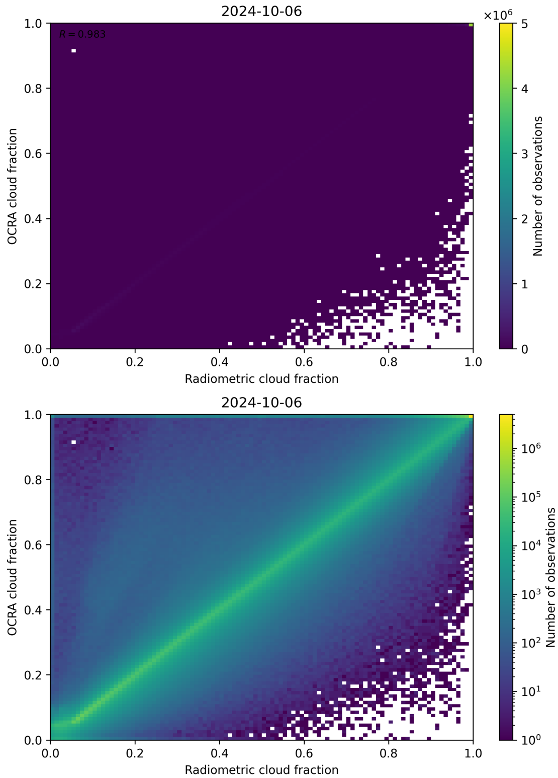
Figure 72: Scatter density plot of “Radiometric cloud fraction” against “OCRA cloud fraction” for 2024-10-05 to 2024-10-07.
