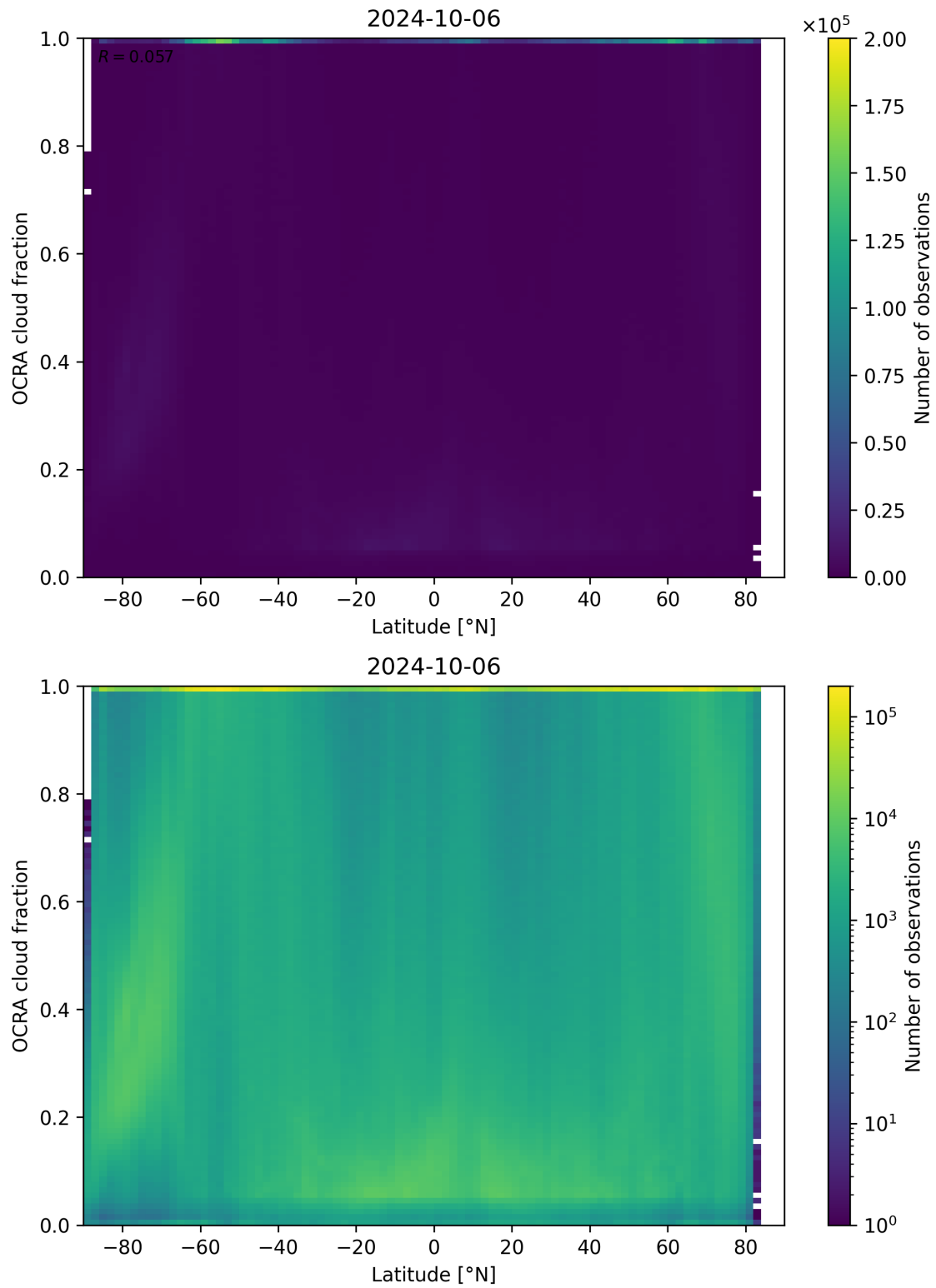
Figure 93: Scatter density plot of “Latitude” against “OCRA cloud fraction” for 2024-10-05 to 2024-10-07.
