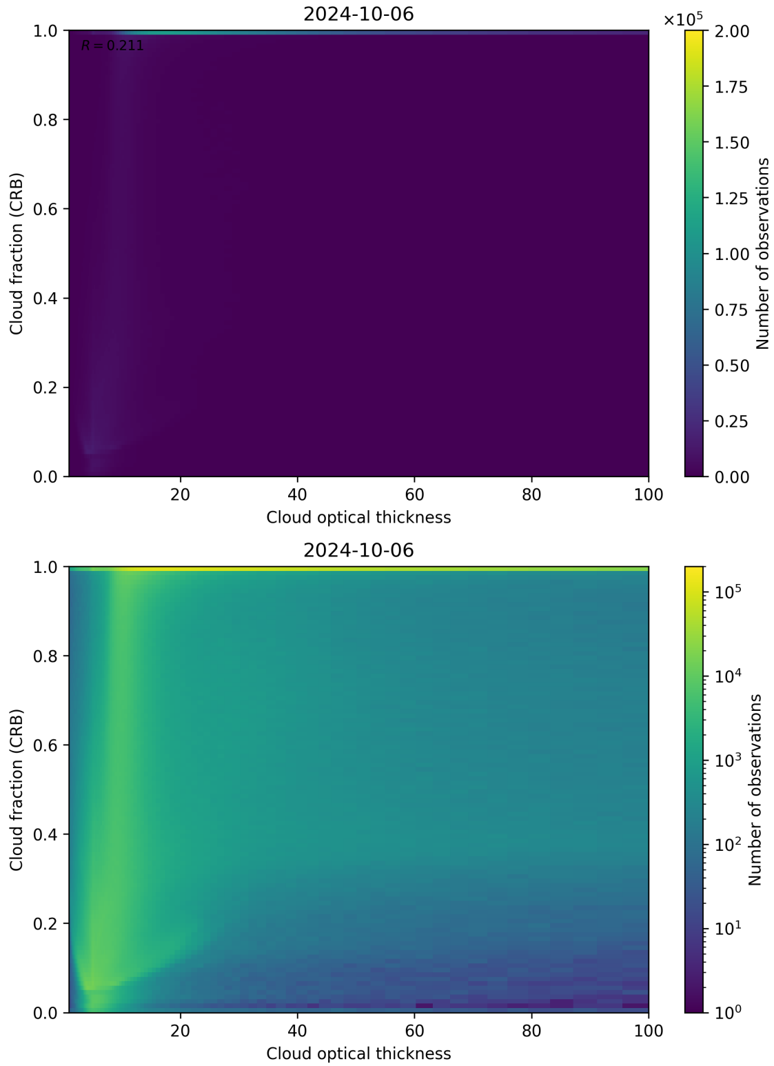
Figure 84: Scatter density plot of “Cloud optical thickness” against “Cloud fraction (CRB)” for 2024-10-05 to 2024-10-07.
