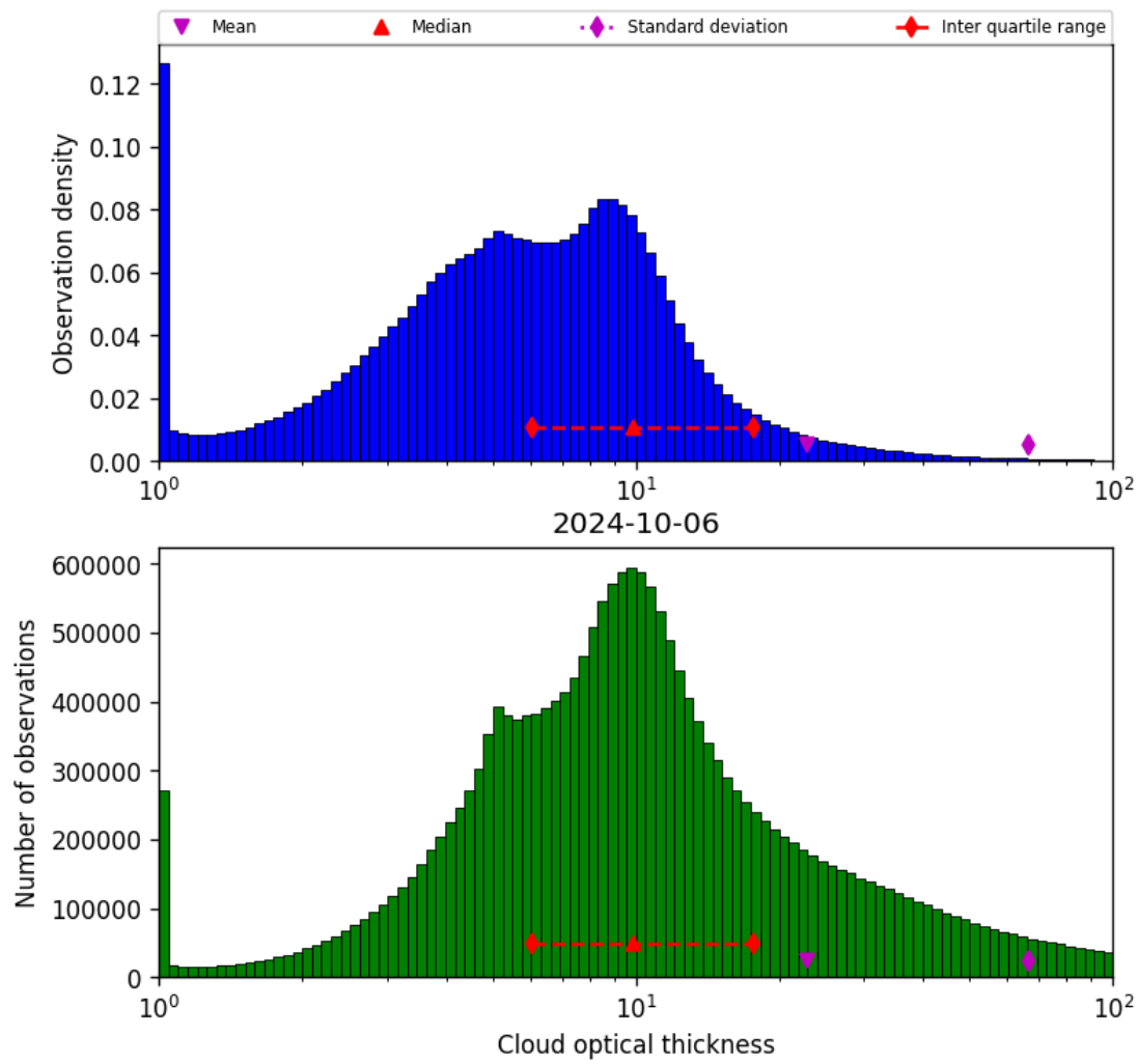
Figure 41: Histogram of “Cloud optical thickness” for 2024-10-05 to 2024-10-07
