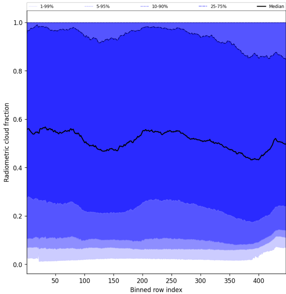
Figure 55: Along track statistics of “Radiometric cloud fraction” for 2024-10-05 to 2024-10-07
