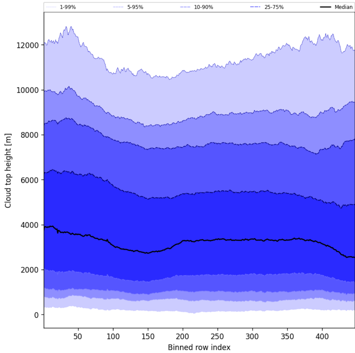
Figure 56: Along track statistics of “Cloud top height” for 2024-10-05 to 2024-10-07
