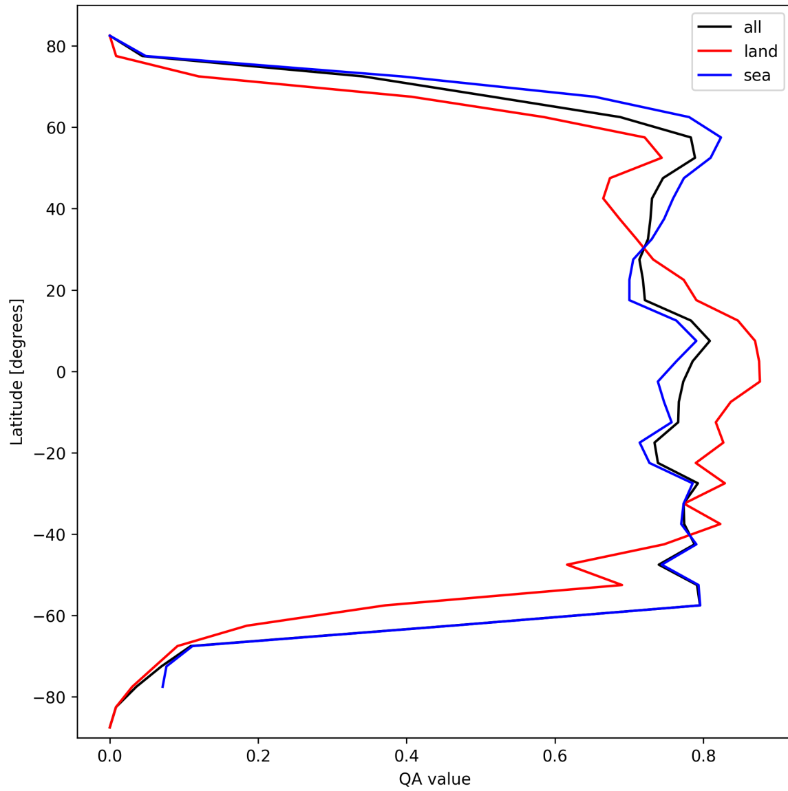
Figure 22: Zonal average of “QA value” for 2024-10-05 to 2024-10-07.
