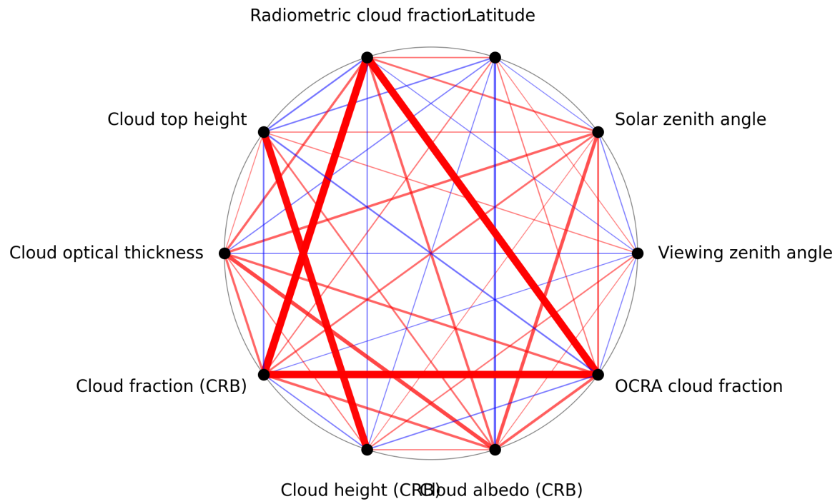
Figure 1: Map of correlation graph for 2024-10-05 to 2024-10-07.
