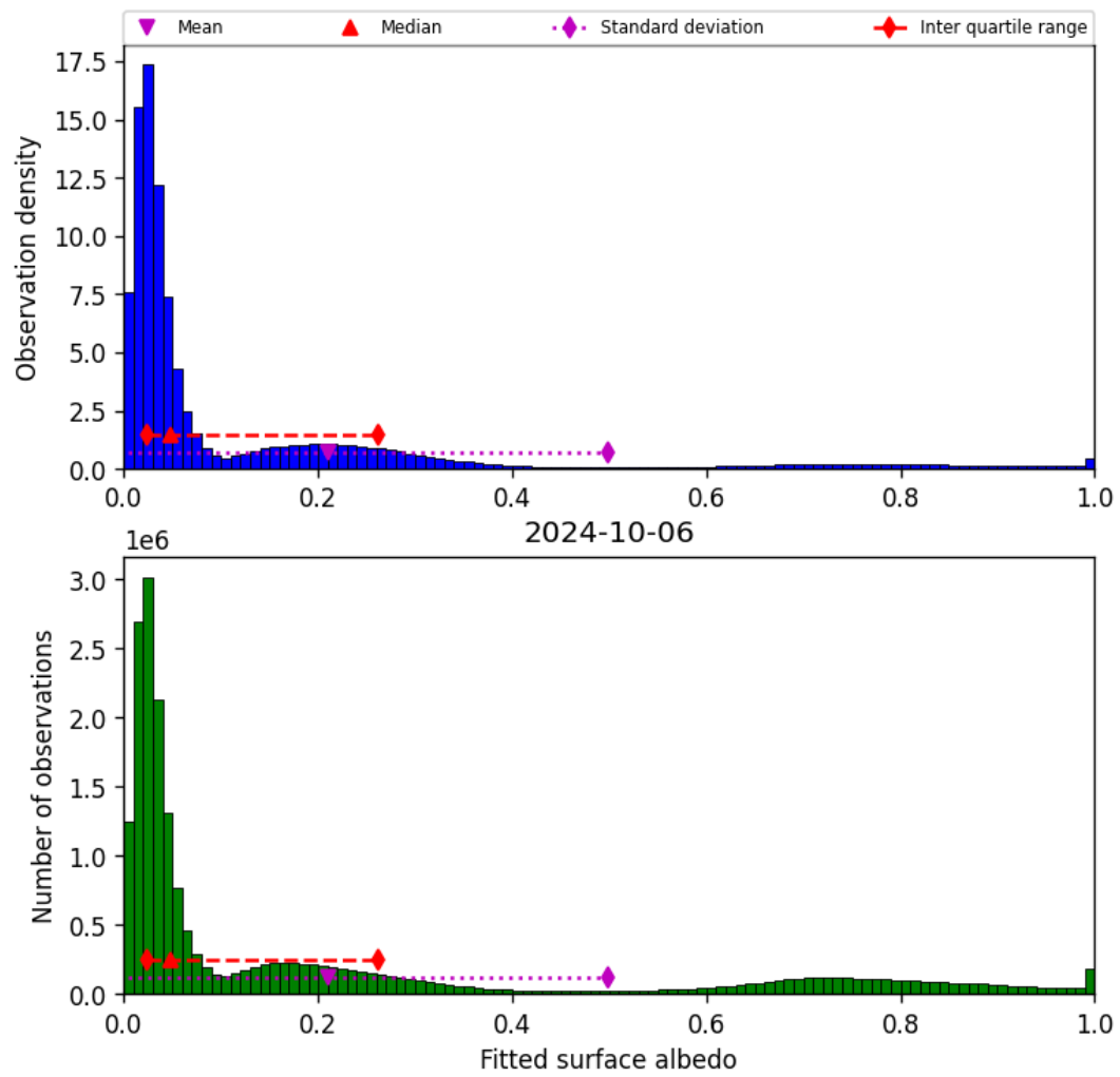
Figure 45: Histogram of “Fitted surface albedo” for 2024-10-05 to 2024-10-07
