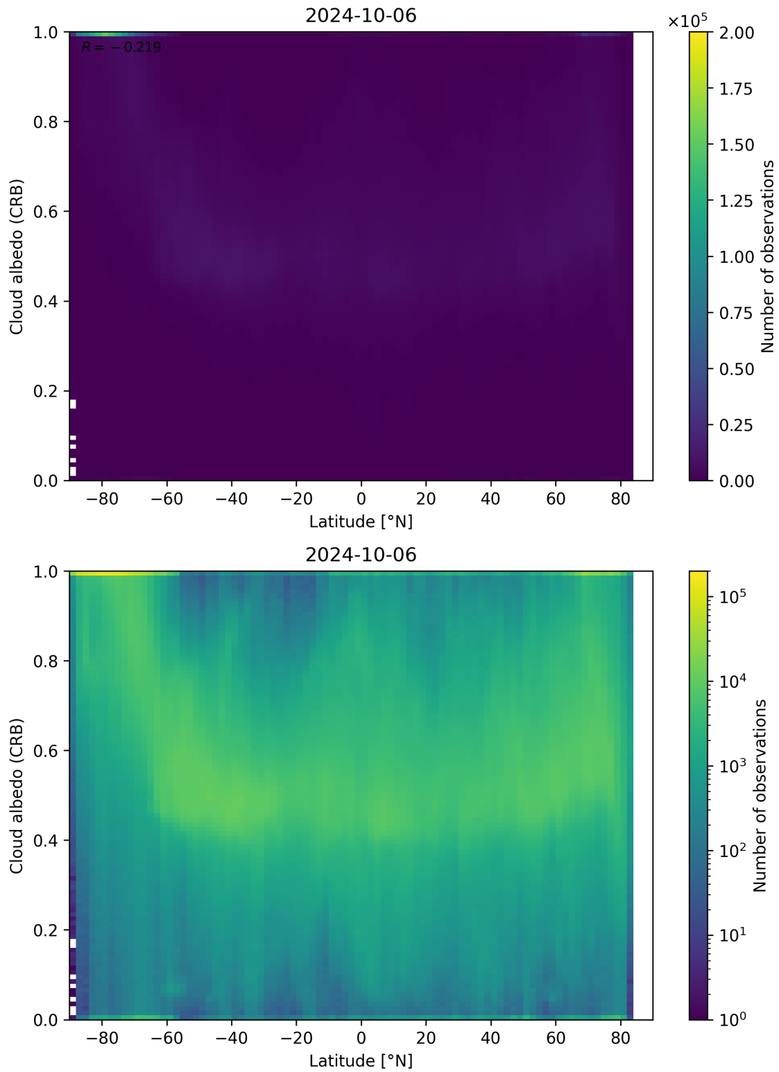
Figure 91: Scatter density plot of “Latitude” against “Cloud albedo (CRB)” for 2024-10-05 to 2024-10-07.
