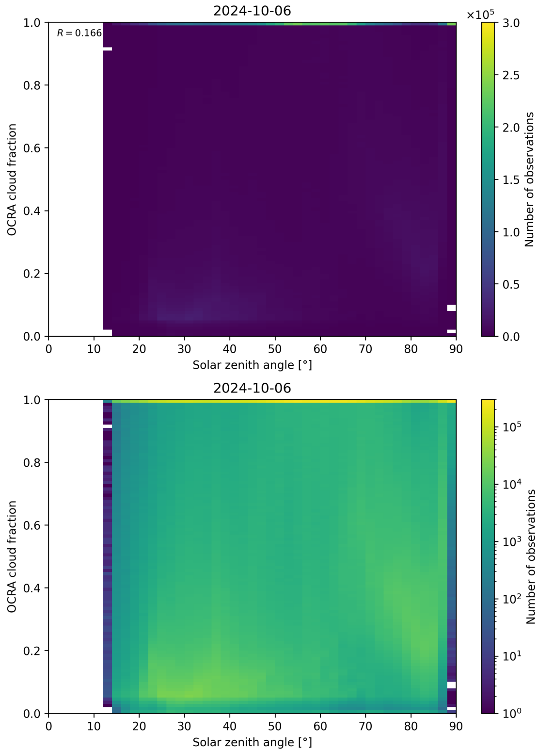
Figure 100: Scatter density plot of “Solar zenith angle” against “OCRA cloud fraction” for 2024-10-05 to 2024-10-07.
