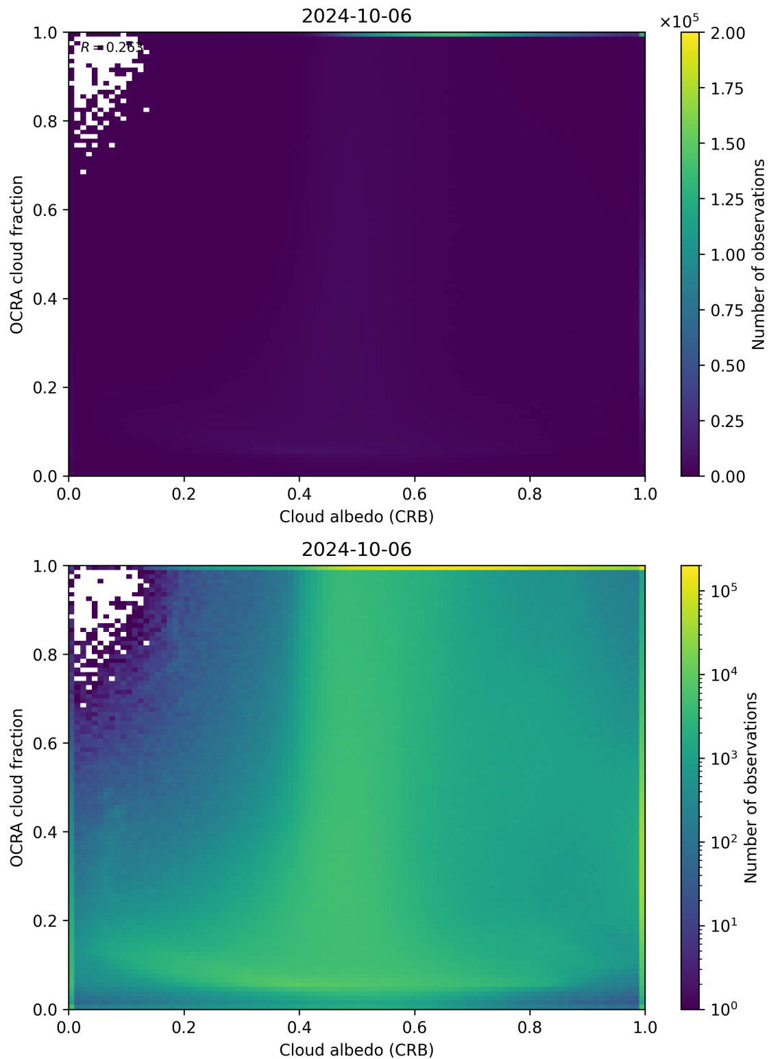
Figure 70: Scatter density plot of “Cloud albedo (CRB)” against “OCRA cloud fraction” for 2024-10-05 to 2024-10-07.
