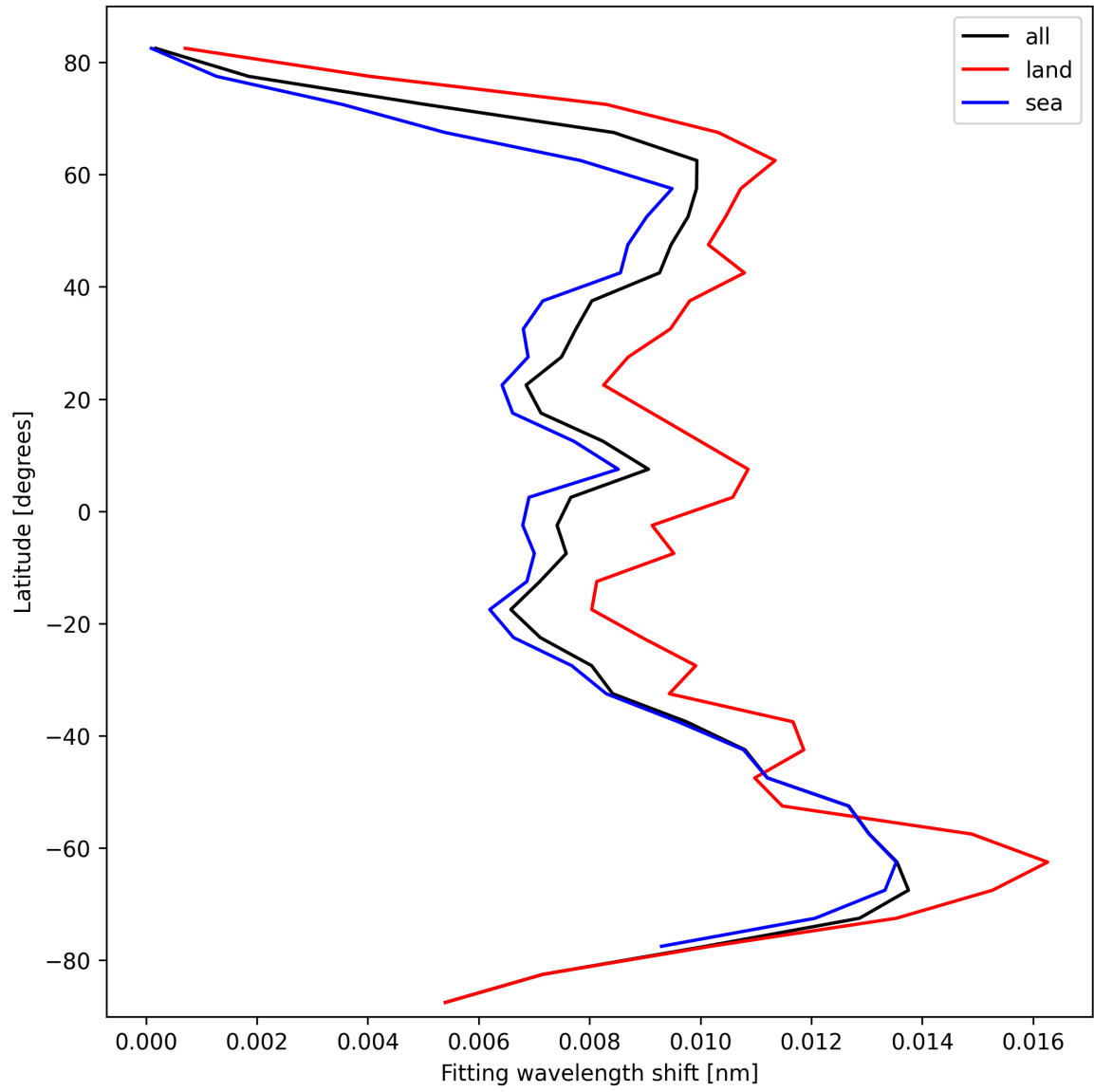
Figure 33: Zonal average of “Fitting wavelength shift” for 2024-10-05 to 2024-10-07.
