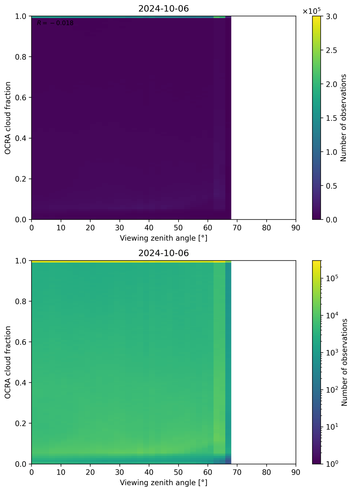
Figure 108: Scatter density plot of “Viewing zenith angle” against “OCRA cloud fraction” for 2024-10-05 to 2024-10-07.
