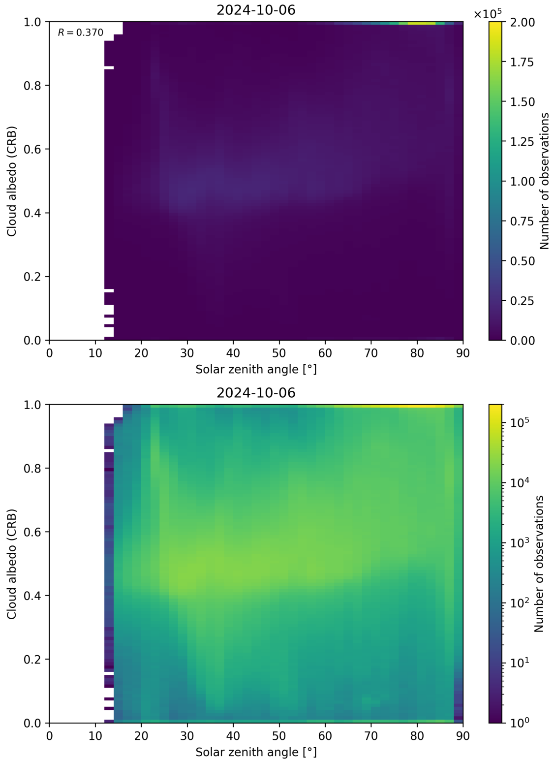
Figure 98: Scatter density plot of “Solar zenith angle” against “Cloud albedo (CRB)” for 2024-10-05 to 2024-10-07.
