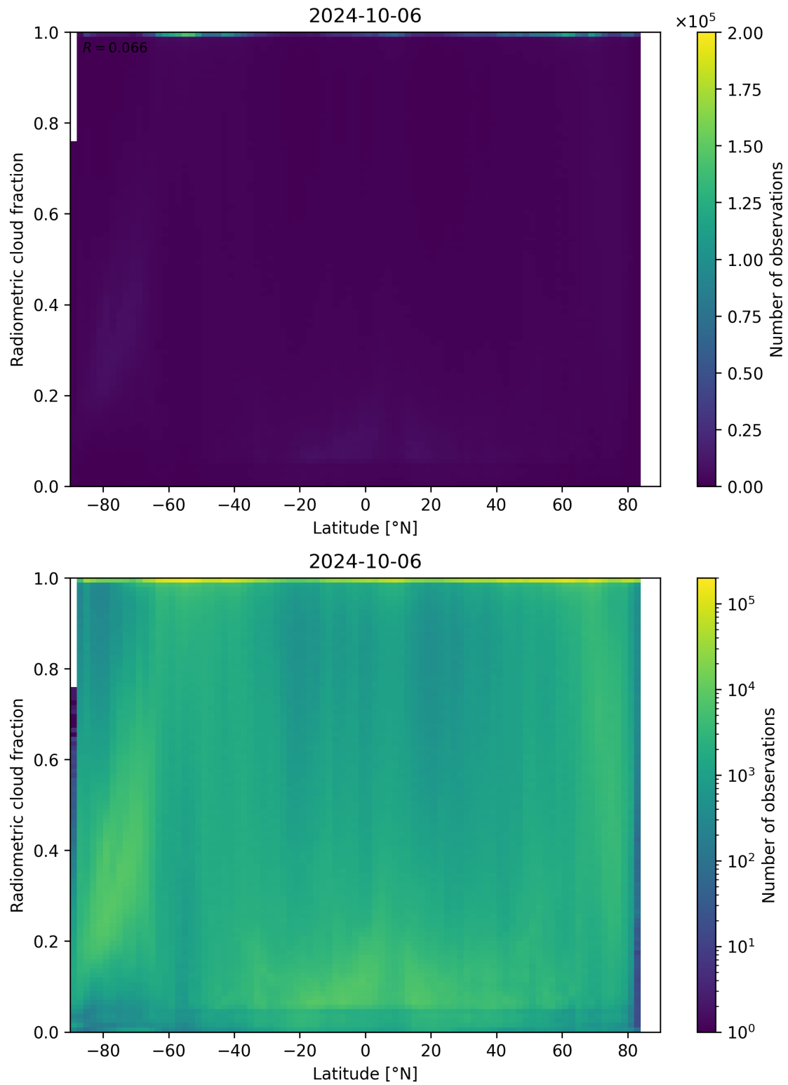
Figure 92: Scatter density plot of “Latitude” against “Radiometric cloud fraction” for 2024-10-05 to 2024-10-07.
