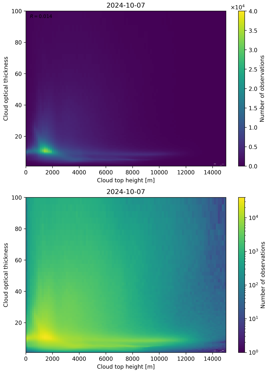
Figure 90: Scatter density plot of “Cloud top height” against “Cloud optical thickness” for 2024-10-06 to 2024-10-08.
