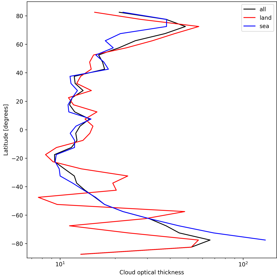
Figure 25: Zonal average of “Cloud optical thickness” for 2024-10-06 to 2024-10-08.
