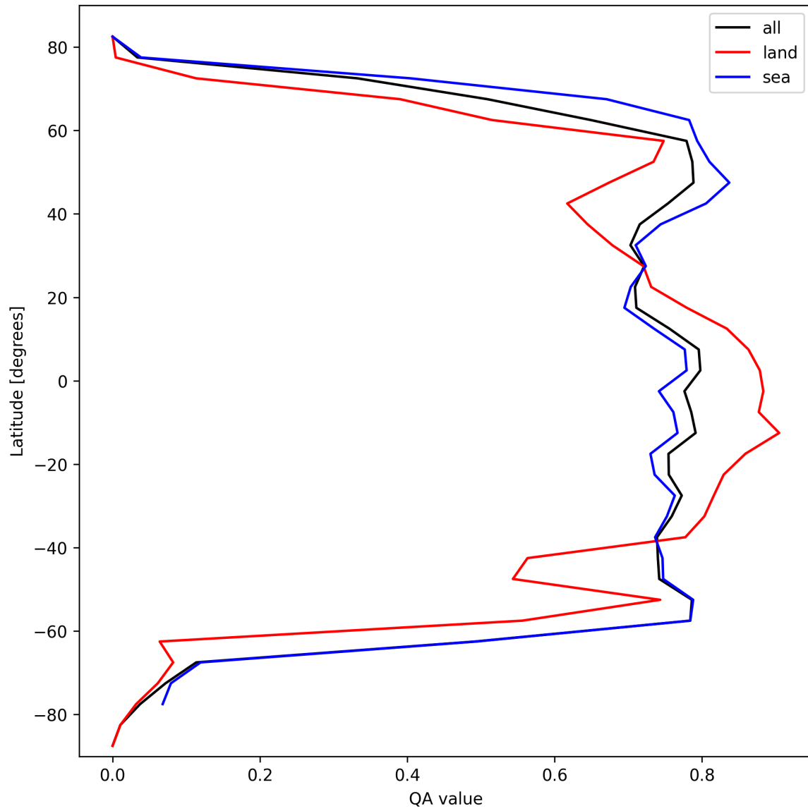
Figure 22: Zonal average of “QA value” for 2024-10-06 to 2024-10-08.
