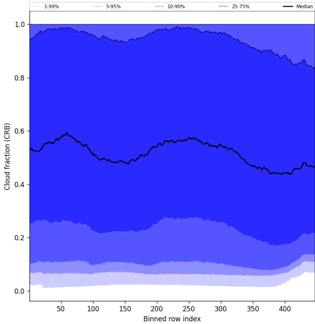
Figure 58: Along track statistics of “Cloud fraction (CRB)” for 2024-10-06 to 2024-10-08
