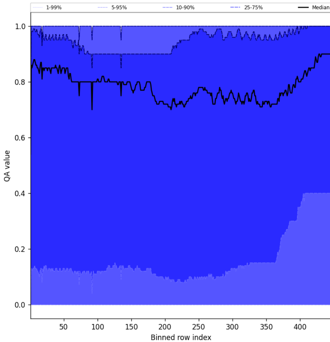
Figure 54: Along track statistics of “QA value” for 2024-10-06 to 2024-10-08
