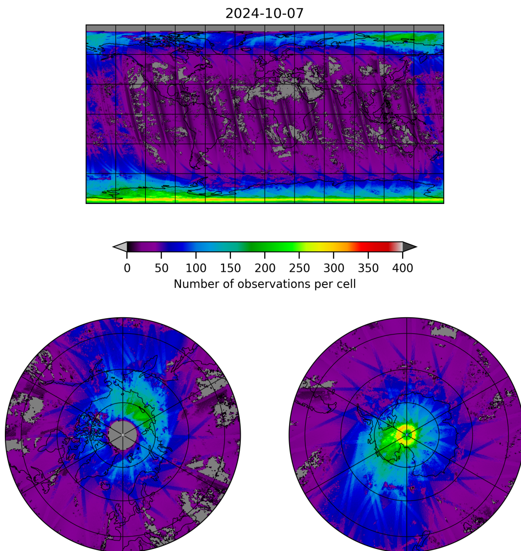
Figure 21: Map of the number of observations for 2024-10-06 to 2024-10-08
