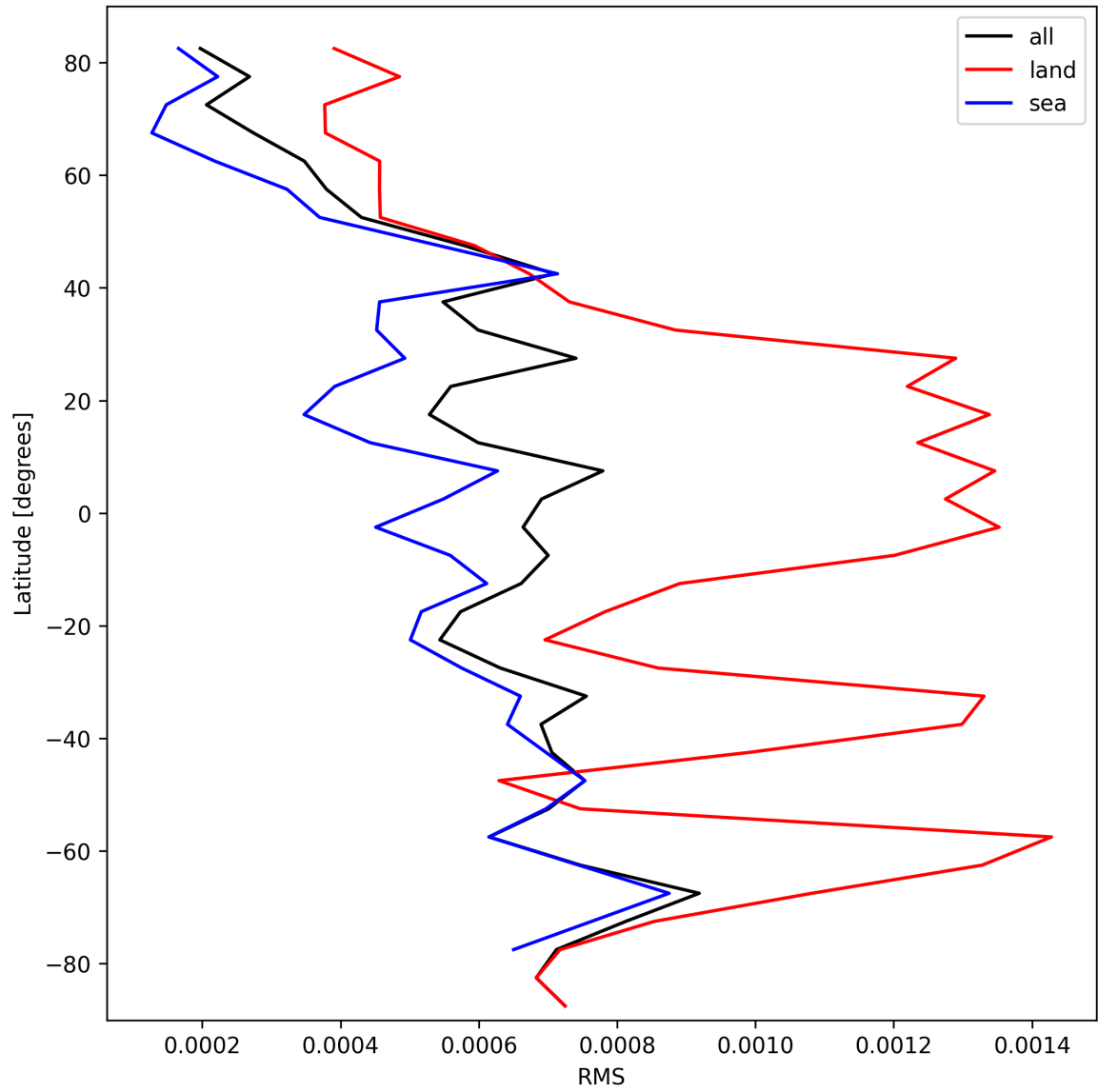
Figure 31: Zonal average of “RMS” for 2024-10-06 to 2024-10-08.
