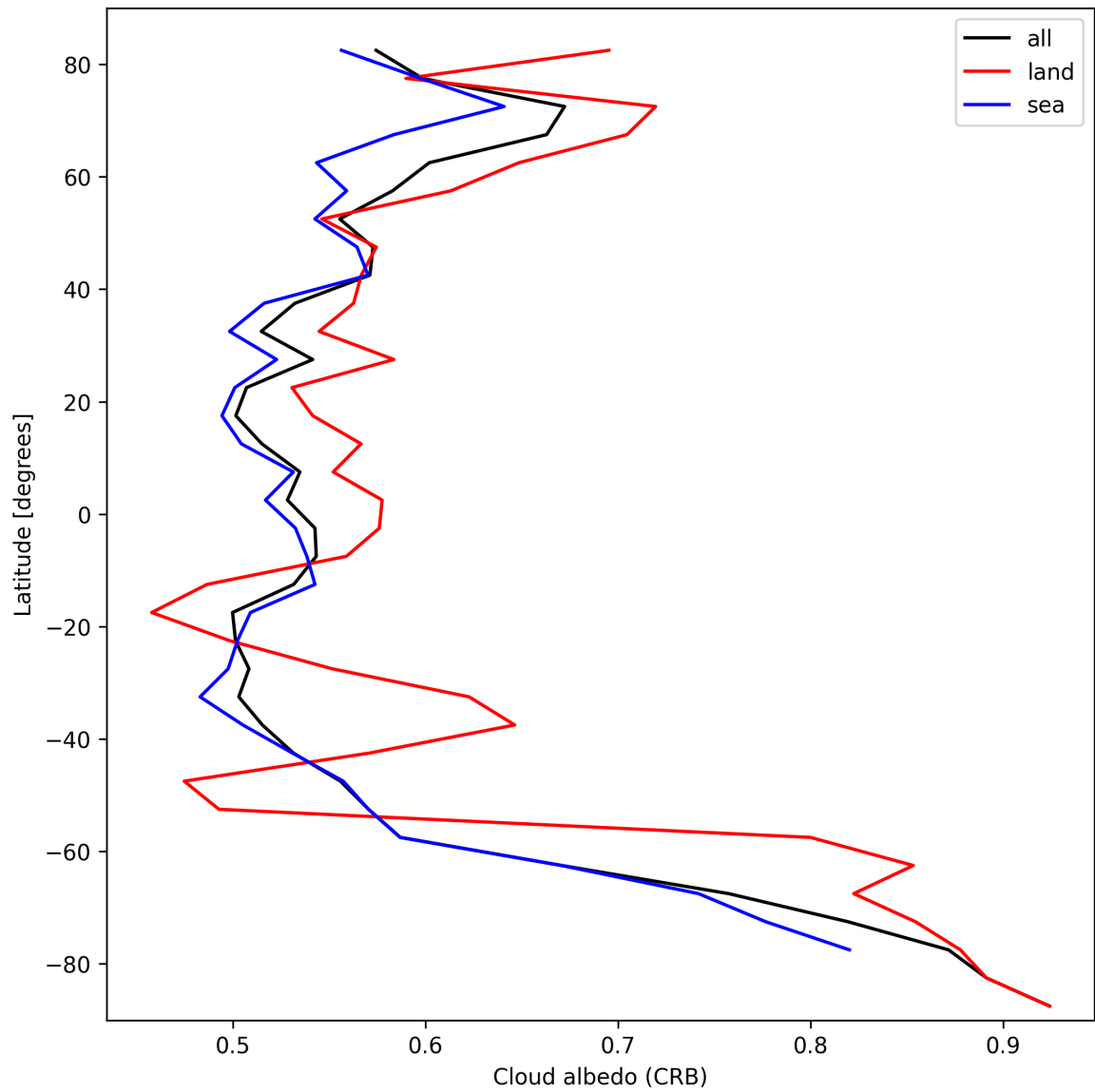
Figure 28: Zonal average of “Cloud albedo (CRB)” for 2024-10-06 to 2024-10-08.
