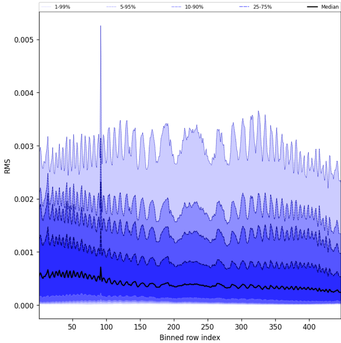
Figure 63: Along track statistics of “RMS” for 2024-10-06 to 2024-10-08
