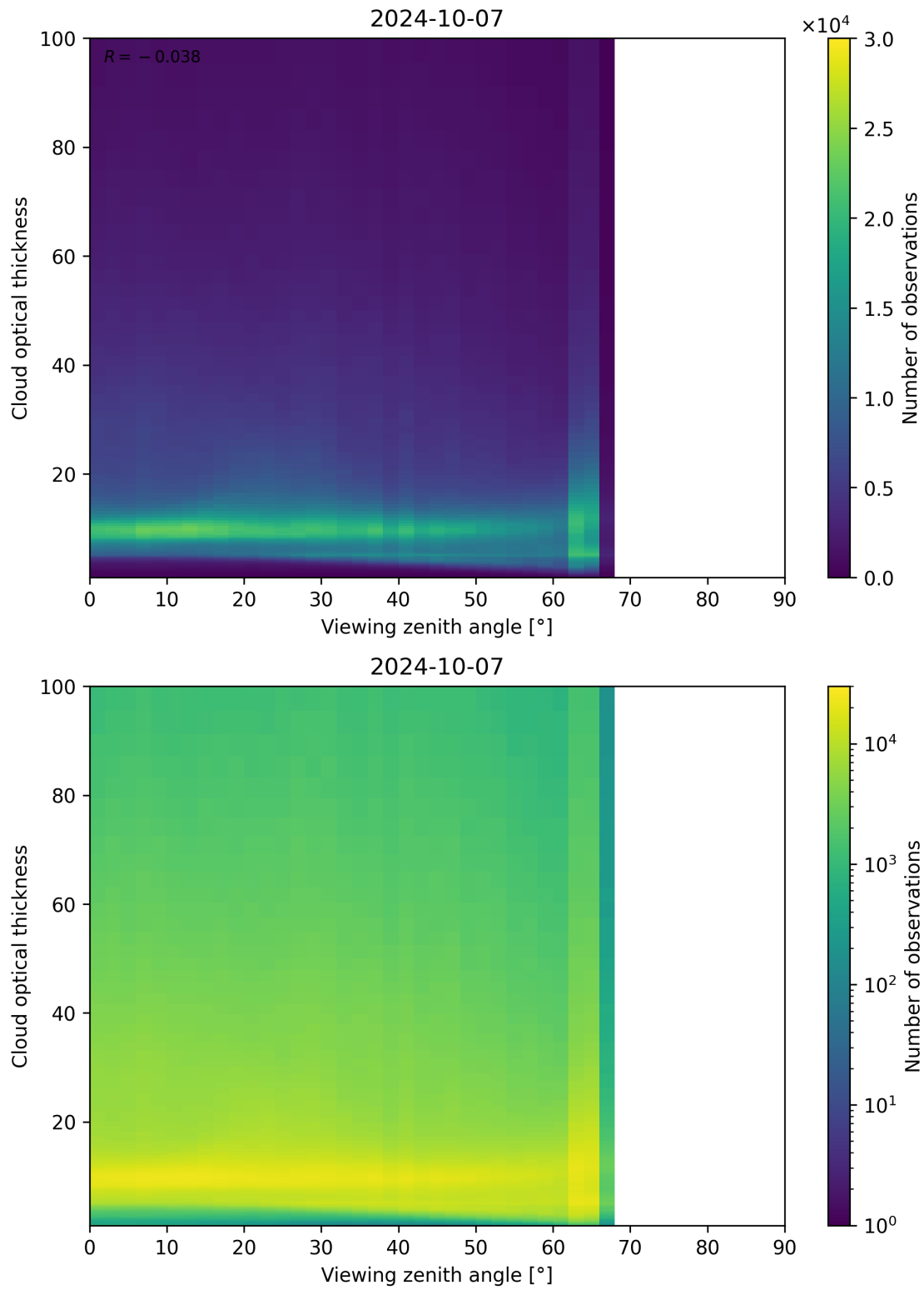
Figure 111: Scatter density plot of “Viewing zenith angle” against “Cloud optical thickness” for 2024-10-06 to 2024-10-08.
