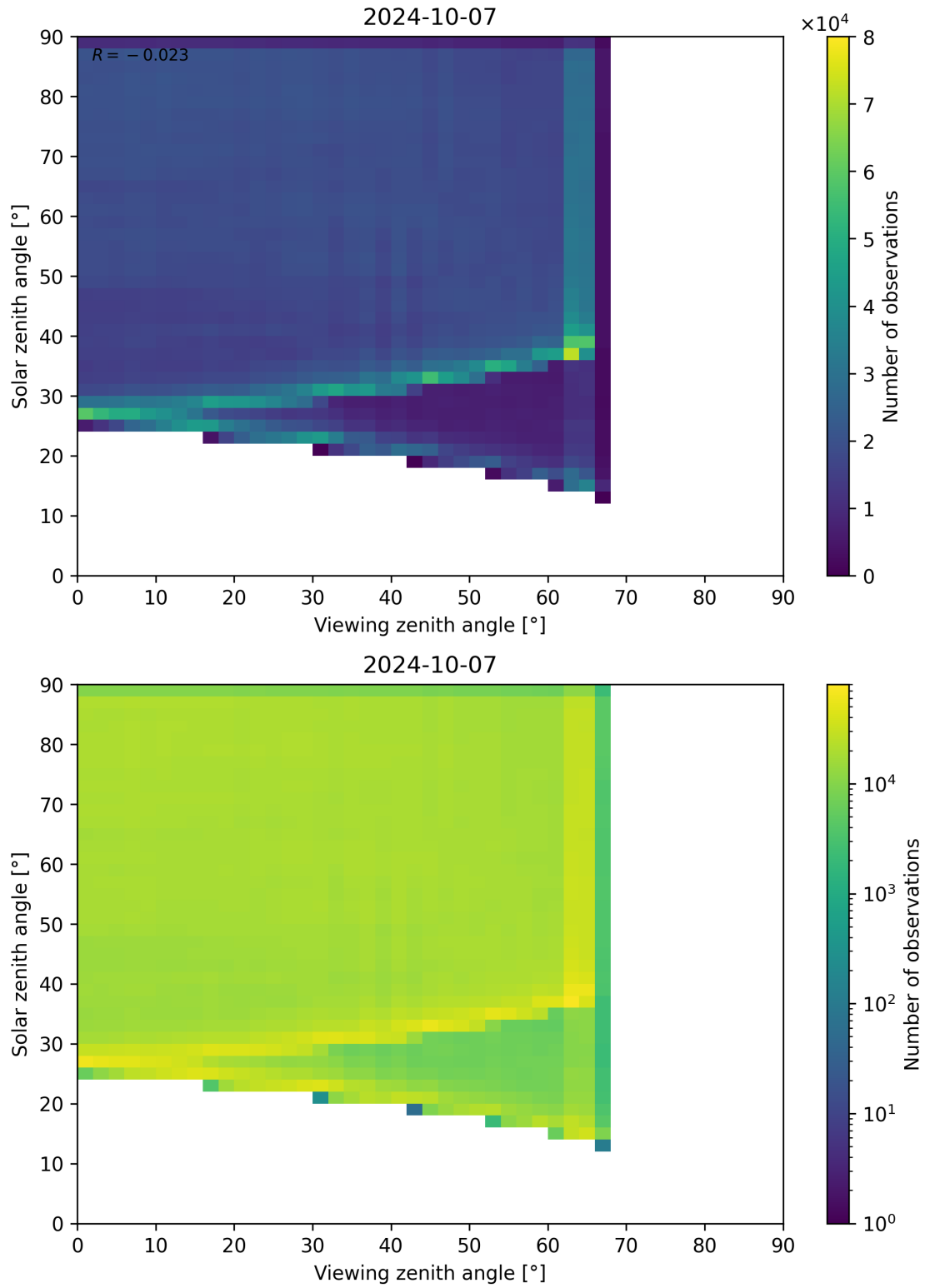
Figure 114: Scatter density plot of “Viewing zenith angle” against “Solar zenith angle” for 2024-10-06 to 2024-10-08.
