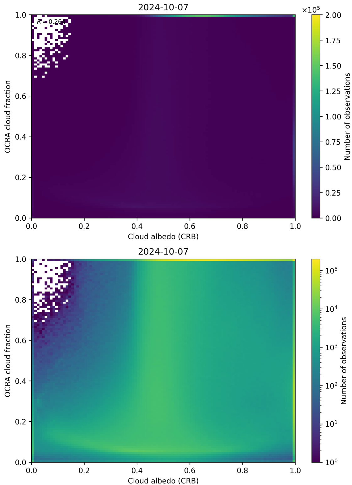
Figure 70: Scatter density plot of “Cloud albedo (CRB)” against “OCRA cloud fraction” for 2024-10-06 to 2024-10-08.
