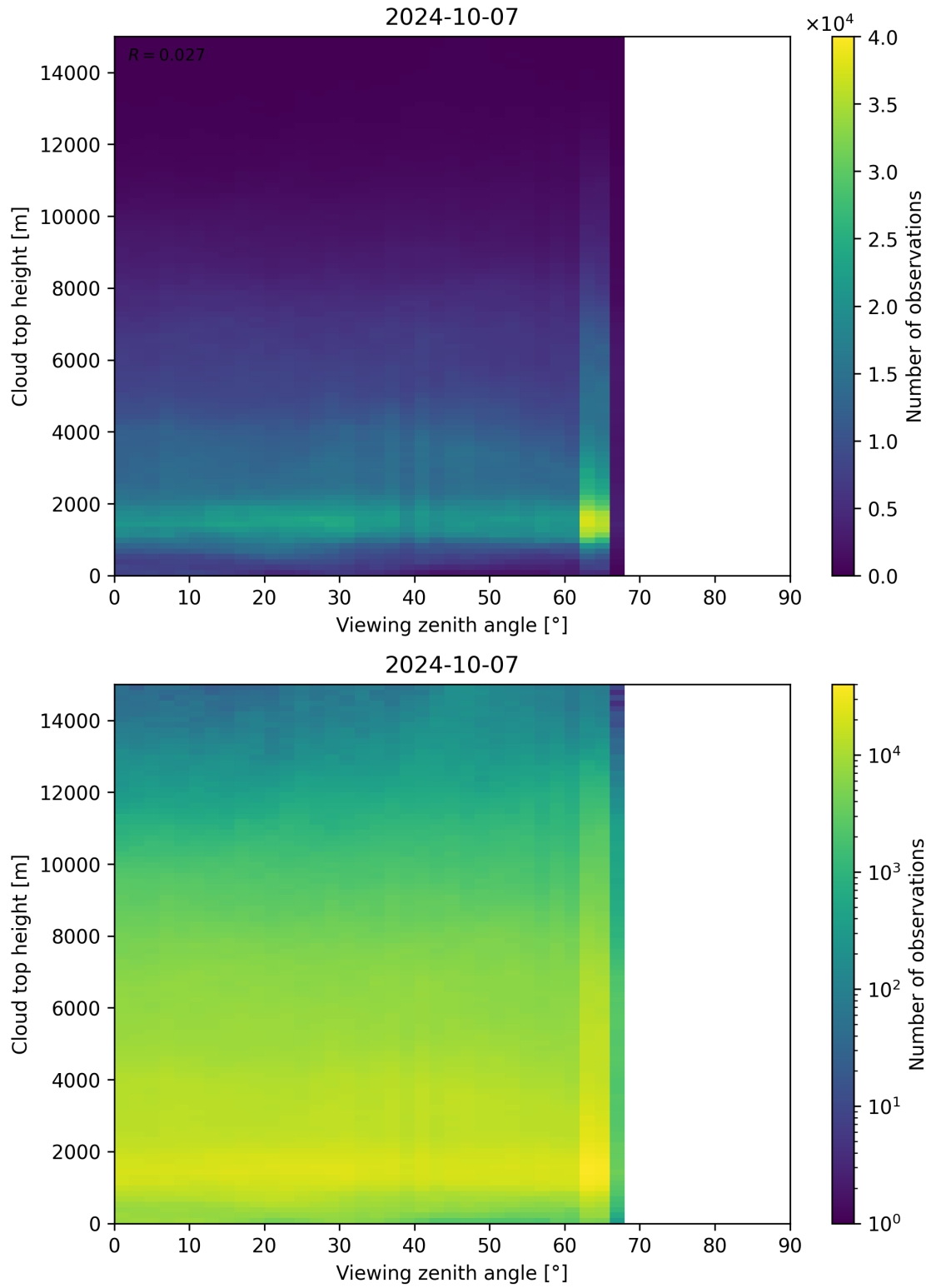
Figure 112: Scatter density plot of “Viewing zenith angle” against “Cloud top height” for 2024-10-06 to 2024-10-08.
