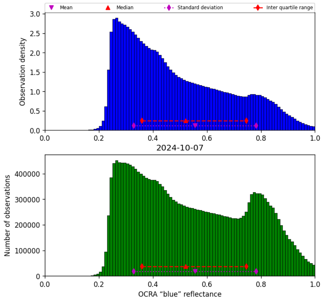
Figure 51: Histogram of “OCRA “blue” reflectance” for 2024-10-06 to 2024-10-08
