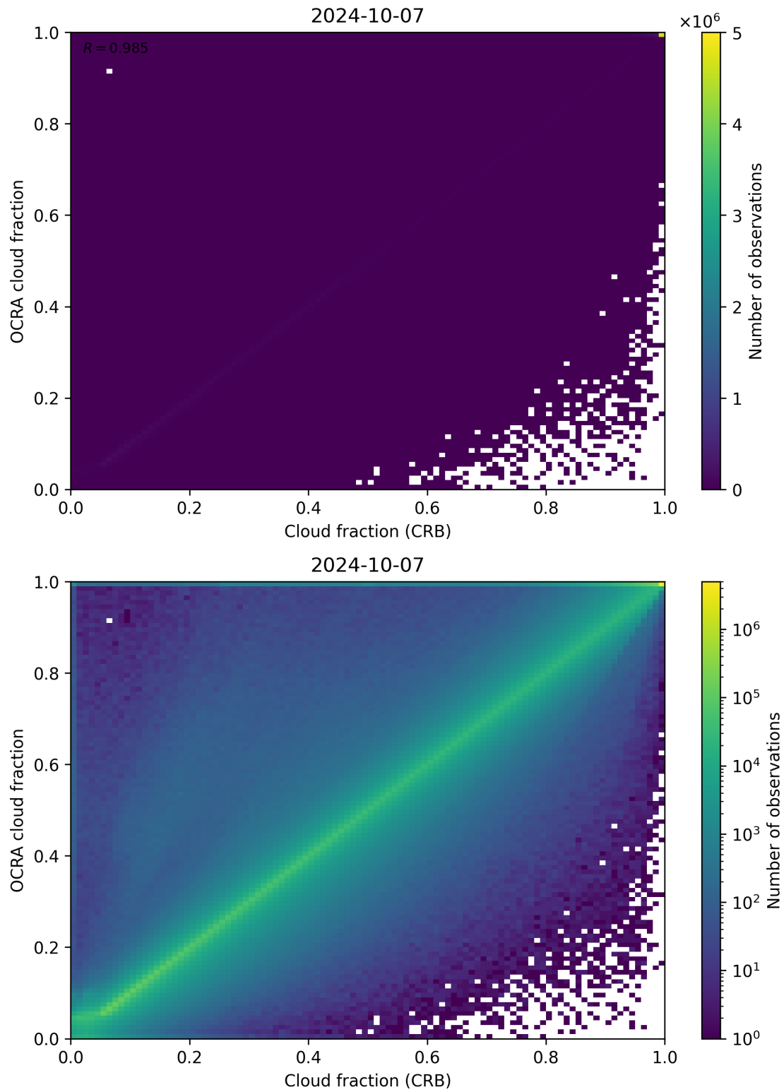
Figure 78: Scatter density plot of “Cloud fraction (CRB)” against “OCRA cloud fraction” for 2024-10-06 to 2024-10-08.
