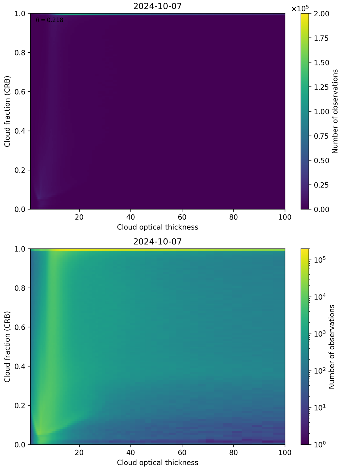
Figure 84: Scatter density plot of “Cloud optical thickness” against “Cloud fraction (CRB)” for 2024-10-06 to 2024-10-08.
