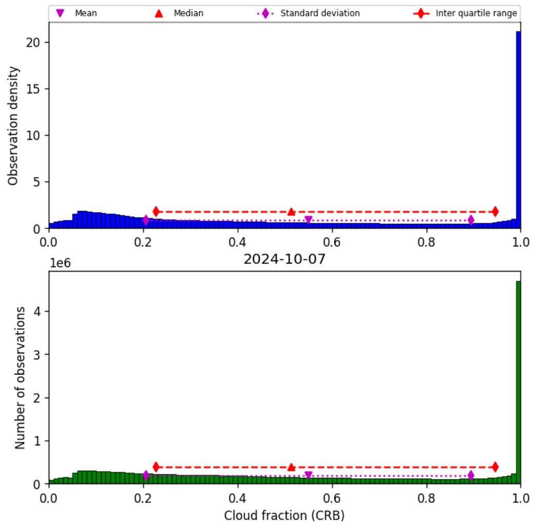
Figure 42: Histogram of “Cloud fraction (CRB)” for 2024-10-06 to 2024-10-08
