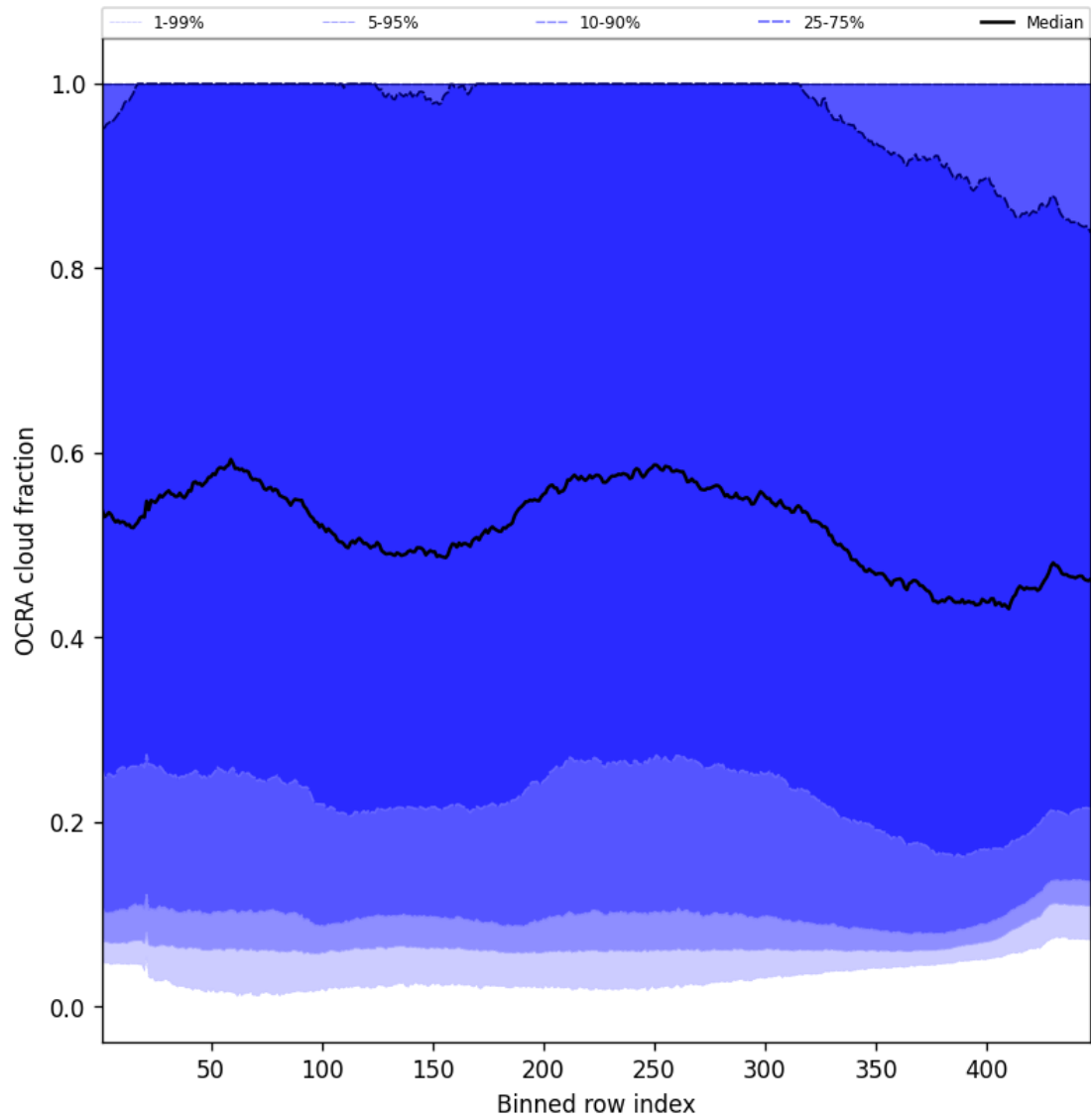
Figure 66: Along track statistics of “OCRA cloud fraction” for 2024-10-06 to 2024-10-08
