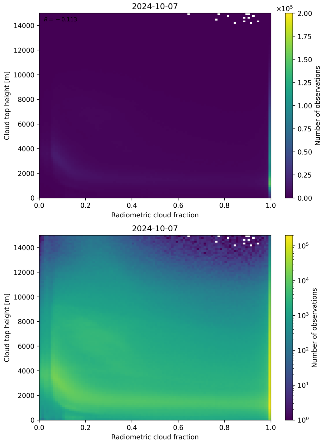
Figure 76: Scatter density plot of “Radiometric cloud fraction” against “Cloud top height” for 2024-10-06 to 2024-10-08.
