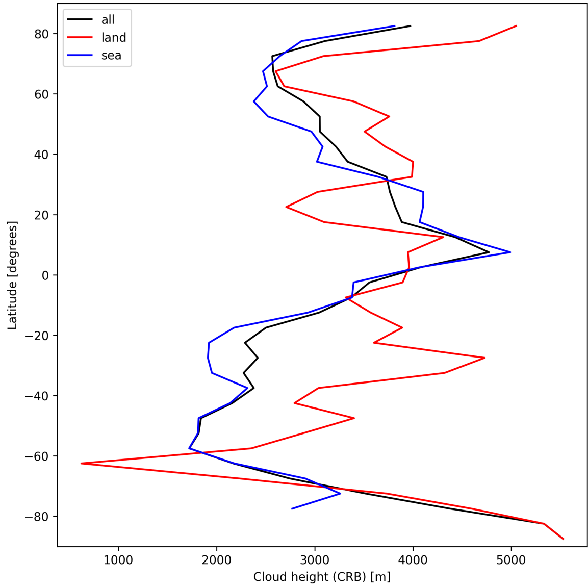
Figure 27: Zonal average of “Cloud height (CRB)” for 2024-10-06 to 2024-10-08.
