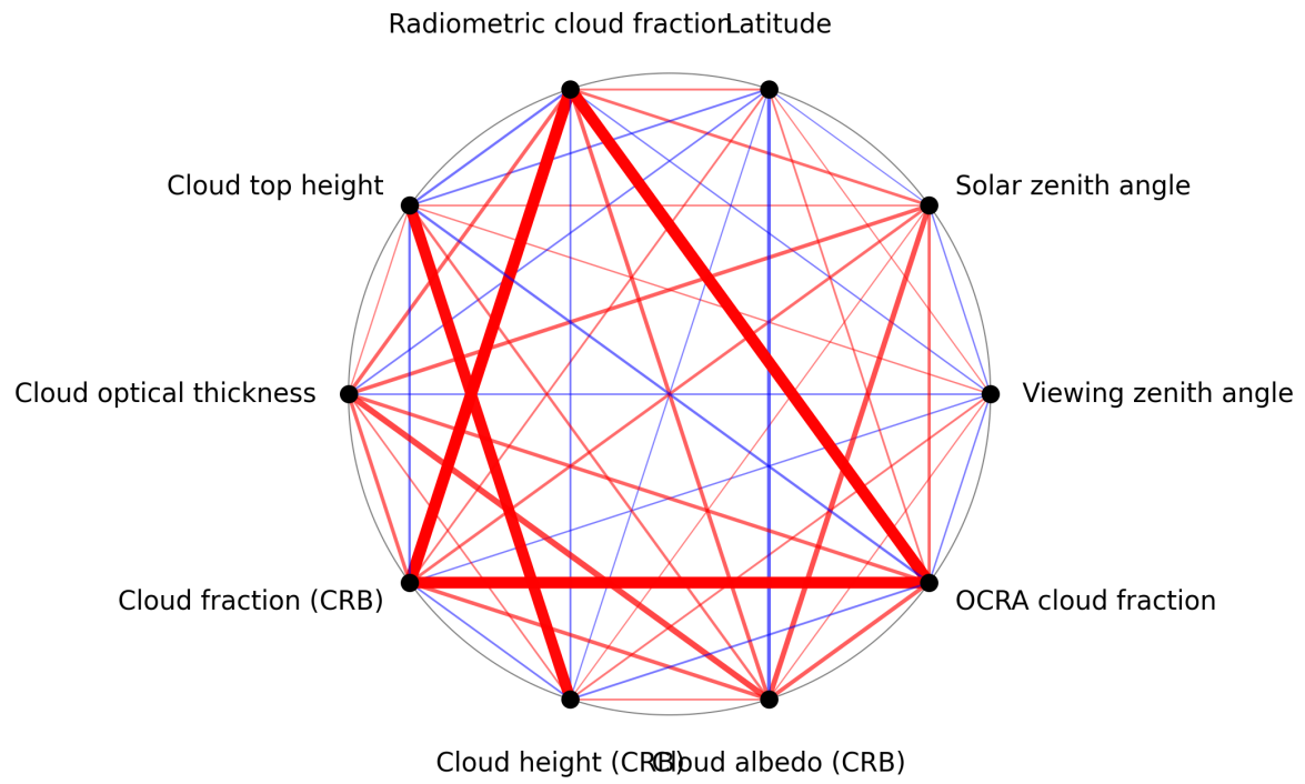
Figure 1: Map of correlation graph for 2024-10-06 to 2024-10-08.
