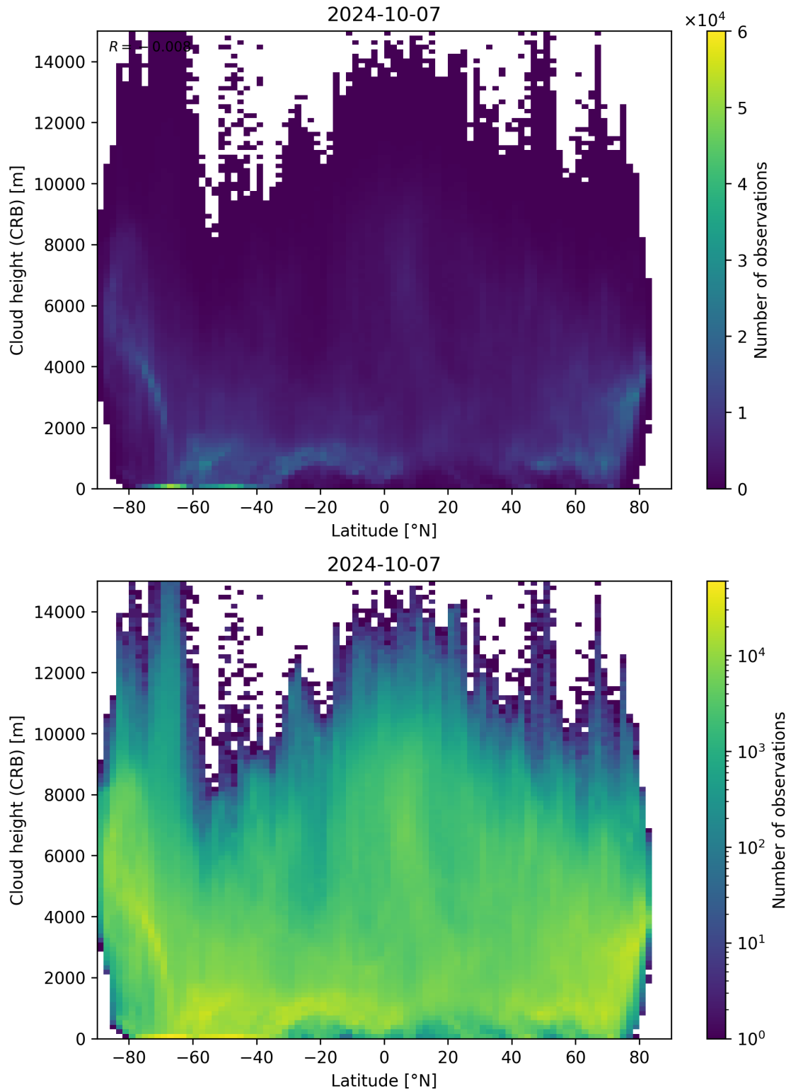
Figure 95: Scatter density plot of “Latitude” against “Cloud height (CRB)” for 2024-10-06 to 2024-10-08.
