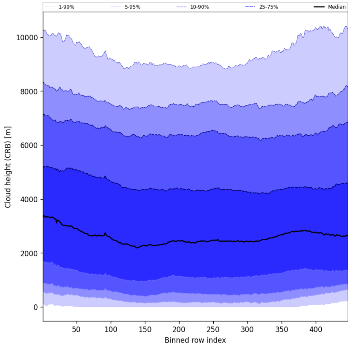
Figure 59: Along track statistics of “Cloud height (CRB)” for 2024-10-06 to 2024-10-08
