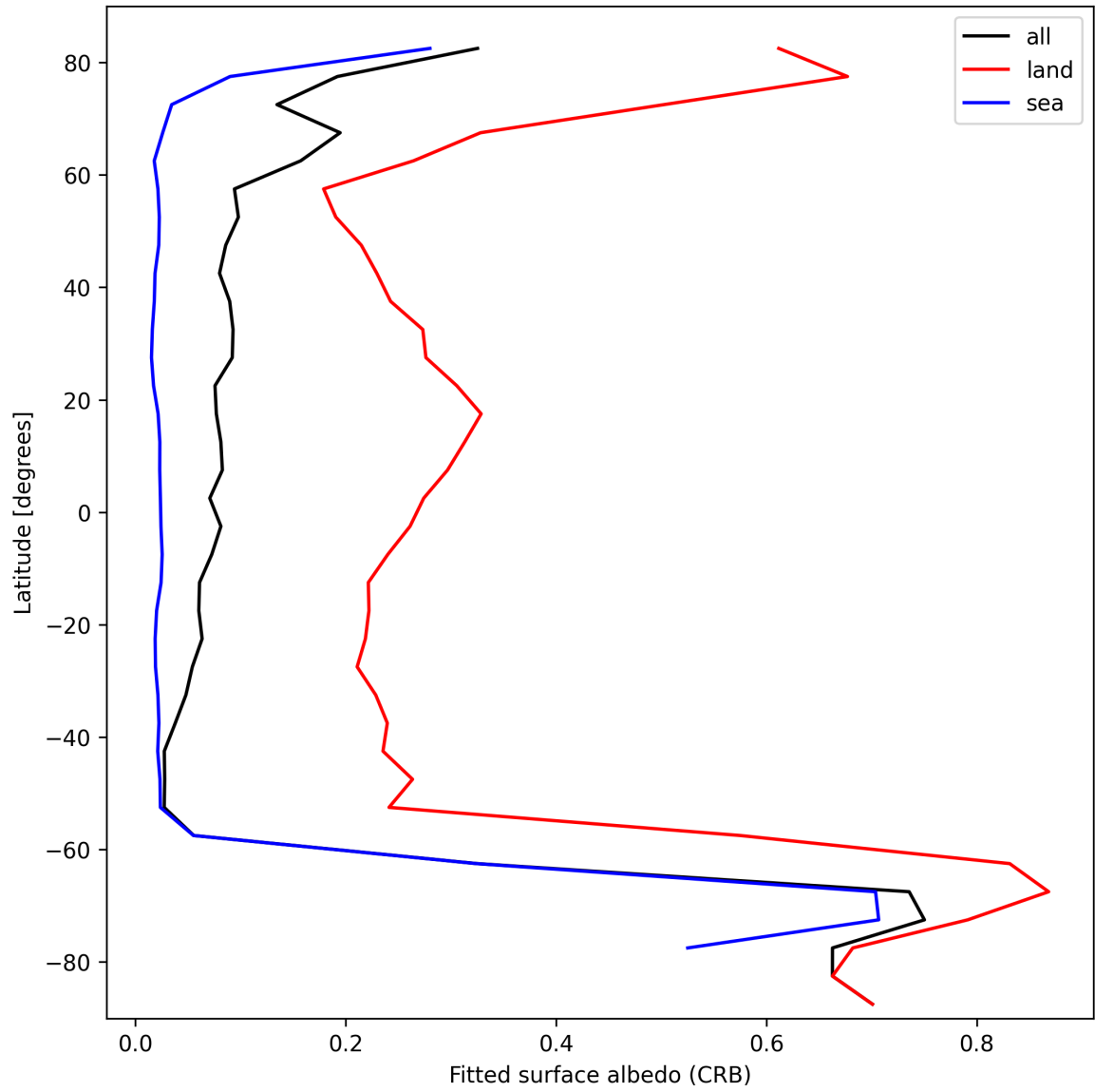
Figure 30: Zonal average of “Fitted surface albedo (CRB)” for 2024-10-06 to 2024-10-08.
