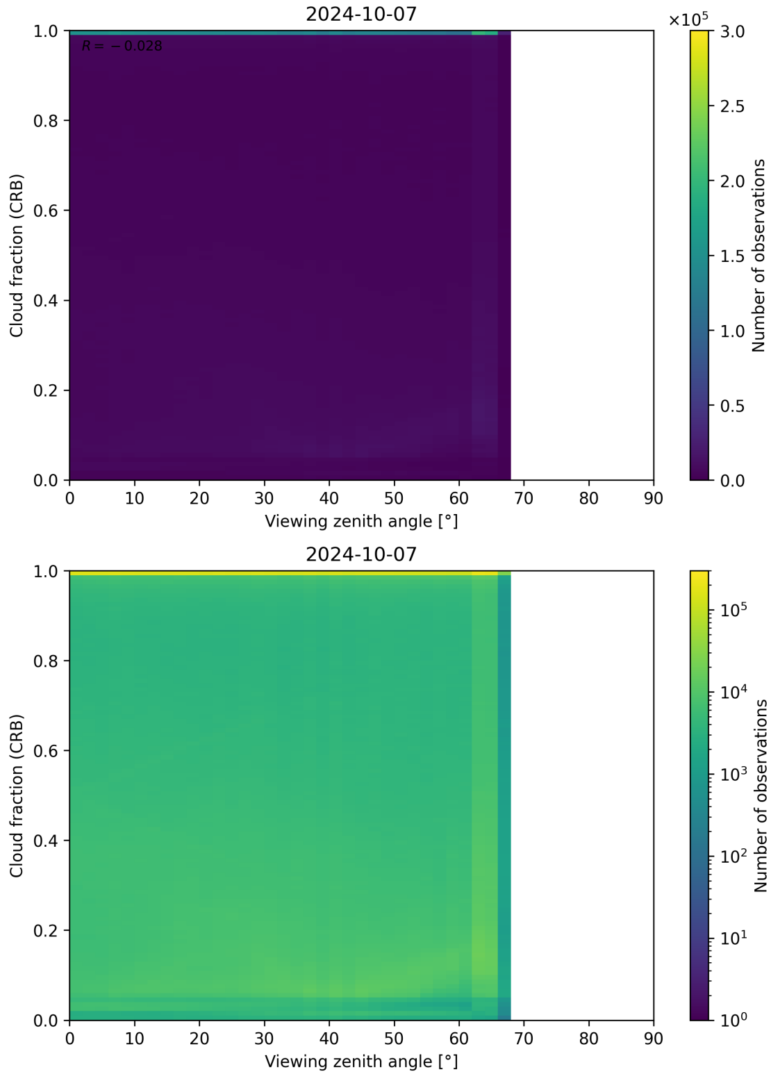
Figure 109: Scatter density plot of “Viewing zenith angle” against “Cloud fraction (CRB)” for 2024-10-06 to 2024-10-08.
