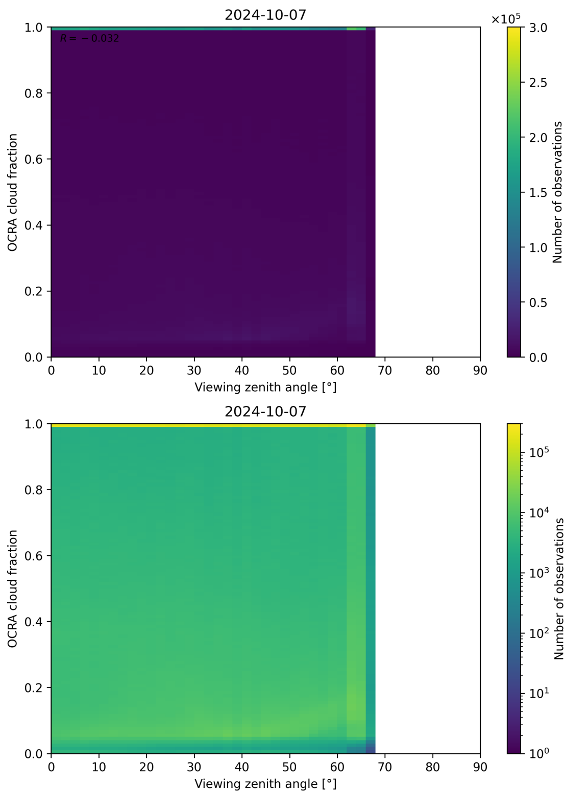
Figure 108: Scatter density plot of “Viewing zenith angle” against “OCRA cloud fraction” for 2024-10-06 to 2024-10-08.
