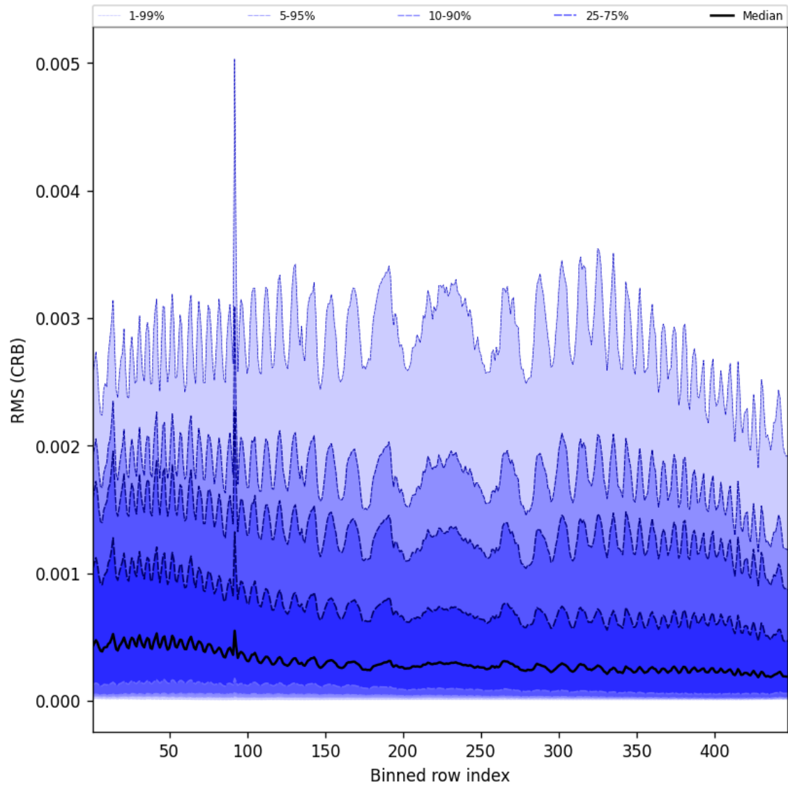
Figure 64: Along track statistics of “RMS (CRB)” for 2024-10-06 to 2024-10-08
