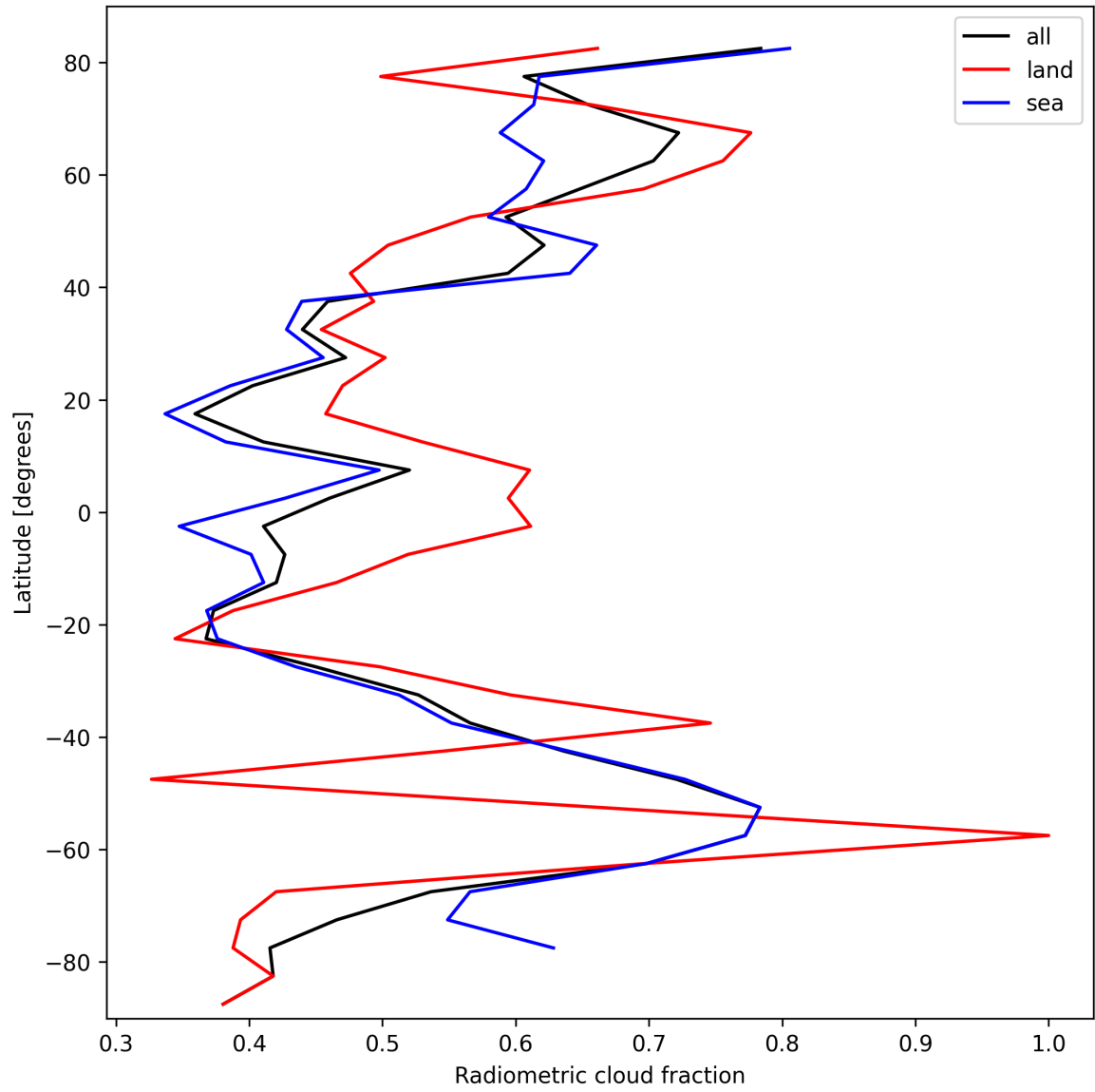
Figure 23: Zonal average of “Radiometric cloud fraction” for 2024-10-06 to 2024-10-08.
