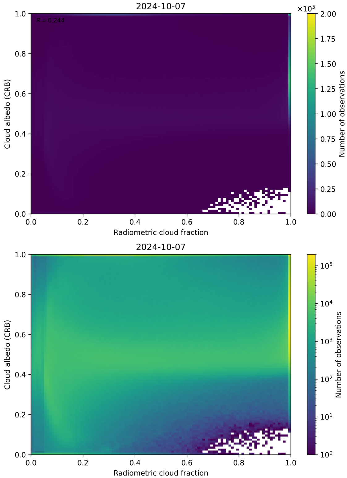
Figure 71: Scatter density plot of “Radiometric cloud fraction” against “Cloud albedo (CRB)” for 2024-10-06 to 2024-10-08.
