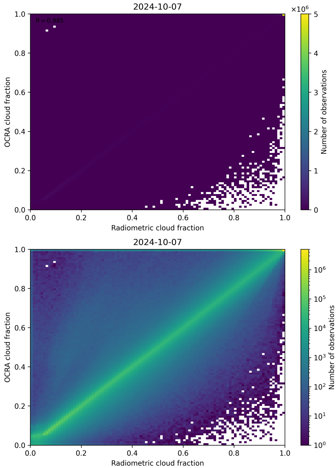
Figure 72: Scatter density plot of “Radiometric cloud fraction” against “OCRA cloud fraction” for 2024-10-06 to 2024-10-08.
