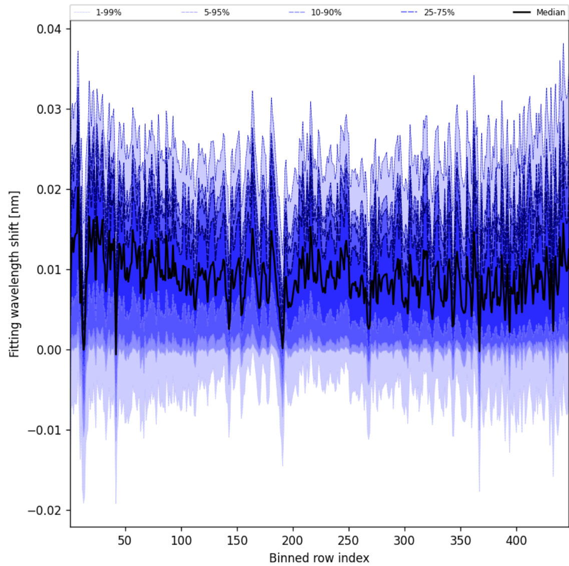
Figure 65: Along track statistics of “Fitting wavelength shift” for 2024-10-06 to 2024-10-08
