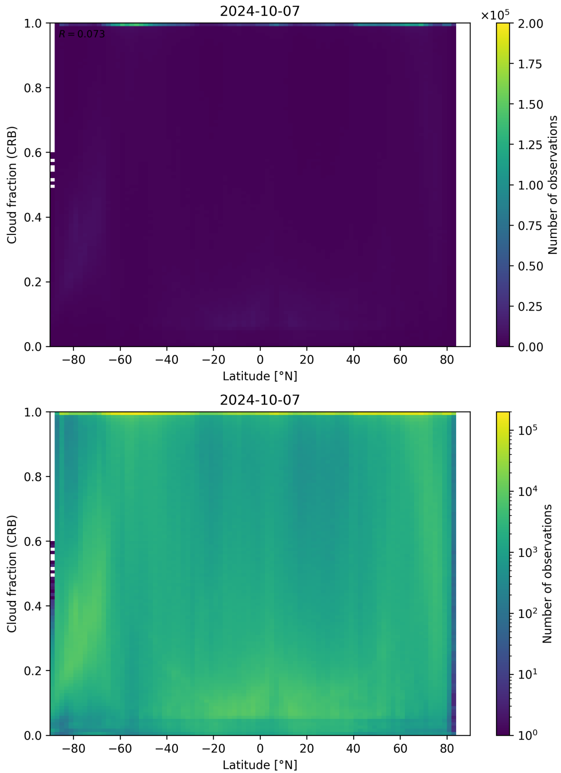
Figure 94: Scatter density plot of “Latitude” against “Cloud fraction (CRB)” for 2024-10-06 to 2024-10-08.
