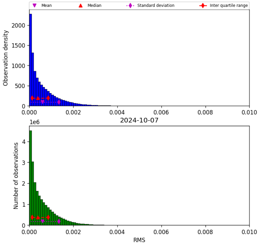
Figure 47: Histogram of “RMS” for 2024-10-06 to 2024-10-08
