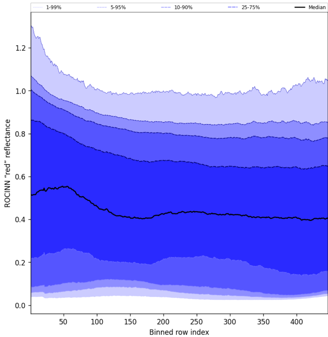
Figure 69: Along track statistics of “ROCINN “red” reflectance” for 2024-10-06 to 2024-10-08
