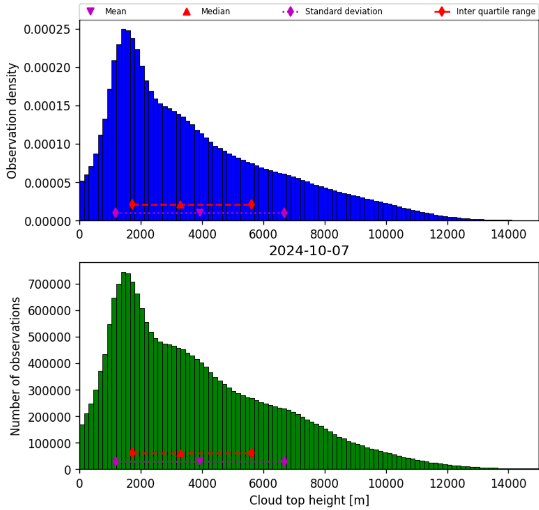
Figure 40: Histogram of “Cloud top height” for 2024-10-06 to 2024-10-08
