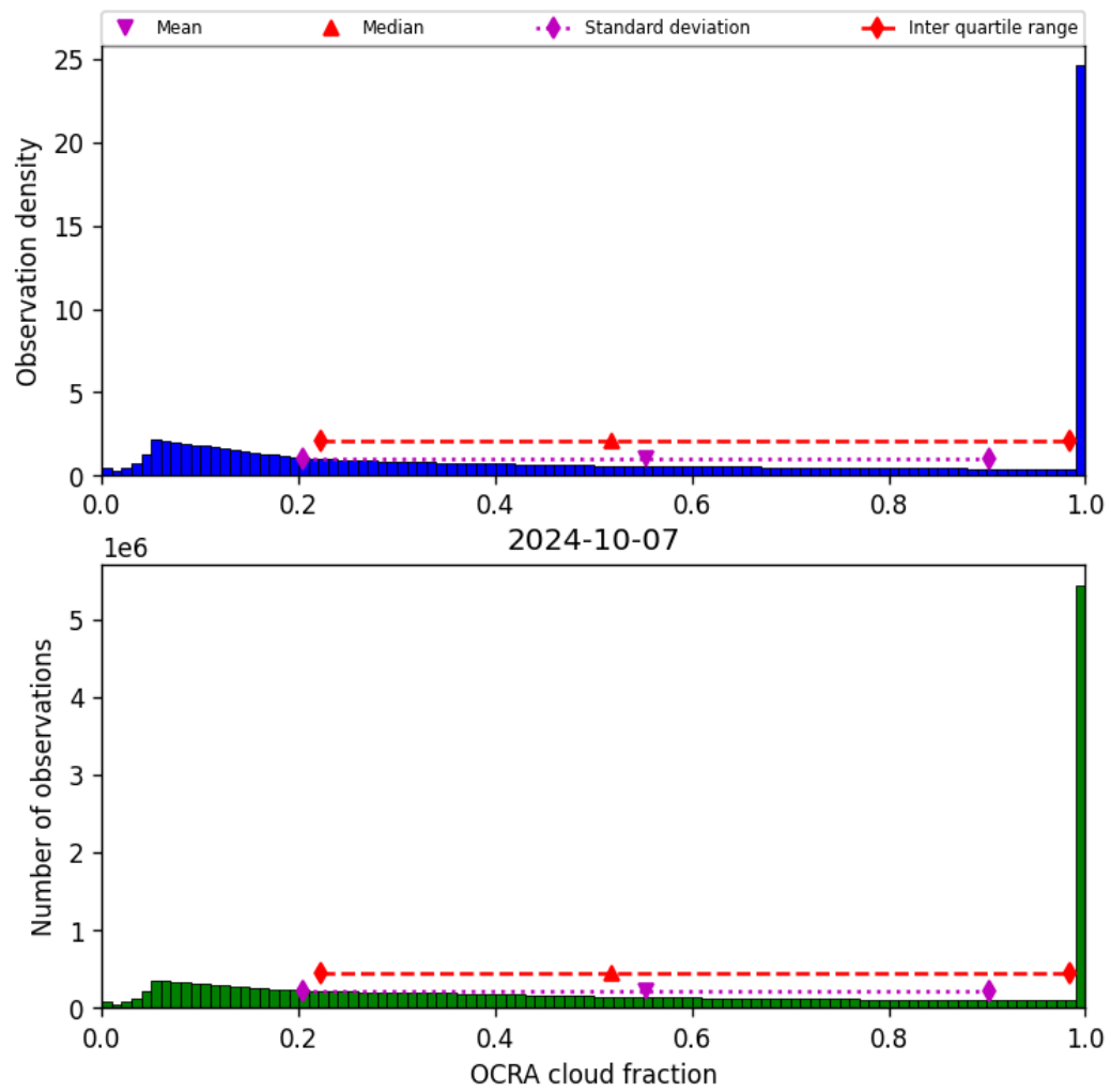
Figure 50: Histogram of “OCRA cloud fraction” for 2024-10-06 to 2024-10-08
