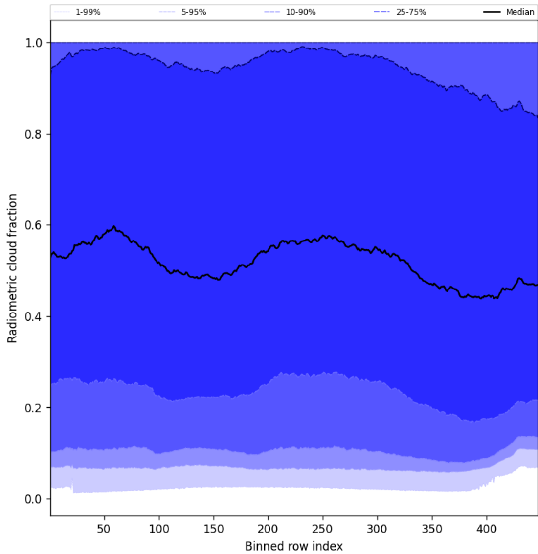
Figure 55: Along track statistics of “Radiometric cloud fraction” for 2024-10-06 to 2024-10-08
