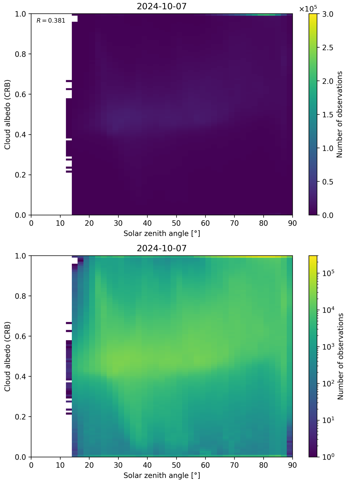
Figure 98: Scatter density plot of “Solar zenith angle” against “Cloud albedo (CRB)” for 2024-10-06 to 2024-10-08.
