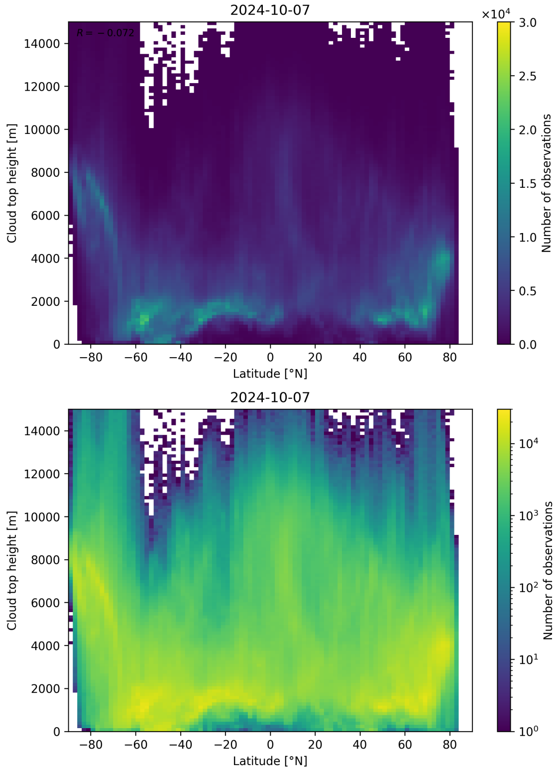
Figure 97: Scatter density plot of “Latitude” against “Cloud top height” for 2024-10-06 to 2024-10-08.
