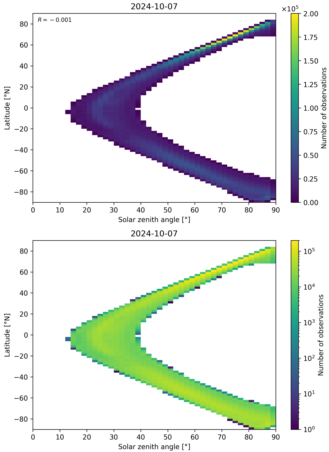
Figure 105: Scatter density plot of “Solar zenith angle” against “Latitude” for 2024-10-06 to 2024-10-08.
