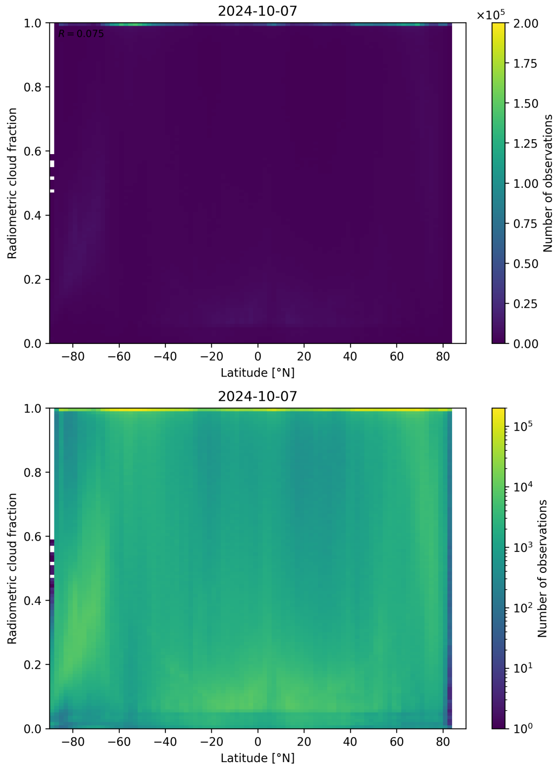
Figure 92: Scatter density plot of “Latitude” against “Radiometric cloud fraction” for 2024-10-06 to 2024-10-08.
