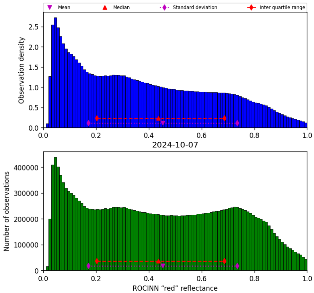
Figure 53: Histogram of “ROCINN “red” reflectance” for 2024-10-06 to 2024-10-08
