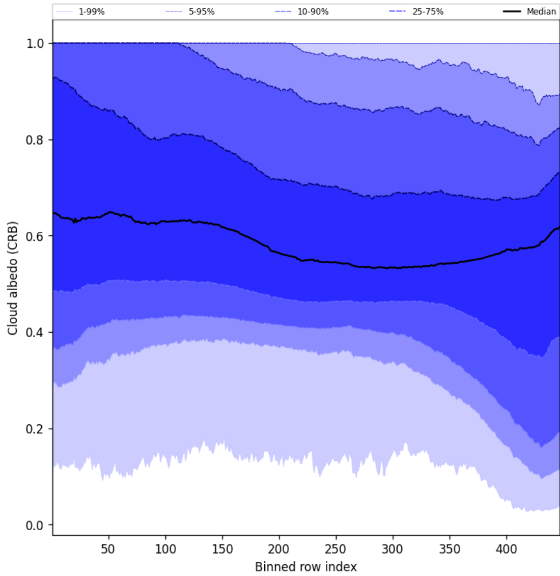
Figure 60: Along track statistics of “Cloud albedo (CRB)” for 2024-10-06 to 2024-10-08
