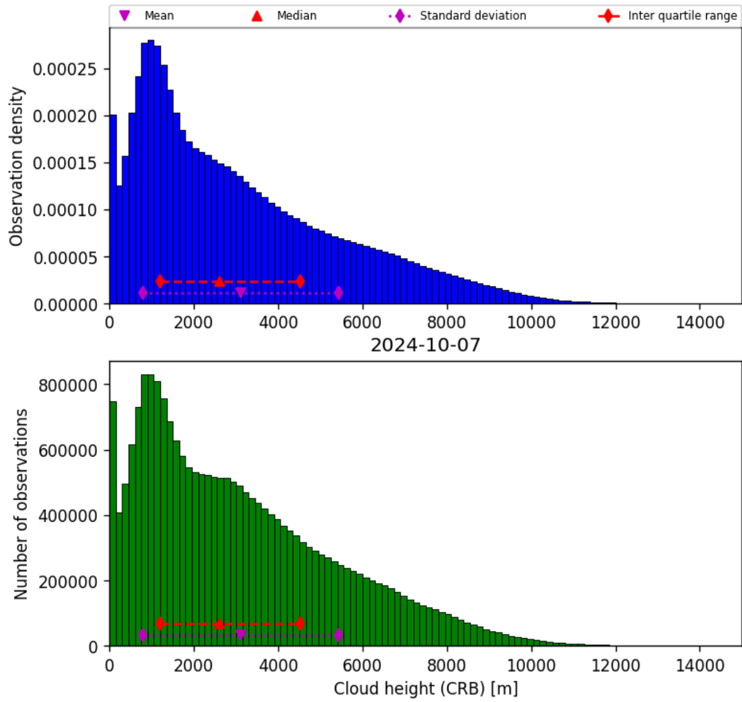
Figure 43: Histogram of “Cloud height (CRB)” for 2024-10-06 to 2024-10-08
