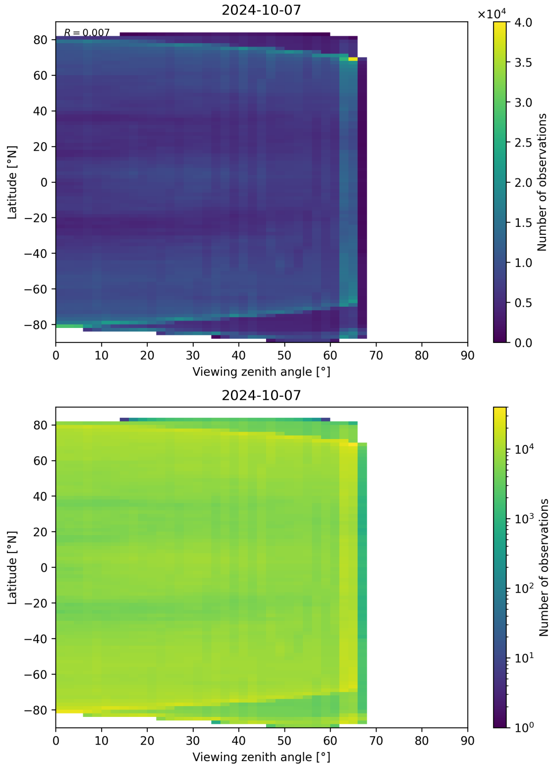
Figure 113: Scatter density plot of “Viewing zenith angle” against “Latitude” for 2024-10-06 to 2024-10-08.
