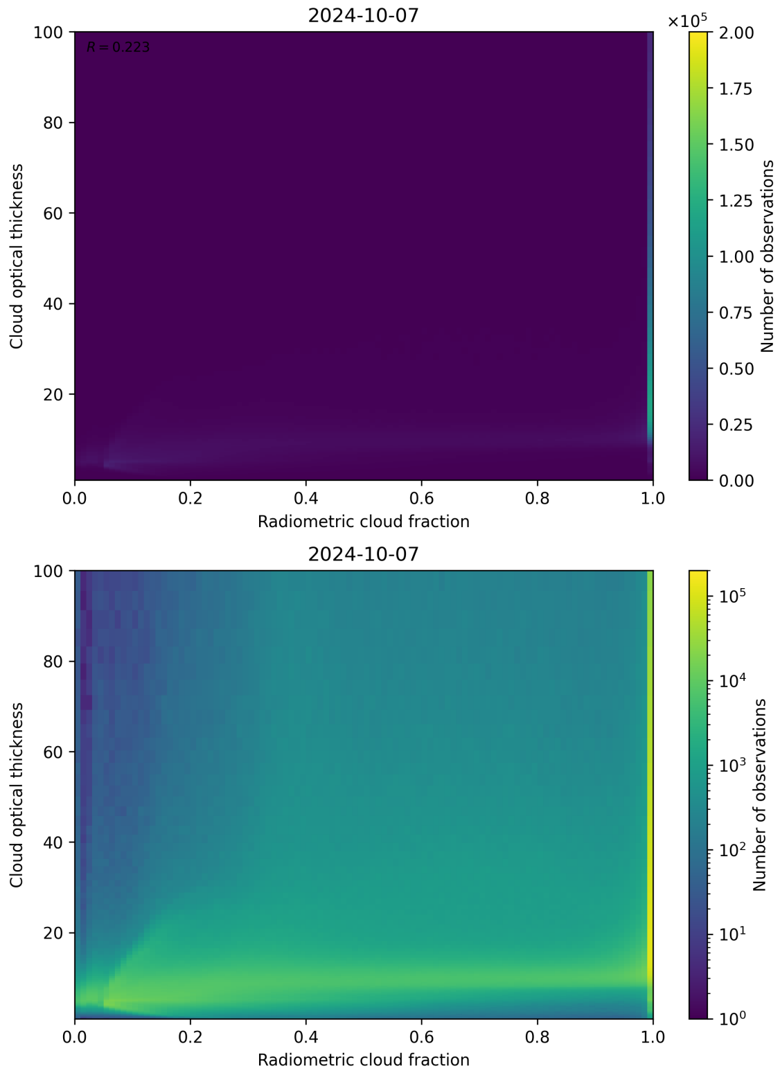
Figure 75: Scatter density plot of “Radiometric cloud fraction” against “Cloud optical thickness” for 2024-10-06 to 2024-10-08.
