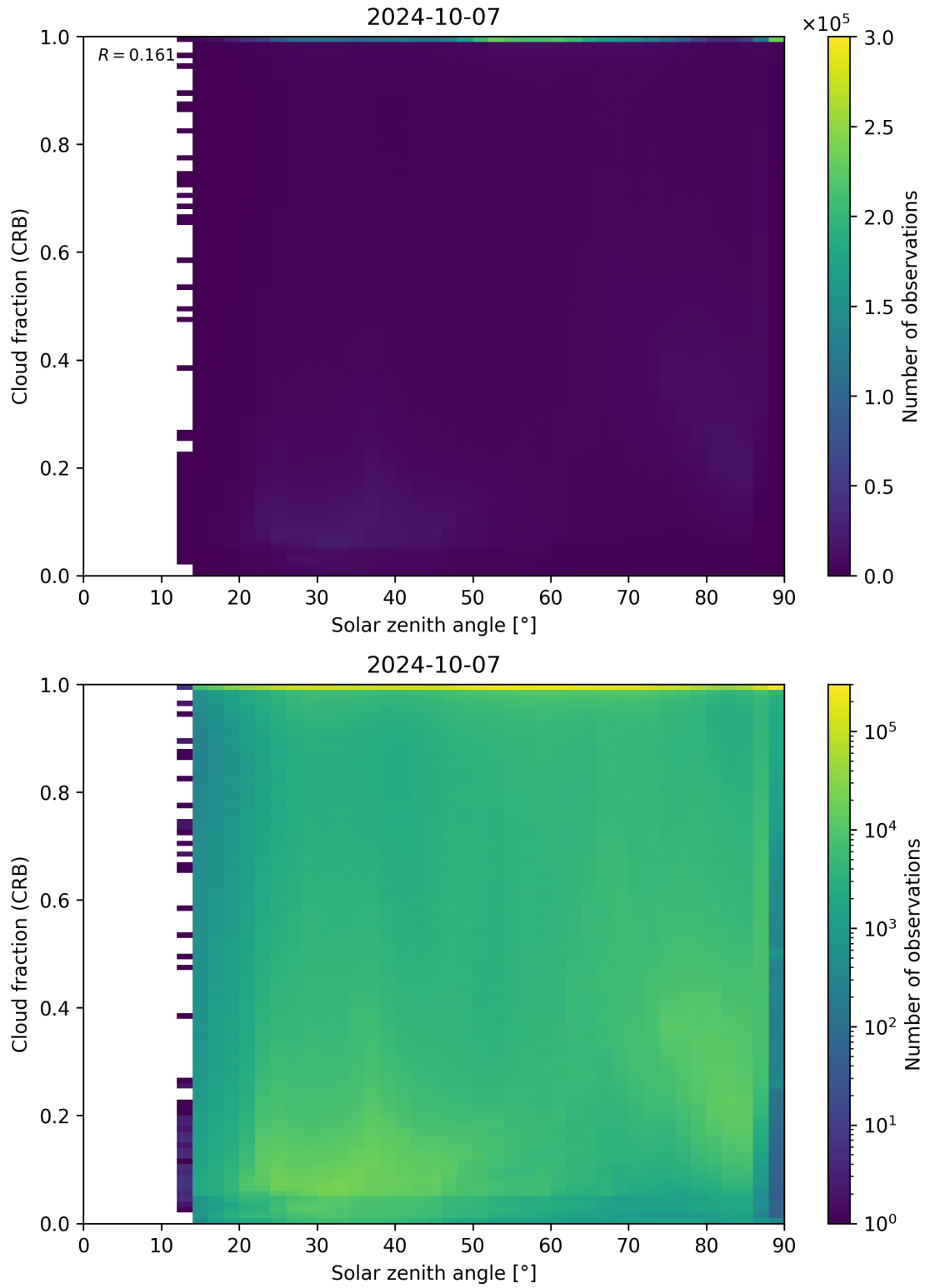
Figure 101: Scatter density plot of “Solar zenith angle” against “Cloud fraction (CRB)” for 2024-10-06 to 2024-10-08.
