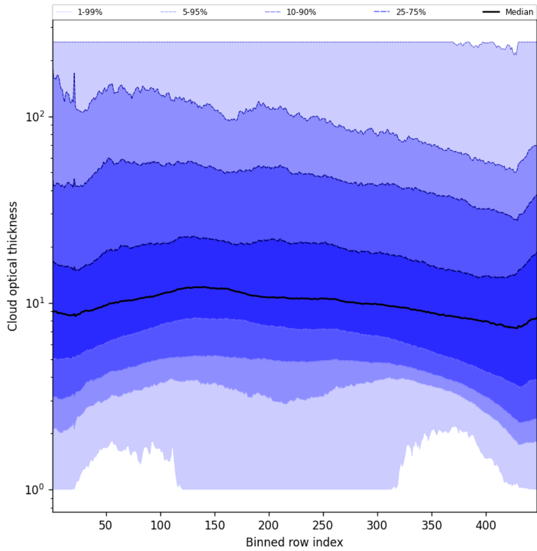
Figure 57: Along track statistics of “Cloud optical thickness” for 2024-10-06 to 2024-10-08
