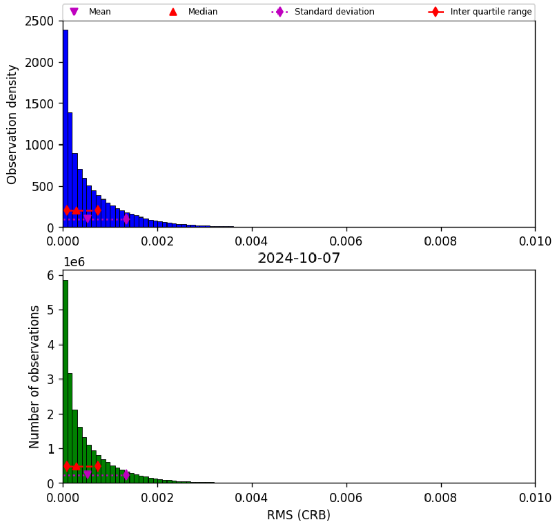
Figure 48: Histogram of “RMS (CRB)” for 2024-10-06 to 2024-10-08
