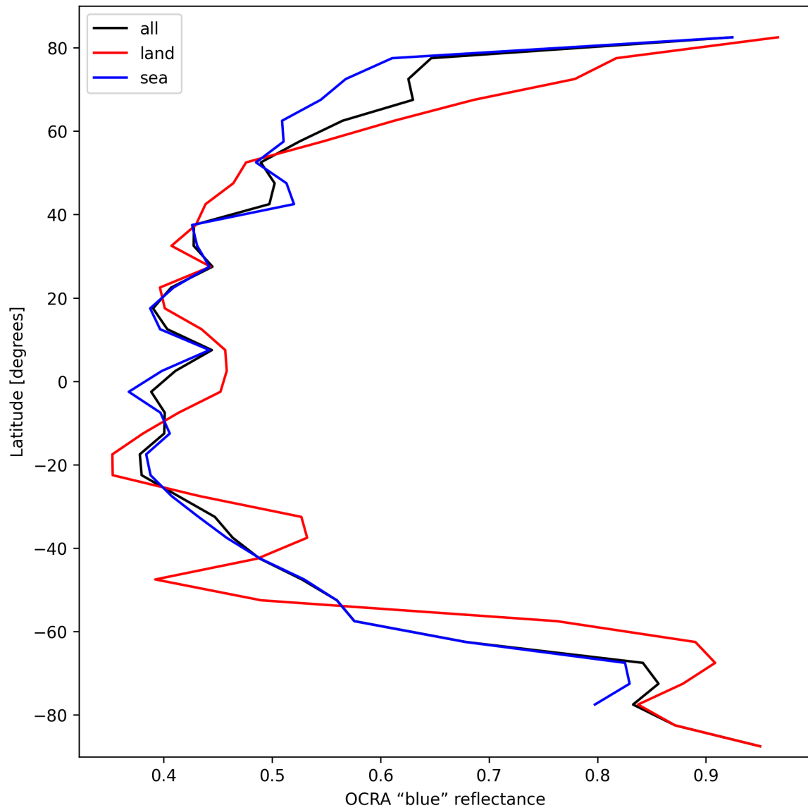
Figure 35: Zonal average of “OCRA “blue” reflectance” for 2024-10-06 to 2024-10-08.
