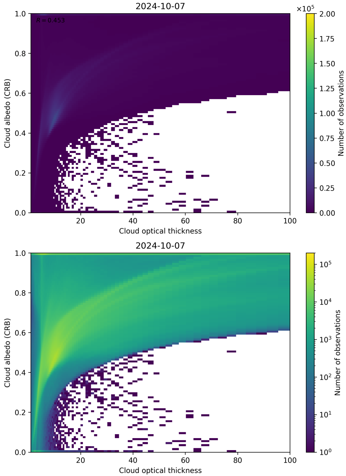
Figure 82: Scatter density plot of “Cloud optical thickness” against “Cloud albedo (CRB)” for 2024-10-06 to 2024-10-08.
