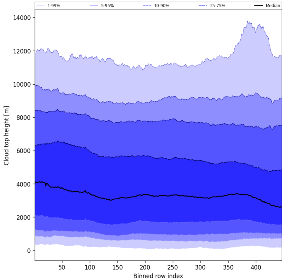
Figure 56: Along track statistics of “Cloud top height” for 2024-10-06 to 2024-10-08
