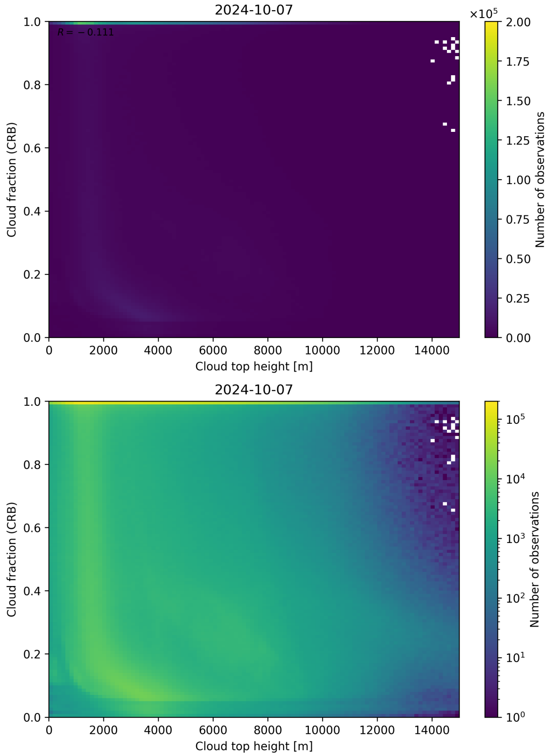
Figure 88: Scatter density plot of “Cloud top height” against “Cloud fraction (CRB)” for 2024-10-06 to 2024-10-08.
