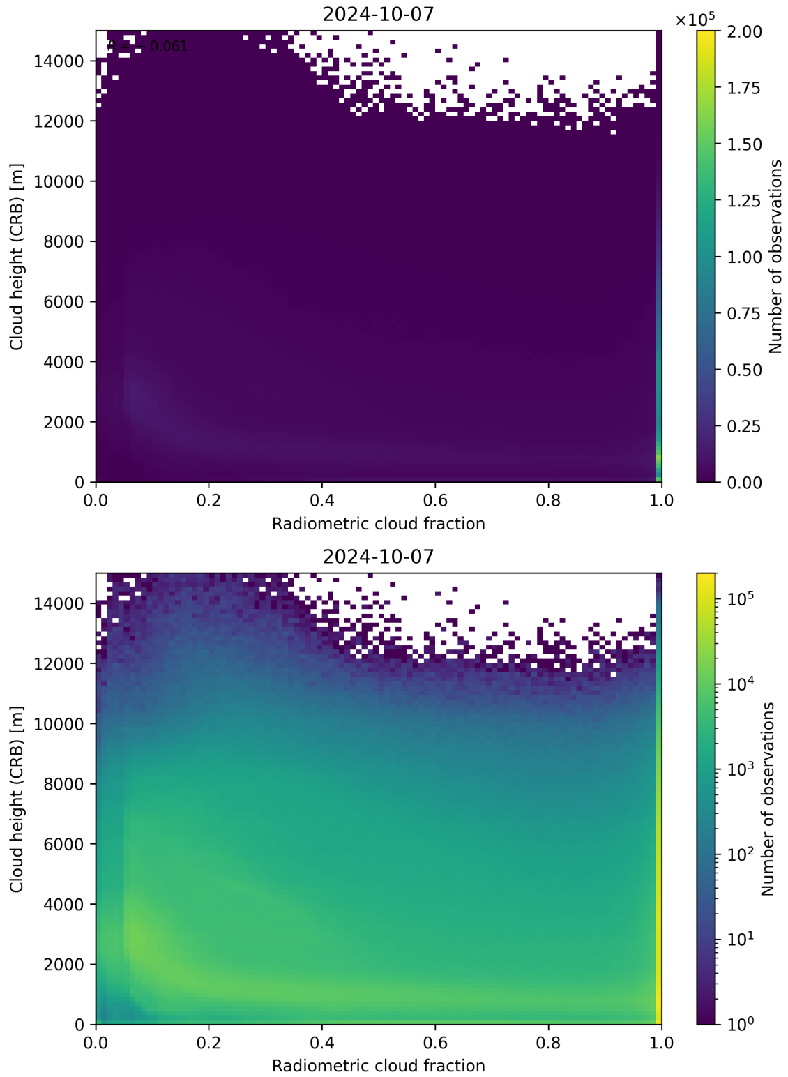
Figure 74: Scatter density plot of “Radiometric cloud fraction” against “Cloud height (CRB)” for 2024-10-06 to 2024-10-08.
