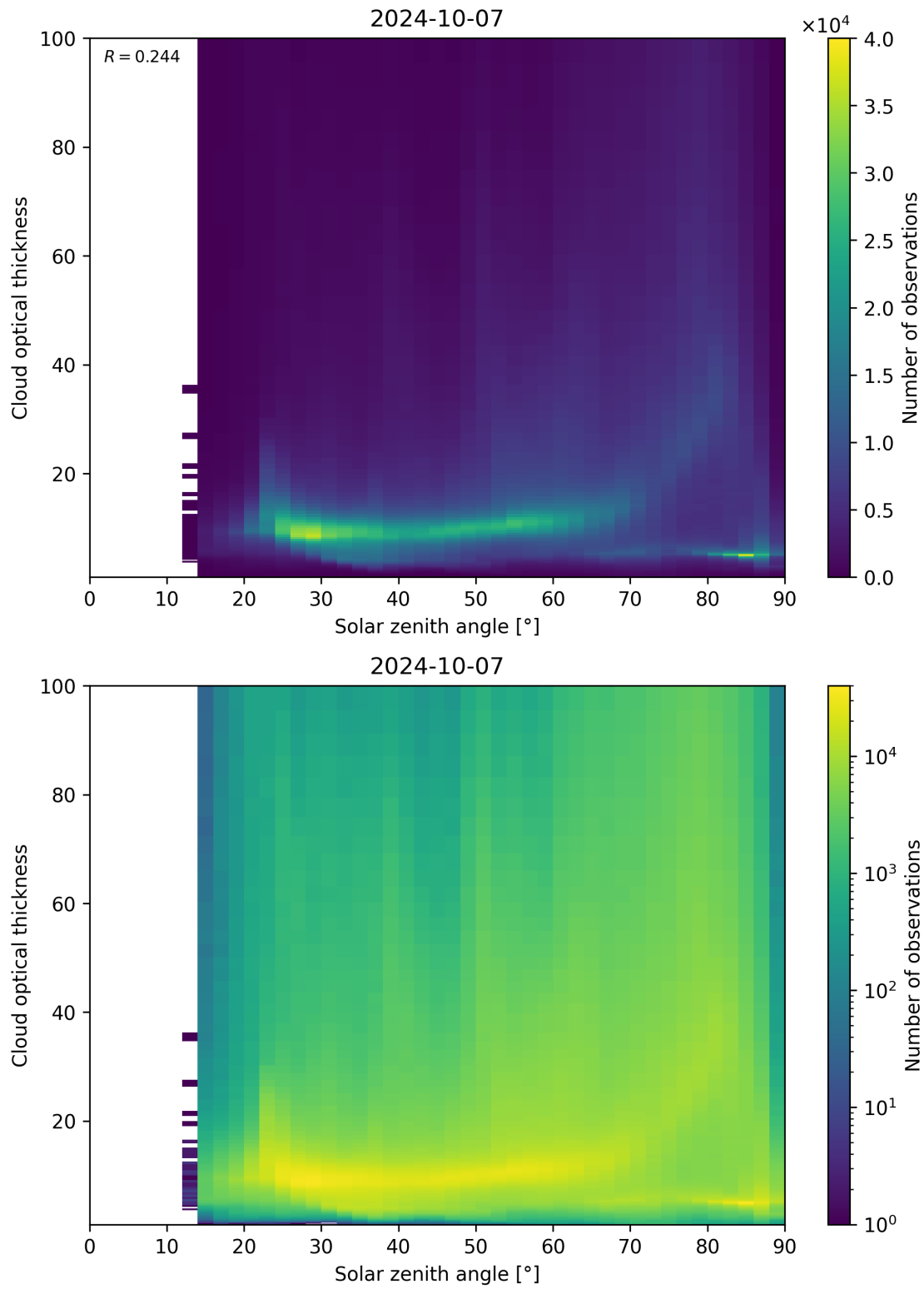
Figure 103: Scatter density plot of “Solar zenith angle” against “Cloud optical thickness” for 2024-10-06 to 2024-10-08.
