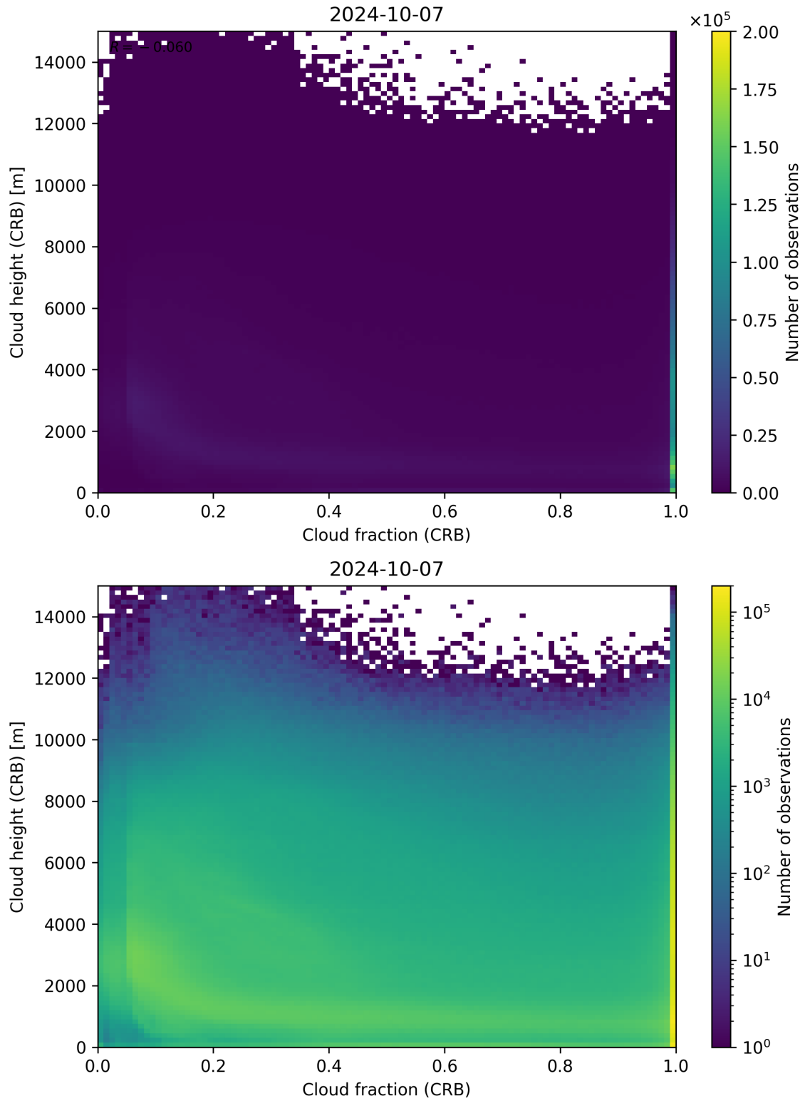
Figure 79: Scatter density plot of “Cloud fraction (CRB)” against “Cloud height (CRB)” for 2024-10-06 to 2024-10-08.
