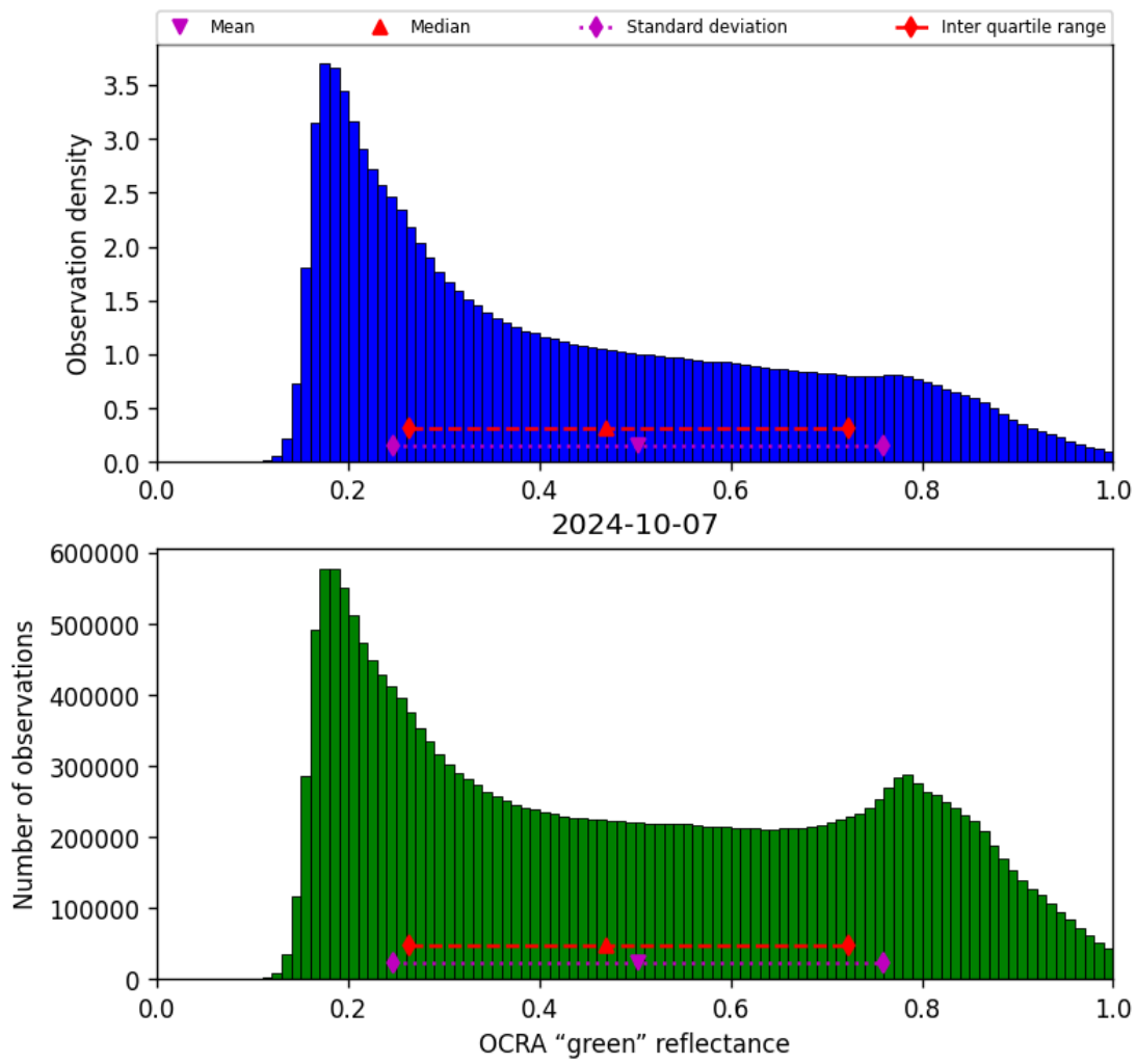
Figure 52: Histogram of “OCRA “green” reflectance” for 2024-10-06 to 2024-10-08
