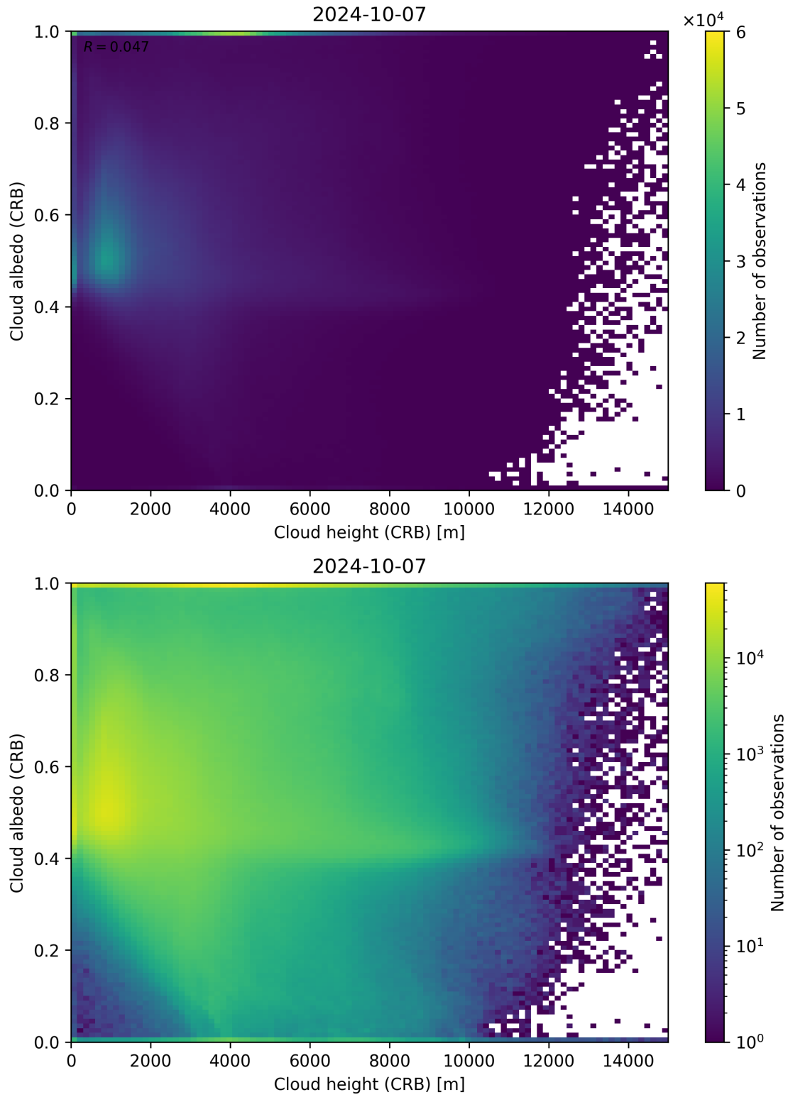
Figure 80: Scatter density plot of “Cloud height (CRB)” against “Cloud albedo (CRB)” for 2024-10-06 to 2024-10-08.
