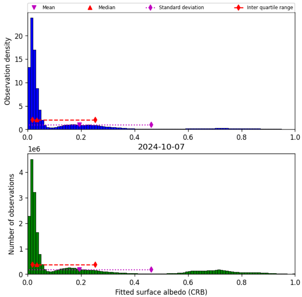
Figure 46: Histogram of “Fitted surface albedo (CRB)” for 2024-10-06 to 2024-10-08
