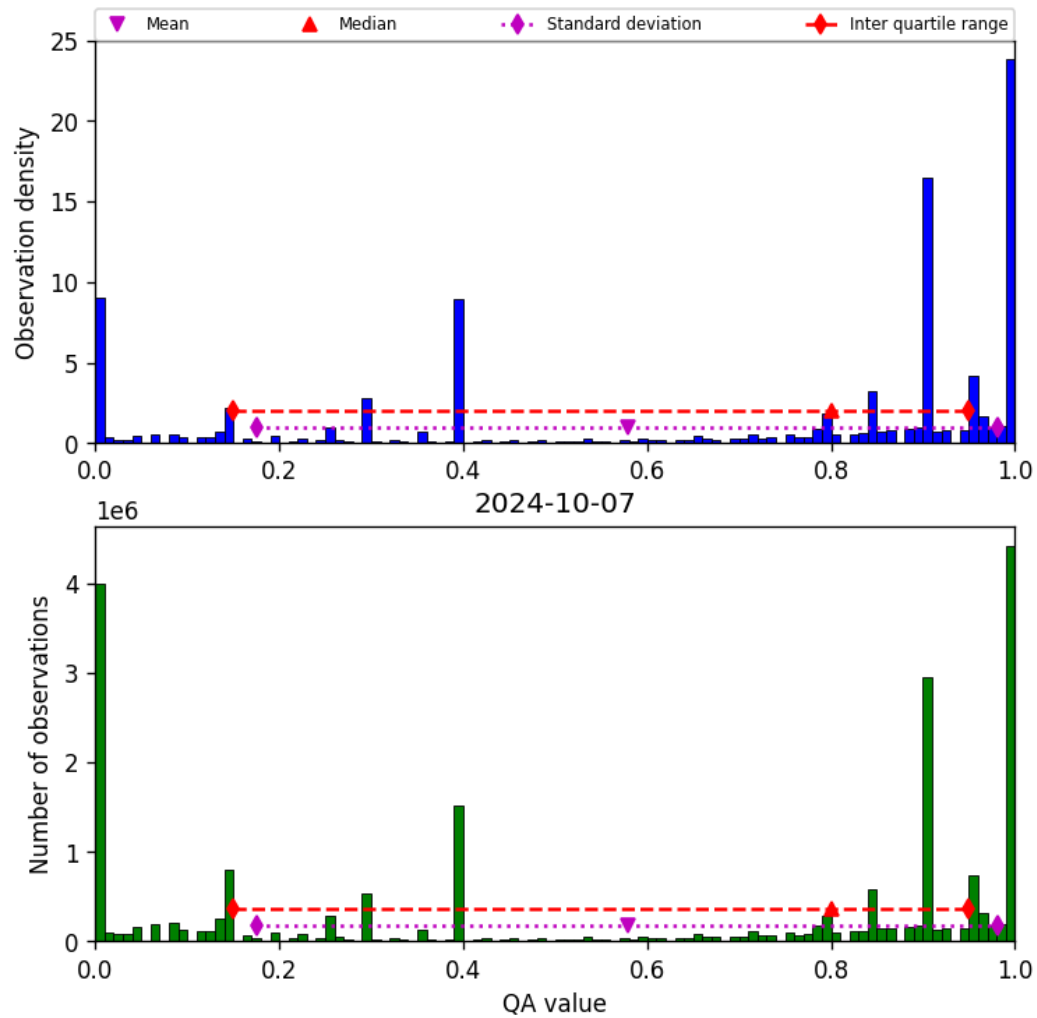
Figure 38: Histogram of “QA value” for 2024-10-06 to 2024-10-08
