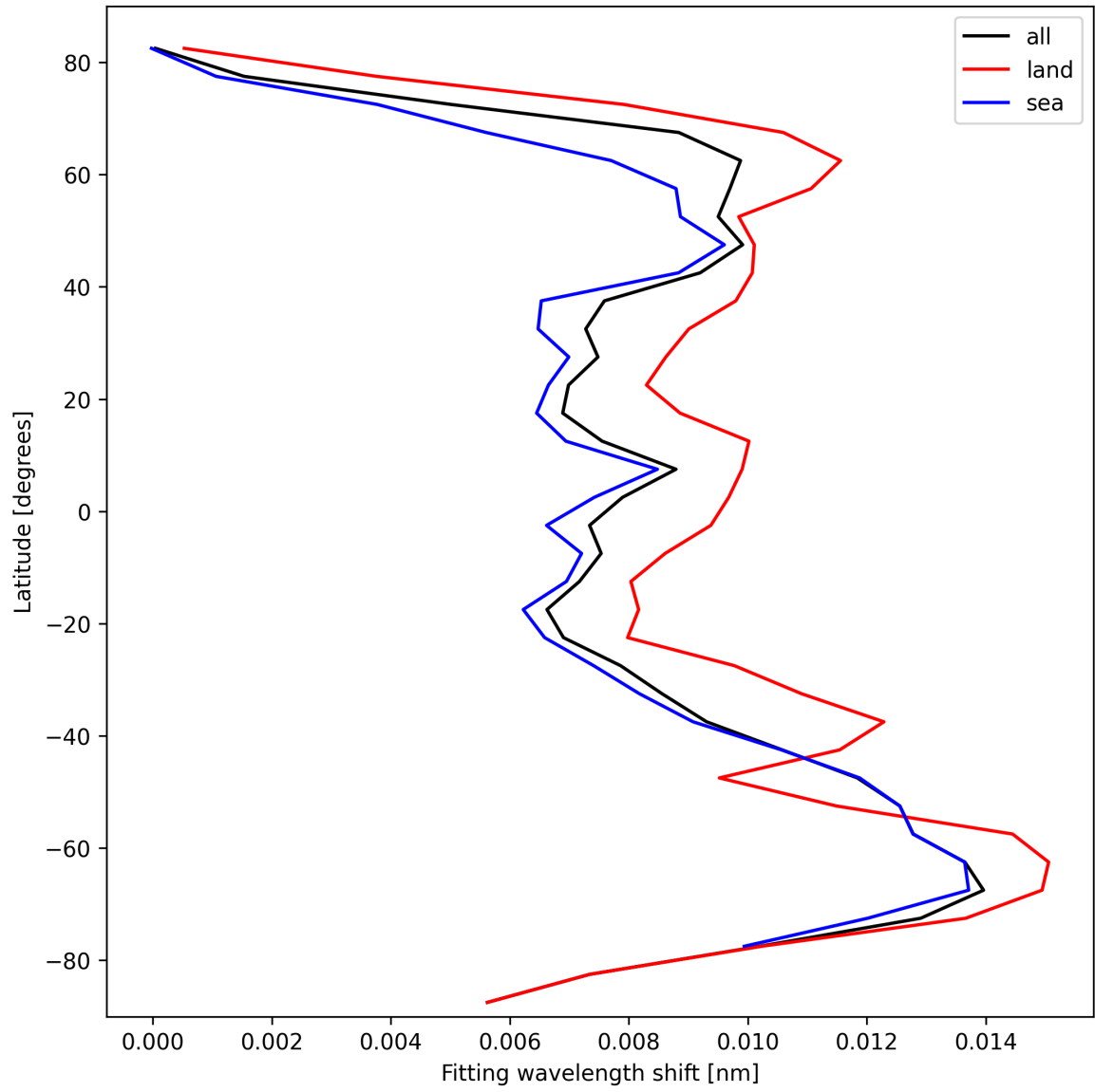
Figure 33: Zonal average of “Fitting wavelength shift” for 2024-10-06 to 2024-10-08.
