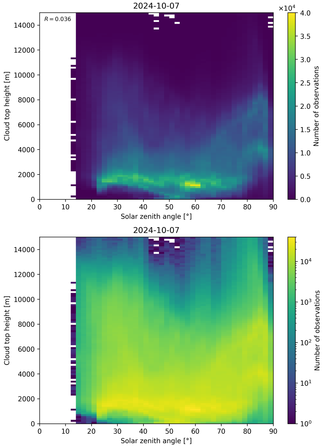
Figure 104: Scatter density plot of “Solar zenith angle” against “Cloud top height” for 2024-10-06 to 2024-10-08.
