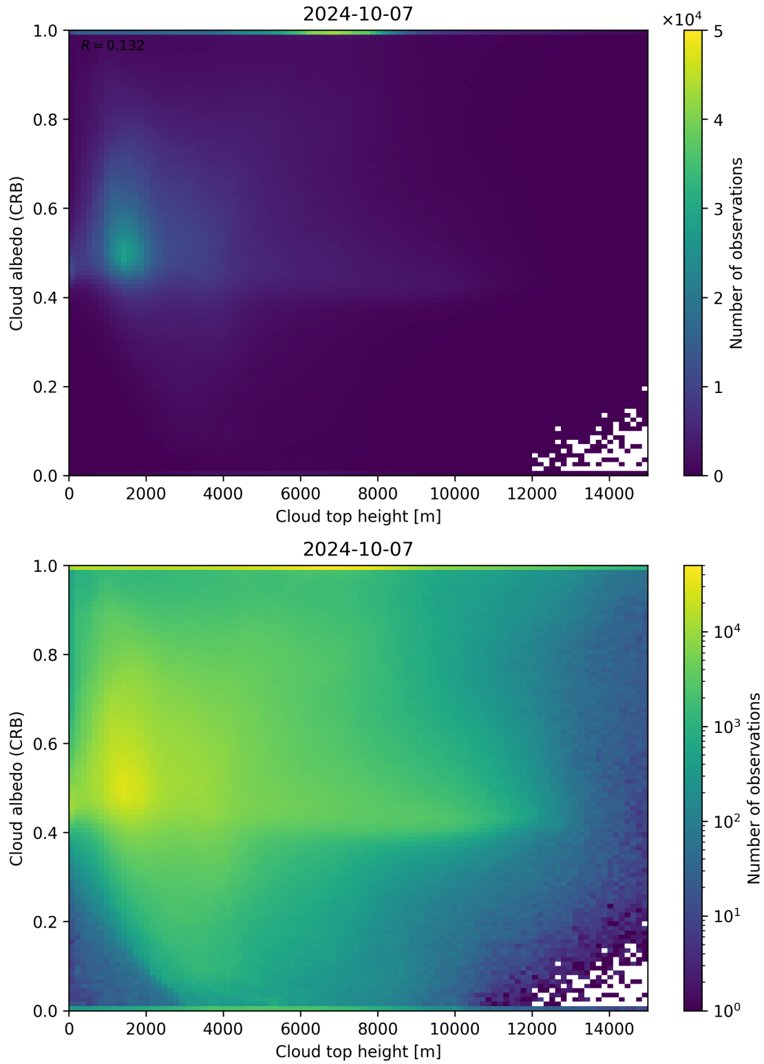
Figure 86: Scatter density plot of “Cloud top height” against “Cloud albedo (CRB)” for 2024-10-06 to 2024-10-08.
