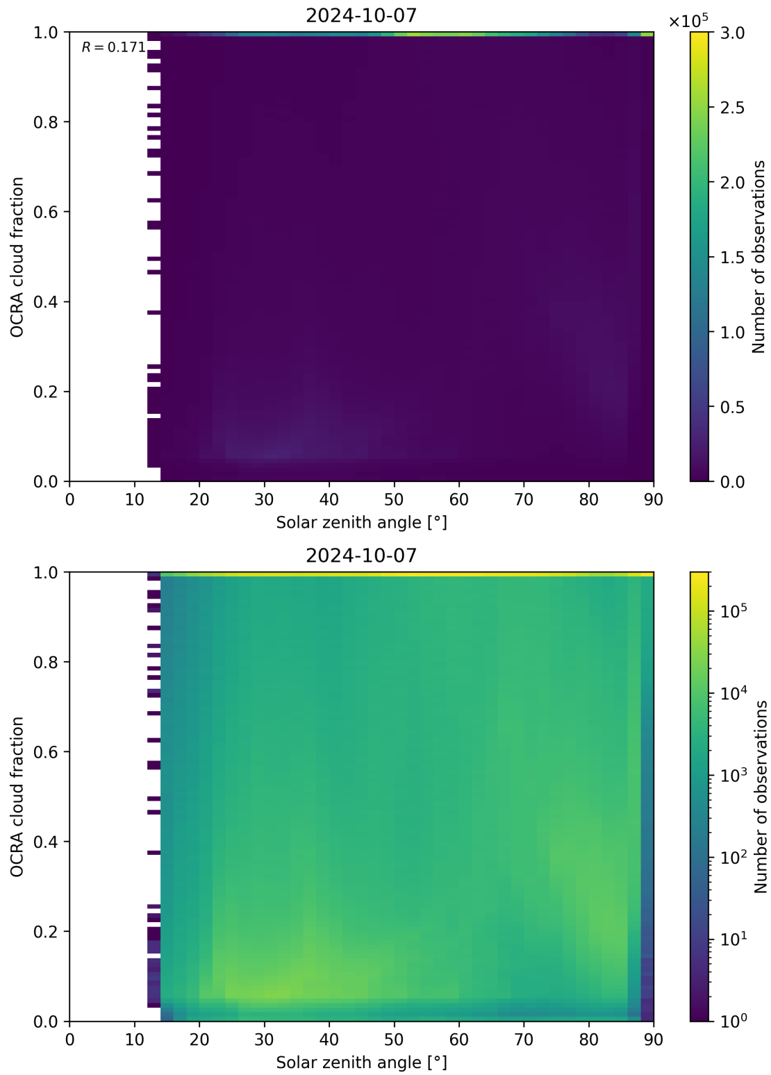
Figure 100: Scatter density plot of “Solar zenith angle” against “OCRA cloud fraction” for 2024-10-06 to 2024-10-08.
