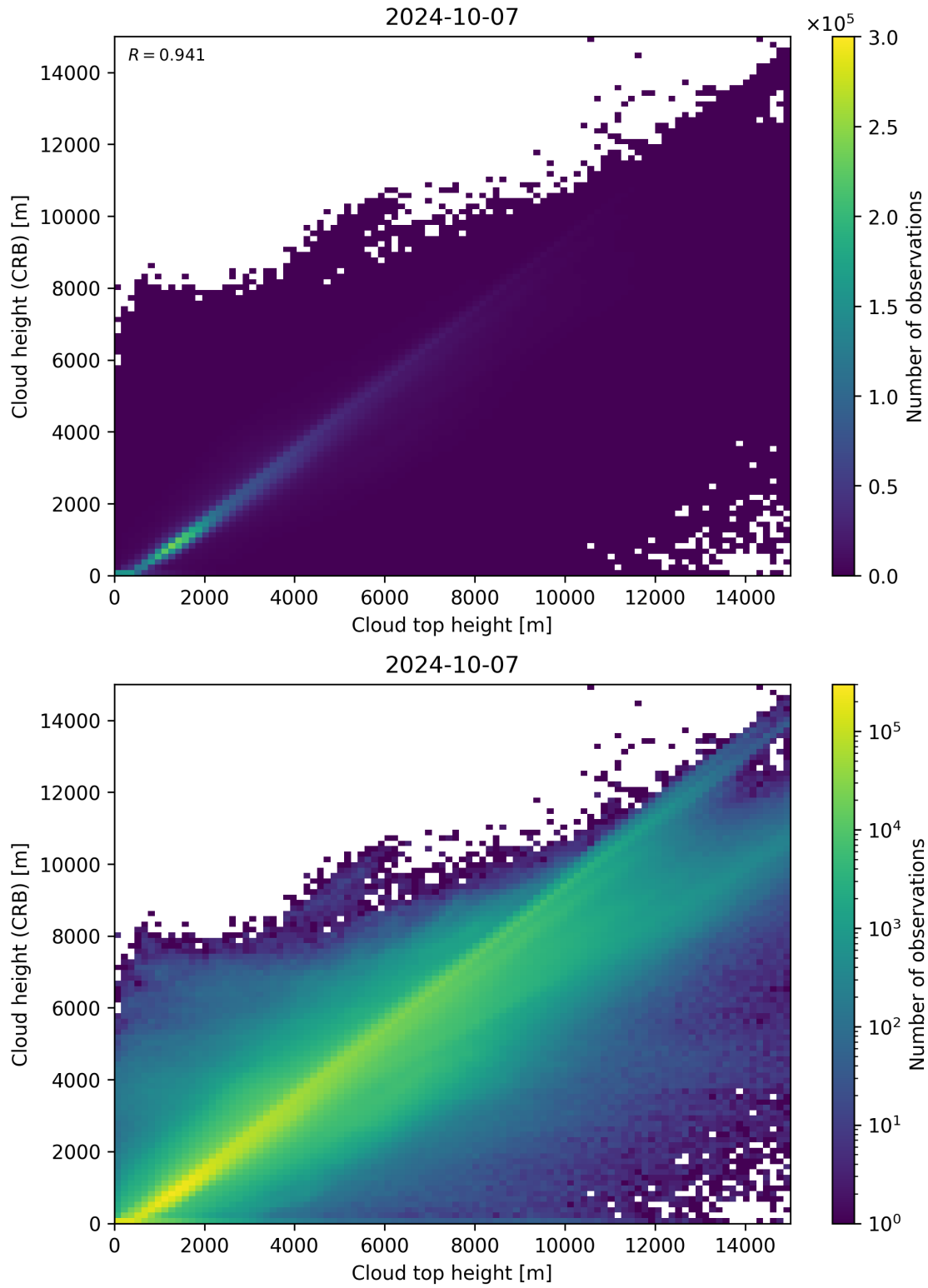
Figure 89: Scatter density plot of “Cloud top height” against “Cloud height (CRB)” for 2024-10-06 to 2024-10-08.
