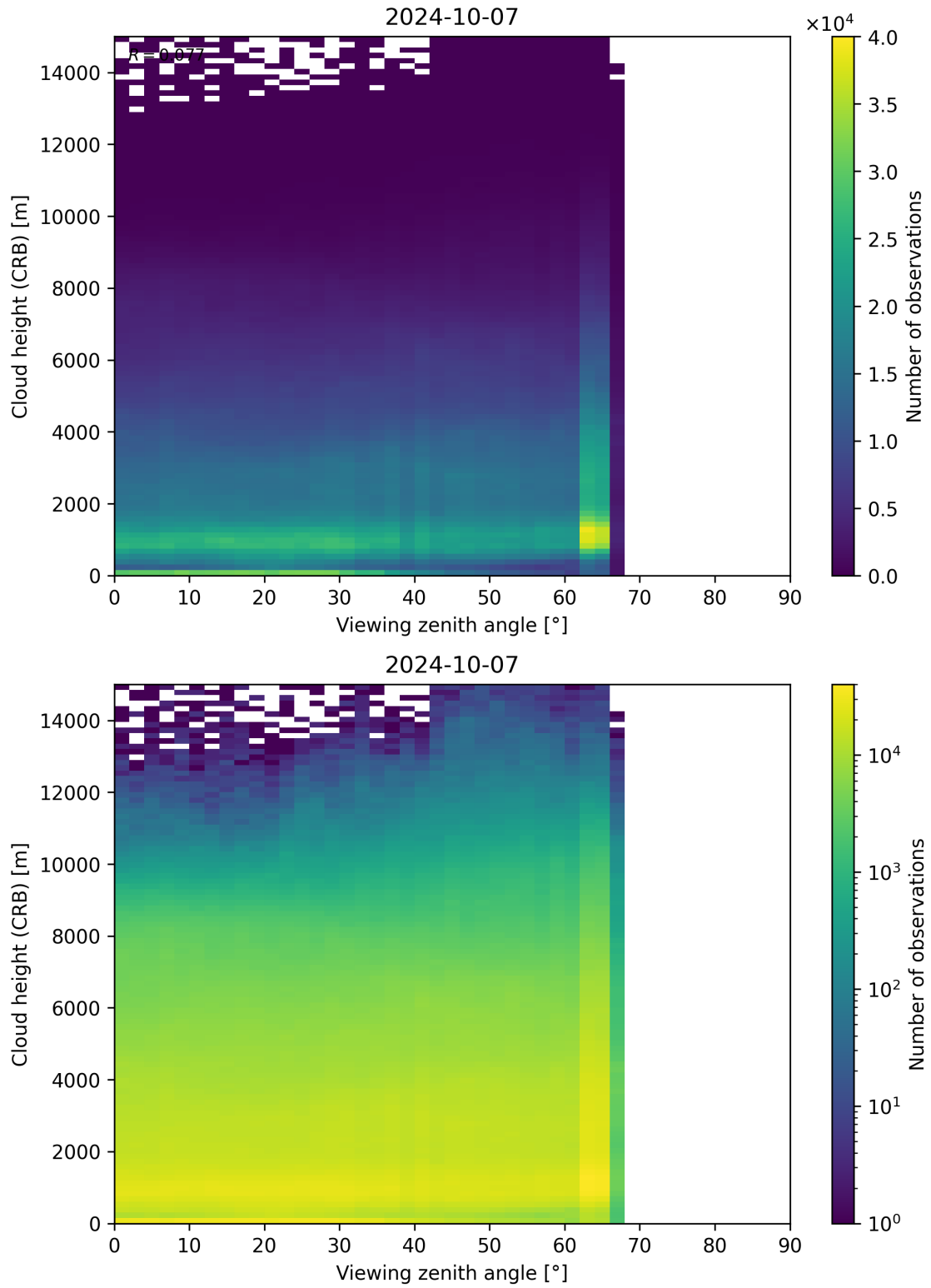
Figure 110: Scatter density plot of “Viewing zenith angle” against “Cloud height (CRB)” for 2024-10-06 to 2024-10-08.
