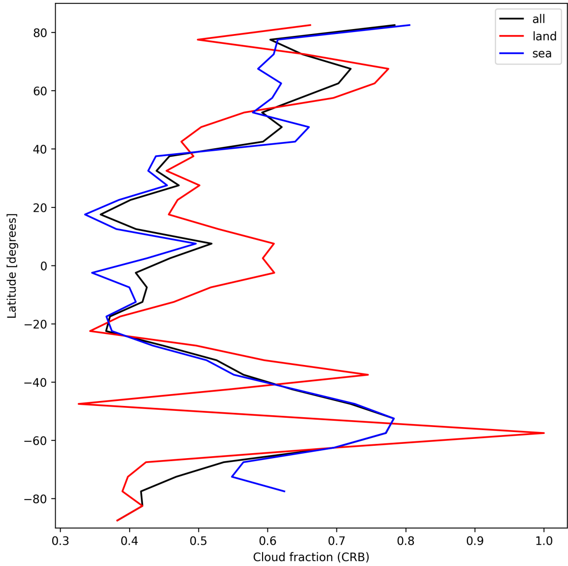
Figure 26: Zonal average of “Cloud fraction (CRB)” for 2024-10-06 to 2024-10-08.
