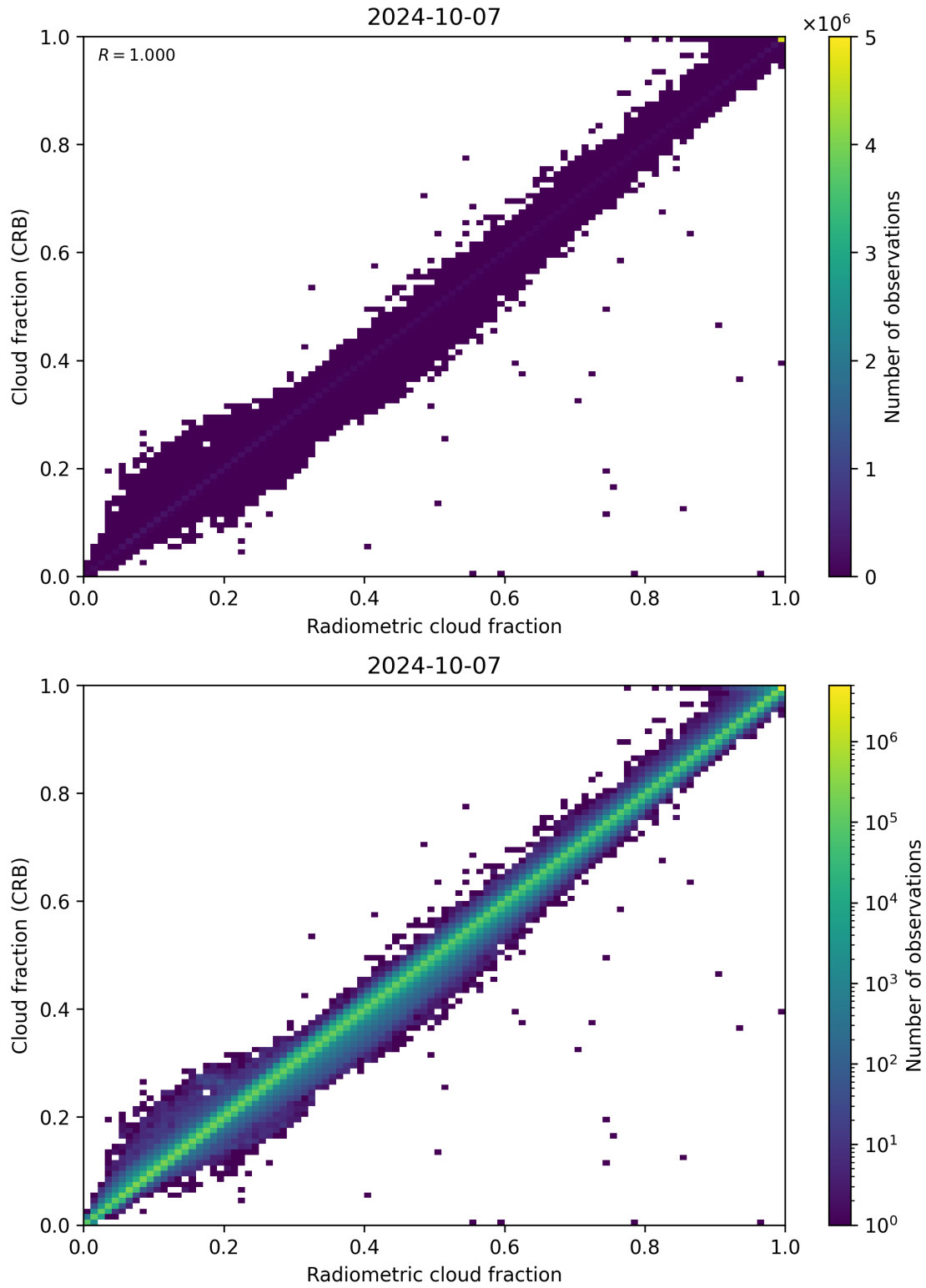
Figure 73: Scatter density plot of “Radiometric cloud fraction” against “Cloud fraction (CRB)” for 2024-10-06 to 2024-10-08.
