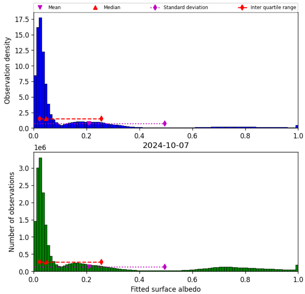
Figure 45: Histogram of “Fitted surface albedo” for 2024-10-06 to 2024-10-08
