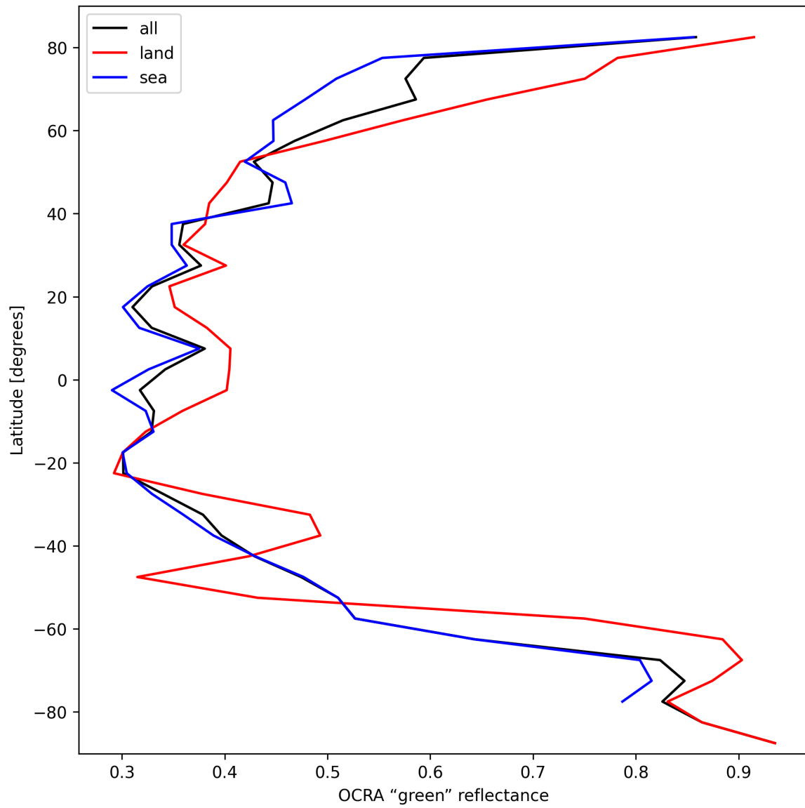
Figure 36: Zonal average of “OCRA “green” reflectance” for 2024-10-06 to 2024-10-08.
