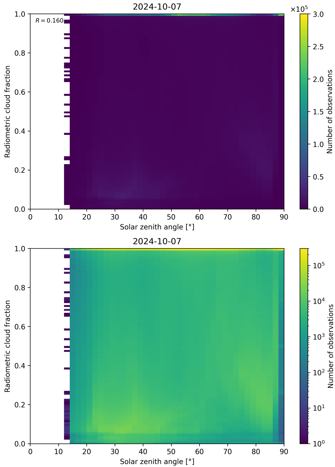
Figure 99: Scatter density plot of “Solar zenith angle” against “Radiometric cloud fraction” for 2024-10-06 to 2024-10-08.
