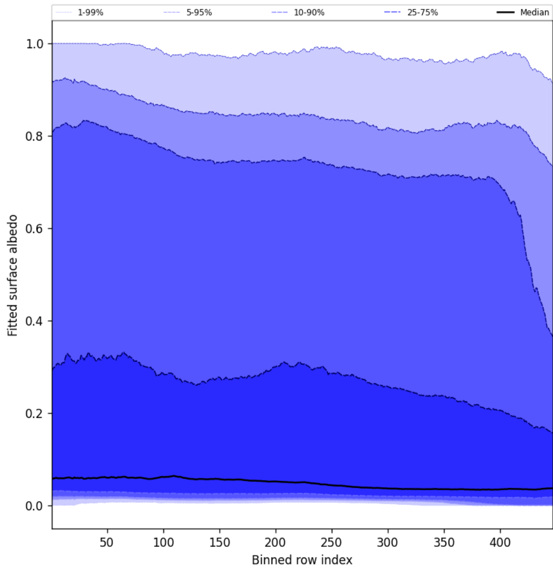
Figure 61: Along track statistics of “Fitted surface albedo” for 2024-10-06 to 2024-10-08
