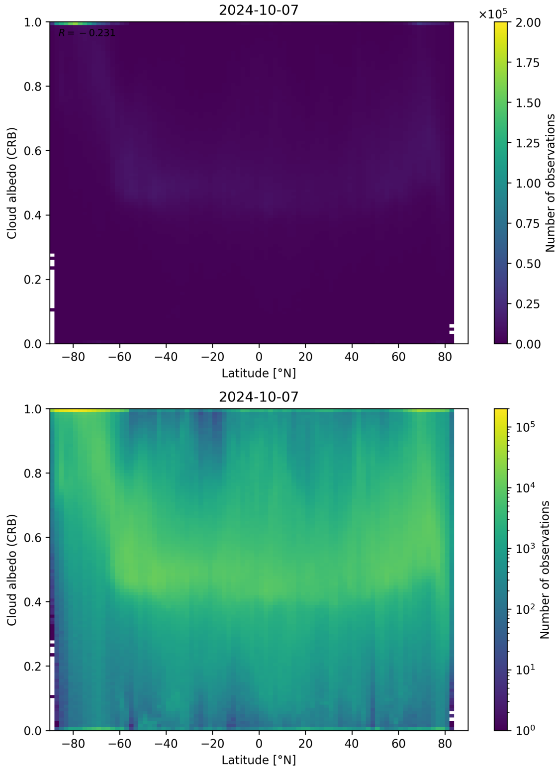
Figure 91: Scatter density plot of “Latitude” against “Cloud albedo (CRB)” for 2024-10-06 to 2024-10-08.
