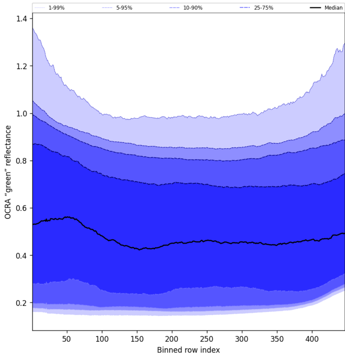
Figure 68: Along track statistics of “OCRA “green” reflectance” for 2024-10-06 to 2024-10-08
