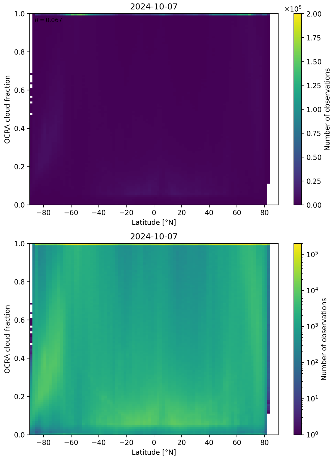
Figure 93: Scatter density plot of “Latitude” against “OCRA cloud fraction” for 2024-10-06 to 2024-10-08.
