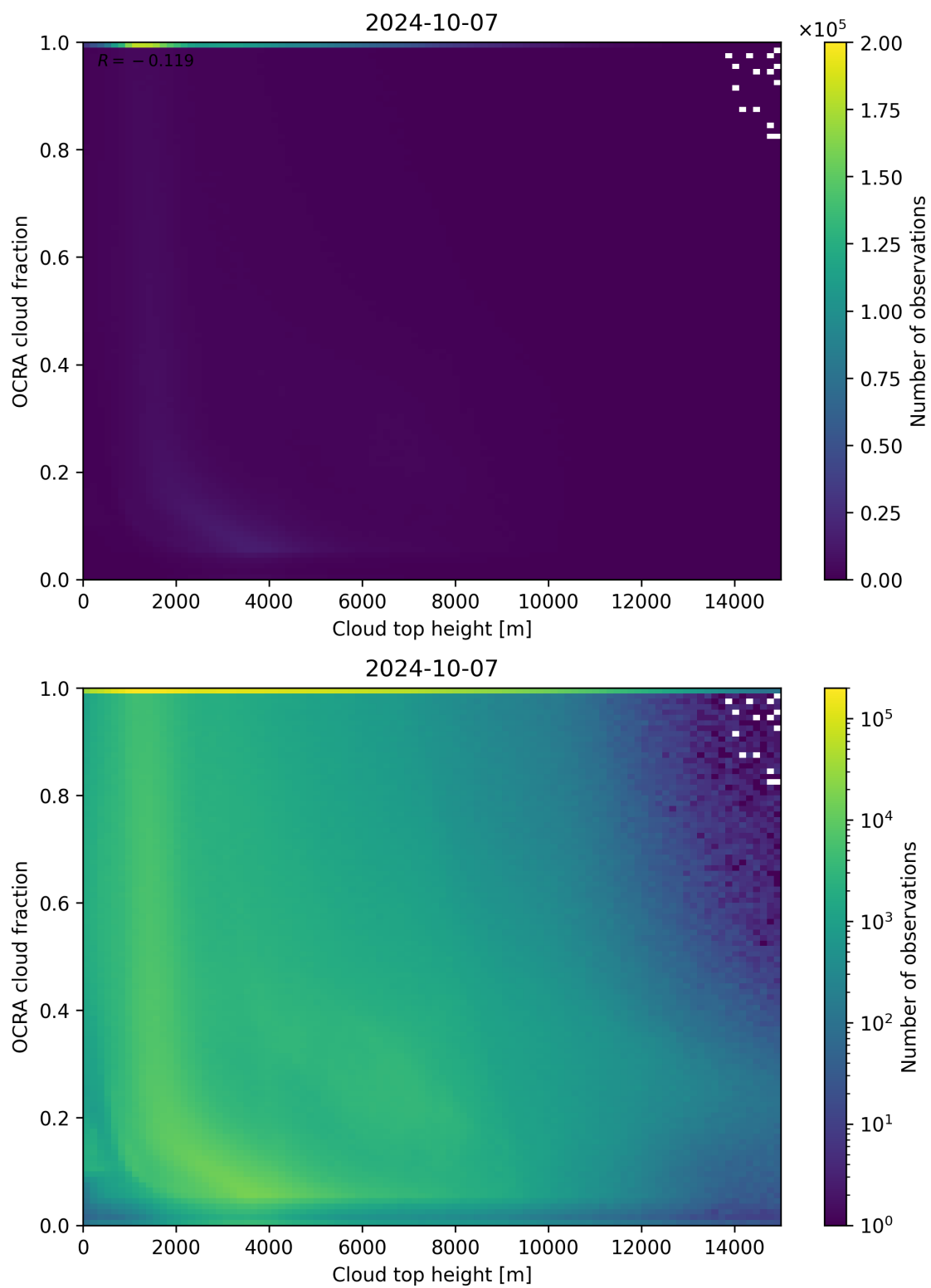
Figure 87: Scatter density plot of “Cloud top height” against “OCRA cloud fraction” for 2024-10-06 to 2024-10-08.
