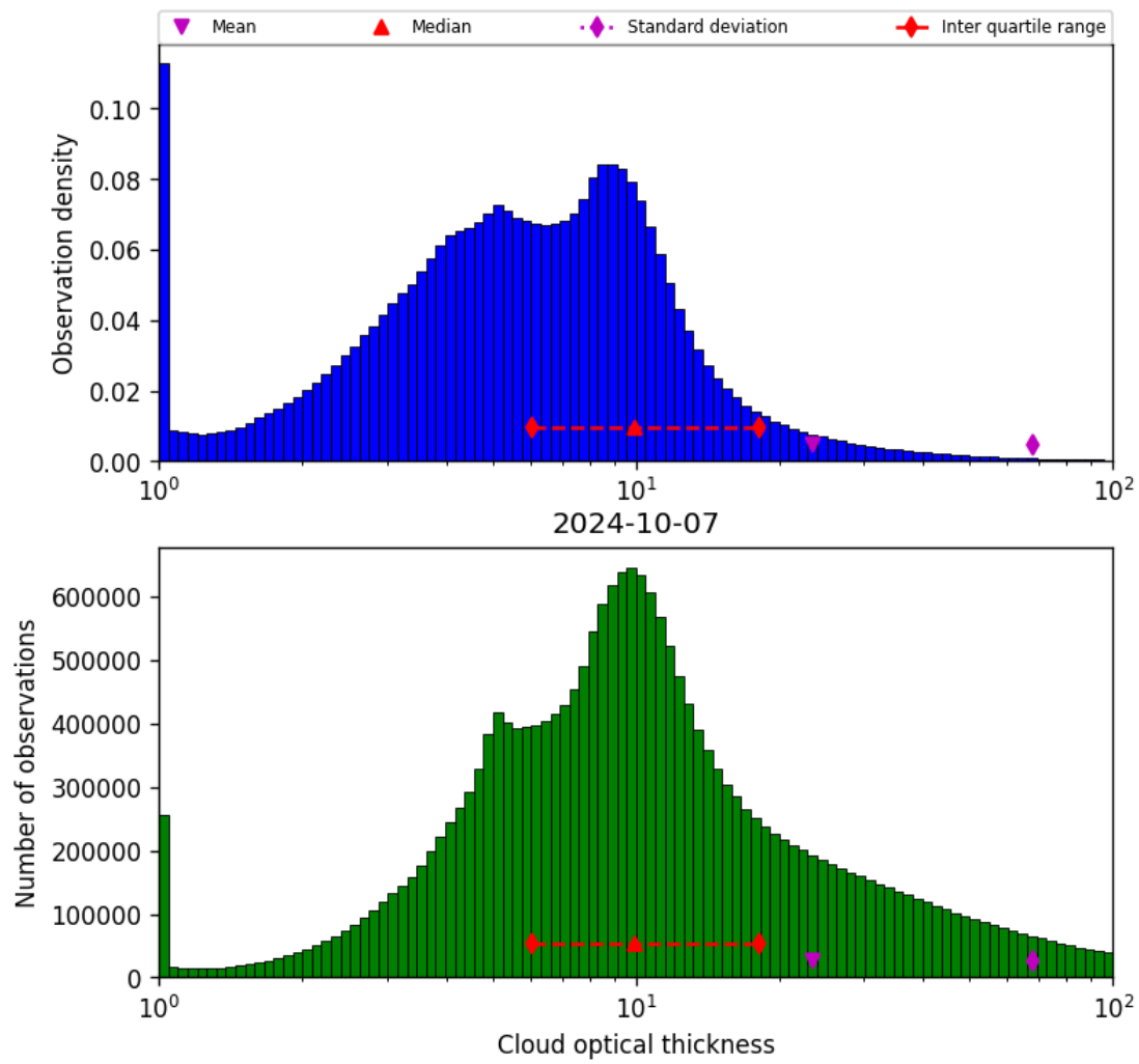
Figure 41: Histogram of “Cloud optical thickness” for 2024-10-06 to 2024-10-08
