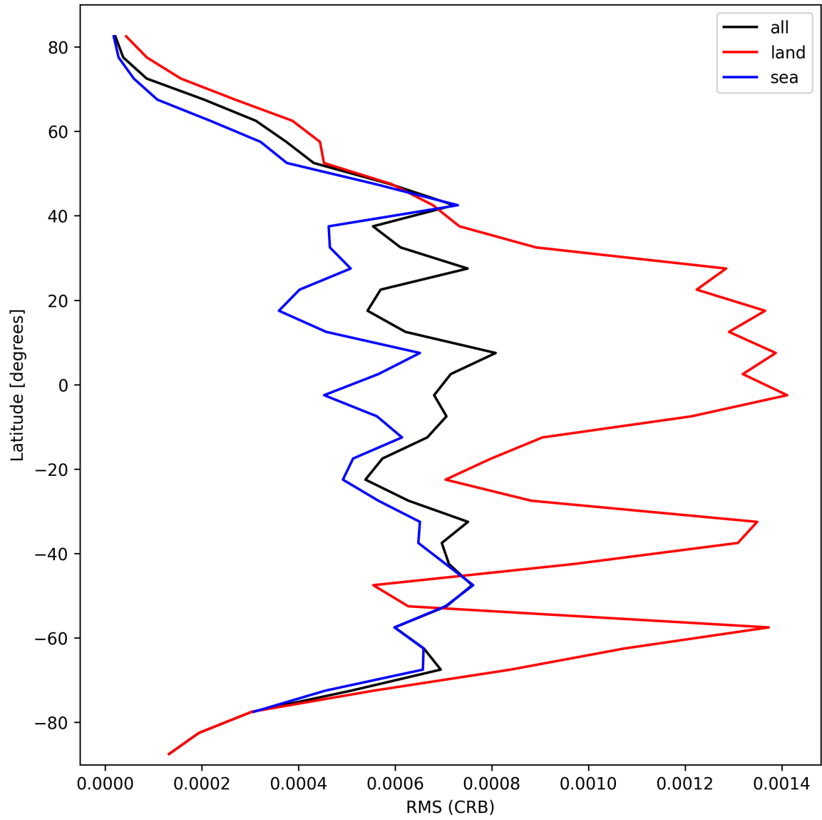
Figure 32: Zonal average of “RMS (CRB)” for 2024-10-06 to 2024-10-08.
