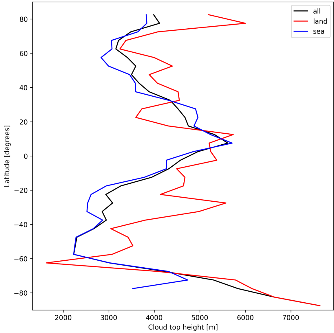
Figure 24: Zonal average of “Cloud top height” for 2024-10-06 to 2024-10-08.
