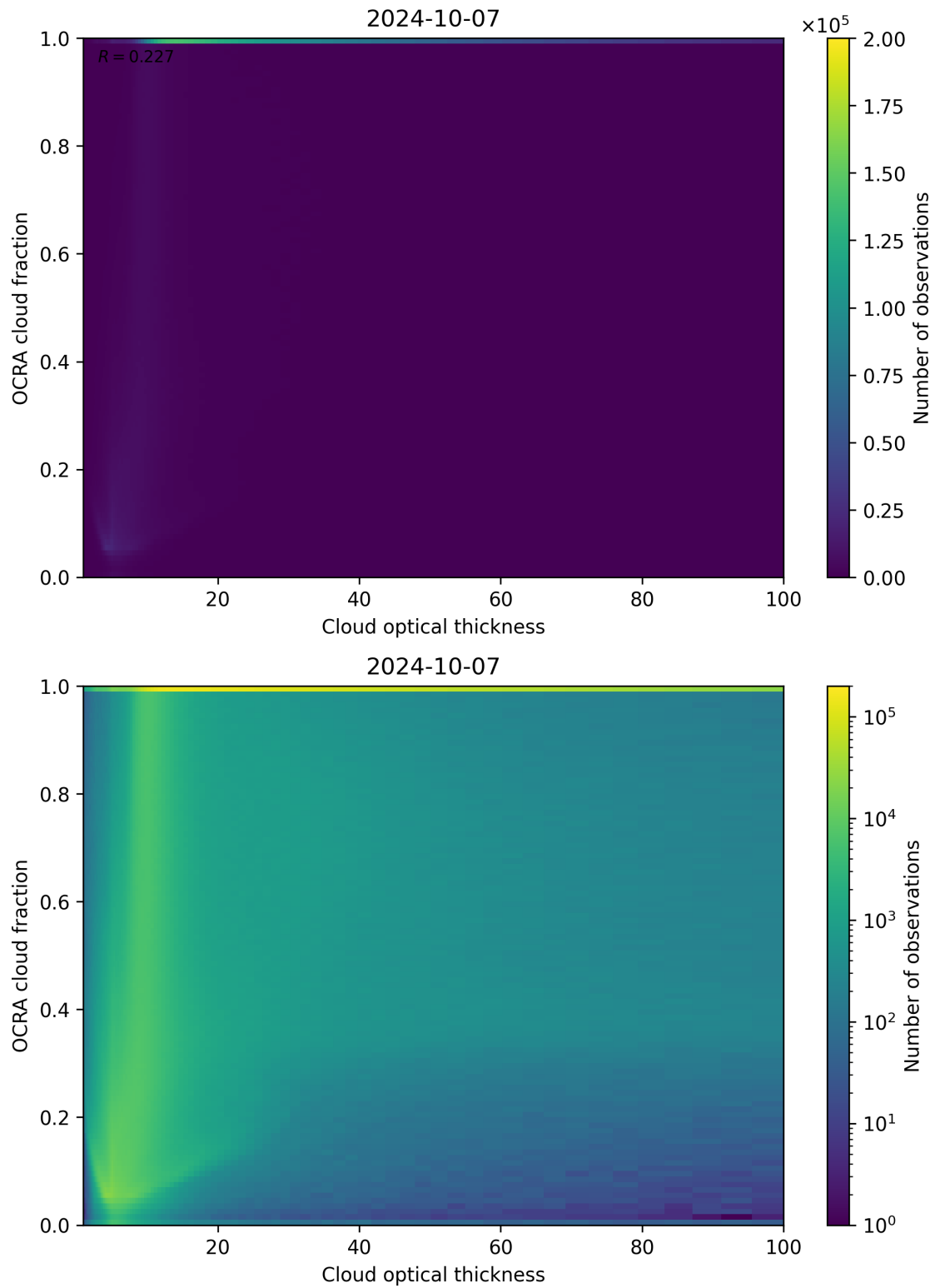
Figure 83: Scatter density plot of “Cloud optical thickness” against “OCRA cloud fraction” for 2024-10-06 to 2024-10-08.
