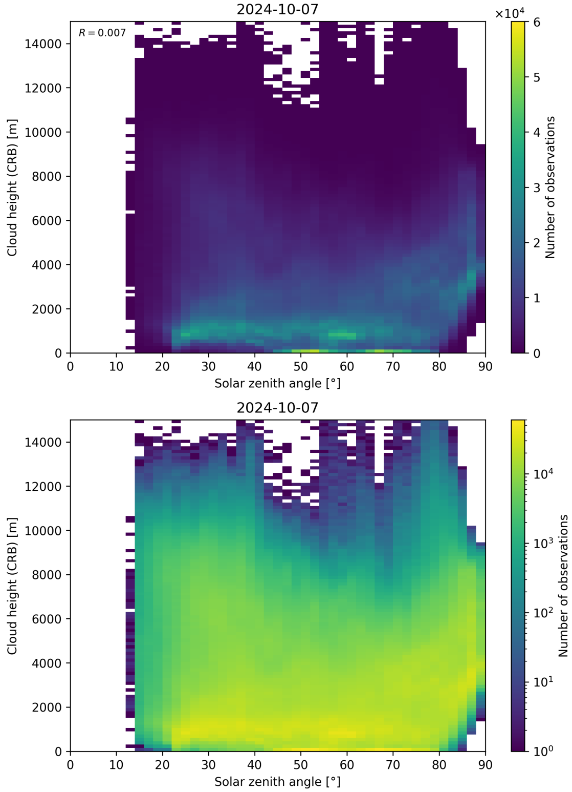
Figure 102: Scatter density plot of “Solar zenith angle” against “Cloud height (CRB)” for 2024-10-06 to 2024-10-08.
