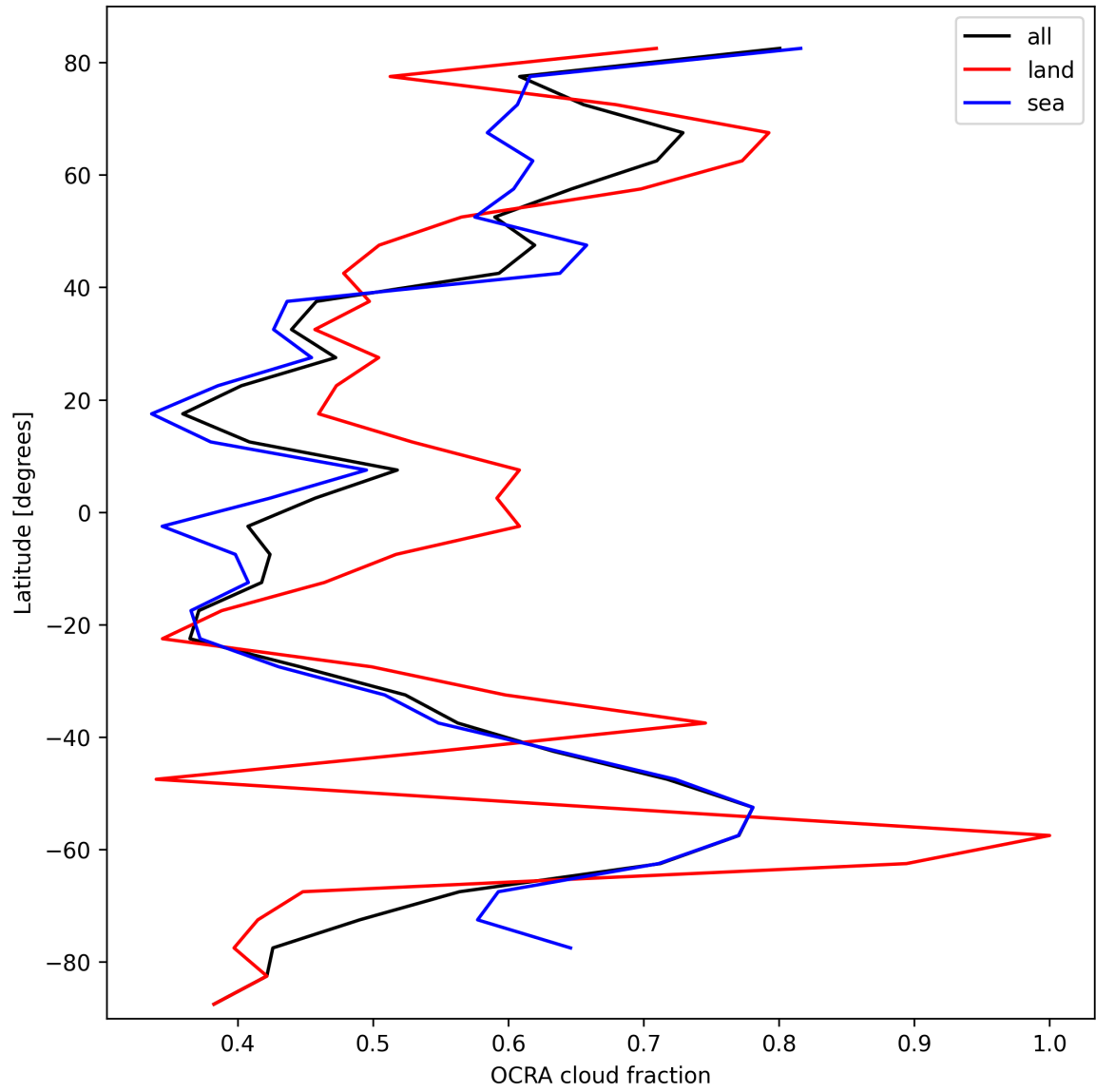
Figure 34: Zonal average of “OCRA cloud fraction” for 2024-10-06 to 2024-10-08.
