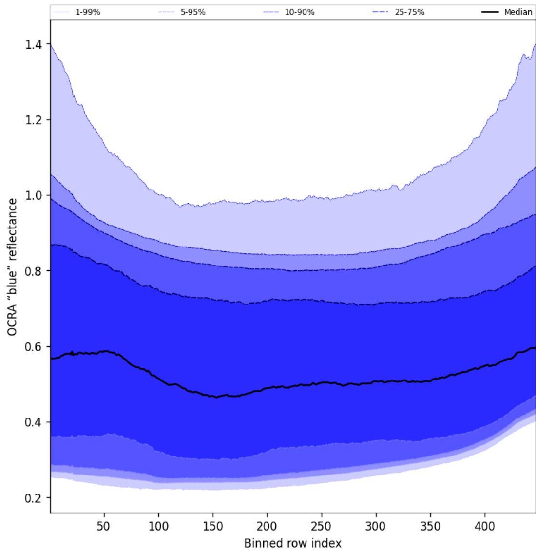
Figure 67: Along track statistics of “OCRA “blue” reflectance” for 2024-10-06 to 2024-10-08
