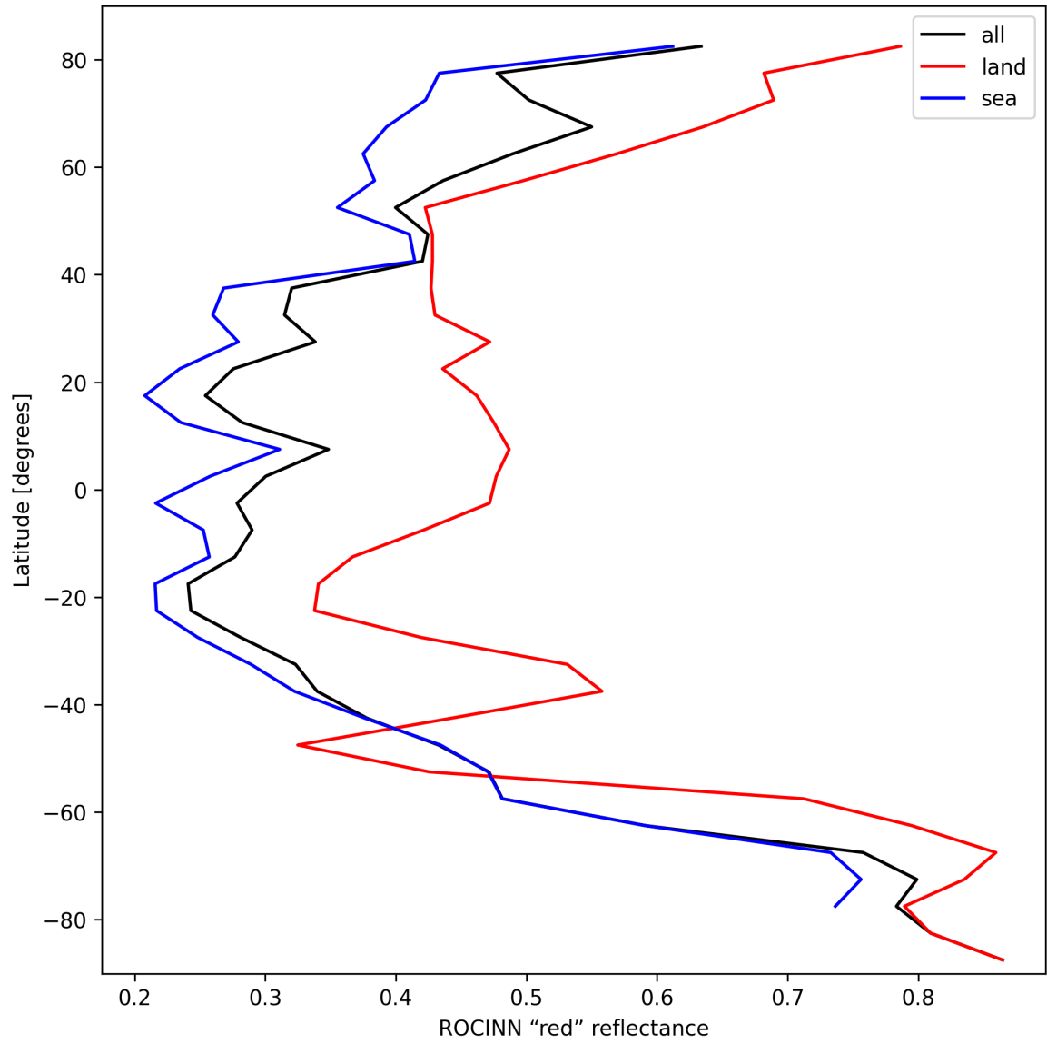
Figure 37: Zonal average of "ROCINN "red" reflectance" for 2024-10-06 to 2024-10-08.
