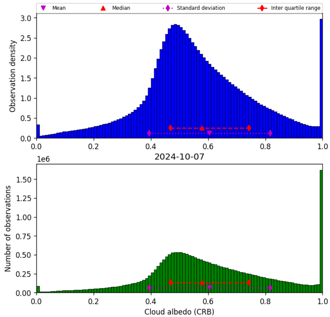
Figure 44: Histogram of “Cloud albedo (CRB)” for 2024-10-06 to 2024-10-08
