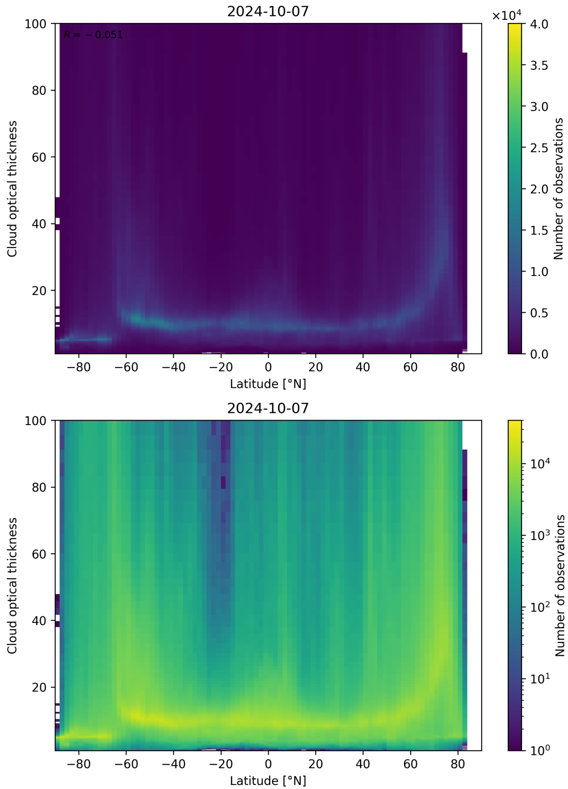
Figure 96: Scatter density plot of “Latitude” against “Cloud optical thickness” for 2024-10-06 to 2024-10-08.
