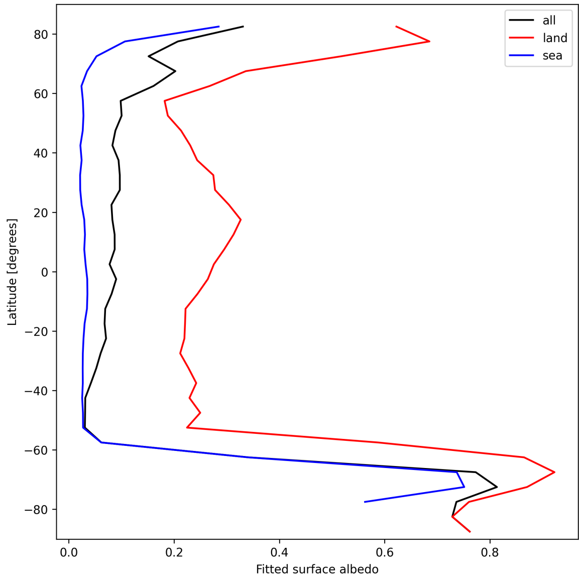
Figure 29: Zonal average of “Fitted surface albedo” for 2024-10-06 to 2024-10-08.
