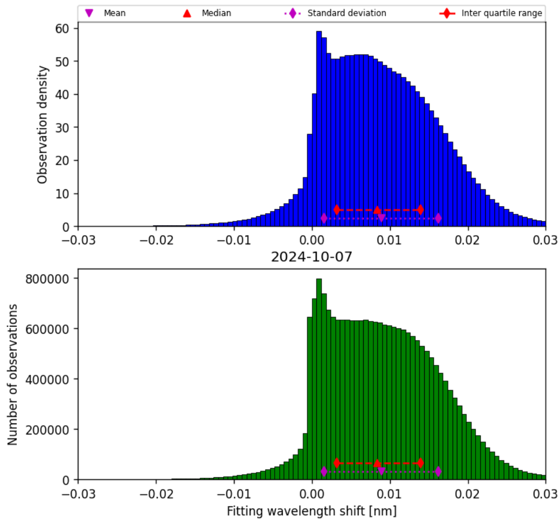
Figure 49: Histogram of “Fitting wavelength shift” for 2024-10-06 to 2024-10-08
