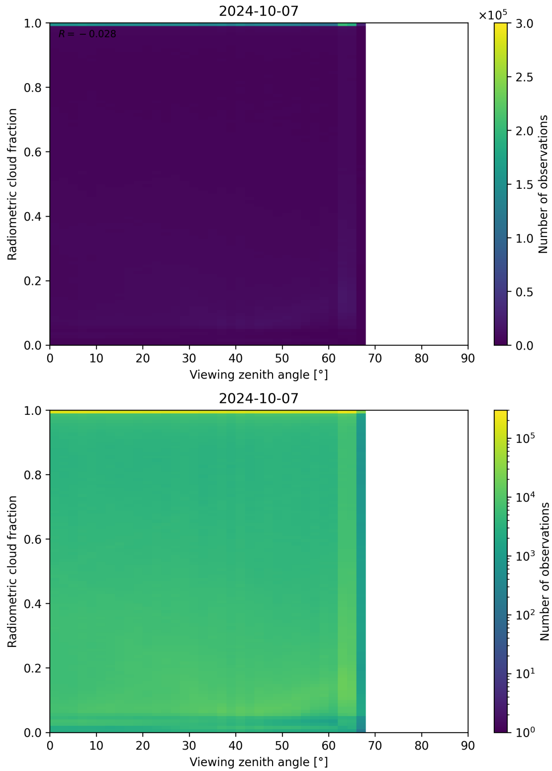
Figure 107: Scatter density plot of “Viewing zenith angle” against “Radiometric cloud fraction” for 2024-10-06 to 2024-10-08.
