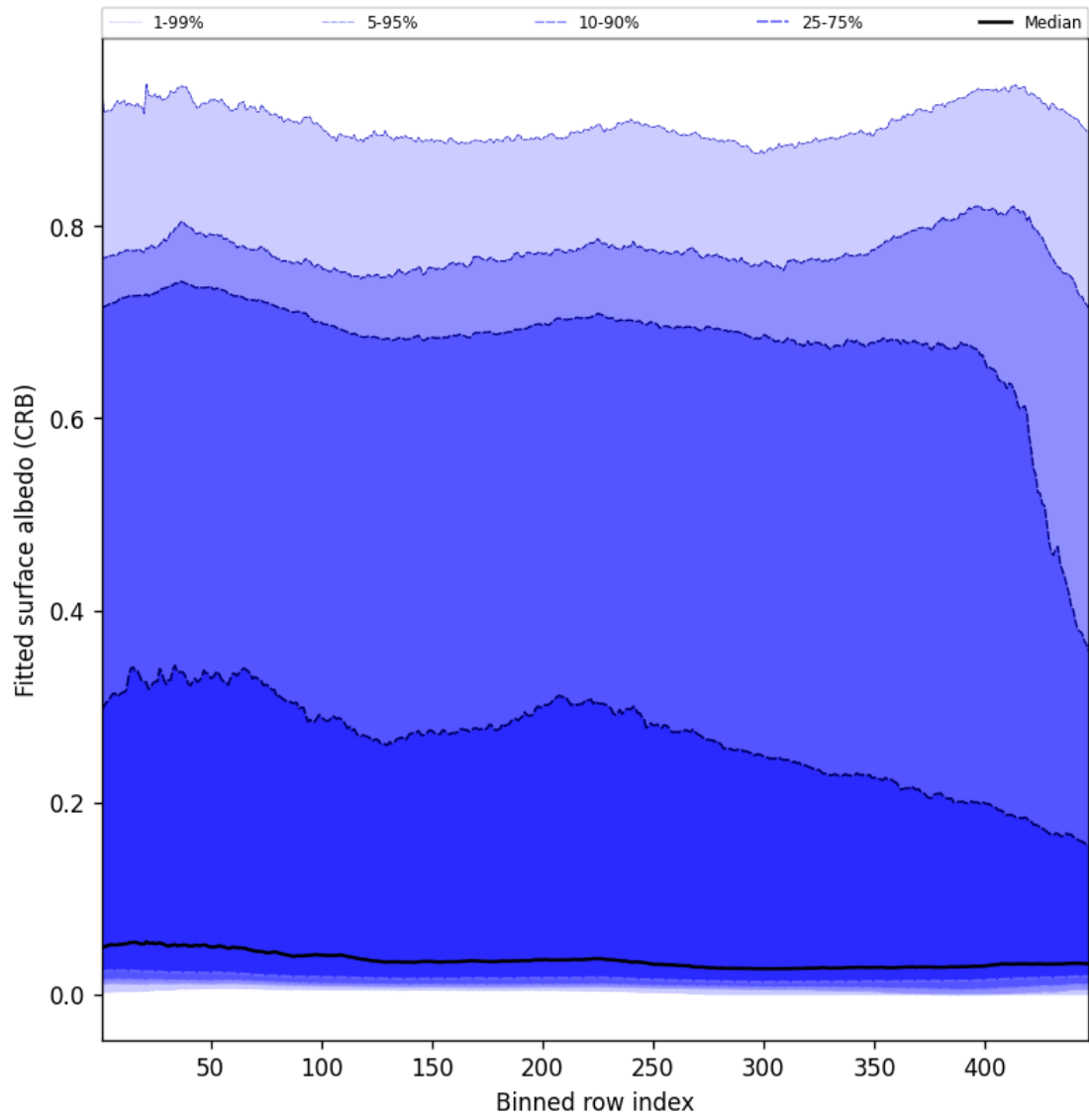
Figure 62: Along track statistics of “Fitted surface albedo (CRB)” for 2024-10-06 to 2024-10-08
