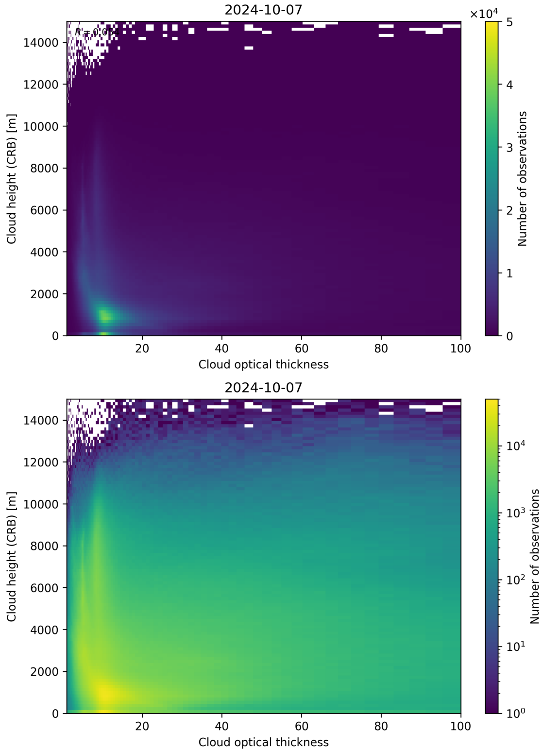
Figure 85: Scatter density plot of “Cloud optical thickness” against “Cloud height (CRB)” for 2024-10-06 to 2024-10-08.
