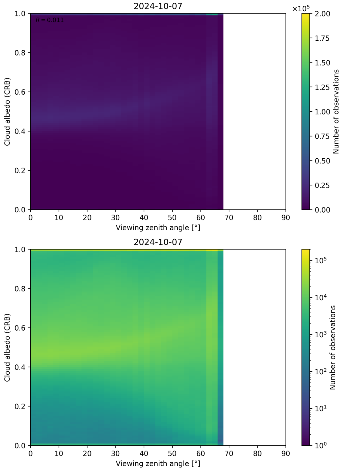
Figure 106: Scatter density plot of “Viewing zenith angle” against “Cloud albedo (CRB)” for 2024-10-06 to 2024-10-08.
