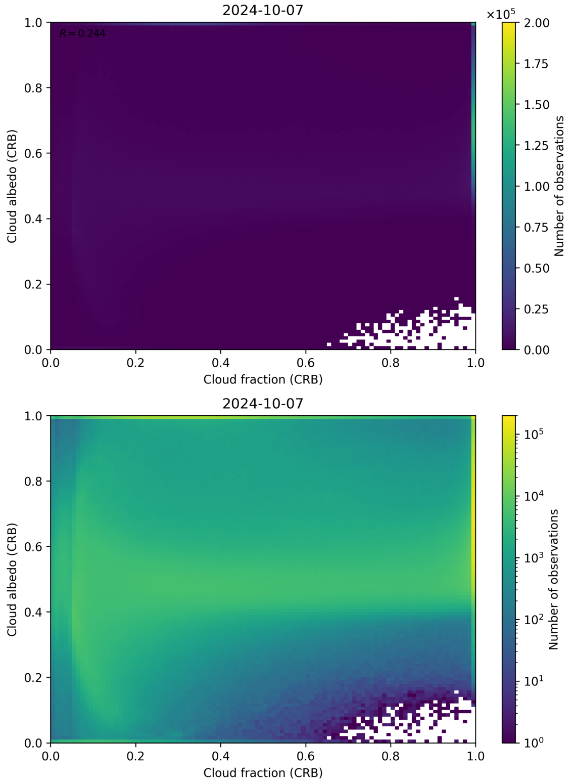
Figure 77: Scatter density plot of “Cloud fraction (CRB)” against “Cloud albedo (CRB)” for 2024-10-06 to 2024-10-08.
