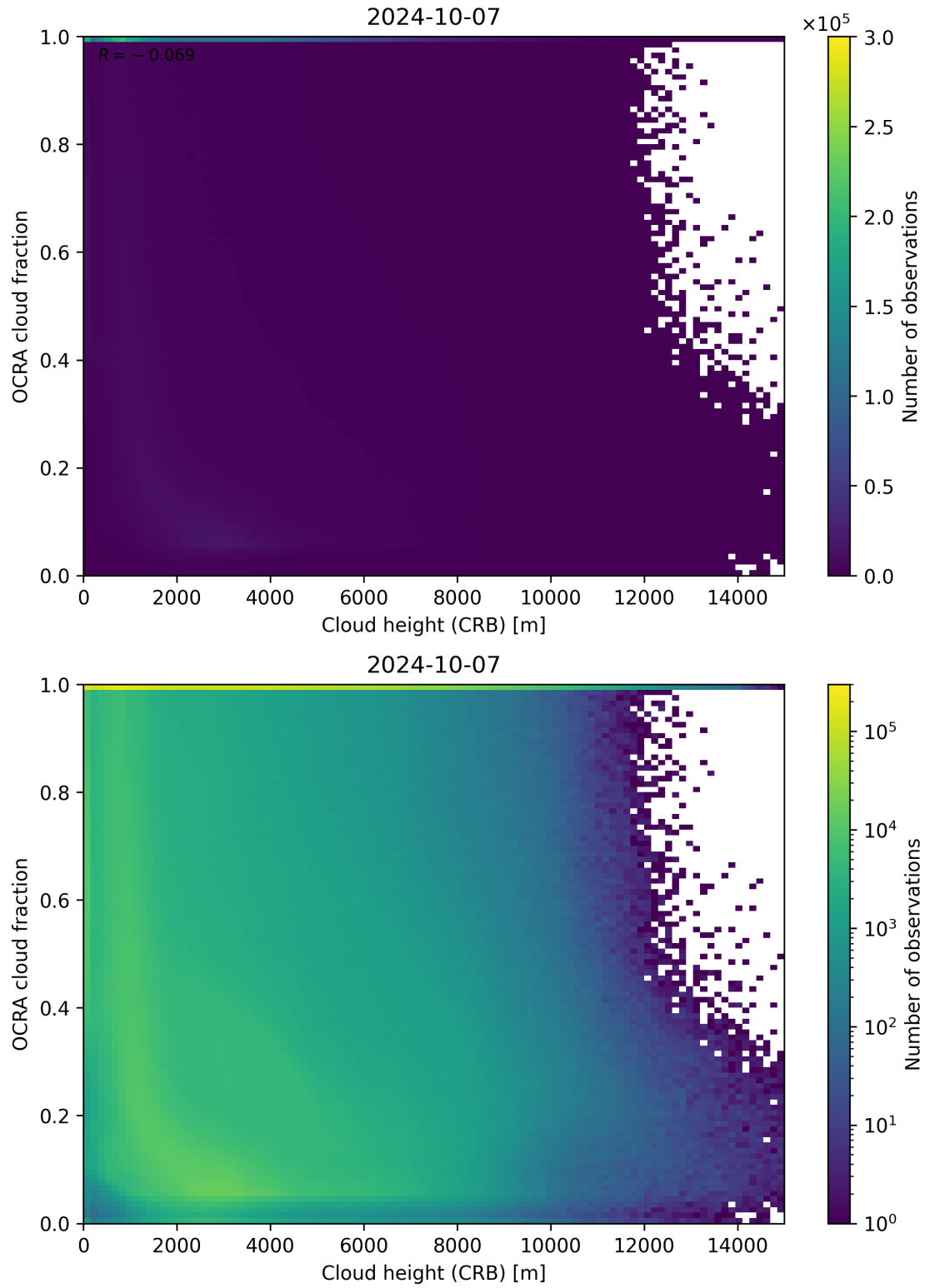
Figure 81: Scatter density plot of “Cloud height (CRB)” against “OCRA cloud fraction” for 2024-10-06 to 2024-10-08.
