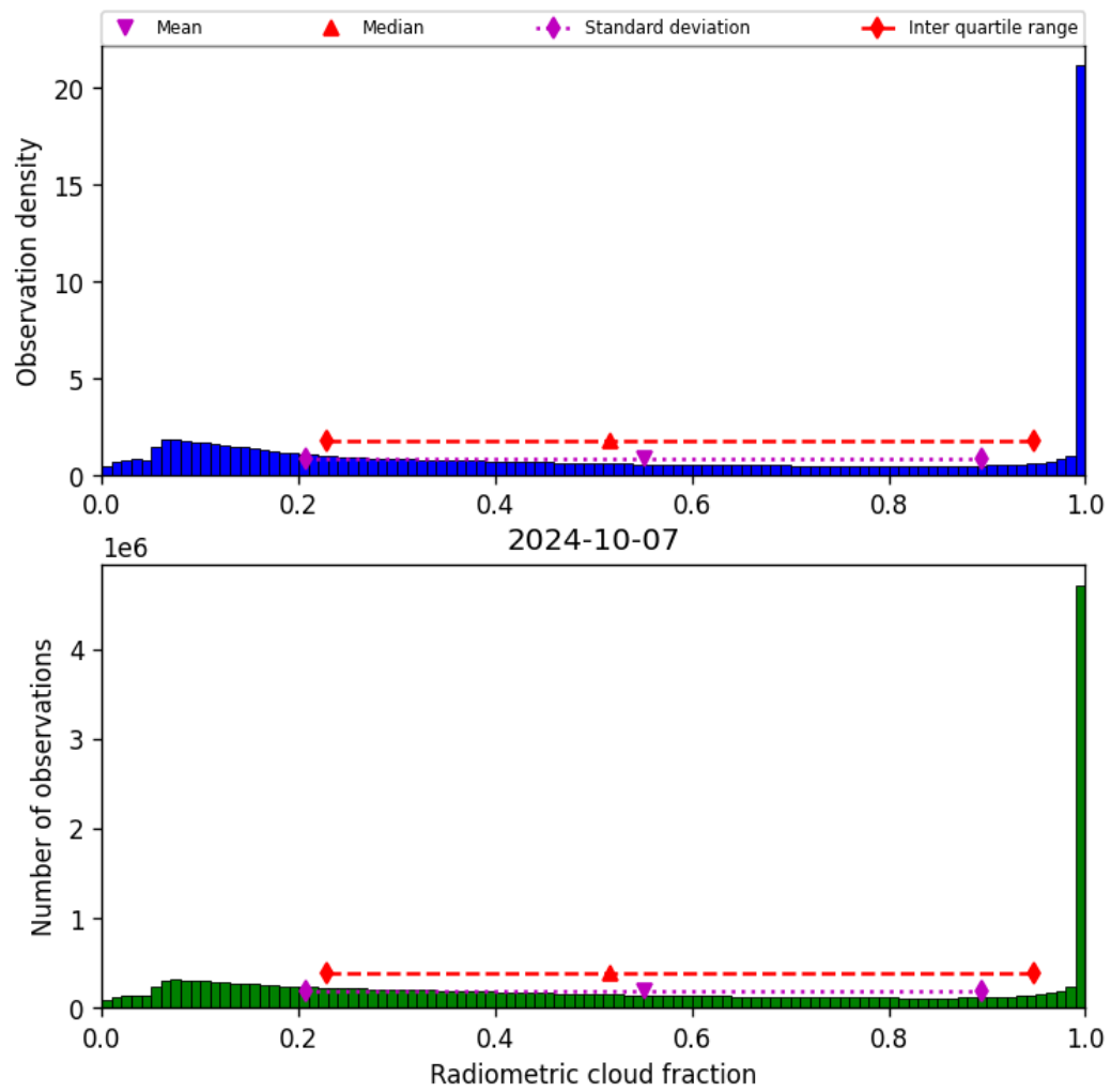
Figure 39: Histogram of “Radiometric cloud fraction” for 2024-10-06 to 2024-10-08
