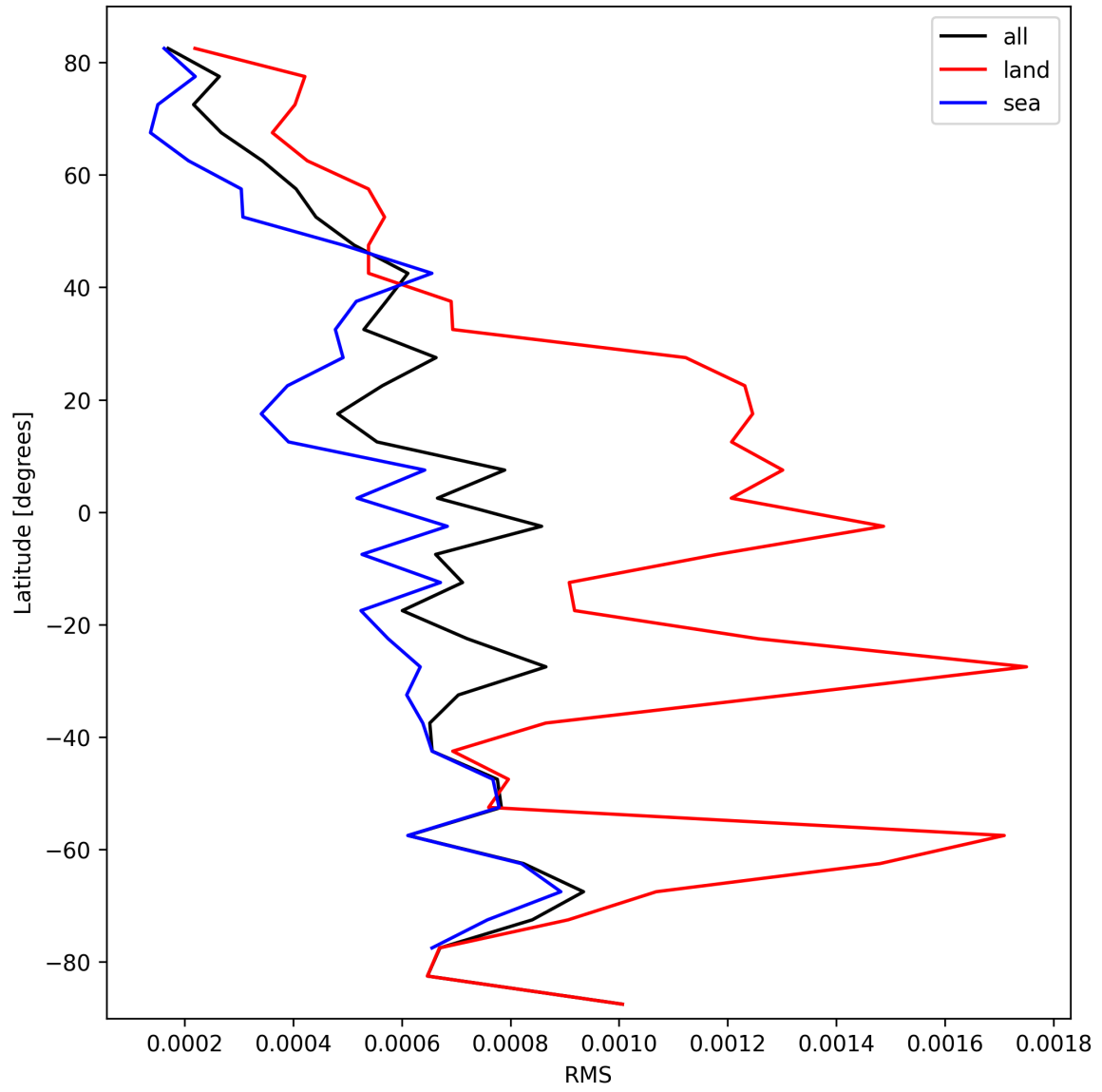
Figure 31: Zonal average of “RMS” for 2024-10-08 to 2024-10-10.
