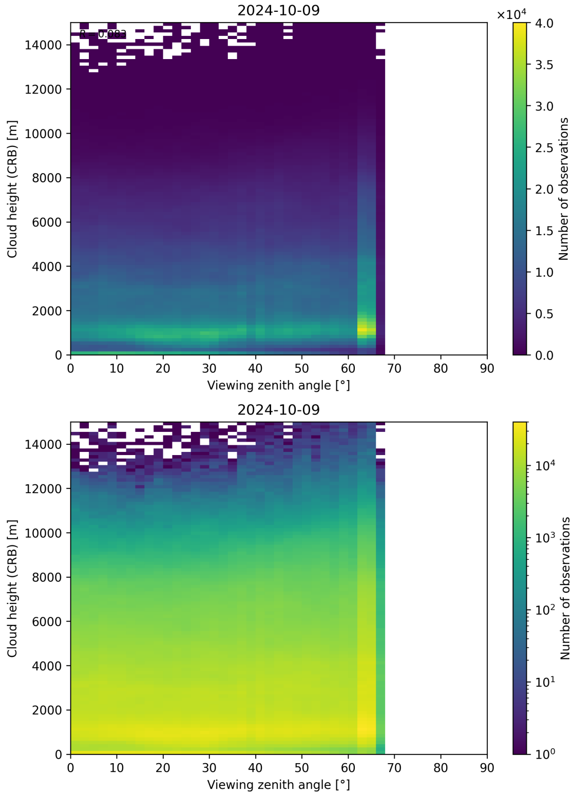
Figure 110: Scatter density plot of “Viewing zenith angle” against “Cloud height (CRB)” for 2024-10-08 to 2024-10-10.
