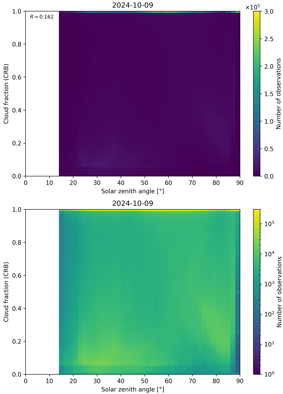
Figure 101: Scatter density plot of “Solar zenith angle” against “Cloud fraction (CRB)” for 2024-10-08 to 2024-10-10.
