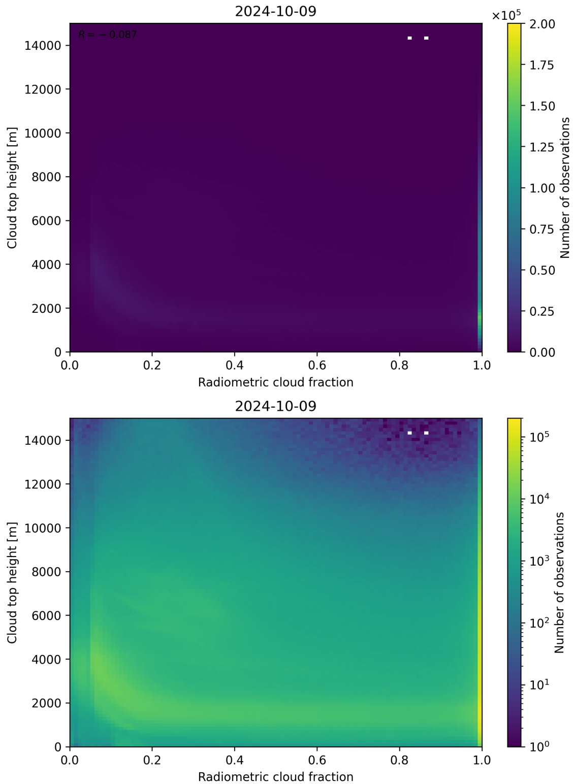
Figure 76: Scatter density plot of “Radiometric cloud fraction” against “Cloud top height” for 2024-10-08 to 2024-10-10.
