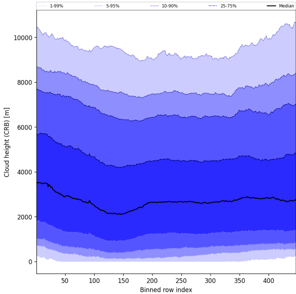
Figure 59: Along track statistics of “Cloud height (CRB)” for 2024-10-08 to 2024-10-10
