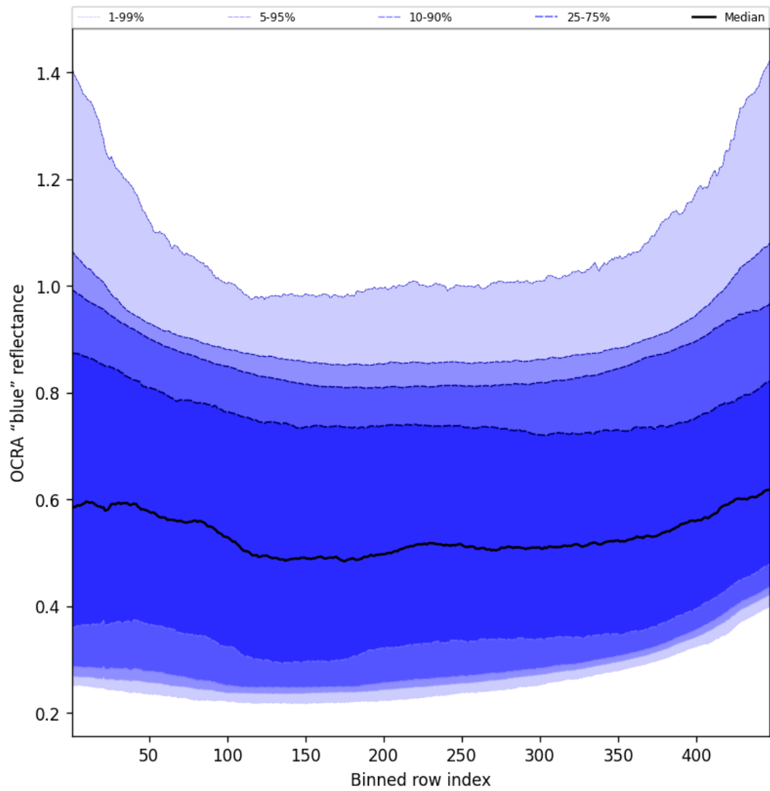
Figure 67: Along track statistics of “OCRA “blue” reflectance” for 2024-10-08 to 2024-10-10
