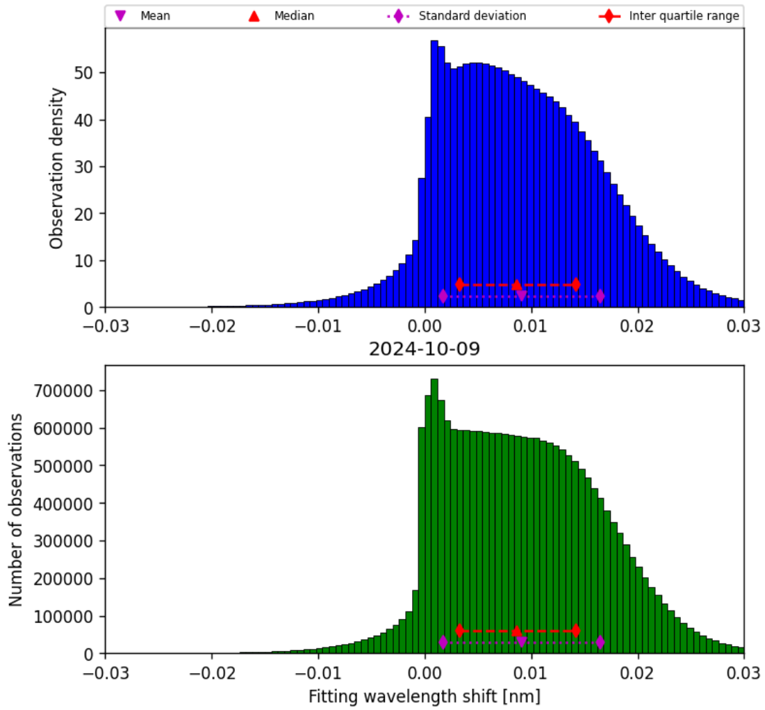
Figure 49: Histogram of “Fitting wavelength shift” for 2024-10-08 to 2024-10-10
