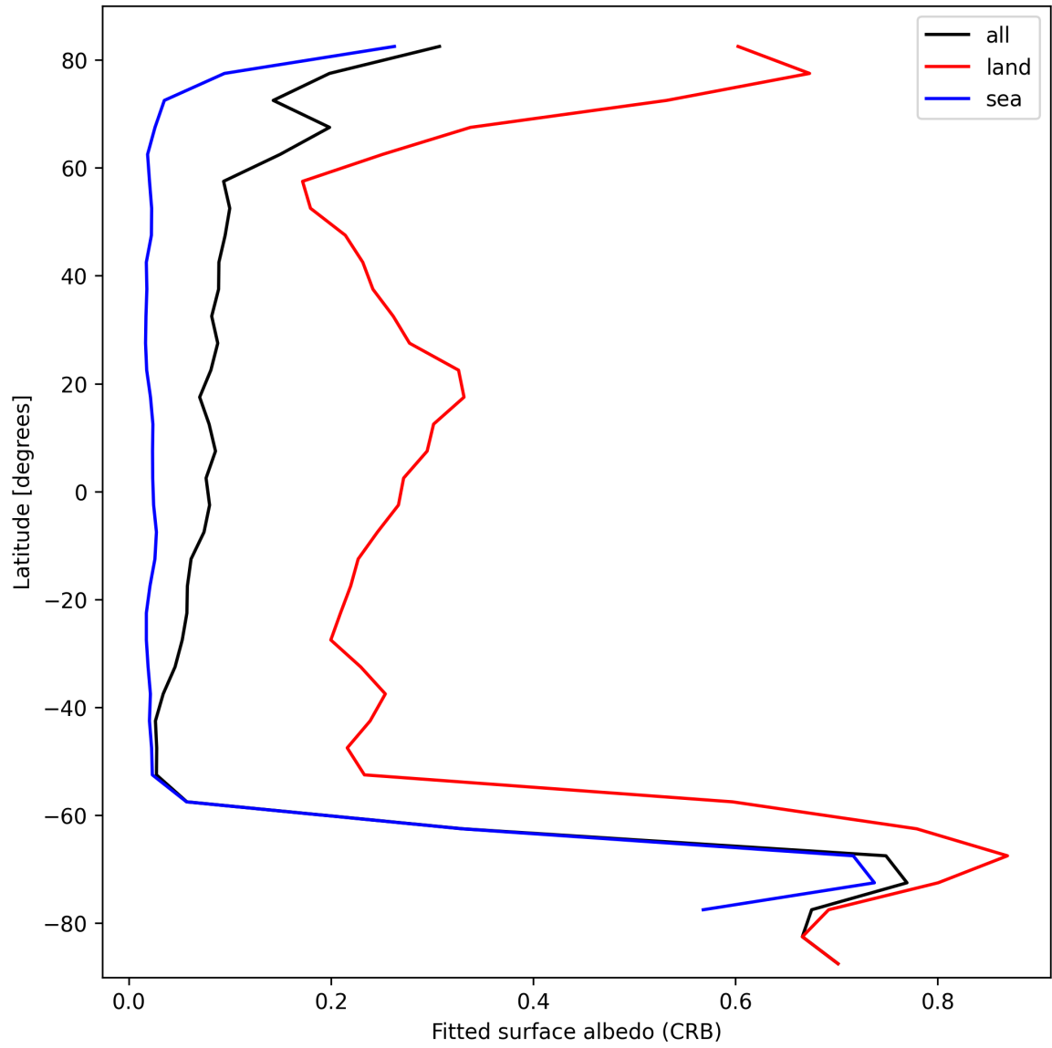
Figure 30: Zonal average of “Fitted surface albedo (CRB)” for 2024-10-08 to 2024-10-10.
