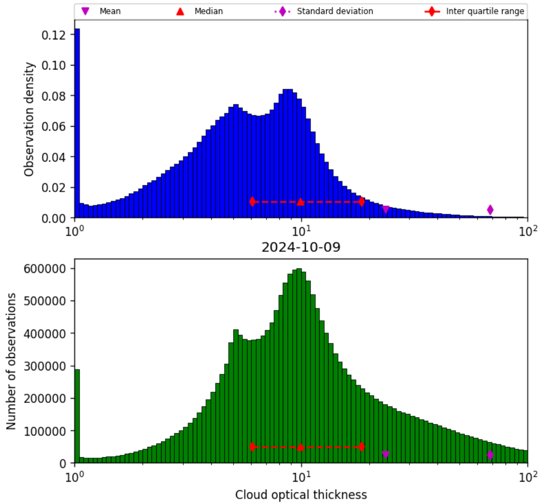
Figure 41: Histogram of “Cloud optical thickness” for 2024-10-08 to 2024-10-10
