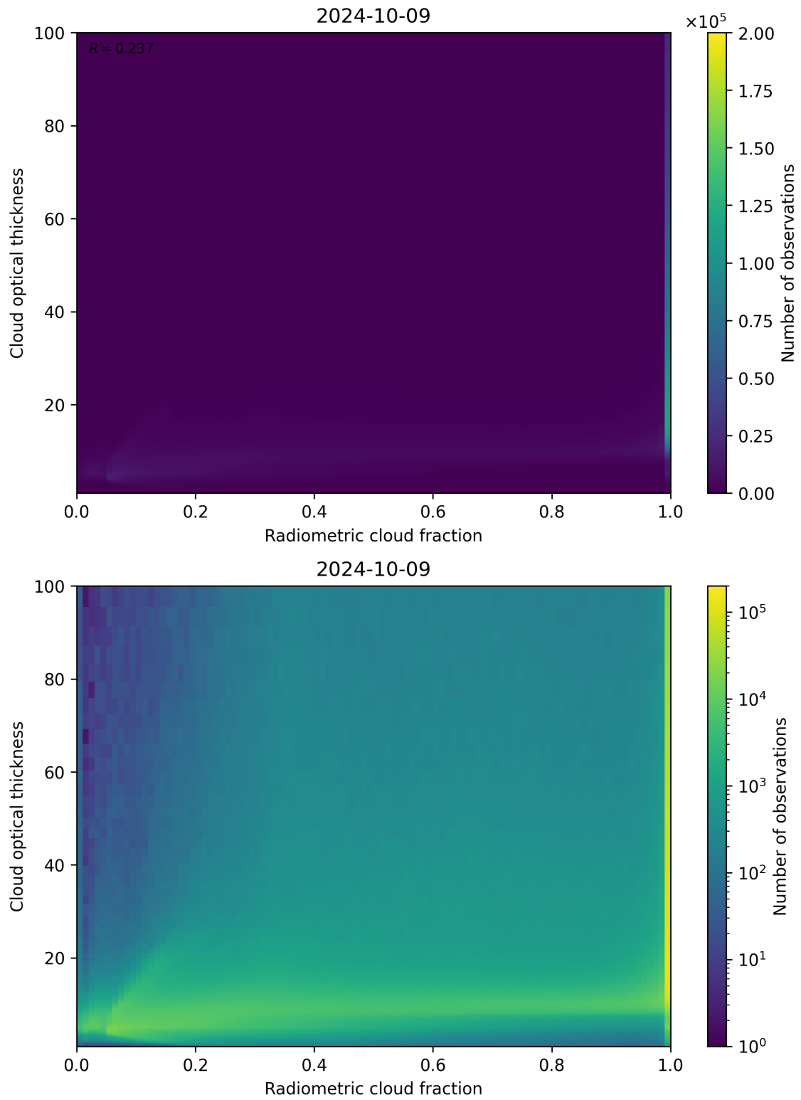
Figure 75: Scatter density plot of “Radiometric cloud fraction” against “Cloud optical thickness” for 2024-10-08 to 2024-10-10.
