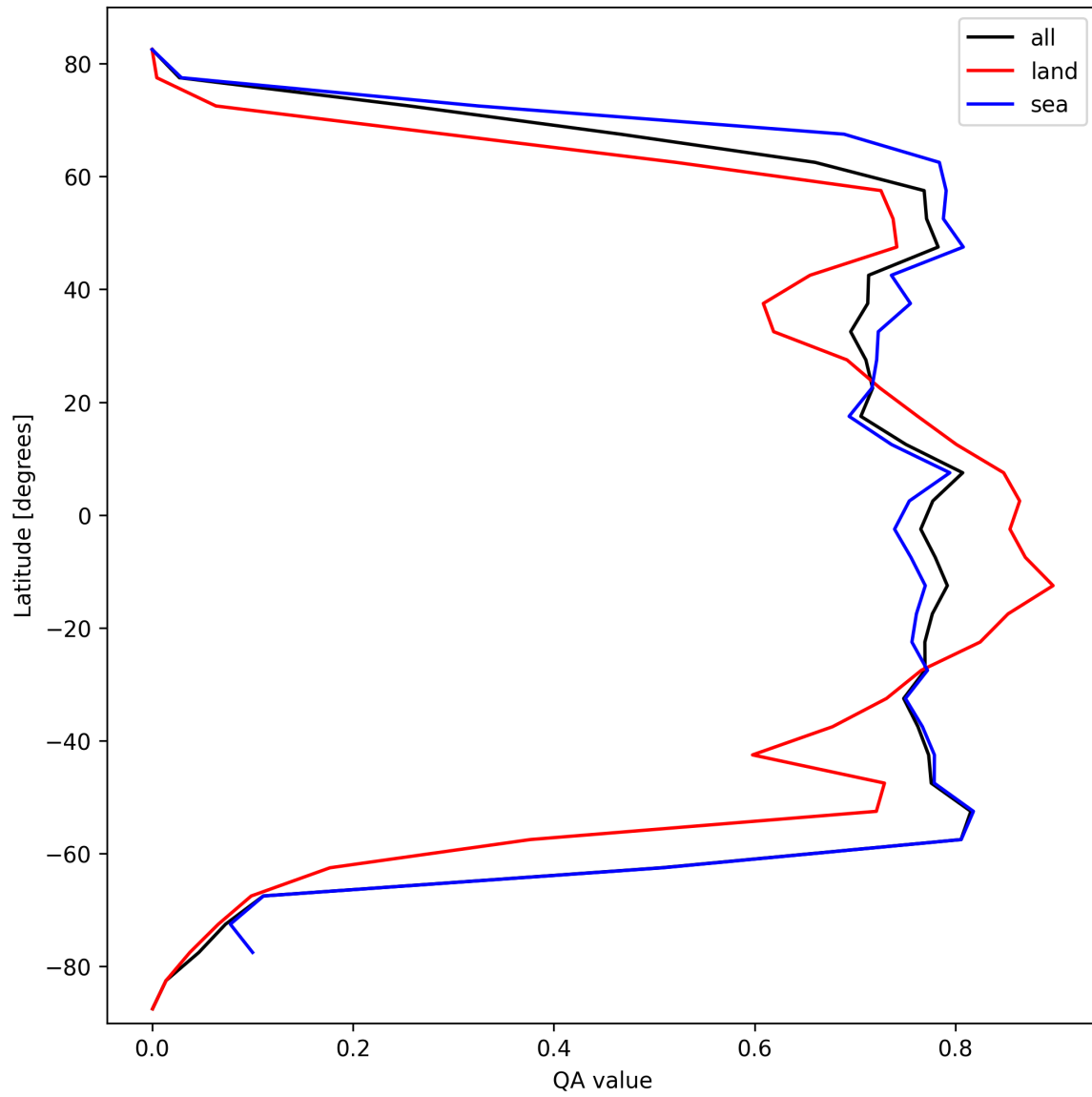
Figure 22: Zonal average of “QA value” for 2024-10-08 to 2024-10-10.
