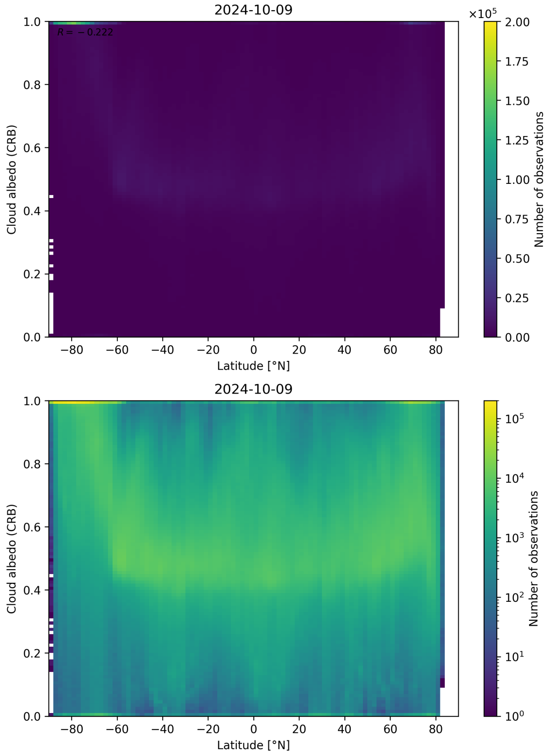
Figure 91: Scatter density plot of “Latitude” against “Cloud albedo (CRB)” for 2024-10-08 to 2024-10-10.
