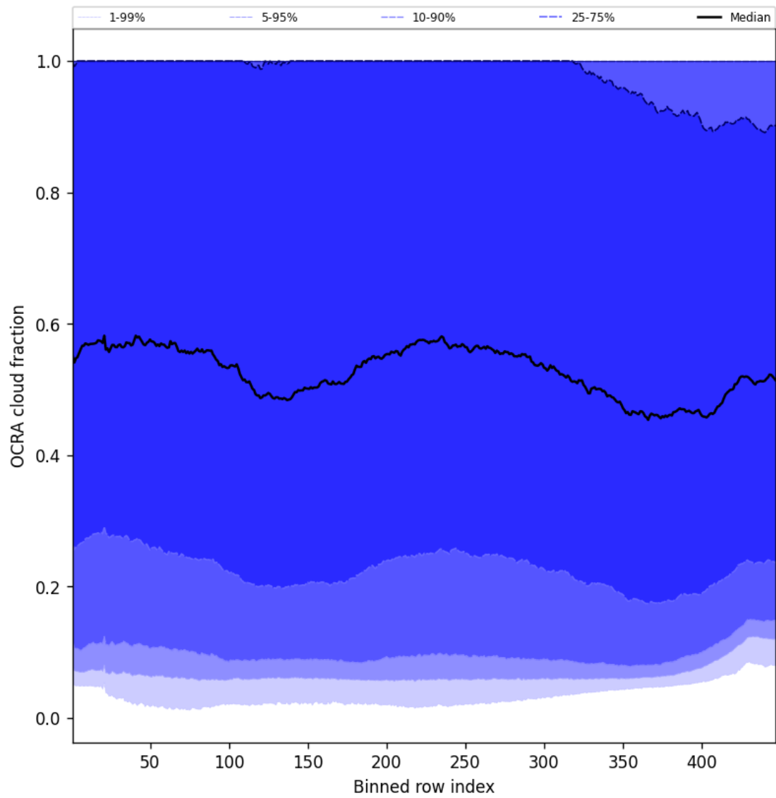
Figure 66: Along track statistics of “OCRA cloud fraction” for 2024-10-08 to 2024-10-10
