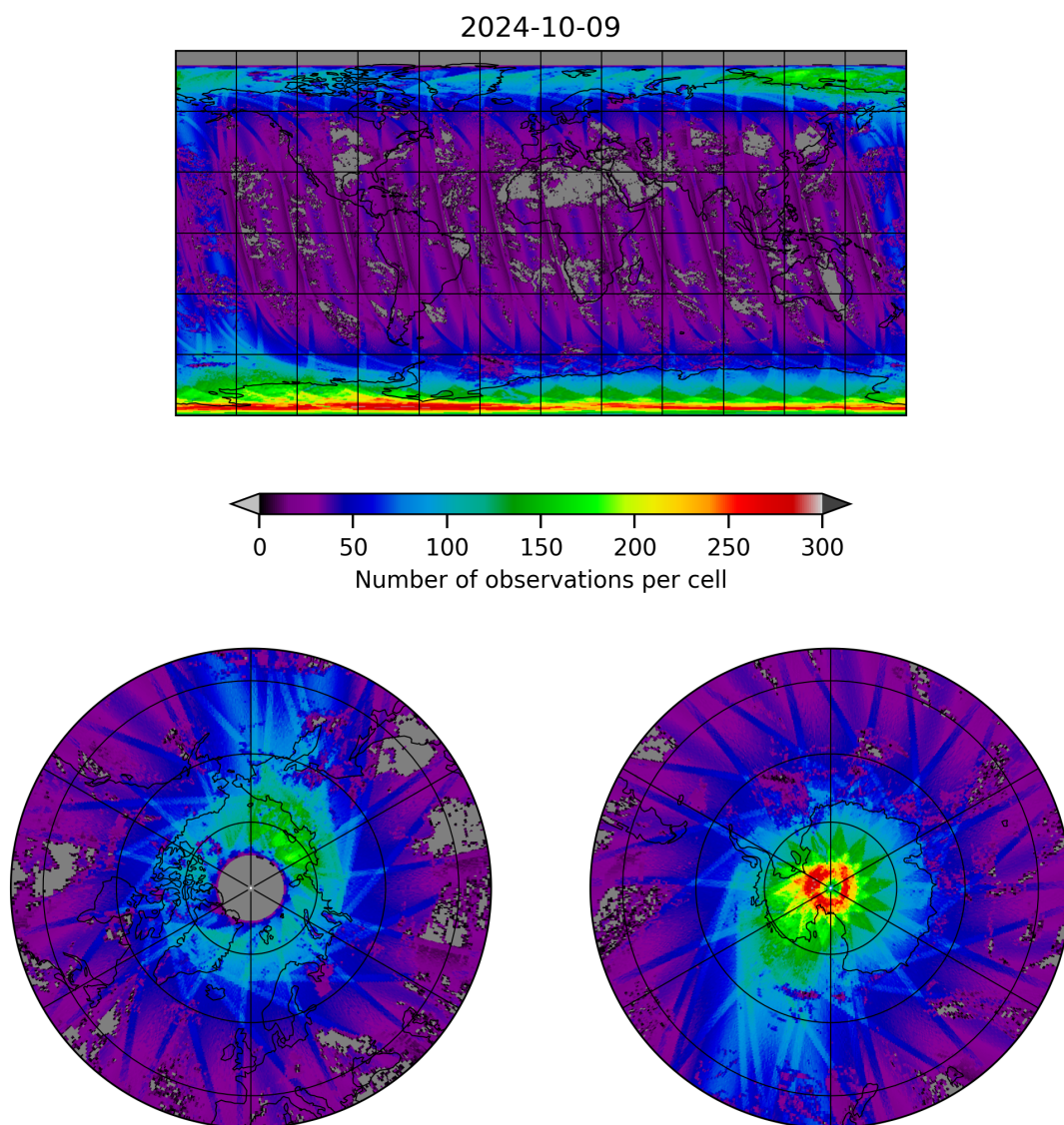
Figure 21: Map of the number of observations for 2024-10-08 to 2024-10-10
