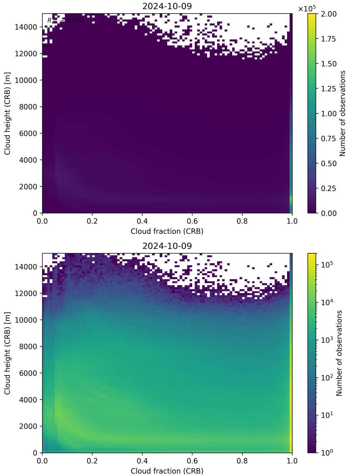
Figure 79: Scatter density plot of “Cloud fraction (CRB)” against “Cloud height (CRB)” for 2024-10-08 to 2024-10-10.
