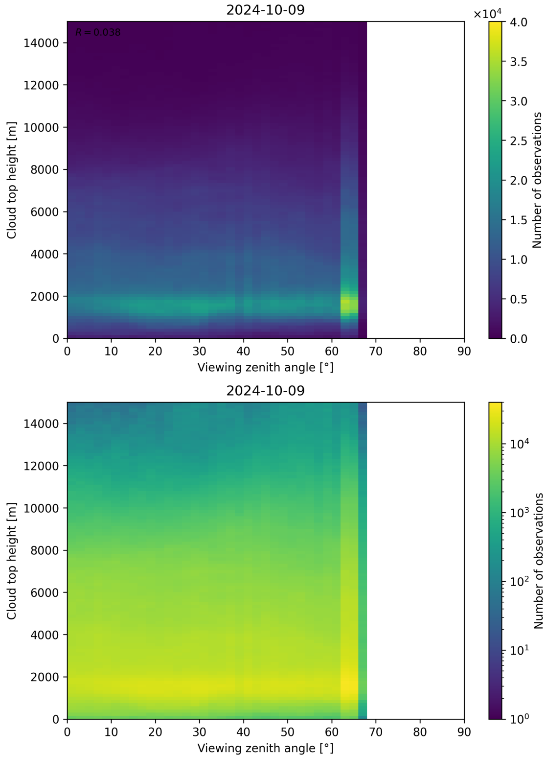
Figure 112: Scatter density plot of “Viewing zenith angle” against “Cloud top height” for 2024-10-08 to 2024-10-10.
