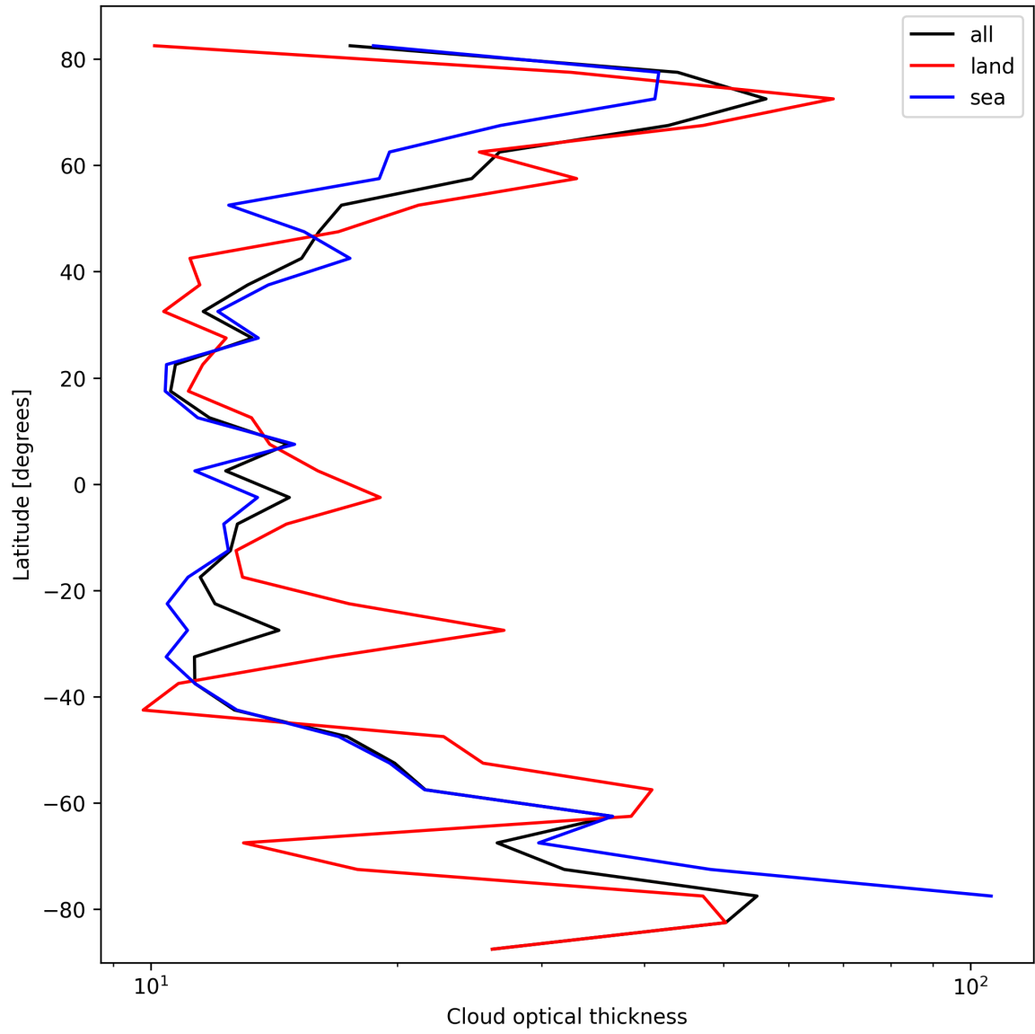
Figure 25: Zonal average of “Cloud optical thickness” for 2024-10-08 to 2024-10-10.
