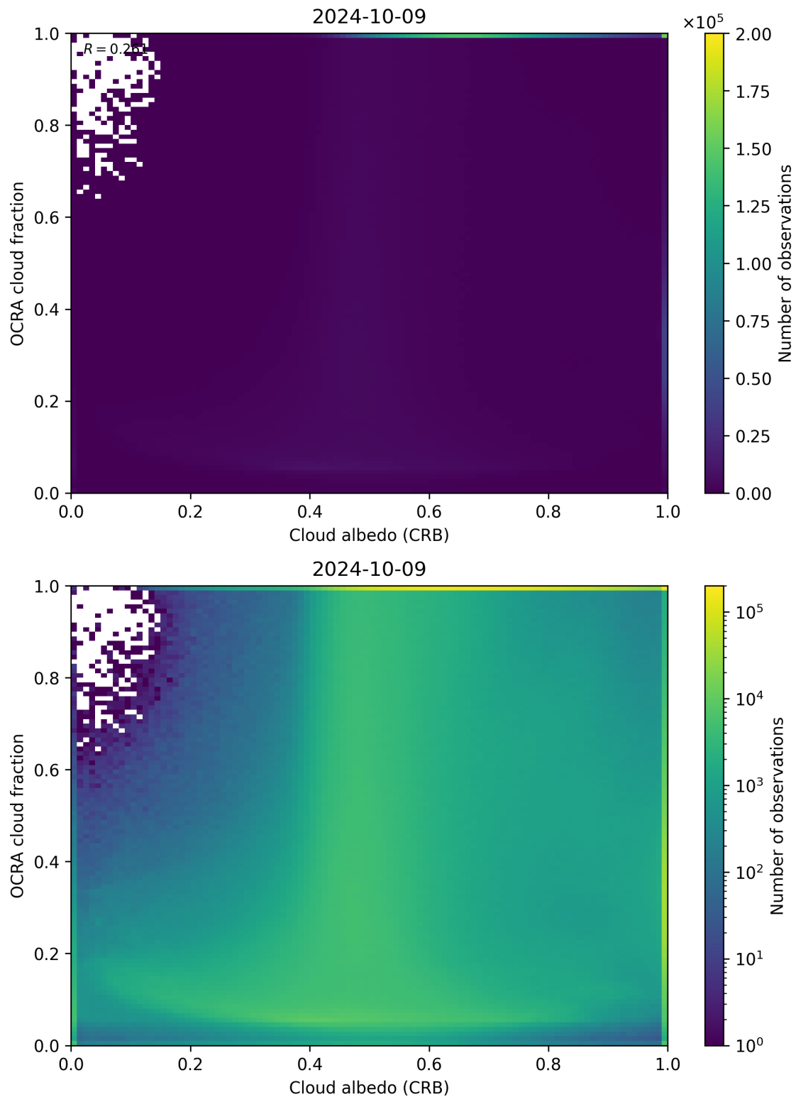
Figure 70: Scatter density plot of “Cloud albedo (CRB)” against “OCRA cloud fraction” for 2024-10-08 to 2024-10-10.
