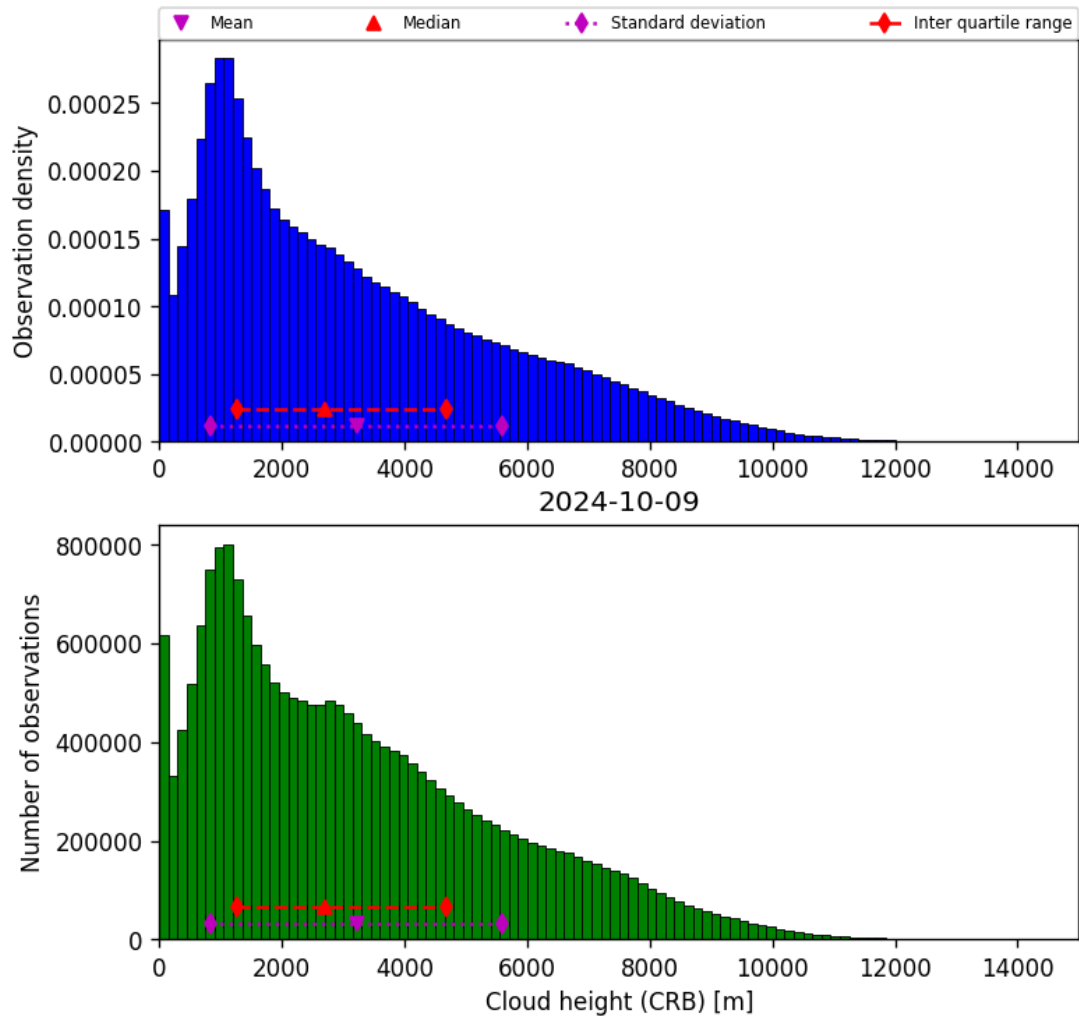
Figure 43: Histogram of “Cloud height (CRB)” for 2024-10-08 to 2024-10-10
