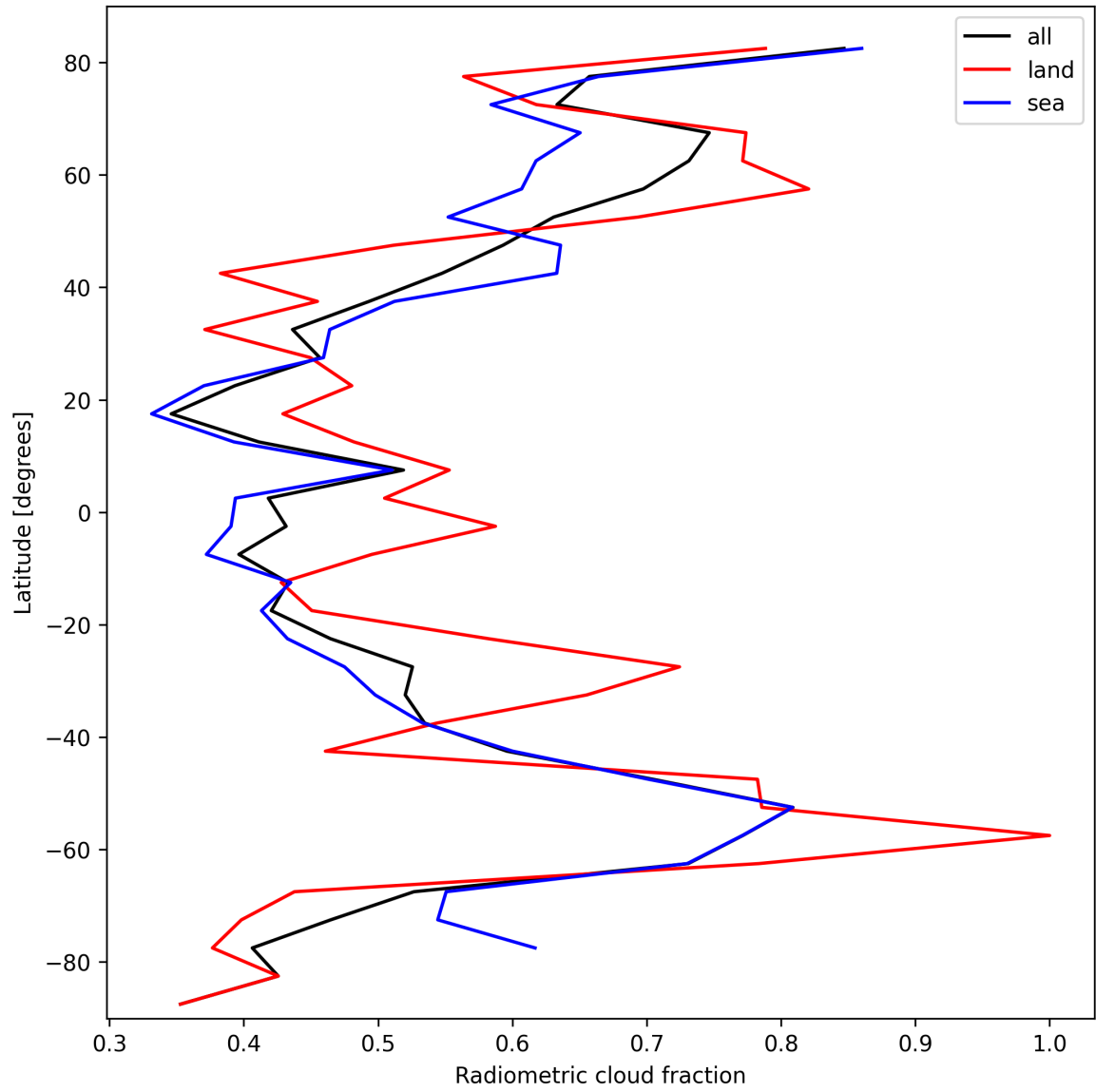
Figure 23: Zonal average of “Radiometric cloud fraction” for 2024-10-08 to 2024-10-10.
