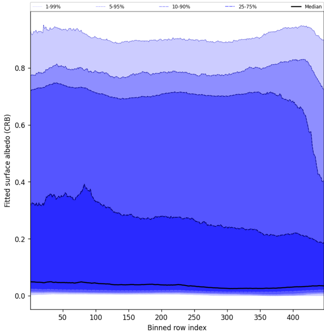
Figure 62: Along track statistics of “Fitted surface albedo (CRB)” for 2024-10-08 to 2024-10-10
