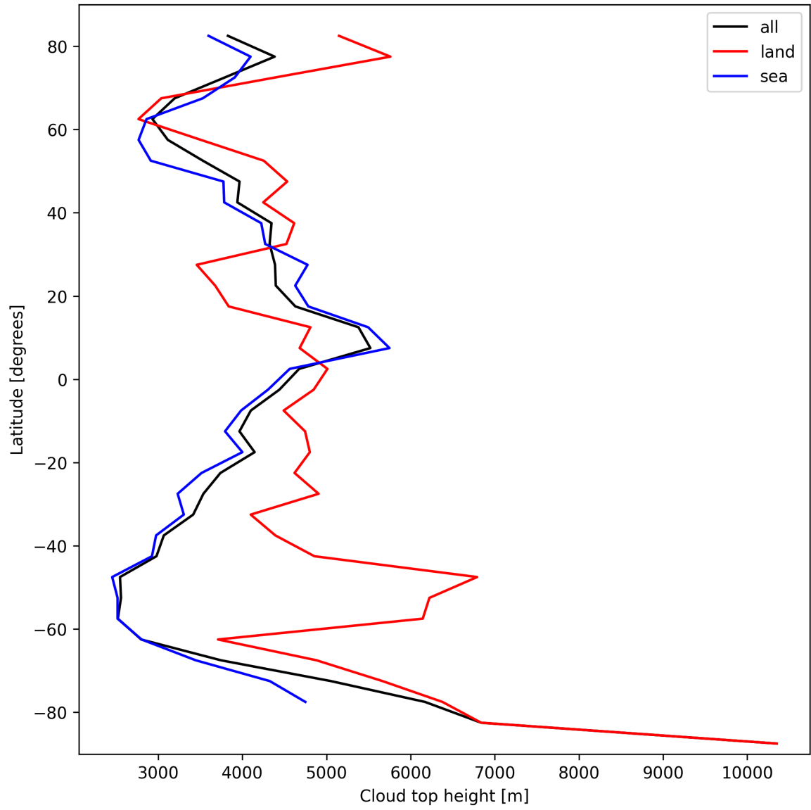
Figure 24: Zonal average of “Cloud top height” for 2024-10-08 to 2024-10-10.
