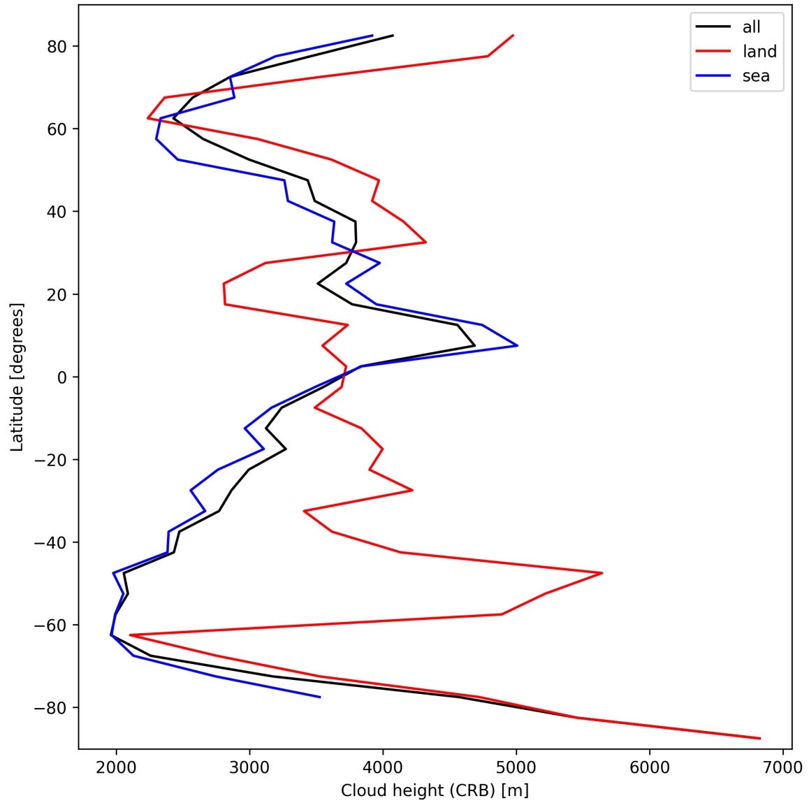
Figure 27: Zonal average of “Cloud height (CRB)” for 2024-10-08 to 2024-10-10.
