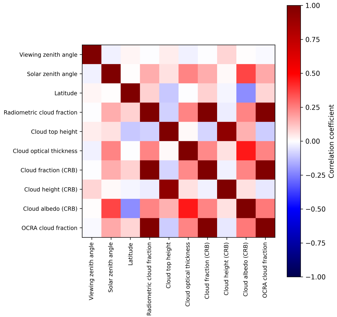
Figure 2: Map of correlation matrix for 2024-10-08 to 2024-10-10.
