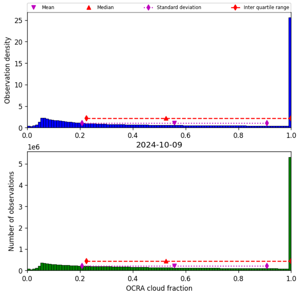
Figure 50: Histogram of “OCRA cloud fraction” for 2024-10-08 to 2024-10-10
