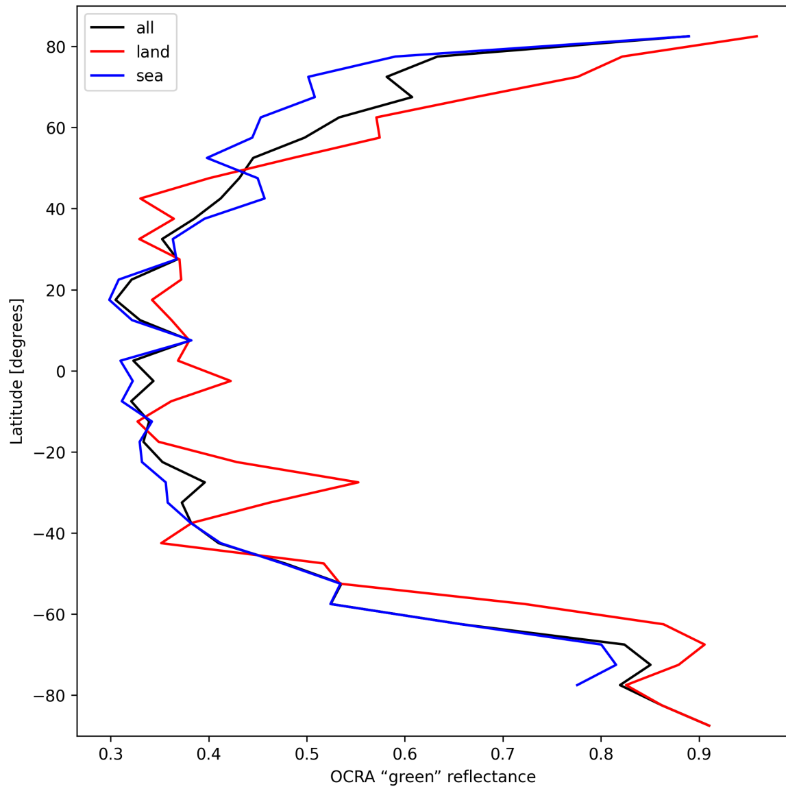
Figure 36: Zonal average of “OCRA “green” reflectance” for 2024-10-08 to 2024-10-10.
