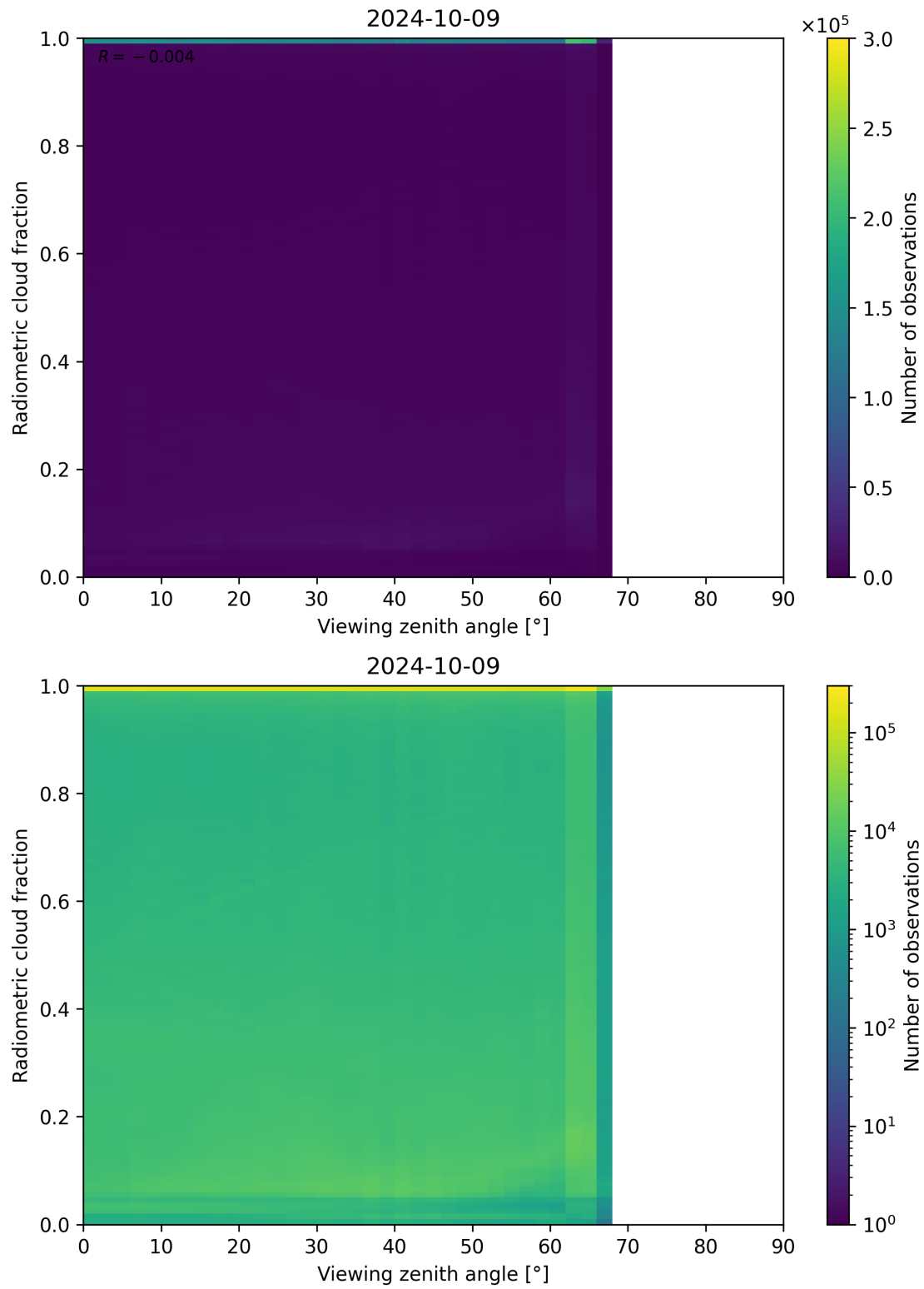
Figure 107: Scatter density plot of “Viewing zenith angle” against “Radiometric cloud fraction” for 2024-10-08 to 2024-10-10.
