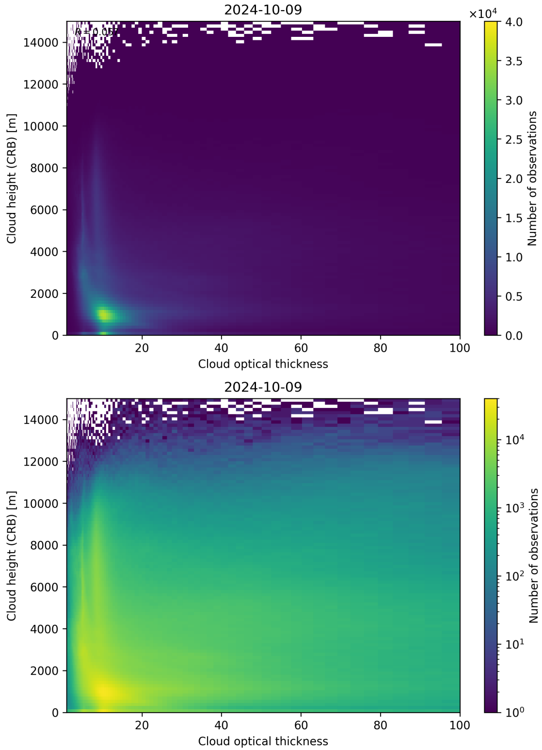
Figure 85: Scatter density plot of “Cloud optical thickness” against “Cloud height (CRB)” for 2024-10-08 to 2024-10-10.
