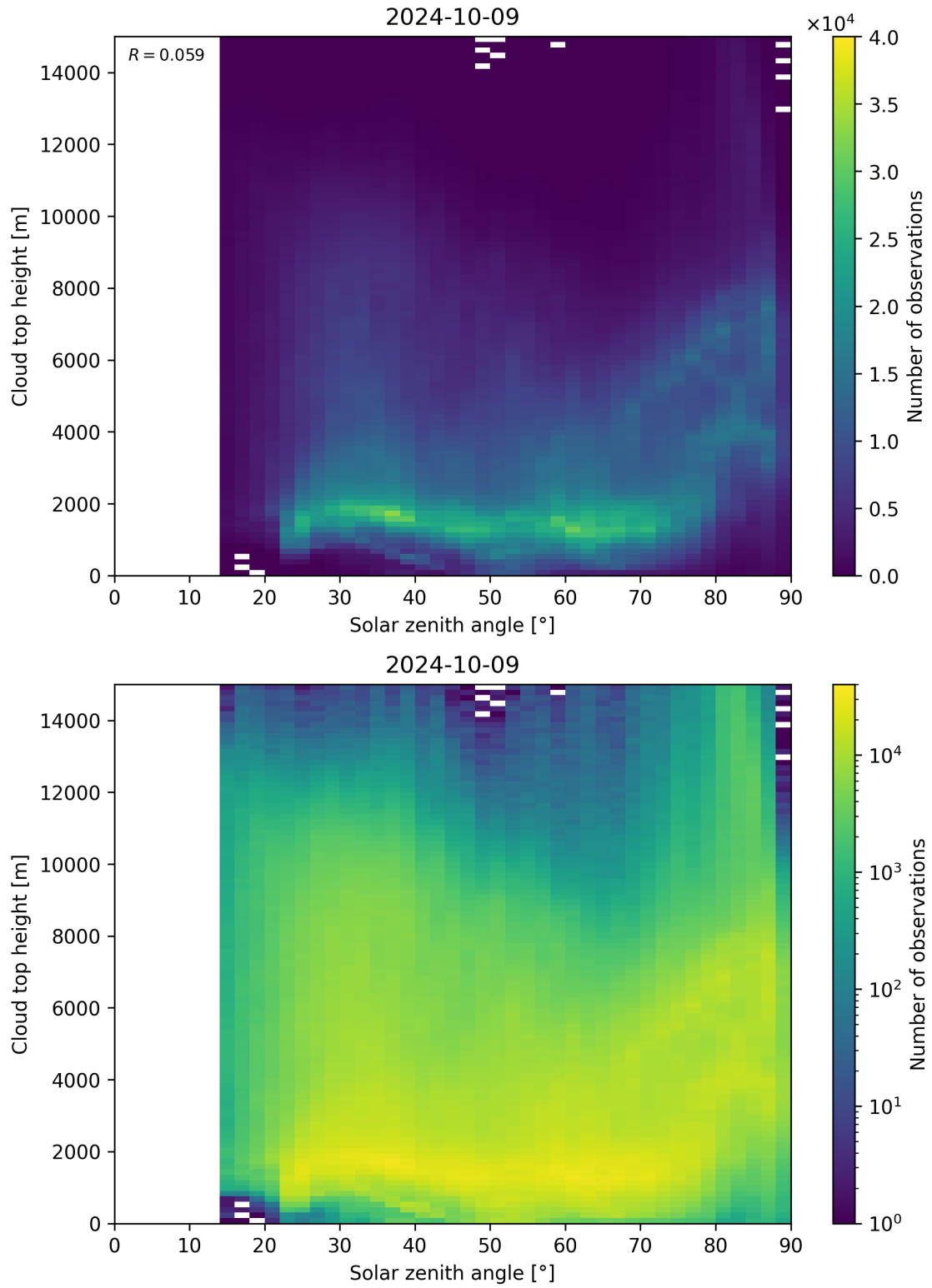
Figure 104: Scatter density plot of “Solar zenith angle” against “Cloud top height” for 2024-10-08 to 2024-10-10.
