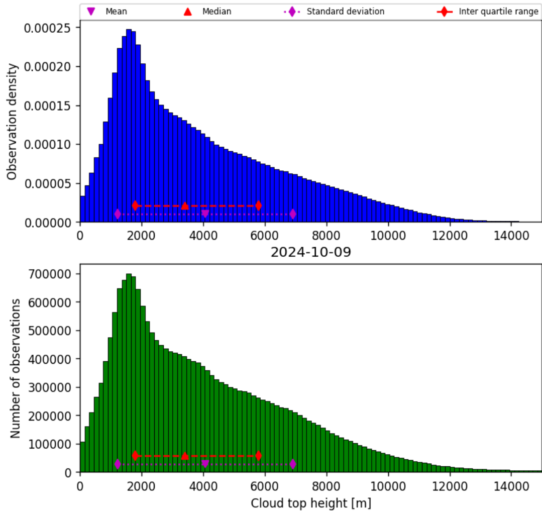
Figure 40: Histogram of “Cloud top height” for 2024-10-08 to 2024-10-10
