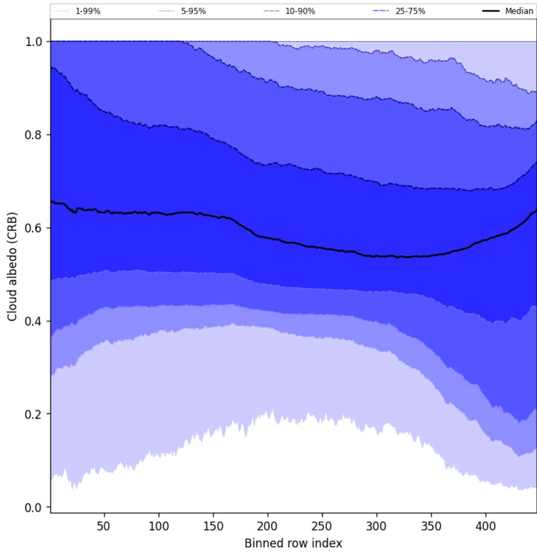
Figure 60: Along track statistics of “Cloud albedo (CRB)” for 2024-10-08 to 2024-10-10
