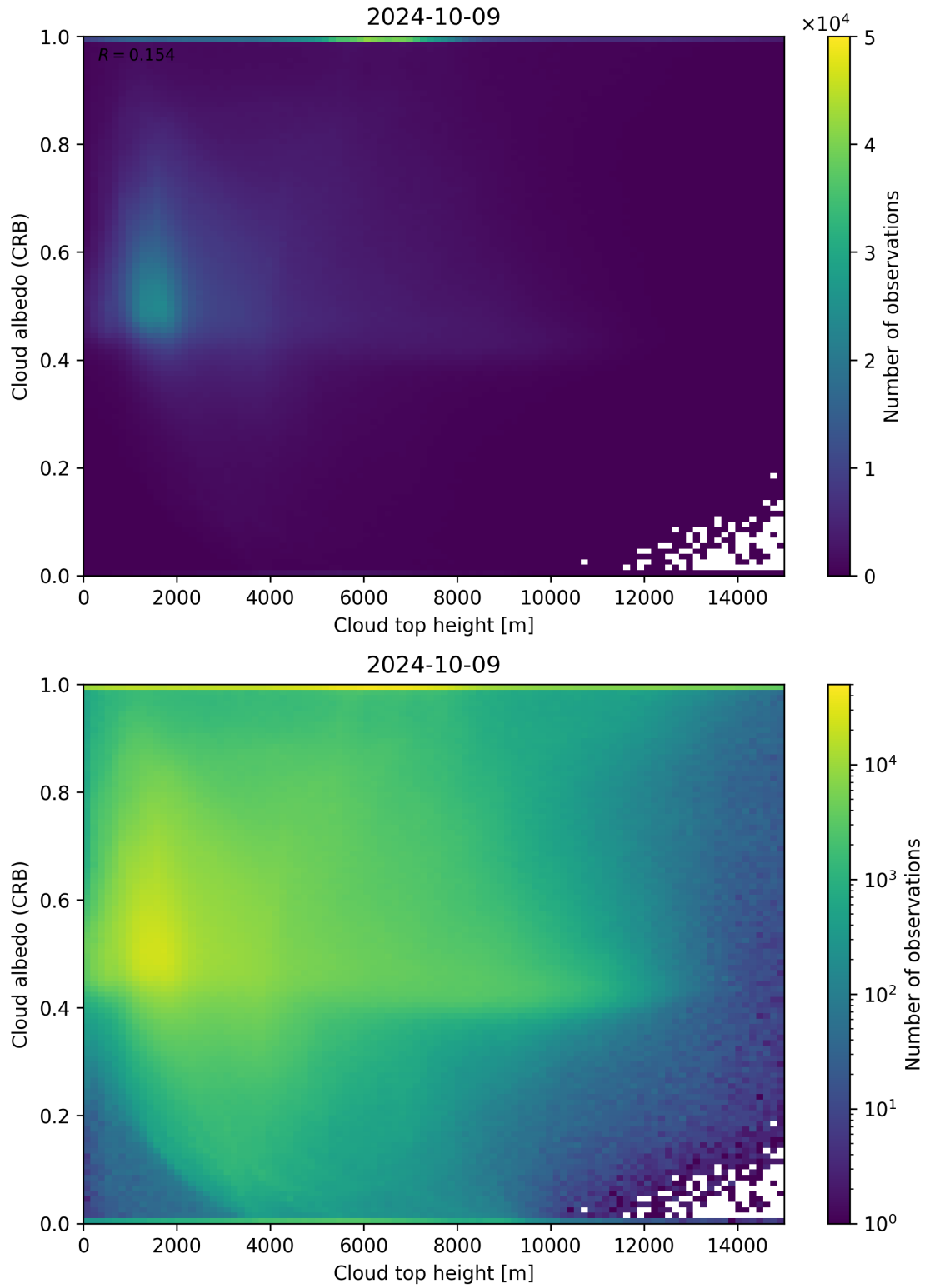
Figure 86: Scatter density plot of “Cloud top height” against “Cloud albedo (CRB)” for 2024-10-08 to 2024-10-10.
