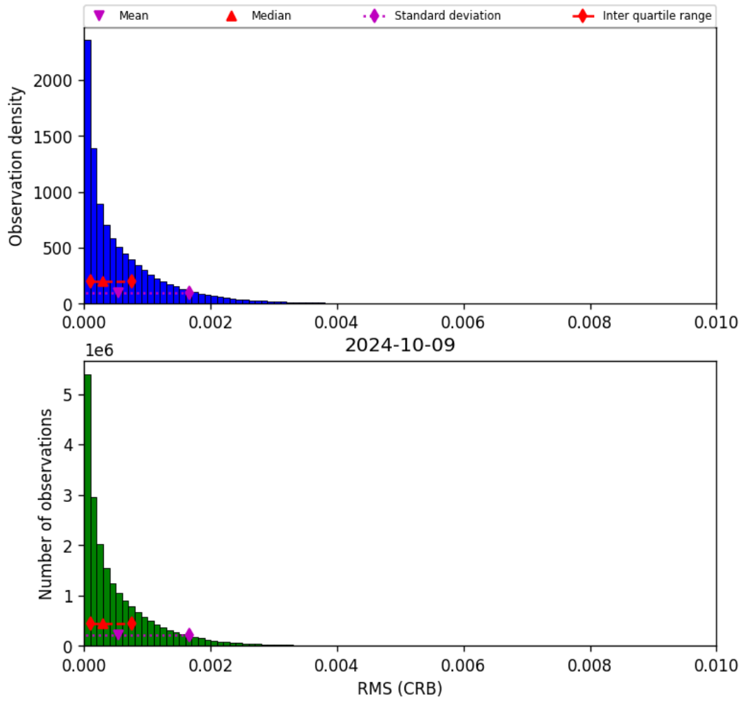
Figure 48: Histogram of “RMS (CRB)” for 2024-10-08 to 2024-10-10
