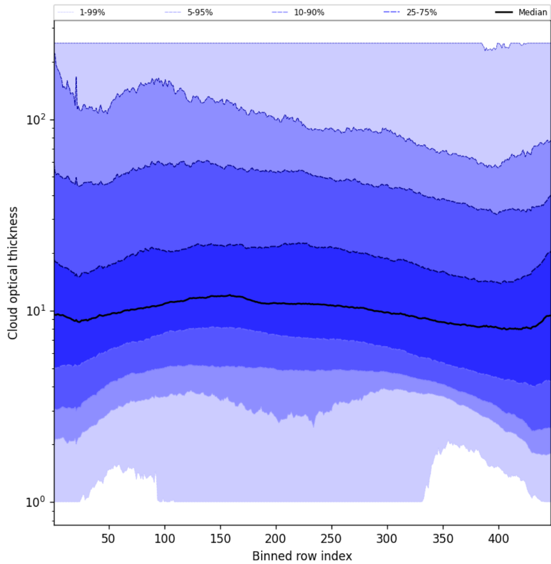
Figure 57: Along track statistics of “Cloud optical thickness” for 2024-10-08 to 2024-10-10
