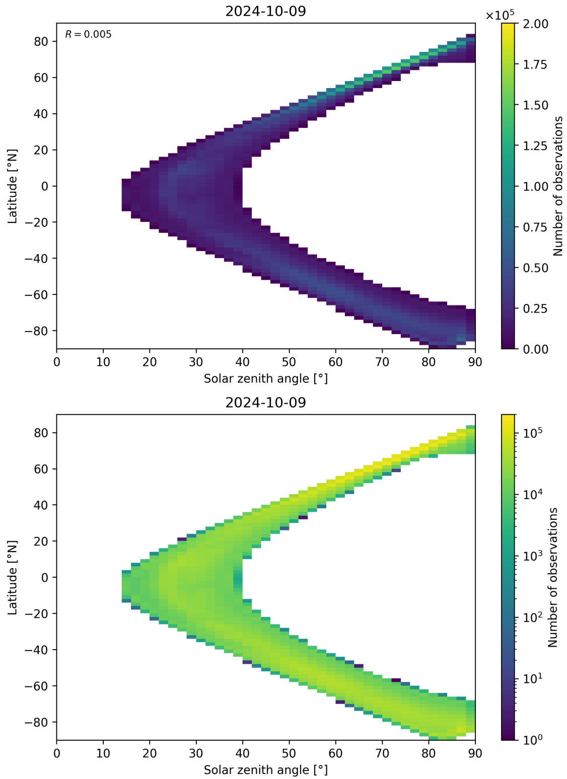
Figure 105: Scatter density plot of “Solar zenith angle” against “Latitude” for 2024-10-08 to 2024-10-10.
