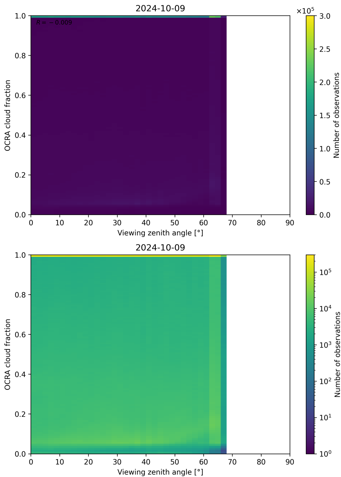
Figure 108: Scatter density plot of “Viewing zenith angle” against “OCRA cloud fraction” for 2024-10-08 to 2024-10-10.
