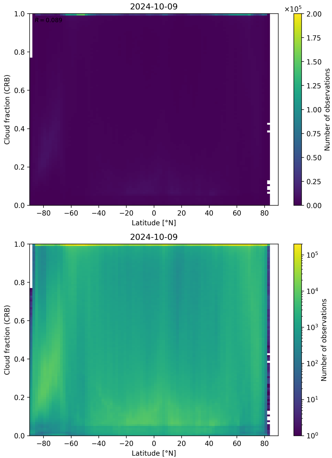
Figure 94: Scatter density plot of “Latitude” against “Cloud fraction (CRB)” for 2024-10-08 to 2024-10-10.
