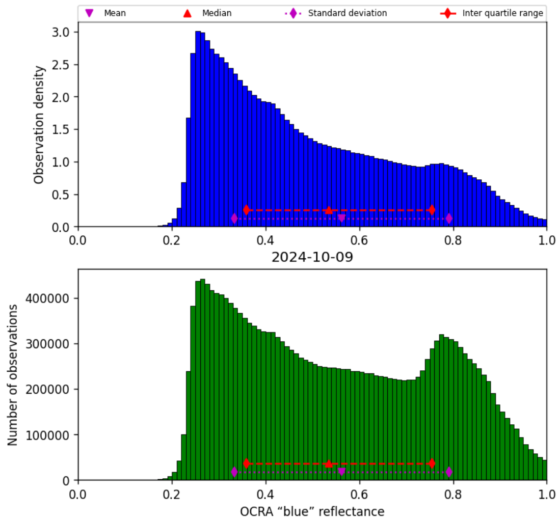
Figure 51: Histogram of “OCRA “blue” reflectance” for 2024-10-08 to 2024-10-10
