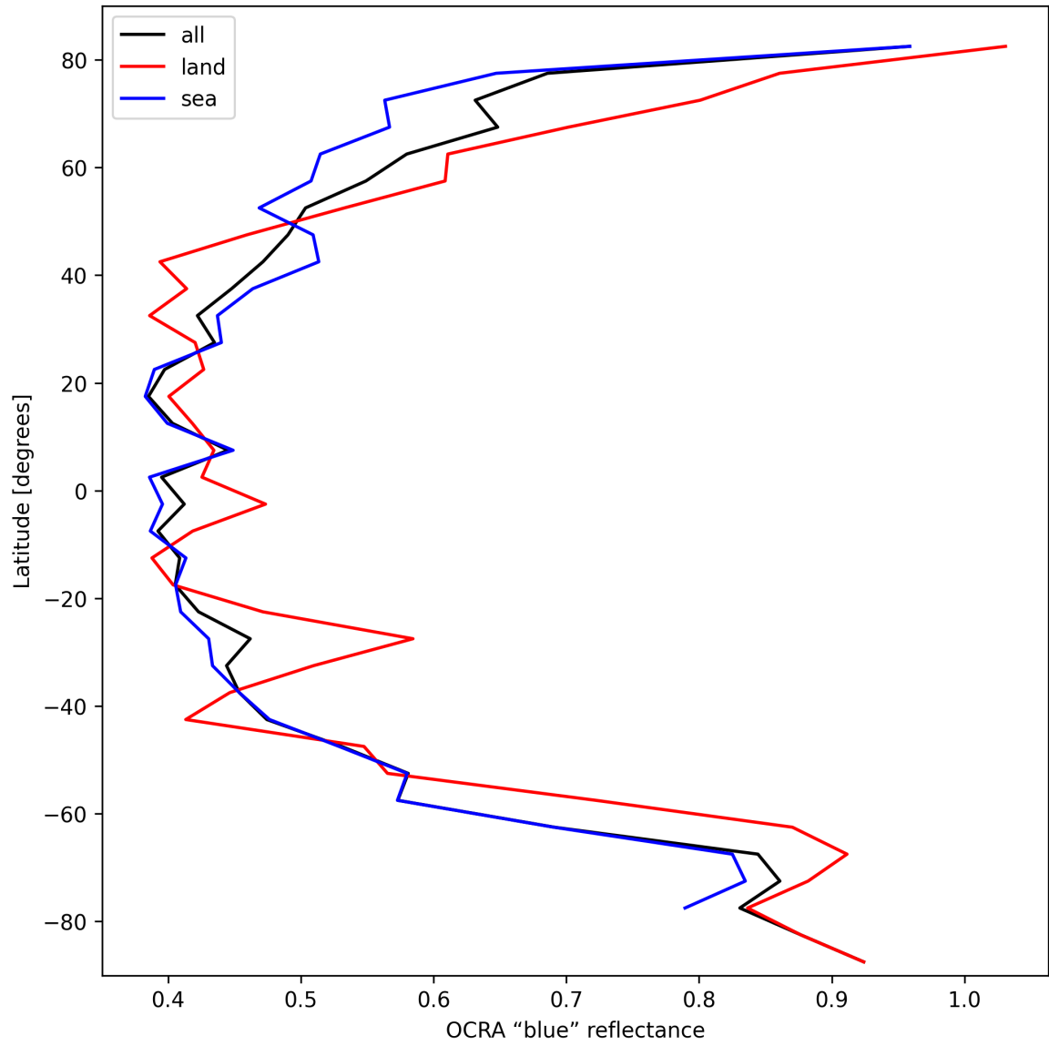
Figure 35: Zonal average of “OCRA “blue” reflectance” for 2024-10-08 to 2024-10-10.
