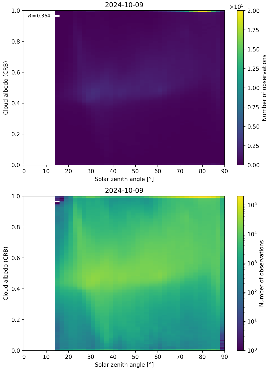
Figure 98: Scatter density plot of “Solar zenith angle” against “Cloud albedo (CRB)” for 2024-10-08 to 2024-10-10.
