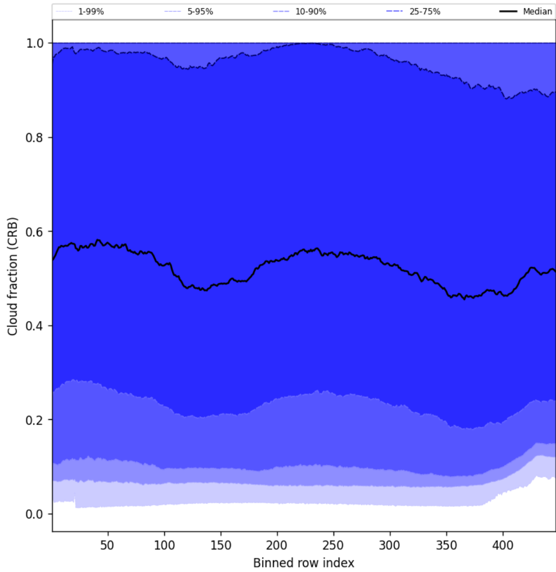
Figure 58: Along track statistics of “Cloud fraction (CRB)” for 2024-10-08 to 2024-10-10
