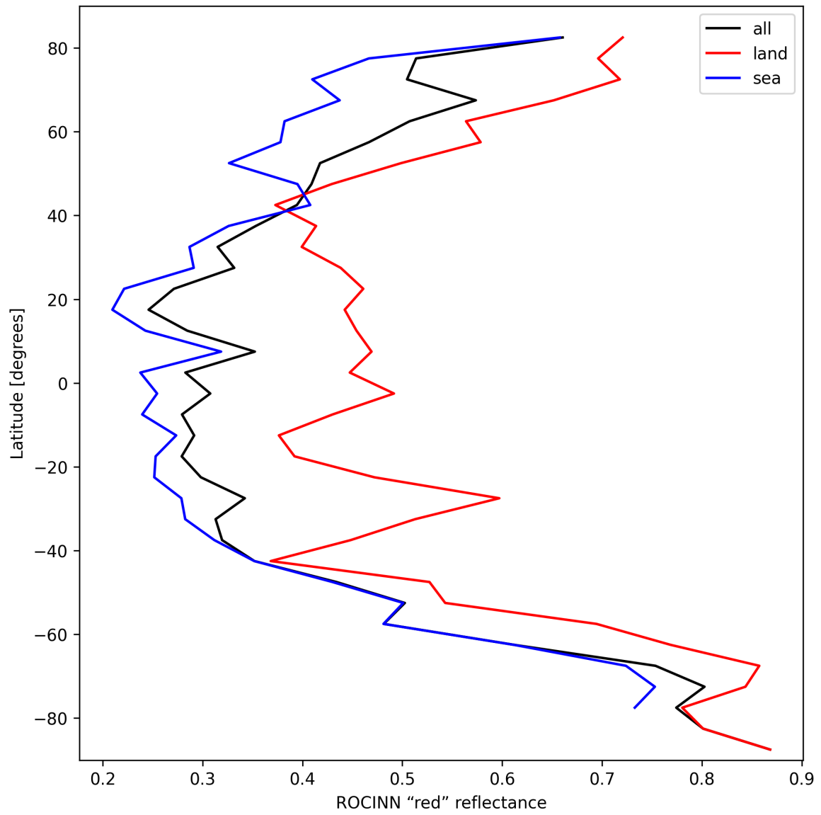
Figure 37: Zonal average of “ROCINN “red” reflectance” for 2024-10-08 to 2024-10-10.
