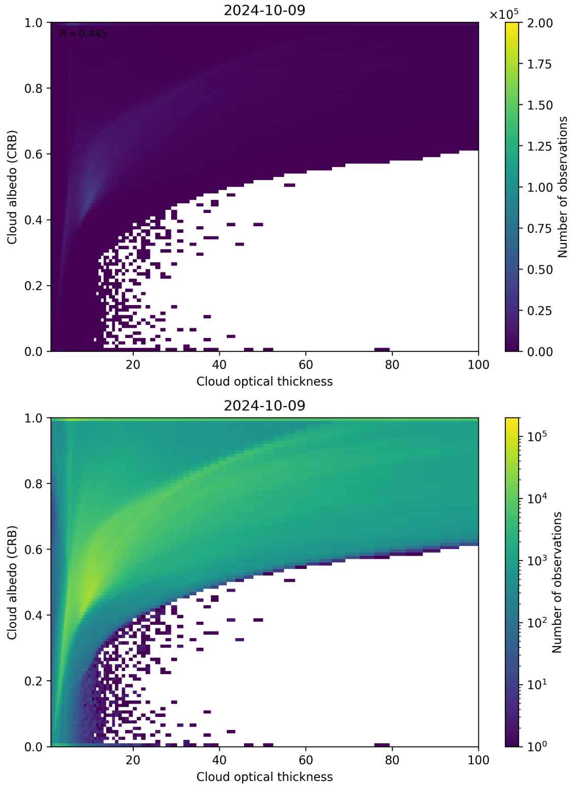
Figure 82: Scatter density plot of “Cloud optical thickness” against “Cloud albedo (CRB)” for 2024-10-08 to 2024-10-10.
