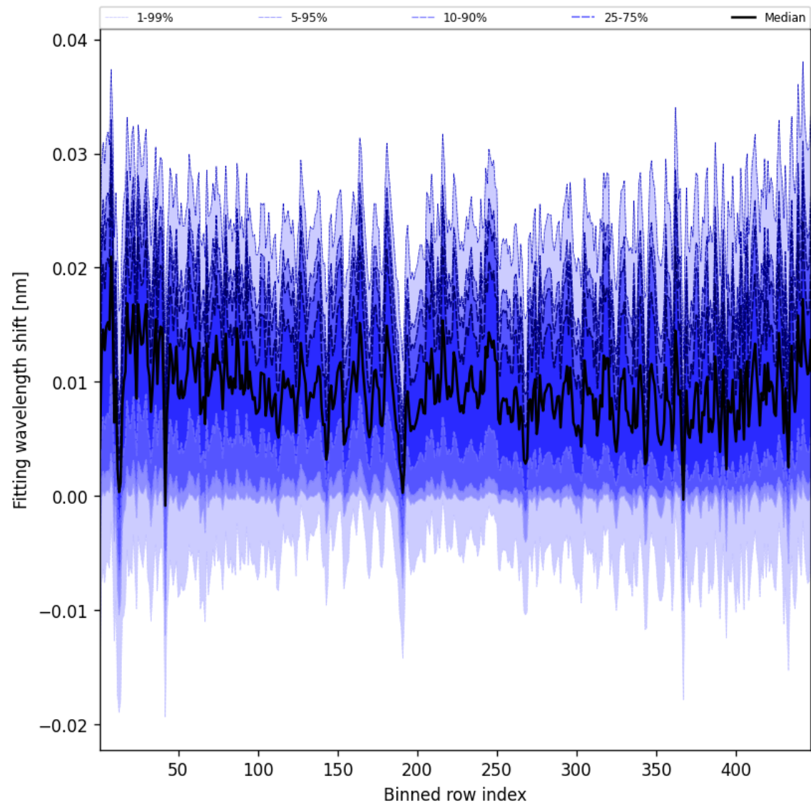
Figure 65: Along track statistics of “Fitting wavelength shift” for 2024-10-08 to 2024-10-10
