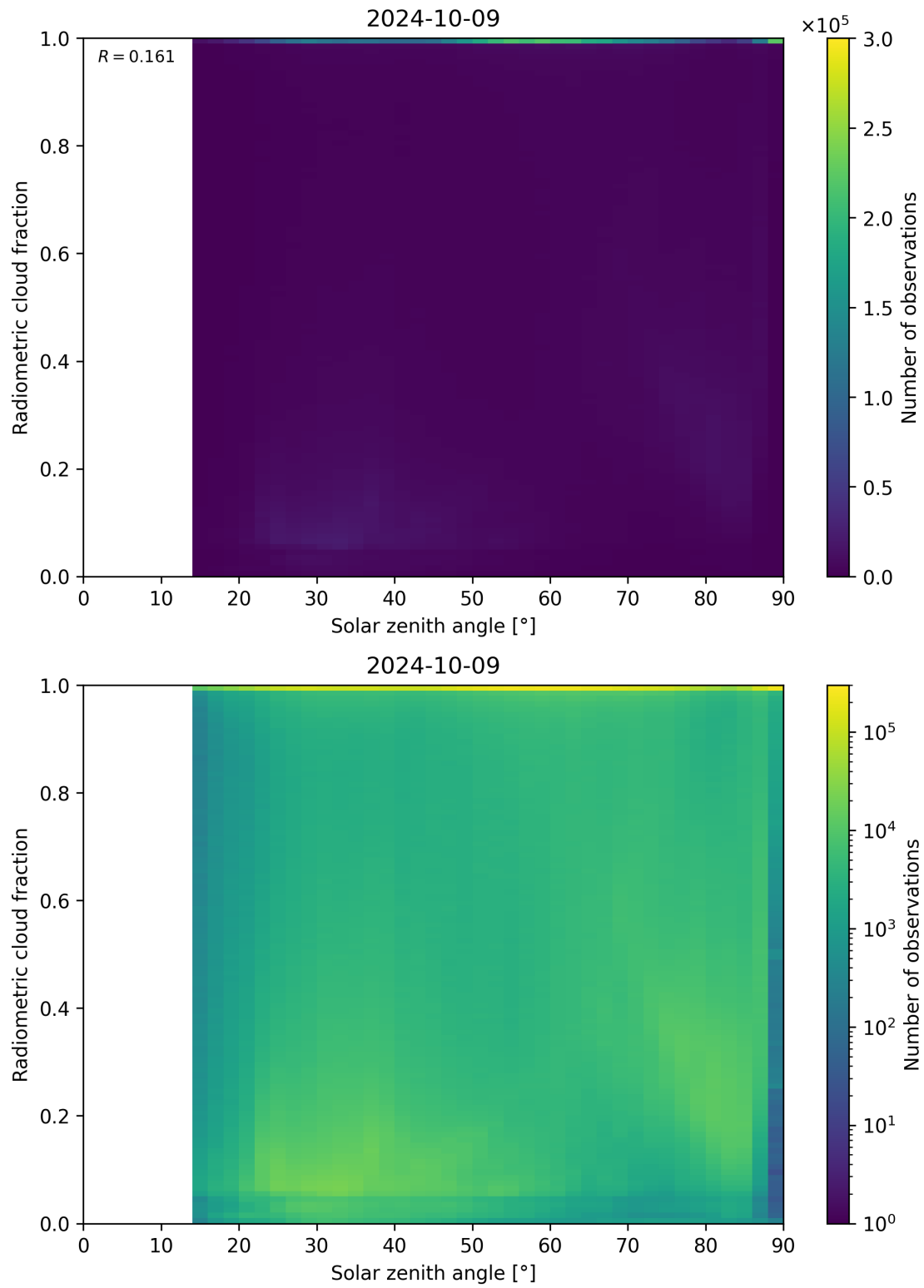
Figure 99: Scatter density plot of “Solar zenith angle” against “Radiometric cloud fraction” for 2024-10-08 to 2024-10-10.
