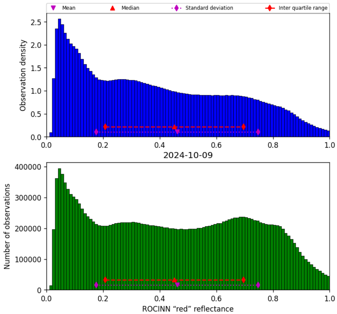
Figure 53: Histogram of “ROCINN “red” reflectance” for 2024-10-08 to 2024-10-10
