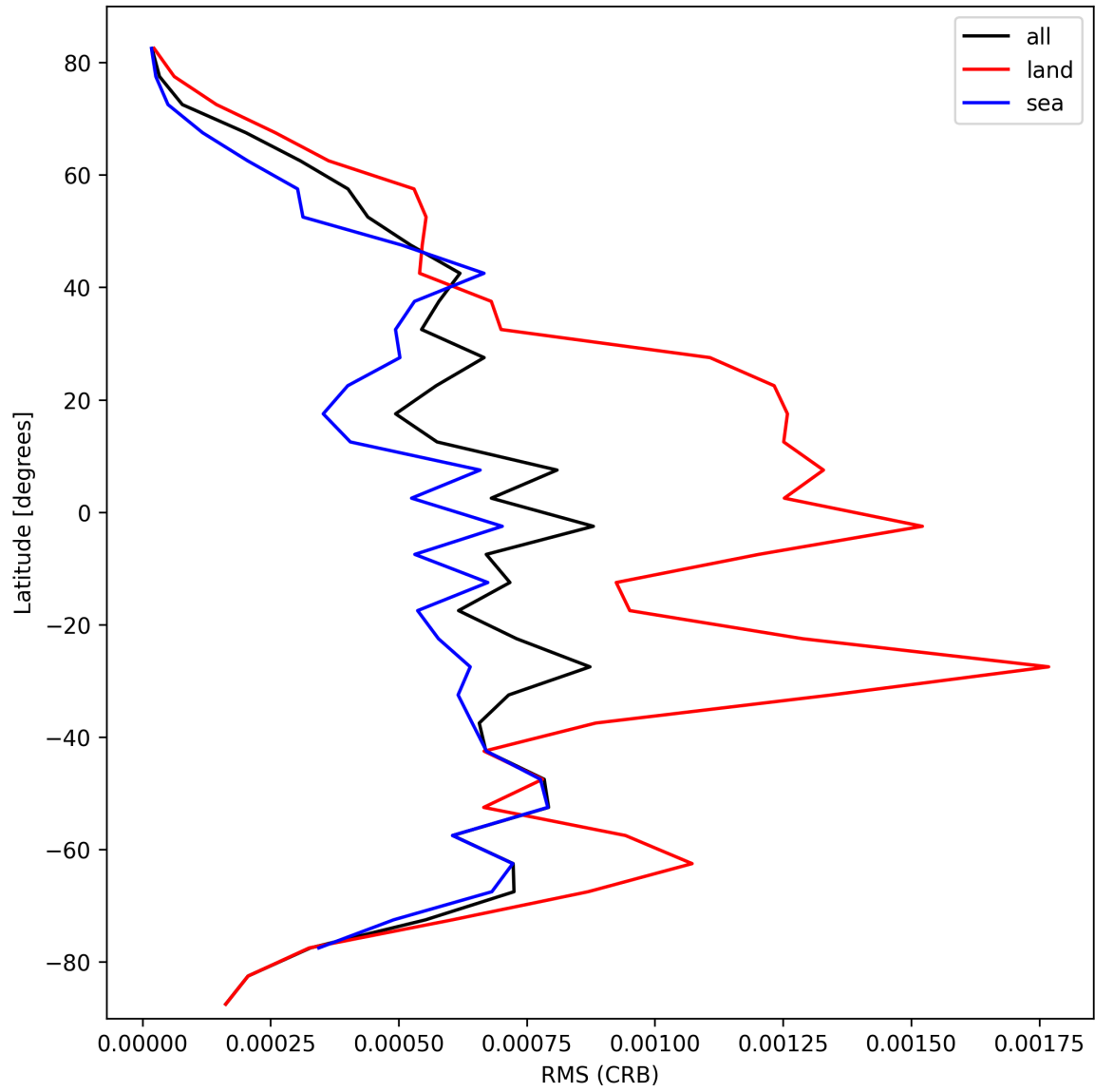
Figure 32: Zonal average of “RMS (CRB)” for 2024-10-08 to 2024-10-10.
