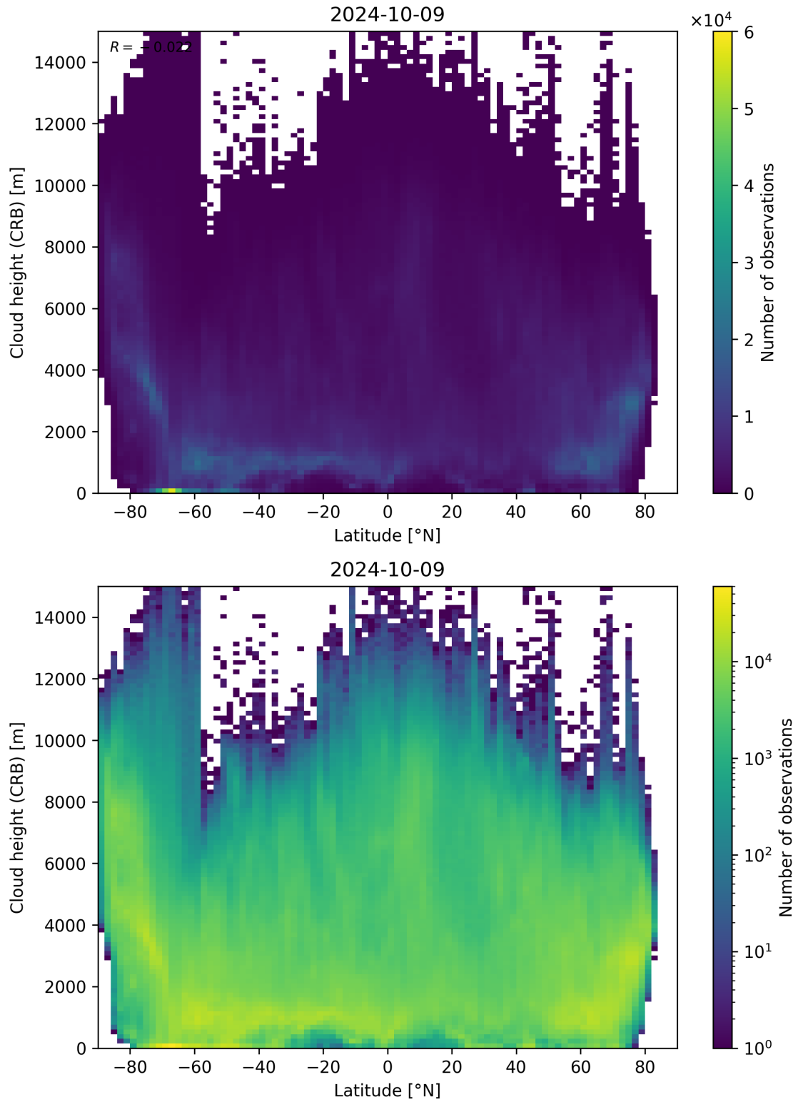
Figure 95: Scatter density plot of “Latitude” against “Cloud height (CRB)” for 2024-10-08 to 2024-10-10.
