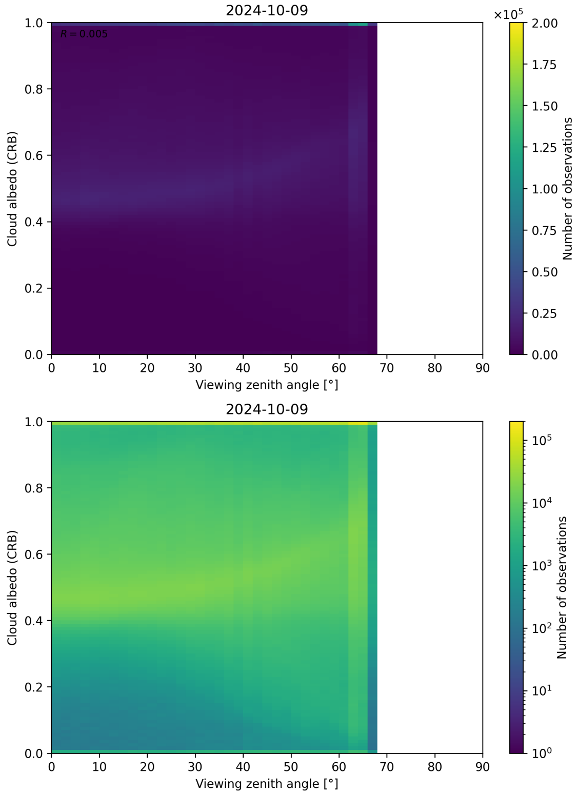
Figure 106: Scatter density plot of “Viewing zenith angle” against “Cloud albedo (CRB)” for 2024-10-08 to 2024-10-10.
