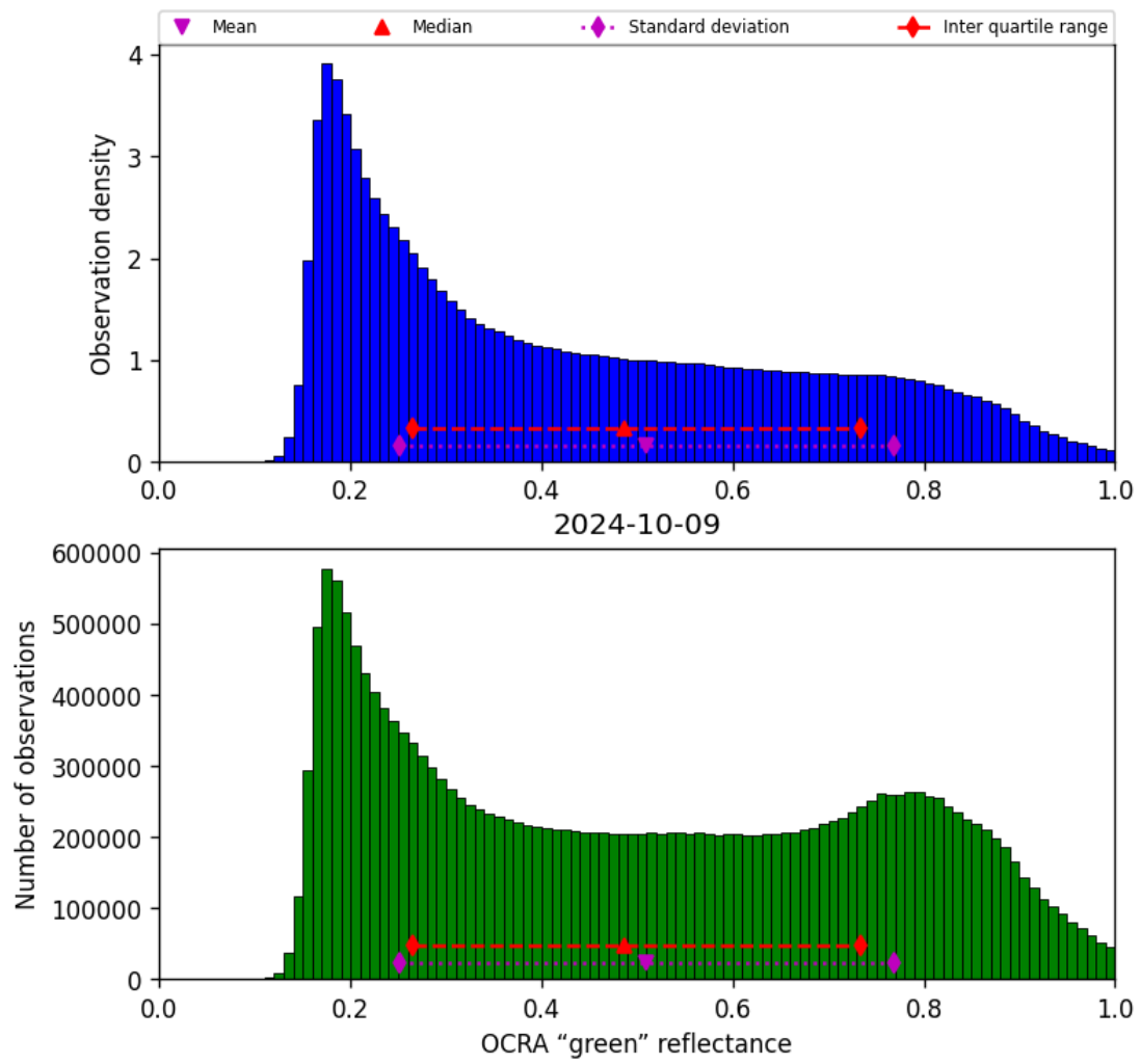
Figure 52: Histogram of “OCRA “green” reflectance” for 2024-10-08 to 2024-10-10
