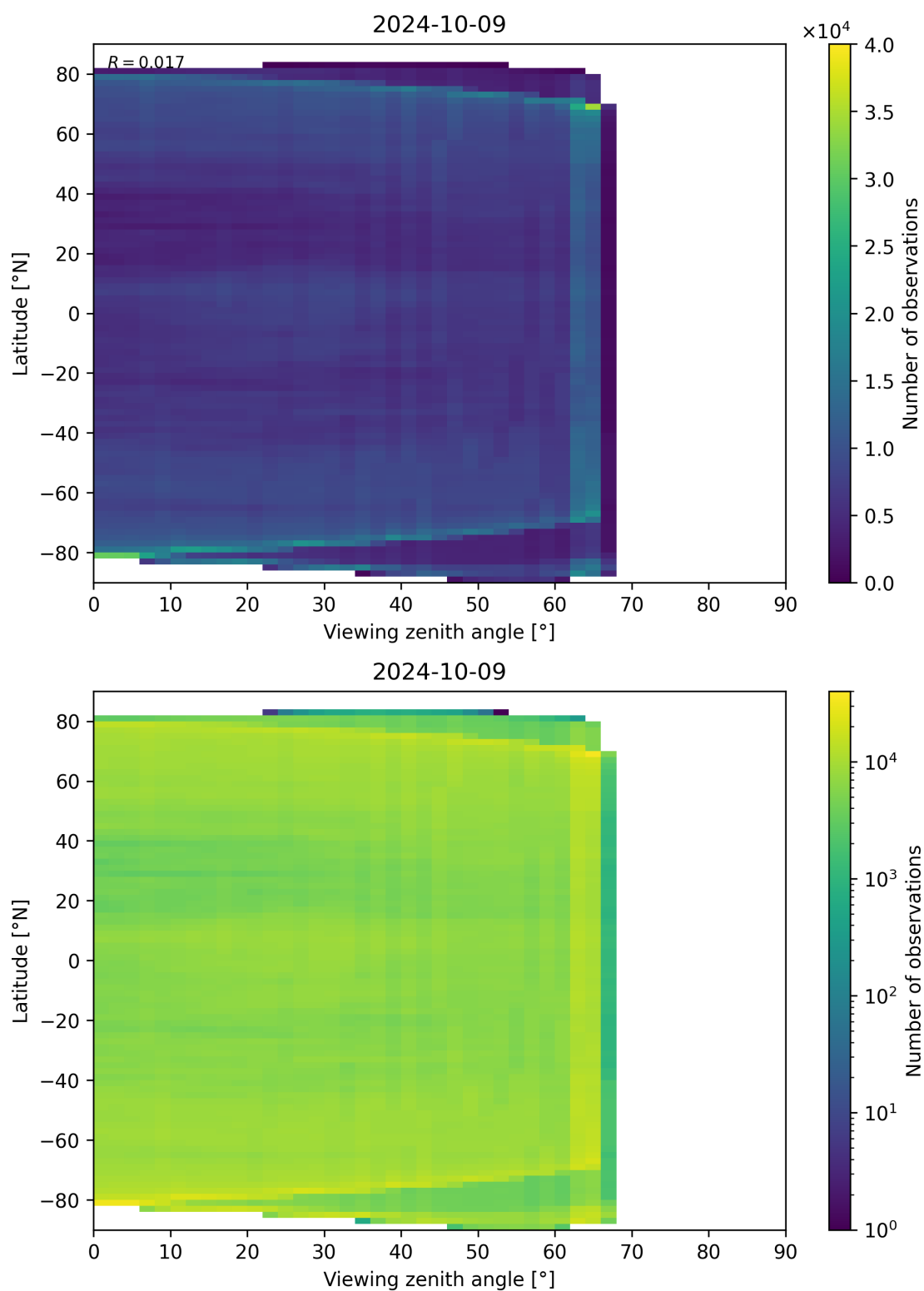
Figure 113: Scatter density plot of “Viewing zenith angle” against “Latitude” for 2024-10-08 to 2024-10-10.
