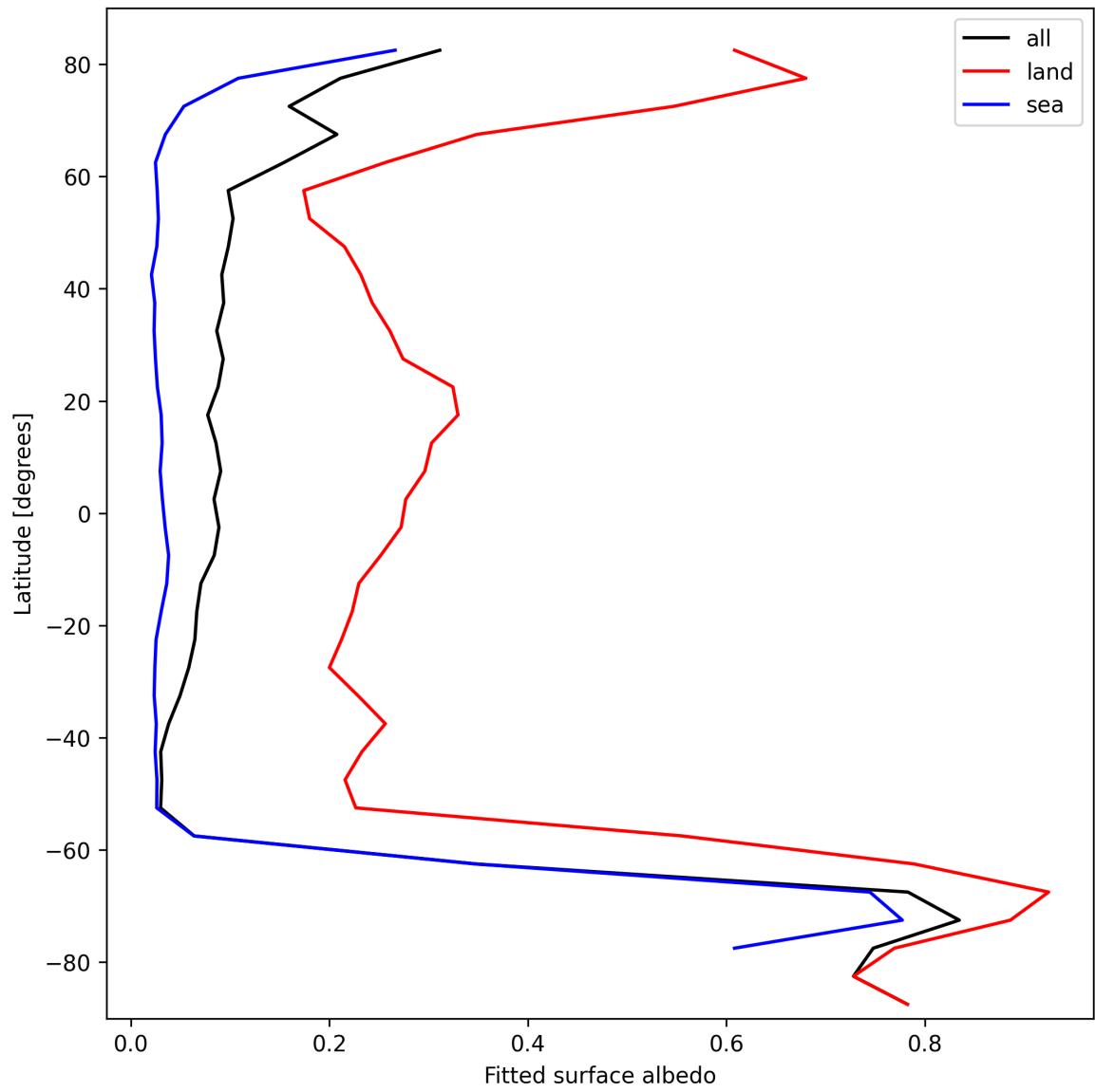
Figure 29: Zonal average of “Fitted surface albedo” for 2024-10-08 to 2024-10-10.
