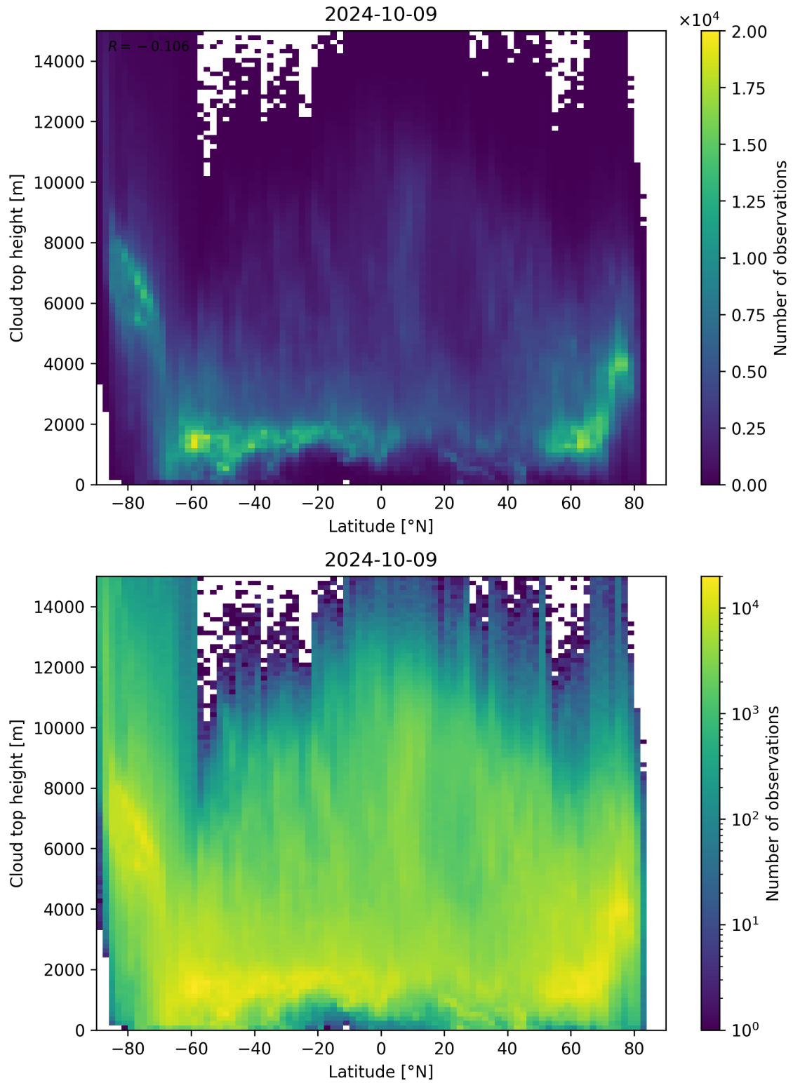
Figure 97: Scatter density plot of “Latitude” against “Cloud top height” for 2024-10-08 to 2024-10-10.
