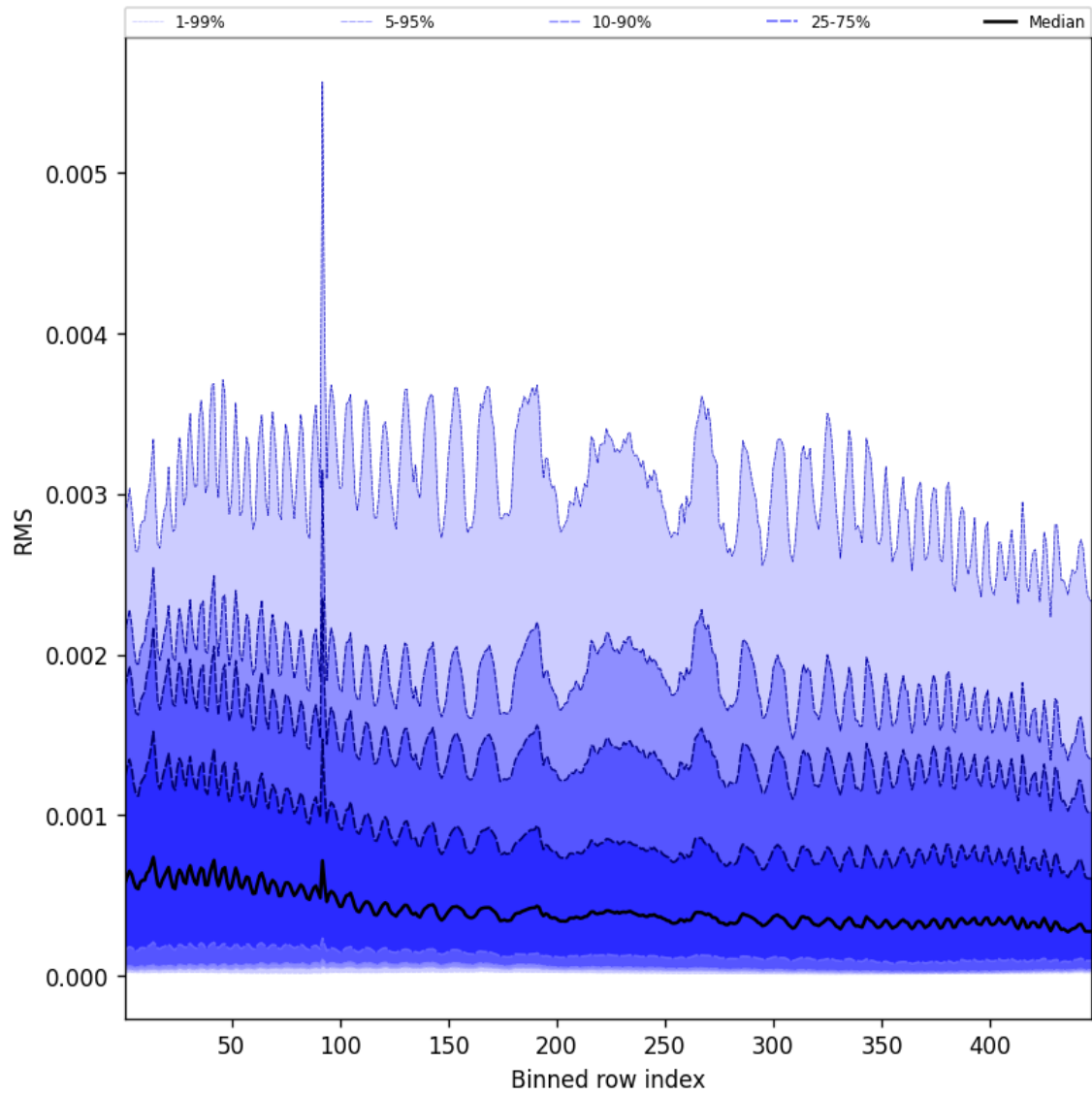
Figure 63: Along track statistics of “RMS” for 2024-10-08 to 2024-10-10
