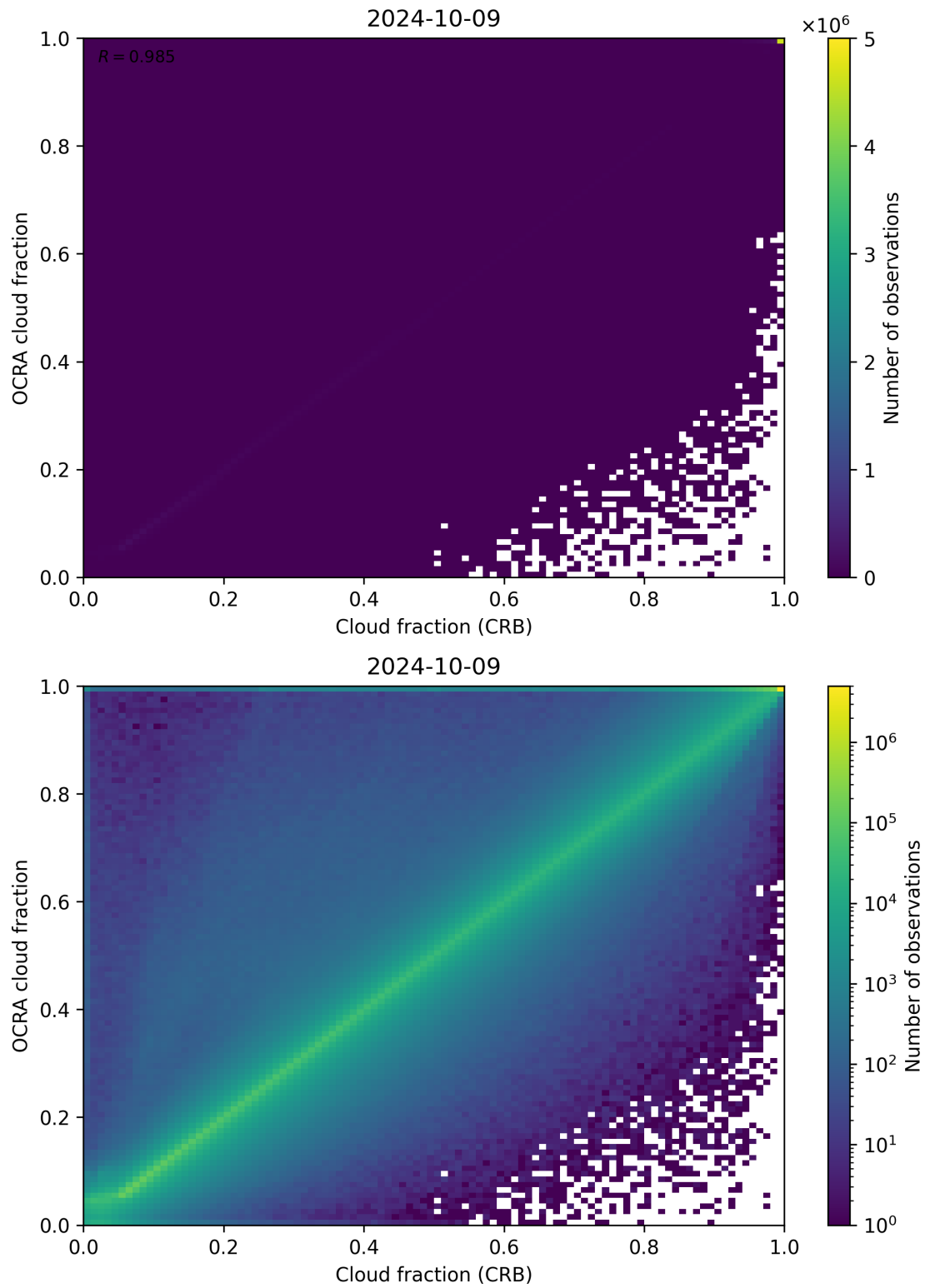
Figure 78: Scatter density plot of “Cloud fraction (CRB)” against “OCRA cloud fraction” for 2024-10-08 to 2024-10-10.
