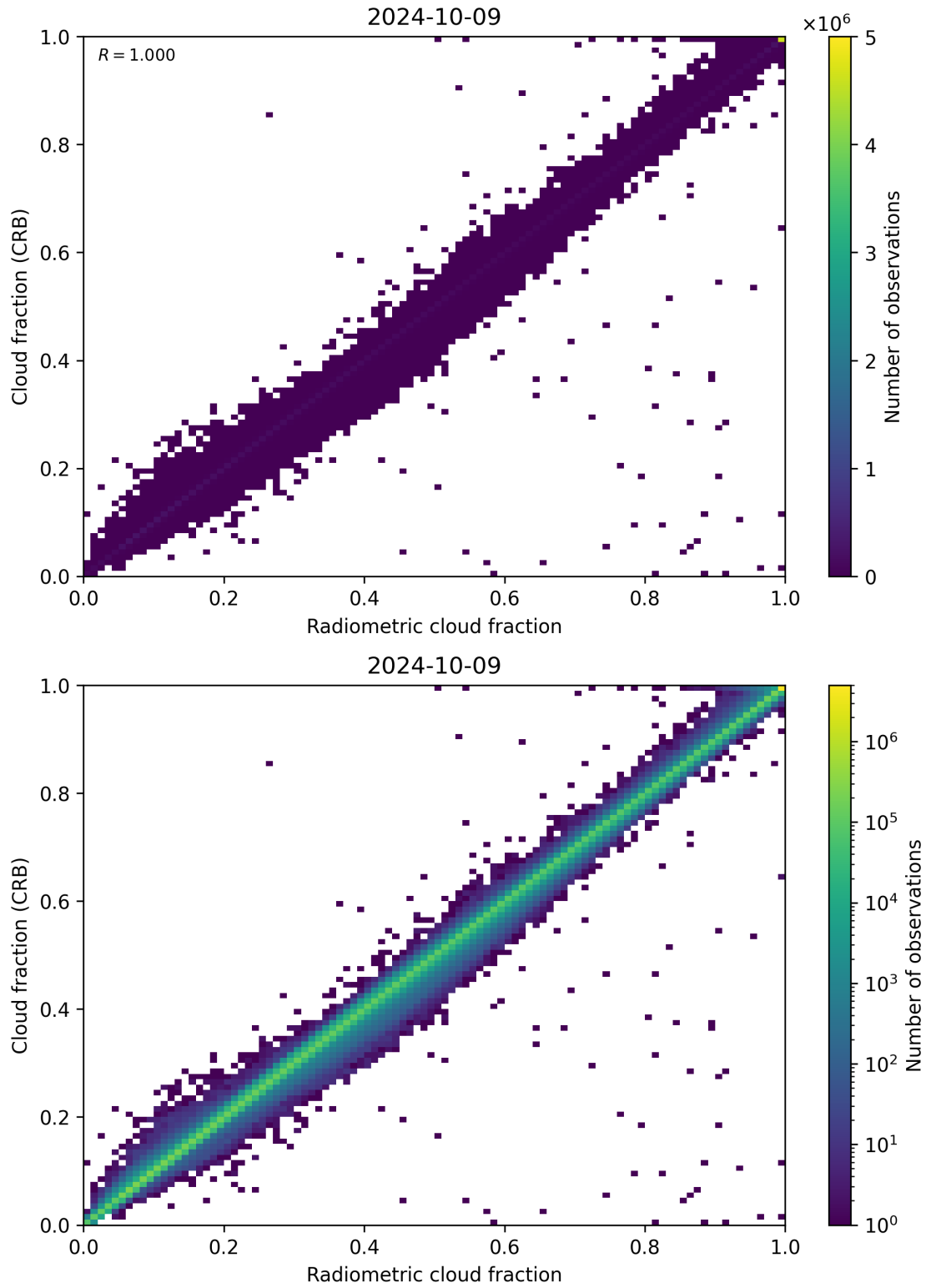
Figure 73: Scatter density plot of “Radiometric cloud fraction” against “Cloud fraction (CRB)” for 2024-10-08 to 2024-10-10.
