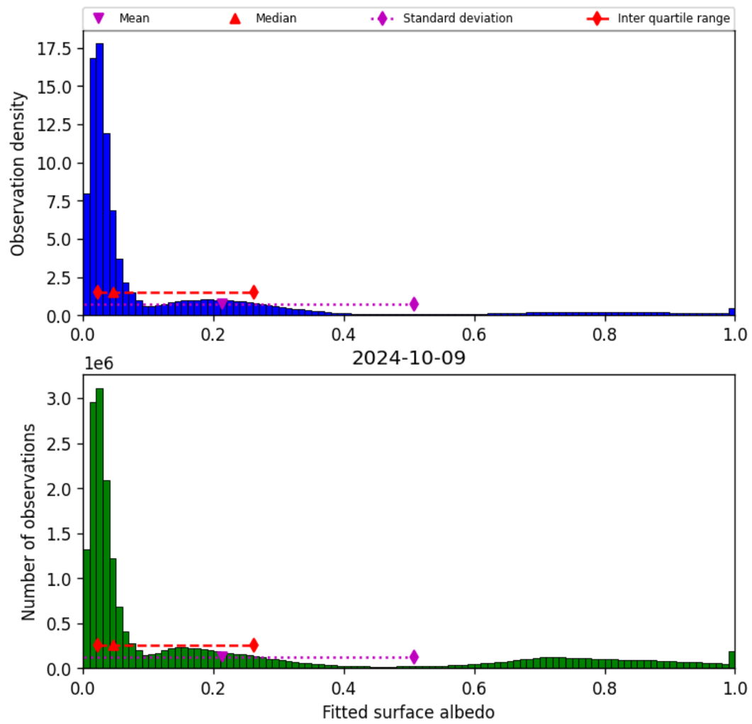
Figure 45: Histogram of “Fitted surface albedo” for 2024-10-08 to 2024-10-10
