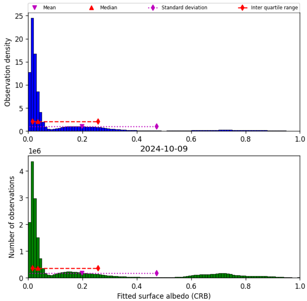
Figure 46: Histogram of “Fitted surface albedo (CRB)” for 2024-10-08 to 2024-10-10
