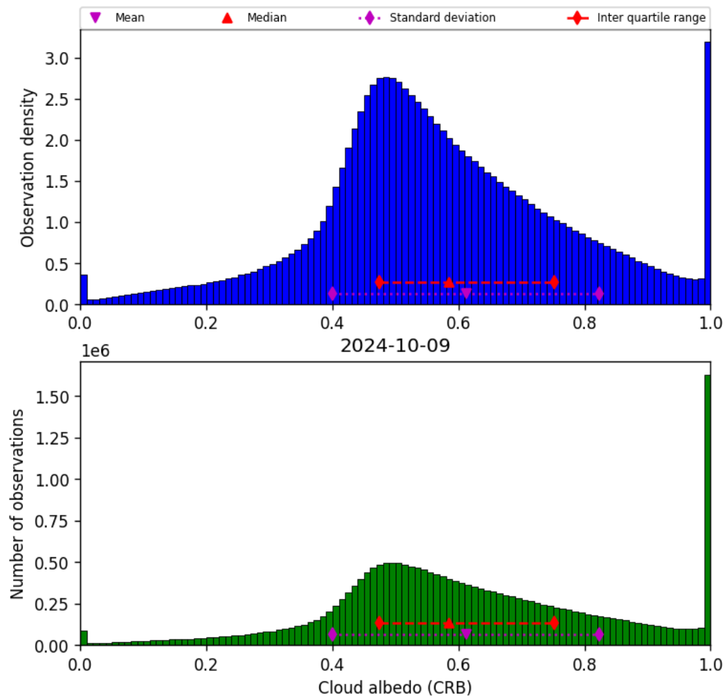
Figure 44: Histogram of “Cloud albedo (CRB)” for 2024-10-08 to 2024-10-10
