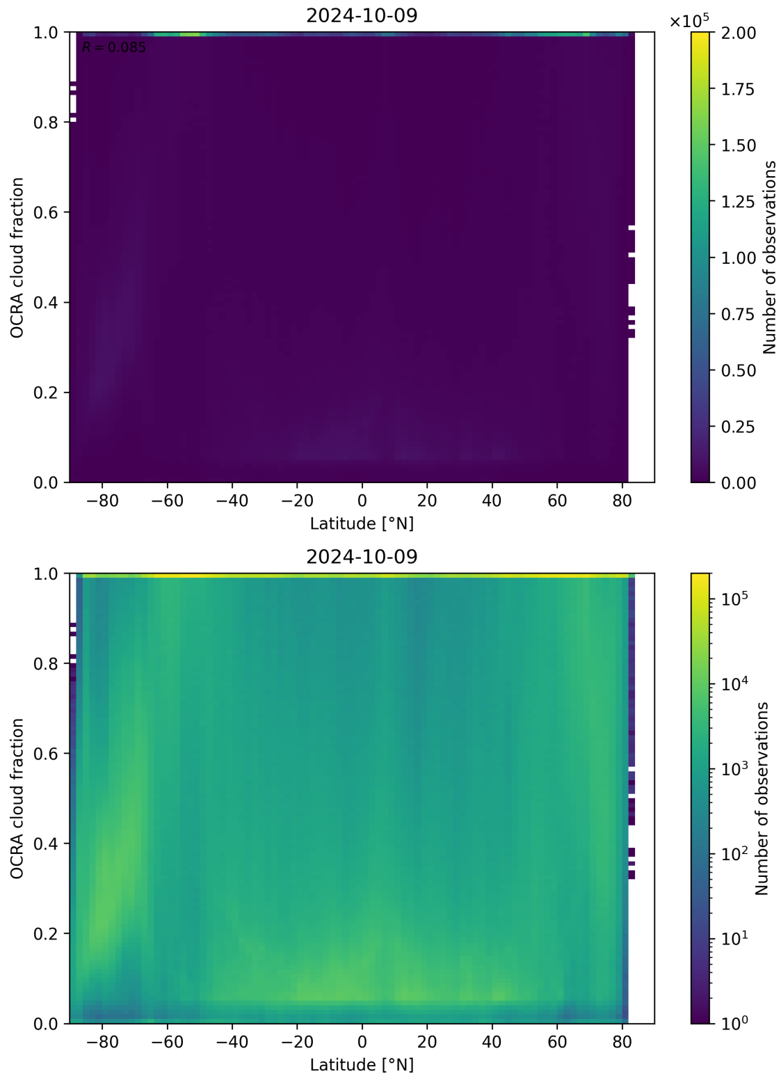
Figure 93: Scatter density plot of “Latitude” against “OCRA cloud fraction” for 2024-10-08 to 2024-10-10.
