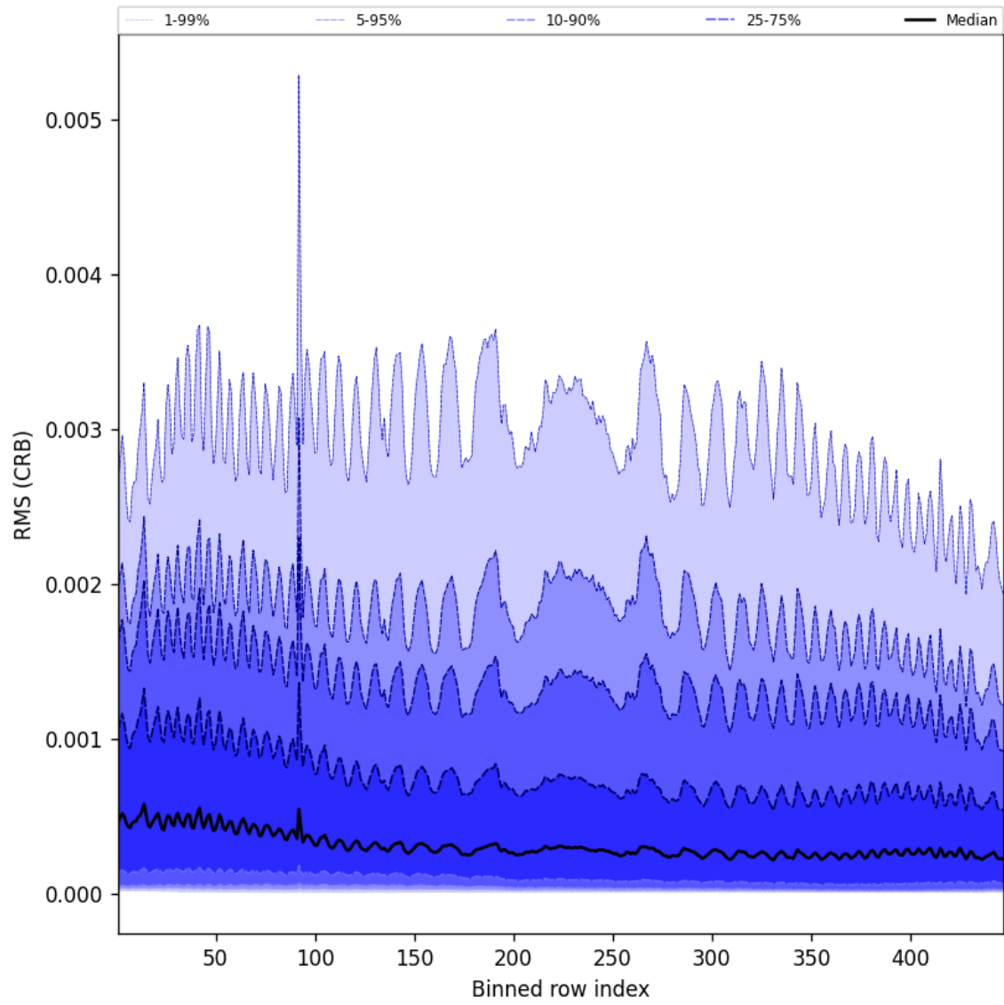
Figure 64: Along track statistics of “RMS (CRB)” for 2024-10-08 to 2024-10-10
