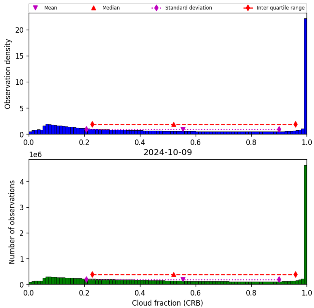
Figure 42: Histogram of “Cloud fraction (CRB)” for 2024-10-08 to 2024-10-10
