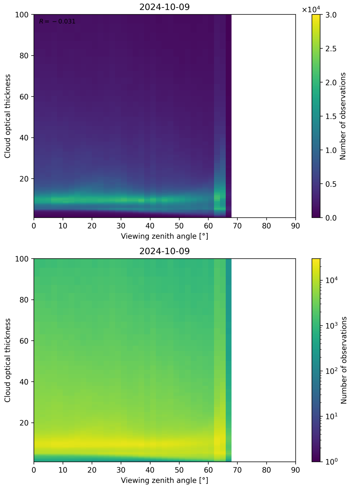
Figure 111: Scatter density plot of “Viewing zenith angle” against “Cloud optical thickness” for 2024-10-08 to 2024-10-10.
