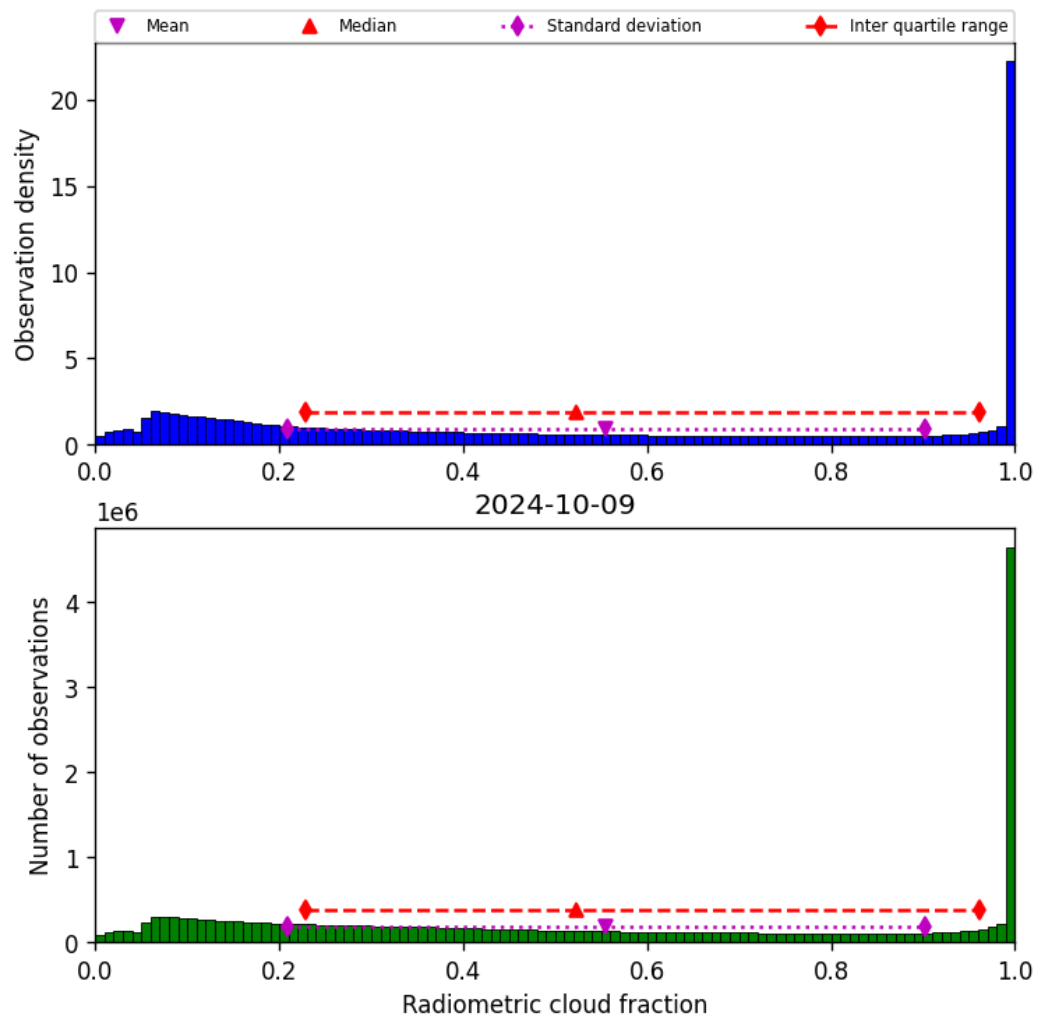
Figure 39: Histogram of “Radiometric cloud fraction” for 2024-10-08 to 2024-10-10
