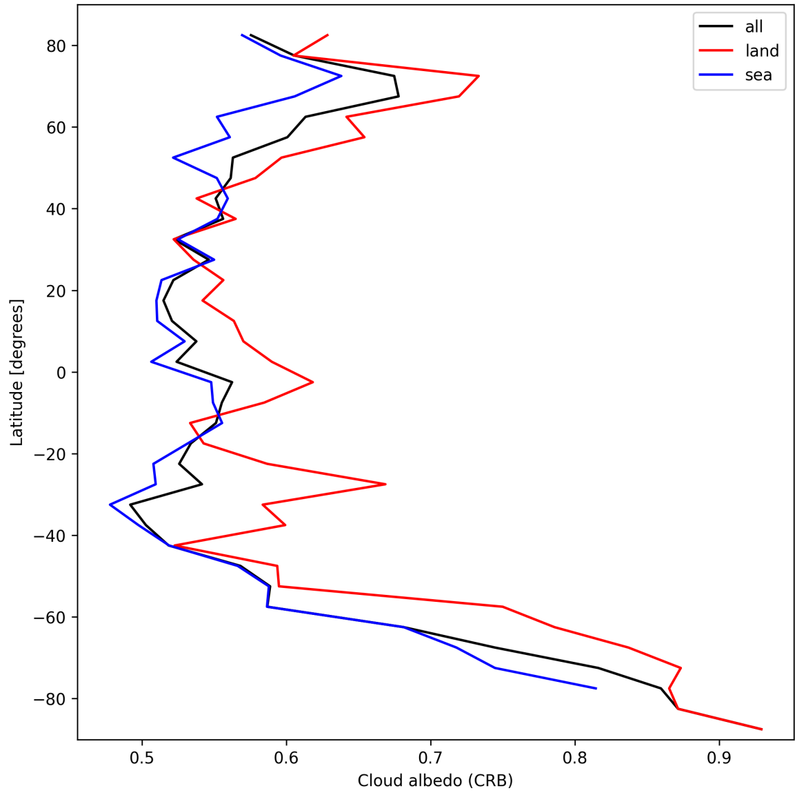
Figure 28: Zonal average of “Cloud albedo (CRB)” for 2024-10-08 to 2024-10-10.
