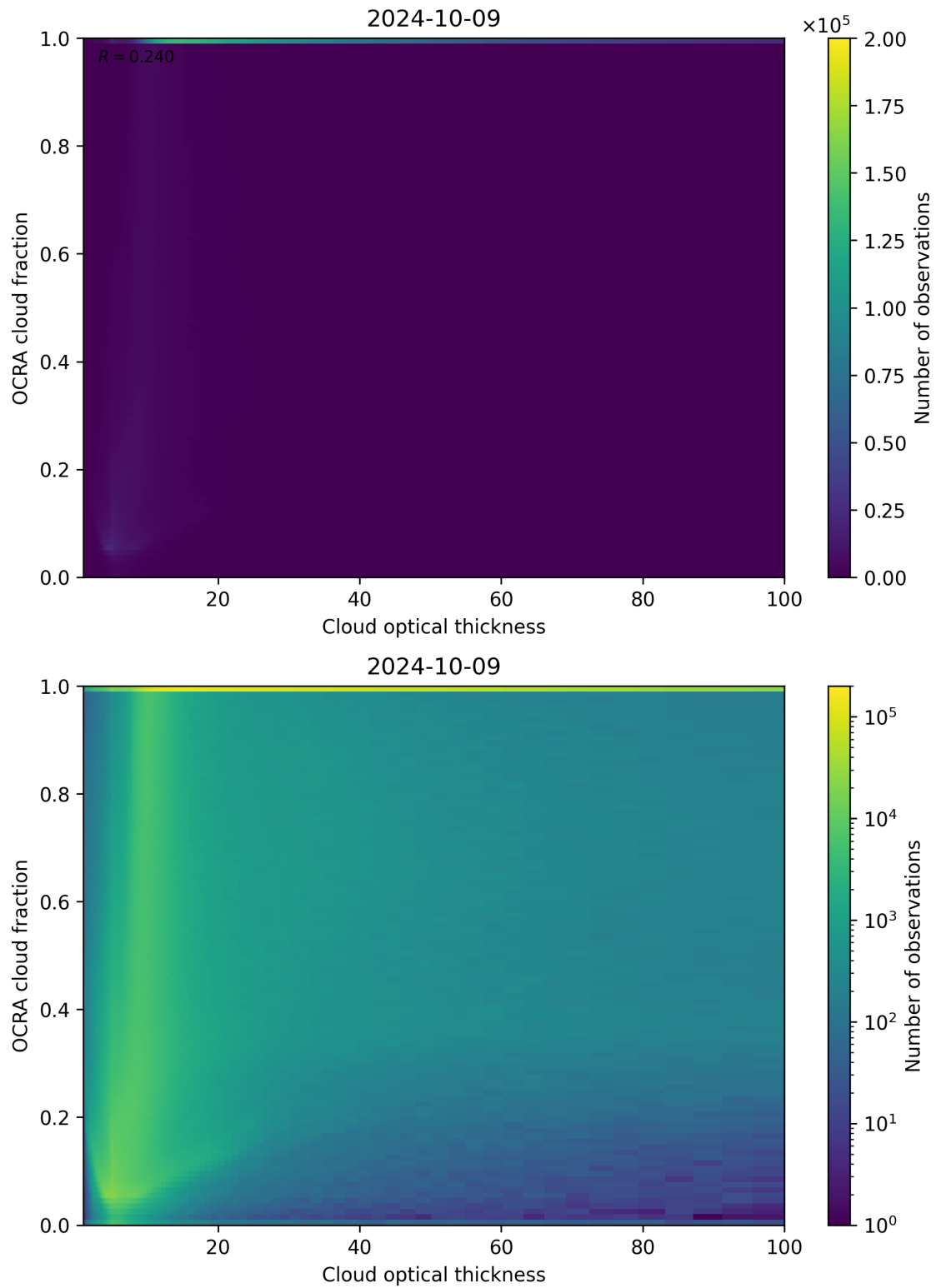
Figure 83: Scatter density plot of “Cloud optical thickness” against “OCRA cloud fraction” for 2024-10-08 to 2024-10-10.
