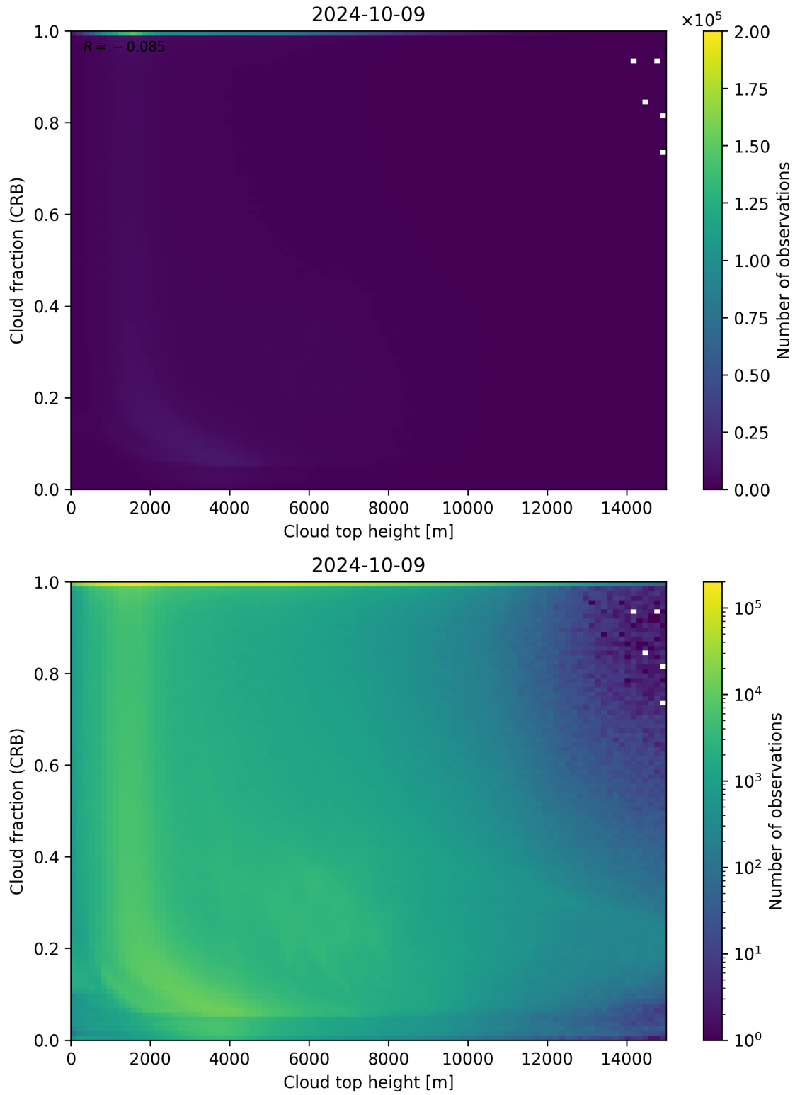
Figure 88: Scatter density plot of “Cloud top height” against “Cloud fraction (CRB)” for 2024-10-08 to 2024-10-10.
