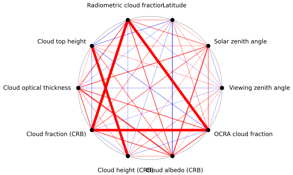
Figure 1: Map of correlation graph for 2024-10-08 to 2024-10-10.
