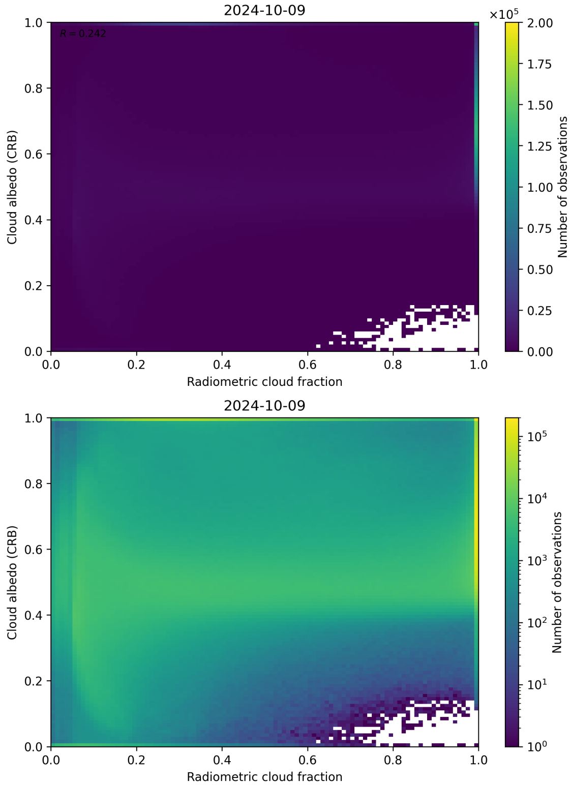
Figure 71: Scatter density plot of “Radiometric cloud fraction” against “Cloud albedo (CRB)” for 2024-10-08 to 2024-10-10.
