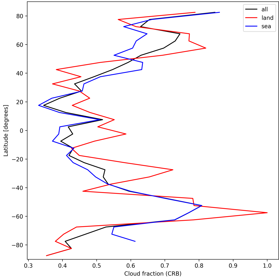
Figure 26: Zonal average of “Cloud fraction (CRB)” for 2024-10-08 to 2024-10-10.
