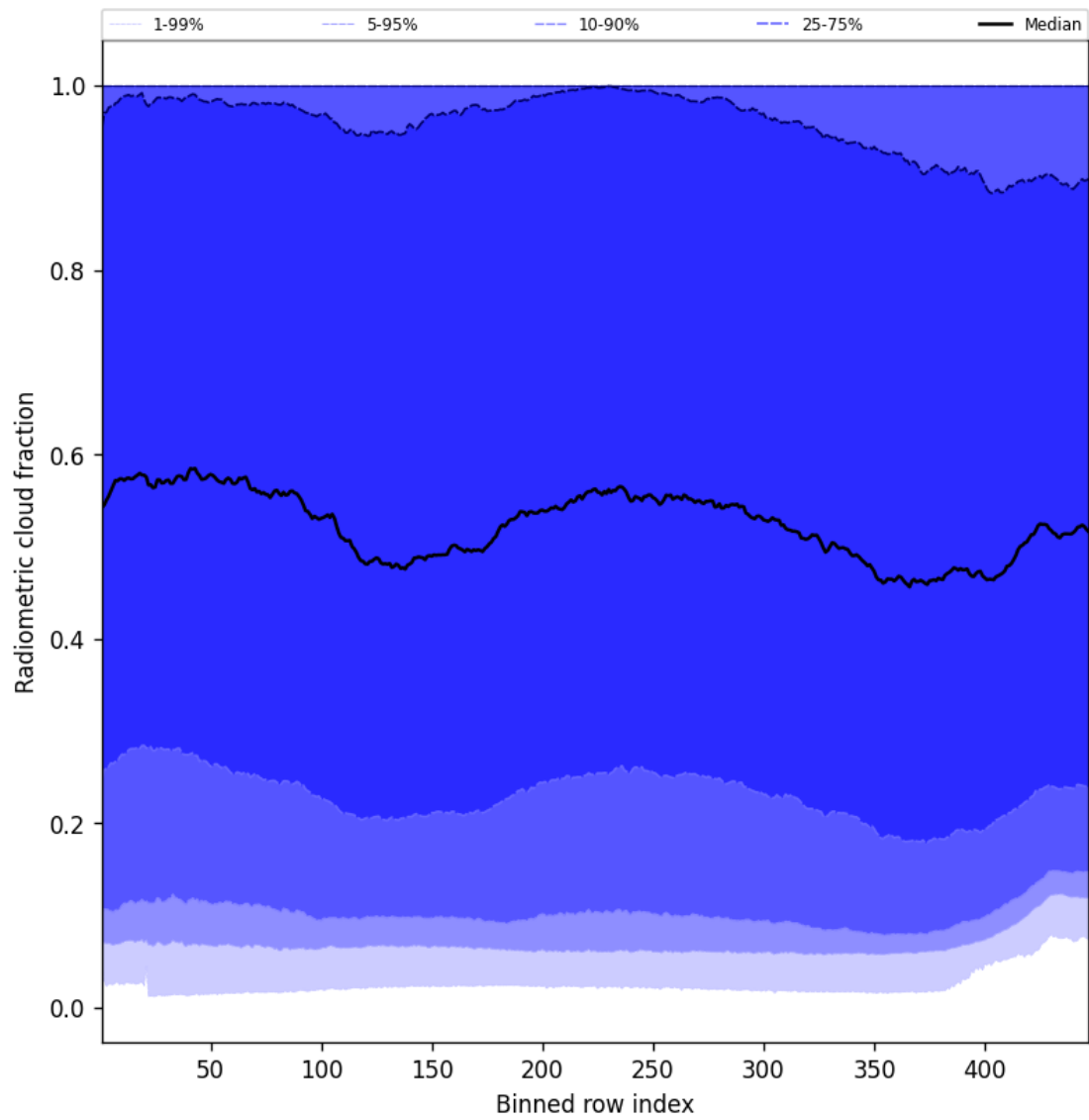
Figure 55: Along track statistics of “Radiometric cloud fraction” for 2024-10-08 to 2024-10-10
