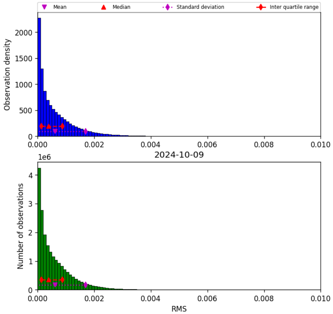
Figure 47: Histogram of “RMS” for 2024-10-08 to 2024-10-10
