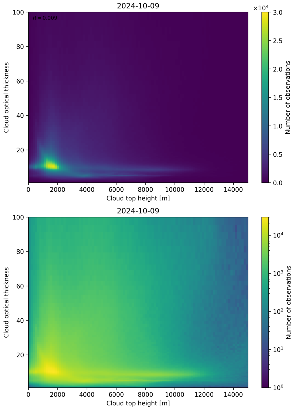
Figure 90: Scatter density plot of “Cloud top height” against “Cloud optical thickness” for 2024-10-08 to 2024-10-10.
