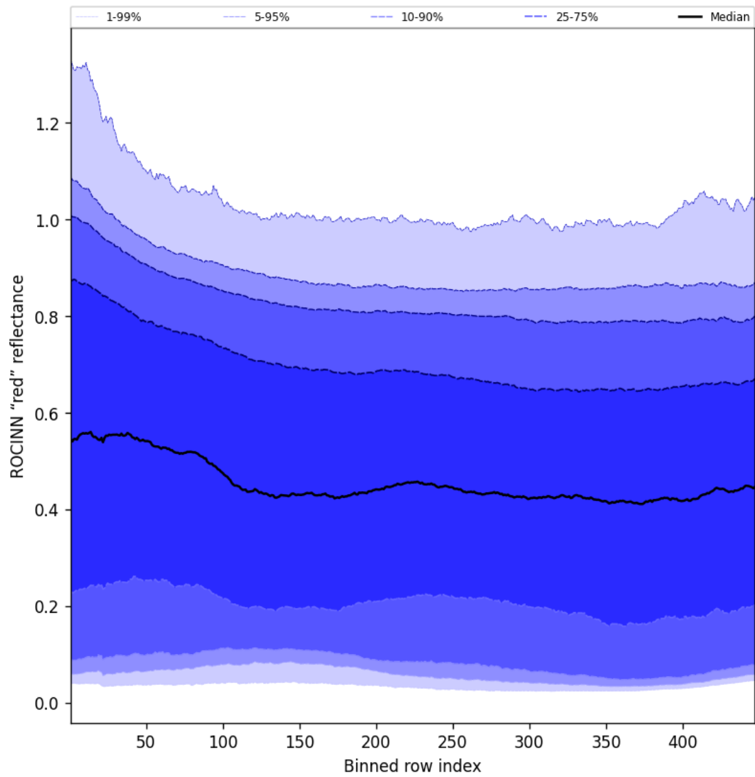
Figure 69: Along track statistics of “ROCINN “red” reflectance” for 2024-10-08 to 2024-10-10
