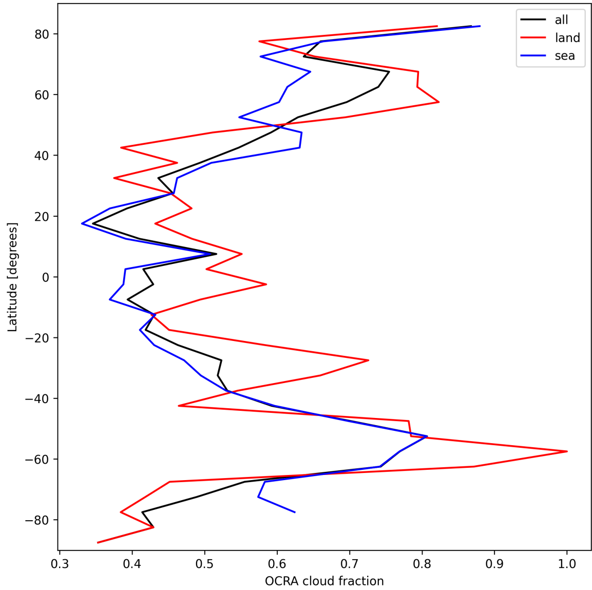
Figure 34: Zonal average of “OCRA cloud fraction” for 2024-10-08 to 2024-10-10.
