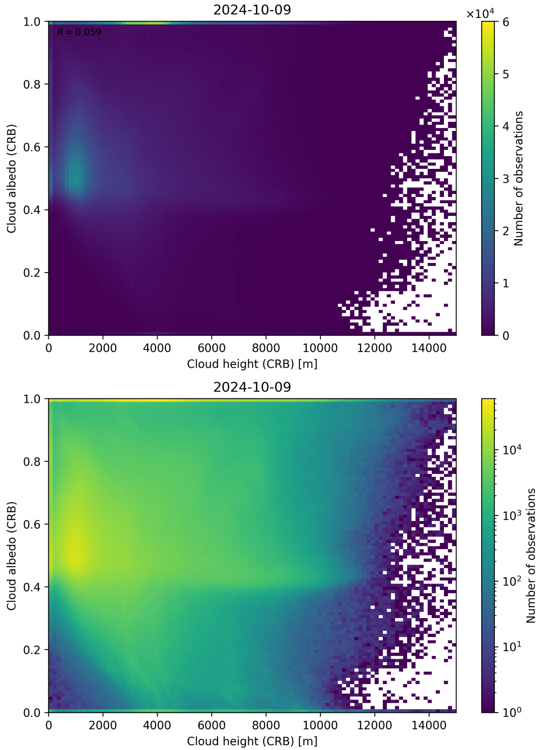
Figure 80: Scatter density plot of “Cloud height (CRB)” against “Cloud albedo (CRB)” for 2024-10-08 to 2024-10-10.
