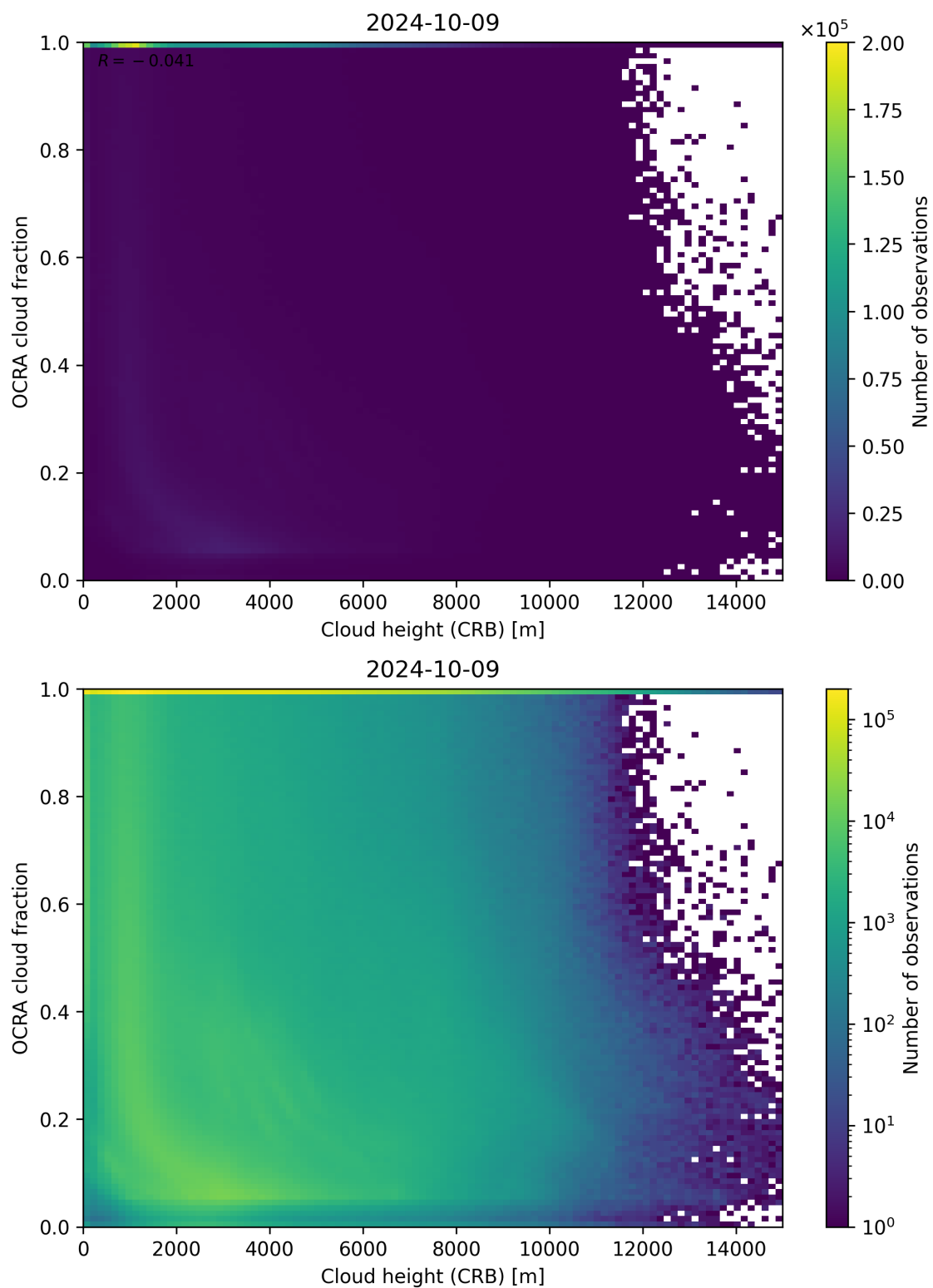
Figure 81: Scatter density plot of “Cloud height (CRB)” against “OCRA cloud fraction” for 2024-10-08 to 2024-10-10.
