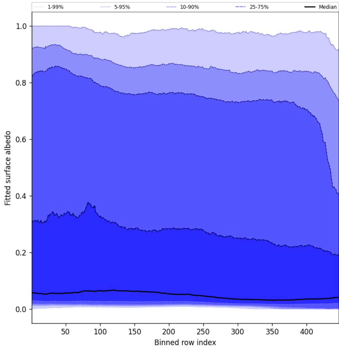
Figure 61: Along track statistics of “Fitted surface albedo” for 2024-10-08 to 2024-10-10
