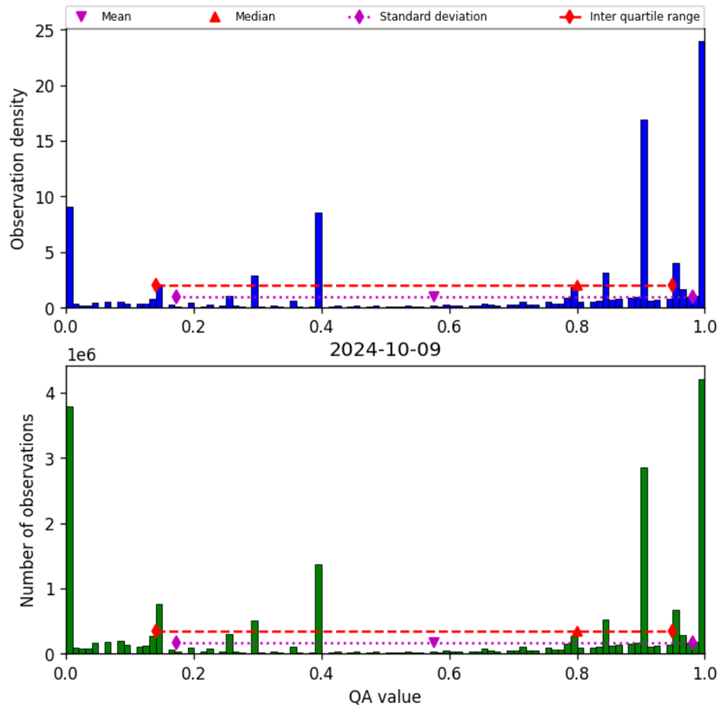
Figure 38: Histogram of “QA value” for 2024-10-08 to 2024-10-10
