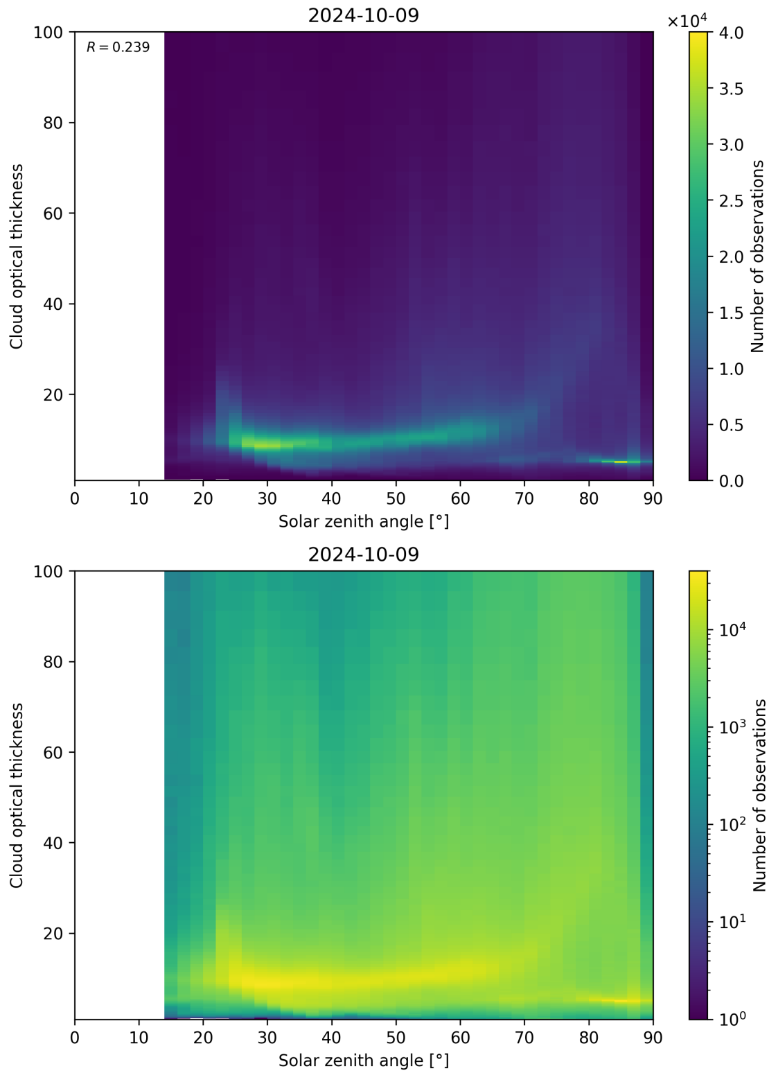
Figure 103: Scatter density plot of “Solar zenith angle” against “Cloud optical thickness” for 2024-10-08 to 2024-10-10.
