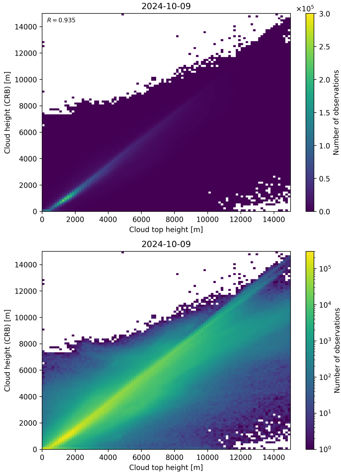
Figure 89: Scatter density plot of “Cloud top height” against “Cloud height (CRB)” for 2024-10-08 to 2024-10-10.
