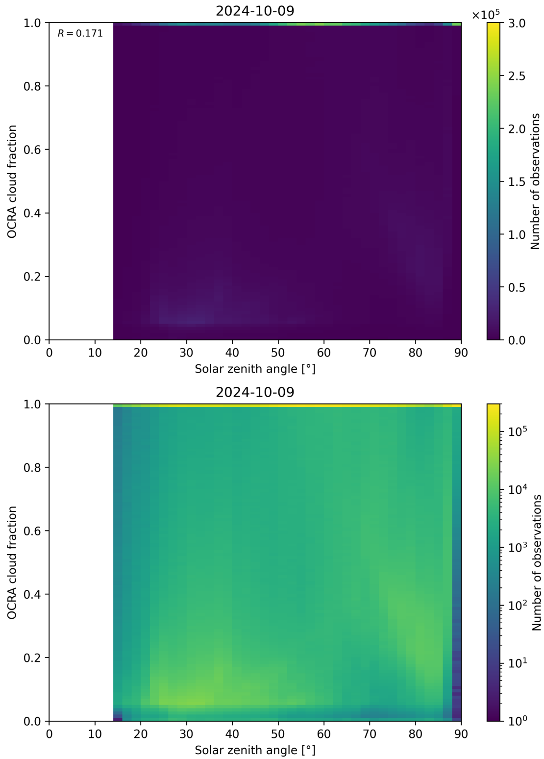
Figure 100: Scatter density plot of “Solar zenith angle” against “OCRA cloud fraction” for 2024-10-08 to 2024-10-10.
