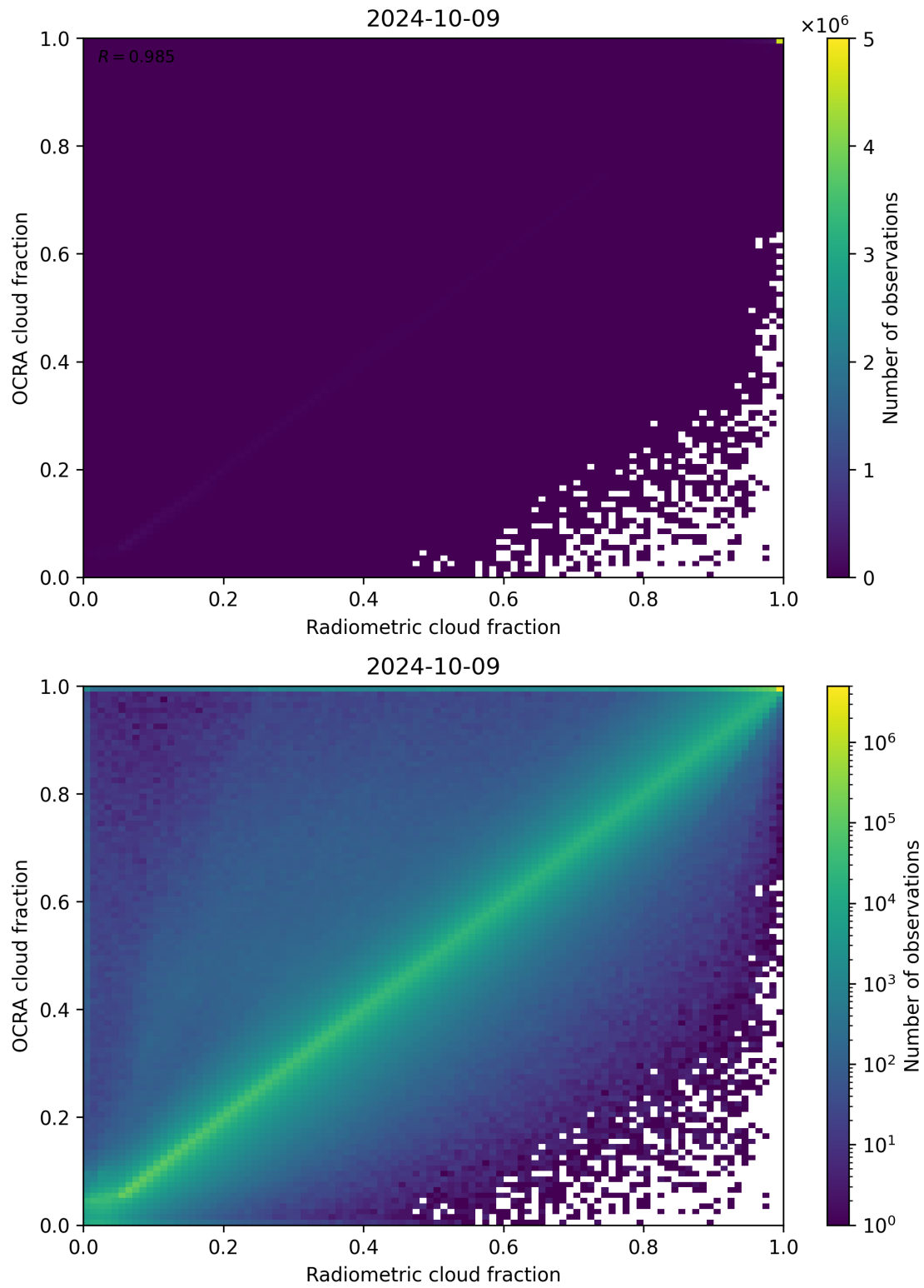
Figure 72: Scatter density plot of “Radiometric cloud fraction” against “OCRA cloud fraction” for 2024-10-08 to 2024-10-10.
