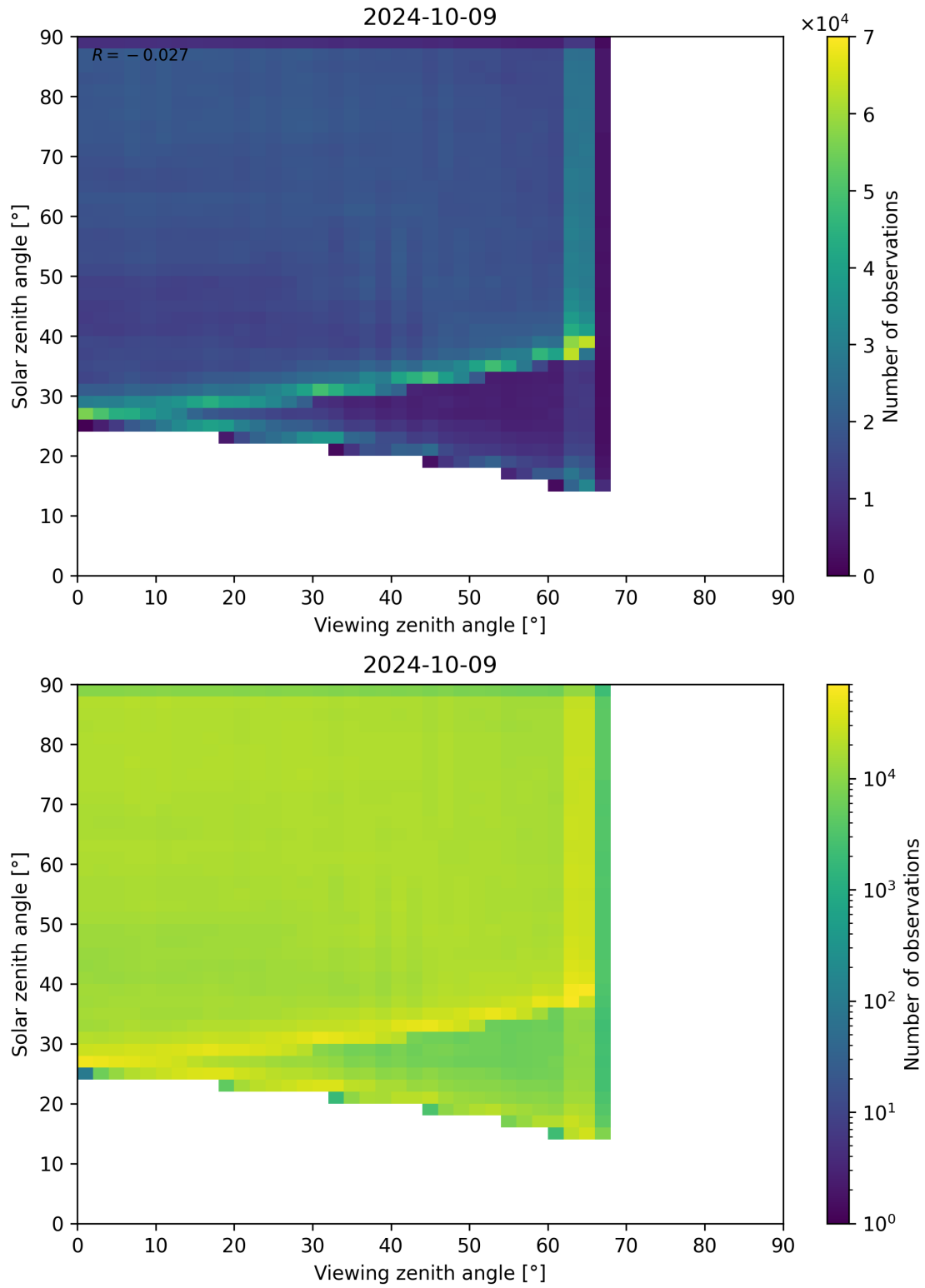
Figure 114: Scatter density plot of “Viewing zenith angle” against “Solar zenith angle” for 2024-10-08 to 2024-10-10.
