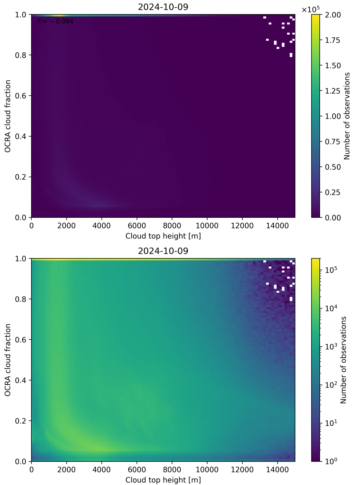
Figure 87: Scatter density plot of “Cloud top height” against “OCRA cloud fraction” for 2024-10-08 to 2024-10-10.
