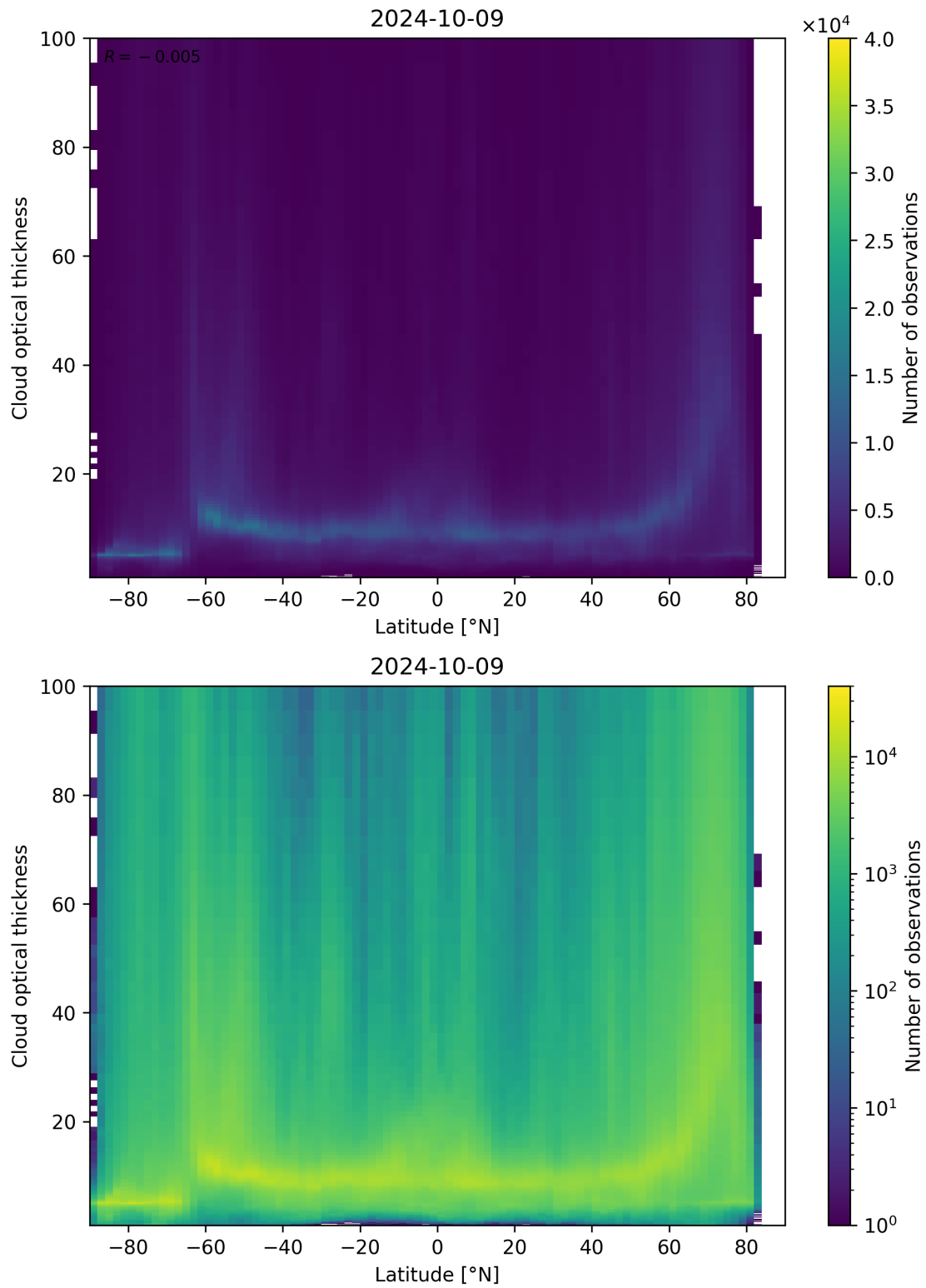
Figure 96: Scatter density plot of “Latitude” against “Cloud optical thickness” for 2024-10-08 to 2024-10-10.
