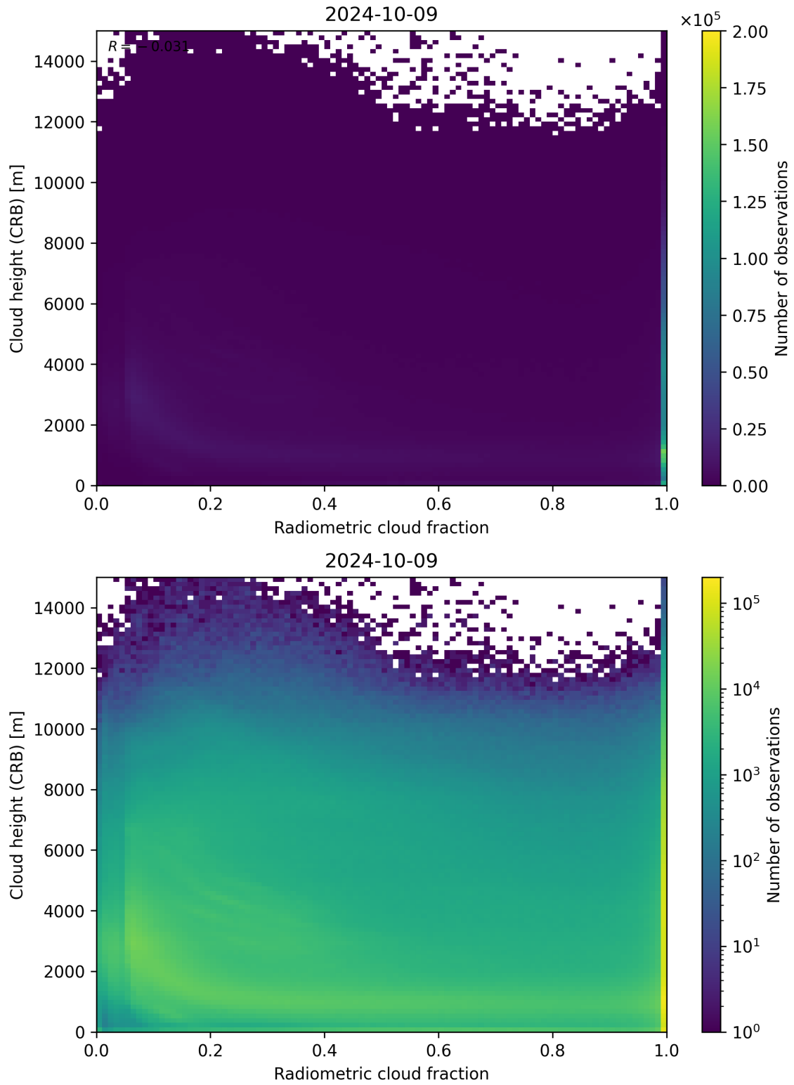
Figure 74: Scatter density plot of “Radiometric cloud fraction” against “Cloud height (CRB)” for 2024-10-08 to 2024-10-10.
