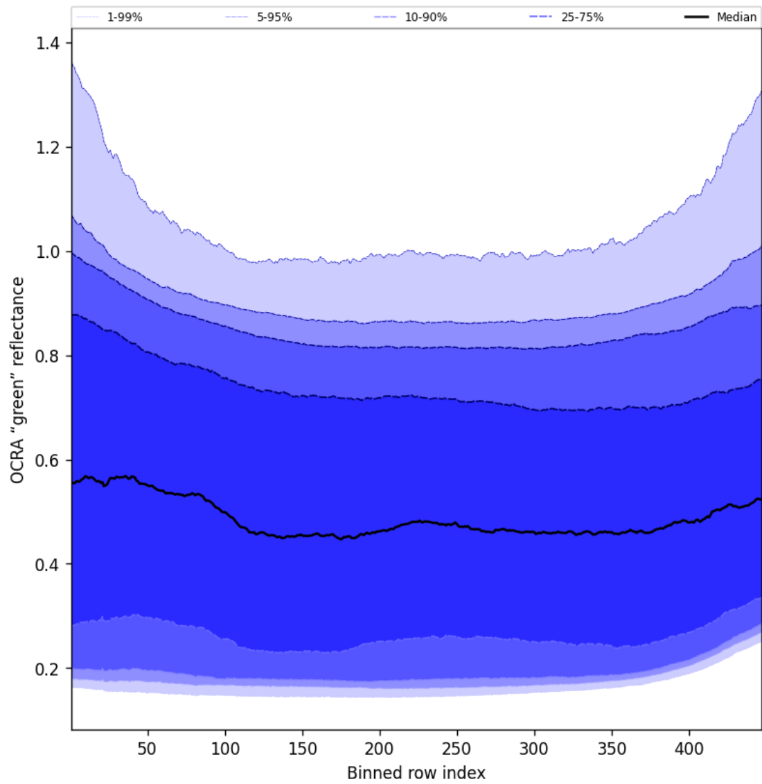
Figure 68: Along track statistics of “OCRA “green” reflectance” for 2024-10-08 to 2024-10-10
