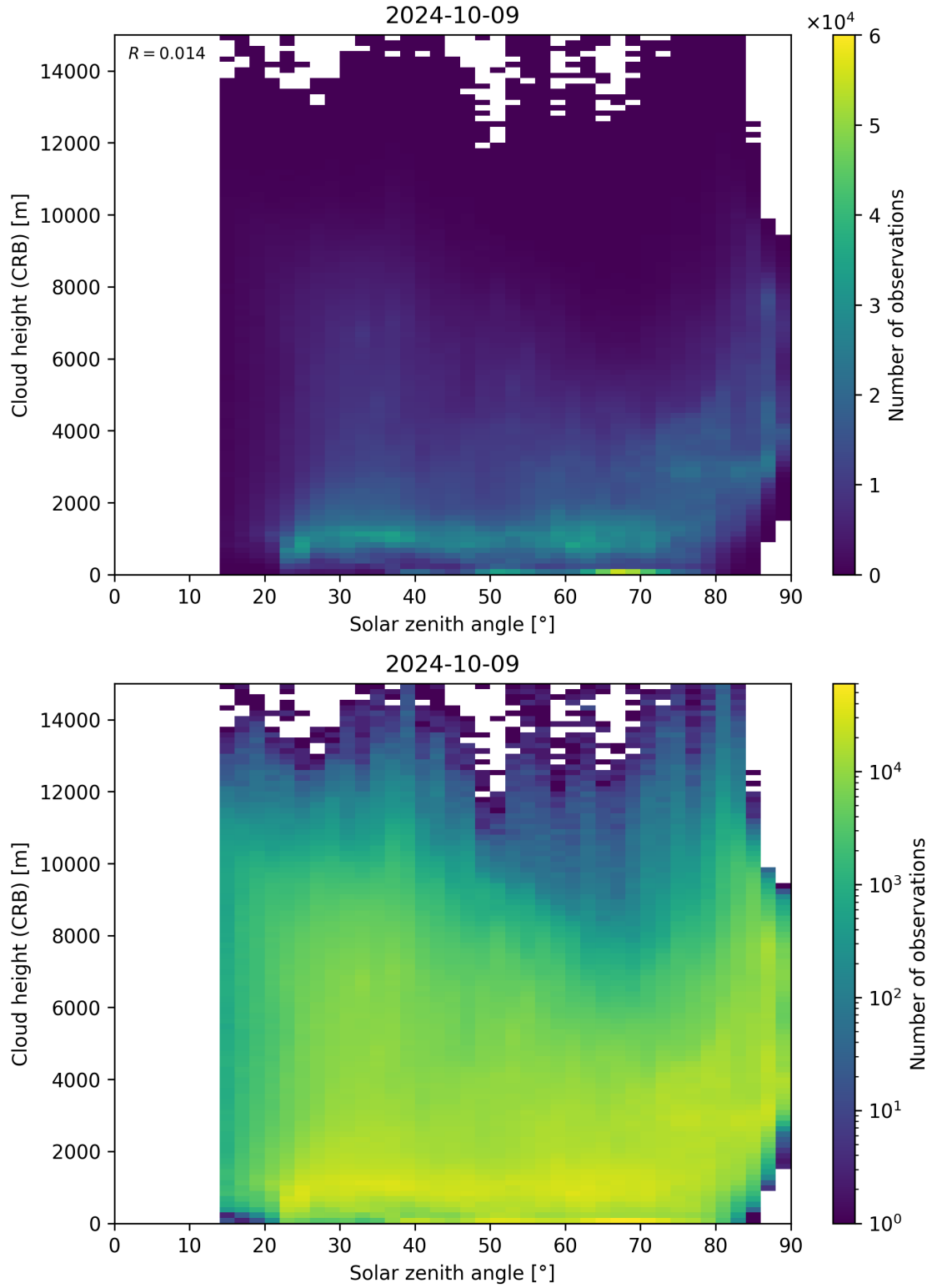
Figure 102: Scatter density plot of “Solar zenith angle” against “Cloud height (CRB)” for 2024-10-08 to 2024-10-10.
