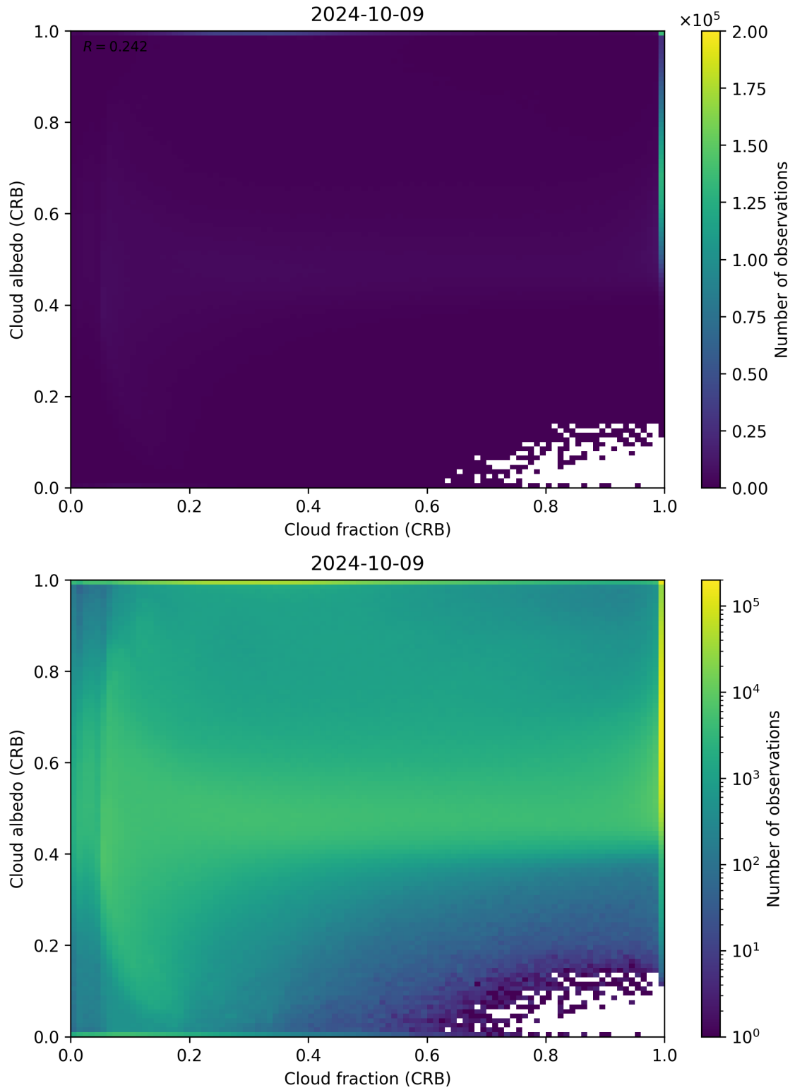
Figure 77: Scatter density plot of “Cloud fraction (CRB)” against “Cloud albedo (CRB)” for 2024-10-08 to 2024-10-10.
