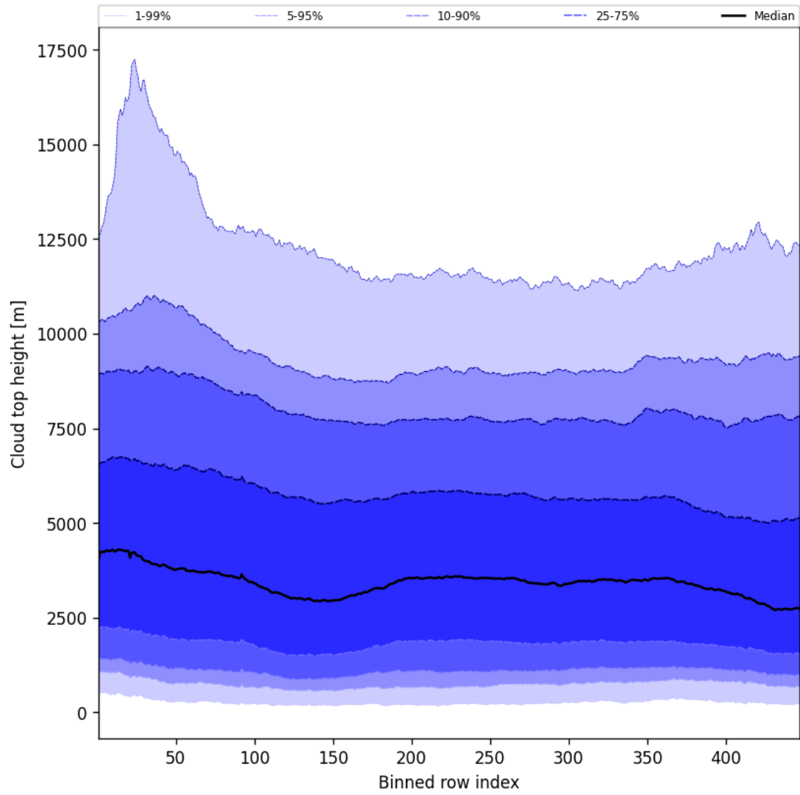
Figure 56: Along track statistics of “Cloud top height” for 2024-10-08 to 2024-10-10
