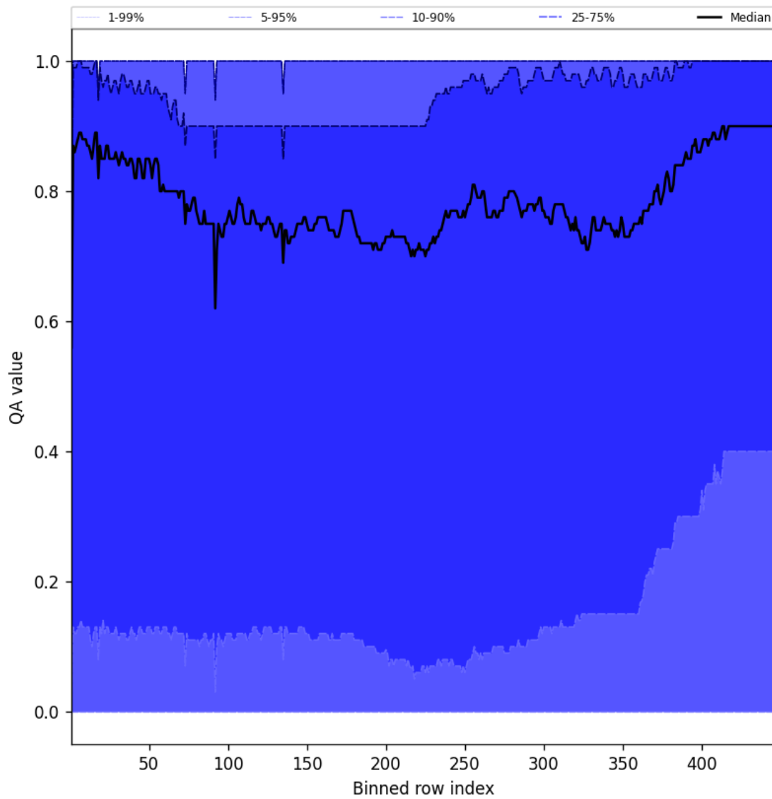
Figure 54: Along track statistics of “QA value” for 2024-10-08 to 2024-10-10
