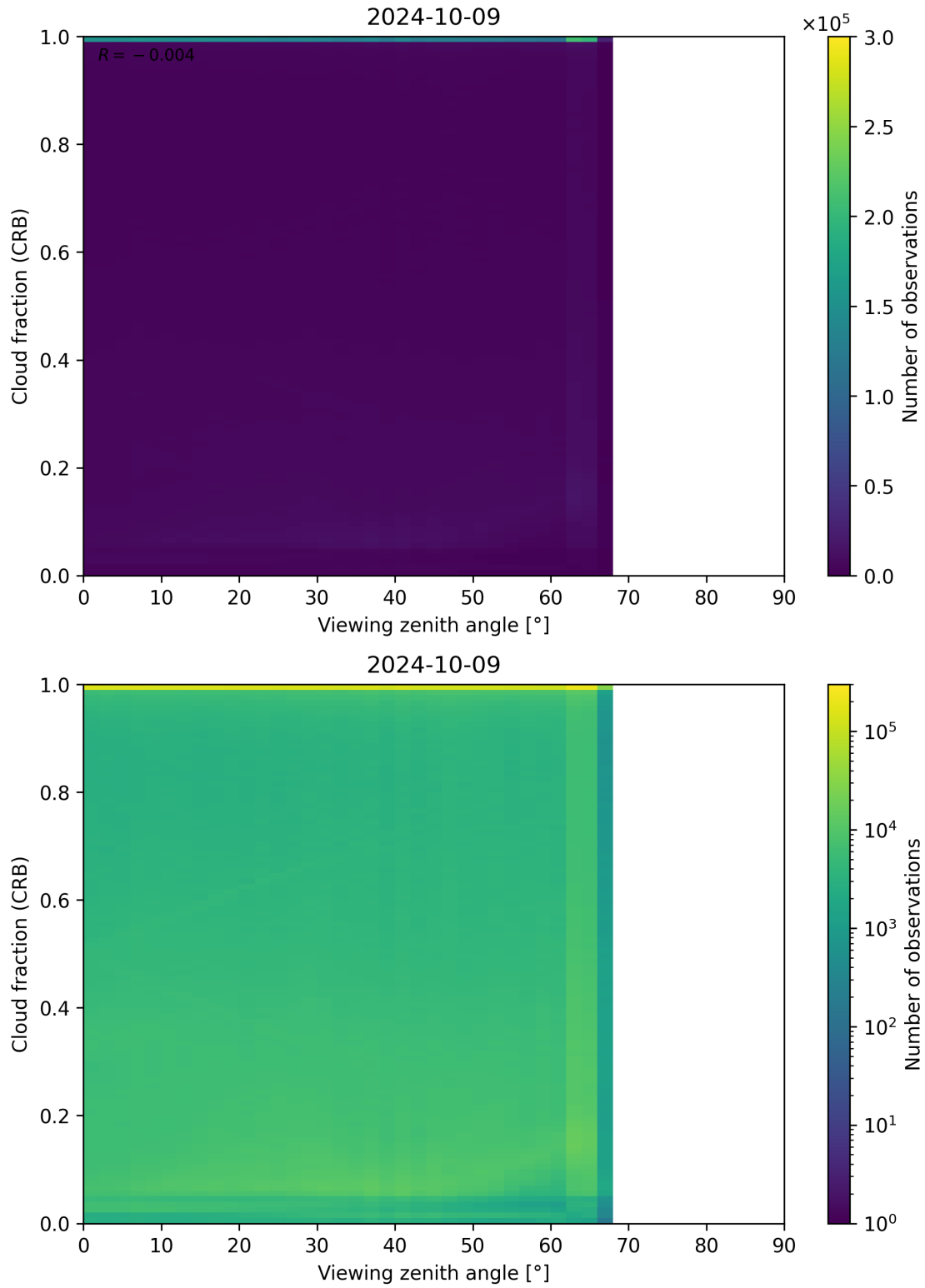
Figure 109: Scatter density plot of “Viewing zenith angle” against “Cloud fraction (CRB)” for 2024-10-08 to 2024-10-10.
