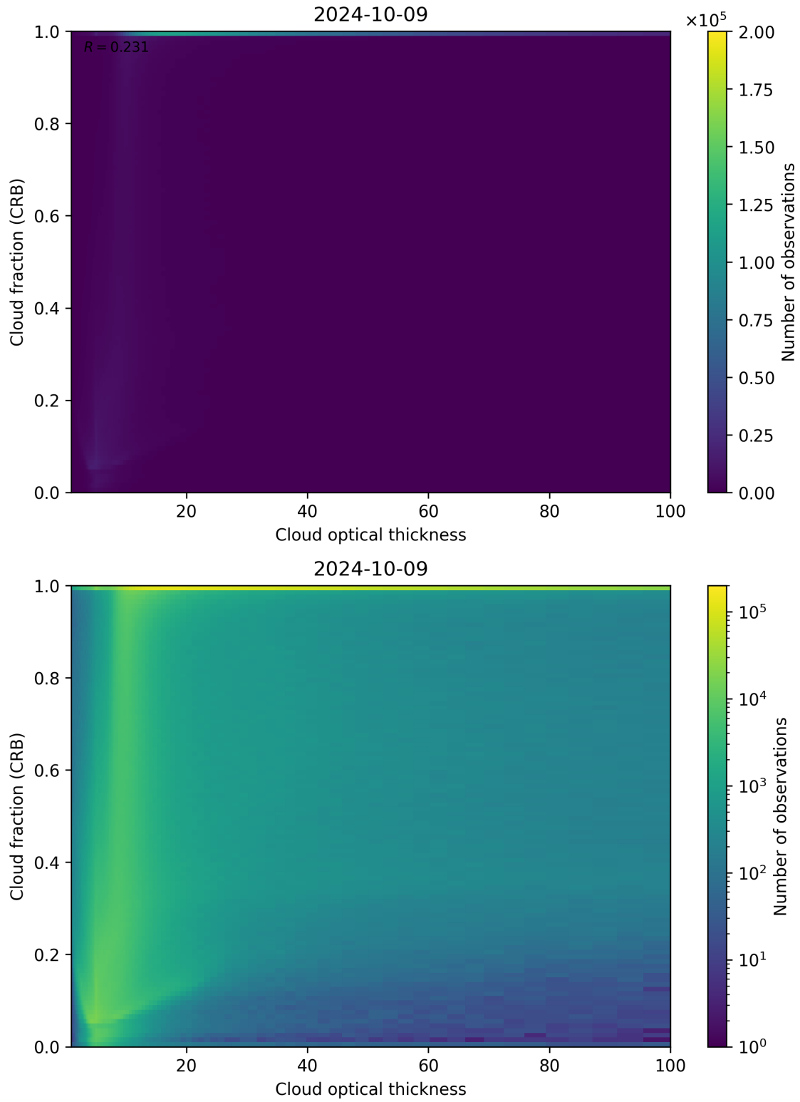
Figure 84: Scatter density plot of “Cloud optical thickness” against “Cloud fraction (CRB)” for 2024-10-08 to 2024-10-10.
