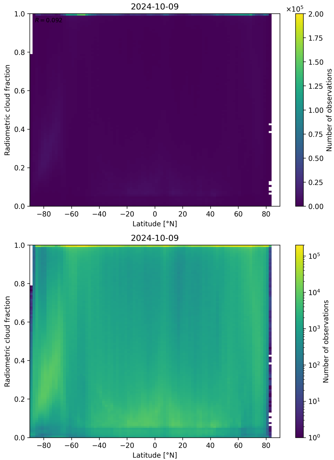
Figure 92: Scatter density plot of “Latitude” against “Radiometric cloud fraction” for 2024-10-08 to 2024-10-10.
