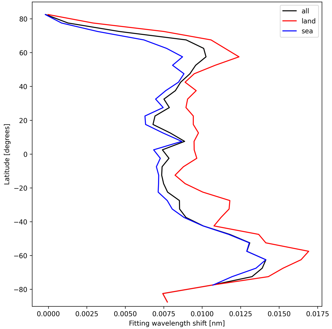
Figure 33: Zonal average of “Fitting wavelength shift” for 2024-10-08 to 2024-10-10.
