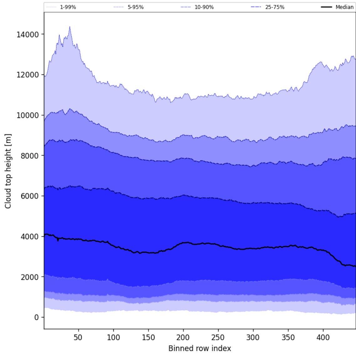
Figure 56: Along track statistics of “Cloud top height” for 2024-10-10 to 2024-10-12
