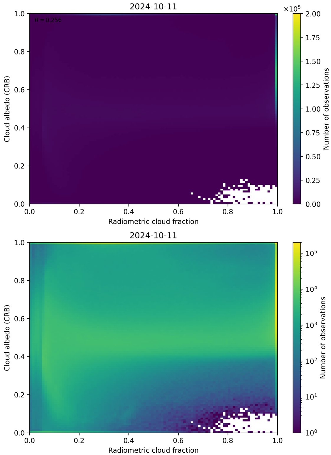
Figure 71: Scatter density plot of “Radiometric cloud fraction” against “Cloud albedo (CRB)” for 2024-10-10 to 2024-10-12.
