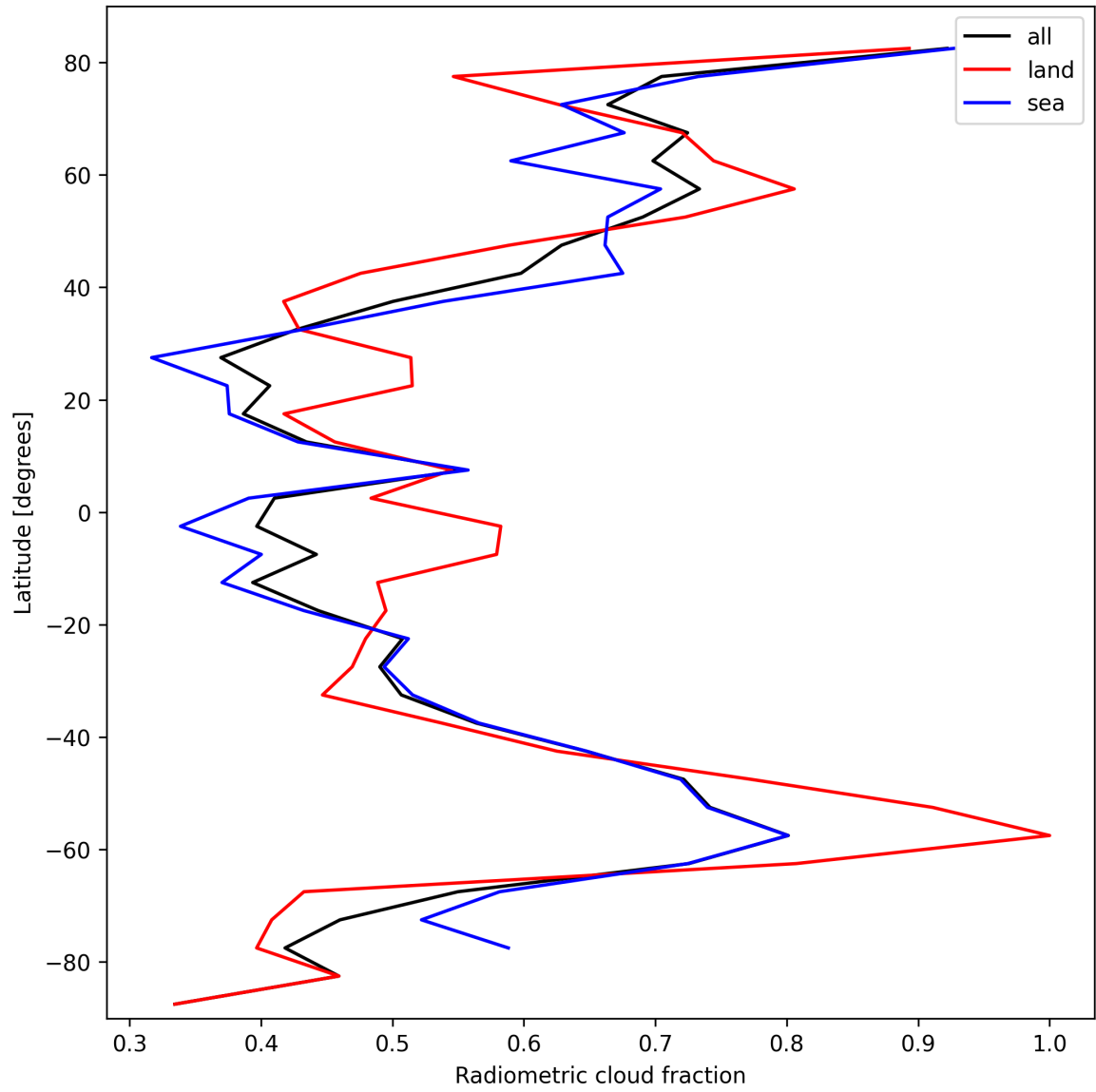
Figure 23: Zonal average of “Radiometric cloud fraction” for 2024-10-10 to 2024-10-12.
