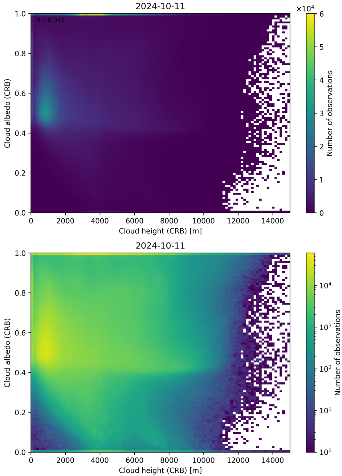
Figure 80: Scatter density plot of “Cloud height (CRB)” against “Cloud albedo (CRB)” for 2024-10-10 to 2024-10-12.
