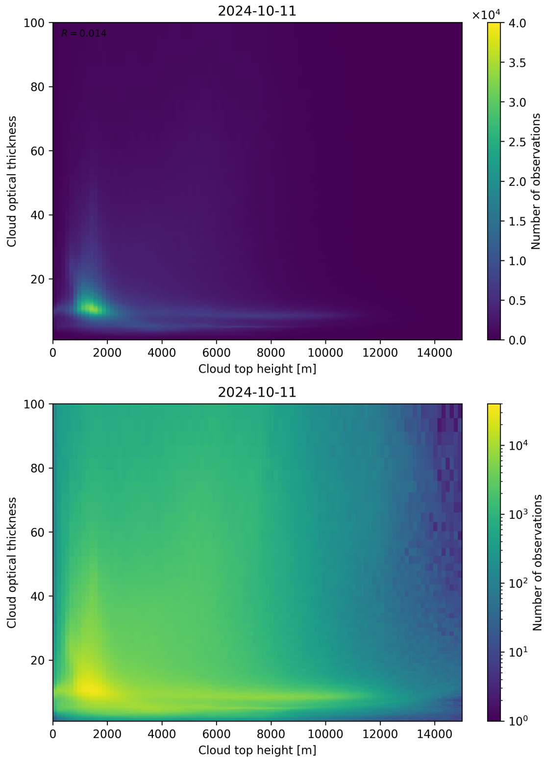
Figure 90: Scatter density plot of “Cloud top height” against “Cloud optical thickness” for 2024-10-10 to 2024-10-12.
