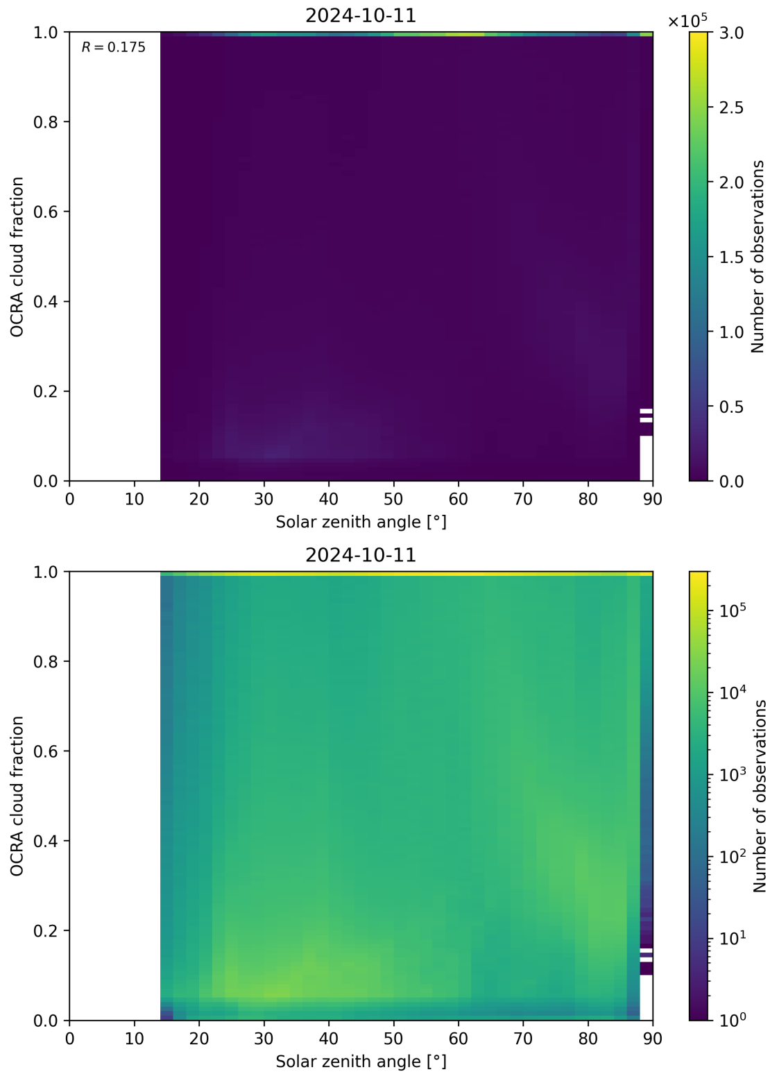
Figure 100: Scatter density plot of “Solar zenith angle” against “OCRA cloud fraction” for 2024-10-10 to 2024-10-12.
