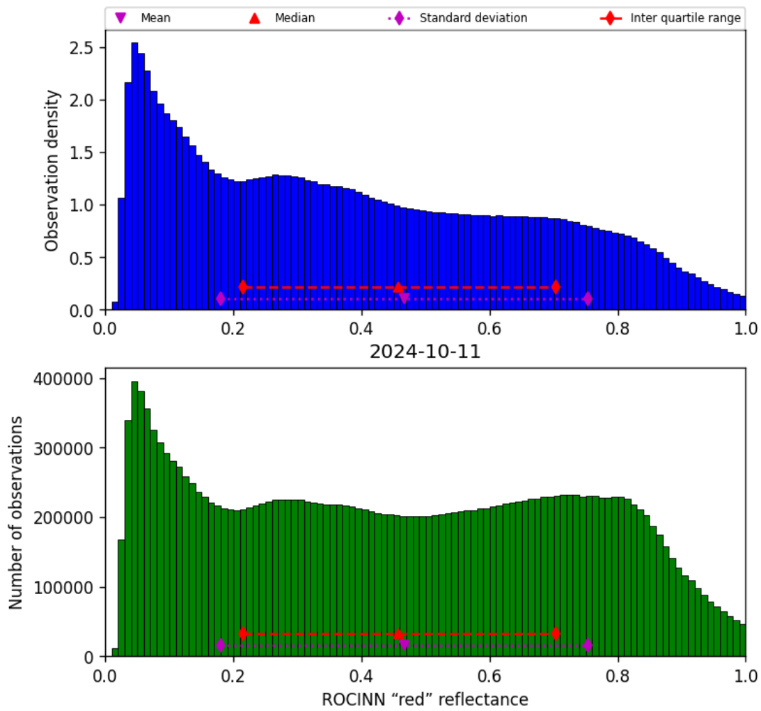
Figure 53: Histogram of “ROCINN “red” reflectance” for 2024-10-10 to 2024-10-12
