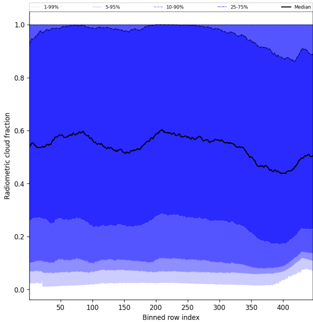
Figure 55: Along track statistics of “Radiometric cloud fraction” for 2024-10-10 to 2024-10-12
