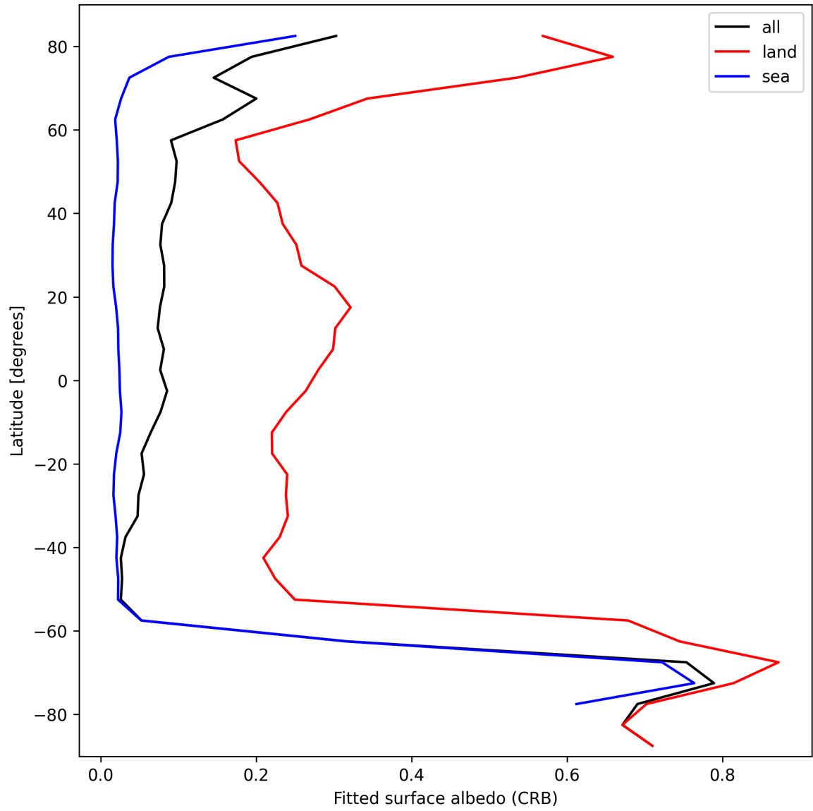
Figure 30: Zonal average of “Fitted surface albedo (CRB)” for 2024-10-10 to 2024-10-12.
