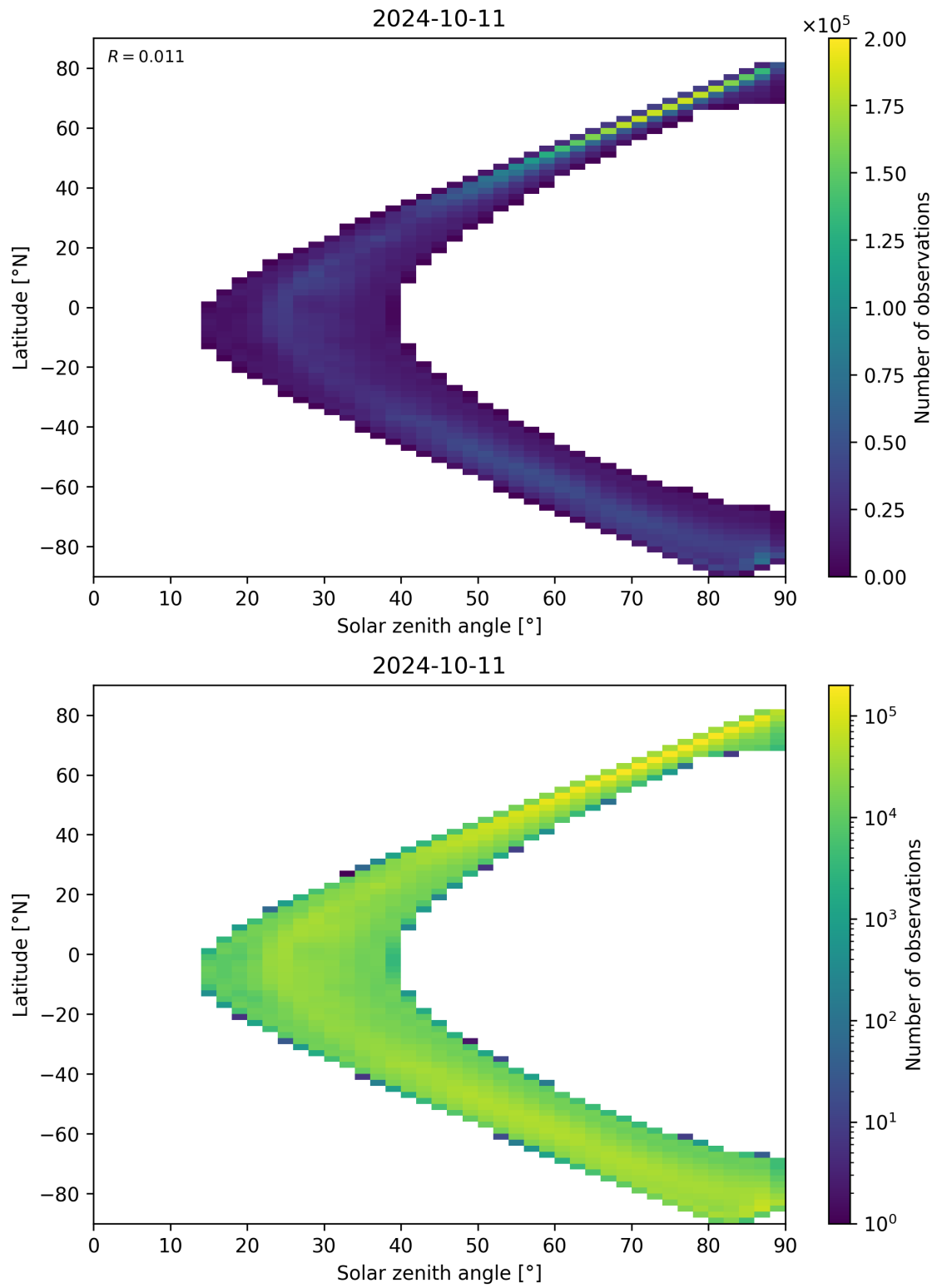
Figure 105: Scatter density plot of “Solar zenith angle” against “Latitude” for 2024-10-10 to 2024-10-12.
