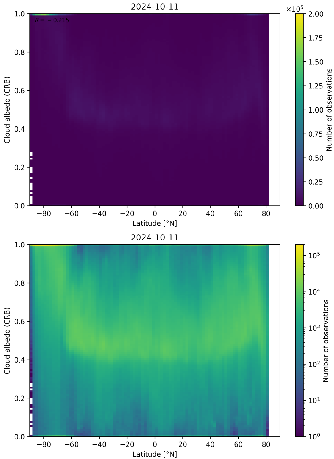
Figure 91: Scatter density plot of “Latitude” against “Cloud albedo (CRB)” for 2024-10-10 to 2024-10-12.
