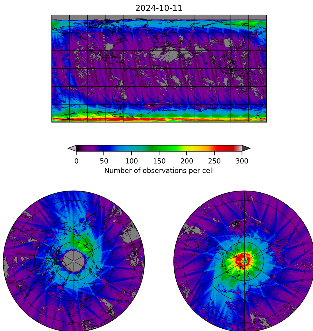
Figure 21: Map of the number of observations for 2024-10-10 to 2024-10-12
