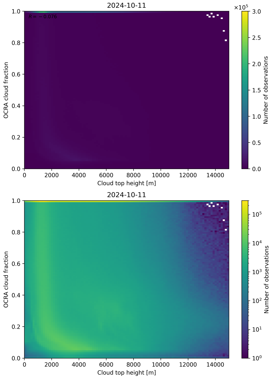
Figure 87: Scatter density plot of “Cloud top height” against “OCRA cloud fraction” for 2024-10-10 to 2024-10-12.
