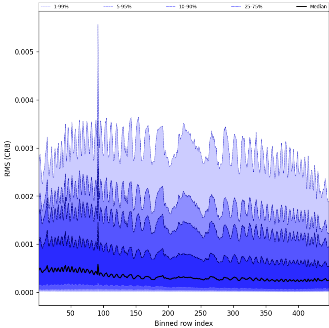
Figure 64: Along track statistics of “RMS (CRB)” for 2024-10-10 to 2024-10-12
