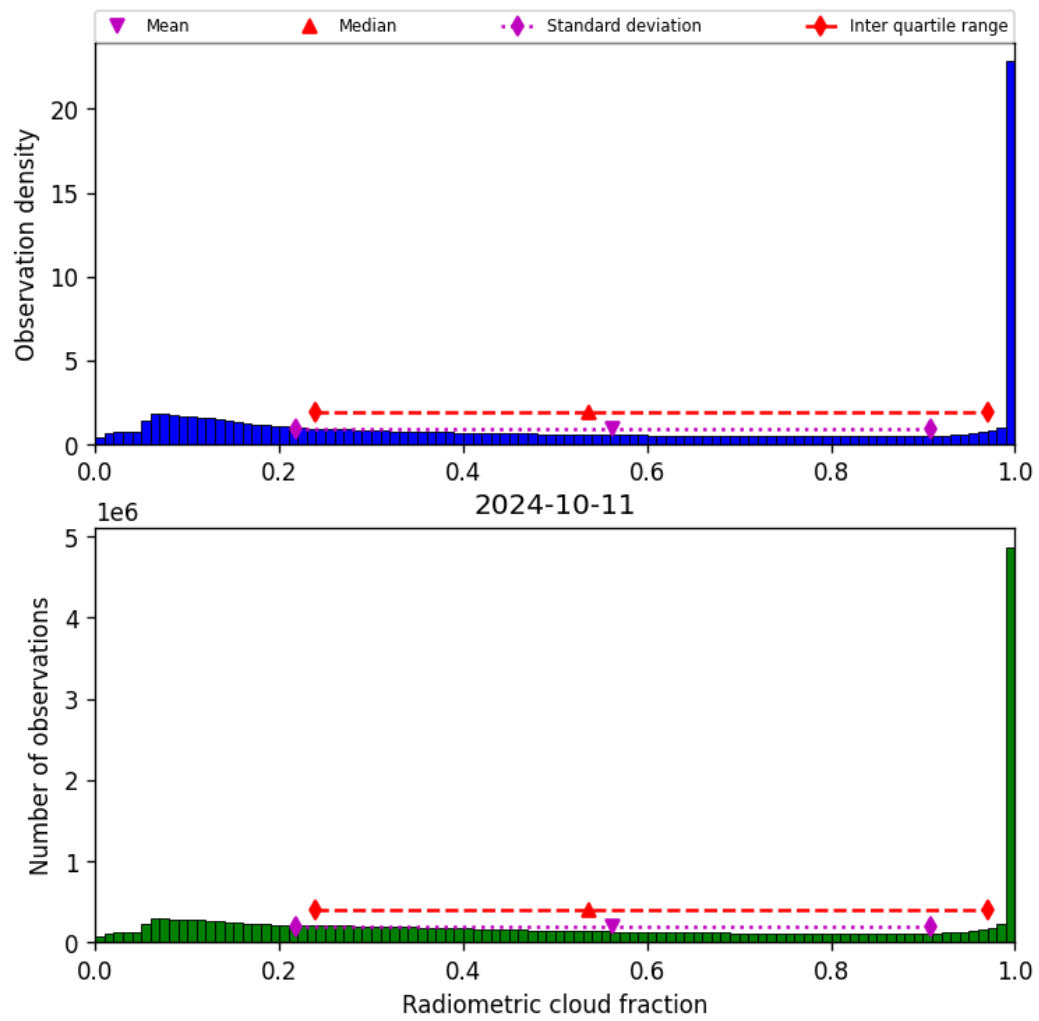
Figure 39: Histogram of “Radiometric cloud fraction” for 2024-10-10 to 2024-10-12
