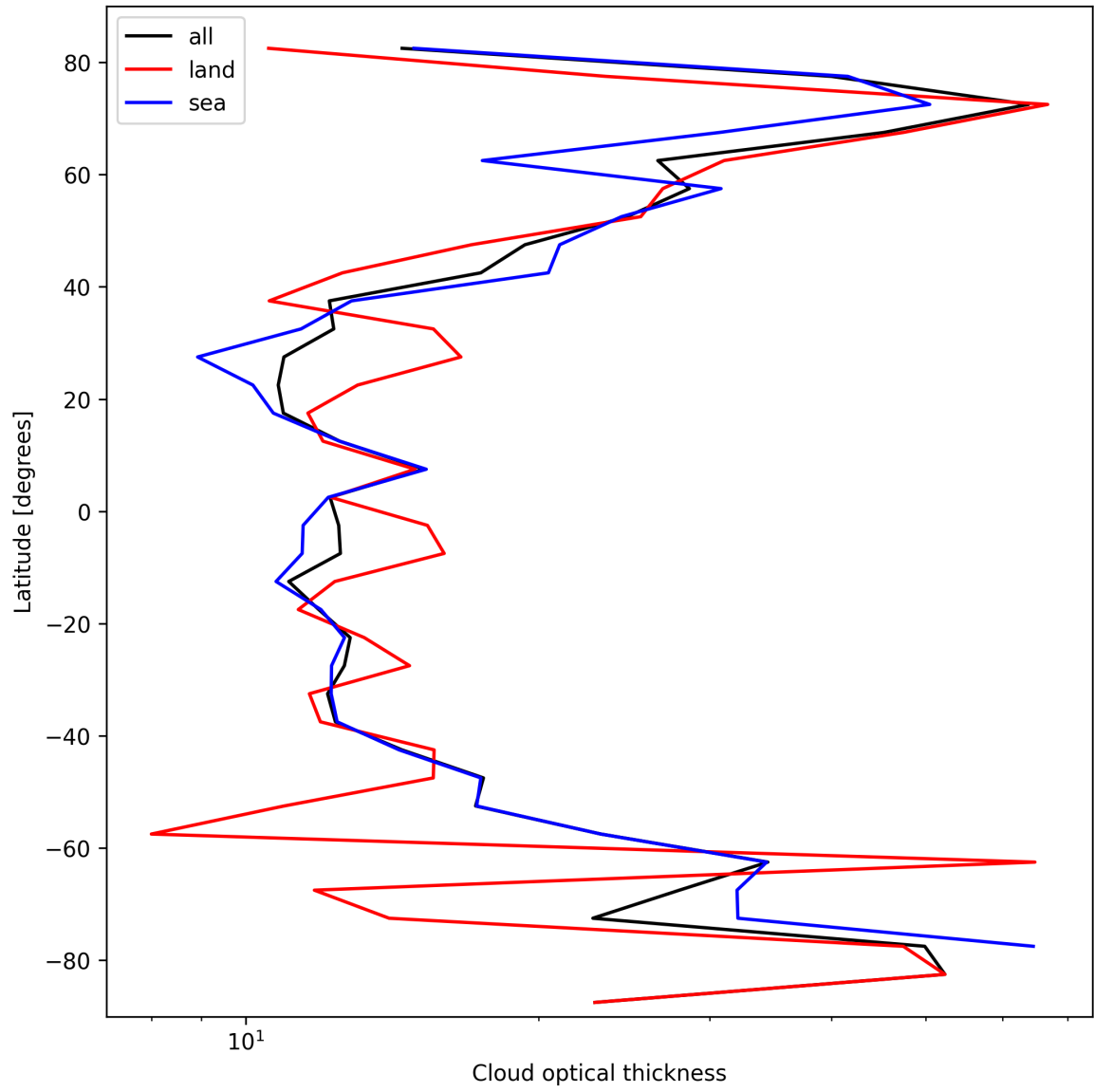
Figure 25: Zonal average of “Cloud optical thickness” for 2024-10-10 to 2024-10-12.
