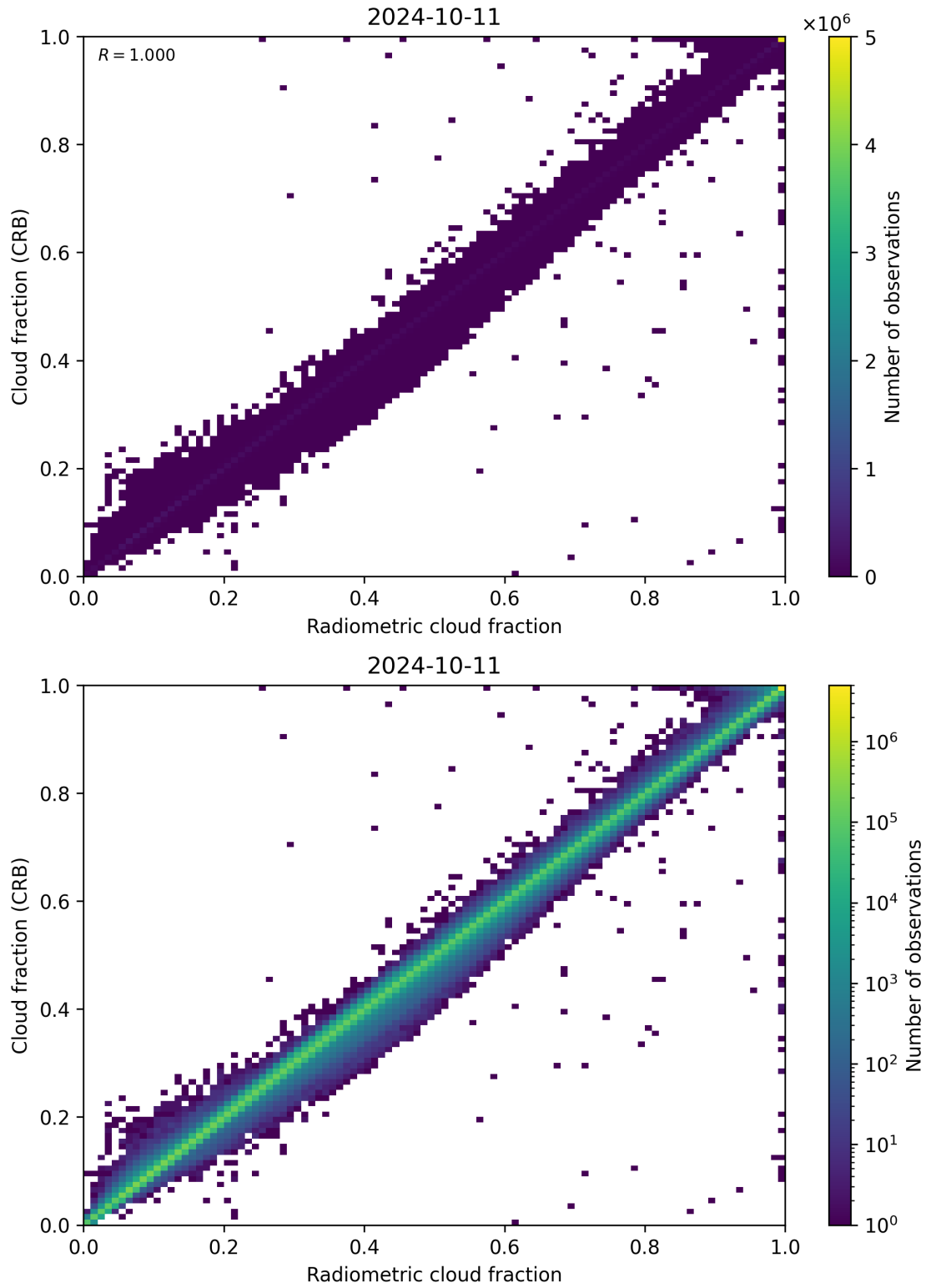
Figure 73: Scatter density plot of “Radiometric cloud fraction” against “Cloud fraction (CRB)” for 2024-10-10 to 2024-10-12.
