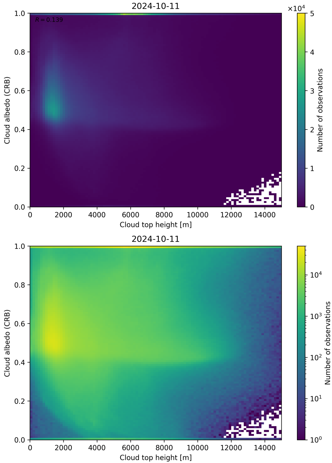
Figure 86: Scatter density plot of “Cloud top height” against “Cloud albedo (CRB)” for 2024-10-10 to 2024-10-12.
