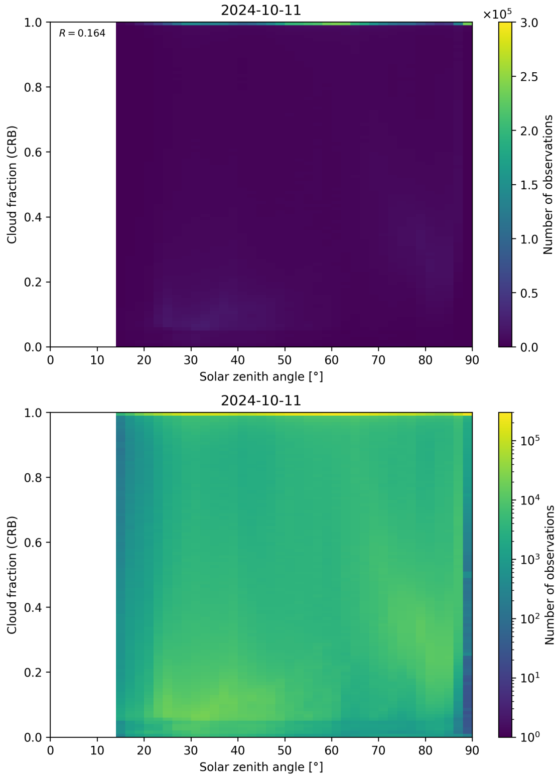
Figure 101: Scatter density plot of “Solar zenith angle” against “Cloud fraction (CRB)” for 2024-10-10 to 2024-10-12.
