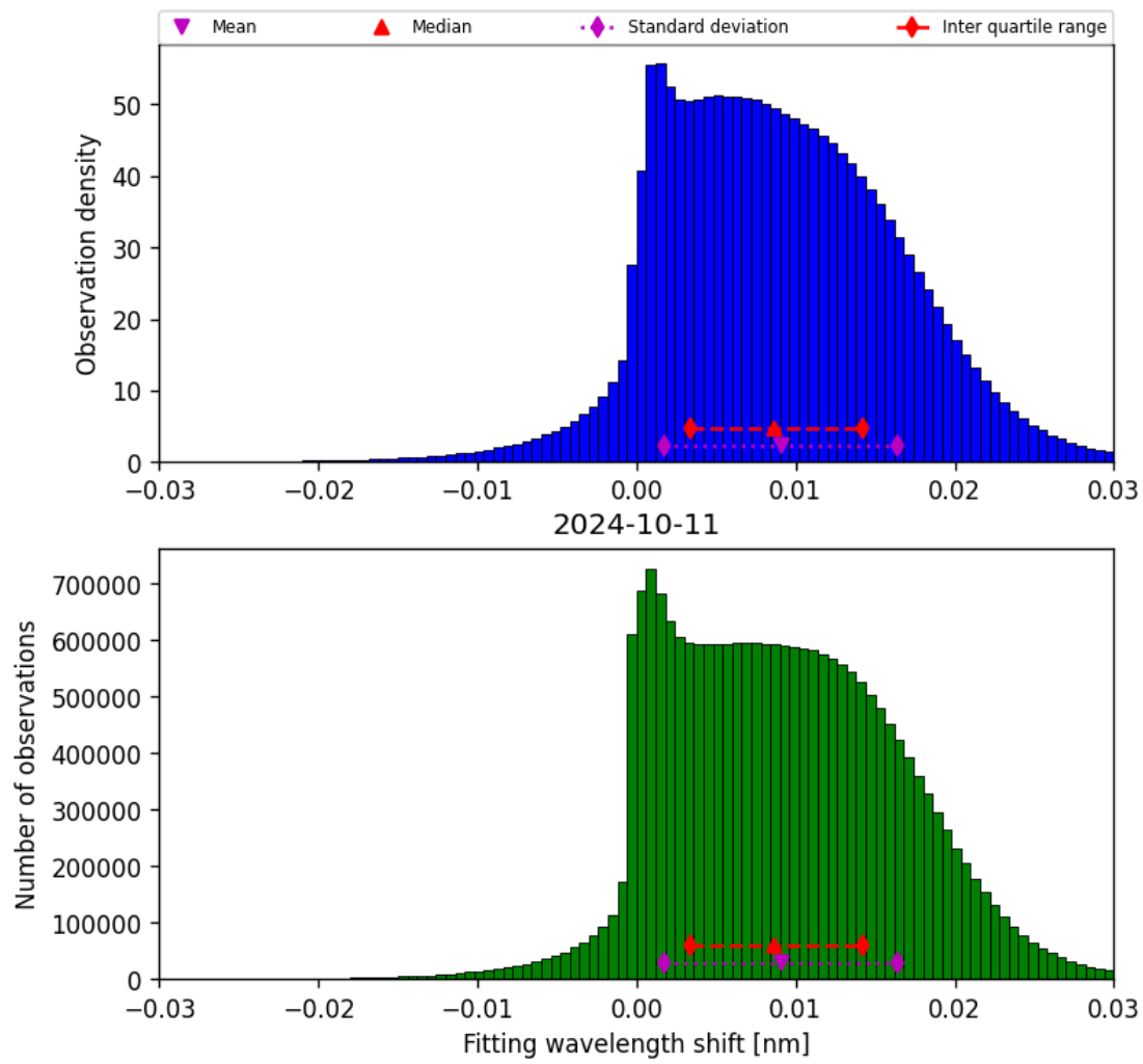
Figure 49: Histogram of “Fitting wavelength shift” for 2024-10-10 to 2024-10-12
