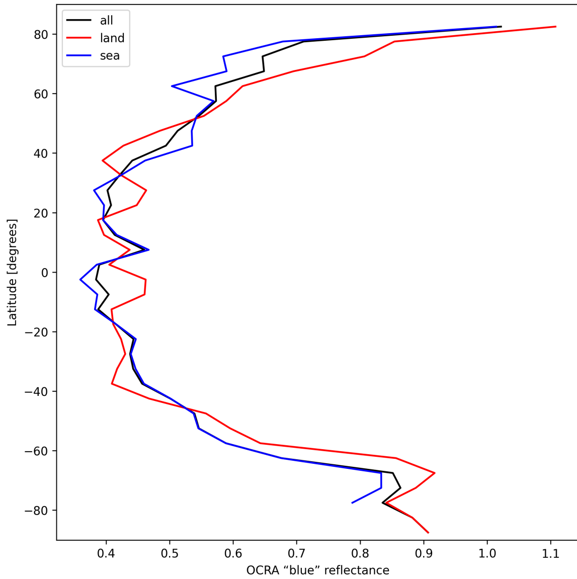
Figure 35: Zonal average of “OCRA “blue” reflectance” for 2024-10-10 to 2024-10-12.
