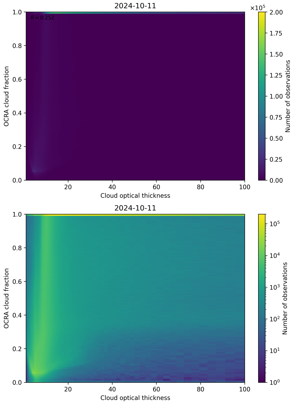
Figure 83: Scatter density plot of “Cloud optical thickness” against “OCRA cloud fraction” for 2024-10-10 to 2024-10-12.
