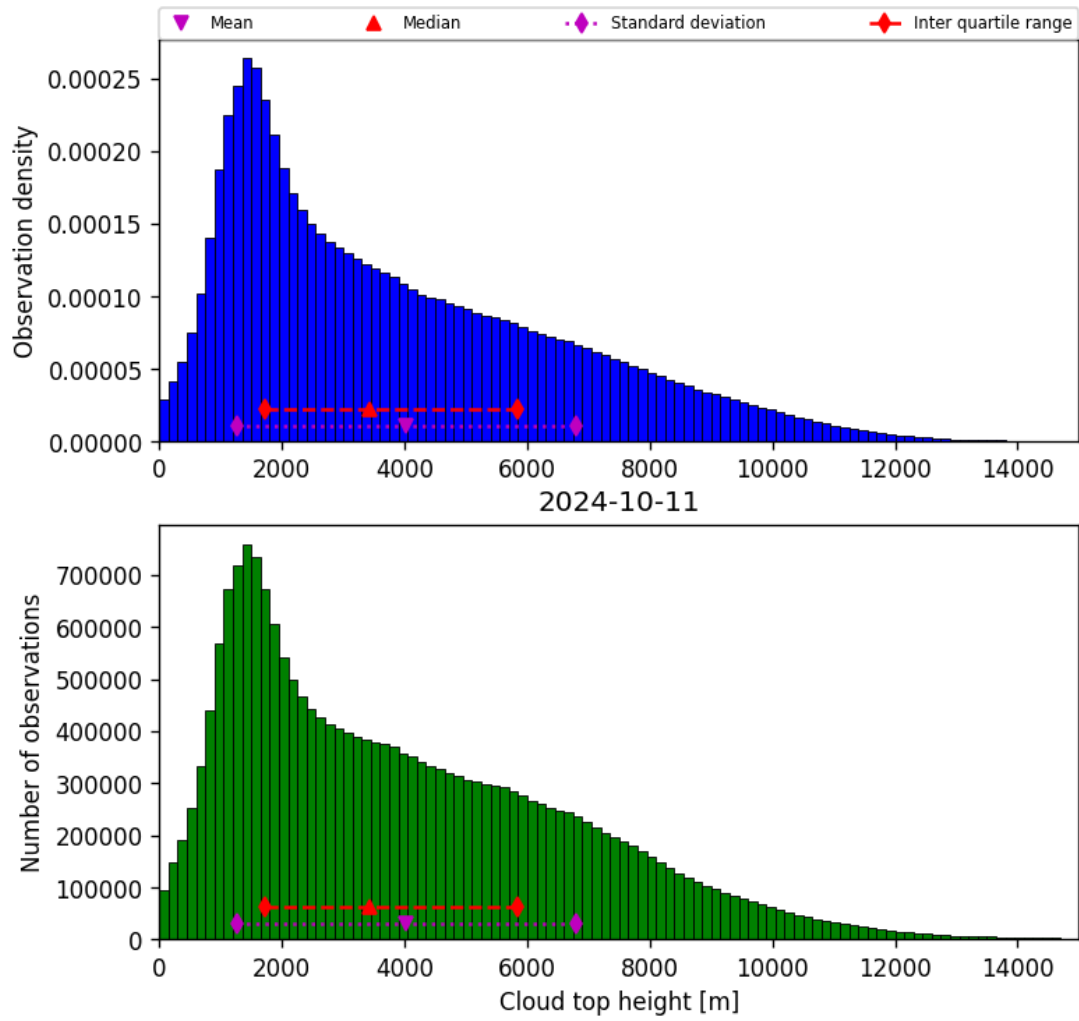
Figure 40: Histogram of “Cloud top height” for 2024-10-10 to 2024-10-12
