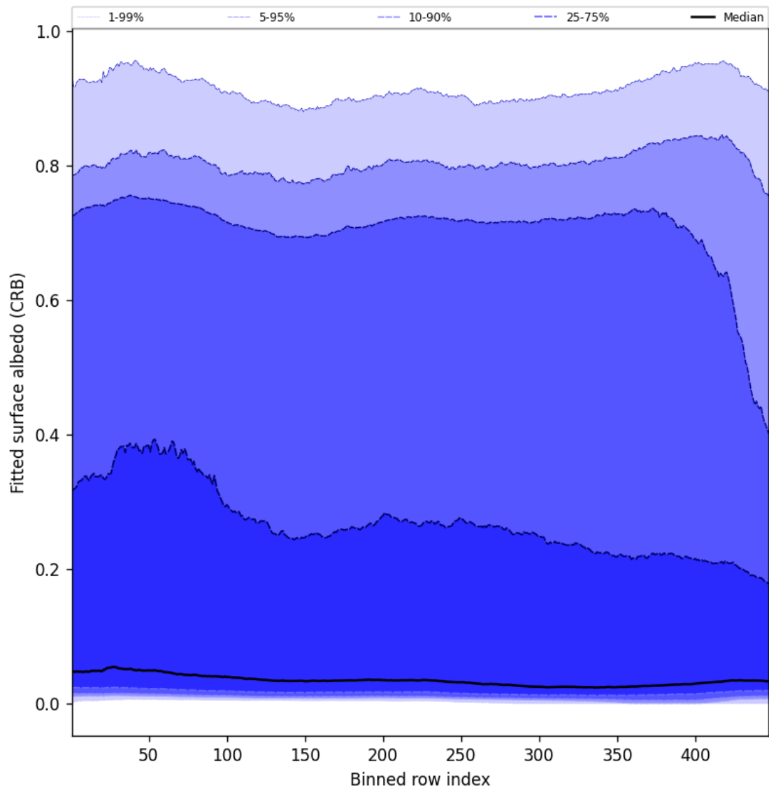
Figure 62: Along track statistics of “Fitted surface albedo (CRB)” for 2024-10-10 to 2024-10-12
