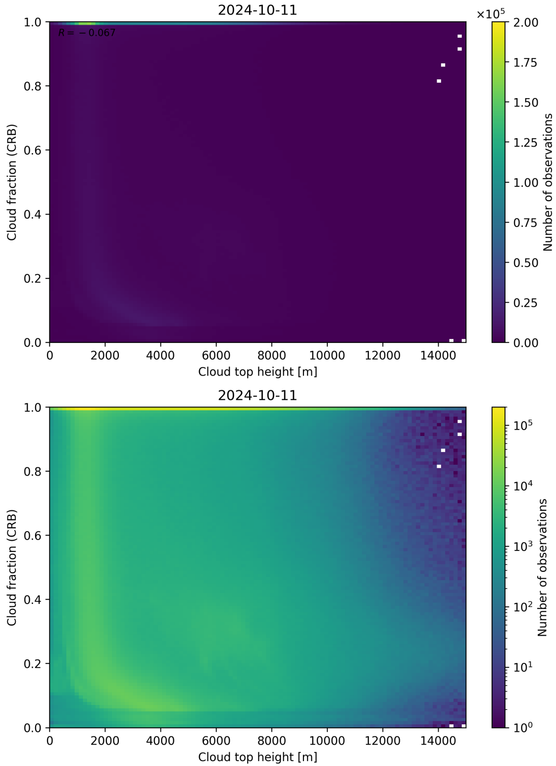
Figure 88: Scatter density plot of “Cloud top height” against “Cloud fraction (CRB)” for 2024-10-10 to 2024-10-12.
