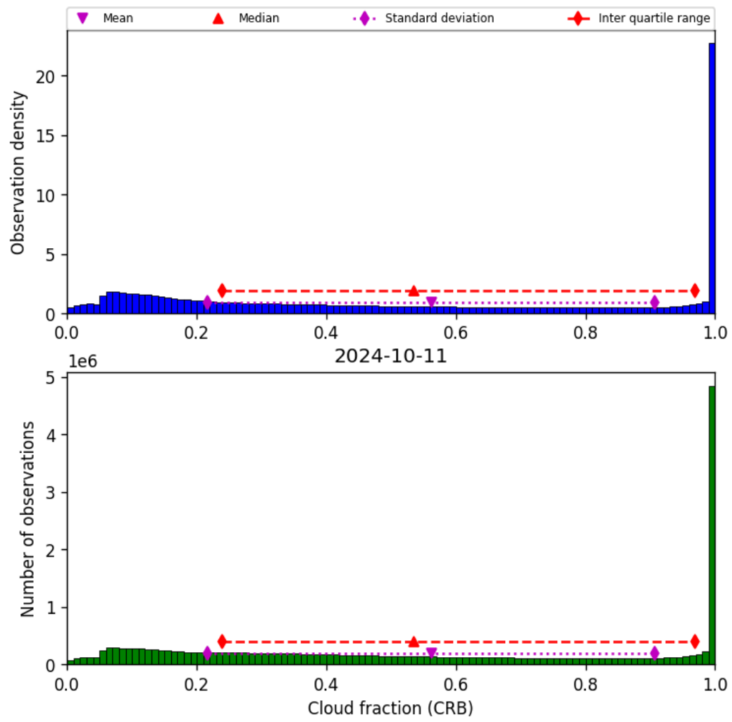
Figure 42: Histogram of “Cloud fraction (CRB)” for 2024-10-10 to 2024-10-12
