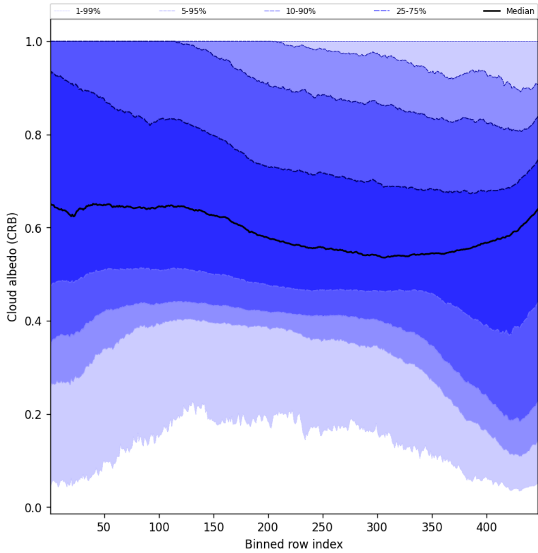
Figure 60: Along track statistics of “Cloud albedo (CRB)” for 2024-10-10 to 2024-10-12
