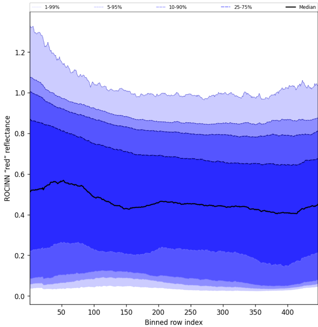
Figure 69: Along track statistics of “ROCINN “red” reflectance” for 2024-10-10 to 2024-10-12
