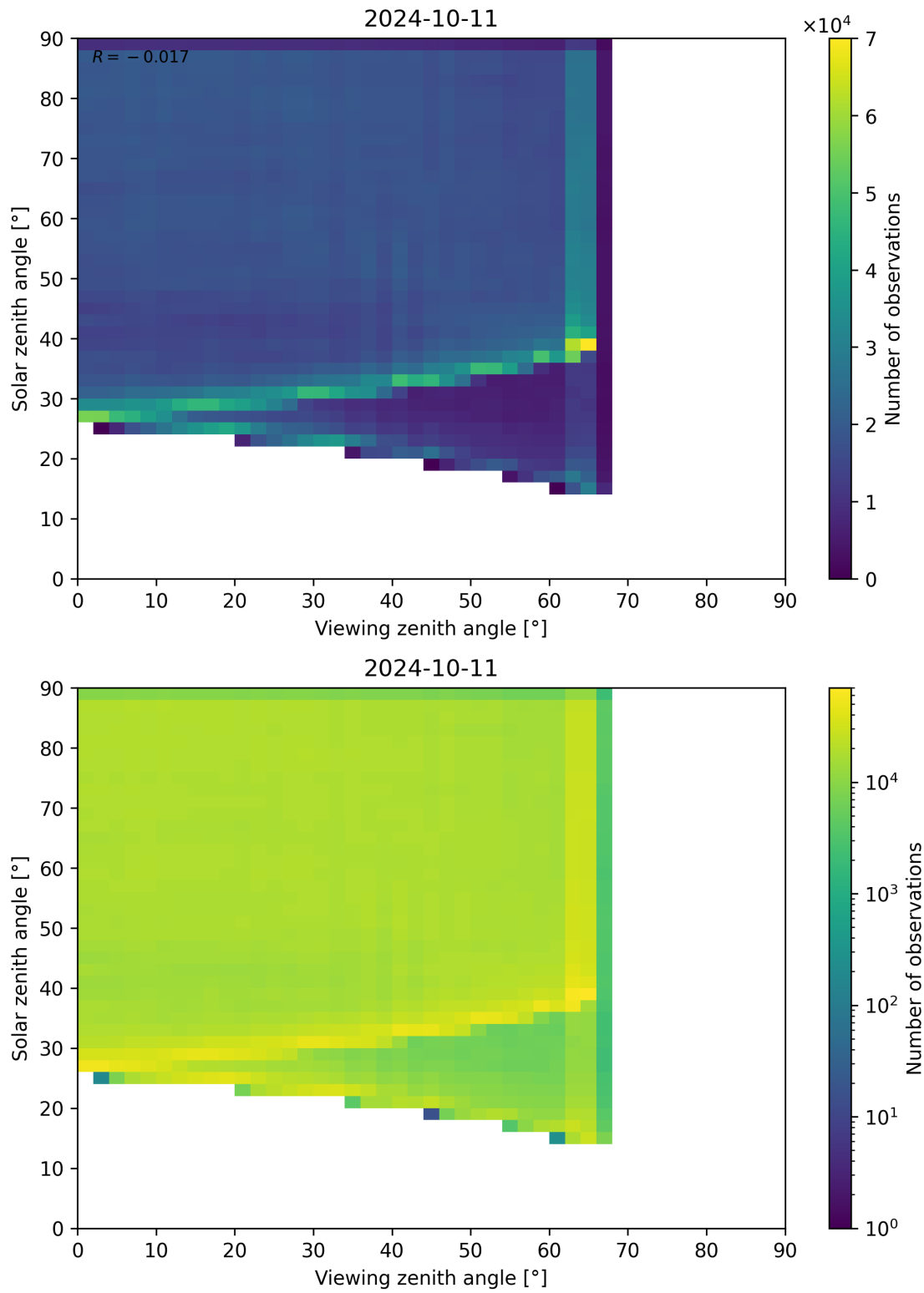
Figure 114: Scatter density plot of “Viewing zenith angle” against “Solar zenith angle” for 2024-10-10 to 2024-10-12.
