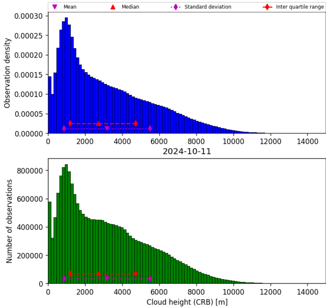
Figure 43: Histogram of “Cloud height (CRB)” for 2024-10-10 to 2024-10-12
