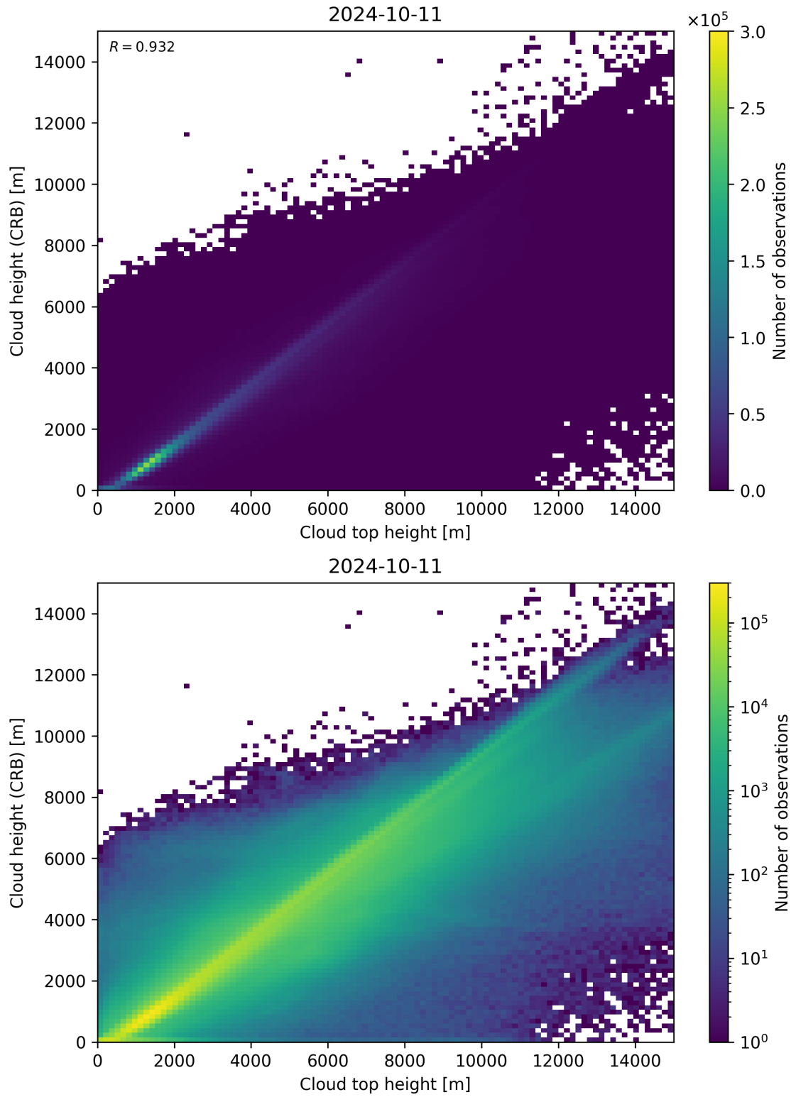
Figure 89: Scatter density plot of “Cloud top height” against “Cloud height (CRB)” for 2024-10-10 to 2024-10-12.
