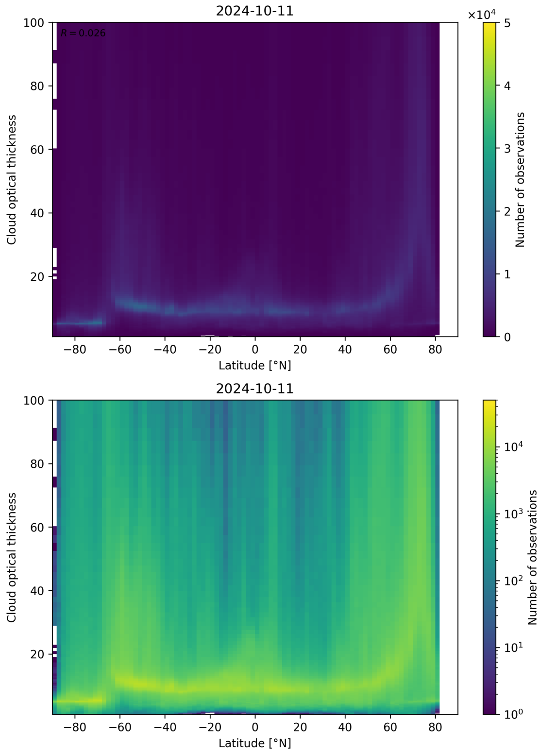
Figure 96: Scatter density plot of “Latitude” against “Cloud optical thickness” for 2024-10-10 to 2024-10-12.
