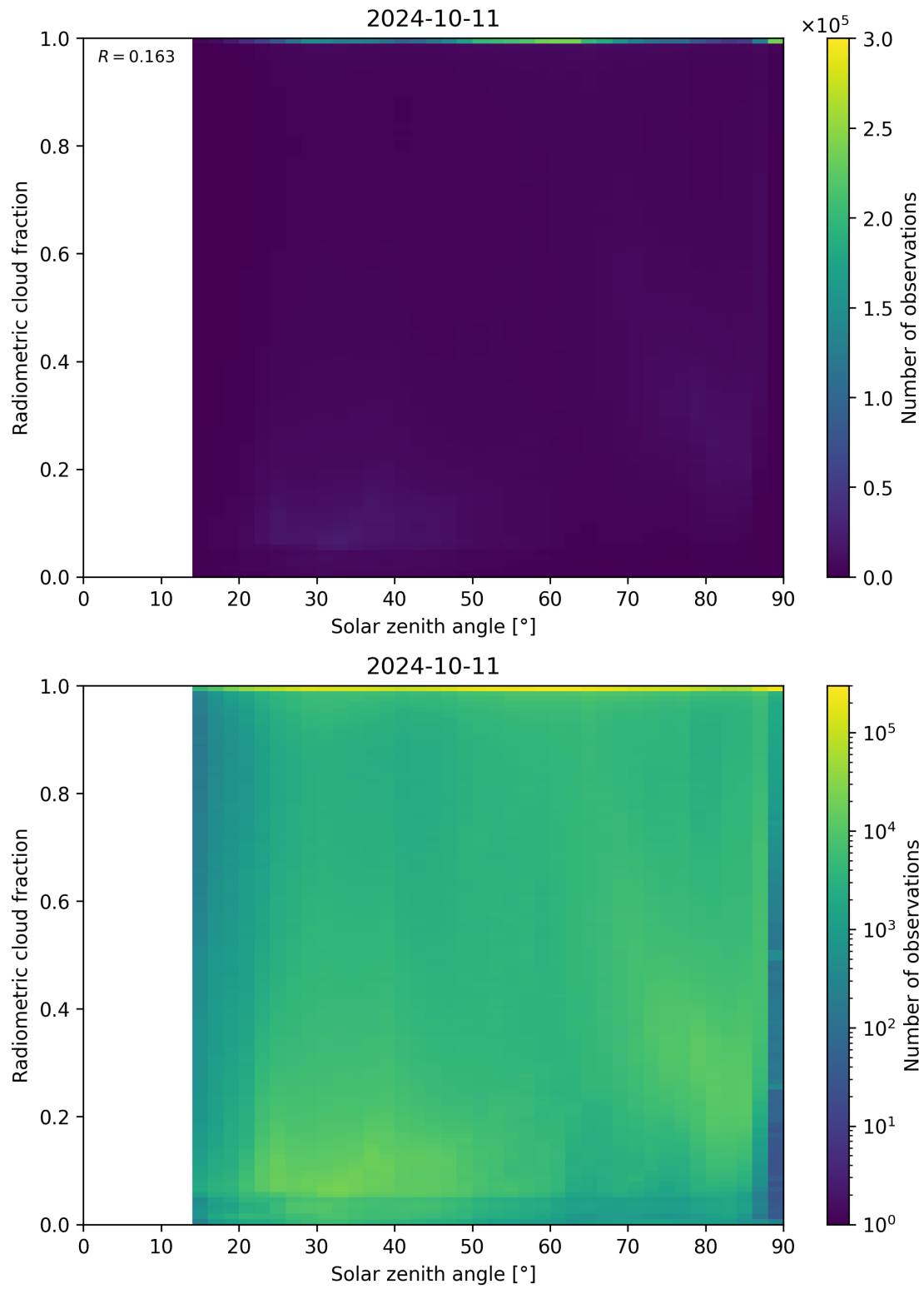
Figure 99: Scatter density plot of “Solar zenith angle” against “Radiometric cloud fraction” for 2024-10-10 to 2024-10-12.
