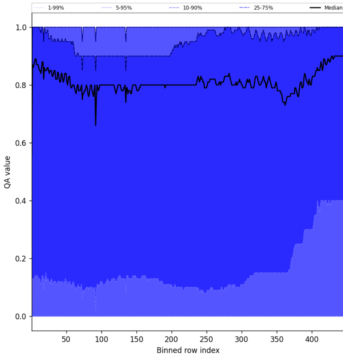
Figure 54: Along track statistics of "QA value" for 2024-10-10 to 2024-10-12
