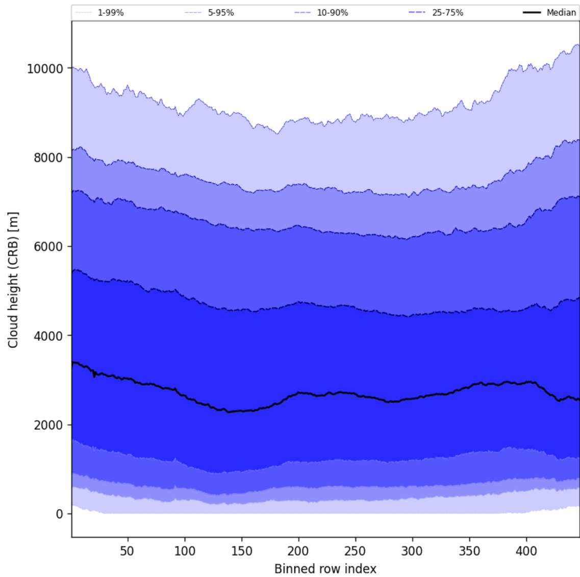
Figure 59: Along track statistics of “Cloud height (CRB)” for 2024-10-10 to 2024-10-12
