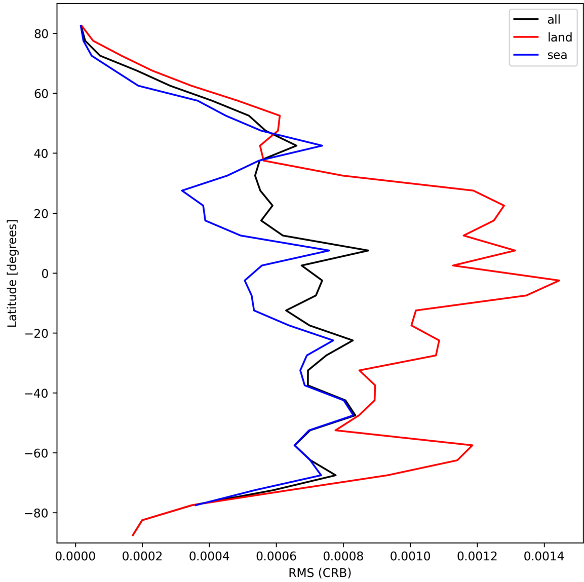
Figure 32: Zonal average of “RMS (CRB)” for 2024-10-10 to 2024-10-12.
