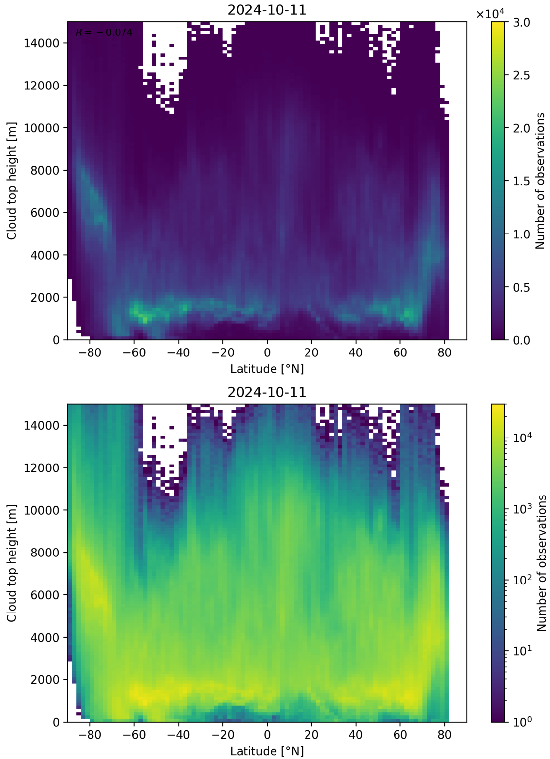
Figure 97: Scatter density plot of “Latitude” against “Cloud top height” for 2024-10-10 to 2024-10-12.
