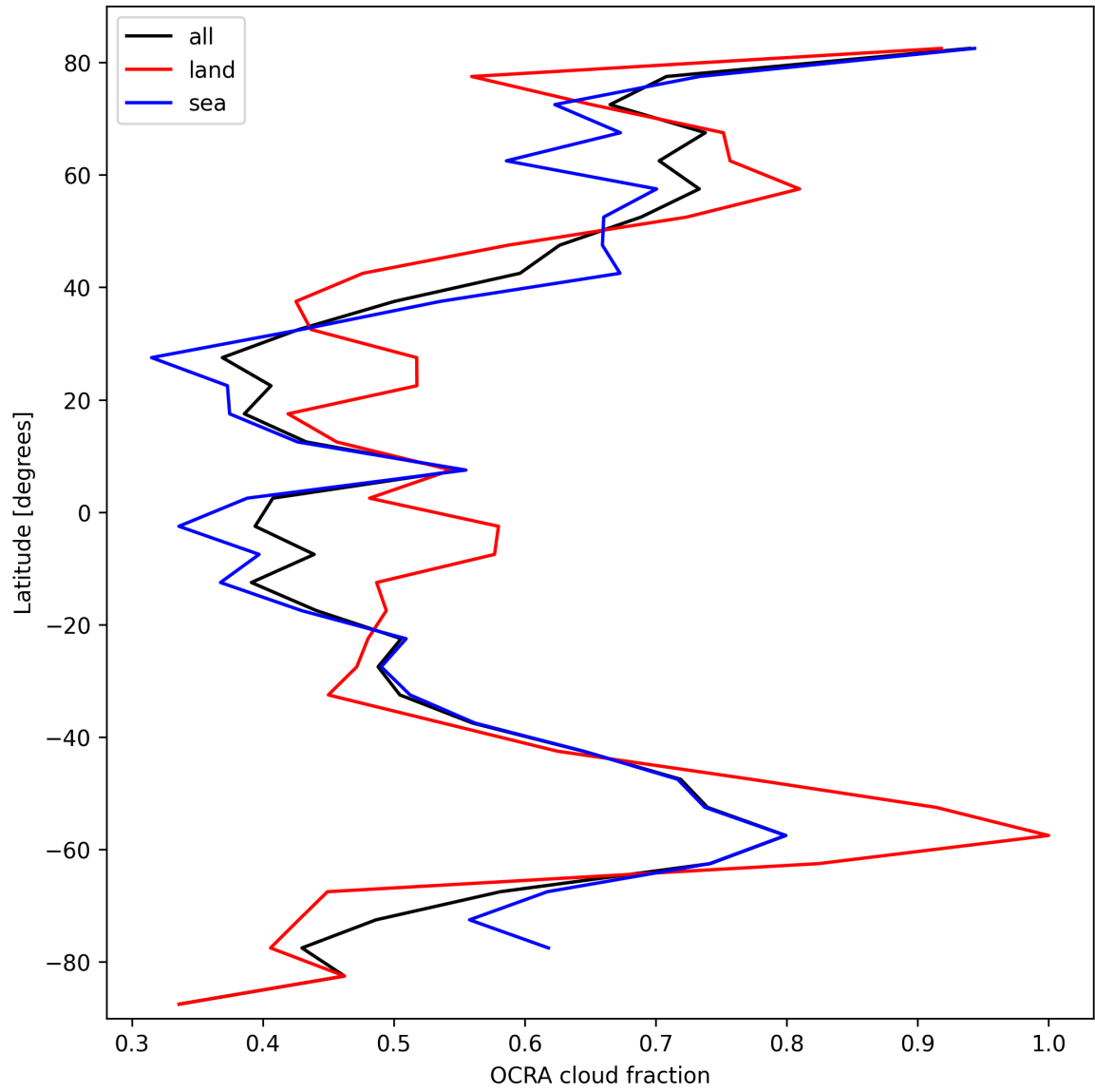
Figure 34: Zonal average of “OCRA cloud fraction” for 2024-10-10 to 2024-10-12.
