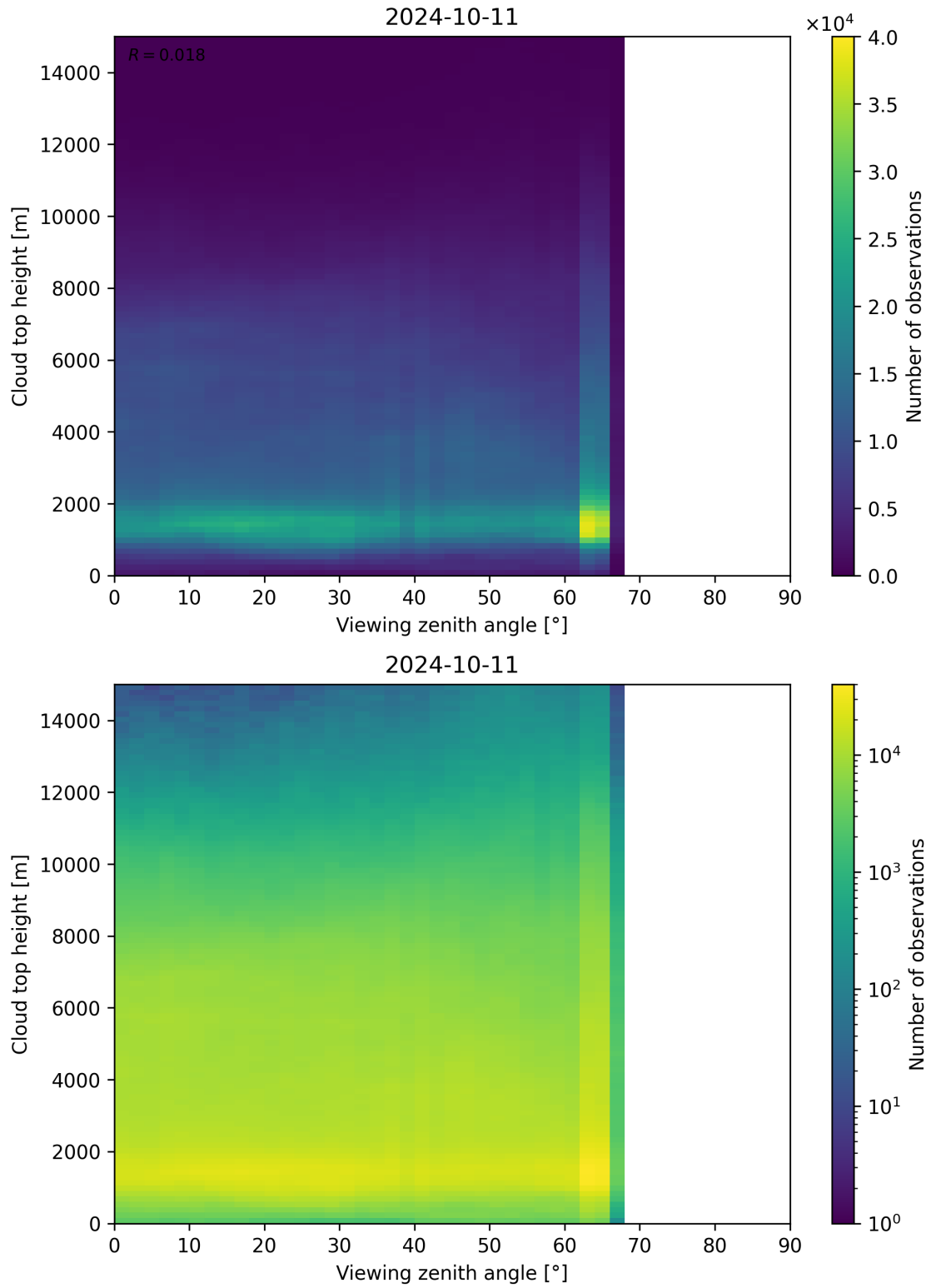
Figure 112: Scatter density plot of “Viewing zenith angle” against “Cloud top height” for 2024-10-10 to 2024-10-12.
