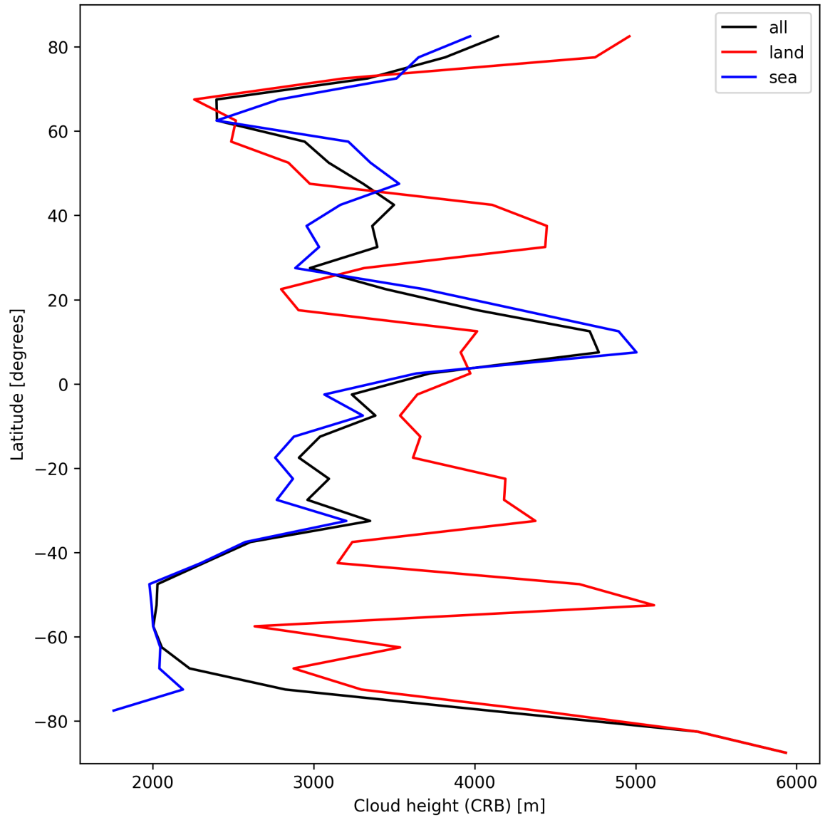
Figure 27: Zonal average of “Cloud height (CRB)” for 2024-10-10 to 2024-10-12.
