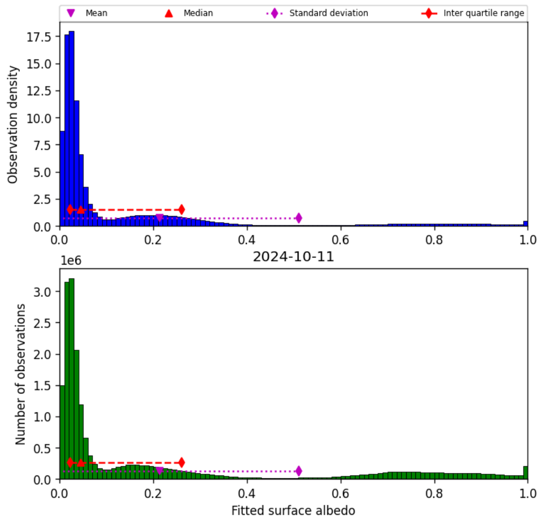
Figure 45: Histogram of “Fitted surface albedo” for 2024-10-10 to 2024-10-12
