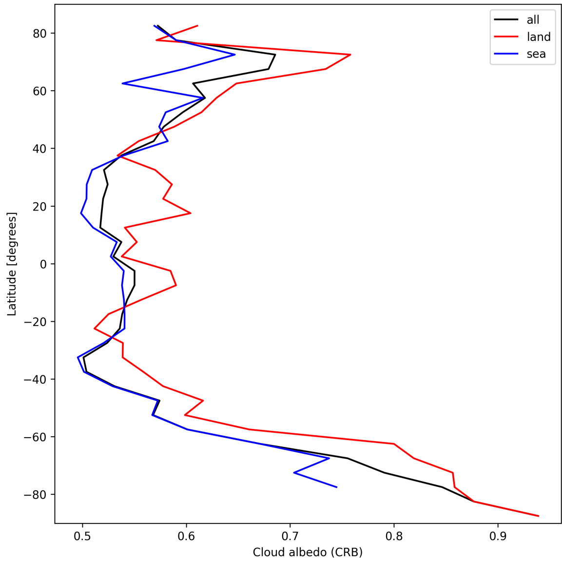
Figure 28: Zonal average of “Cloud albedo (CRB)” for 2024-10-10 to 2024-10-12.
