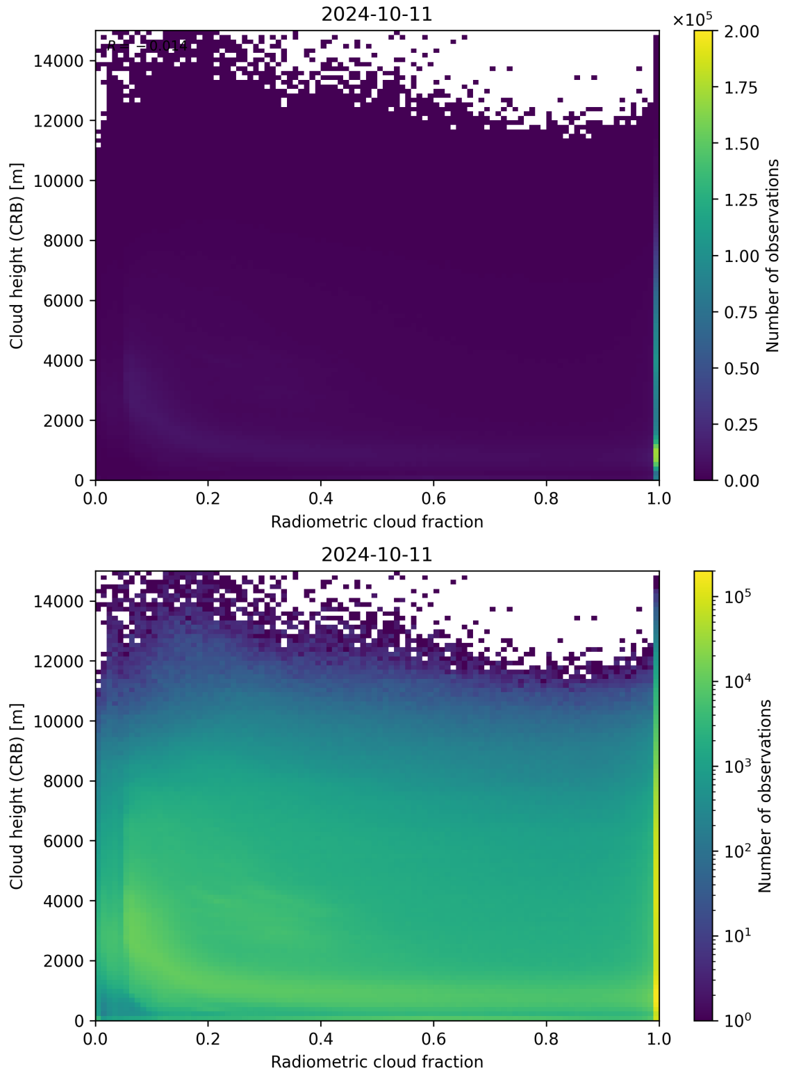
Figure 74: Scatter density plot of “Radiometric cloud fraction” against “Cloud height (CRB)” for 2024-10-10 to 2024-10-12.
