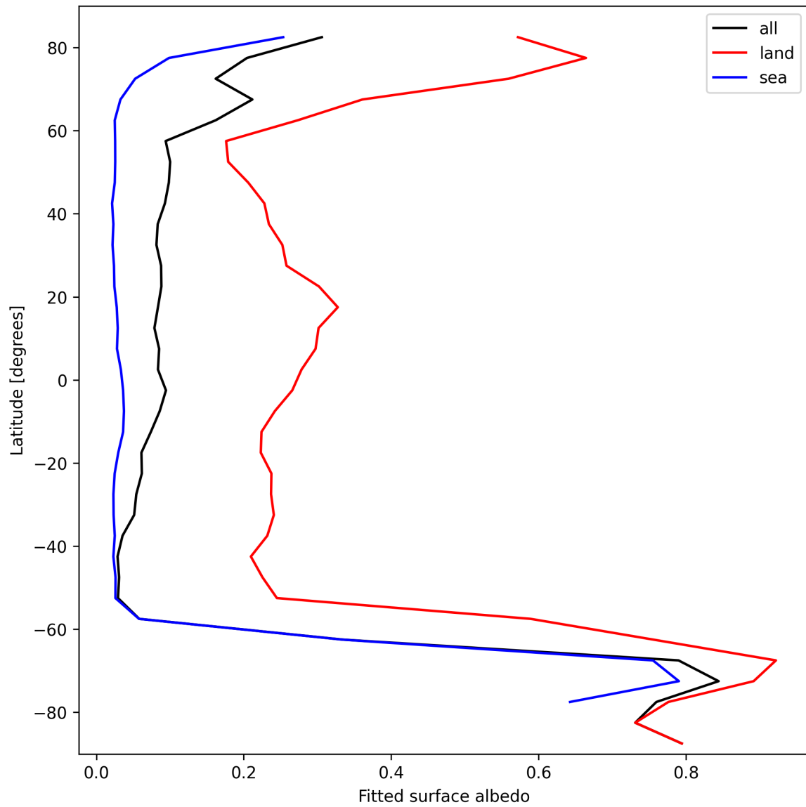
Figure 29: Zonal average of “Fitted surface albedo” for 2024-10-10 to 2024-10-12.
