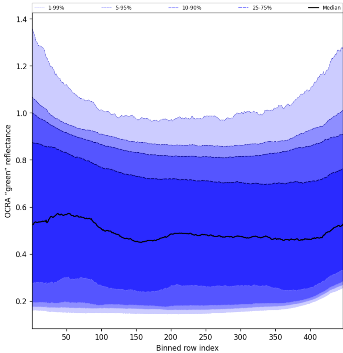
Figure 68: Along track statistics of “OCRA “green” reflectance” for 2024-10-10 to 2024-10-12
