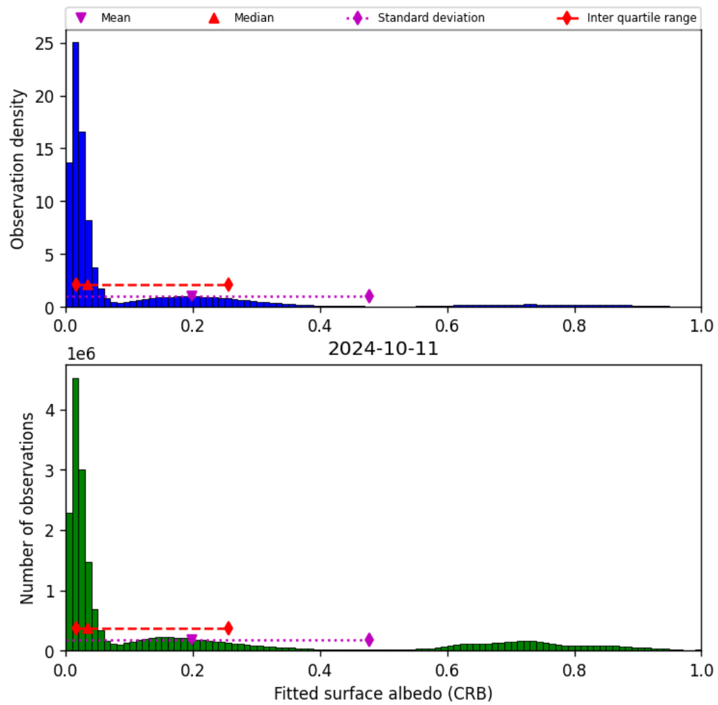
Figure 46: Histogram of “Fitted surface albedo (CRB)” for 2024-10-10 to 2024-10-12
