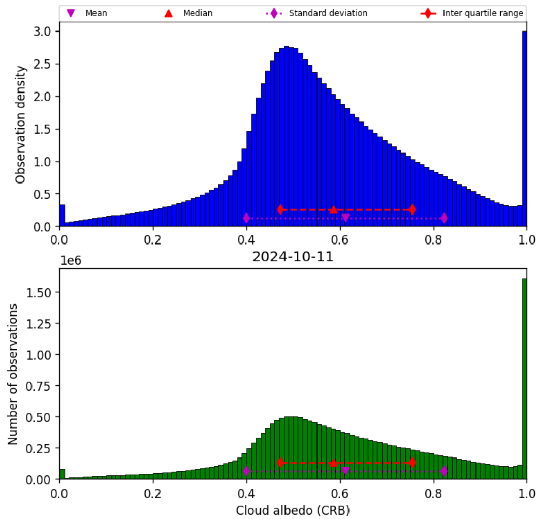
Figure 44: Histogram of “Cloud albedo (CRB)” for 2024-10-10 to 2024-10-12
