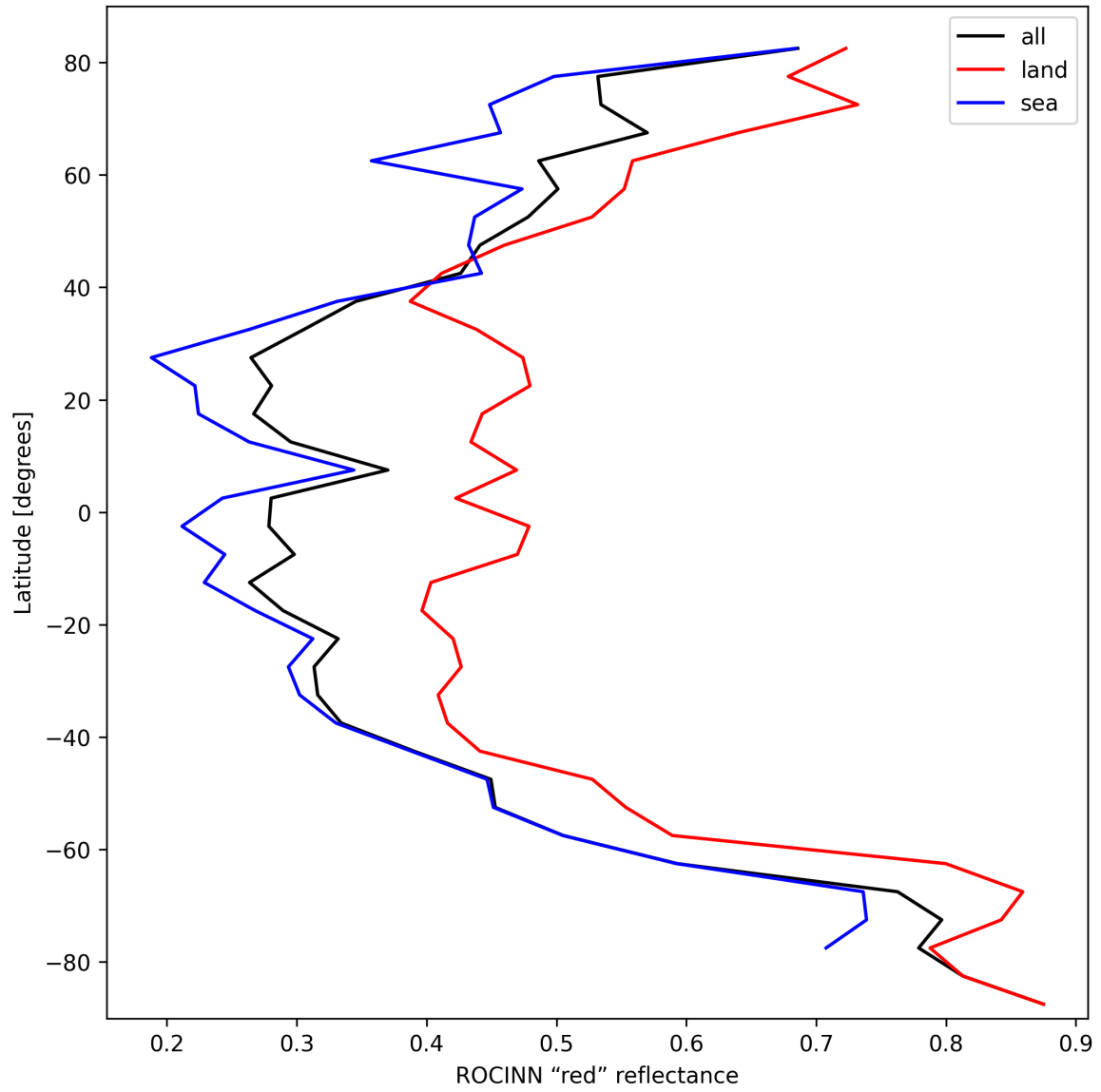
Figure 37: Zonal average of “ROCINN “red” reflectance” for 2024-10-10 to 2024-10-12.
