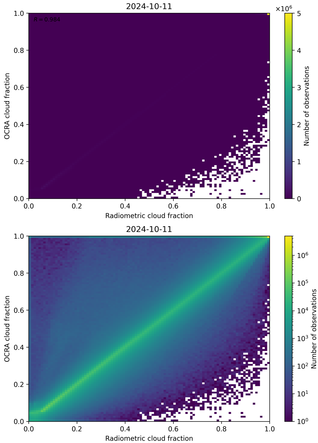
Figure 72: Scatter density plot of “Radiometric cloud fraction” against “OCRA cloud fraction” for 2024-10-10 to 2024-10-12.
