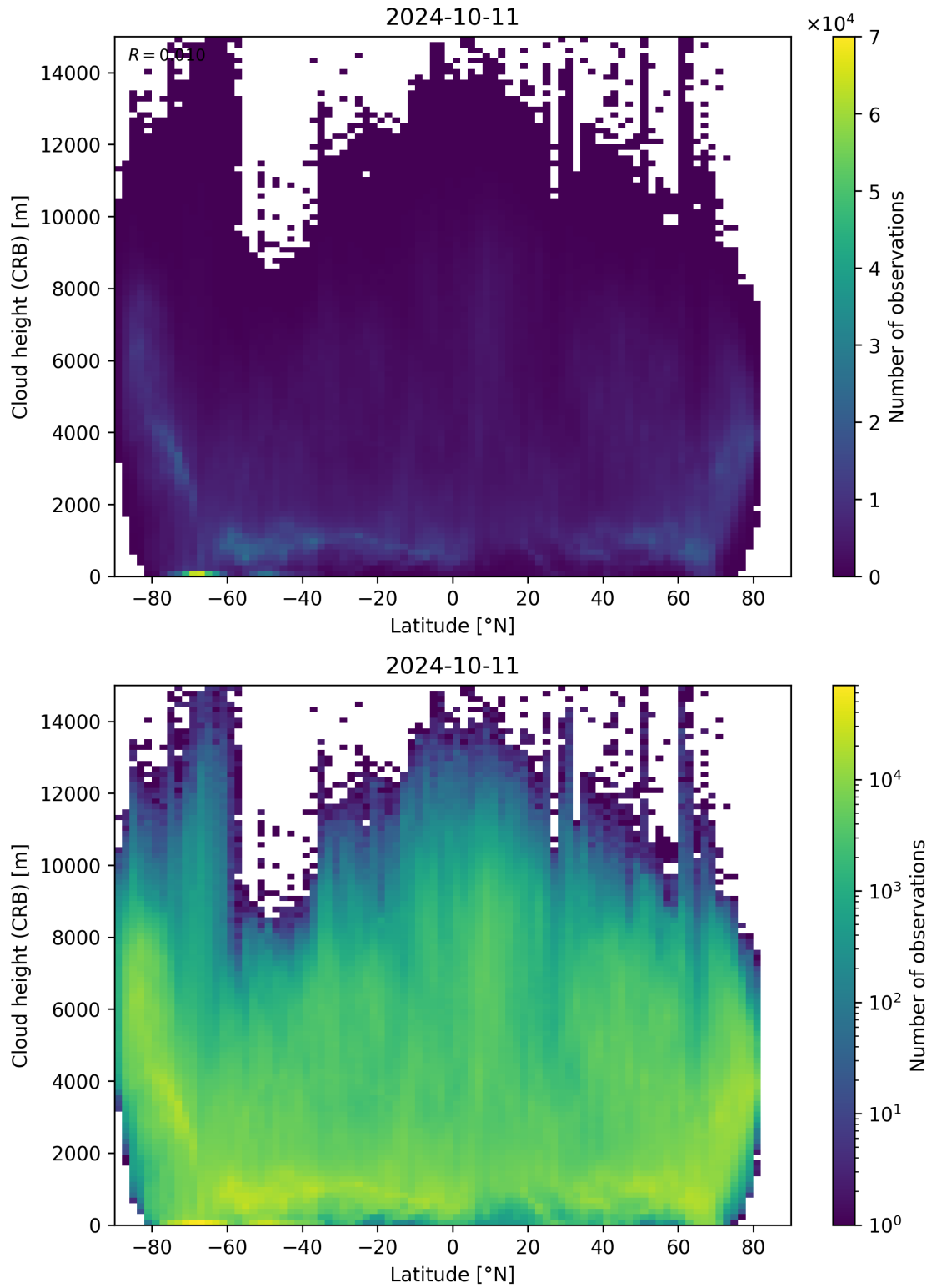
Figure 95: Scatter density plot of “Latitude” against “Cloud height (CRB)” for 2024-10-10 to 2024-10-12.
