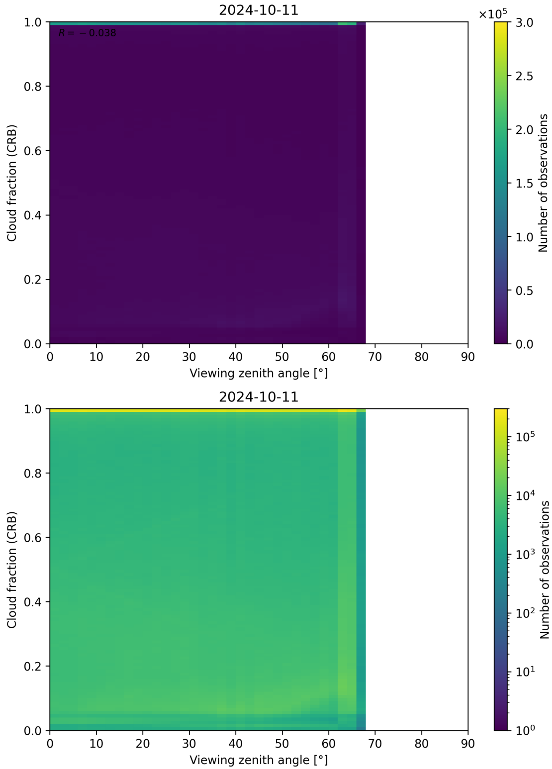
Figure 109: Scatter density plot of “Viewing zenith angle” against “Cloud fraction (CRB)” for 2024-10-10 to 2024-10-12.
