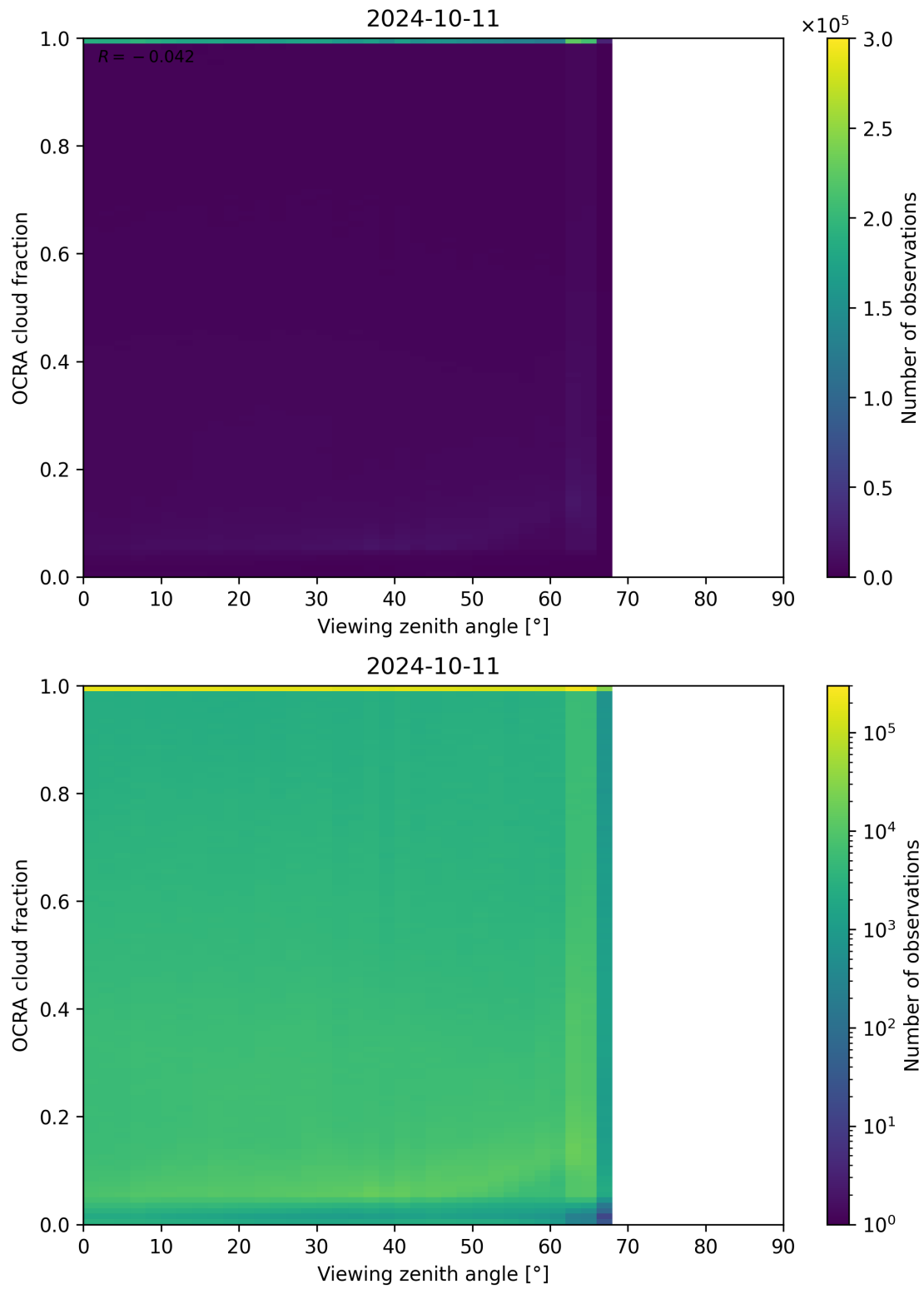
Figure 108: Scatter density plot of “Viewing zenith angle” against “OCRA cloud fraction” for 2024-10-10 to 2024-10-12.
