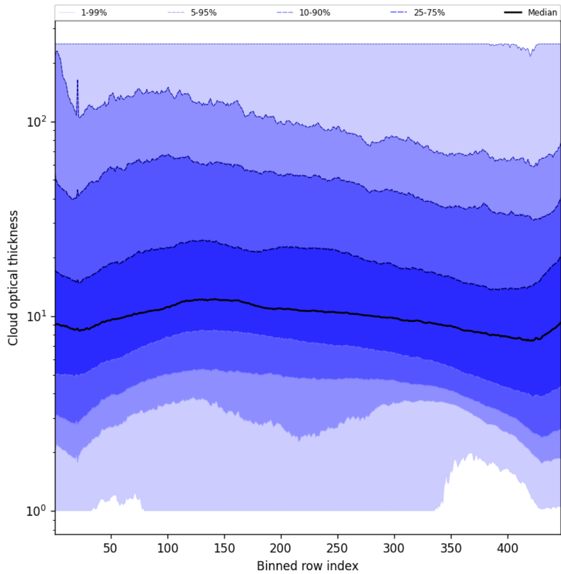
Figure 57: Along track statistics of “Cloud optical thickness” for 2024-10-10 to 2024-10-12
