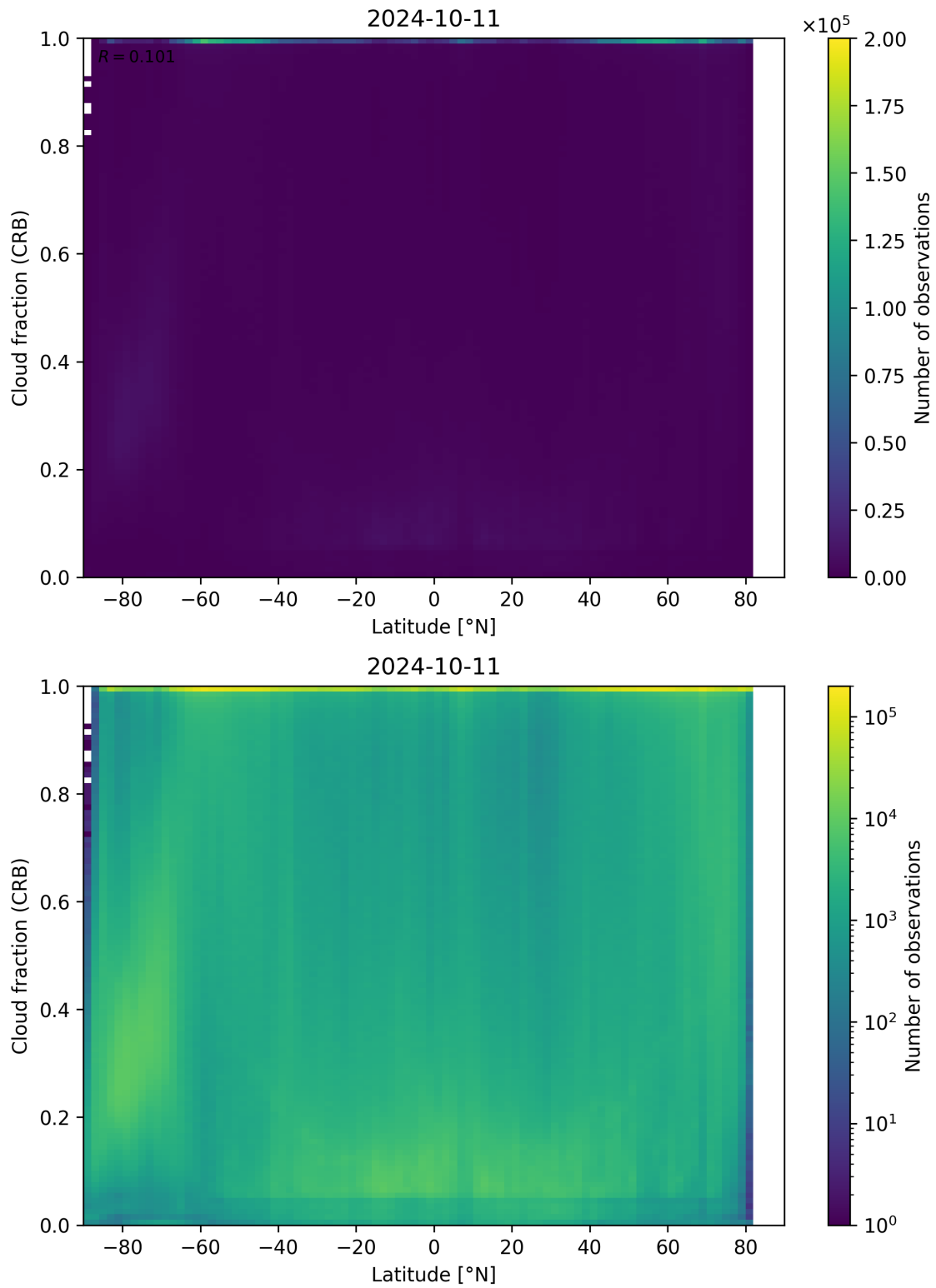
Figure 94: Scatter density plot of “Latitude” against “Cloud fraction (CRB)” for 2024-10-10 to 2024-10-12.
