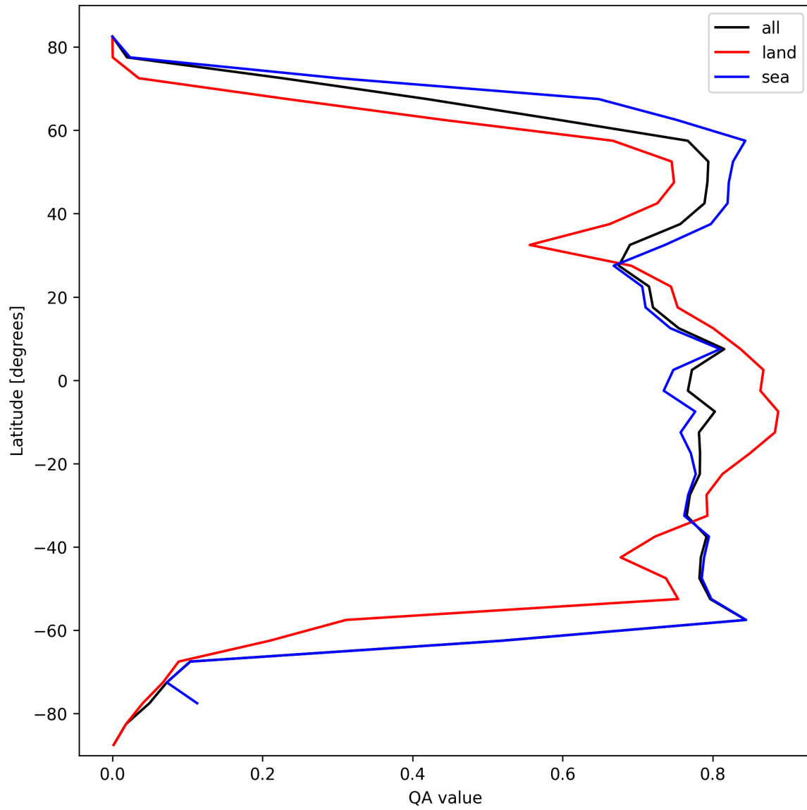
Figure 22: Zonal average of “QA value” for 2024-10-10 to 2024-10-12.
