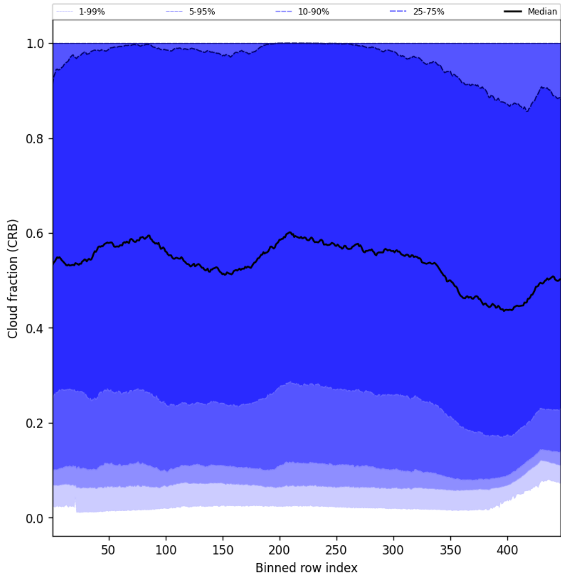
Figure 58: Along track statistics of “Cloud fraction (CRB)” for 2024-10-10 to 2024-10-12
