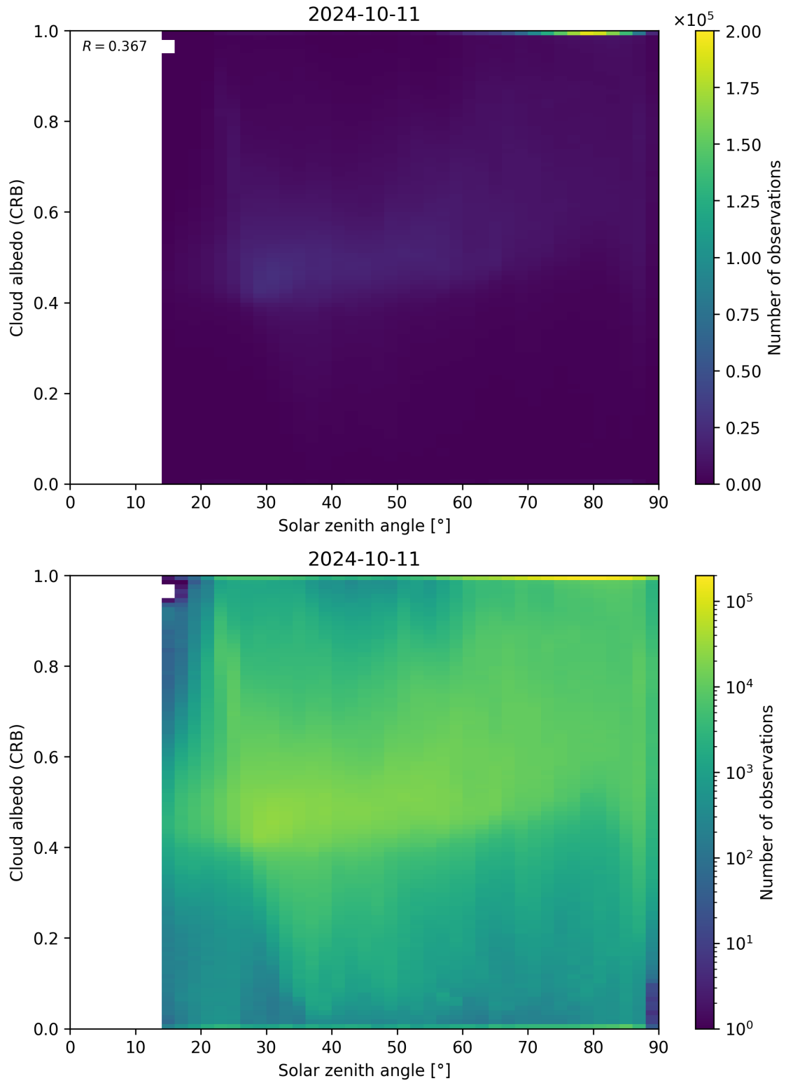
Figure 98: Scatter density plot of “Solar zenith angle” against “Cloud albedo (CRB)” for 2024-10-10 to 2024-10-12.
