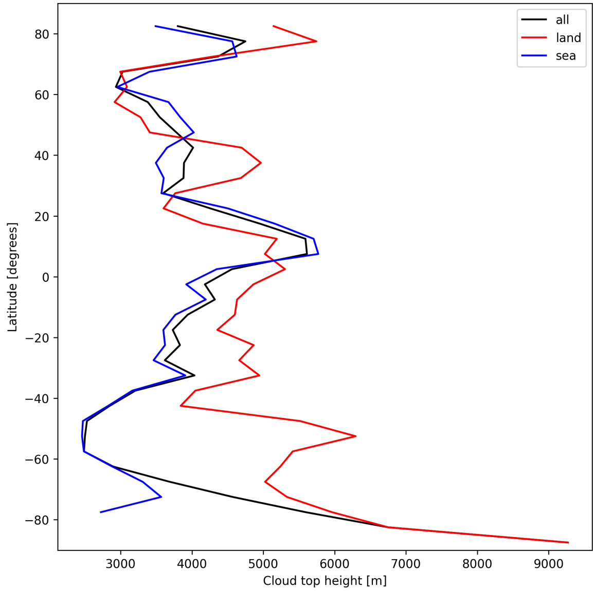
Figure 24: Zonal average of “Cloud top height” for 2024-10-10 to 2024-10-12.
