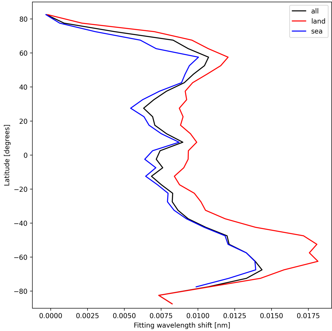
Figure 33: Zonal average of “Fitting wavelength shift” for 2024-10-10 to 2024-10-12.
