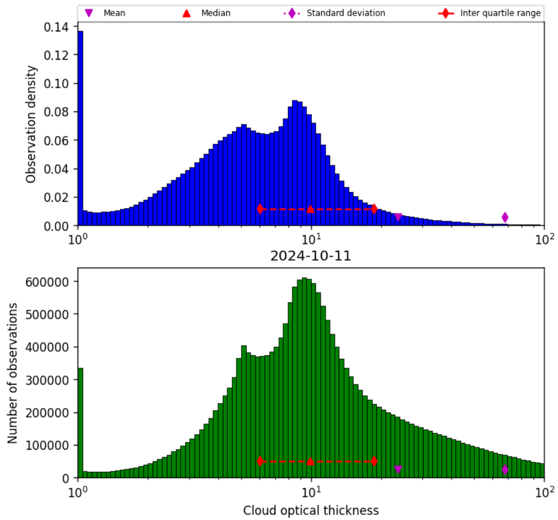
Figure 41: Histogram of “Cloud optical thickness” for 2024-10-10 to 2024-10-12
