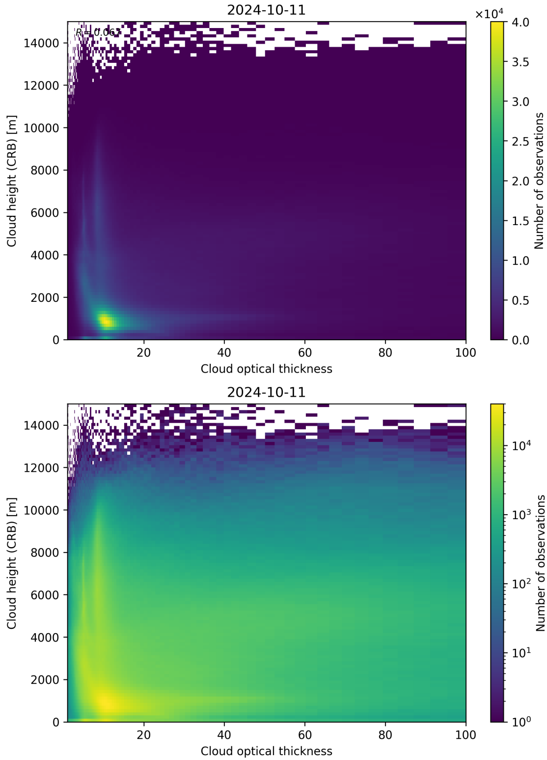
Figure 85: Scatter density plot of “Cloud optical thickness” against “Cloud height (CRB)” for 2024-10-10 to 2024-10-12.
