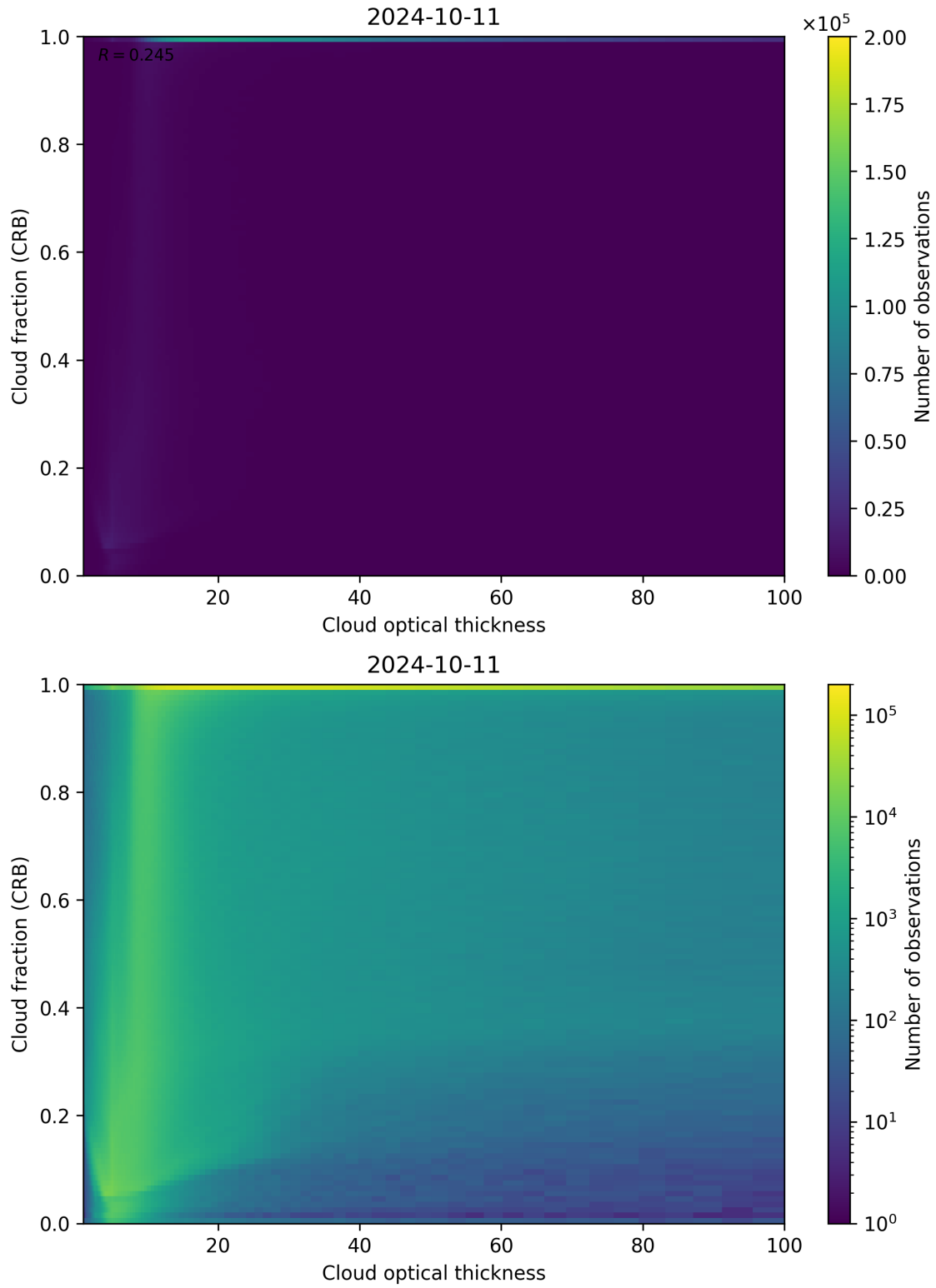
Figure 84: Scatter density plot of “Cloud optical thickness” against “Cloud fraction (CRB)” for 2024-10-10 to 2024-10-12.
