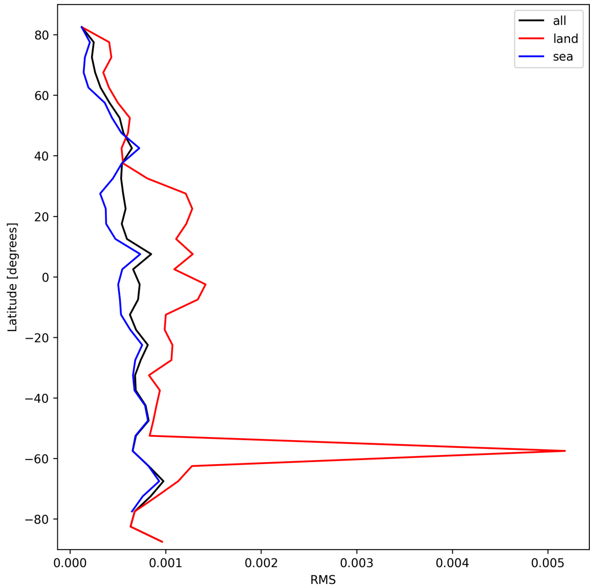
Figure 31: Zonal average of “RMS” for 2024-10-10 to 2024-10-12.
