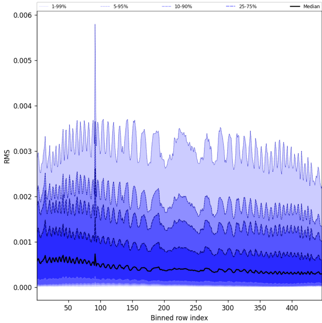
Figure 63: Along track statistics of “RMS” for 2024-10-10 to 2024-10-12
