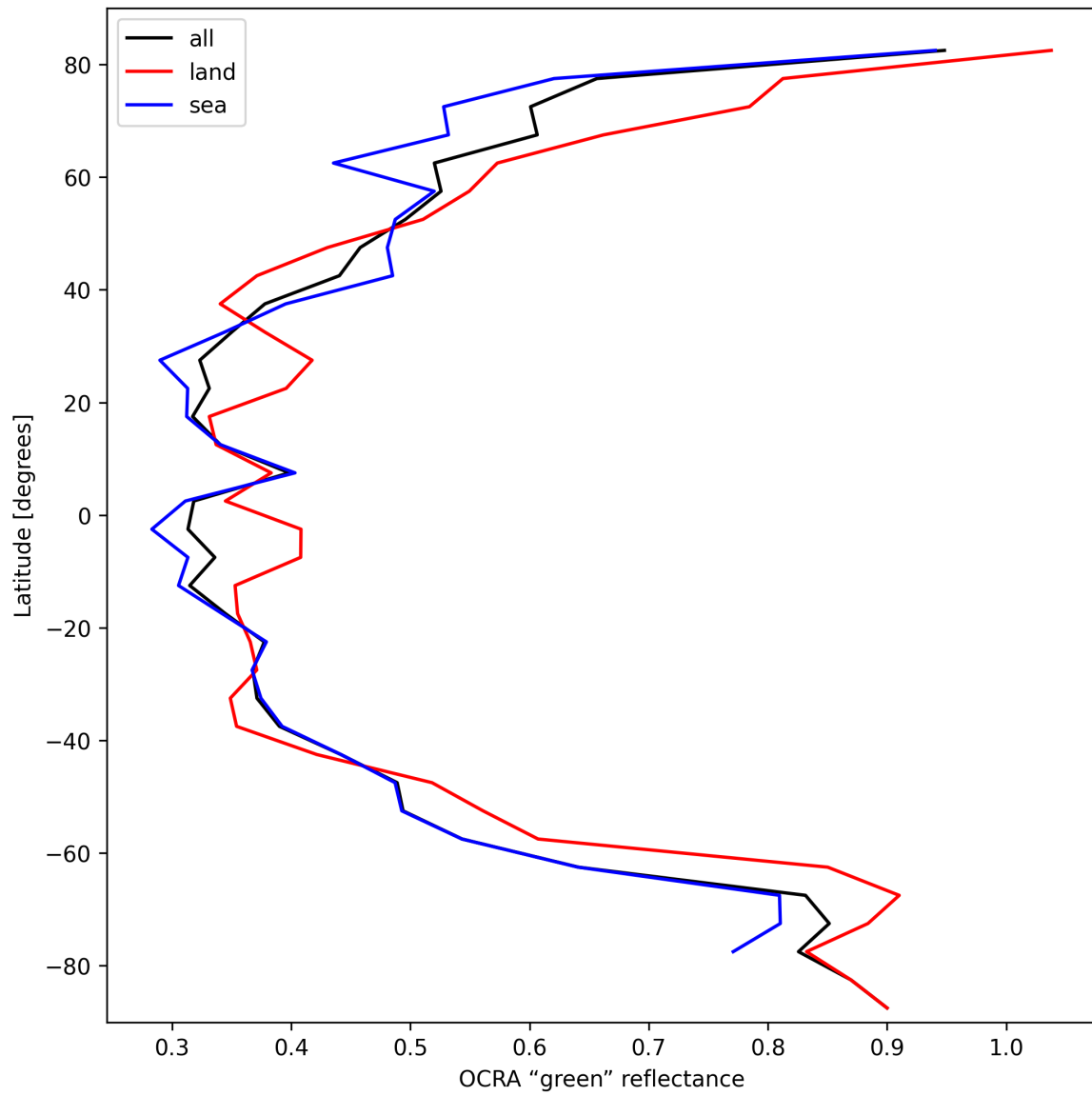
Figure 36: Zonal average of “OCRA “green” reflectance” for 2024-10-10 to 2024-10-12.
