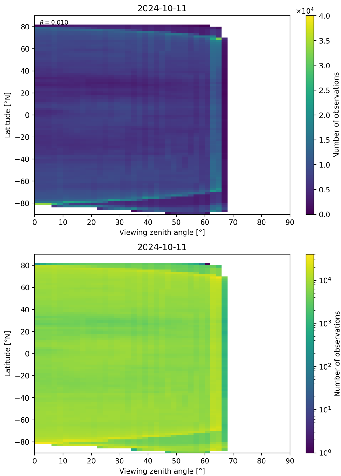
Figure 113: Scatter density plot of “Viewing zenith angle” against “Latitude” for 2024-10-10 to 2024-10-12.
