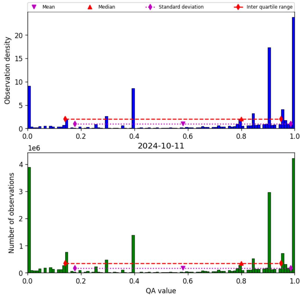
Figure 38: Histogram of “QA value” for 2024-10-10 to 2024-10-12
