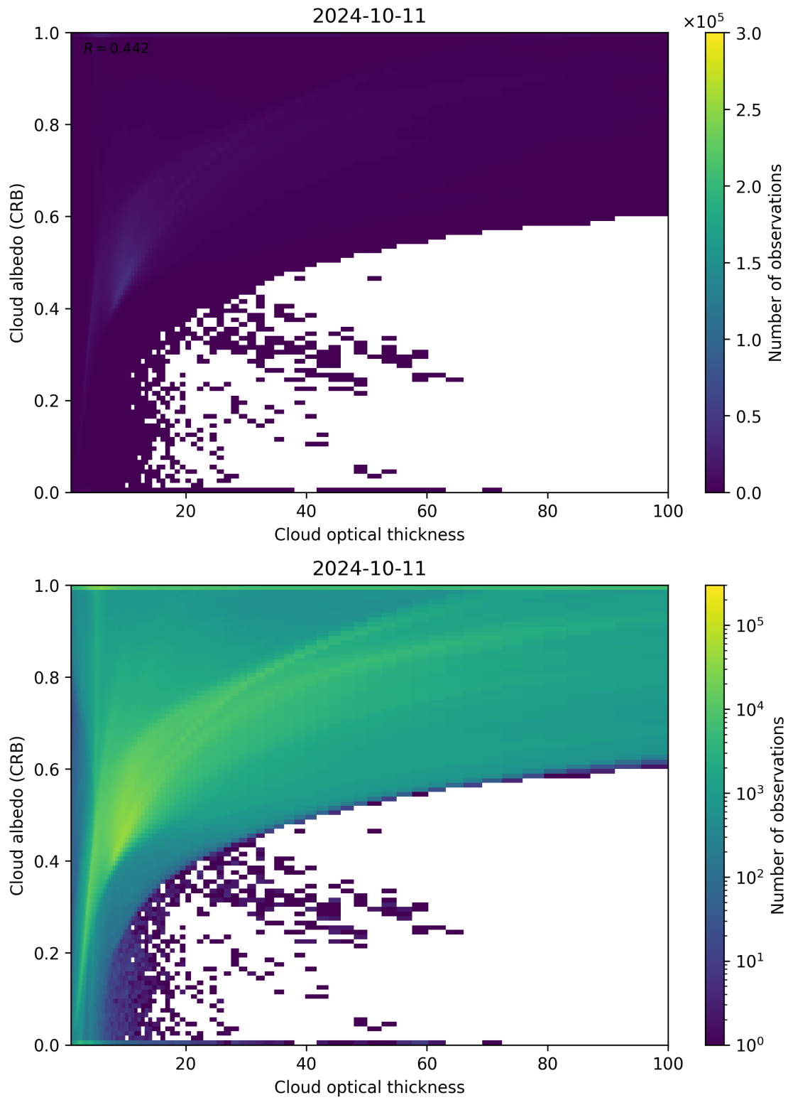
Figure 82: Scatter density plot of “Cloud optical thickness” against “Cloud albedo (CRB)” for 2024-10-10 to 2024-10-12.
