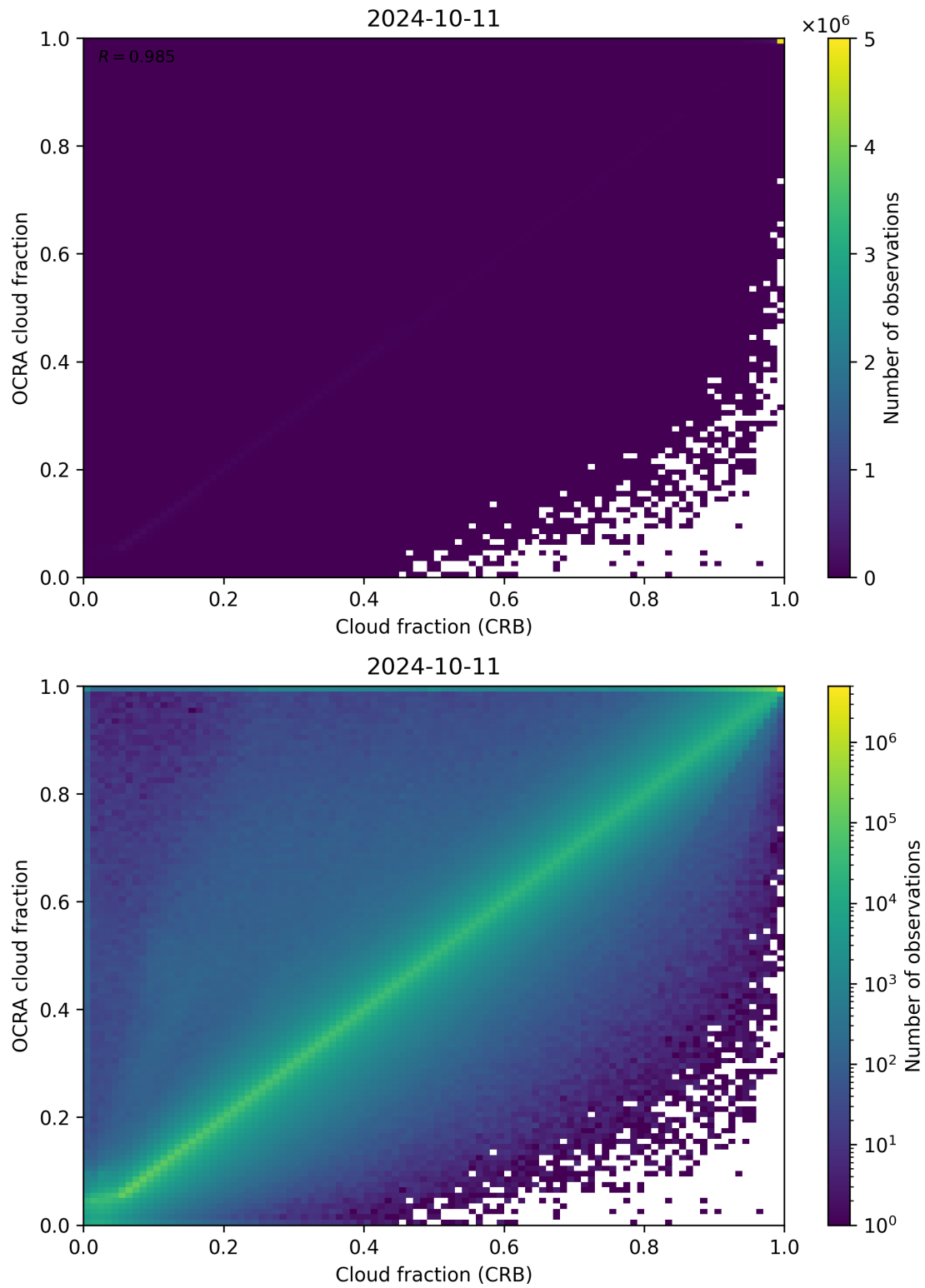
Figure 78: Scatter density plot of “Cloud fraction (CRB)” against “OCRA cloud fraction” for 2024-10-10 to 2024-10-12.
