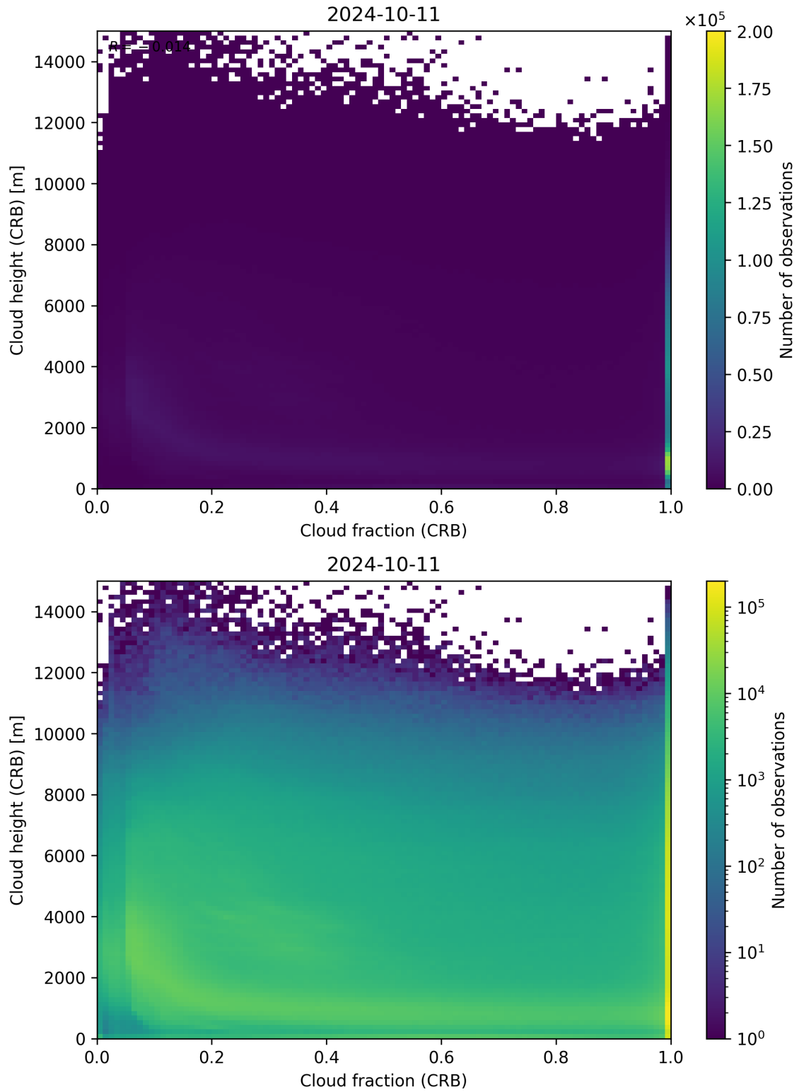
Figure 79: Scatter density plot of “Cloud fraction (CRB)” against “Cloud height (CRB)” for 2024-10-10 to 2024-10-12.
