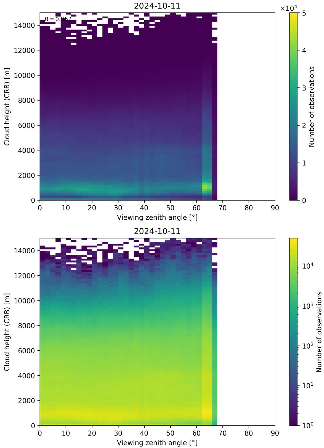
Figure 110: Scatter density plot of “Viewing zenith angle” against “Cloud height (CRB)” for 2024-10-10 to 2024-10-12.
