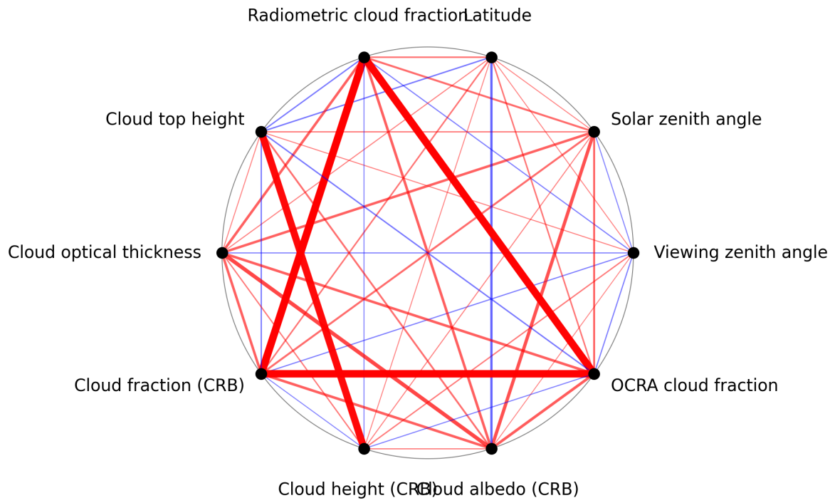
Figure 1: Map of correlation graph for 2024-10-10 to 2024-10-12.
