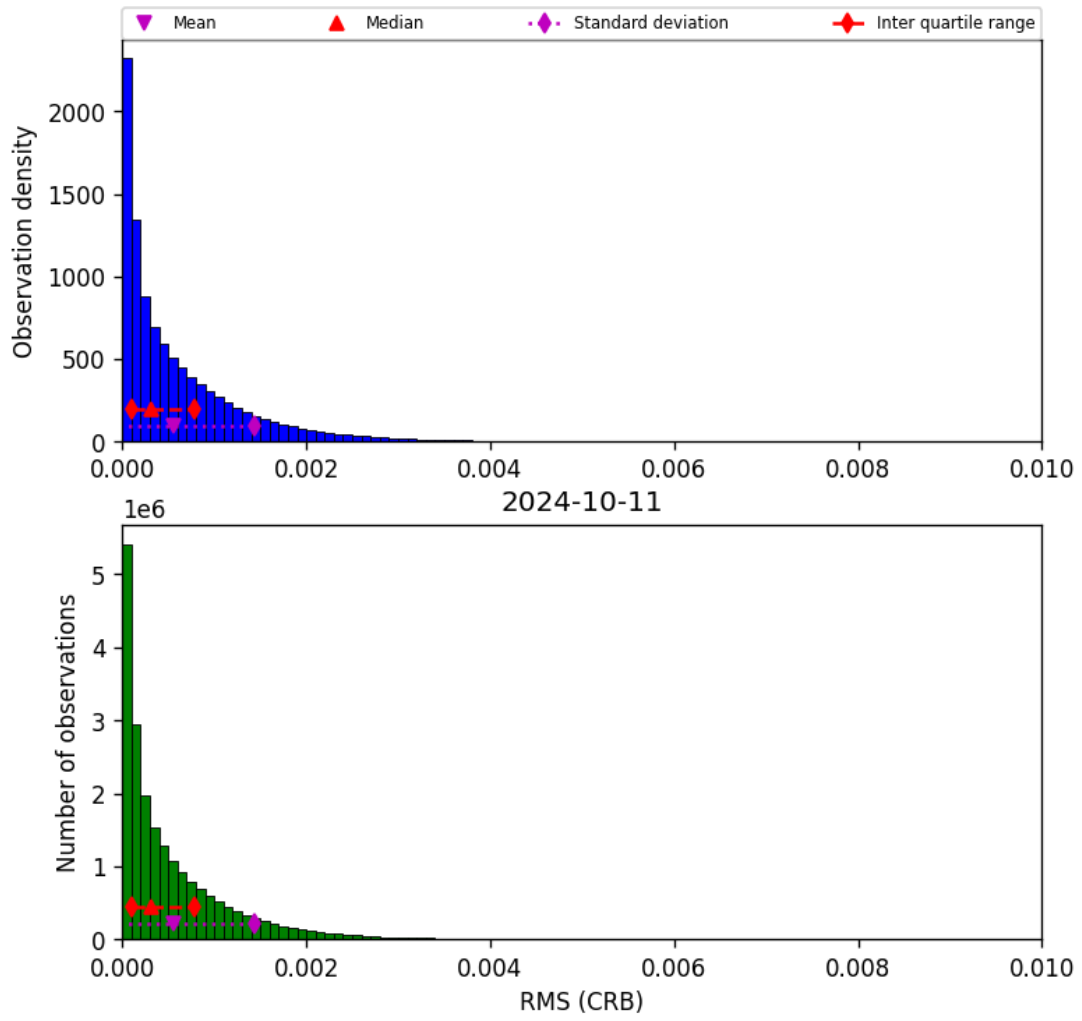
Figure 48: Histogram of “RMS (CRB)” for 2024-10-10 to 2024-10-12
