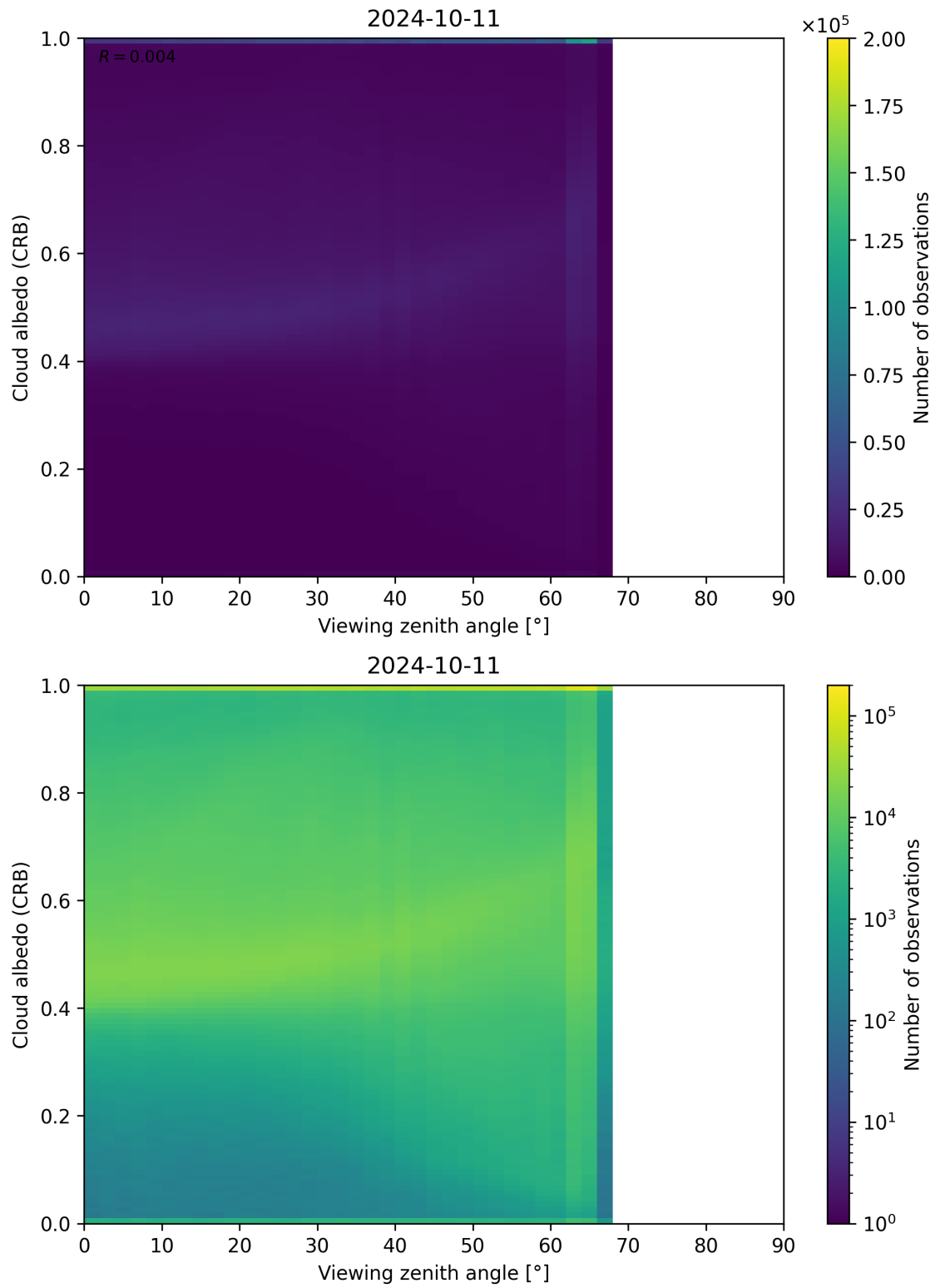
Figure 106: Scatter density plot of “Viewing zenith angle” against “Cloud albedo (CRB)” for 2024-10-10 to 2024-10-12.
