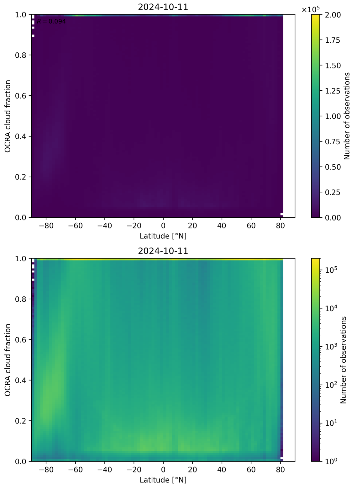
Figure 93: Scatter density plot of “Latitude” against “OCRA cloud fraction” for 2024-10-10 to 2024-10-12.
