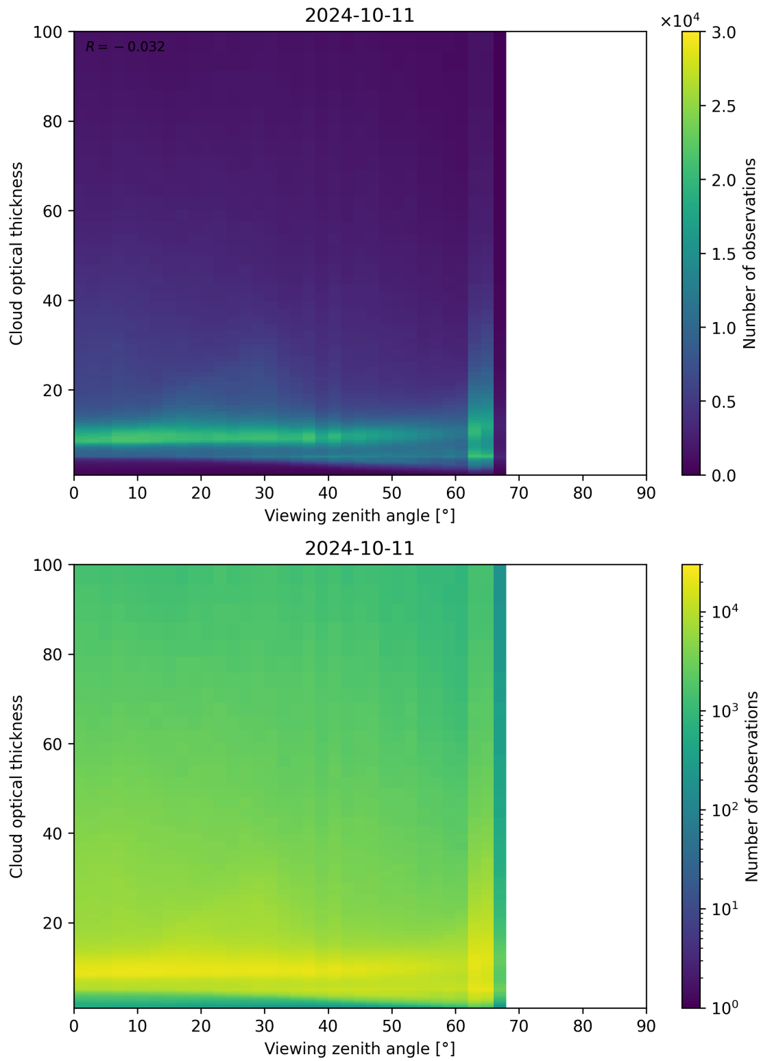
Figure 111: Scatter density plot of “Viewing zenith angle” against “Cloud optical thickness” for 2024-10-10 to 2024-10-12.
