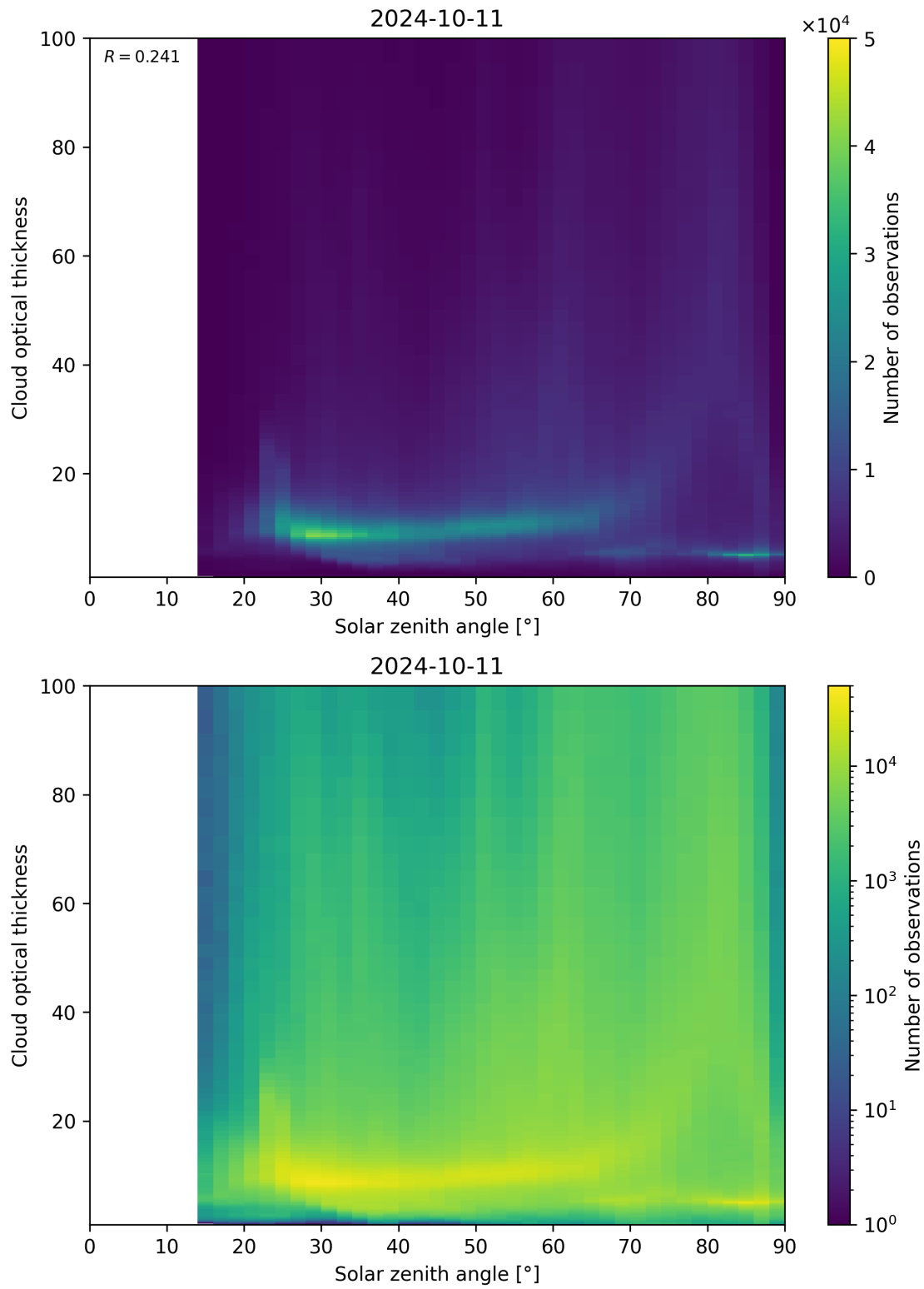
Figure 103: Scatter density plot of “Solar zenith angle” against “Cloud optical thickness” for 2024-10-10 to 2024-10-12.
