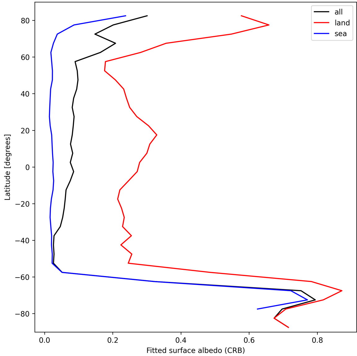
Figure 30: Zonal average of “Fitted surface albedo (CRB)” for 2024-10-11 to 2024-10-13.
