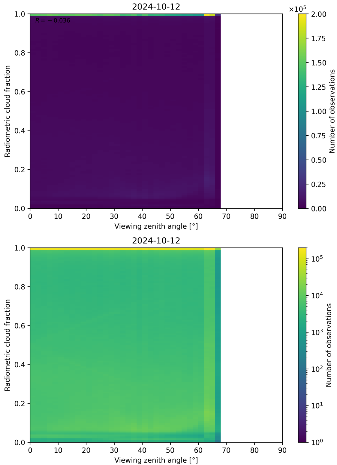
Figure 107: Scatter density plot of “Viewing zenith angle” against “Radiometric cloud fraction” for 2024-10-11 to 2024-10-13.
