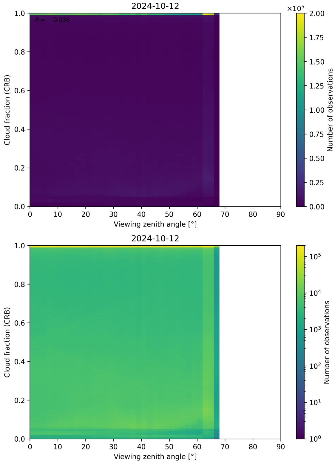
Figure 109: Scatter density plot of “Viewing zenith angle” against “Cloud fraction (CRB)” for 2024-10-11 to 2024-10-13.
