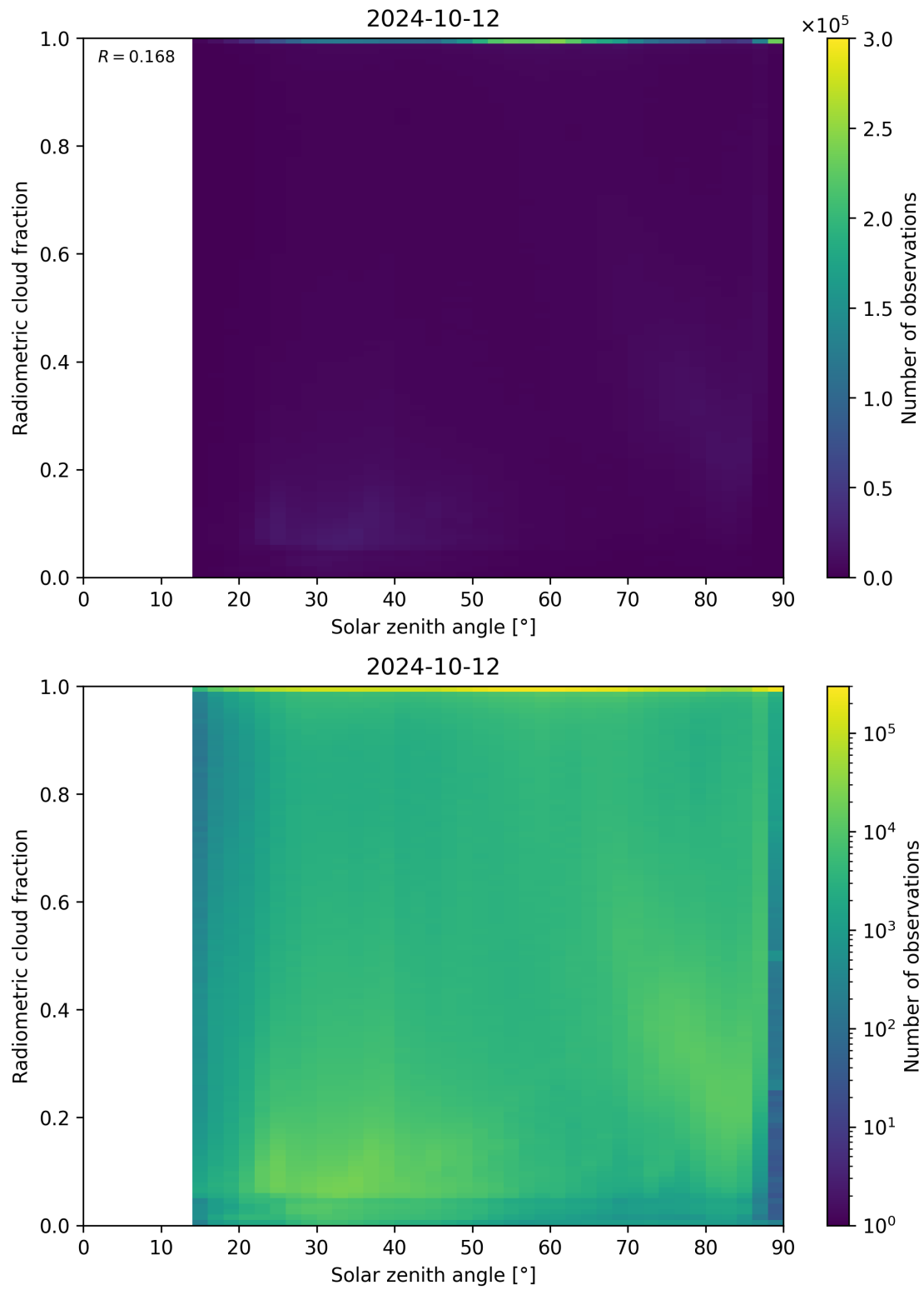
Figure 99: Scatter density plot of “Solar zenith angle” against “Radiometric cloud fraction” for 2024-10-11 to 2024-10-13.
