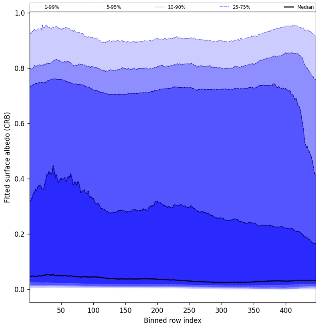
Figure 62: Along track statistics of “Fitted surface albedo (CRB)” for 2024-10-11 to 2024-10-13
