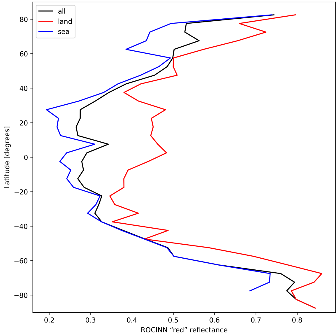
Figure 37: Zonal average of “ROCINN “red” reflectance” for 2024-10-11 to 2024-10-13.
