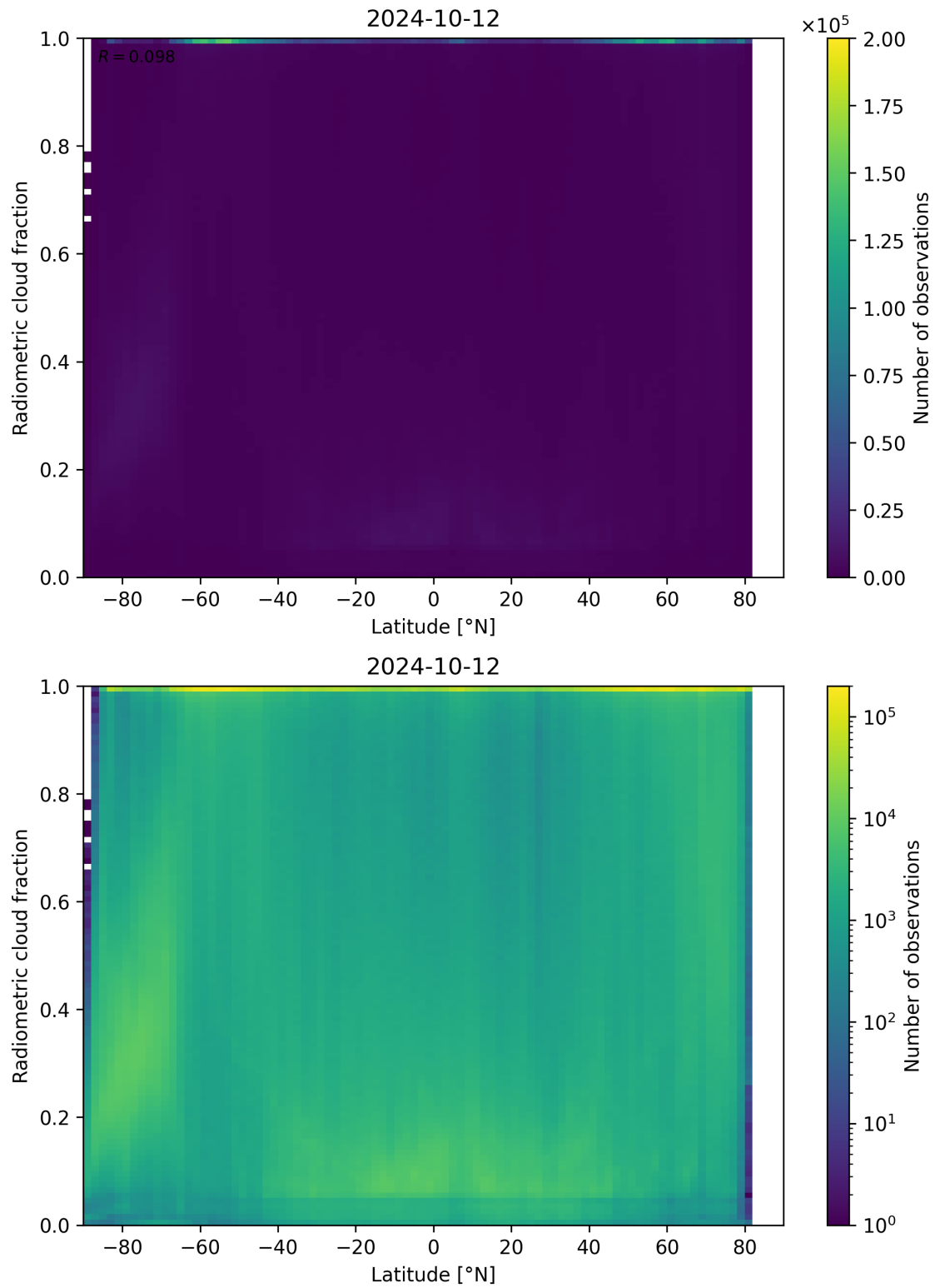
Figure 92: Scatter density plot of “Latitude” against “Radiometric cloud fraction” for 2024-10-11 to 2024-10-13.
