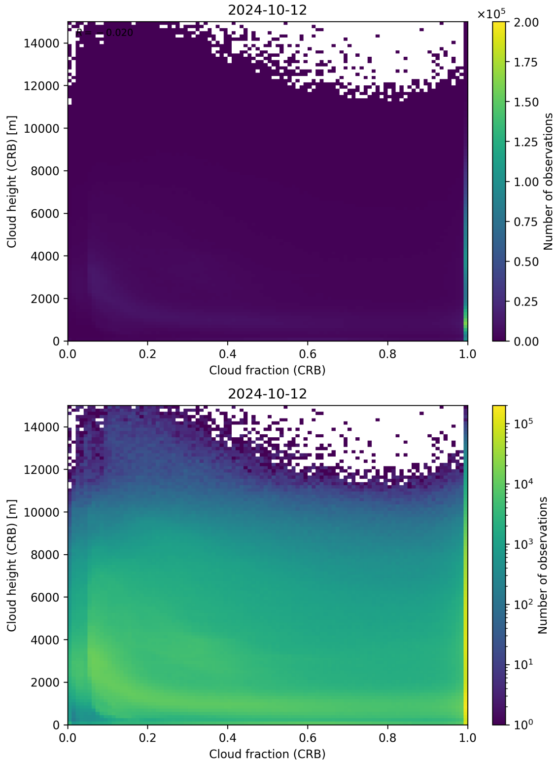
Figure 79: Scatter density plot of “Cloud fraction (CRB)” against “Cloud height (CRB)” for 2024-10-11 to 2024-10-13.
