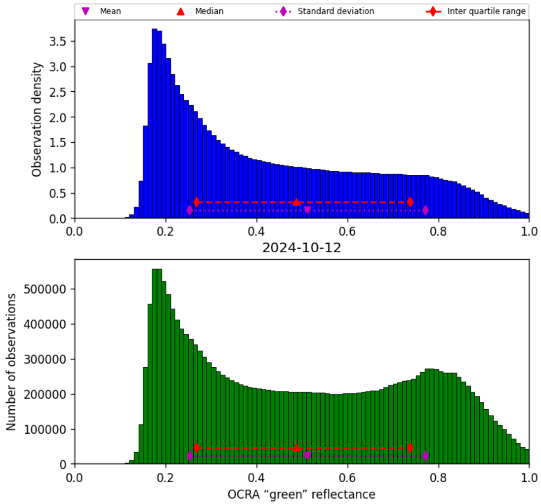
Figure 52: Histogram of “OCRA “green” reflectance” for 2024-10-11 to 2024-10-13
