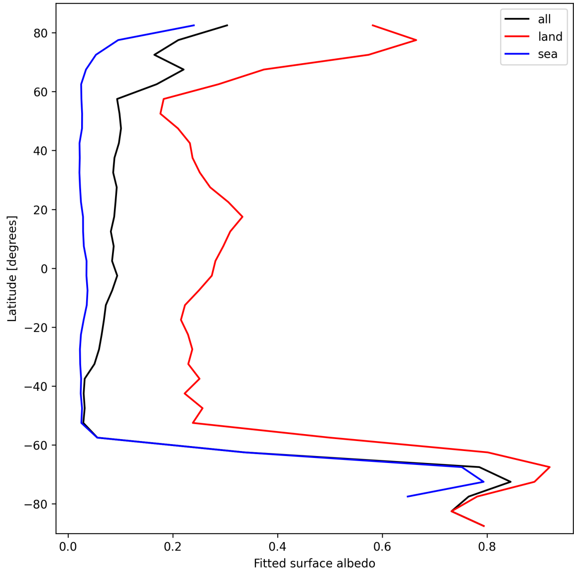
Figure 29: Zonal average of “Fitted surface albedo” for 2024-10-11 to 2024-10-13.
