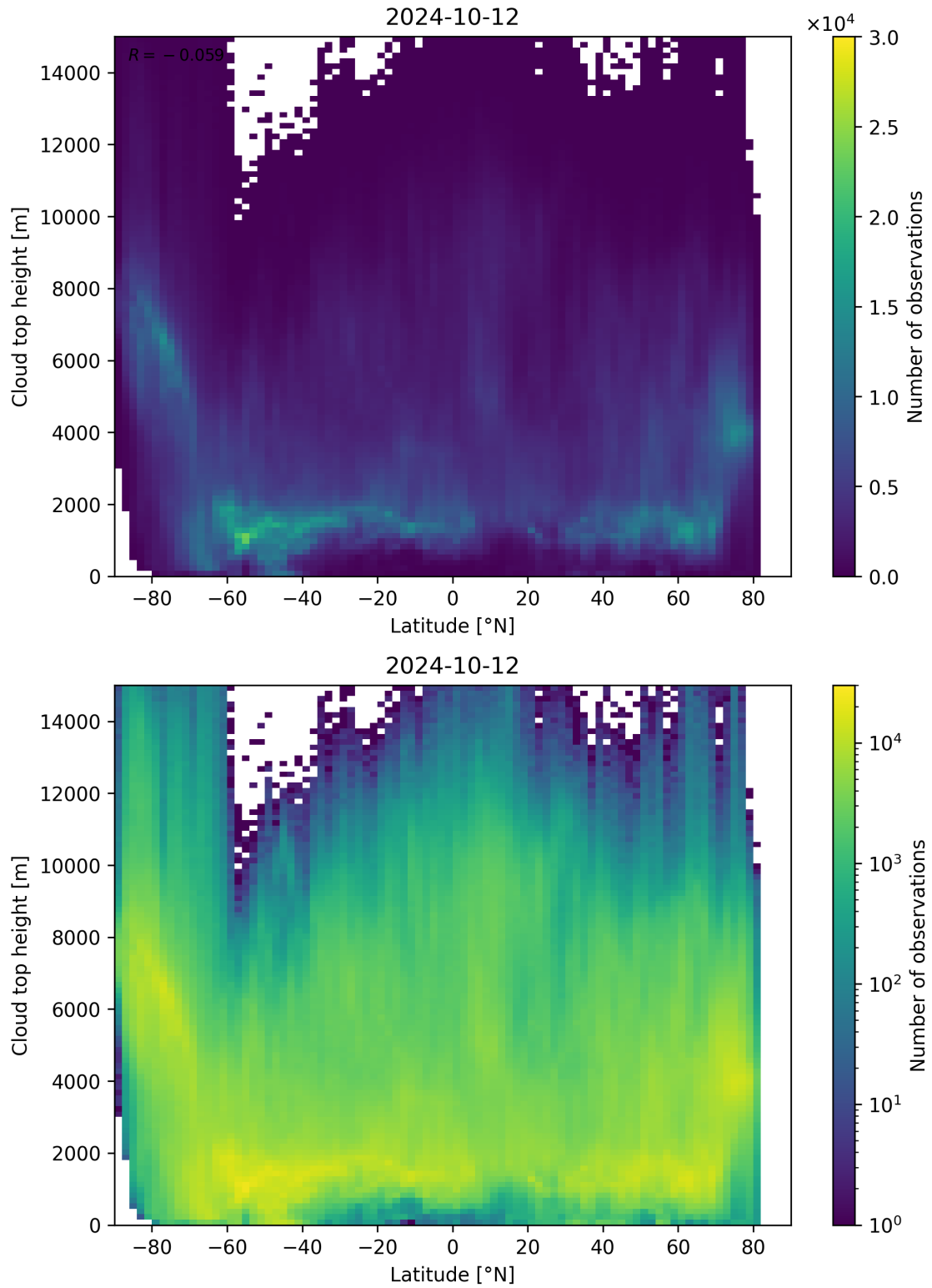
Figure 97: Scatter density plot of “Latitude” against “Cloud top height” for 2024-10-11 to 2024-10-13.
