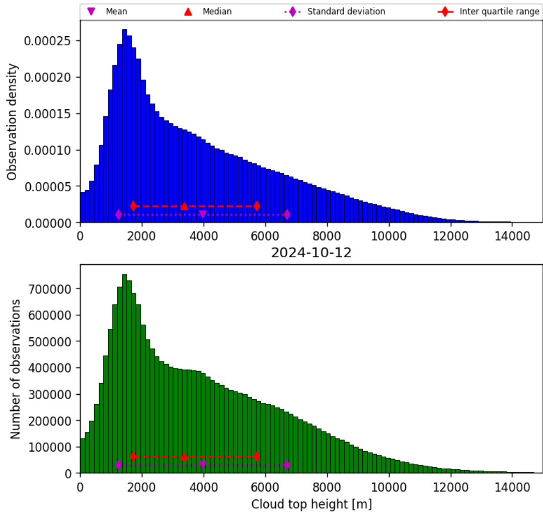
Figure 40: Histogram of “Cloud top height” for 2024-10-11 to 2024-10-13
