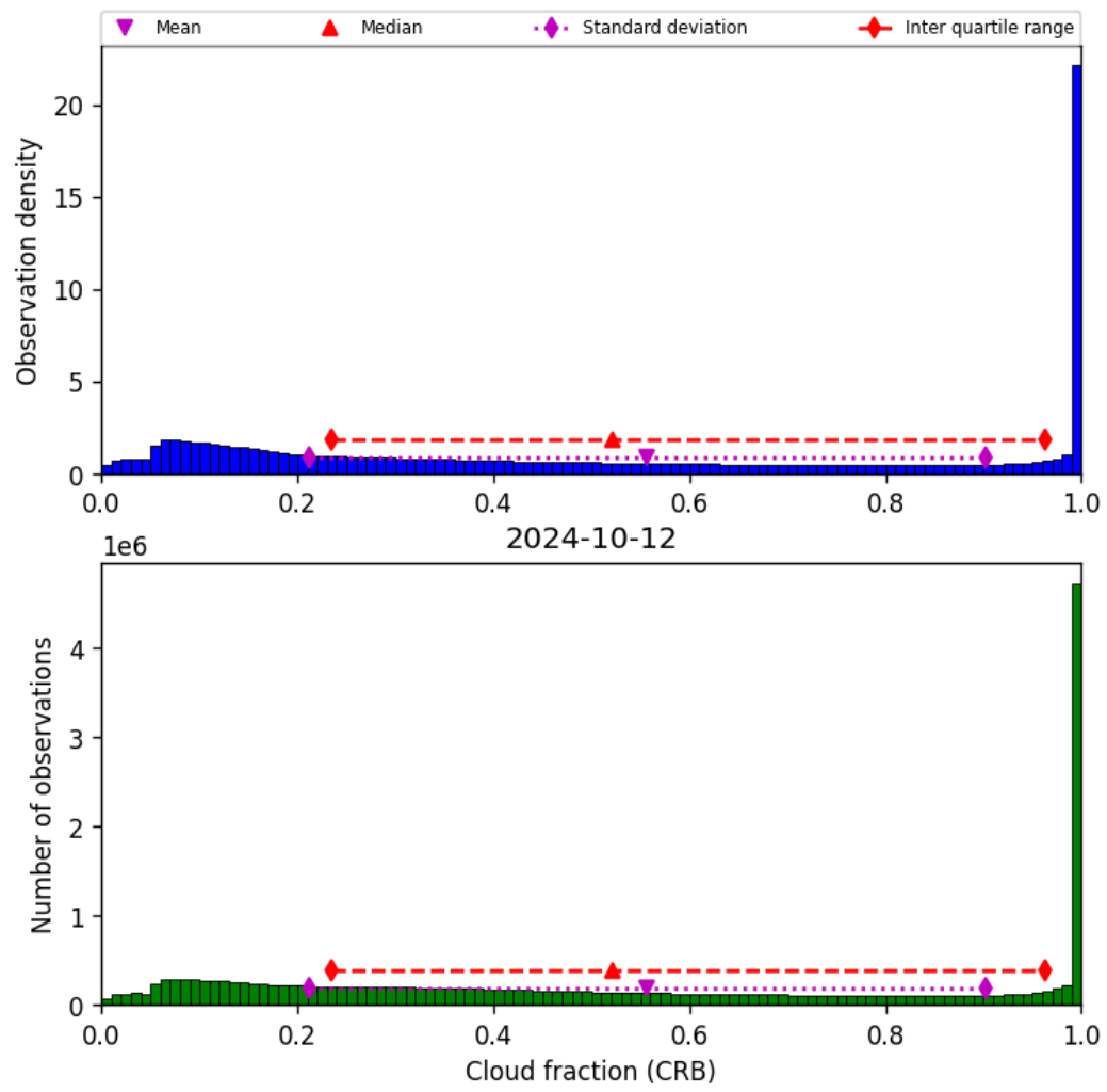
Figure 42: Histogram of “Cloud fraction (CRB)” for 2024-10-11 to 2024-10-13
