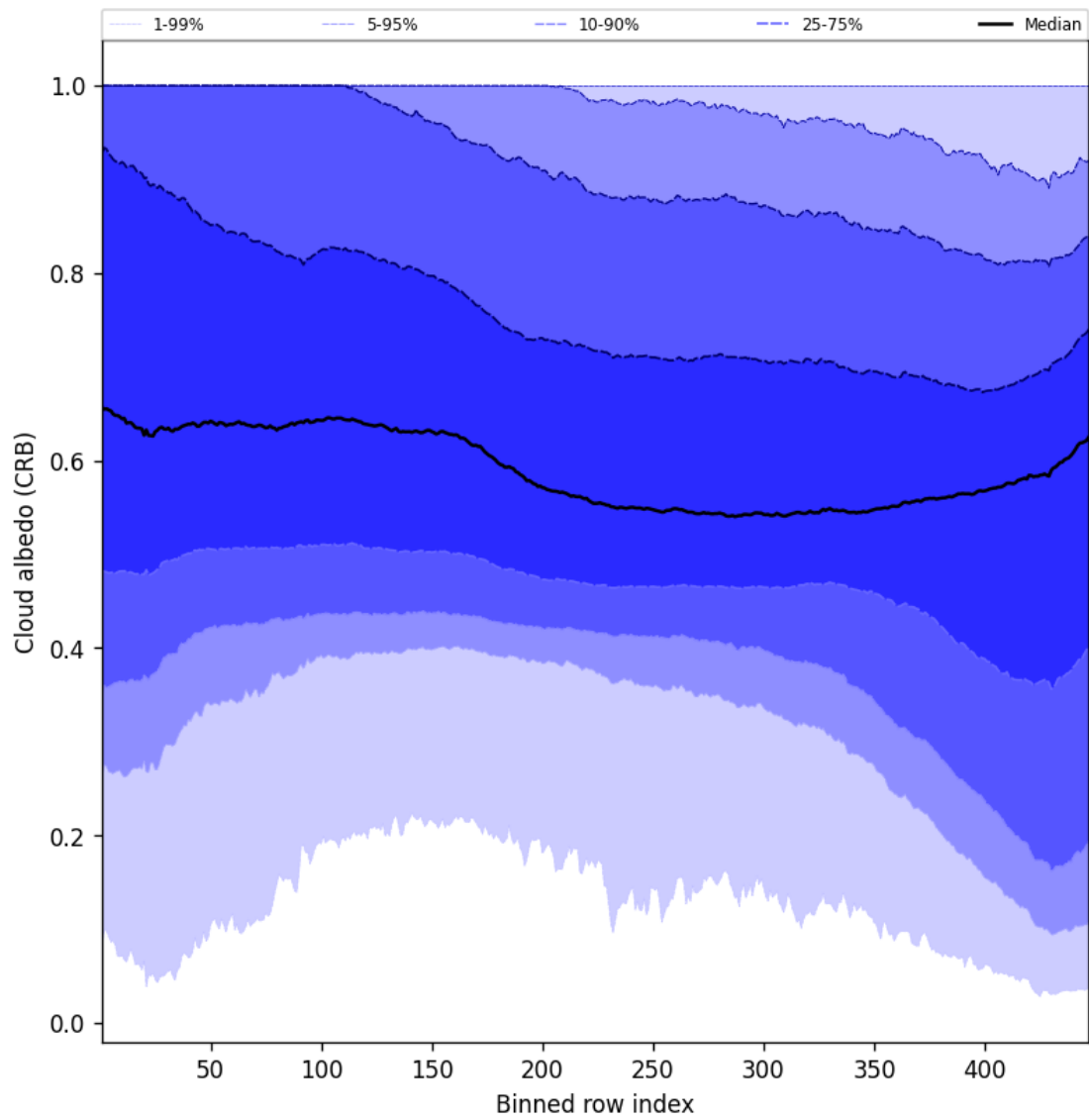
Figure 60: Along track statistics of “Cloud albedo (CRB)” for 2024-10-11 to 2024-10-13
