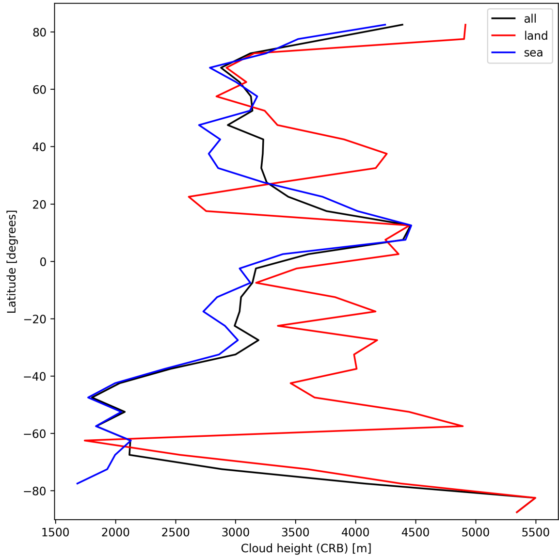
Figure 27: Zonal average of “Cloud height (CRB)” for 2024-10-11 to 2024-10-13.
