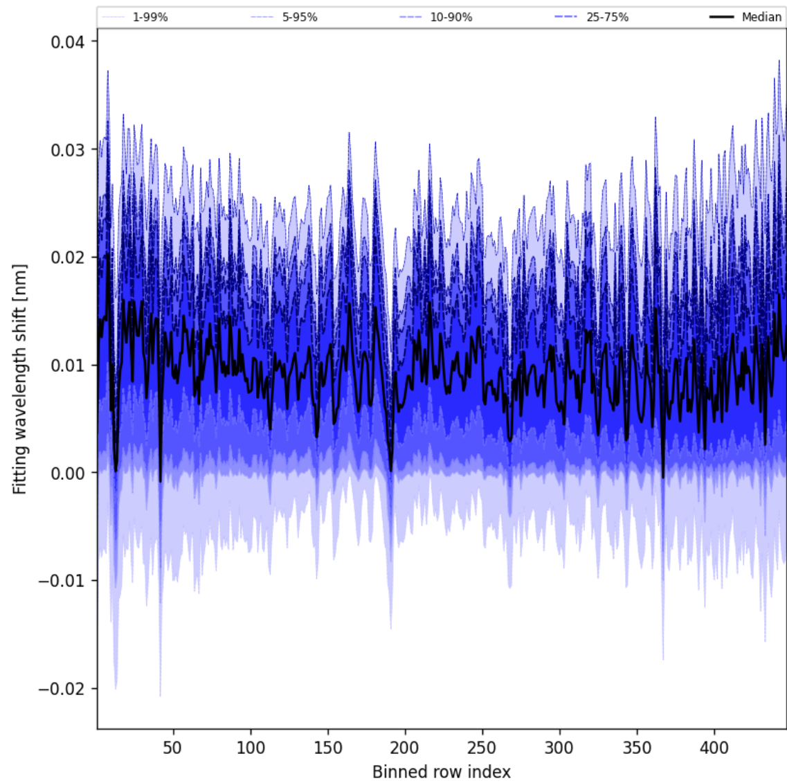
Figure 65: Along track statistics of “Fitting wavelength shift” for 2024-10-11 to 2024-10-13
