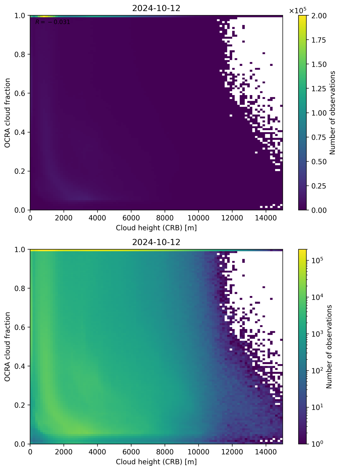
Figure 81: Scatter density plot of “Cloud height (CRB)” against “OCRA cloud fraction” for 2024-10-11 to 2024-10-13.
