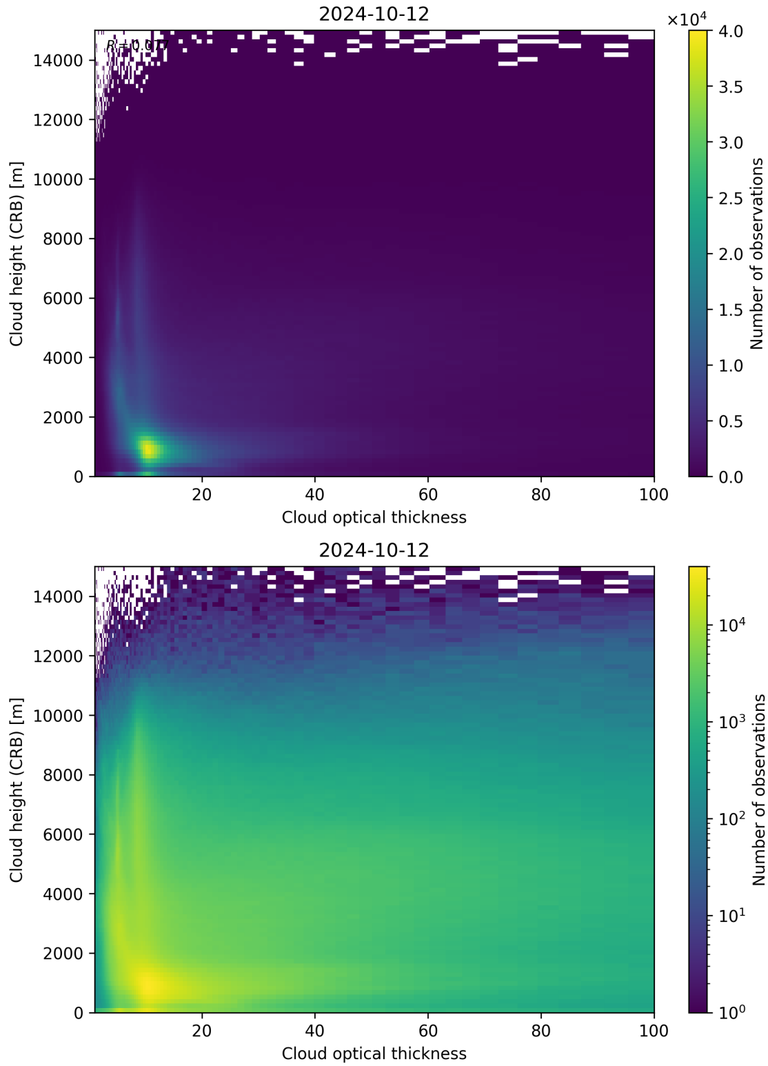
Figure 85: Scatter density plot of “Cloud optical thickness” against “Cloud height (CRB)” for 2024-10-11 to 2024-10-13.
