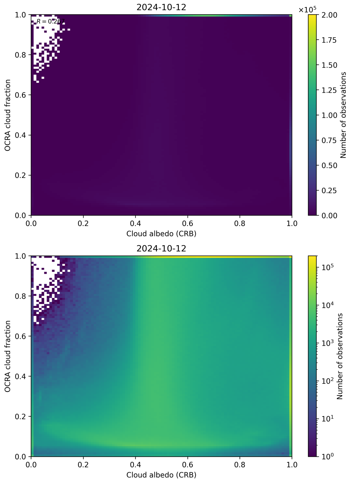
Figure 70: Scatter density plot of “Cloud albedo (CRB)” against “OCRA cloud fraction” for 2024-10-11 to 2024-10-13.
