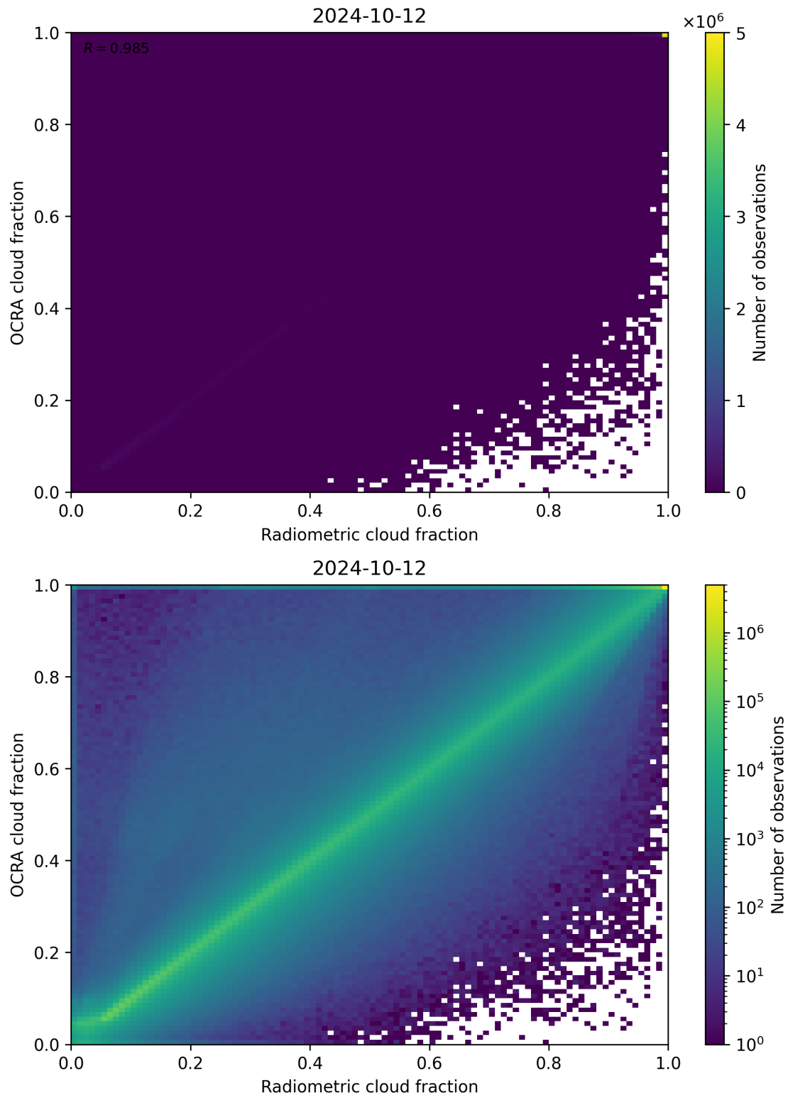
Figure 72: Scatter density plot of “Radiometric cloud fraction” against “OCRA cloud fraction” for 2024-10-11 to 2024-10-13.
