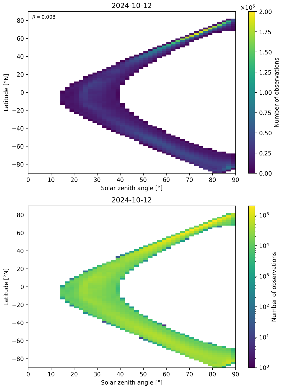
Figure 105: Scatter density plot of “Solar zenith angle” against “Latitude” for 2024-10-11 to 2024-10-13.
