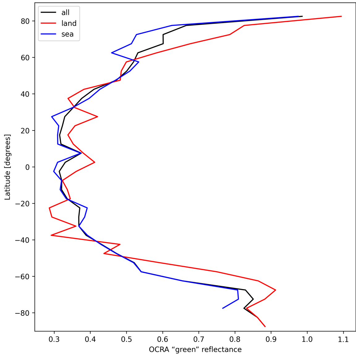
Figure 36: Zonal average of “OCRA “green” reflectance” for 2024-10-11 to 2024-10-13.
