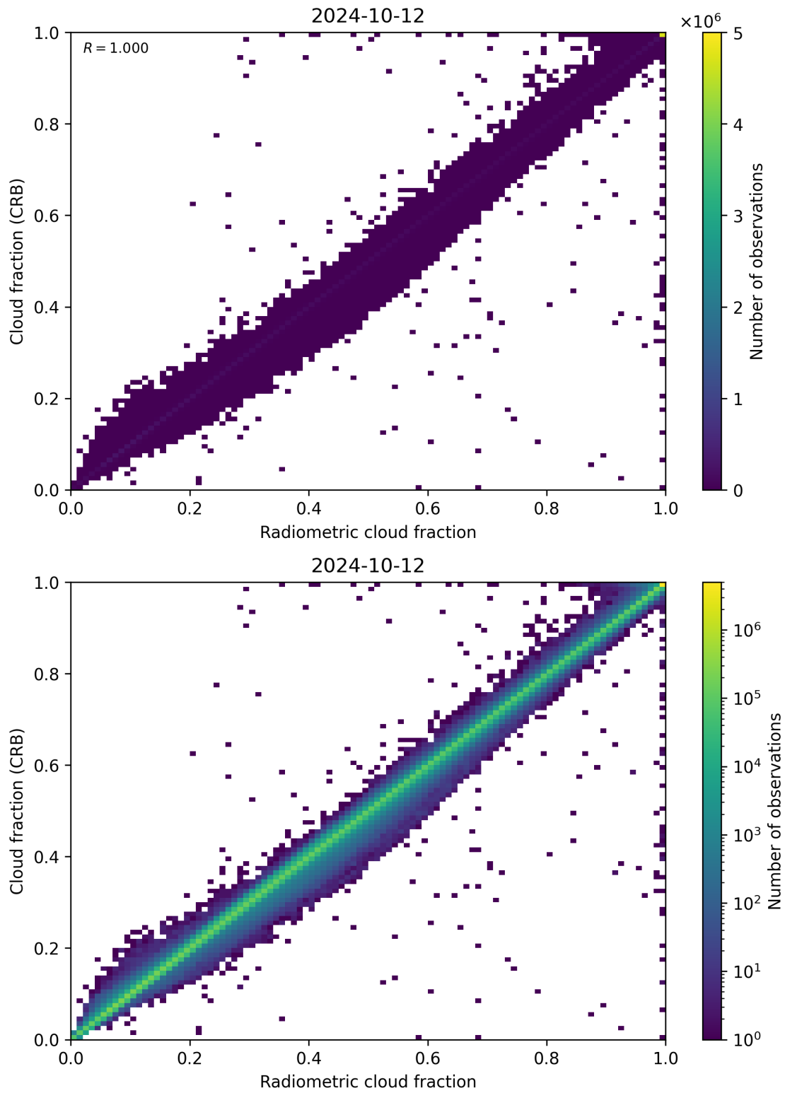
Figure 73: Scatter density plot of “Radiometric cloud fraction” against “Cloud fraction (CRB)” for 2024-10-11 to 2024-10-13.
