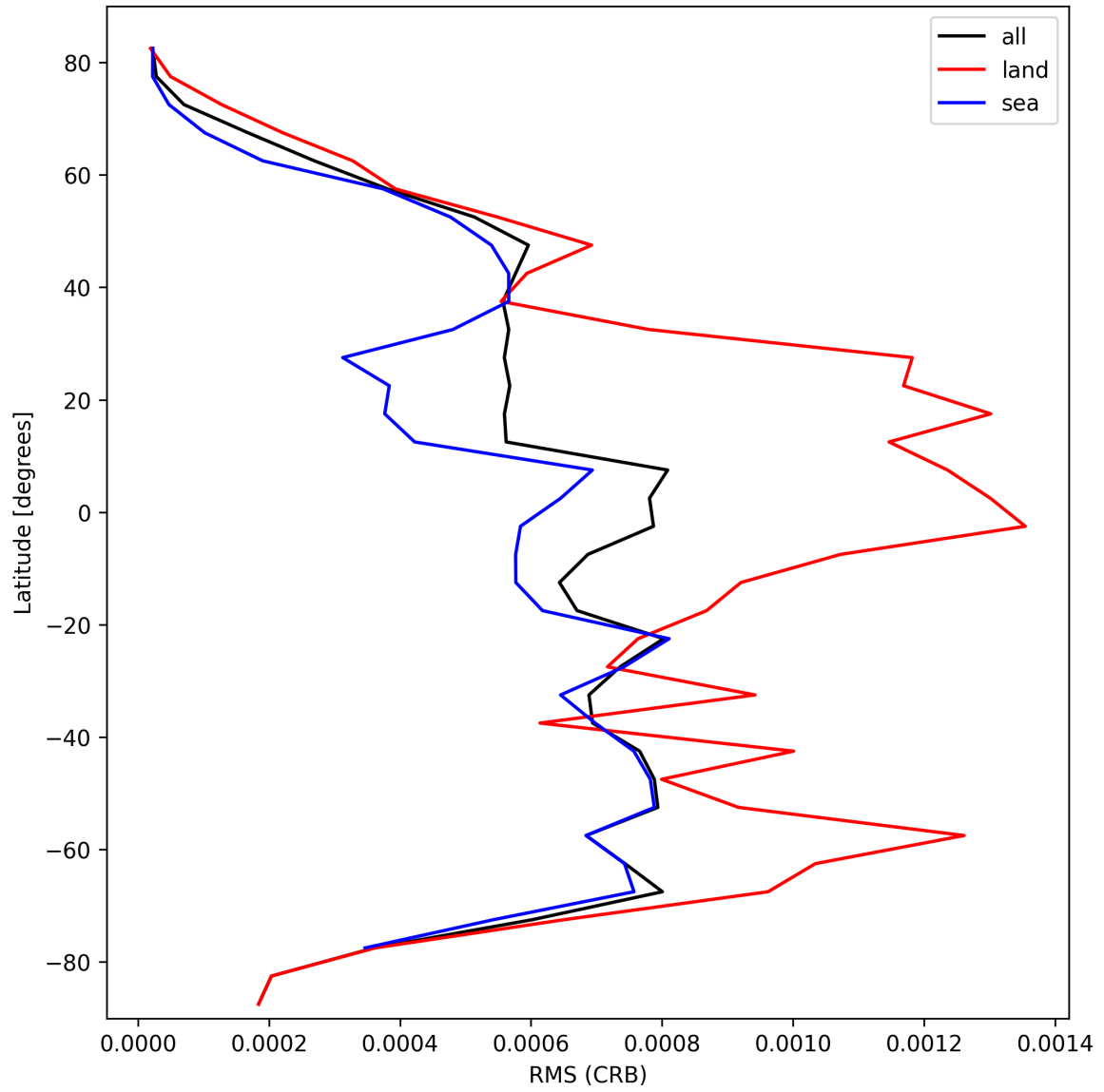
Figure 32: Zonal average of “RMS (CRB)” for 2024-10-11 to 2024-10-13.
