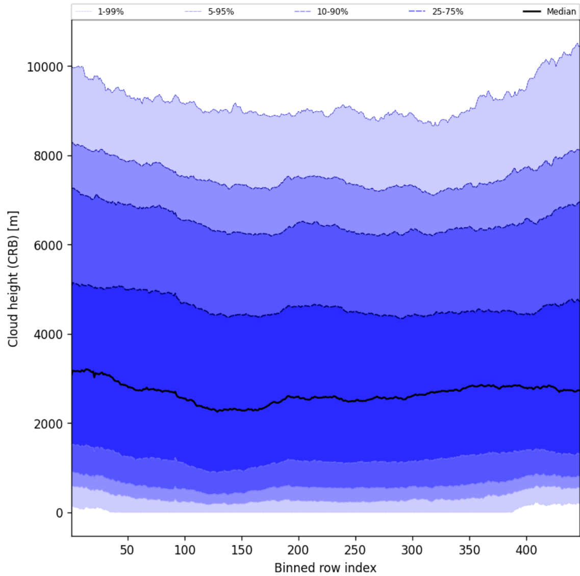
Figure 59: Along track statistics of “Cloud height (CRB)” for 2024-10-11 to 2024-10-13
