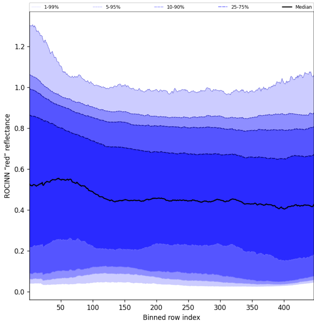
Figure 69: Along track statistics of “ROCINN “red” reflectance” for 2024-10-11 to 2024-10-13
