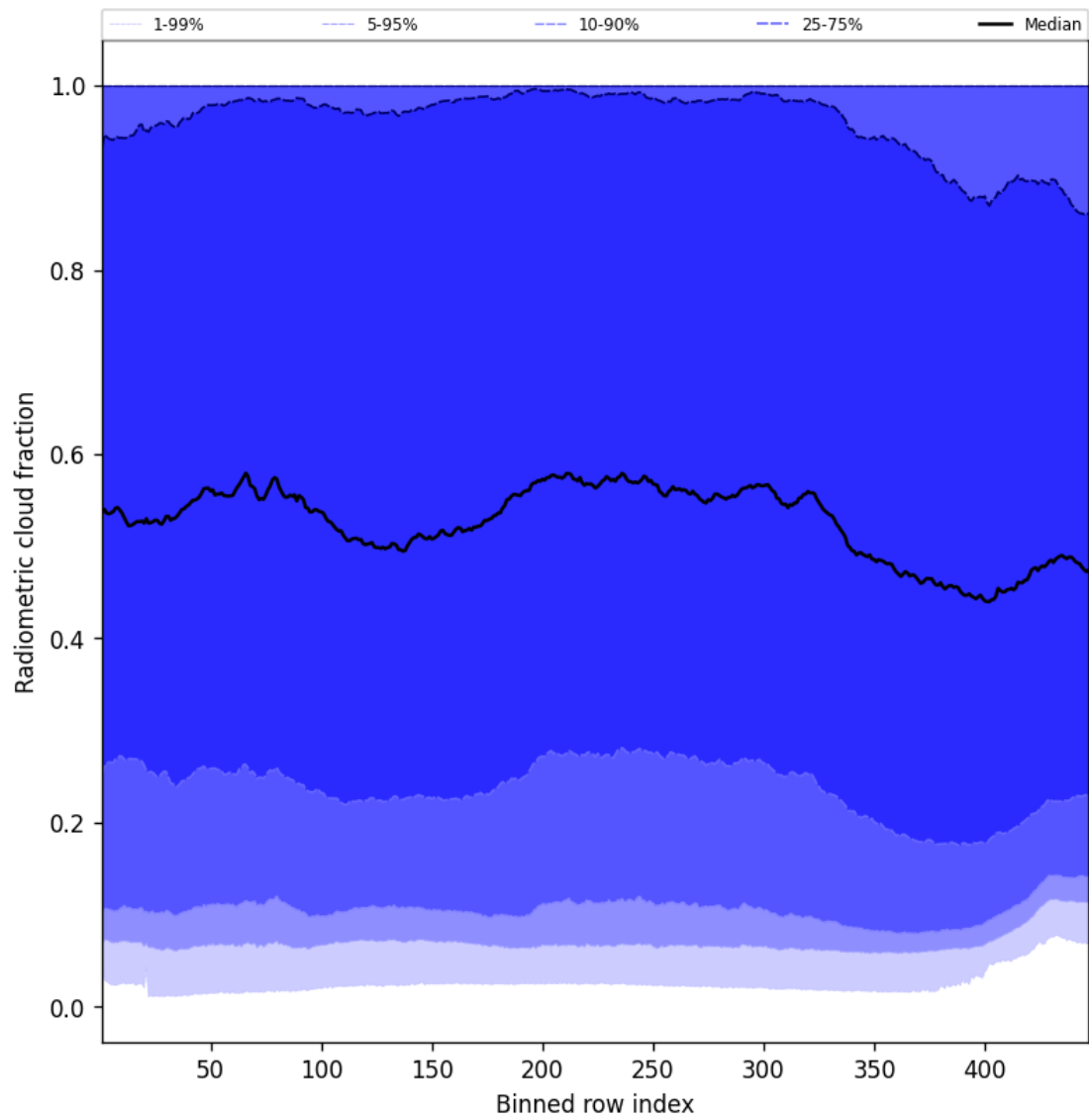
Figure 55: Along track statistics of “Radiometric cloud fraction” for 2024-10-11 to 2024-10-13
