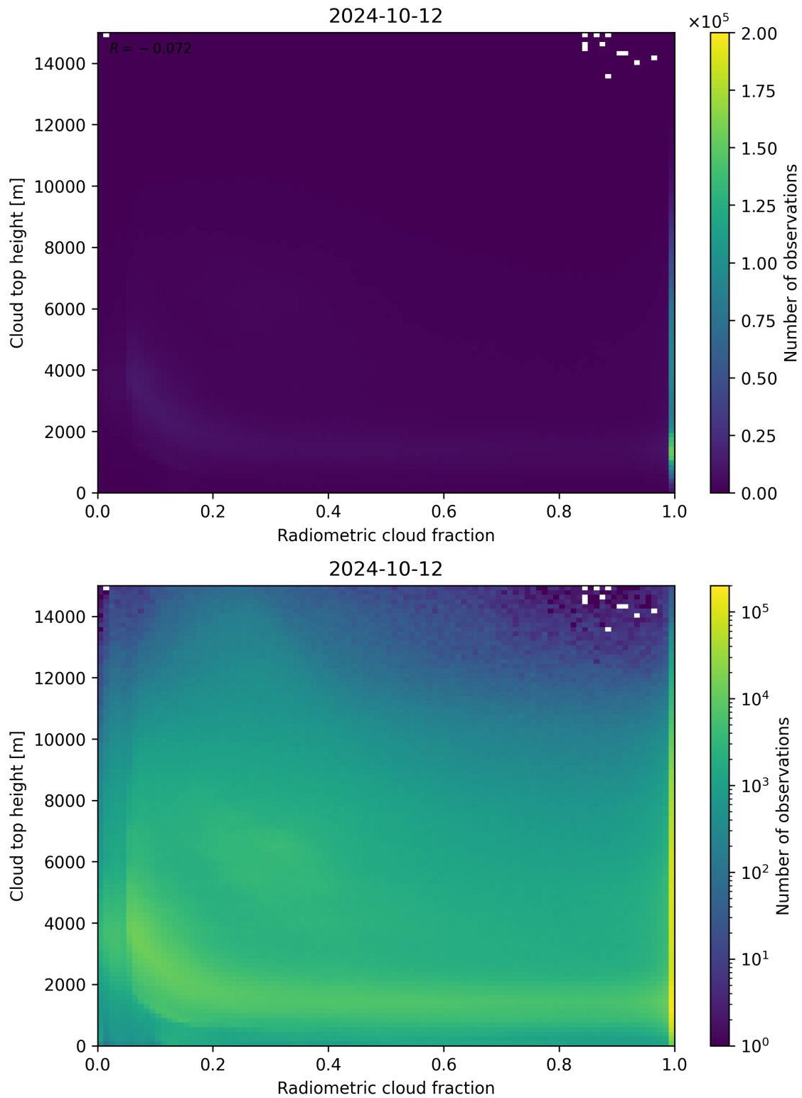
Figure 76: Scatter density plot of “Radiometric cloud fraction” against “Cloud top height” for 2024-10-11 to 2024-10-13.
