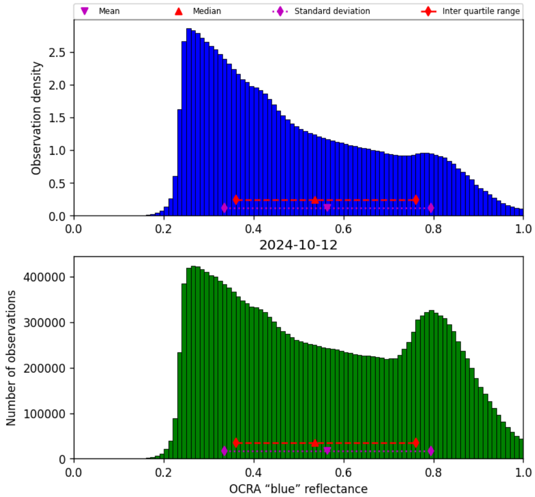
Figure 51: Histogram of “OCRA “blue” reflectance” for 2024-10-11 to 2024-10-13
