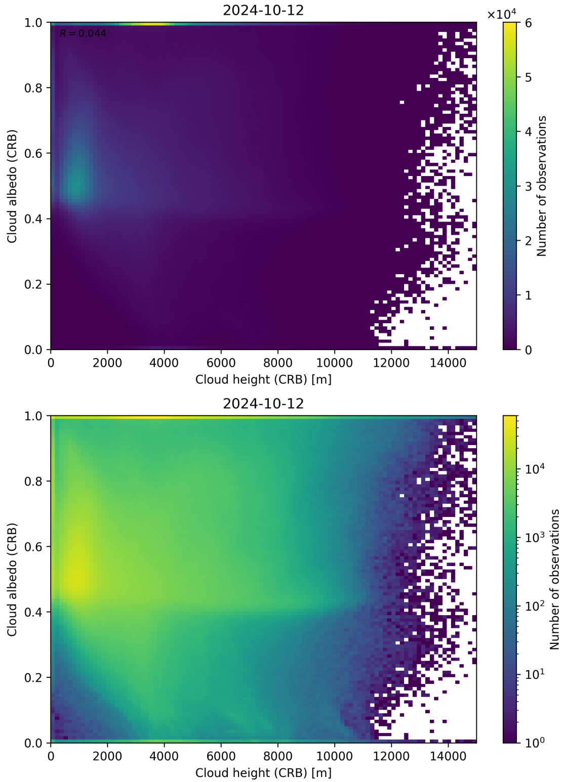
Figure 80: Scatter density plot of “Cloud height (CRB)” against “Cloud albedo (CRB)” for 2024-10-11 to 2024-10-13.
