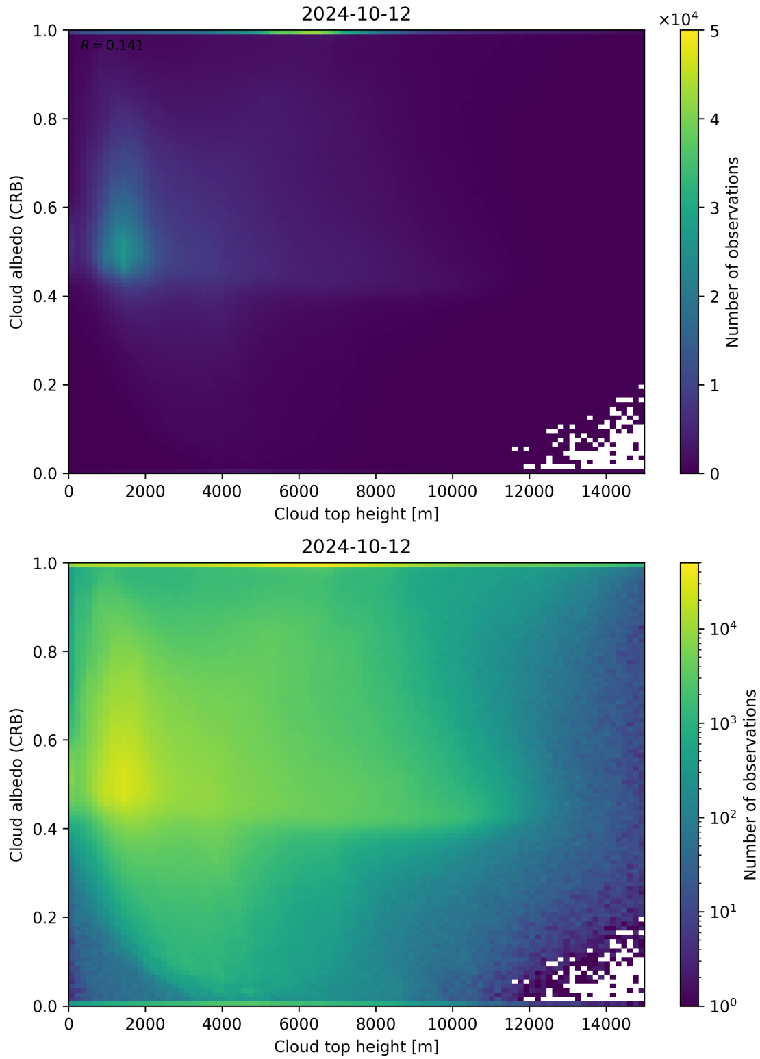
Figure 86: Scatter density plot of “Cloud top height” against “Cloud albedo (CRB)” for 2024-10-11 to 2024-10-13.
