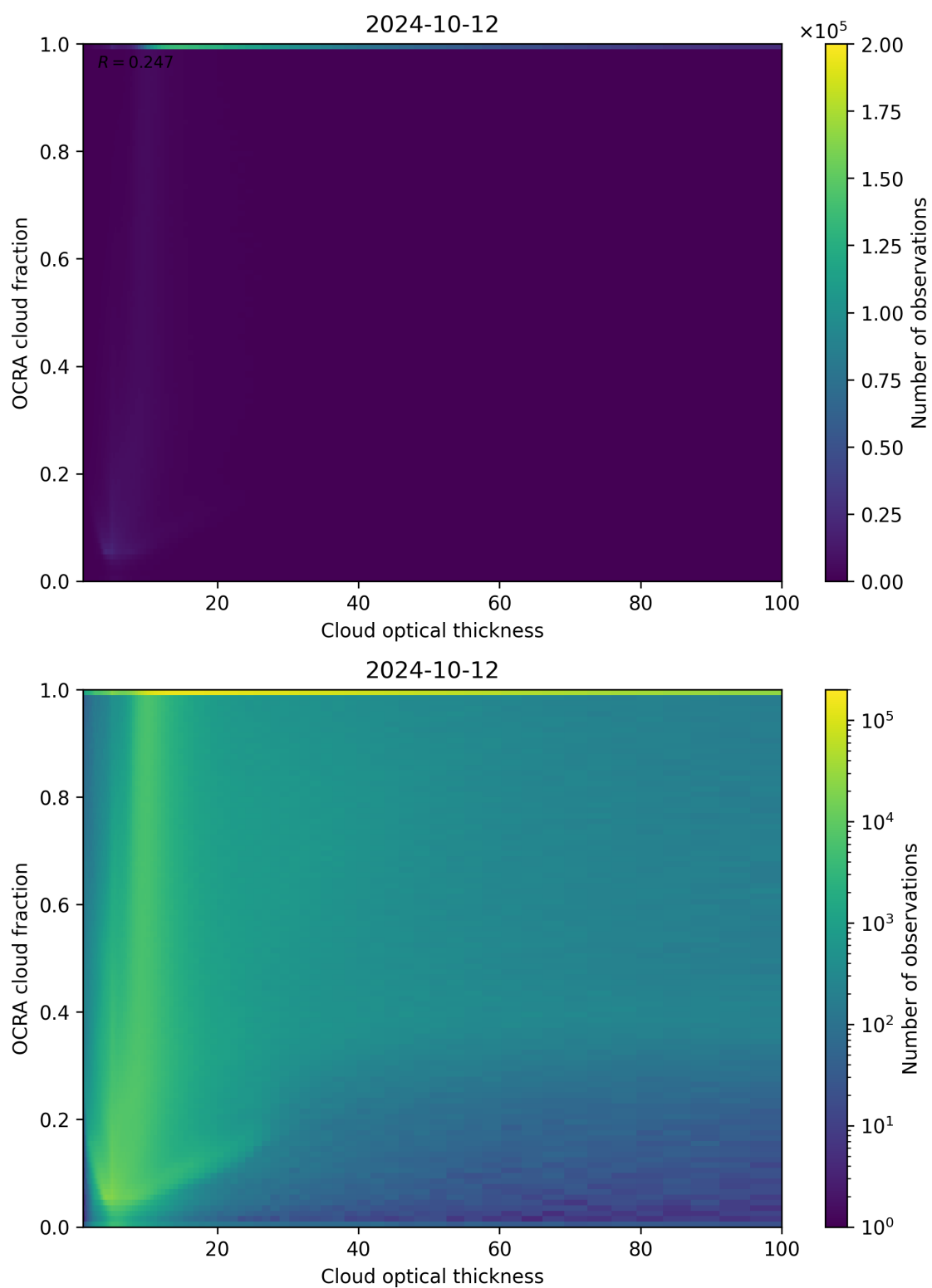
Figure 83: Scatter density plot of “Cloud optical thickness” against “OCRA cloud fraction” for 2024-10-11 to 2024-10-13.
