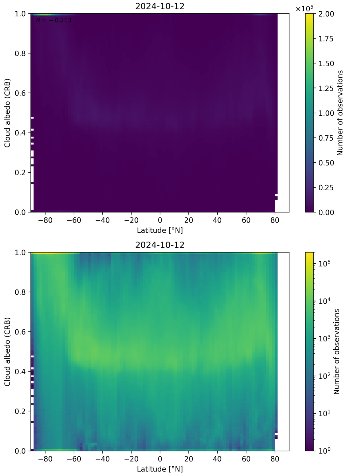
Figure 91: Scatter density plot of “Latitude” against “Cloud albedo (CRB)” for 2024-10-11 to 2024-10-13.
