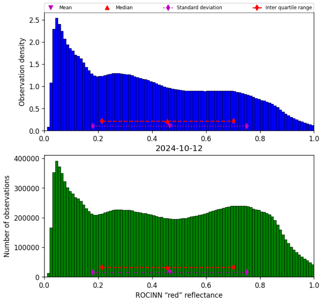
Figure 53: Histogram of “ROCINN “red” reflectance” for 2024-10-11 to 2024-10-13
