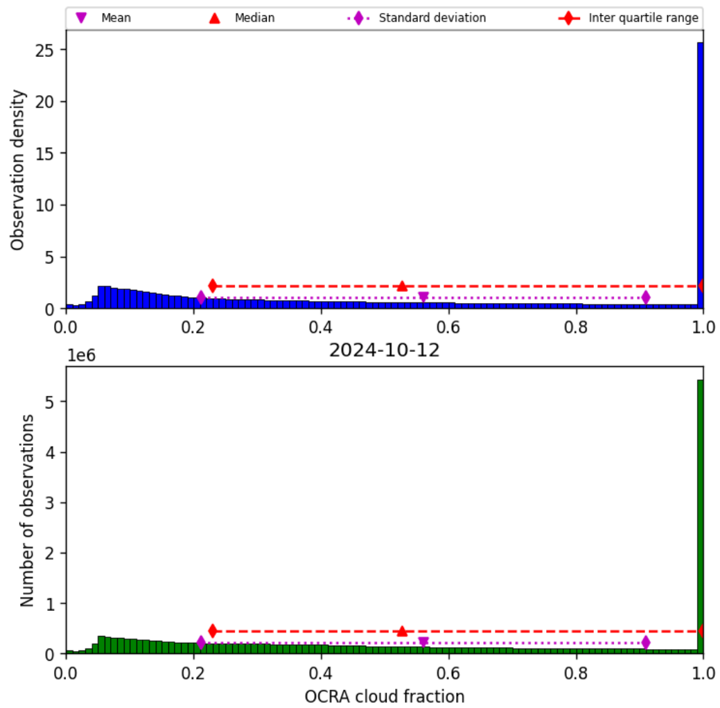
Figure 50: Histogram of “OCRA cloud fraction” for 2024-10-11 to 2024-10-13
