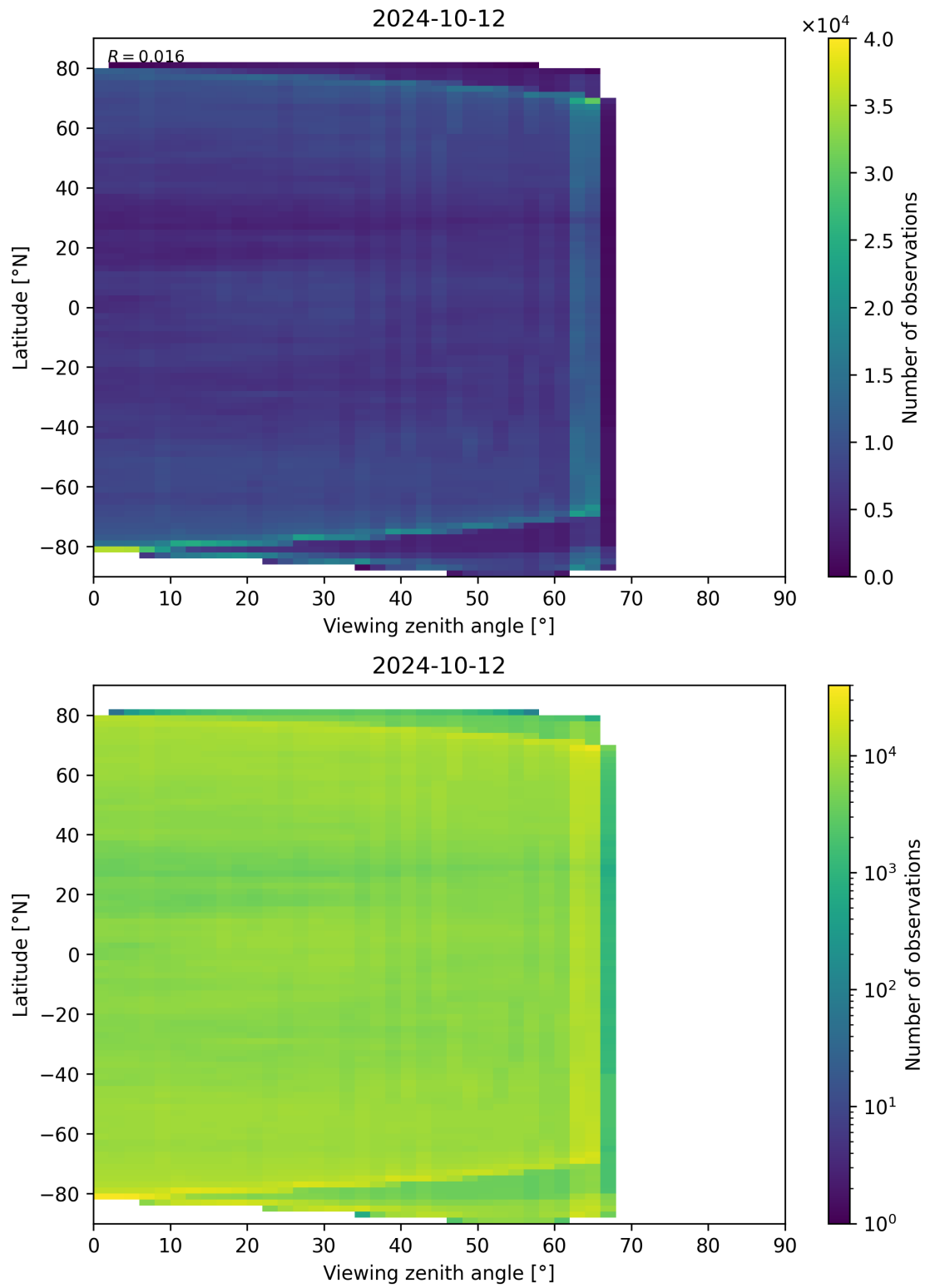
Figure 113: Scatter density plot of “Viewing zenith angle” against “Latitude” for 2024-10-11 to 2024-10-13.
