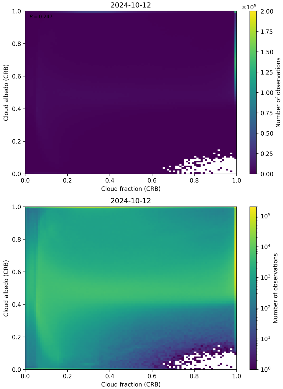
Figure 77: Scatter density plot of “Cloud fraction (CRB)” against “Cloud albedo (CRB)” for 2024-10-11 to 2024-10-13.
