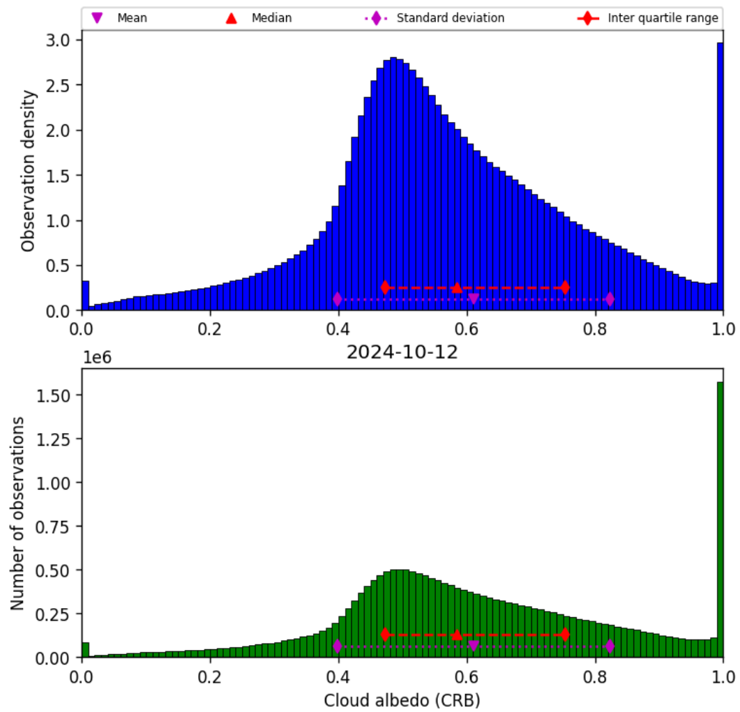
Figure 44: Histogram of “Cloud albedo (CRB)” for 2024-10-11 to 2024-10-13
