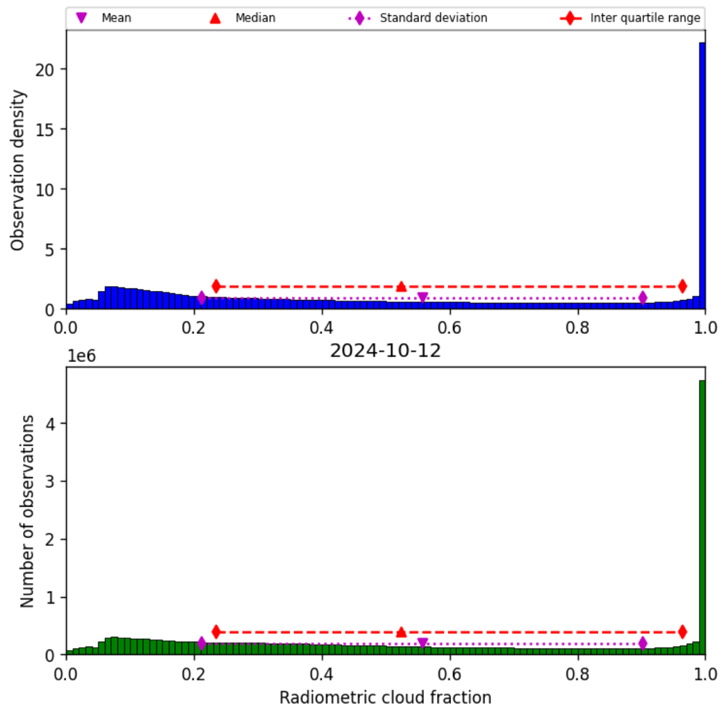
Figure 39: Histogram of “Radiometric cloud fraction” for 2024-10-11 to 2024-10-13
