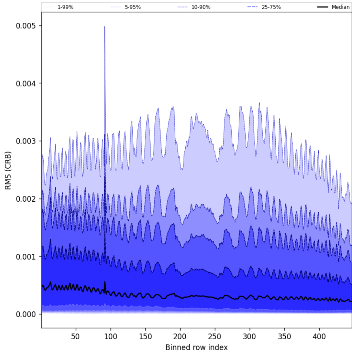
Figure 64: Along track statistics of “RMS (CRB)” for 2024-10-11 to 2024-10-13
