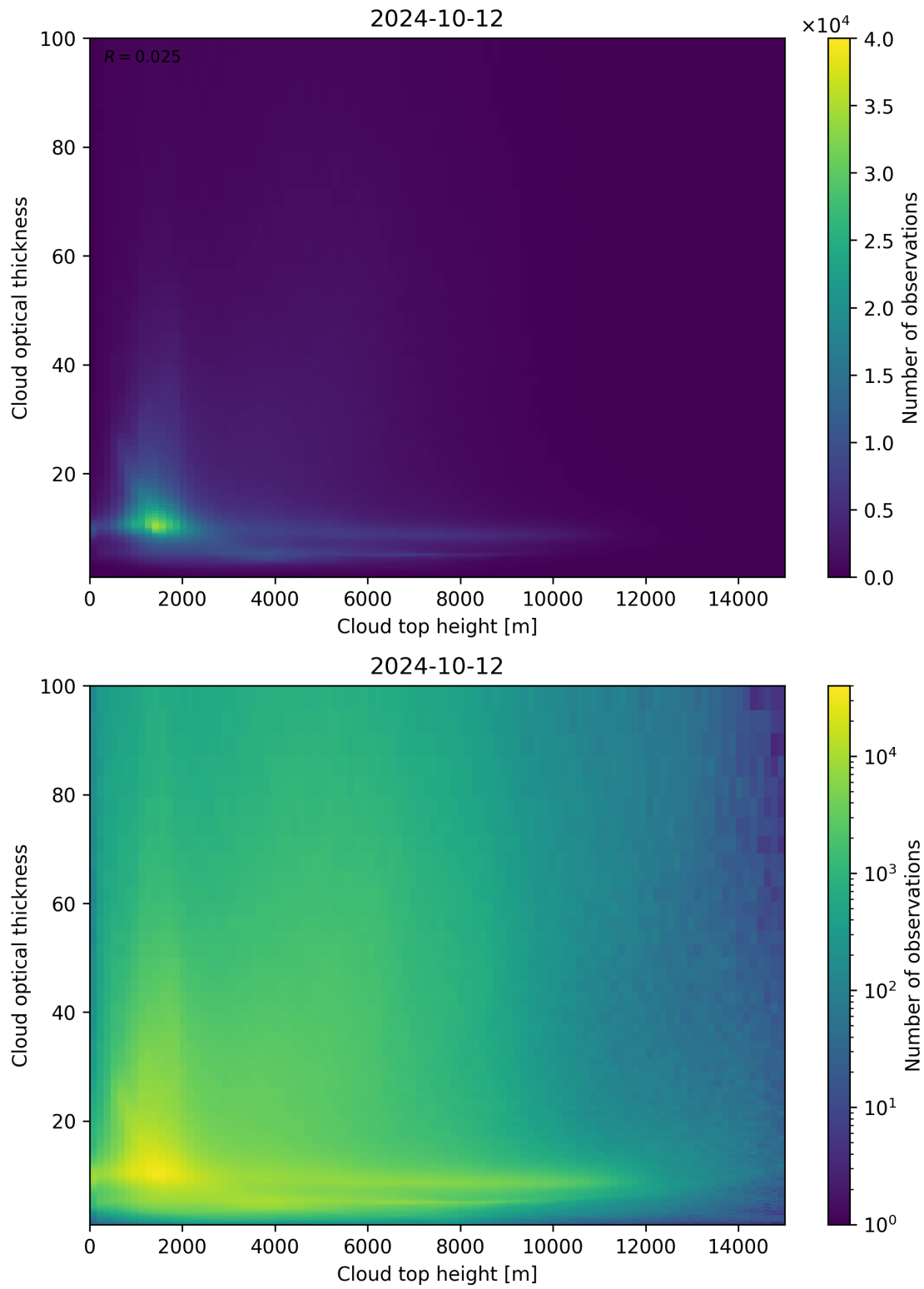
Figure 90: Scatter density plot of “Cloud top height” against “Cloud optical thickness” for 2024-10-11 to 2024-10-13.
