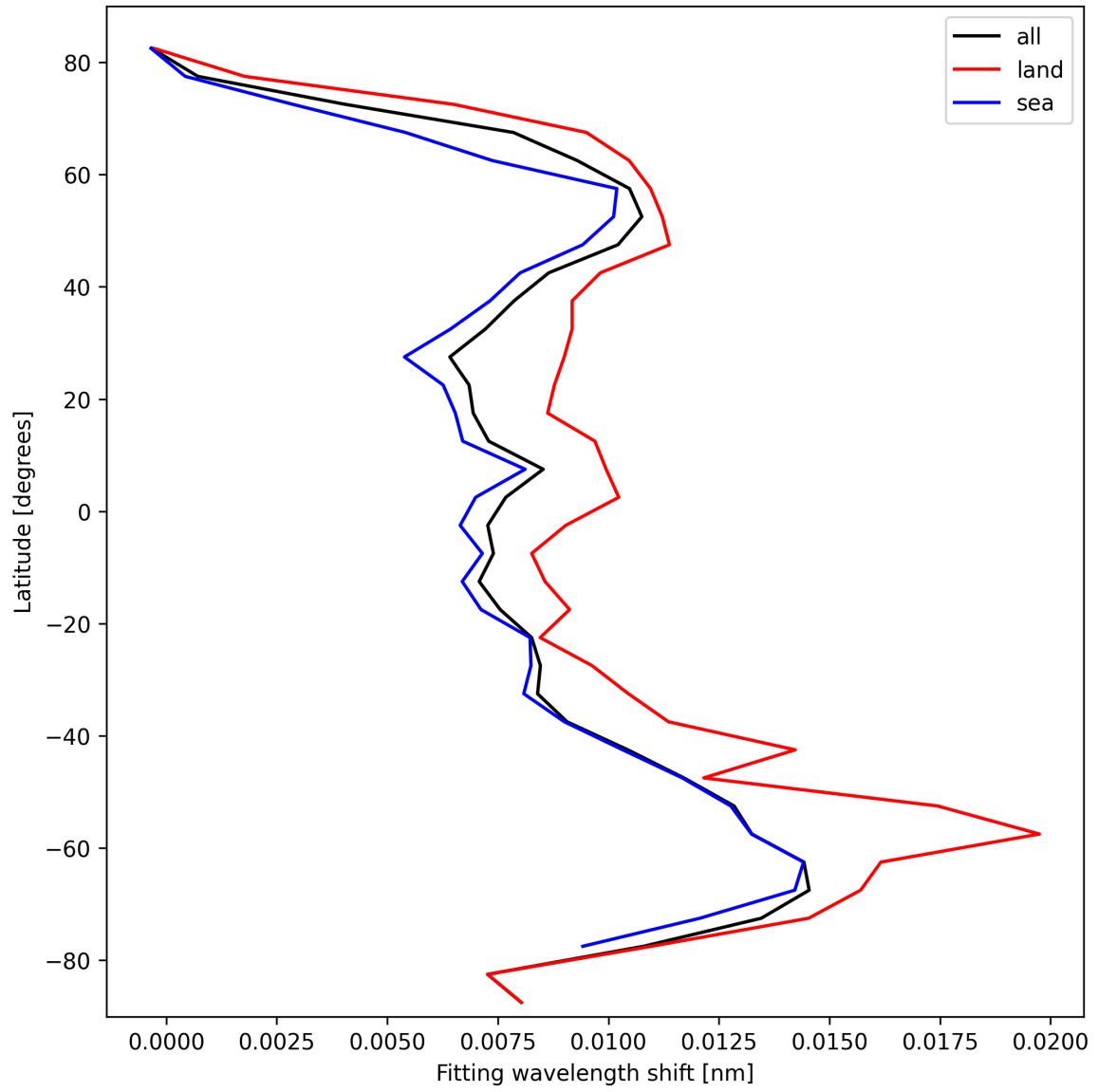
Figure 33: Zonal average of “Fitting wavelength shift” for 2024-10-11 to 2024-10-13.
