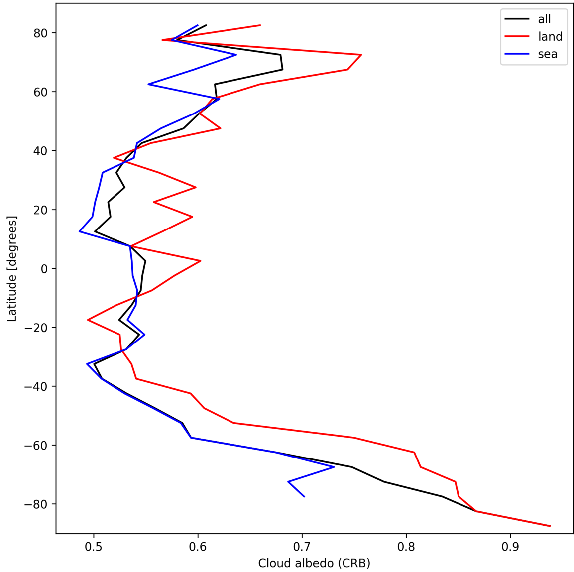
Figure 28: Zonal average of “Cloud albedo (CRB)” for 2024-10-11 to 2024-10-13.
