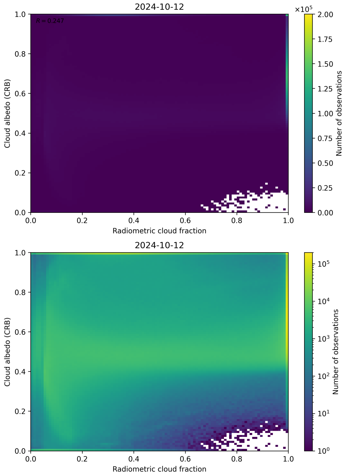
Figure 71: Scatter density plot of “Radiometric cloud fraction” against “Cloud albedo (CRB)” for 2024-10-11 to 2024-10-13.
