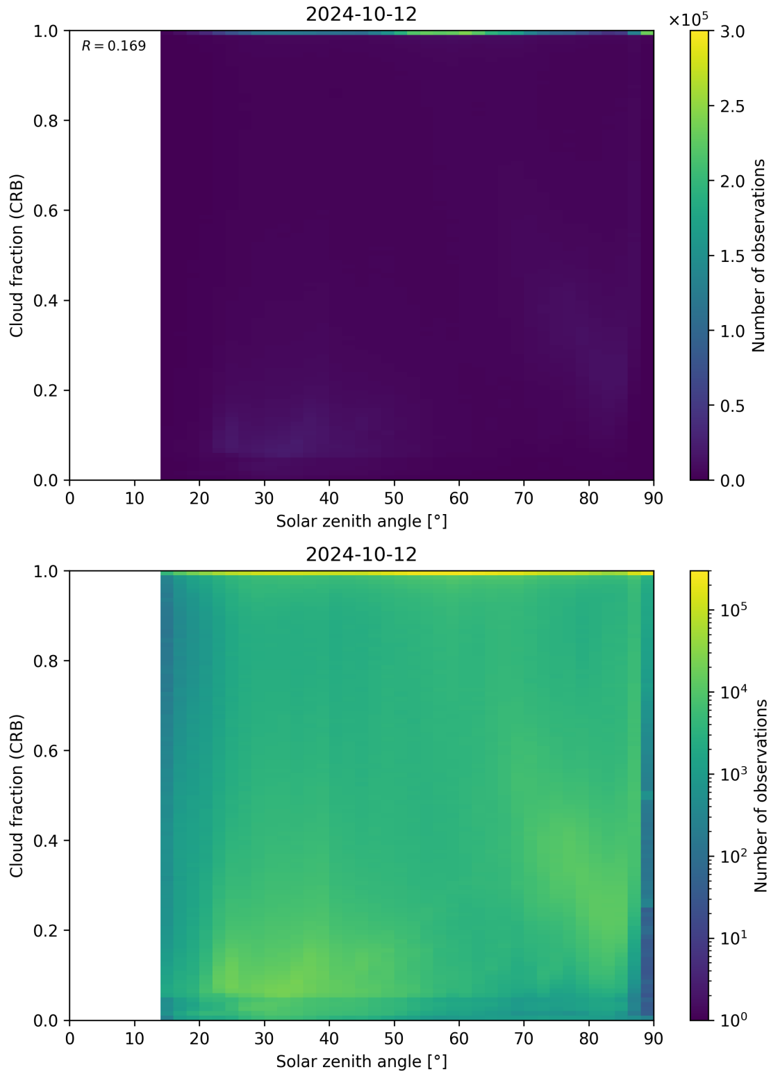
Figure 101: Scatter density plot of “Solar zenith angle” against “Cloud fraction (CRB)” for 2024-10-11 to 2024-10-13.
