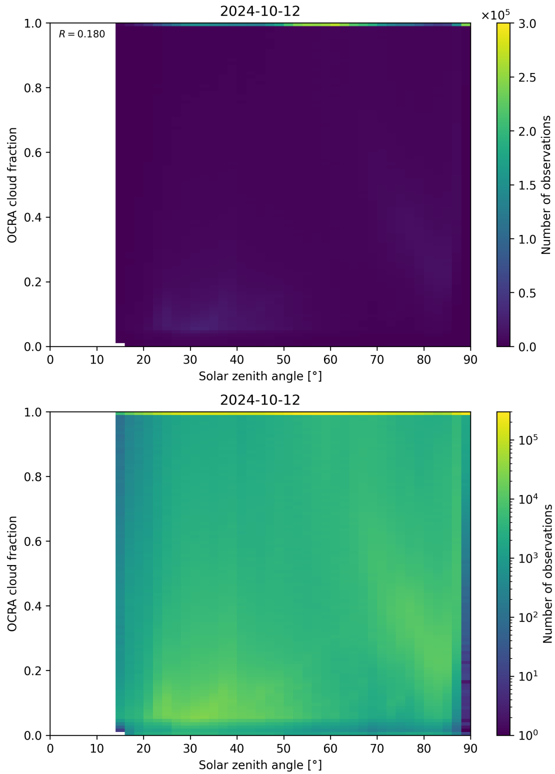
Figure 100: Scatter density plot of “Solar zenith angle” against “OCRA cloud fraction” for 2024-10-11 to 2024-10-13.
