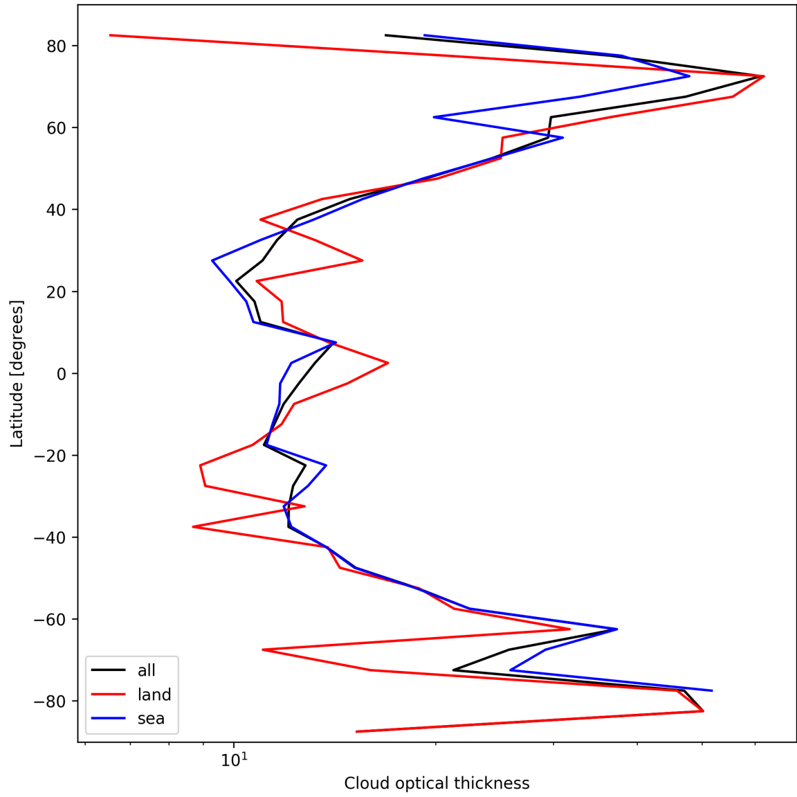
Figure 25: Zonal average of “Cloud optical thickness” for 2024-10-11 to 2024-10-13.
