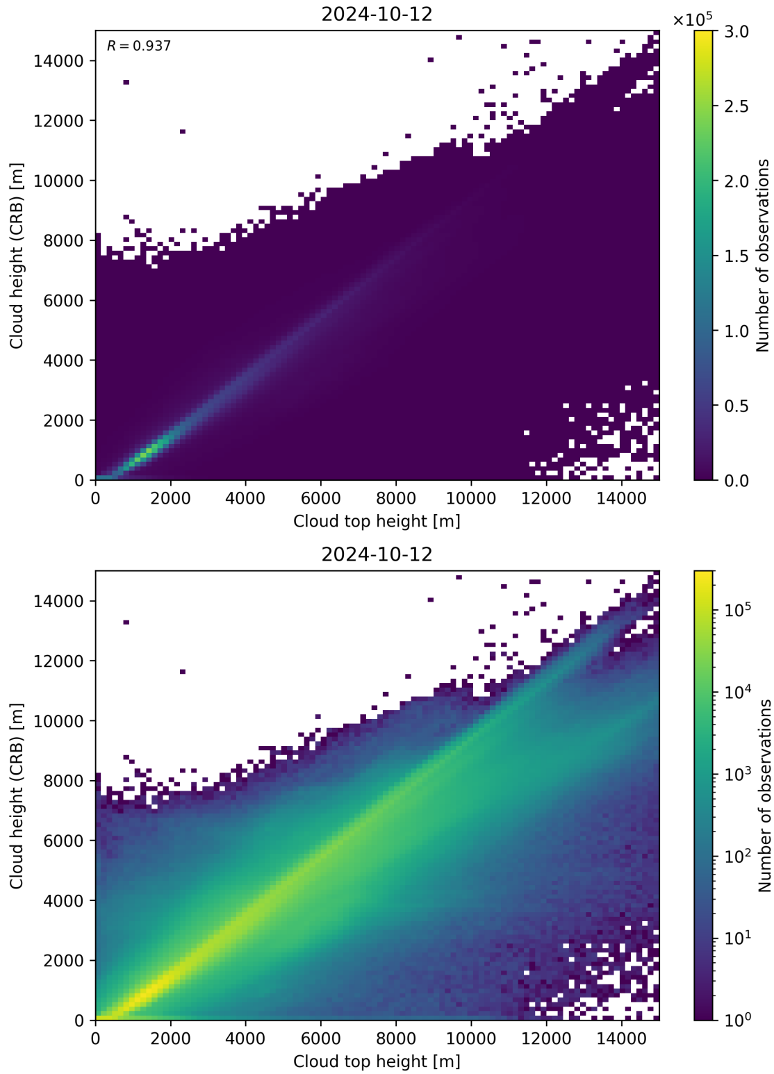
Figure 89: Scatter density plot of “Cloud top height” against “Cloud height (CRB)” for 2024-10-11 to 2024-10-13.
