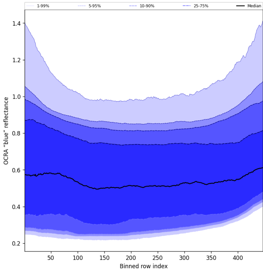
Figure 67: Along track statistics of "OCRA "blue" reflectance" for 2024-10-11 to 2024-10-13
