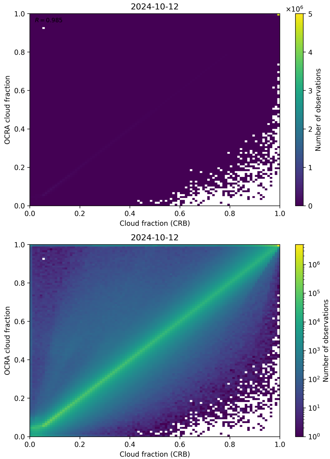
Figure 78: Scatter density plot of “Cloud fraction (CRB)” against “OCRA cloud fraction” for 2024-10-11 to 2024-10-13.
