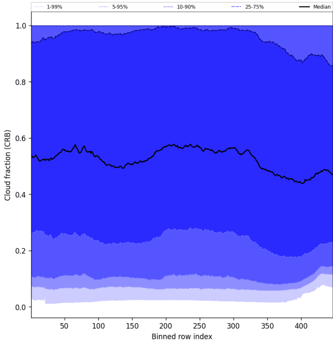
Figure 58: Along track statistics of “Cloud fraction (CRB)” for 2024-10-11 to 2024-10-13
