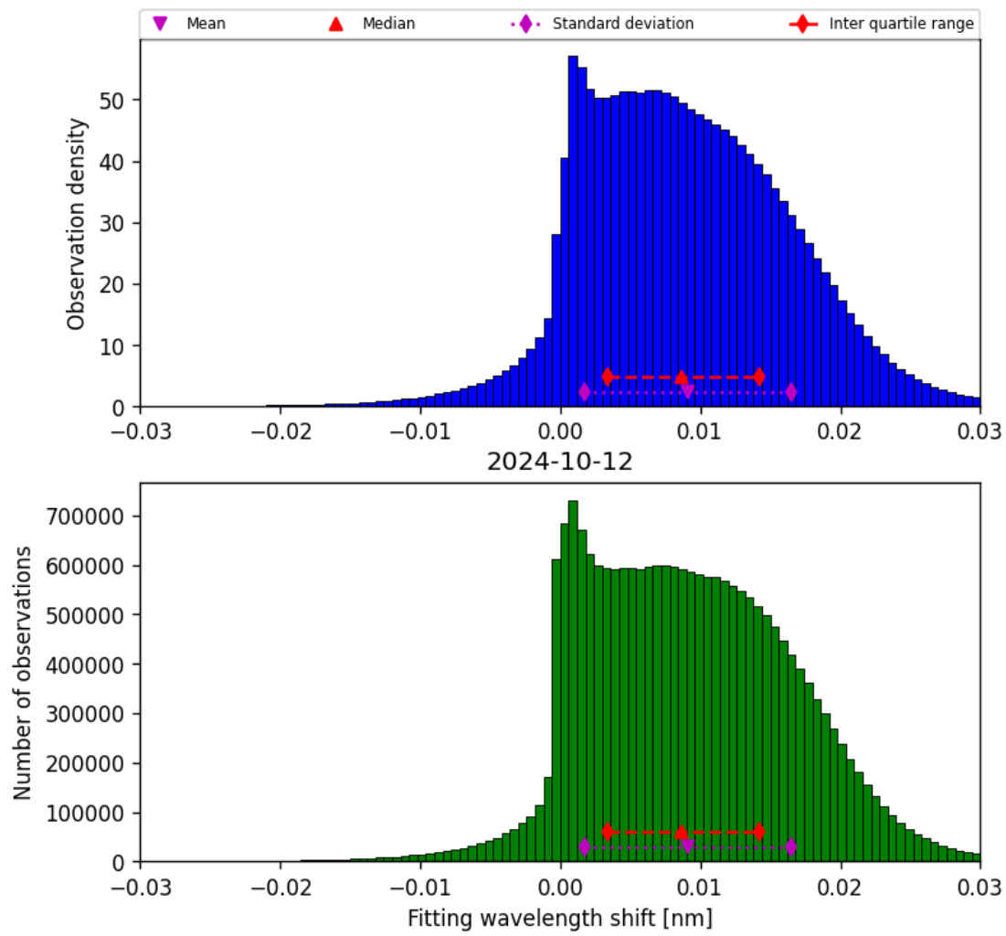
Figure 49: Histogram of “Fitting wavelength shift” for 2024-10-11 to 2024-10-13
