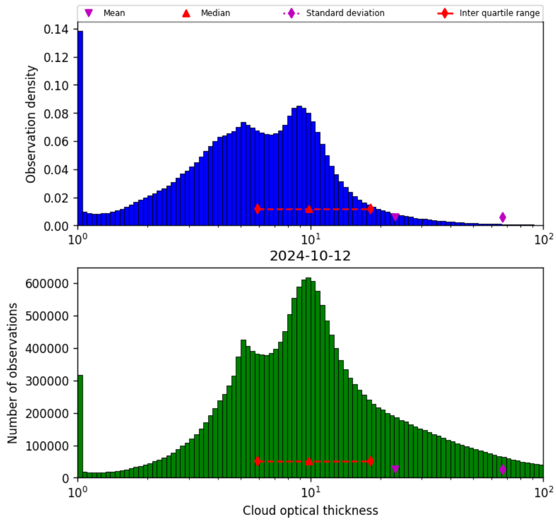
Figure 41: Histogram of “Cloud optical thickness” for 2024-10-11 to 2024-10-13
