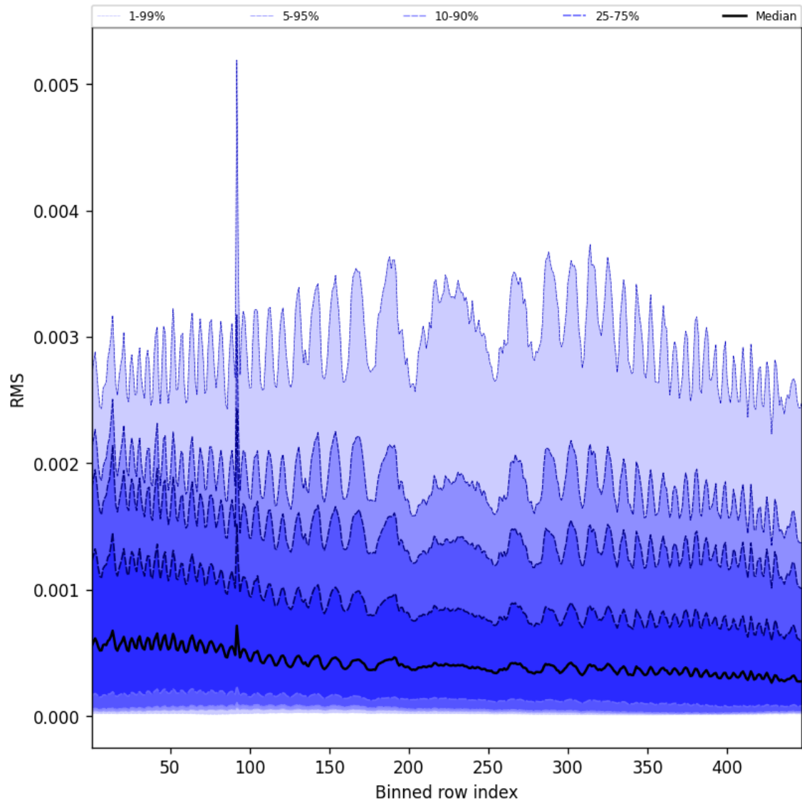
Figure 63: Along track statistics of “RMS” for 2024-10-11 to 2024-10-13
