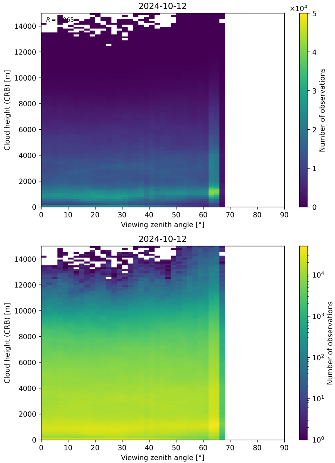
Figure 110: Scatter density plot of “Viewing zenith angle” against “Cloud height (CRB)” for 2024-10-11 to 2024-10-13.
