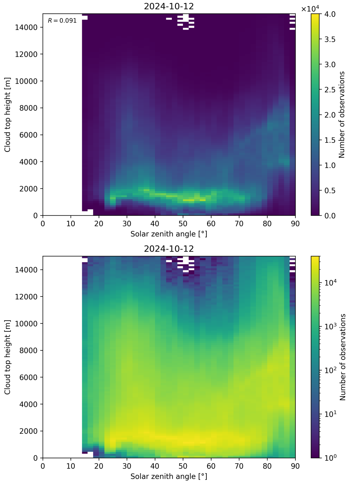
Figure 104: Scatter density plot of “Solar zenith angle” against “Cloud top height” for 2024-10-11 to 2024-10-13.
