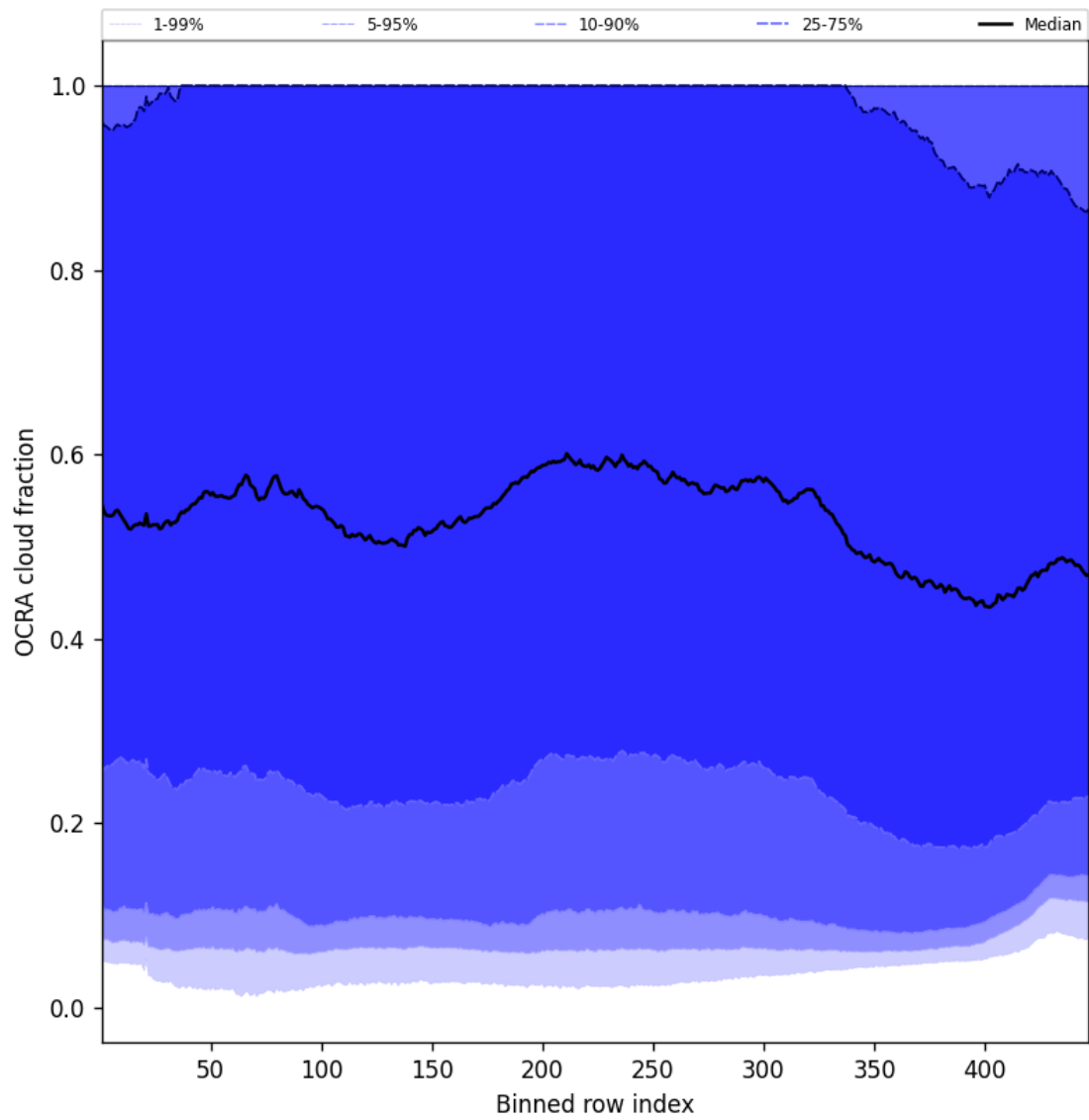
Figure 66: Along track statistics of “OCRA cloud fraction” for 2024-10-11 to 2024-10-13
