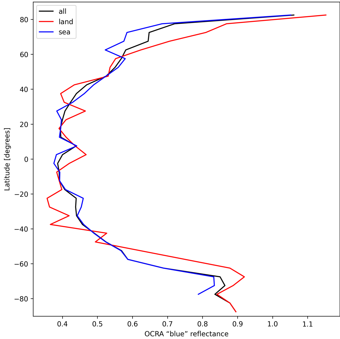
Figure 35: Zonal average of "OCRA "blue" reflectance" for 2024-10-11 to 2024-10-13.
