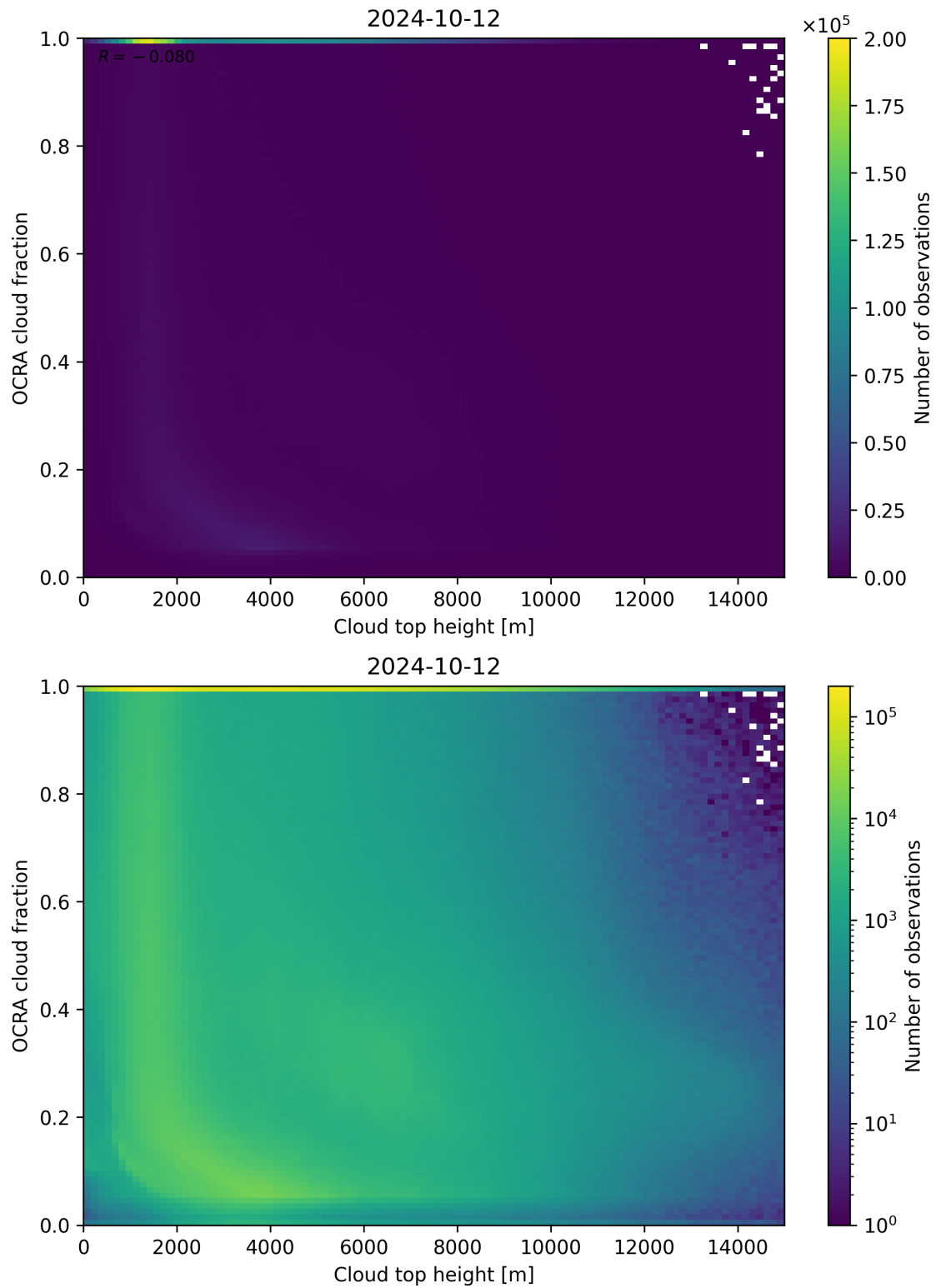
Figure 87: Scatter density plot of “Cloud top height” against “OCRA cloud fraction” for 2024-10-11 to 2024-10-13.
