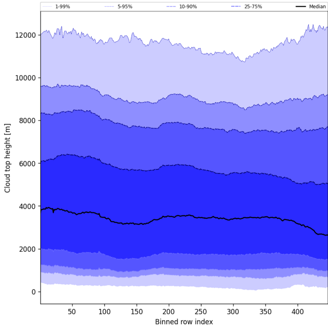
Figure 56: Along track statistics of “Cloud top height” for 2024-10-11 to 2024-10-13
