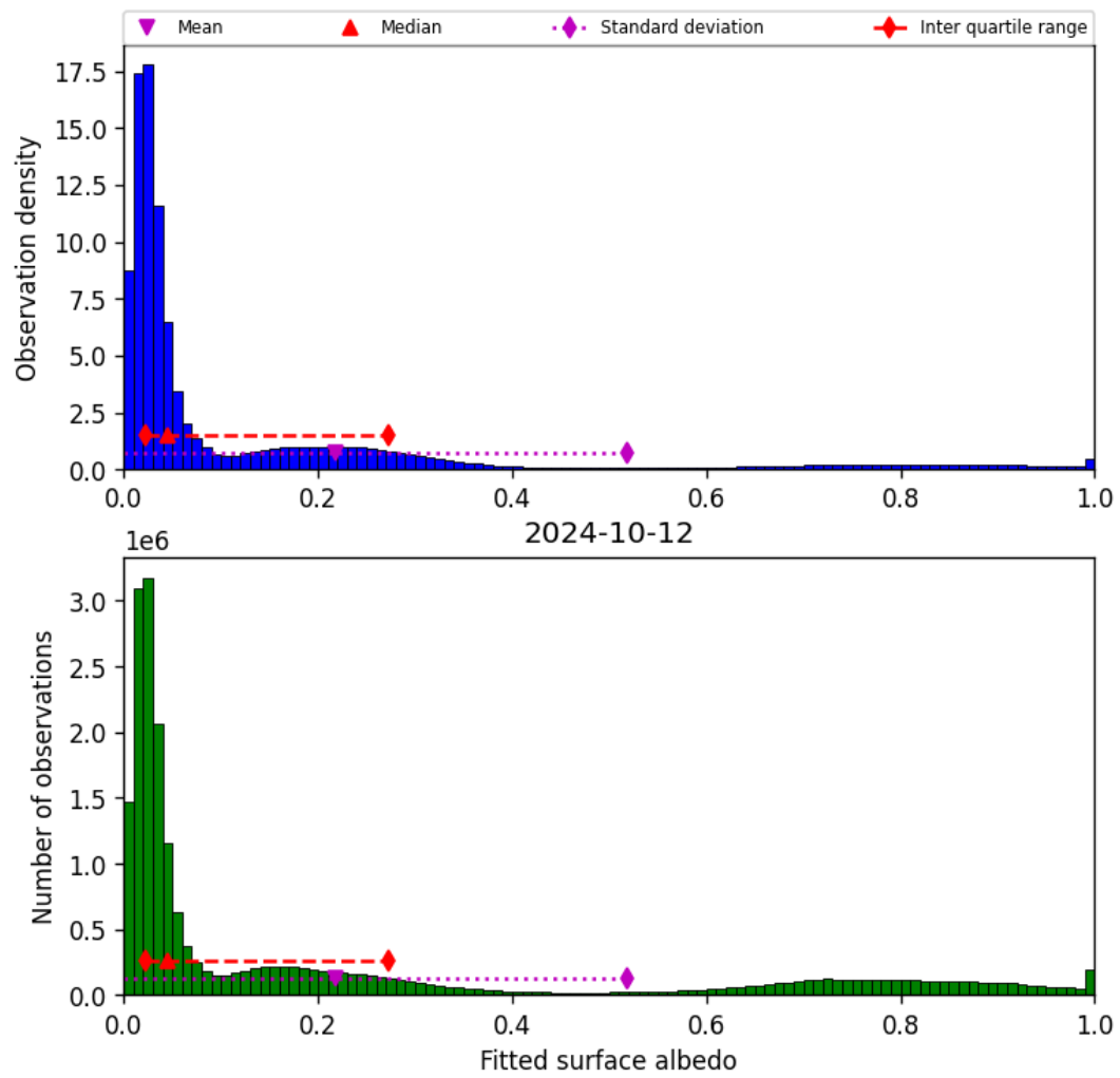
Figure 45: Histogram of “Fitted surface albedo” for 2024-10-11 to 2024-10-13
