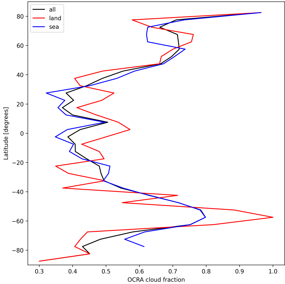
Figure 34: Zonal average of “OCRA cloud fraction” for 2024-10-11 to 2024-10-13.
