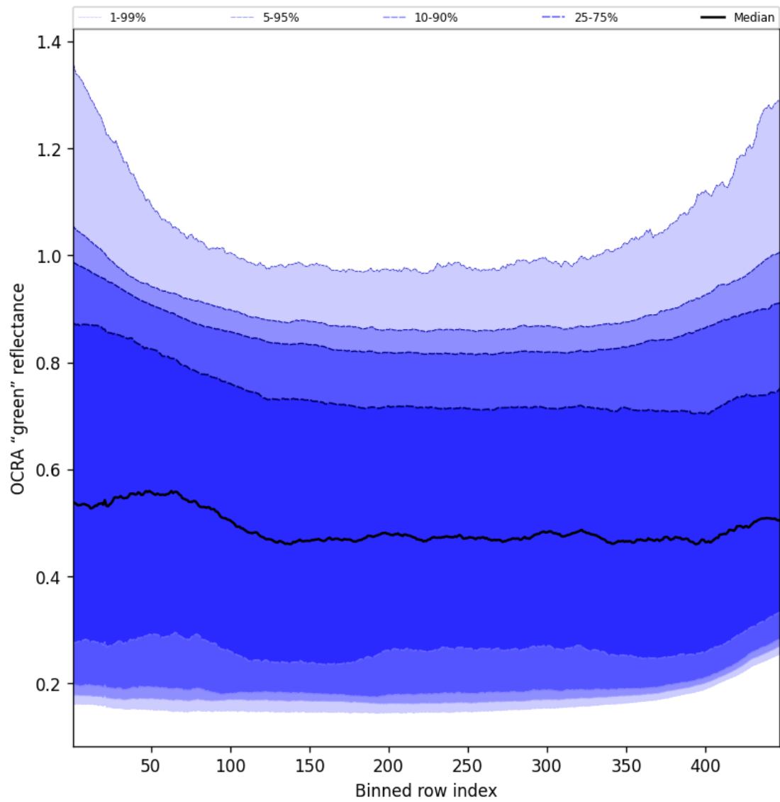
Figure 68: Along track statistics of “OCRA “green” reflectance” for 2024-10-11 to 2024-10-13
