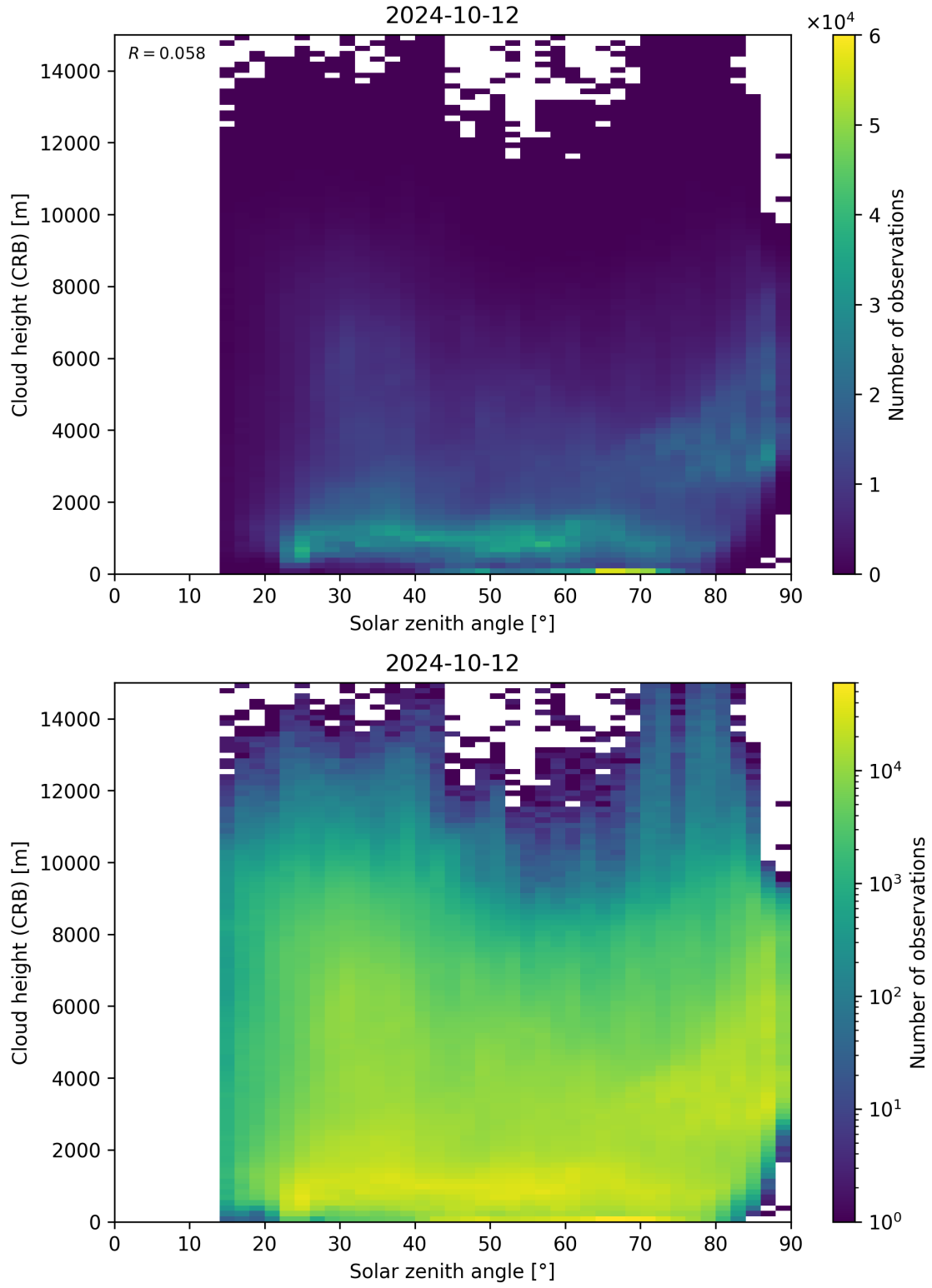
Figure 102: Scatter density plot of “Solar zenith angle” against “Cloud height (CRB)” for 2024-10-11 to 2024-10-13.
