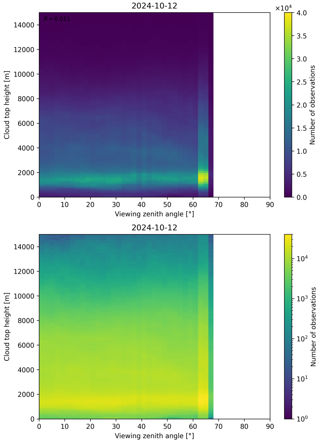
Figure 112: Scatter density plot of “Viewing zenith angle” against “Cloud top height” for 2024-10-11 to 2024-10-13.
