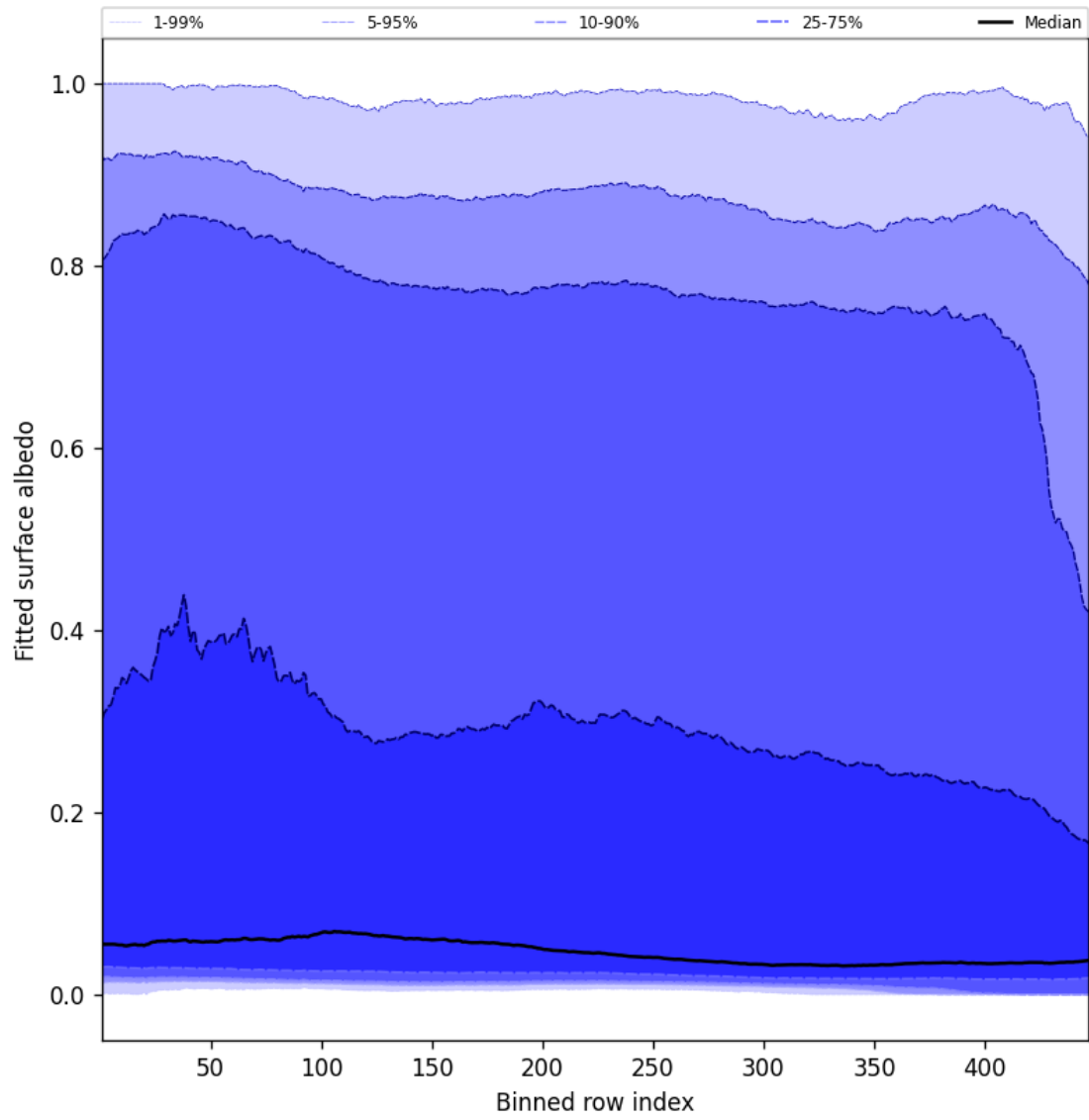
Figure 61: Along track statistics of “Fitted surface albedo” for 2024-10-11 to 2024-10-13
