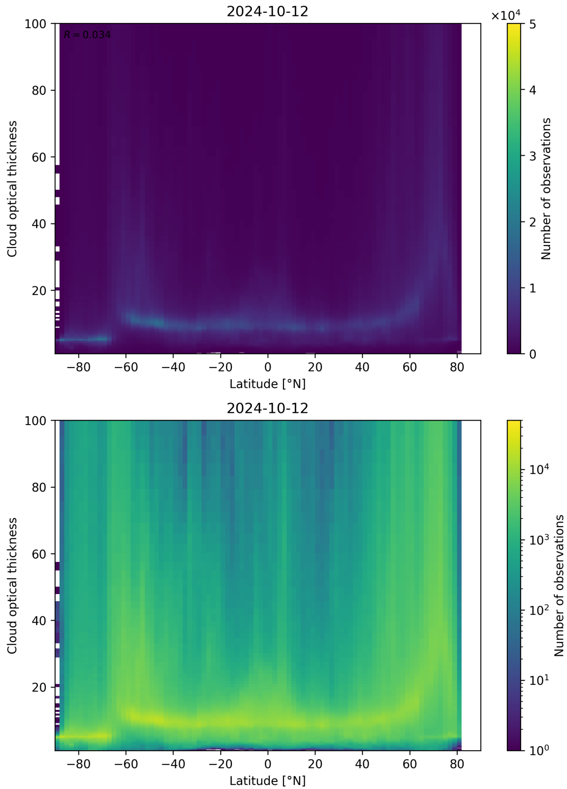
Figure 96: Scatter density plot of “Latitude” against “Cloud optical thickness” for 2024-10-11 to 2024-10-13.
