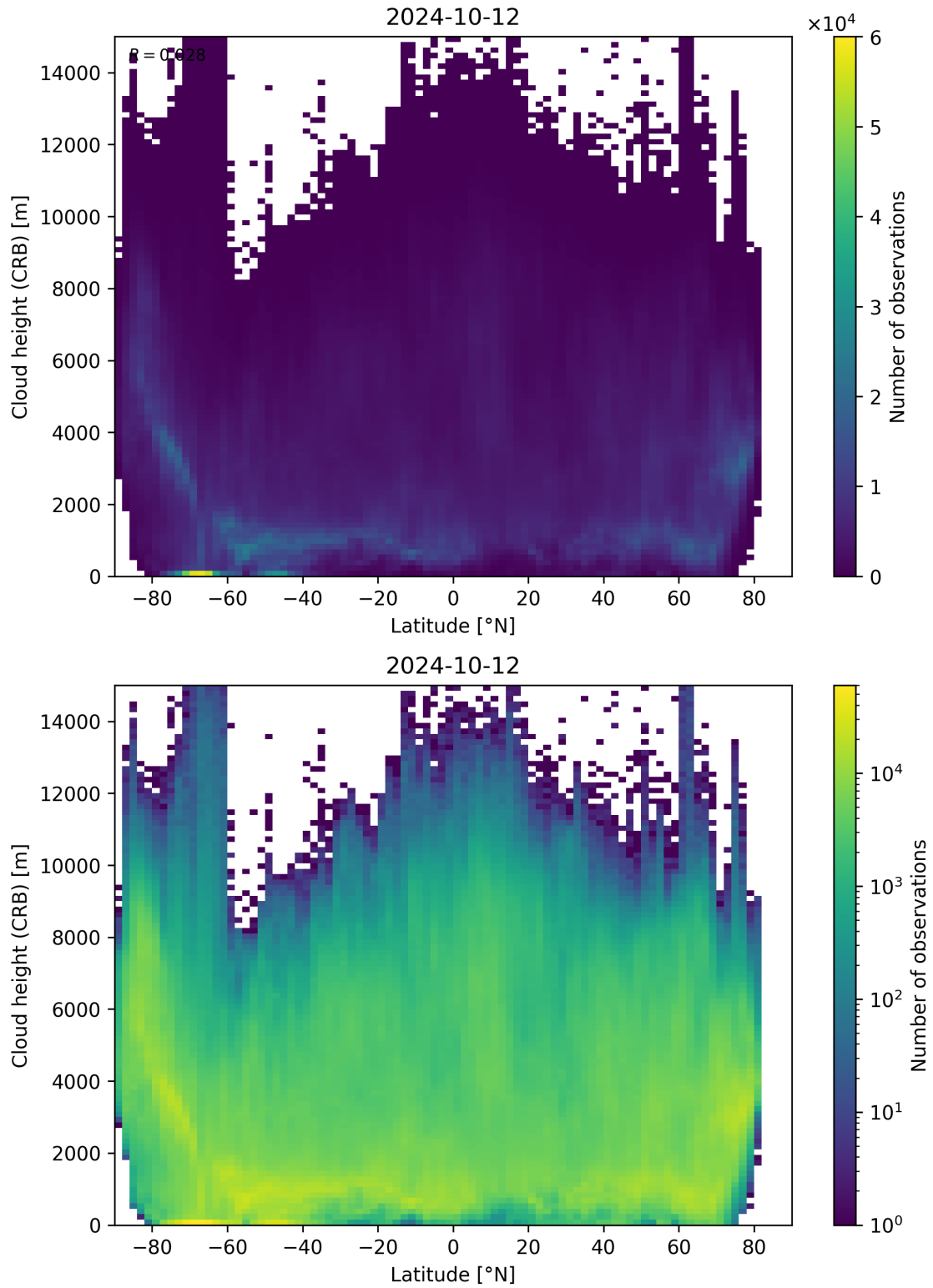
Figure 95: Scatter density plot of “Latitude” against “Cloud height (CRB)” for 2024-10-11 to 2024-10-13.
