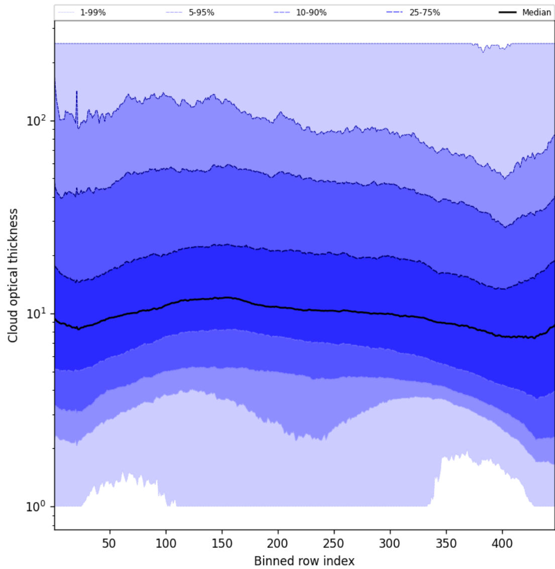
Figure 57: Along track statistics of “Cloud optical thickness” for 2024-10-11 to 2024-10-13
