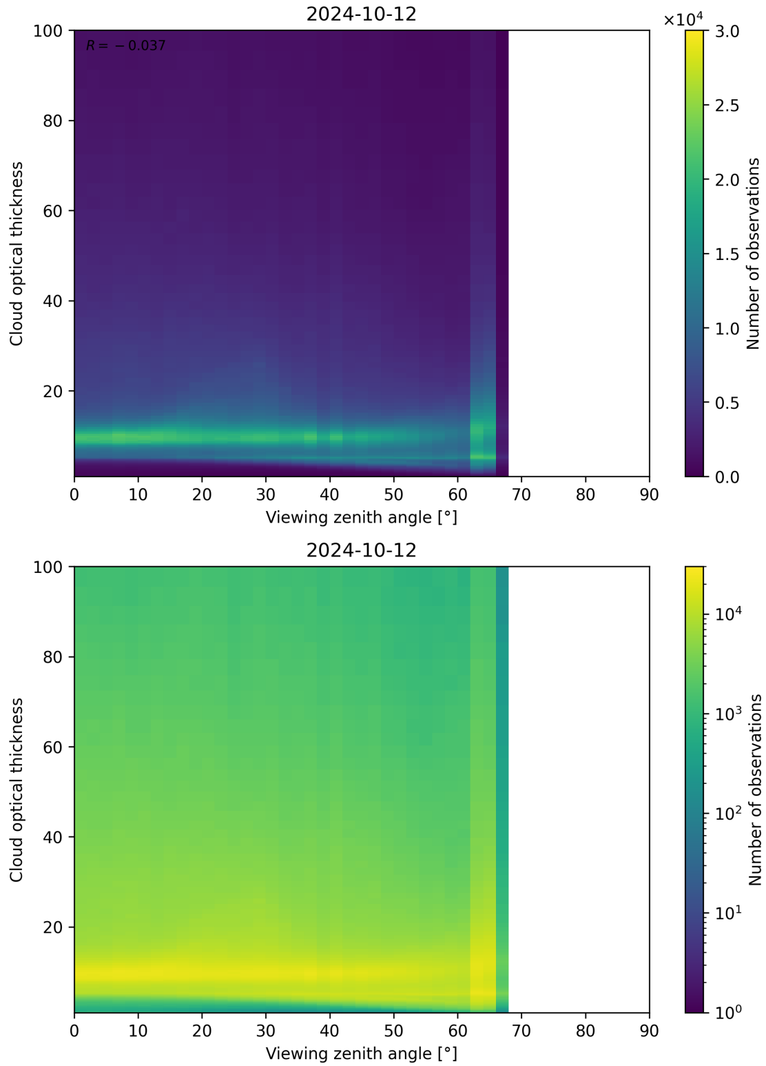
Figure 111: Scatter density plot of “Viewing zenith angle” against “Cloud optical thickness” for 2024-10-11 to 2024-10-13.
