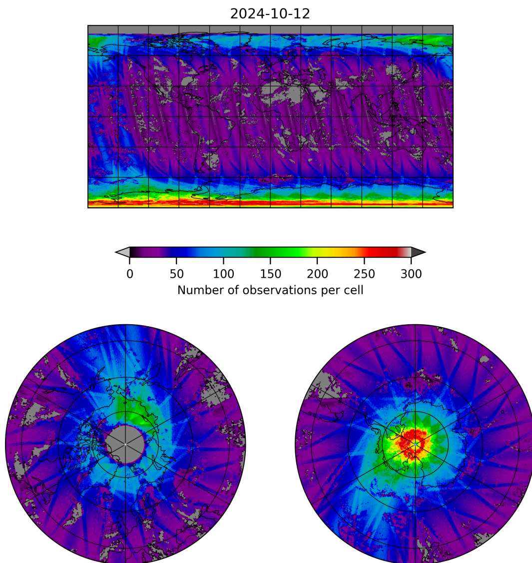
Figure 21: Map of the number of observations for 2024-10-11 to 2024-10-13
