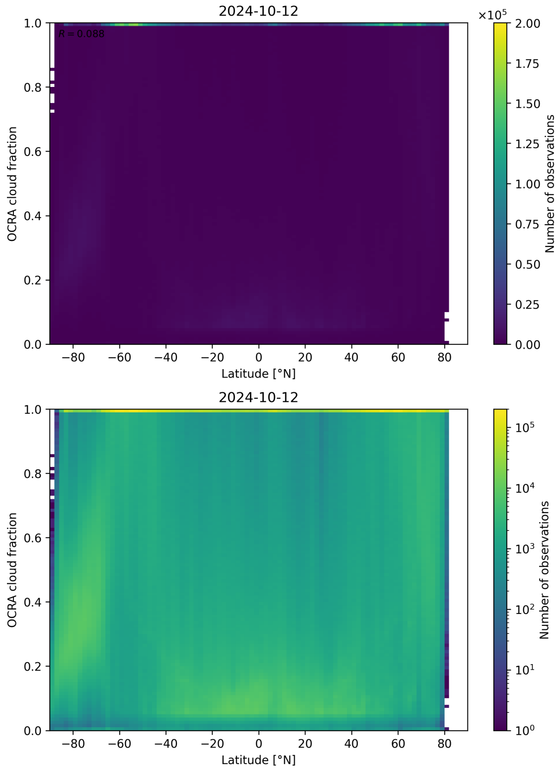
Figure 93: Scatter density plot of “Latitude” against “OCRA cloud fraction” for 2024-10-11 to 2024-10-13.
