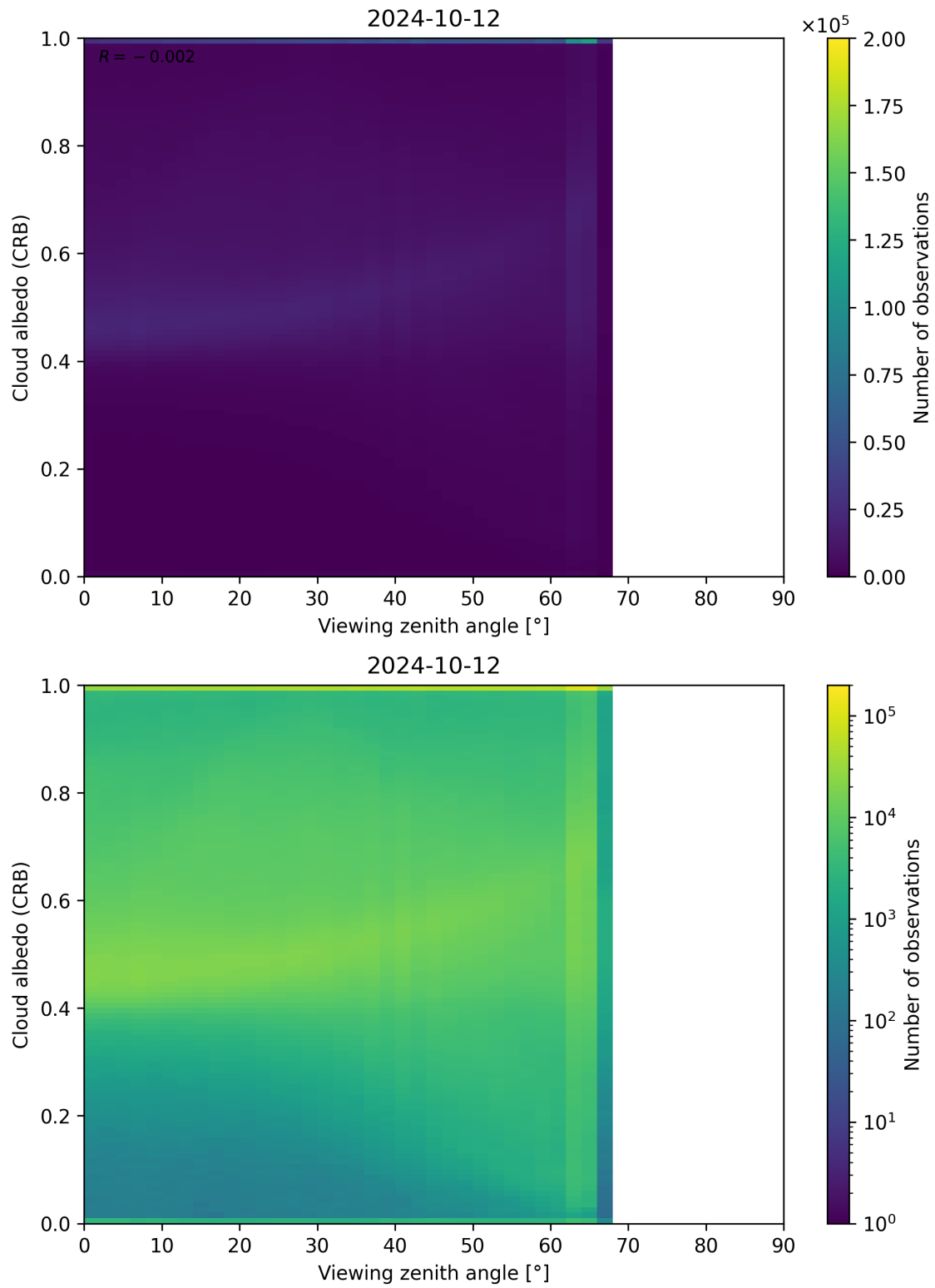
Figure 106: Scatter density plot of “Viewing zenith angle” against “Cloud albedo (CRB)” for 2024-10-11 to 2024-10-13.
