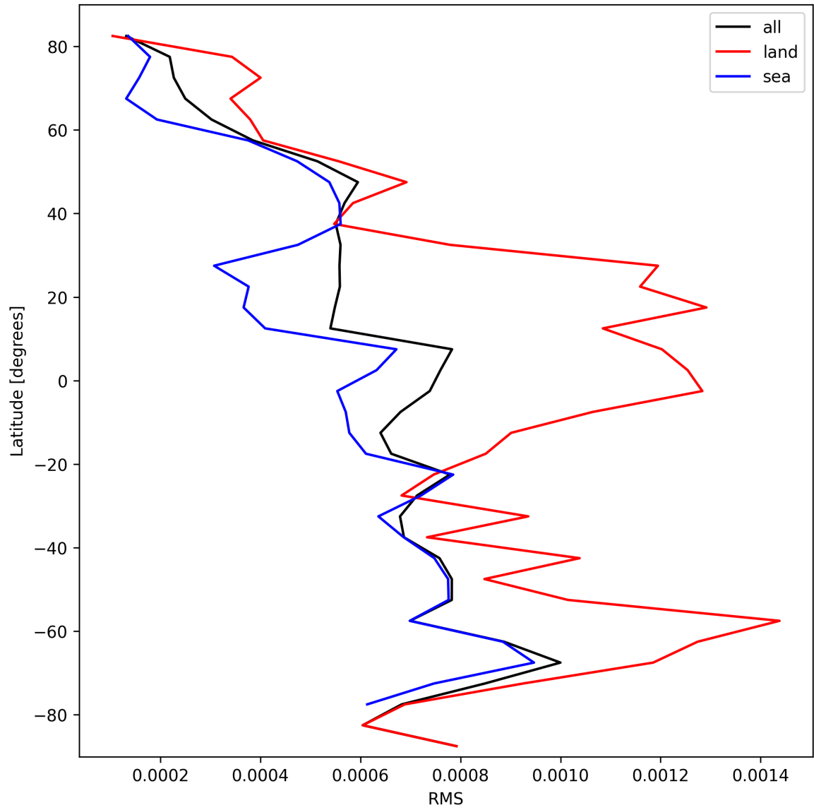
Figure 31: Zonal average of “RMS” for 2024-10-11 to 2024-10-13.
