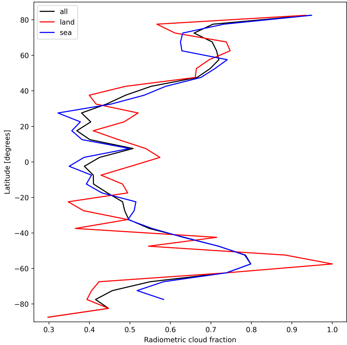
Figure 23: Zonal average of “Radiometric cloud fraction” for 2024-10-11 to 2024-10-13.
