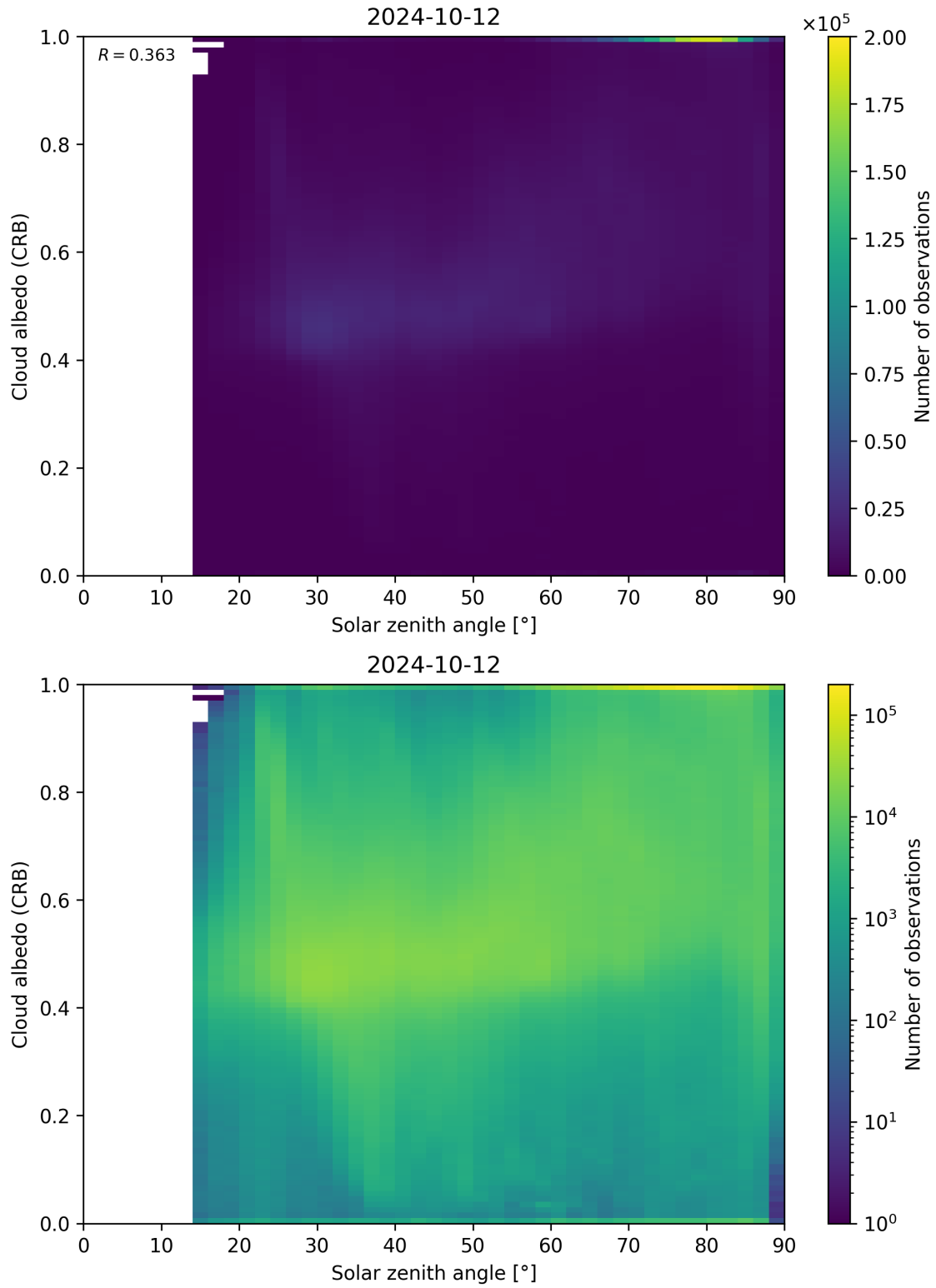
Figure 98: Scatter density plot of “Solar zenith angle” against “Cloud albedo (CRB)” for 2024-10-11 to 2024-10-13.
