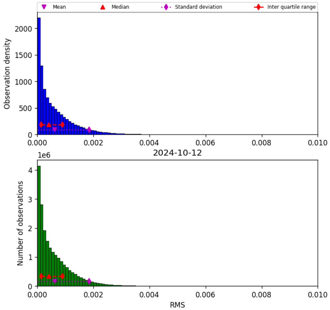
Figure 47: Histogram of “RMS” for 2024-10-11 to 2024-10-13
