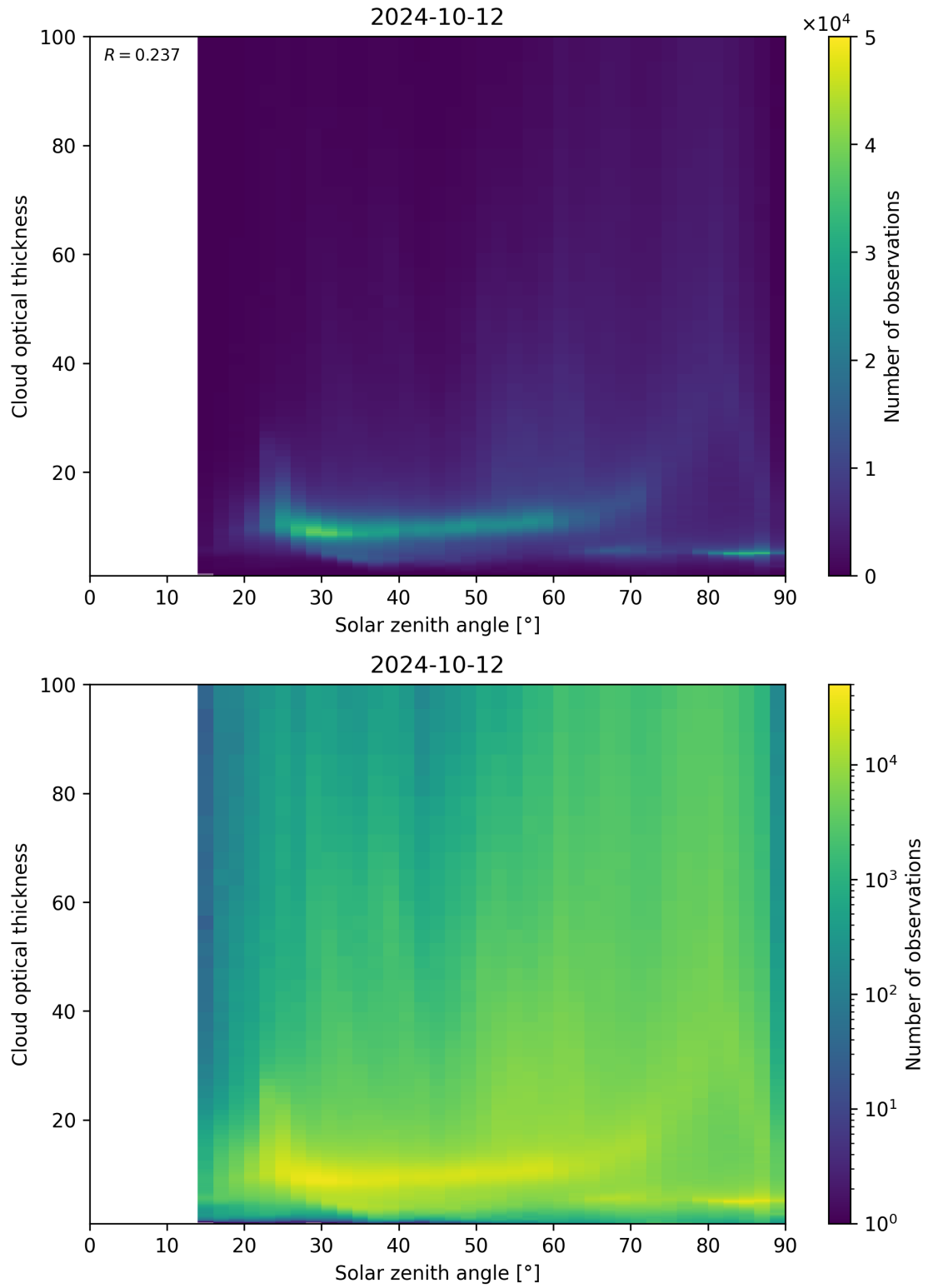
Figure 103: Scatter density plot of “Solar zenith angle” against “Cloud optical thickness” for 2024-10-11 to 2024-10-13.
