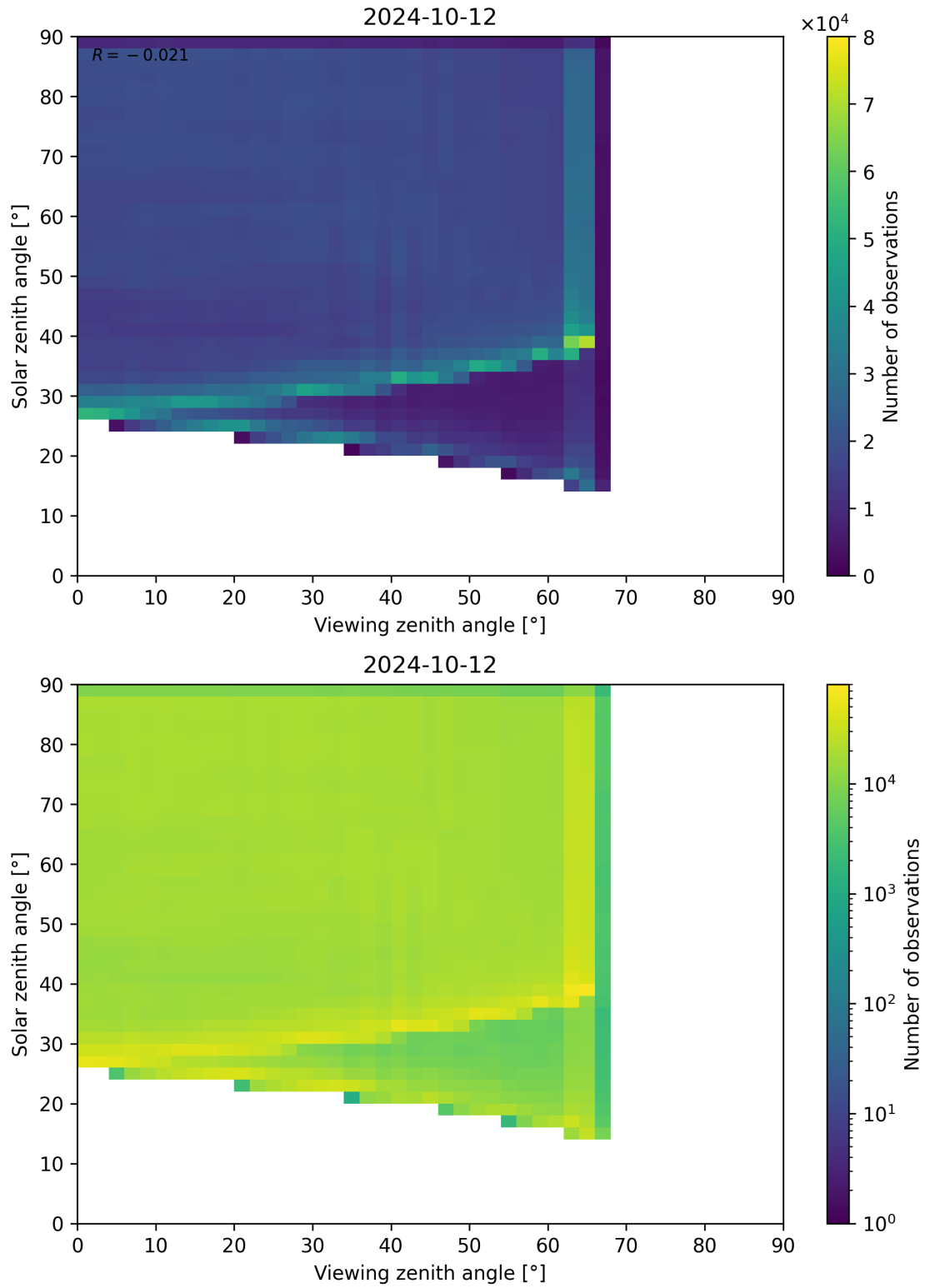
Figure 114: Scatter density plot of “Viewing zenith angle” against “Solar zenith angle” for 2024-10-11 to 2024-10-13.
