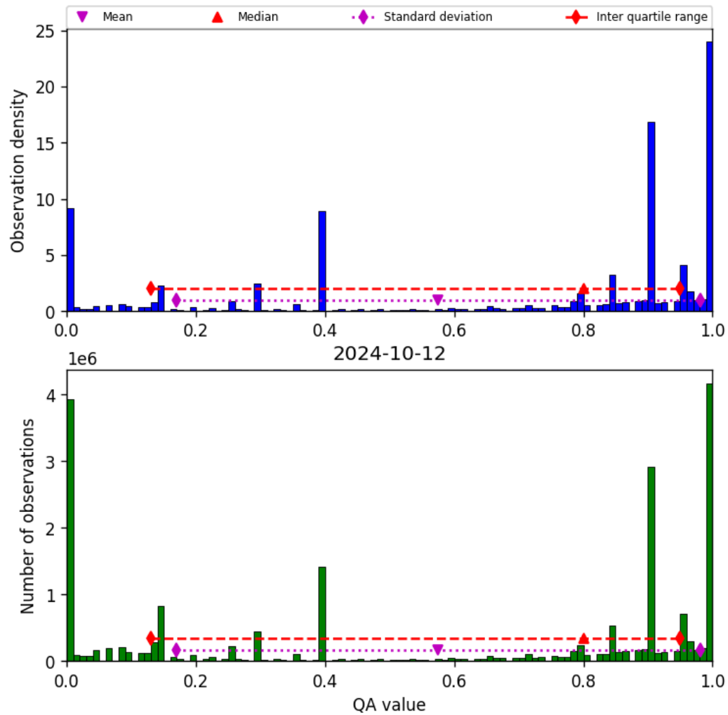
Figure 38: Histogram of “QA value” for 2024-10-11 to 2024-10-13
