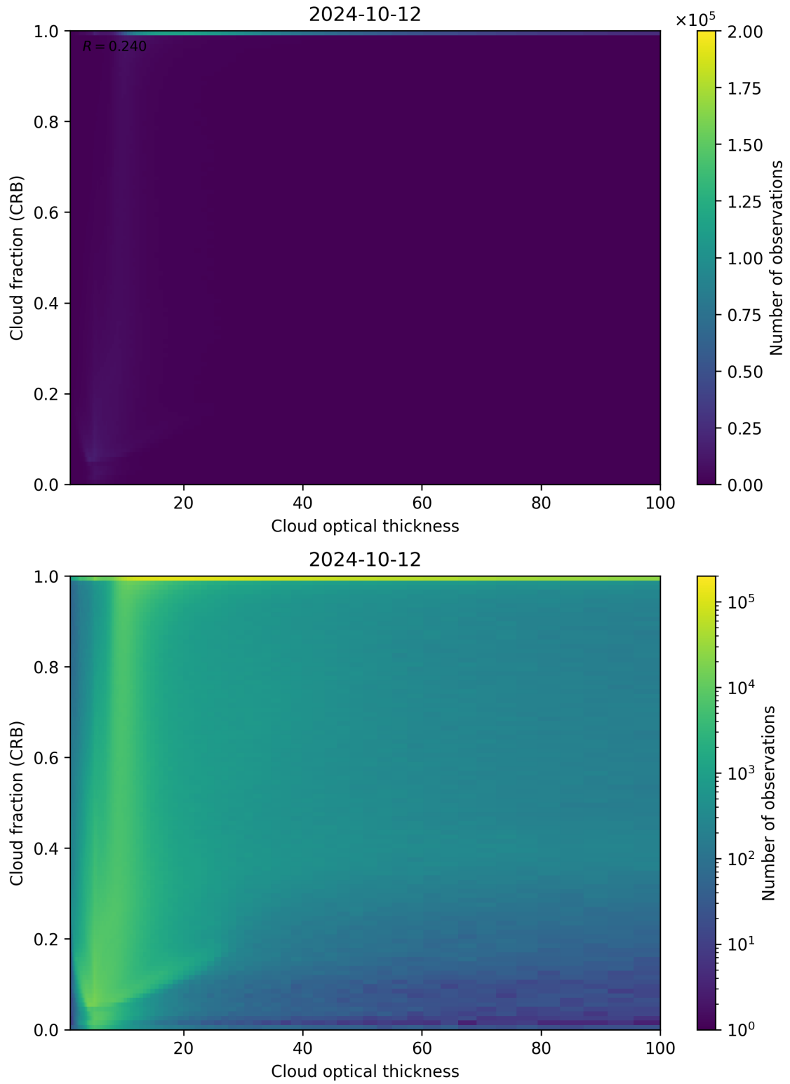
Figure 84: Scatter density plot of “Cloud optical thickness” against “Cloud fraction (CRB)” for 2024-10-11 to 2024-10-13.
