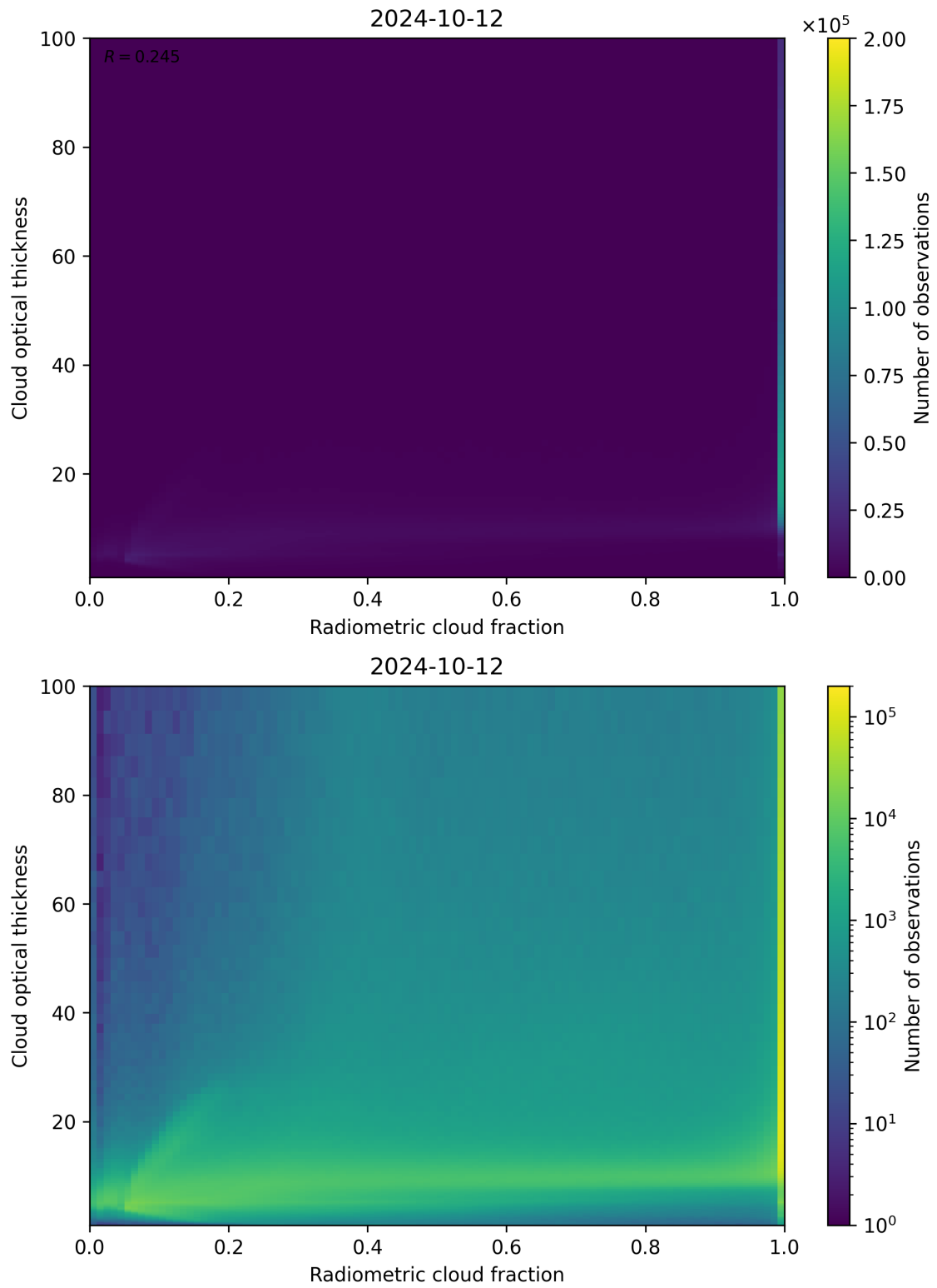
Figure 75: Scatter density plot of “Radiometric cloud fraction” against “Cloud optical thickness” for 2024-10-11 to 2024-10-13.
