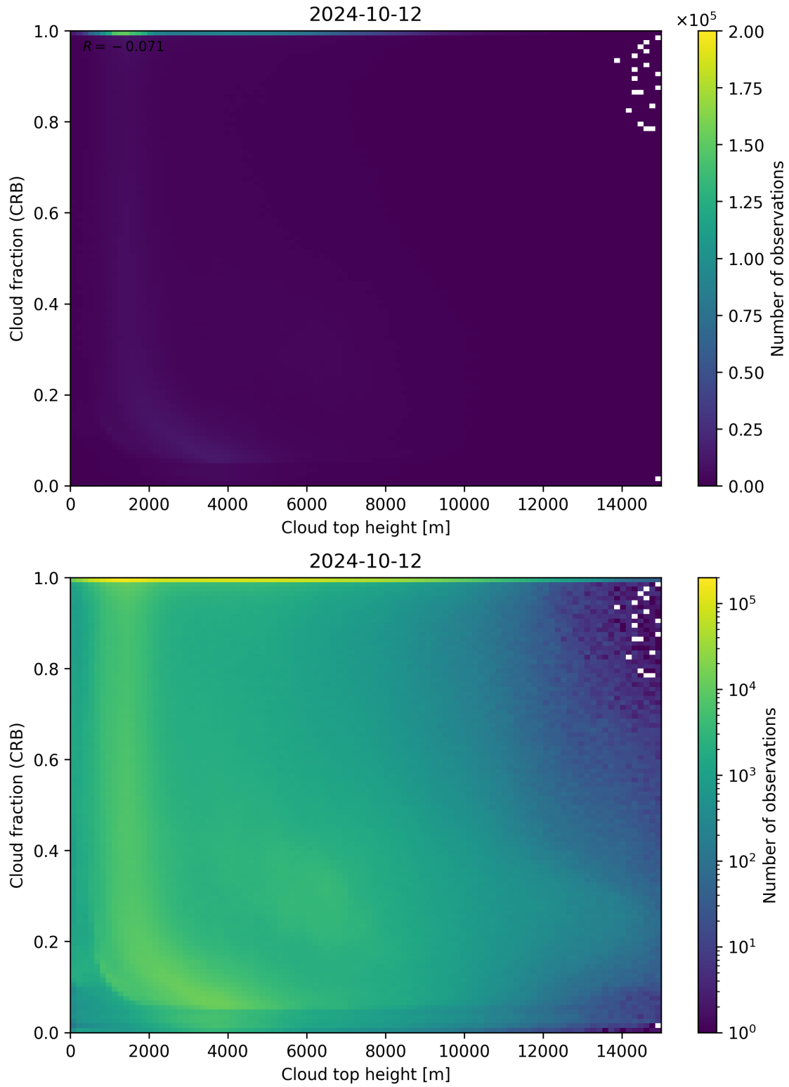
Figure 88: Scatter density plot of “Cloud top height” against “Cloud fraction (CRB)” for 2024-10-11 to 2024-10-13.
