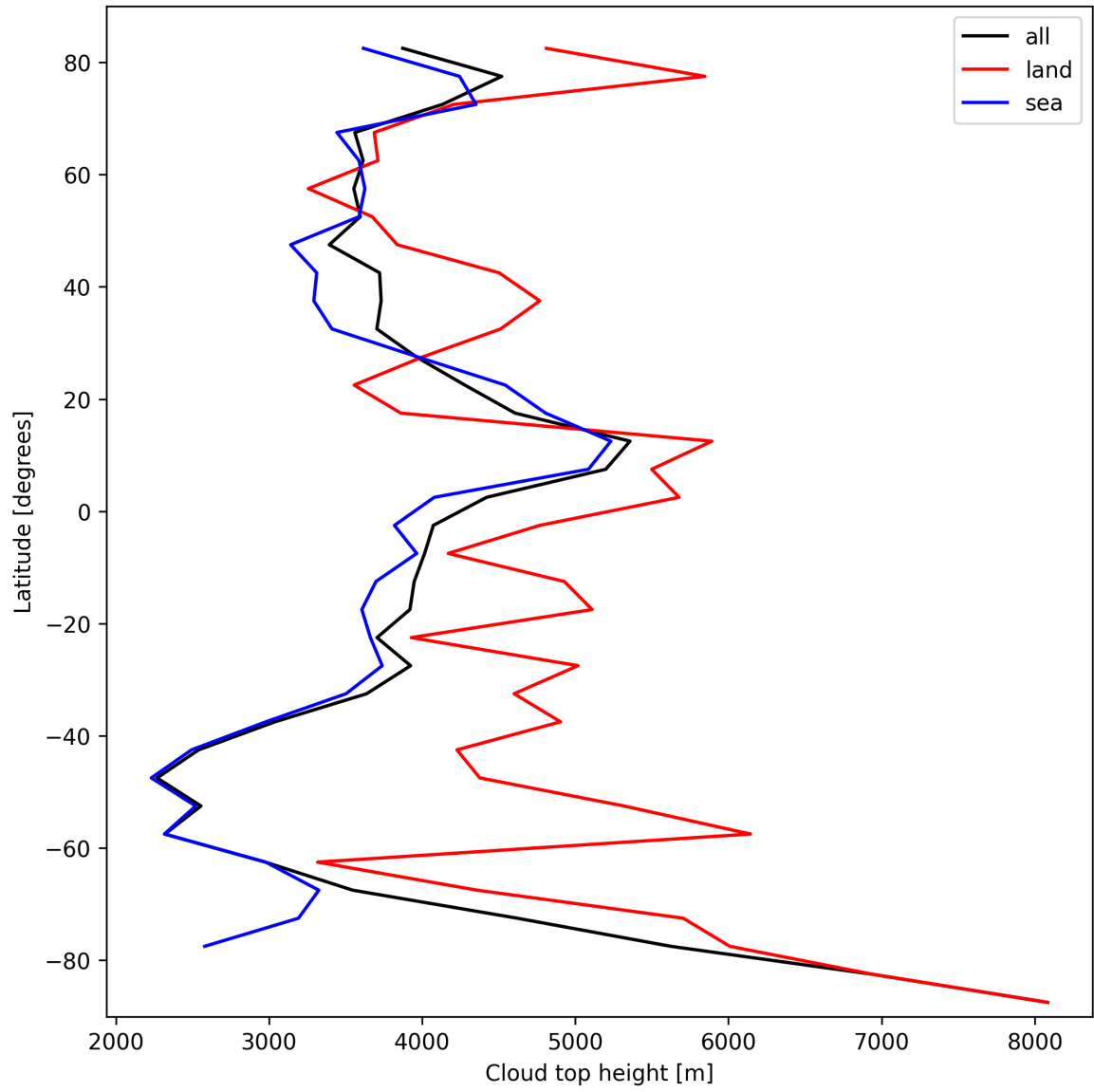
Figure 24: Zonal average of “Cloud top height” for 2024-10-11 to 2024-10-13.
