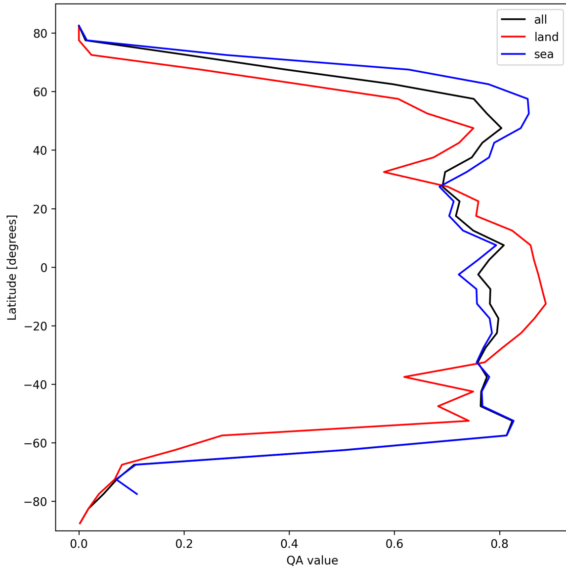
Figure 22: Zonal average of “QA value” for 2024-10-11 to 2024-10-13.
