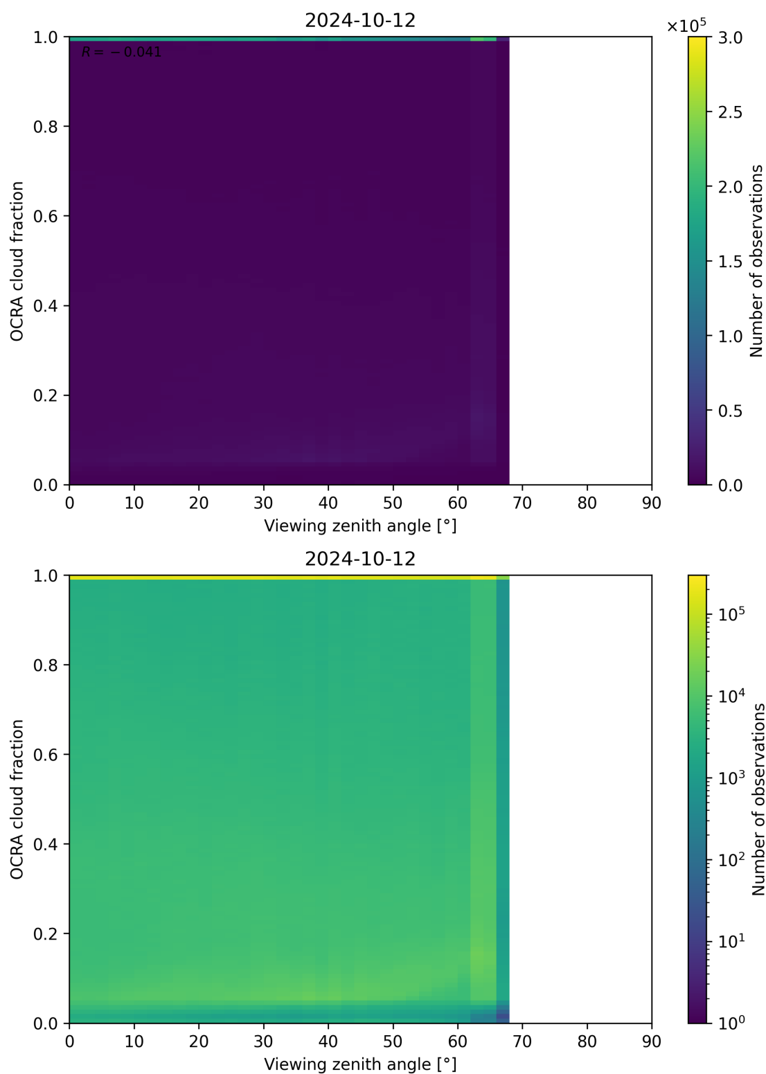
Figure 108: Scatter density plot of “Viewing zenith angle” against “OCRA cloud fraction” for 2024-10-11 to 2024-10-13.
