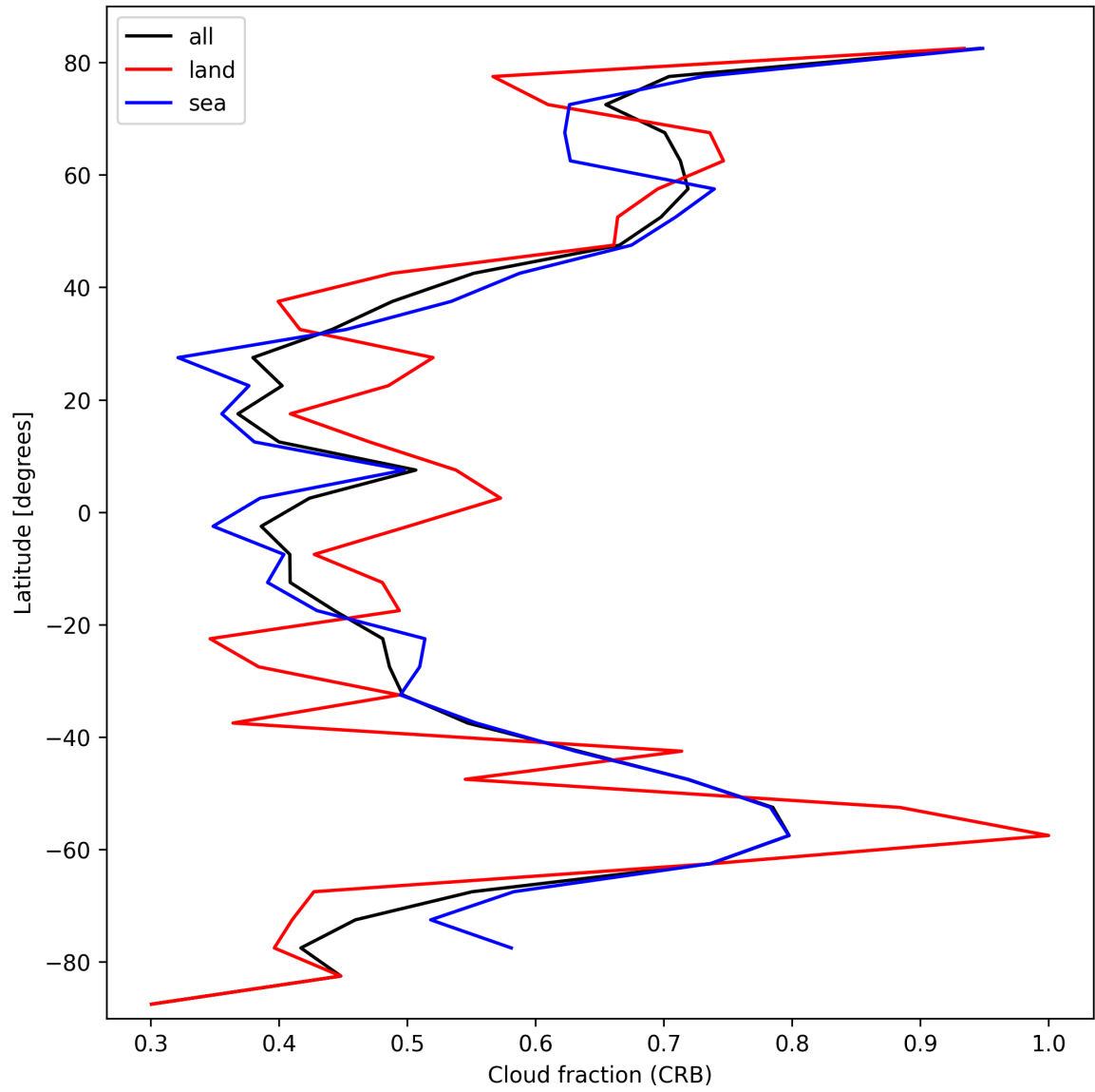
Figure 26: Zonal average of “Cloud fraction (CRB)” for 2024-10-11 to 2024-10-13.
