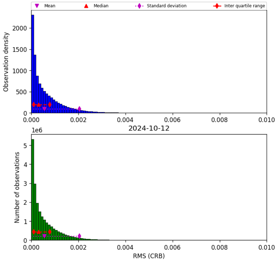
Figure 48: Histogram of “RMS (CRB)” for 2024-10-11 to 2024-10-13
