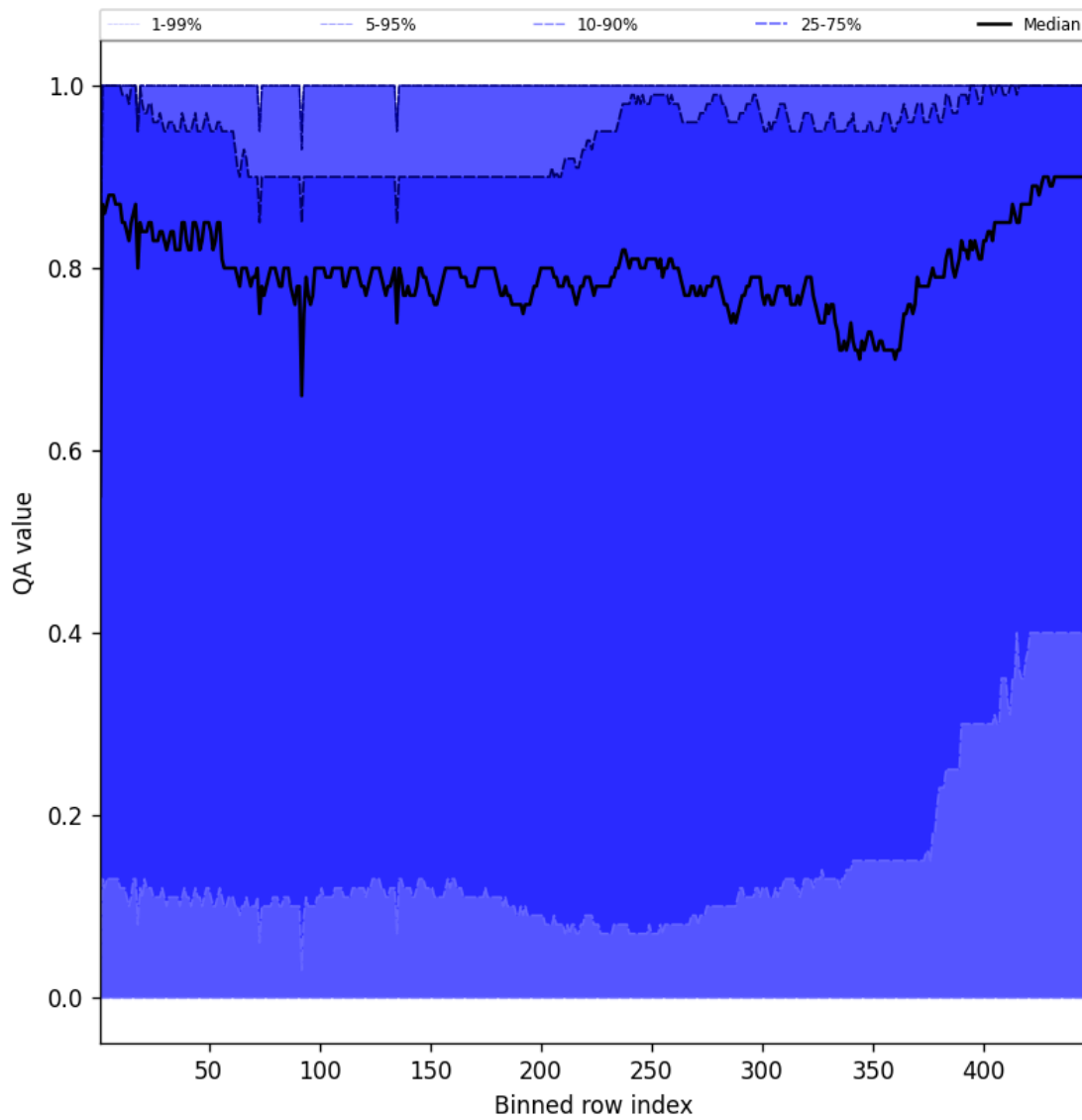
Figure 54: Along track statistics of “QA value” for 2024-10-11 to 2024-10-13
