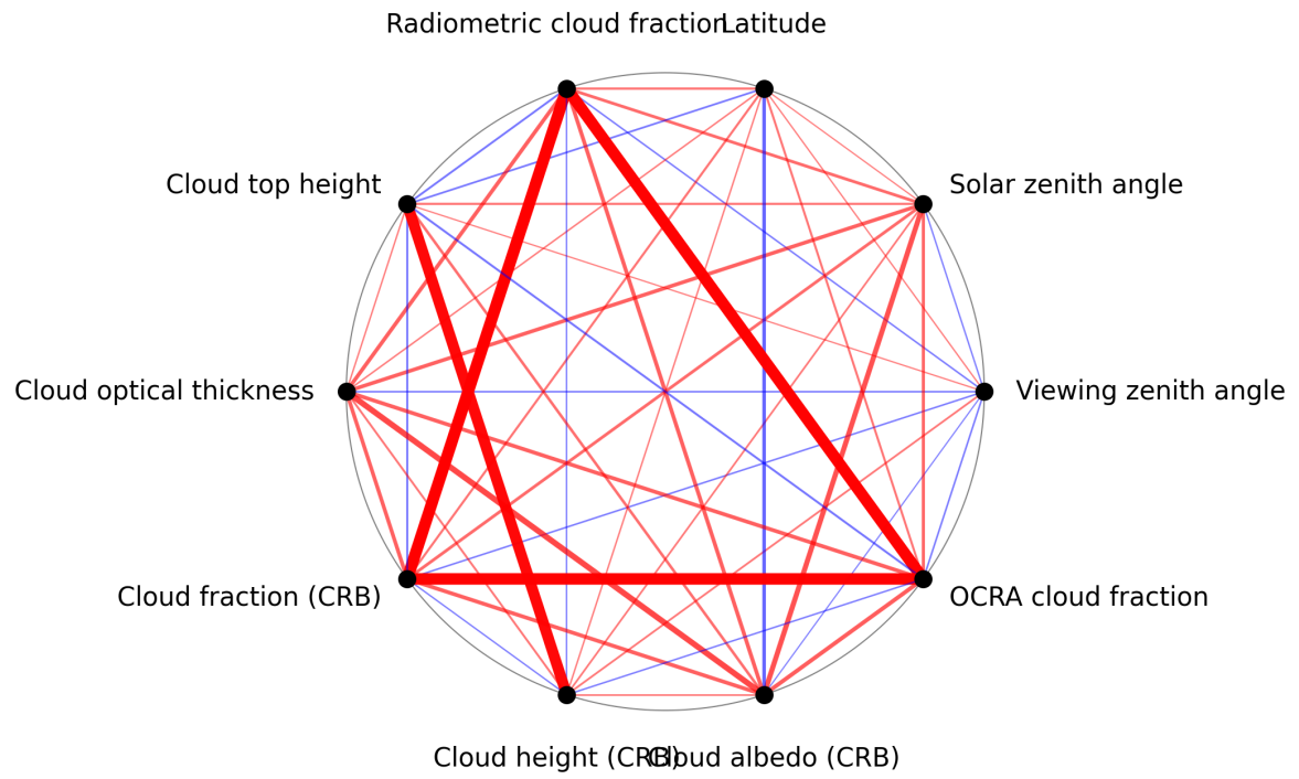
Figure 1: Map of correlation graph for 2024-10-11 to 2024-10-13.
