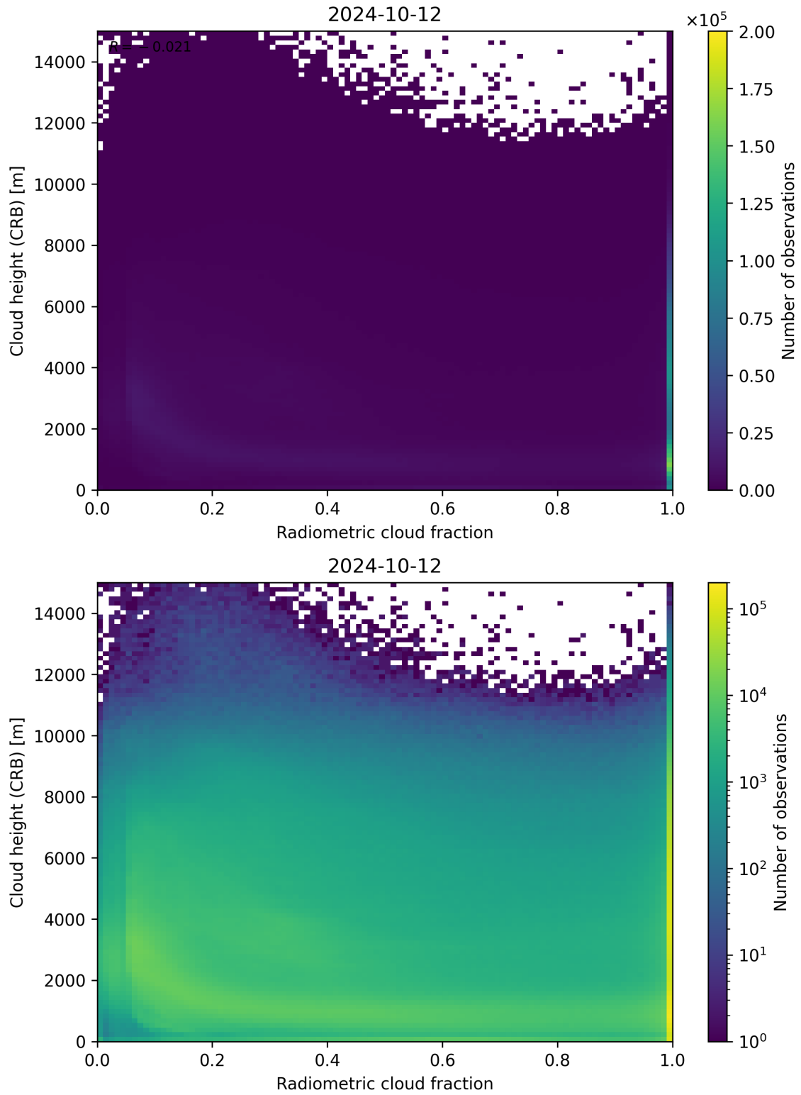
Figure 74: Scatter density plot of “Radiometric cloud fraction” against “Cloud height (CRB)” for 2024-10-11 to 2024-10-13.
