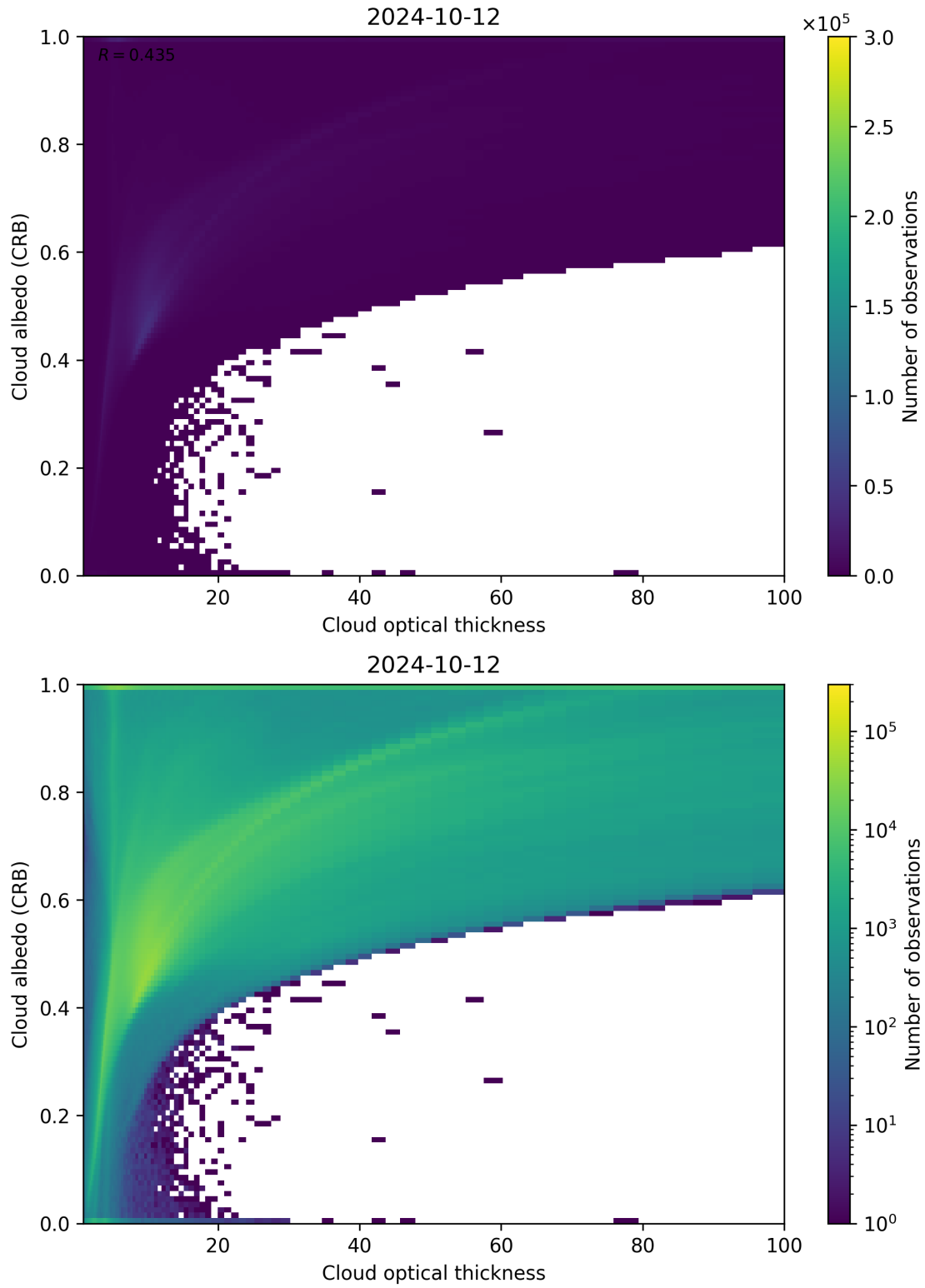
Figure 82: Scatter density plot of “Cloud optical thickness” against “Cloud albedo (CRB)” for 2024-10-11 to 2024-10-13.
