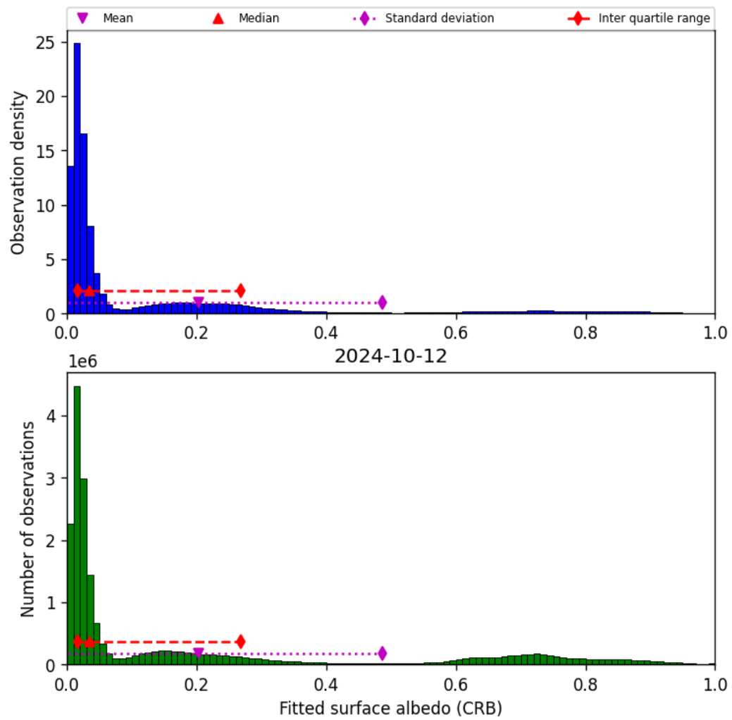
Figure 46: Histogram of “Fitted surface albedo (CRB)” for 2024-10-11 to 2024-10-13
