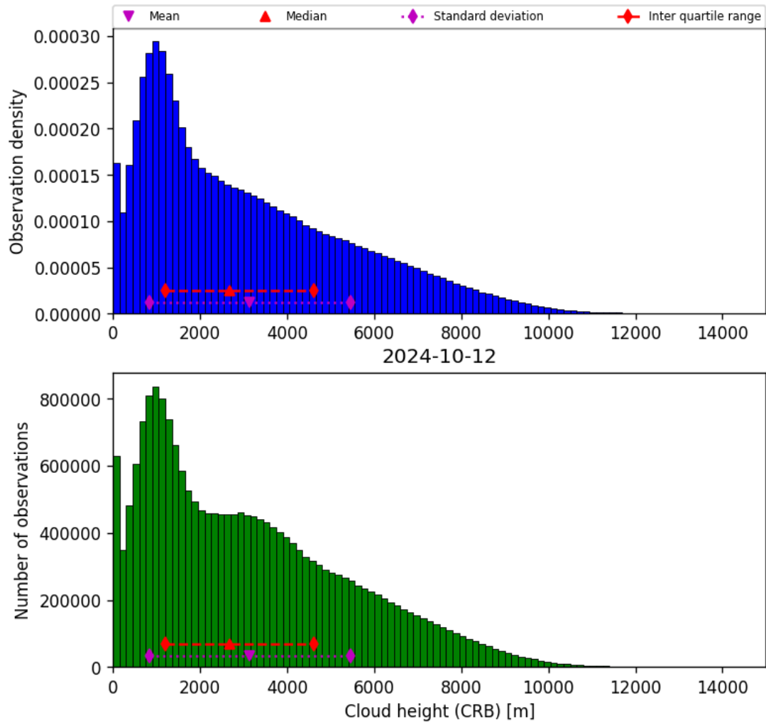
Figure 43: Histogram of “Cloud height (CRB)” for 2024-10-11 to 2024-10-13
