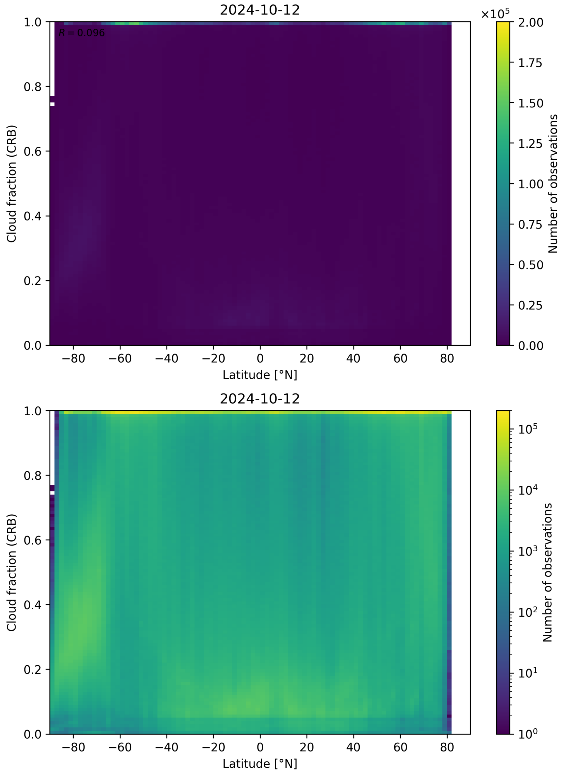
Figure 94: Scatter density plot of “Latitude” against “Cloud fraction (CRB)” for 2024-10-11 to 2024-10-13.
