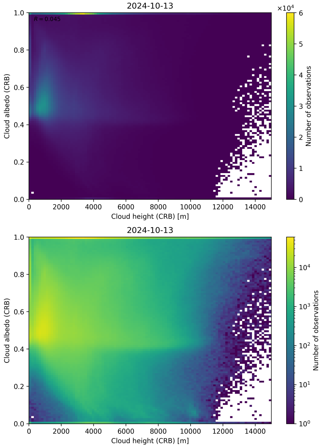
Figure 80: Scatter density plot of “Cloud height (CRB)” against “Cloud albedo (CRB)” for 2024-10-12 to 2024-10-14.
