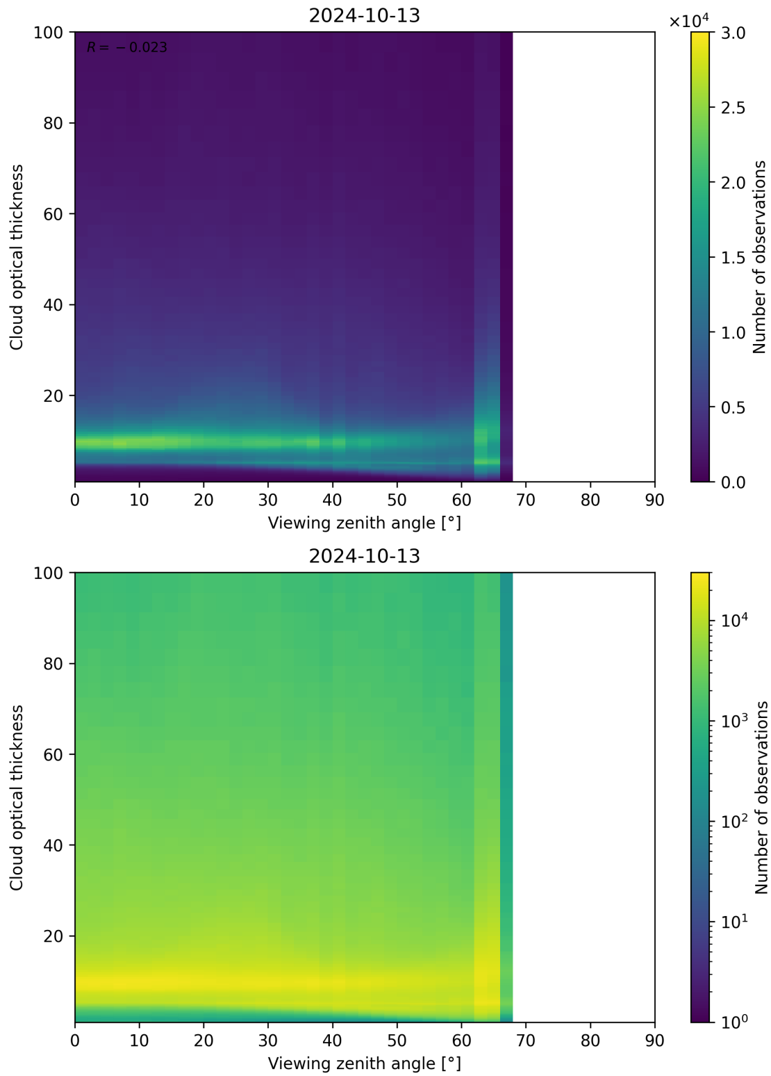
Figure 111: Scatter density plot of “Viewing zenith angle” against “Cloud optical thickness” for 2024-10-12 to 2024-10-14.
