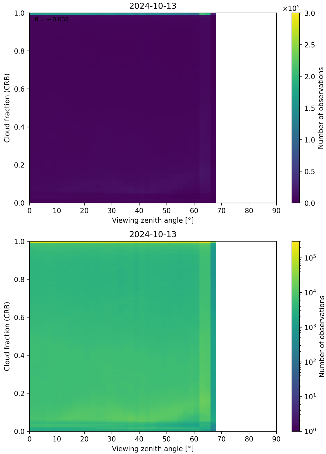
Figure 109: Scatter density plot of “Viewing zenith angle” against “Cloud fraction (CRB)” for 2024-10-12 to 2024-10-14.
