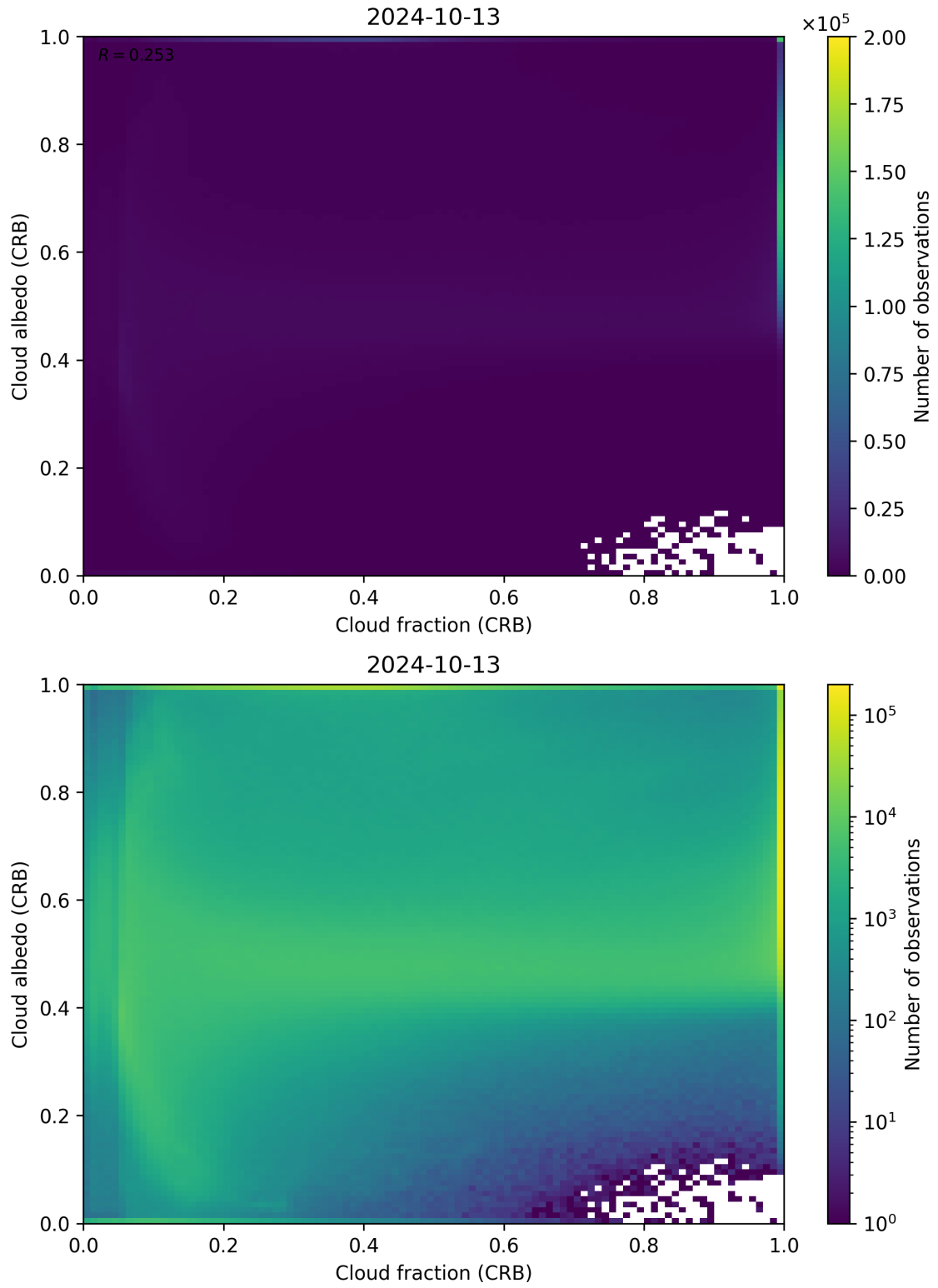
Figure 77: Scatter density plot of “Cloud fraction (CRB)” against “Cloud albedo (CRB)” for 2024-10-12 to 2024-10-14.
