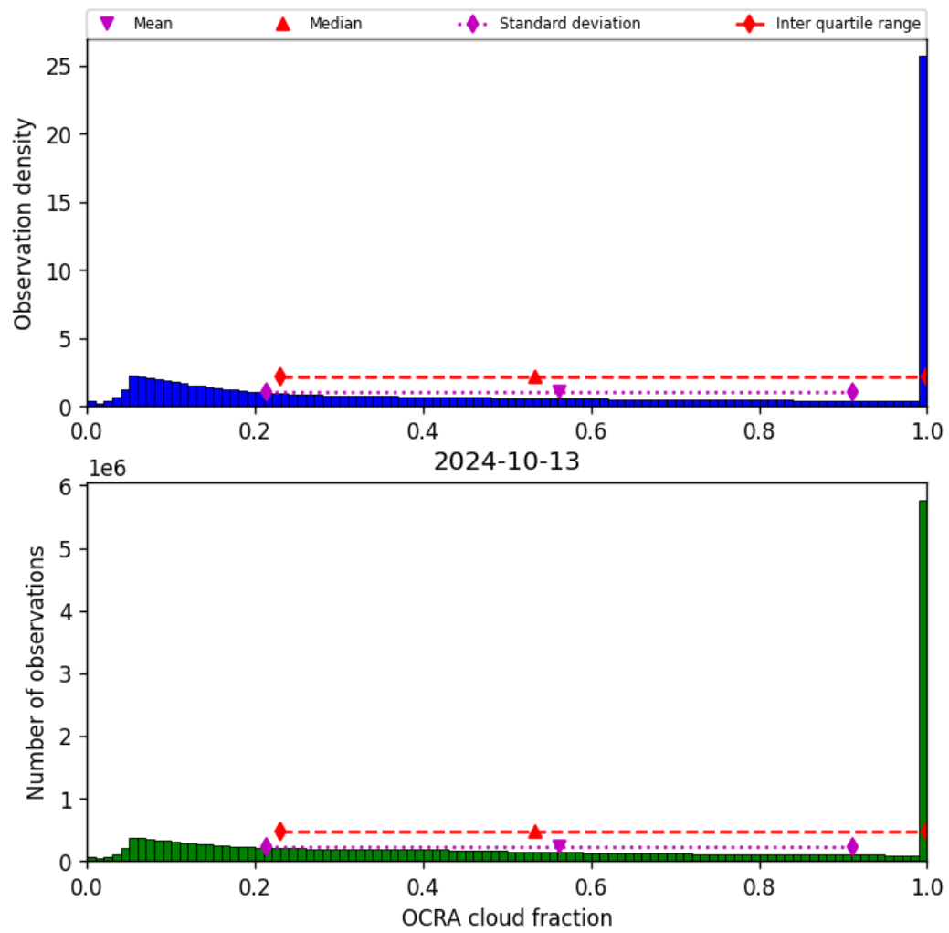
Figure 50: Histogram of “OCRA cloud fraction” for 2024-10-12 to 2024-10-14
