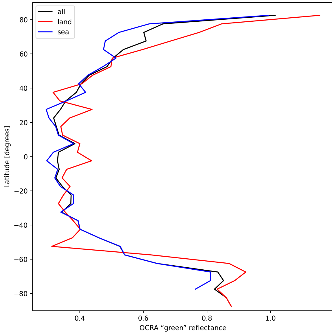
Figure 36: Zonal average of “OCRA “green” reflectance” for 2024-10-12 to 2024-10-14.
