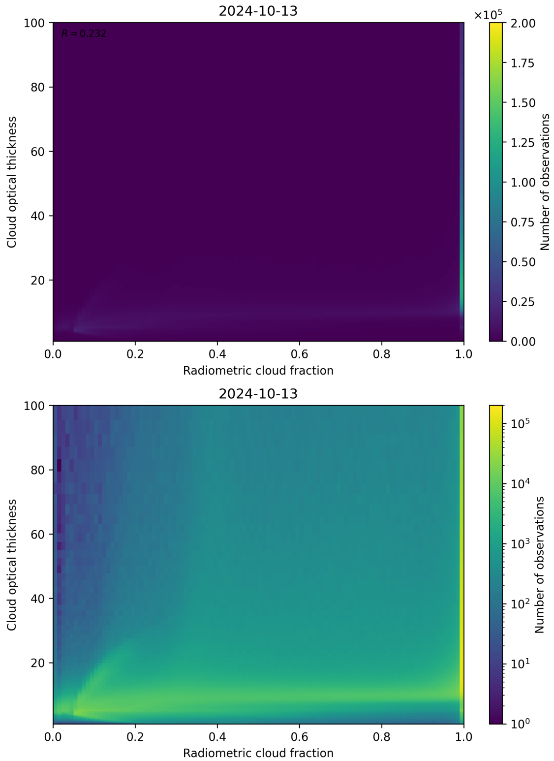
Figure 75: Scatter density plot of “Radiometric cloud fraction” against “Cloud optical thickness” for 2024-10-12 to 2024-10-14.
