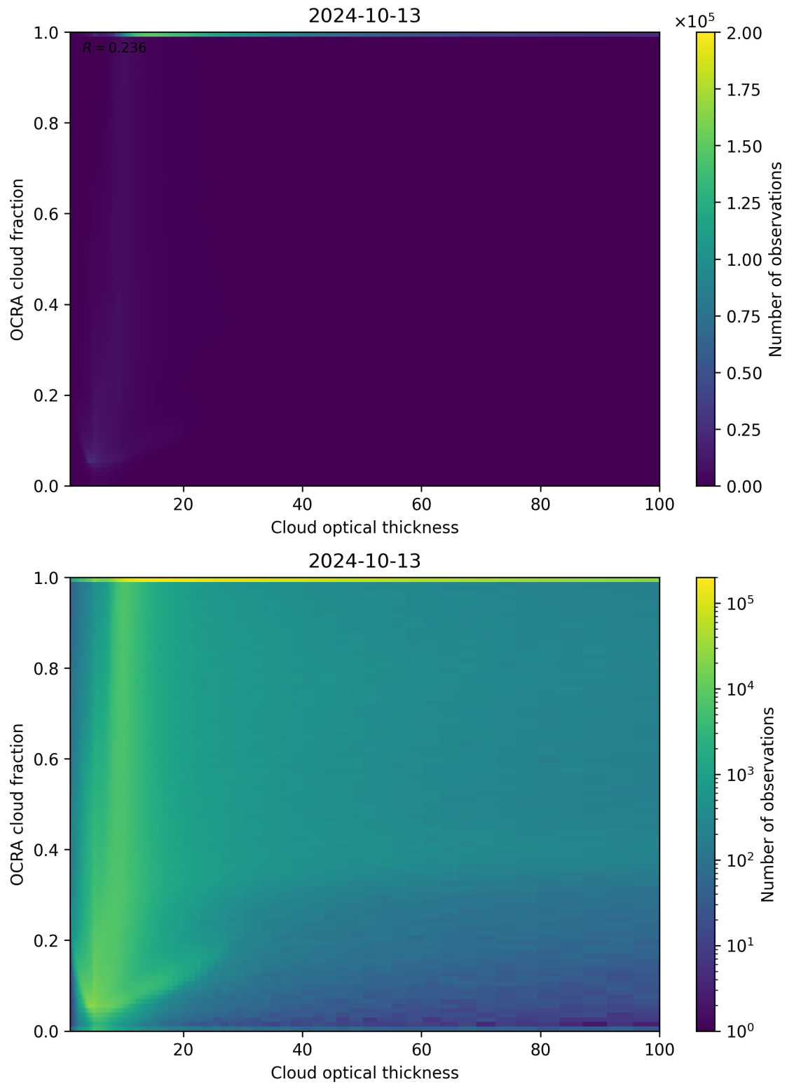
Figure 83: Scatter density plot of “Cloud optical thickness” against “OCRA cloud fraction” for 2024-10-12 to 2024-10-14.
