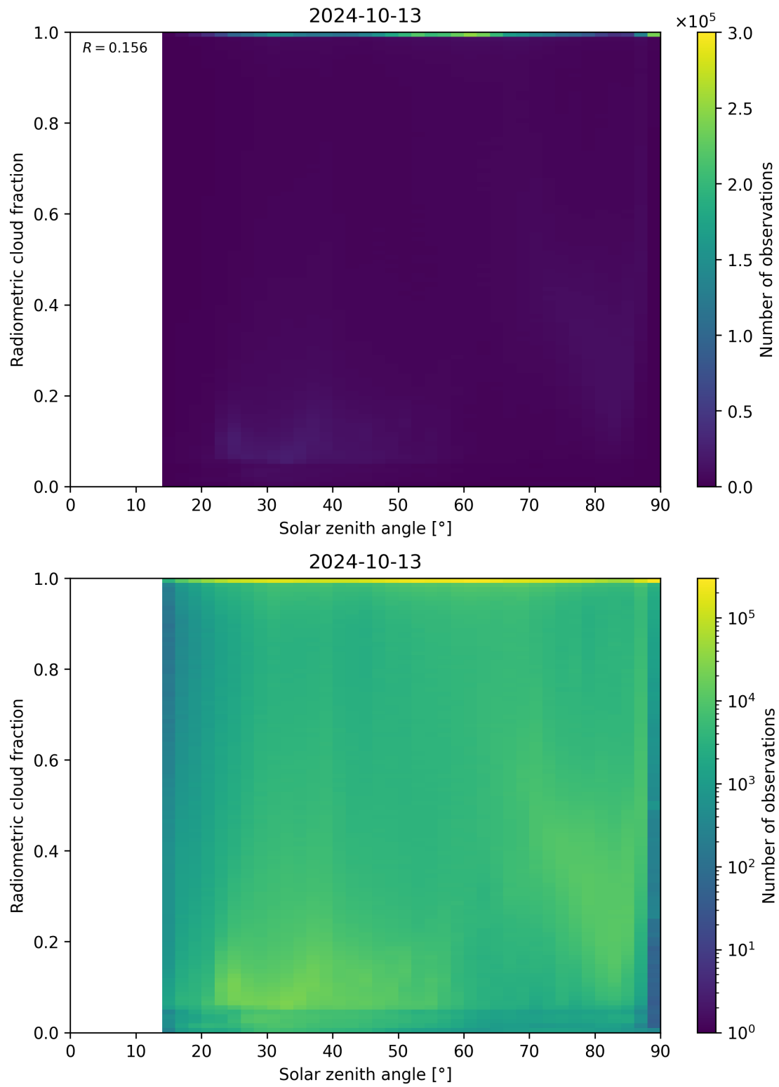
Figure 99: Scatter density plot of “Solar zenith angle” against “Radiometric cloud fraction” for 2024-10-12 to 2024-10-14.
