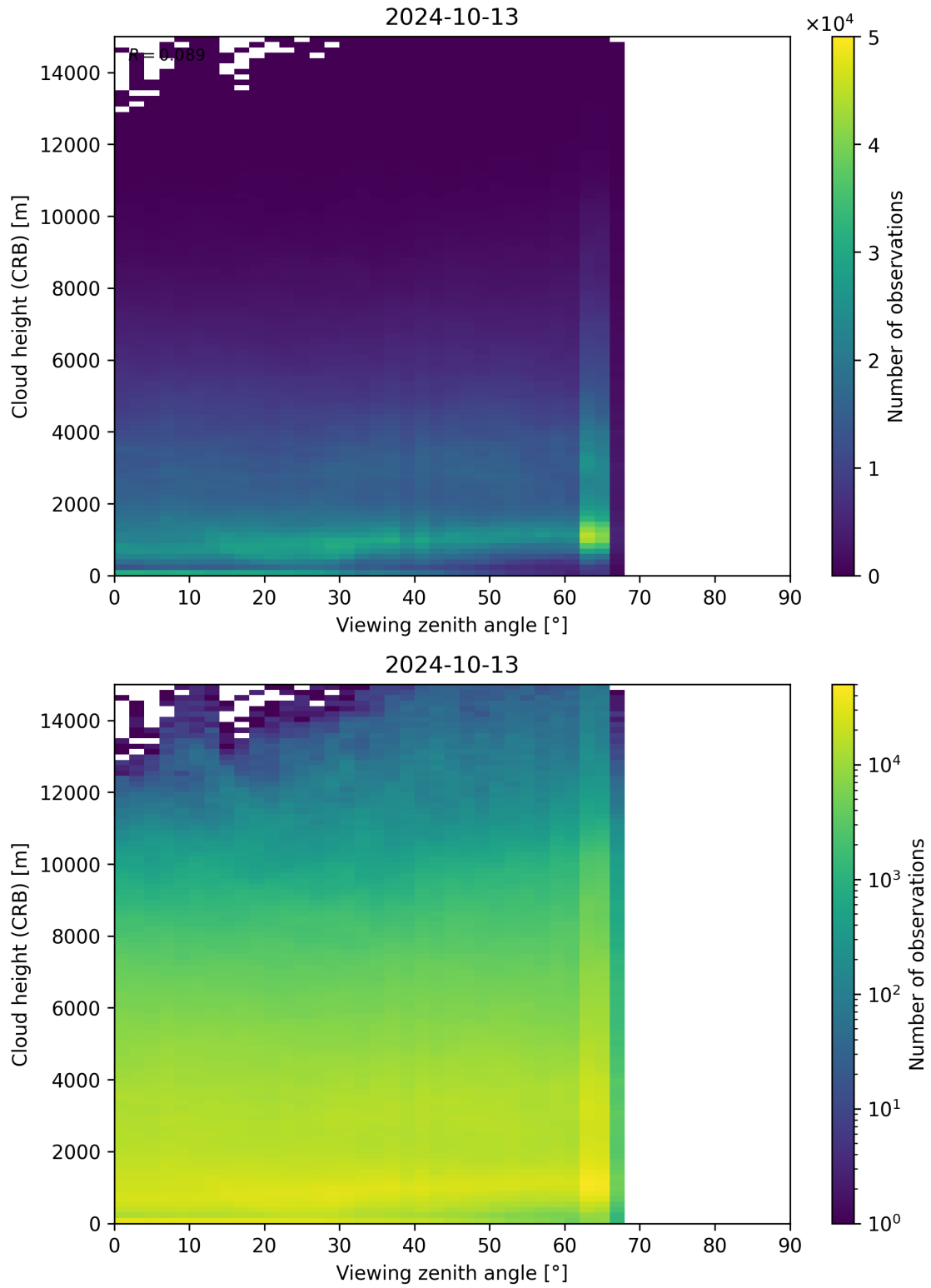
Figure 110: Scatter density plot of “Viewing zenith angle” against “Cloud height (CRB)” for 2024-10-12 to 2024-10-14.
