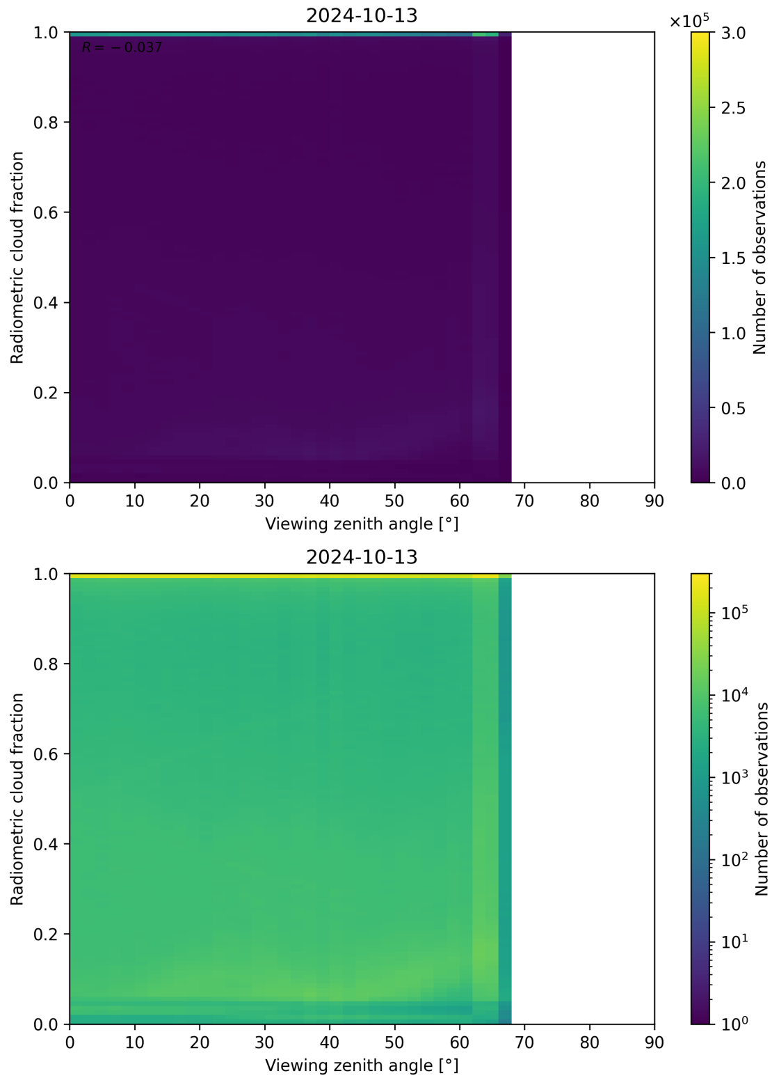
Figure 107: Scatter density plot of “Viewing zenith angle” against “Radiometric cloud fraction” for 2024-10-12 to 2024-10-14.
