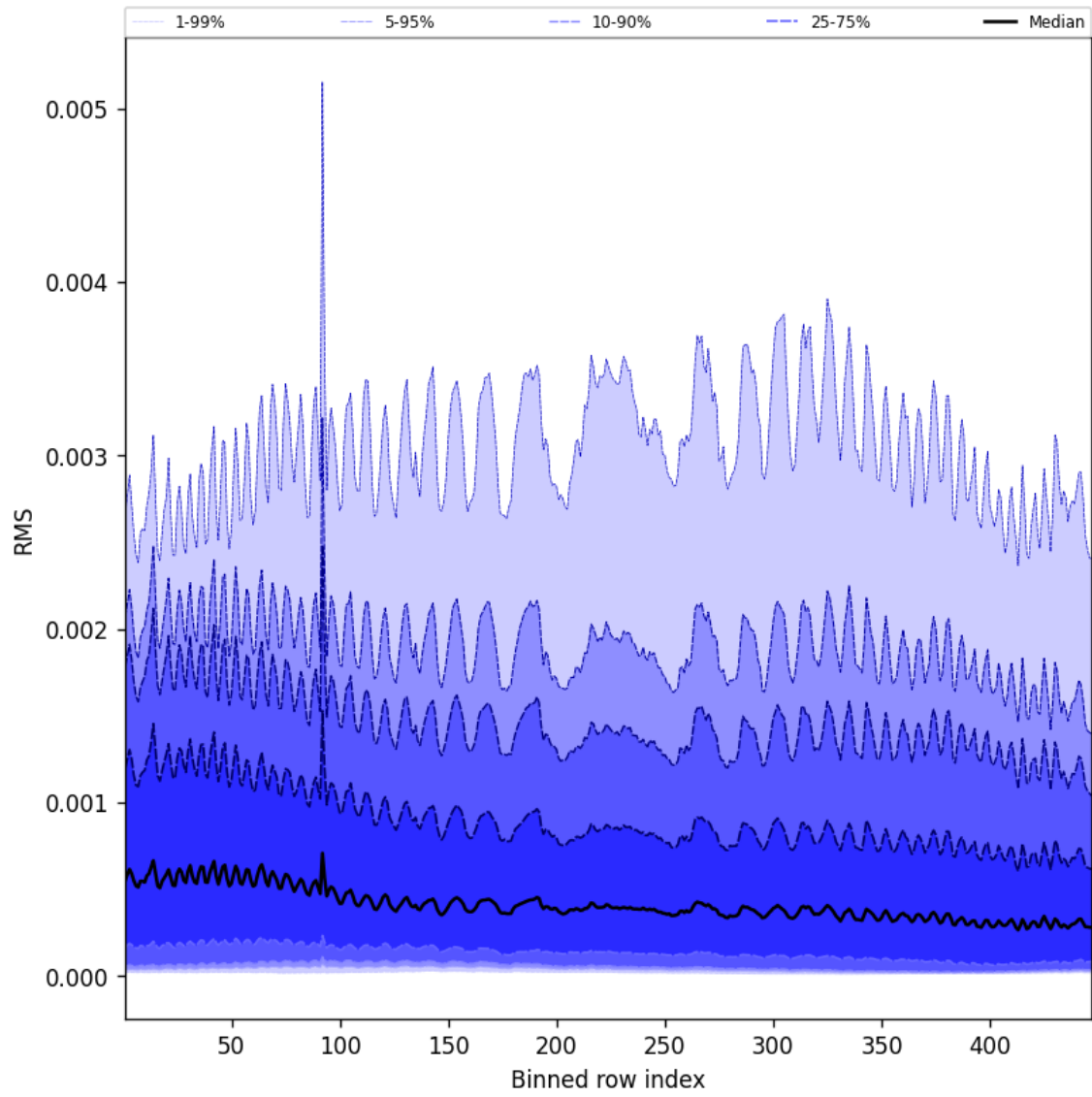
Figure 63: Along track statistics of “RMS” for 2024-10-12 to 2024-10-14
