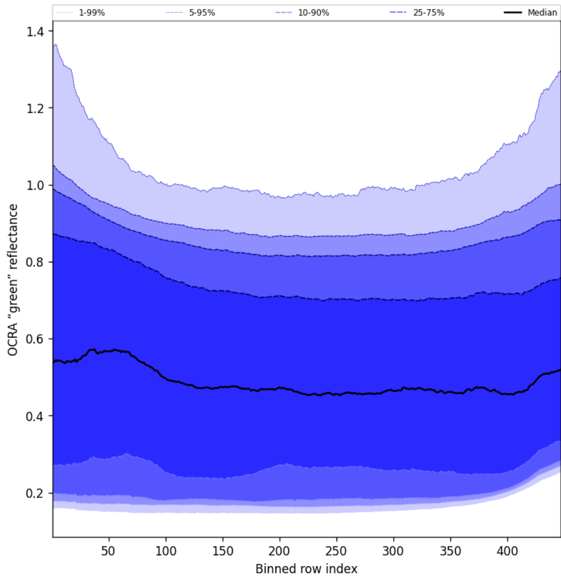
Figure 68: Along track statistics of “OCRA “green” reflectance” for 2024-10-12 to 2024-10-14
