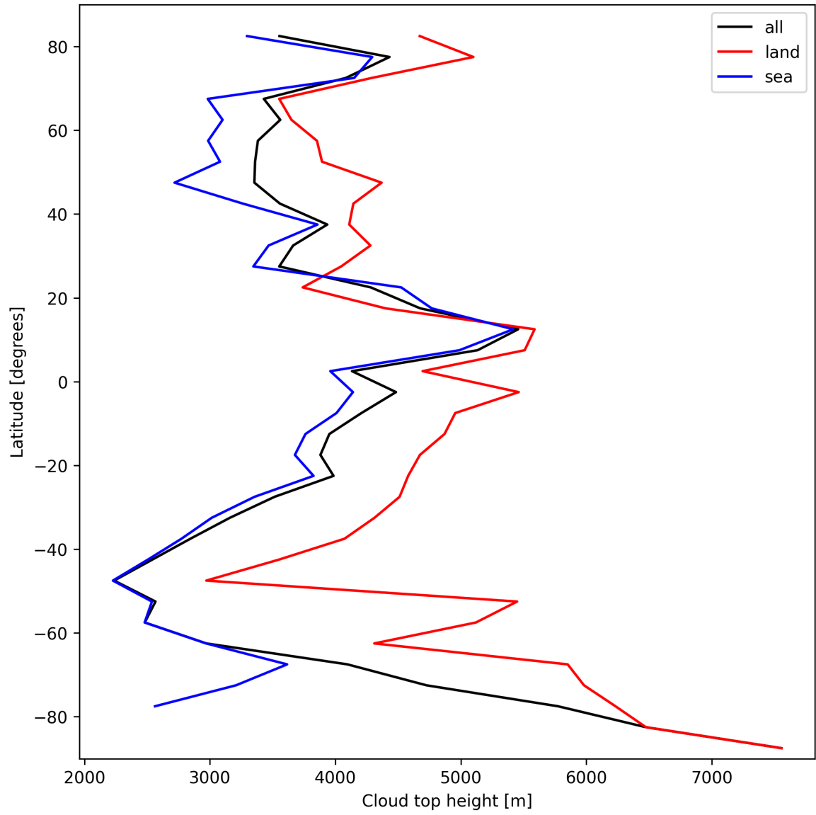
Figure 24: Zonal average of “Cloud top height” for 2024-10-12 to 2024-10-14.
