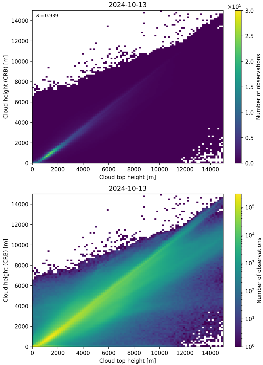
Figure 89: Scatter density plot of “Cloud top height” against “Cloud height (CRB)” for 2024-10-12 to 2024-10-14.
