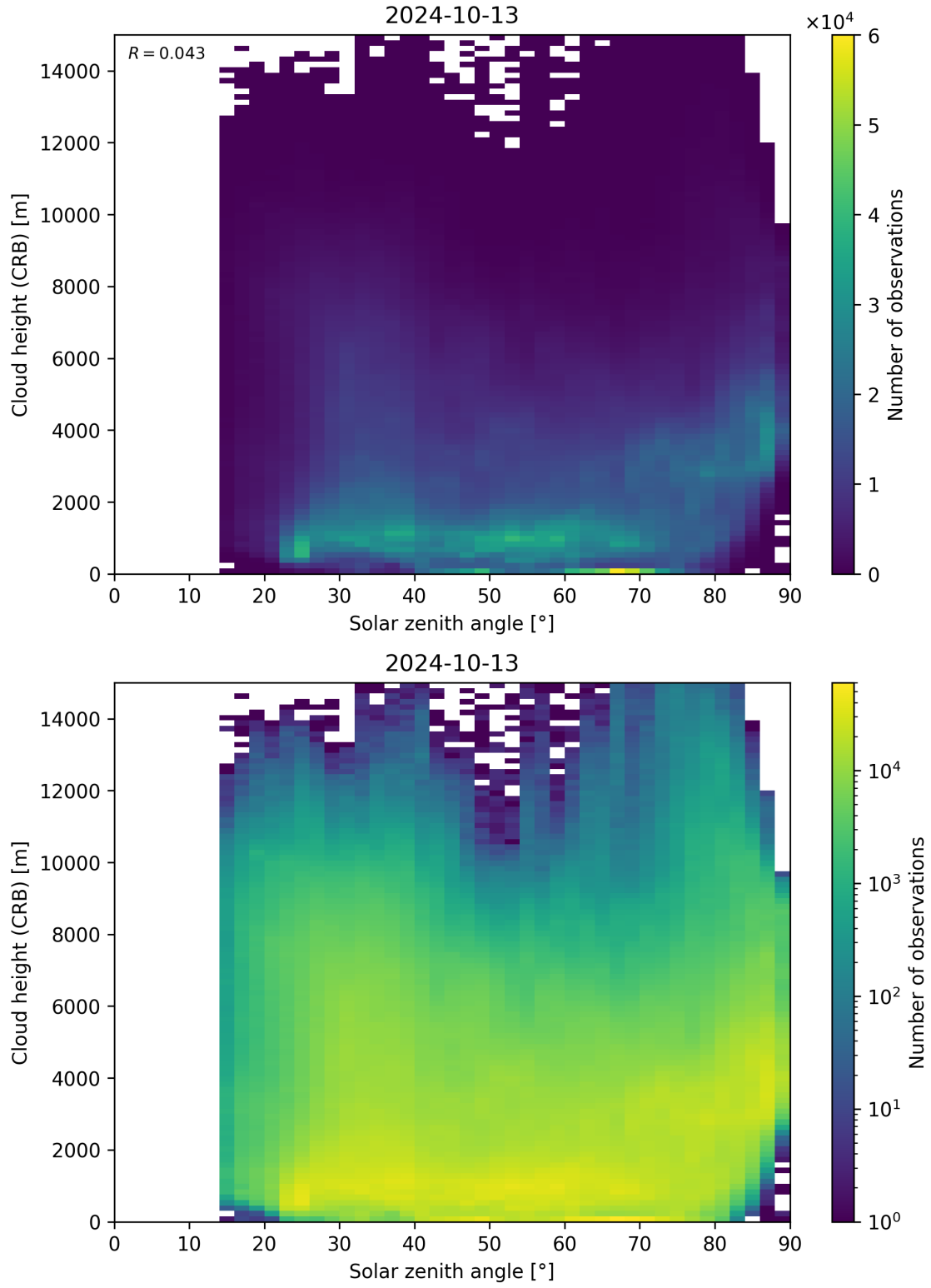
Figure 102: Scatter density plot of “Solar zenith angle” against “Cloud height (CRB)” for 2024-10-12 to 2024-10-14.
