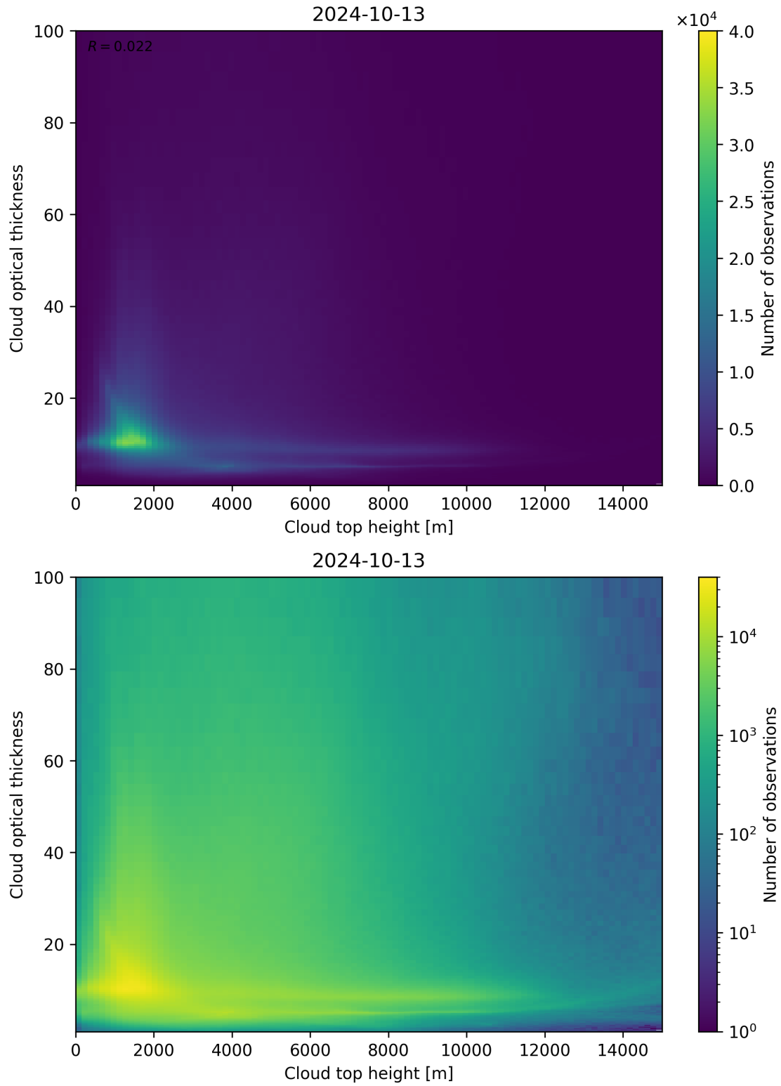
Figure 90: Scatter density plot of “Cloud top height” against “Cloud optical thickness” for 2024-10-12 to 2024-10-14.
