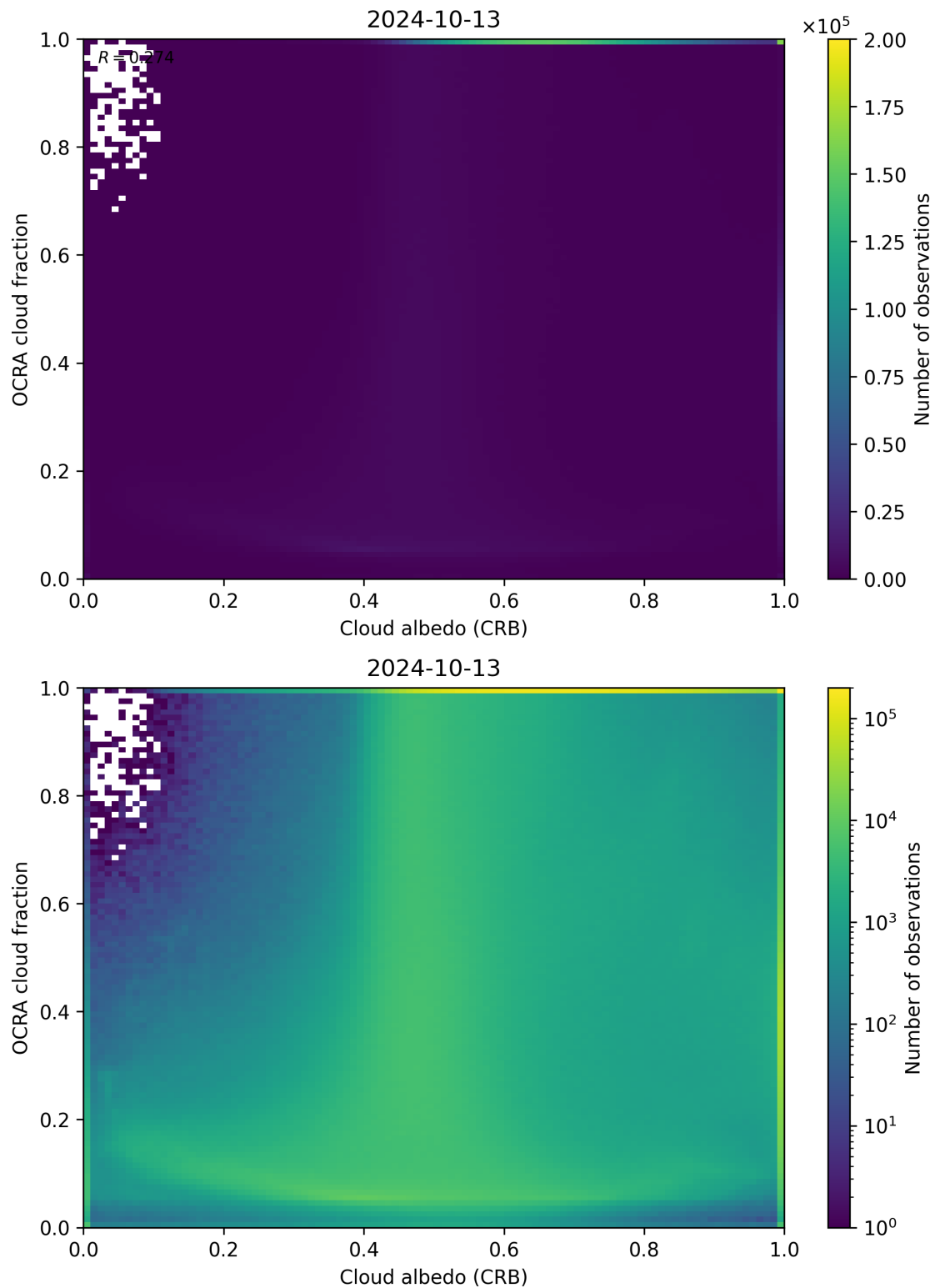
Figure 70: Scatter density plot of “Cloud albedo (CRB)” against “OCRA cloud fraction” for 2024-10-12 to 2024-10-14.
