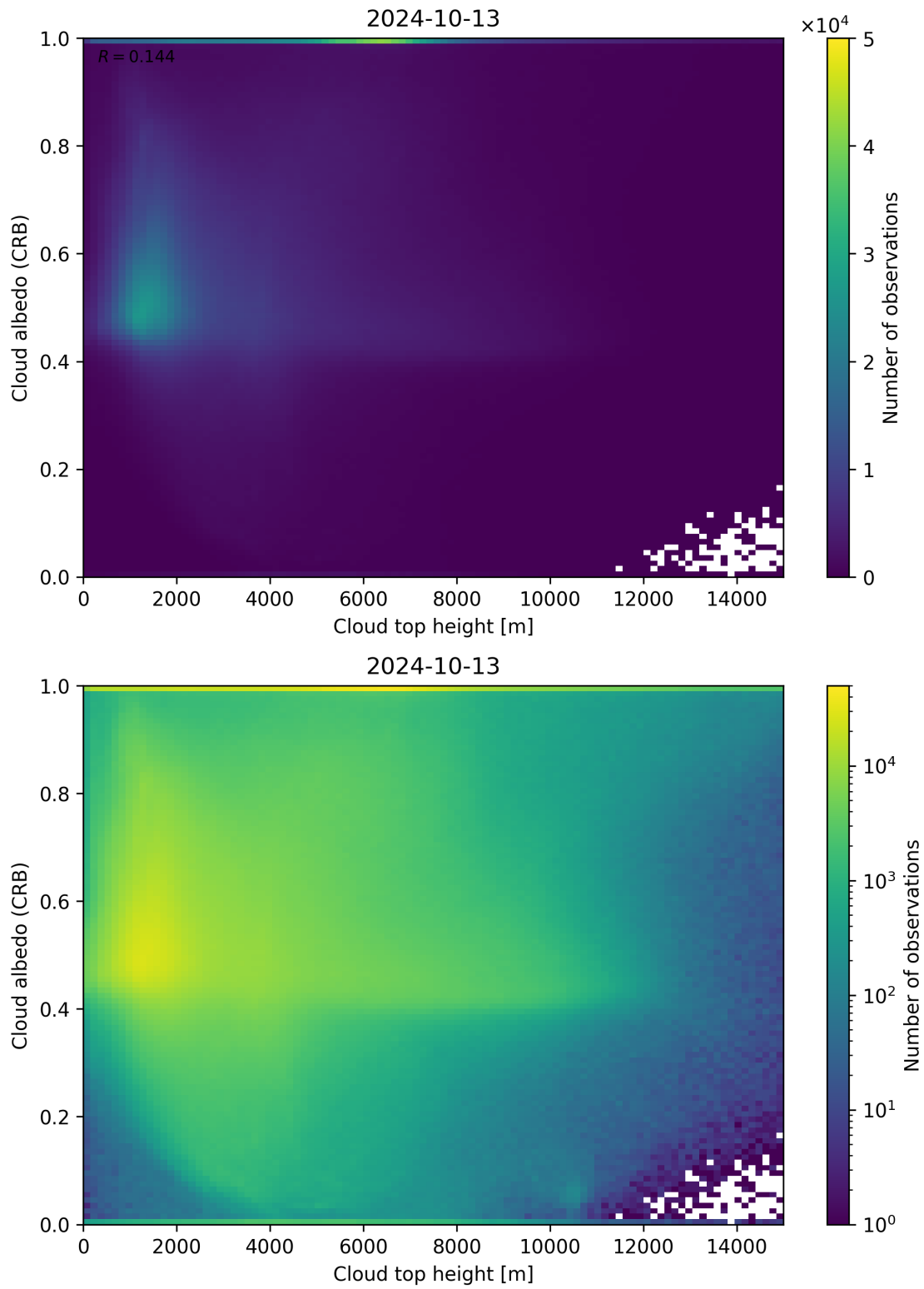
Figure 86: Scatter density plot of “Cloud top height” against “Cloud albedo (CRB)” for 2024-10-12 to 2024-10-14.
