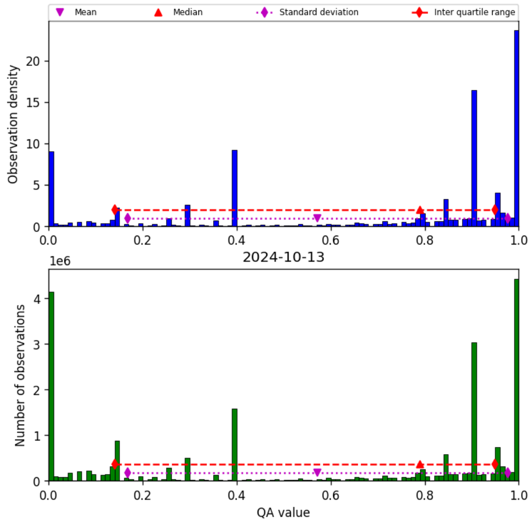
Figure 38: Histogram of “QA value” for 2024-10-12 to 2024-10-14
