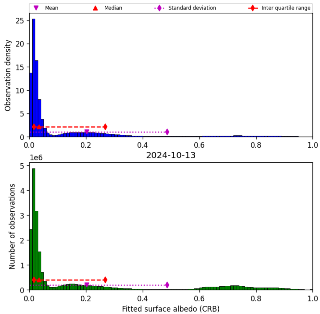
Figure 46: Histogram of “Fitted surface albedo (CRB)” for 2024-10-12 to 2024-10-14
