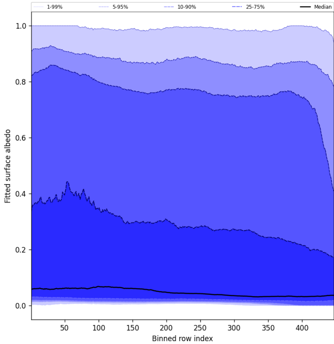
Figure 61: Along track statistics of “Fitted surface albedo” for 2024-10-12 to 2024-10-14
