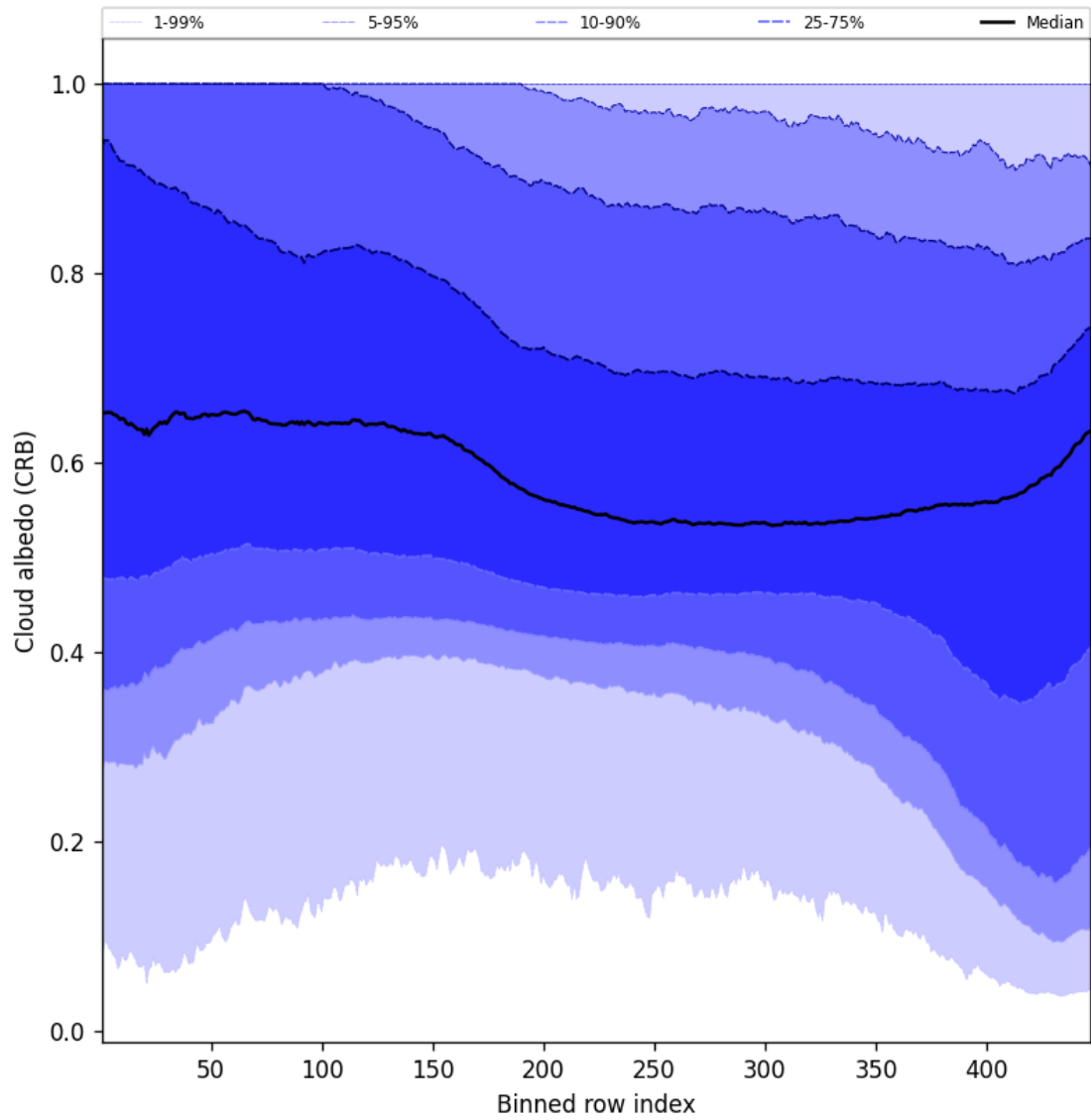
Figure 60: Along track statistics of “Cloud albedo (CRB)” for 2024-10-12 to 2024-10-14
