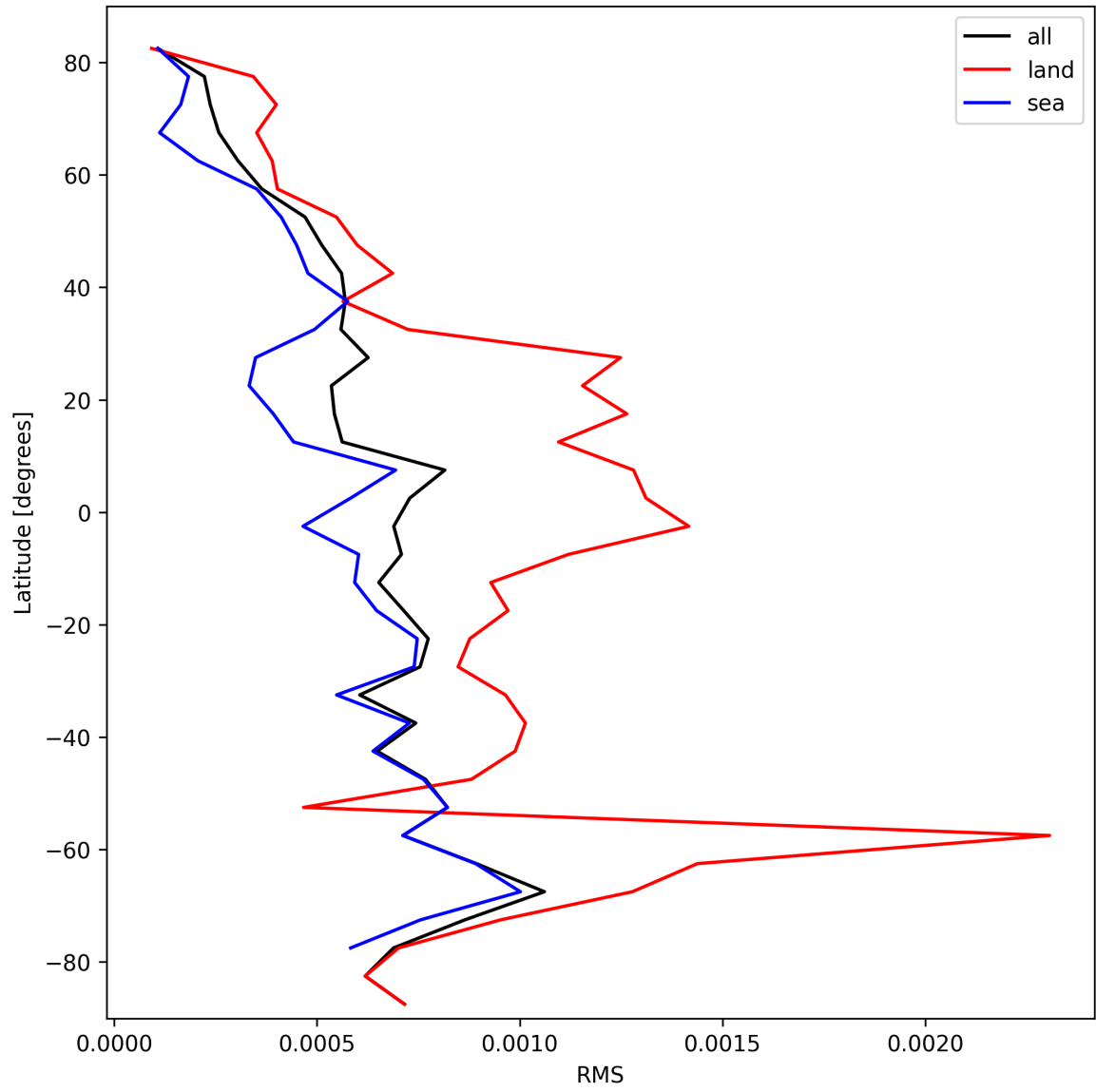
Figure 31: Zonal average of “RMS” for 2024-10-12 to 2024-10-14.
