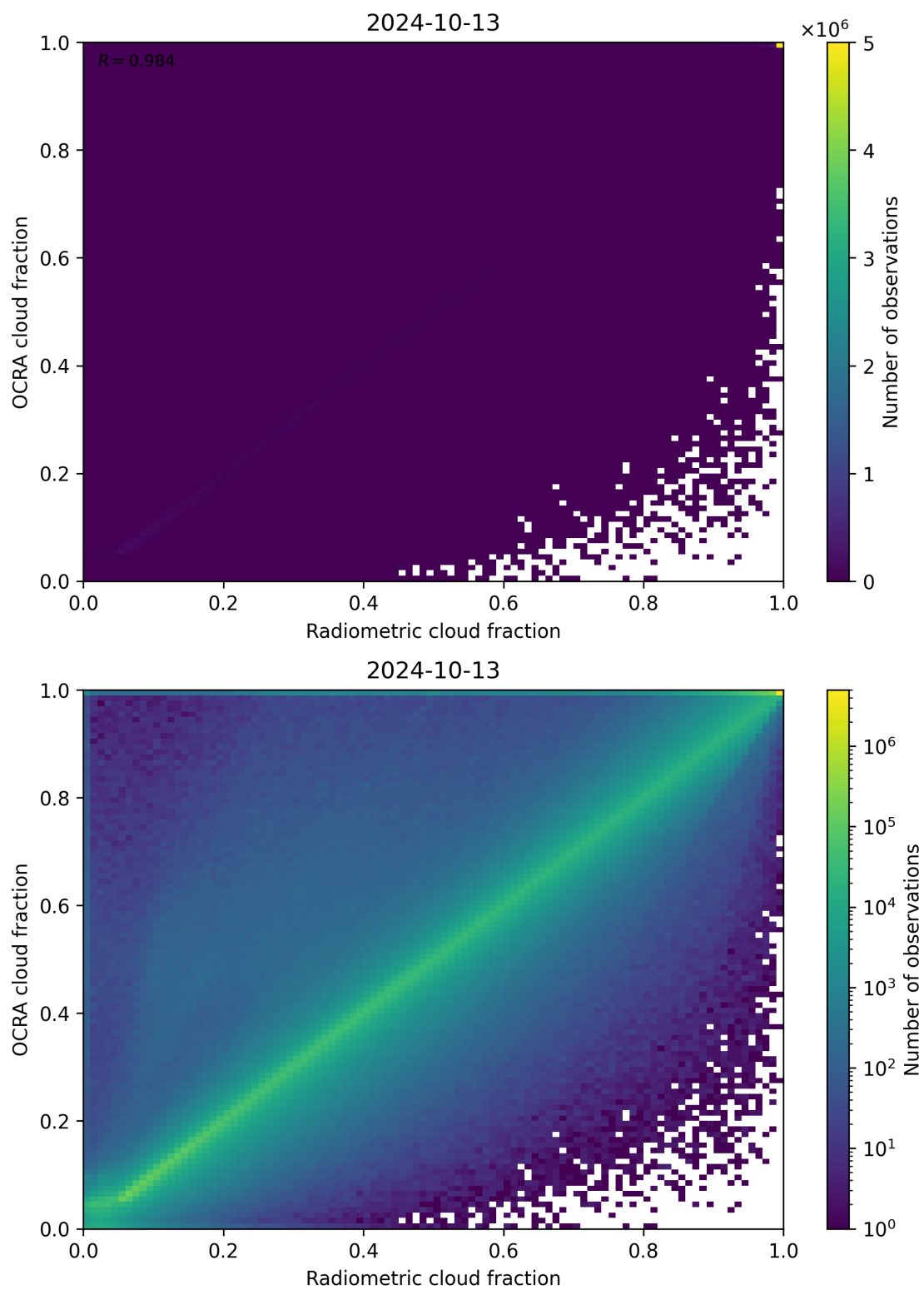
Figure 72: Scatter density plot of “Radiometric cloud fraction” against “OCRA cloud fraction” for 2024-10-12 to 2024-10-14.
