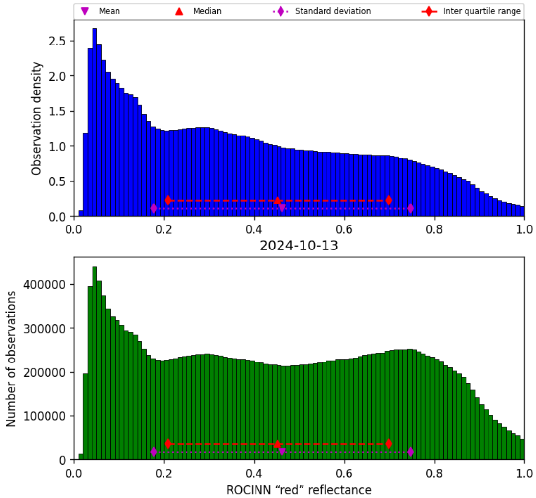
Figure 53: Histogram of “ROCINN “red” reflectance” for 2024-10-12 to 2024-10-14
