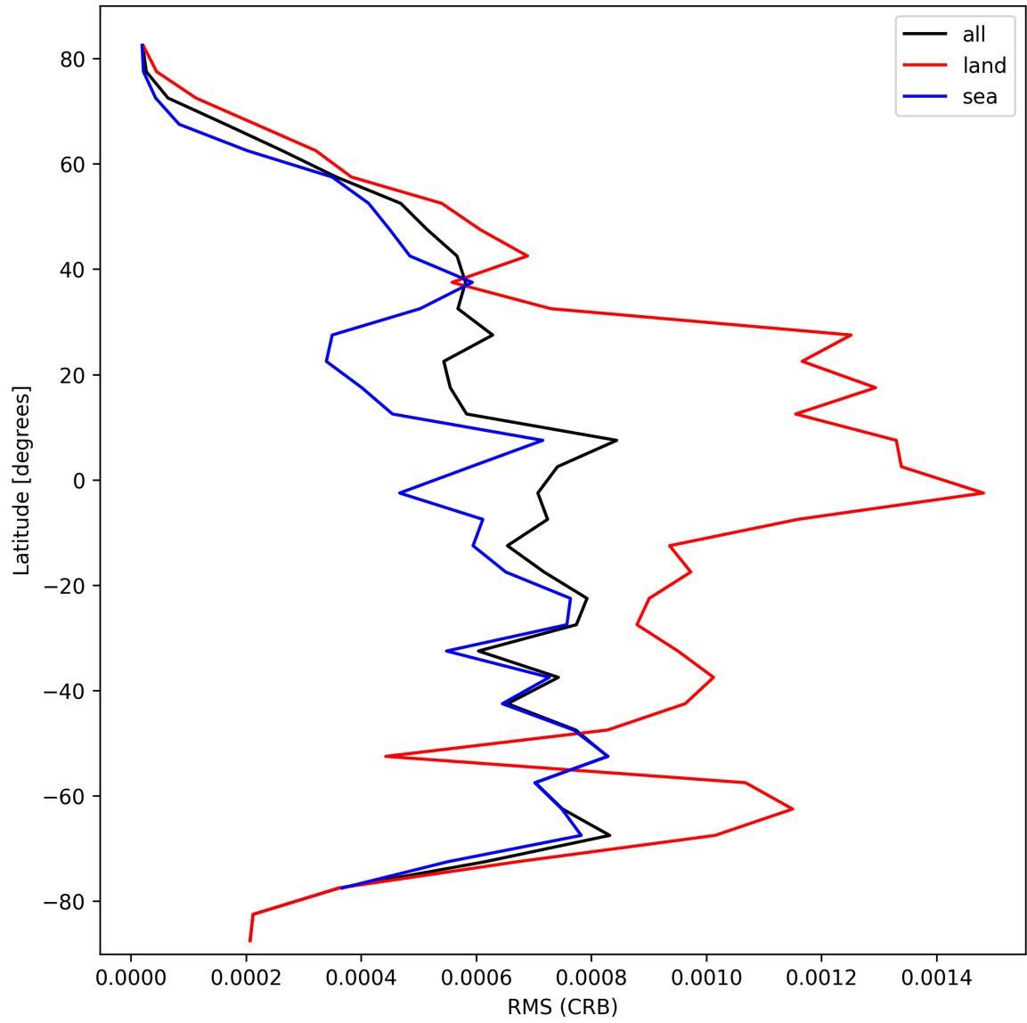
Figure 32: Zonal average of “RMS (CRB)” for 2024-10-12 to 2024-10-14.
