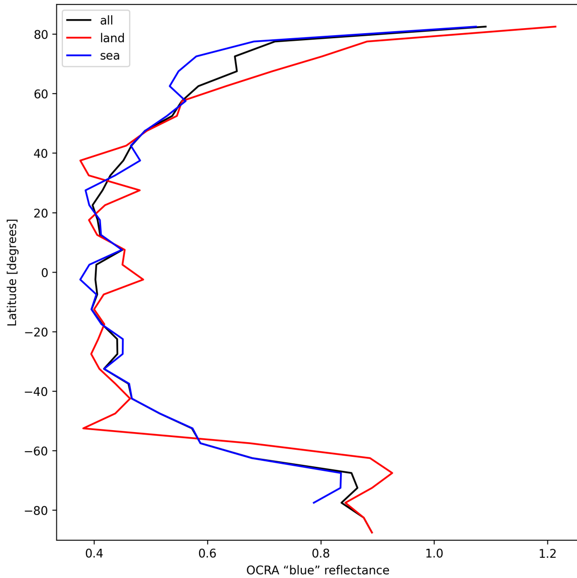
Figure 35: Zonal average of “OCRA “blue” reflectance” for 2024-10-12 to 2024-10-14.
