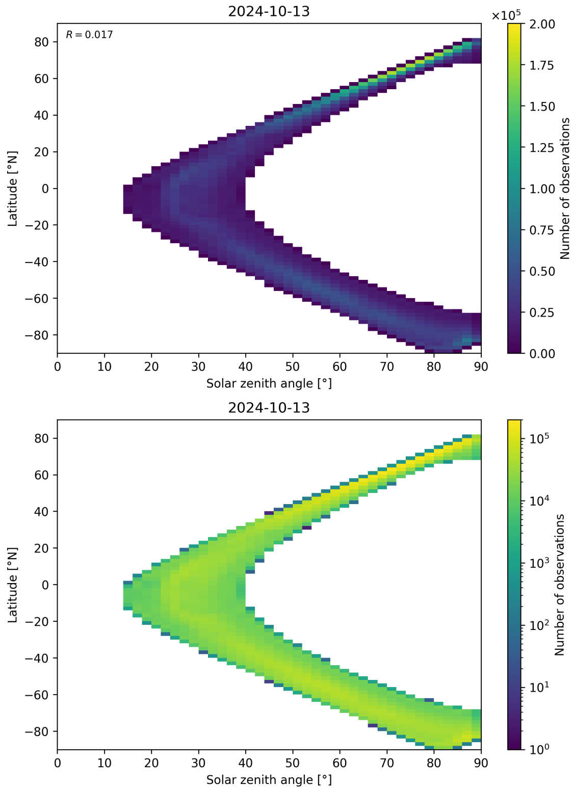
Figure 105: Scatter density plot of “Solar zenith angle” against “Latitude” for 2024-10-12 to 2024-10-14.
