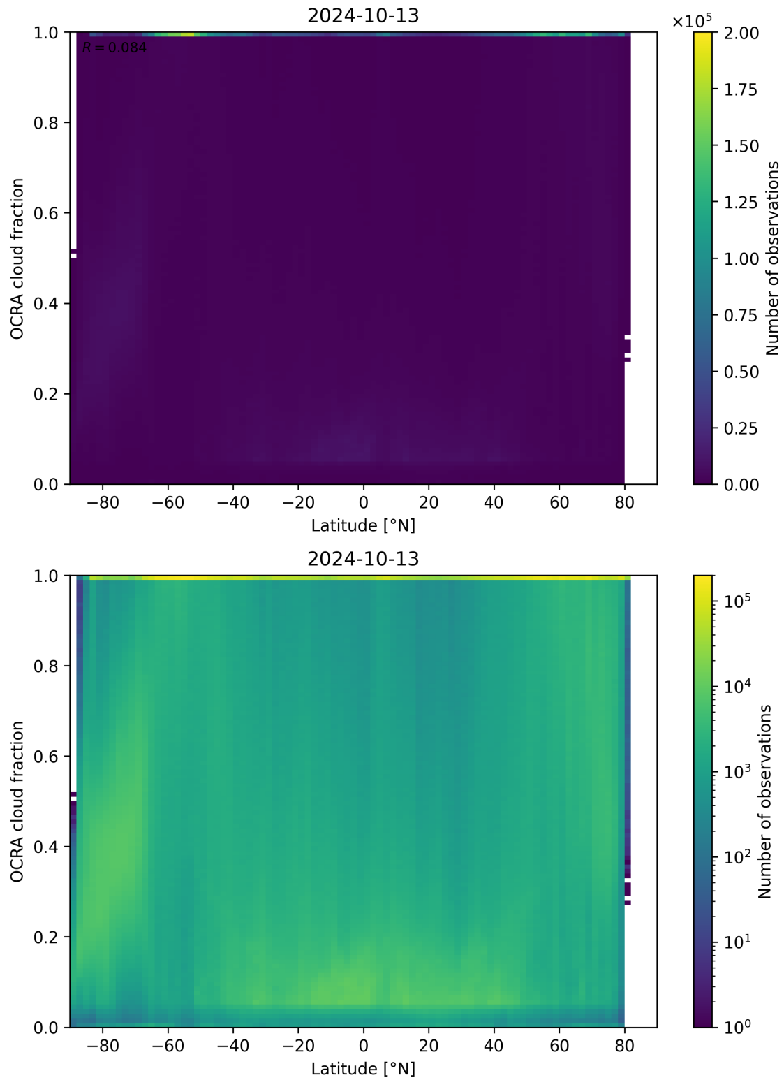
Figure 93: Scatter density plot of “Latitude” against “OCRA cloud fraction” for 2024-10-12 to 2024-10-14.
