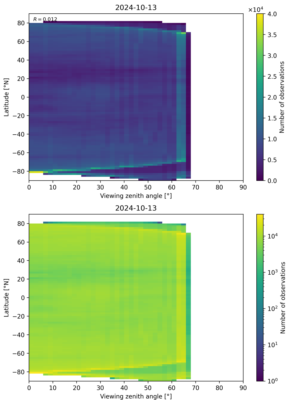
Figure 113: Scatter density plot of “Viewing zenith angle” against “Latitude” for 2024-10-12 to 2024-10-14.
