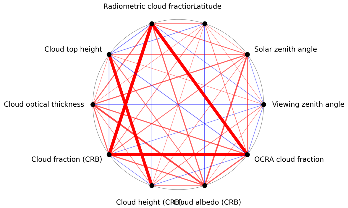
Figure 1: Map of correlation graph for 2024-10-12 to 2024-10-14.
