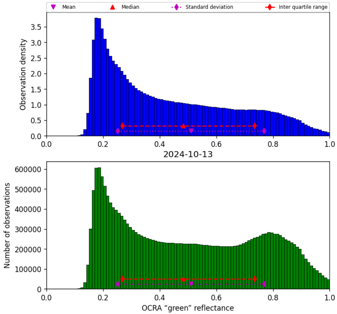
Figure 52: Histogram of “OCRA “green” reflectance” for 2024-10-12 to 2024-10-14
