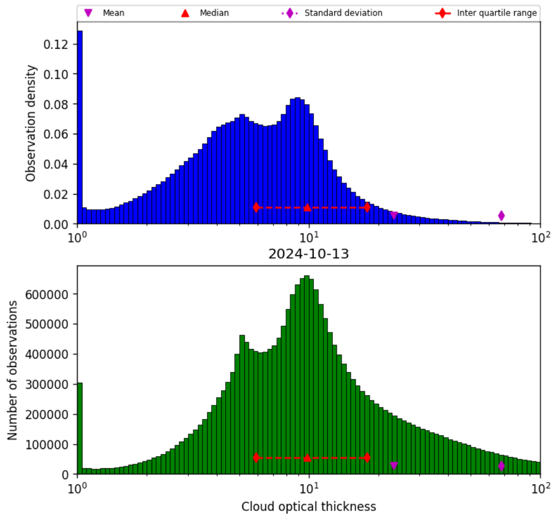
Figure 41: Histogram of “Cloud optical thickness” for 2024-10-12 to 2024-10-14
