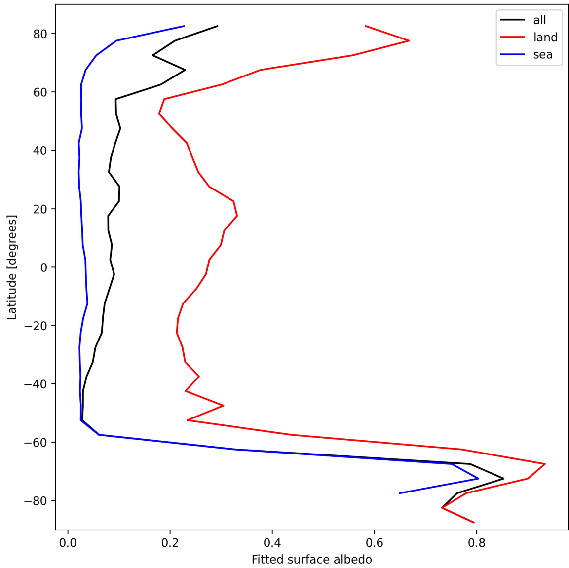
Figure 29: Zonal average of “Fitted surface albedo” for 2024-10-12 to 2024-10-14.
