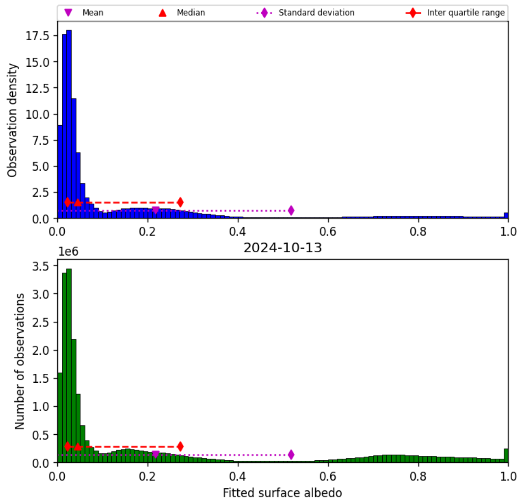
Figure 45: Histogram of “Fitted surface albedo” for 2024-10-12 to 2024-10-14
