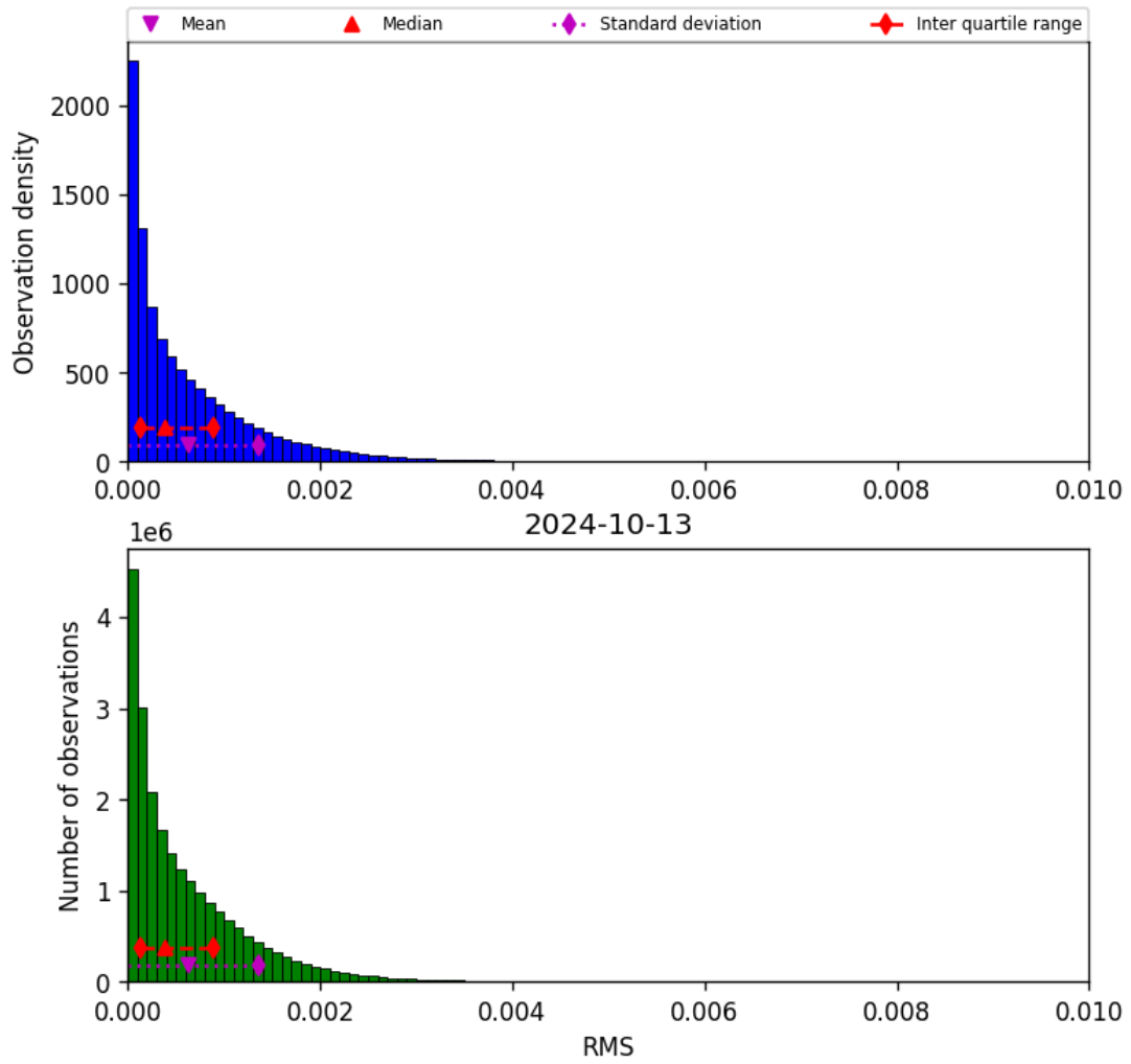
Figure 47: Histogram of “RMS” for 2024-10-12 to 2024-10-14
