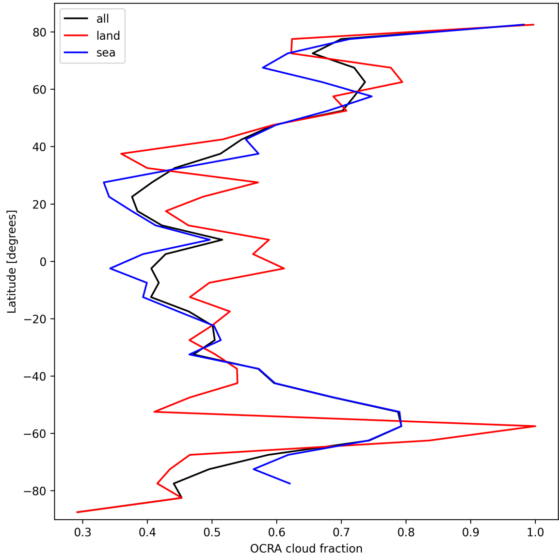
Figure 34: Zonal average of “OCRA cloud fraction” for 2024-10-12 to 2024-10-14.
