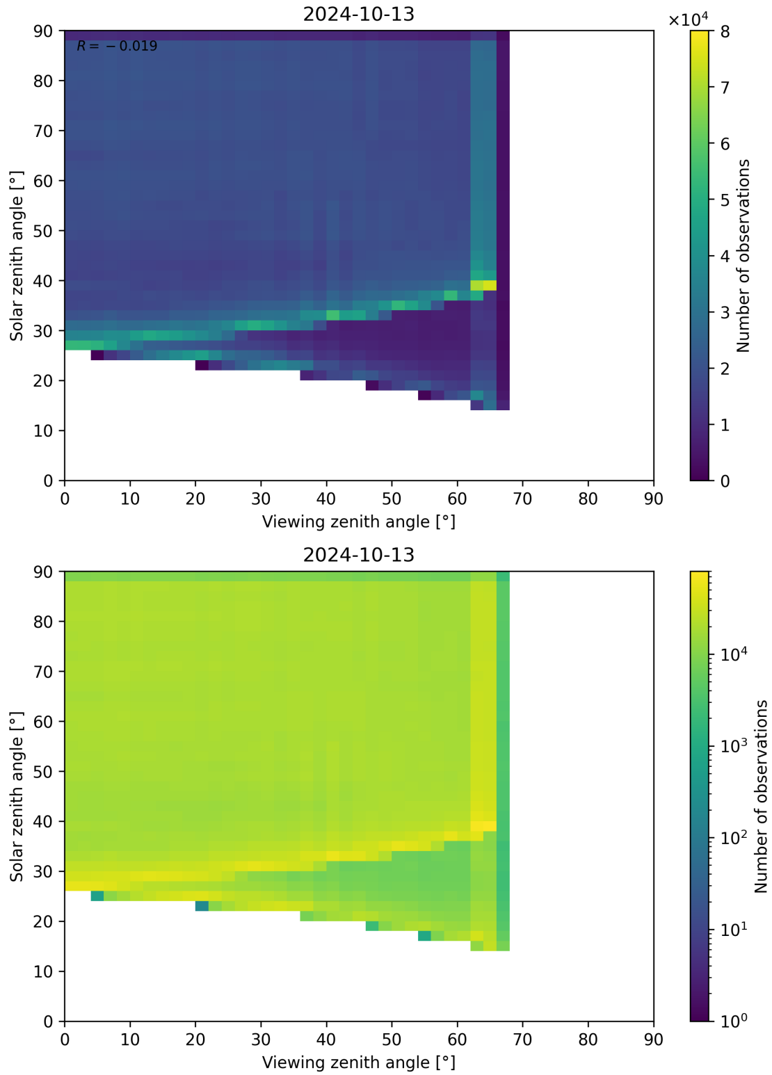
Figure 114: Scatter density plot of “Viewing zenith angle” against “Solar zenith angle” for 2024-10-12 to 2024-10-14.
