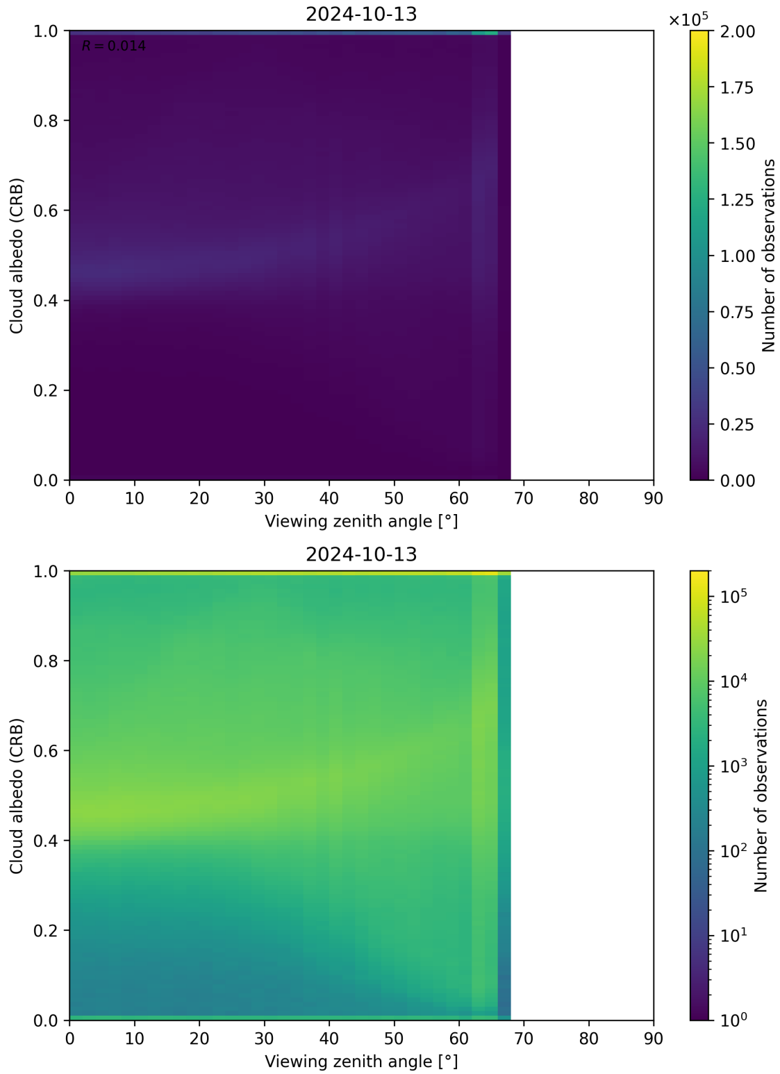
Figure 106: Scatter density plot of “Viewing zenith angle” against “Cloud albedo (CRB)” for 2024-10-12 to 2024-10-14.
