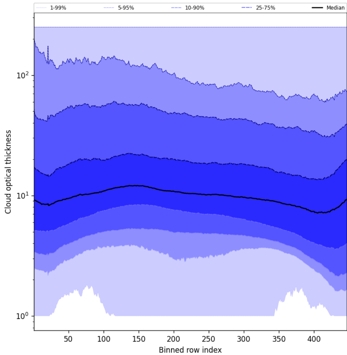
Figure 57: Along track statistics of “Cloud optical thickness” for 2024-10-12 to 2024-10-14
