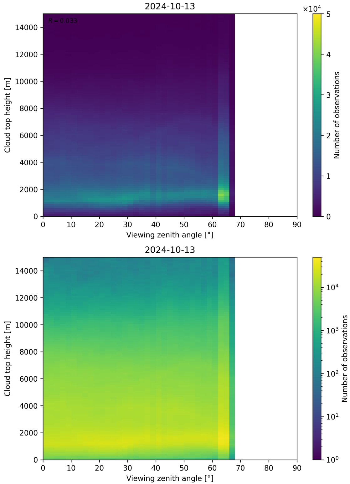
Figure 112: Scatter density plot of “Viewing zenith angle” against “Cloud top height” for 2024-10-12 to 2024-10-14.
