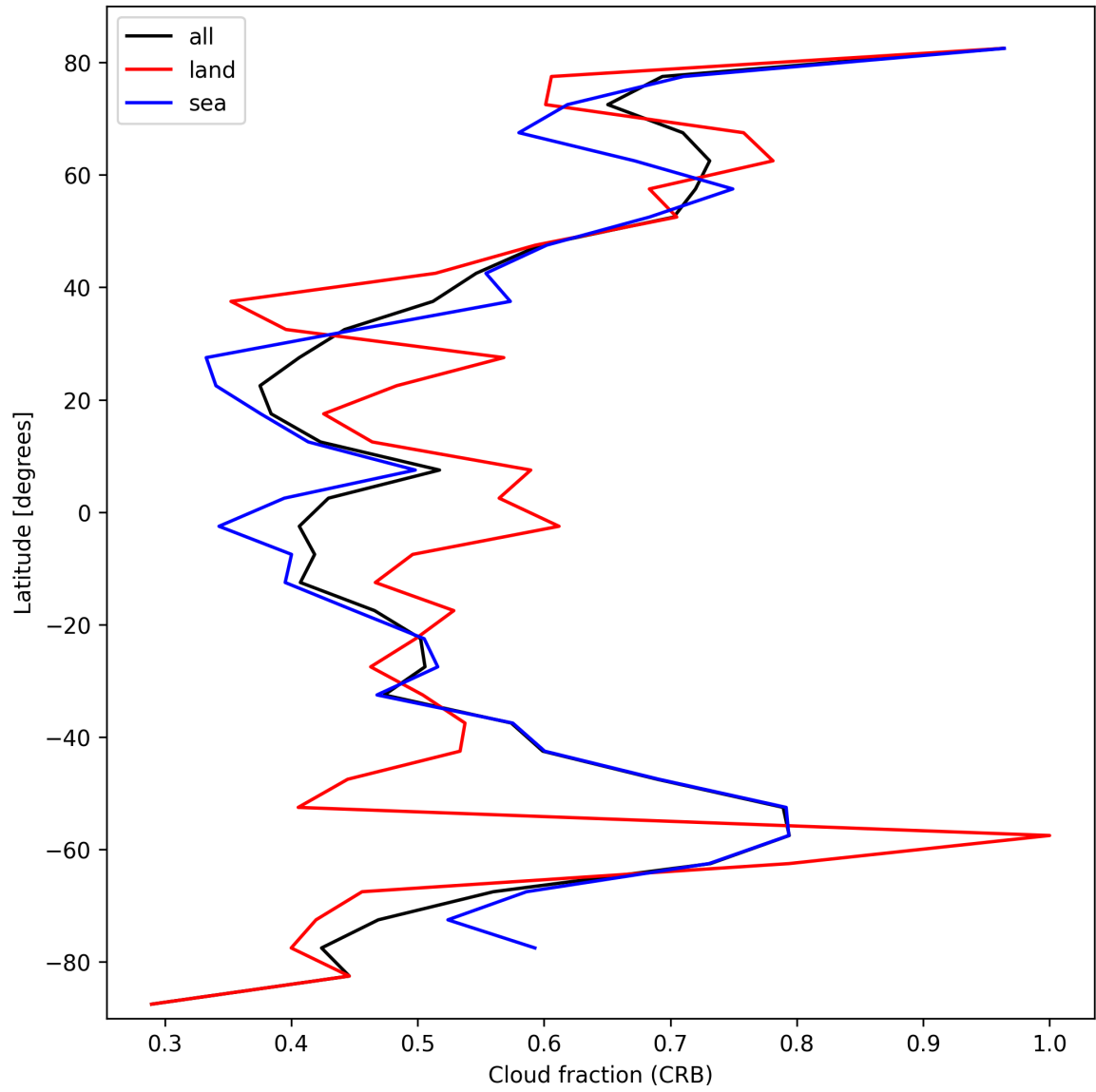
Figure 26: Zonal average of “Cloud fraction (CRB)” for 2024-10-12 to 2024-10-14.
