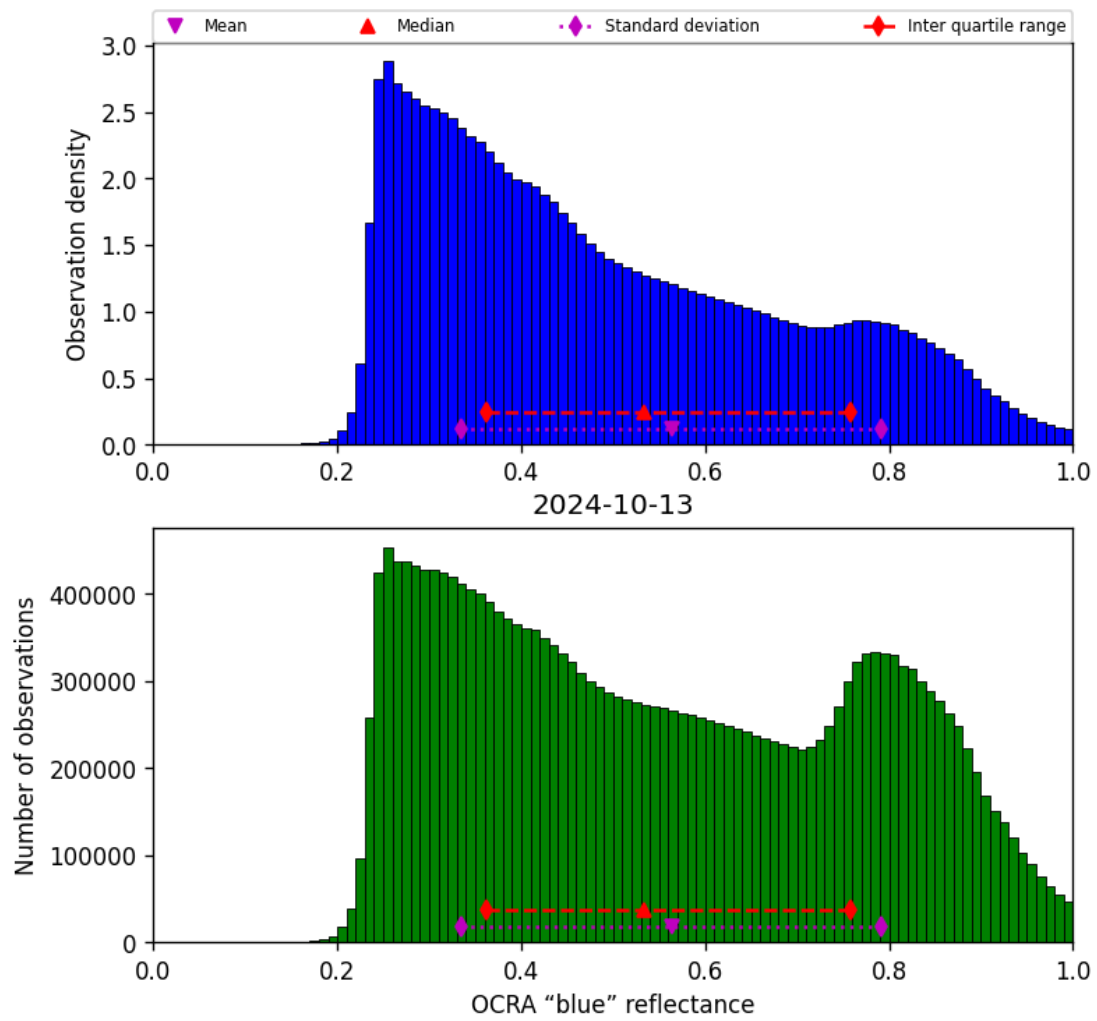
Figure 51: Histogram of “OCRA “blue” reflectance” for 2024-10-12 to 2024-10-14
