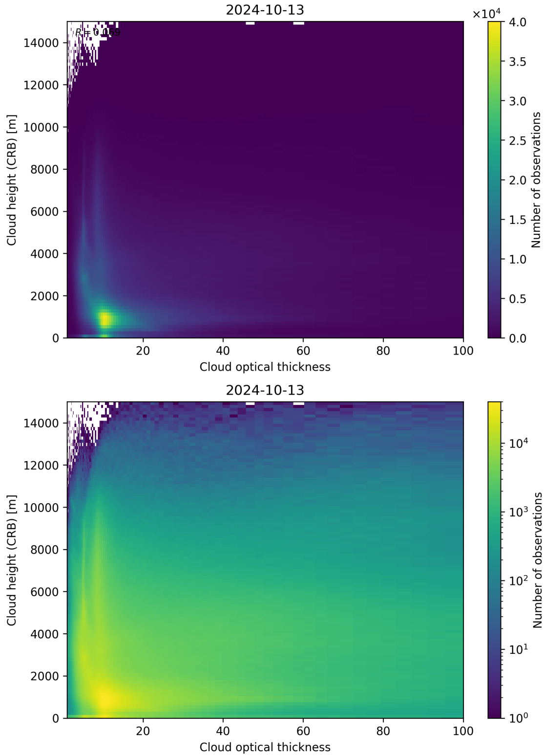
Figure 85: Scatter density plot of “Cloud optical thickness” against “Cloud height (CRB)” for 2024-10-12 to 2024-10-14.
