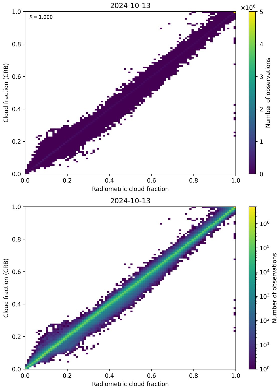
Figure 73: Scatter density plot of “Radiometric cloud fraction” against “Cloud fraction (CRB)” for 2024-10-12 to 2024-10-14.
