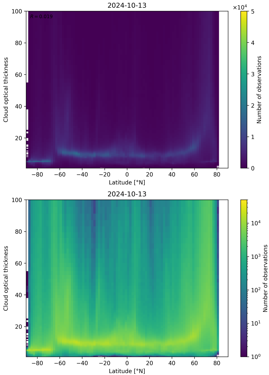
Figure 96: Scatter density plot of “Latitude” against “Cloud optical thickness” for 2024-10-12 to 2024-10-14.
