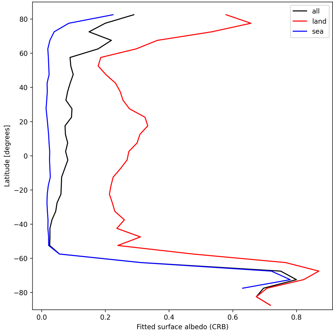
Figure 30: Zonal average of “Fitted surface albedo (CRB)” for 2024-10-12 to 2024-10-14.
