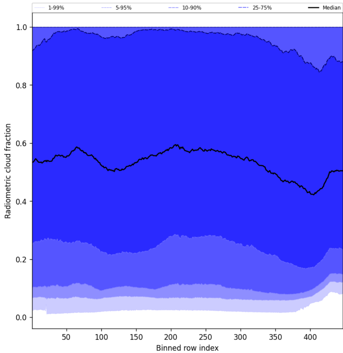
Figure 55: Along track statistics of “Radiometric cloud fraction” for 2024-10-12 to 2024-10-14
