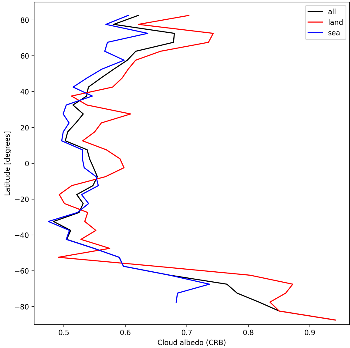
Figure 28: Zonal average of “Cloud albedo (CRB)” for 2024-10-12 to 2024-10-14.
