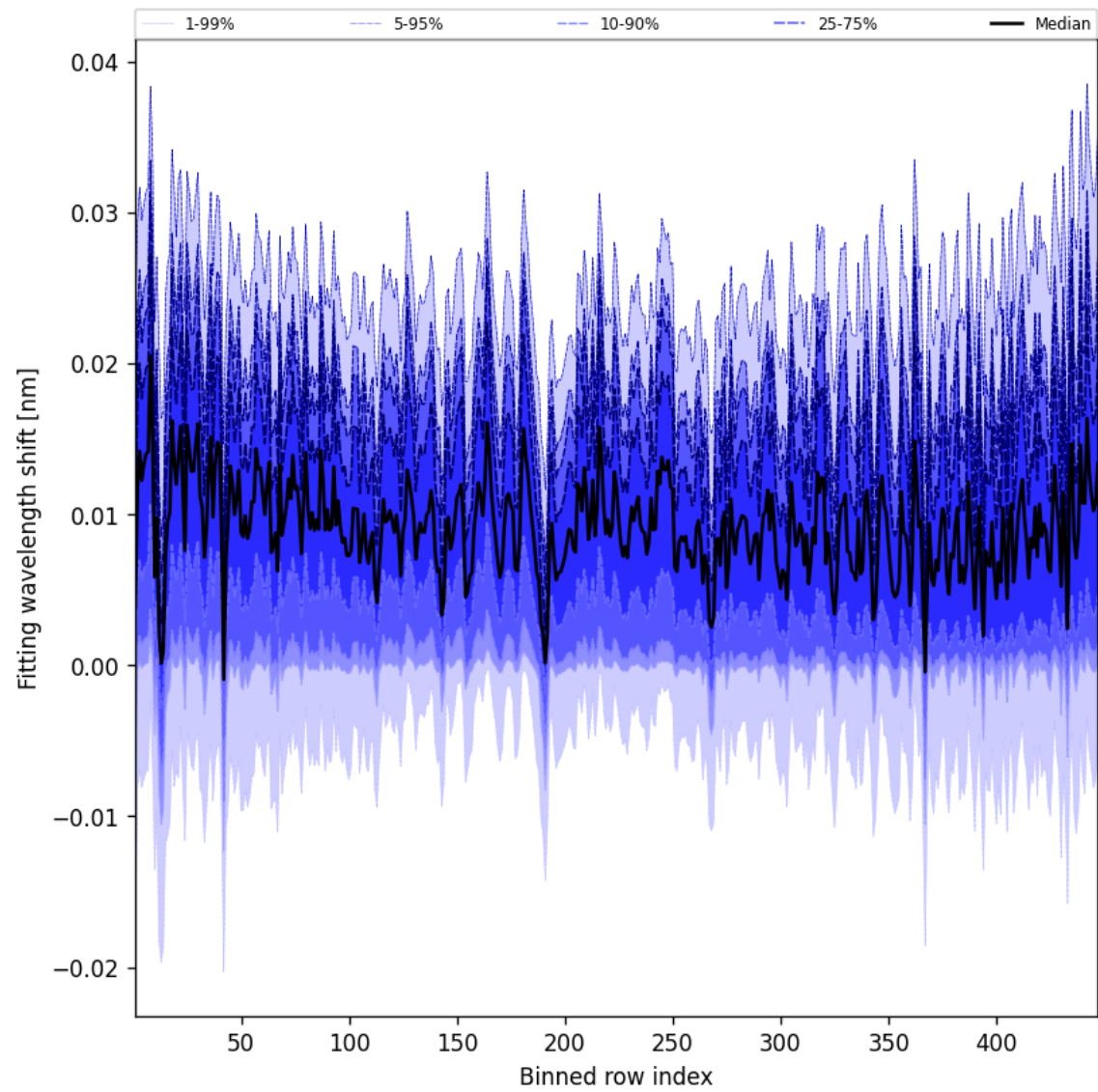
Figure 65: Along track statistics of “Fitting wavelength shift” for 2024-10-12 to 2024-10-14
