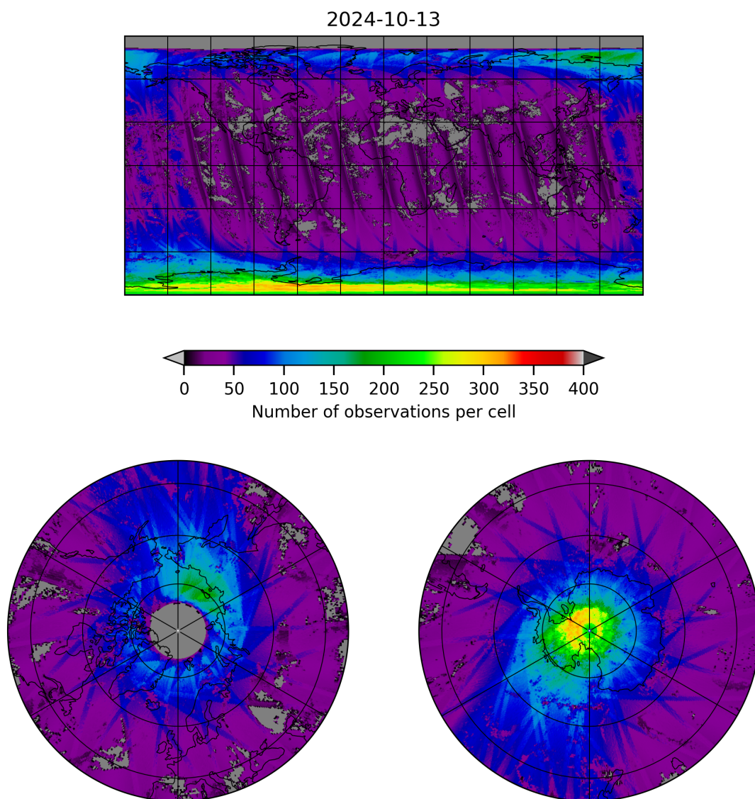
Figure 21: Map of the number of observations for 2024-10-12 to 2024-10-14
