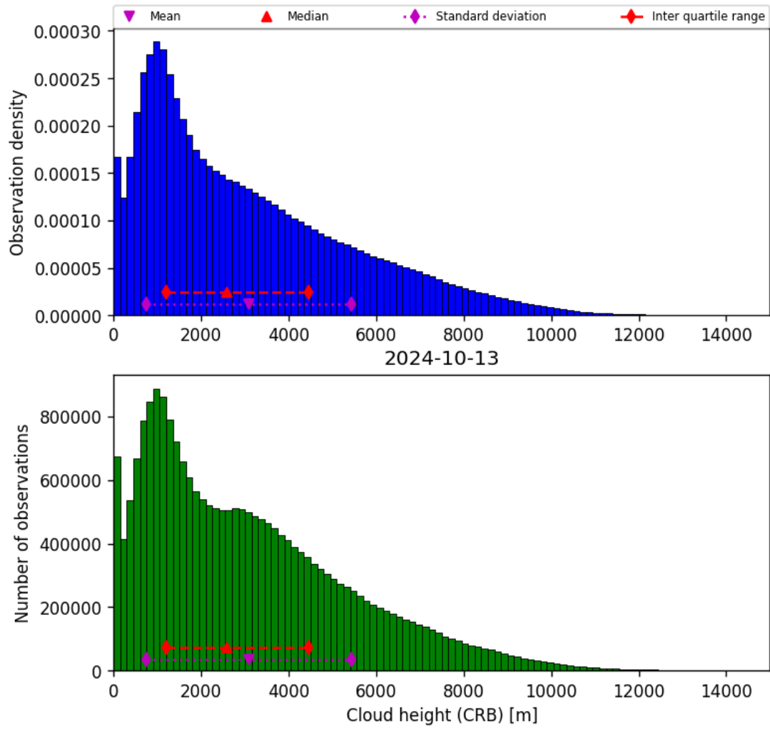
Figure 43: Histogram of “Cloud height (CRB)” for 2024-10-12 to 2024-10-14
