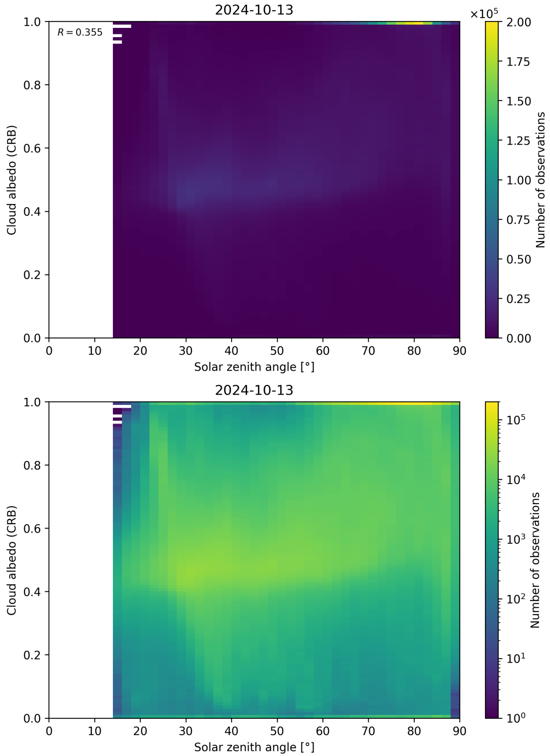
Figure 98: Scatter density plot of “Solar zenith angle” against “Cloud albedo (CRB)” for 2024-10-12 to 2024-10-14.
