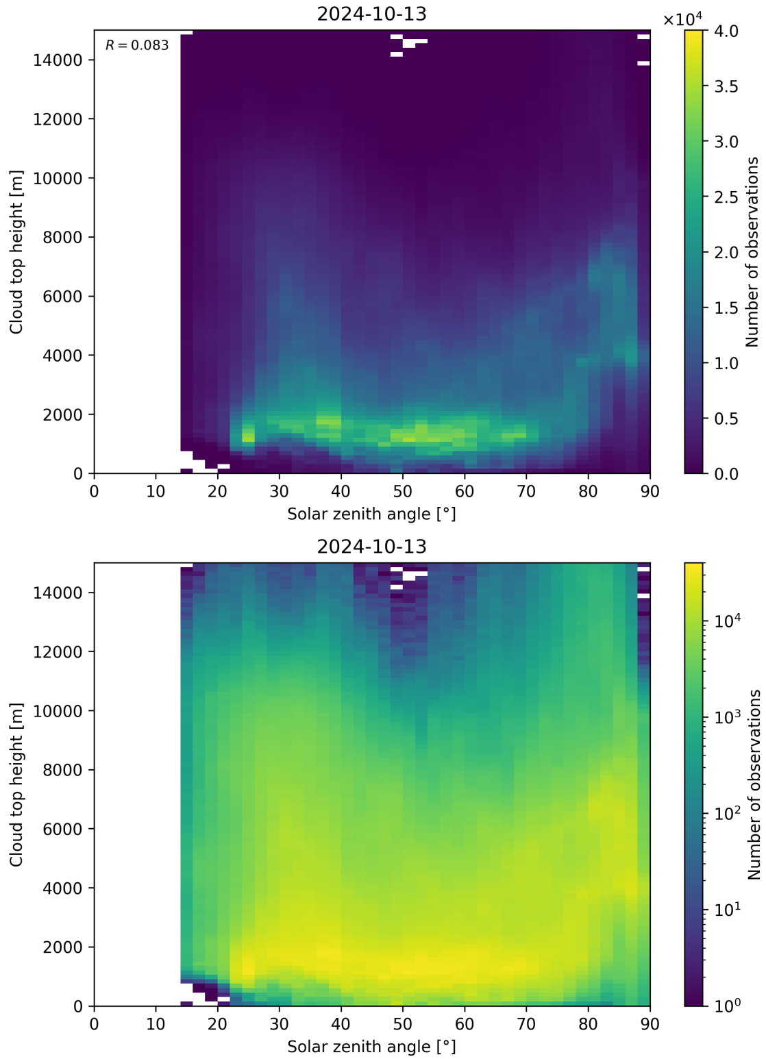
Figure 104: Scatter density plot of “Solar zenith angle” against “Cloud top height” for 2024-10-12 to 2024-10-14.
