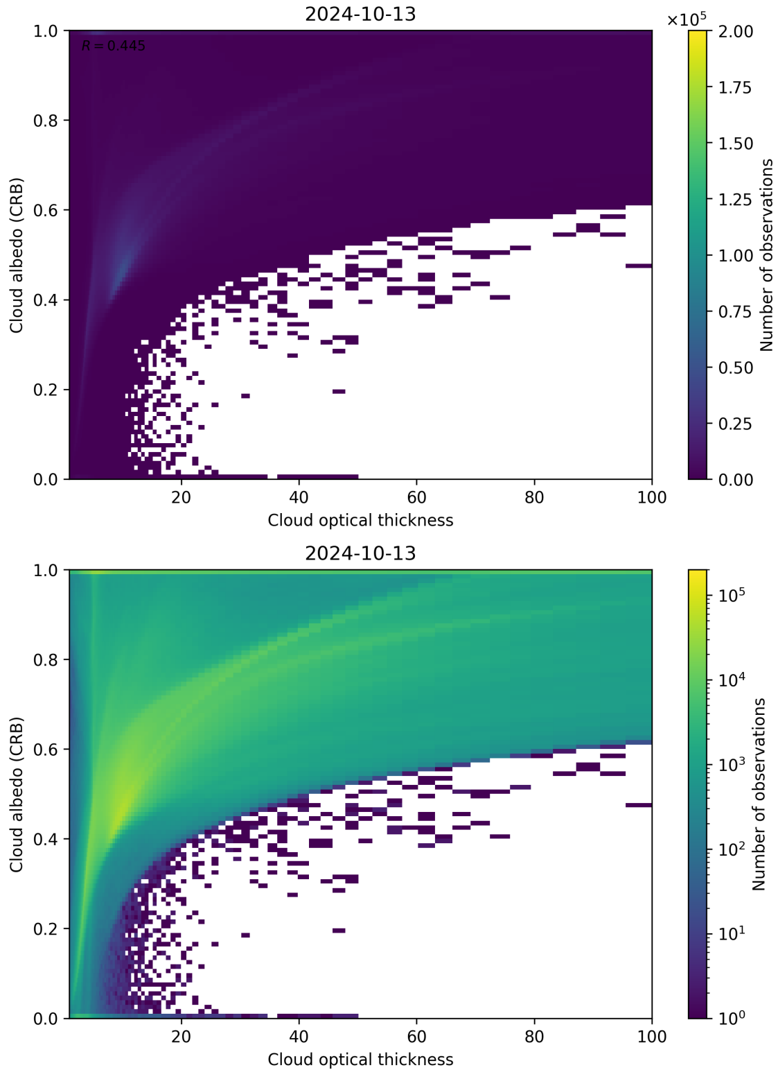
Figure 82: Scatter density plot of “Cloud optical thickness” against “Cloud albedo (CRB)” for 2024-10-12 to 2024-10-14.
