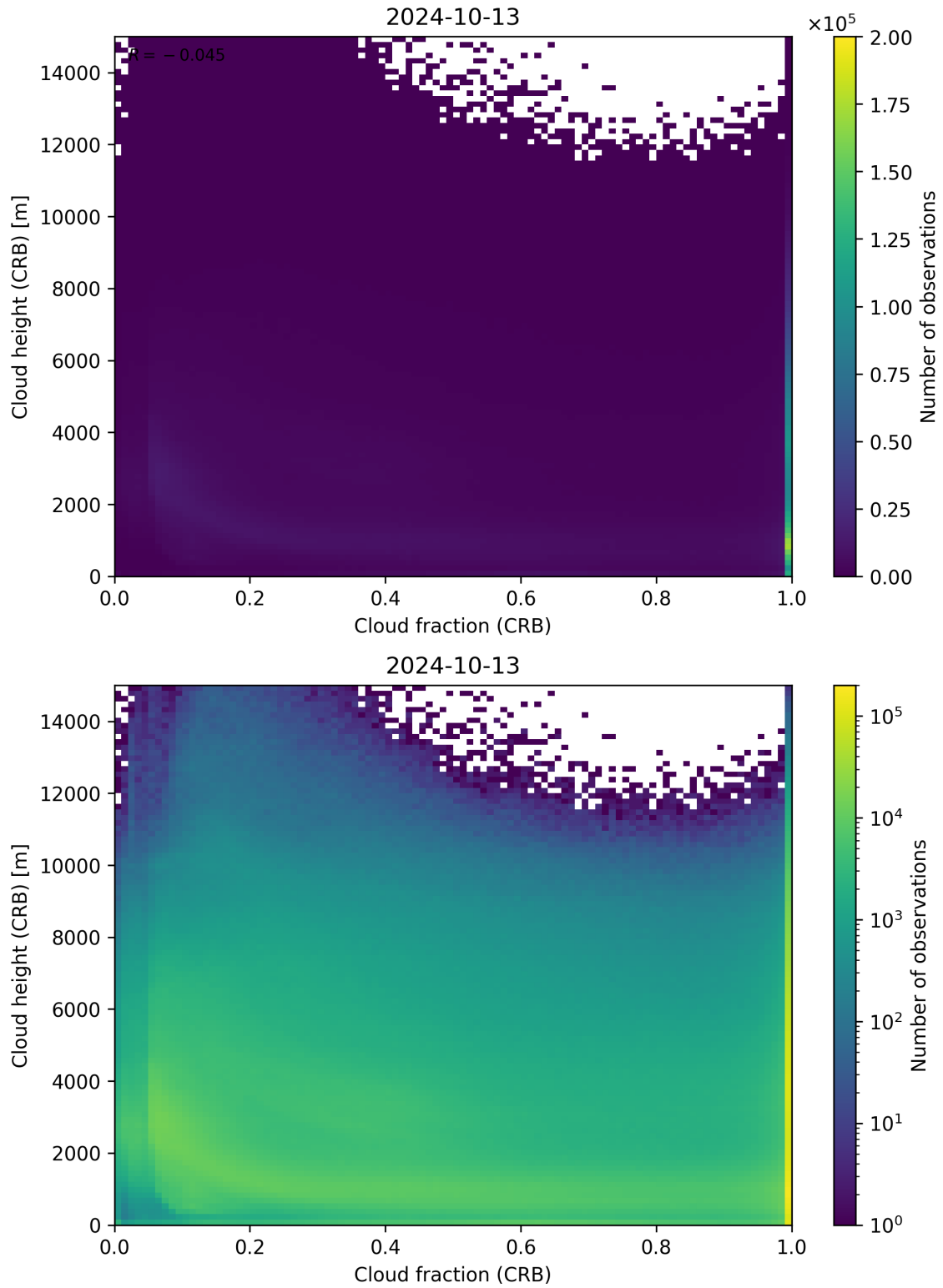
Figure 79: Scatter density plot of “Cloud fraction (CRB)” against “Cloud height (CRB)” for 2024-10-12 to 2024-10-14.
