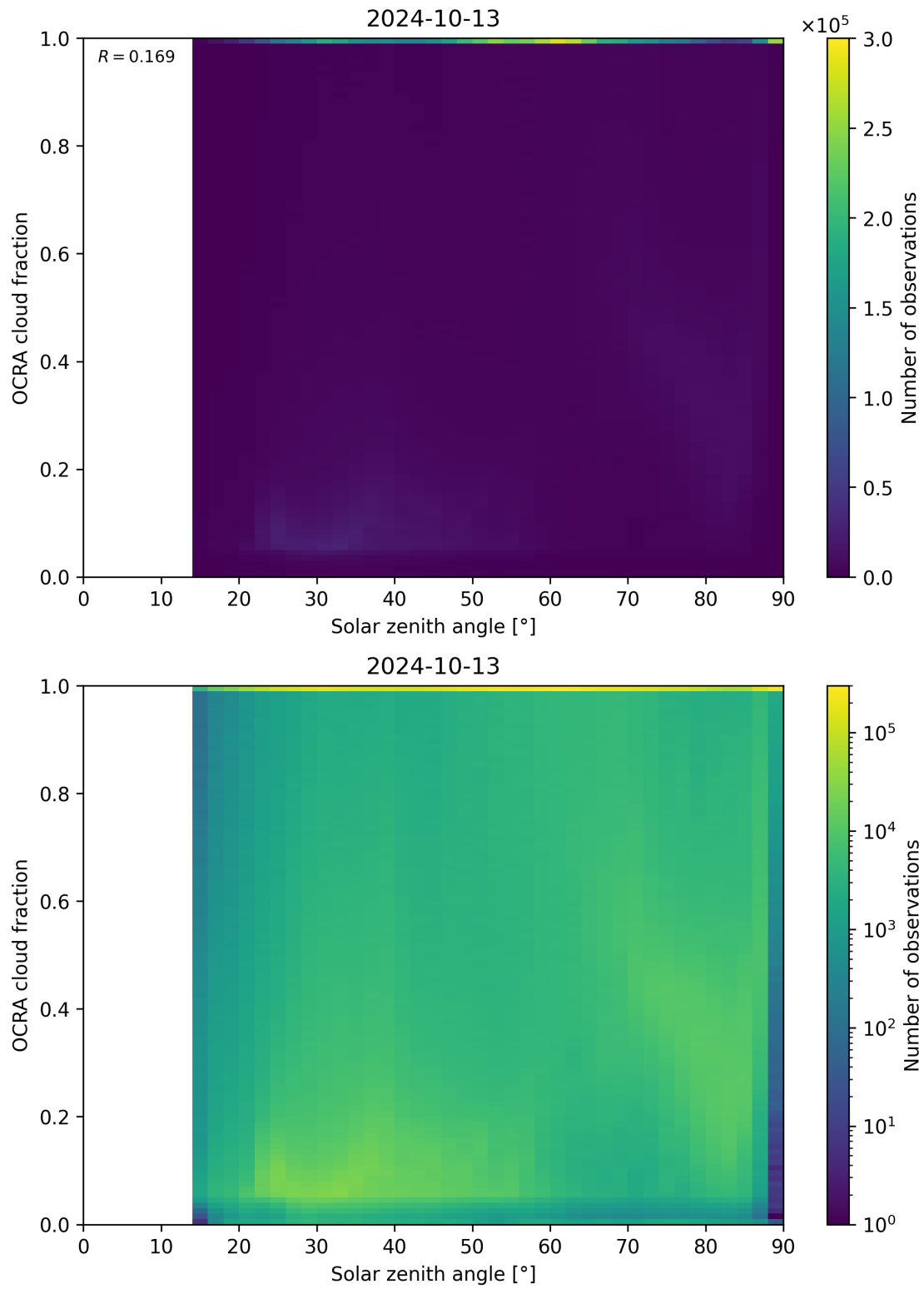
Figure 100: Scatter density plot of “Solar zenith angle” against “OCRA cloud fraction” for 2024-10-12 to 2024-10-14.
