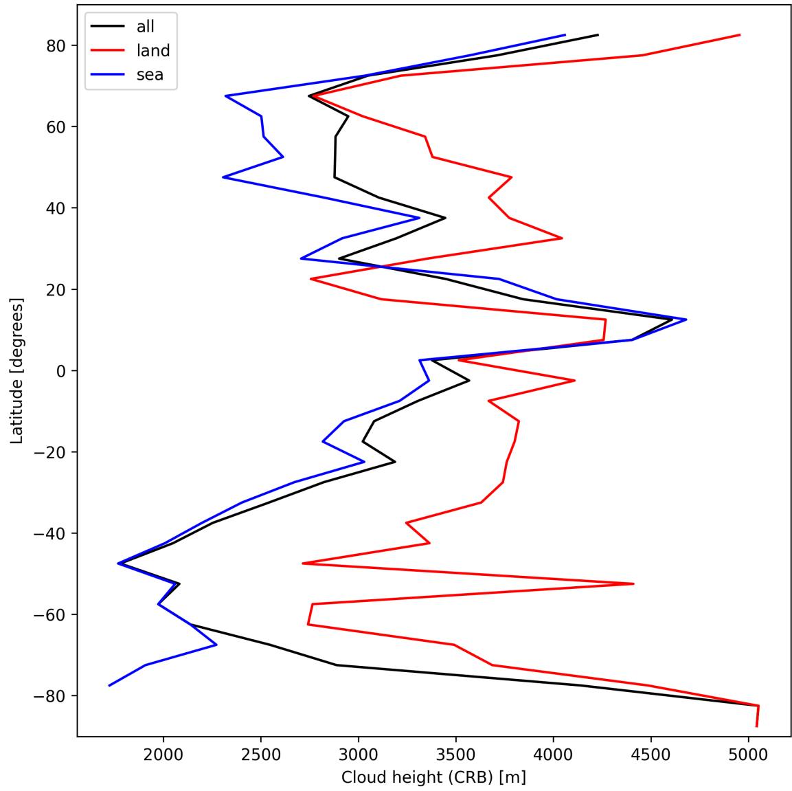
Figure 27: Zonal average of “Cloud height (CRB)” for 2024-10-12 to 2024-10-14.
