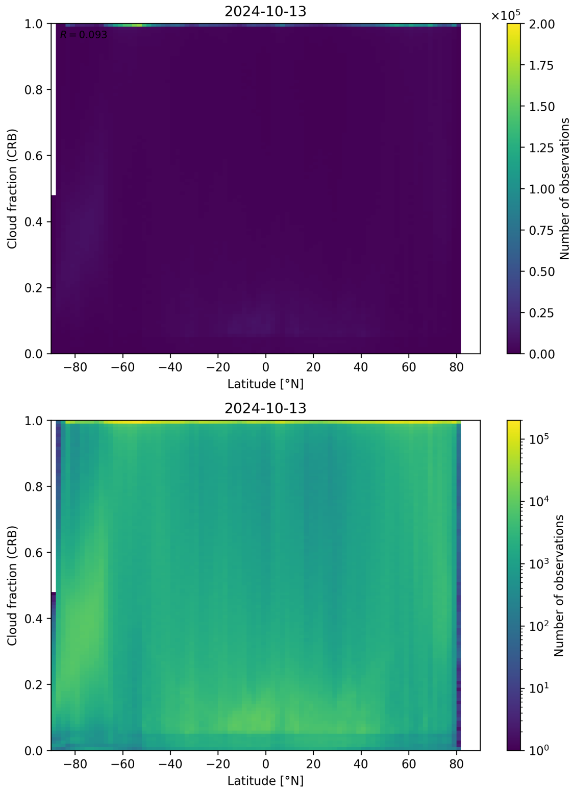
Figure 94: Scatter density plot of “Latitude” against “Cloud fraction (CRB)” for 2024-10-12 to 2024-10-14.
