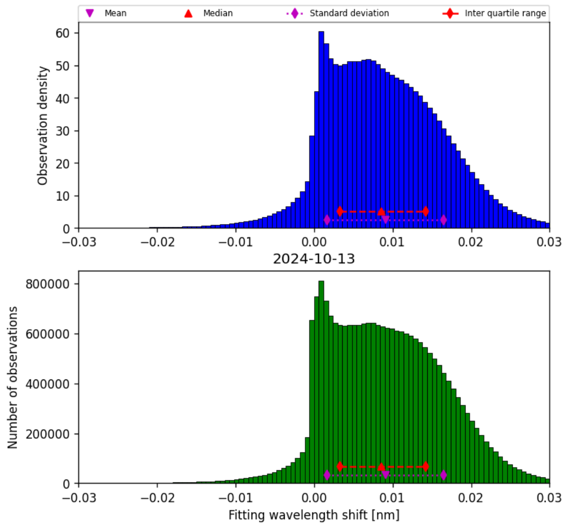
Figure 49: Histogram of “Fitting wavelength shift” for 2024-10-12 to 2024-10-14
