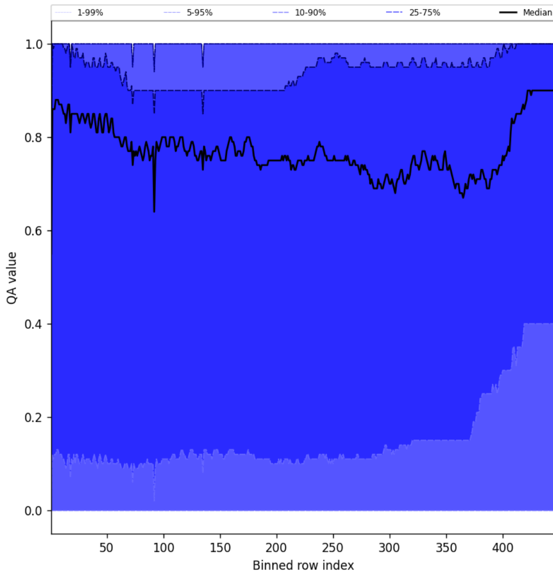
Figure 54: Along track statistics of “QA value” for 2024-10-12 to 2024-10-14
