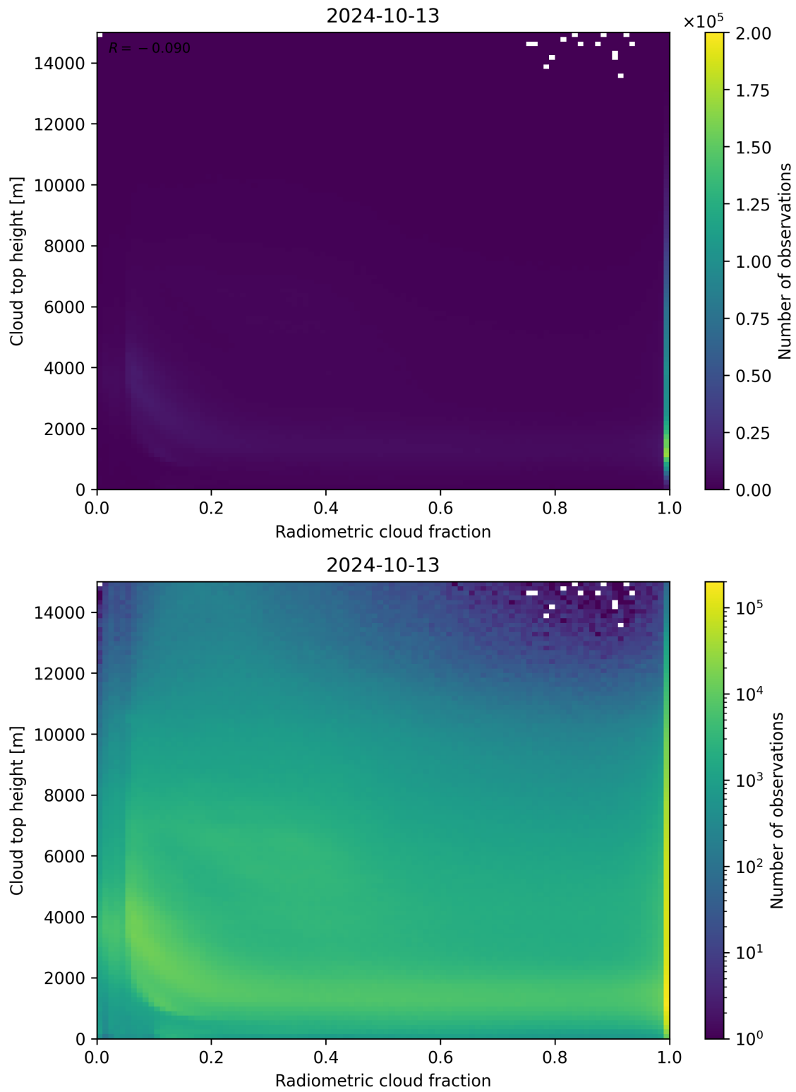
Figure 76: Scatter density plot of “Radiometric cloud fraction” against “Cloud top height” for 2024-10-12 to 2024-10-14.
