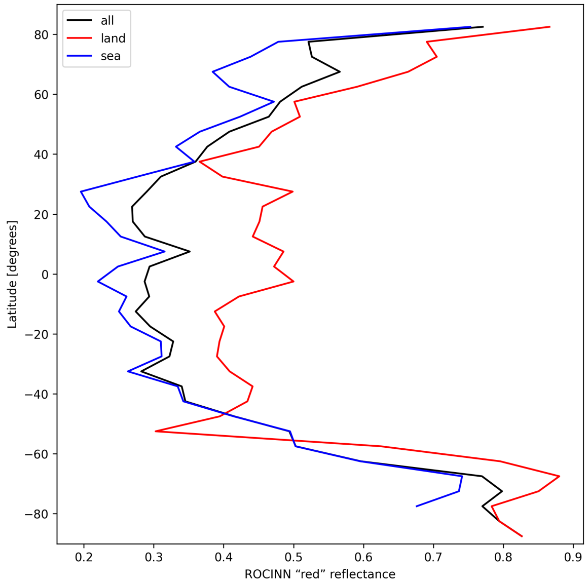
Figure 37: Zonal average of “ROCINN “red” reflectance” for 2024-10-12 to 2024-10-14.
