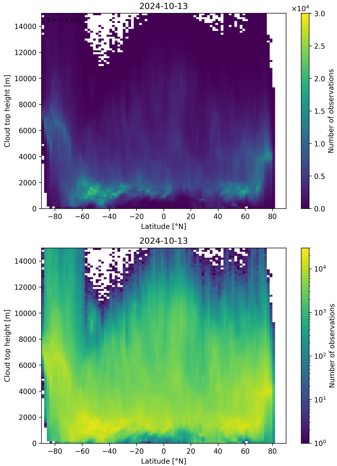
Figure 97: Scatter density plot of “Latitude” against “Cloud top height” for 2024-10-12 to 2024-10-14.
