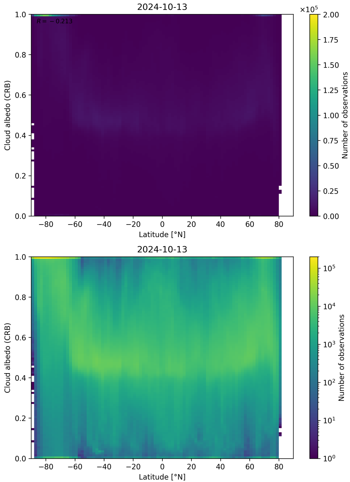
Figure 91: Scatter density plot of “Latitude” against “Cloud albedo (CRB)” for 2024-10-12 to 2024-10-14.
