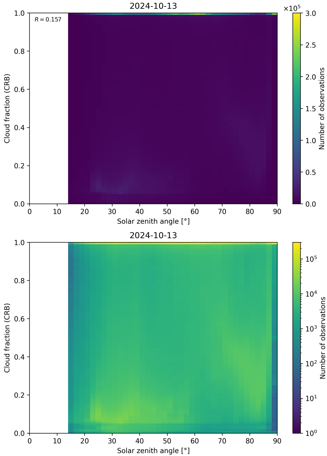
Figure 101: Scatter density plot of “Solar zenith angle” against “Cloud fraction (CRB)” for 2024-10-12 to 2024-10-14.
