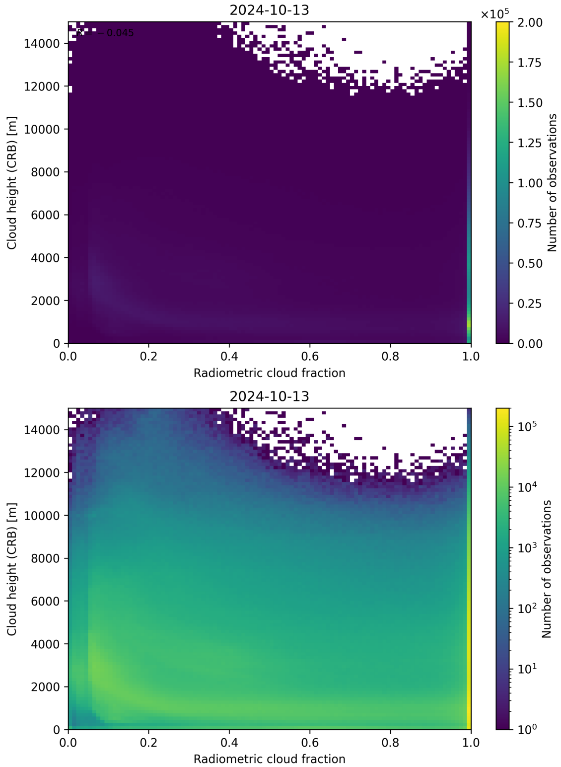
Figure 74: Scatter density plot of “Radiometric cloud fraction” against “Cloud height (CRB)” for 2024-10-12 to 2024-10-14.
