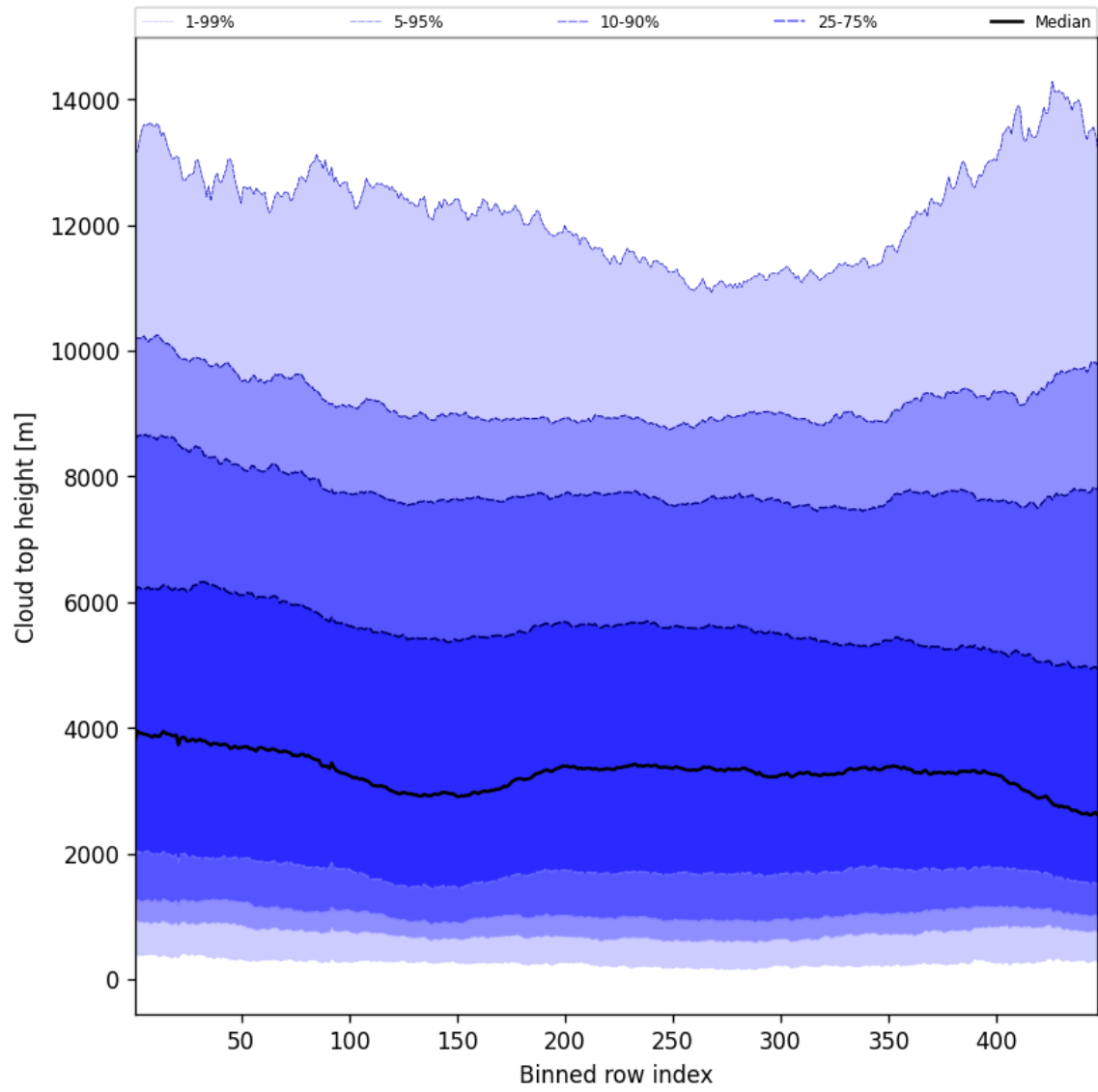
Figure 56: Along track statistics of “Cloud top height” for 2024-10-12 to 2024-10-14
