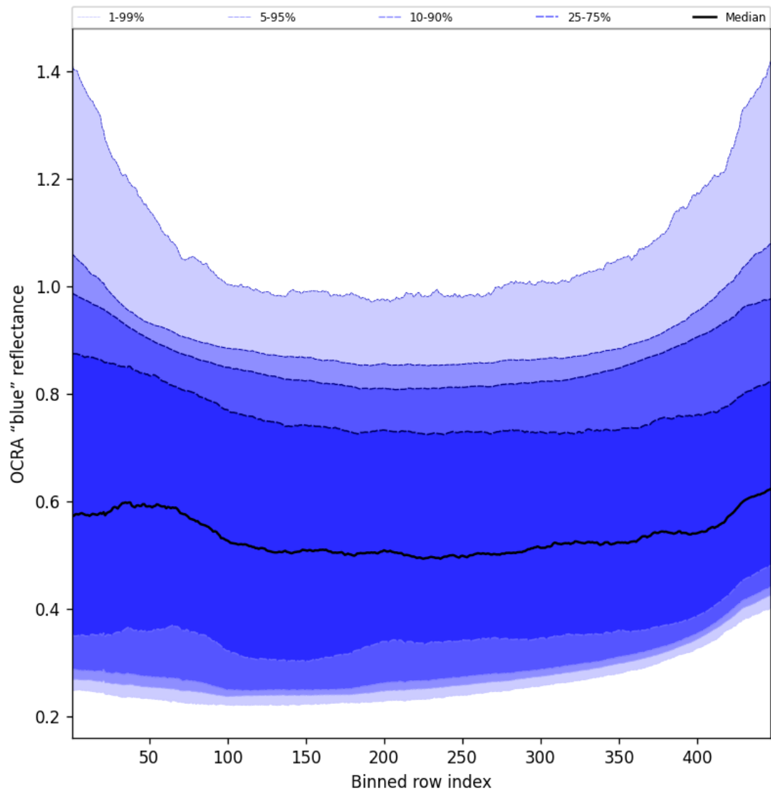
Figure 67: Along track statistics of “OCRA “blue” reflectance” for 2024-10-12 to 2024-10-14
