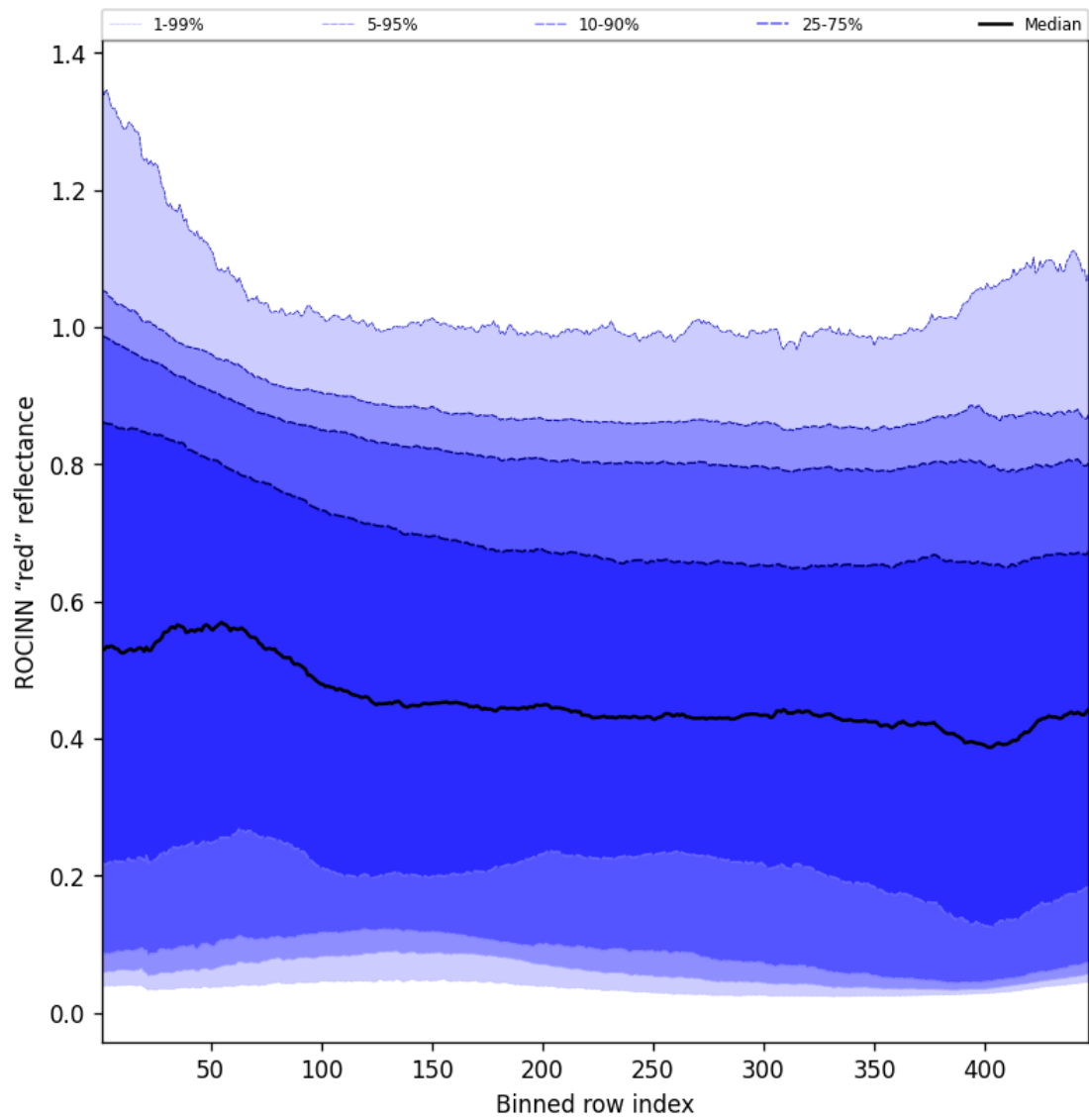
Figure 69: Along track statistics of “ROCINN “red” reflectance” for 2024-10-12 to 2024-10-14
