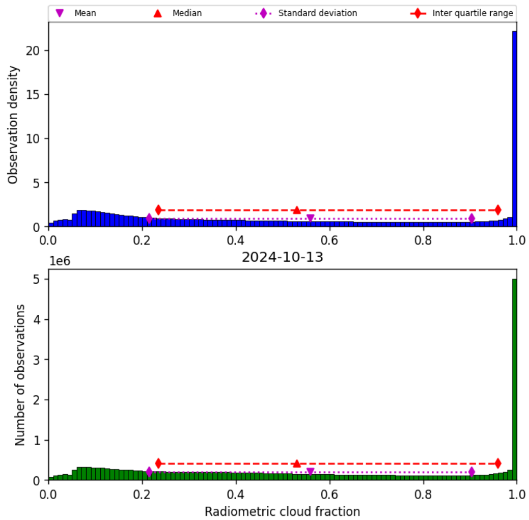
Figure 39: Histogram of “Radiometric cloud fraction” for 2024-10-12 to 2024-10-14
