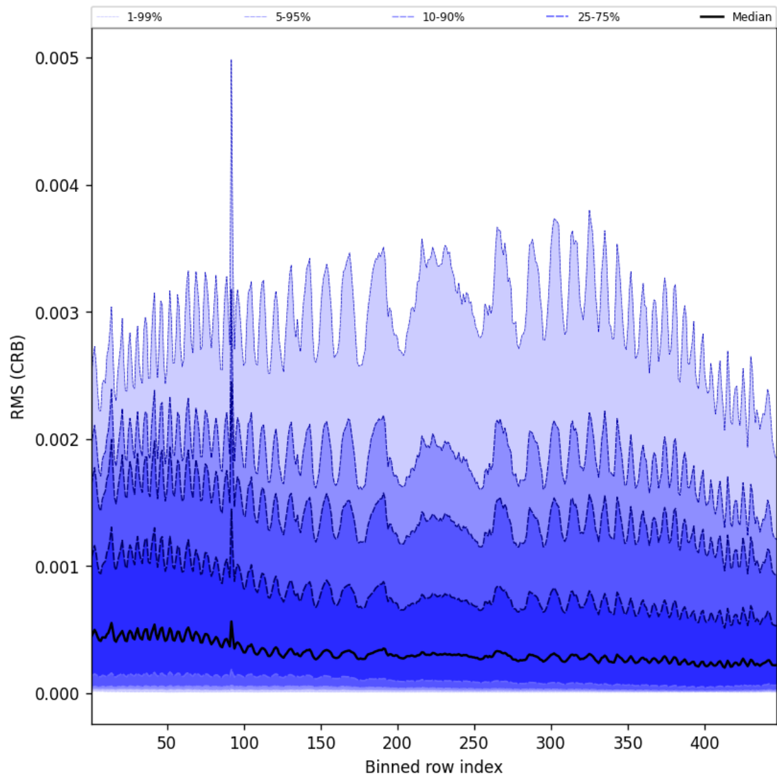
Figure 64: Along track statistics of “RMS (CRB)” for 2024-10-12 to 2024-10-14
