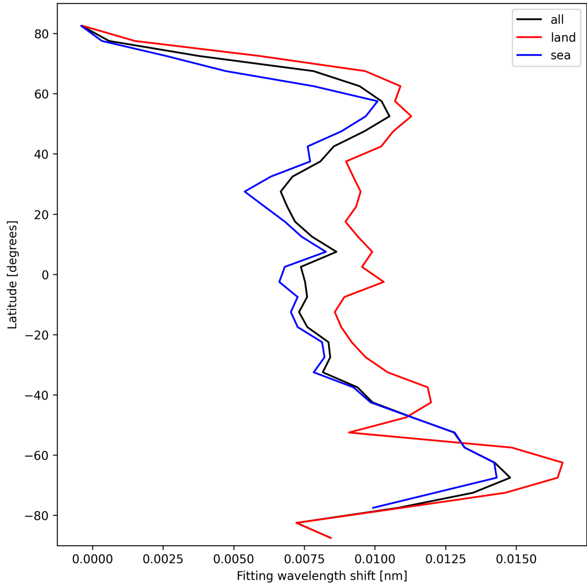
Figure 33: Zonal average of “Fitting wavelength shift” for 2024-10-12 to 2024-10-14.
