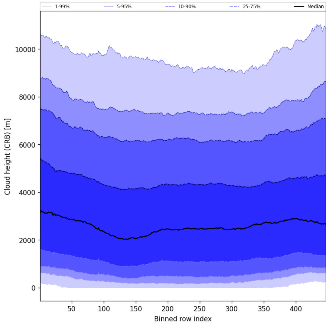
Figure 59: Along track statistics of “Cloud height (CRB)” for 2024-10-12 to 2024-10-14
