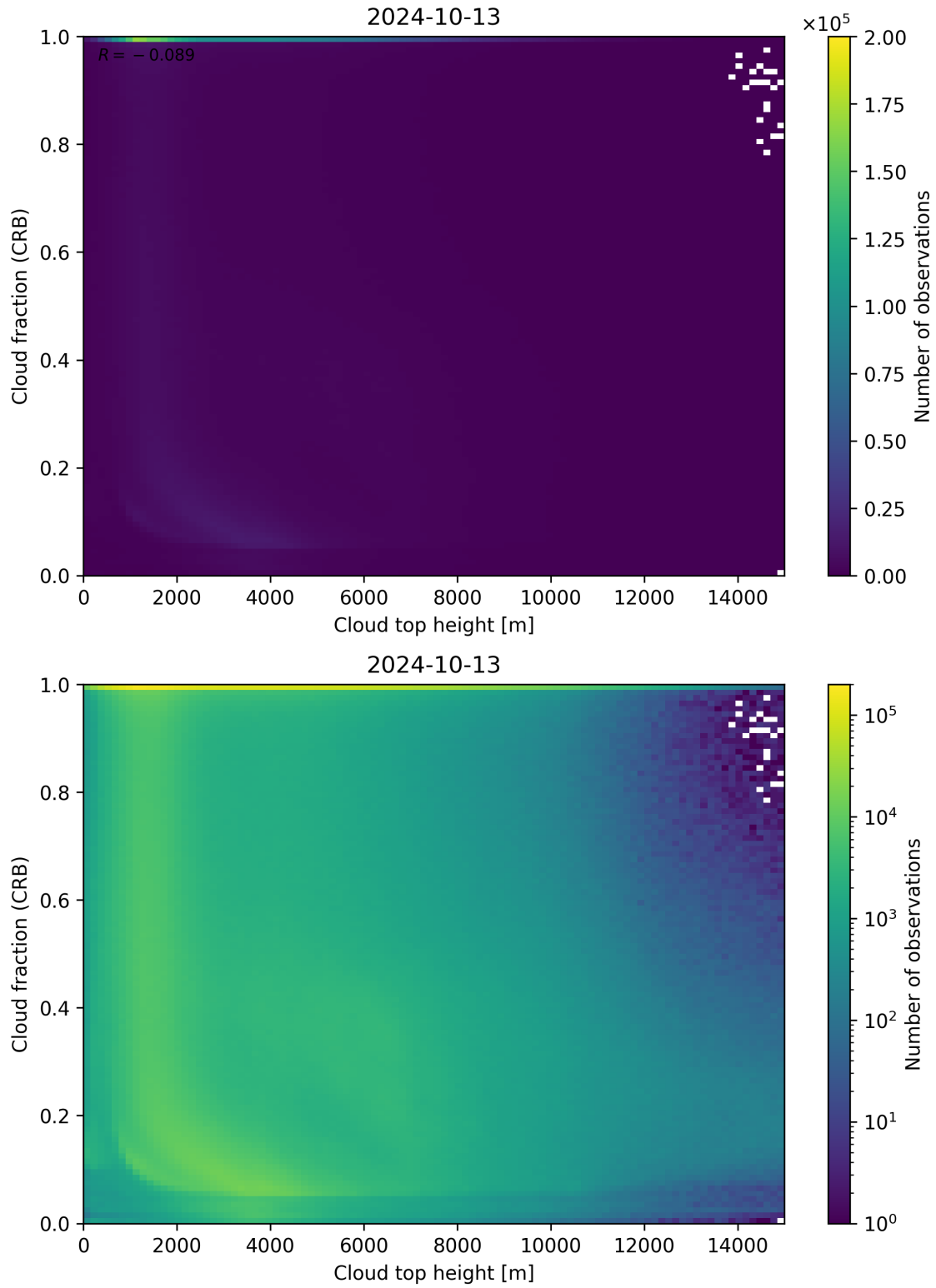
Figure 88: Scatter density plot of “Cloud top height” against “Cloud fraction (CRB)” for 2024-10-12 to 2024-10-14.
