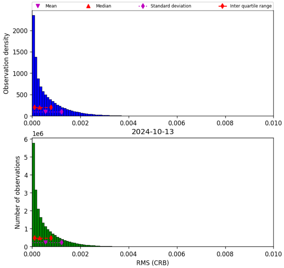
Figure 48: Histogram of “RMS (CRB)” for 2024-10-12 to 2024-10-14
