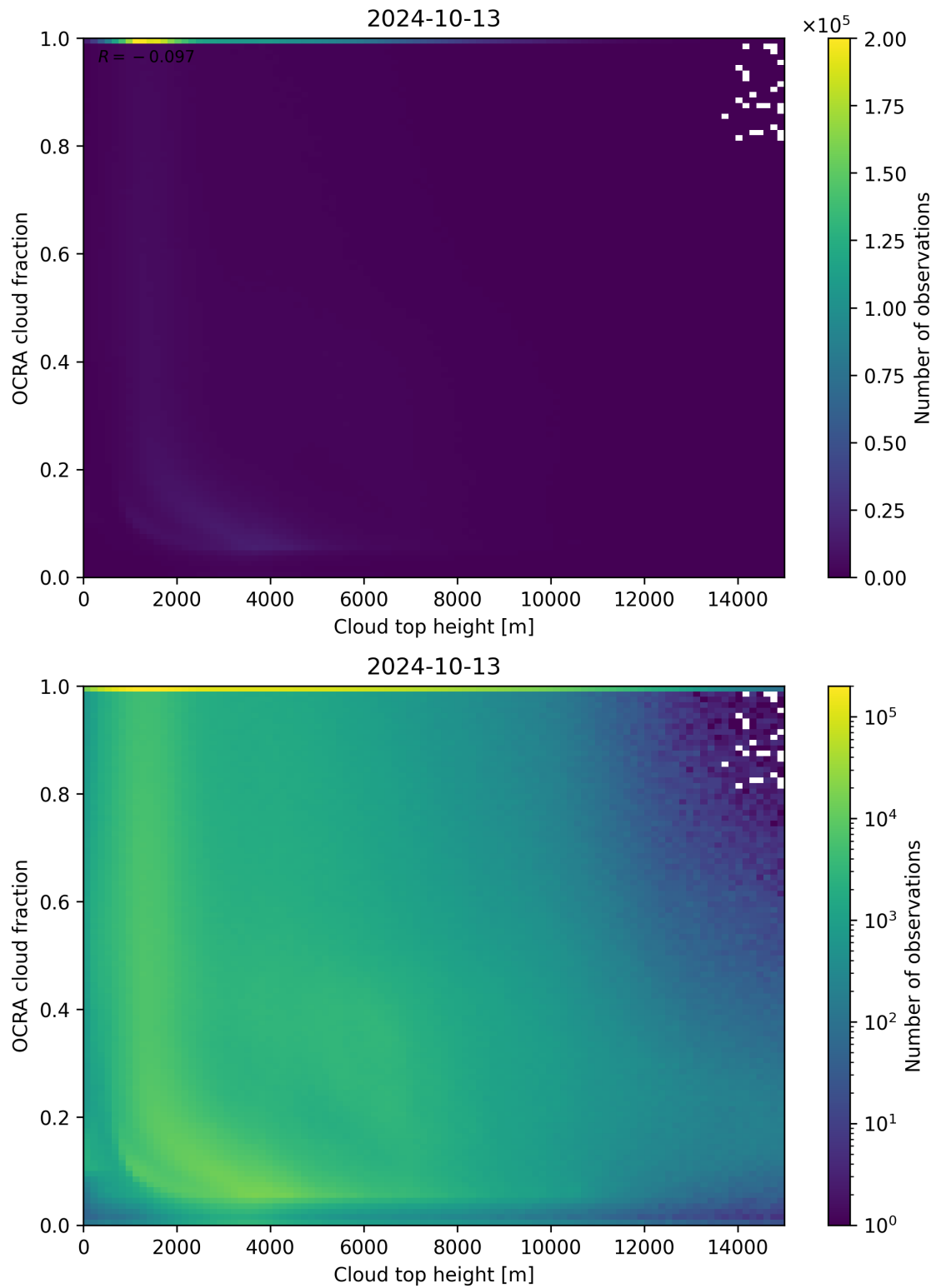
Figure 87: Scatter density plot of “Cloud top height” against “OCRA cloud fraction” for 2024-10-12 to 2024-10-14.
