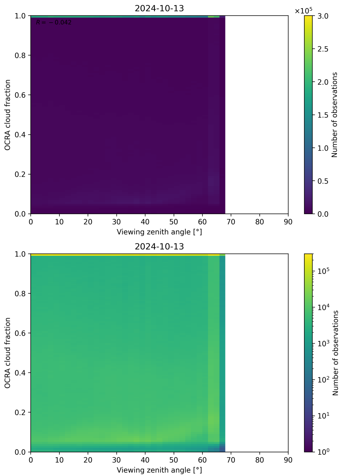
Figure 108: Scatter density plot of “Viewing zenith angle” against “OCRA cloud fraction” for 2024-10-12 to 2024-10-14.
