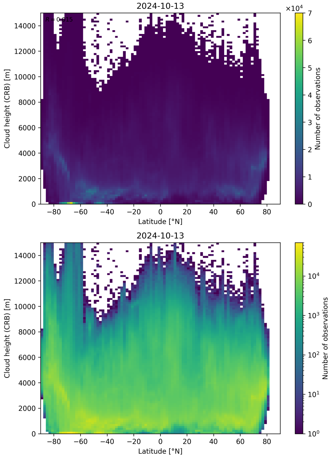
Figure 95: Scatter density plot of “Latitude” against “Cloud height (CRB)” for 2024-10-12 to 2024-10-14.
