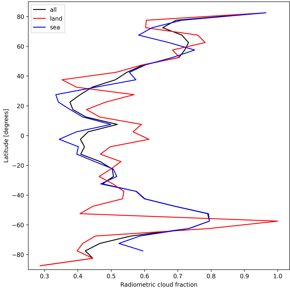
Figure 23: Zonal average of “Radiometric cloud fraction” for 2024-10-12 to 2024-10-14.
