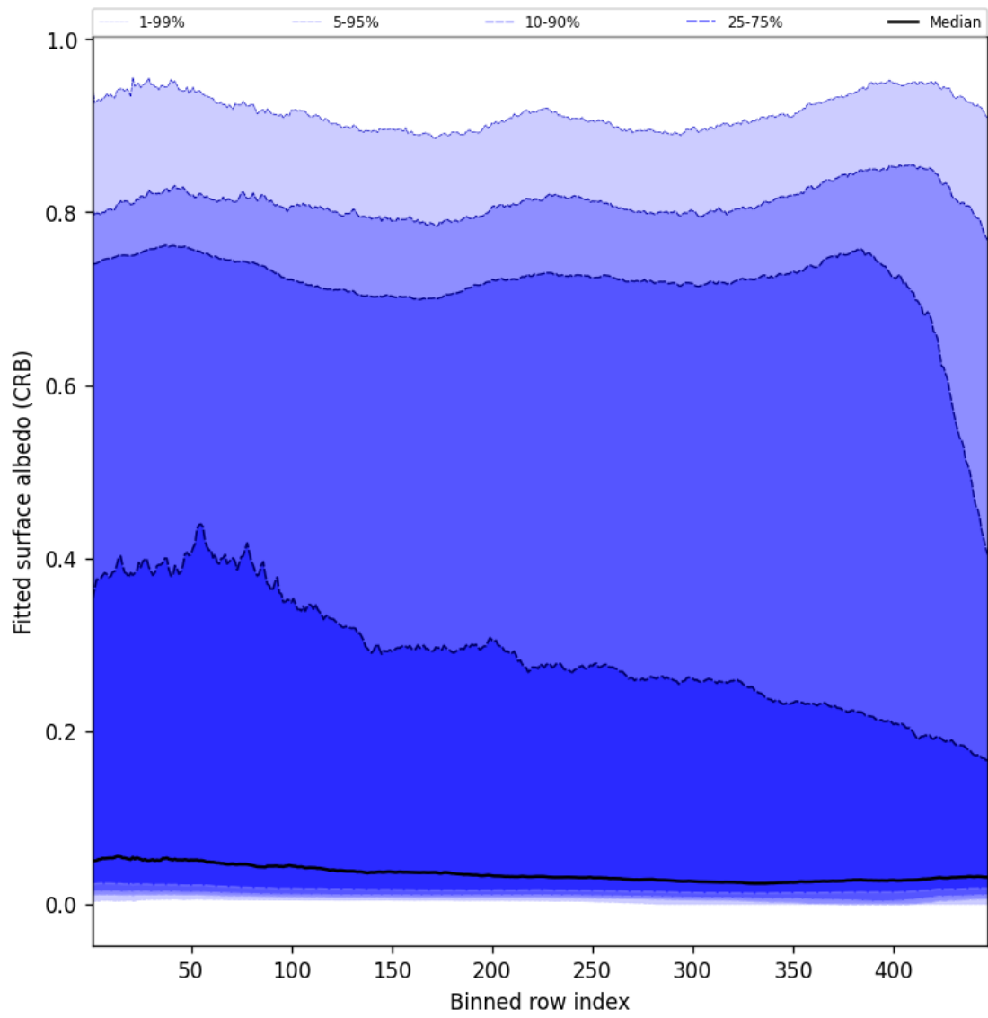
Figure 62: Along track statistics of “Fitted surface albedo (CRB)” for 2024-10-12 to 2024-10-14
