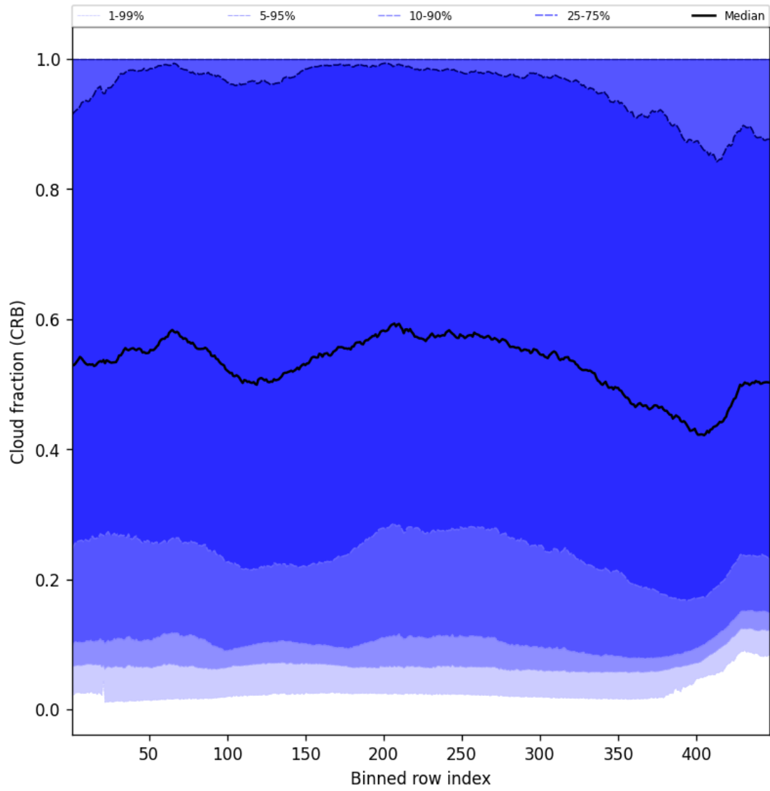
Figure 58: Along track statistics of “Cloud fraction (CRB)” for 2024-10-12 to 2024-10-14
