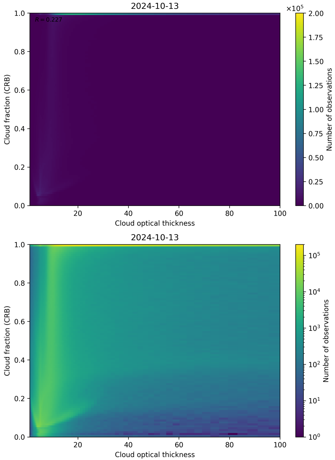
Figure 84: Scatter density plot of “Cloud optical thickness” against “Cloud fraction (CRB)” for 2024-10-12 to 2024-10-14.
