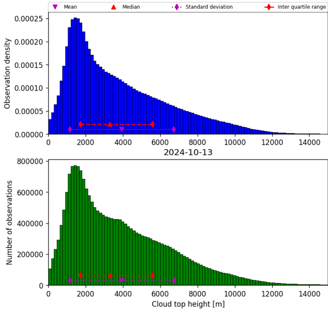
Figure 40: Histogram of “Cloud top height” for 2024-10-12 to 2024-10-14
