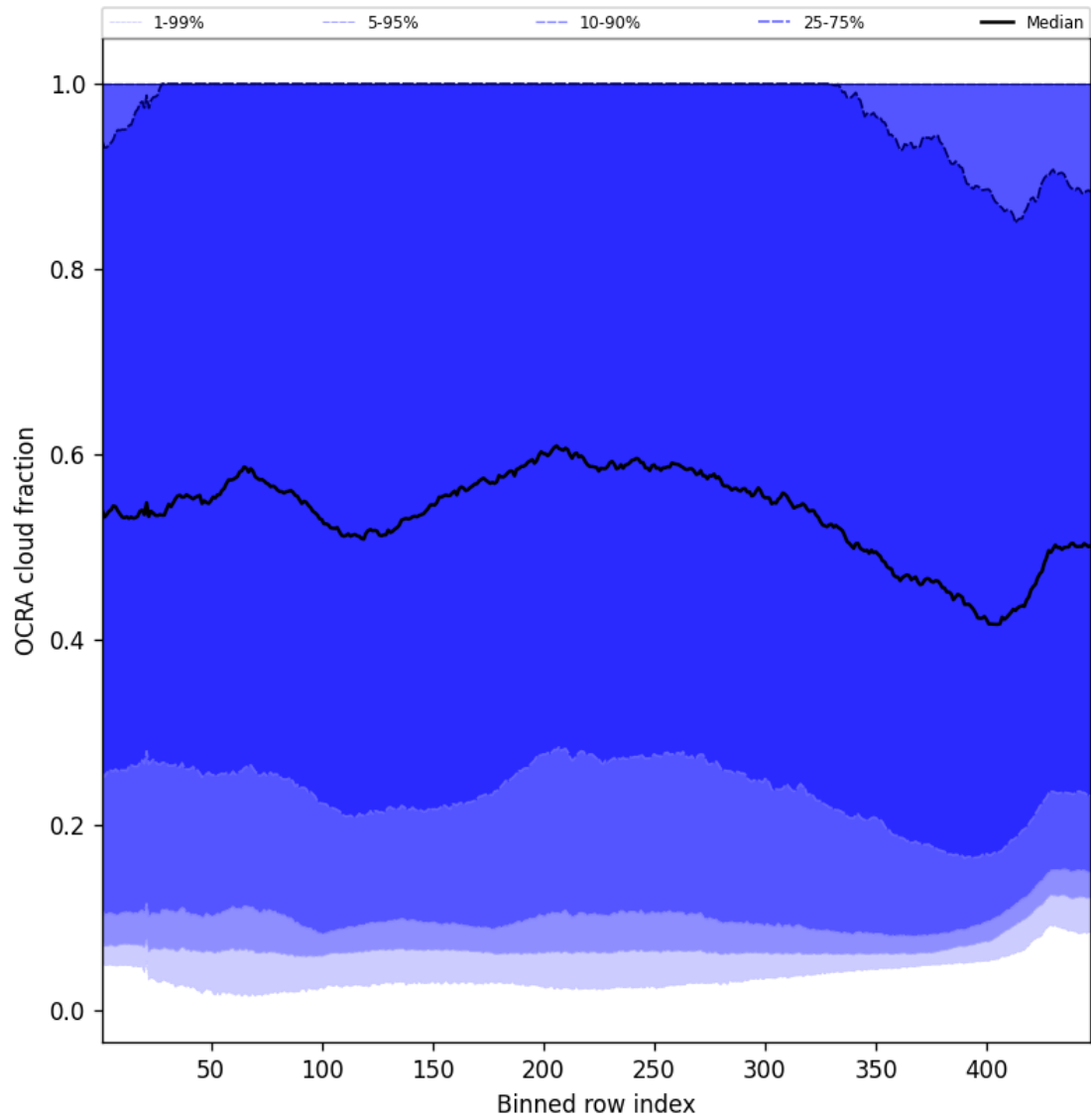
Figure 66: Along track statistics of “OCRA cloud fraction” for 2024-10-12 to 2024-10-14
