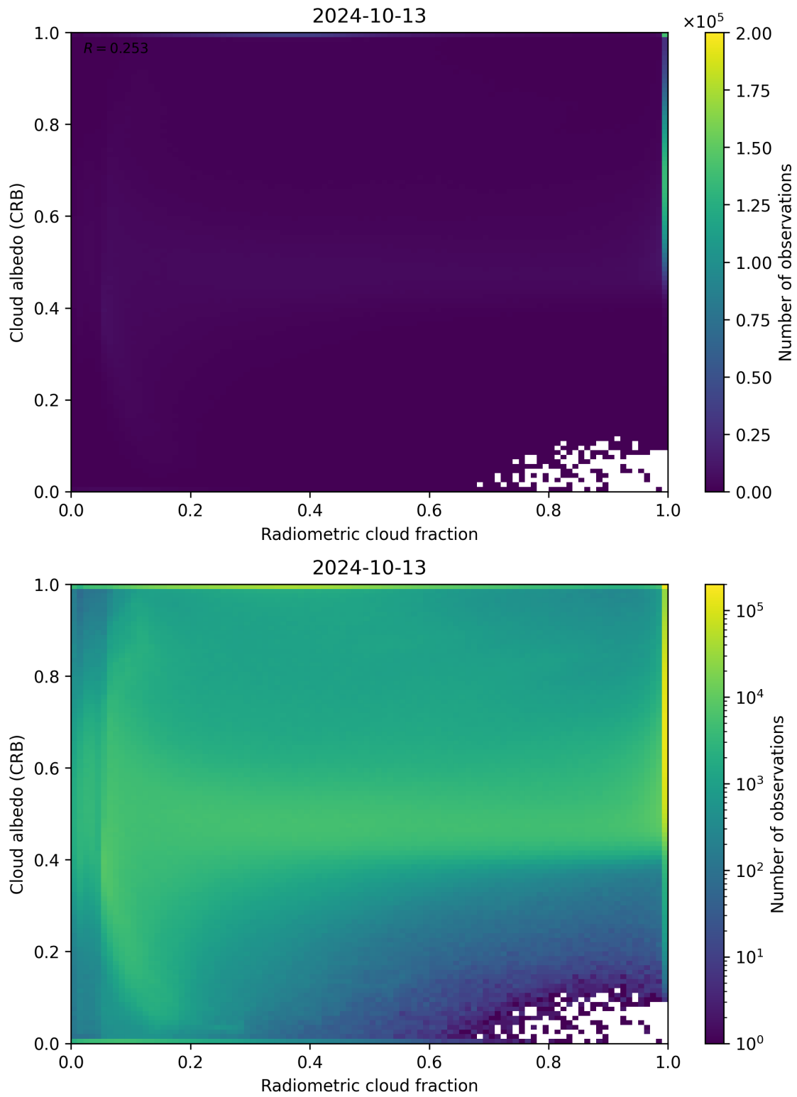
Figure 71: Scatter density plot of “Radiometric cloud fraction” against “Cloud albedo (CRB)” for 2024-10-12 to 2024-10-14.
