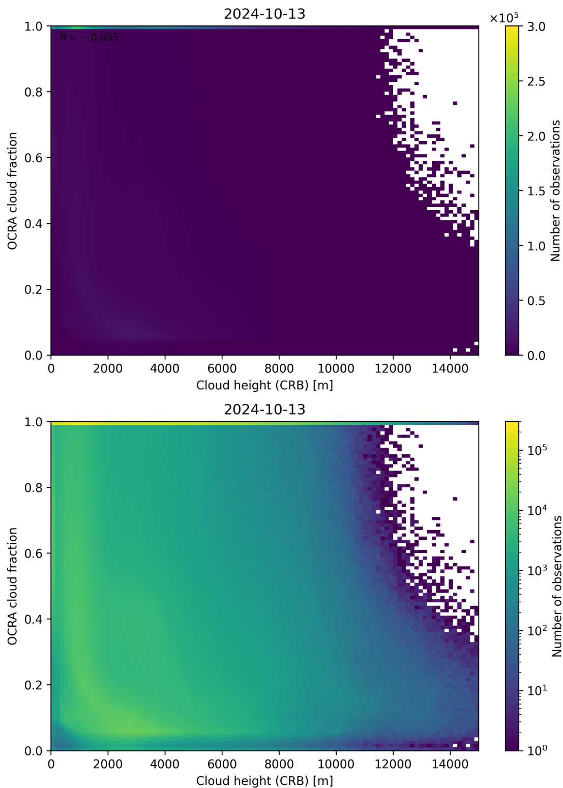
Figure 81: Scatter density plot of “Cloud height (CRB)” against “OCRA cloud fraction” for 2024-10-12 to 2024-10-14.
