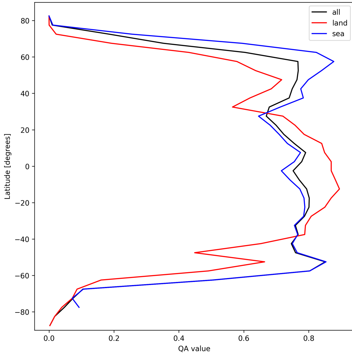
Figure 22: Zonal average of “QA value” for 2024-10-12 to 2024-10-14.
