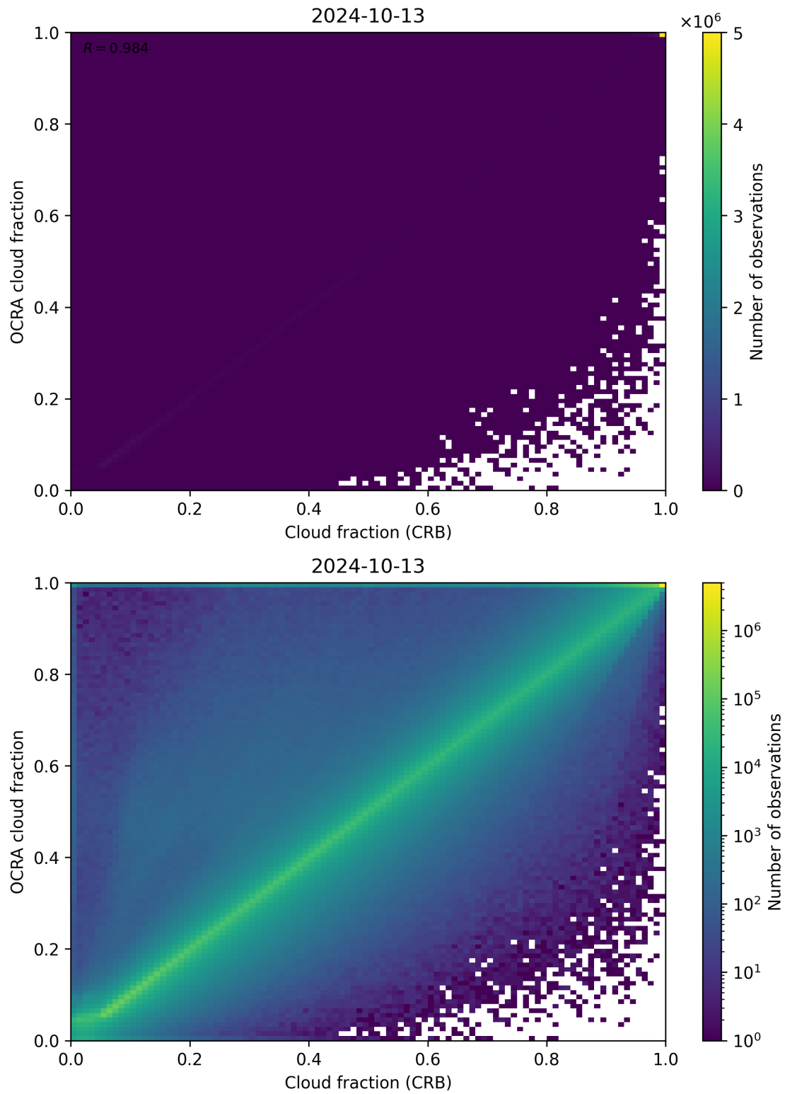
Figure 78: Scatter density plot of “Cloud fraction (CRB)” against “OCRA cloud fraction” for 2024-10-12 to 2024-10-14.
