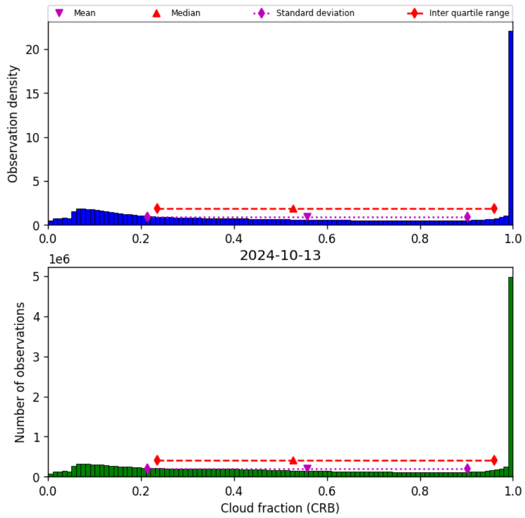
Figure 42: Histogram of “Cloud fraction (CRB)” for 2024-10-12 to 2024-10-14
