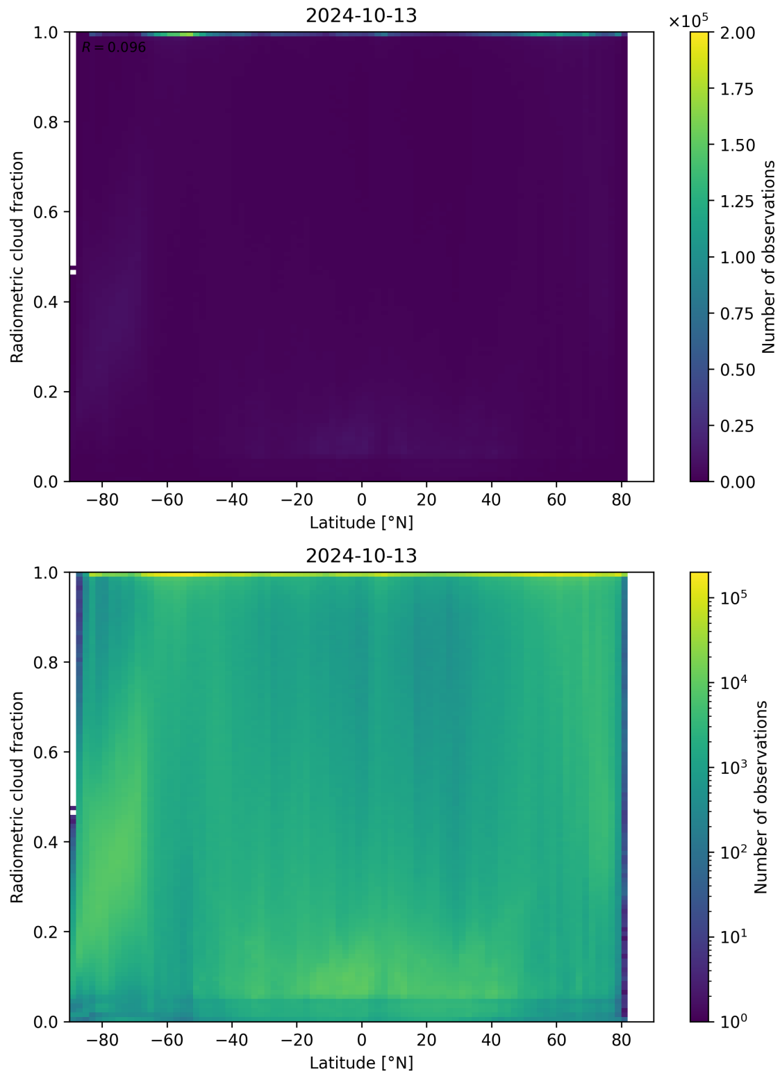
Figure 92: Scatter density plot of “Latitude” against “Radiometric cloud fraction” for 2024-10-12 to 2024-10-14.
