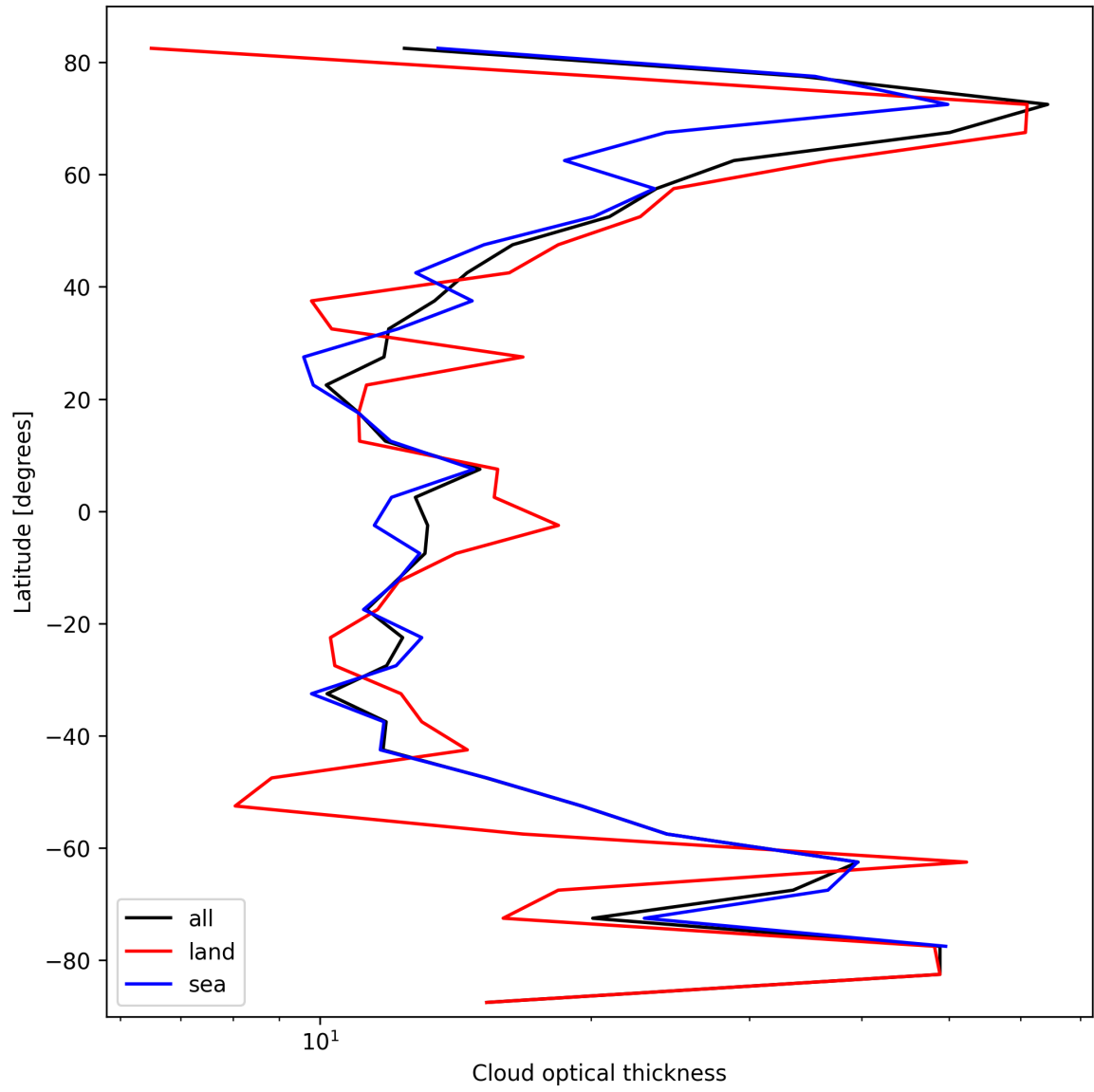
Figure 25: Zonal average of “Cloud optical thickness” for 2024-10-12 to 2024-10-14.
