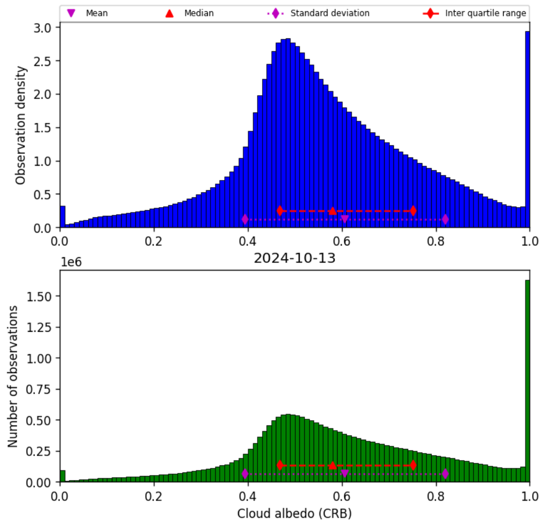
Figure 44: Histogram of “Cloud albedo (CRB)” for 2024-10-12 to 2024-10-14
