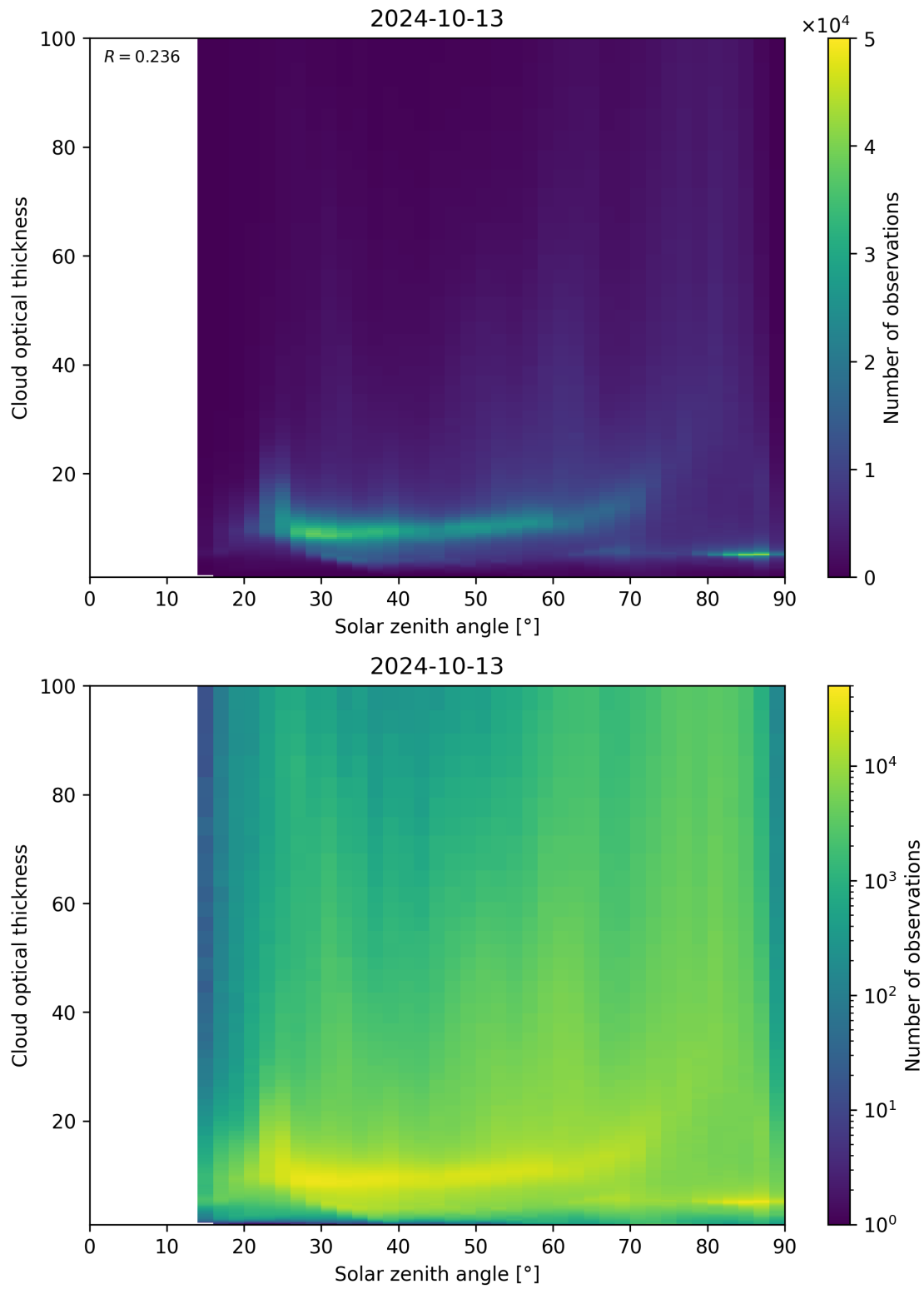
Figure 103: Scatter density plot of “Solar zenith angle” against “Cloud optical thickness” for 2024-10-12 to 2024-10-14.
