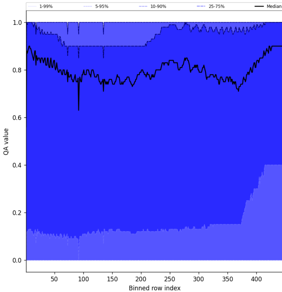
Figure 54: Along track statistics of “QA value” for 2024-10-14 to 2024-10-15
