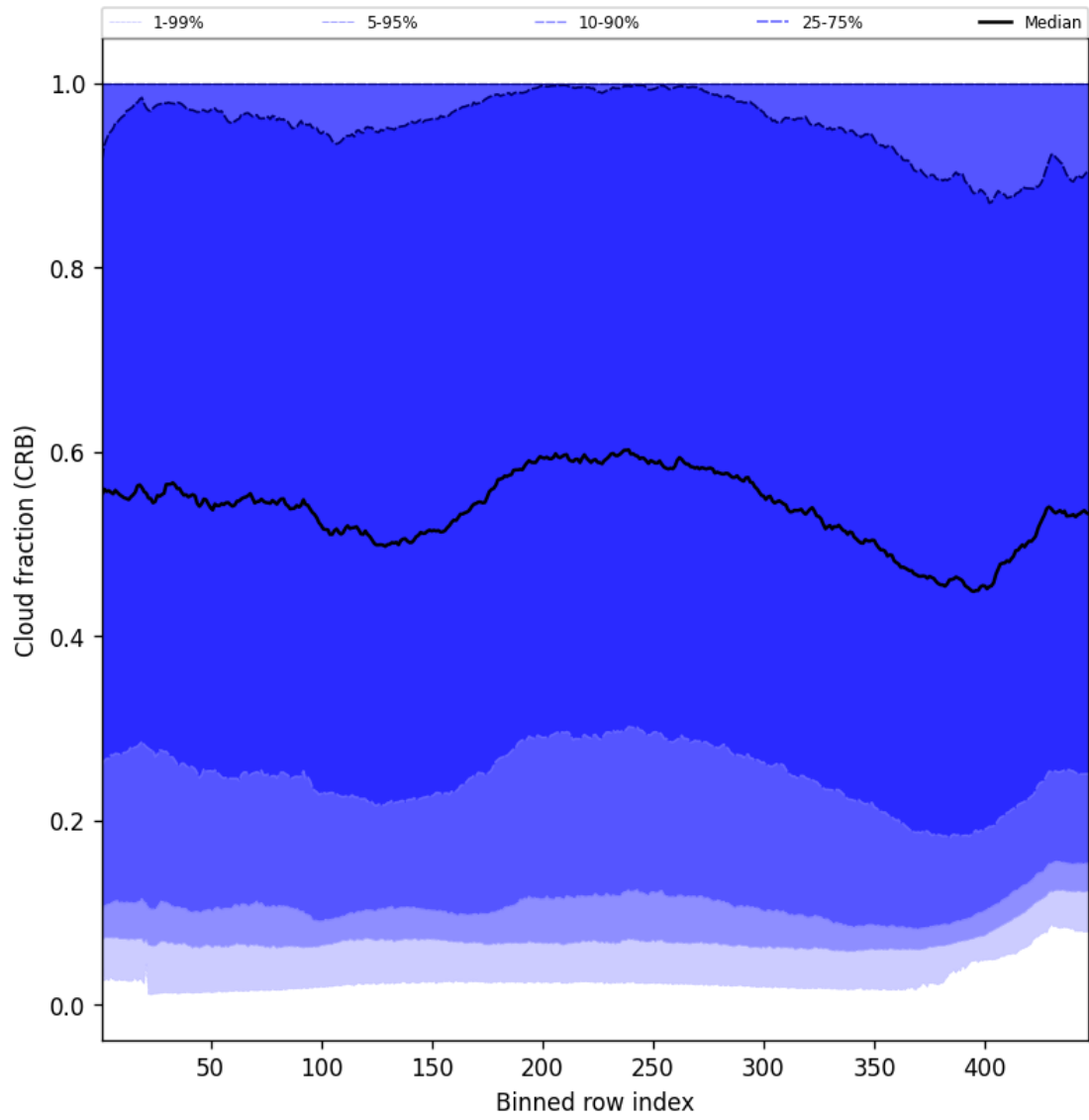
Figure 58: Along track statistics of “Cloud fraction (CRB)” for 2024-10-14 to 2024-10-15
