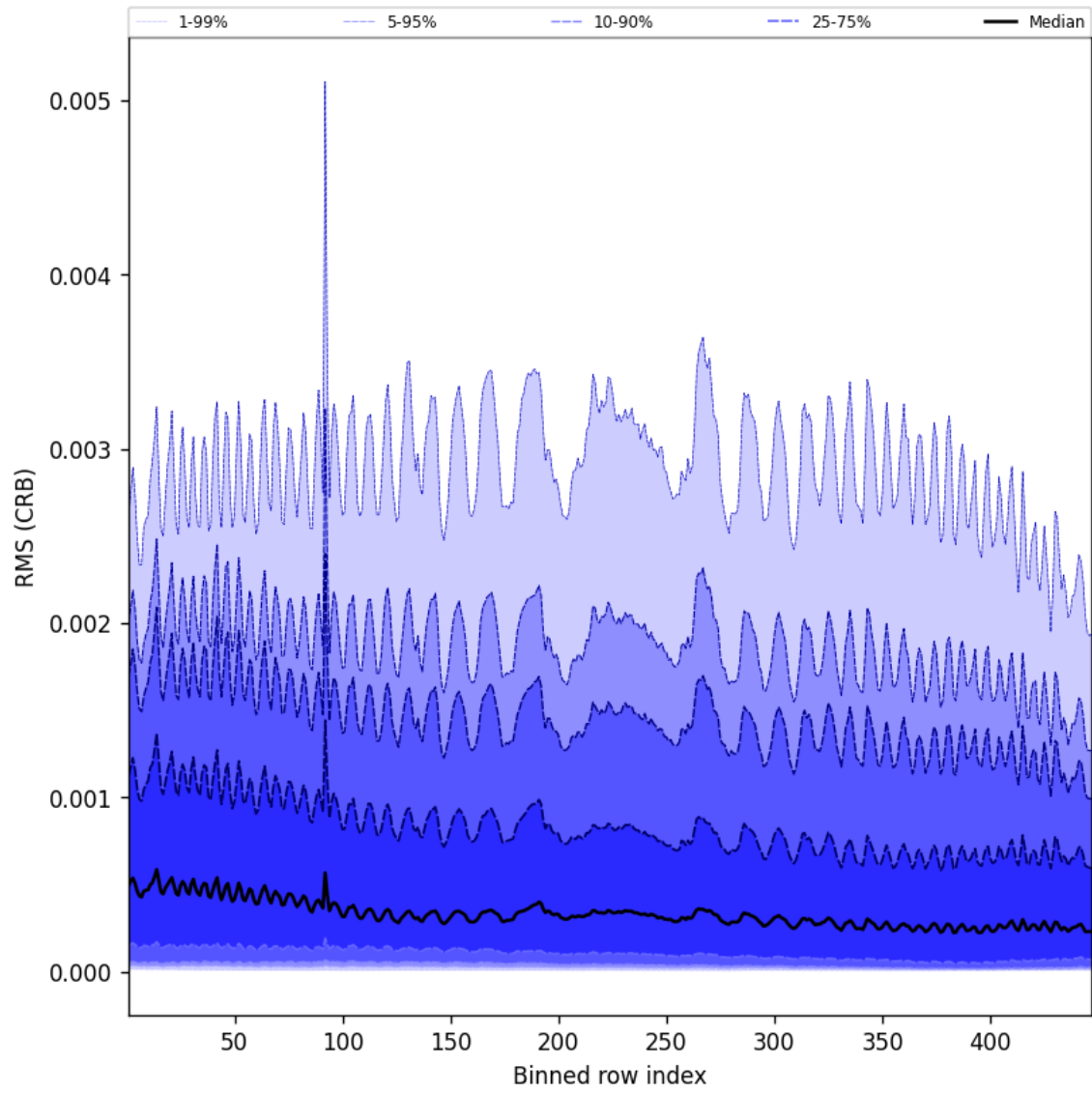
Figure 64: Along track statistics of “RMS (CRB)” for 2024-10-14 to 2024-10-15
