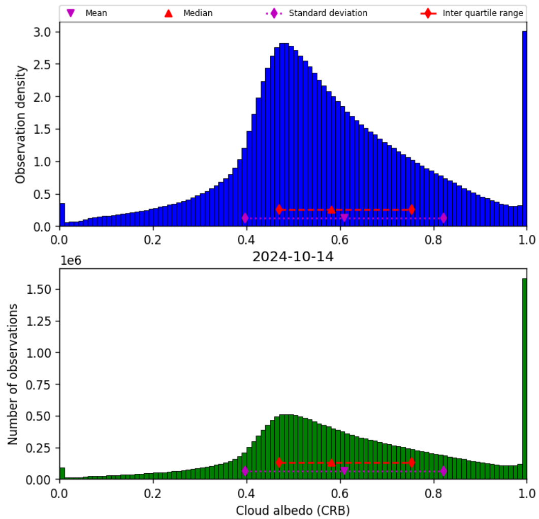
Figure 44: Histogram of “Cloud albedo (CRB)” for 2024-10-14 to 2024-10-15
