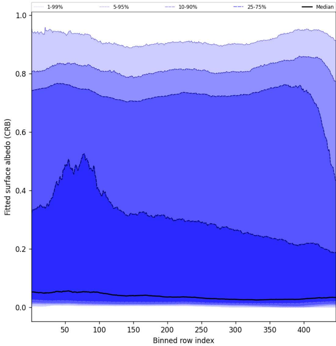
Figure 62: Along track statistics of “Fitted surface albedo (CRB)” for 2024-10-14 to 2024-10-15
