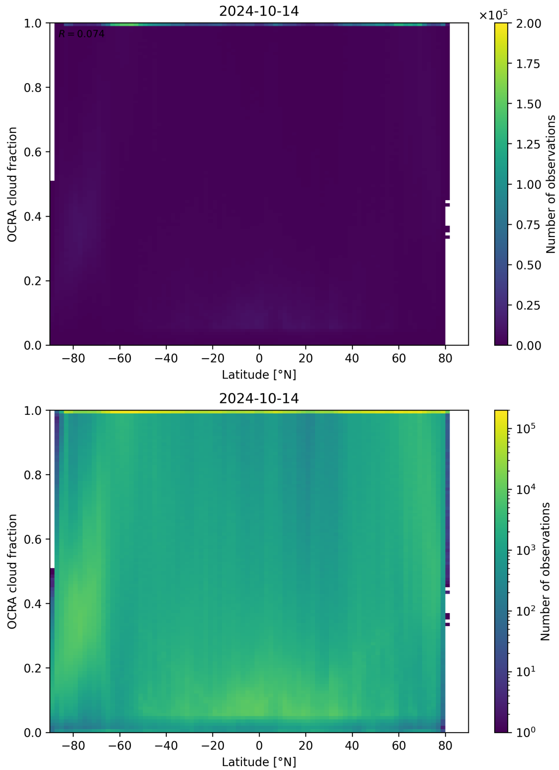
Figure 93: Scatter density plot of “Latitude” against “OCRA cloud fraction” for 2024-10-14 to 2024-10-15.
