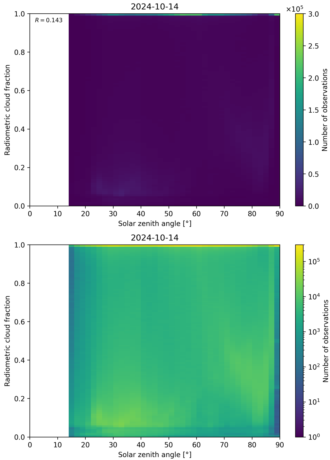
Figure 99: Scatter density plot of “Solar zenith angle” against “Radiometric cloud fraction” for 2024-10-14 to 2024-10-15.
