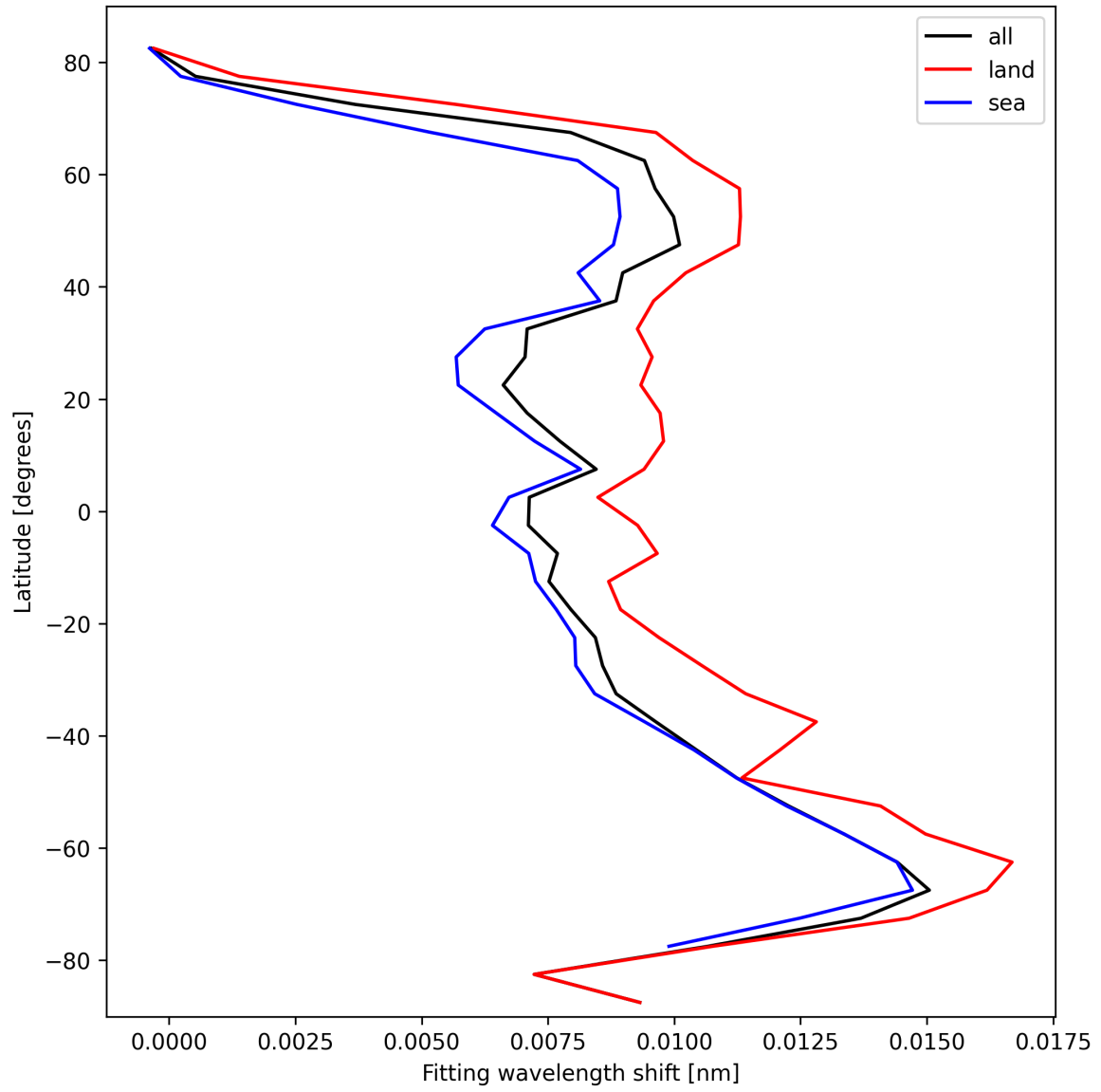
Figure 33: Zonal average of “Fitting wavelength shift” for 2024-10-14 to 2024-10-15.
