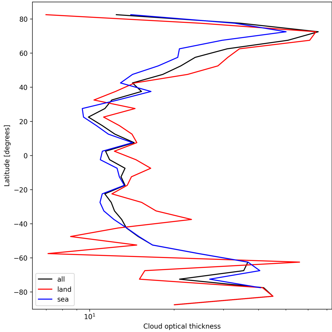
Figure 25: Zonal average of “Cloud optical thickness” for 2024-10-14 to 2024-10-15.
