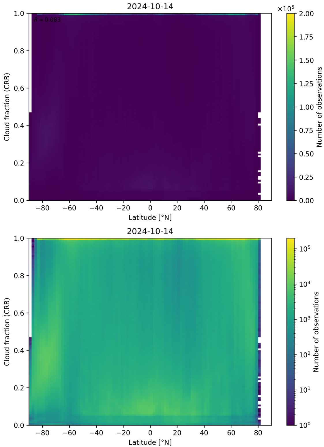
Figure 94: Scatter density plot of “Latitude” against “Cloud fraction (CRB)” for 2024-10-14 to 2024-10-15.
