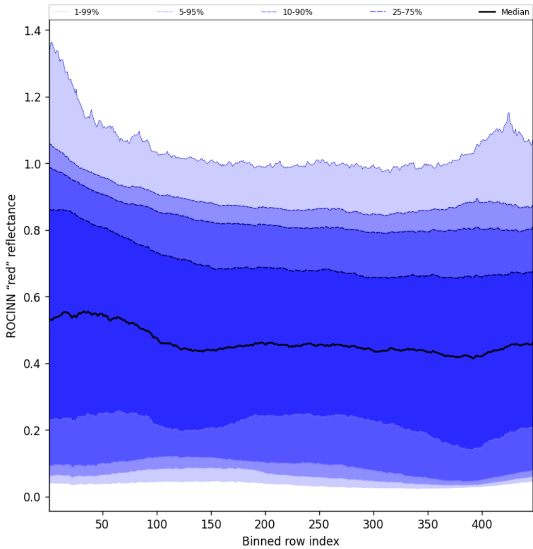
Figure 69: Along track statistics of "ROCINN "red" reflectance" for 2024-10-14 to 2024-10-15
