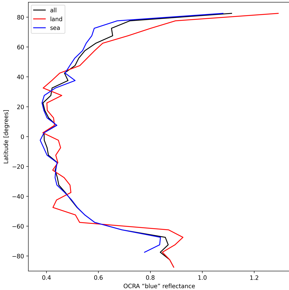
Figure 35: Zonal average of “OCRA “blue” reflectance” for 2024-10-14 to 2024-10-15.
