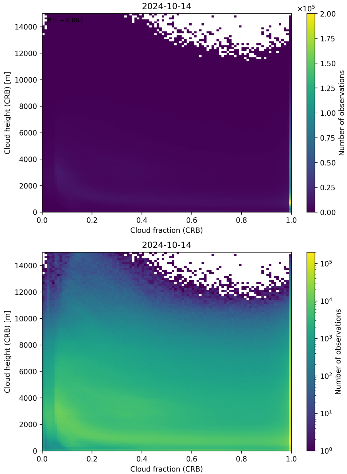
Figure 79: Scatter density plot of “Cloud fraction (CRB)” against “Cloud height (CRB)” for 2024-10-14 to 2024-10-15.
