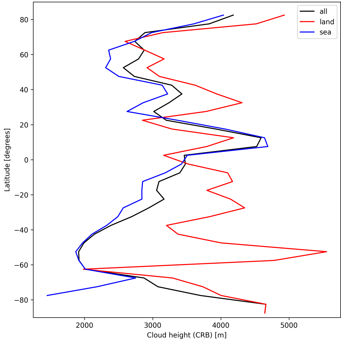
Figure 27: Zonal average of “Cloud height (CRB)” for 2024-10-14 to 2024-10-15.
