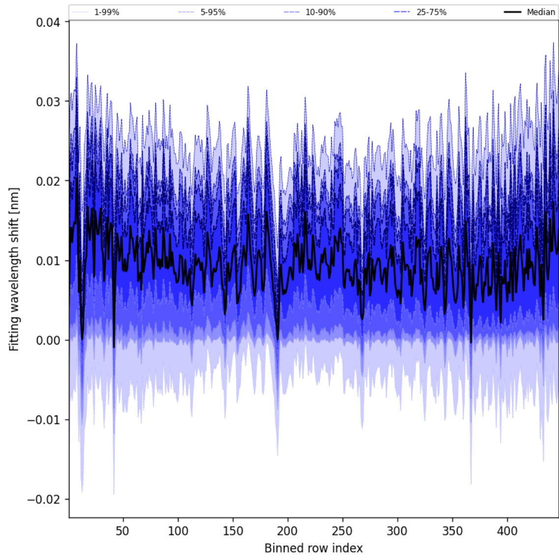
Figure 65: Along track statistics of “Fitting wavelength shift” for 2024-10-14 to 2024-10-15
