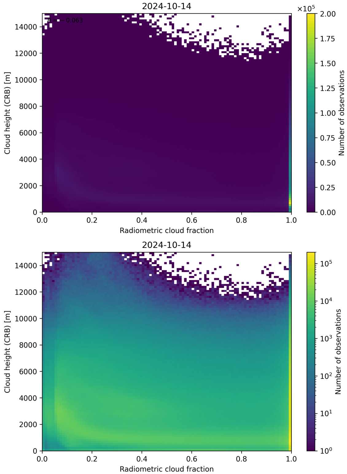
Figure 74: Scatter density plot of “Radiometric cloud fraction” against “Cloud height (CRB)” for 2024-10-14 to 2024-10-15.
