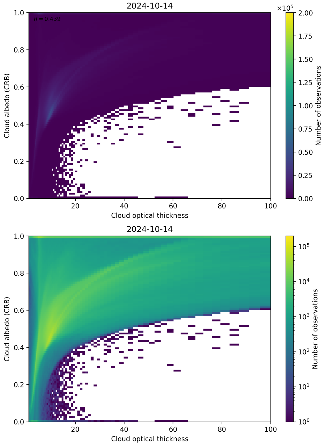
Figure 82: Scatter density plot of “Cloud optical thickness” against “Cloud albedo (CRB)” for 2024-10-14 to 2024-10-15.
