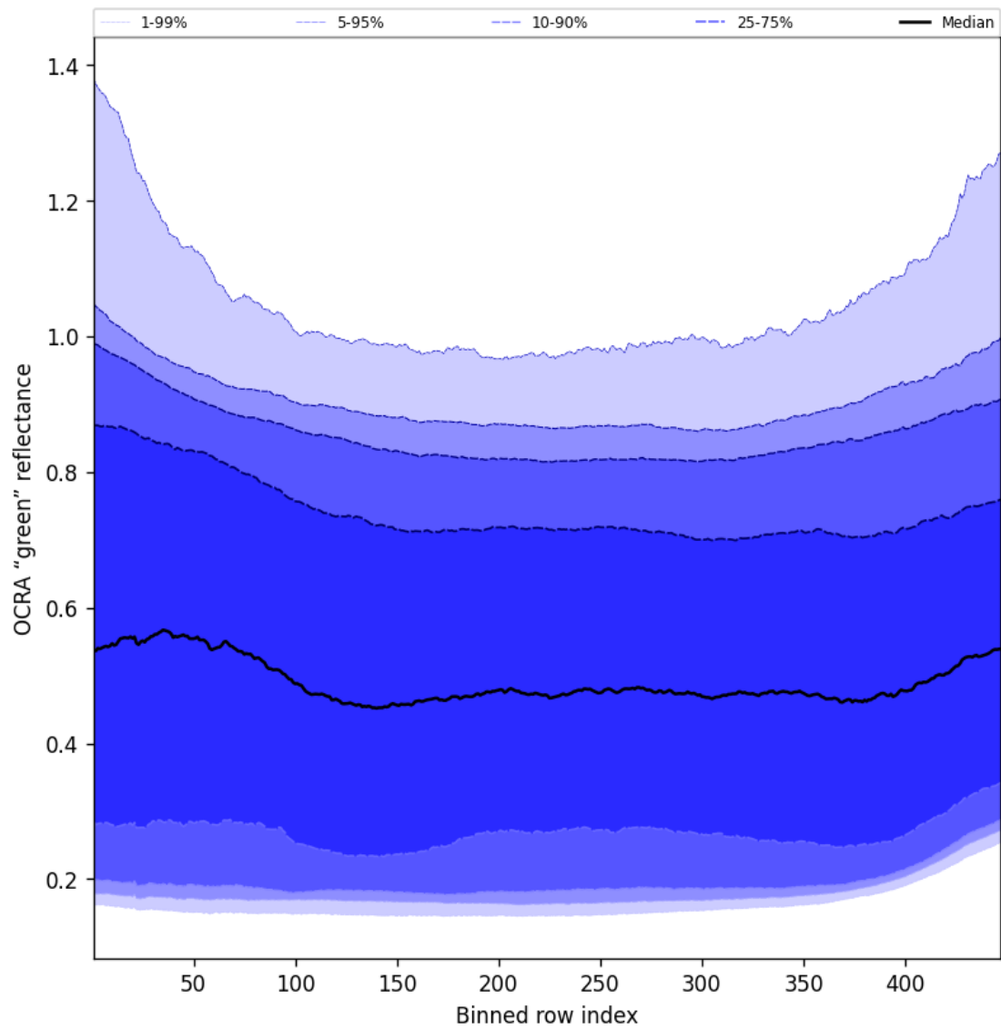
Figure 68: Along track statistics of "OCRA "green" reflectance" for 2024-10-14 to 2024-10-15
