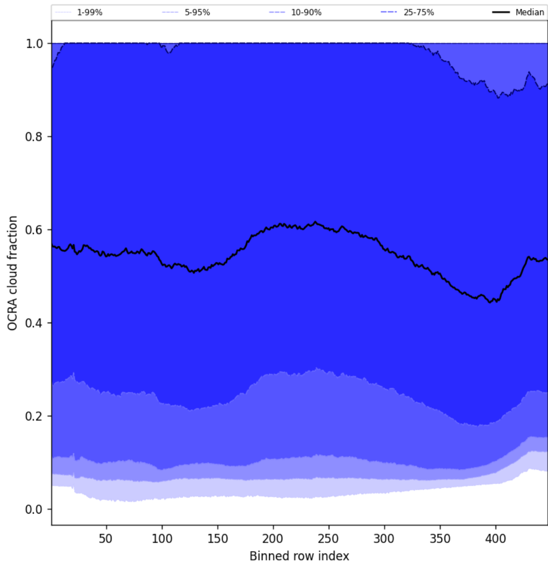
Figure 66: Along track statistics of “OCRA cloud fraction” for 2024-10-14 to 2024-10-15
