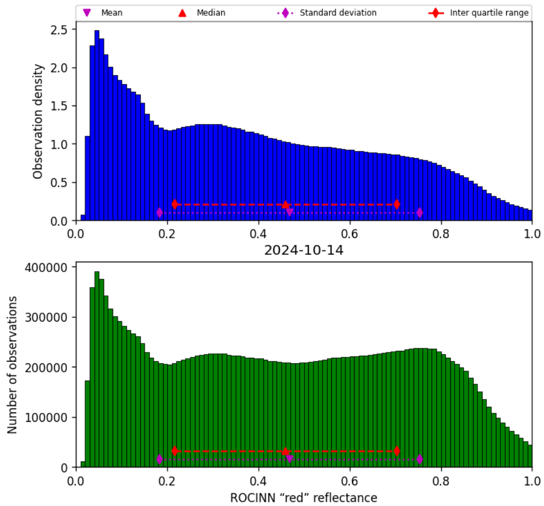
Figure 53: Histogram of “ROCINN “red” reflectance” for 2024-10-14 to 2024-10-15
