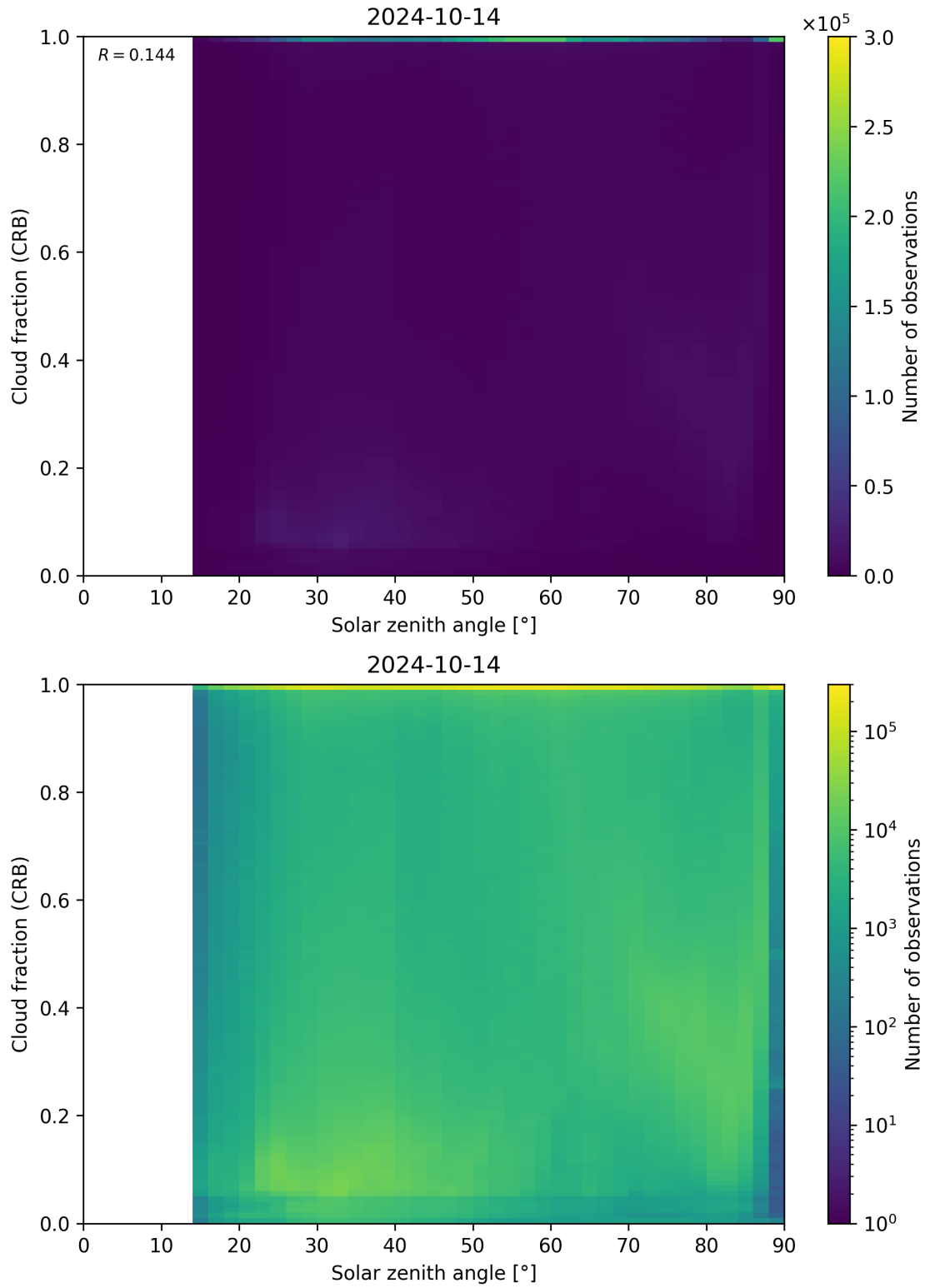
Figure 101: Scatter density plot of “Solar zenith angle” against “Cloud fraction (CRB)” for 2024-10-14 to 2024-10-15.
