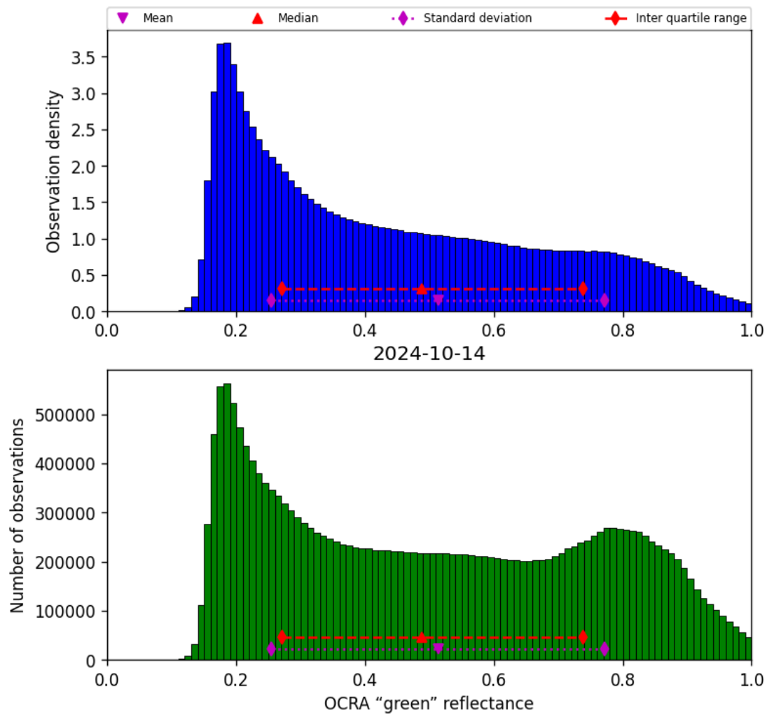
Figure 52: Histogram of “OCRA “green” reflectance” for 2024-10-14 to 2024-10-15
