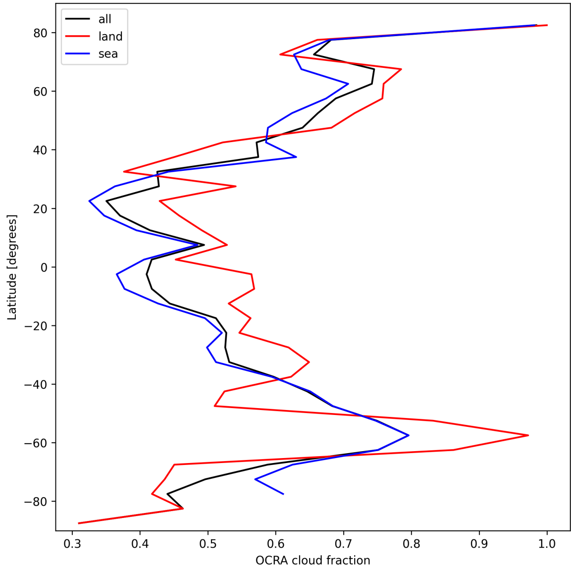
Figure 34: Zonal average of “OCRA cloud fraction” for 2024-10-14 to 2024-10-15.
