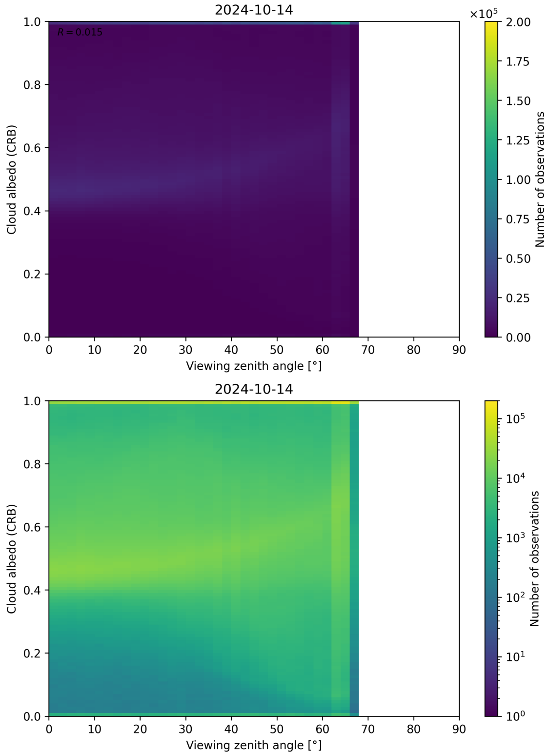
Figure 106: Scatter density plot of “Viewing zenith angle” against “Cloud albedo (CRB)” for 2024-10-14 to 2024-10-15.
