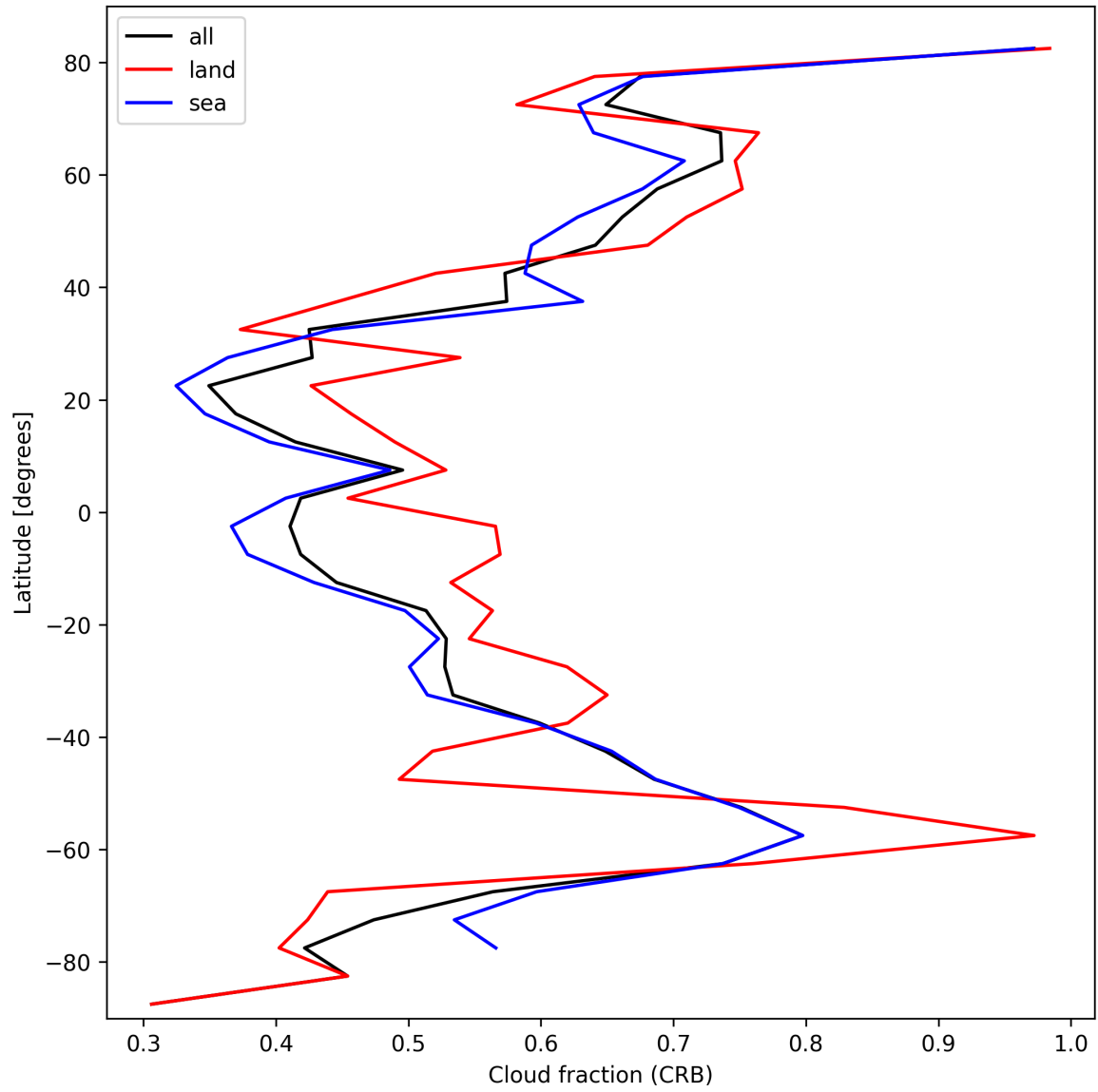
Figure 26: Zonal average of “Cloud fraction (CRB)” for 2024-10-14 to 2024-10-15.
