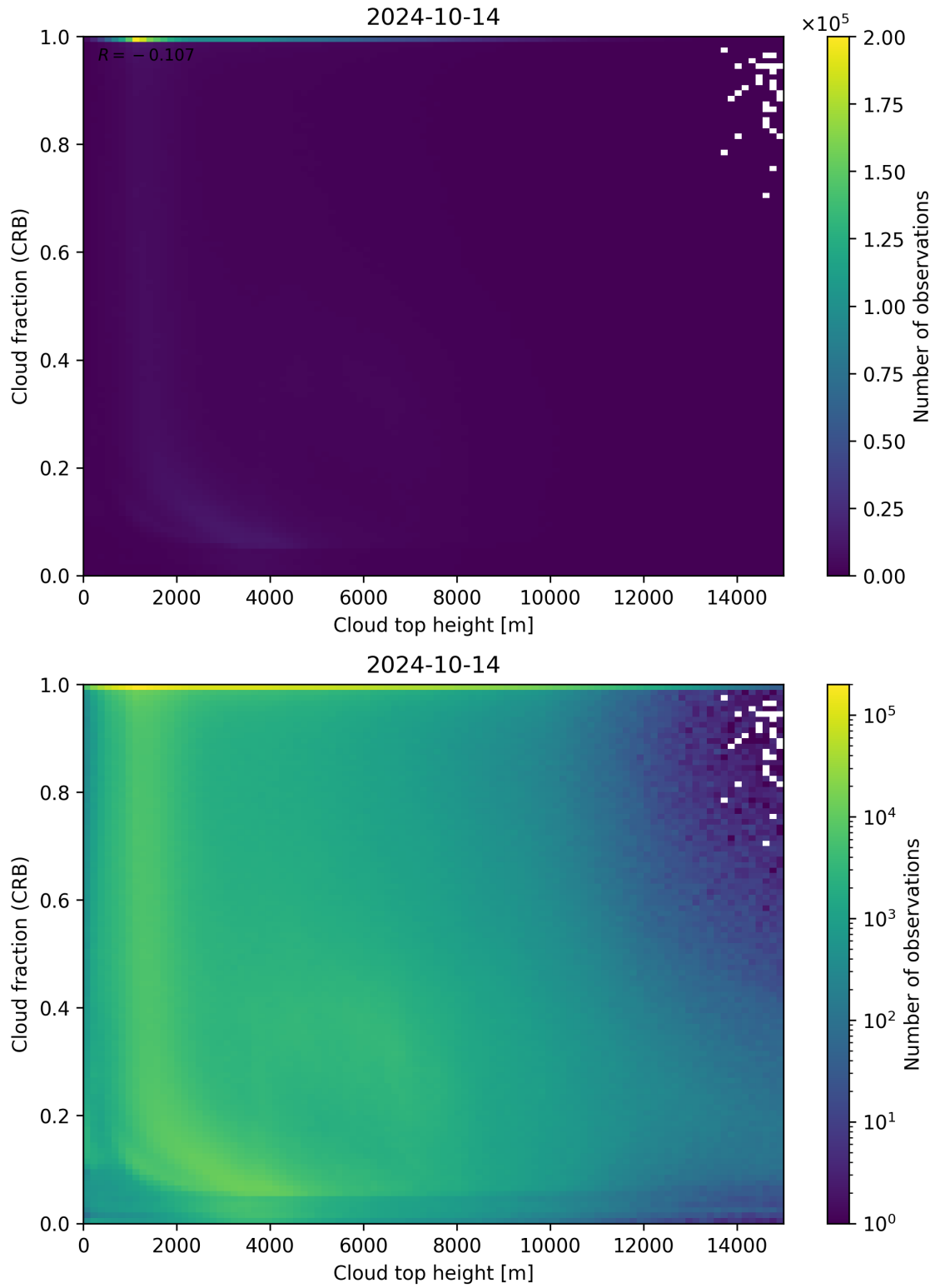
Figure 88: Scatter density plot of “Cloud top height” against “Cloud fraction (CRB)” for 2024-10-14 to 2024-10-15.
