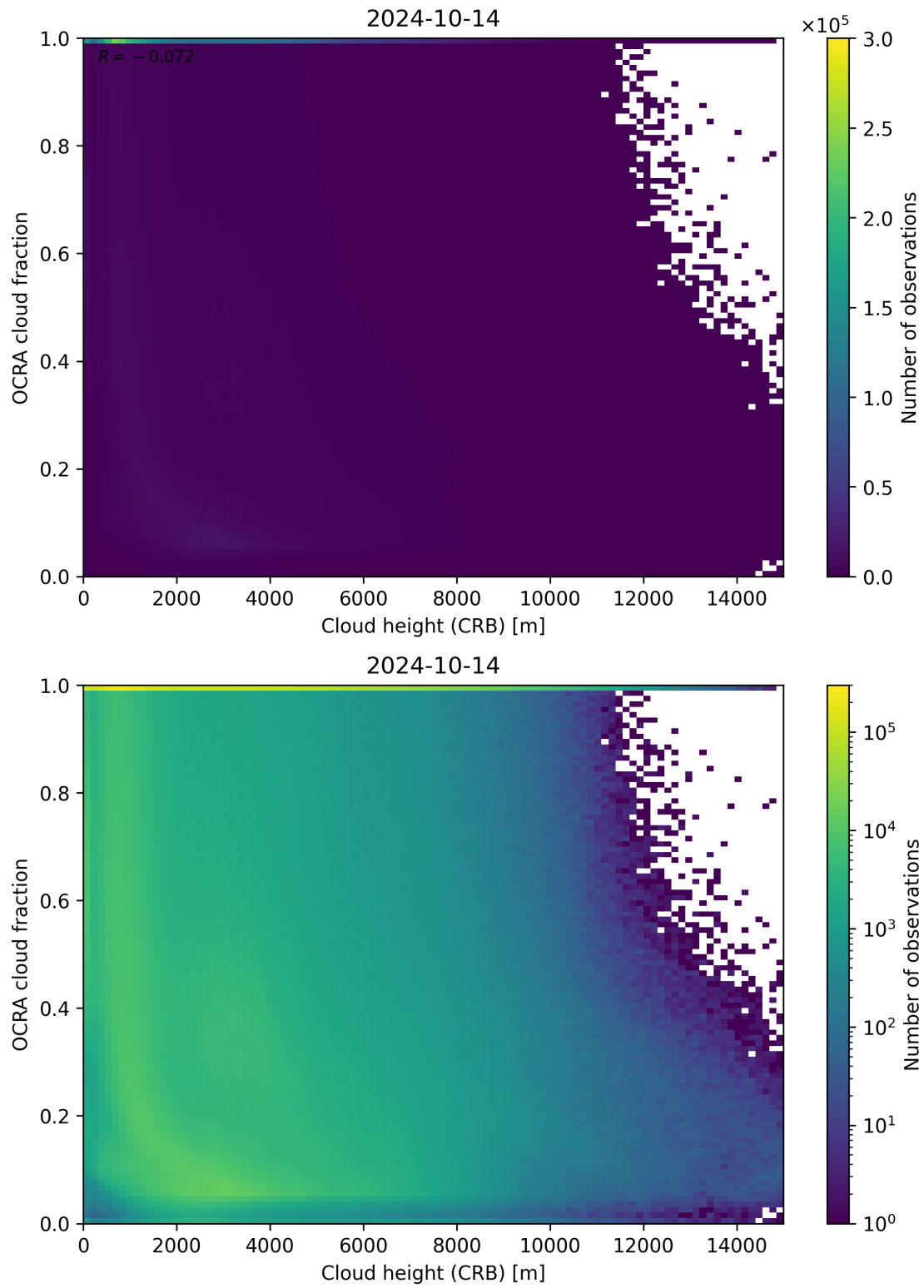
Figure 81: Scatter density plot of “Cloud height (CRB)” against “OCRA cloud fraction” for 2024-10-14 to 2024-10-15.
