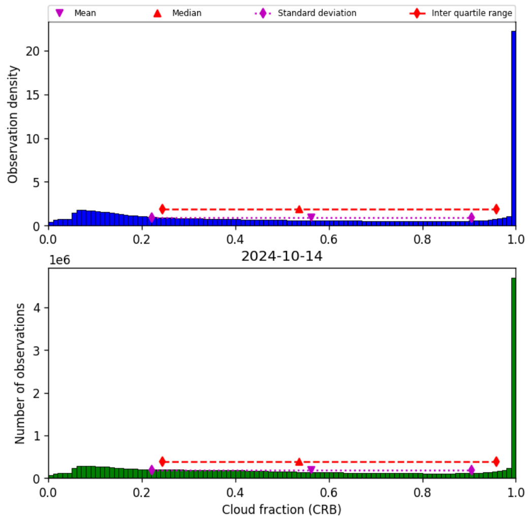
Figure 42: Histogram of “Cloud fraction (CRB)” for 2024-10-14 to 2024-10-15
