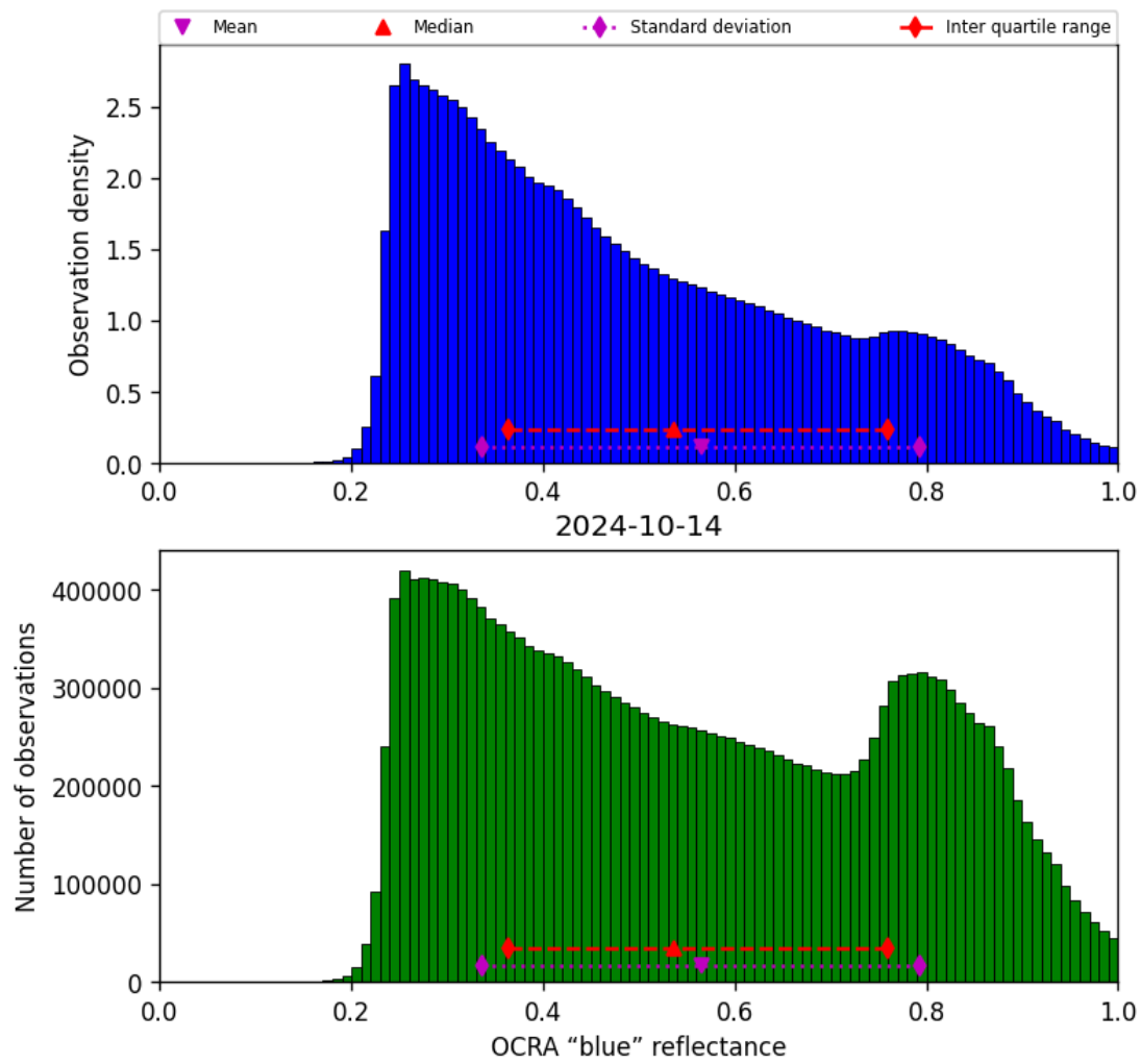
Figure 51: Histogram of “OCRA “blue” reflectance” for 2024-10-14 to 2024-10-15
