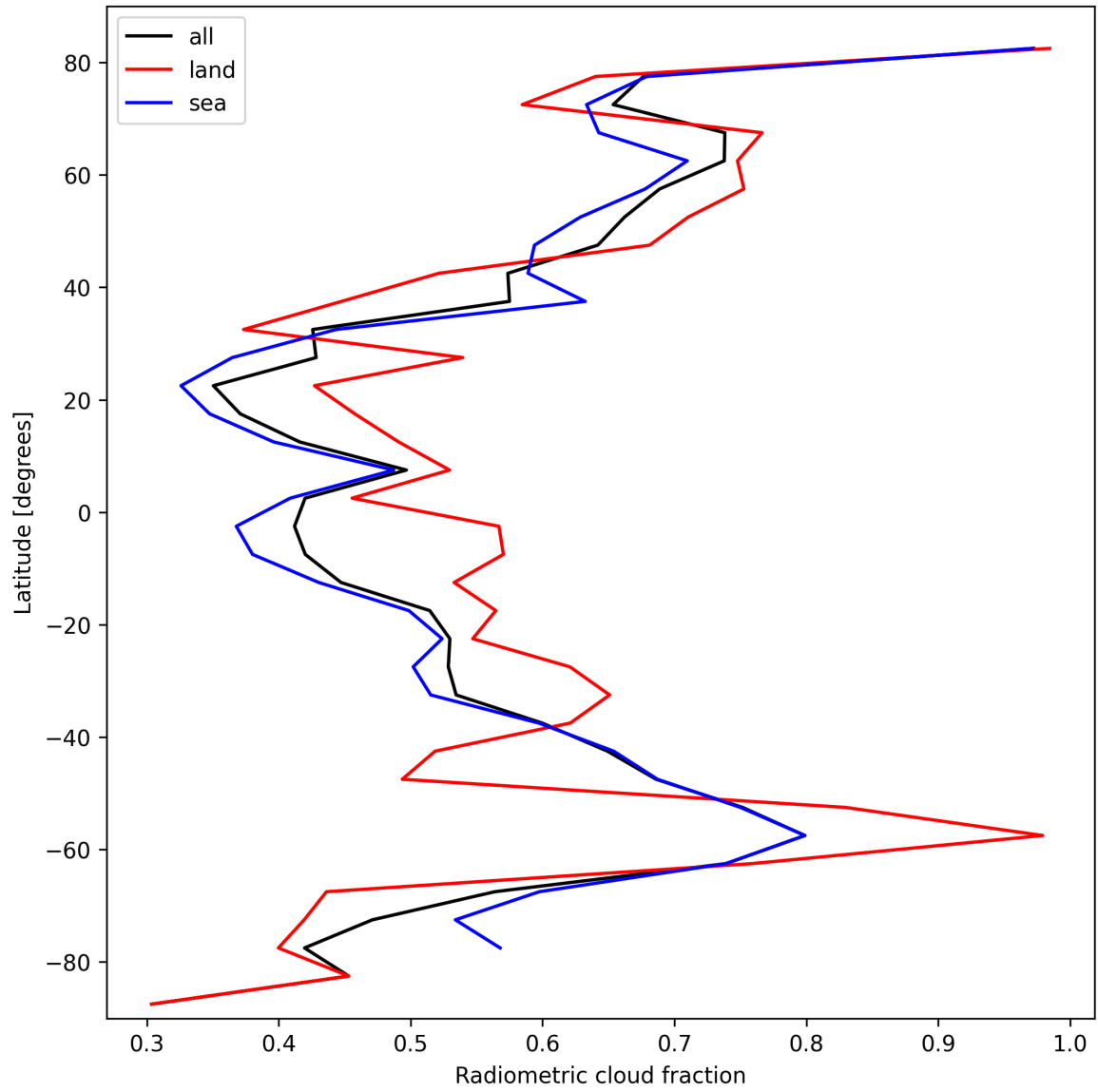
Figure 23: Zonal average of “Radiometric cloud fraction” for 2024-10-14 to 2024-10-15.
