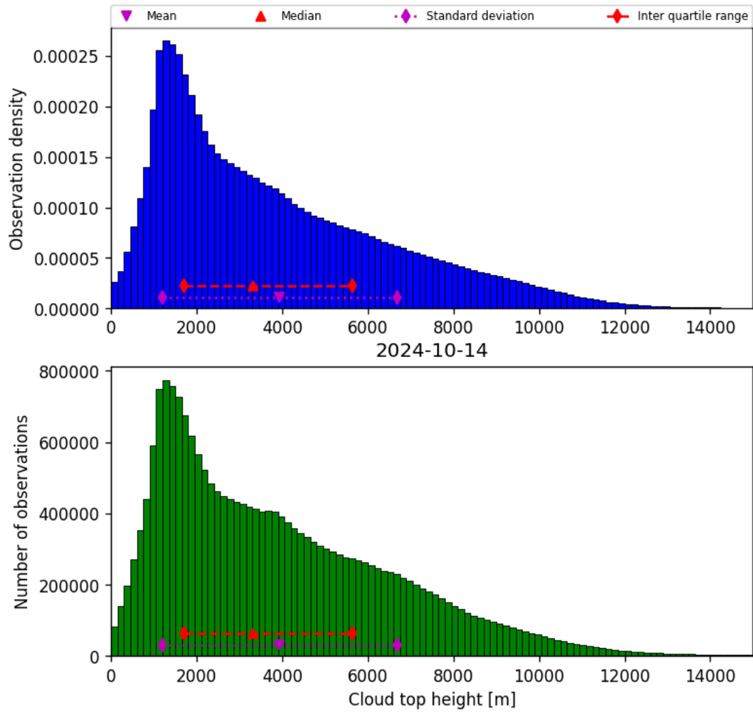
Figure 40: Histogram of “Cloud top height” for 2024-10-14 to 2024-10-15
