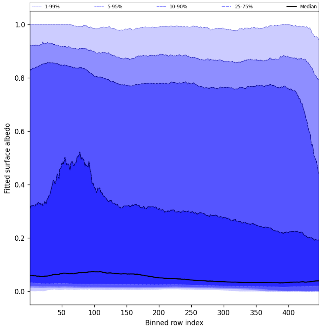
Figure 61: Along track statistics of “Fitted surface albedo” for 2024-10-14 to 2024-10-15
