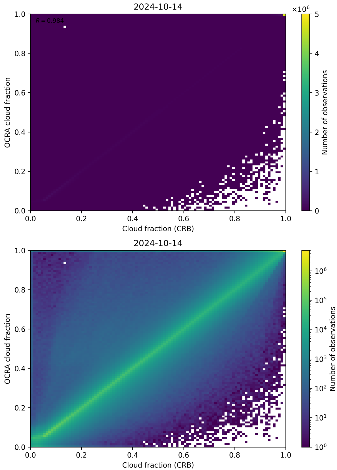
Figure 78: Scatter density plot of “Cloud fraction (CRB)” against “OCRA cloud fraction” for 2024-10-14 to 2024-10-15.
