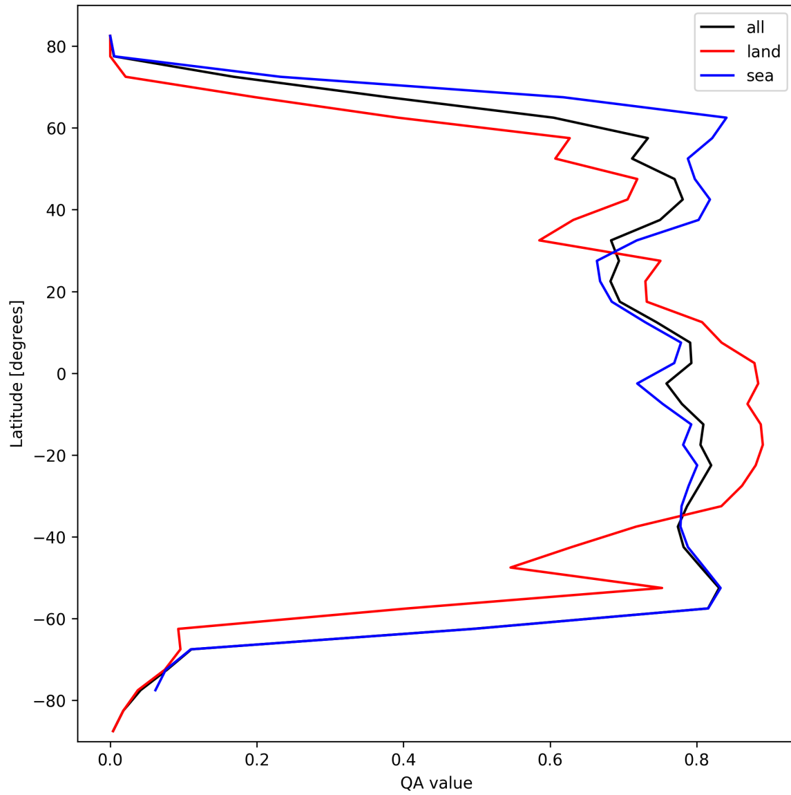
Figure 22: Zonal average of “QA value” for 2024-10-14 to 2024-10-15.
