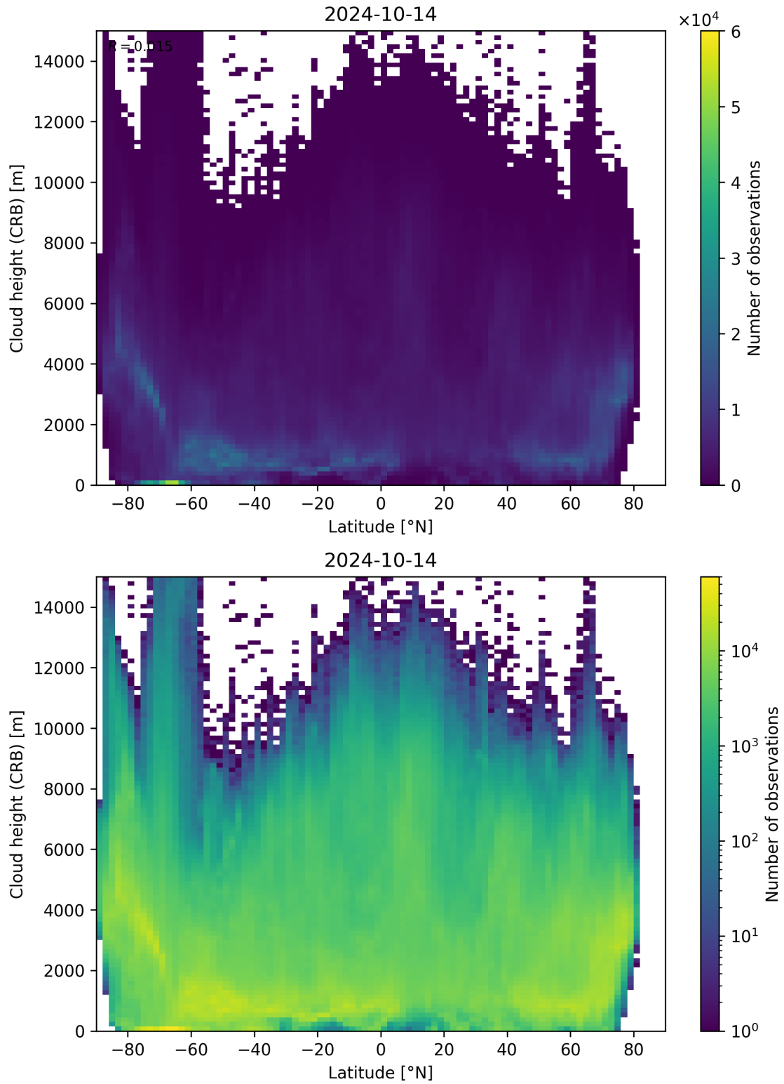
Figure 95: Scatter density plot of “Latitude” against “Cloud height (CRB)” for 2024-10-14 to 2024-10-15.
