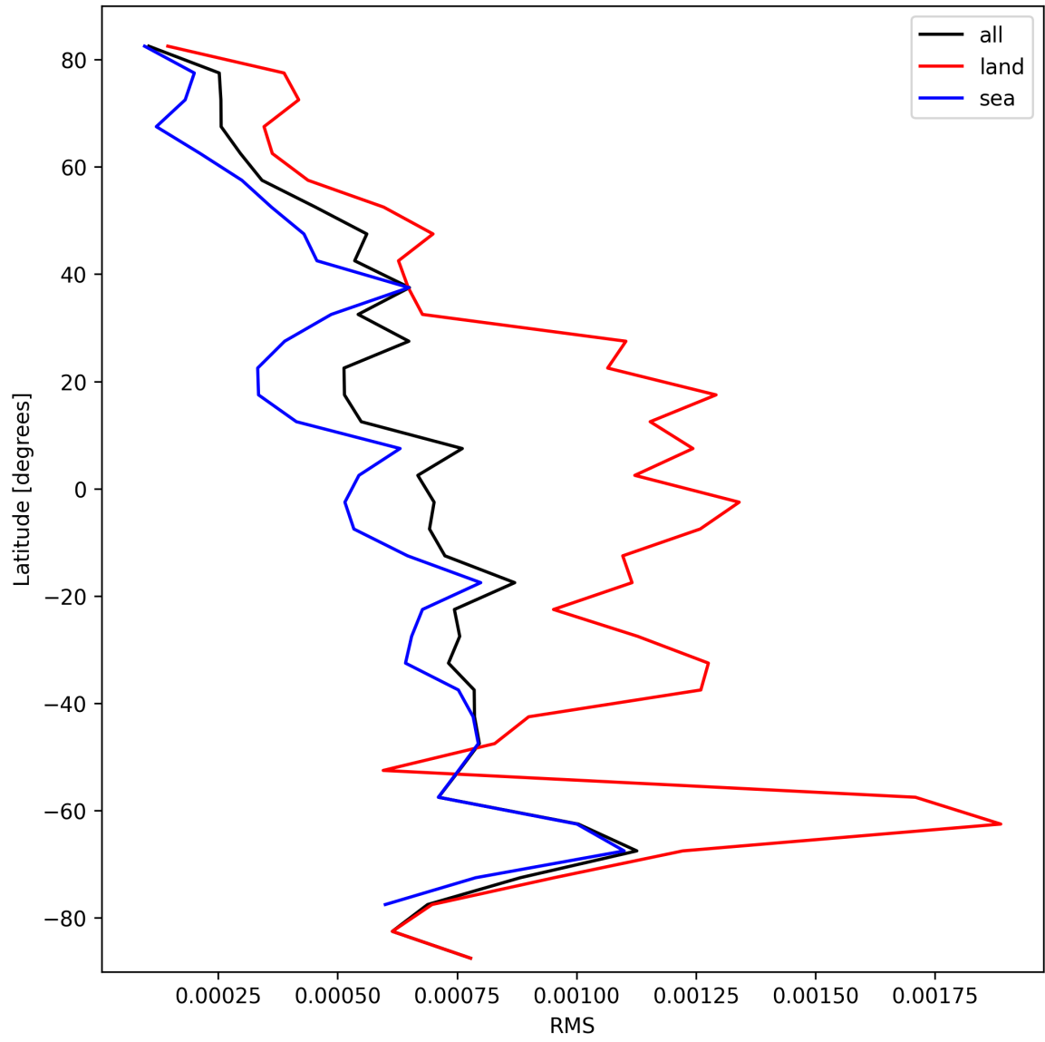
Figure 31: Zonal average of “RMS” for 2024-10-14 to 2024-10-15.
