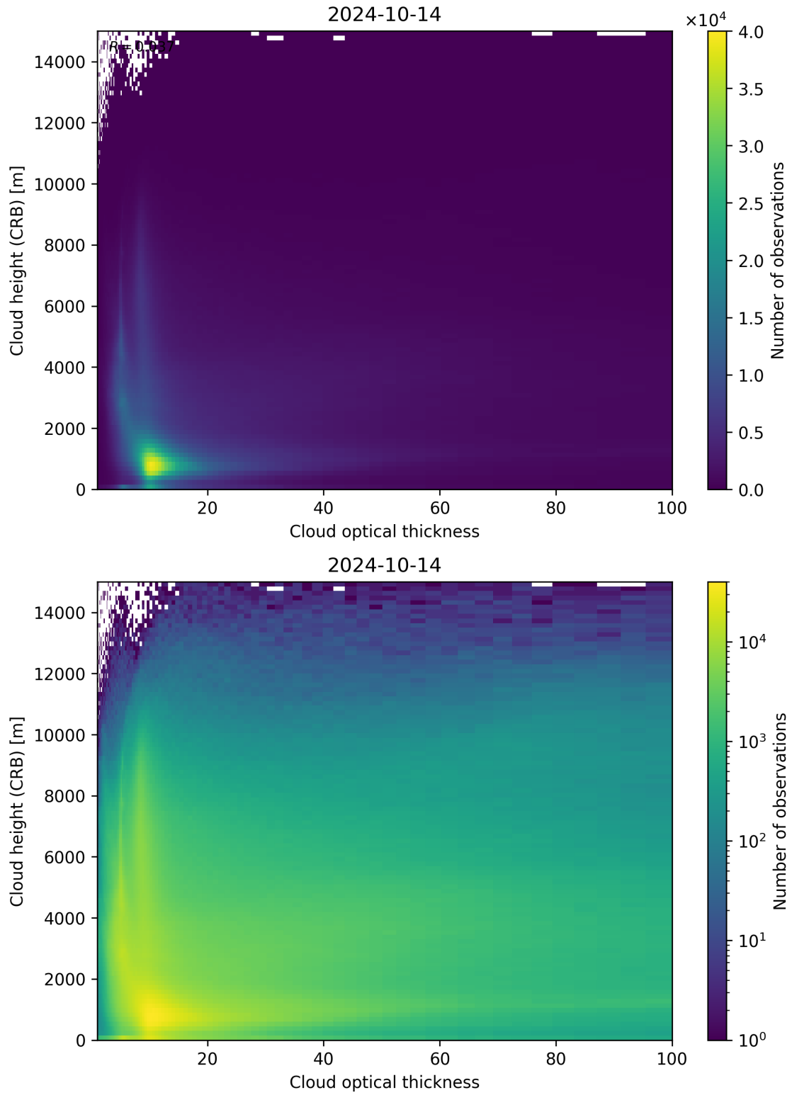
Figure 85: Scatter density plot of “Cloud optical thickness” against “Cloud height (CRB)” for 2024-10-14 to 2024-10-15.
