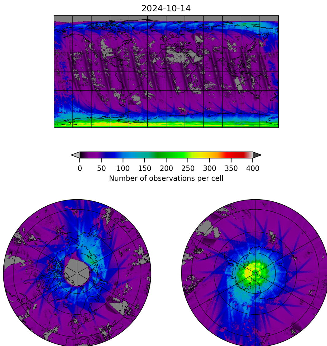
Figure 21: Map of the number of observations for 2024-10-14 to 2024-10-15
