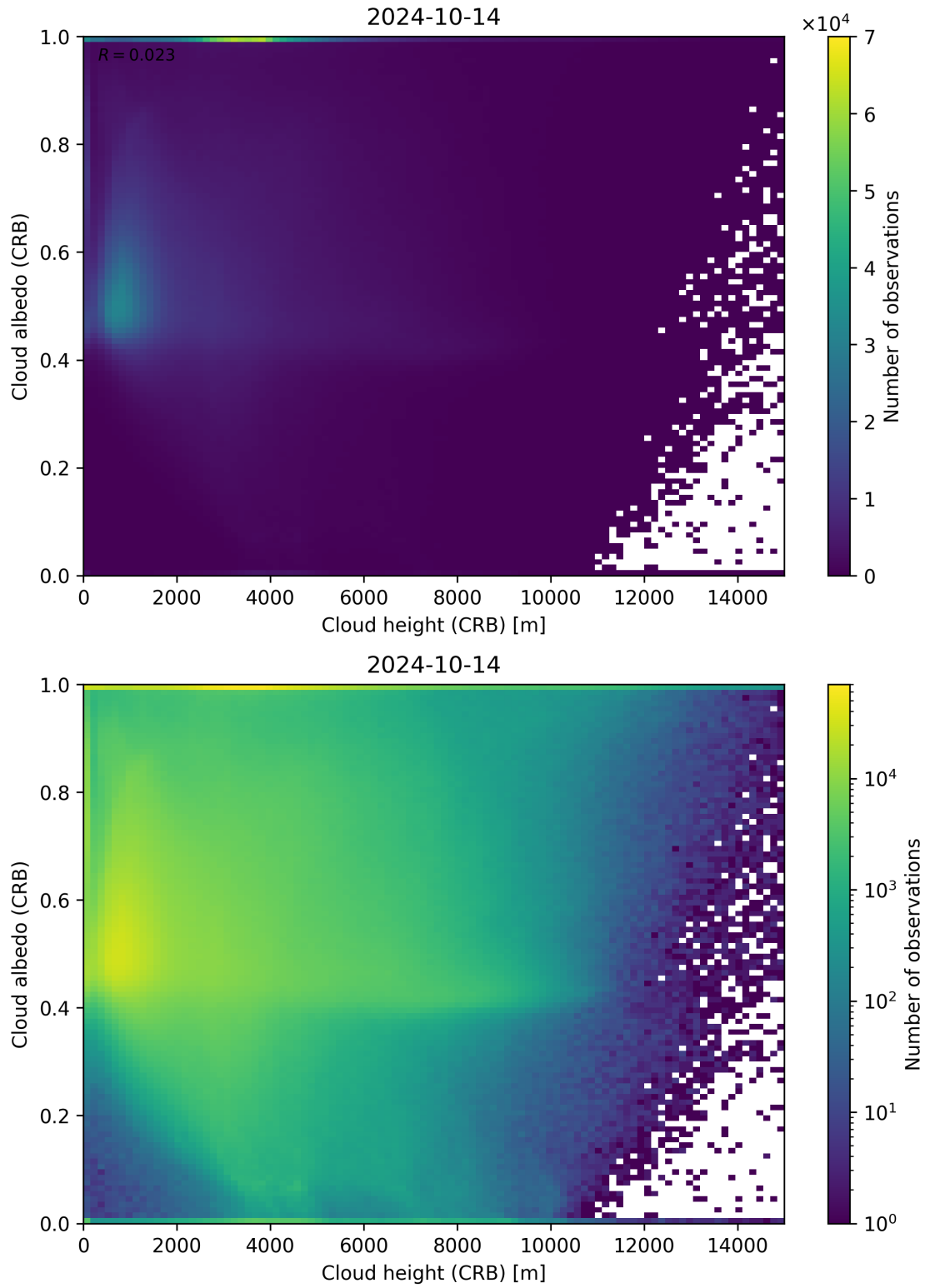
Figure 80: Scatter density plot of “Cloud height (CRB)” against “Cloud albedo (CRB)” for 2024-10-14 to 2024-10-15.
