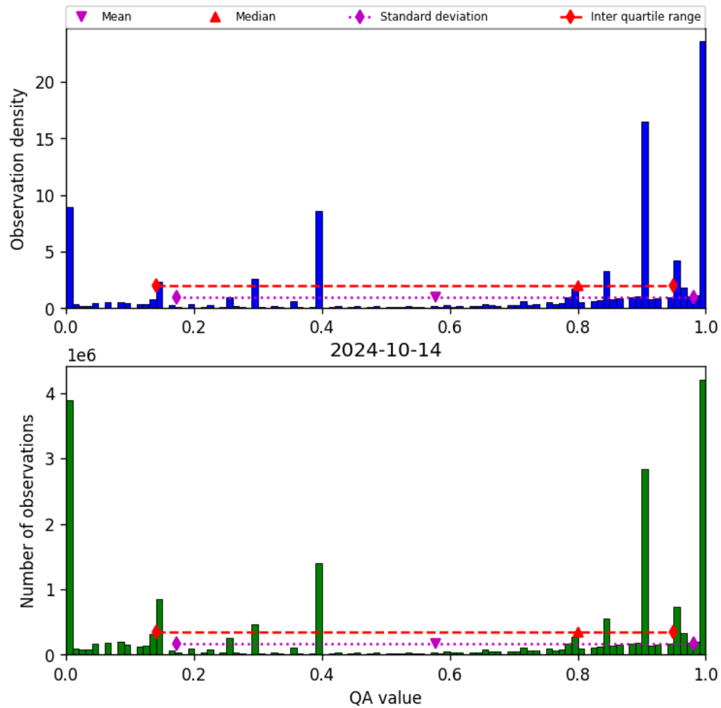
Figure 38: Histogram of “QA value” for 2024-10-14 to 2024-10-15
