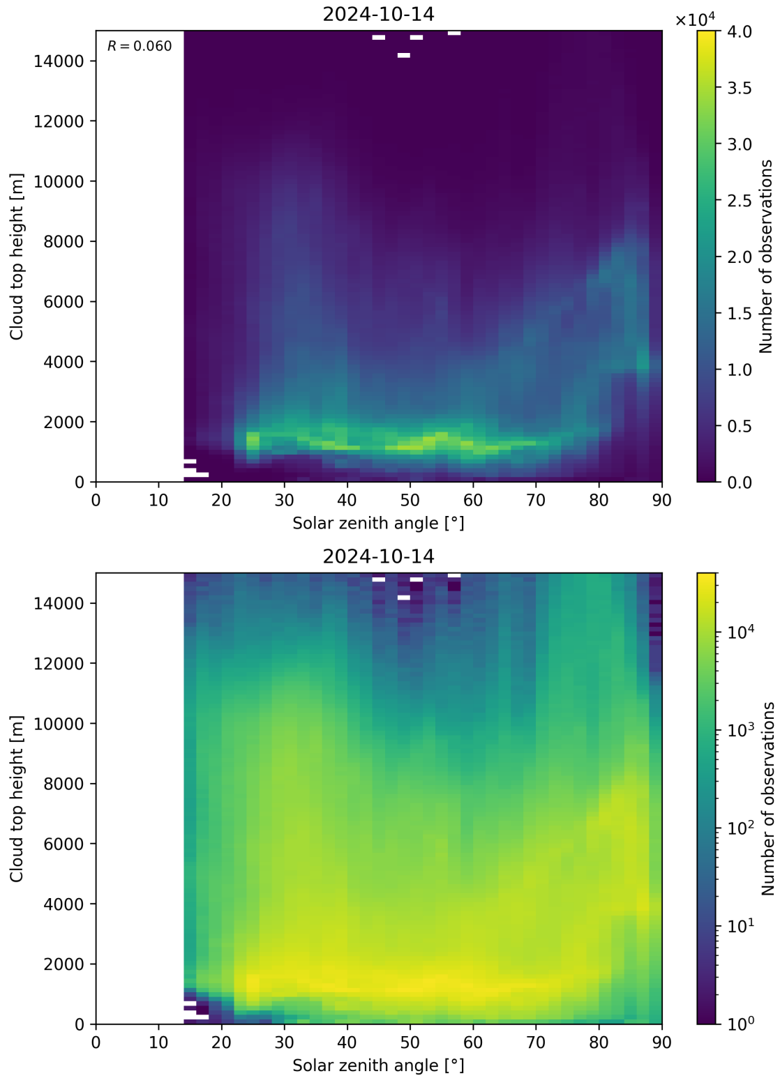
Figure 104: Scatter density plot of “Solar zenith angle” against “Cloud top height” for 2024-10-14 to 2024-10-15.
