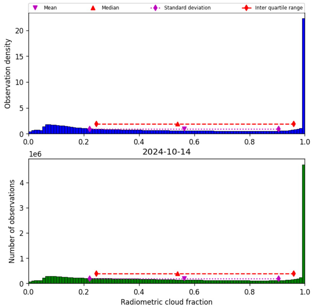
Figure 39: Histogram of “Radiometric cloud fraction” for 2024-10-14 to 2024-10-15
