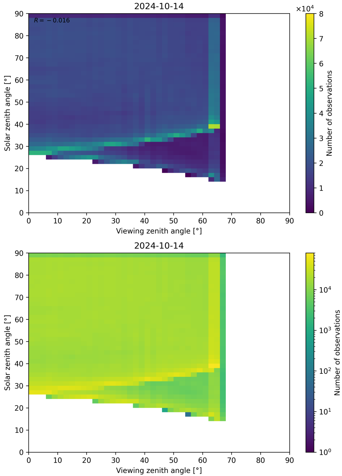
Figure 114: Scatter density plot of “Viewing zenith angle” against “Solar zenith angle” for 2024-10-14 to 2024-10-15.
