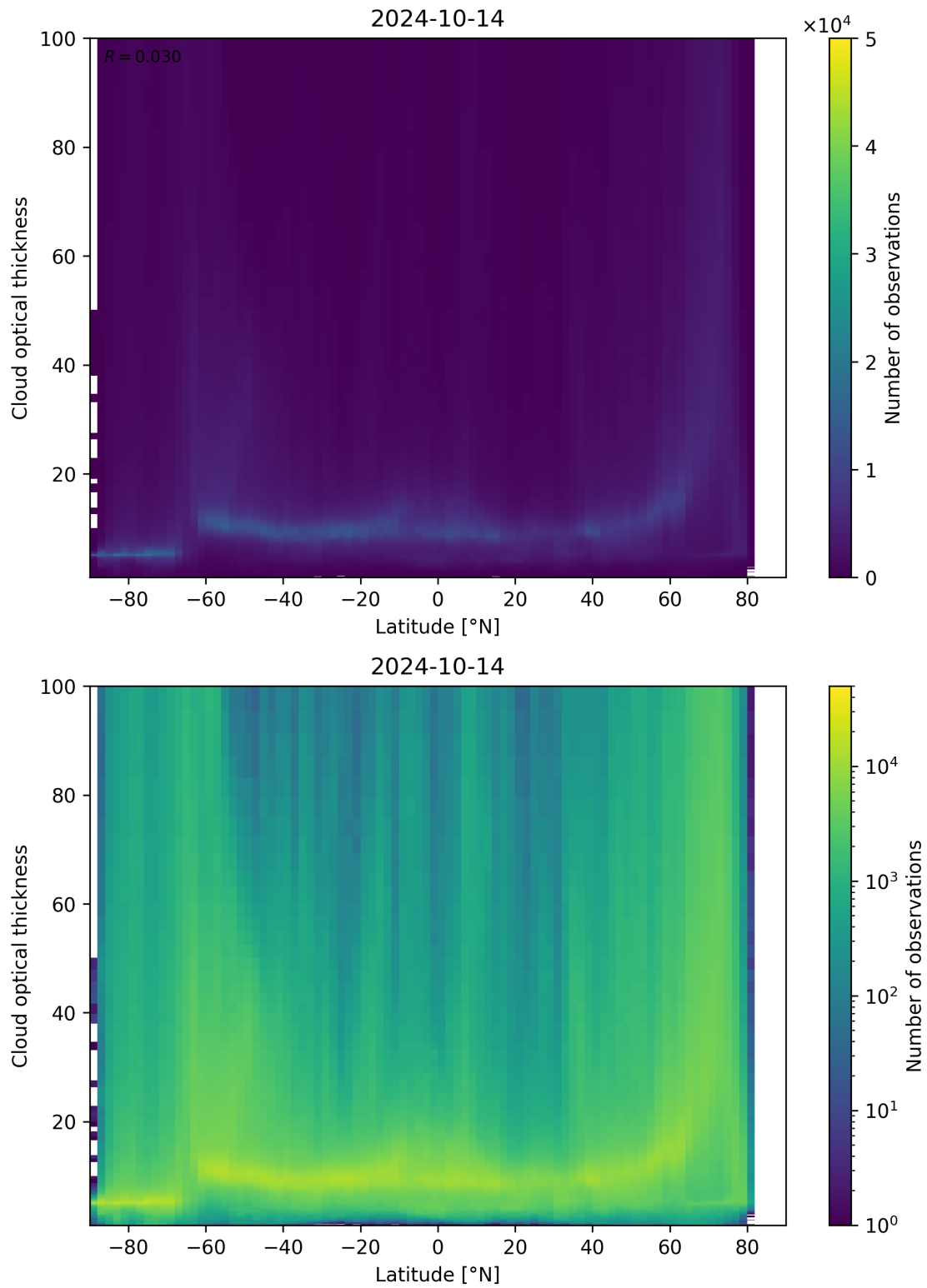
Figure 96: Scatter density plot of “Latitude” against “Cloud optical thickness” for 2024-10-14 to 2024-10-15.
