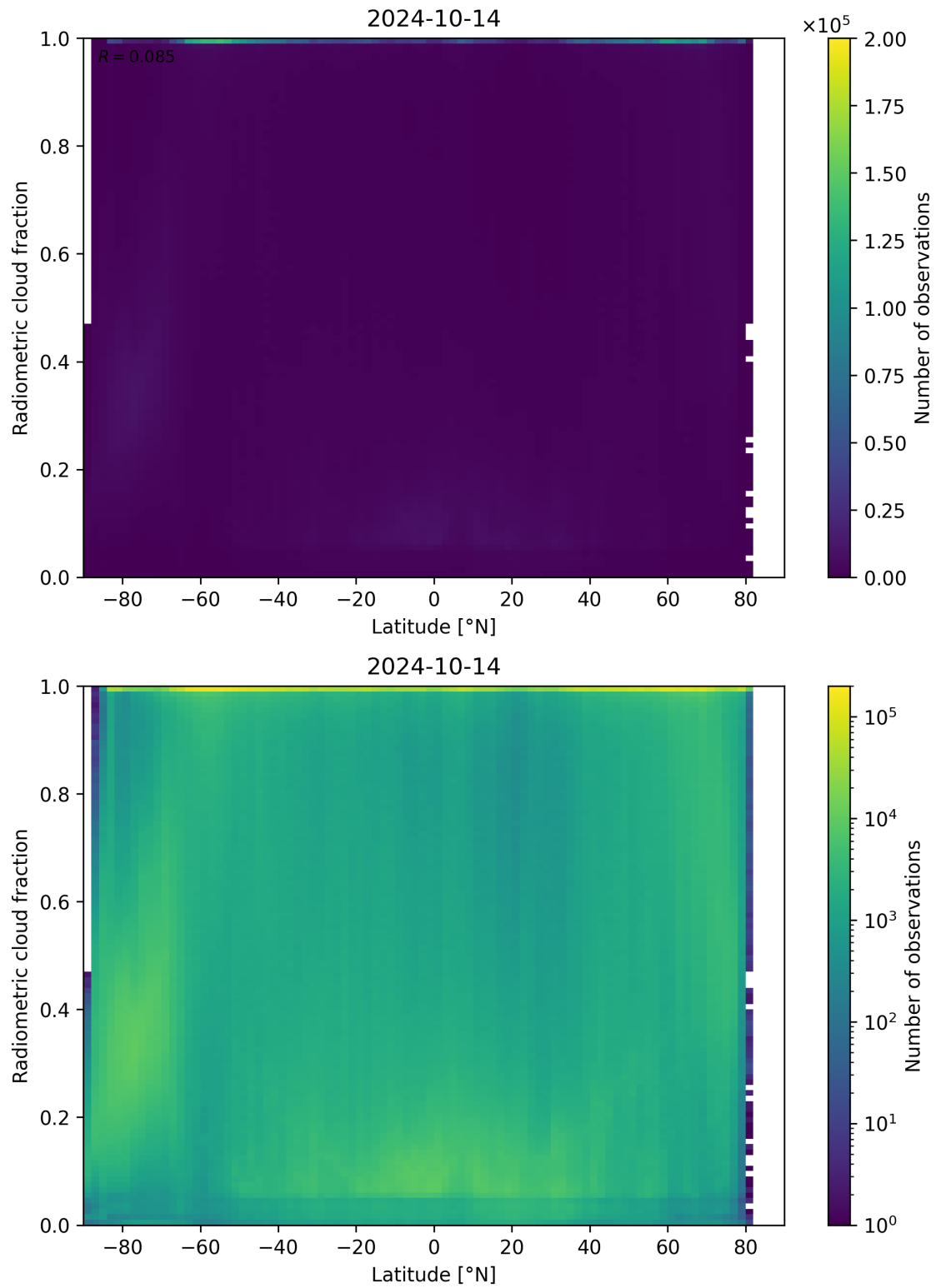
Figure 92: Scatter density plot of “Latitude” against “Radiometric cloud fraction” for 2024-10-14 to 2024-10-15.
