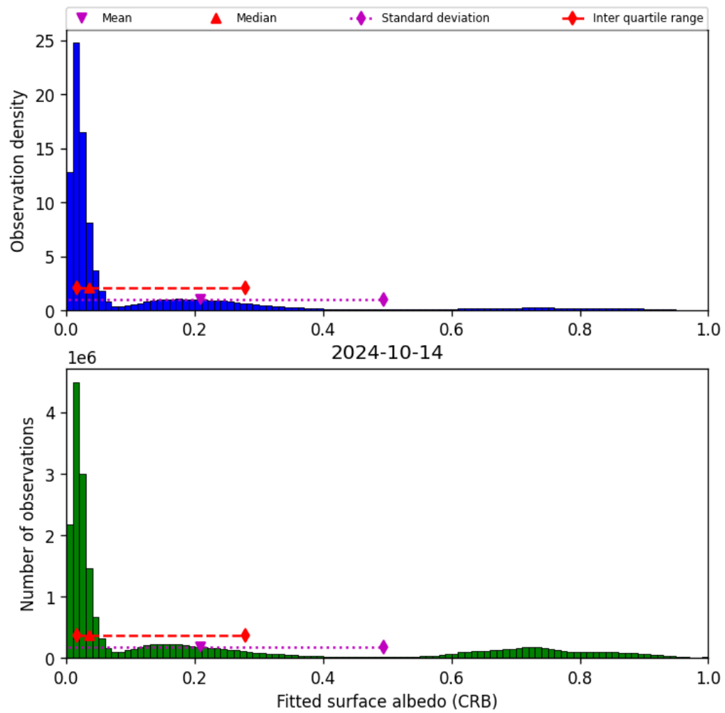
Figure 46: Histogram of “Fitted surface albedo (CRB)” for 2024-10-14 to 2024-10-15
