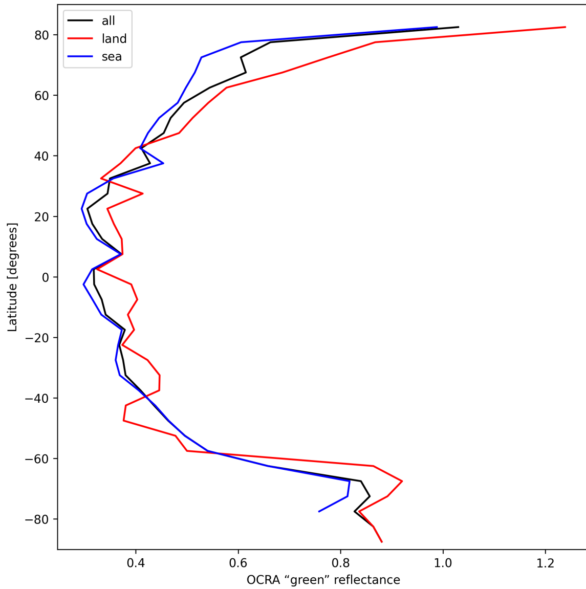
Figure 36: Zonal average of “OCRA “green” reflectance” for 2024-10-14 to 2024-10-15.
