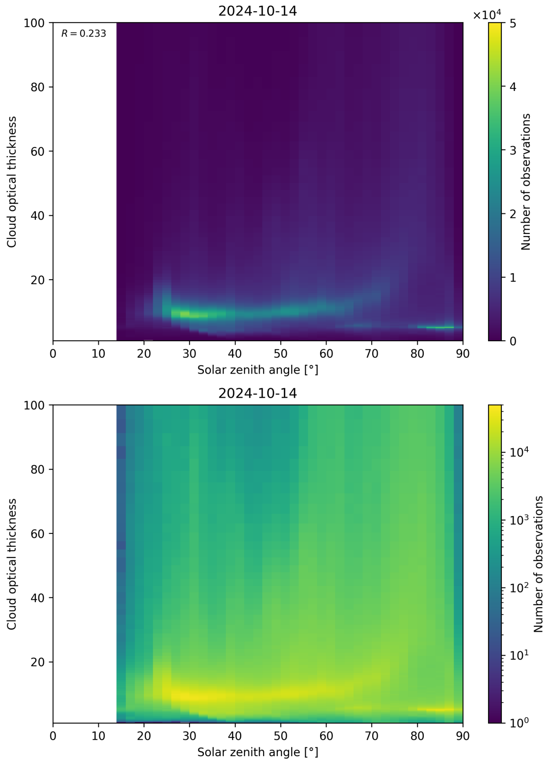
Figure 103: Scatter density plot of “Solar zenith angle” against “Cloud optical thickness” for 2024-10-14 to 2024-10-15.
