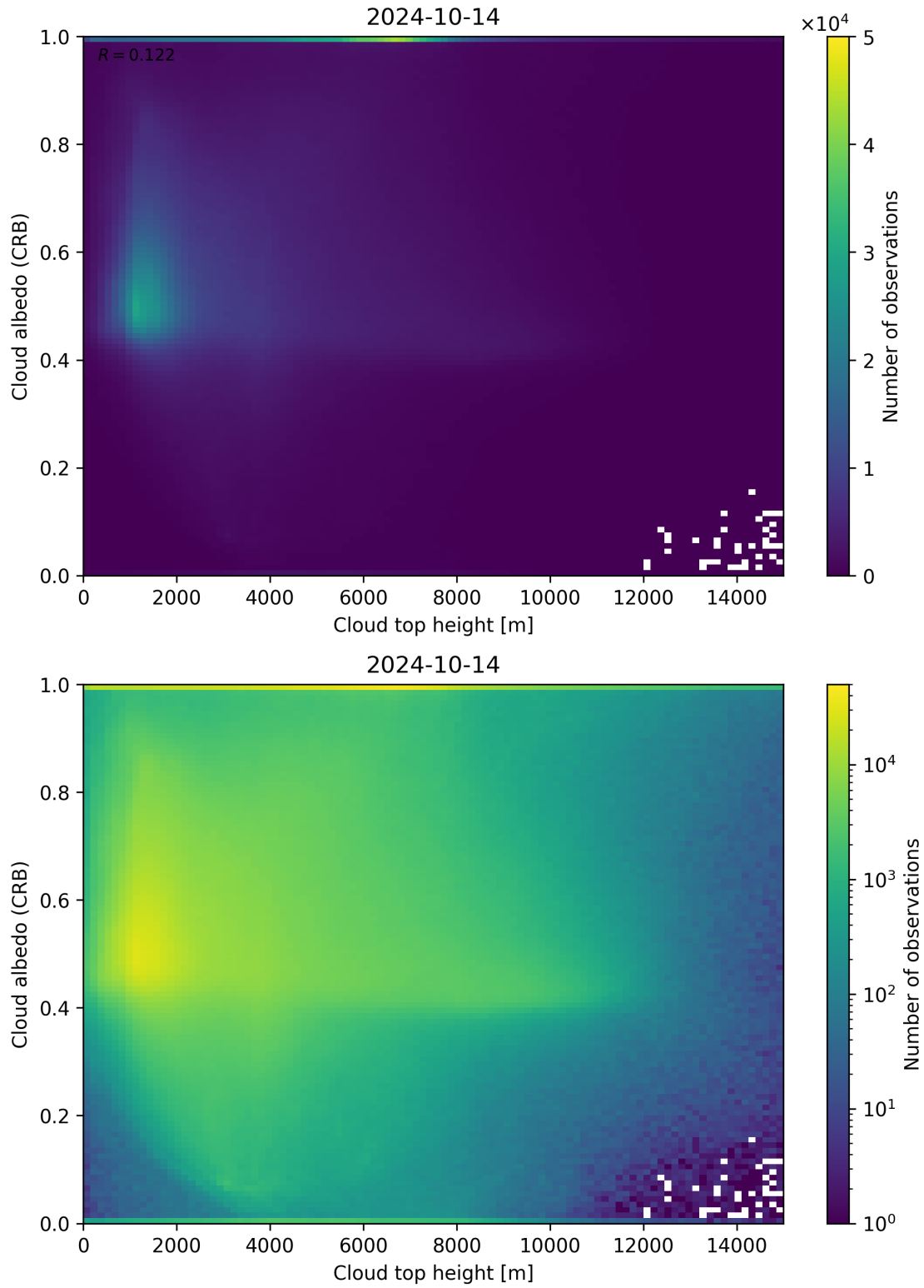
Figure 86: Scatter density plot of “Cloud top height” against “Cloud albedo (CRB)” for 2024-10-14 to 2024-10-15.
