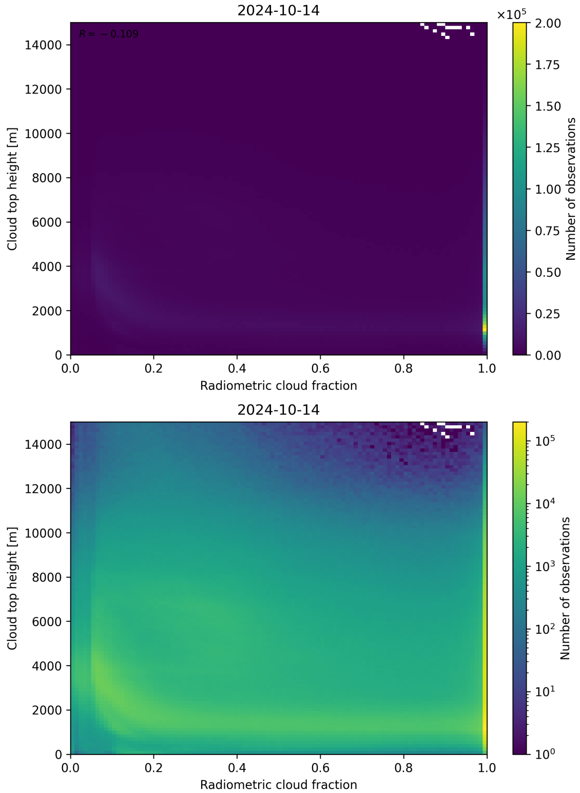
Figure 76: Scatter density plot of “Radiometric cloud fraction” against “Cloud top height” for 2024-10-14 to 2024-10-15.
