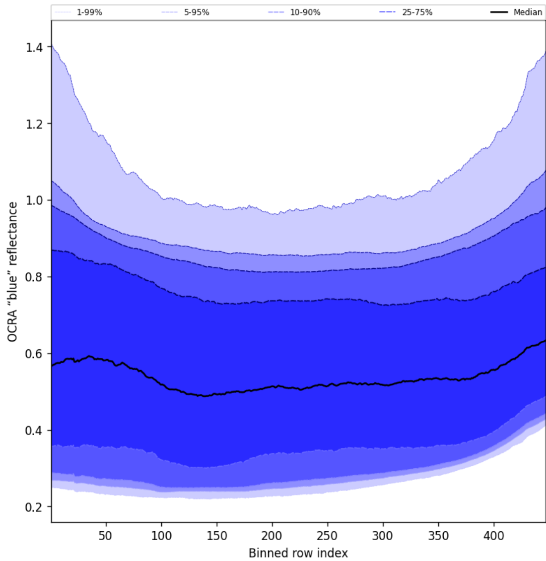
Figure 67: Along track statistics of “OCRA “blue” reflectance” for 2024-10-14 to 2024-10-15
