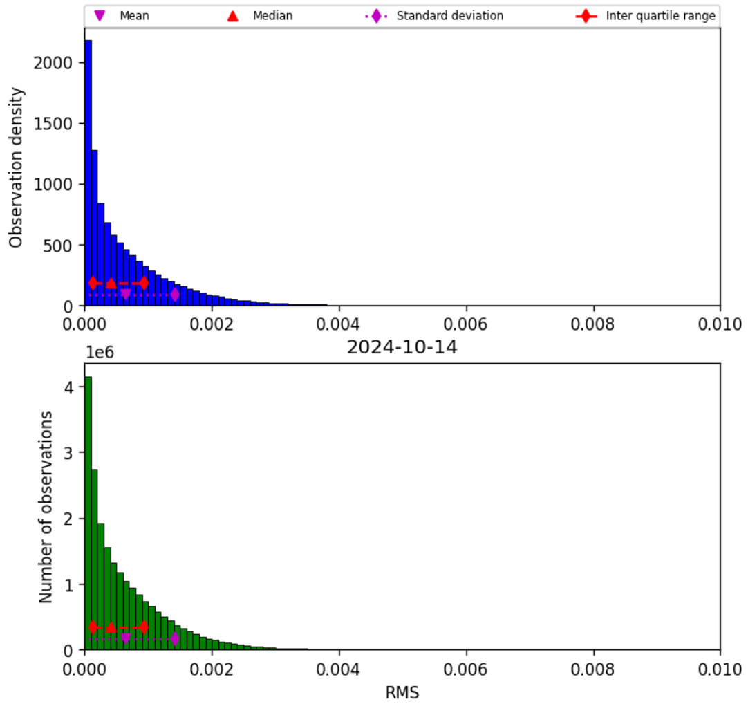
Figure 47: Histogram of “RMS” for 2024-10-14 to 2024-10-15
