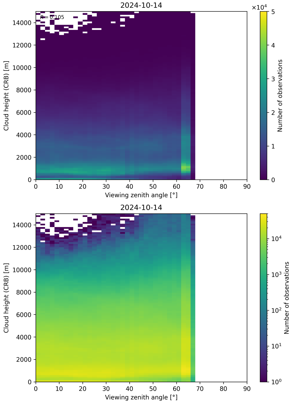
Figure 110: Scatter density plot of “Viewing zenith angle” against “Cloud height (CRB)” for 2024-10-14 to 2024-10-15.
