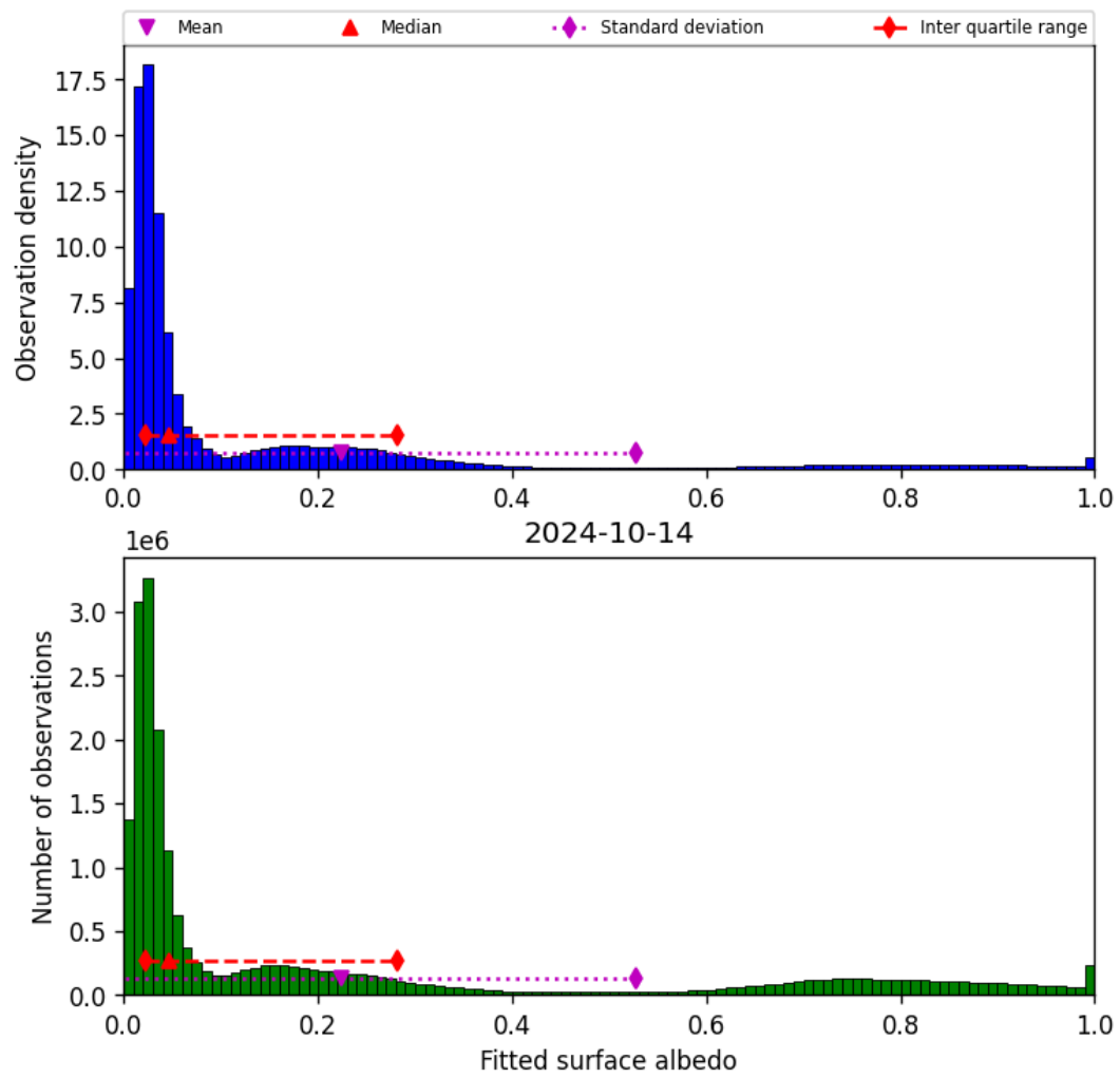
Figure 45: Histogram of “Fitted surface albedo” for 2024-10-14 to 2024-10-15
