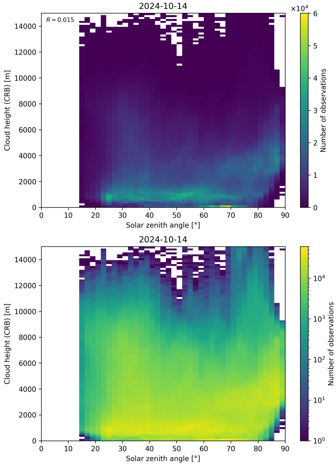
Figure 102: Scatter density plot of “Solar zenith angle” against “Cloud height (CRB)” for 2024-10-14 to 2024-10-15.
