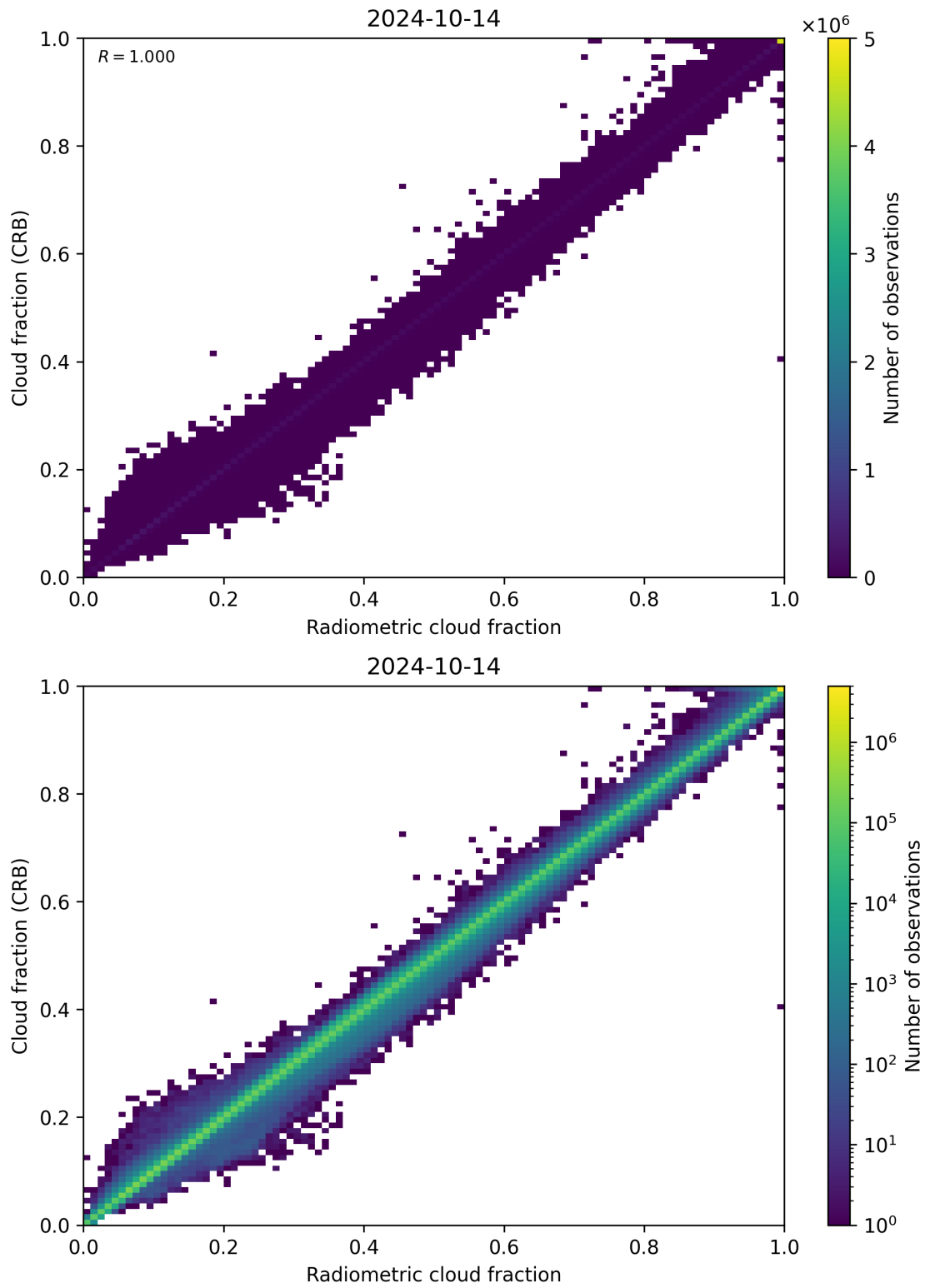
Figure 73: Scatter density plot of “Radiometric cloud fraction” against “Cloud fraction (CRB)” for 2024-10-14 to 2024-10-15.
