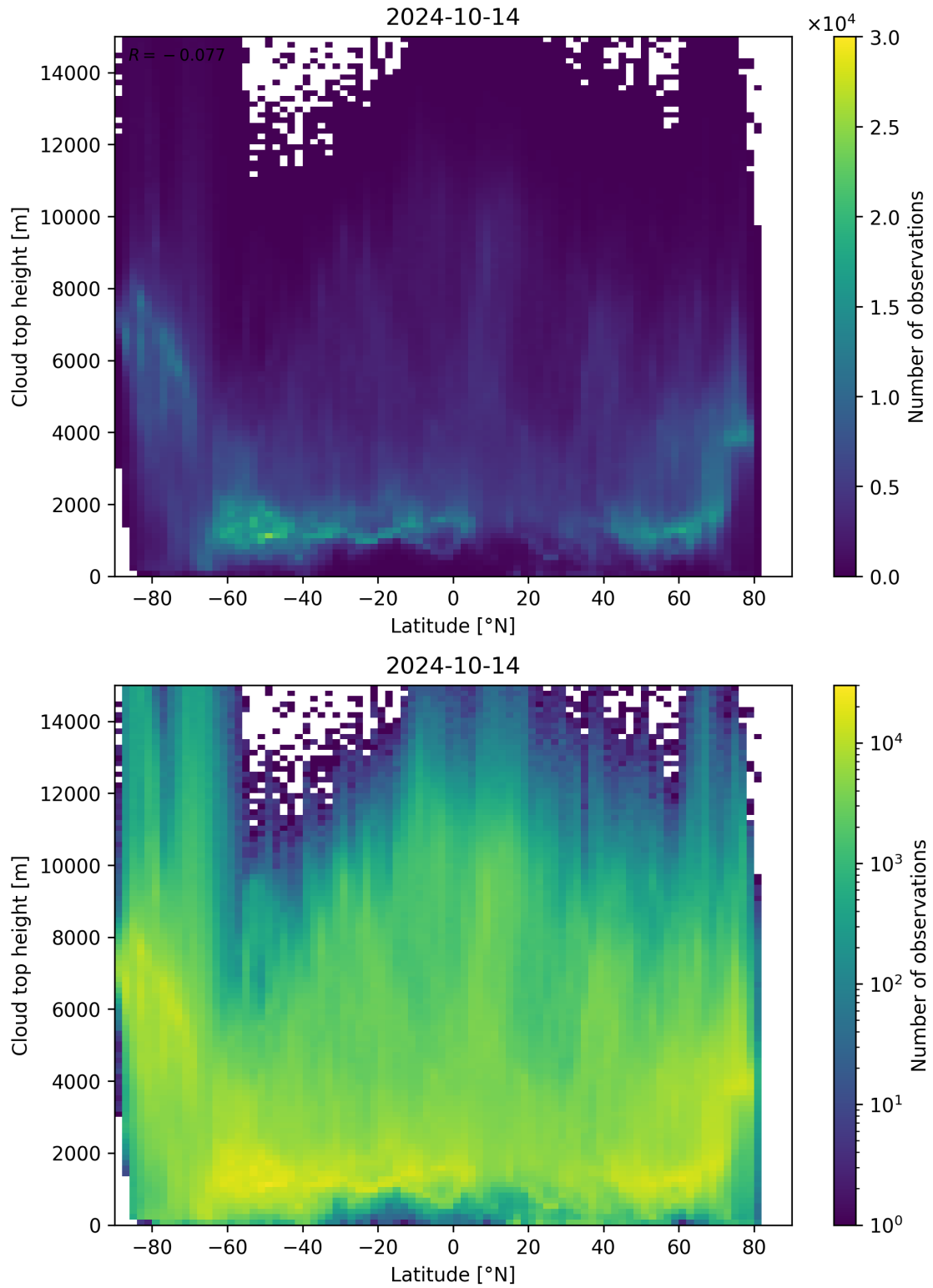
Figure 97: Scatter density plot of “Latitude” against “Cloud top height” for 2024-10-14 to 2024-10-15.
