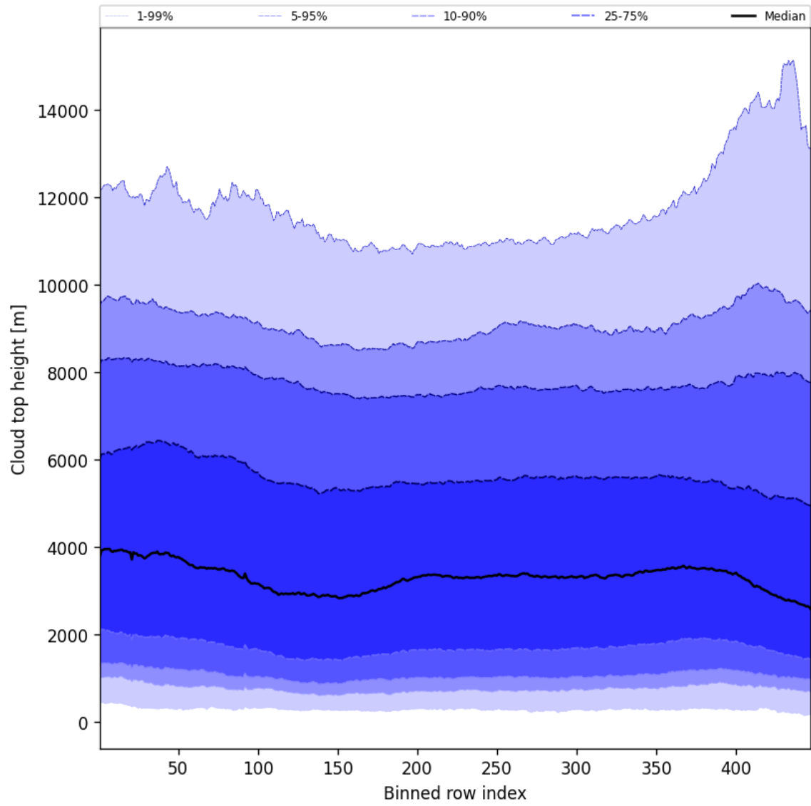
Figure 56: Along track statistics of “Cloud top height” for 2024-10-14 to 2024-10-15
