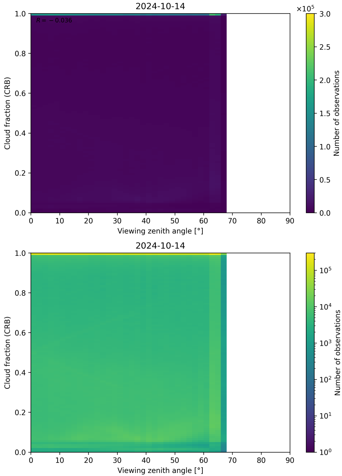
Figure 109: Scatter density plot of “Viewing zenith angle” against “Cloud fraction (CRB)” for 2024-10-14 to 2024-10-15.
