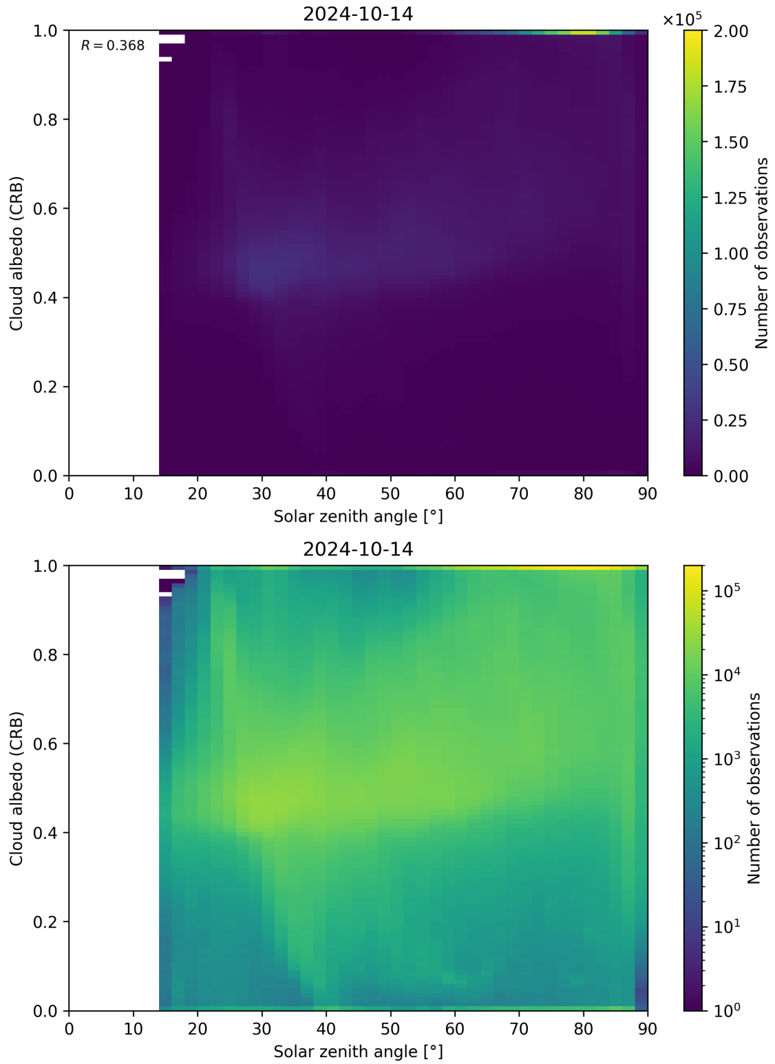
Figure 98: Scatter density plot of “Solar zenith angle” against “Cloud albedo (CRB)” for 2024-10-14 to 2024-10-15.
