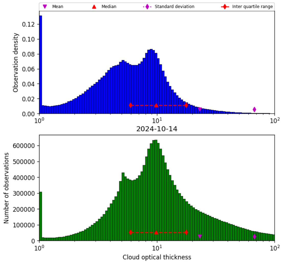
Figure 41: Histogram of “Cloud optical thickness” for 2024-10-14 to 2024-10-15
