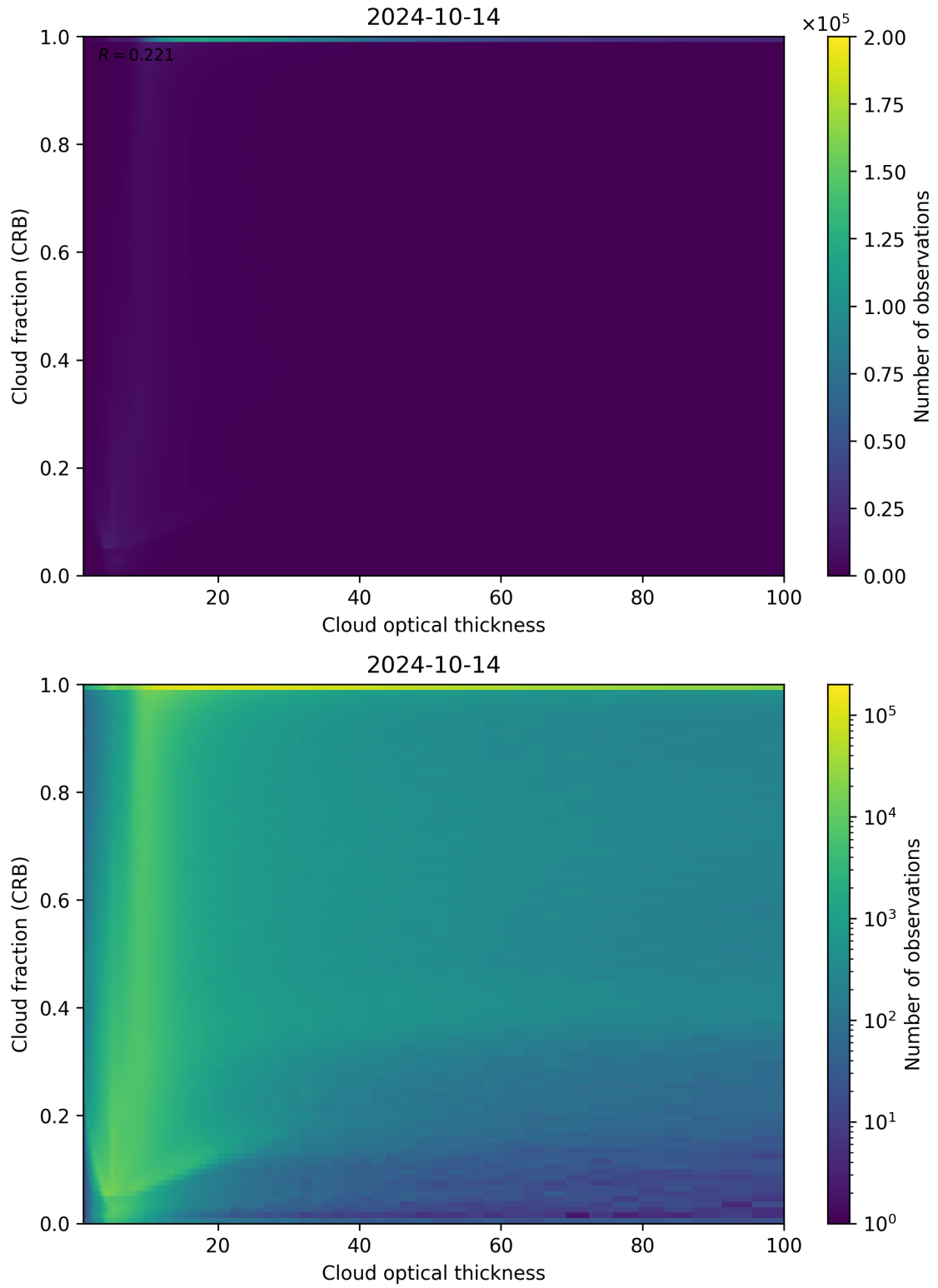
Figure 84: Scatter density plot of “Cloud optical thickness” against “Cloud fraction (CRB)” for 2024-10-14 to 2024-10-15.
