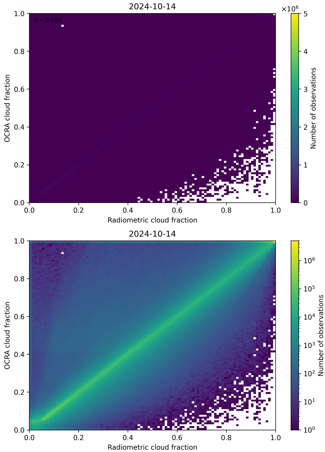
Figure 72: Scatter density plot of “Radiometric cloud fraction” against “OCRA cloud fraction” for 2024-10-14 to 2024-10-15.
