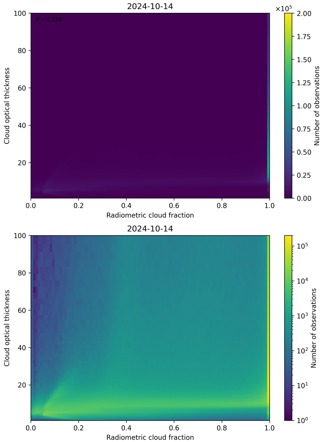
Figure 75: Scatter density plot of “Radiometric cloud fraction” against “Cloud optical thickness” for 2024-10-14 to 2024-10-15.
