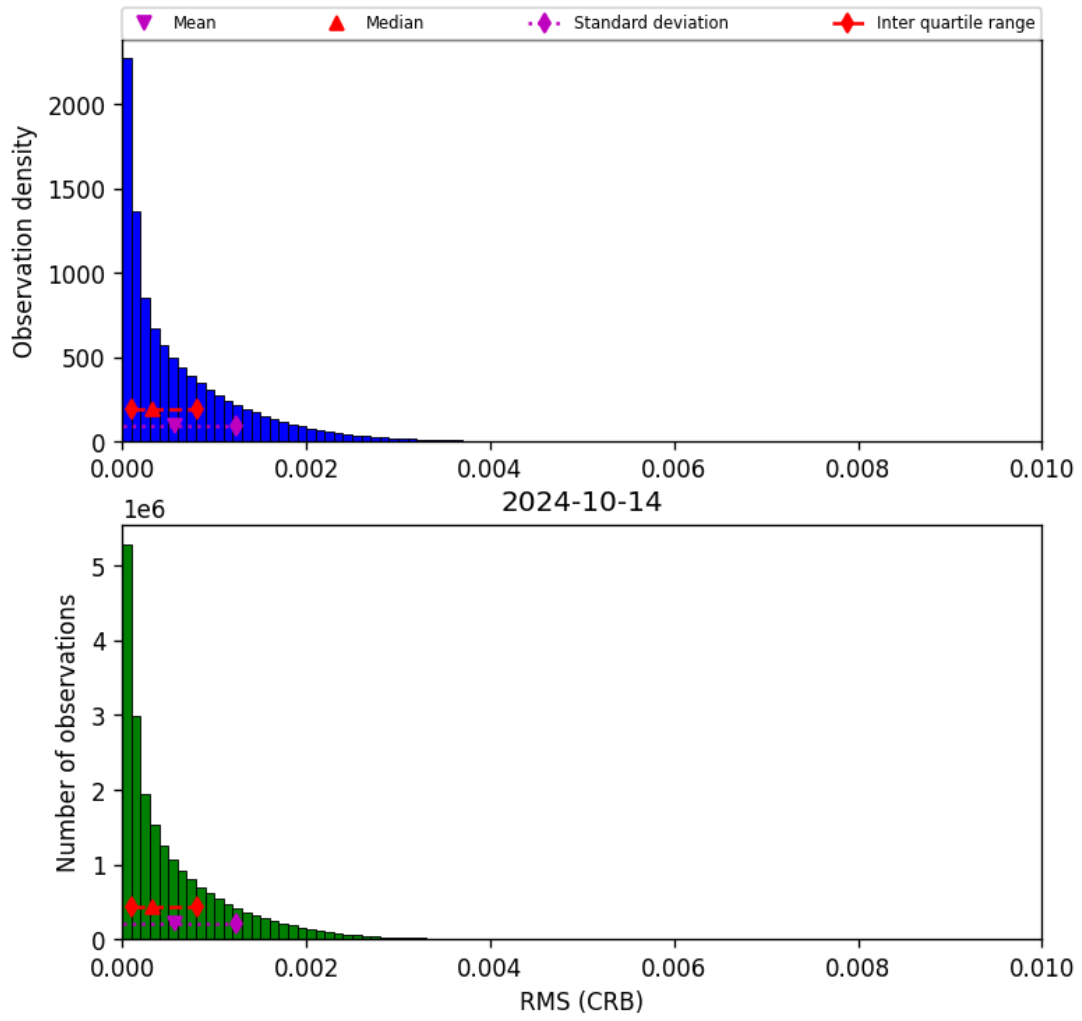
Figure 48: Histogram of "RMS (CRB)" for 2024-10-14 to 2024-10-15
