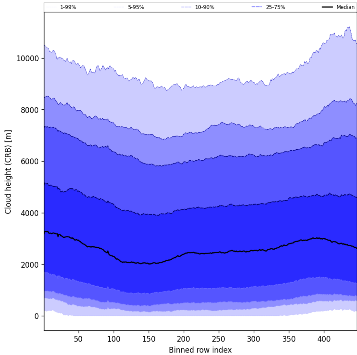
Figure 59: Along track statistics of “Cloud height (CRB)” for 2024-10-14 to 2024-10-15
