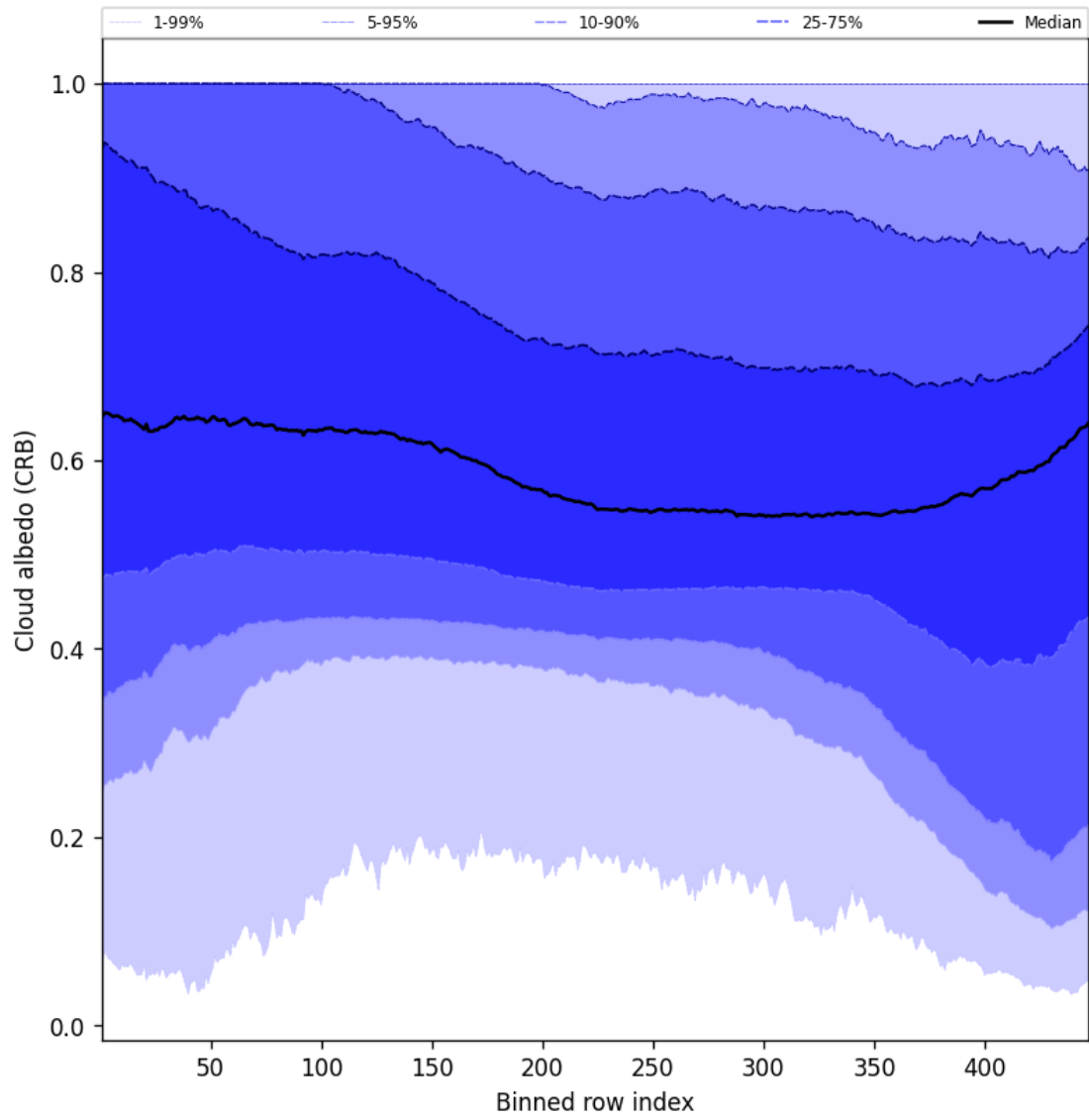
Figure 60: Along track statistics of “Cloud albedo (CRB)” for 2024-10-14 to 2024-10-15
