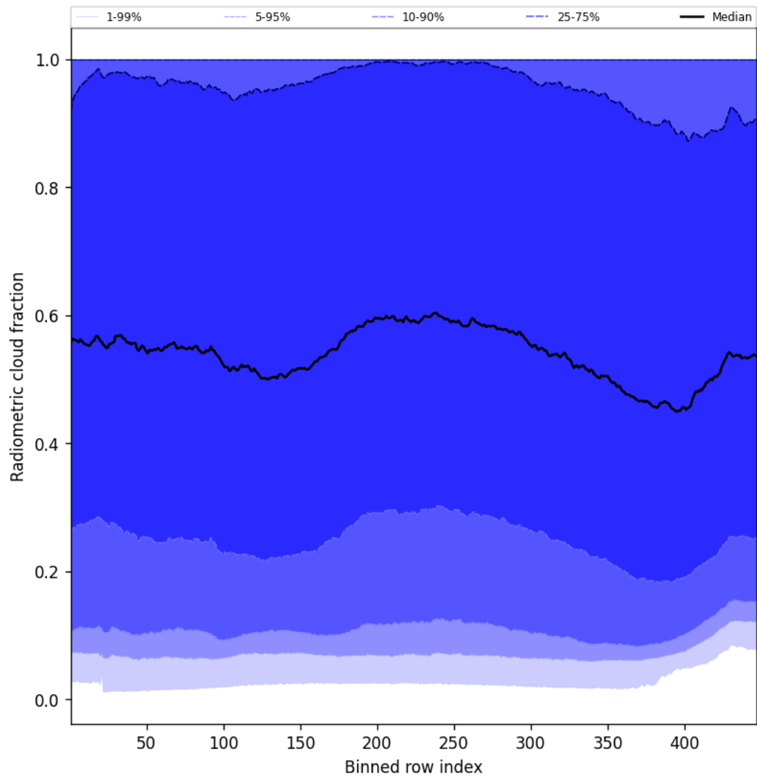
Figure 55: Along track statistics of “Radiometric cloud fraction” for 2024-10-14 to 2024-10-15
