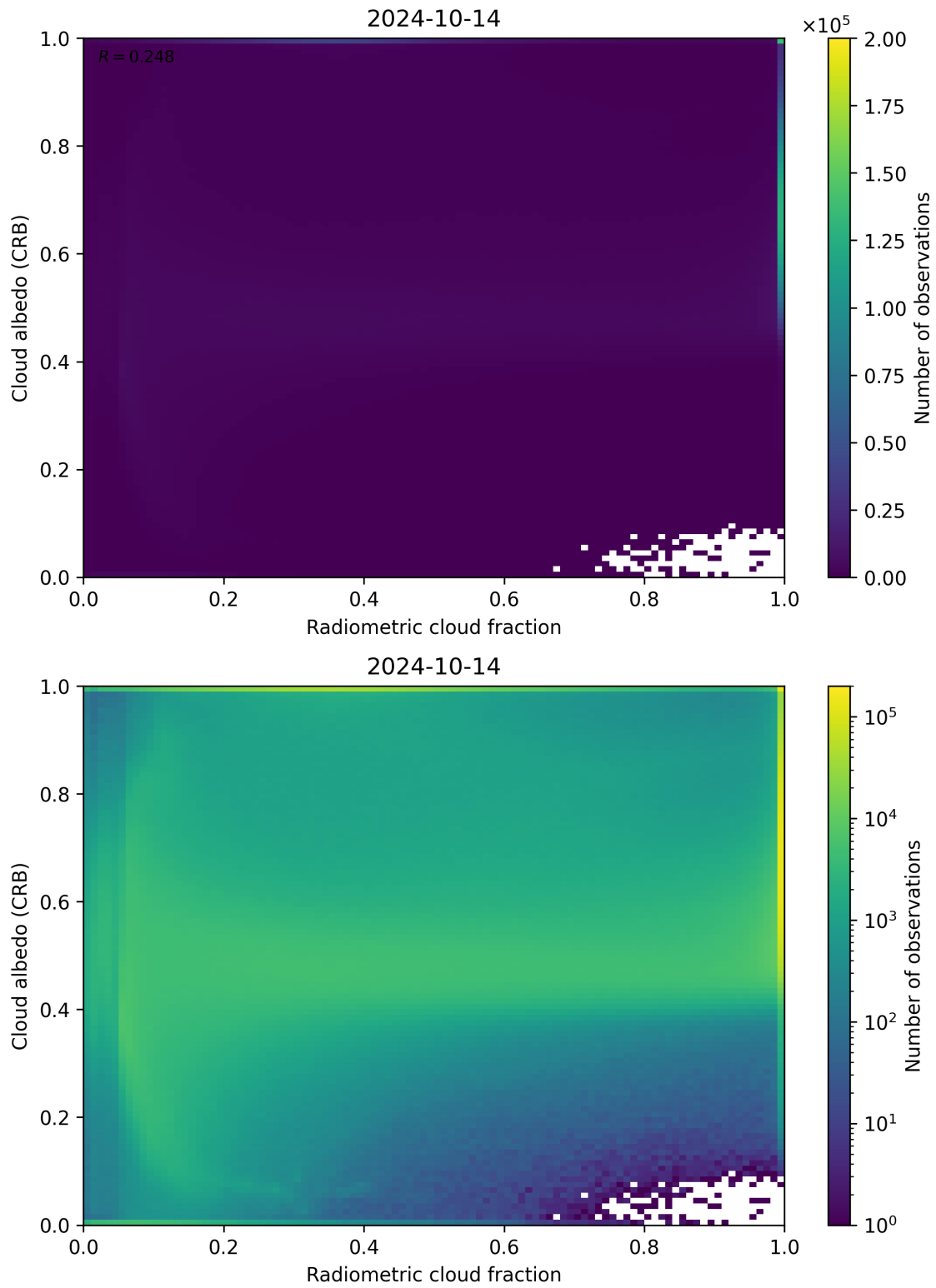
Figure 71: Scatter density plot of “Radiometric cloud fraction” against “Cloud albedo (CRB)” for 2024-10-14 to 2024-10-15.
