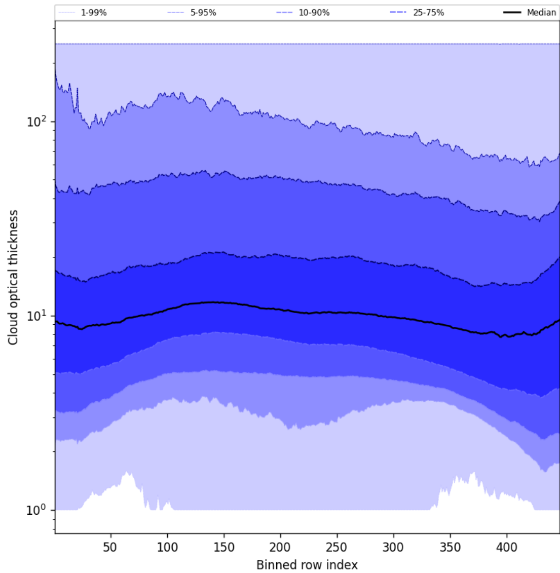
Figure 57: Along track statistics of “Cloud optical thickness” for 2024-10-14 to 2024-10-15
