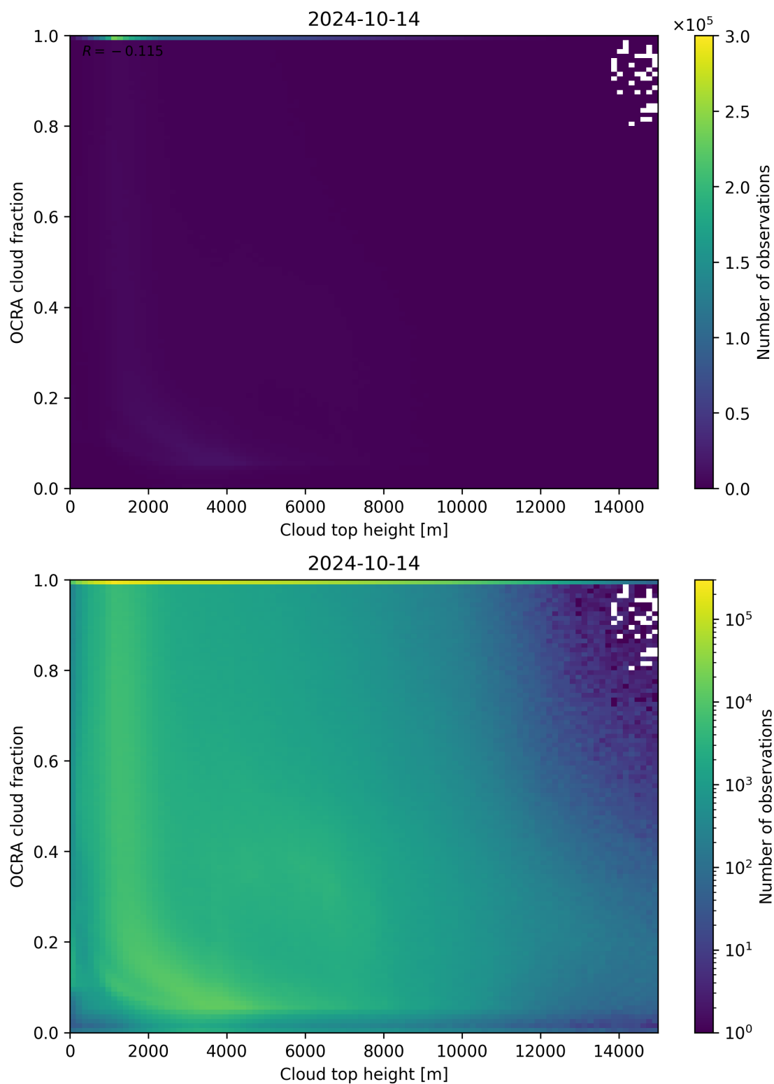
Figure 87: Scatter density plot of “Cloud top height” against “OCRA cloud fraction” for 2024-10-14 to 2024-10-15.
