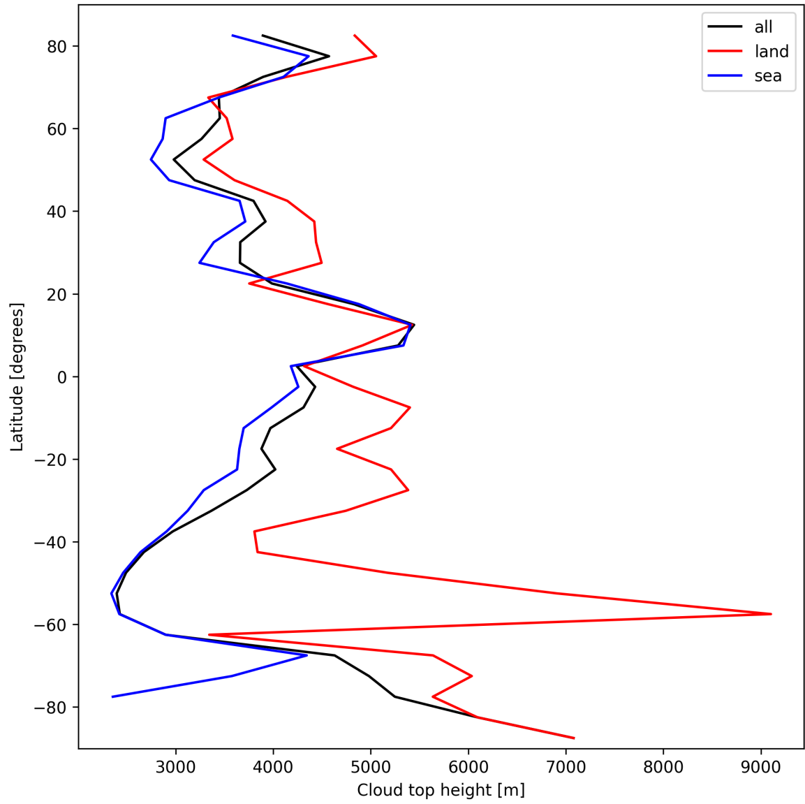
Figure 24: Zonal average of “Cloud top height” for 2024-10-14 to 2024-10-15.
