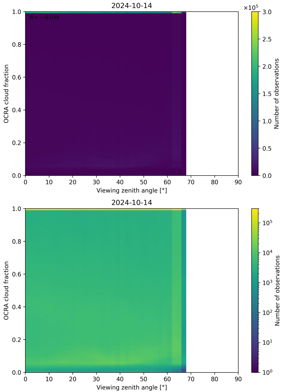
Figure 108: Scatter density plot of “Viewing zenith angle” against “OCRA cloud fraction” for 2024-10-14 to 2024-10-15.
