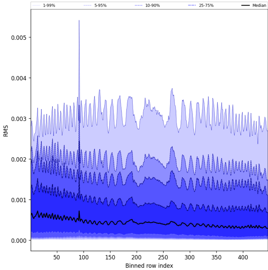
Figure 63: Along track statistics of “RMS” for 2024-10-14 to 2024-10-15
