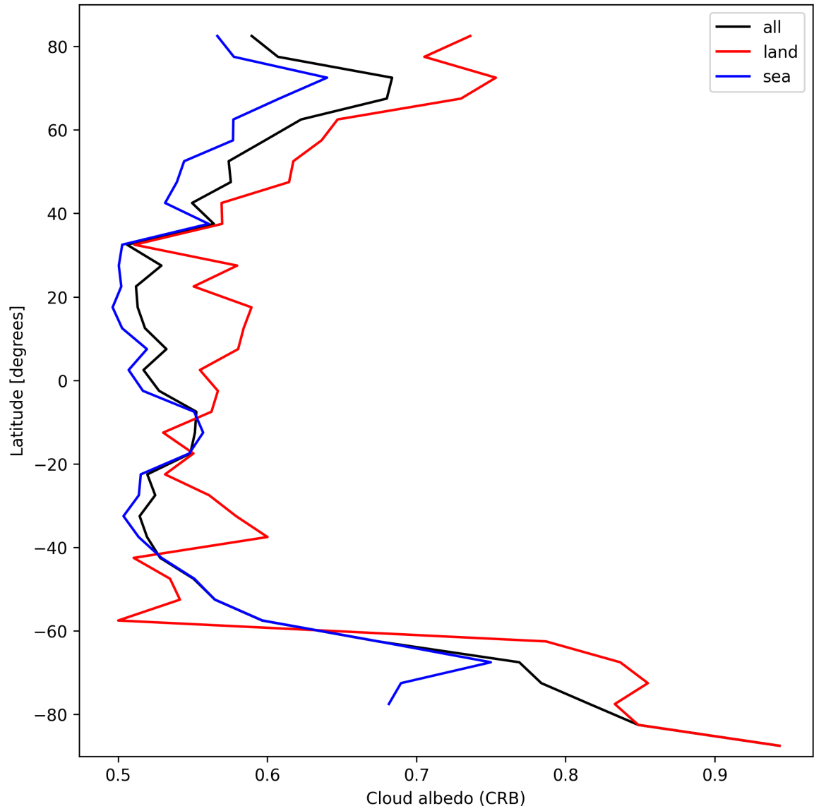
Figure 28: Zonal average of “Cloud albedo (CRB)” for 2024-10-14 to 2024-10-15.
