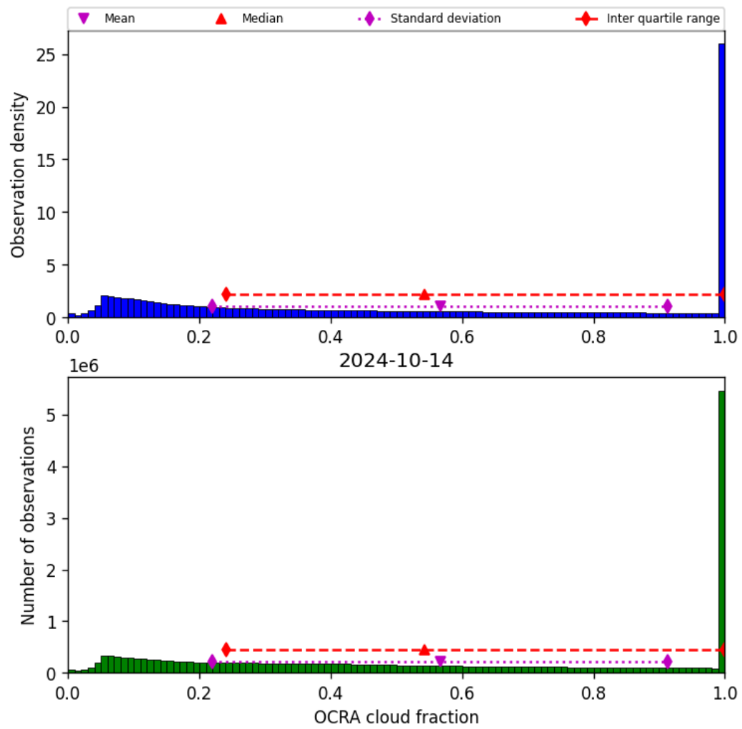
Figure 50: Histogram of “OCRA cloud fraction” for 2024-10-14 to 2024-10-15
