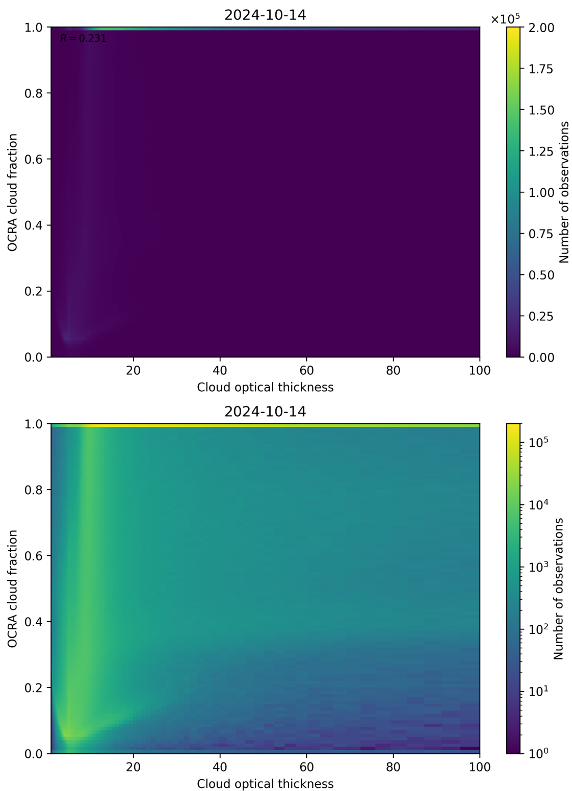
Figure 83: Scatter density plot of “Cloud optical thickness” against “OCRA cloud fraction” for 2024-10-14 to 2024-10-15.
