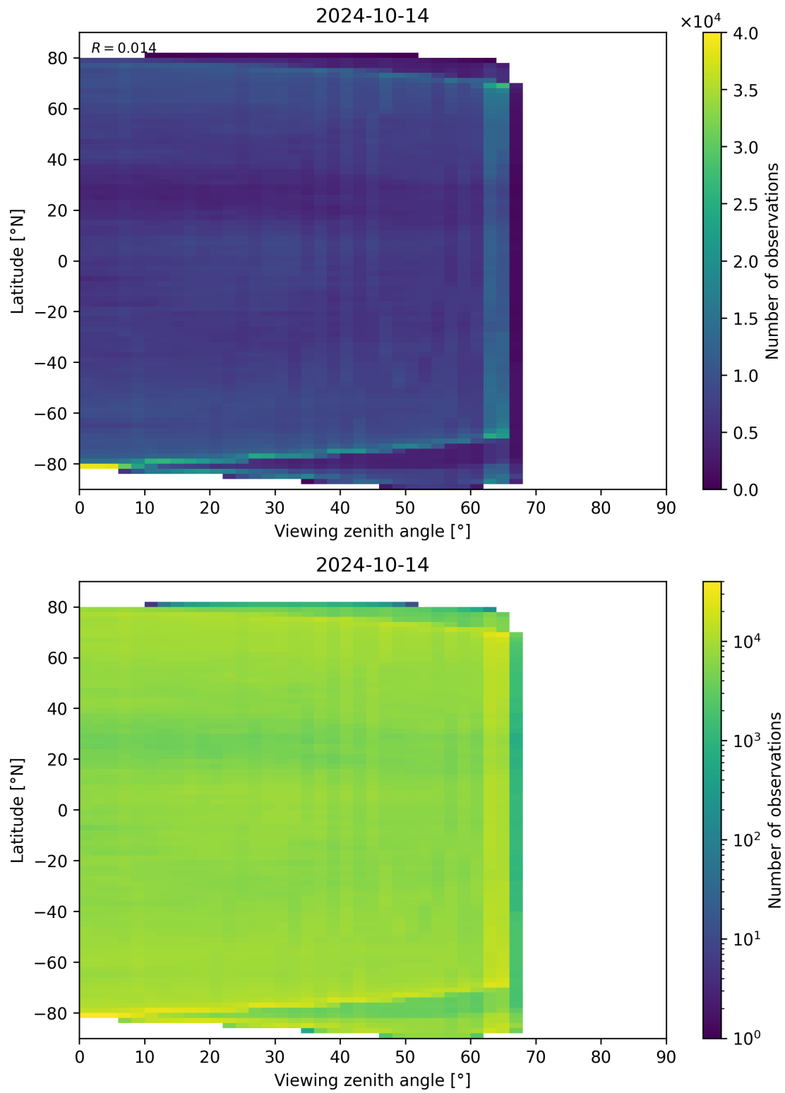
Figure 113: Scatter density plot of “Viewing zenith angle” against “Latitude” for 2024-10-14 to 2024-10-15.
