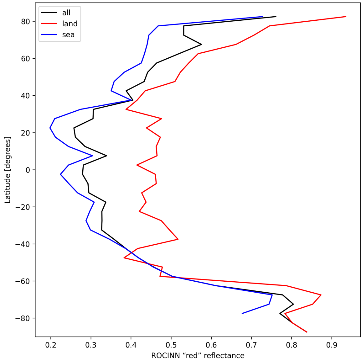
Figure 37: Zonal average of “ROCINN “red” reflectance” for 2024-10-14 to 2024-10-15.
