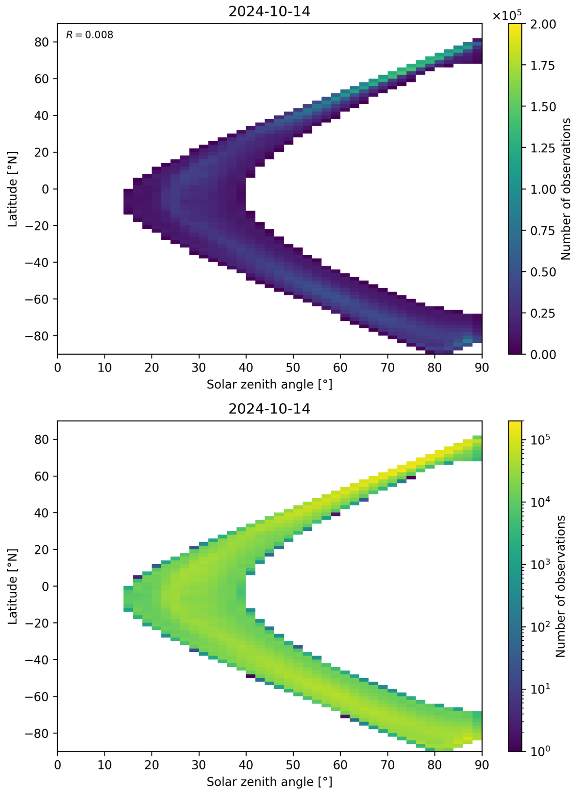
Figure 105: Scatter density plot of “Solar zenith angle” against “Latitude” for 2024-10-14 to 2024-10-15.
