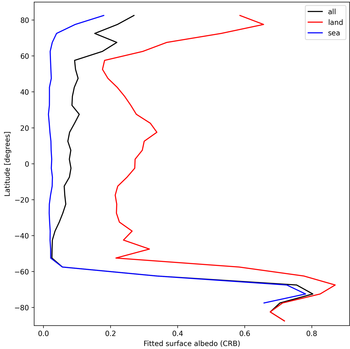
Figure 30: Zonal average of “Fitted surface albedo (CRB)” for 2024-10-14 to 2024-10-15.
