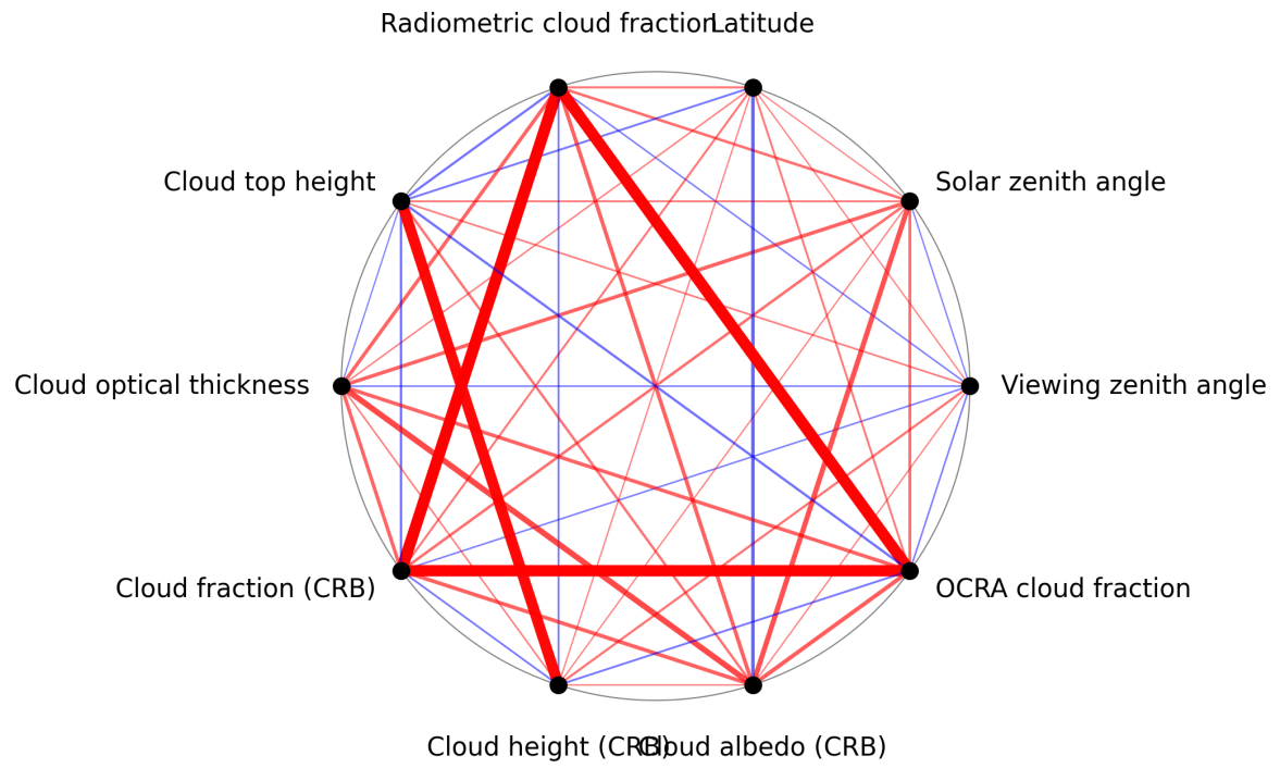
Figure 1: Map of correlation graph for 2024-10-14 to 2024-10-15.
