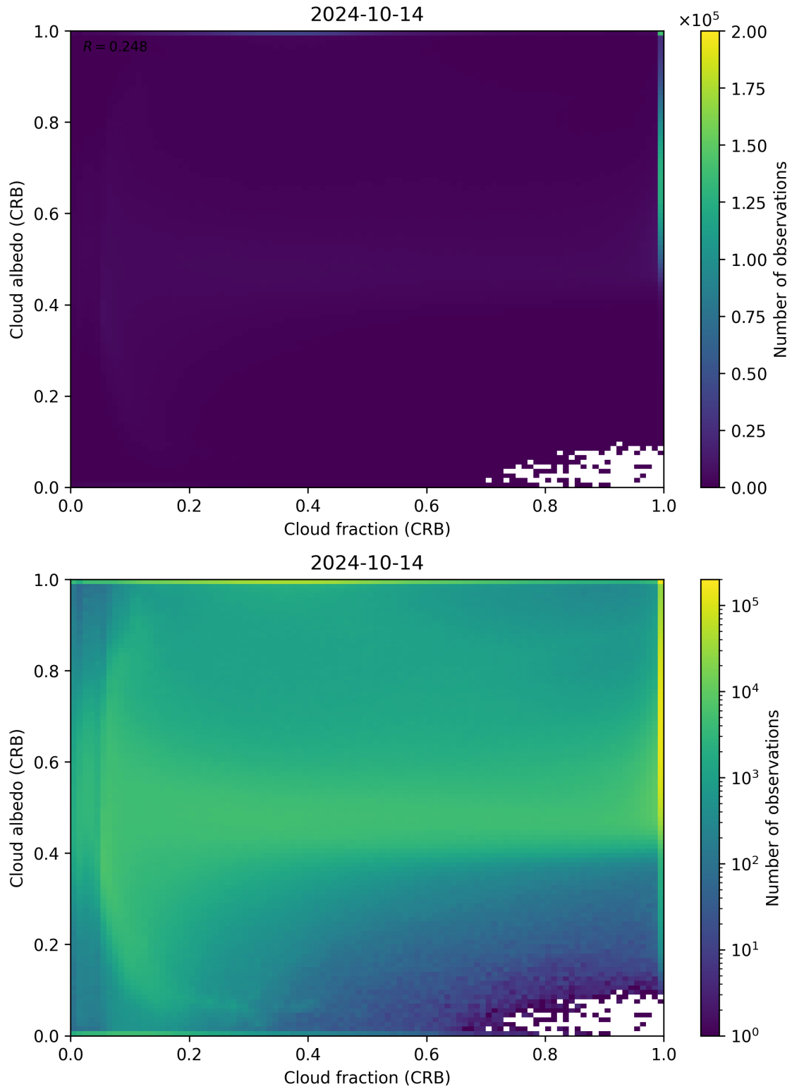
Figure 77: Scatter density plot of “Cloud fraction (CRB)” against “Cloud albedo (CRB)” for 2024-10-14 to 2024-10-15.
