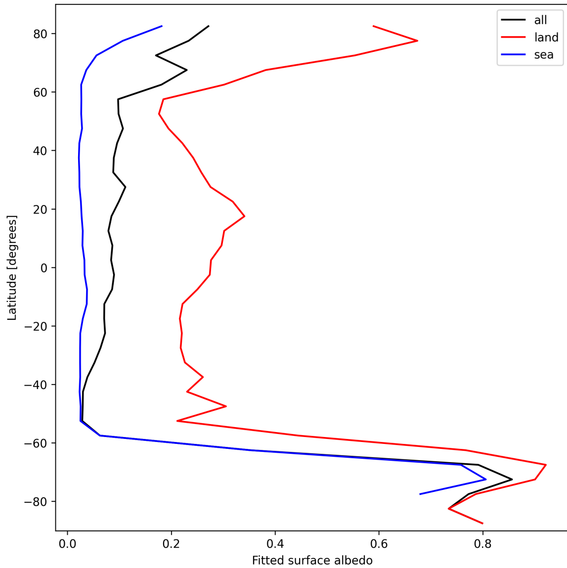
Figure 29: Zonal average of “Fitted surface albedo” for 2024-10-14 to 2024-10-15.
