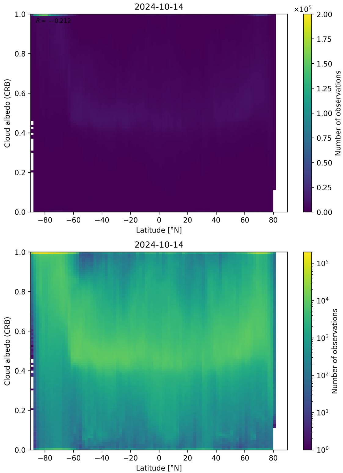
Figure 91: Scatter density plot of “Latitude” against “Cloud albedo (CRB)” for 2024-10-14 to 2024-10-15.
