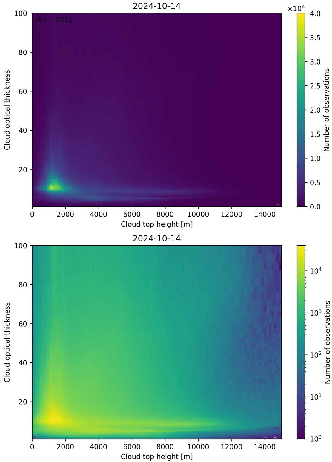
Figure 90: Scatter density plot of “Cloud top height” against “Cloud optical thickness” for 2024-10-14 to 2024-10-15.
