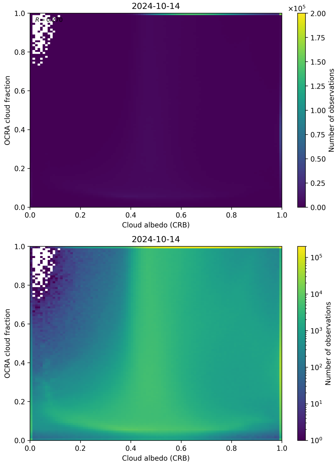
Figure 70: Scatter density plot of “Cloud albedo (CRB)” against “OCRA cloud fraction” for 2024-10-14 to 2024-10-15.
