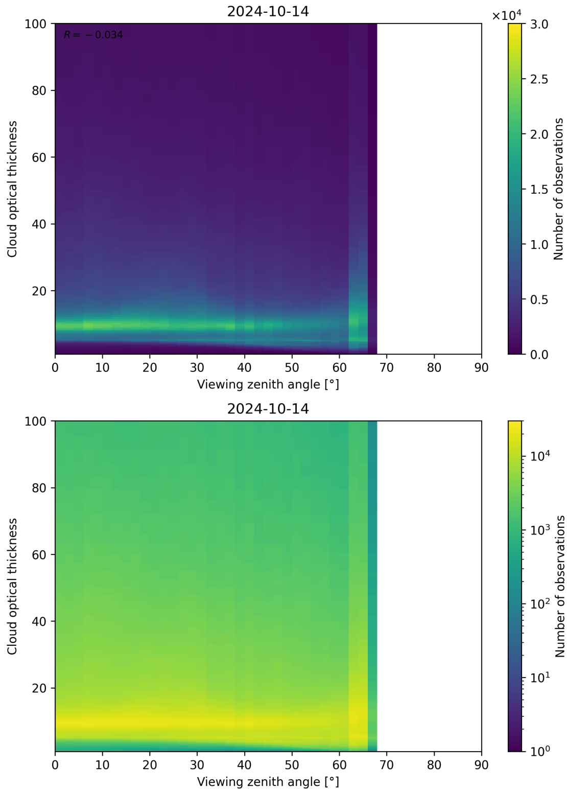
Figure 111: Scatter density plot of “Viewing zenith angle” against “Cloud optical thickness” for 2024-10-14 to 2024-10-15.
