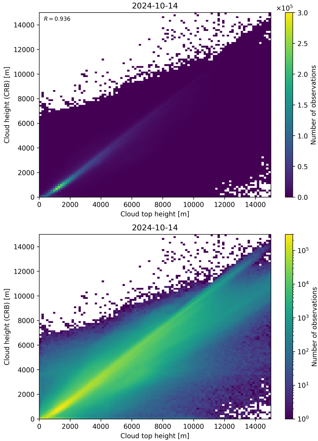
Figure 89: Scatter density plot of “Cloud top height” against “Cloud height (CRB)” for 2024-10-14 to 2024-10-15.
