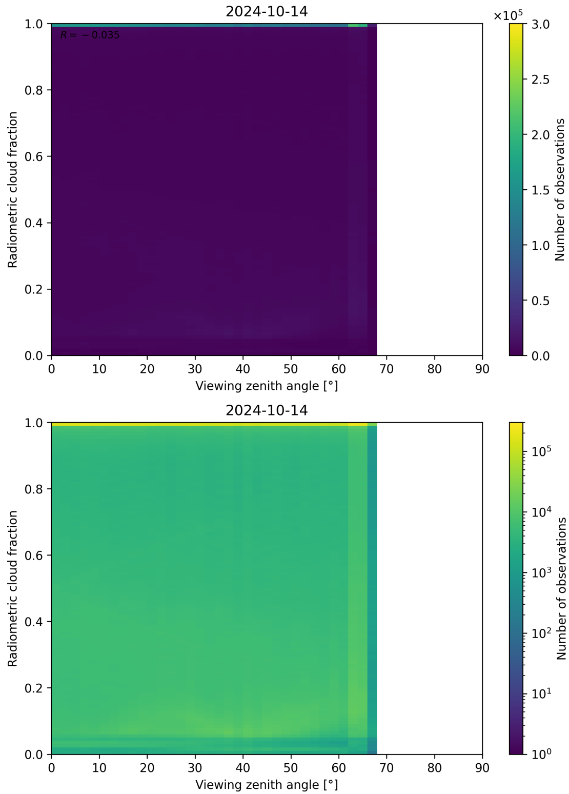
Figure 107: Scatter density plot of “Viewing zenith angle” against “Radiometric cloud fraction” for 2024-10-14 to 2024-10-15.
