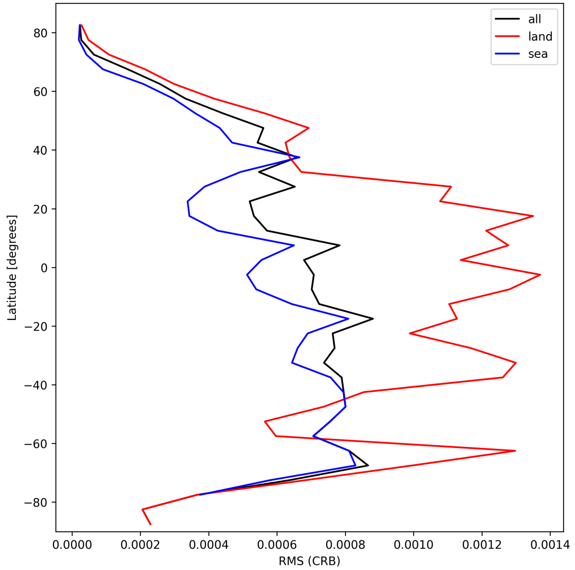
Figure 32: Zonal average of “RMS (CRB)” for 2024-10-14 to 2024-10-15.
