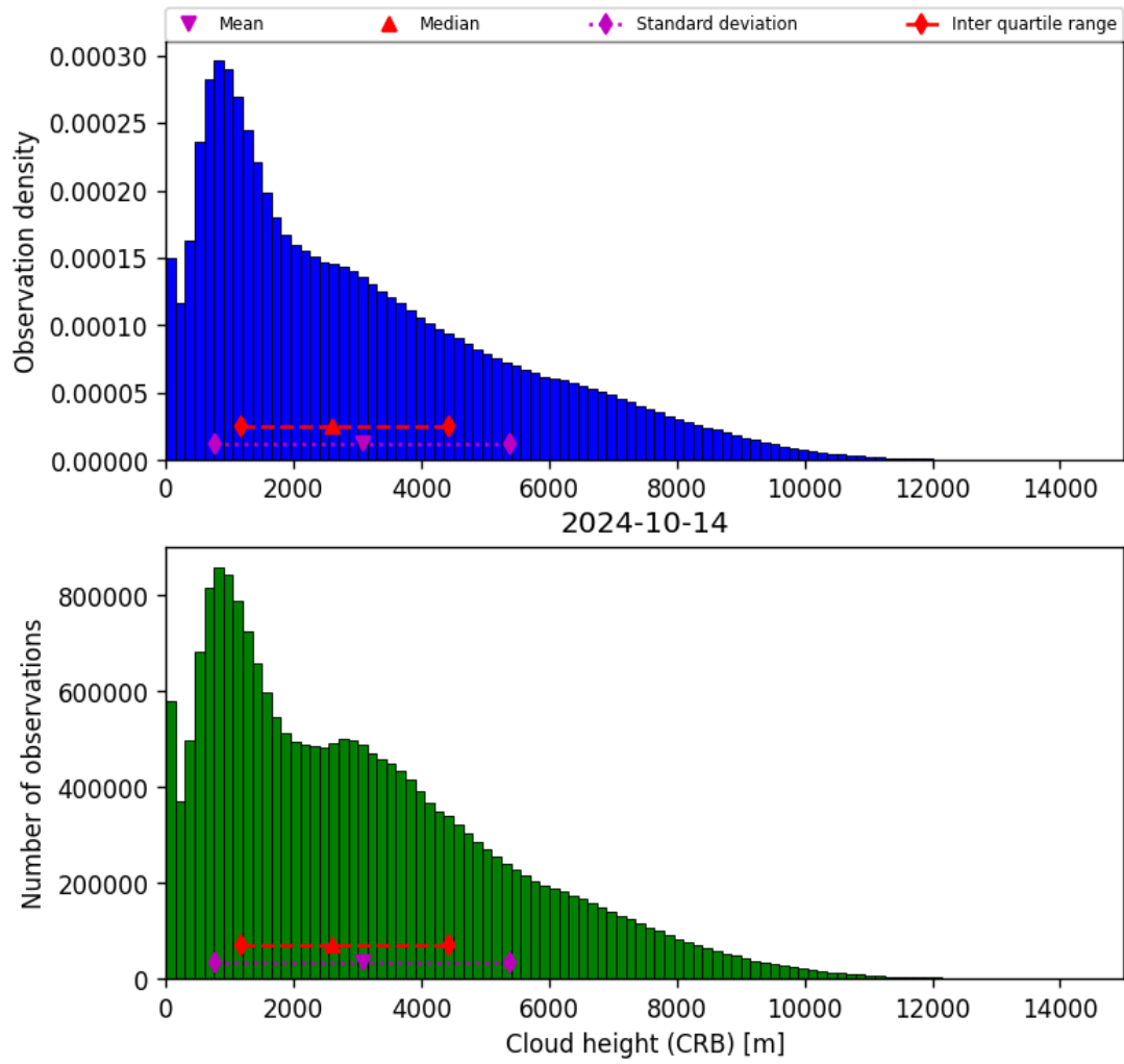
Figure 43: Histogram of “Cloud height (CRB)” for 2024-10-14 to 2024-10-15
