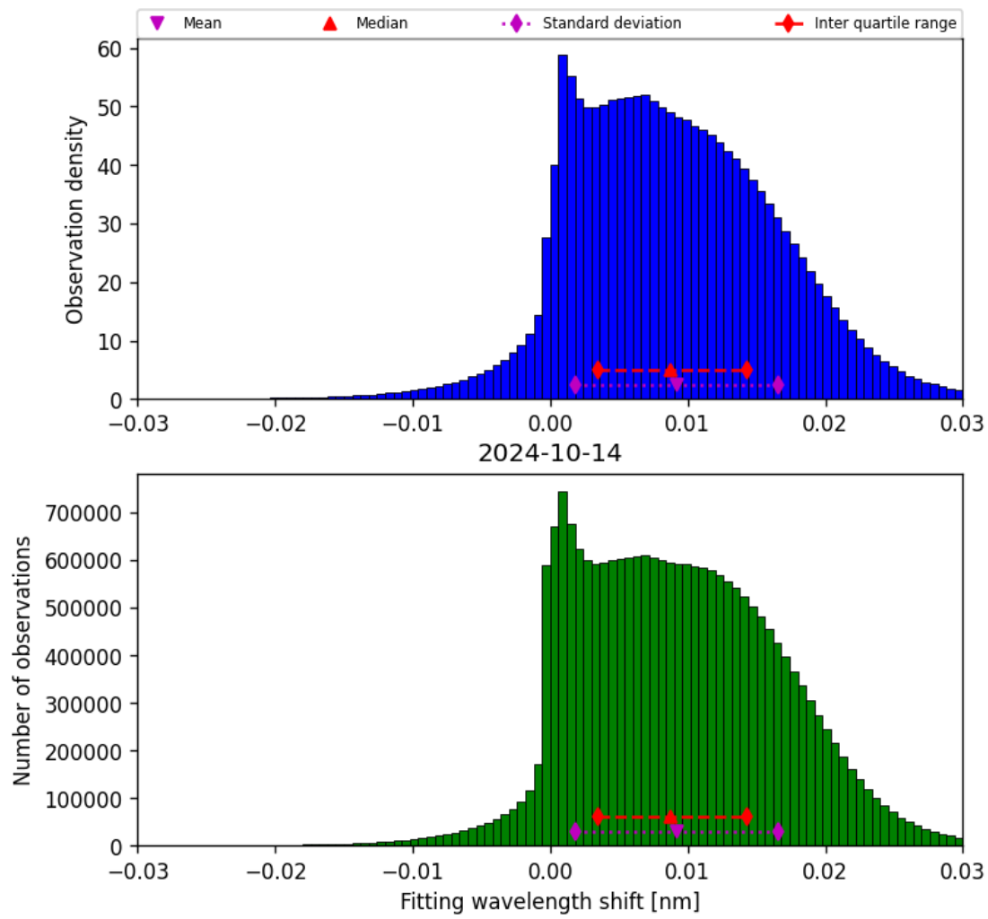
Figure 49: Histogram of “Fitting wavelength shift” for 2024-10-14 to 2024-10-15
