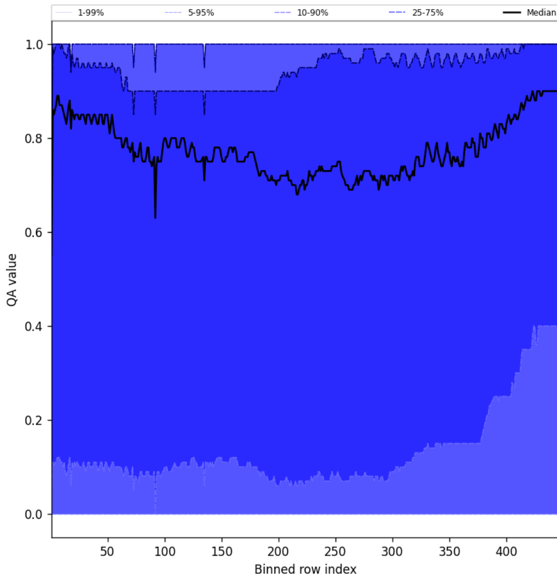
Figure 54: Along track statistics of “QA value” for 2024-10-15 to 2024-10-17
