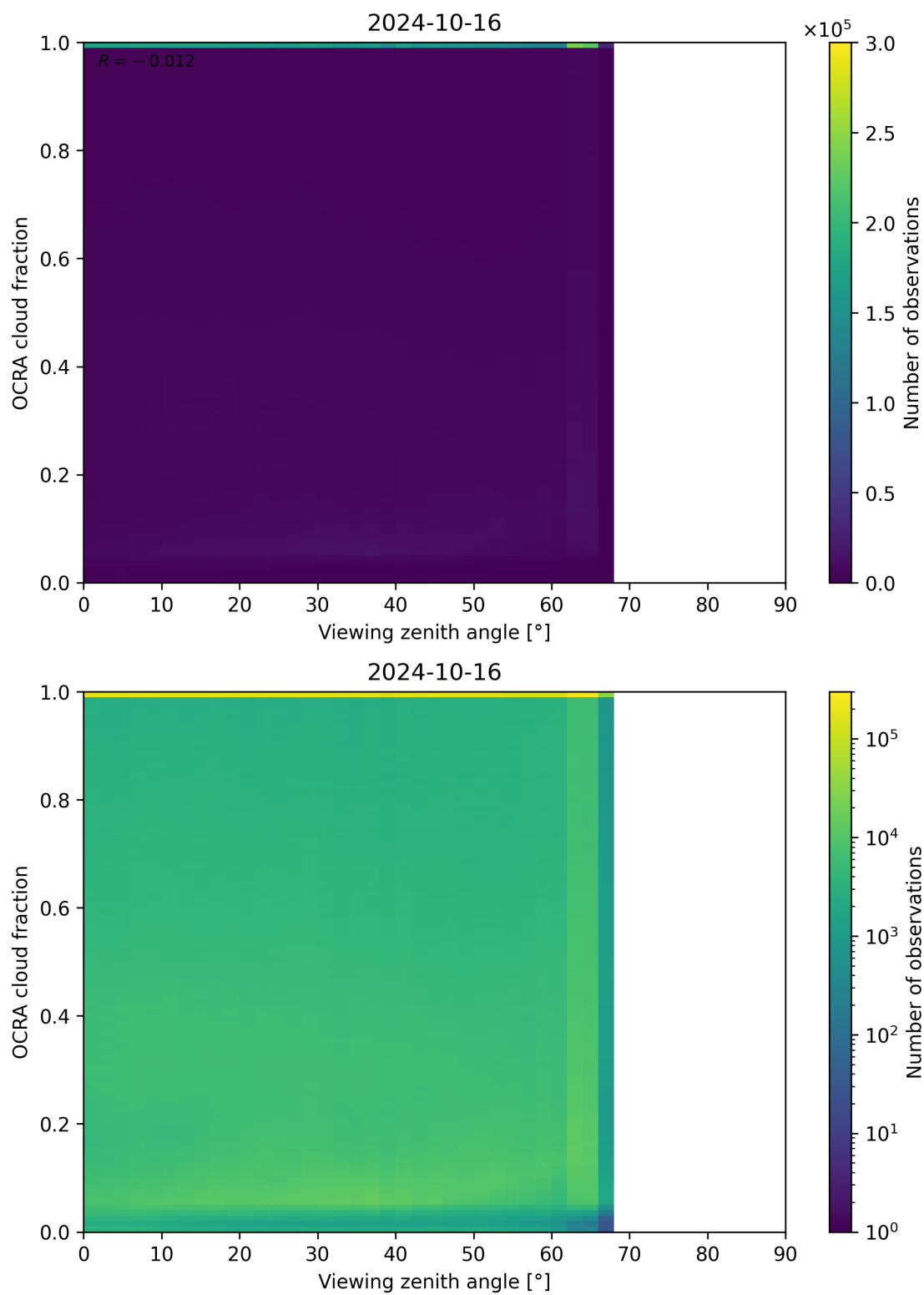
Figure 108: Scatter density plot of “Viewing zenith angle” against “OCRA cloud fraction” for 2024-10-15 to 2024-10-17.
