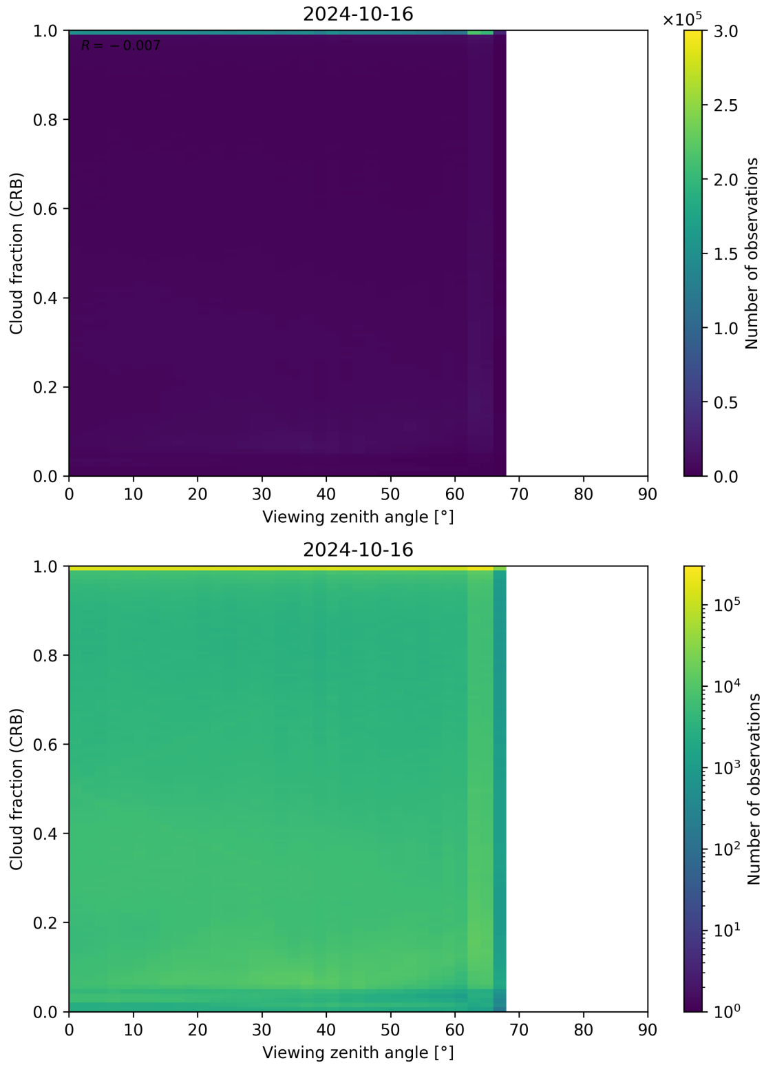
Figure 109: Scatter density plot of “Viewing zenith angle” against “Cloud fraction (CRB)” for 2024-10-15 to 2024-10-17.
