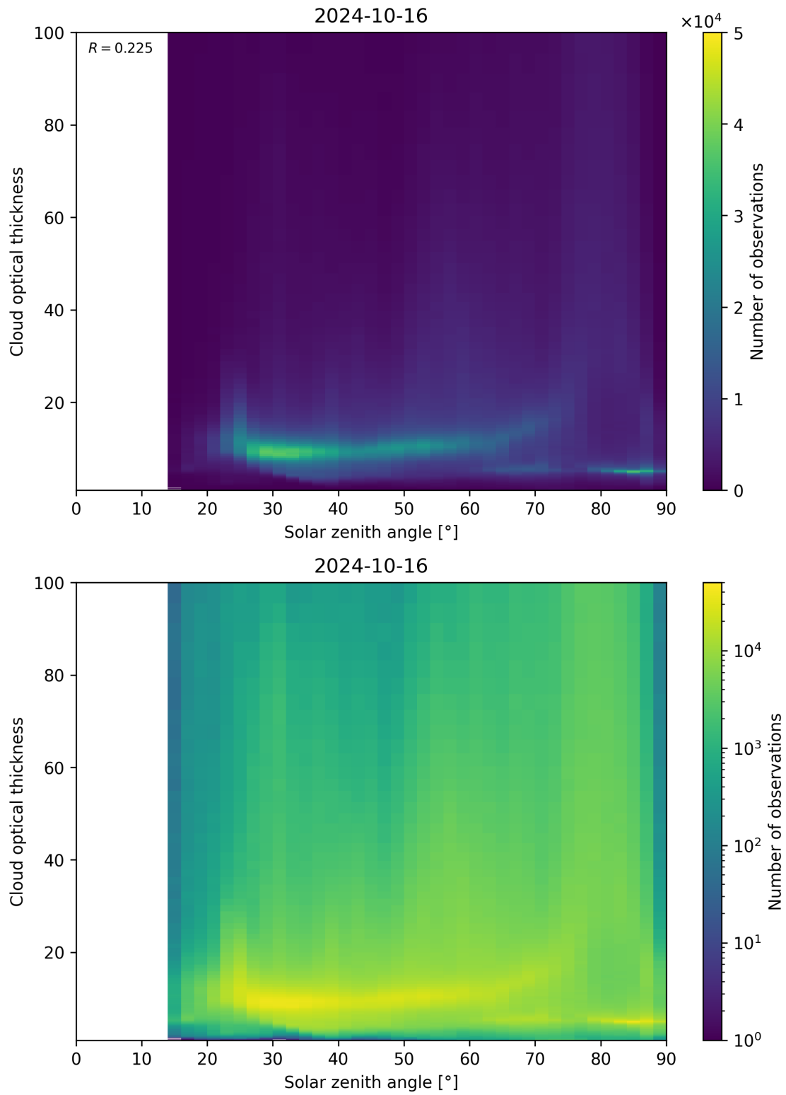
Figure 103: Scatter density plot of “Solar zenith angle” against “Cloud optical thickness” for 2024-10-15 to 2024-10-17.
