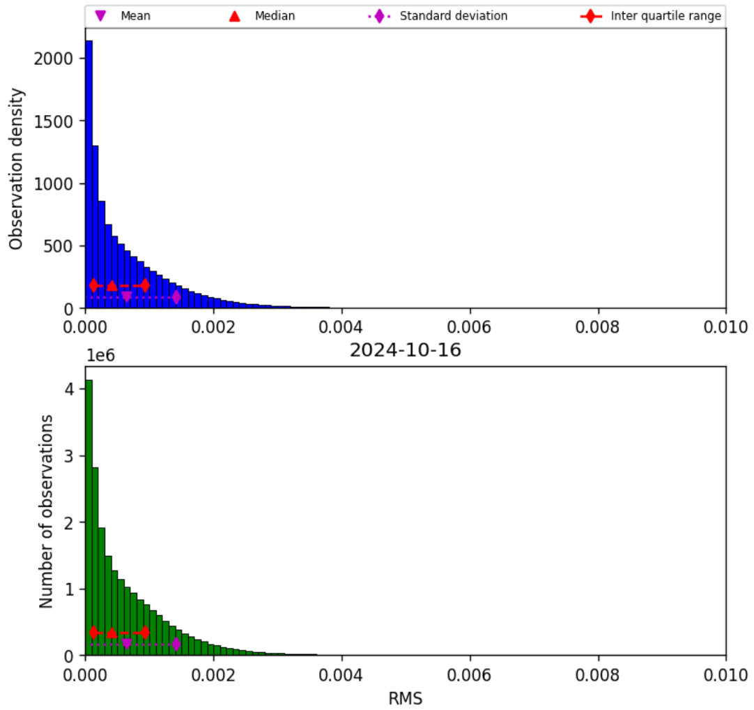
Figure 47: Histogram of “RMS” for 2024-10-15 to 2024-10-17
