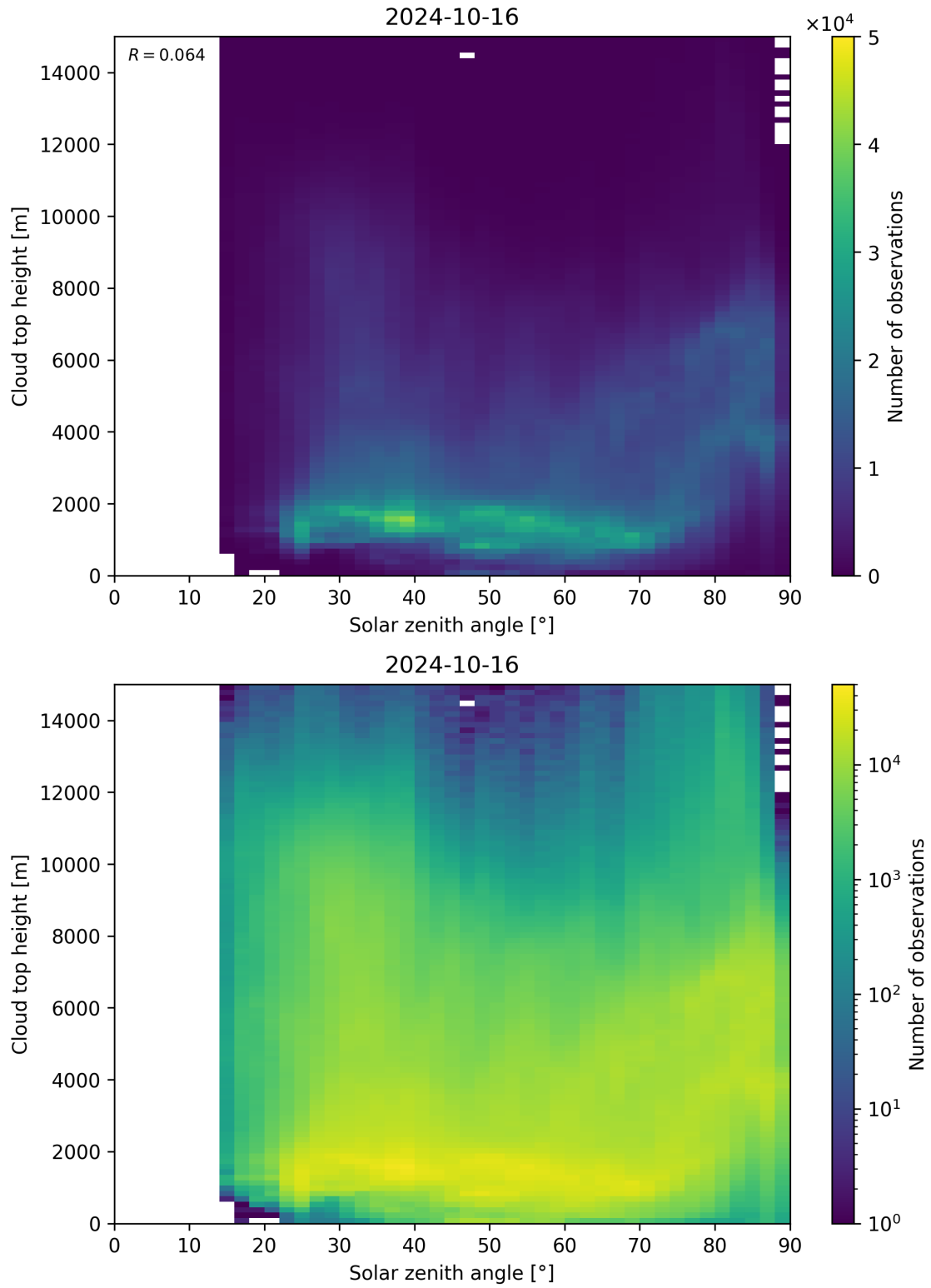
Figure 104: Scatter density plot of “Solar zenith angle” against “Cloud top height” for 2024-10-15 to 2024-10-17.
