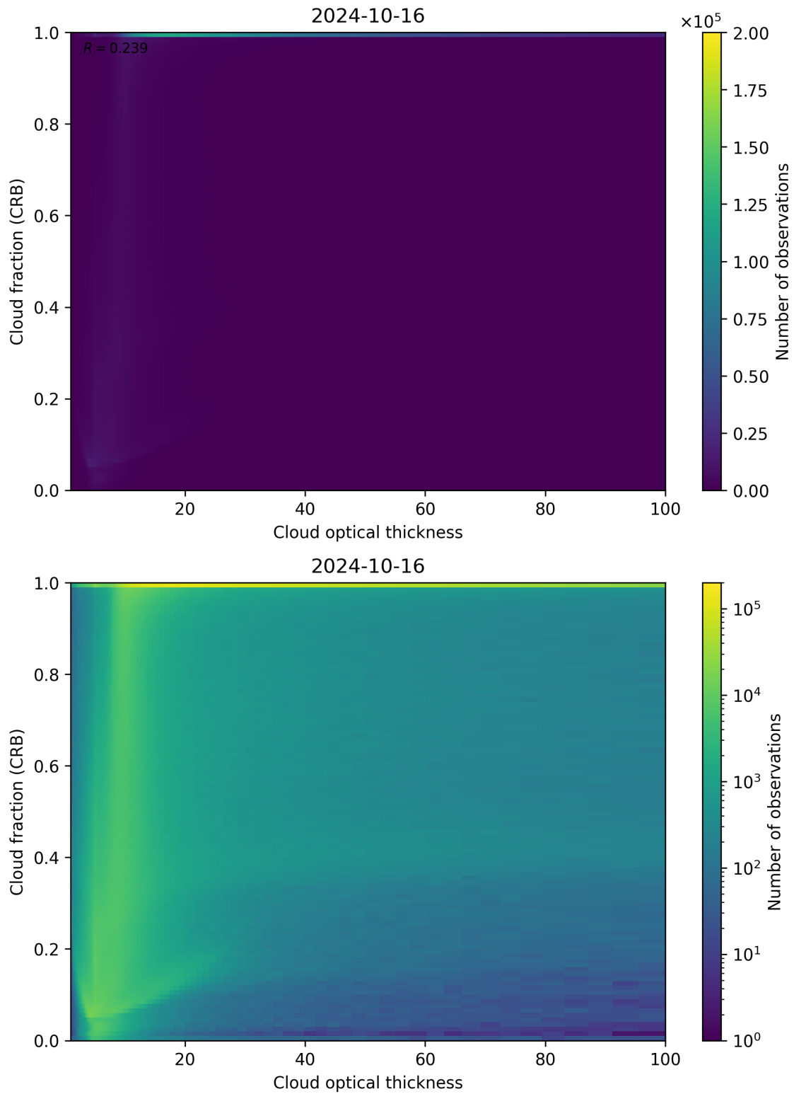
Figure 84: Scatter density plot of “Cloud optical thickness” against “Cloud fraction (CRB)” for 2024-10-15 to 2024-10-17.
