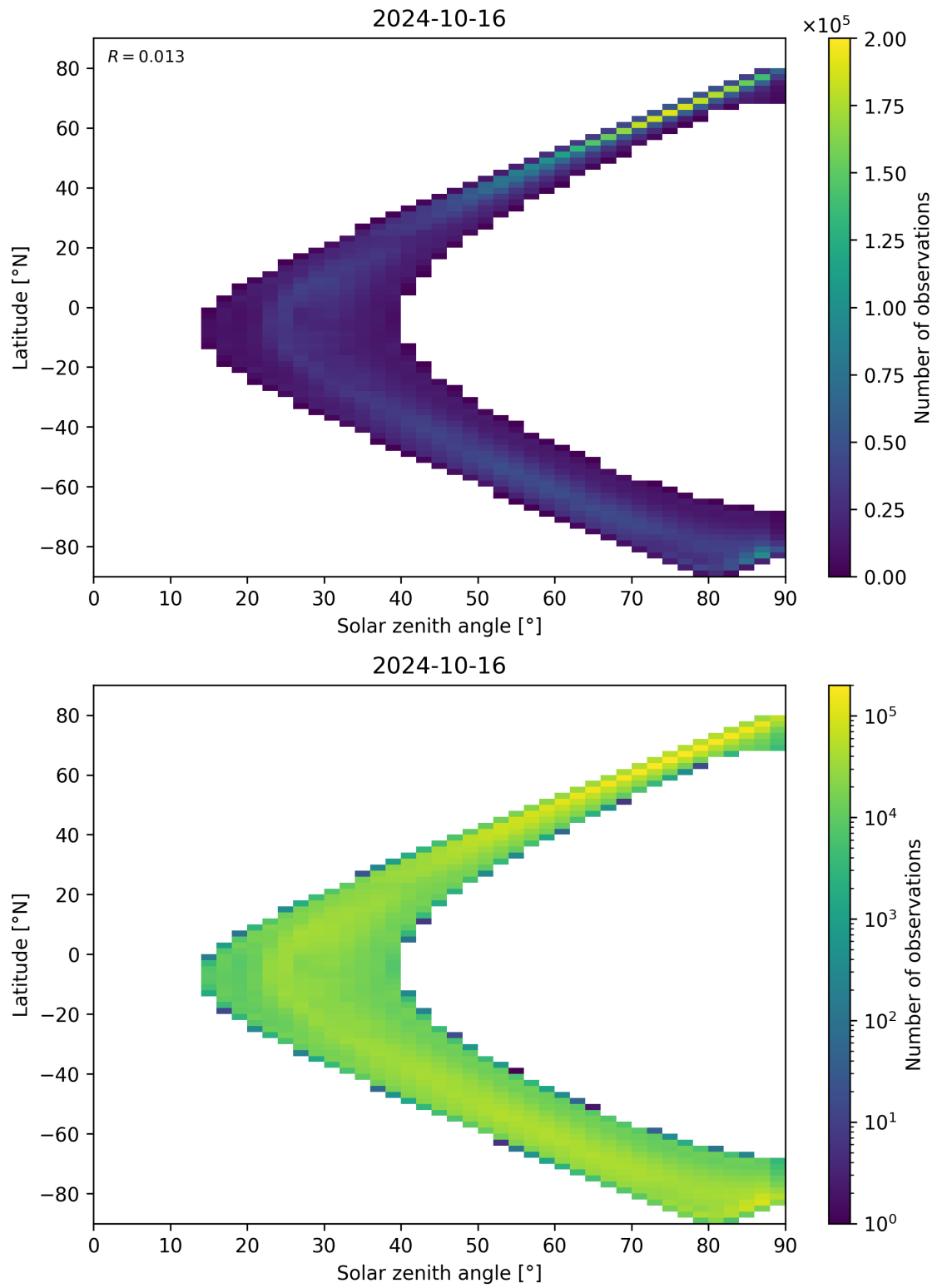
Figure 105: Scatter density plot of “Solar zenith angle” against “Latitude” for 2024-10-15 to 2024-10-17.
