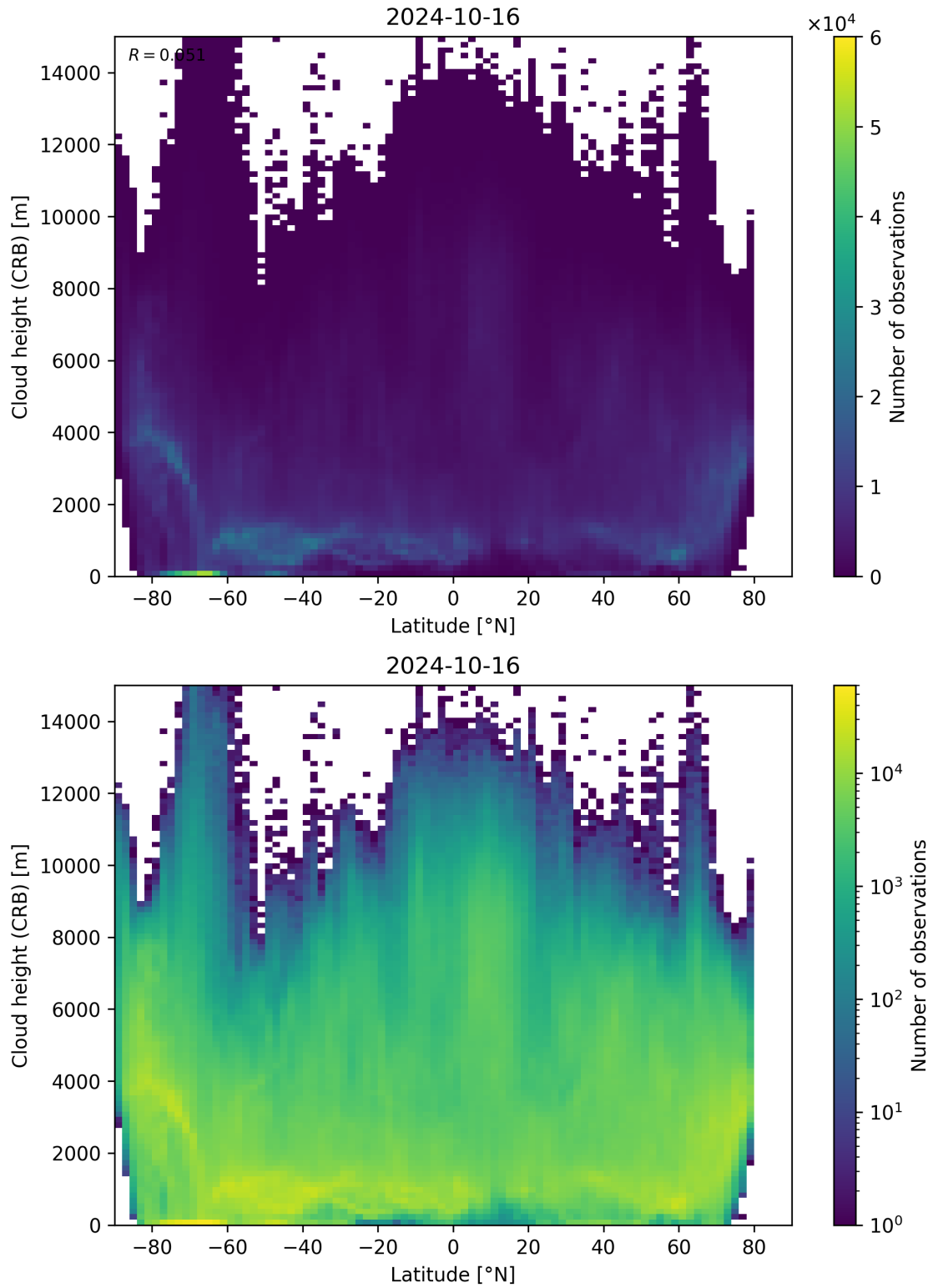
Figure 95: Scatter density plot of “Latitude” against “Cloud height (CRB)” for 2024-10-15 to 2024-10-17.
