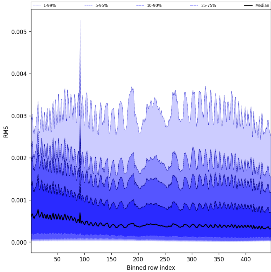
Figure 63: Along track statistics of “RMS” for 2024-10-15 to 2024-10-17
