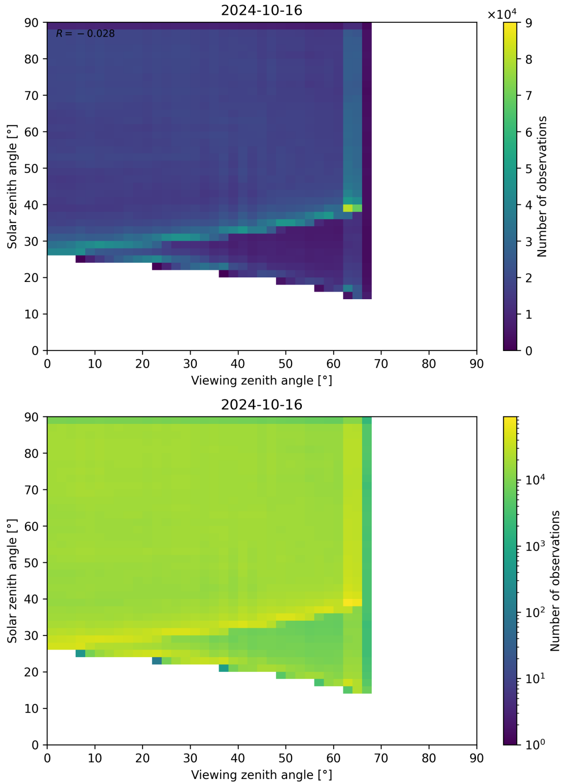
Figure 114: Scatter density plot of “Viewing zenith angle” against “Solar zenith angle” for 2024-10-15 to 2024-10-17.
