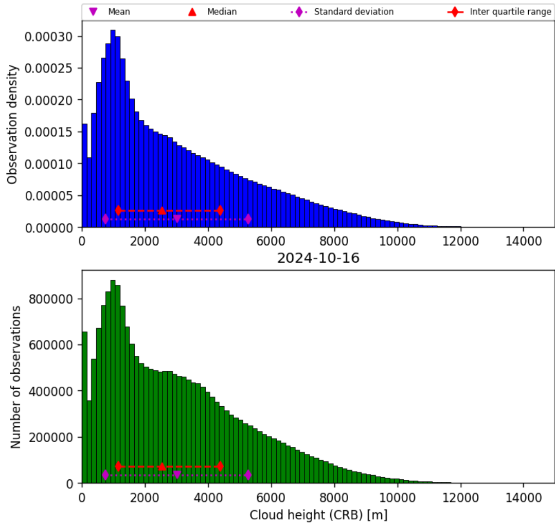
Figure 43: Histogram of “Cloud height (CRB)” for 2024-10-15 to 2024-10-17
