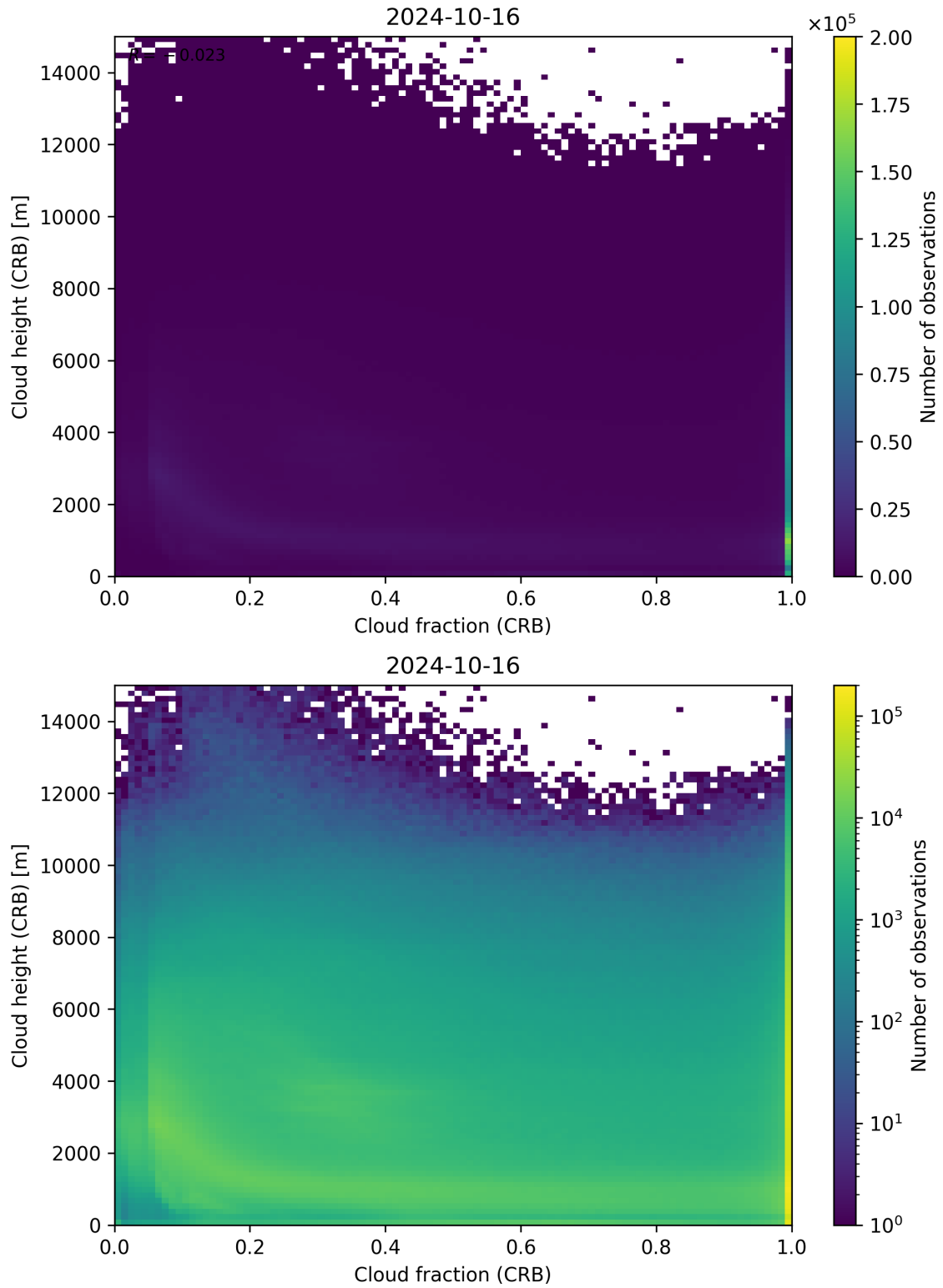
Figure 79: Scatter density plot of “Cloud fraction (CRB)” against “Cloud height (CRB)” for 2024-10-15 to 2024-10-17.
