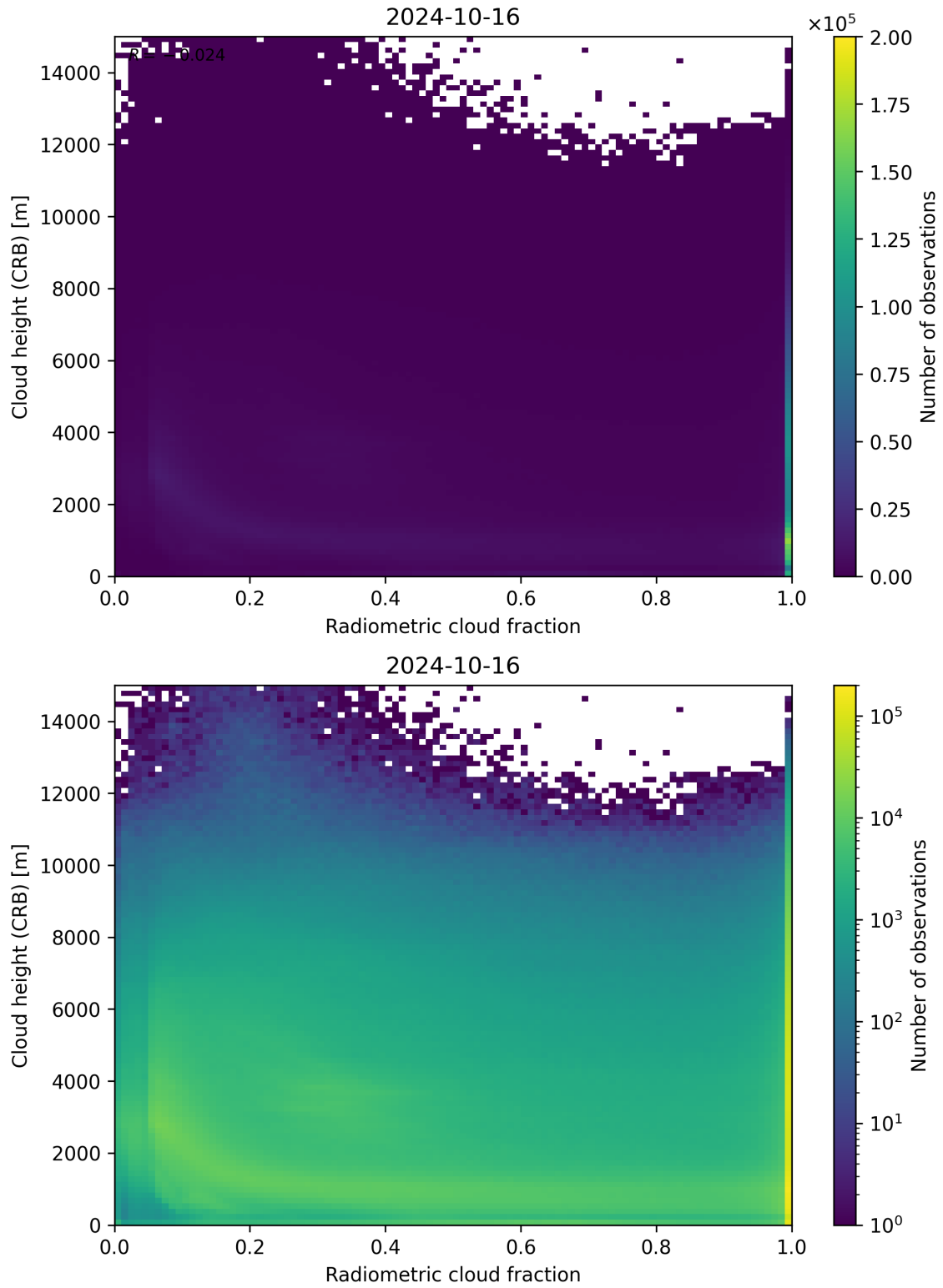
Figure 74: Scatter density plot of “Radiometric cloud fraction” against “Cloud height (CRB)” for 2024-10-15 to 2024-10-17.
