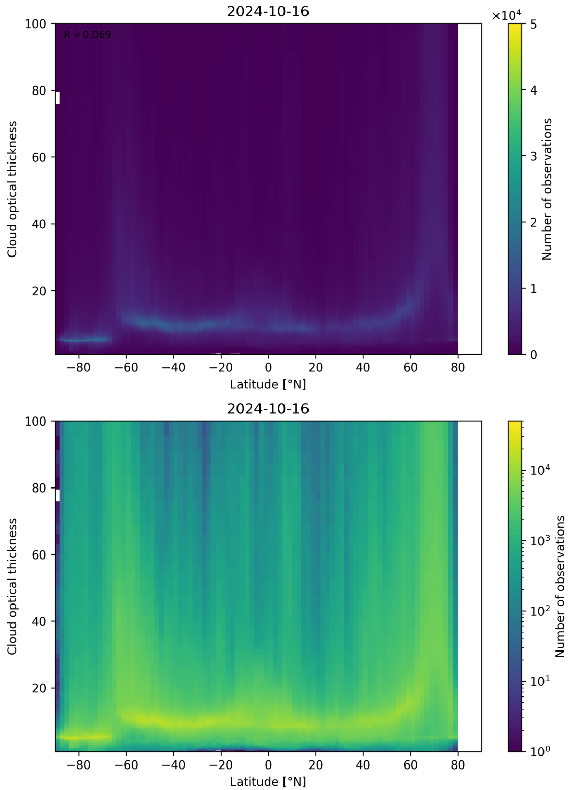
Figure 96: Scatter density plot of “Latitude” against “Cloud optical thickness” for 2024-10-15 to 2024-10-17.
