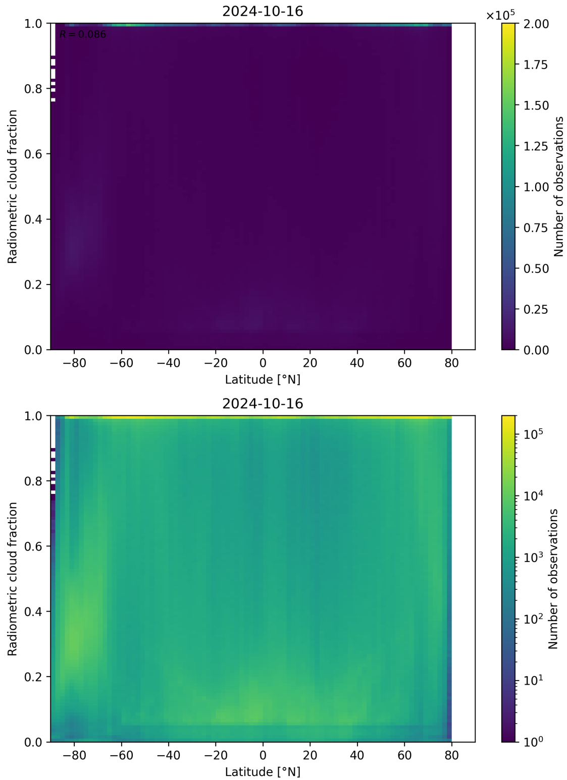
Figure 92: Scatter density plot of “Latitude” against “Radiometric cloud fraction” for 2024-10-15 to 2024-10-17.
