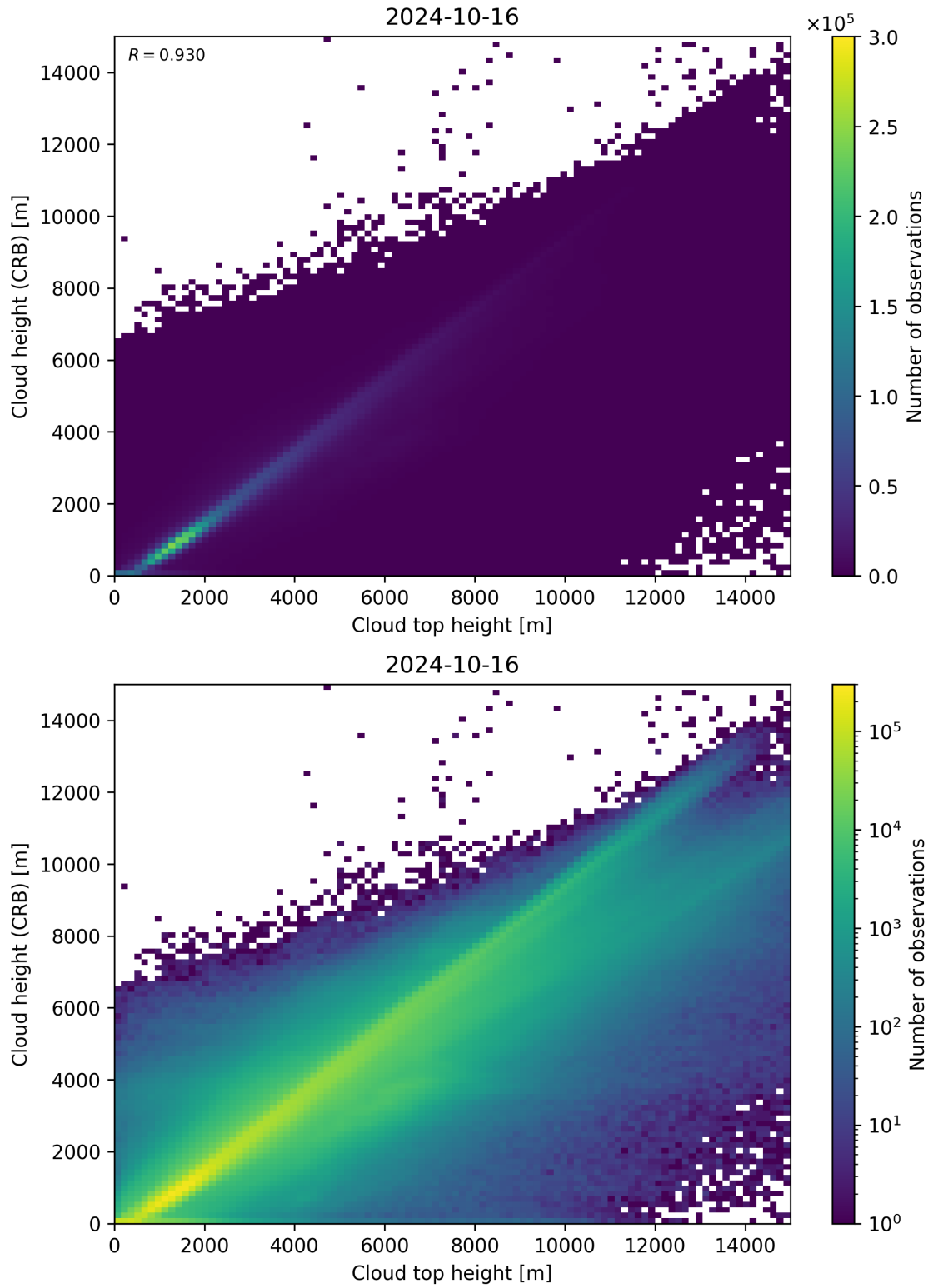
Figure 89: Scatter density plot of “Cloud top height” against “Cloud height (CRB)” for 2024-10-15 to 2024-10-17.
