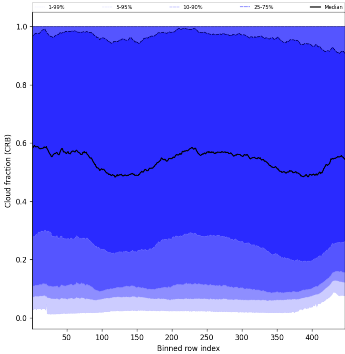
Figure 58: Along track statistics of “Cloud fraction (CRB)” for 2024-10-15 to 2024-10-17
