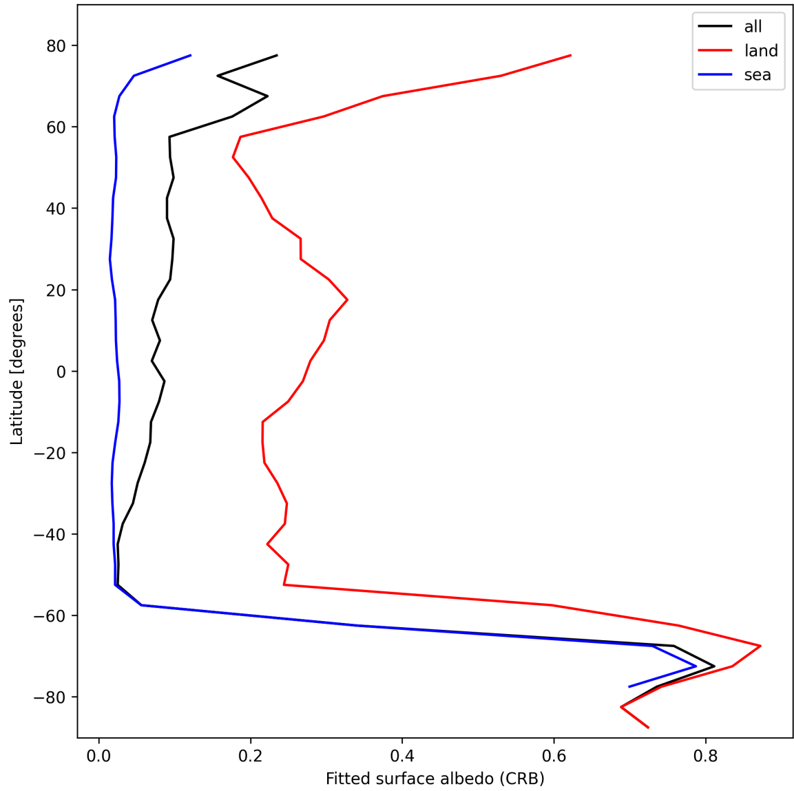
Figure 30: Zonal average of “Fitted surface albedo (CRB)” for 2024-10-15 to 2024-10-17.
