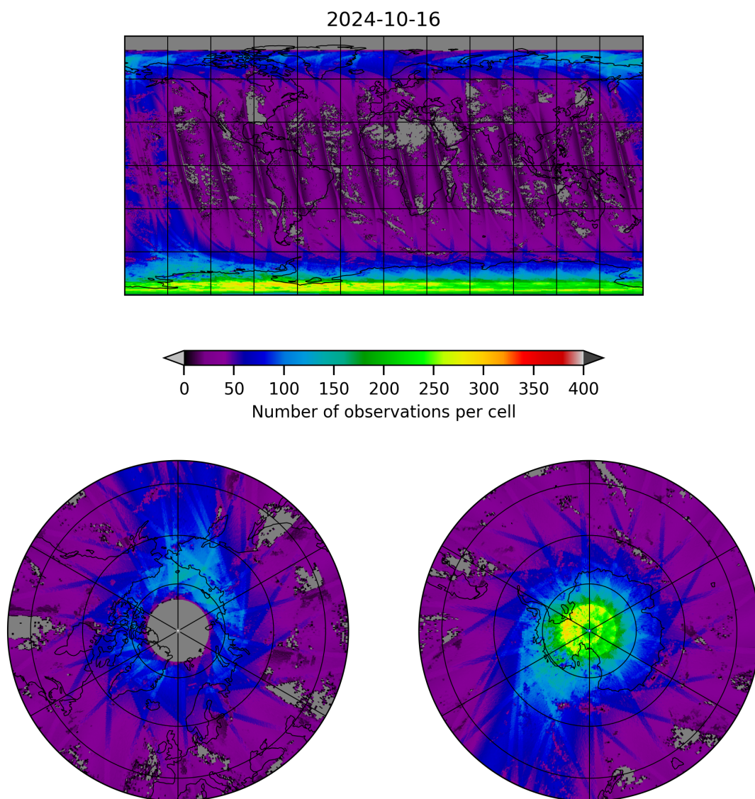
Figure 21: Map of the number of observations for 2024-10-15 to 2024-10-17
