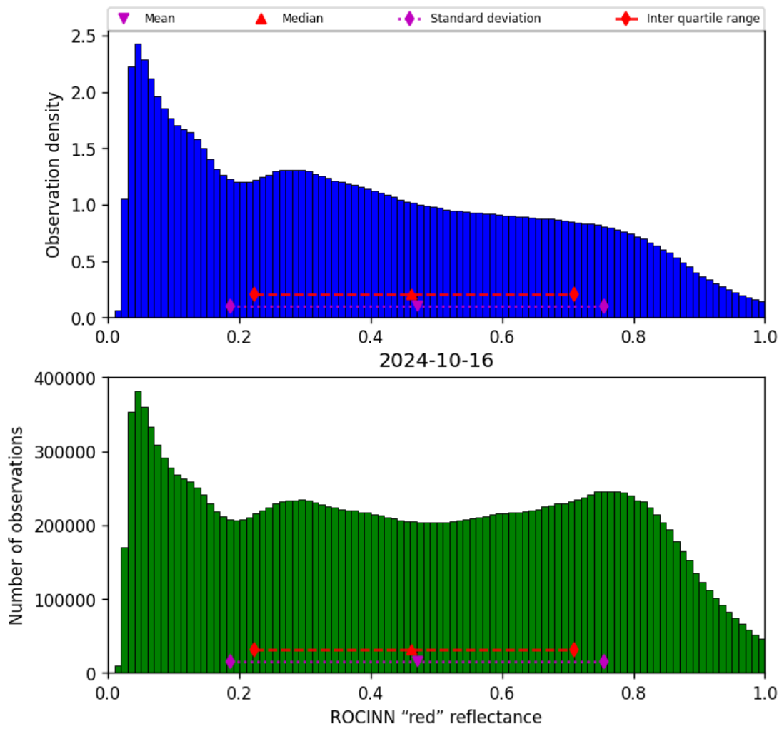
Figure 53: Histogram of “ROCINN “red” reflectance” for 2024-10-15 to 2024-10-17
