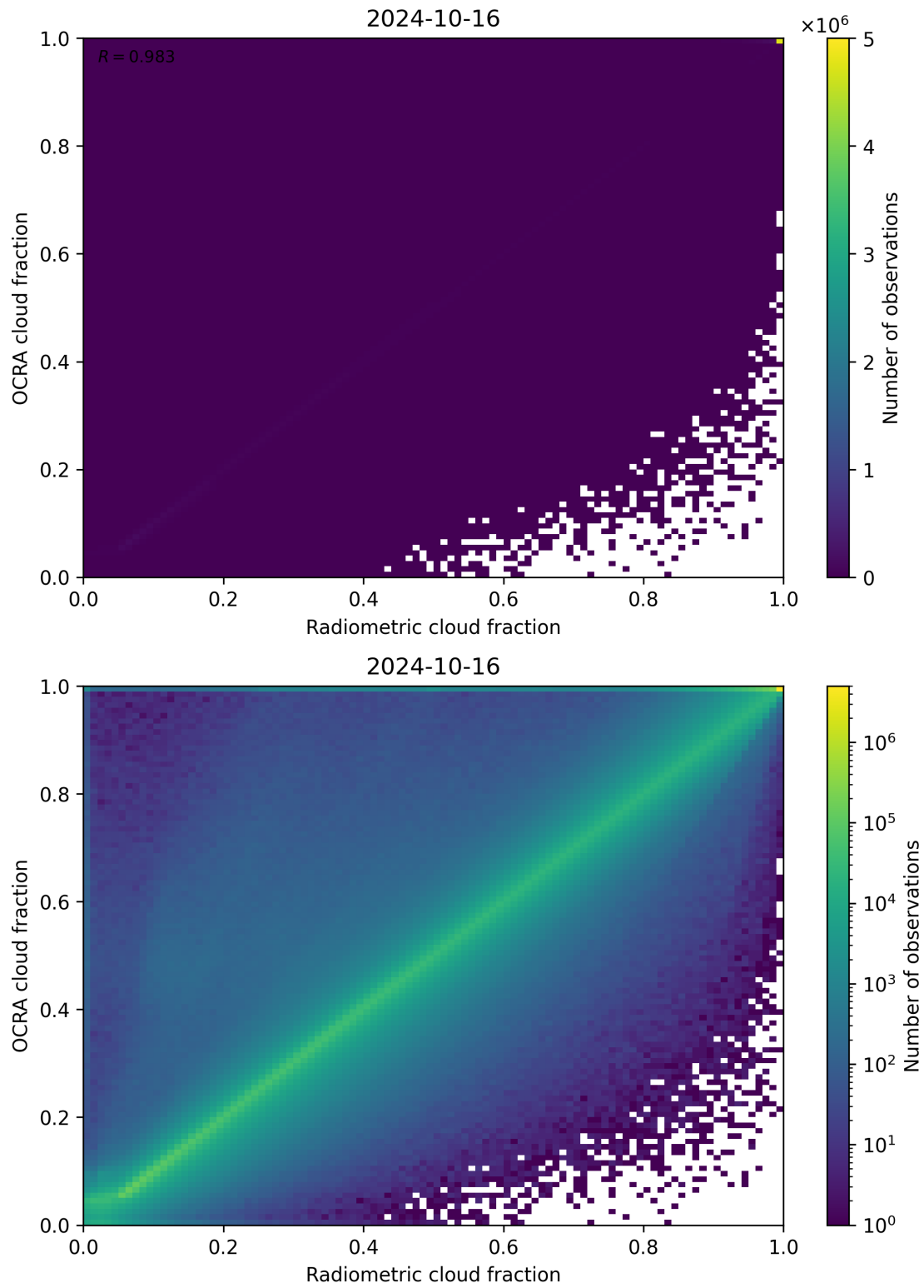
Figure 72: Scatter density plot of “Radiometric cloud fraction” against “OCRA cloud fraction” for 2024-10-15 to 2024-10-17.
