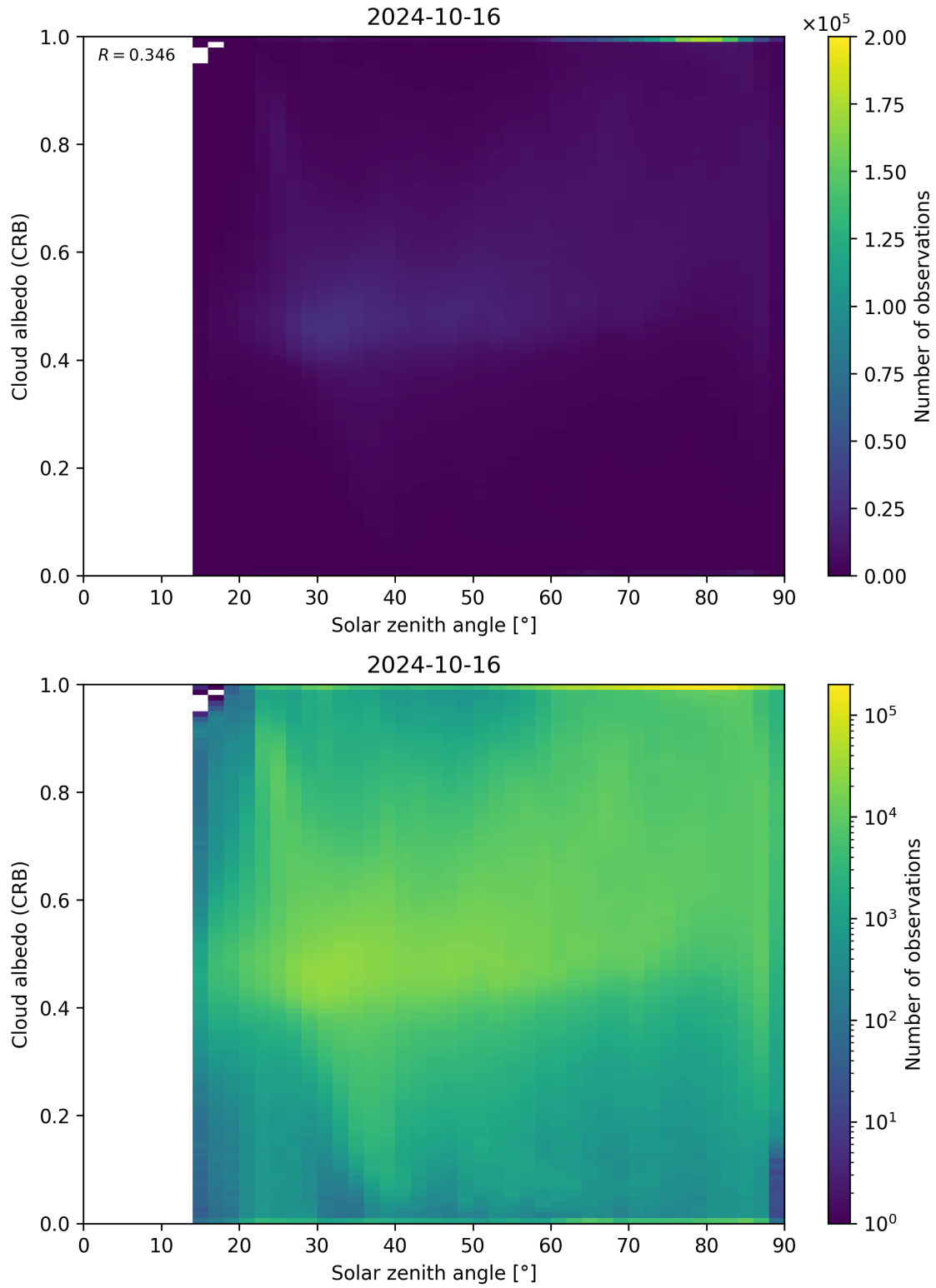
Figure 98: Scatter density plot of “Solar zenith angle” against “Cloud albedo (CRB)” for 2024-10-15 to 2024-10-17.
