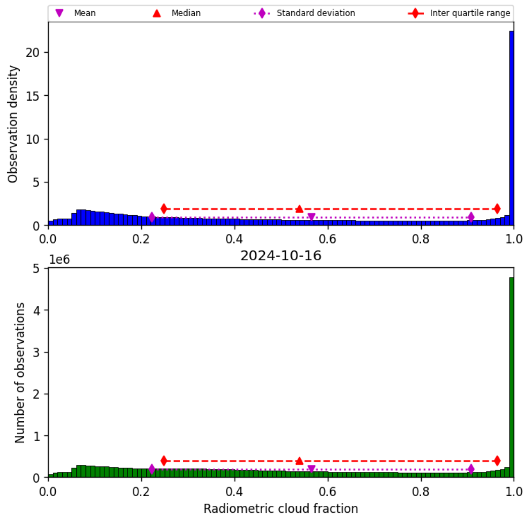
Figure 39: Histogram of “Radiometric cloud fraction” for 2024-10-15 to 2024-10-17
