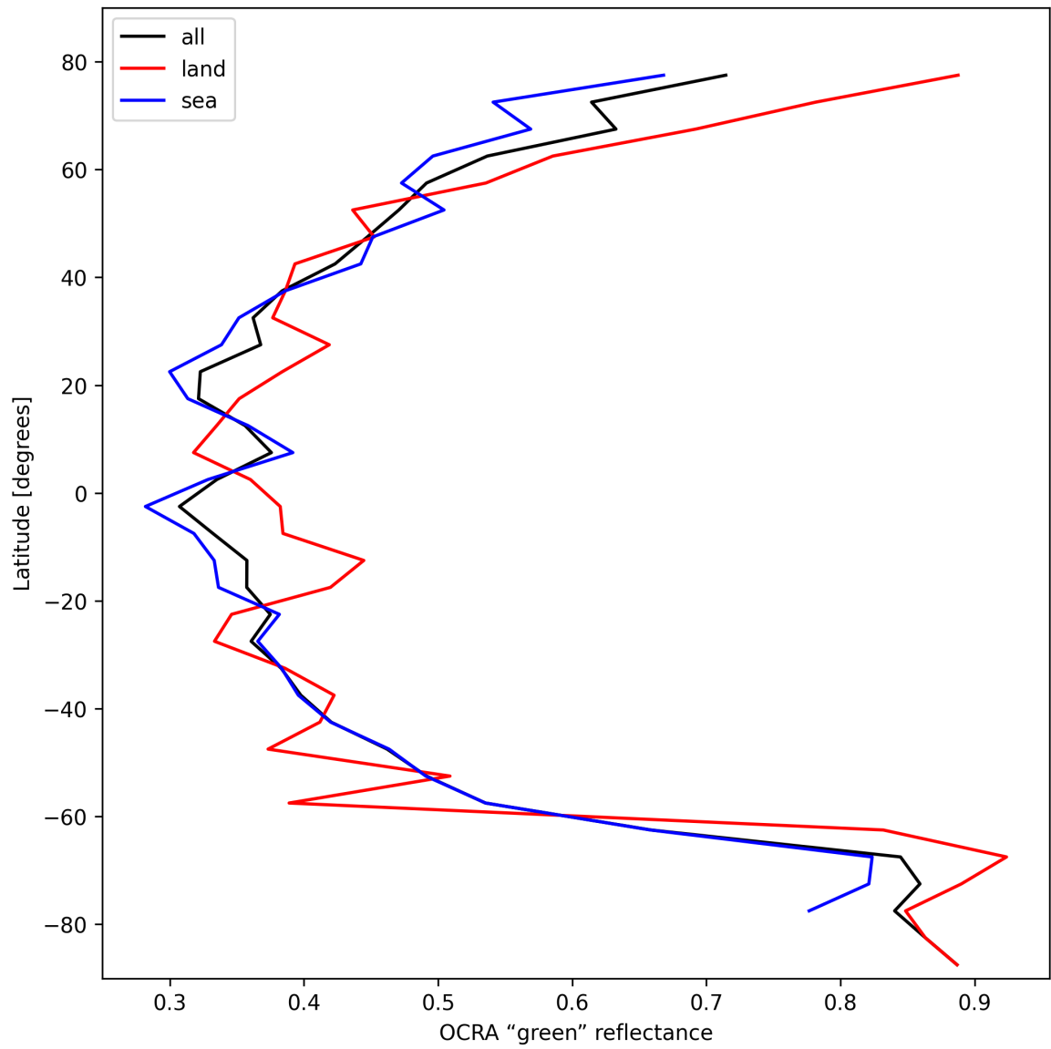
Figure 36: Zonal average of “OCRA “green” reflectance” for 2024-10-15 to 2024-10-17.
