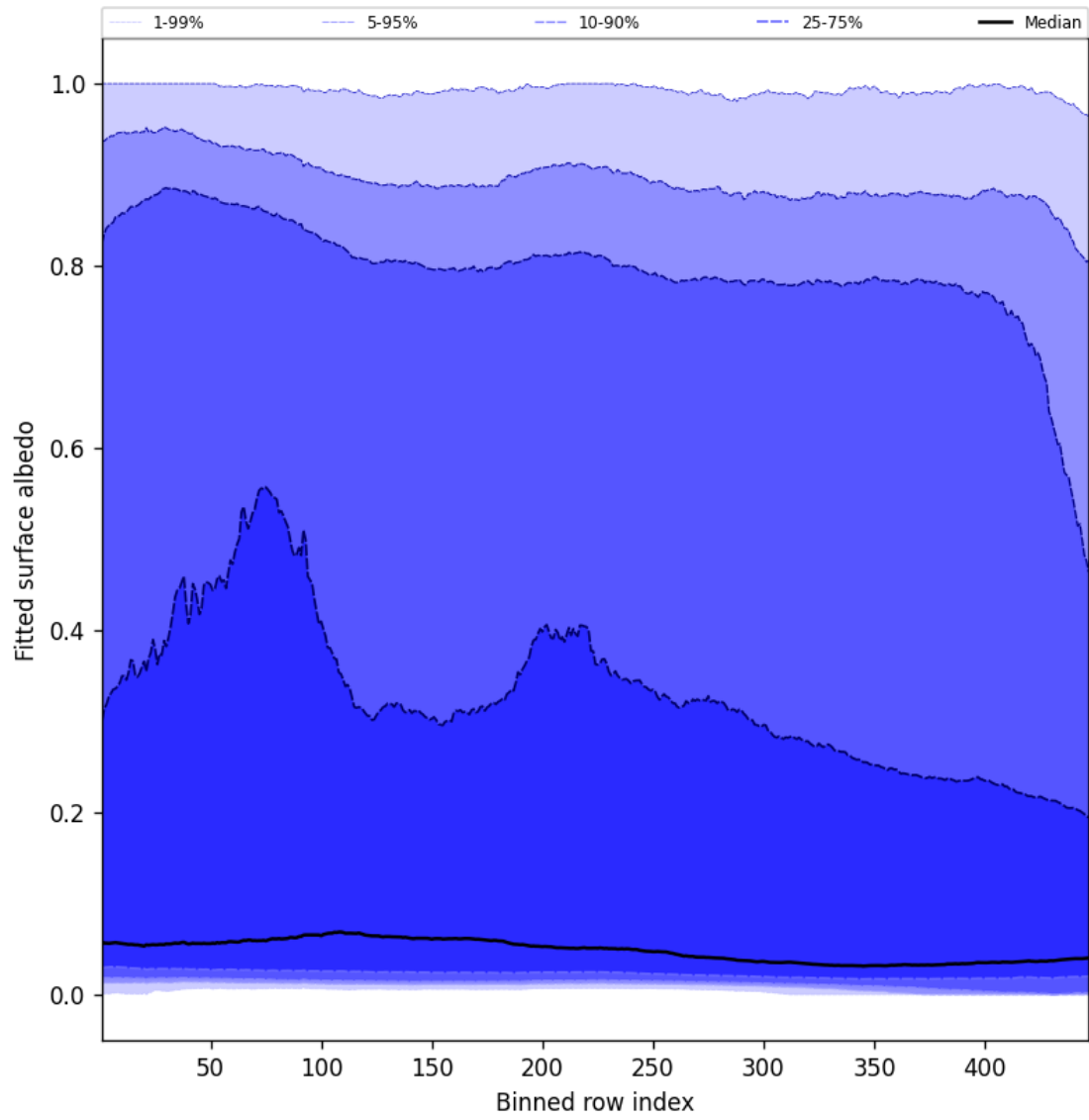
Figure 61: Along track statistics of “Fitted surface albedo” for 2024-10-15 to 2024-10-17
