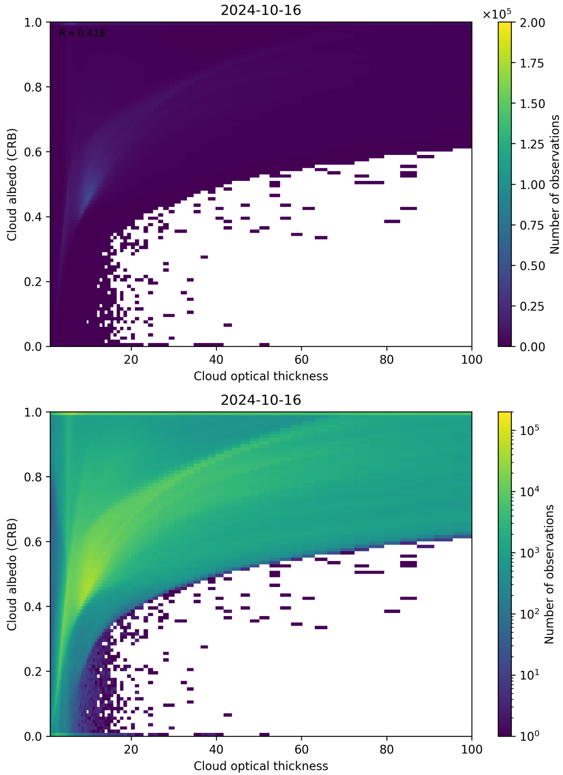
Figure 82: Scatter density plot of “Cloud optical thickness” against “Cloud albedo (CRB)” for 2024-10-15 to 2024-10-17.
