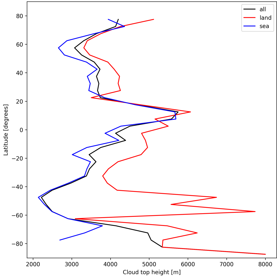
Figure 24: Zonal average of “Cloud top height” for 2024-10-15 to 2024-10-17.
