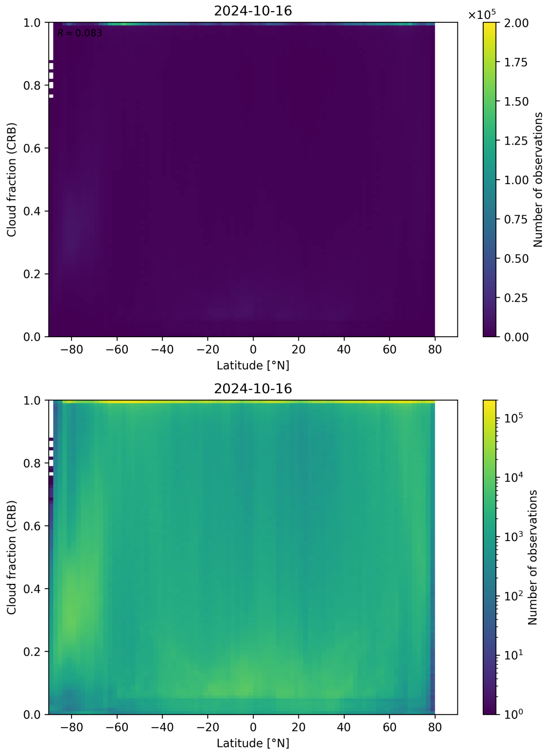
Figure 94: Scatter density plot of “Latitude” against “Cloud fraction (CRB)” for 2024-10-15 to 2024-10-17.
