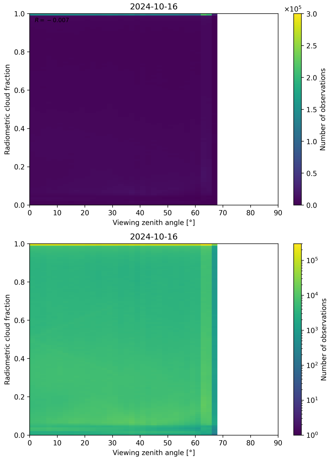
Figure 107: Scatter density plot of “Viewing zenith angle” against “Radiometric cloud fraction” for 2024-10-15 to 2024-10-17.
