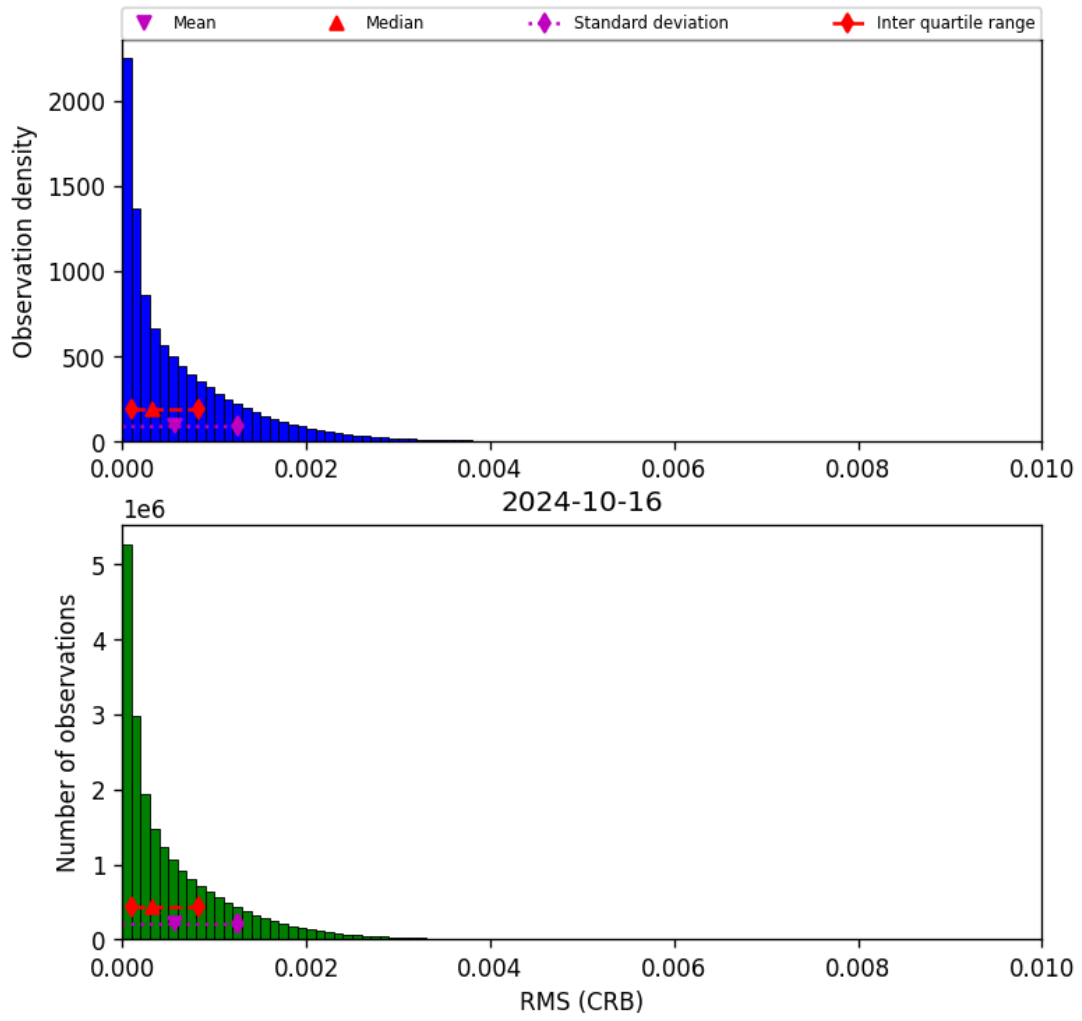
Figure 48: Histogram of “RMS (CRB)” for 2024-10-15 to 2024-10-17
