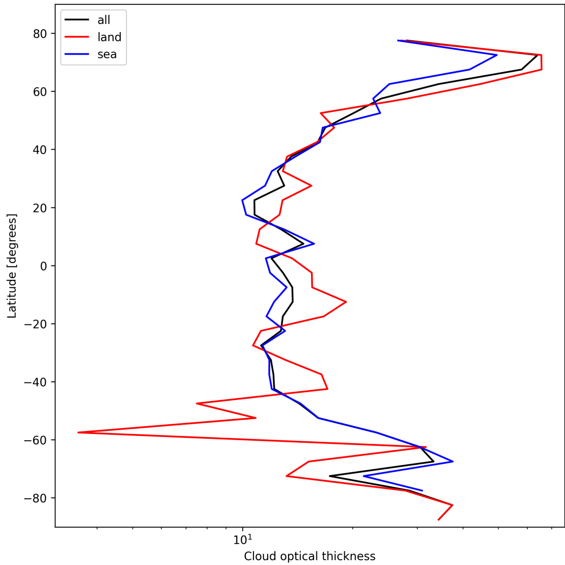
Figure 25: Zonal average of “Cloud optical thickness” for 2024-10-15 to 2024-10-17.
