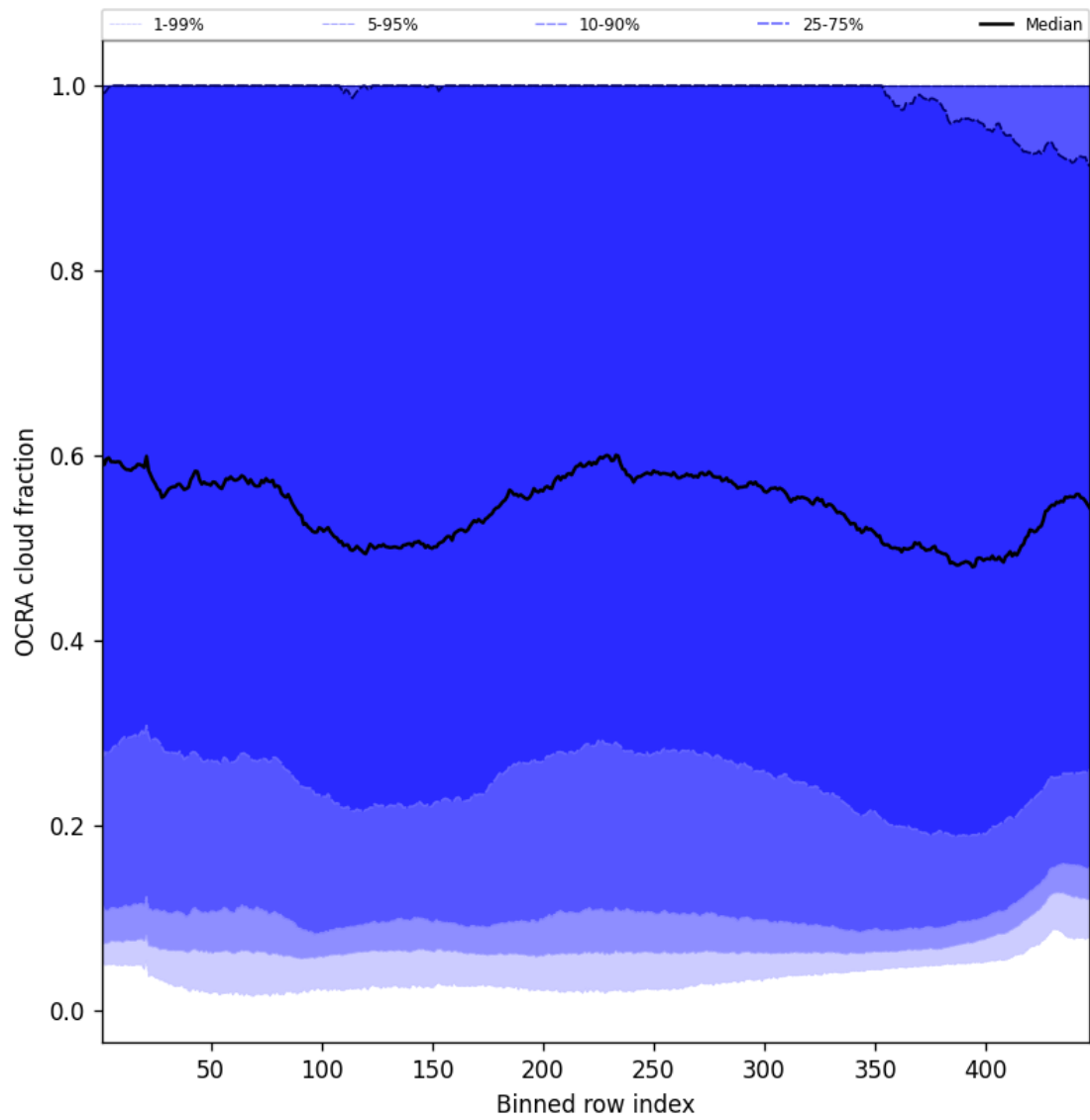
Figure 66: Along track statistics of “OCRA cloud fraction” for 2024-10-15 to 2024-10-17
