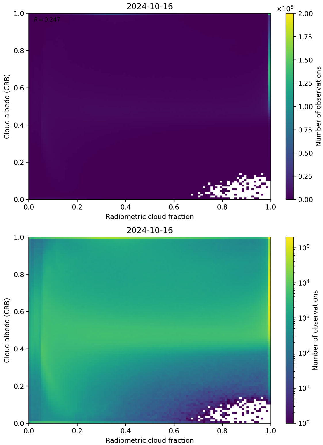
Figure 71: Scatter density plot of “Radiometric cloud fraction” against “Cloud albedo (CRB)” for 2024-10-15 to 2024-10-17.
