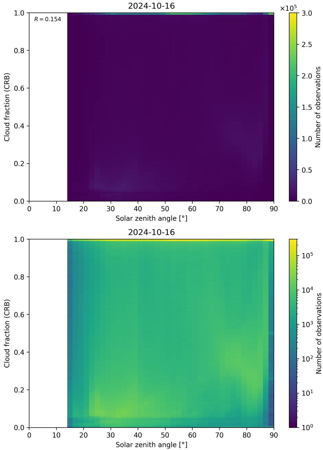
Figure 101: Scatter density plot of “Solar zenith angle” against “Cloud fraction (CRB)” for 2024-10-15 to 2024-10-17.
