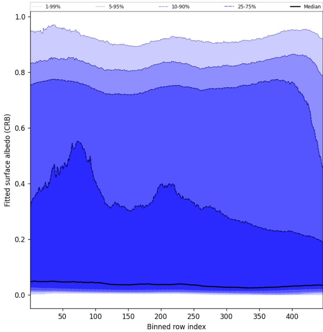
Figure 62: Along track statistics of “Fitted surface albedo (CRB)” for 2024-10-15 to 2024-10-17
