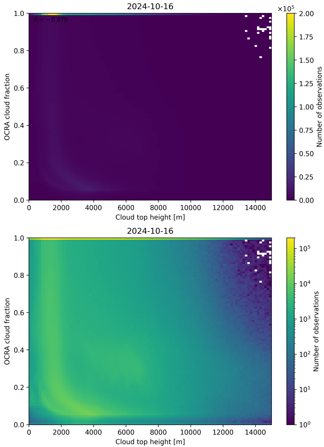
Figure 87: Scatter density plot of “Cloud top height” against “OCRA cloud fraction” for 2024-10-15 to 2024-10-17.
