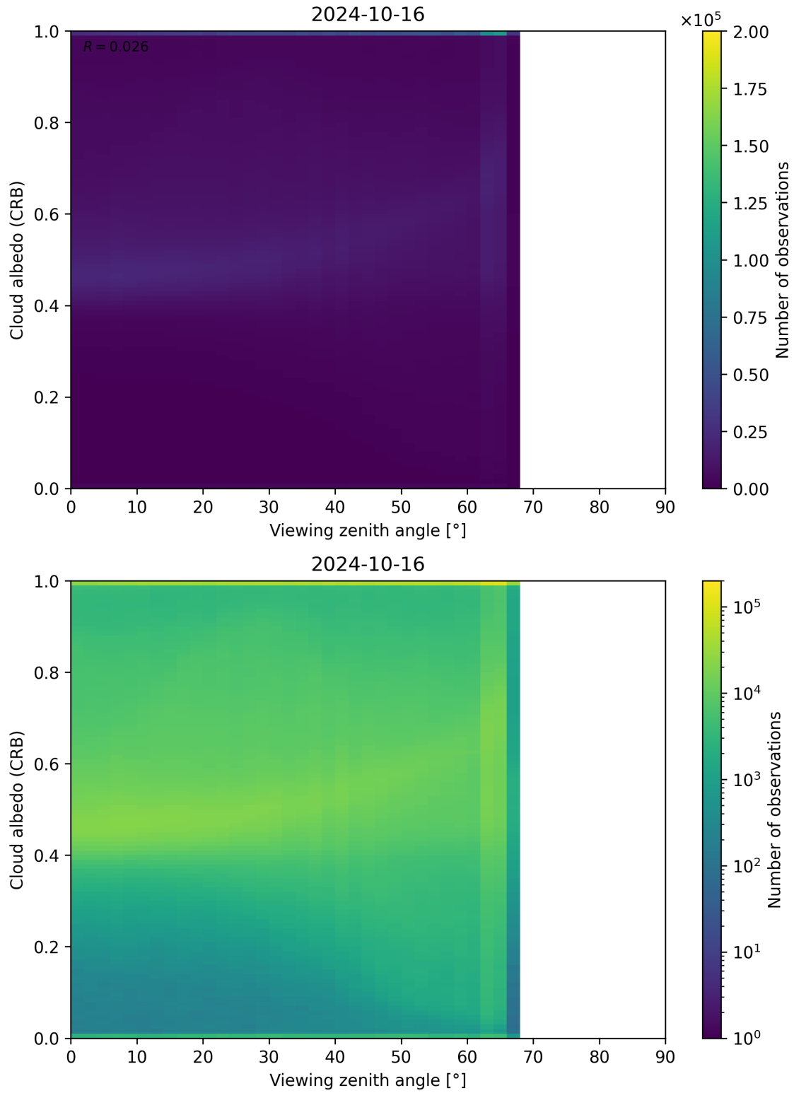
Figure 106: Scatter density plot of “Viewing zenith angle” against “Cloud albedo (CRB)” for 2024-10-15 to 2024-10-17.
