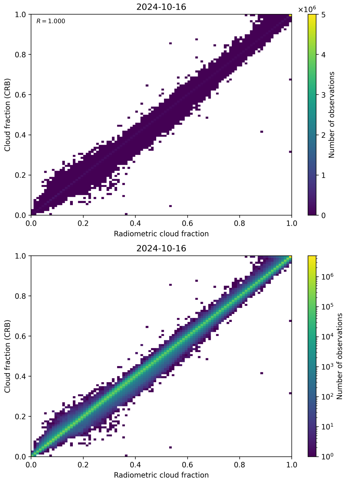
Figure 73: Scatter density plot of “Radiometric cloud fraction” against “Cloud fraction (CRB)” for 2024-10-15 to 2024-10-17.
