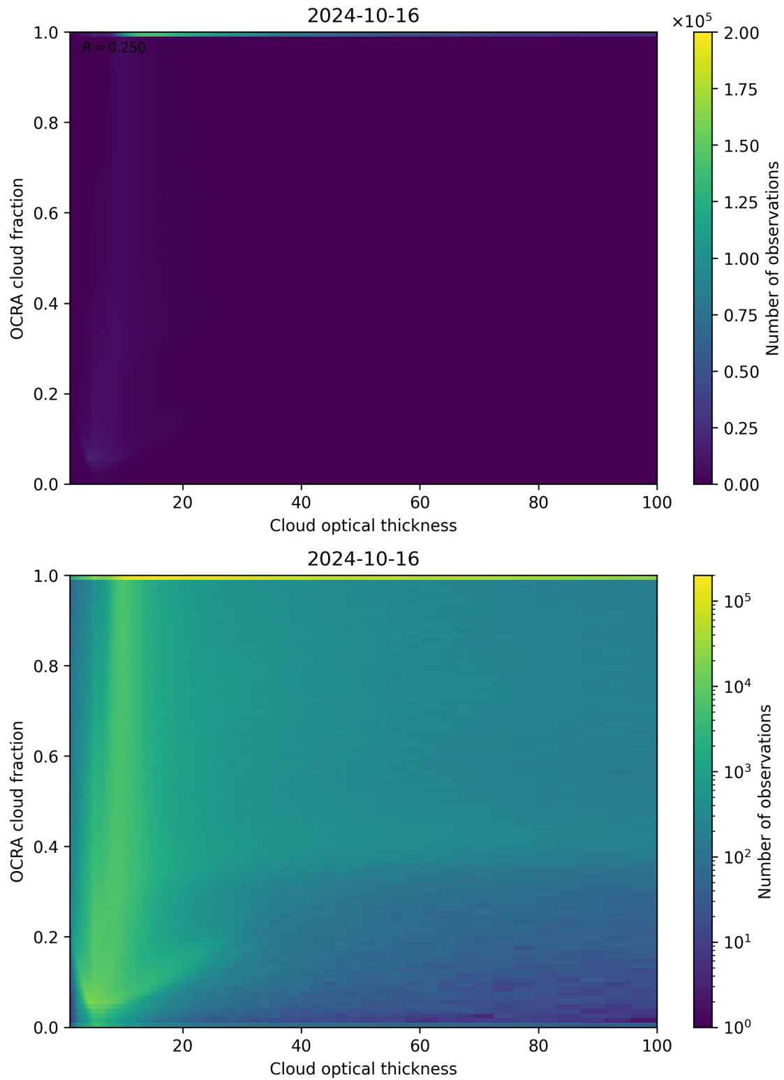
Figure 83: Scatter density plot of “Cloud optical thickness” against “OCRA cloud fraction” for 2024-10-15 to 2024-10-17.
