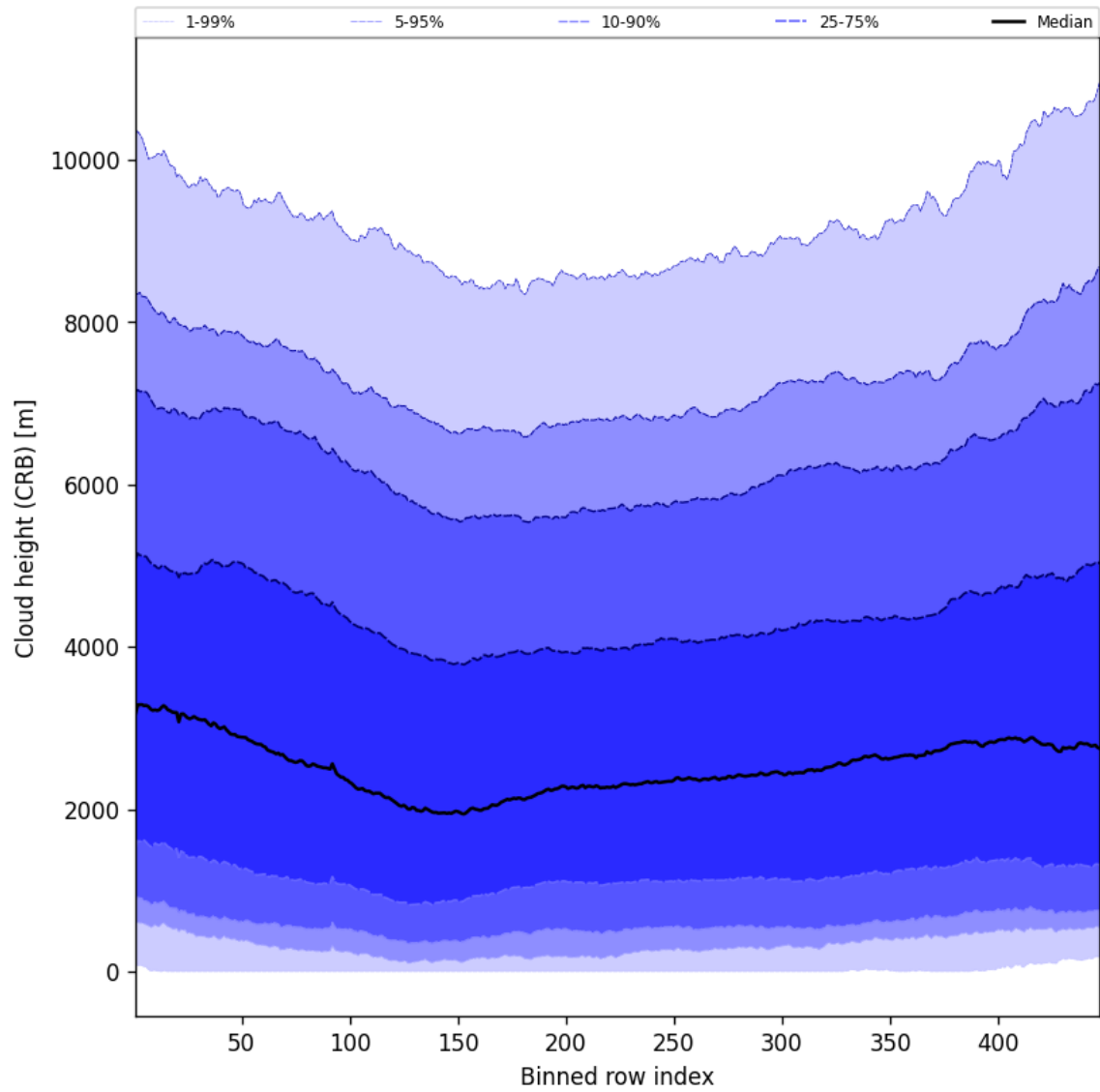
Figure 59: Along track statistics of “Cloud height (CRB)” for 2024-10-15 to 2024-10-17
