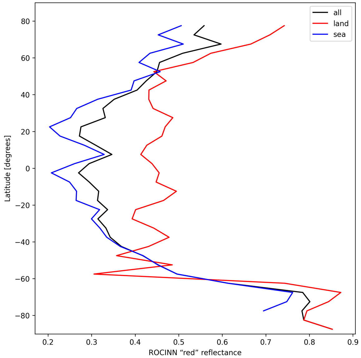
Figure 37: Zonal average of "ROCINN "red" reflectance" for 2024-10-15 to 2024-10-17.
