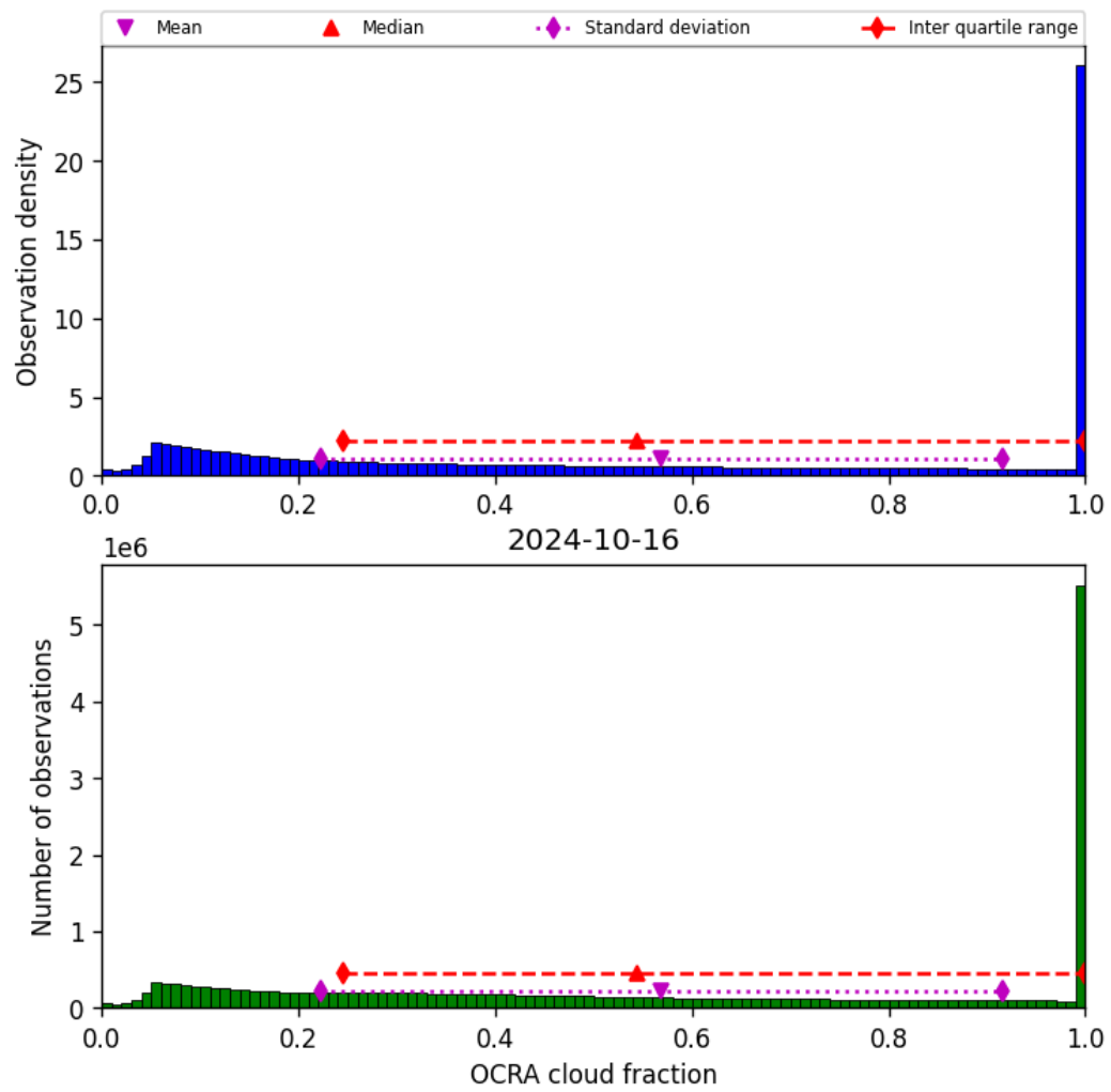
Figure 50: Histogram of “OCRA cloud fraction” for 2024-10-15 to 2024-10-17
