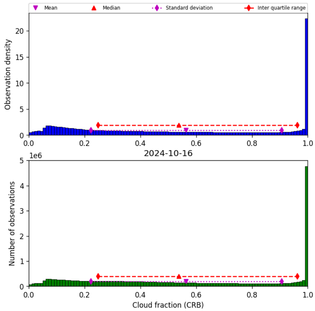
Figure 42: Histogram of “Cloud fraction (CRB)” for 2024-10-15 to 2024-10-17
