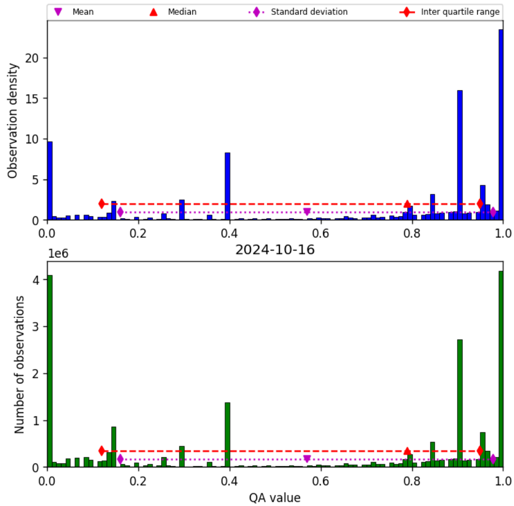
Figure 38: Histogram of “QA value” for 2024-10-15 to 2024-10-17
