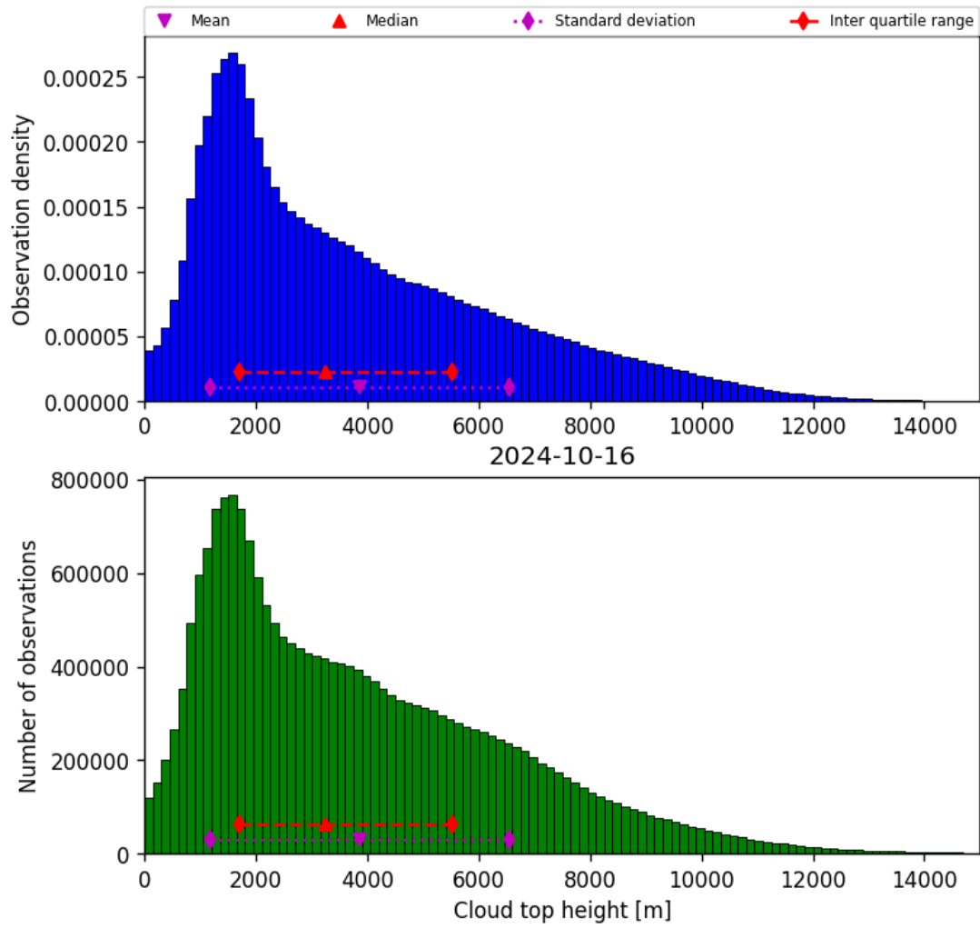
Figure 40: Histogram of “Cloud top height” for 2024-10-15 to 2024-10-17
