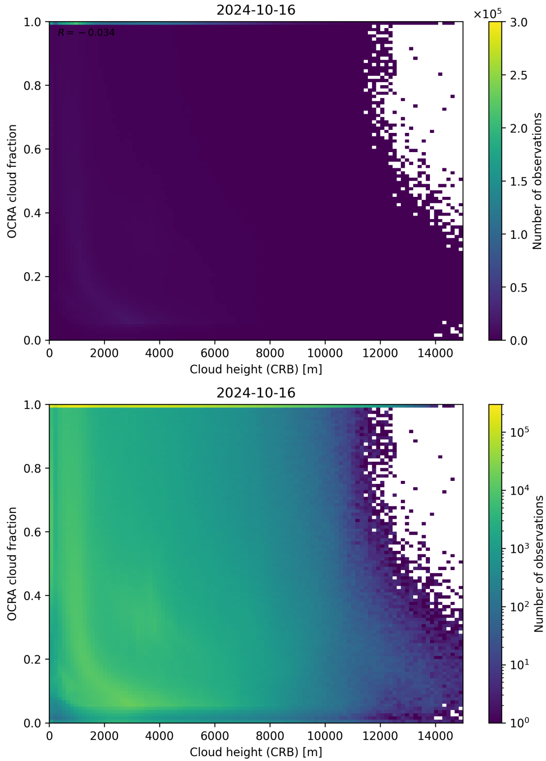
Figure 81: Scatter density plot of “Cloud height (CRB)” against “OCRA cloud fraction” for 2024-10-15 to 2024-10-17.
