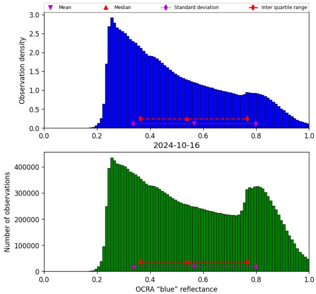
Figure 51: Histogram of “OCRA “blue” reflectance” for 2024-10-15 to 2024-10-17
