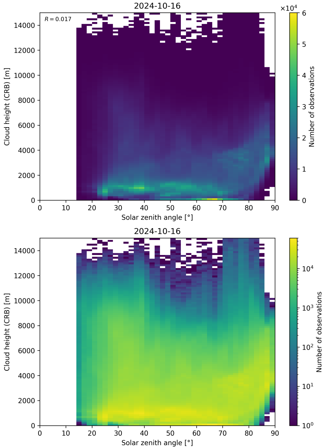
Figure 102: Scatter density plot of “Solar zenith angle” against “Cloud height (CRB)” for 2024-10-15 to 2024-10-17.
