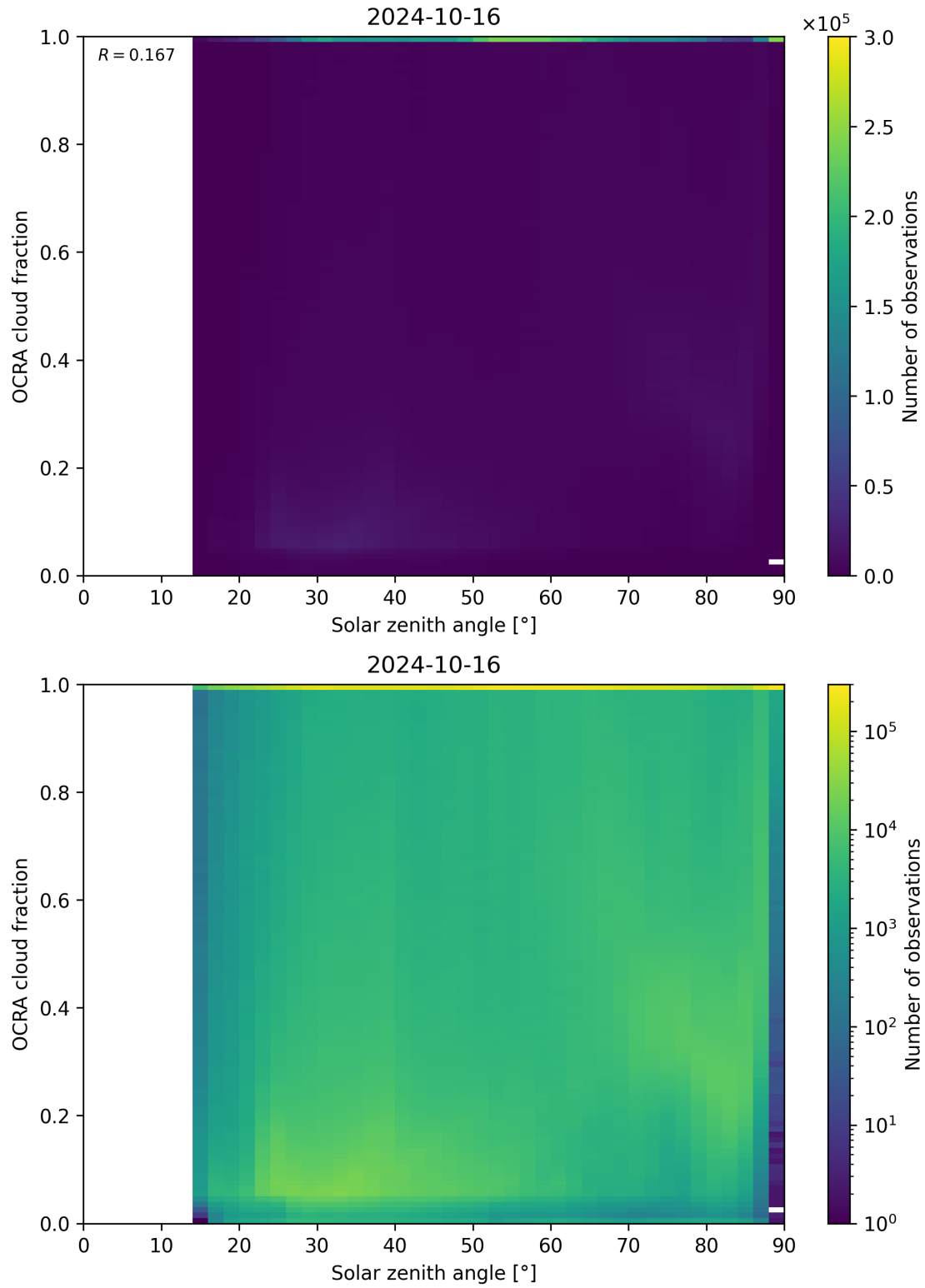
Figure 100: Scatter density plot of “Solar zenith angle” against “OCRA cloud fraction” for 2024-10-15 to 2024-10-17.
