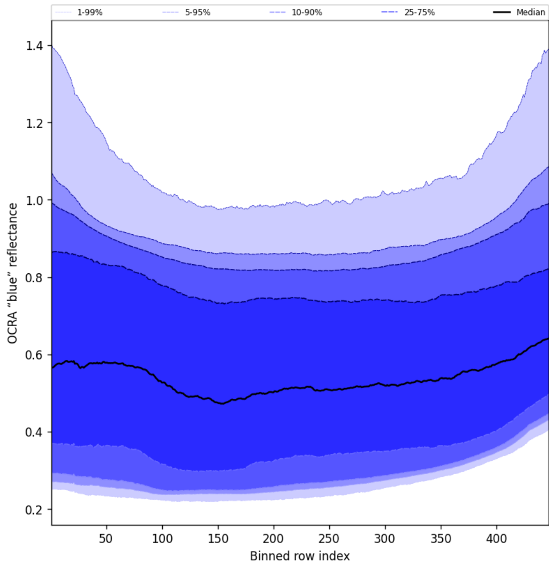
Figure 67: Along track statistics of “OCRA “blue” reflectance” for 2024-10-15 to 2024-10-17
