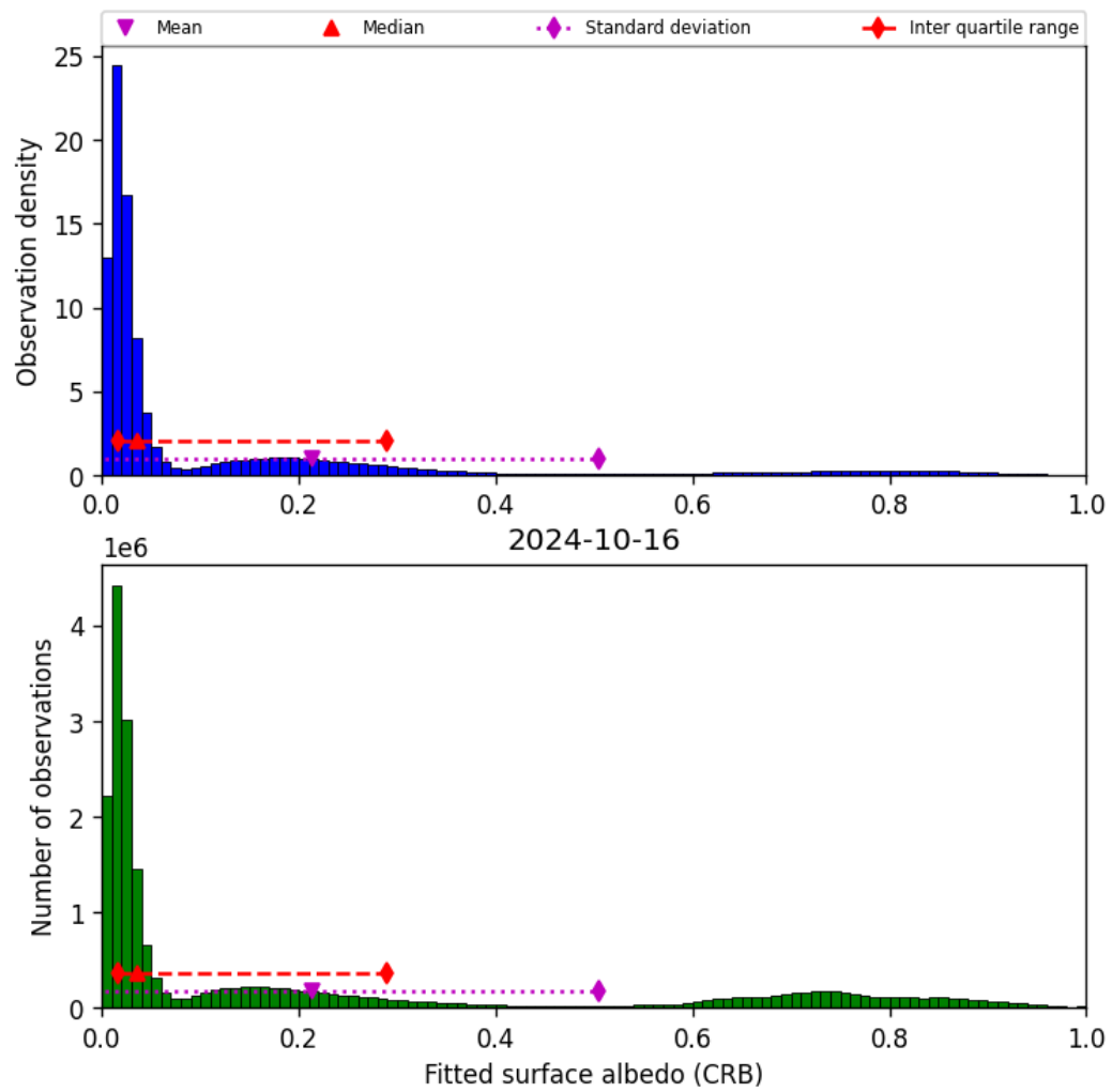
Figure 46: Histogram of “Fitted surface albedo (CRB)” for 2024-10-15 to 2024-10-17
