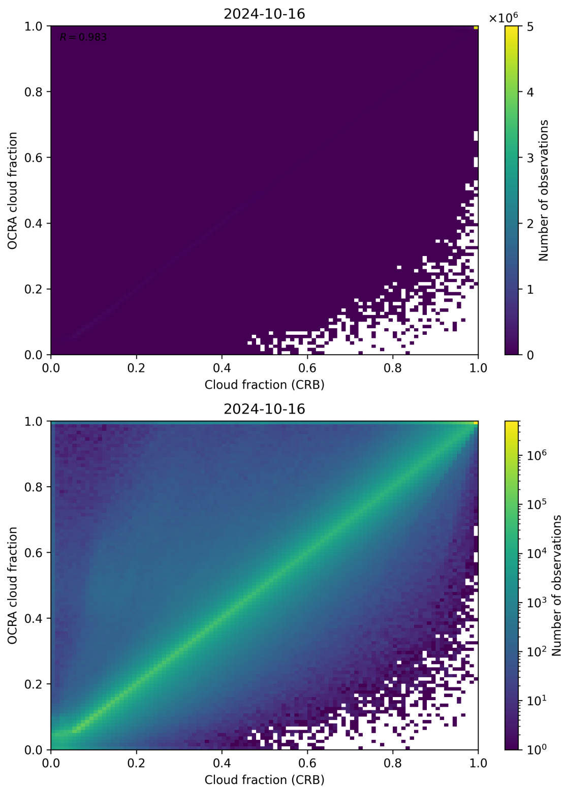
Figure 78: Scatter density plot of “Cloud fraction (CRB)” against “OCRA cloud fraction” for 2024-10-15 to 2024-10-17.
