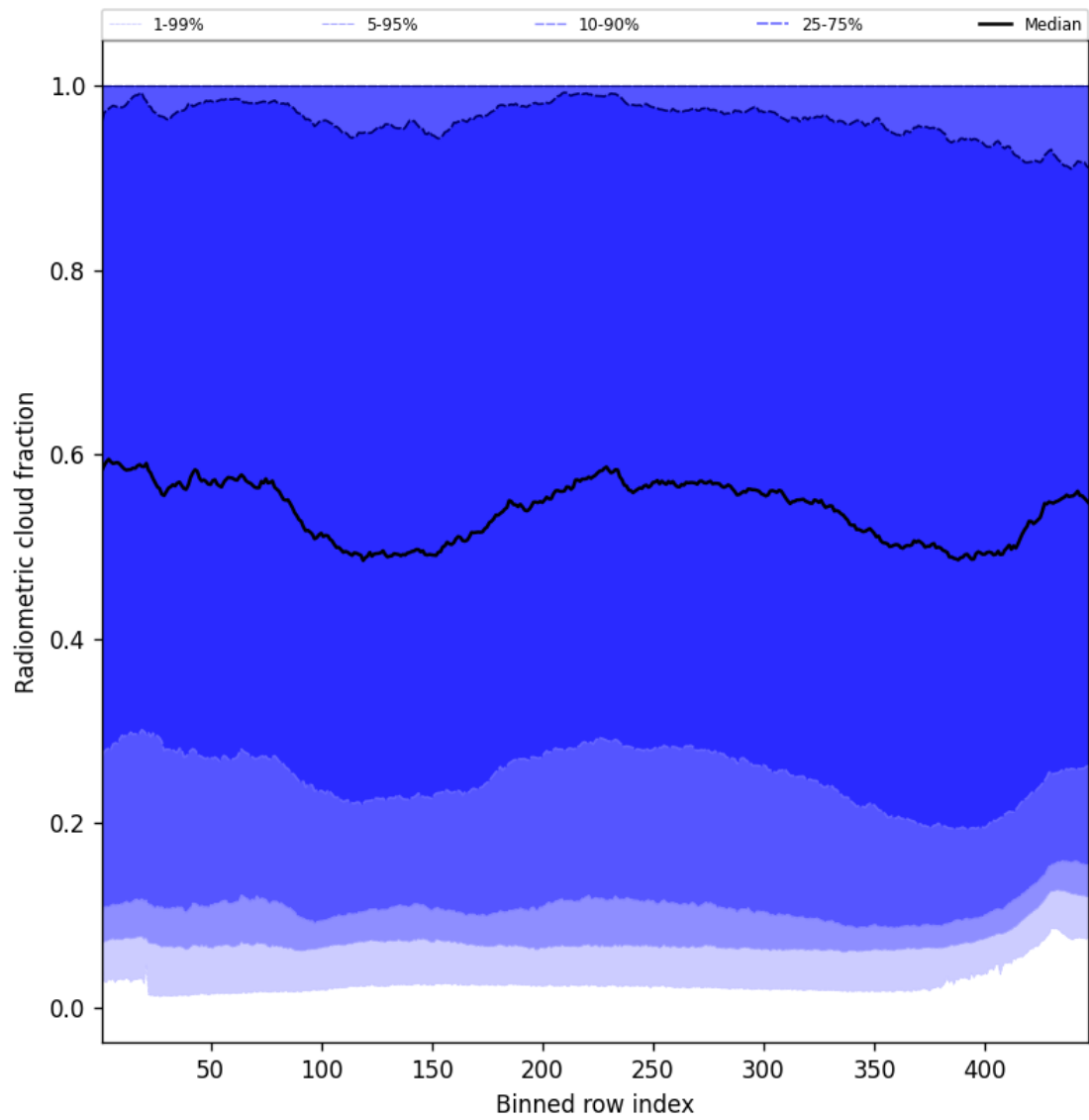
Figure 55: Along track statistics of “Radiometric cloud fraction” for 2024-10-15 to 2024-10-17
