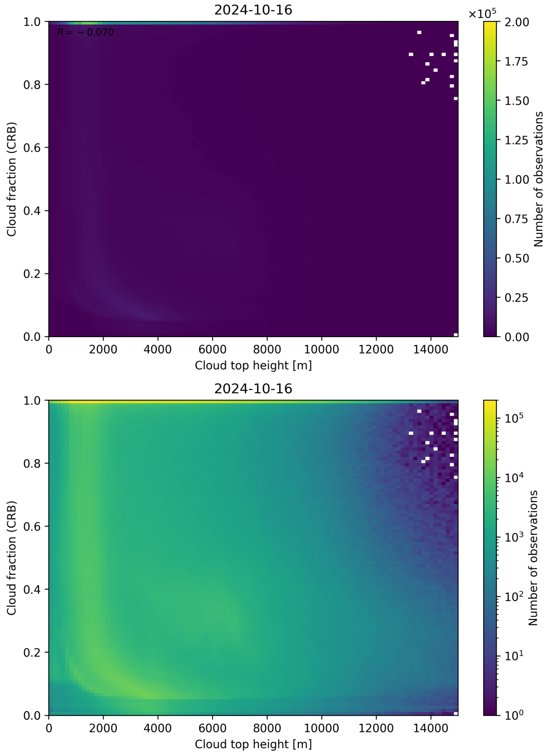
Figure 88: Scatter density plot of “Cloud top height” against “Cloud fraction (CRB)” for 2024-10-15 to 2024-10-17.
