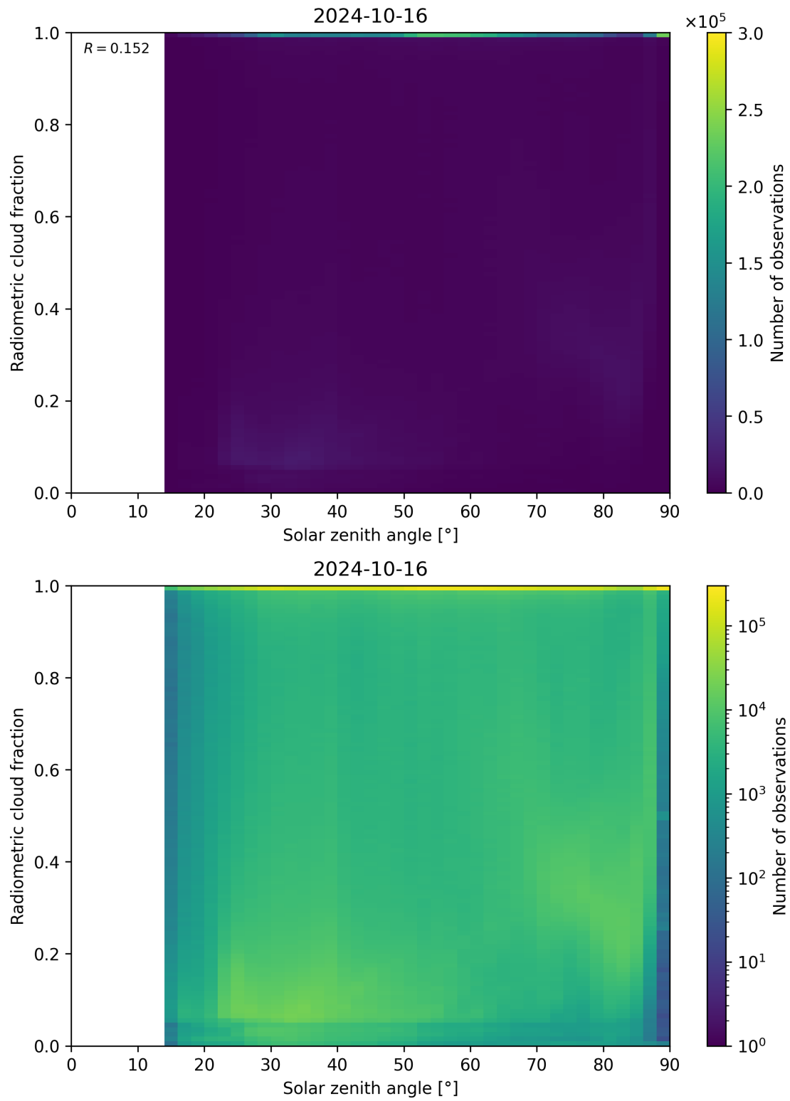
Figure 99: Scatter density plot of “Solar zenith angle” against “Radiometric cloud fraction” for 2024-10-15 to 2024-10-17.
