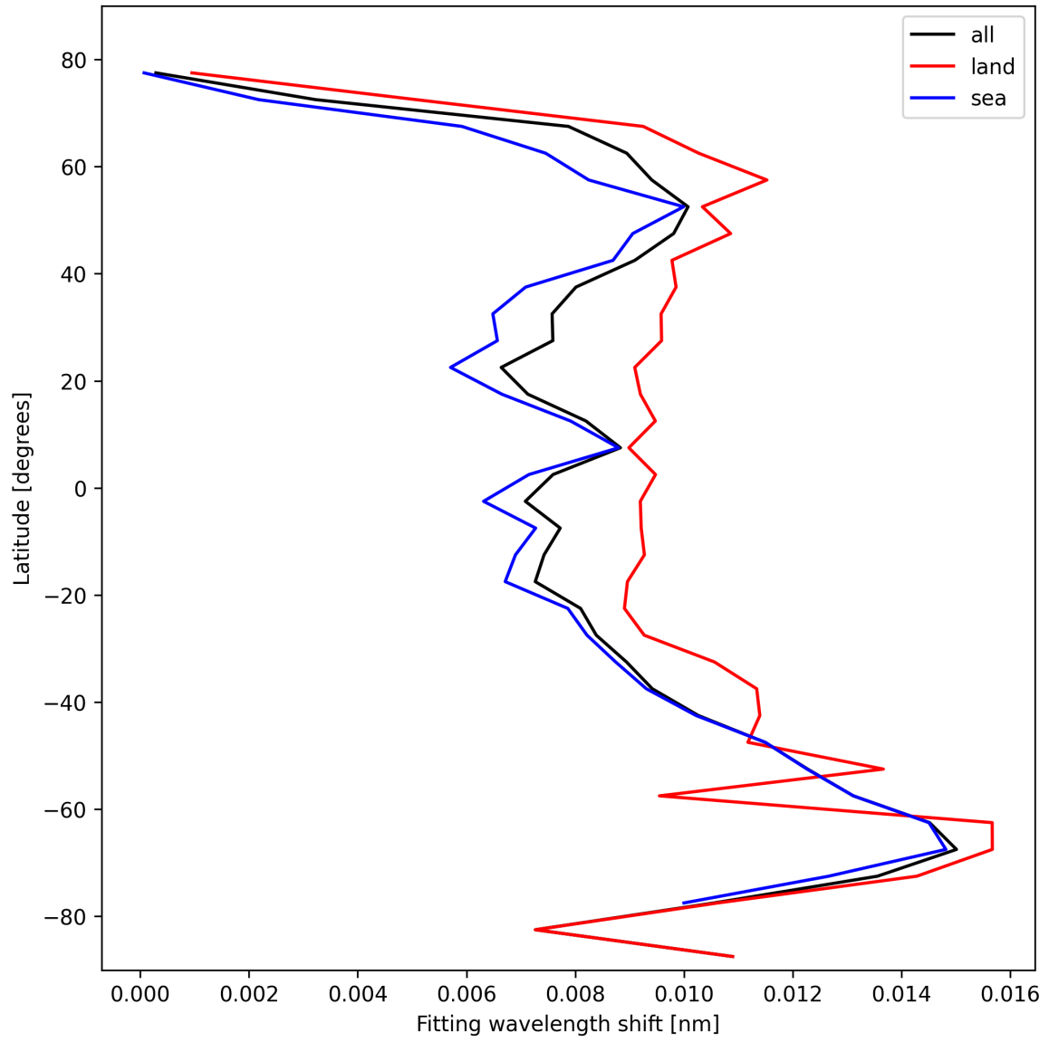
Figure 33: Zonal average of “Fitting wavelength shift” for 2024-10-15 to 2024-10-17.
