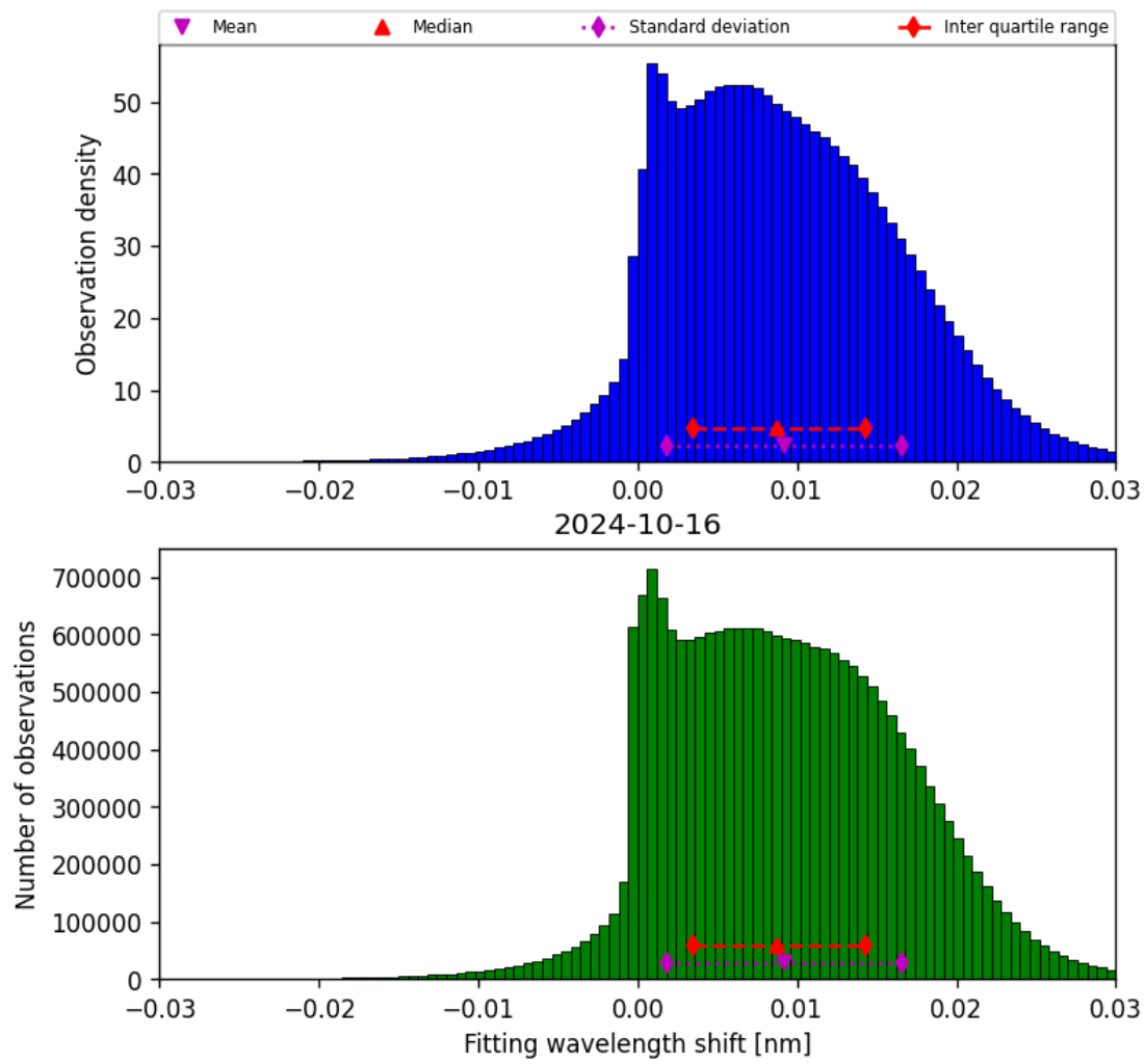
Figure 49: Histogram of “Fitting wavelength shift” for 2024-10-15 to 2024-10-17
