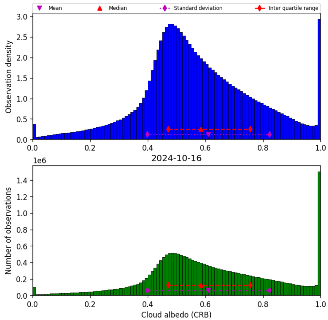
Figure 44: Histogram of “Cloud albedo (CRB)” for 2024-10-15 to 2024-10-17
