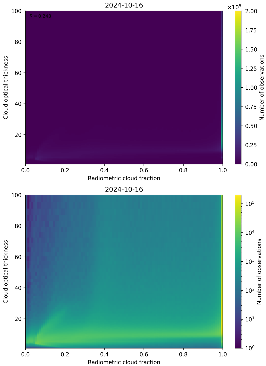
Figure 75: Scatter density plot of “Radiometric cloud fraction” against “Cloud optical thickness” for 2024-10-15 to 2024-10-17.
