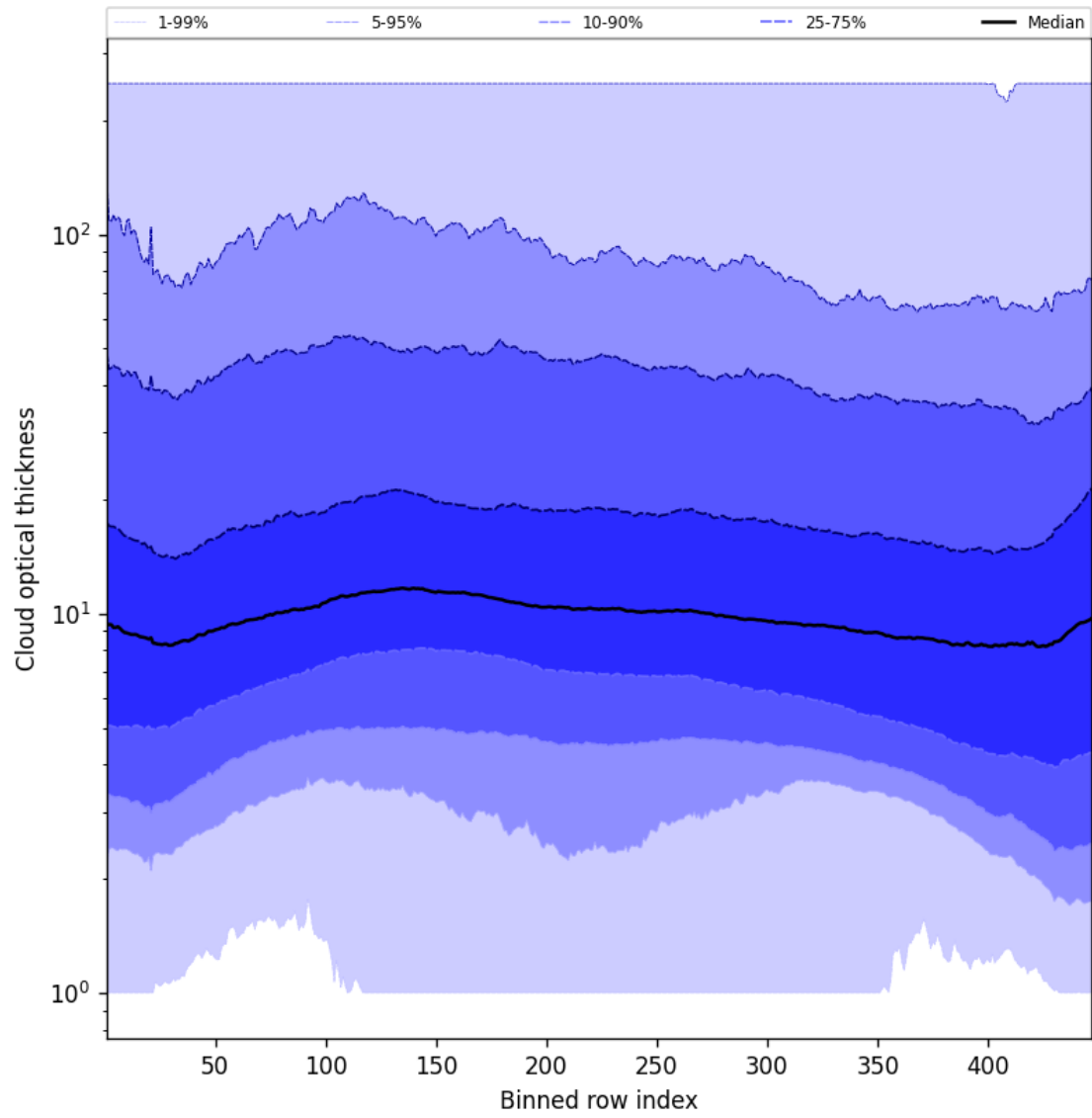
Figure 57: Along track statistics of “Cloud optical thickness” for 2024-10-15 to 2024-10-17
