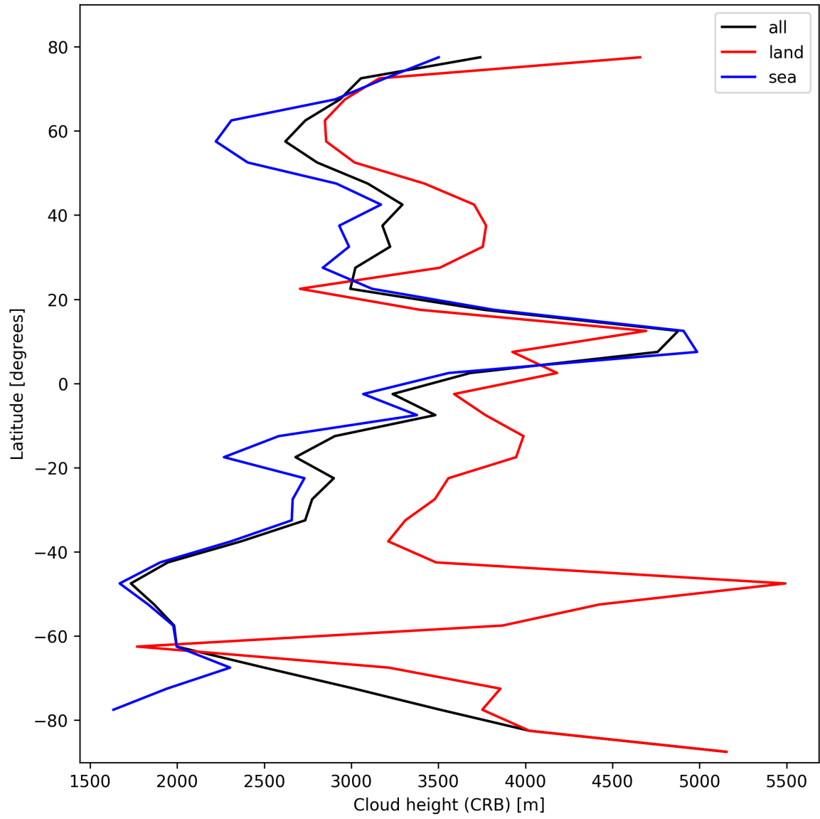
Figure 27: Zonal average of “Cloud height (CRB)” for 2024-10-15 to 2024-10-17.
