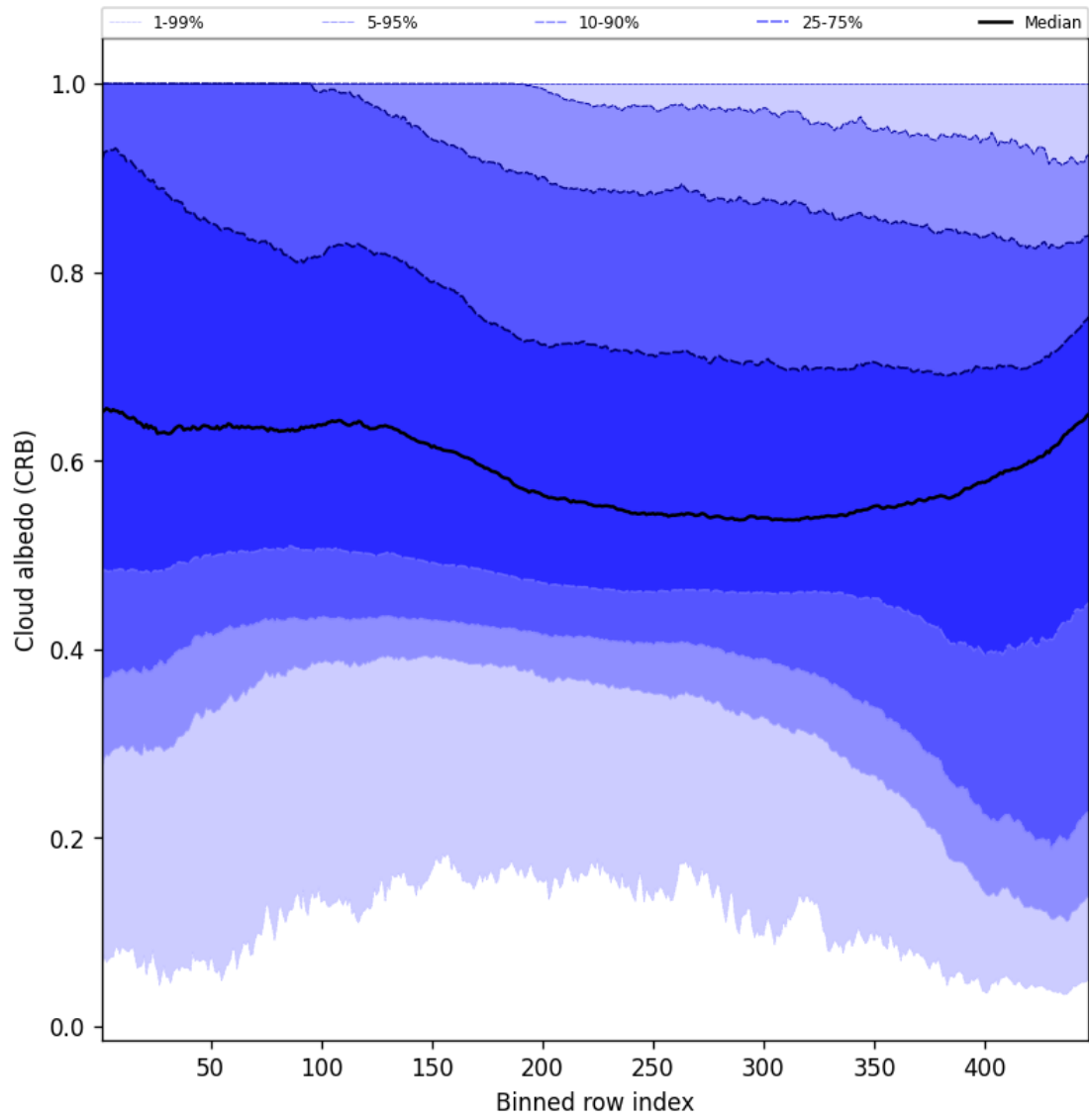
Figure 60: Along track statistics of “Cloud albedo (CRB)” for 2024-10-15 to 2024-10-17
