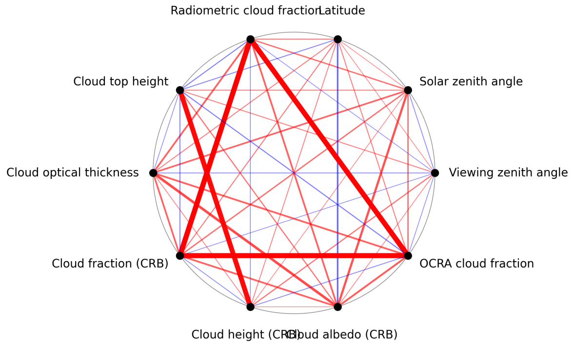
Figure 1: Map of correlation graph for 2024-10-15 to 2024-10-17.
