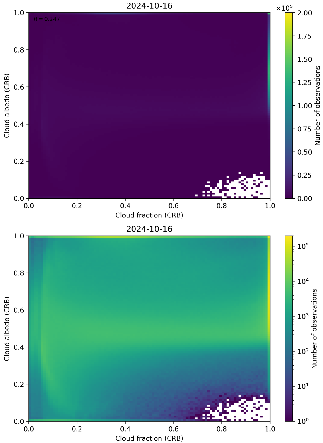
Figure 77: Scatter density plot of “Cloud fraction (CRB)” against “Cloud albedo (CRB)” for 2024-10-15 to 2024-10-17.
