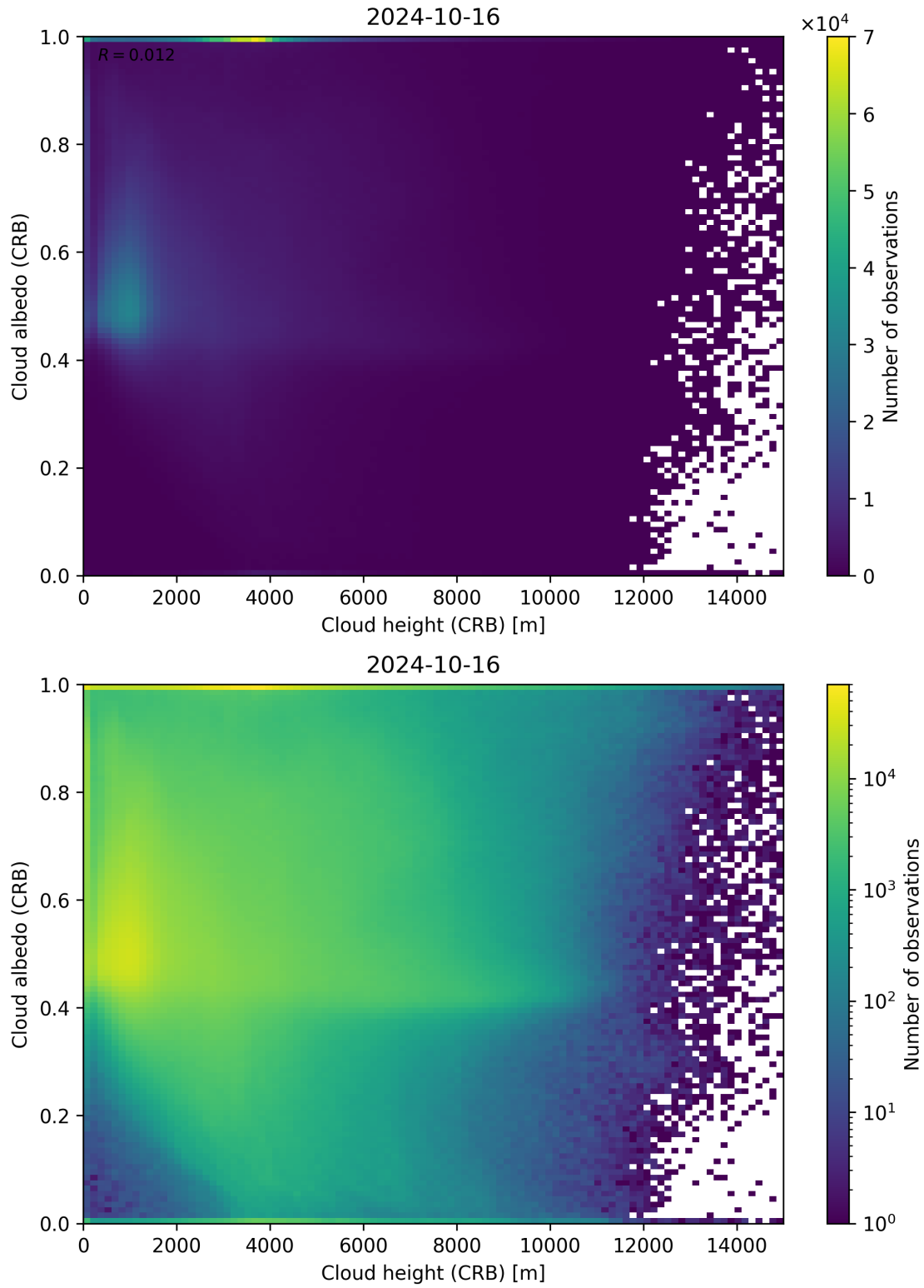
Figure 80: Scatter density plot of “Cloud height (CRB)” against “Cloud albedo (CRB)” for 2024-10-15 to 2024-10-17.
