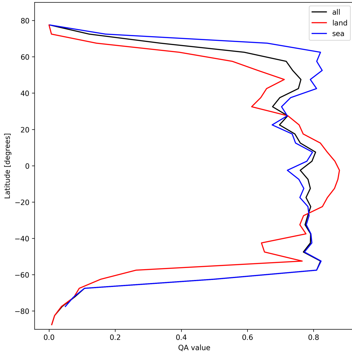
Figure 22: Zonal average of “QA value” for 2024-10-15 to 2024-10-17.
