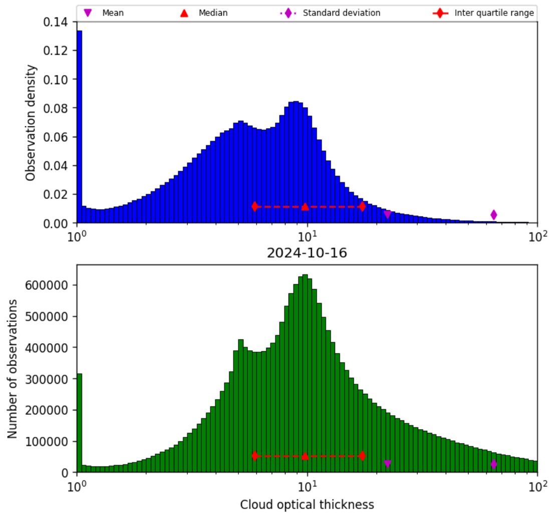
Figure 41: Histogram of “Cloud optical thickness” for 2024-10-15 to 2024-10-17
