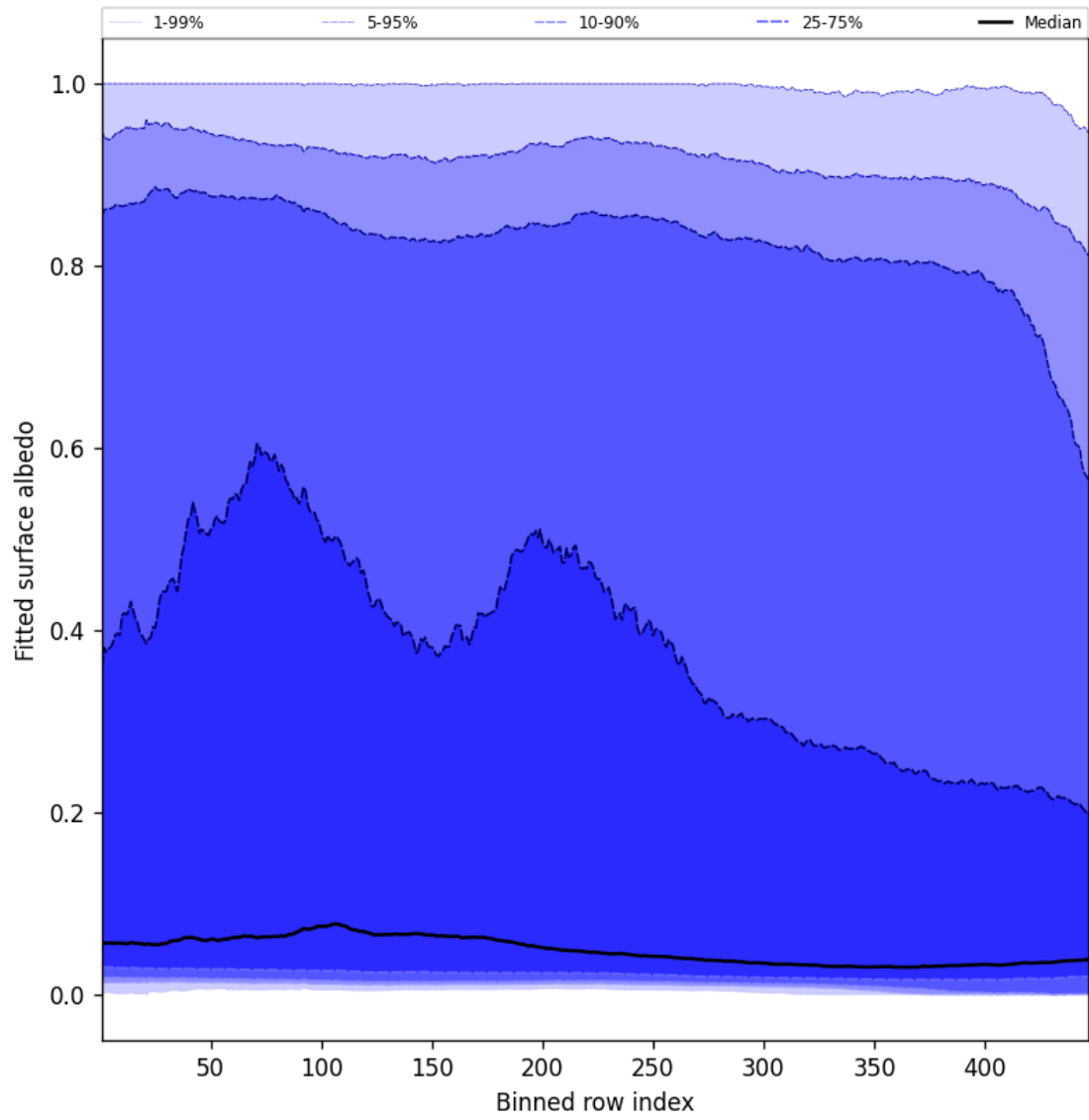
Figure 61: Along track statistics of “Fitted surface albedo” for 2024-10-19 to 2024-10-20
