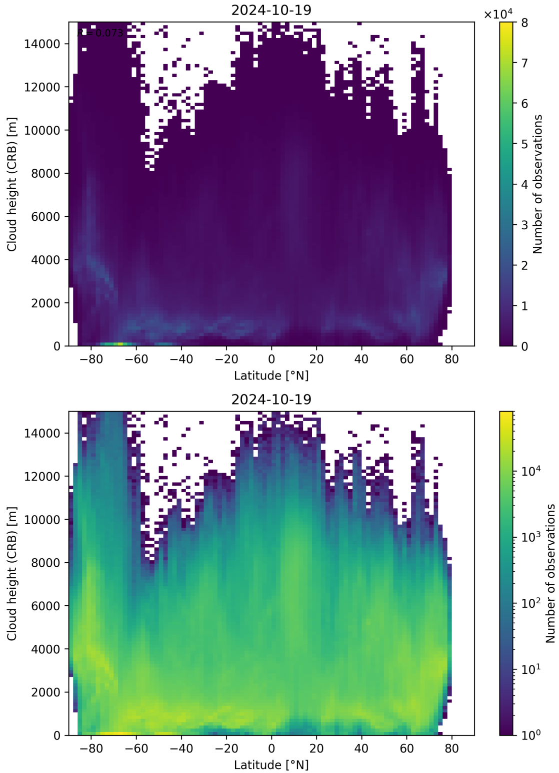
Figure 95: Scatter density plot of “Latitude” against “Cloud height (CRB)” for 2024-10-19 to 2024-10-20.
