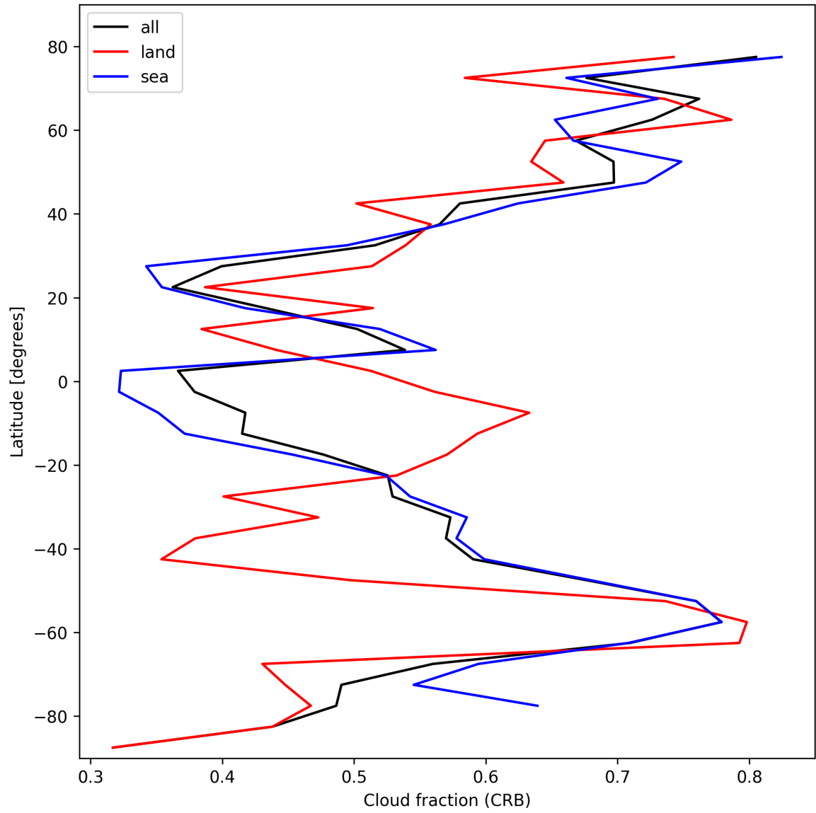
Figure 26: Zonal average of “Cloud fraction (CRB)” for 2024-10-19 to 2024-10-20.
