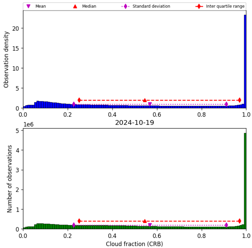
Figure 42: Histogram of “Cloud fraction (CRB)” for 2024-10-19 to 2024-10-20
