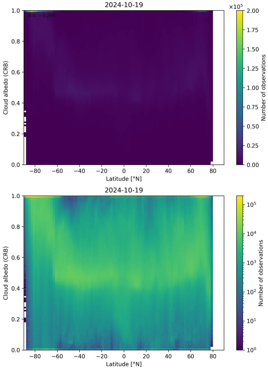
Figure 91: Scatter density plot of “Latitude” against “Cloud albedo (CRB)” for 2024-10-19 to 2024-10-20.
