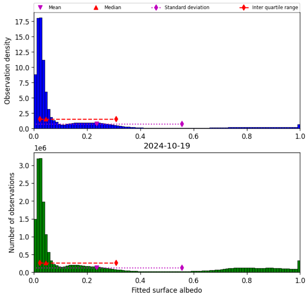
Figure 45: Histogram of “Fitted surface albedo” for 2024-10-19 to 2024-10-20
