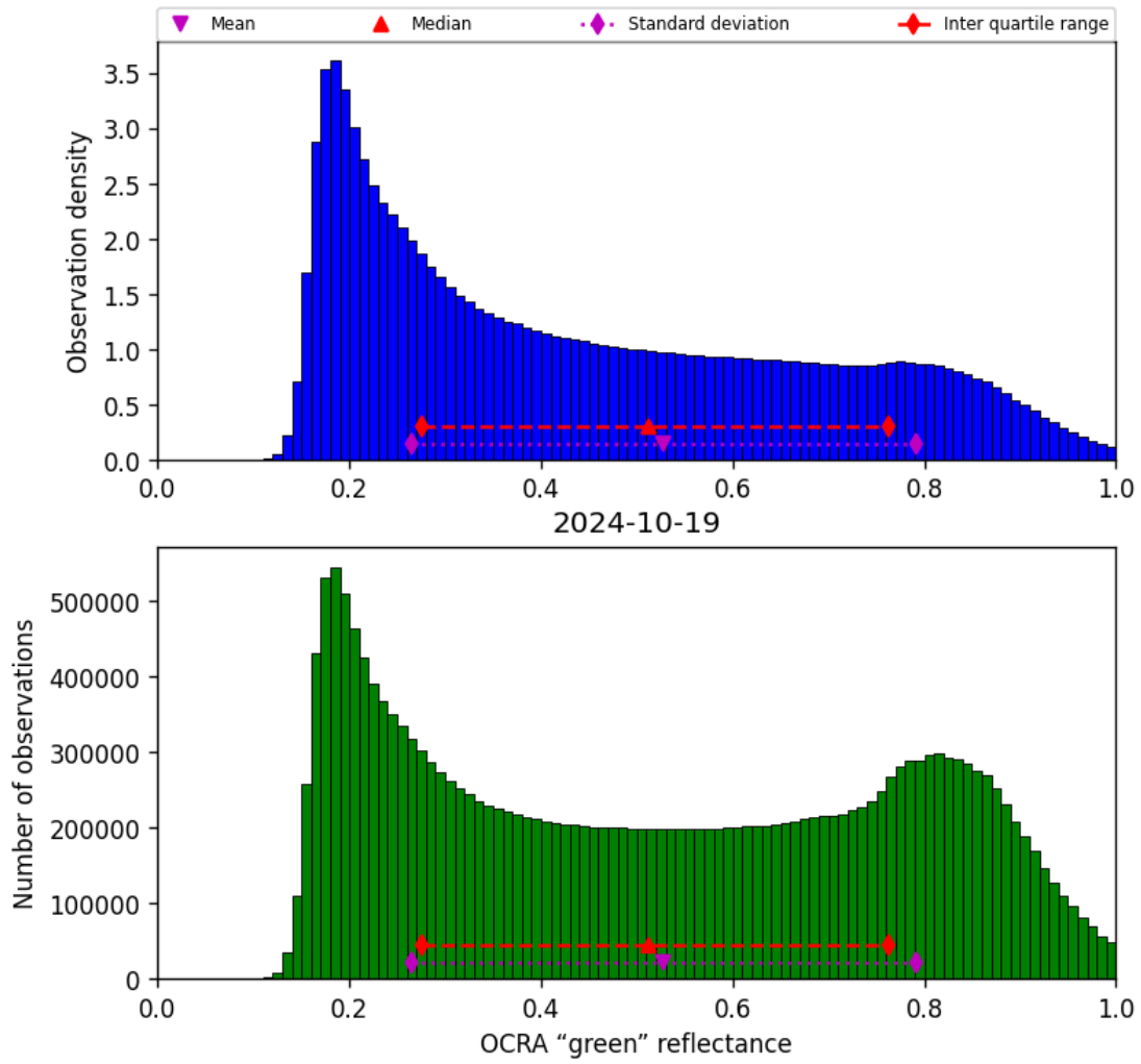
Figure 52: Histogram of “OCRA “green” reflectance” for 2024-10-19 to 2024-10-20
