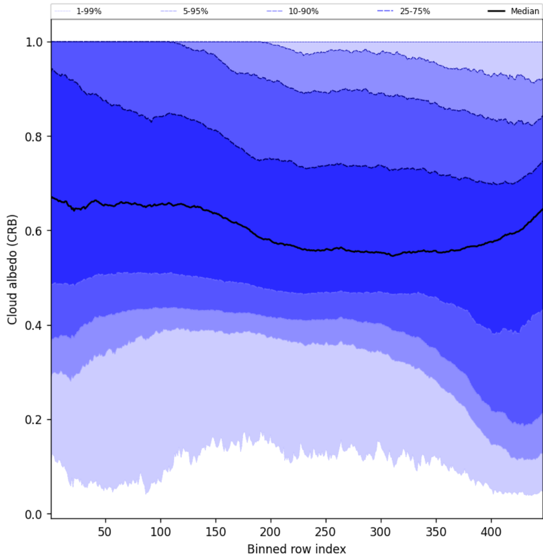
Figure 60: Along track statistics of “Cloud albedo (CRB)” for 2024-10-19 to 2024-10-20
