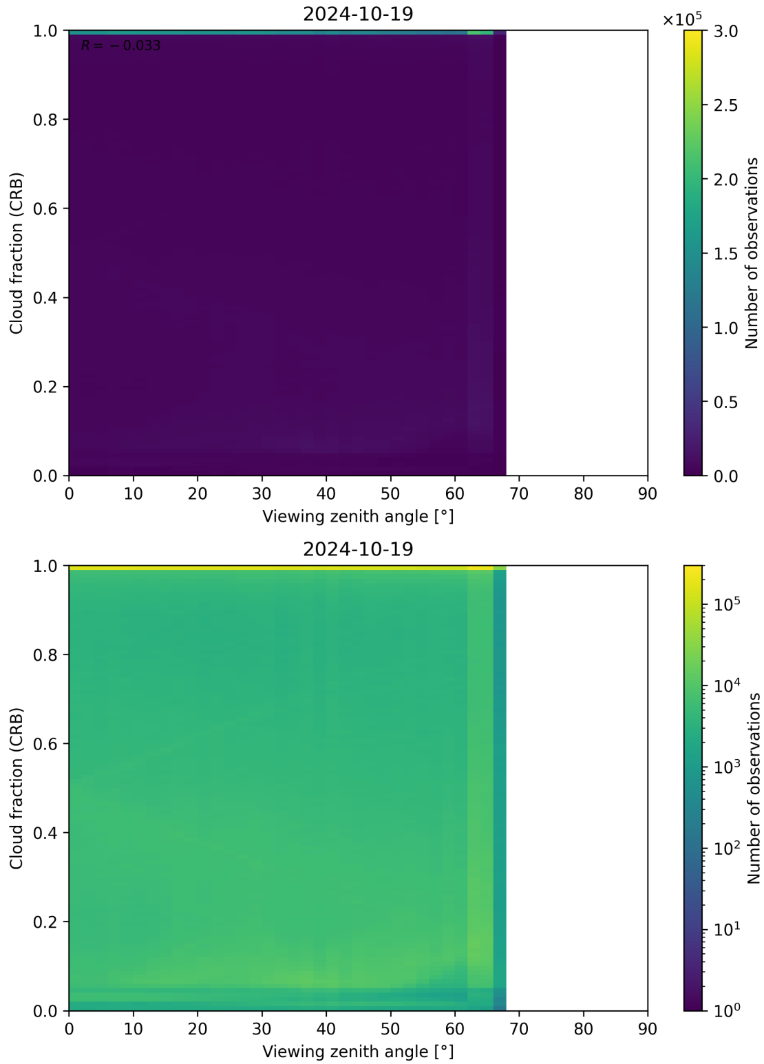
Figure 109: Scatter density plot of “Viewing zenith angle” against “Cloud fraction (CRB)” for 2024-10-19 to 2024-10-20.
