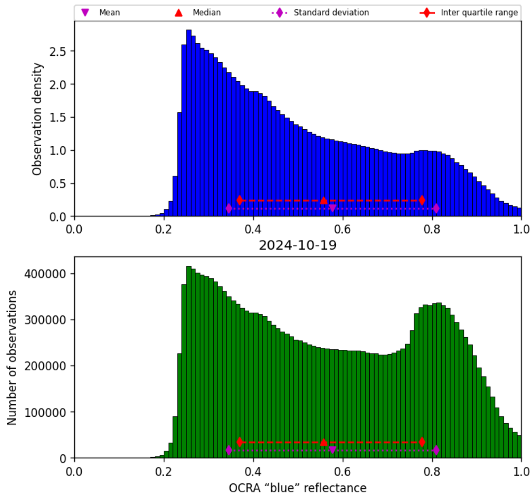
Figure 51: Histogram of “OCRA “blue” reflectance” for 2024-10-19 to 2024-10-20
