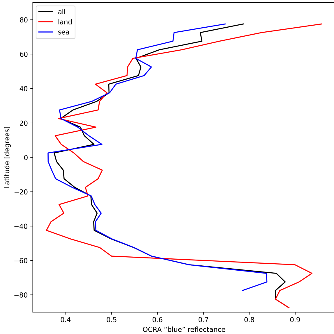
Figure 35: Zonal average of "OCRA "blue" reflectance" for 2024-10-19 to 2024-10-20.
