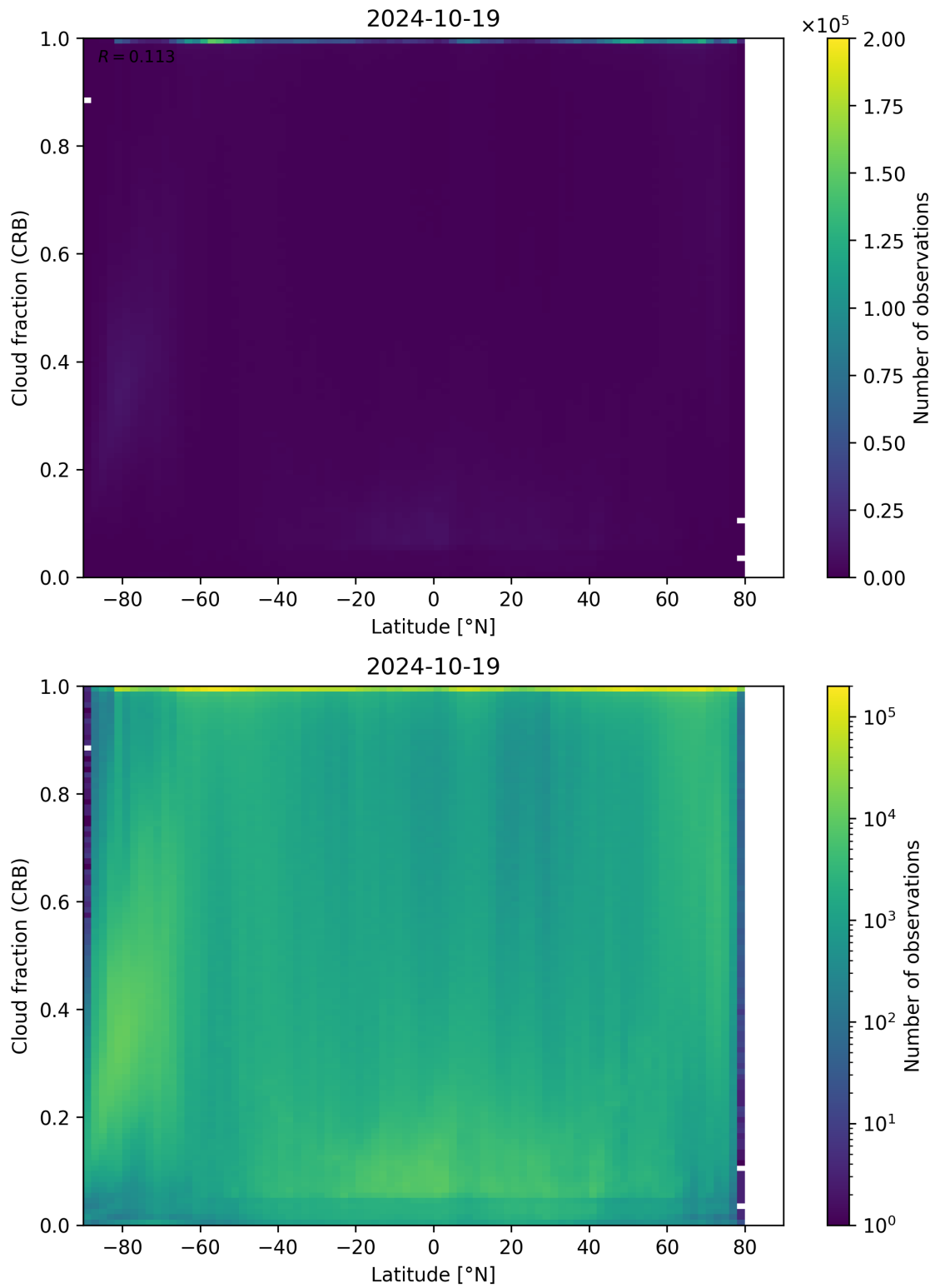
Figure 94: Scatter density plot of “Latitude” against “Cloud fraction (CRB)” for 2024-10-19 to 2024-10-20.
