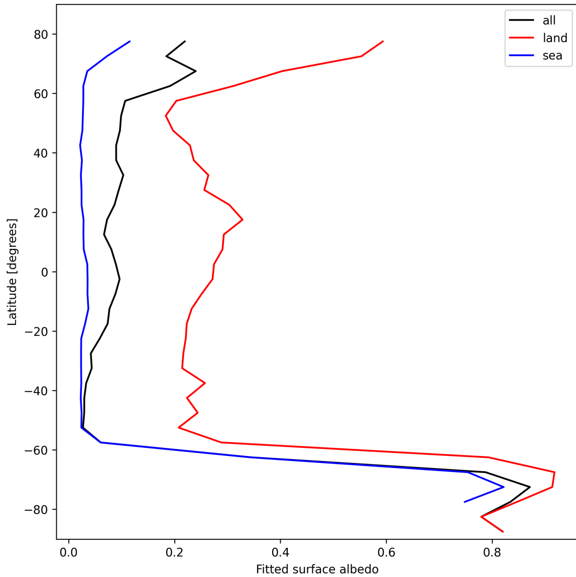
Figure 29: Zonal average of “Fitted surface albedo” for 2024-10-19 to 2024-10-20.
