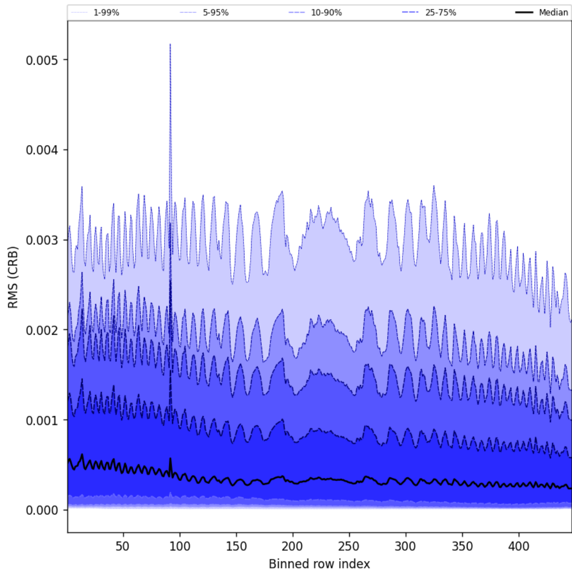
Figure 64: Along track statistics of “RMS (CRB)” for 2024-10-19 to 2024-10-20
