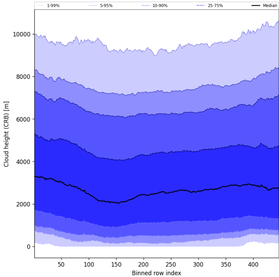
Figure 59: Along track statistics of “Cloud height (CRB)” for 2024-10-19 to 2024-10-20
