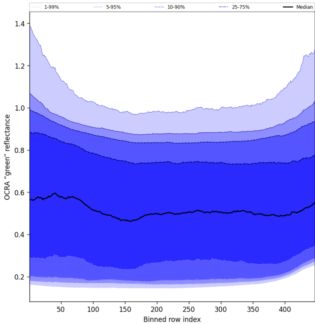
Figure 68: Along track statistics of “OCRA “green” reflectance” for 2024-10-19 to 2024-10-20
