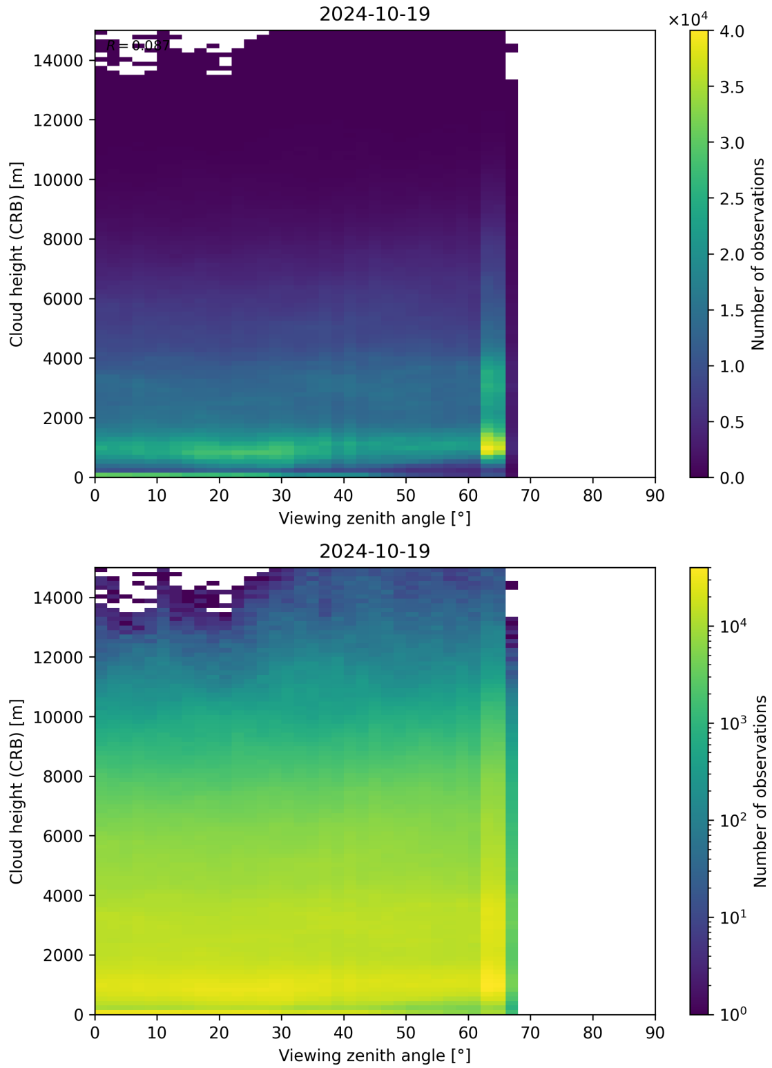
Figure 110: Scatter density plot of “Viewing zenith angle” against “Cloud height (CRB)” for 2024-10-19 to 2024-10-20.
