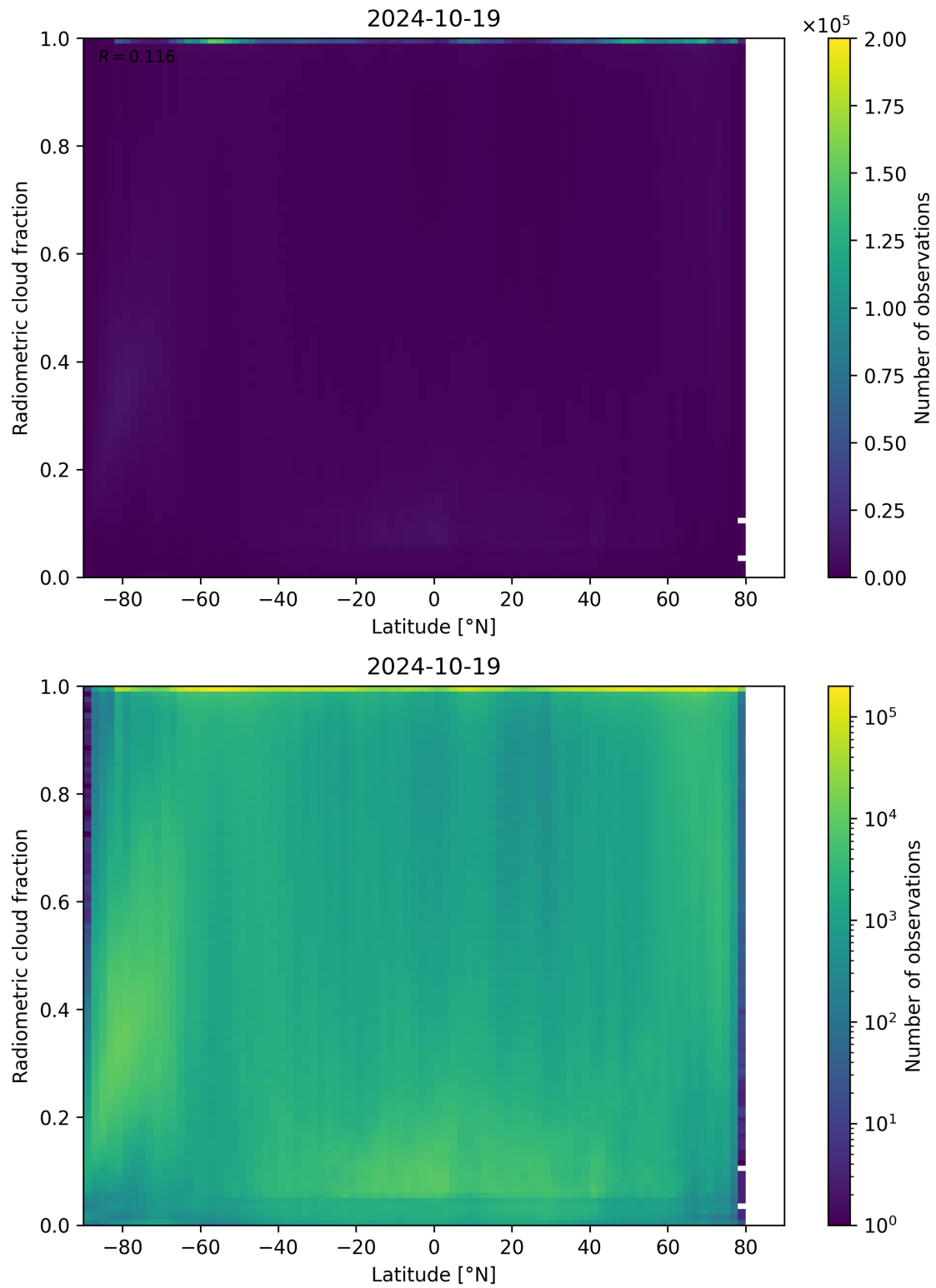
Figure 92: Scatter density plot of “Latitude” against “Radiometric cloud fraction” for 2024-10-19 to 2024-10-20.
