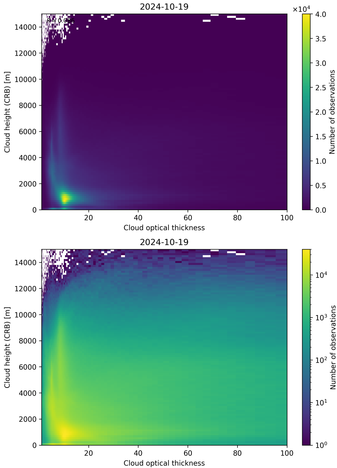
Figure 85: Scatter density plot of “Cloud optical thickness” against “Cloud height (CRB)” for 2024-10-19 to 2024-10-20.
