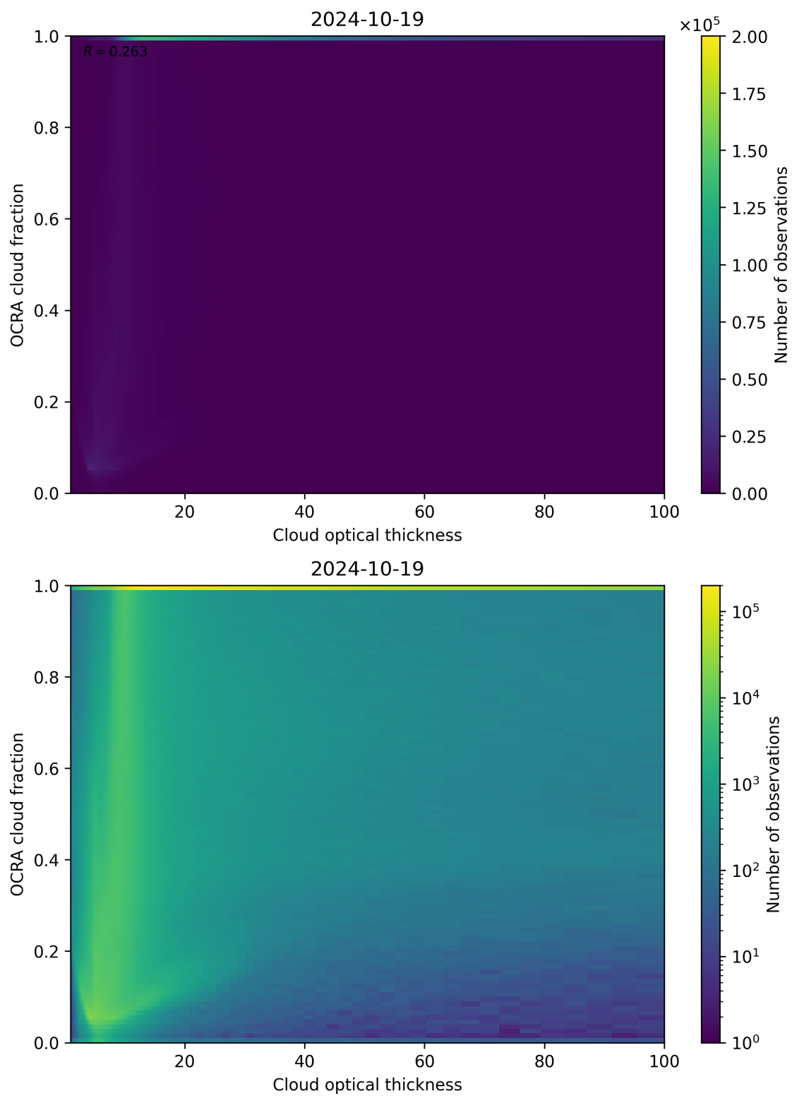
Figure 83: Scatter density plot of “Cloud optical thickness” against “OCRA cloud fraction” for 2024-10-19 to 2024-10-20.
