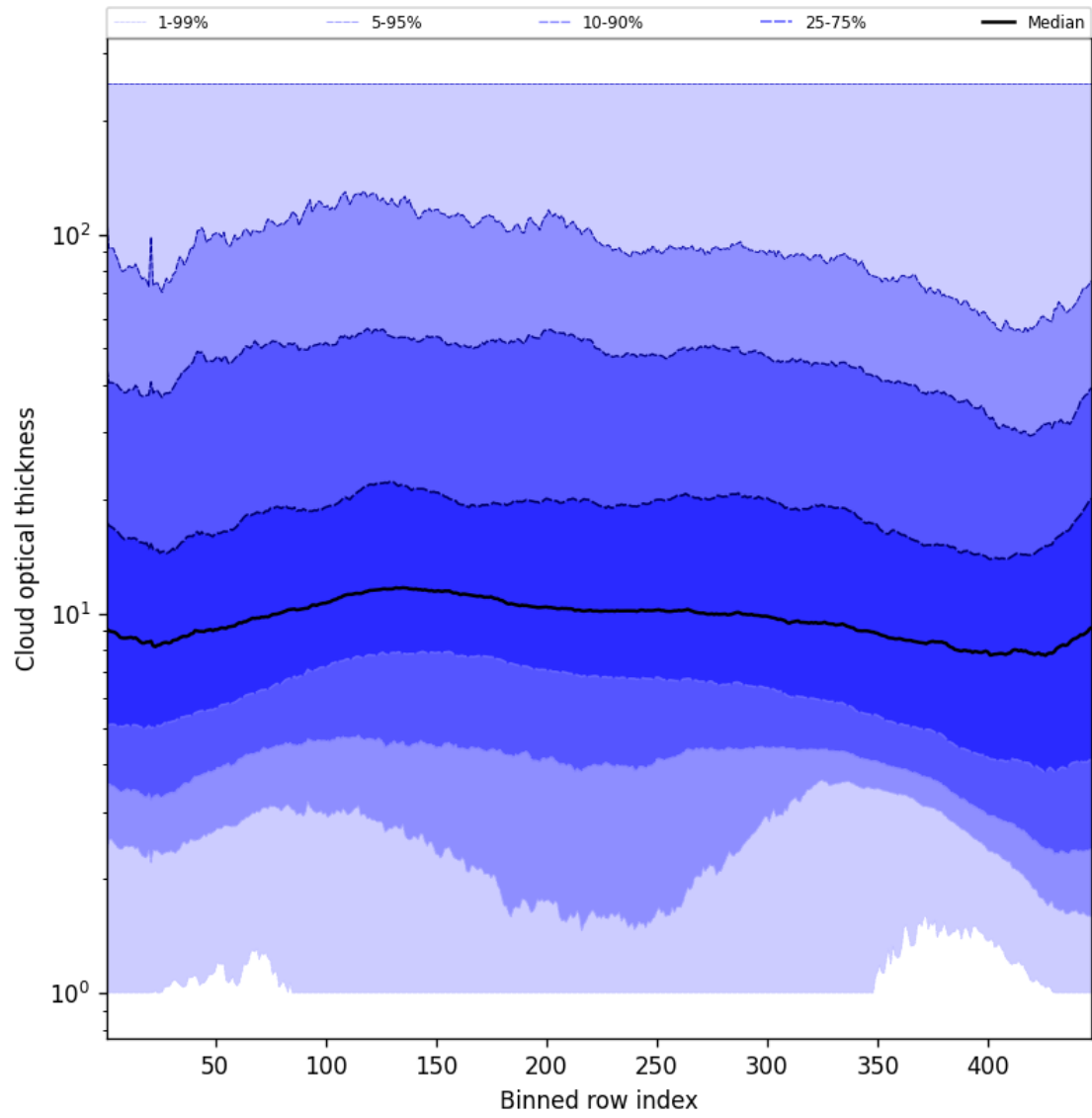
Figure 57: Along track statistics of “Cloud optical thickness” for 2024-10-19 to 2024-10-20
