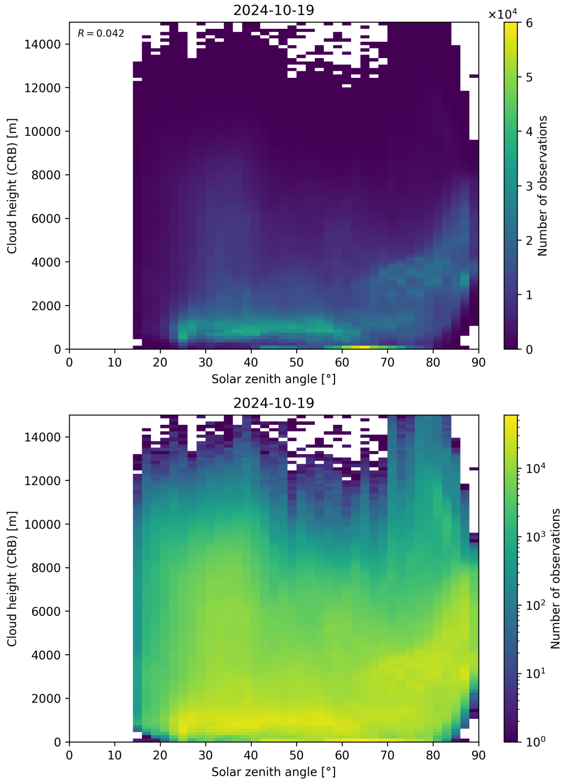
Figure 102: Scatter density plot of “Solar zenith angle” against “Cloud height (CRB)” for 2024-10-19 to 2024-10-20.
