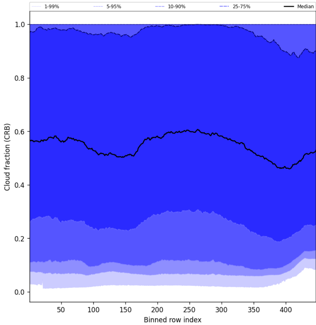
Figure 58: Along track statistics of “Cloud fraction (CRB)” for 2024-10-19 to 2024-10-20
