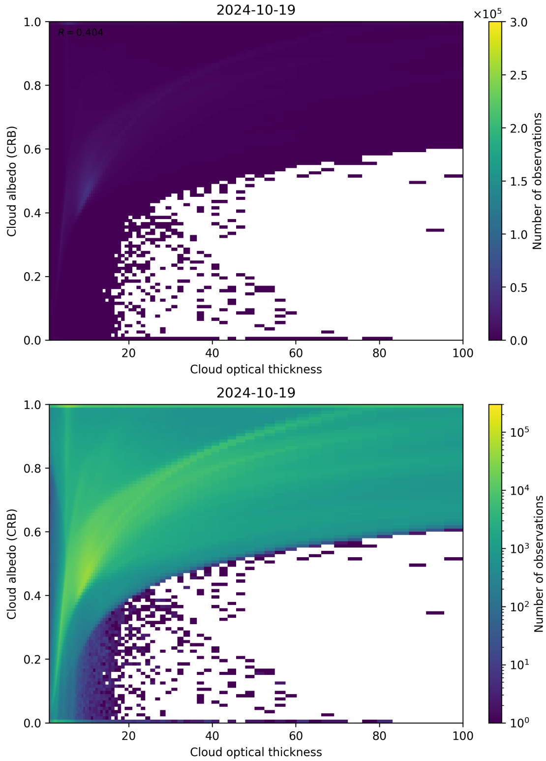
Figure 82: Scatter density plot of “Cloud optical thickness” against “Cloud albedo (CRB)” for 2024-10-19 to 2024-10-20.
