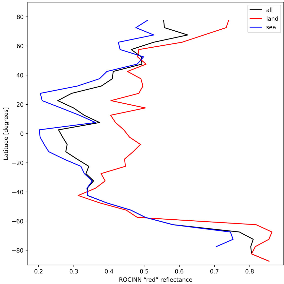
Figure 37: Zonal average of “ROCINN “red” reflectance” for 2024-10-19 to 2024-10-20.
