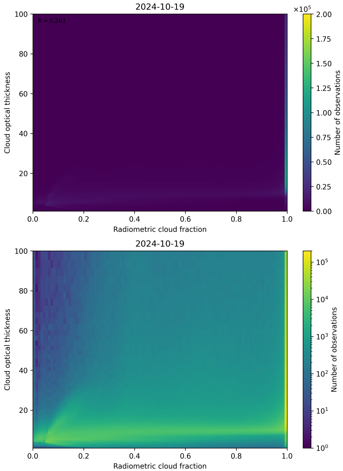
Figure 75: Scatter density plot of “Radiometric cloud fraction” against “Cloud optical thickness” for 2024-10-19 to 2024-10-20.
