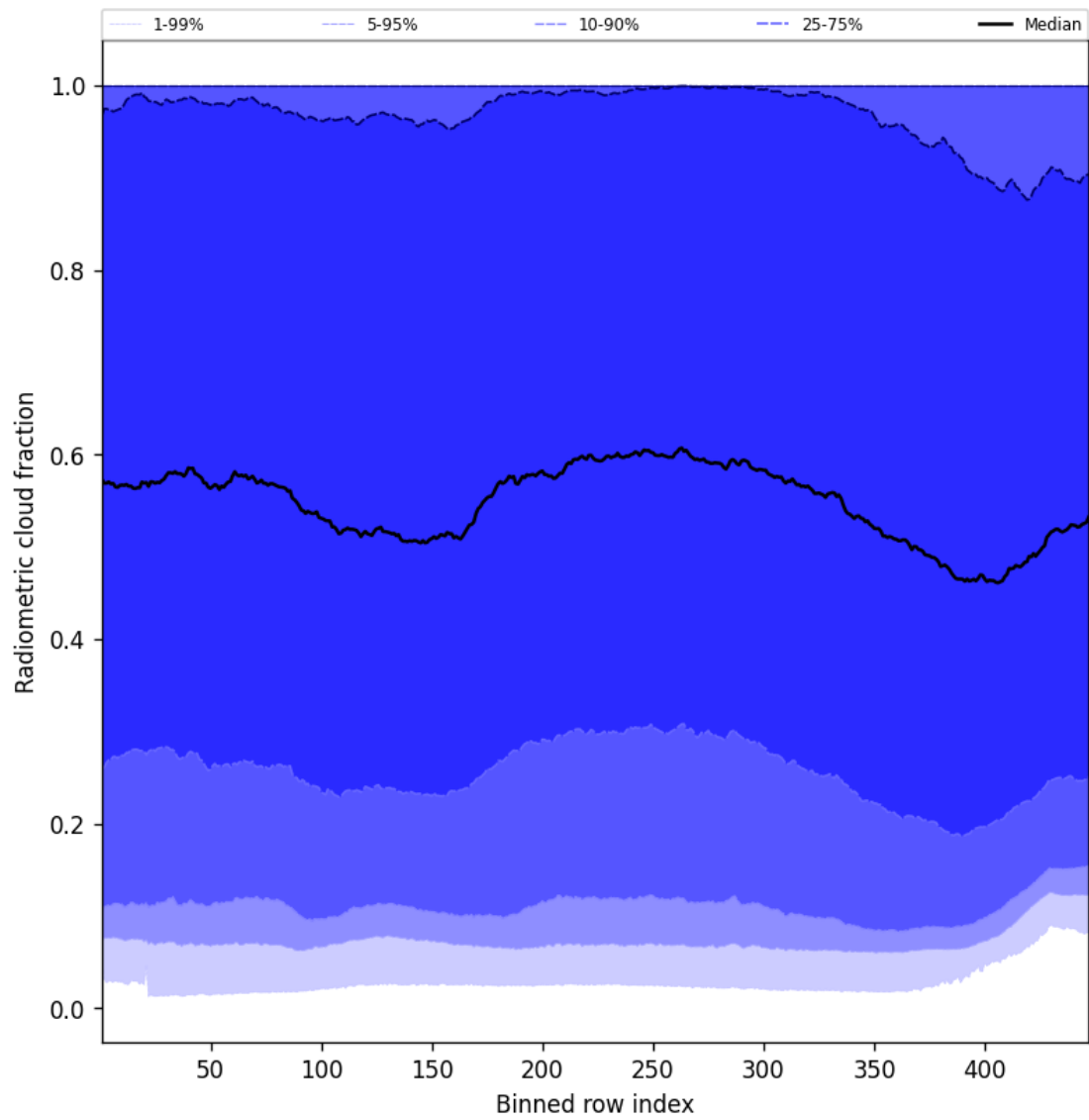
Figure 55: Along track statistics of “Radiometric cloud fraction” for 2024-10-19 to 2024-10-20
