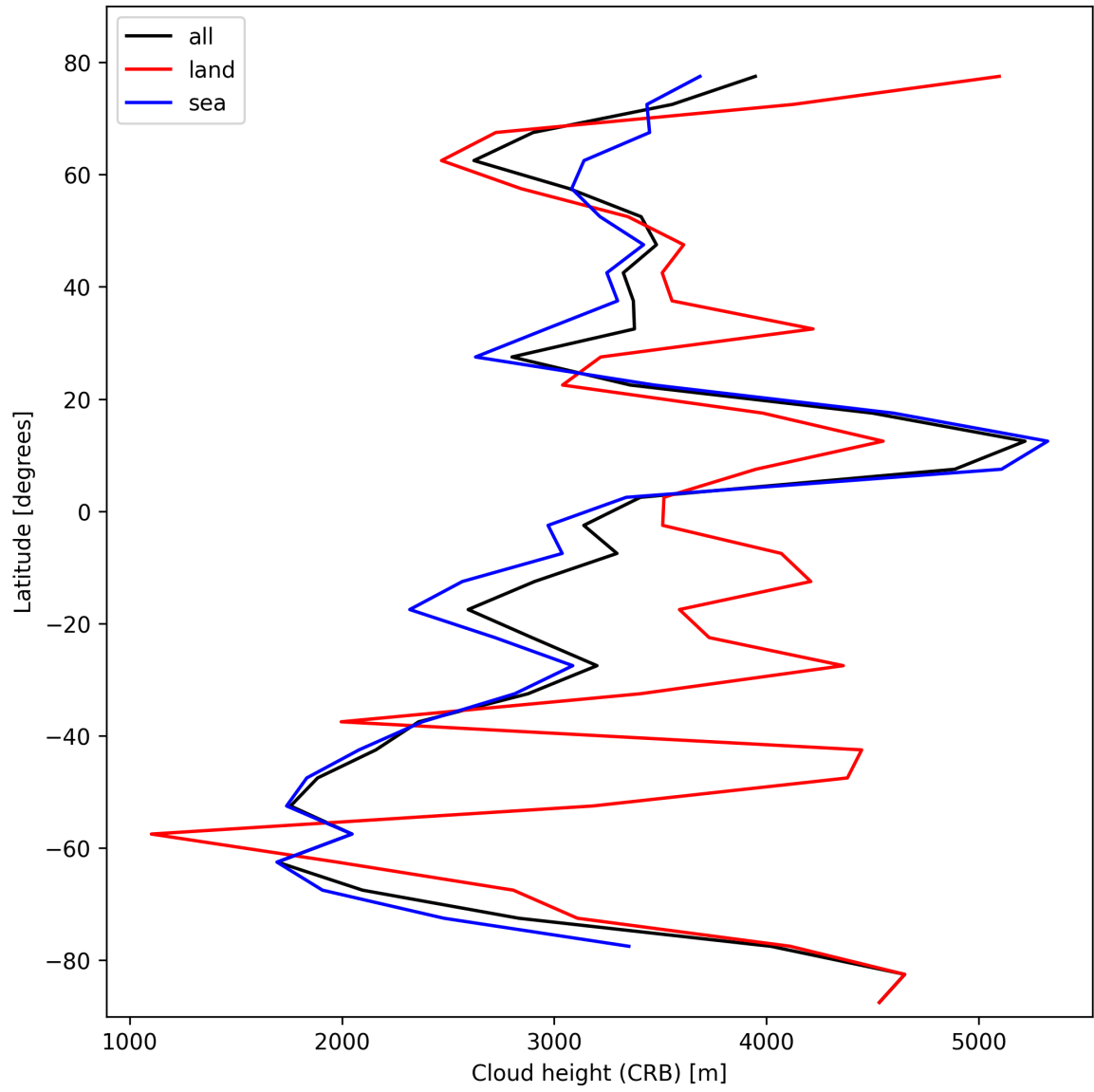
Figure 27: Zonal average of “Cloud height (CRB)” for 2024-10-19 to 2024-10-20.
