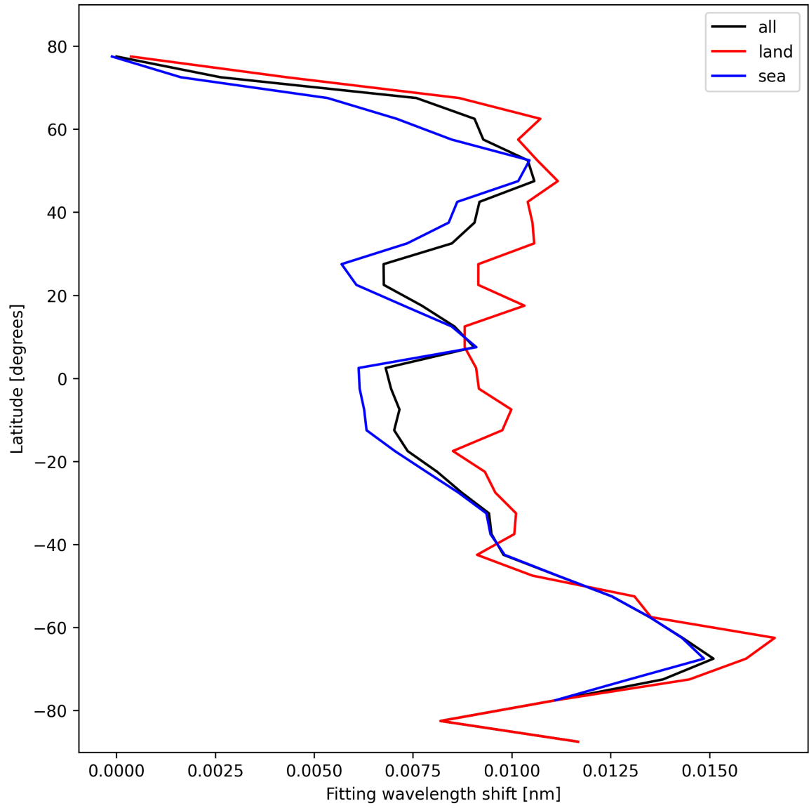
Figure 33: Zonal average of “Fitting wavelength shift” for 2024-10-19 to 2024-10-20.
