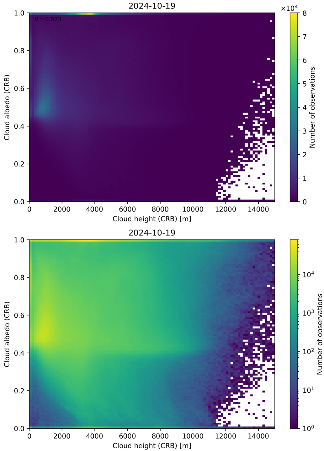
Figure 80: Scatter density plot of “Cloud height (CRB)” against “Cloud albedo (CRB)” for 2024-10-19 to 2024-10-20.
