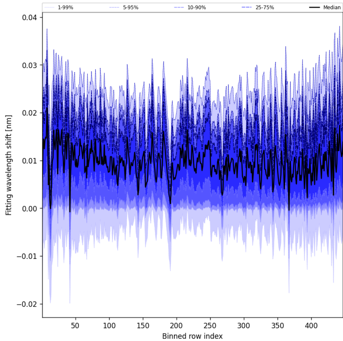
Figure 65: Along track statistics of “Fitting wavelength shift” for 2024-10-19 to 2024-10-20
