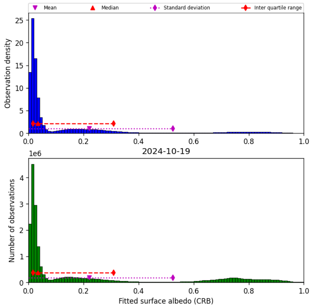
Figure 46: Histogram of “Fitted surface albedo (CRB)” for 2024-10-19 to 2024-10-20
