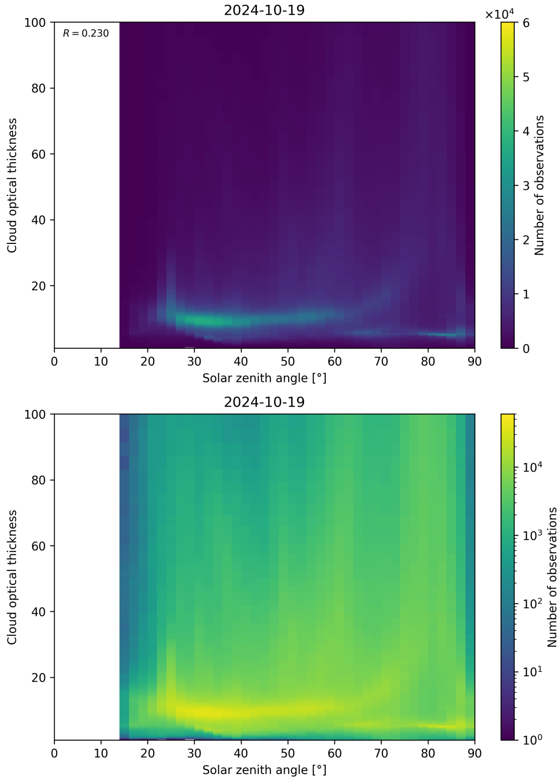
Figure 103: Scatter density plot of “Solar zenith angle” against “Cloud optical thickness” for 2024-10-19 to 2024-10-20.
