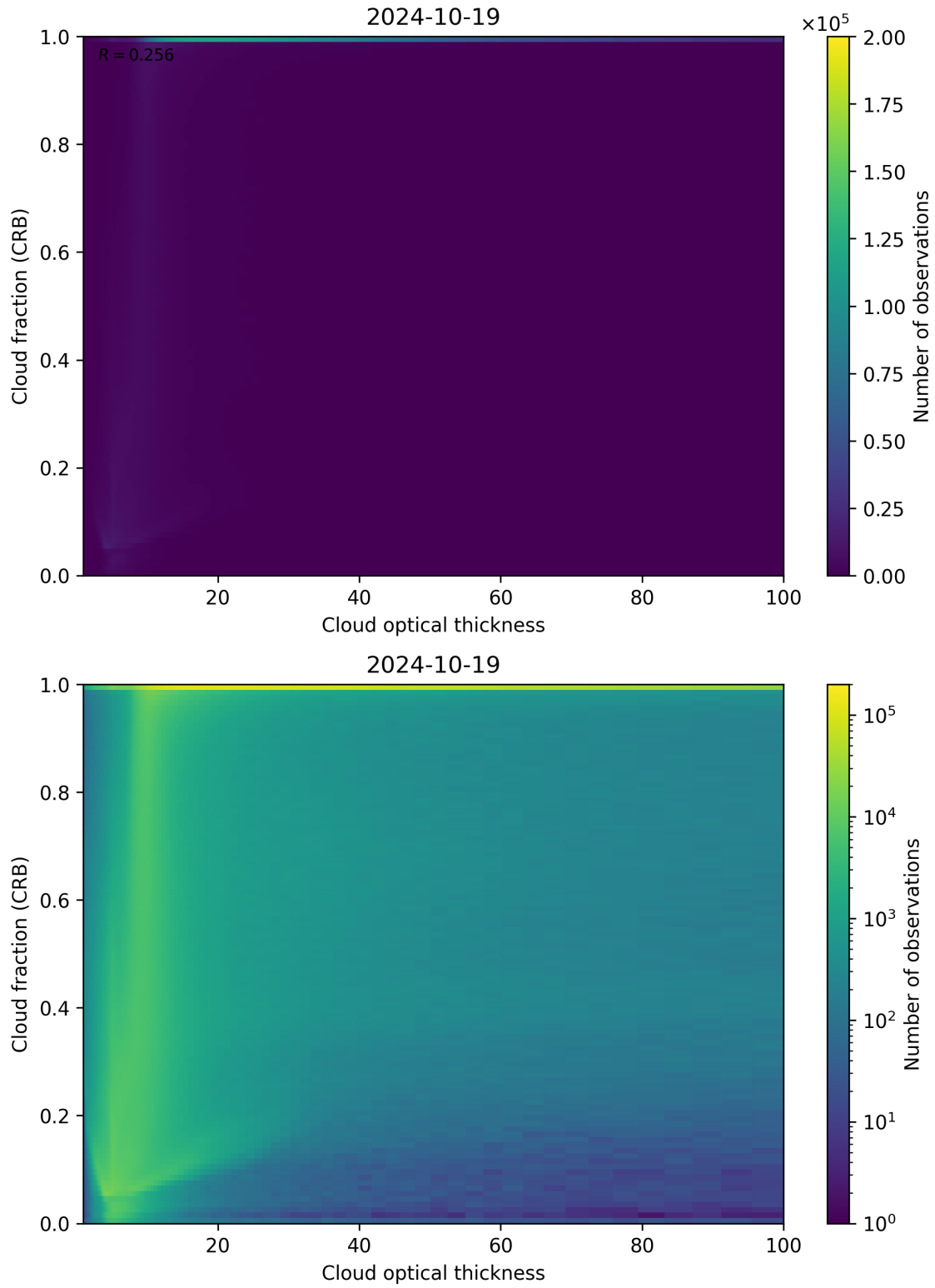
Figure 84: Scatter density plot of “Cloud optical thickness” against “Cloud fraction (CRB)” for 2024-10-19 to 2024-10-20.
