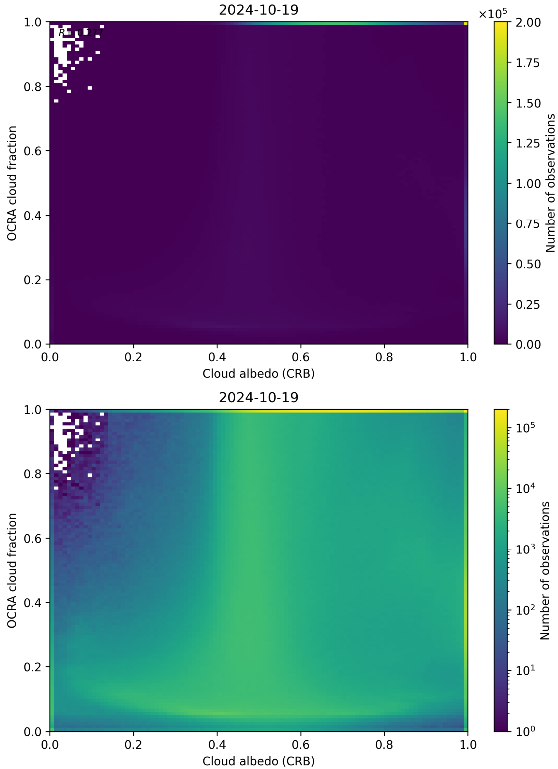
Figure 70: Scatter density plot of “Cloud albedo (CRB)” against “OCRA cloud fraction” for 2024-10-19 to 2024-10-20.
