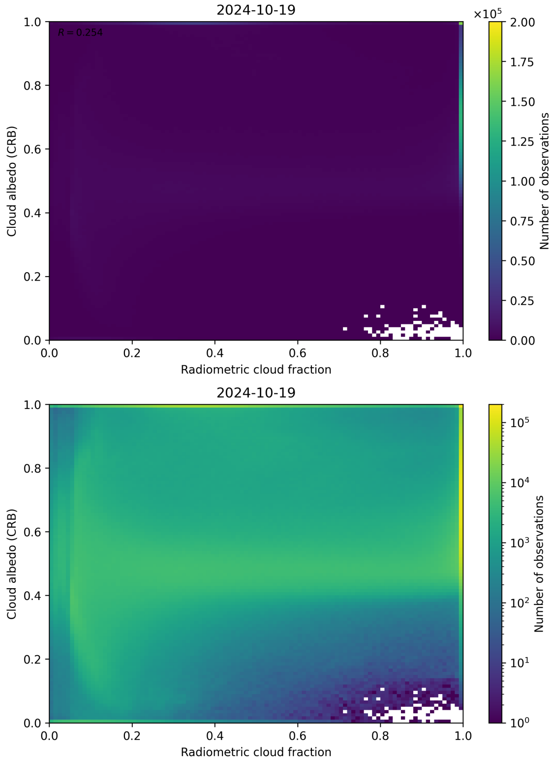
Figure 71: Scatter density plot of “Radiometric cloud fraction” against “Cloud albedo (CRB)” for 2024-10-19 to 2024-10-20.
