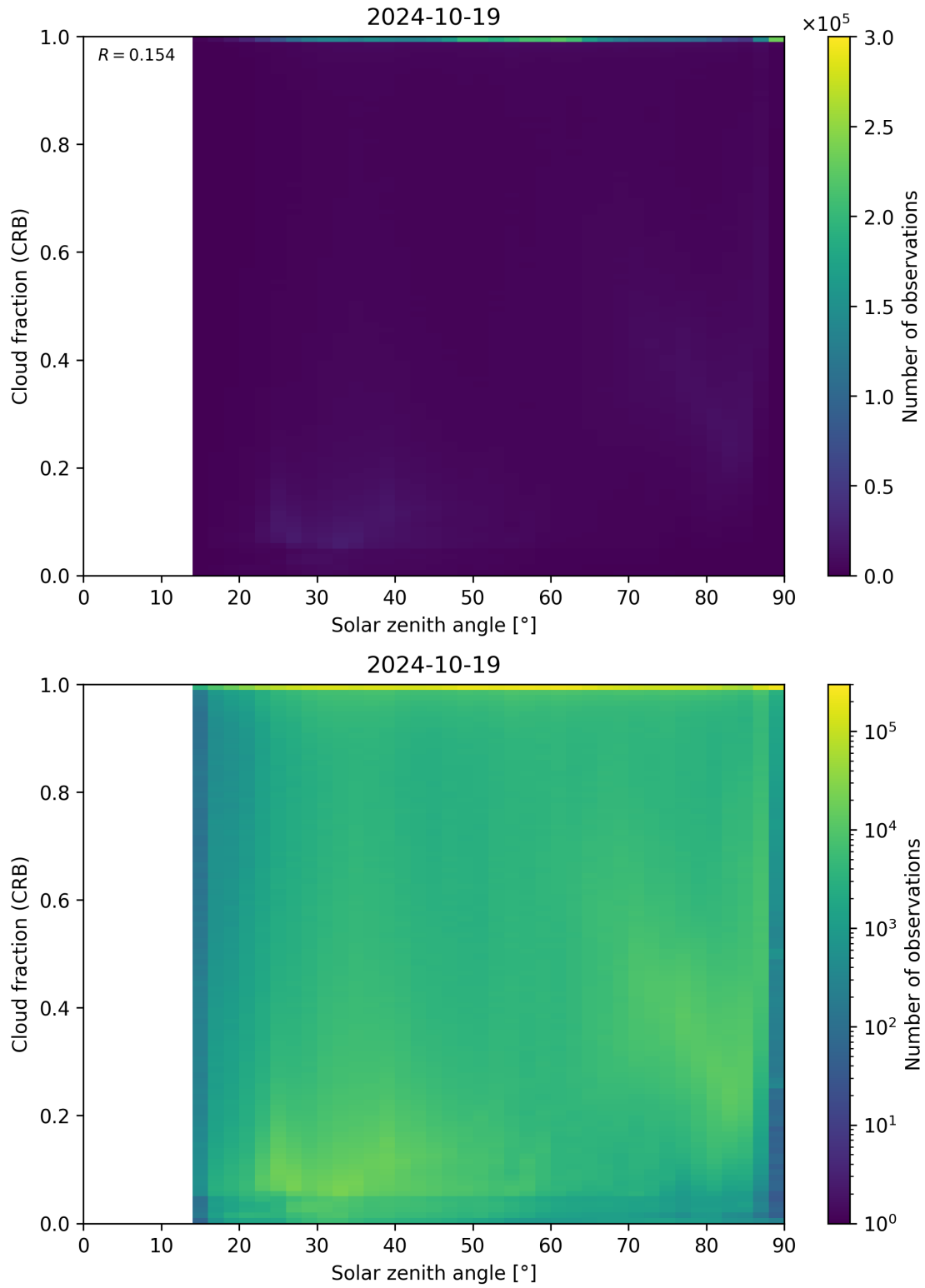
Figure 101: Scatter density plot of “Solar zenith angle” against “Cloud fraction (CRB)” for 2024-10-19 to 2024-10-20.
