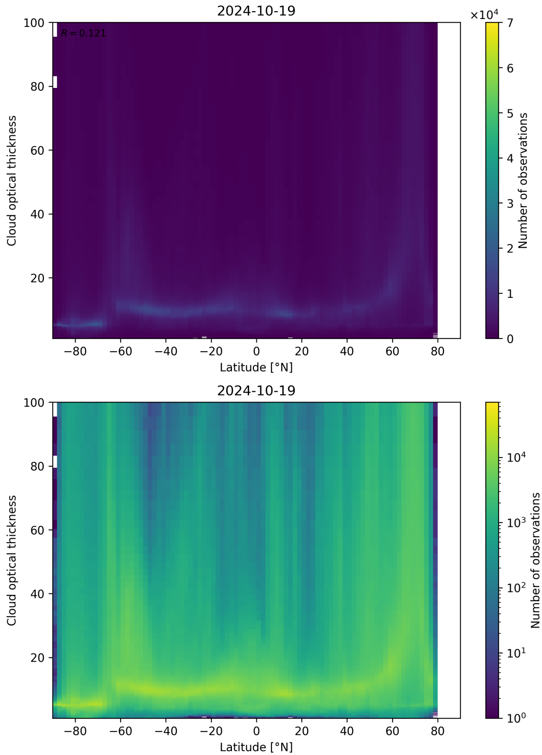
Figure 96: Scatter density plot of “Latitude” against “Cloud optical thickness” for 2024-10-19 to 2024-10-20.
