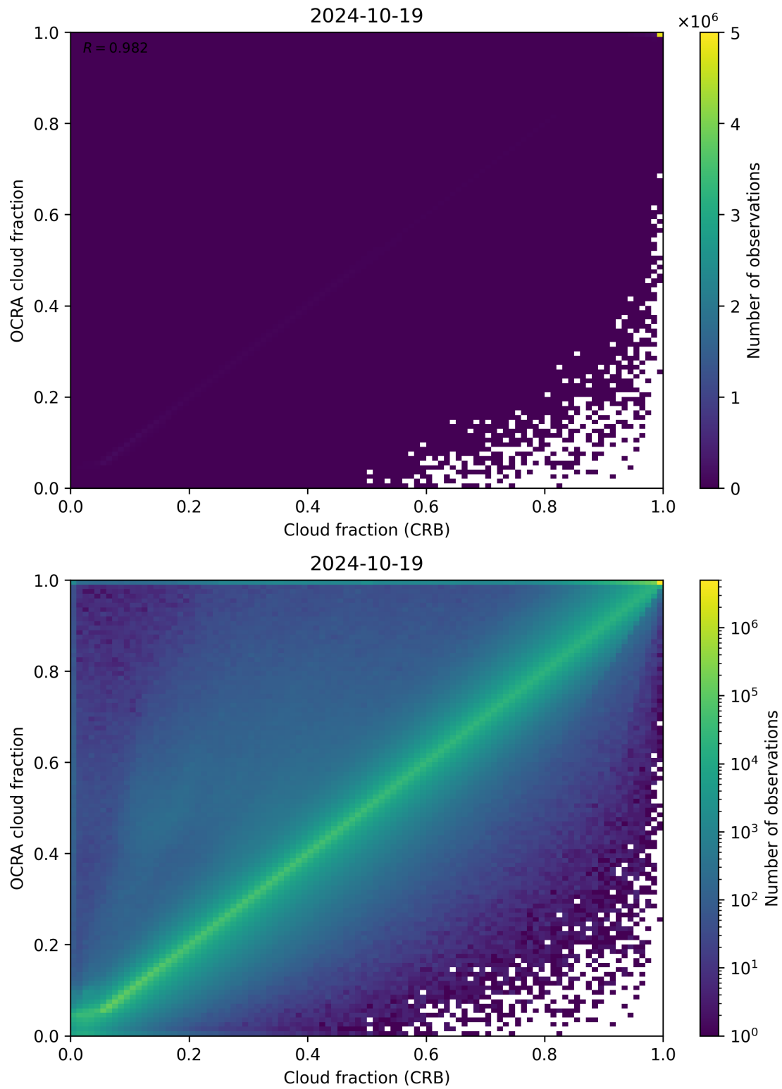
Figure 78: Scatter density plot of “Cloud fraction (CRB)” against “OCRA cloud fraction” for 2024-10-19 to 2024-10-20.
