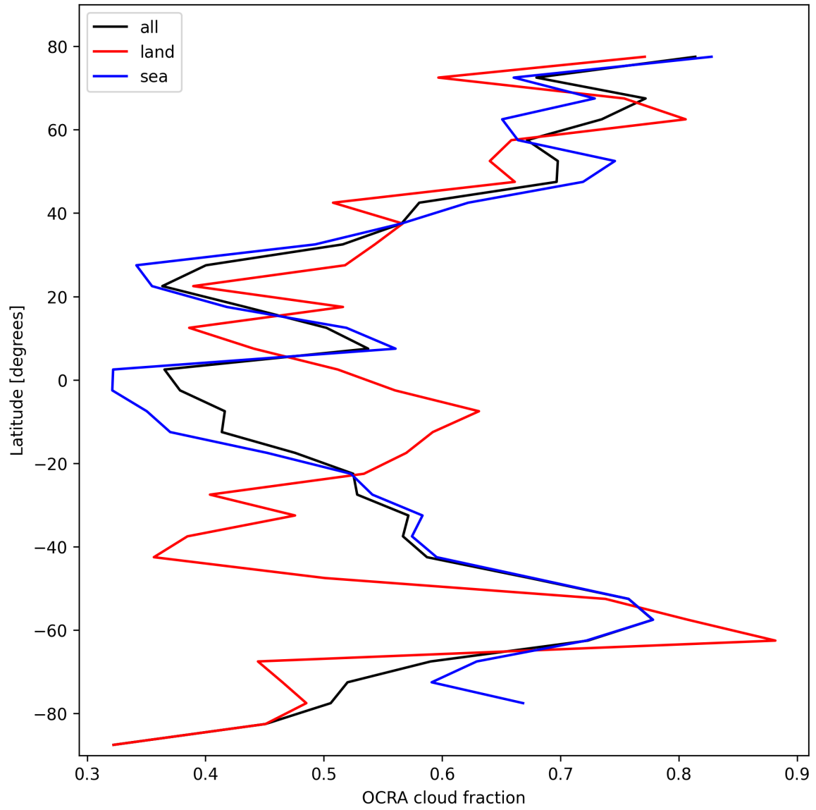
Figure 34: Zonal average of “OCRA cloud fraction” for 2024-10-19 to 2024-10-20.
