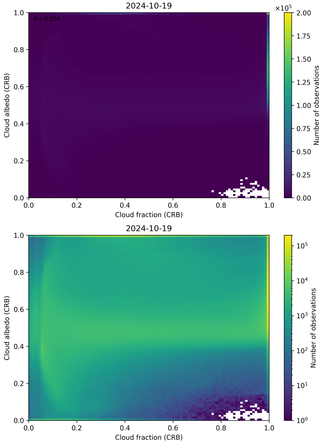
Figure 77: Scatter density plot of “Cloud fraction (CRB)” against “Cloud albedo (CRB)” for 2024-10-19 to 2024-10-20.
