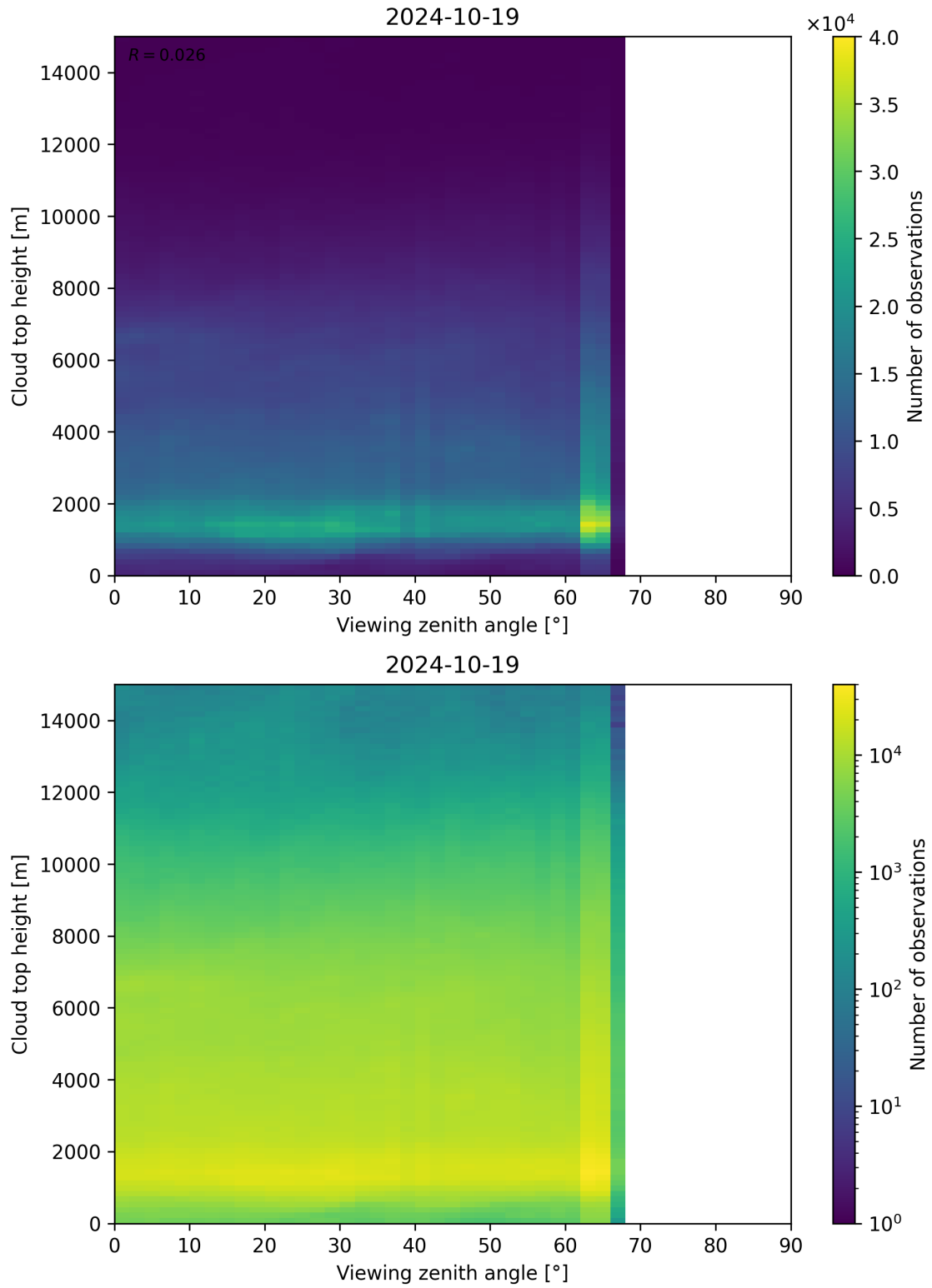
Figure 112: Scatter density plot of “Viewing zenith angle” against “Cloud top height” for 2024-10-19 to 2024-10-20.
