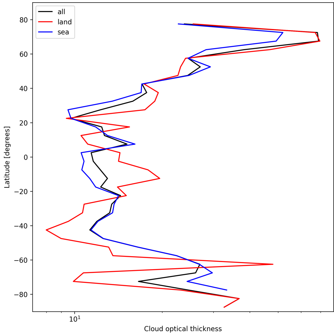
Figure 25: Zonal average of “Cloud optical thickness” for 2024-10-19 to 2024-10-20.
