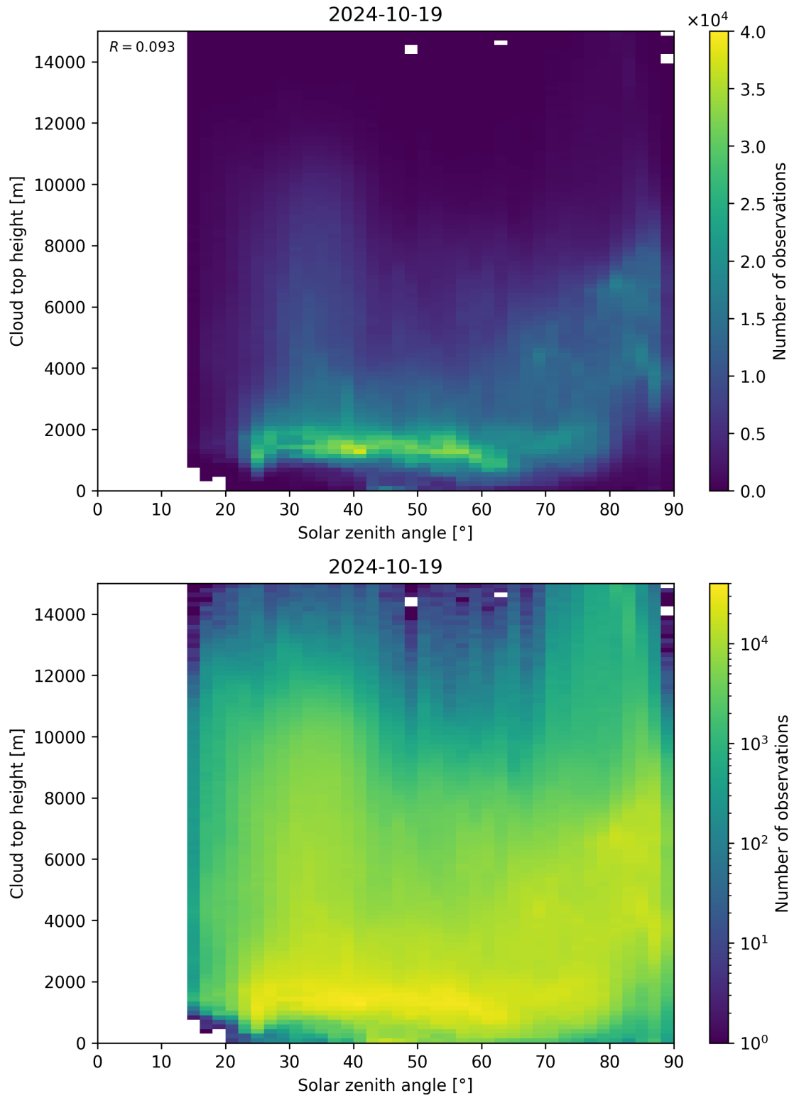
Figure 104: Scatter density plot of “Solar zenith angle” against “Cloud top height” for 2024-10-19 to 2024-10-20.
