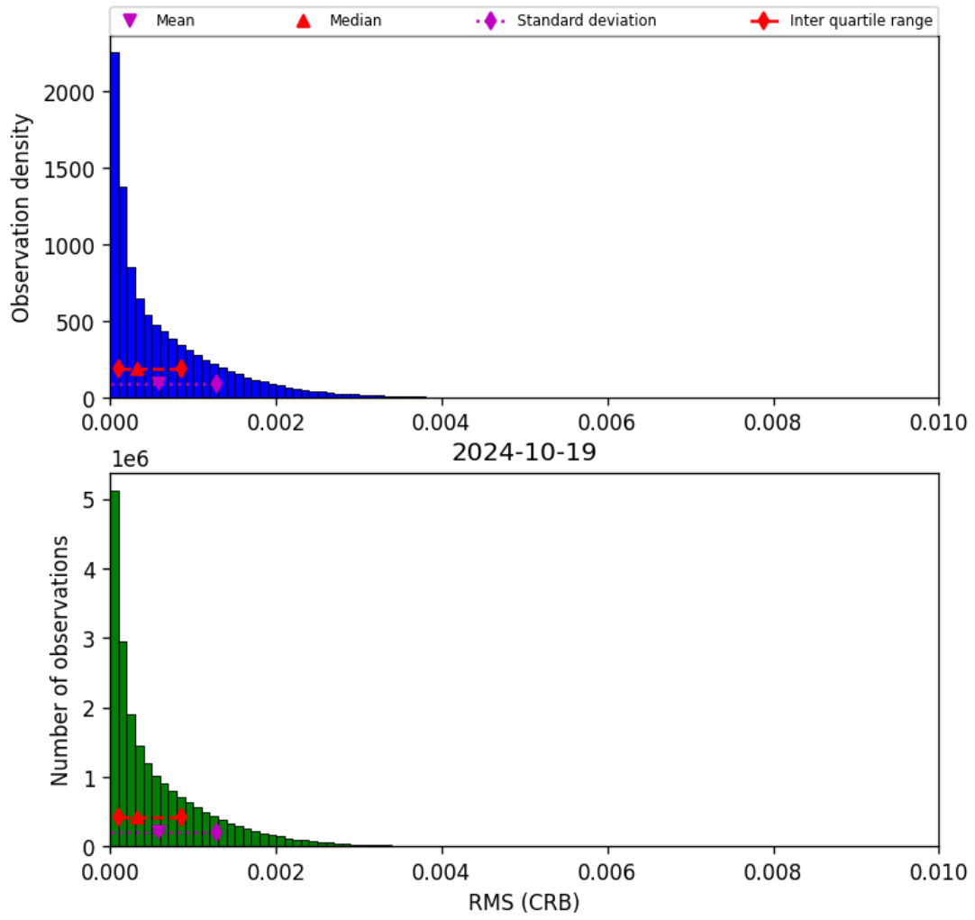
Figure 48: Histogram of “RMS (CRB)” for 2024-10-19 to 2024-10-20
