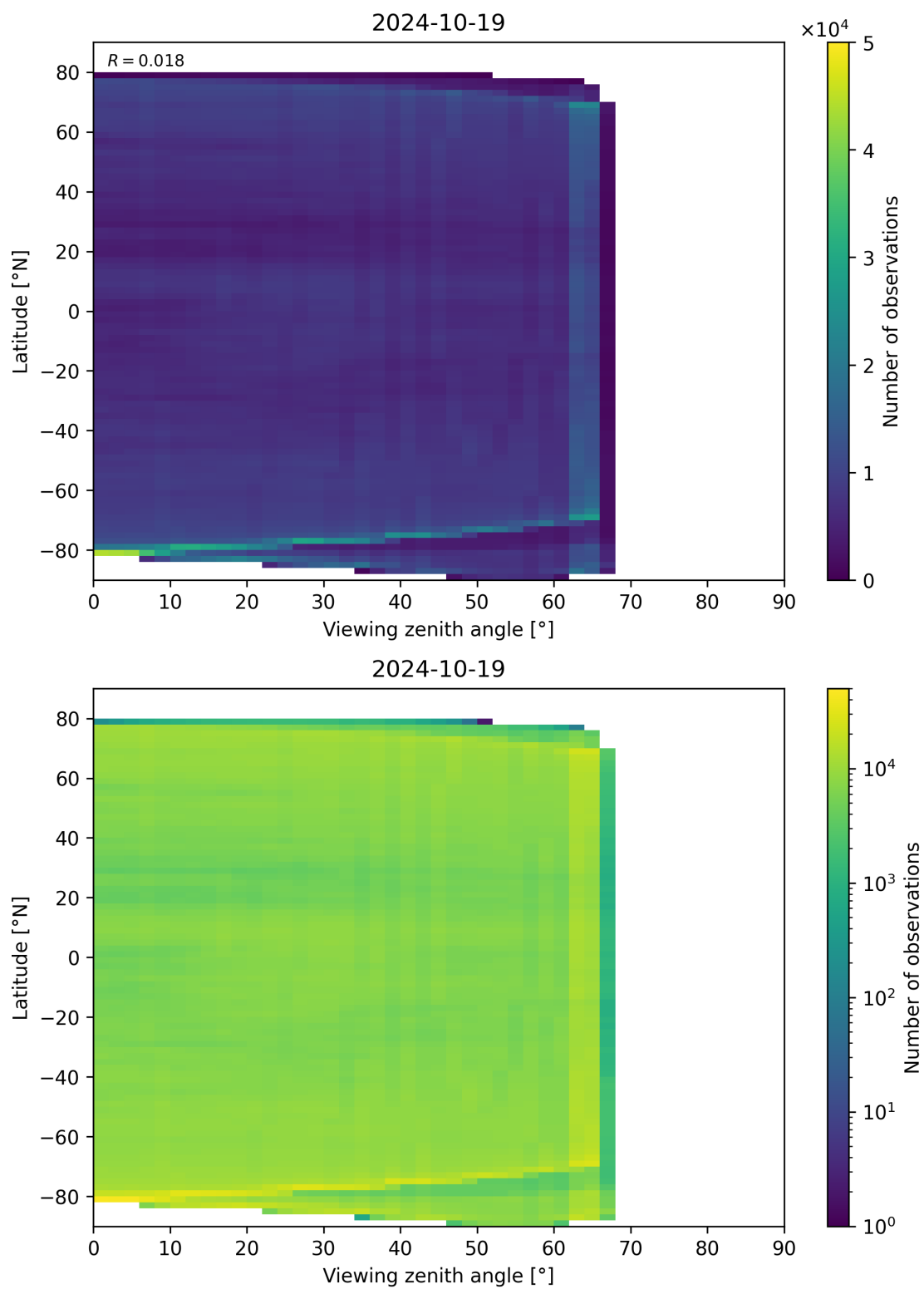
Figure 113: Scatter density plot of “Viewing zenith angle” against “Latitude” for 2024-10-19 to 2024-10-20.
