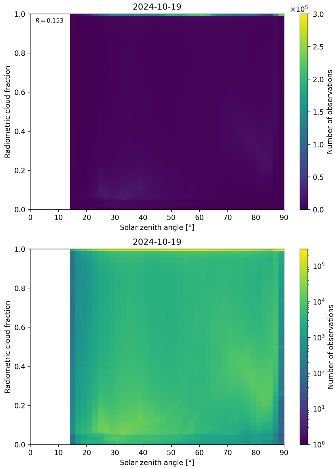
Figure 99: Scatter density plot of “Solar zenith angle” against “Radiometric cloud fraction” for 2024-10-19 to 2024-10-20.
