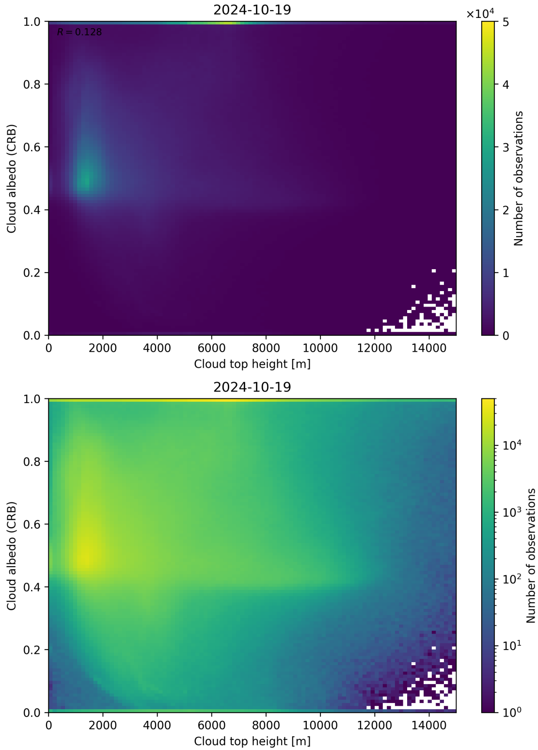
Figure 86: Scatter density plot of “Cloud top height” against “Cloud albedo (CRB)” for 2024-10-19 to 2024-10-20.
