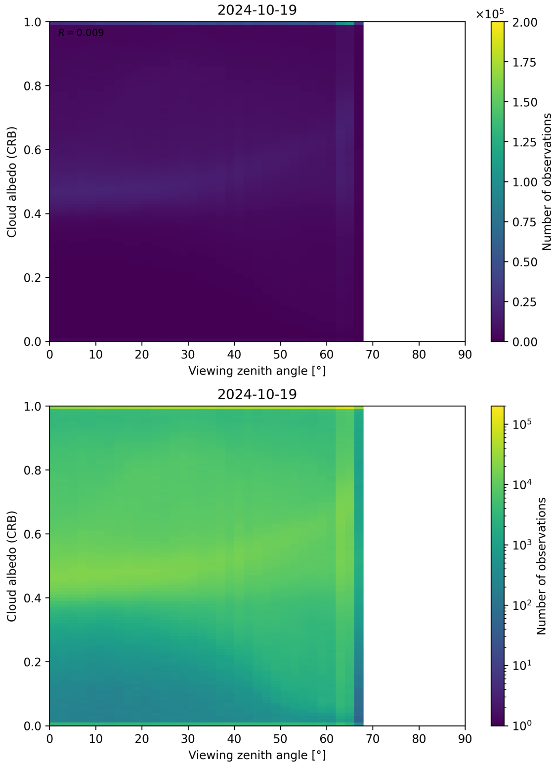
Figure 106: Scatter density plot of “Viewing zenith angle” against “Cloud albedo (CRB)” for 2024-10-19 to 2024-10-20.
