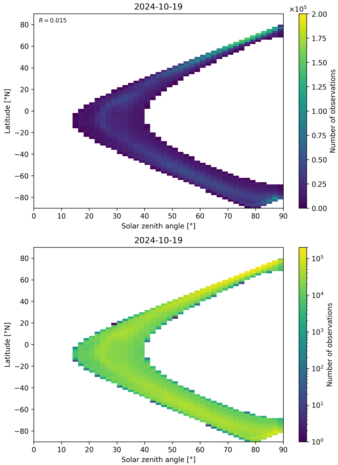
Figure 105: Scatter density plot of “Solar zenith angle” against “Latitude” for 2024-10-19 to 2024-10-20.
