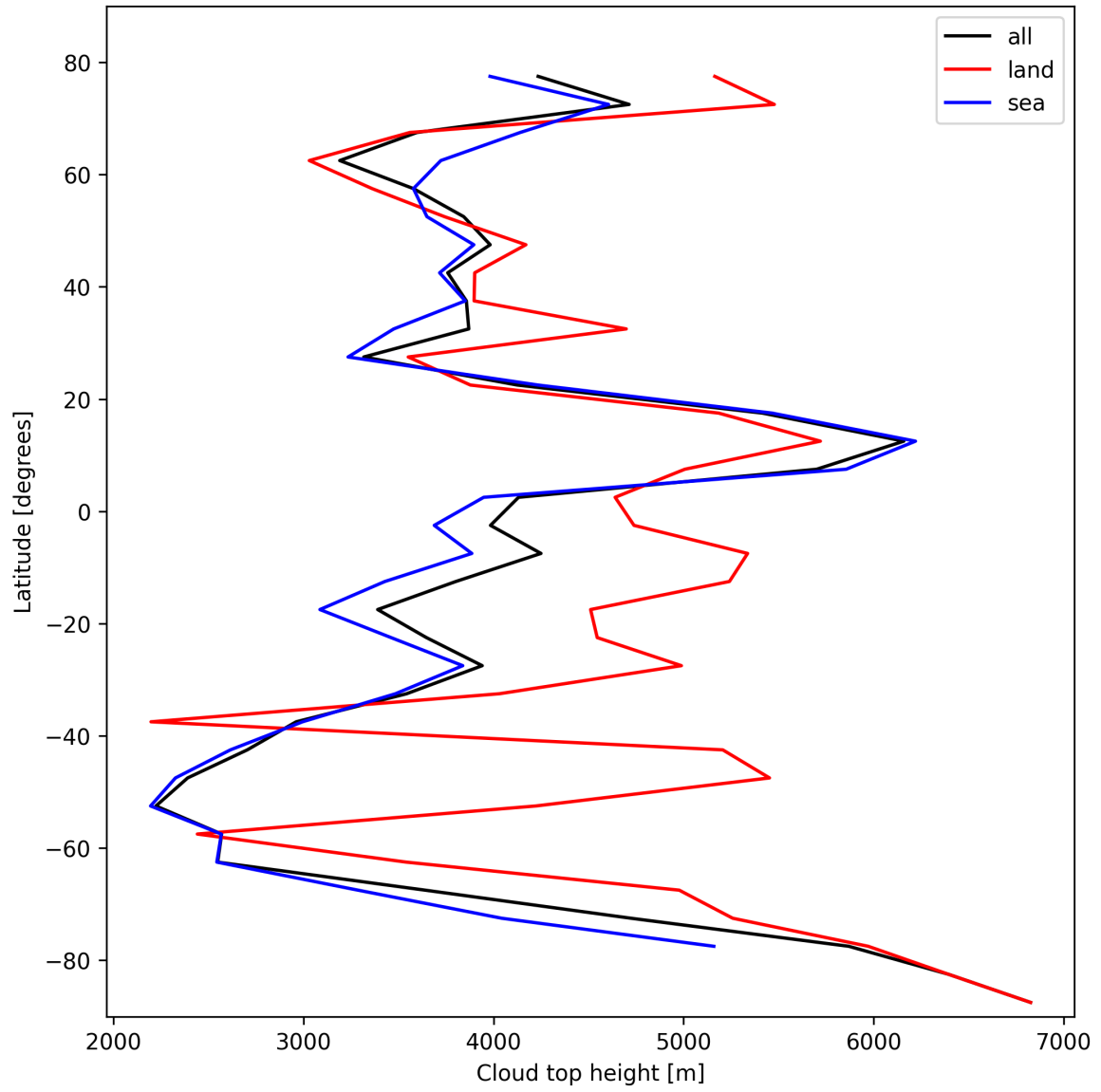
Figure 24: Zonal average of “Cloud top height” for 2024-10-19 to 2024-10-20.
