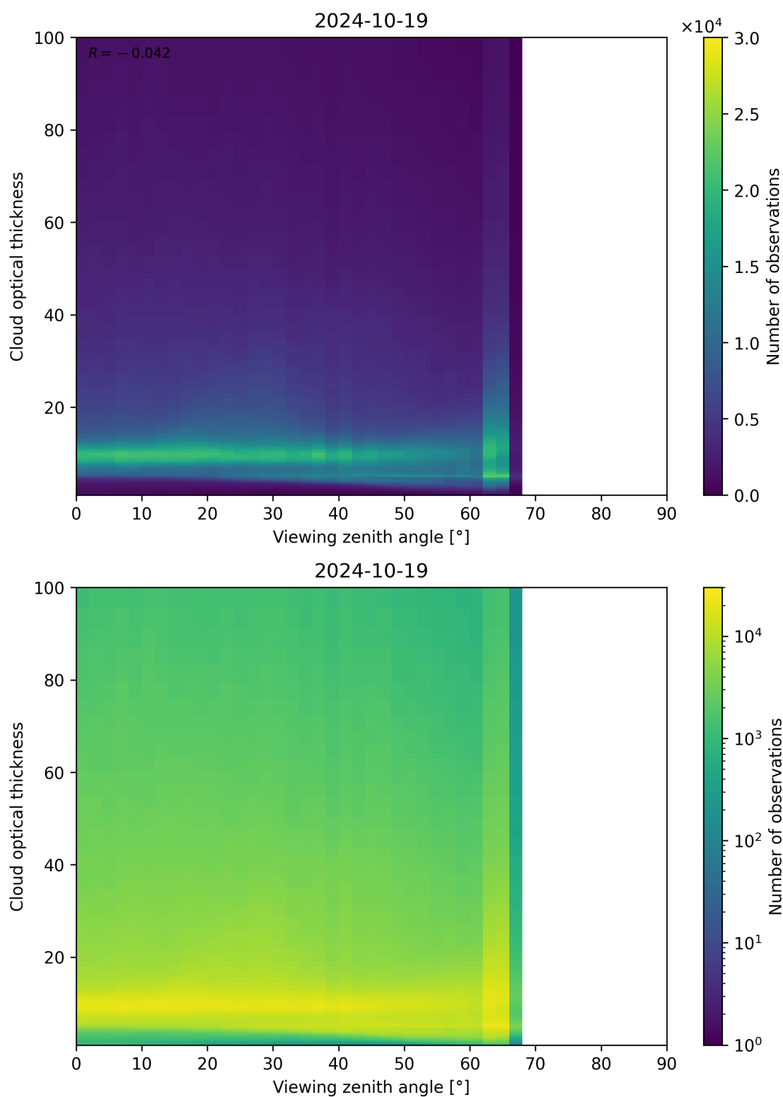
Figure 111: Scatter density plot of “Viewing zenith angle” against “Cloud optical thickness” for 2024-10-19 to 2024-10-20.
