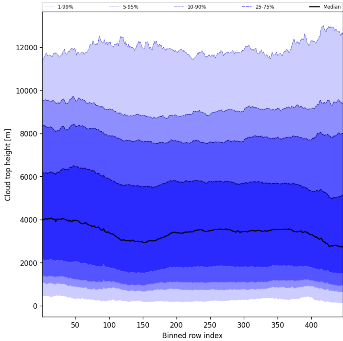
Figure 56: Along track statistics of “Cloud top height” for 2024-10-19 to 2024-10-20
