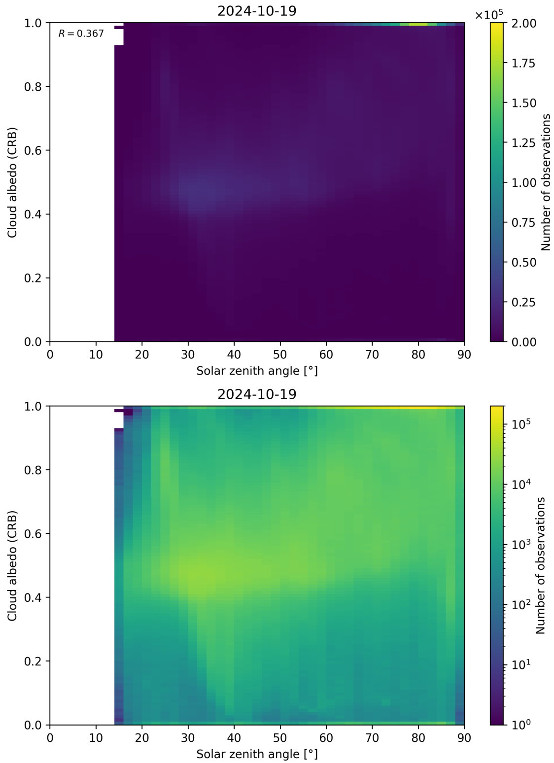
Figure 98: Scatter density plot of “Solar zenith angle” against “Cloud albedo (CRB)” for 2024-10-19 to 2024-10-20.
