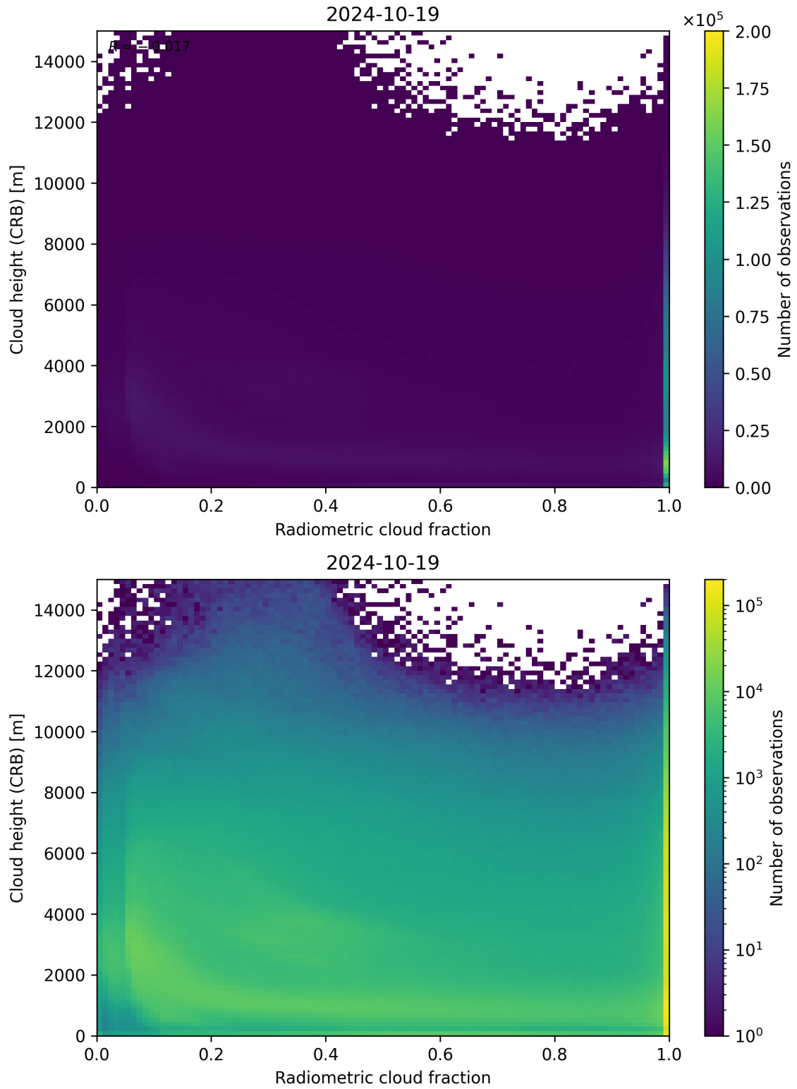
Figure 74: Scatter density plot of “Radiometric cloud fraction” against “Cloud height (CRB)” for 2024-10-19 to 2024-10-20.
