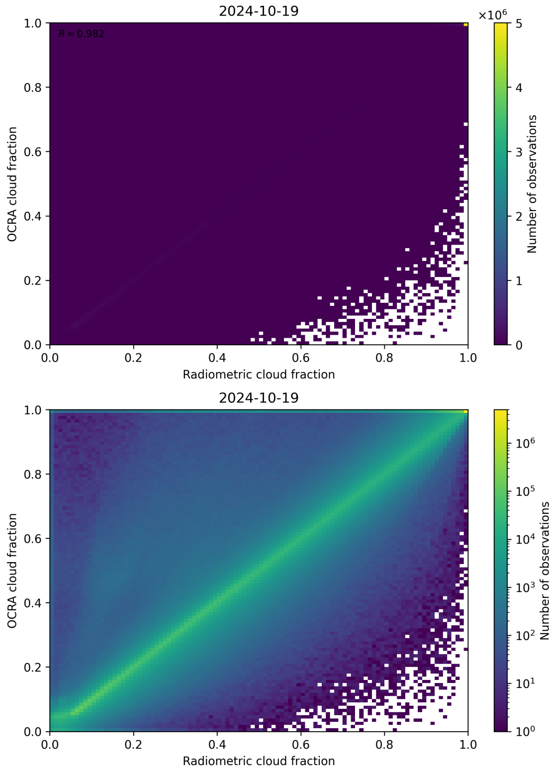
Figure 72: Scatter density plot of “Radiometric cloud fraction” against “OCRA cloud fraction” for 2024-10-19 to 2024-10-20.
