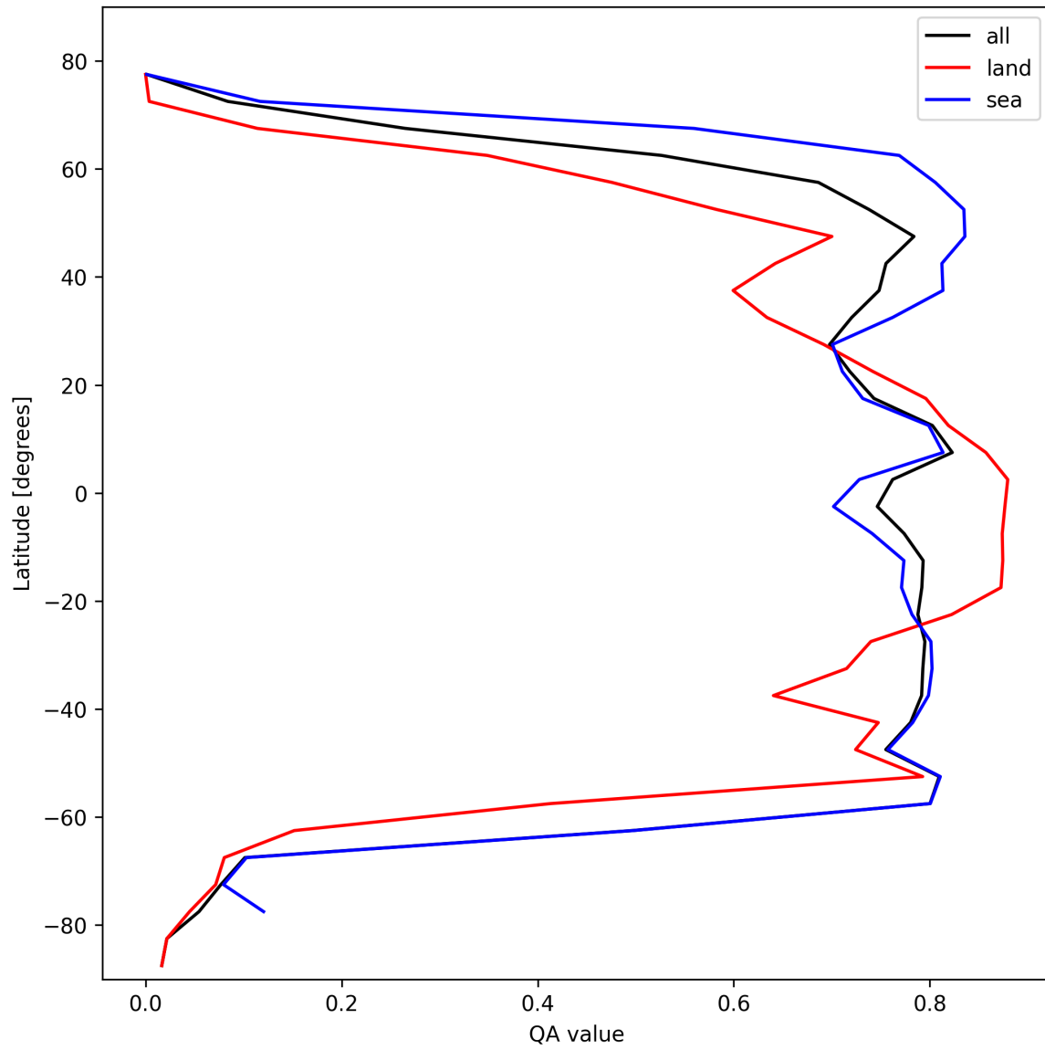
Figure 22: Zonal average of “QA value” for 2024-10-19 to 2024-10-20.
