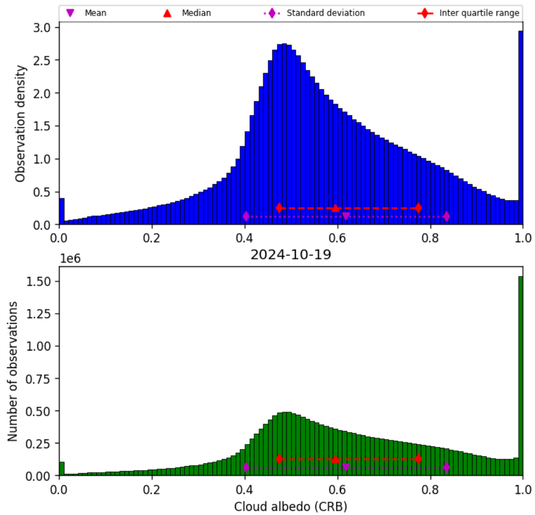
Figure 44: Histogram of “Cloud albedo (CRB)” for 2024-10-19 to 2024-10-20
