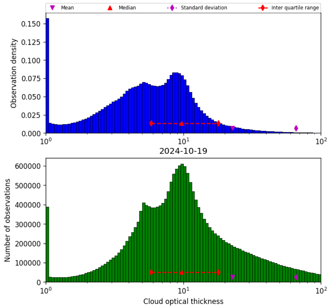
Figure 41: Histogram of “Cloud optical thickness” for 2024-10-19 to 2024-10-20
