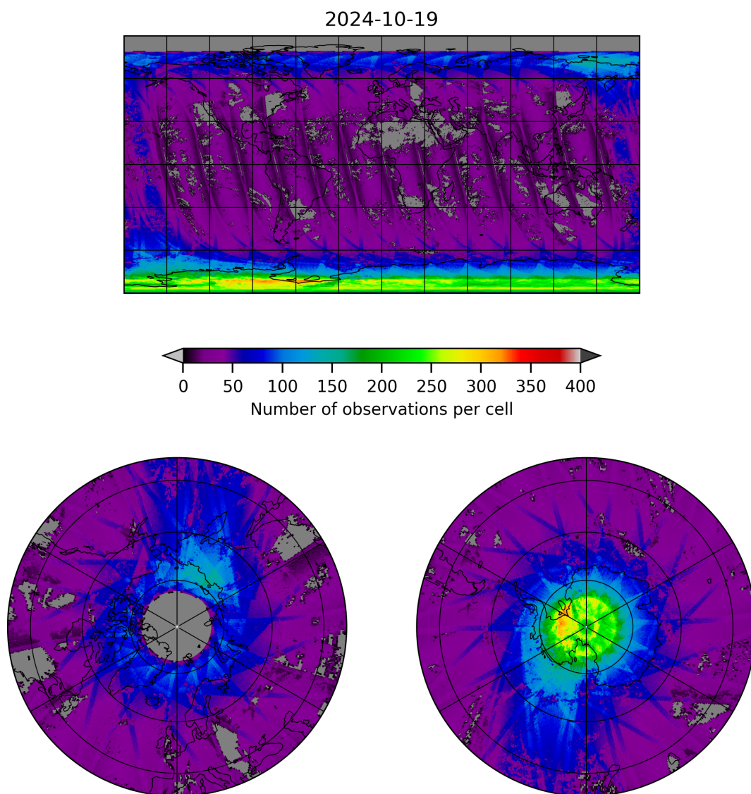
Figure 21: Map of the number of observations for 2024-10-19 to 2024-10-20
