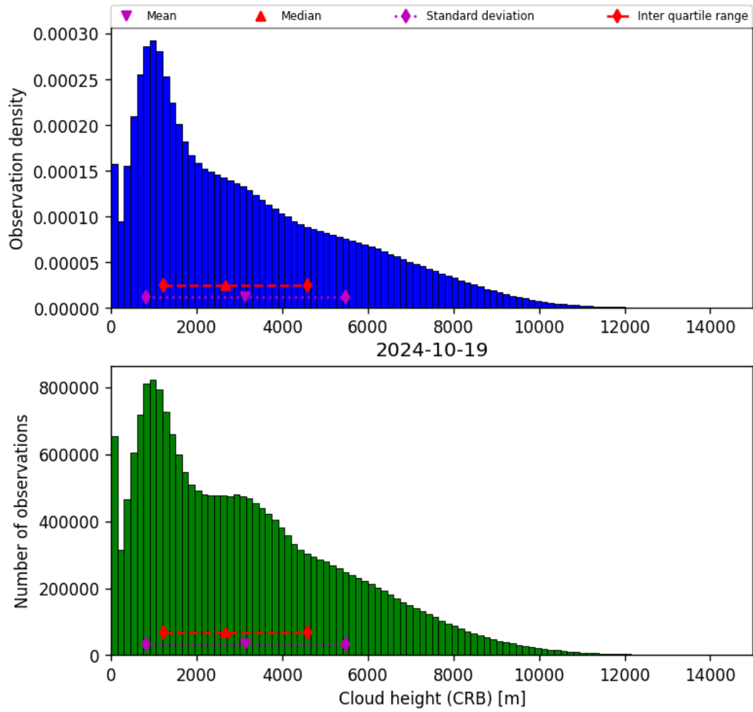
Figure 43: Histogram of “Cloud height (CRB)” for 2024-10-19 to 2024-10-20
