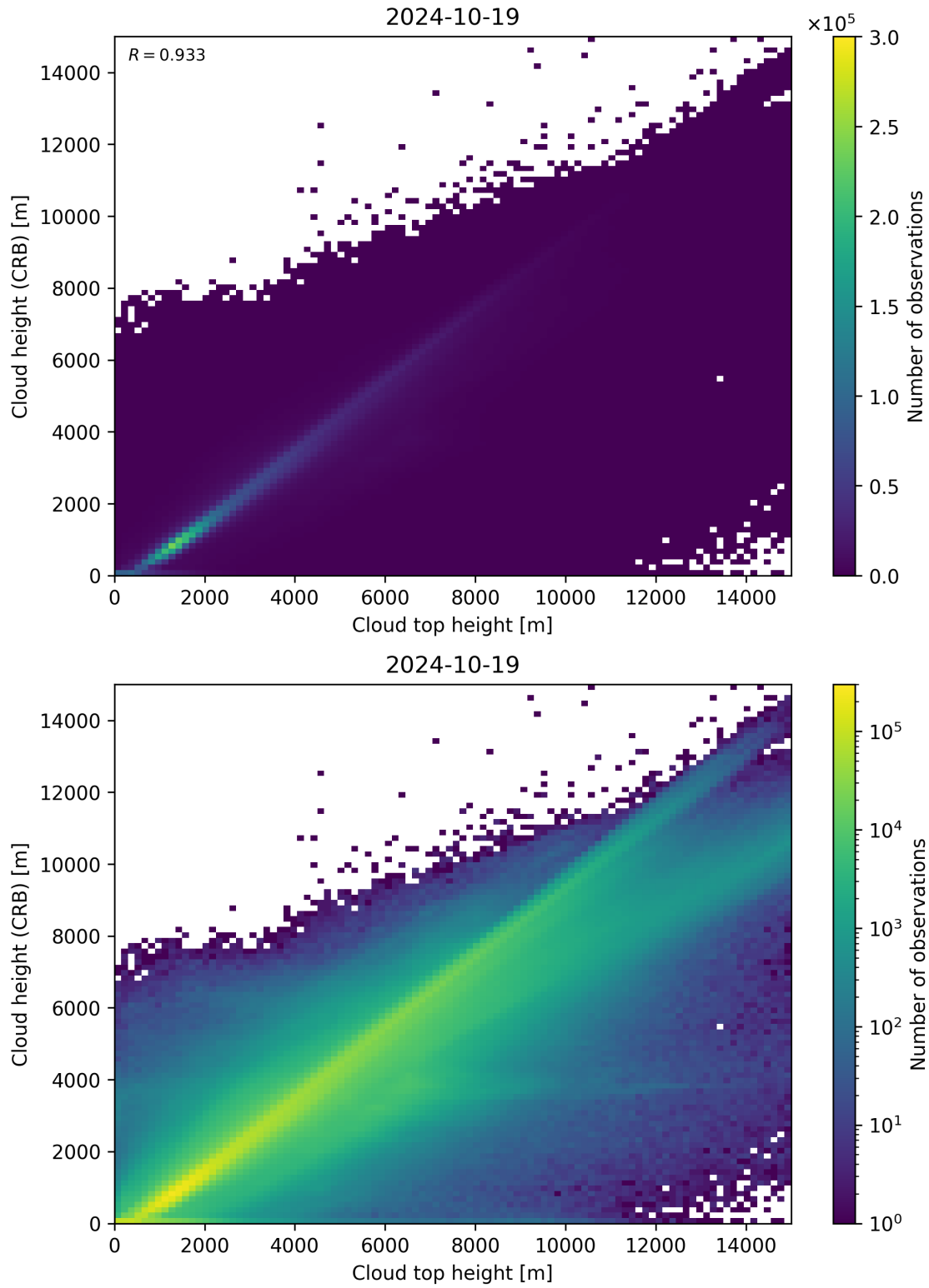
Figure 89: Scatter density plot of “Cloud top height” against “Cloud height (CRB)” for 2024-10-19 to 2024-10-20.
