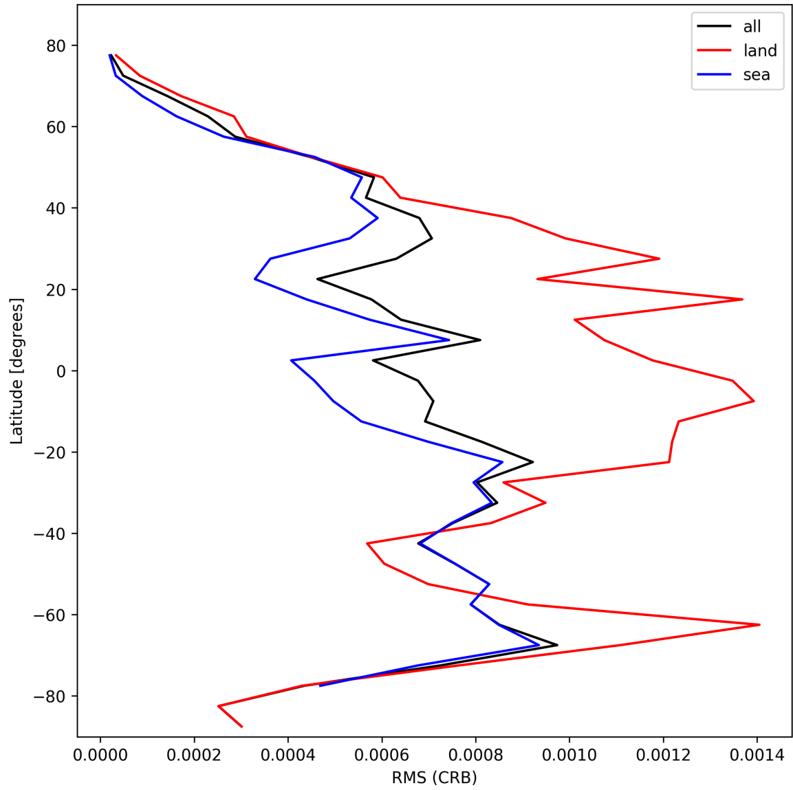
Figure 32: Zonal average of “RMS (CRB)” for 2024-10-19 to 2024-10-20.
