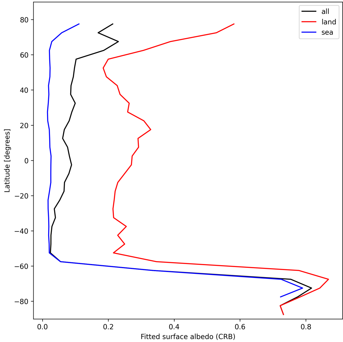
Figure 30: Zonal average of “Fitted surface albedo (CRB)” for 2024-10-19 to 2024-10-20.
