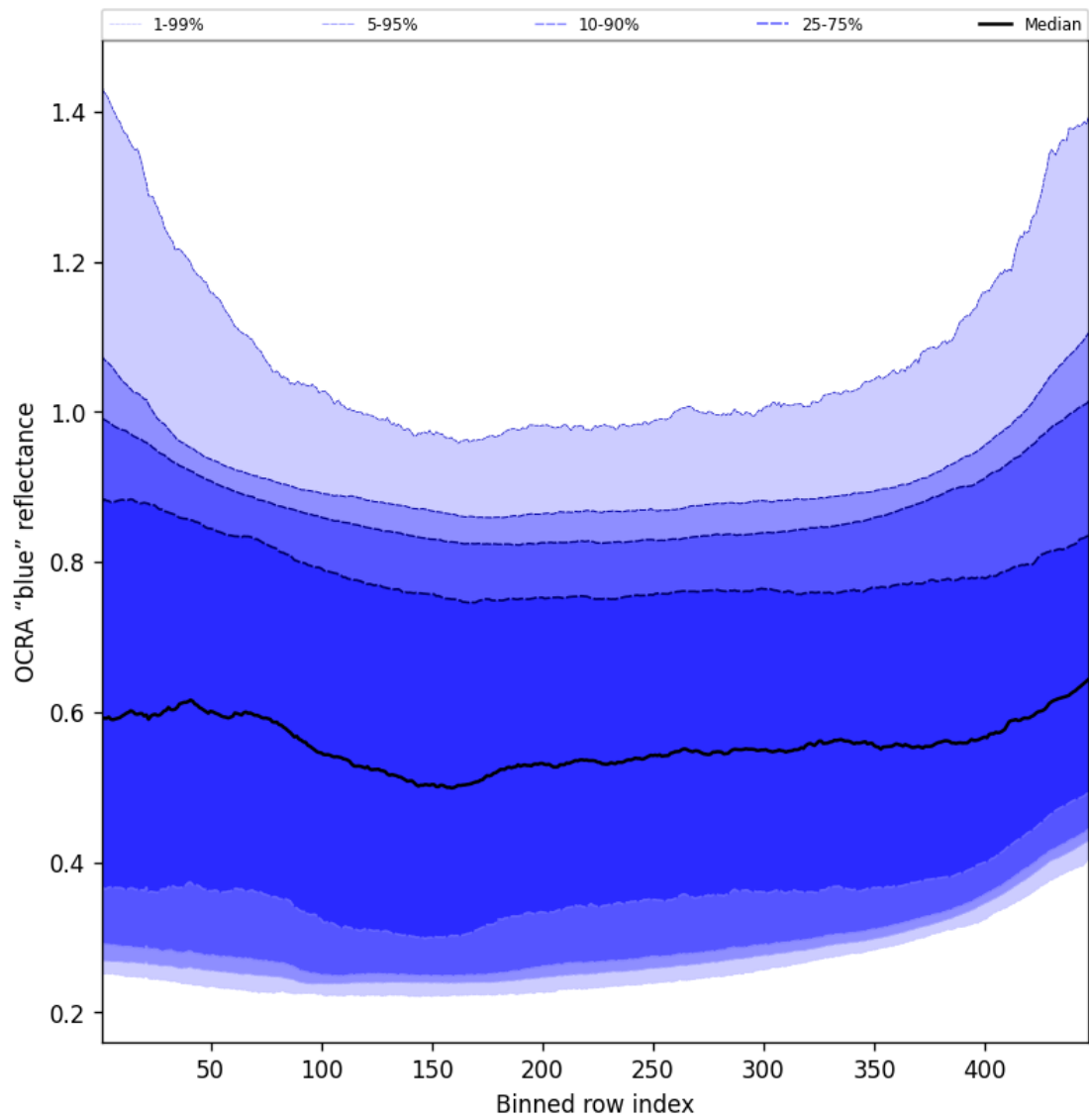
Figure 67: Along track statistics of “OCRA “blue” reflectance” for 2024-10-19 to 2024-10-20
