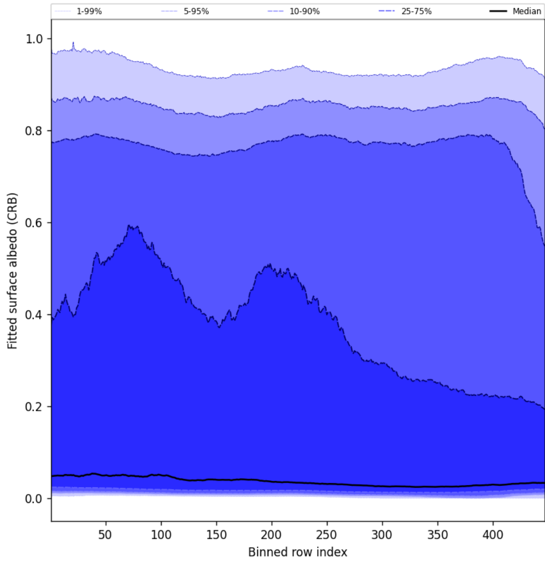
Figure 62: Along track statistics of “Fitted surface albedo (CRB)” for 2024-10-19 to 2024-10-20
