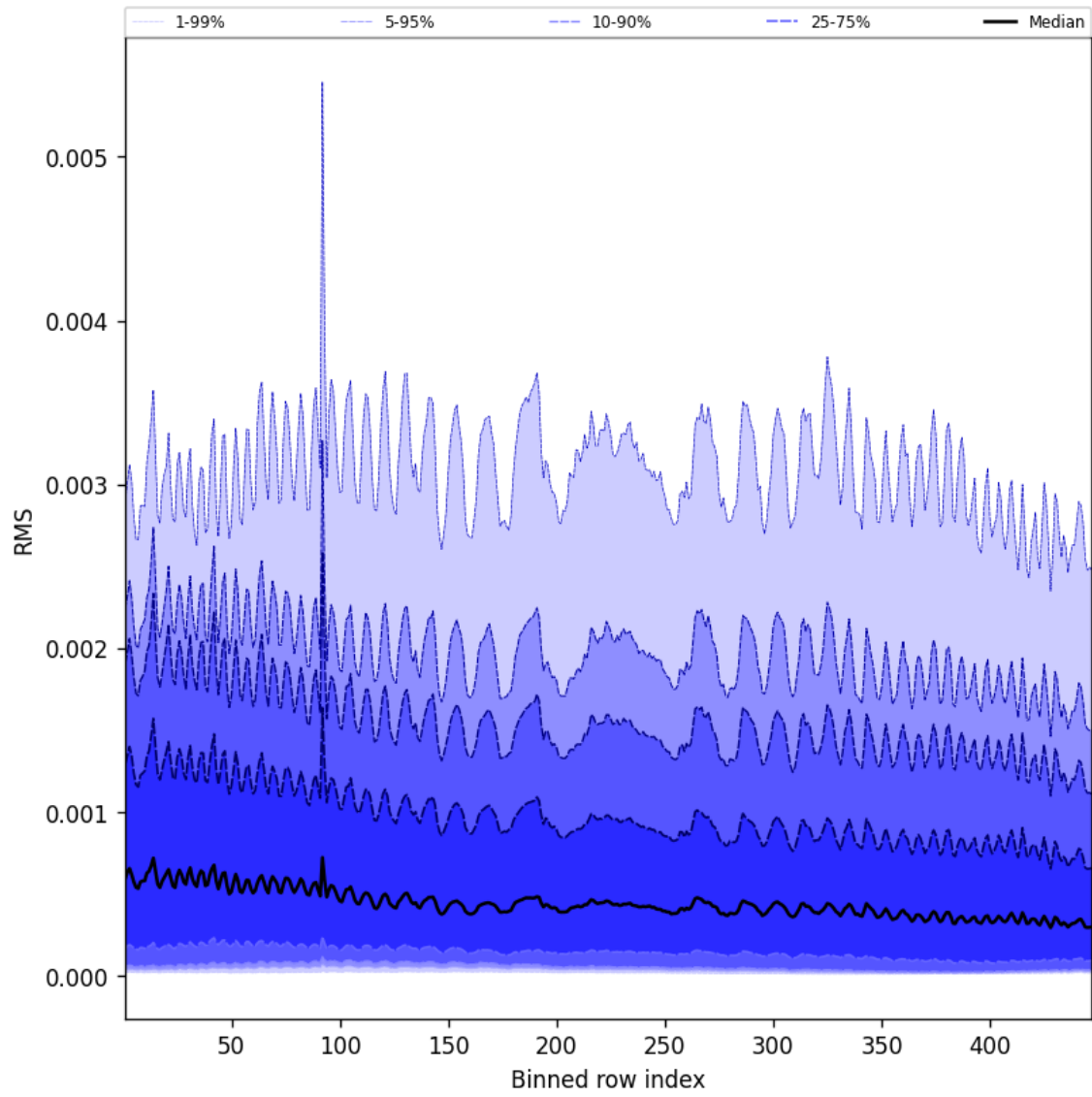
Figure 63: Along track statistics of “RMS” for 2024-10-19 to 2024-10-20
