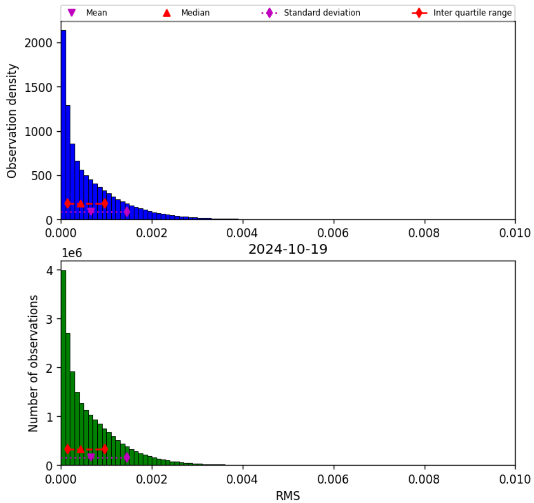
Figure 47: Histogram of “RMS” for 2024-10-19 to 2024-10-20
