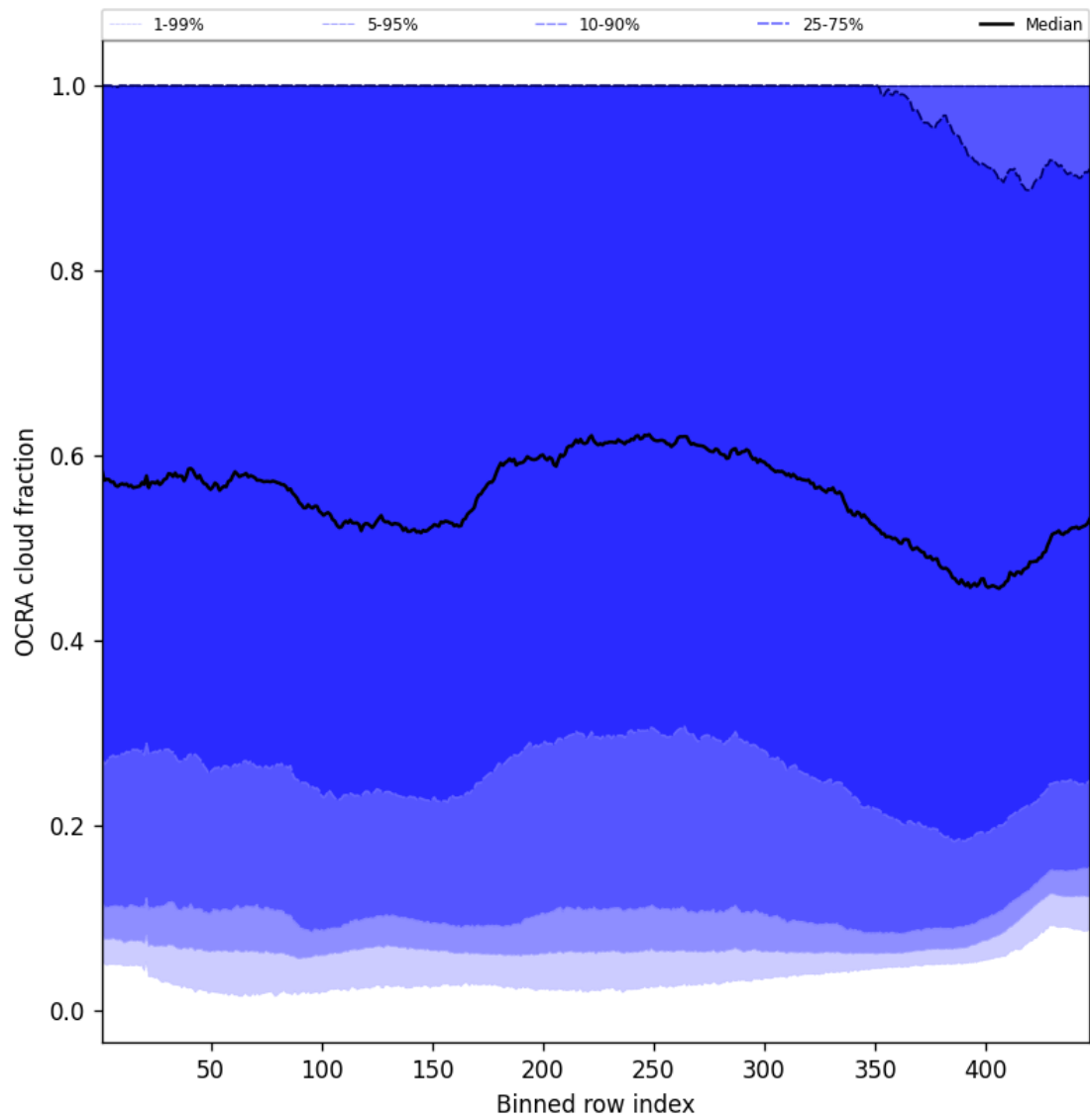
Figure 66: Along track statistics of “OCRA cloud fraction” for 2024-10-19 to 2024-10-20
