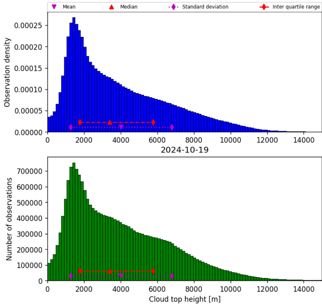
Figure 40: Histogram of “Cloud top height” for 2024-10-19 to 2024-10-20
