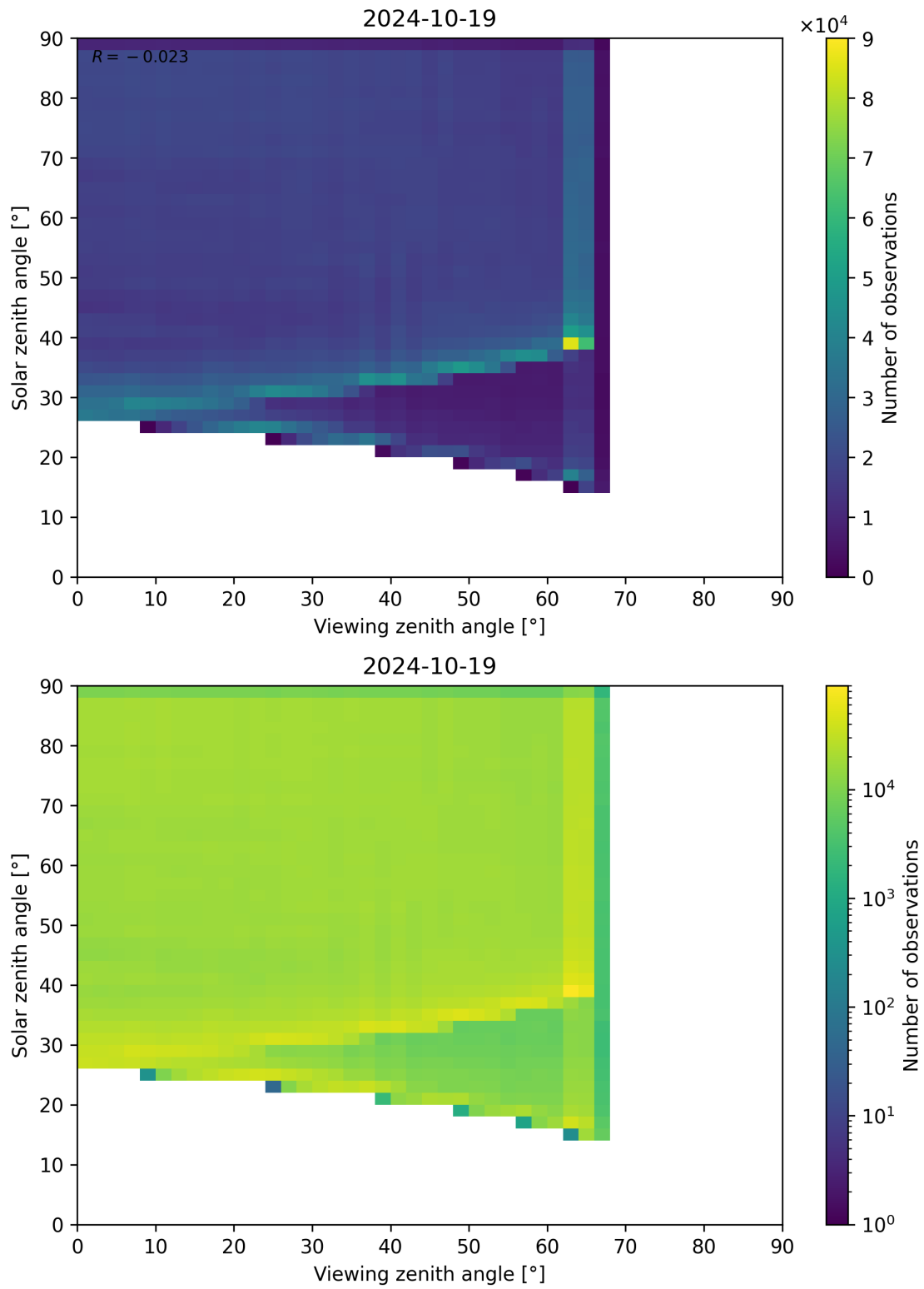
Figure 114: Scatter density plot of “Viewing zenith angle” against “Solar zenith angle” for 2024-10-19 to 2024-10-20.
