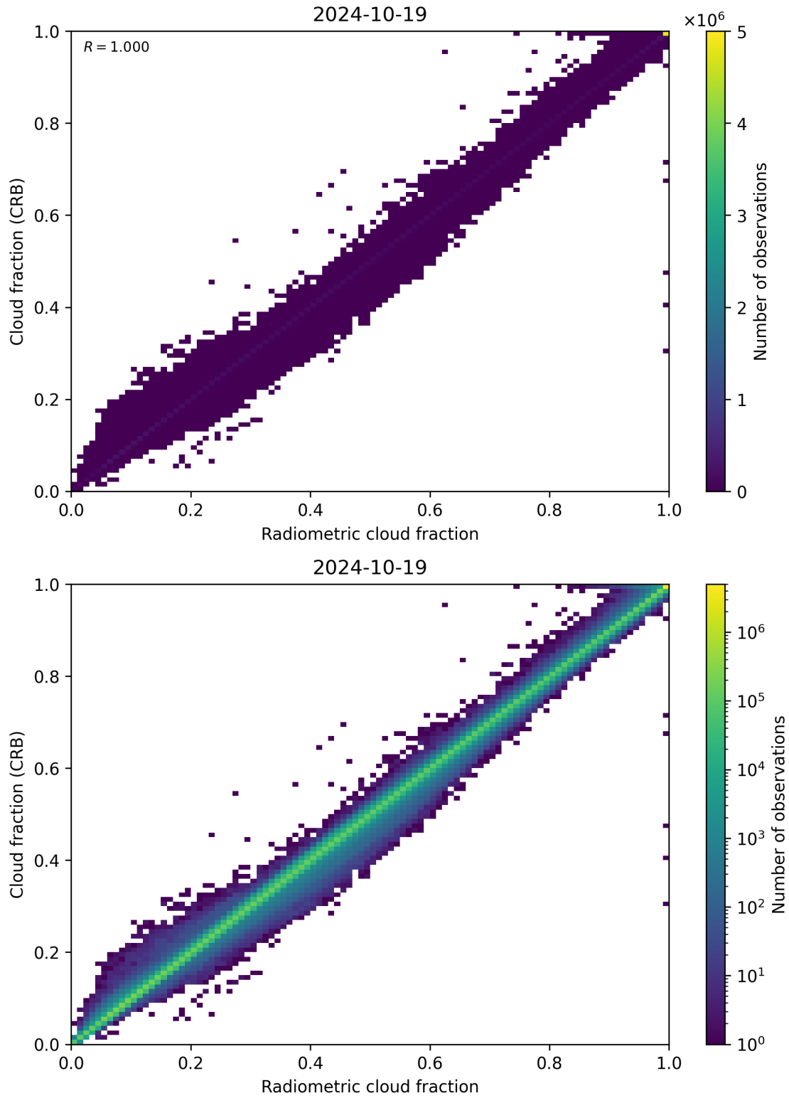
Figure 73: Scatter density plot of “Radiometric cloud fraction” against “Cloud fraction (CRB)” for 2024-10-19 to 2024-10-20.
