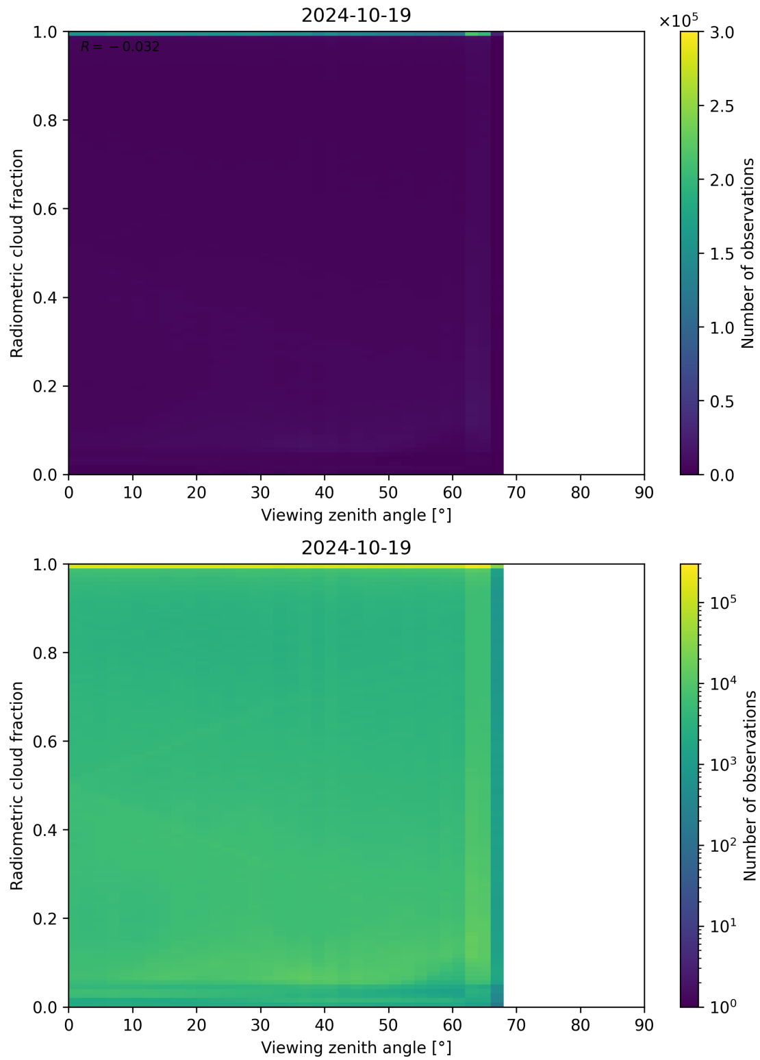
Figure 107: Scatter density plot of “Viewing zenith angle” against “Radiometric cloud fraction” for 2024-10-19 to 2024-10-20.
