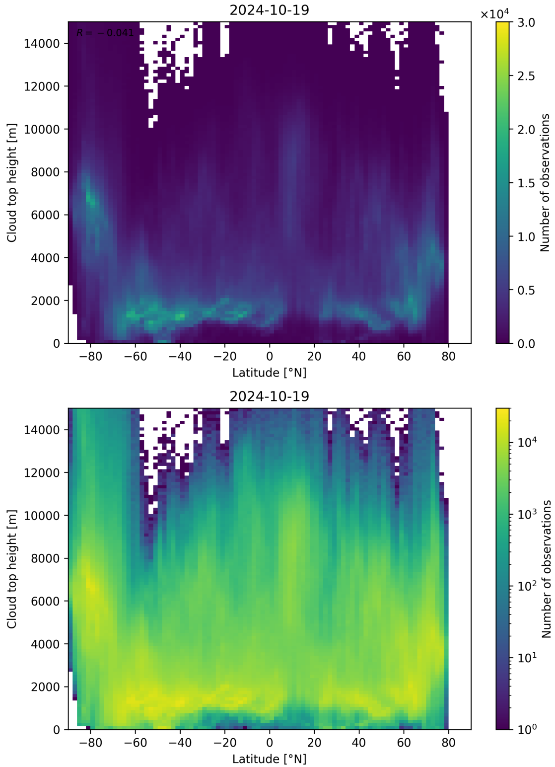
Figure 97: Scatter density plot of “Latitude” against “Cloud top height” for 2024-10-19 to 2024-10-20.
