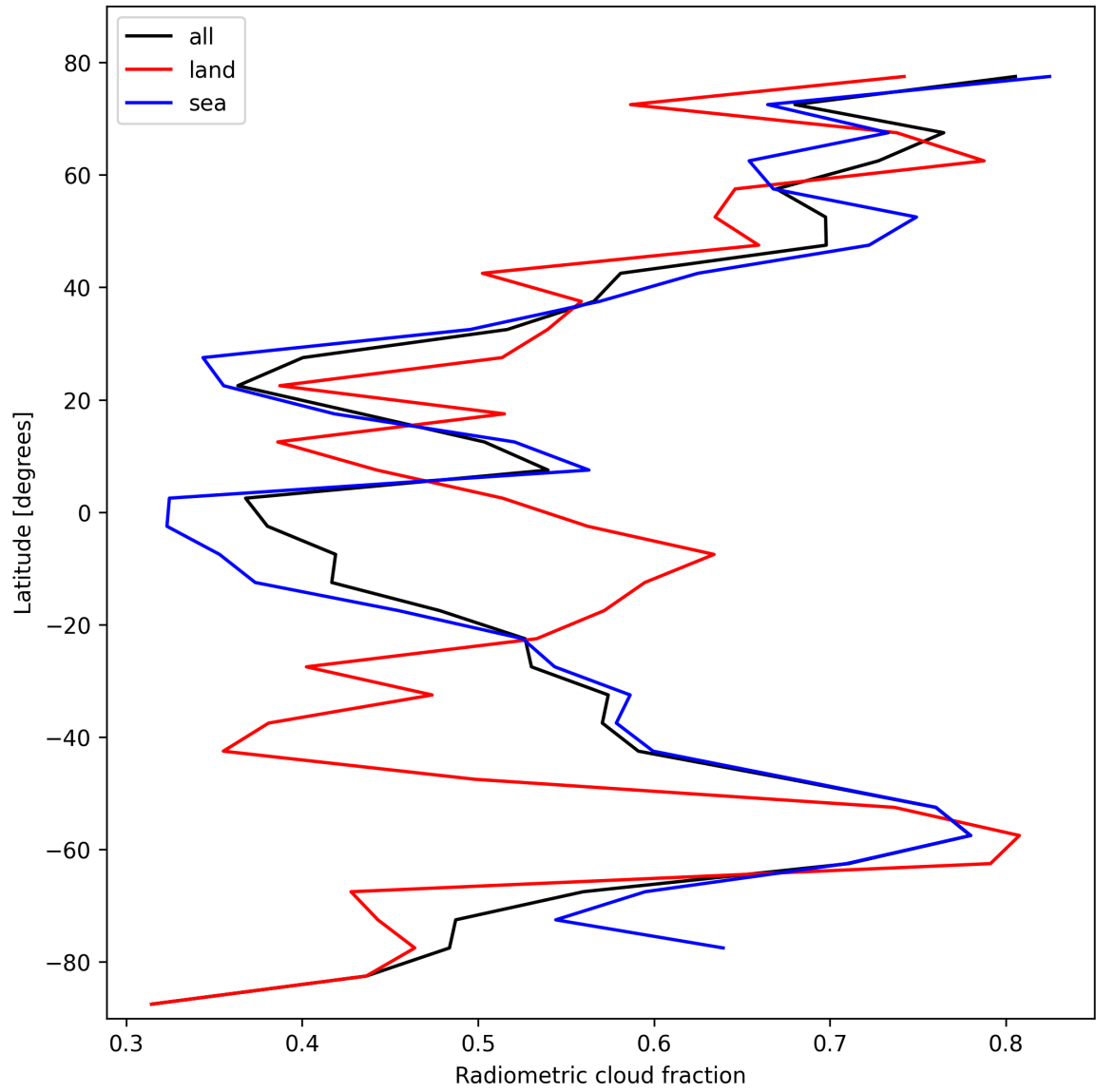
Figure 23: Zonal average of “Radiometric cloud fraction” for 2024-10-19 to 2024-10-20.
