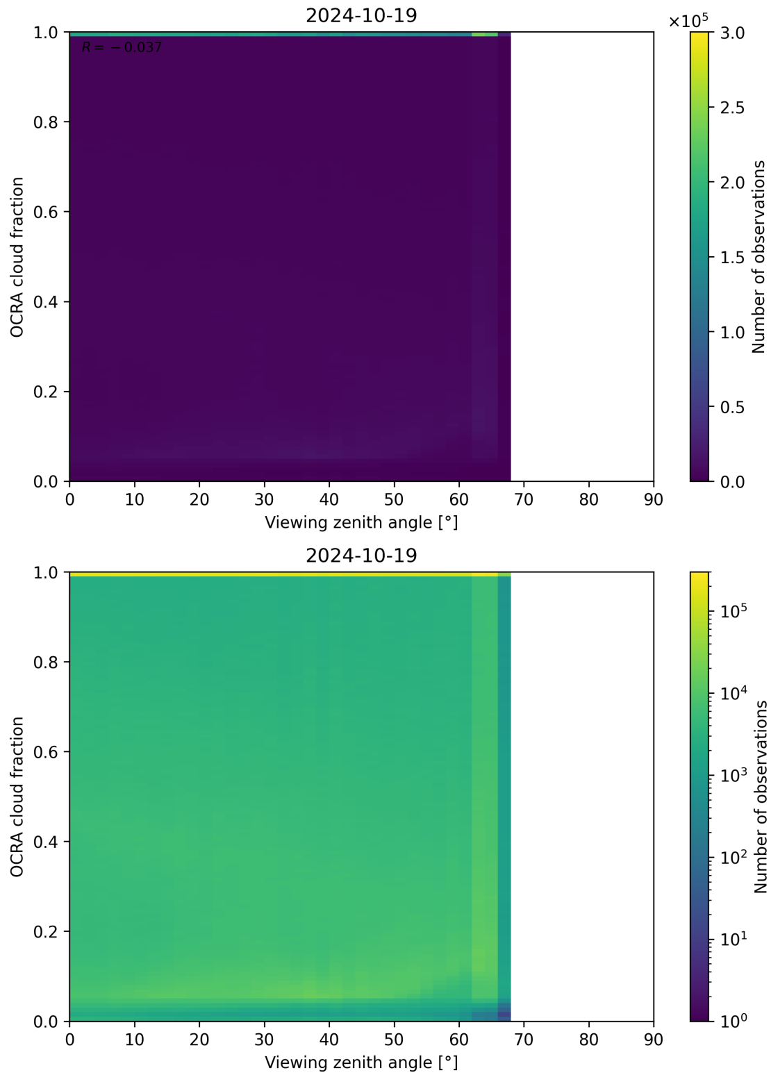
Figure 108: Scatter density plot of “Viewing zenith angle” against “OCRA cloud fraction” for 2024-10-19 to 2024-10-20.
