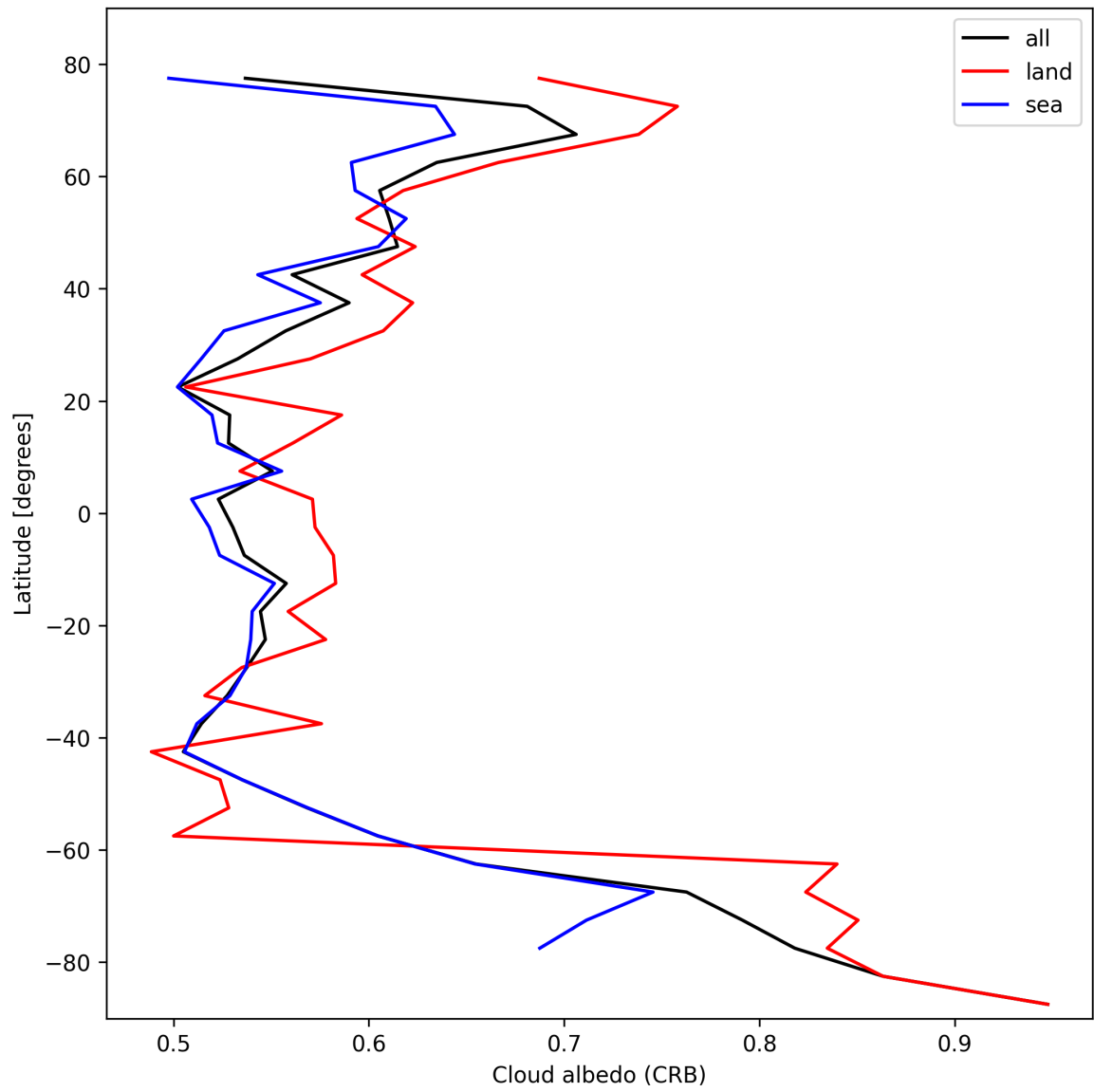
Figure 28: Zonal average of “Cloud albedo (CRB)” for 2024-10-19 to 2024-10-20.
