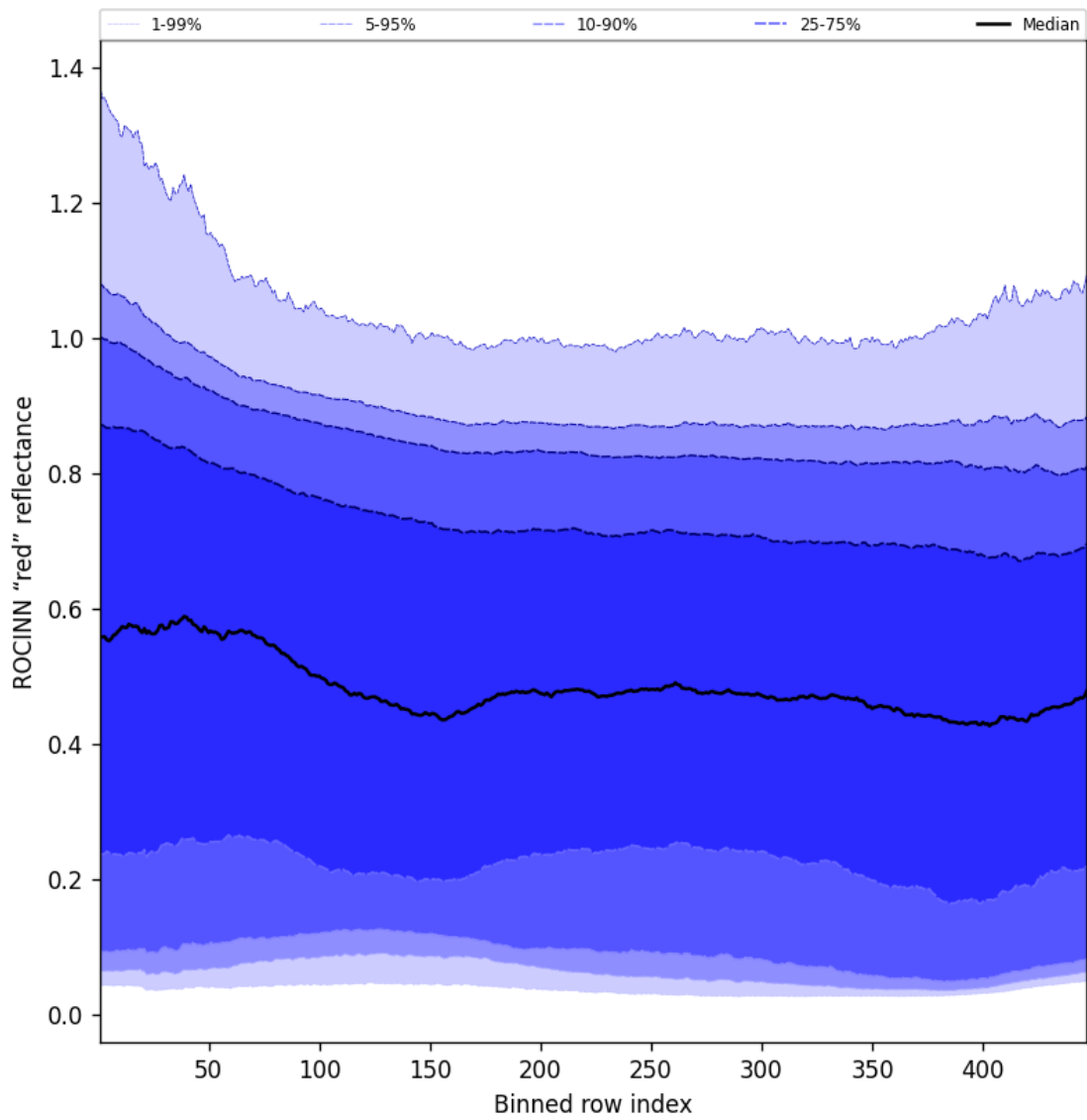
Figure 69: Along track statistics of “ROCINN “red” reflectance” for 2024-10-19 to 2024-10-20
