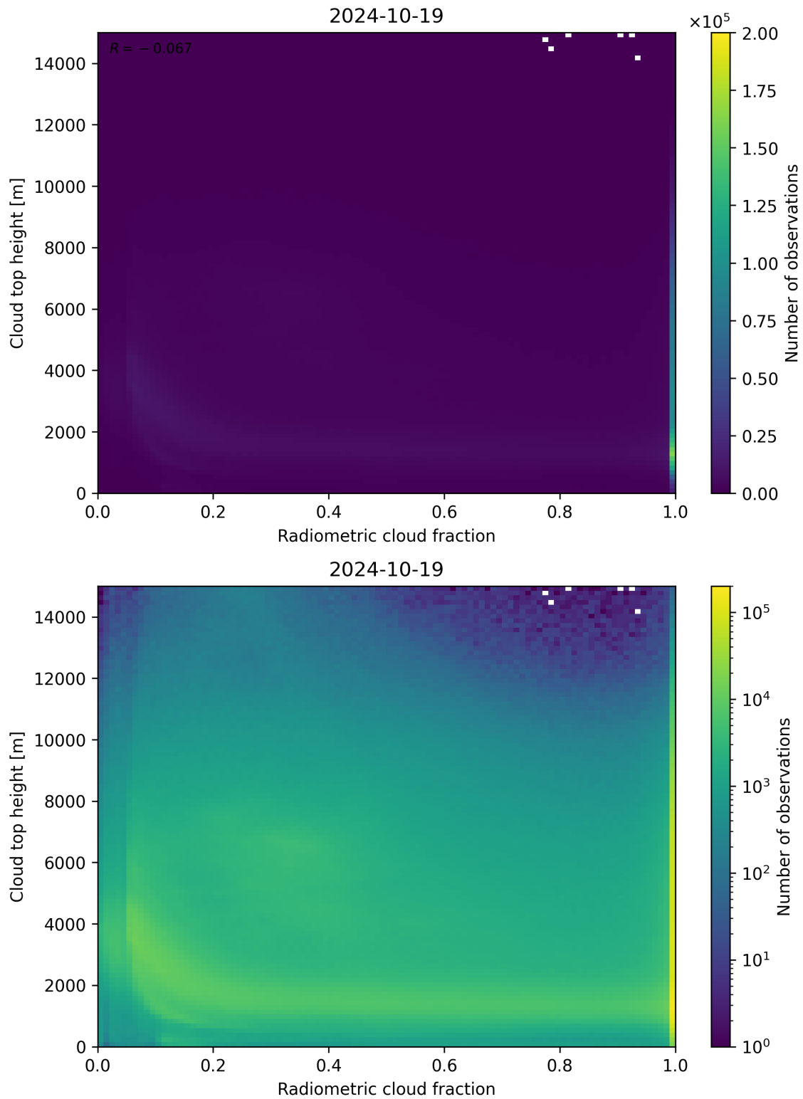
Figure 76: Scatter density plot of “Radiometric cloud fraction” against “Cloud top height” for 2024-10-19 to 2024-10-20.
