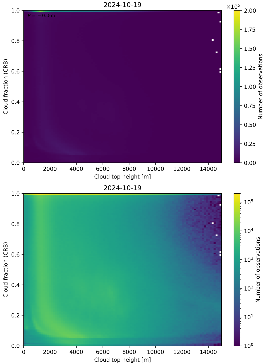
Figure 88: Scatter density plot of “Cloud top height” against “Cloud fraction (CRB)” for 2024-10-19 to 2024-10-20.
