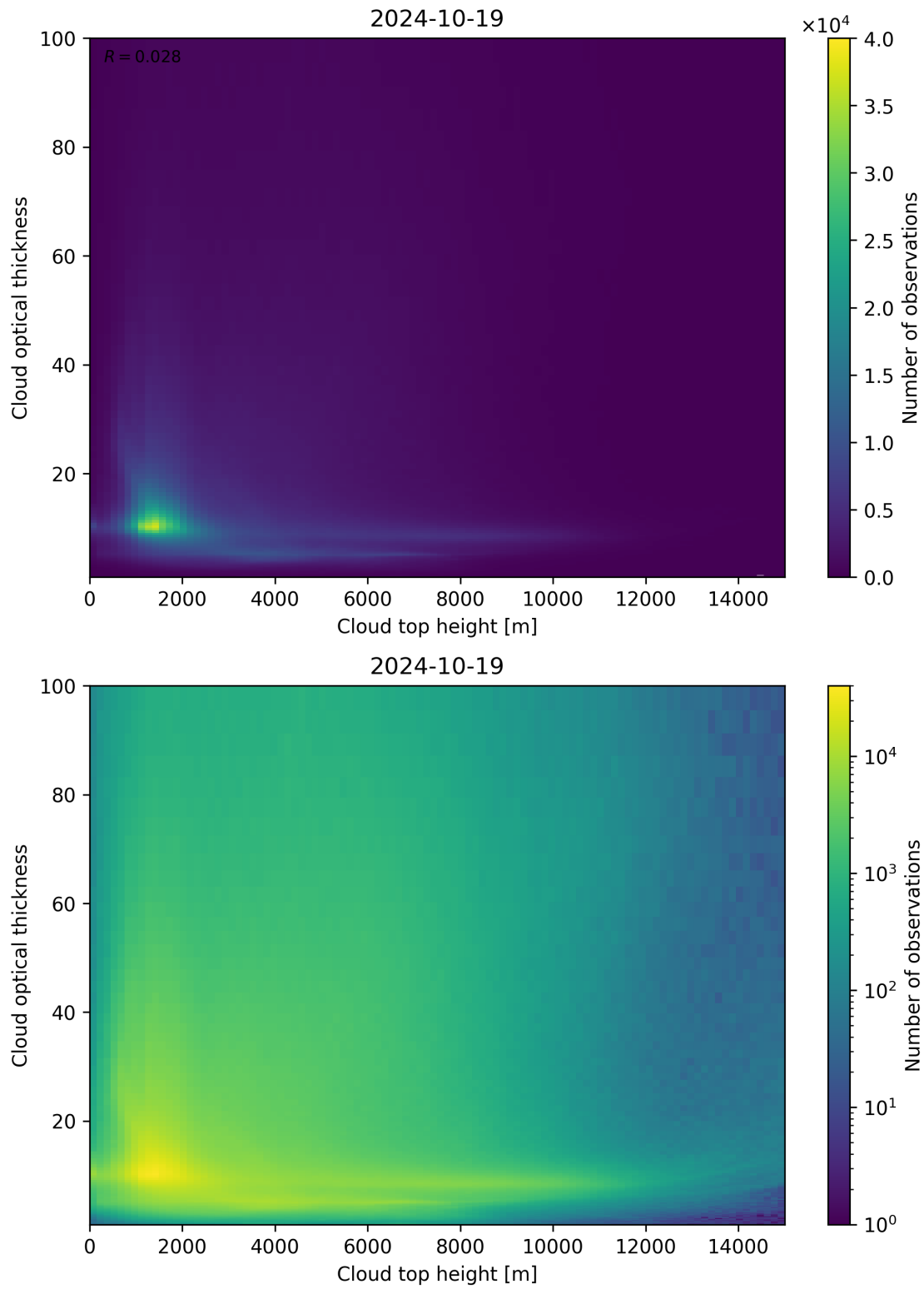
Figure 90: Scatter density plot of “Cloud top height” against “Cloud optical thickness” for 2024-10-19 to 2024-10-20.
