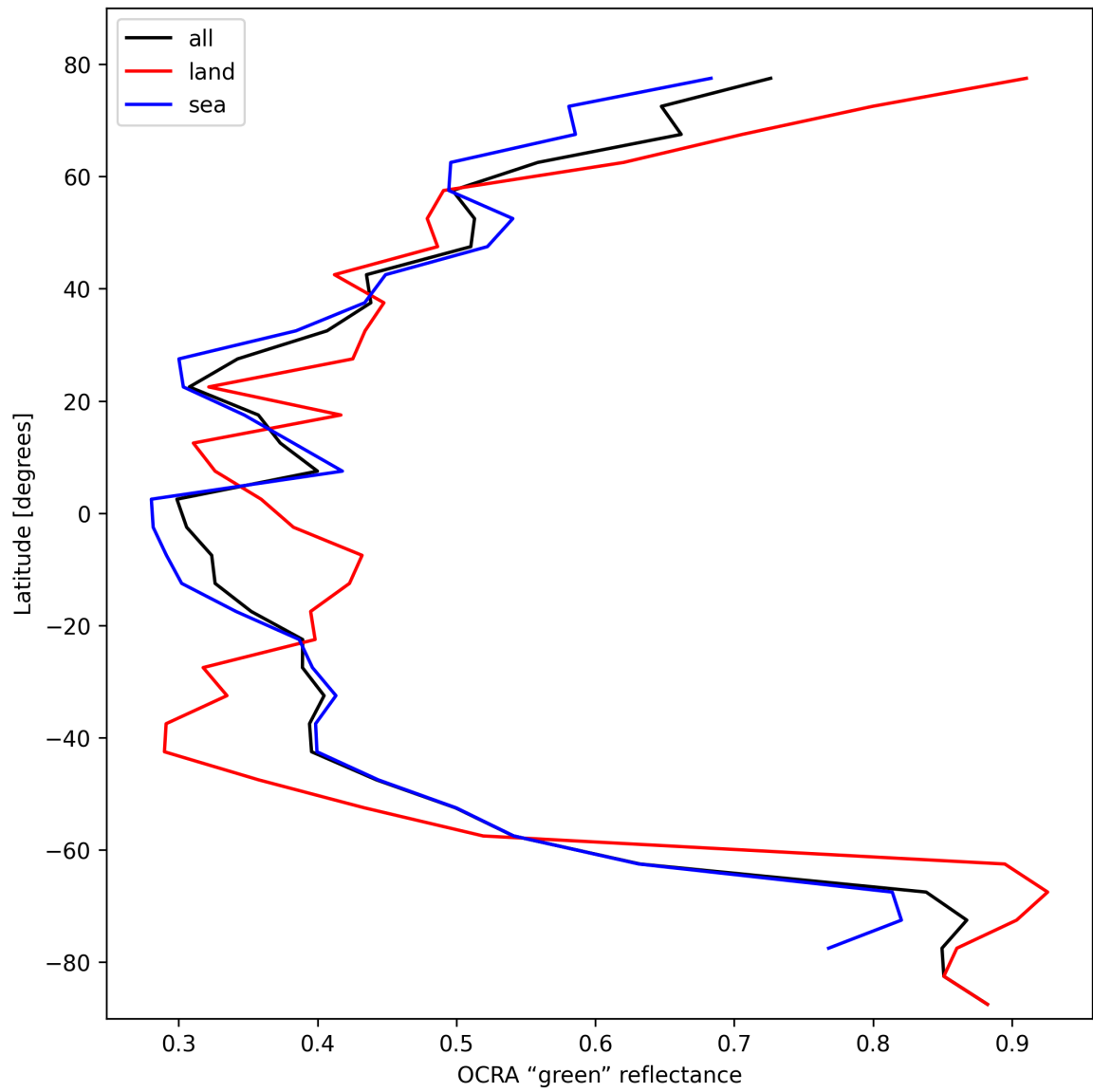
Figure 36: Zonal average of “OCRA “green” reflectance” for 2024-10-19 to 2024-10-20.
