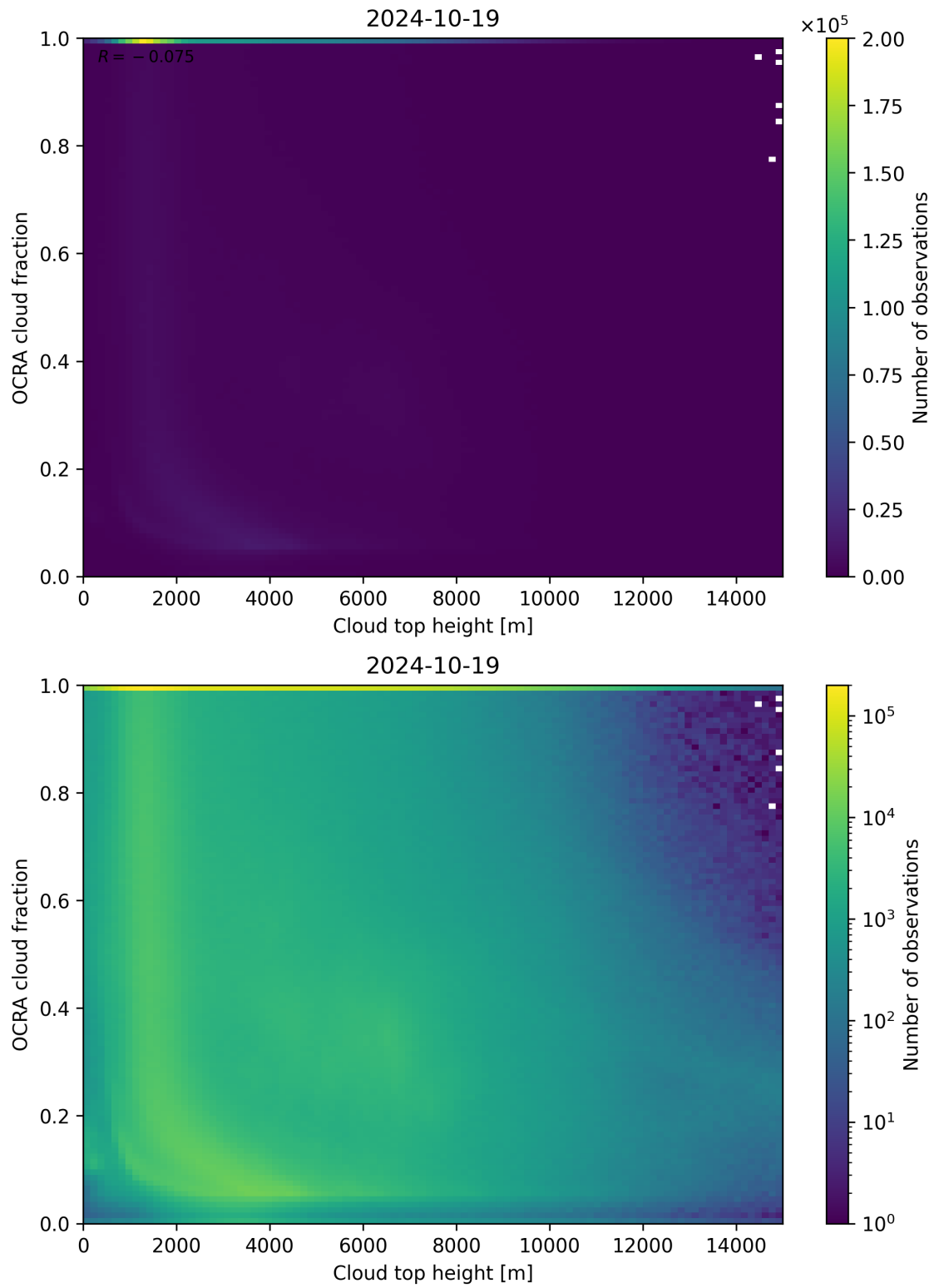
Figure 87: Scatter density plot of “Cloud top height” against “OCRA cloud fraction” for 2024-10-19 to 2024-10-20.
