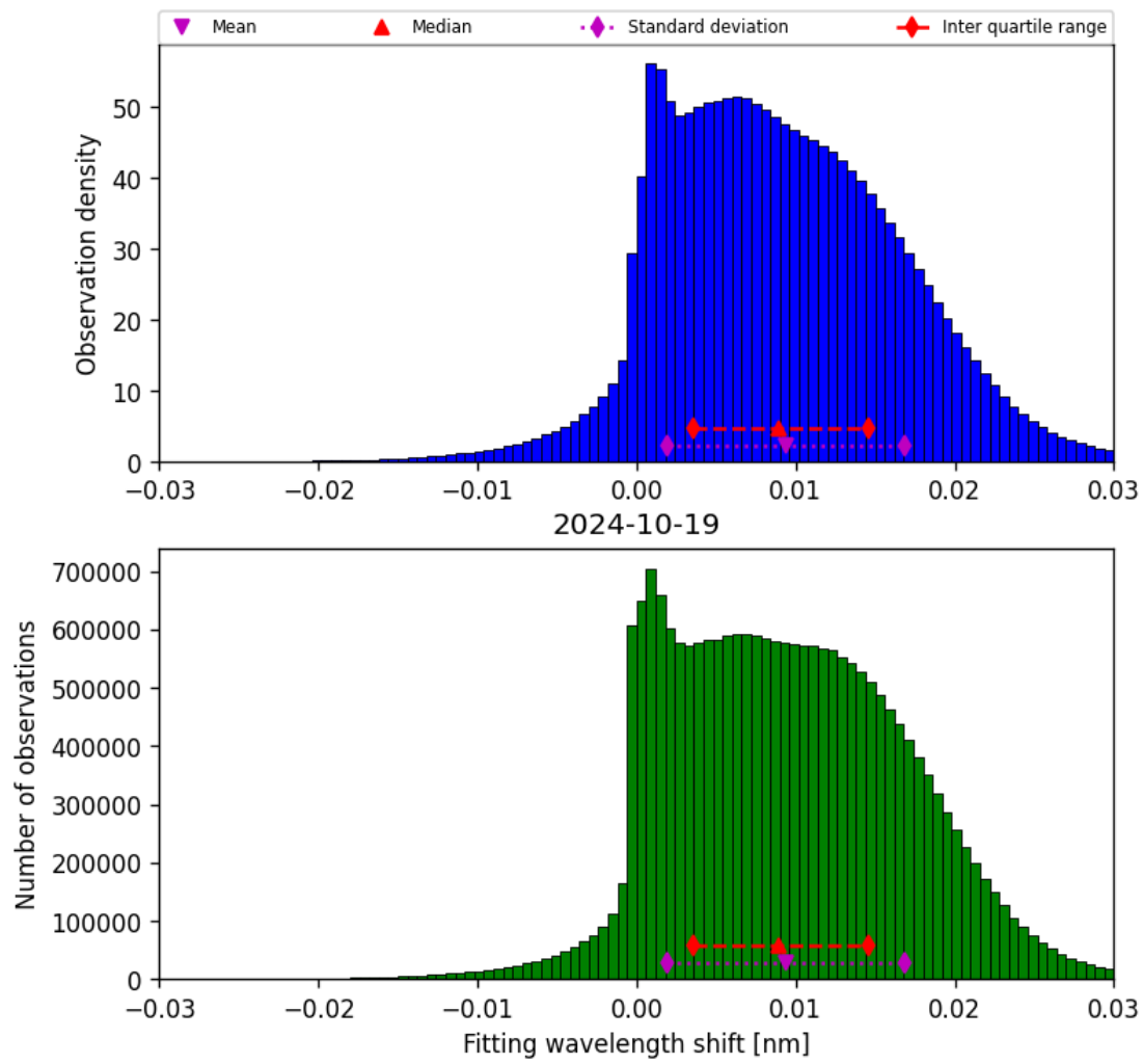
Figure 49: Histogram of “Fitting wavelength shift” for 2024-10-19 to 2024-10-20
