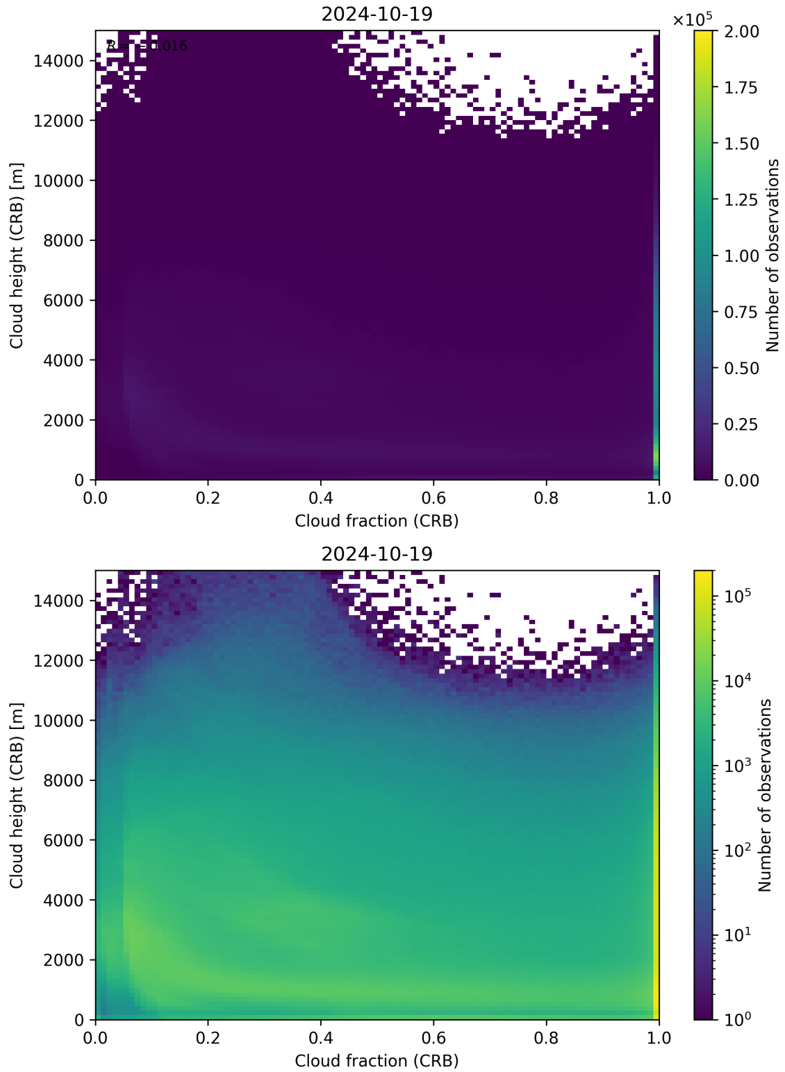
Figure 79: Scatter density plot of “Cloud fraction (CRB)” against “Cloud height (CRB)” for 2024-10-19 to 2024-10-20.
