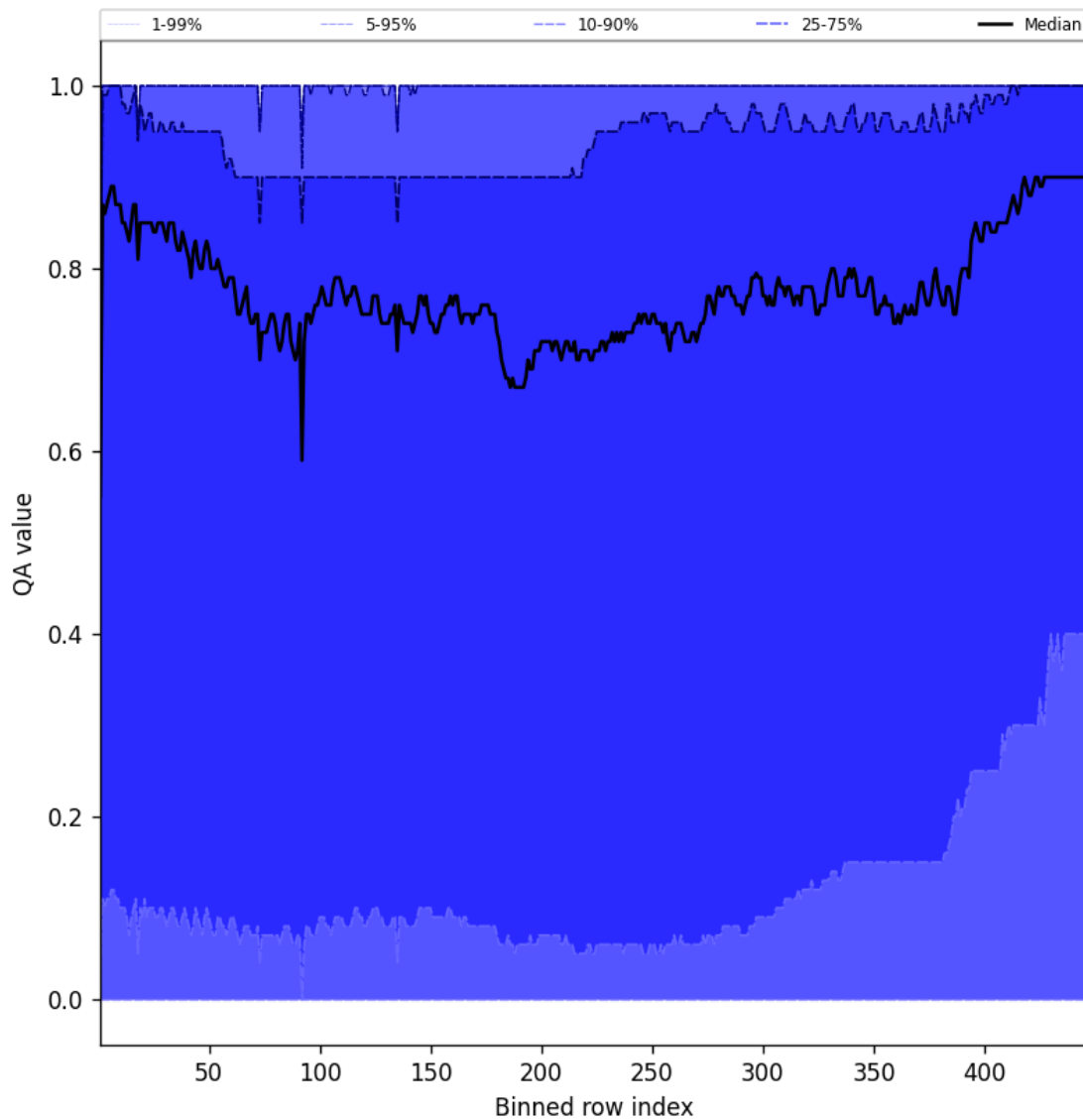
Figure 54: Along track statistics of “QA value” for 2024-10-19 to 2024-10-20
