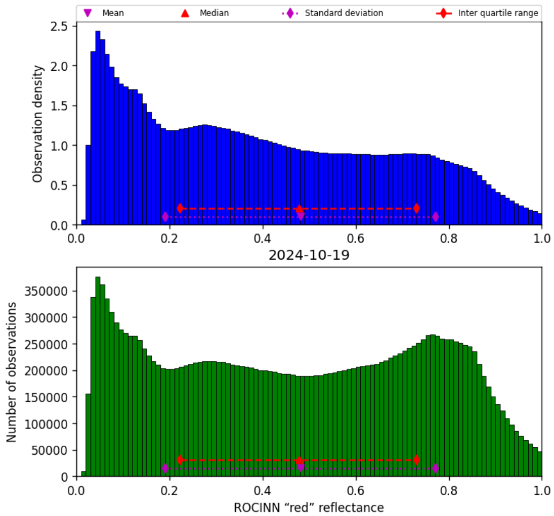
Figure 53: Histogram of “ROCINN “red” reflectance” for 2024-10-19 to 2024-10-20
