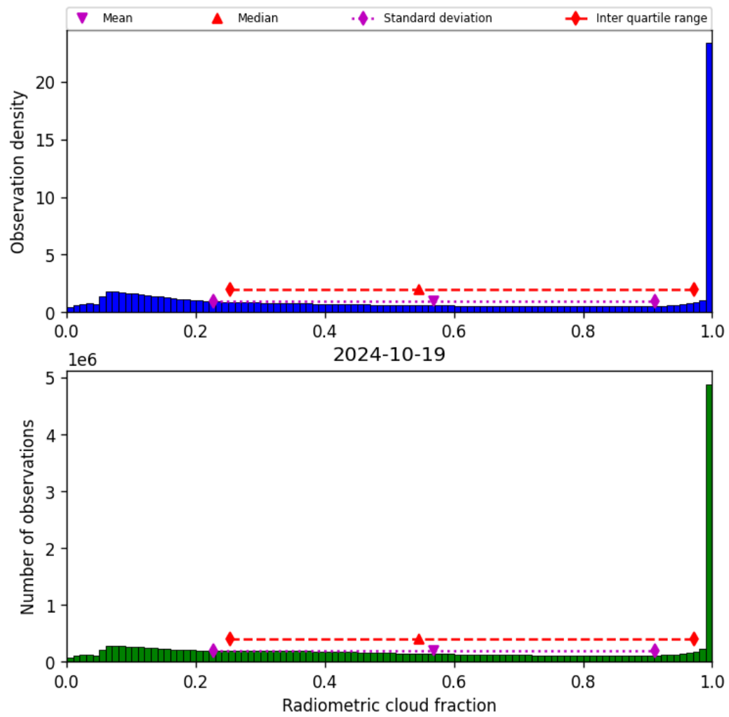
Figure 39: Histogram of “Radiometric cloud fraction” for 2024-10-19 to 2024-10-20
