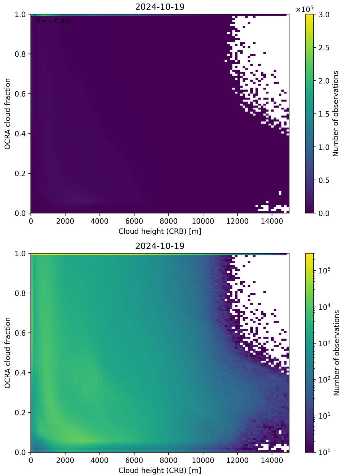
Figure 81: Scatter density plot of “Cloud height (CRB)” against “OCRA cloud fraction” for 2024-10-19 to 2024-10-20.
