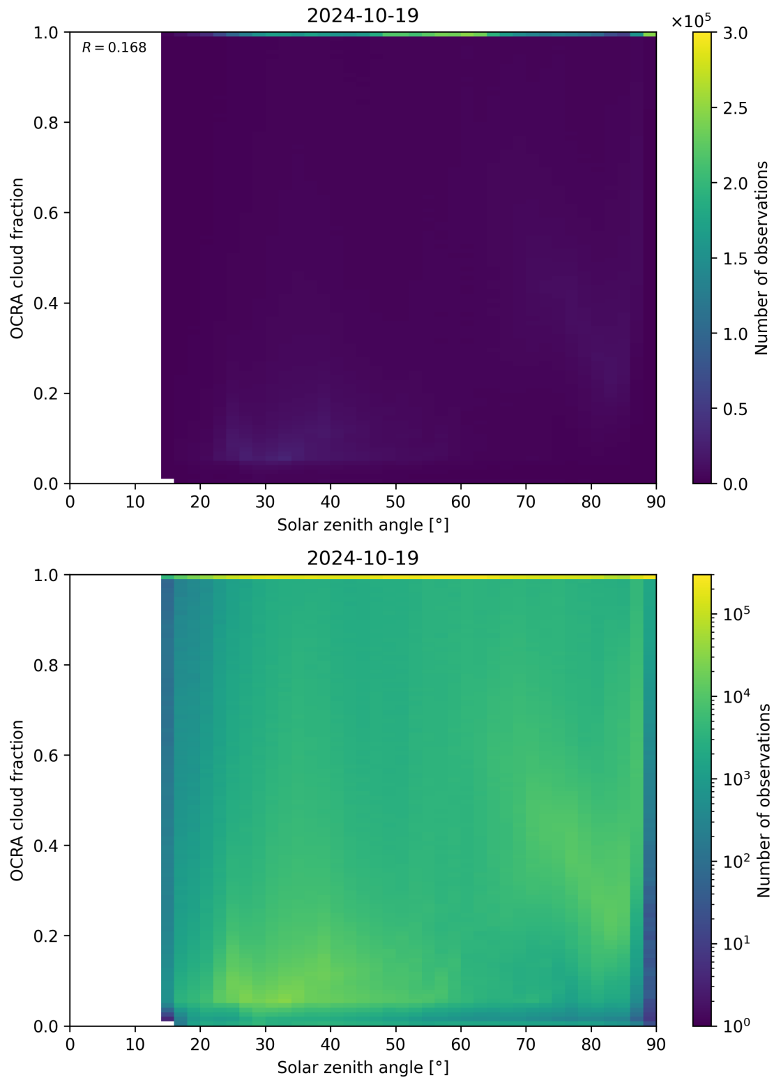
Figure 100: Scatter density plot of “Solar zenith angle” against “OCRA cloud fraction” for 2024-10-19 to 2024-10-20.
