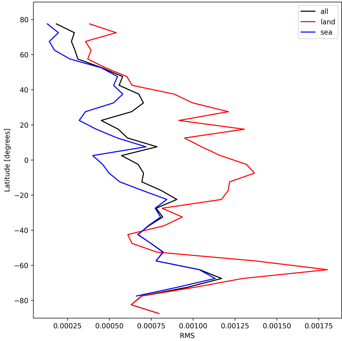
Figure 31: Zonal average of “RMS” for 2024-10-19 to 2024-10-20.
