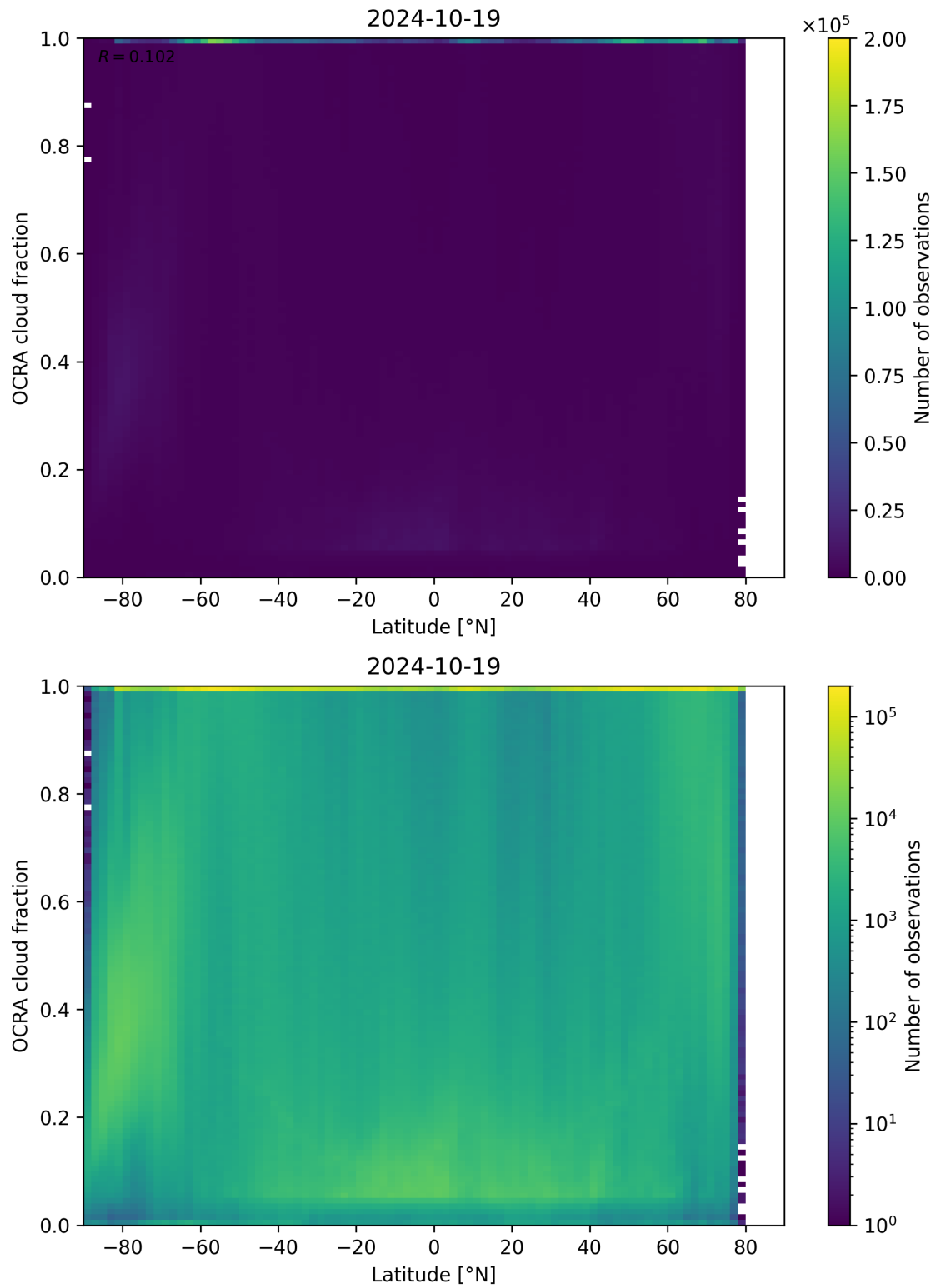
Figure 93: Scatter density plot of “Latitude” against “OCRA cloud fraction” for 2024-10-19 to 2024-10-20.
