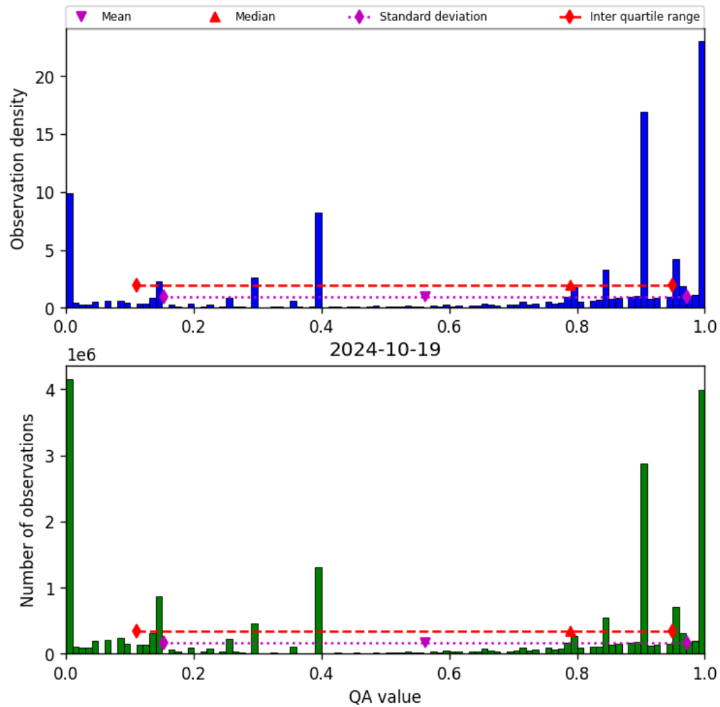
Figure 38: Histogram of “QA value” for 2024-10-19 to 2024-10-20
