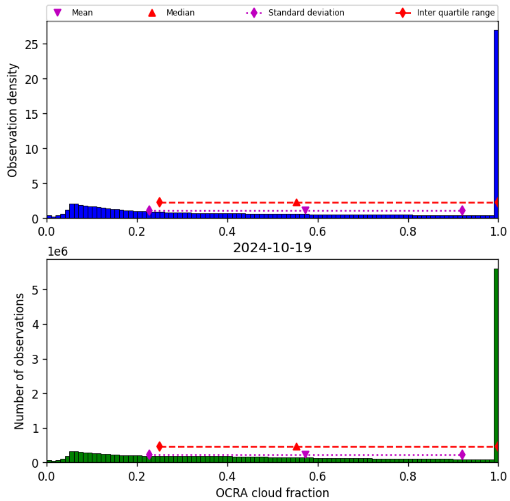
Figure 50: Histogram of “OCRA cloud fraction” for 2024-10-19 to 2024-10-20
